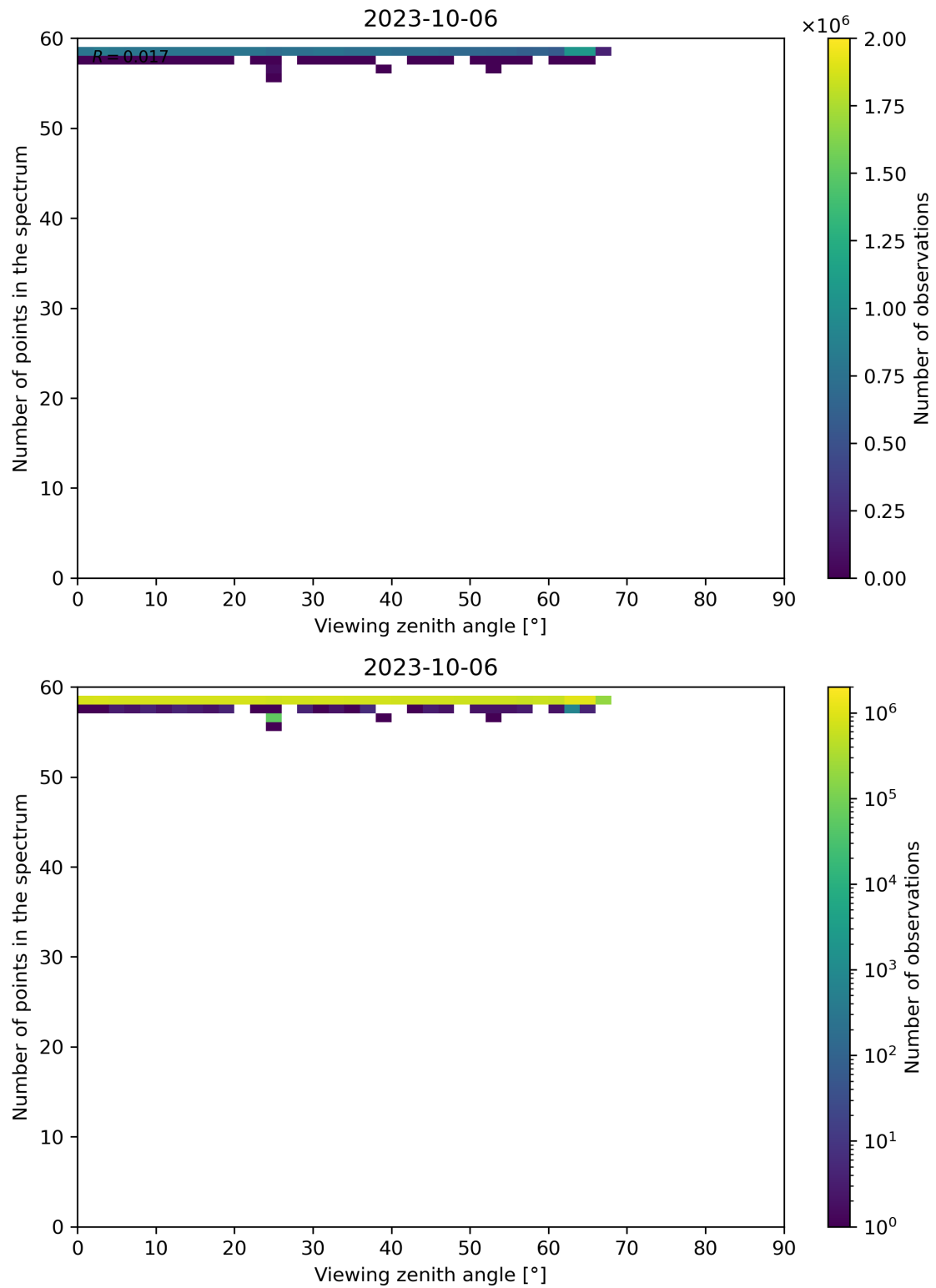
Figure 137: Scatter density plot of “Viewing zenith angle” against “Number of points in the spectrum” for 2023-10-06 to 2023-10-07.
