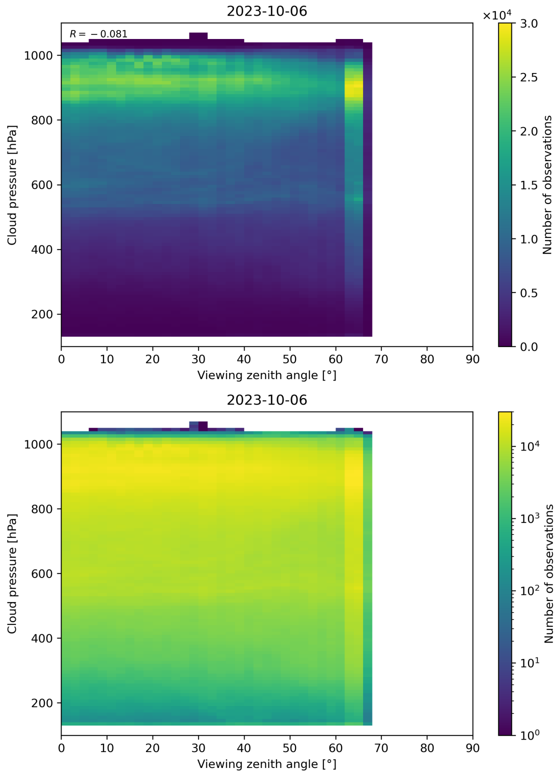
Figure 133: Scatter density plot of “Viewing zenith angle” against “Cloud pressure” for 2023-10-06 to 2023-10-07.
