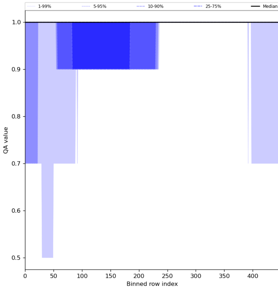
Figure 46: Along track statistics of “QA value” for 2023-10-06 to 2023-10-07
