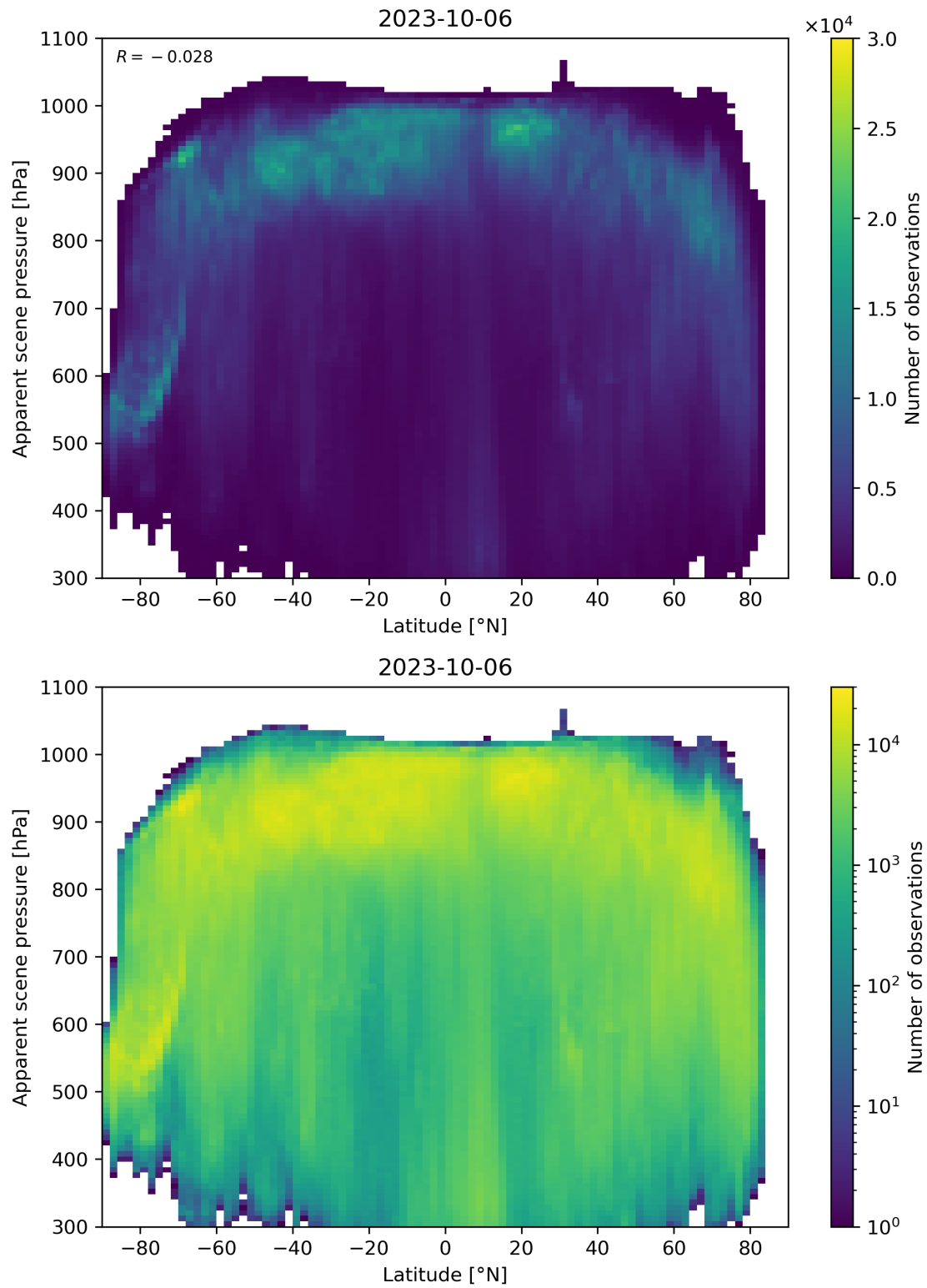
Figure 96: Scatter density plot of “Latitude” against “Apparent scene pressure” for 2023-10-06 to 2023-10-07.
