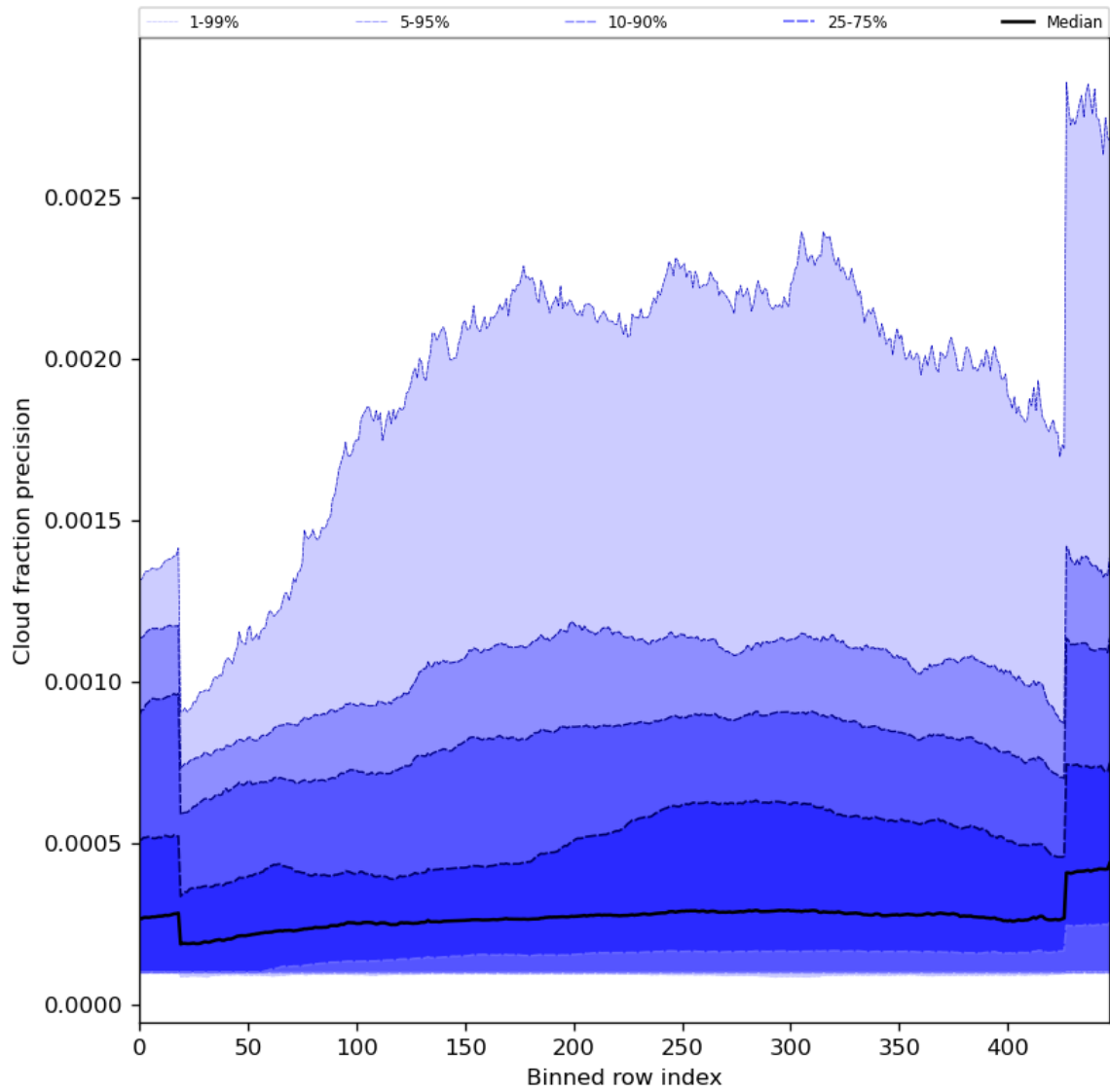
Figure 50: Along track statistics of “Cloud fraction precision” for 2023-10-06 to 2023-10-07
