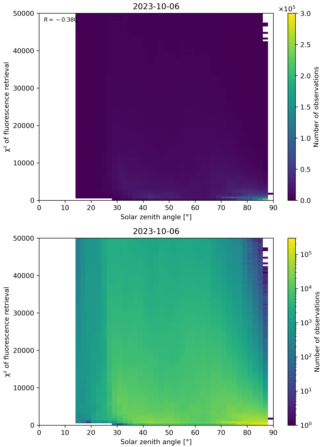
Figure 120: Scatter density plot of “Solar zenith angle” against “ \chi^2 of fluorescence retrieval” for 2023-10-06 to 2023-10-07.
