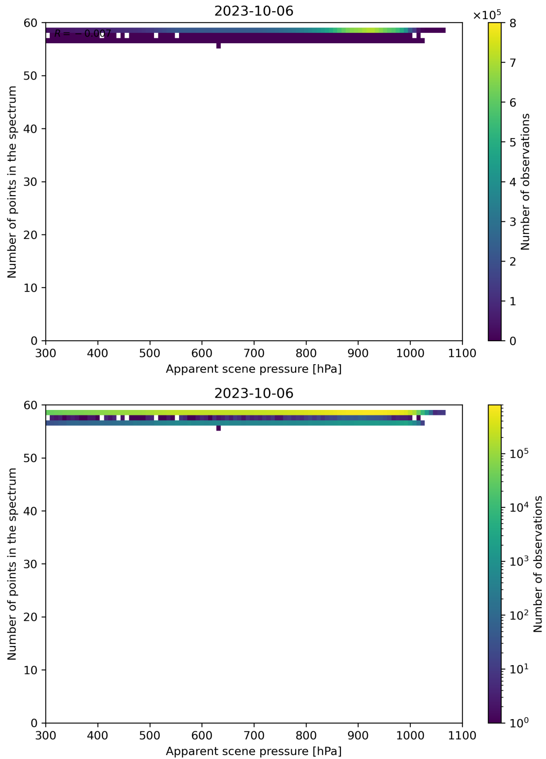
Figure 67: Scatter density plot of “Apparent scene pressure” against “Number of points in the spectrum” for 2023-10-06 to 2023-10-07.
