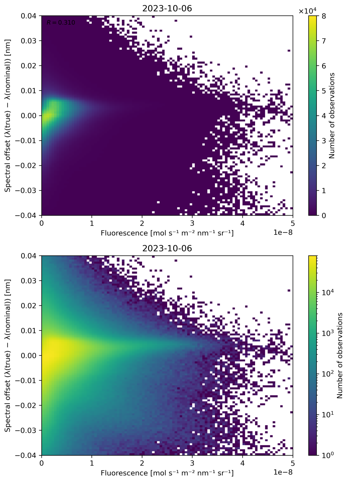
Figure 95: Scatter density plot of “Fluorescence” against “Spectral offset ( \lambda(\text{true}) - \lambda(\text{nominal}) )” for 2023-10-06 to 2023-10-07.
