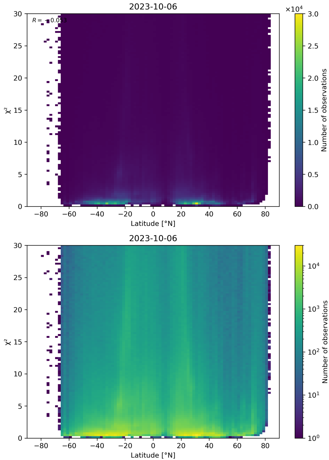
Figure 97: Scatter density plot of “Latitude” against “ \chi^2 ” for 2023-10-06 to 2023-10-07.
