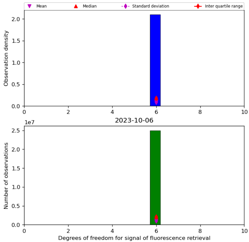
Figure 43: Histogram of “Degrees of freedom for signal of fluorescence retrieval” for 2023-10-06 to 2023-10-07
