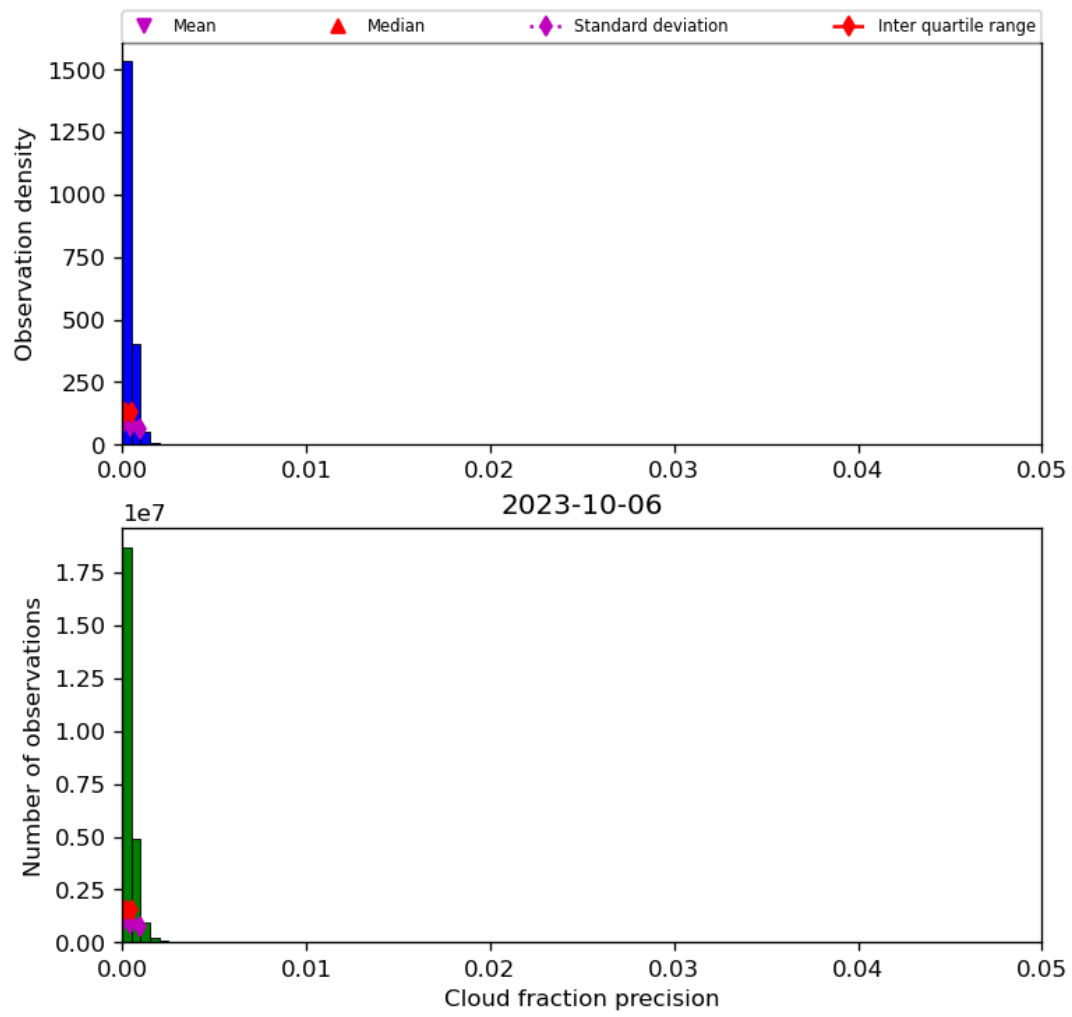
Figure 33: Histogram of “Cloud fraction precision” for 2023-10-06 to 2023-10-07
