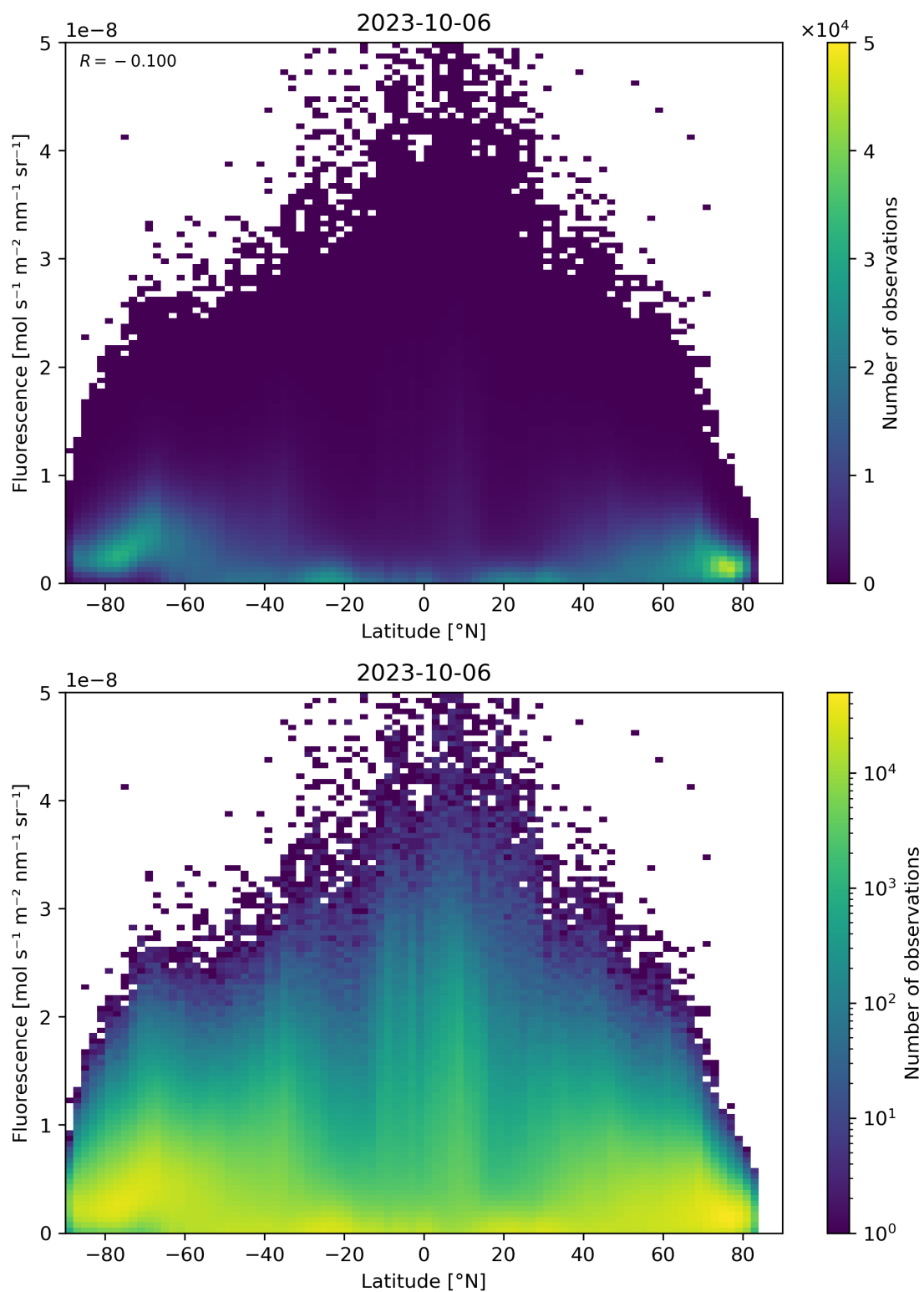
Figure 101: Scatter density plot of “Latitude” against “Fluorescence” for 2023-10-06 to 2023-10-07.
