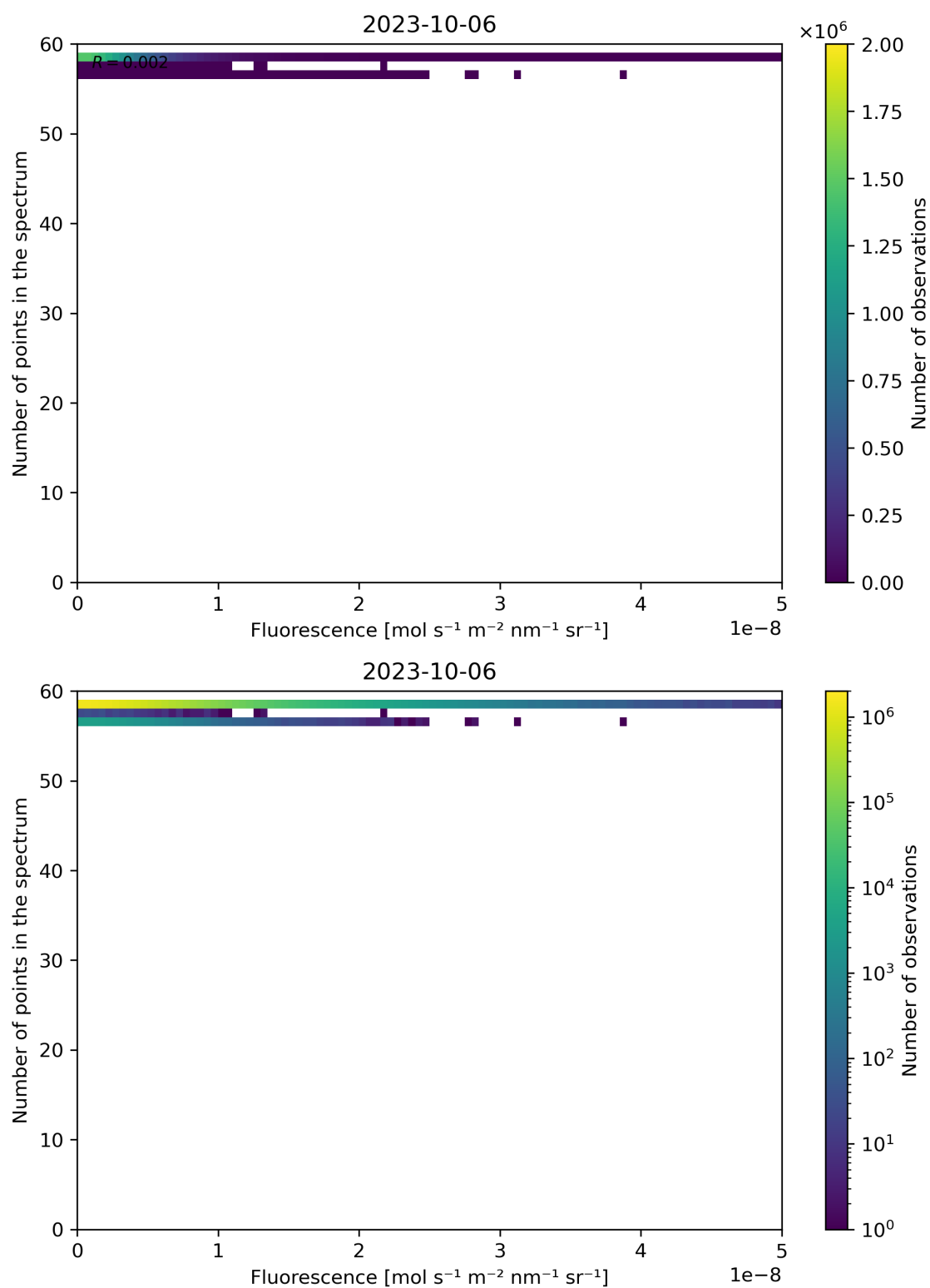
Figure 94: Scatter density plot of “Fluorescence” against “Number of points in the spectrum” for 2023-10-06 to 2023-10-07.
