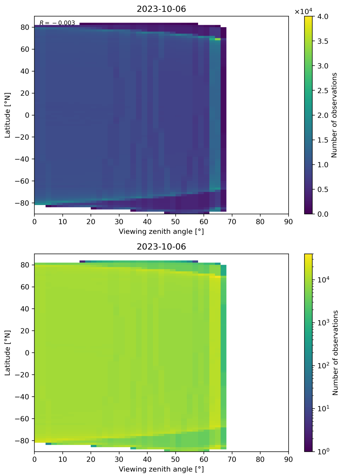
Figure 135: Scatter density plot of “Viewing zenith angle” against “Latitude” for 2023-10-06 to 2023-10-07.
