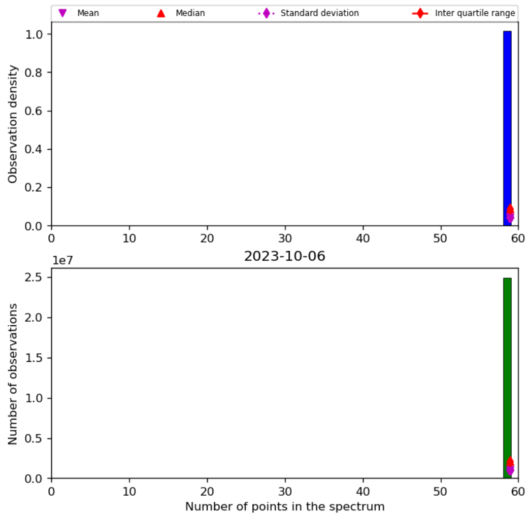
Figure 44: Histogram of “Number of points in the spectrum” for 2023-10-06 to 2023-10-07
