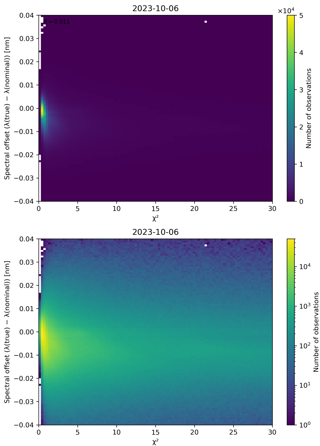
Figure 75: Scatter density plot of “ \chi^2 ” against “Spectral offset ( \lambda(\text{true}) - \lambda(\text{nominal}) )” for 2023-10-06 to 2023-10-07.
