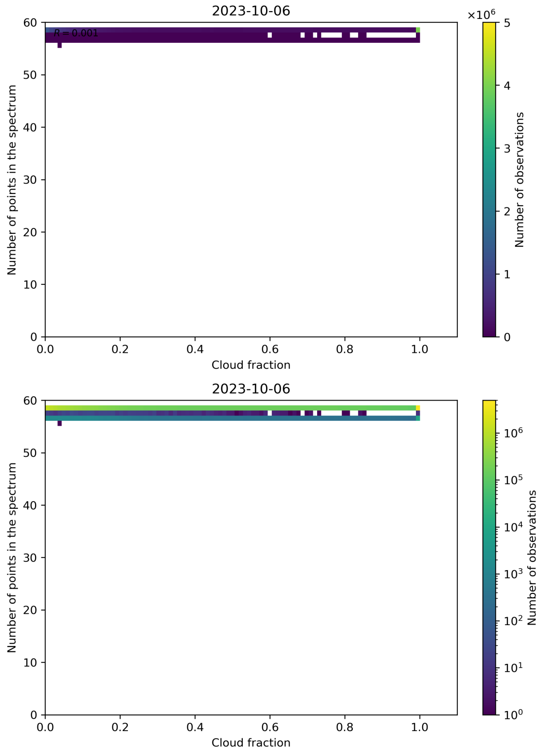
Figure 81: Scatter density plot of “Cloud fraction” against “Number of points in the spectrum” for 2023-10-06 to 2023-10-07.
