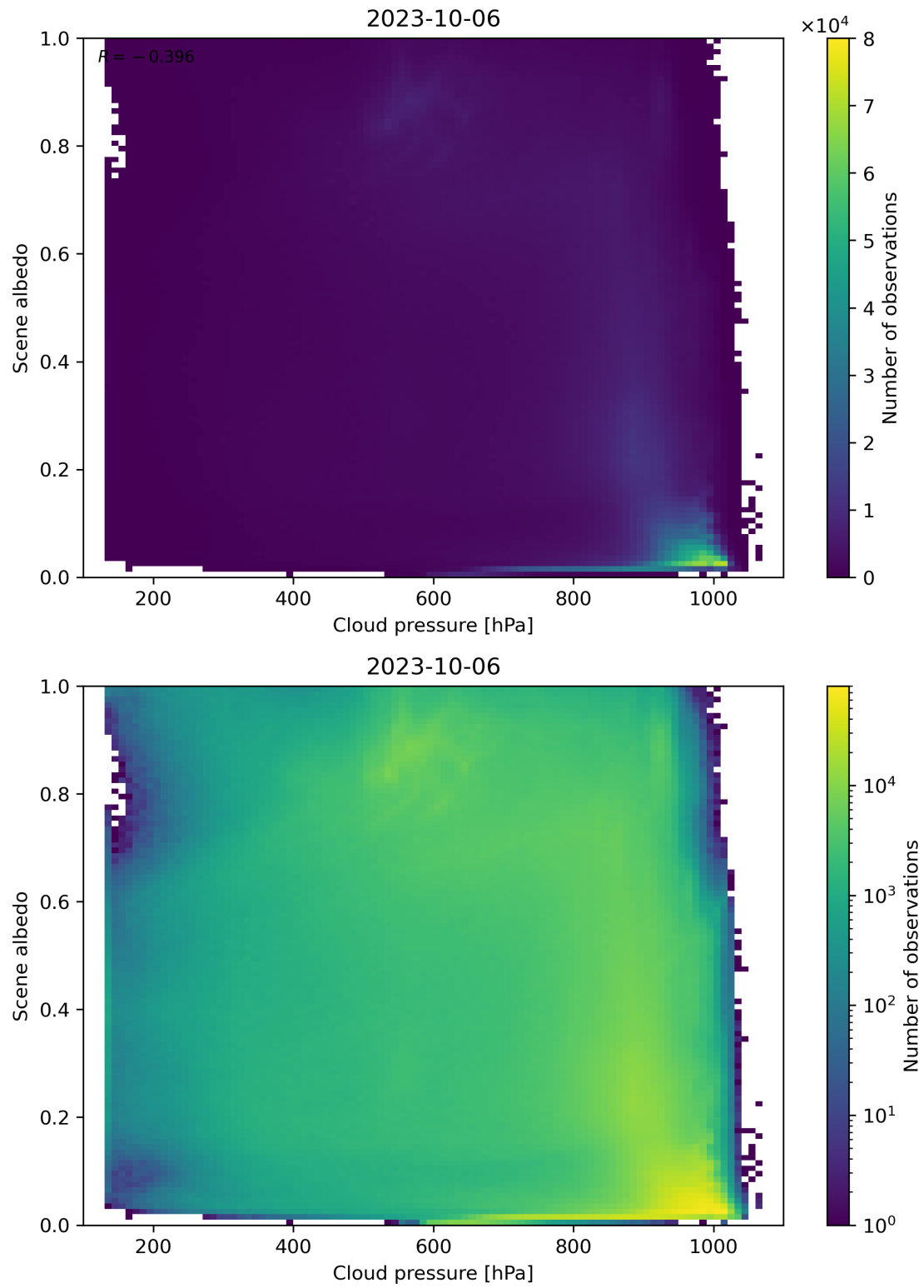
Figure 91: Scatter density plot of “Cloud pressure” against “Scene albedo” for 2023-10-06 to 2023-10-07.
