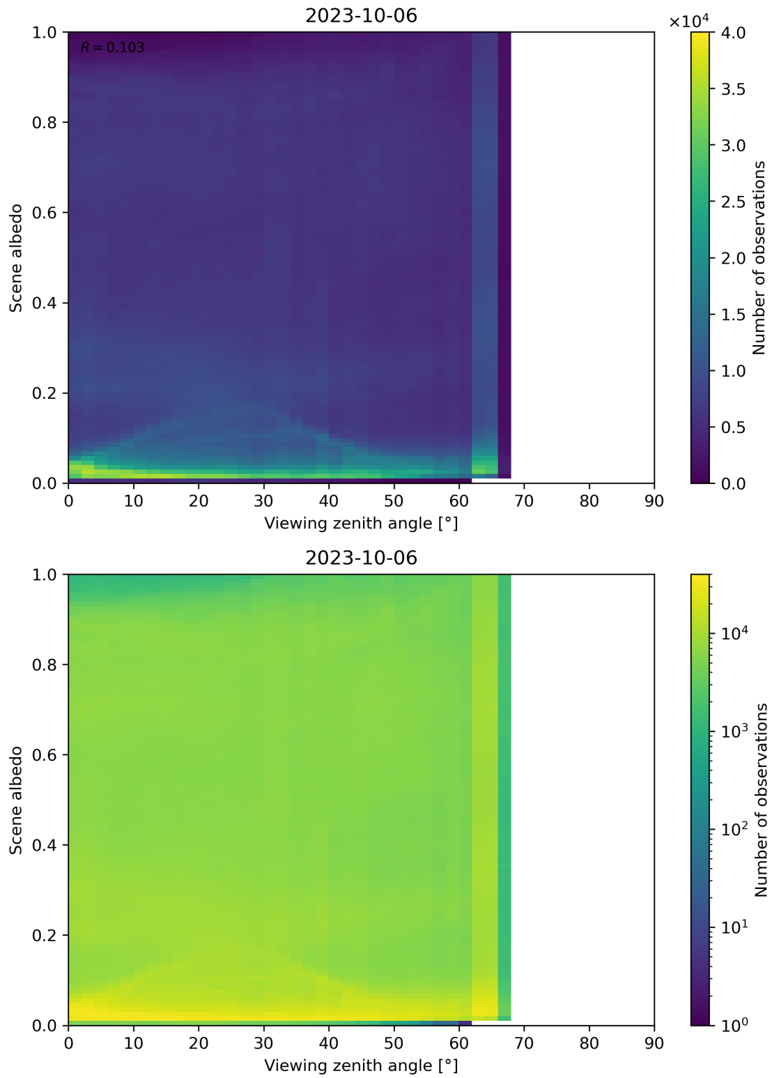
Figure 138: Scatter density plot of “Viewing zenith angle” against “Scene albedo” for 2023-10-06 to 2023-10-07.
