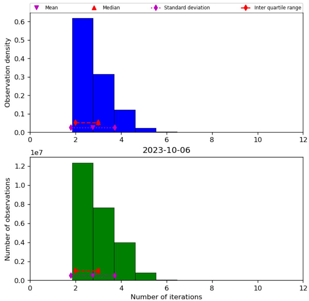
Figure 39: Histogram of “Number of iterations” for 2023-10-06 to 2023-10-07
