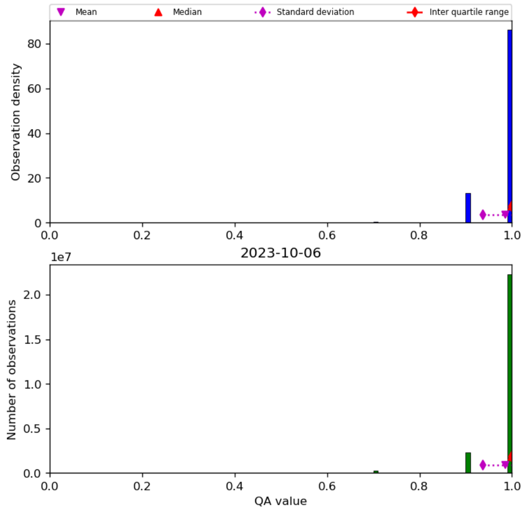
Figure 29: Histogram of “QA value” for 2023-10-06 to 2023-10-07
