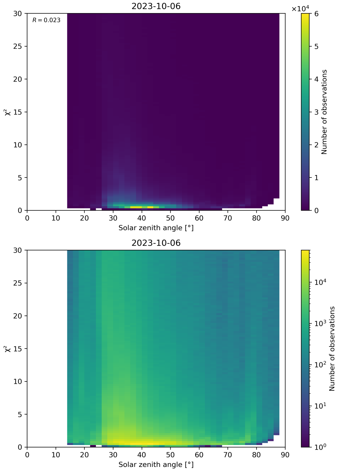
Figure 119: Scatter density plot of “Solar zenith angle” against “ \chi^2 ” for 2023-10-06 to 2023-10-07.
