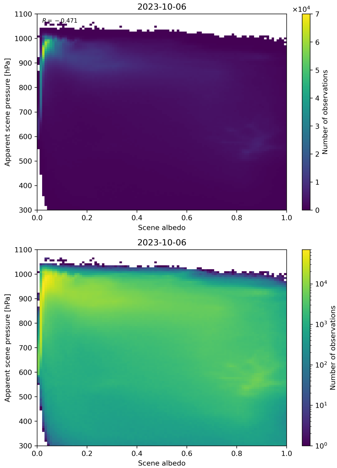
Figure 111: Scatter density plot of “Scene albedo” against “Apparent scene pressure” for 2023-10-06 to 2023-10-07.
