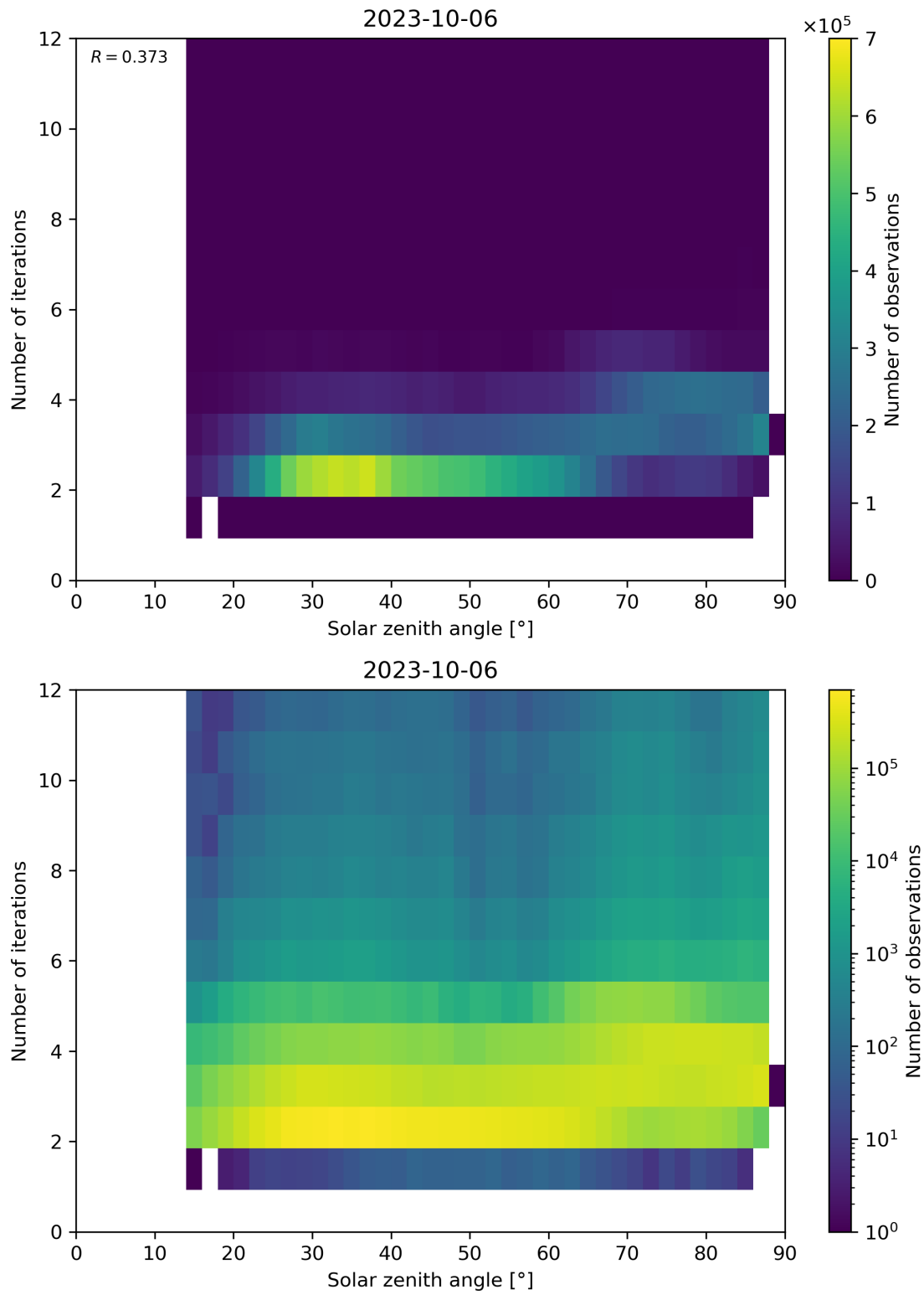
Figure 125: Scatter density plot of “Solar zenith angle” against “Number of iterations” for 2023-10-06 to 2023-10-07.
