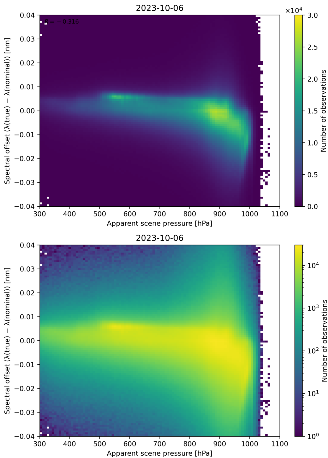
Figure 68: Scatter density plot of “Apparent scene pressure” against “Spectral offset ( \lambda(\text{true}) - \lambda(\text{nominal}) )” for 2023-10-06 to 2023-10-07.
