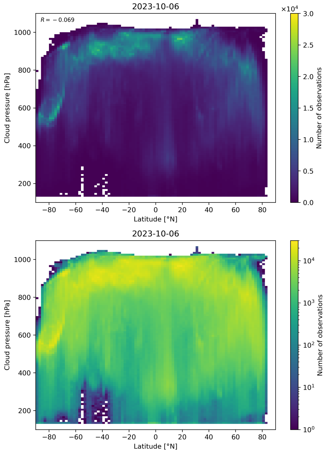
Figure 100: Scatter density plot of “Latitude” against “Cloud pressure” for 2023-10-06 to 2023-10-07.
