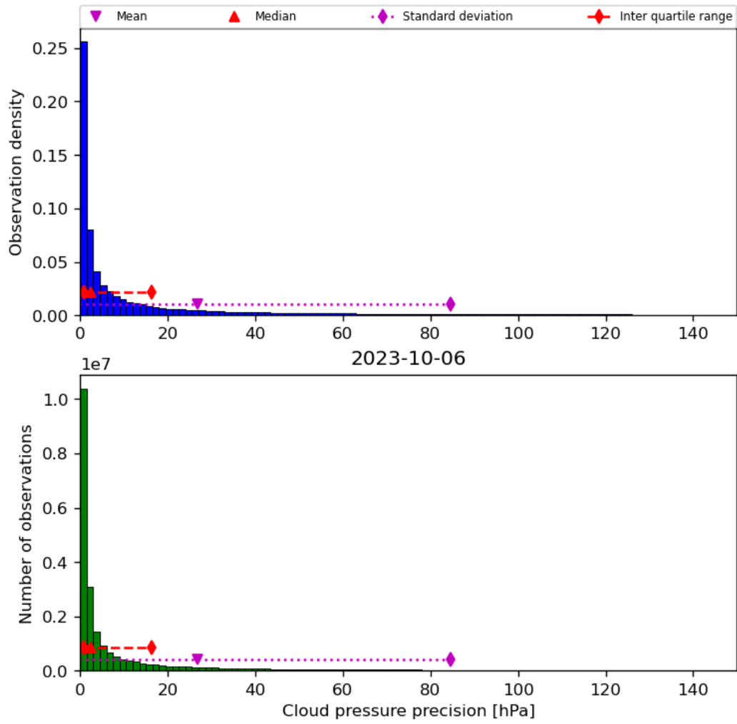
Figure 31: Histogram of “Cloud pressure precision” for 2023-10-06 to 2023-10-07
