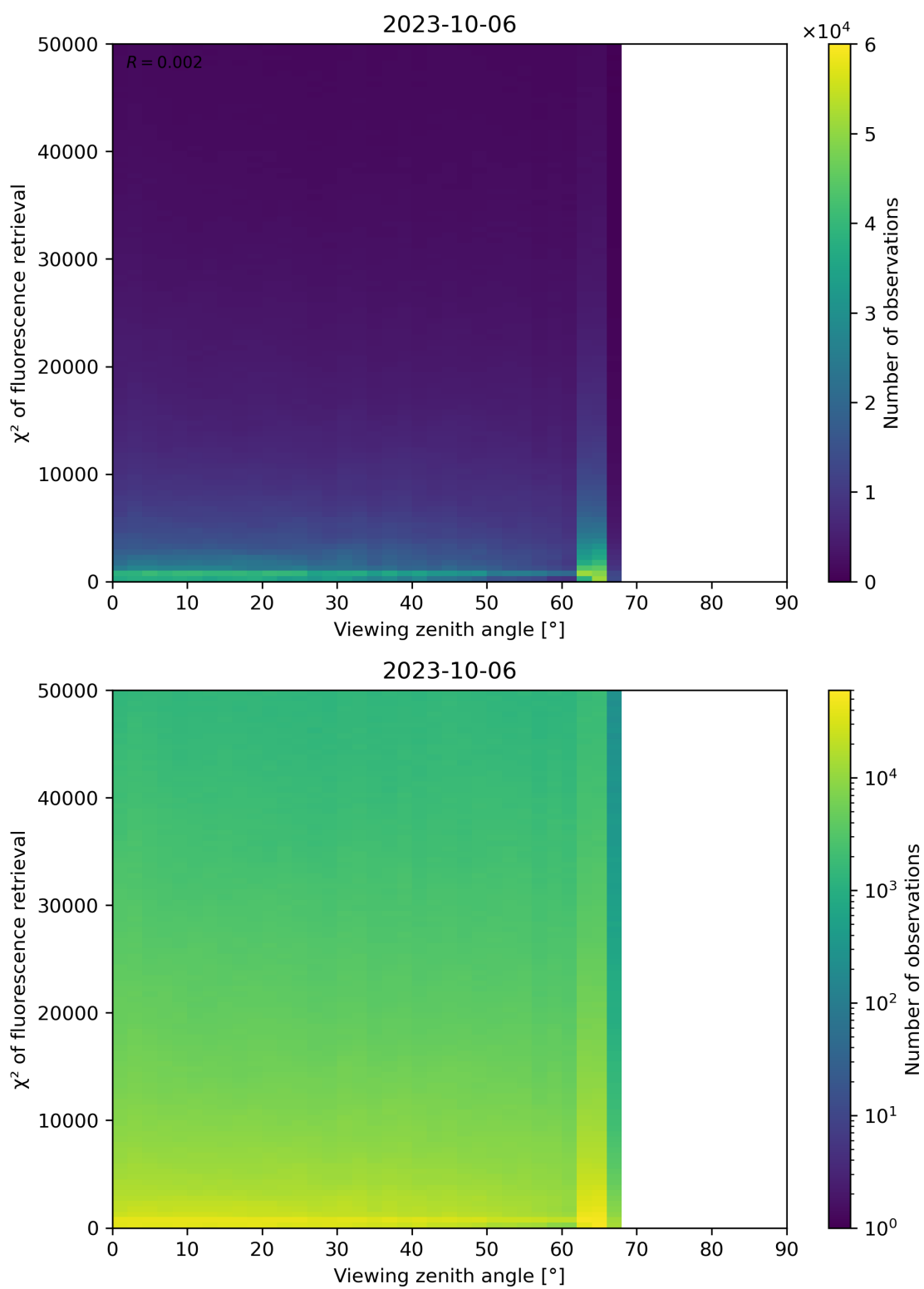
Figure 131: Scatter density plot of “Viewing zenith angle” against “ \chi^2 of fluorescence retrieval” for 2023-10-06 to 2023-10-07.
