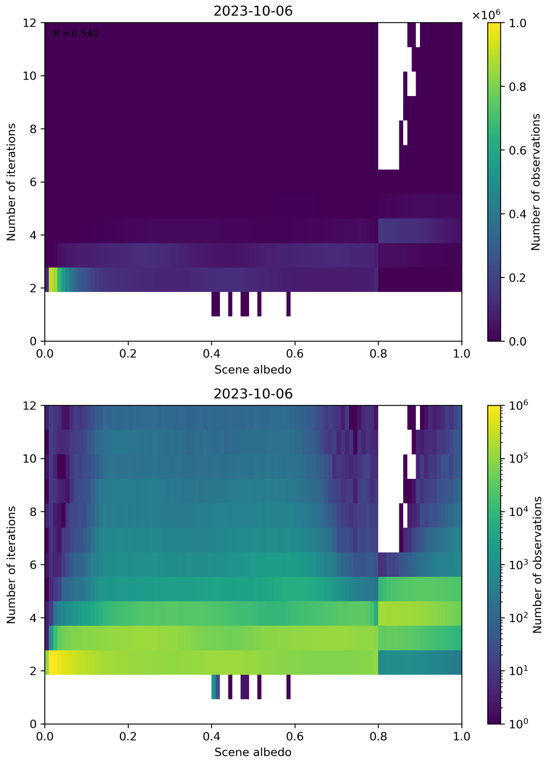
Figure 115: Scatter density plot of “Scene albedo” against “Number of iterations” for 2023-10-06 to 2023-10-07.
