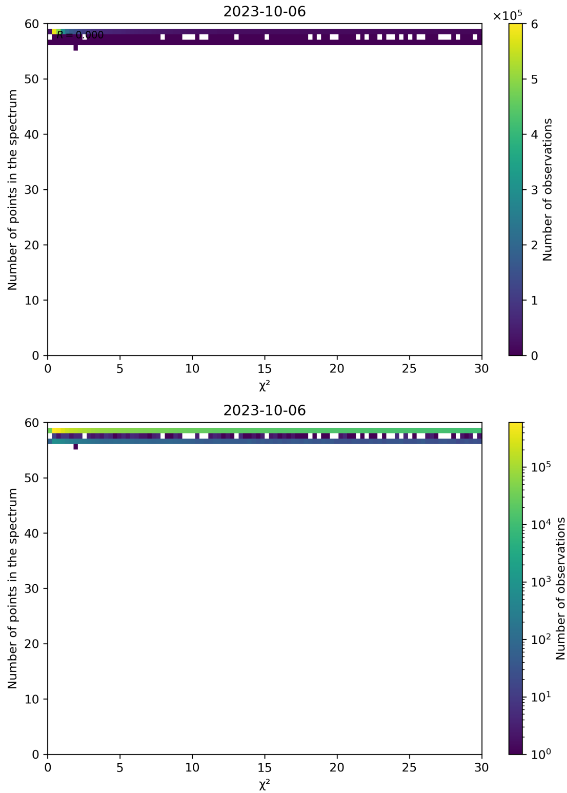
Figure 74: Scatter density plot of " \chi^2 " against "Number of points in the spectrum" for 2023-10-06 to 2023-10-07.
