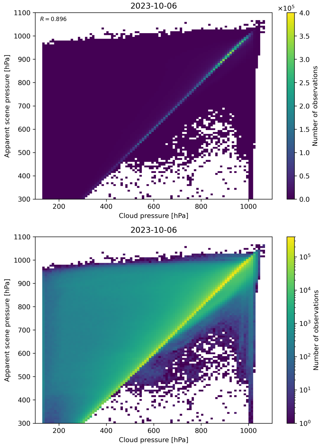
Figure 84: Scatter density plot of “Cloud pressure” against “Apparent scene pressure” for 2023-10-06 to 2023-10-07.
