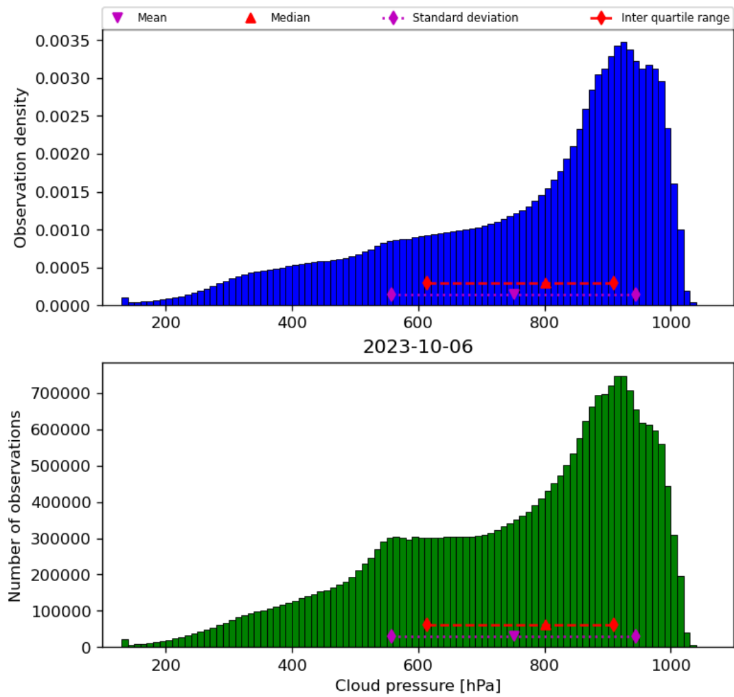
Figure 30: Histogram of “Cloud pressure” for 2023-10-06 to 2023-10-07
