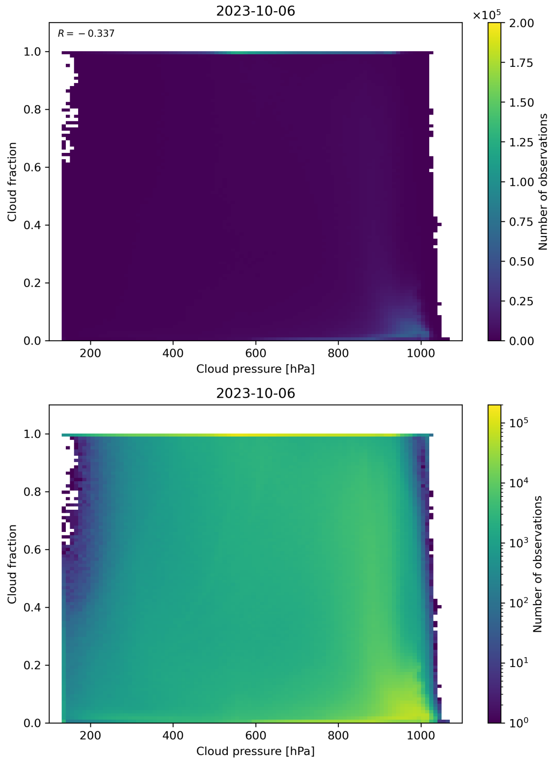
Figure 87: Scatter density plot of “Cloud pressure” against “Cloud fraction” for 2023-10-06 to 2023-10-07.
