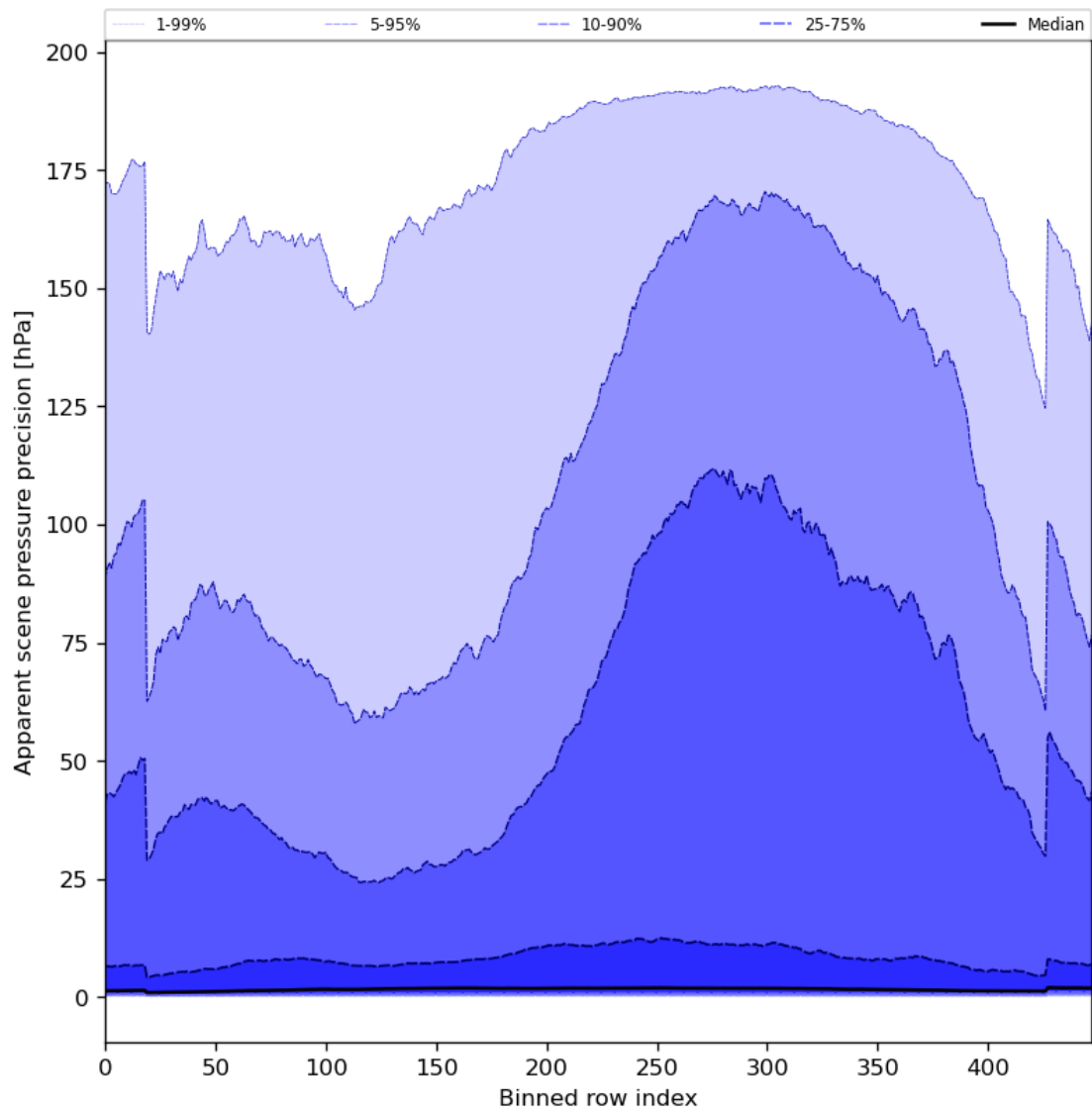
Figure 54: Along track statistics of “Apparent scene pressure precision” for 2023-10-06 to 2023-10-07
