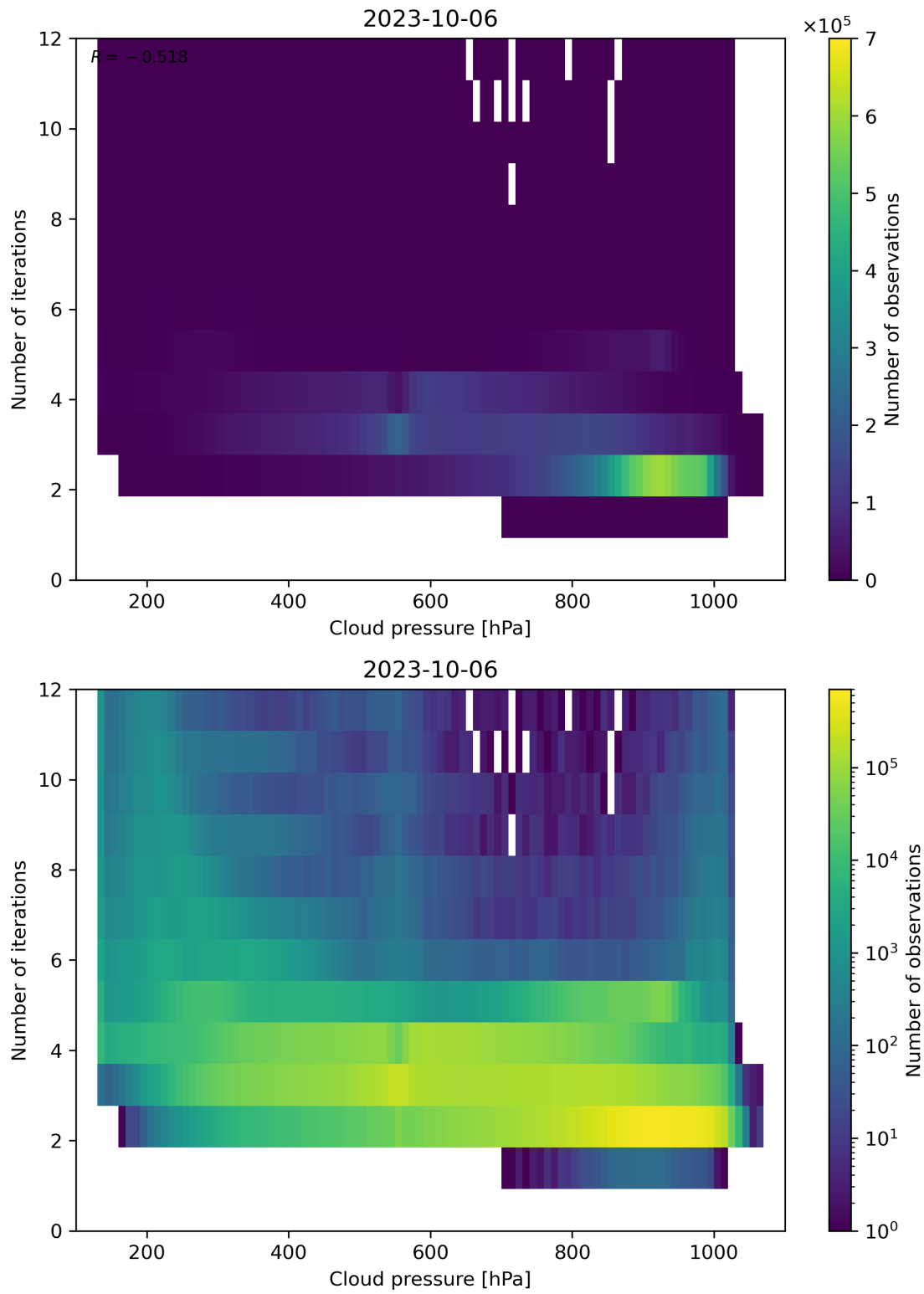
Figure 89: Scatter density plot of “Cloud pressure” against “Number of iterations” for 2023-10-06 to 2023-10-07.
