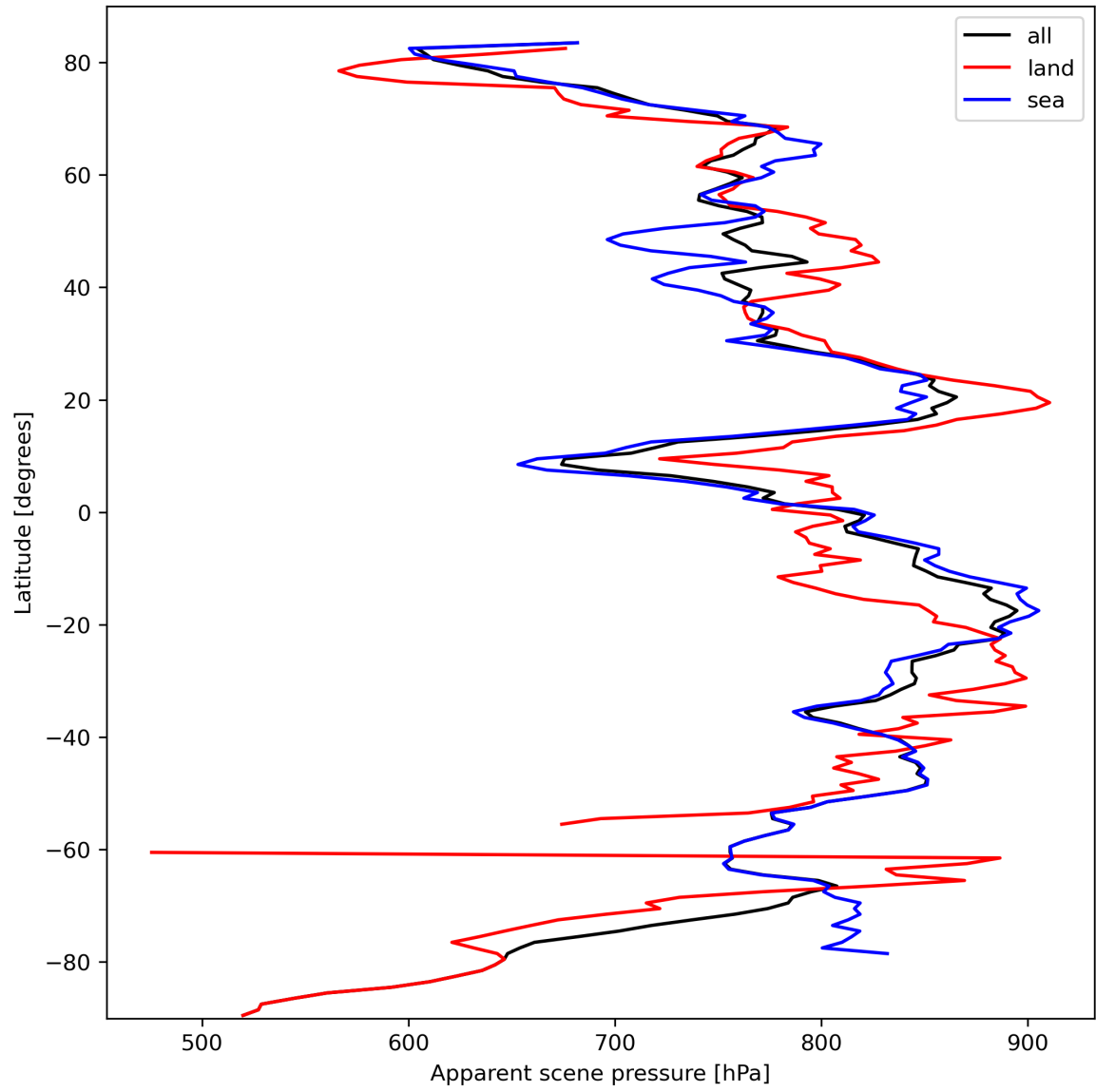
Figure 19: Zonal average of “Apparent scene pressure” for 2023-10-06 to 2023-10-07.
