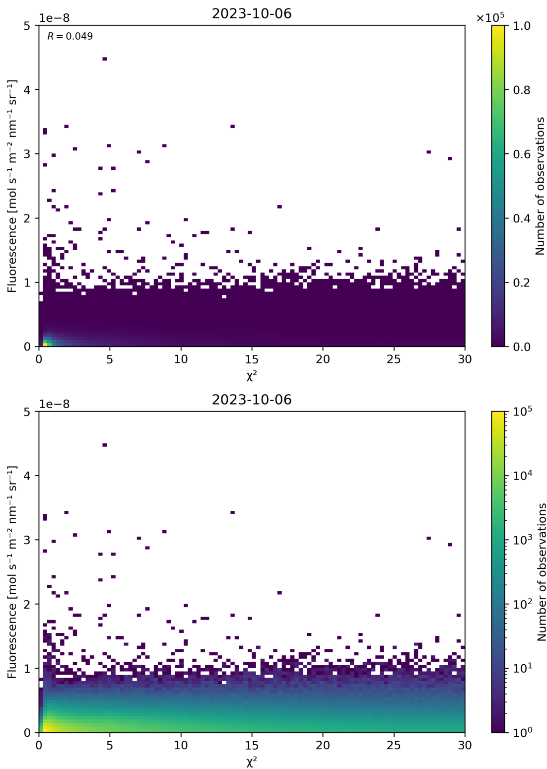
Figure 70: Scatter density plot of “ \chi^2 ” against “Fluorescence” for 2023-10-06 to 2023-10-07.
