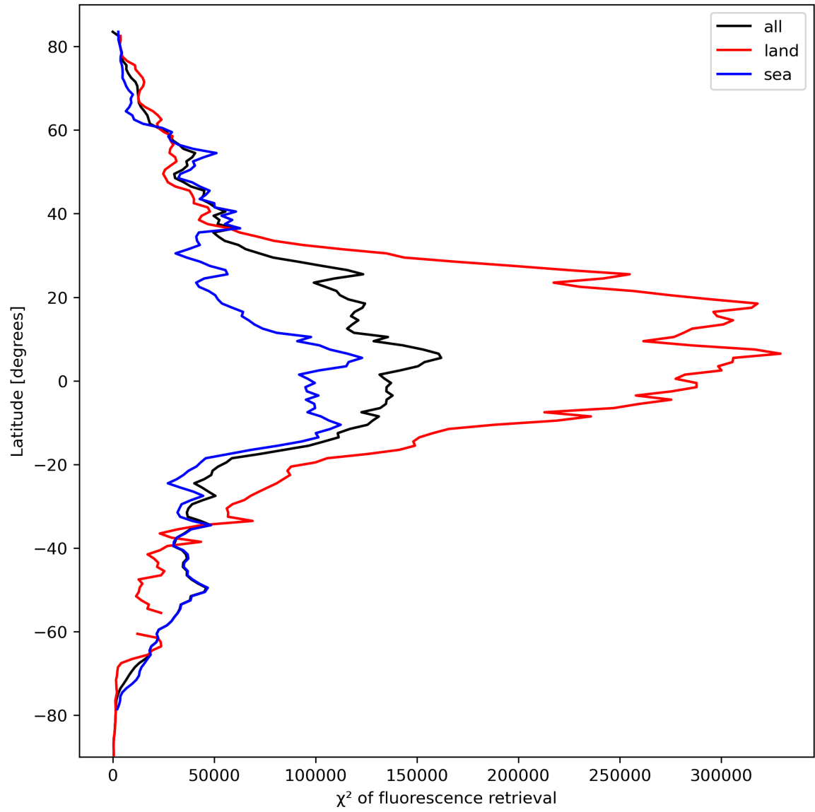
Figure 25: Zonal average of “ \chi^2 of fluorescence retrieval” for 2023-10-06 to 2023-10-07.
