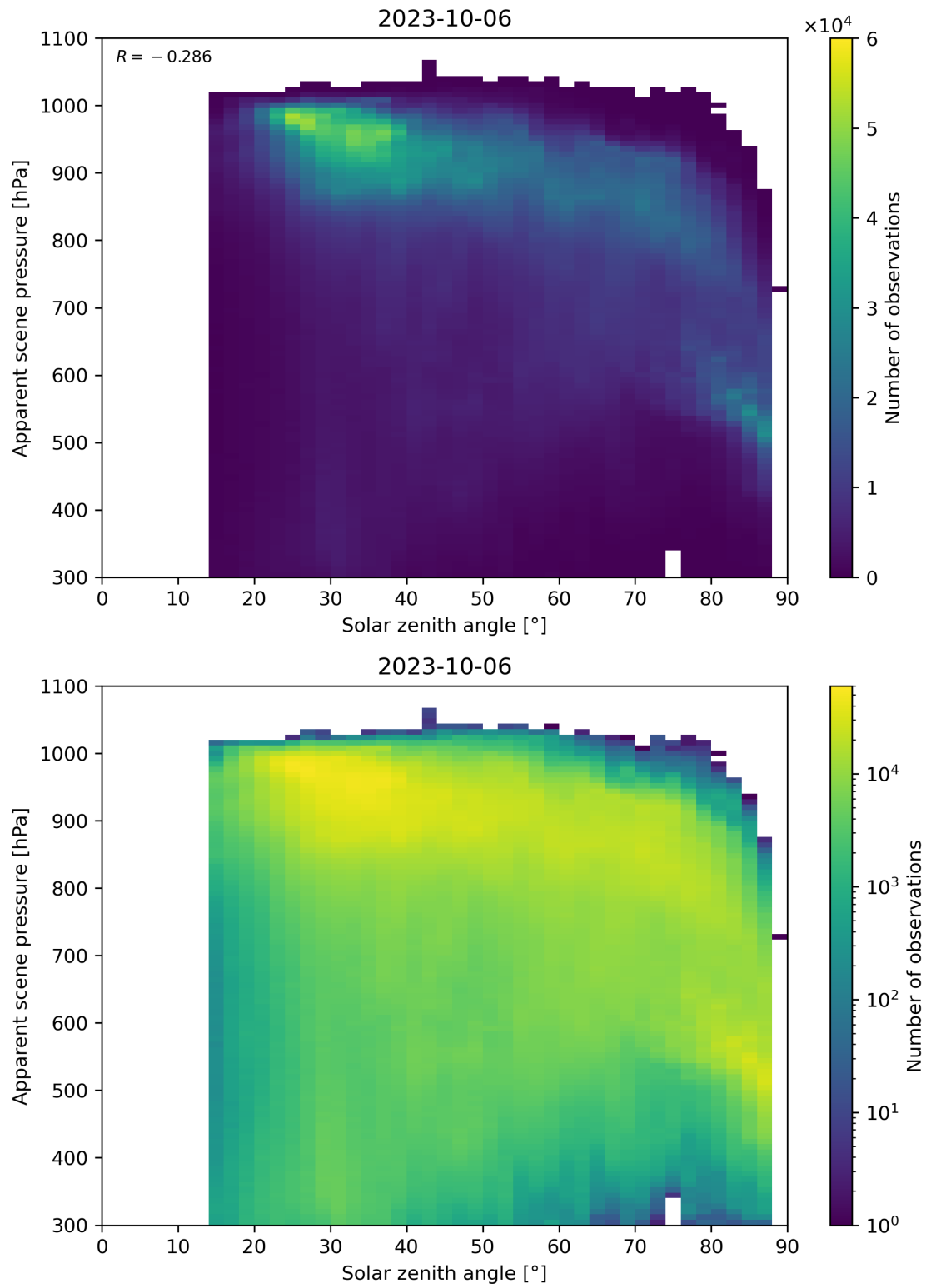
Figure 118: Scatter density plot of “Solar zenith angle” against “Apparent scene pressure” for 2023-10-06 to 2023-10-07.
