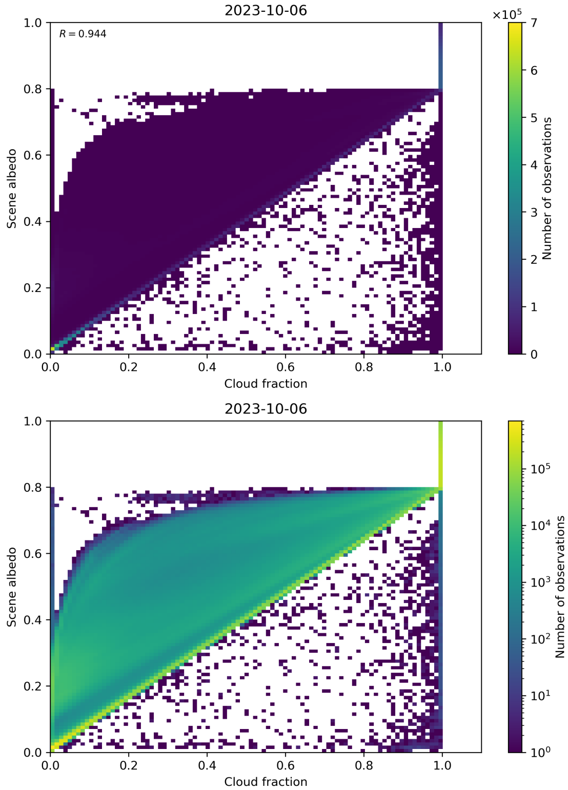
Figure 82: Scatter density plot of “Cloud fraction” against “Scene albedo” for 2023-10-06 to 2023-10-07.
