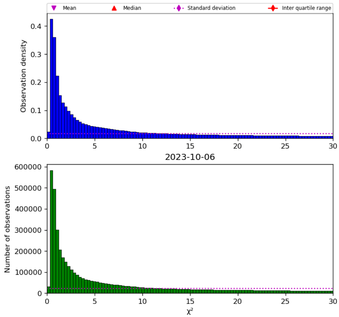
Figure 38: Histogram of " \chi^2 " for 2023-10-06 to 2023-10-07
