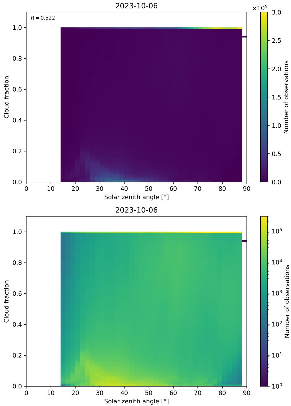
Figure 121: Scatter density plot of “Solar zenith angle” against “Cloud fraction” for 2023-10-06 to 2023-10-07.
