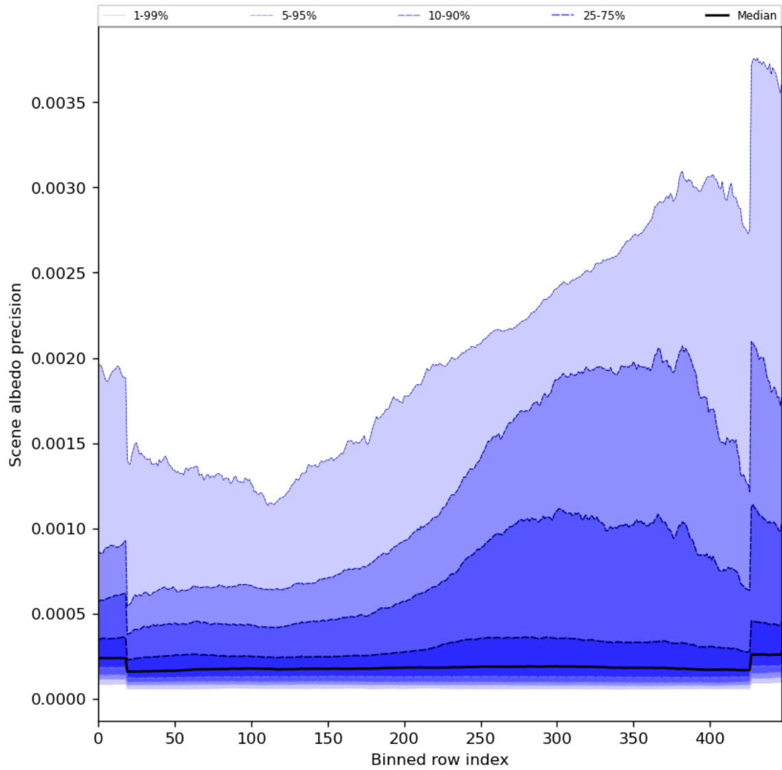
Figure 52: Along track statistics of “Scene albedo precision” for 2023-10-06 to 2023-10-07
