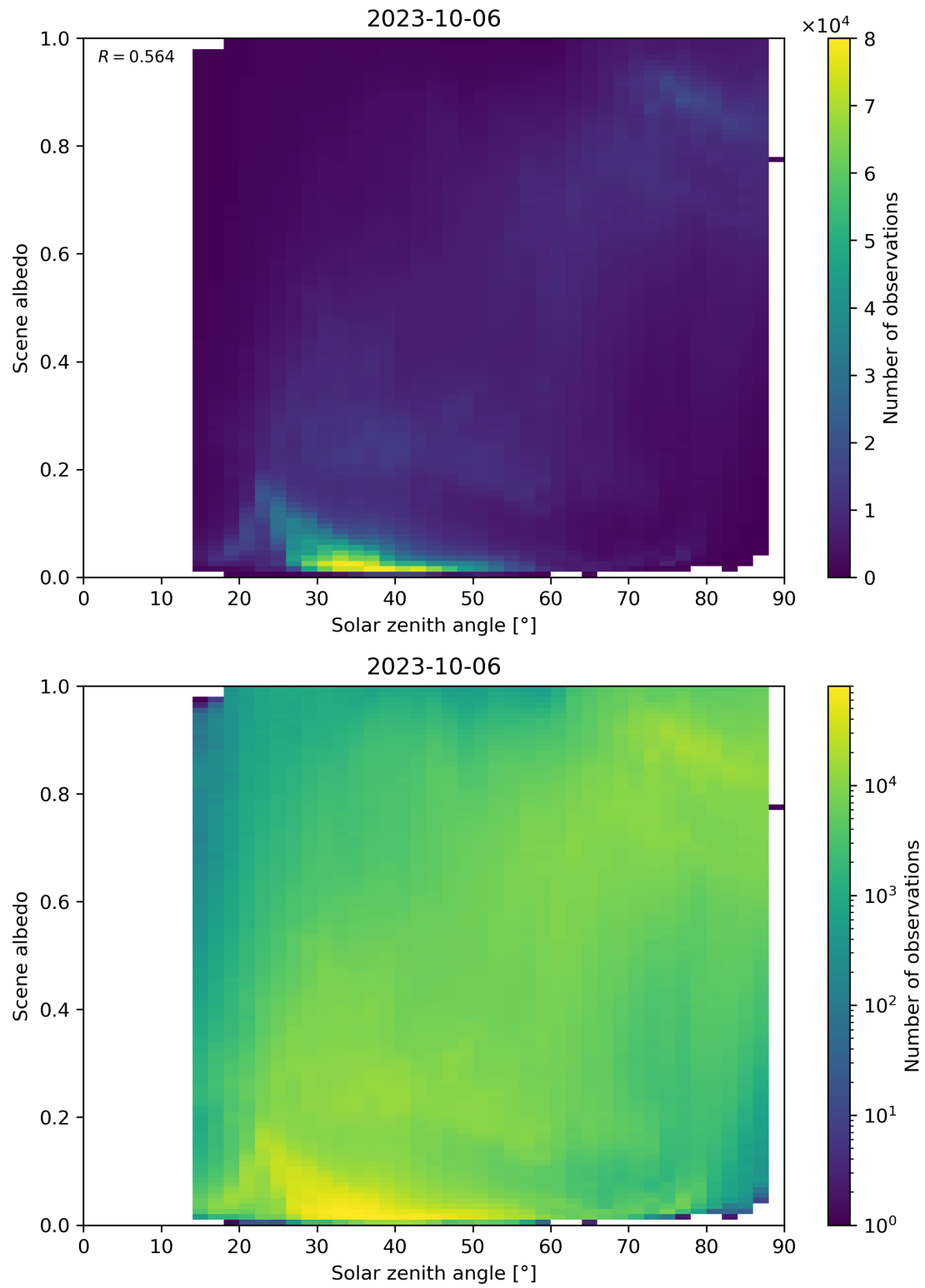
Figure 127: Scatter density plot of “Solar zenith angle” against “Scene albedo” for 2023-10-06 to 2023-10-07.
