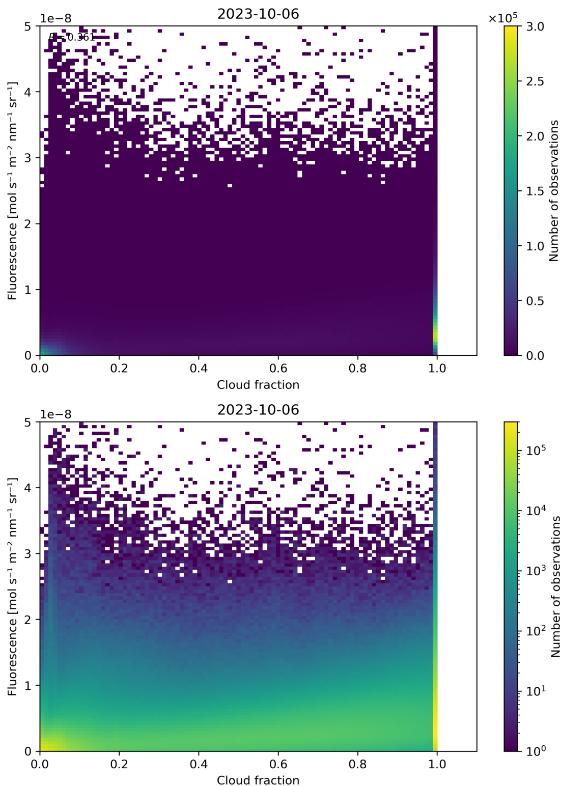
Figure 79: Scatter density plot of “Cloud fraction” against “Fluorescence” for 2023-10-06 to 2023-10-07.
