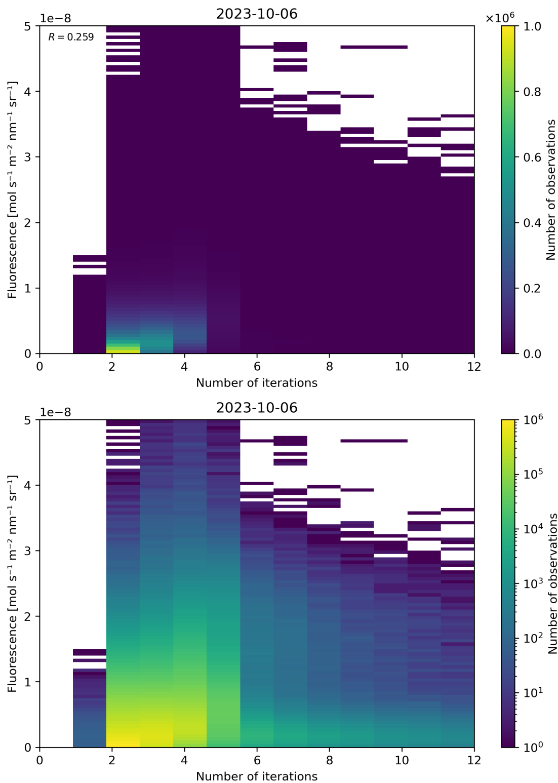
Figure 107: Scatter density plot of “Number of iterations” against “Fluorescence” for 2023-10-06 to 2023-10-07.
