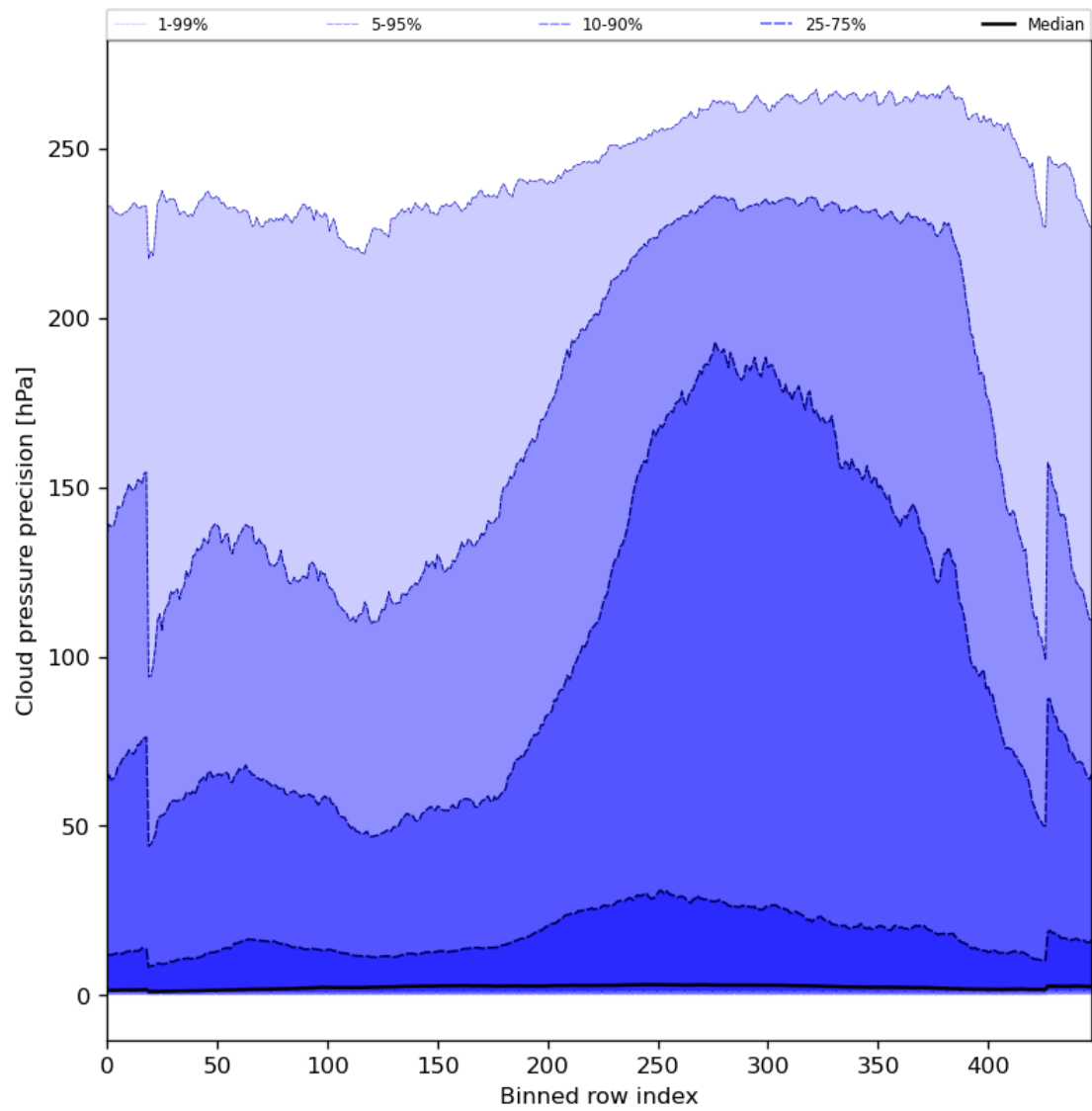
Figure 48: Along track statistics of “Cloud pressure precision” for 2023-10-06 to 2023-10-07
