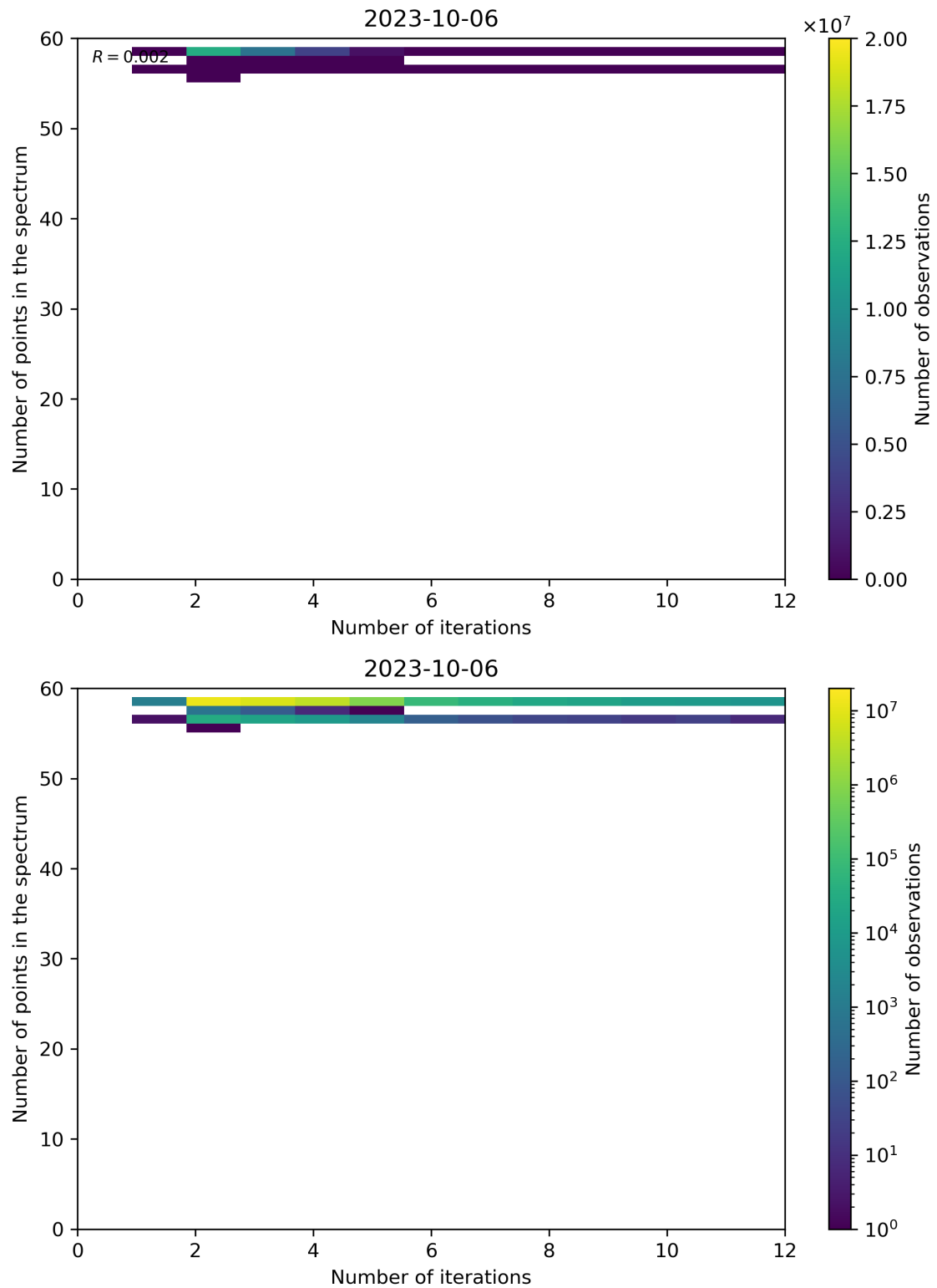
Figure 108: Scatter density plot of “Number of iterations” against “Number of points in the spectrum” for 2023-10-06 to 2023-10-07.
