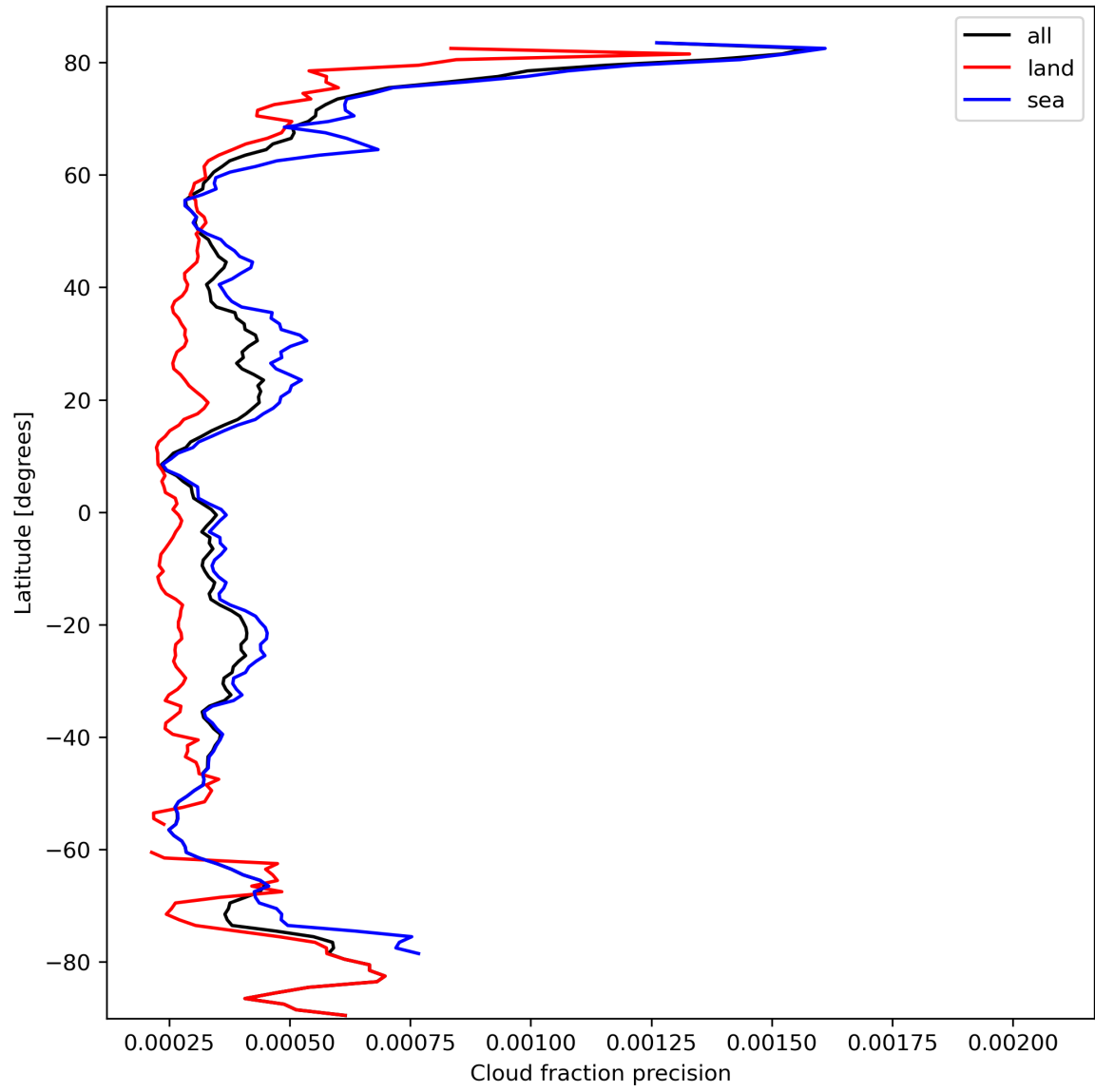
Figure 16: Zonal average of “Cloud fraction precision” for 2023-10-06 to 2023-10-07.
