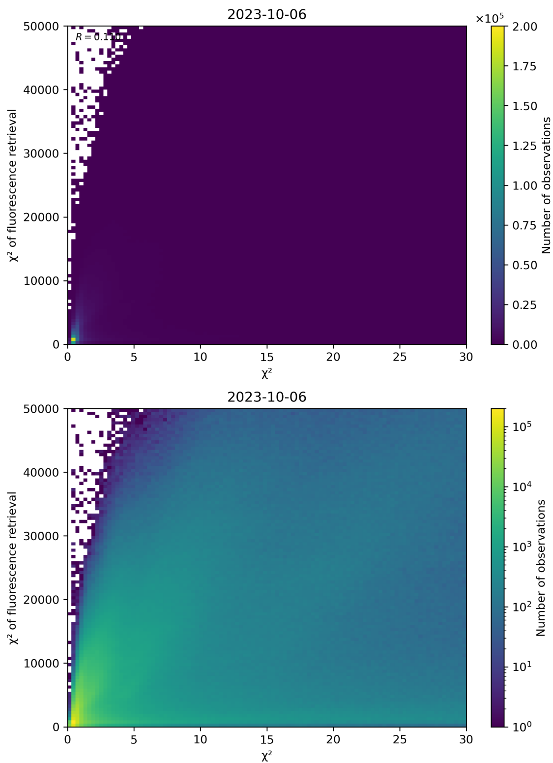
Figure 69: Scatter density plot of “ \chi^2 ” against “ \chi^2 of fluorescence retrieval” for 2023-10-06 to 2023-10-07.
