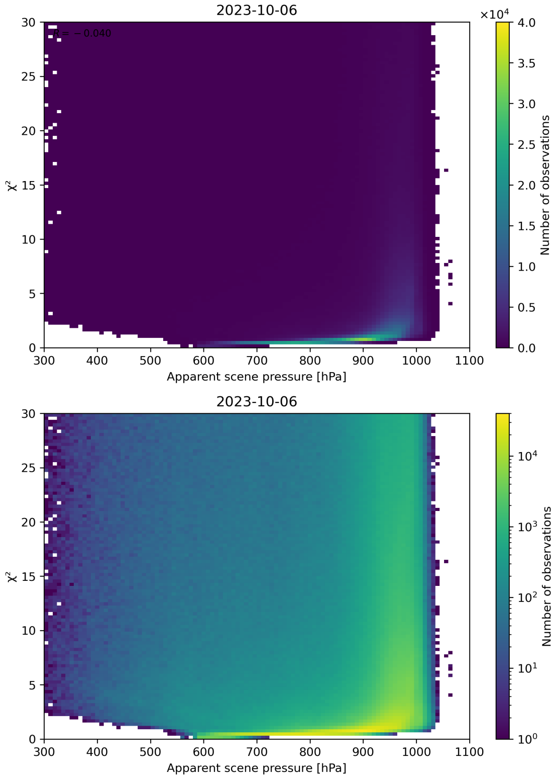
Figure 63: Scatter density plot of “Apparent scene pressure” against “ \chi^2 ” for 2023-10-06 to 2023-10-07.
