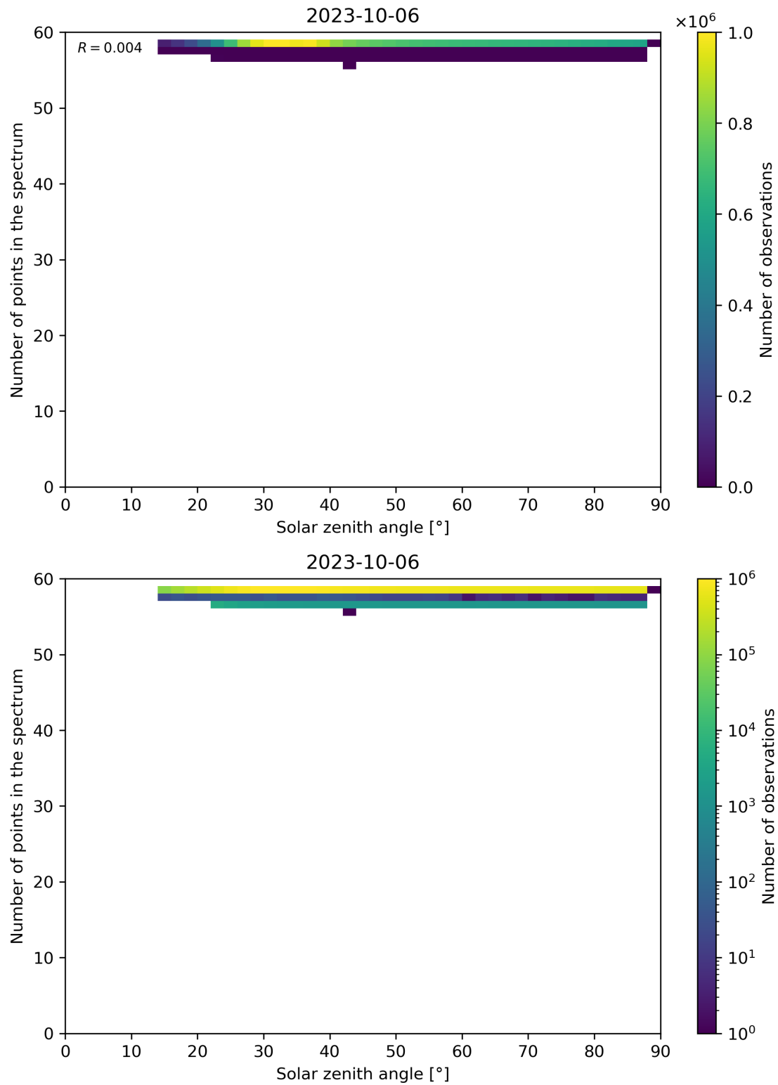
Figure 126: Scatter density plot of “Solar zenith angle” against “Number of points in the spectrum” for 2023-10-06 to 2023-10-07.
