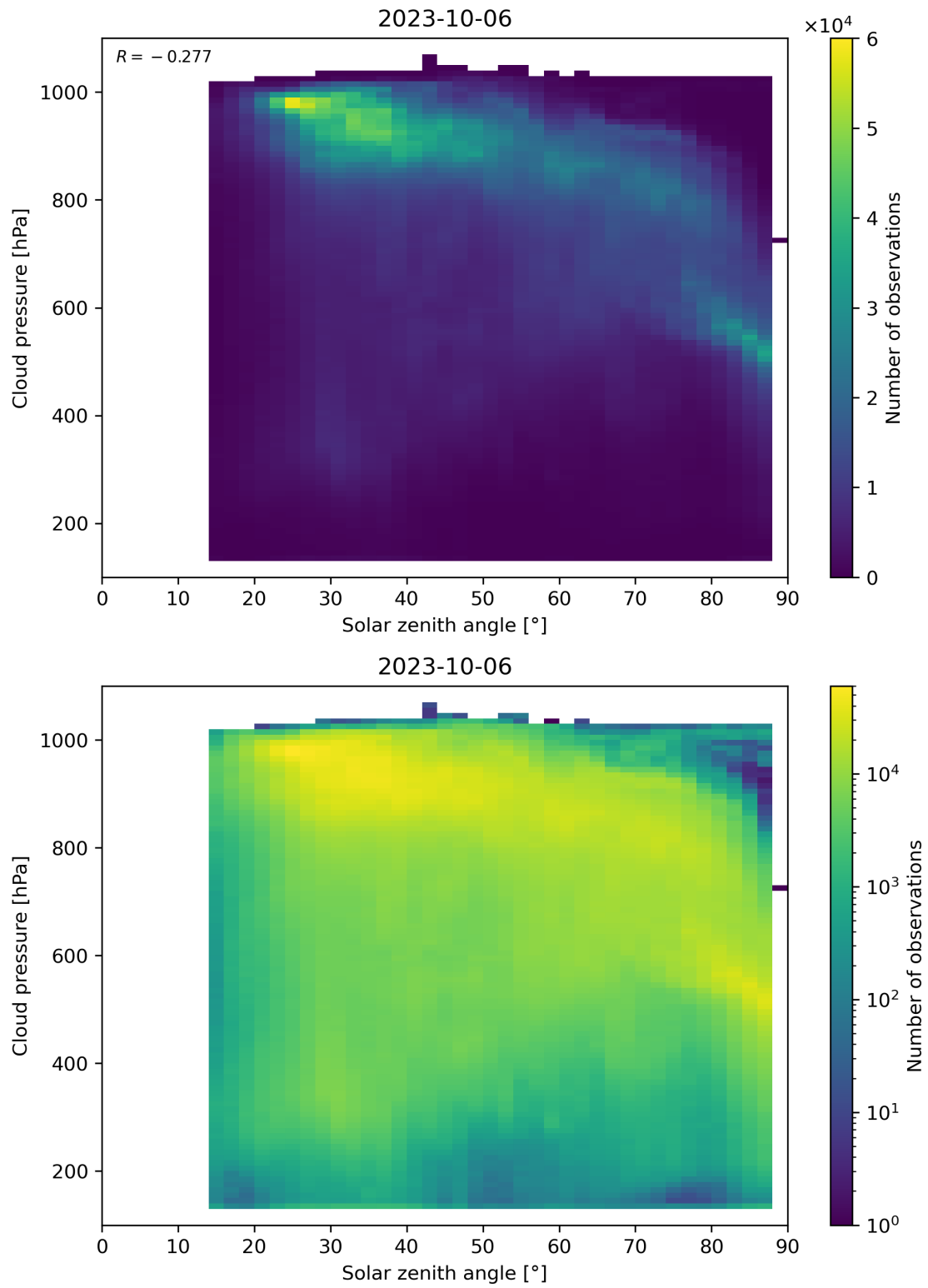
Figure 122: Scatter density plot of “Solar zenith angle” against “Cloud pressure” for 2023-10-06 to 2023-10-07.
