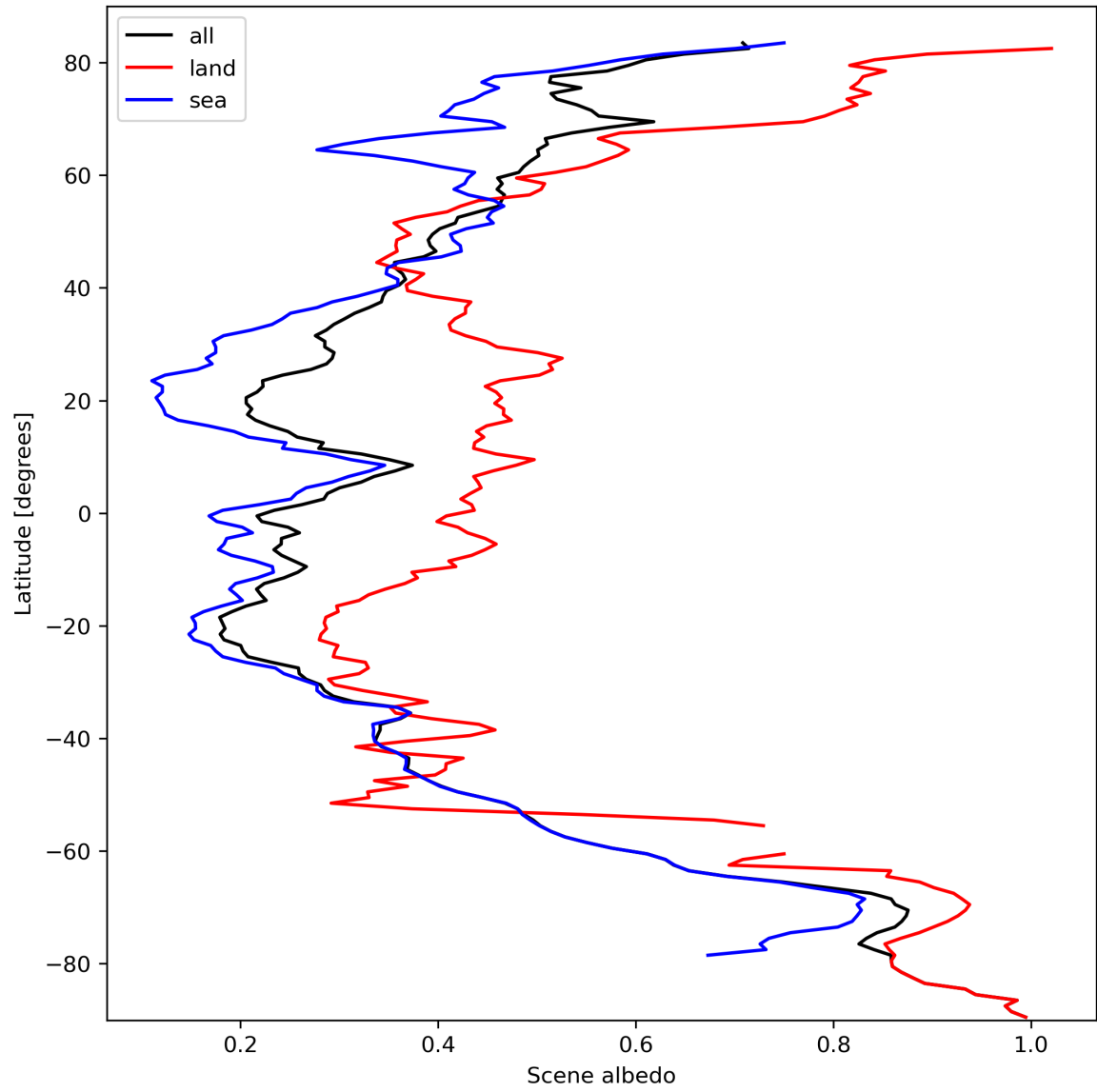
Figure 17: Zonal average of “Scene albedo” for 2023-10-06 to 2023-10-07.
