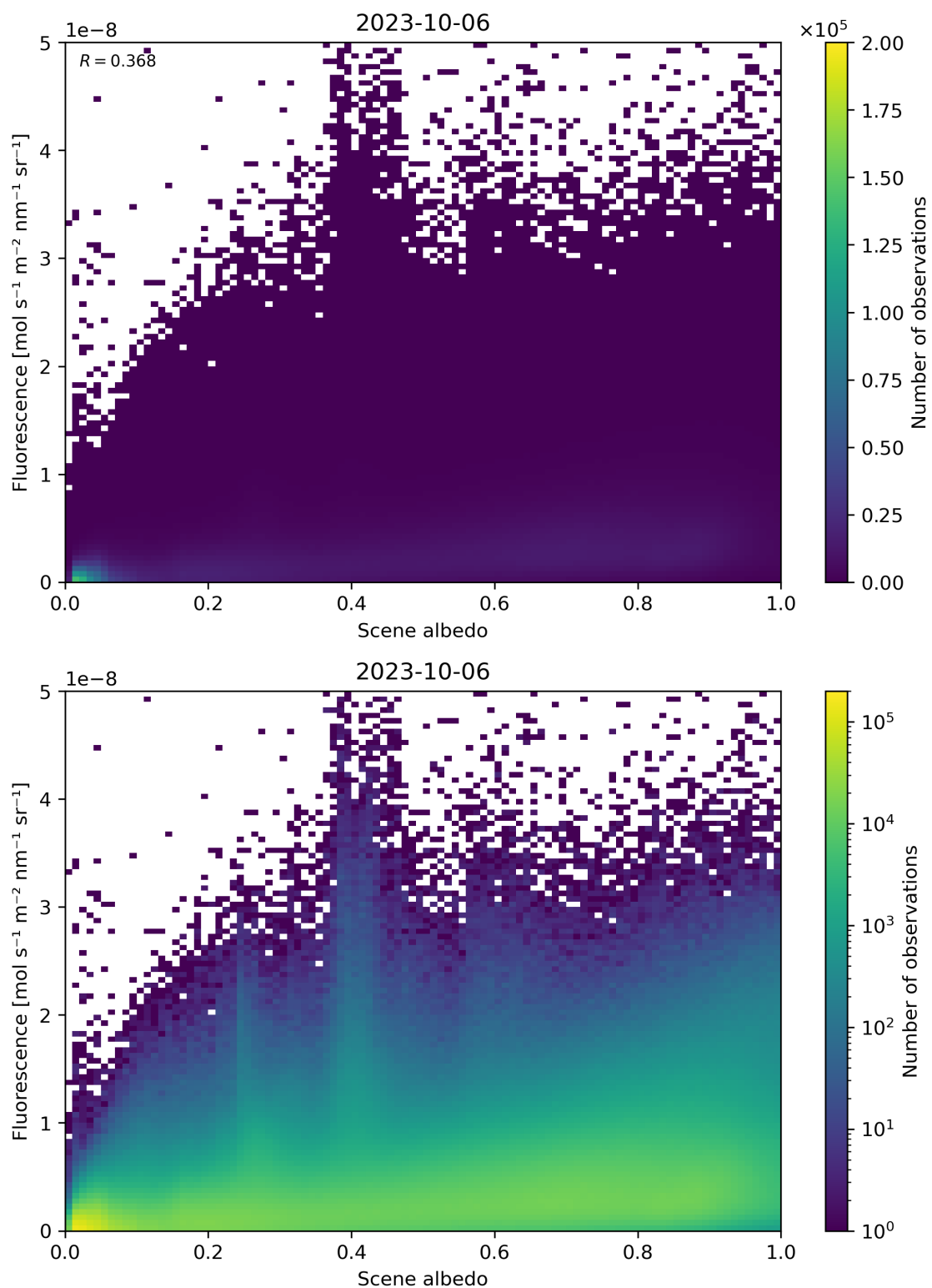
Figure 114: Scatter density plot of “Scene albedo” against “Fluorescence” for 2023-10-06 to 2023-10-07.
