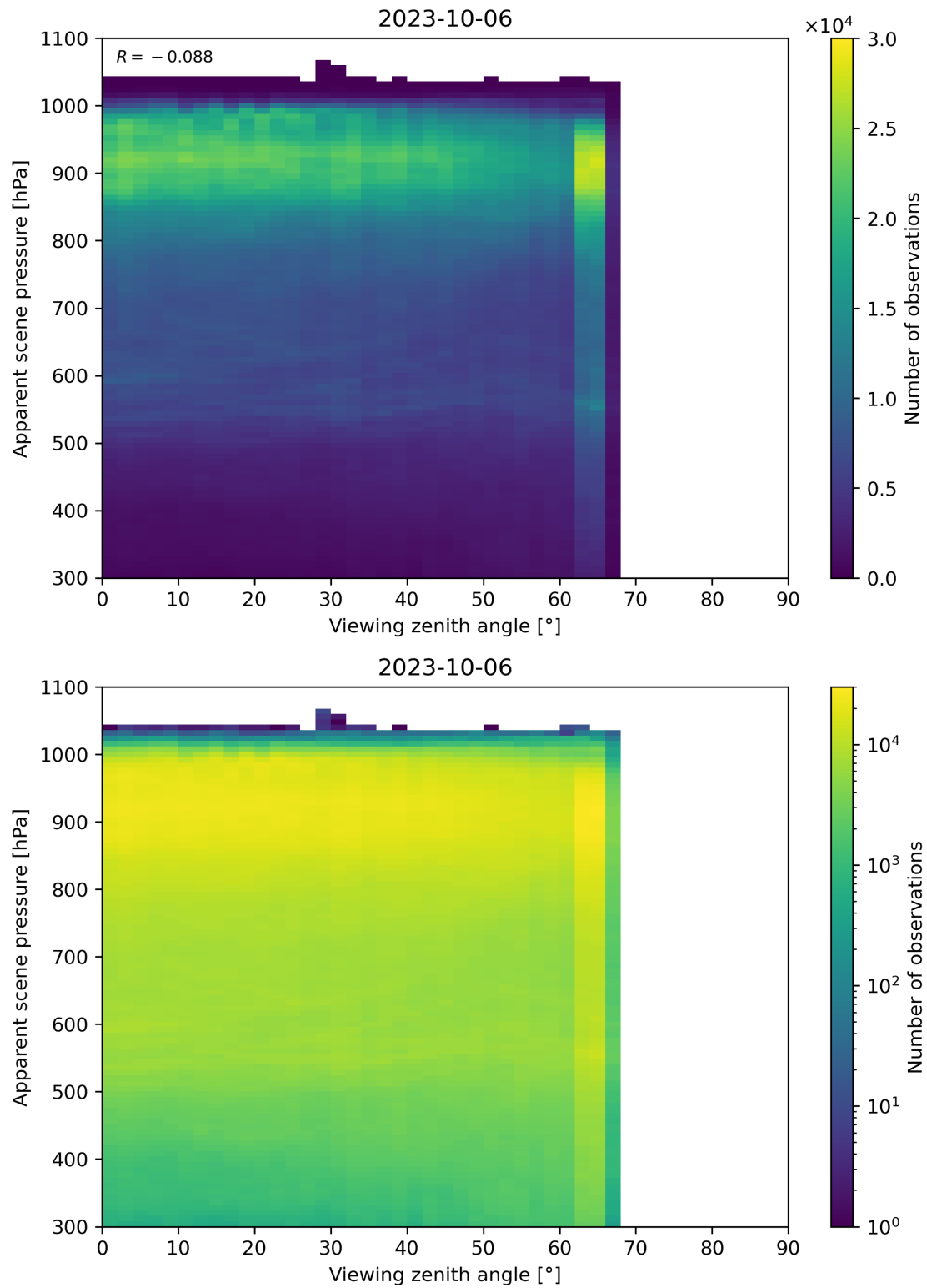
Figure 129: Scatter density plot of “Viewing zenith angle” against “Apparent scene pressure” for 2023-10-06 to 2023-10-07.
