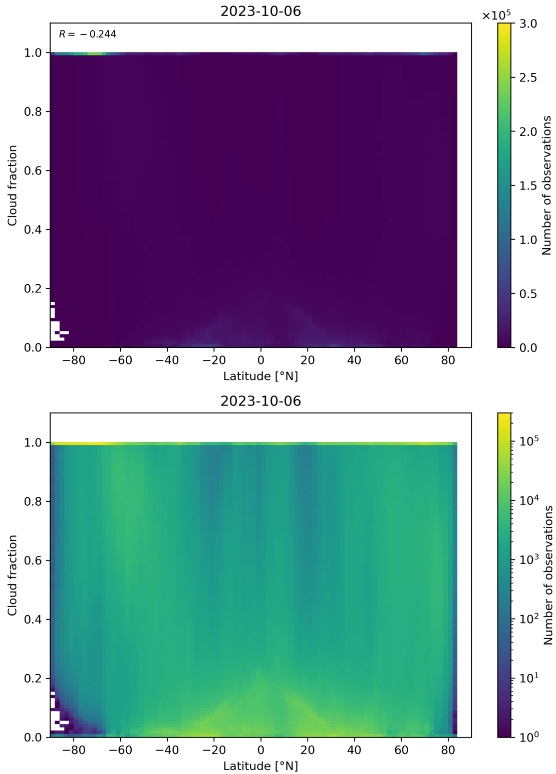
Figure 99: Scatter density plot of “Latitude” against “Cloud fraction” for 2023-10-06 to 2023-10-07.
