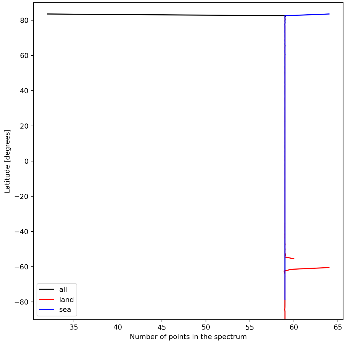
Figure 27: Zonal average of “Number of points in the spectrum” for 2023-10-06 to 2023-10-07.
