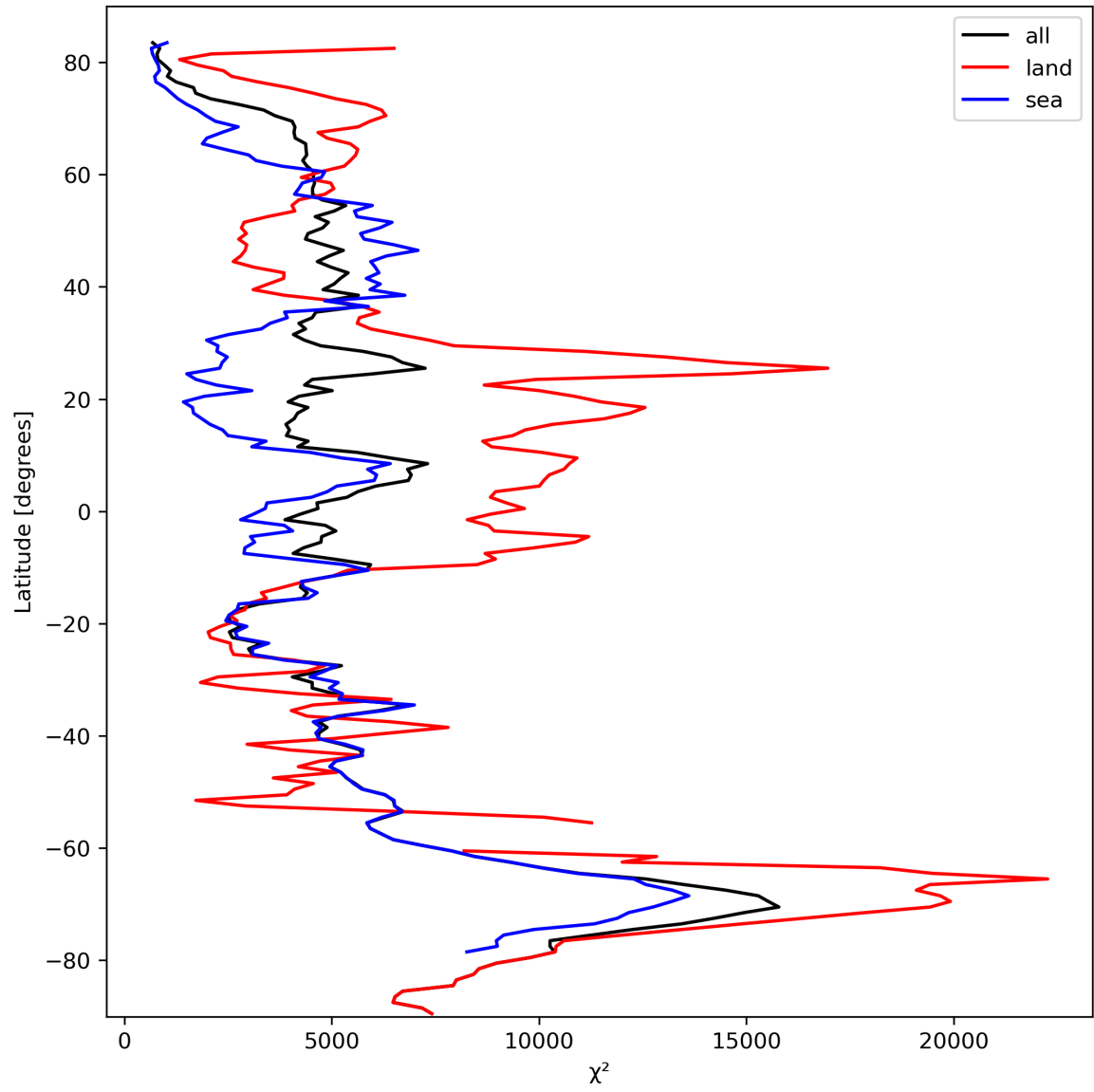
Figure 21: Zonal average of “ \chi^2 ” for 2023-10-06 to 2023-10-07.
