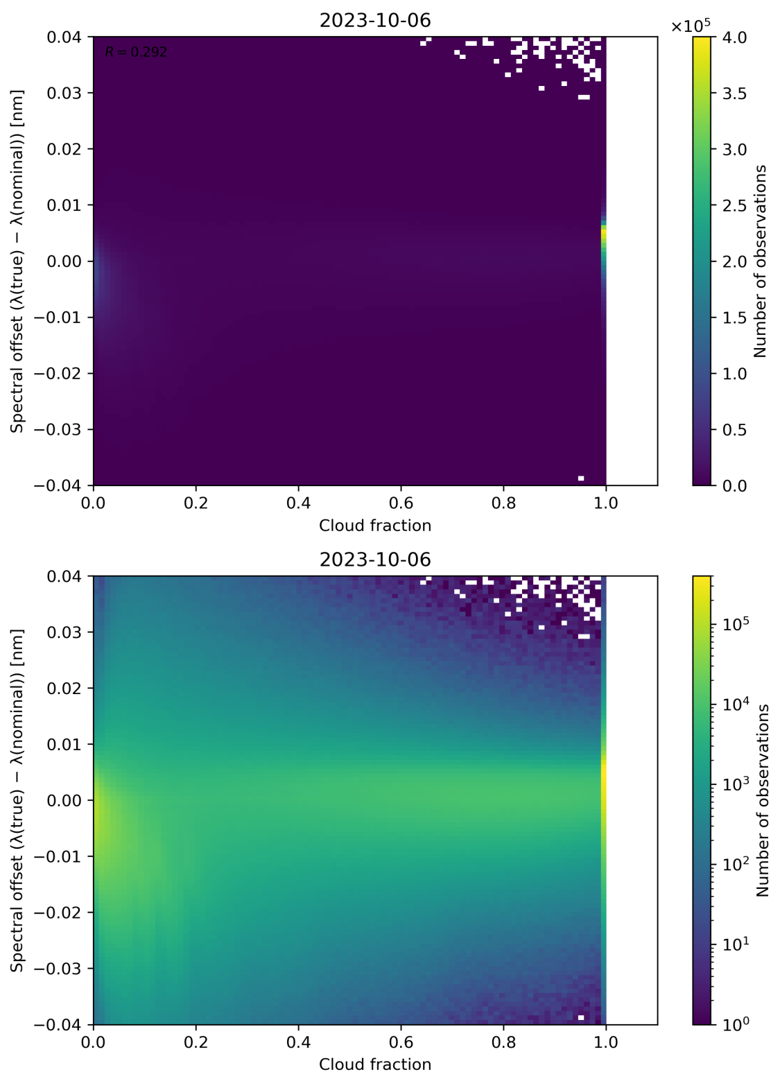
Figure 83: Scatter density plot of “Cloud fraction” against “Spectral offset ( \lambda(\text{true}) - \lambda(\text{nominal}) )” for 2023-10-06 to 2023-10-07.
