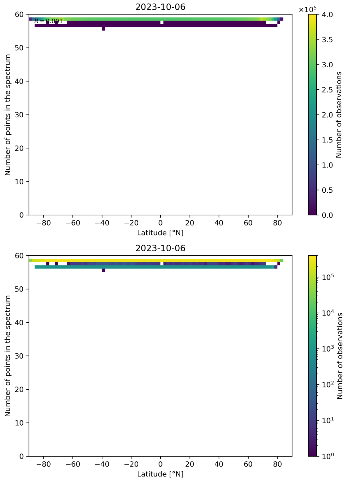
Figure 103: Scatter density plot of “Latitude” against “Number of points in the spectrum” for 2023-10-06 to 2023-10-07.
