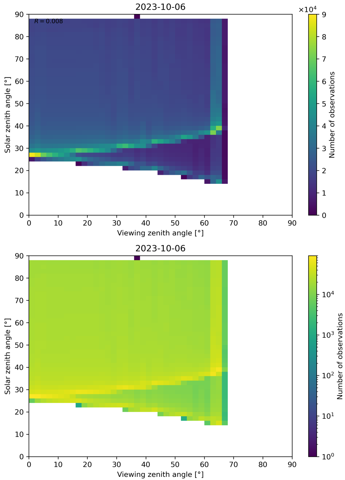
Figure 139: Scatter density plot of “Viewing zenith angle” against “Solar zenith angle” for 2023-10-06 to 2023-10-07.
