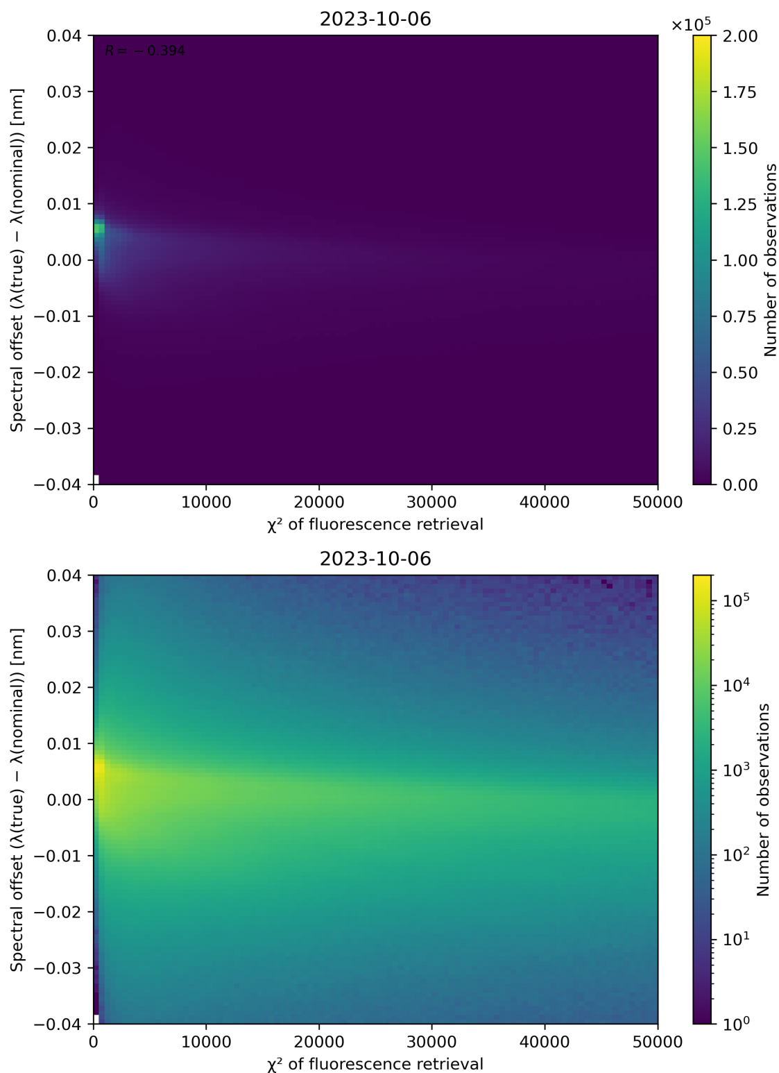
Figure 72: Scatter density plot of " \chi^2 of fluorescence retrieval" against "Spectral offset ( \lambda(\text{true}) - \lambda(\text{nominal})) " for 2023-10-06 to 2023-10-07.
