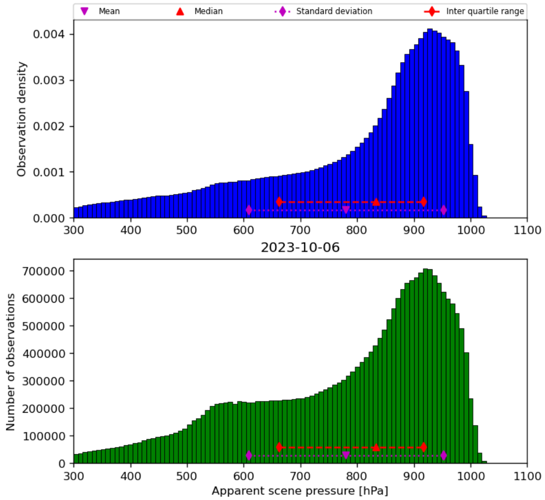
Figure 36: Histogram of “Apparent scene pressure” for 2023-10-06 to 2023-10-07
