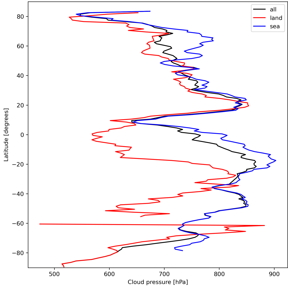
Figure 13: Zonal average of “Cloud pressure” for 2023-10-06 to 2023-10-07.
