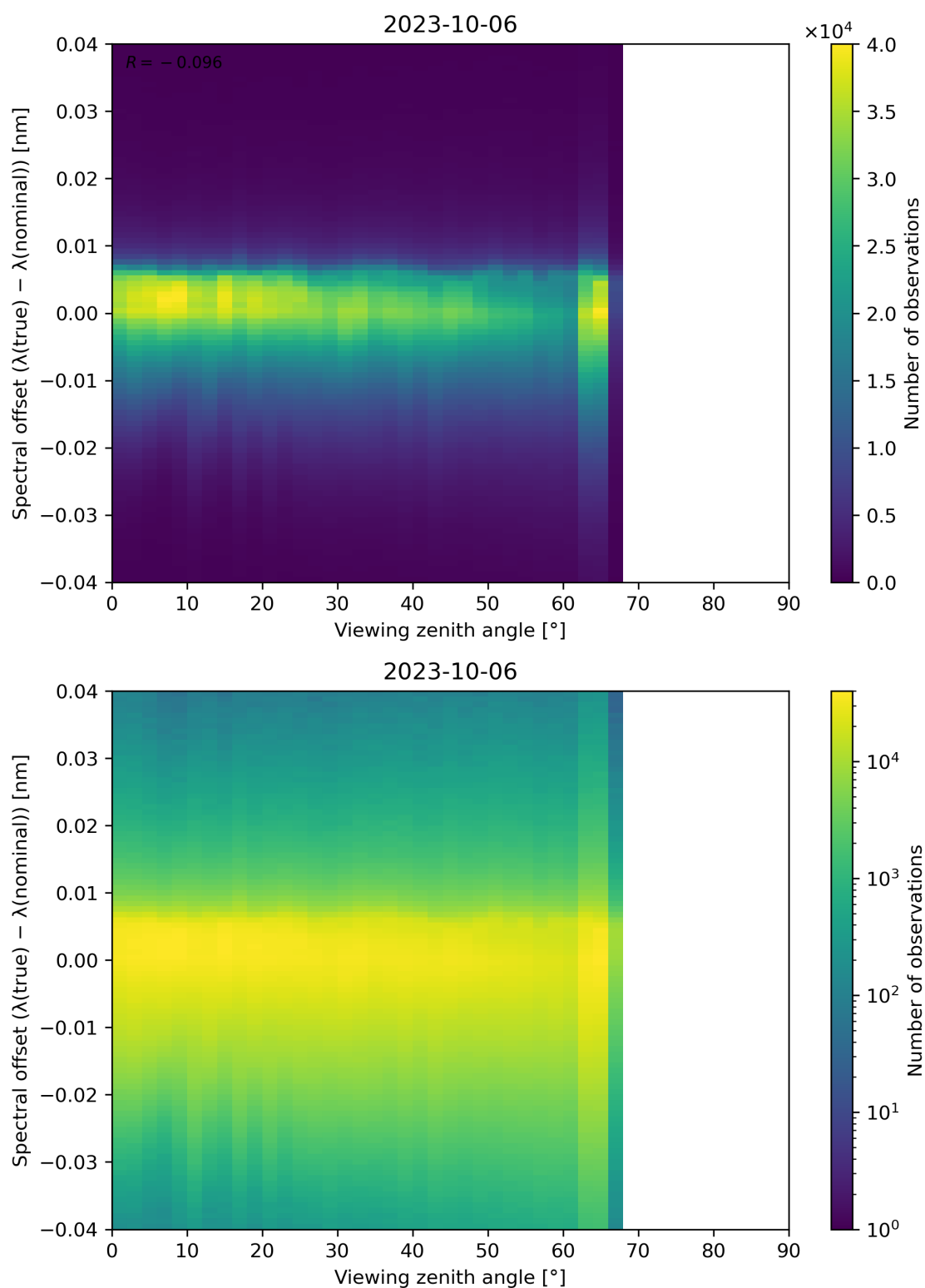
Figure 140: Scatter density plot of “Viewing zenith angle” against “Spectral offset ( \lambda(\text{true}) - \lambda(\text{nominal}) )” for 2023-10-06 to 2023-10-07.
