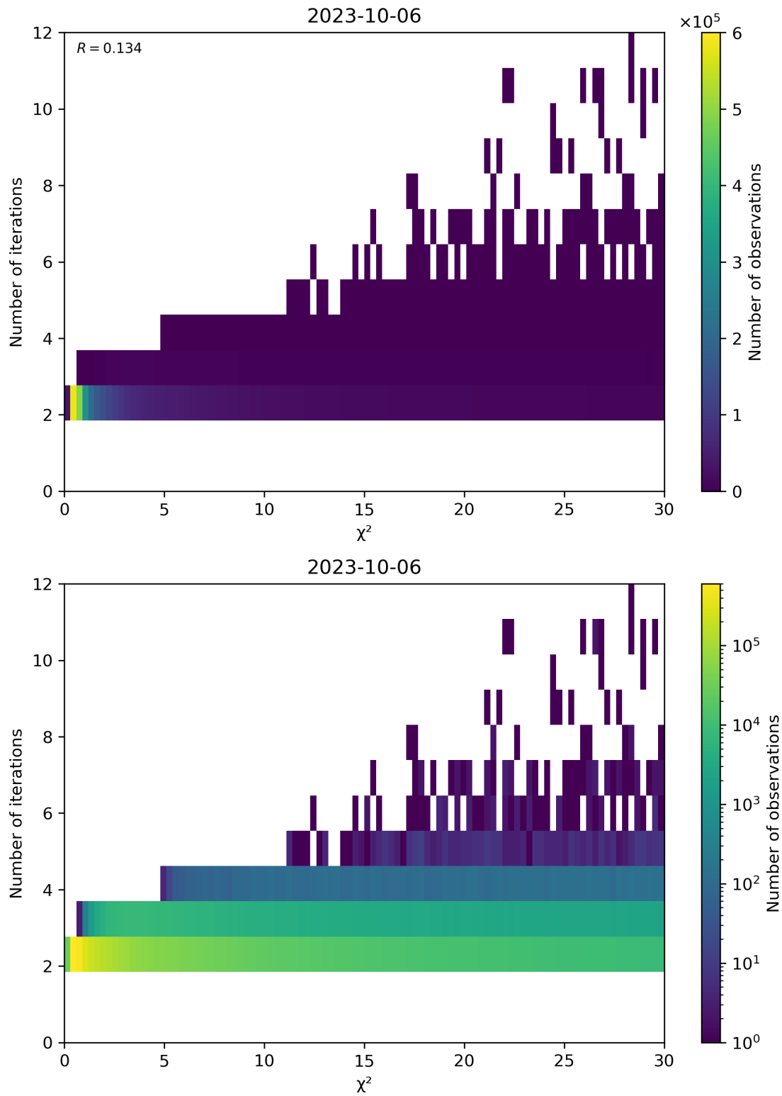
Figure 73: Scatter density plot of “ \chi^2 ” against “Number of iterations” for 2023-10-06 to 2023-10-07.
