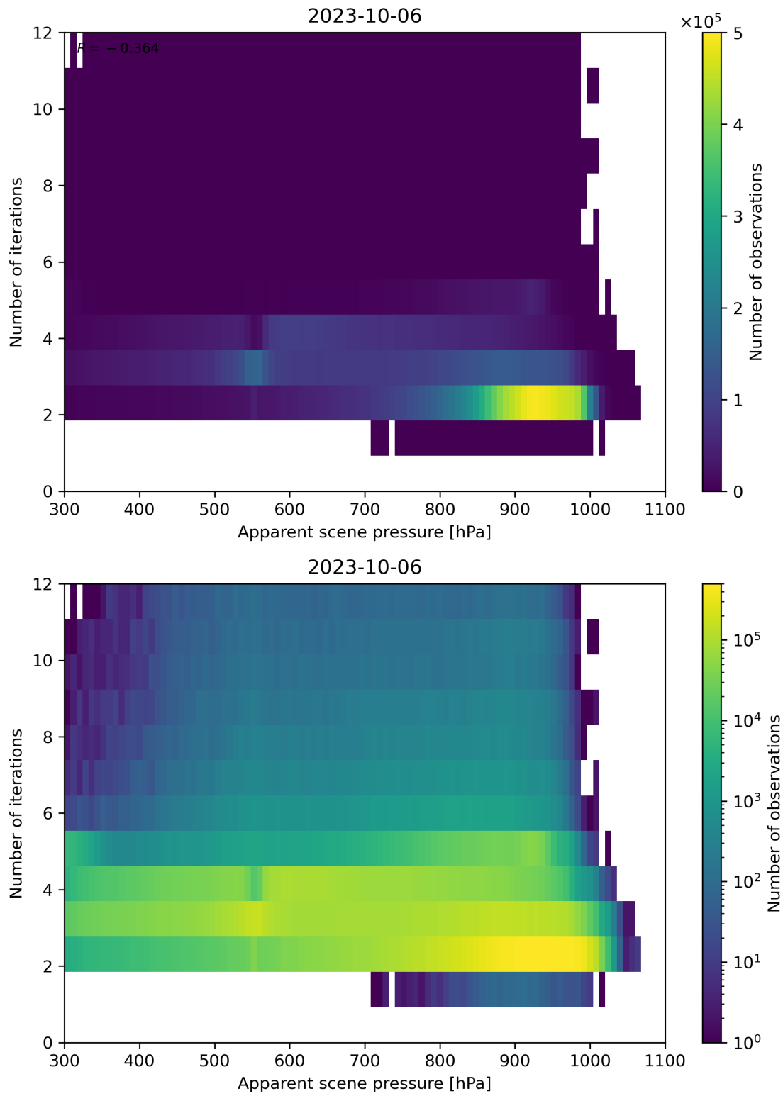
Figure 66: Scatter density plot of “Apparent scene pressure” against “Number of iterations” for 2023-10-06 to 2023-10-07.
