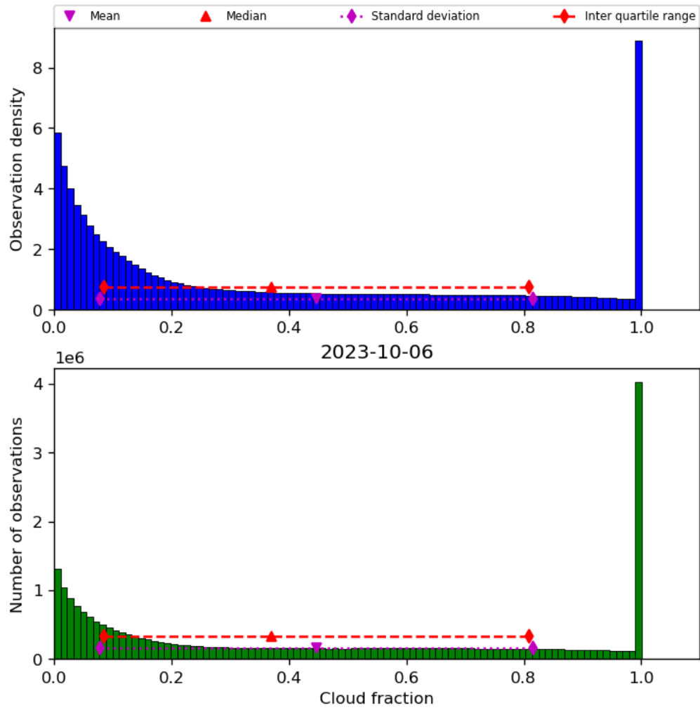
Figure 32: Histogram of “Cloud fraction” for 2023-10-06 to 2023-10-07
