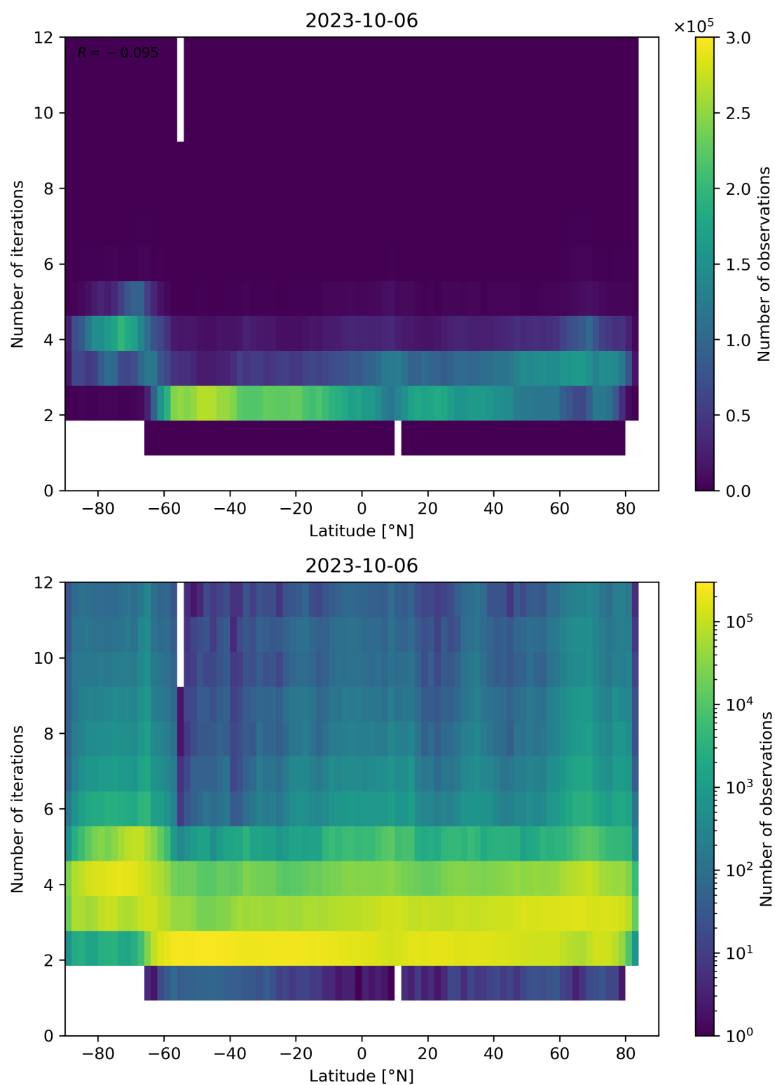
Figure 102: Scatter density plot of “Latitude” against “Number of iterations” for 2023-10-06 to 2023-10-07.
