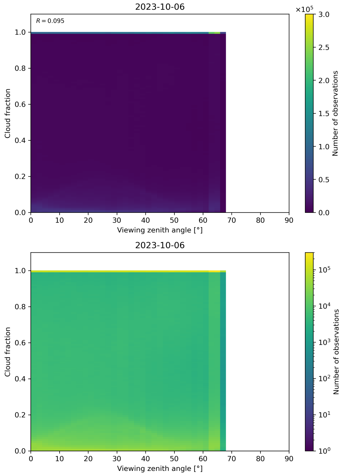
Figure 132: Scatter density plot of “Viewing zenith angle” against “Cloud fraction” for 2023-10-06 to 2023-10-07.
