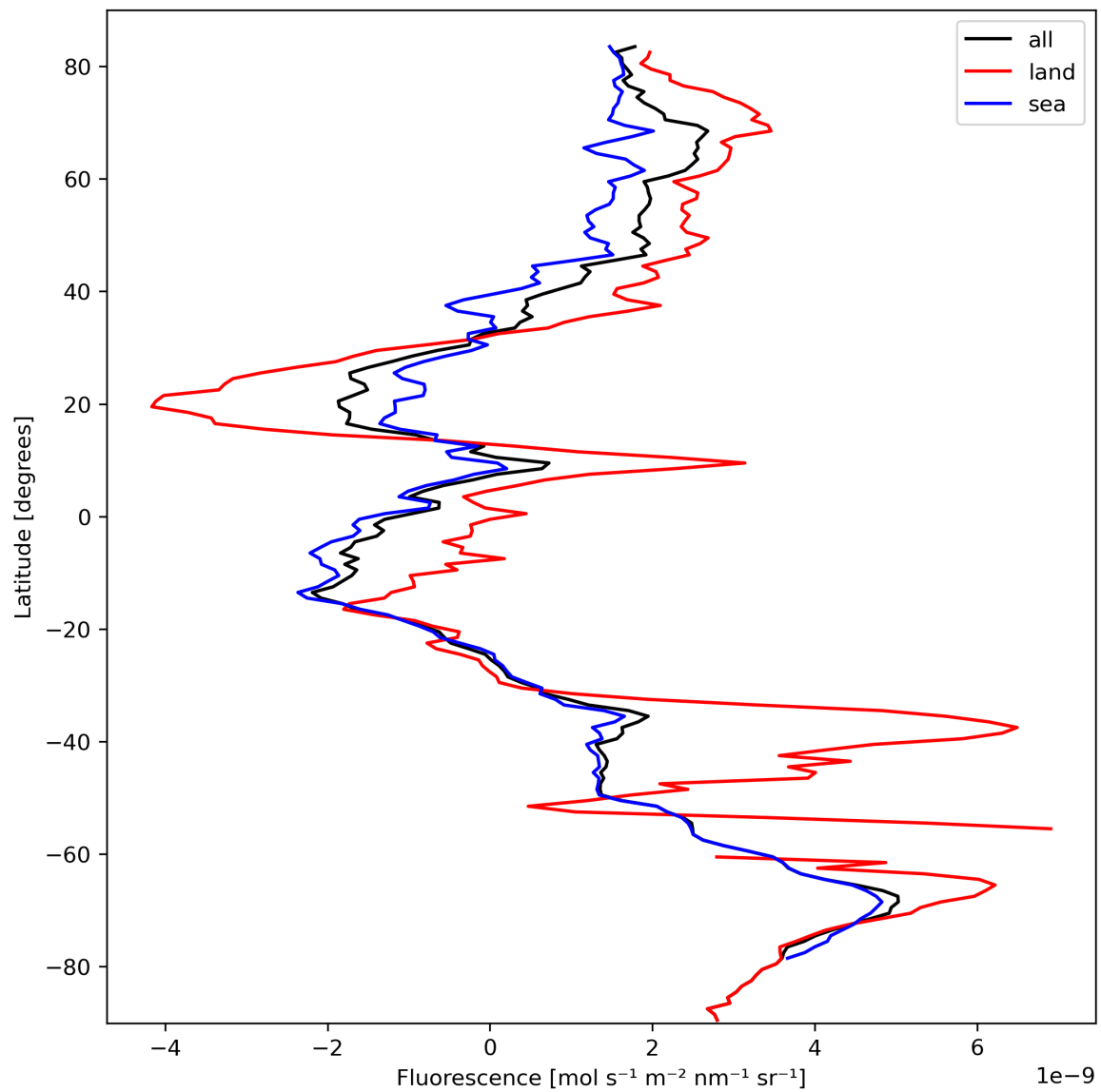
Figure 23: Zonal average of “Fluorescence” for 2023-10-06 to 2023-10-07.
