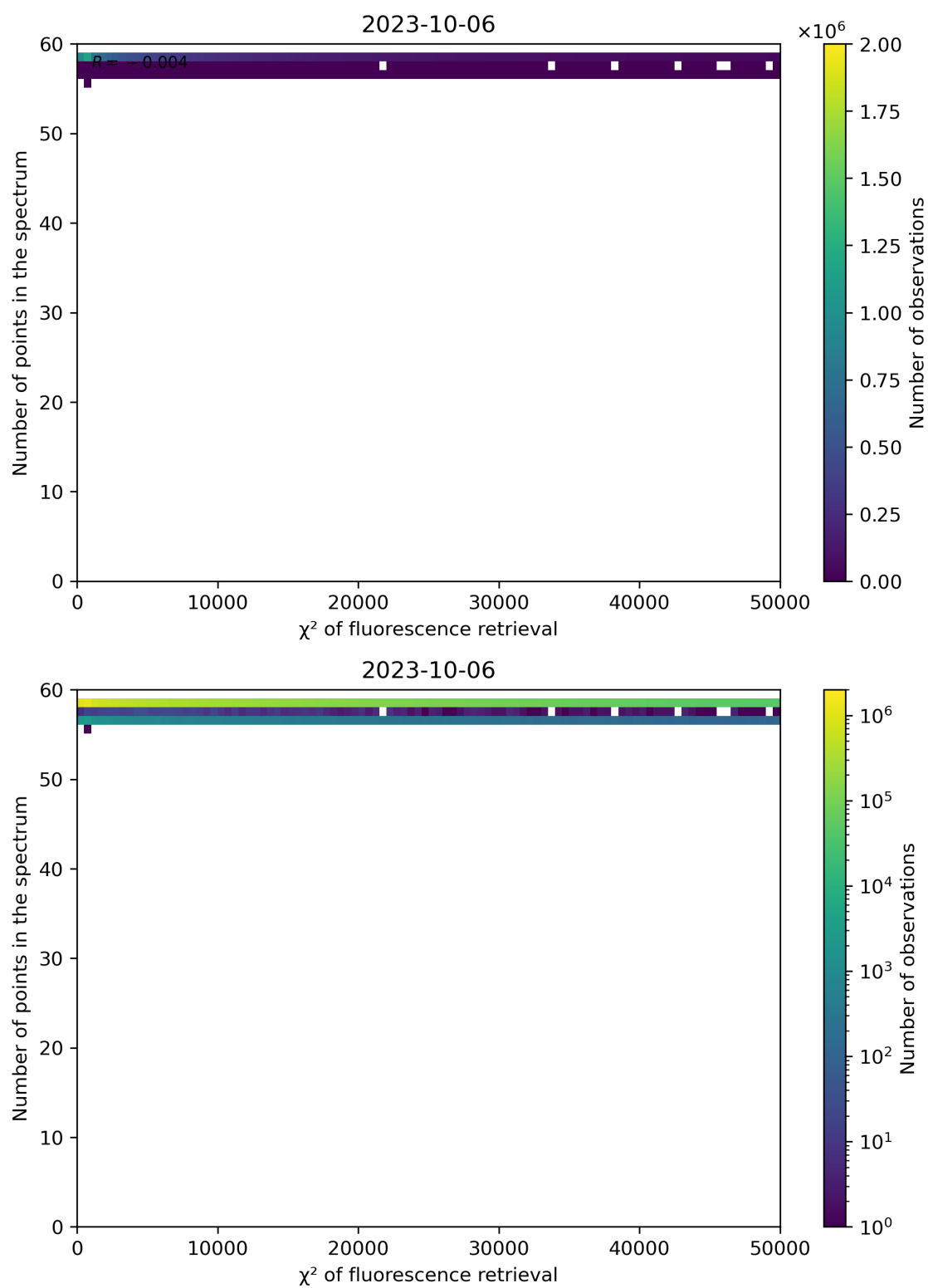
Figure 71: Scatter density plot of " \chi^2 of fluorescence retrieval" against "Number of points in the spectrum" for 2023-10-06 to 2023-10-07.
