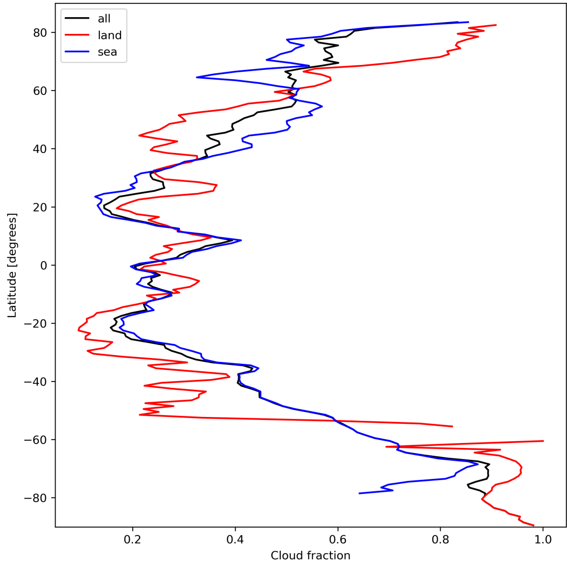
Figure 15: Zonal average of “Cloud fraction” for 2023-10-06 to 2023-10-07.
