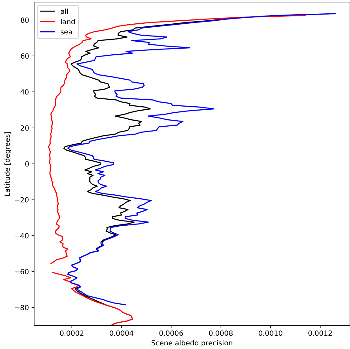
Figure 18: Zonal average of “Scene albedo precision” for 2023-10-06 to 2023-10-07.
