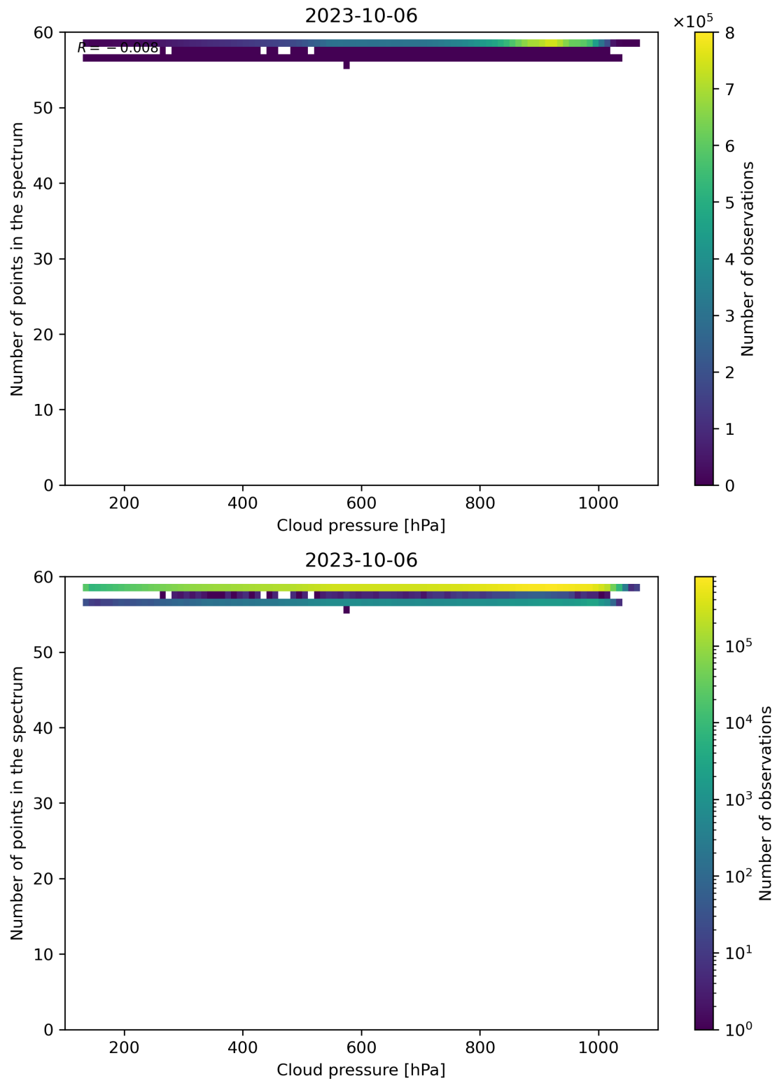
Figure 90: Scatter density plot of “Cloud pressure” against “Number of points in the spectrum” for 2023-10-06 to 2023-10-07.
