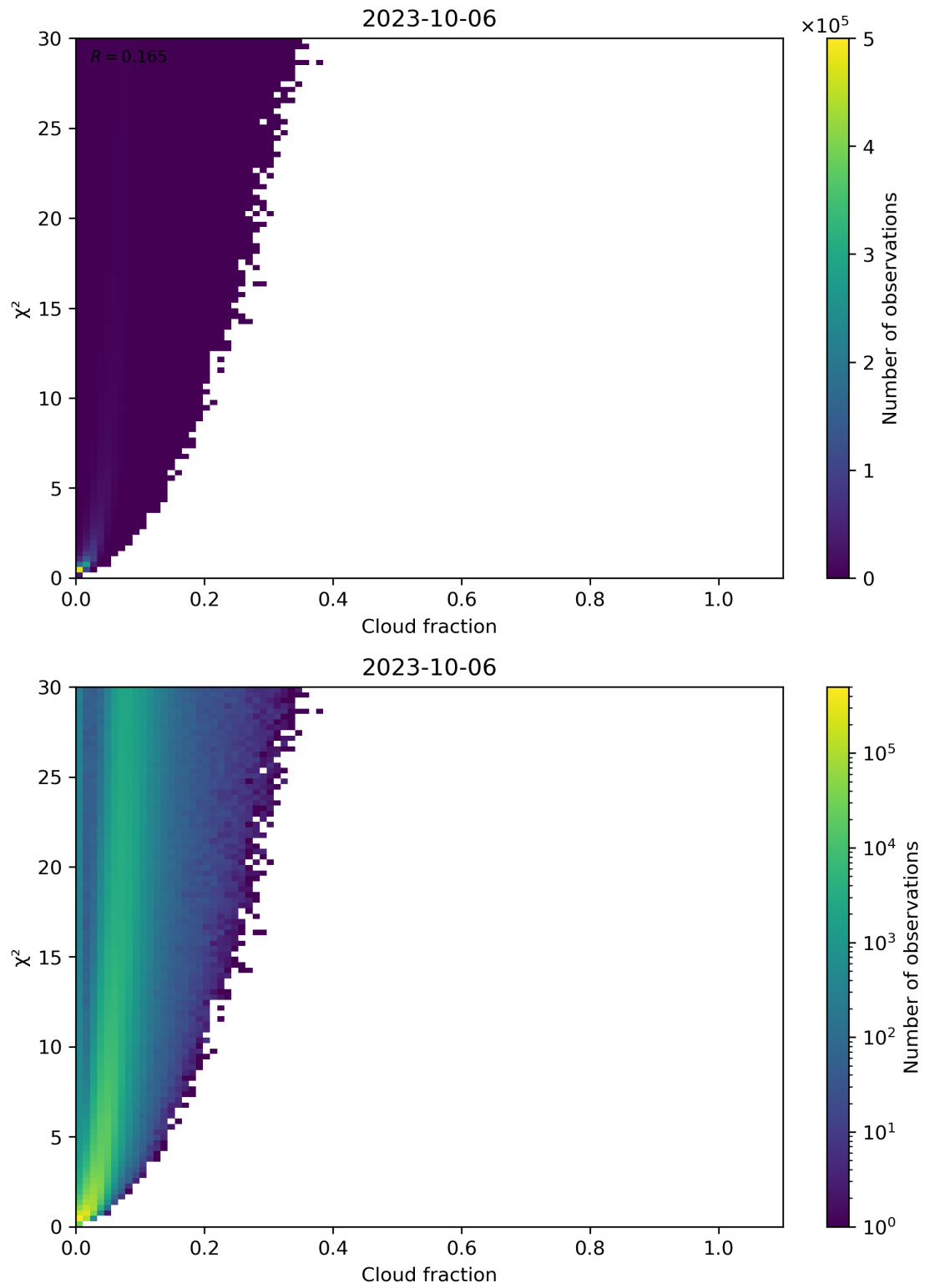
Figure 77: Scatter density plot of “Cloud fraction” against “ \chi^2 ” for 2023-10-06 to 2023-10-07.
