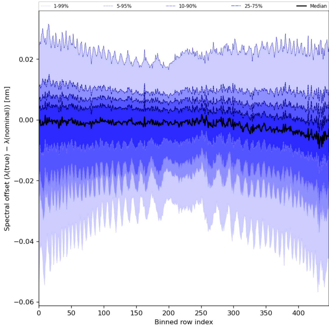
Figure 62: Along track statistics of “Spectral offset ( \lambda(\text{true}) - \lambda(\text{nominal}) )” for 2023-10-06 to 2023-10-07
