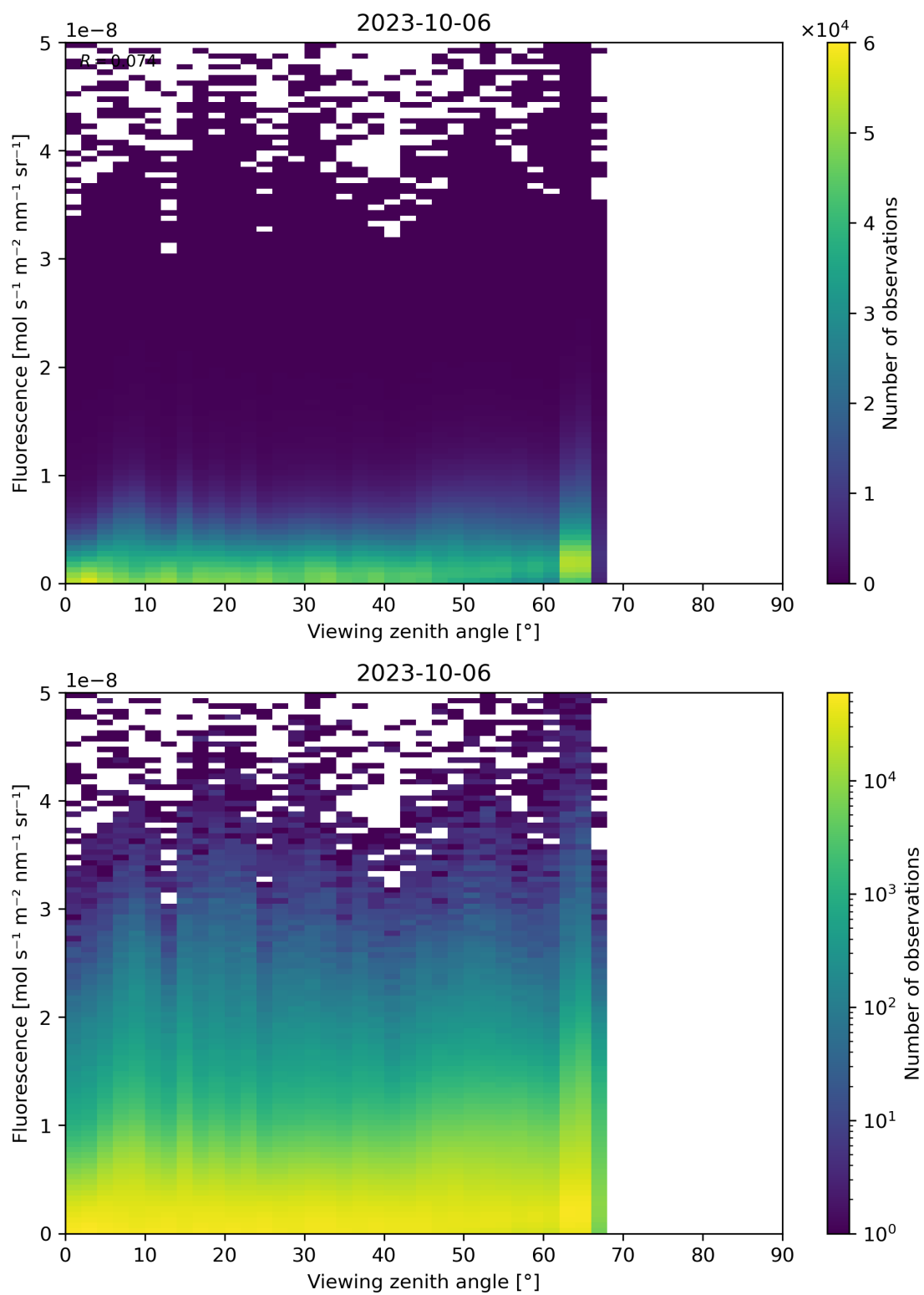
Figure 134: Scatter density plot of “Viewing zenith angle” against “Fluorescence” for 2023-10-06 to 2023-10-07.
