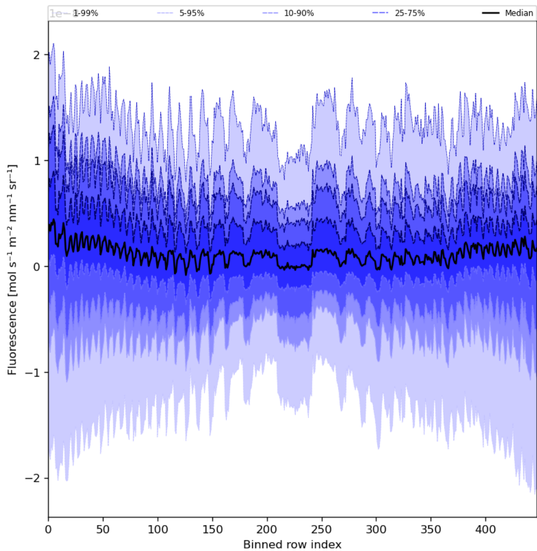
Figure 57: Along track statistics of “Fluorescence” for 2023-10-06 to 2023-10-07
