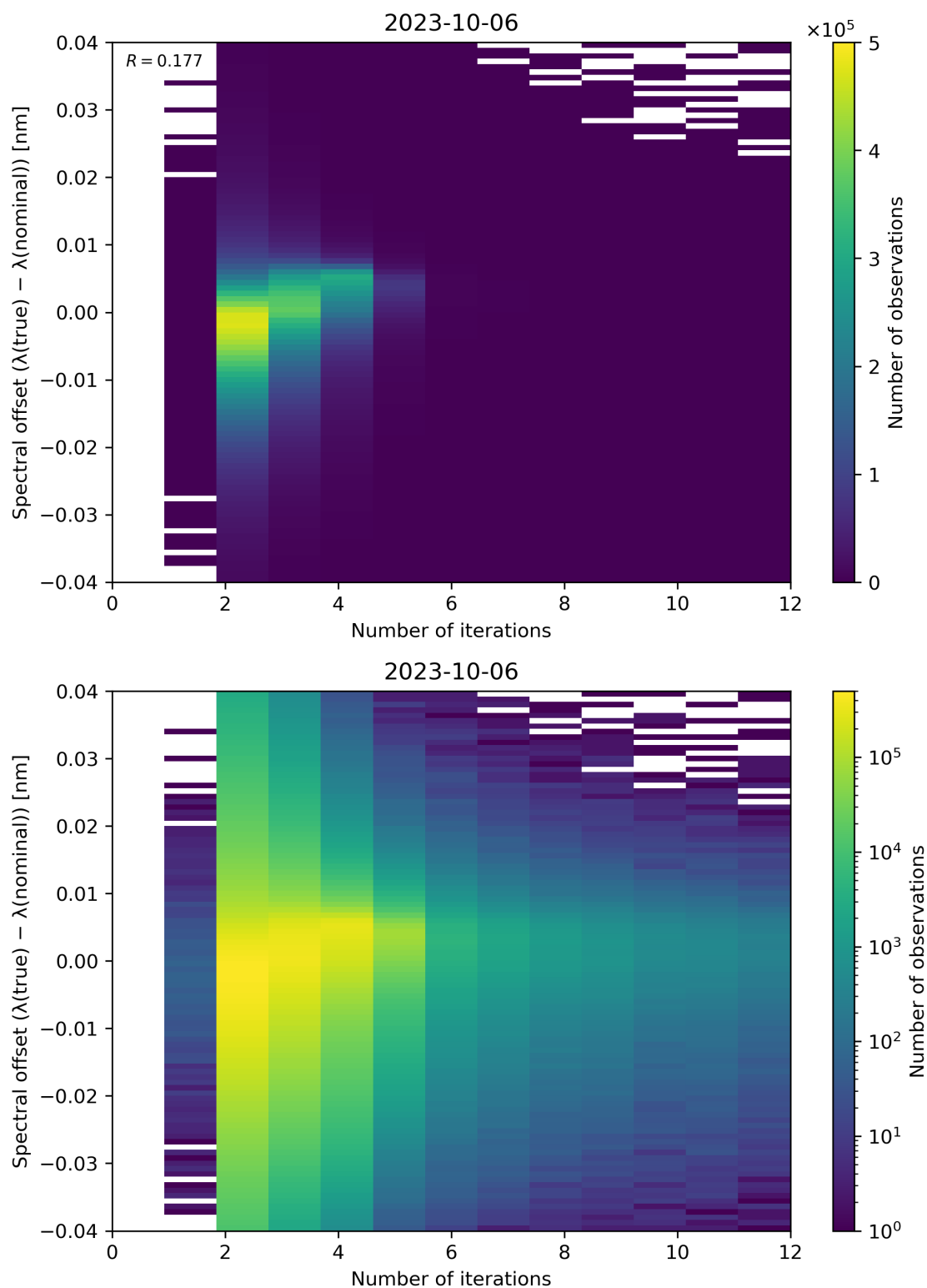
Figure 109: Scatter density plot of “Number of iterations” against “Spectral offset ( \lambda(\text{true}) - \lambda(\text{nominal}) )” for 2023-10-06 to 2023-10-07.
