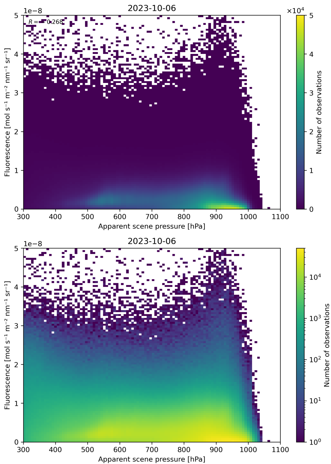
Figure 65: Scatter density plot of “Apparent scene pressure” against “Fluorescence” for 2023-10-06 to 2023-10-07.
