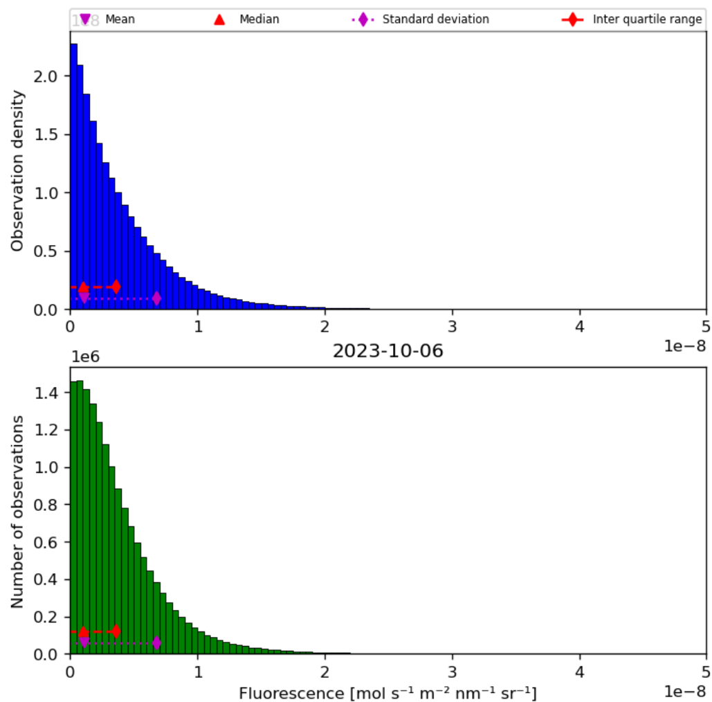
Figure 40: Histogram of “Fluorescence” for 2023-10-06 to 2023-10-07
