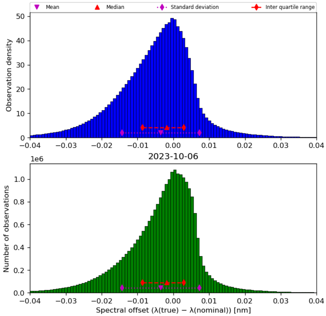
Figure 45: Histogram of “Spectral offset ( \lambda(\text{true}) - \lambda(\text{nominal}) )” for 2023-10-06 to 2023-10-07
