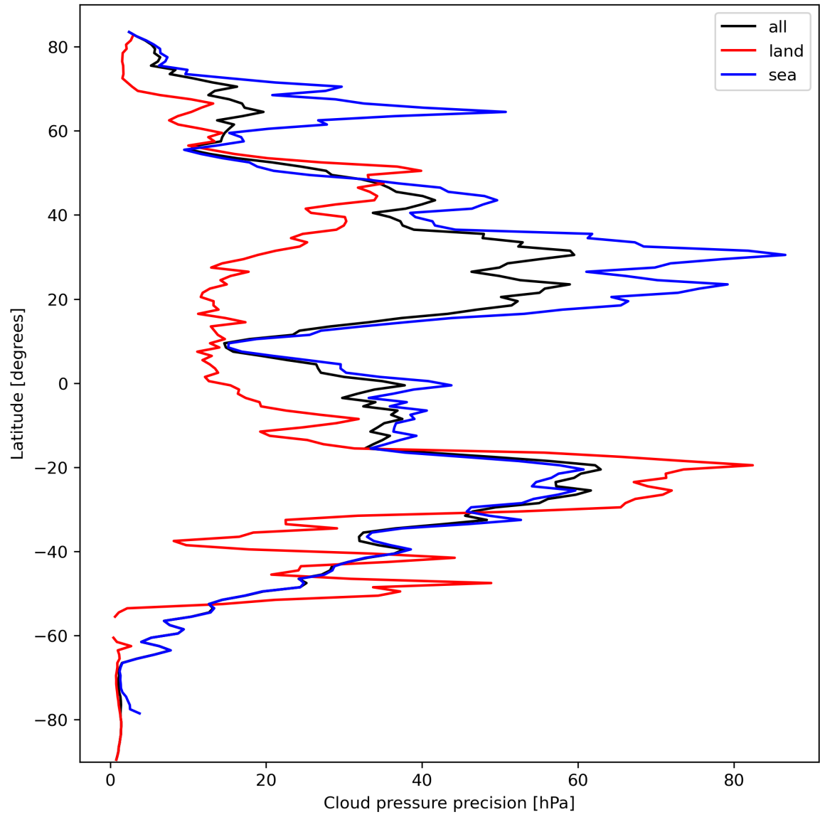
Figure 14: Zonal average of “Cloud pressure precision” for 2023-10-06 to 2023-10-07.
