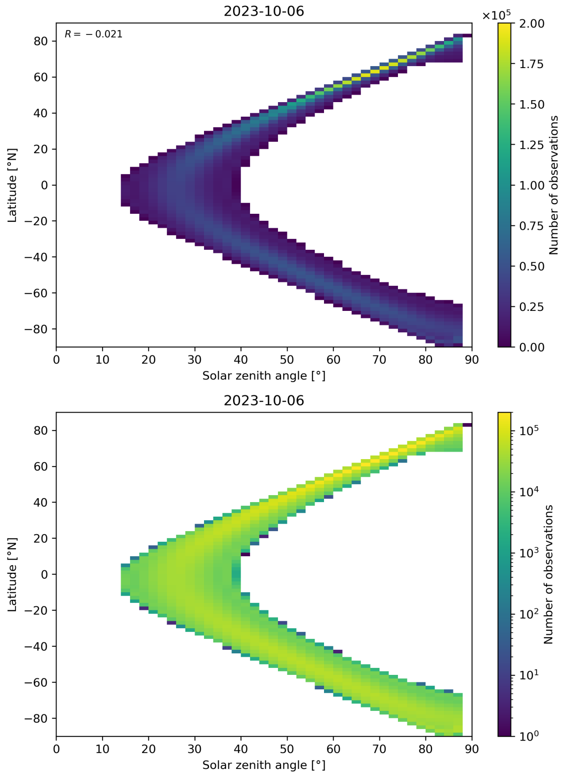
Figure 124: Scatter density plot of “Solar zenith angle” against “Latitude” for 2023-10-06 to 2023-10-07.
