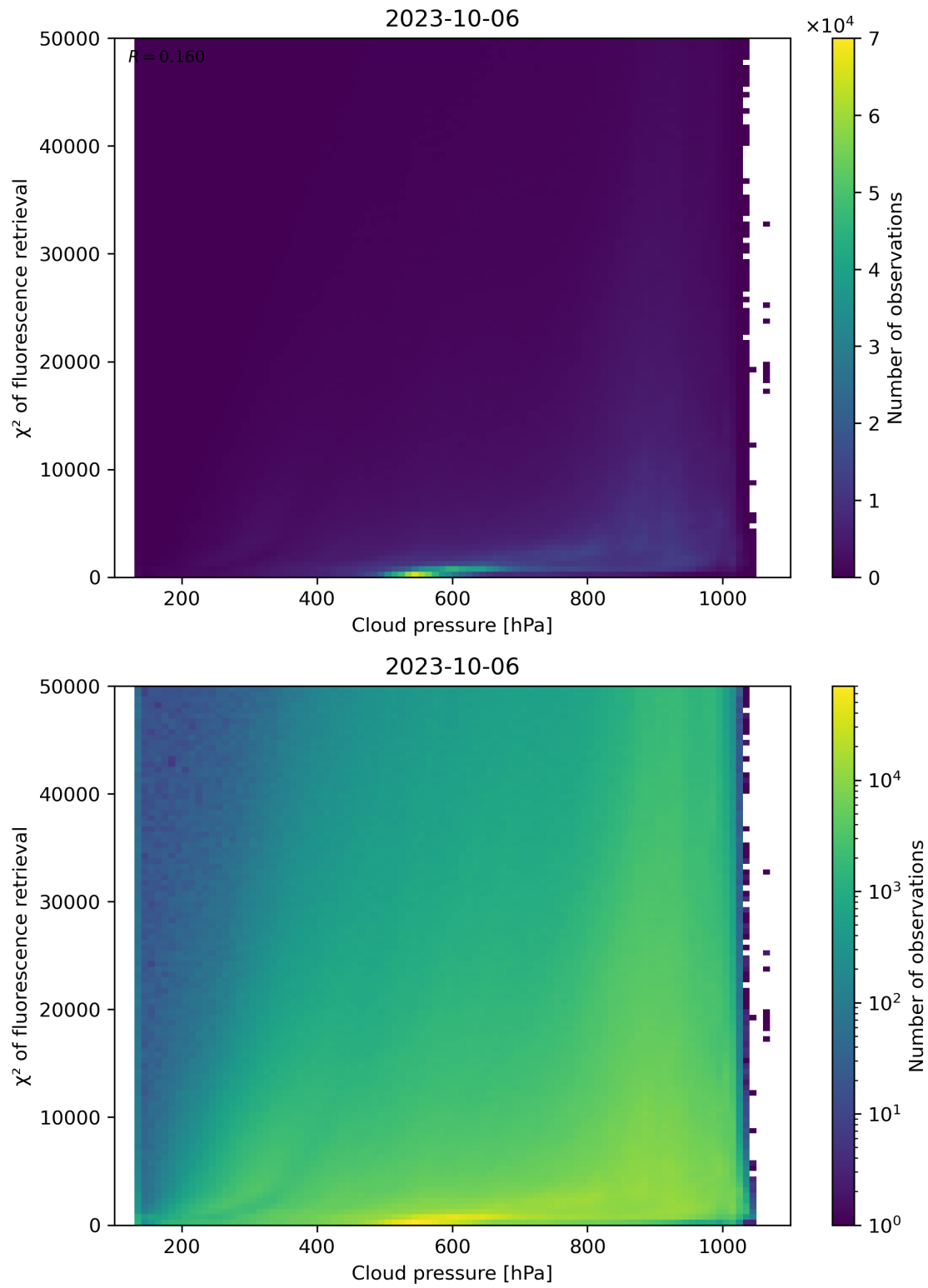
Figure 86: Scatter density plot of “Cloud pressure” against “ \chi^2 of fluorescence retrieval” for 2023-10-06 to 2023-10-07.
