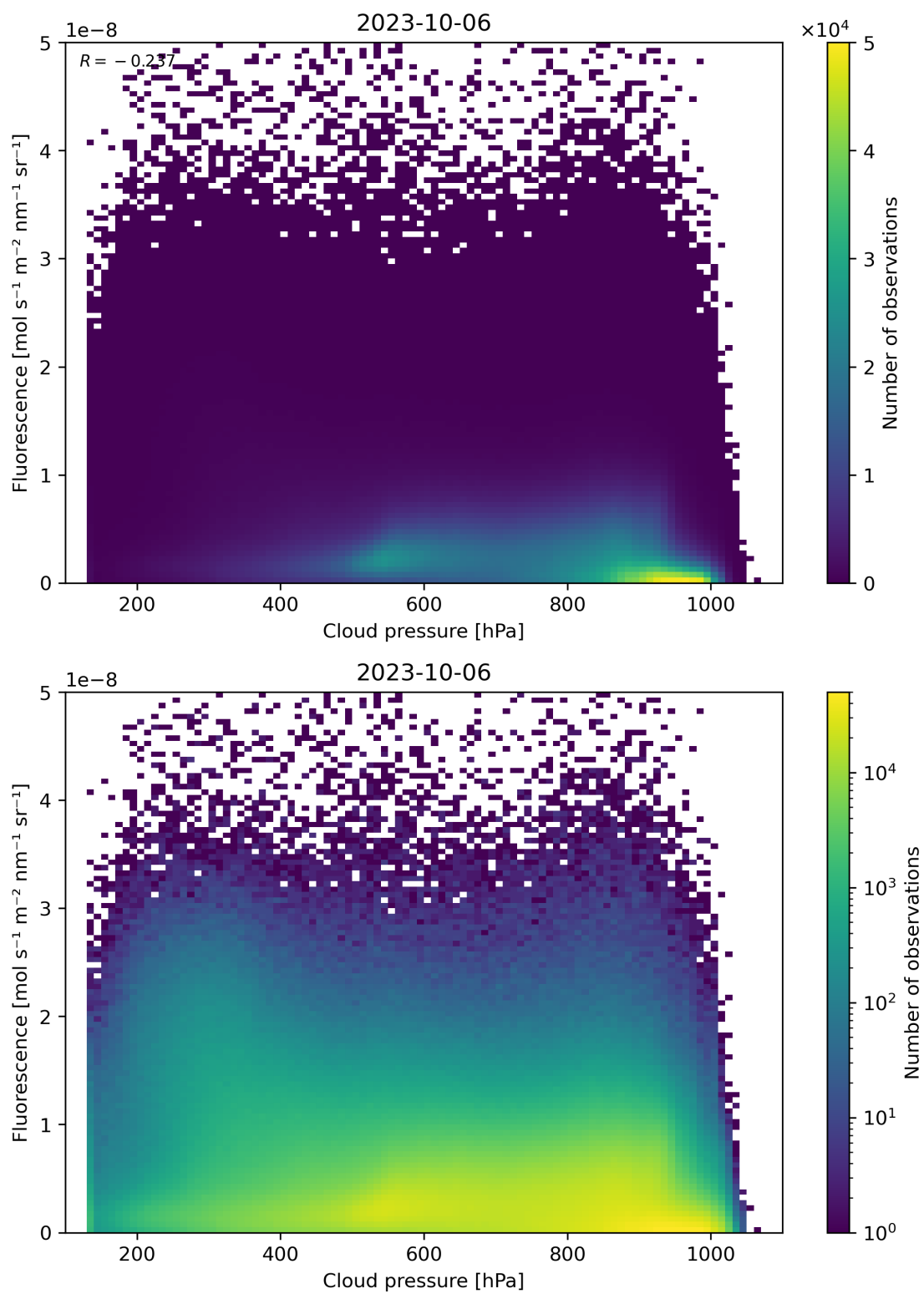
Figure 88: Scatter density plot of “Cloud pressure” against “Fluorescence” for 2023-10-06 to 2023-10-07.
