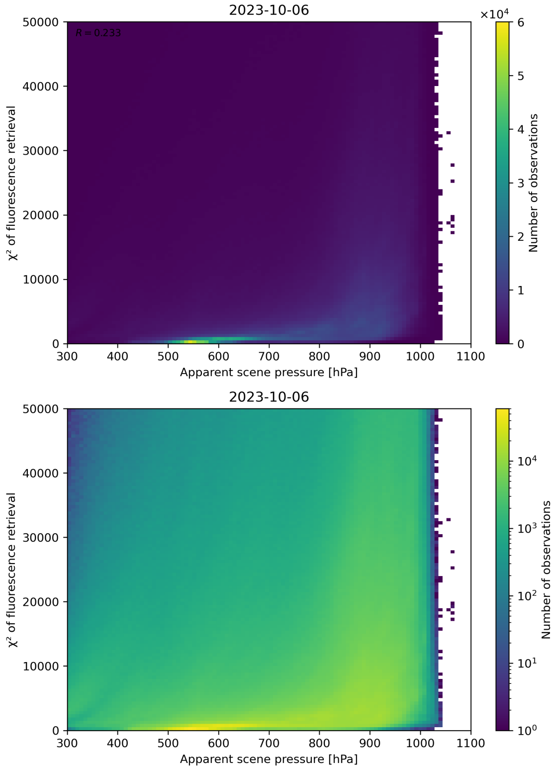
Figure 64: Scatter density plot of “Apparent scene pressure” against “ \chi^2 of fluorescence retrieval” for 2023-10-06 to 2023-10-07.
