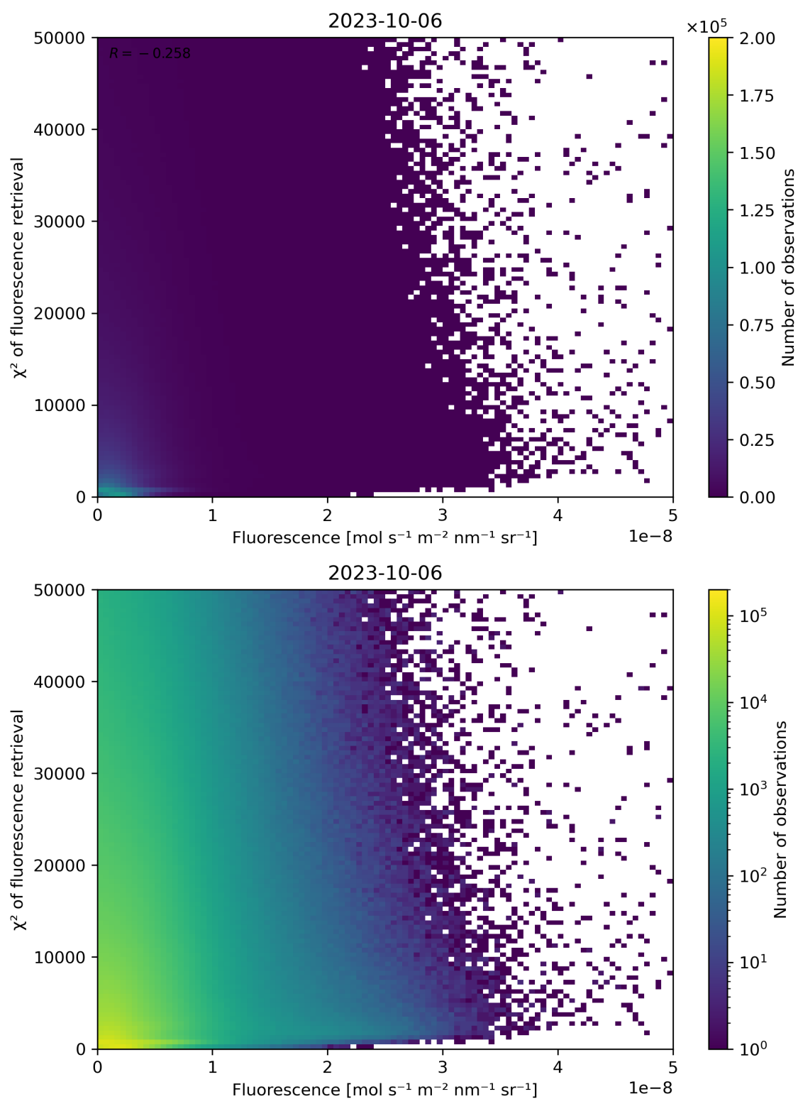
Figure 93: Scatter density plot of “Fluorescence” against “ \chi^2 of fluorescence retrieval” for 2023-10-06 to 2023-10-07.
