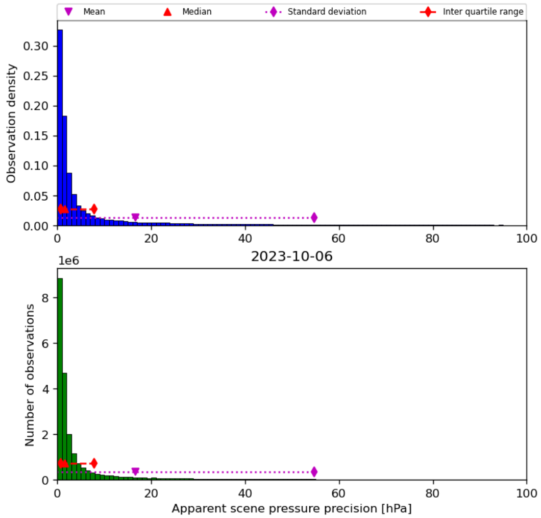
Figure 37: Histogram of “Apparent scene pressure precision” for 2023-10-06 to 2023-10-07
