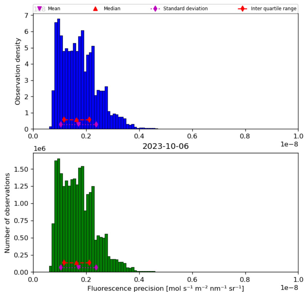
Figure 41: Histogram of “Fluorescence precision” for 2023-10-06 to 2023-10-07
