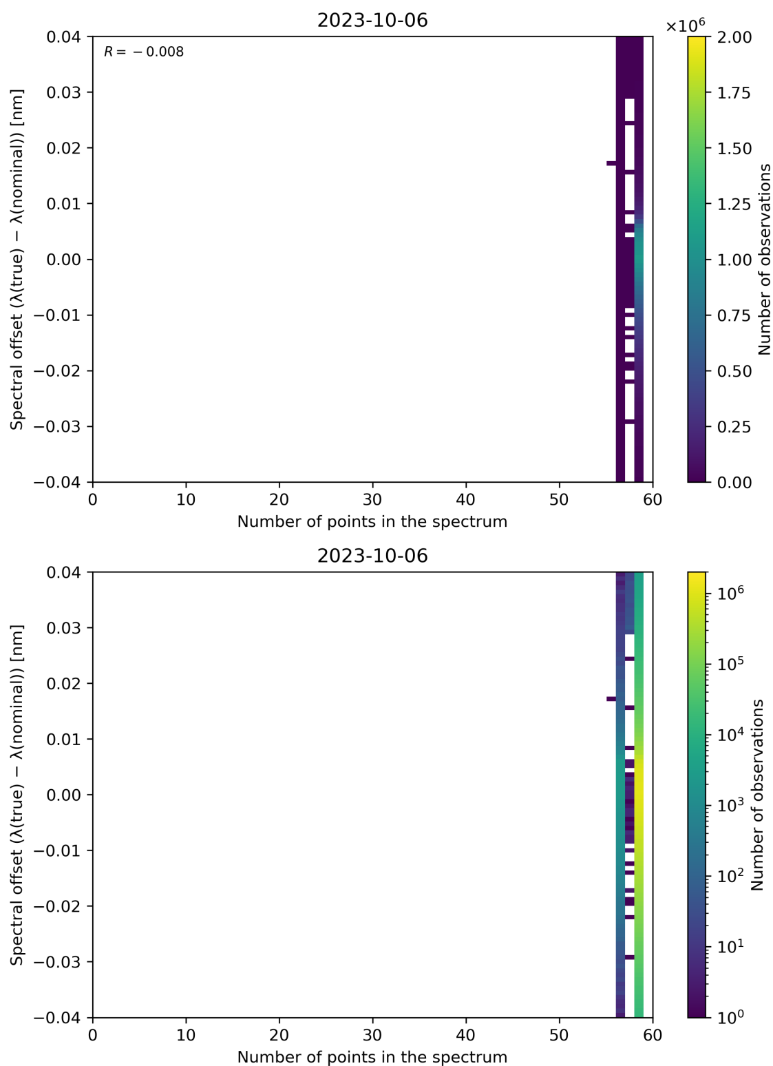
Figure 110: Scatter density plot of “Number of points in the spectrum” against “Spectral offset ( \lambda(\text{true}) - \lambda(\text{nominal}) )” for 2023-10-06 to 2023-10-07.
