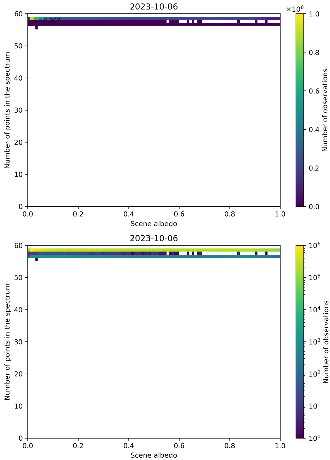
Figure 116: Scatter density plot of “Scene albedo” against “Number of points in the spectrum” for 2023-10-06 to 2023-10-07.
