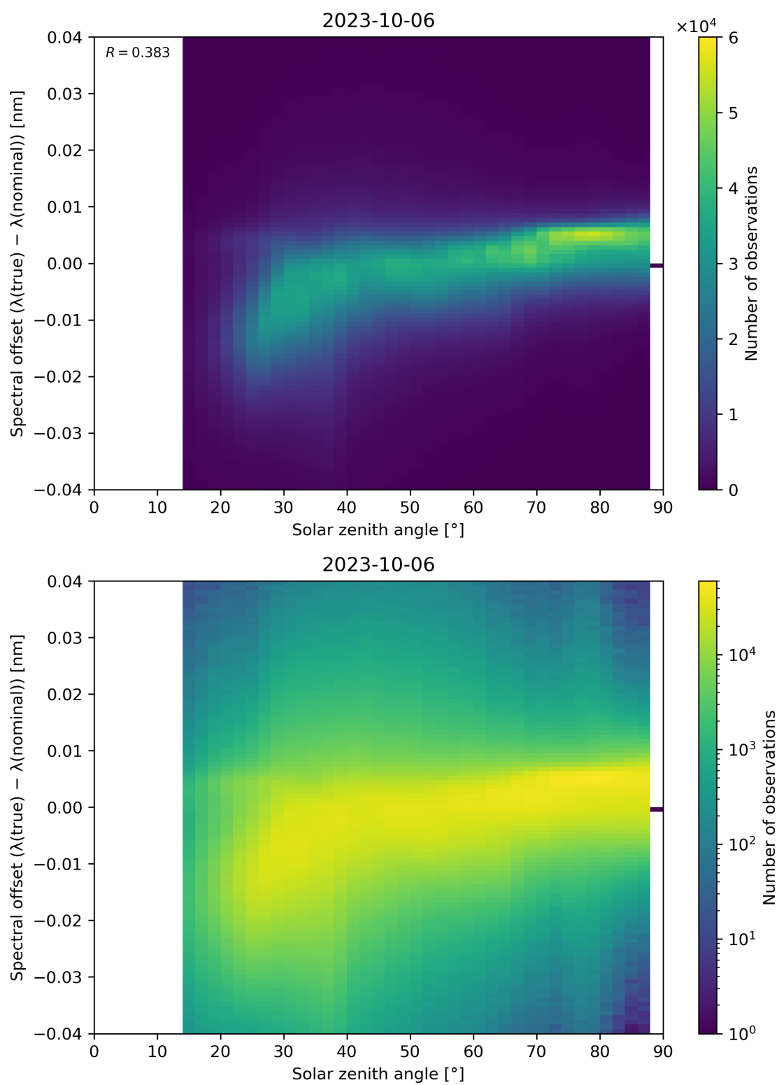
Figure 128: Scatter density plot of “Solar zenith angle” against “Spectral offset ( \lambda(\text{true}) - \lambda(\text{nominal}) )” for 2023-10-06 to 2023-10-07.
