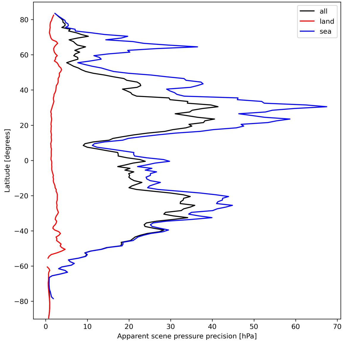
Figure 20: Zonal average of “Apparent scene pressure precision” for 2023-10-06 to 2023-10-07.
