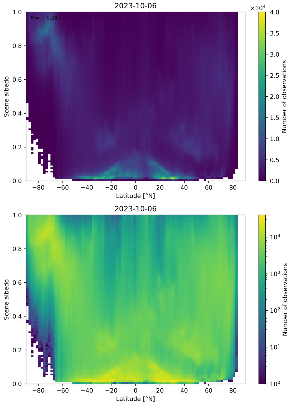
Figure 104: Scatter density plot of “Latitude” against “Scene albedo” for 2023-10-06 to 2023-10-07.
