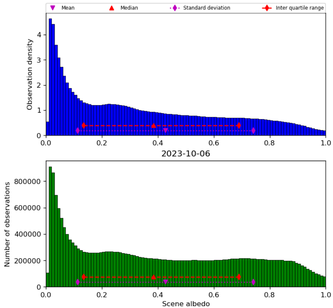
Figure 34: Histogram of “Scene albedo” for 2023-10-06 to 2023-10-07
