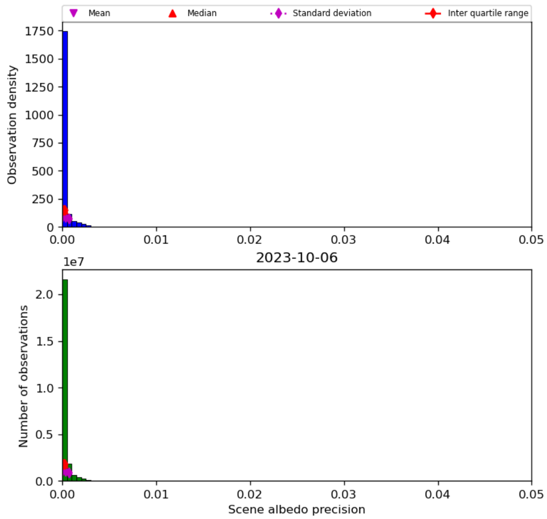
Figure 35: Histogram of “Scene albedo precision” for 2023-10-06 to 2023-10-07
