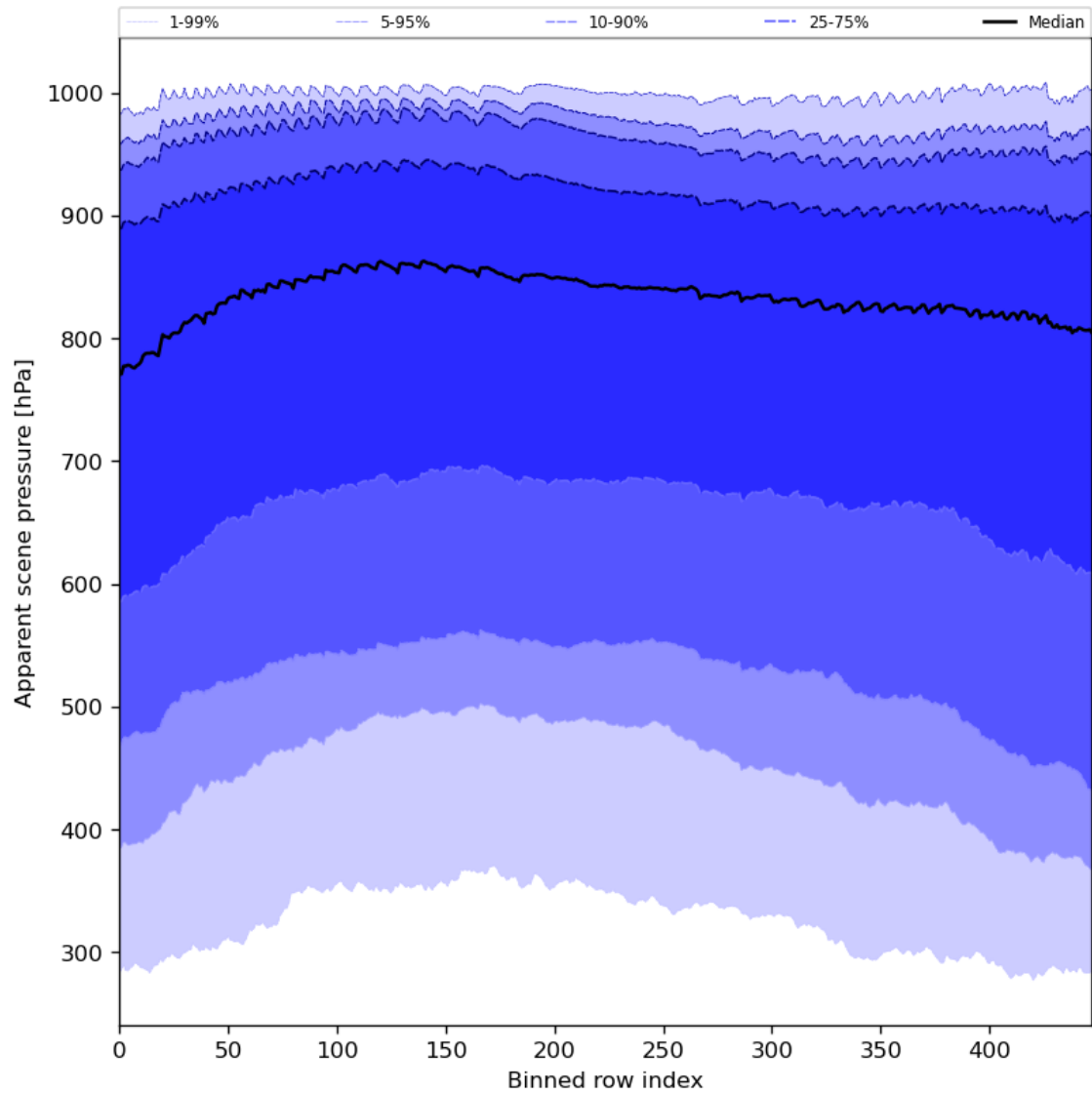
Figure 53: Along track statistics of “Apparent scene pressure” for 2023-10-06 to 2023-10-07
