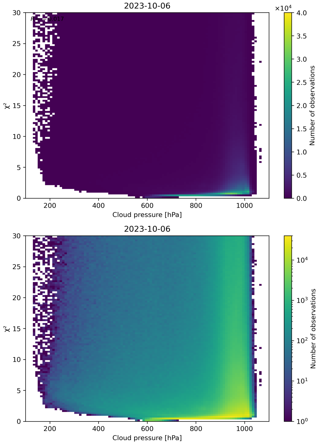
Figure 85: Scatter density plot of “Cloud pressure” against “ \chi^2 ” for 2023-10-06 to 2023-10-07.
