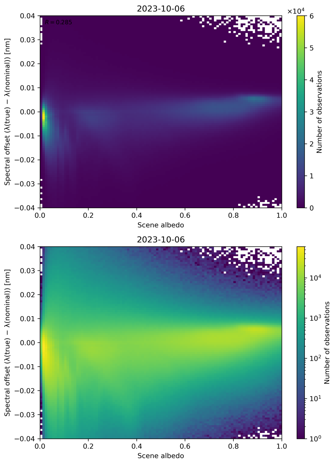
Figure 117: Scatter density plot of “Scene albedo” against “Spectral offset ( \lambda(\text{true}) - \lambda(\text{nominal}) )” for 2023-10-06 to 2023-10-07.
