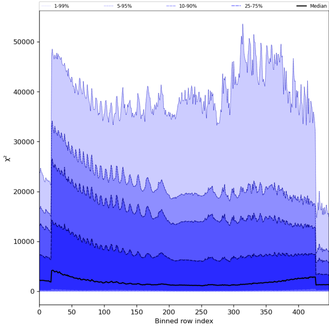
Figure 55: Along track statistics of “ \chi^2 ” for 2023-10-06 to 2023-10-07
