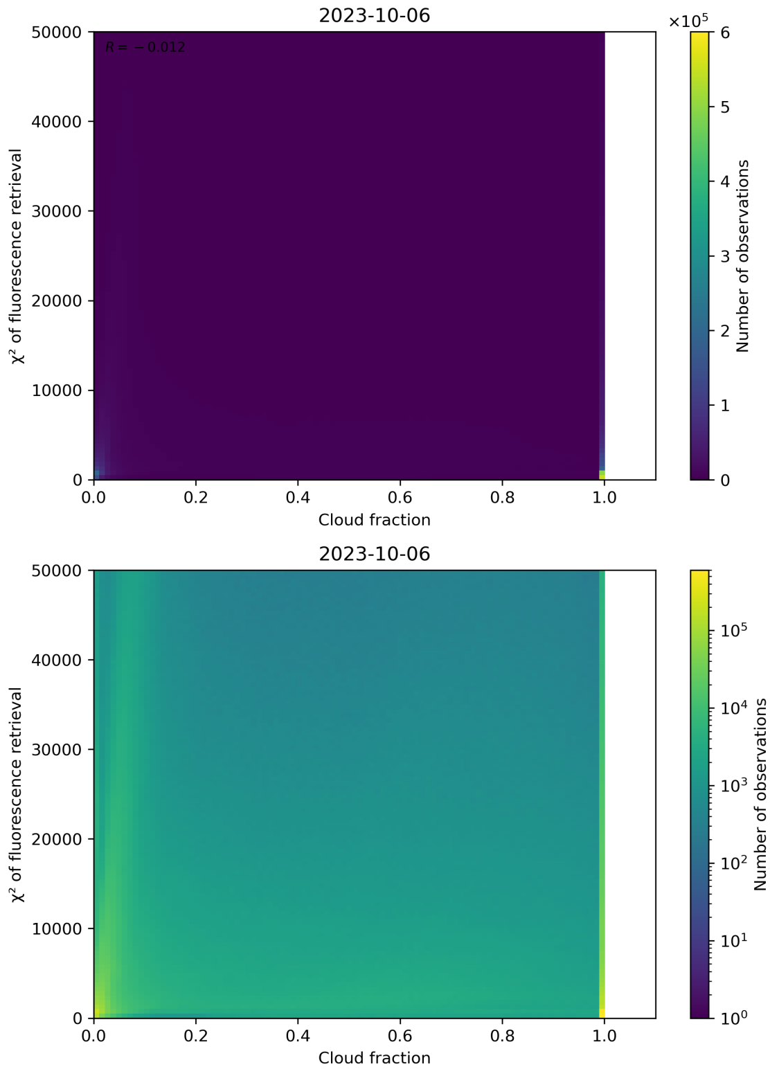
Figure 78: Scatter density plot of “Cloud fraction” against “ \chi^2 of fluorescence retrieval” for 2023-10-06 to 2023-10-07.
