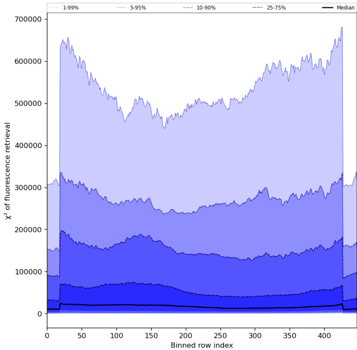
Figure 59: Along track statistics of “ \chi^2 of fluorescence retrieval” for 2023-10-06 to 2023-10-07
