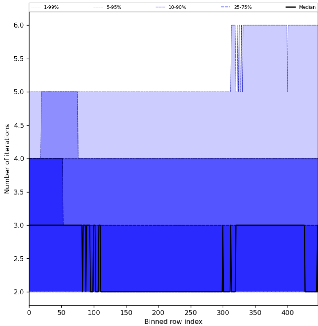
Figure 56: Along track statistics of “Number of iterations” for 2023-10-06 to 2023-10-07
