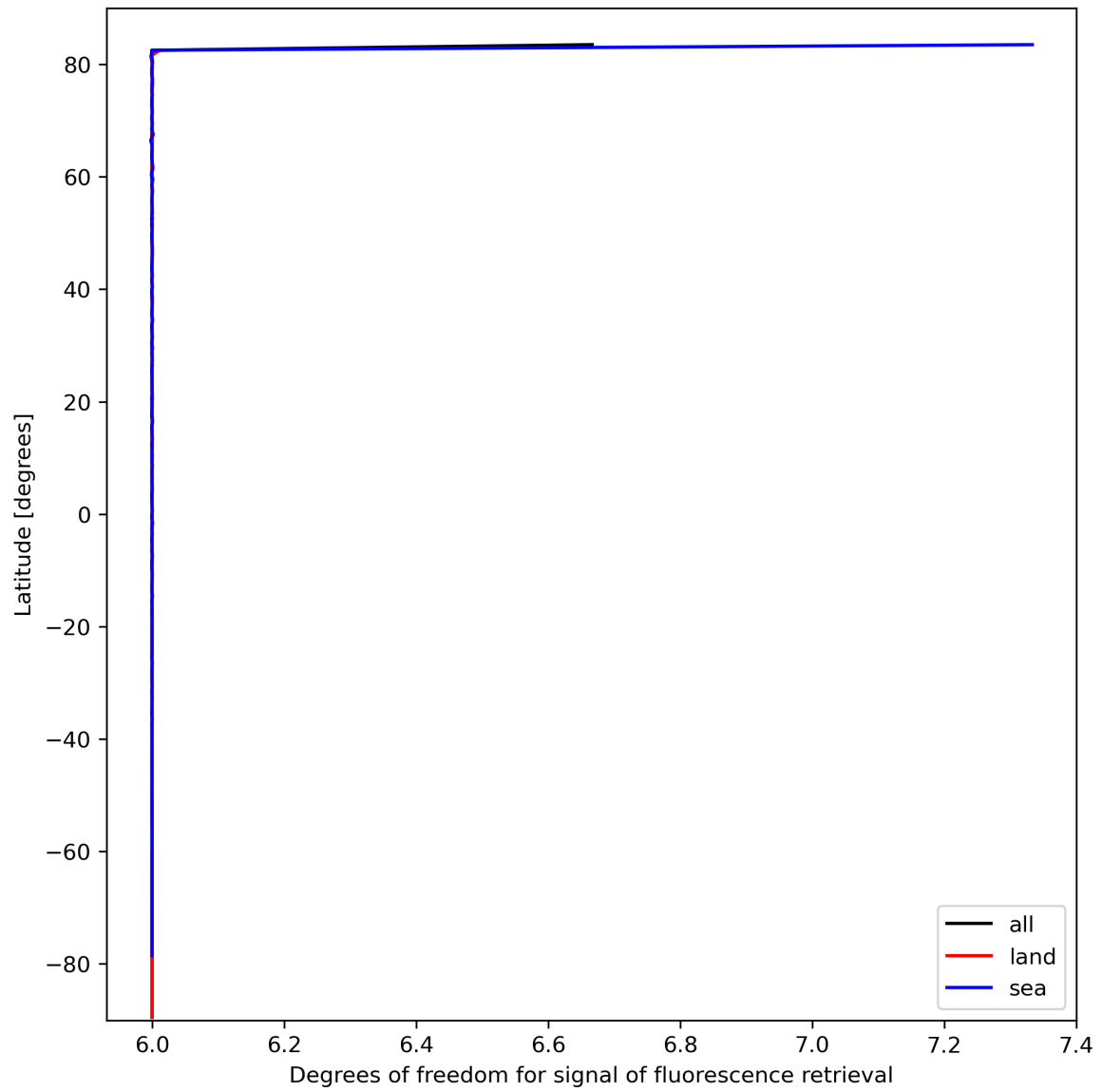
Figure 26: Zonal average of “Degrees of freedom for signal of fluorescence retrieval” for 2023-10-06 to 2023-10-07.
