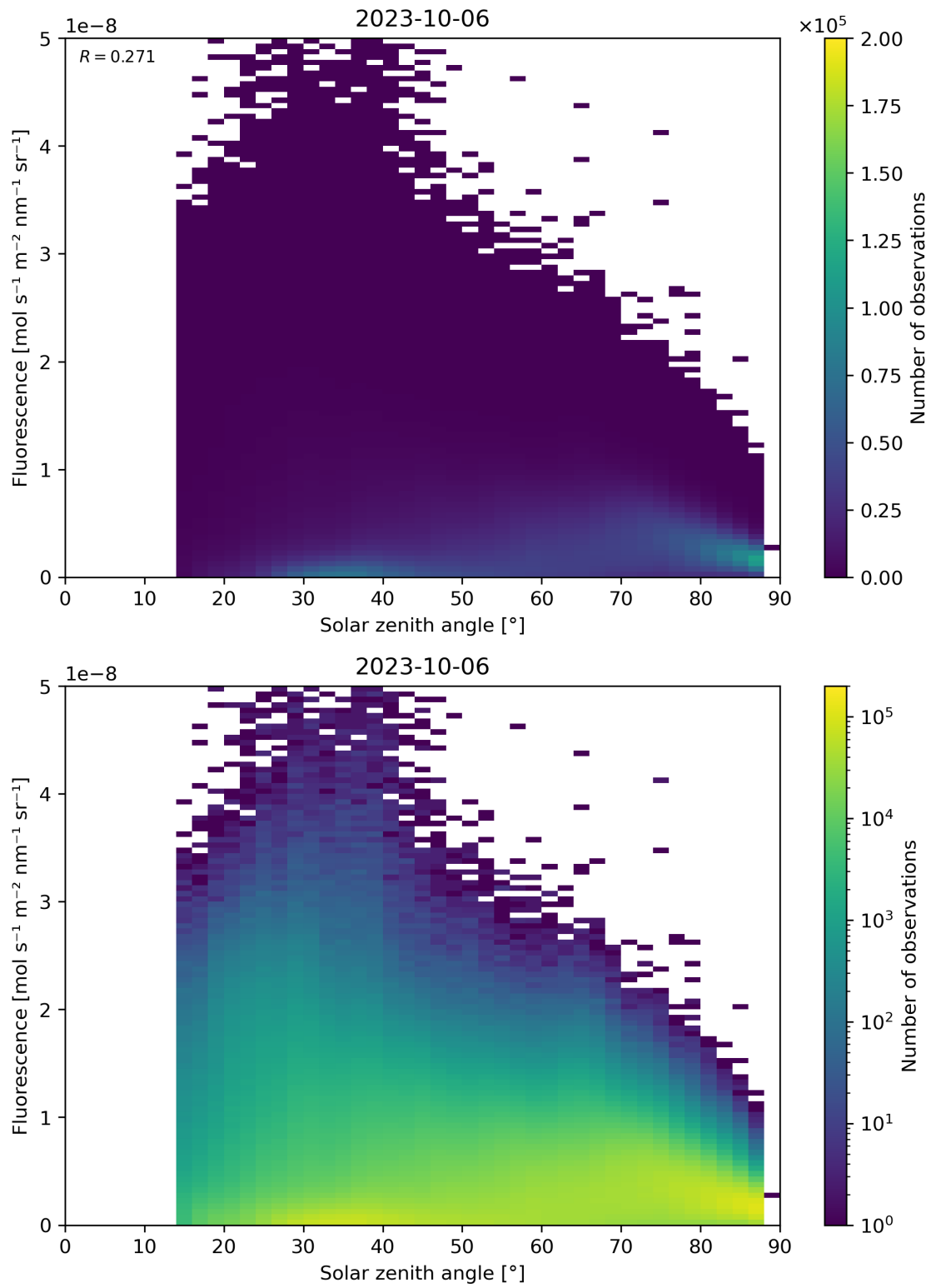
Figure 123: Scatter density plot of “Solar zenith angle” against “Fluorescence” for 2023-10-06 to 2023-10-07.
