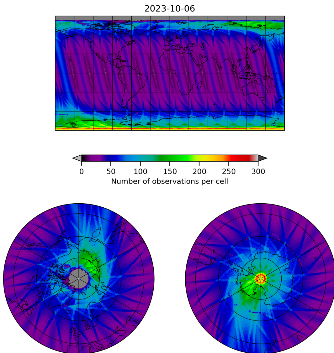
Figure 11: Map of the number of observations for 2023-10-06 to 2023-10-07
