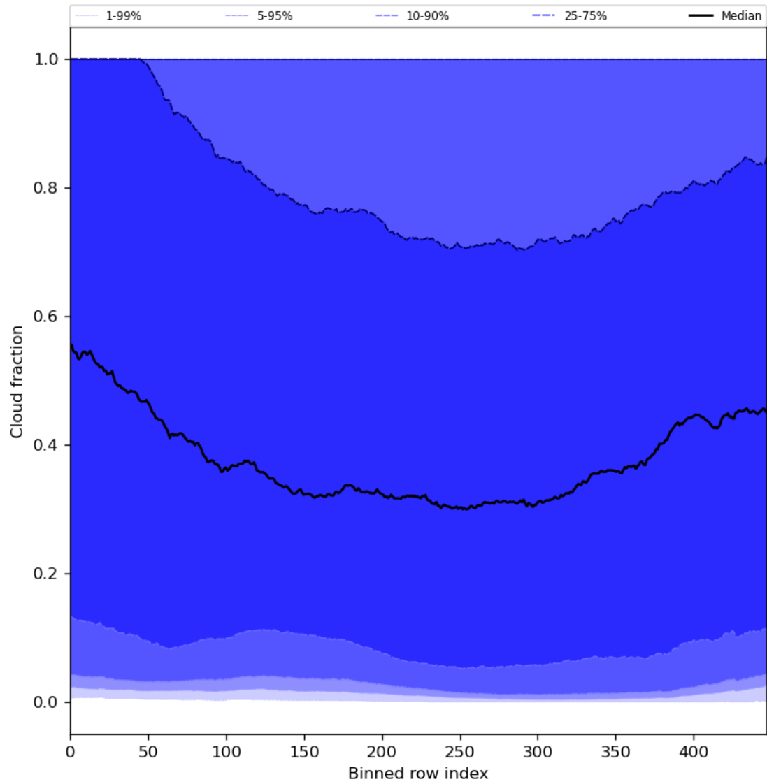
Figure 49: Along track statistics of “Cloud fraction” for 2023-10-06 to 2023-10-07
