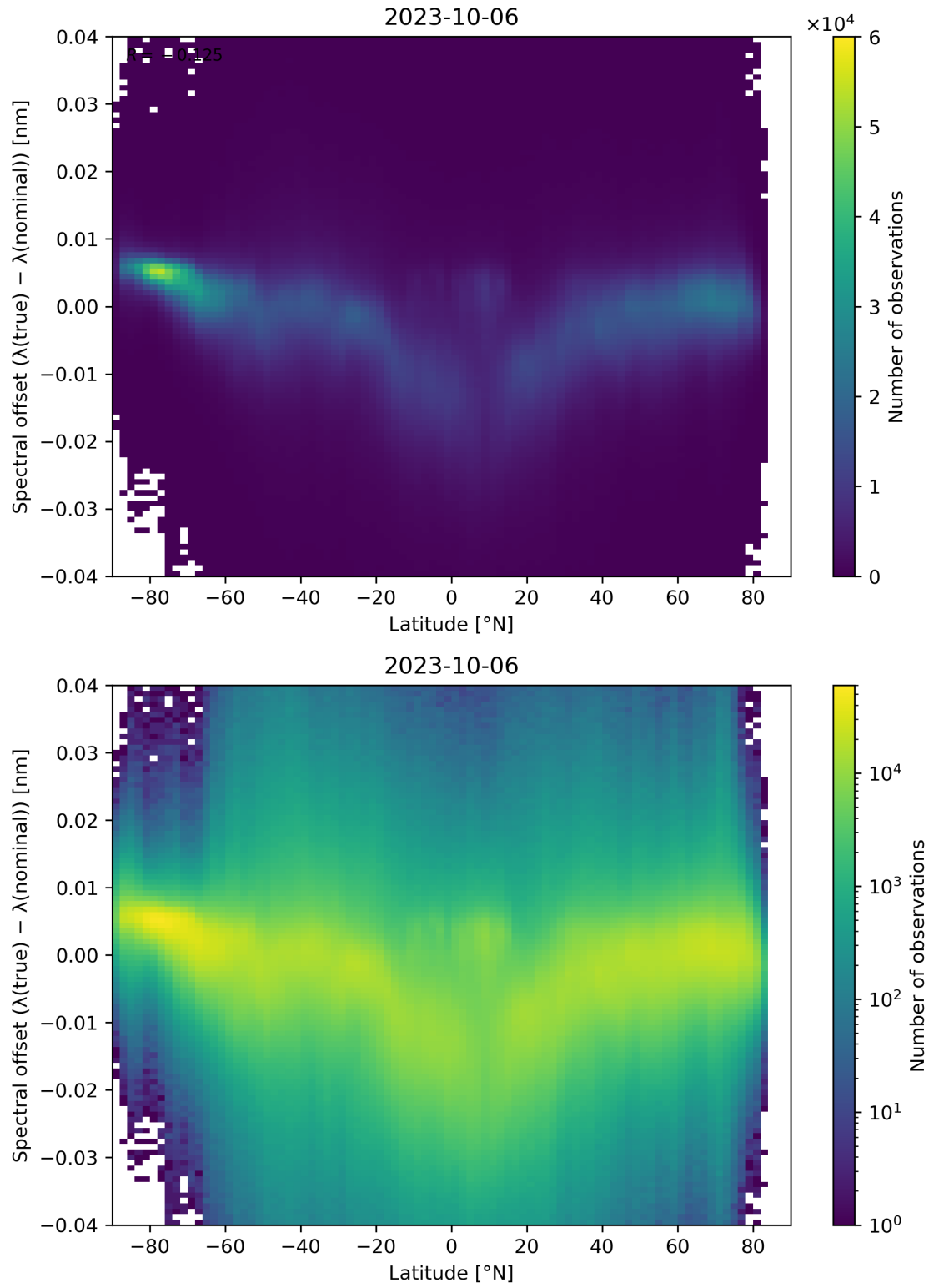
Figure 105: Scatter density plot of “Latitude” against “Spectral offset ( \lambda(\text{true}) - \lambda(\text{nominal}) )” for 2023-10-06 to 2023-10-07.
