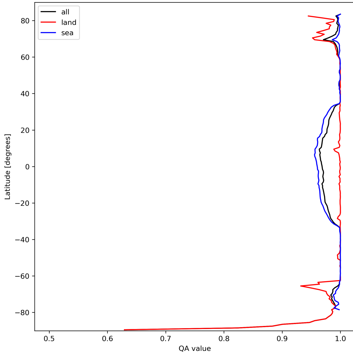
Figure 12: Zonal average of “QA value” for 2023-10-06 to 2023-10-07.
