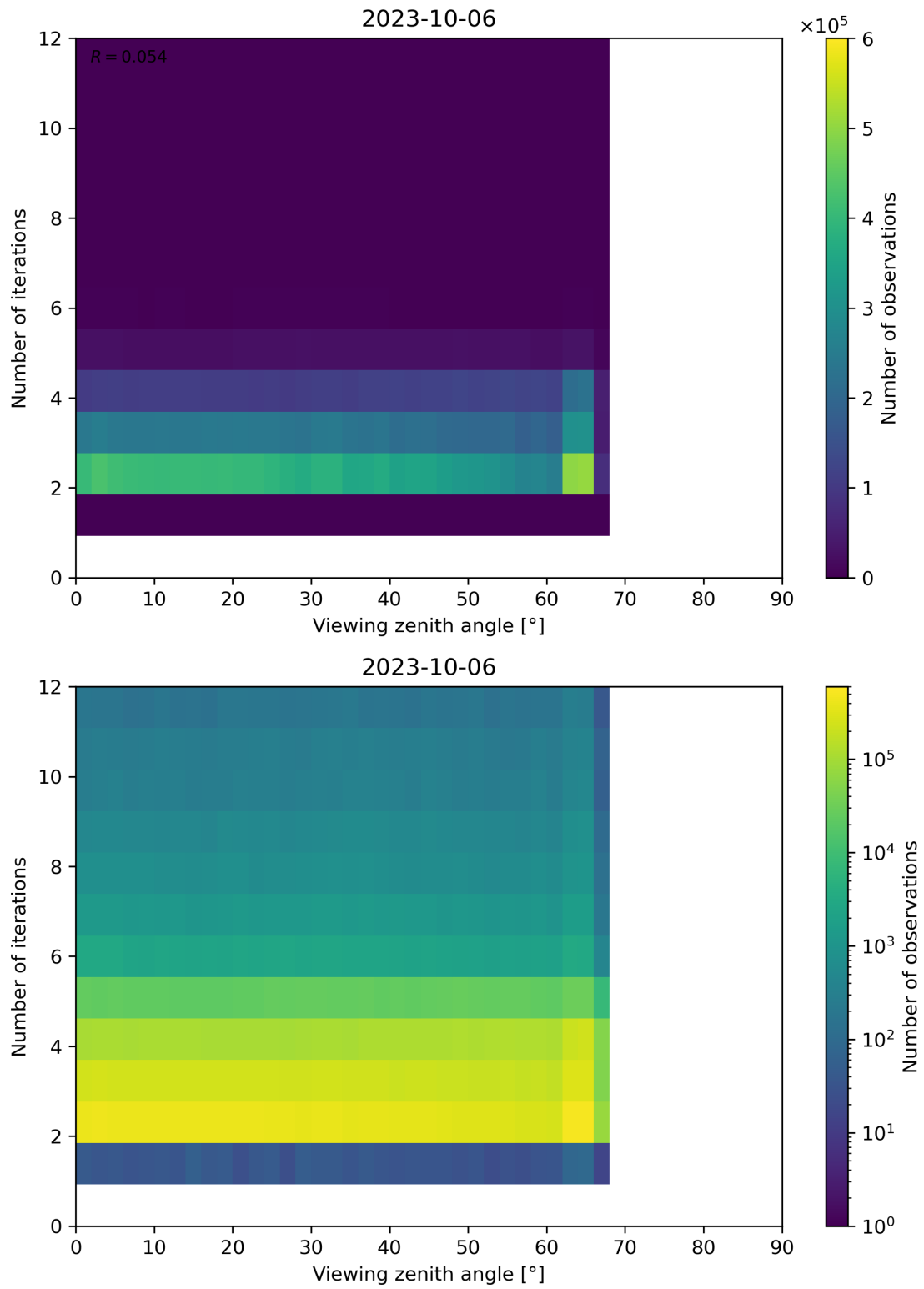
Figure 136: Scatter density plot of “Viewing zenith angle” against “Number of iterations” for 2023-10-06 to 2023-10-07.
