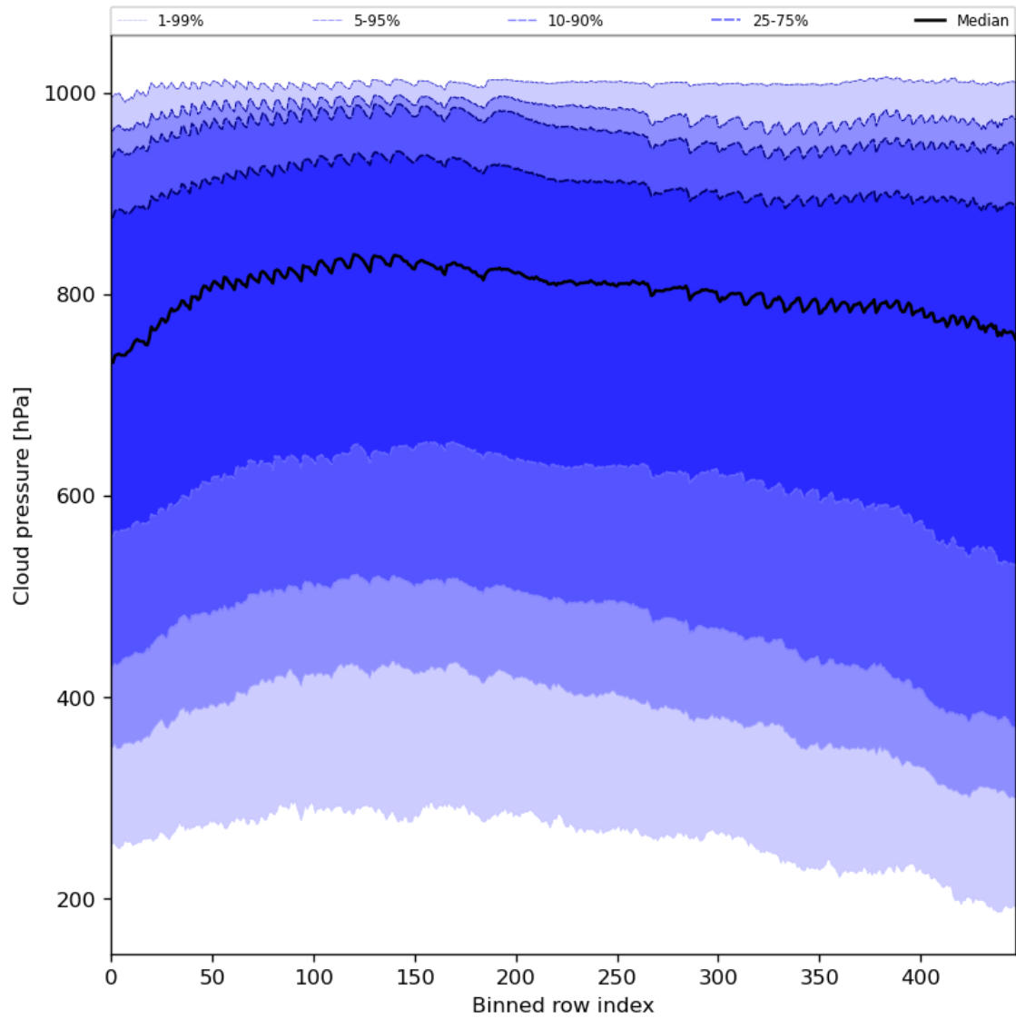
Figure 47: Along track statistics of “Cloud pressure” for 2023-10-06 to 2023-10-07
