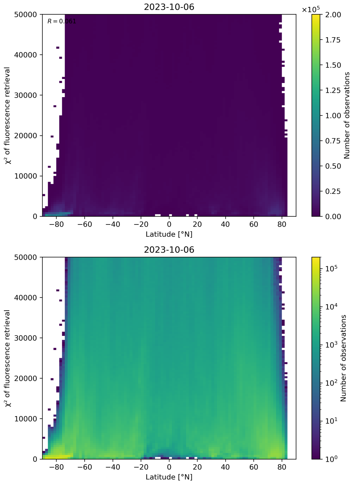
Figure 98: Scatter density plot of “Latitude” against “ \chi^2 of fluorescence retrieval” for 2023-10-06 to 2023-10-07.
