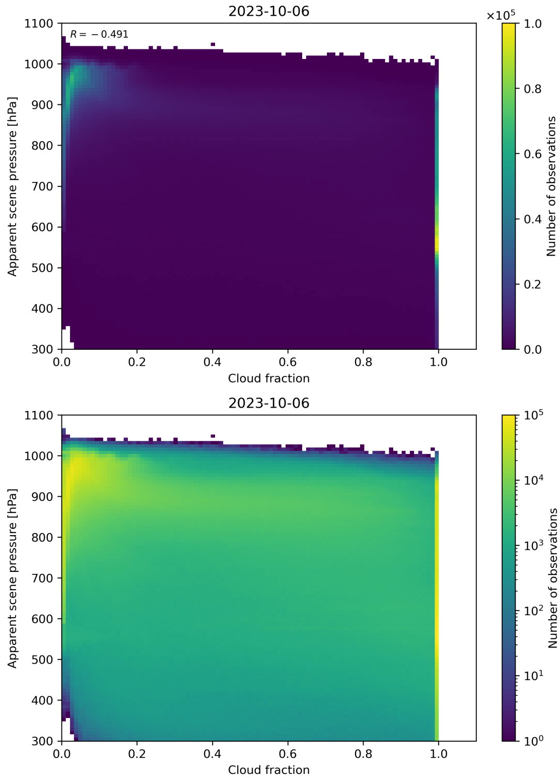
Figure 76: Scatter density plot of “Cloud fraction” against “Apparent scene pressure” for 2023-10-06 to 2023-10-07.
