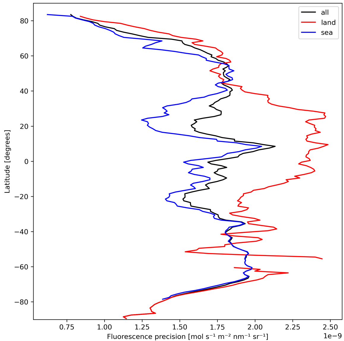
Figure 24: Zonal average of “Fluorescence precision” for 2023-10-06 to 2023-10-07.
