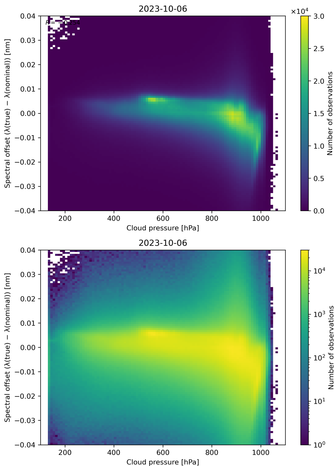
Figure 92: Scatter density plot of “Cloud pressure” against “Spectral offset ( \lambda(\text{true}) - \lambda(\text{nominal}) )” for 2023-10-06 to 2023-10-07.
