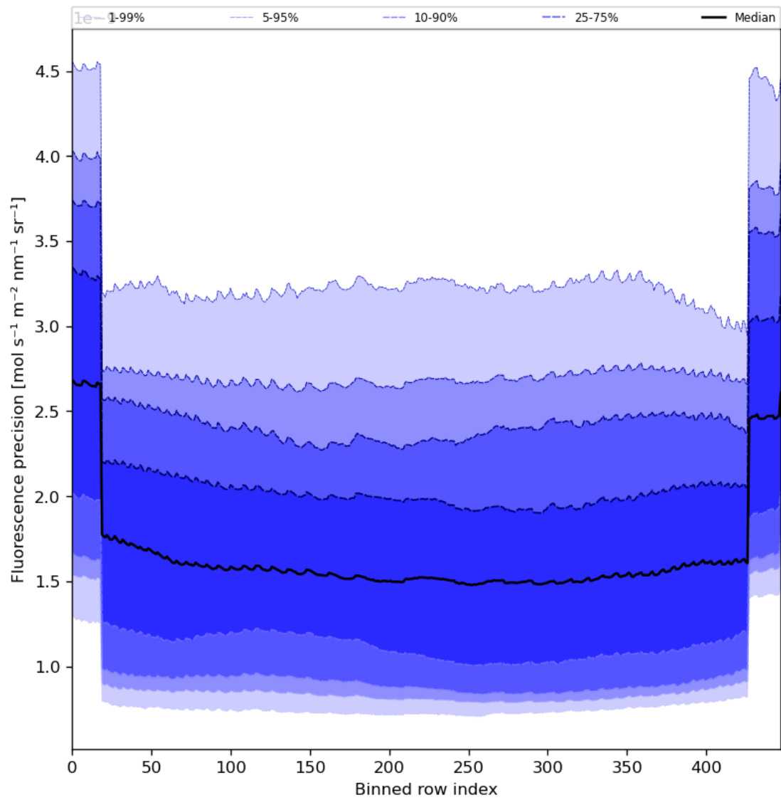
Figure 58: Along track statistics of “Fluorescence precision” for 2023-10-06 to 2023-10-07
