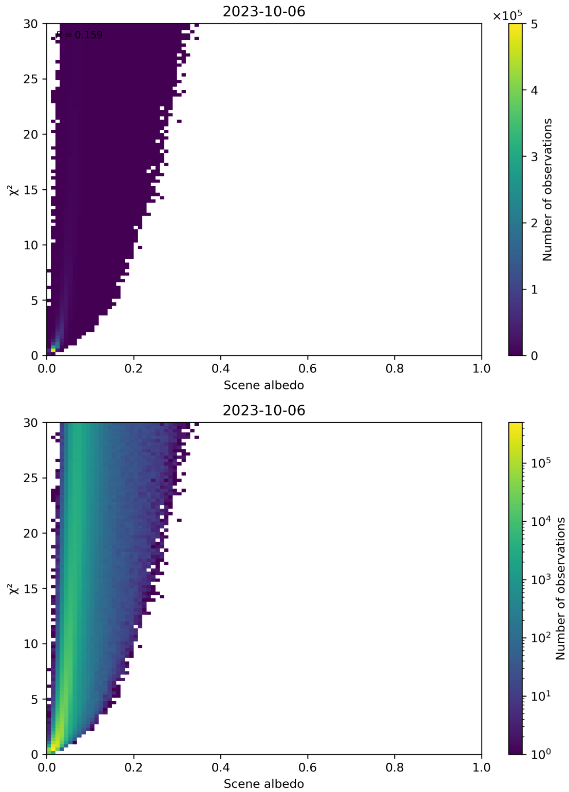
Figure 112: Scatter density plot of “Scene albedo” against “ \chi^2 ” for 2023-10-06 to 2023-10-07.
