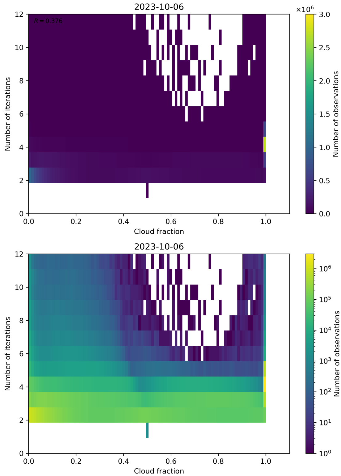
Figure 80: Scatter density plot of “Cloud fraction” against “Number of iterations” for 2023-10-06 to 2023-10-07.
