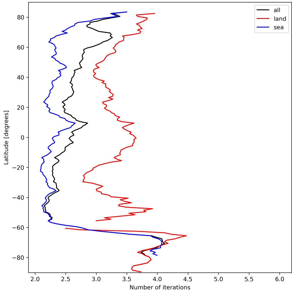
Figure 22: Zonal average of “Number of iterations” for 2023-10-06 to 2023-10-07.
