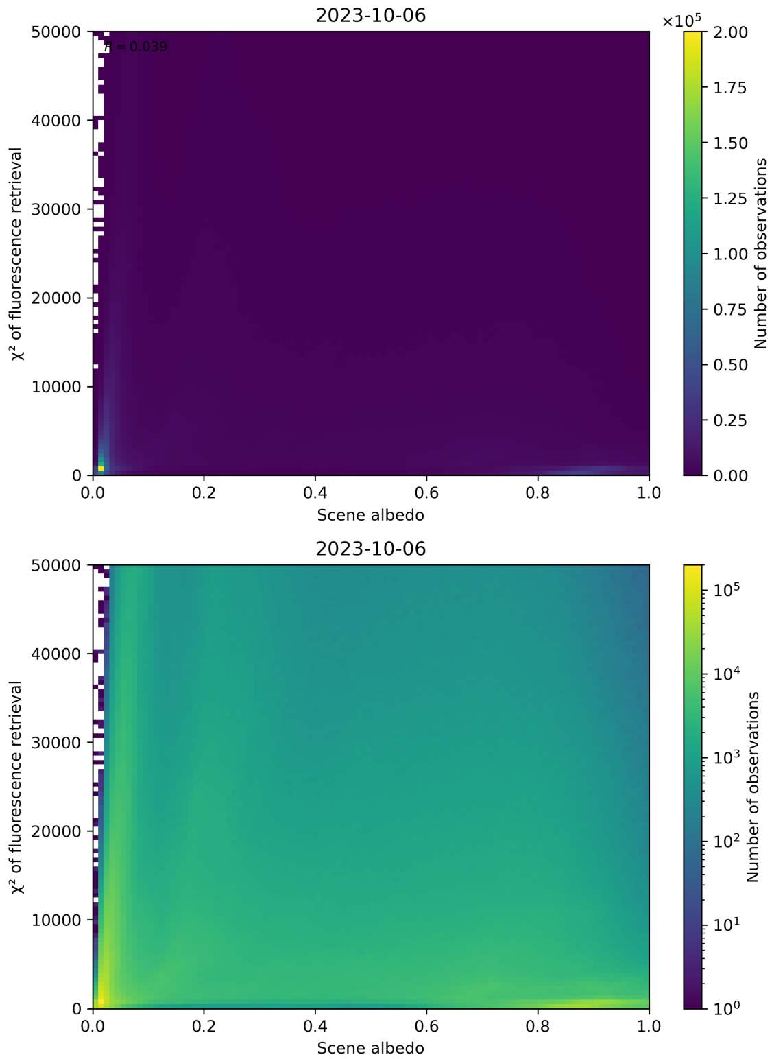
Figure 113: Scatter density plot of “Scene albedo” against “ \chi^2 of fluorescence retrieval” for 2023-10-06 to 2023-10-07.
