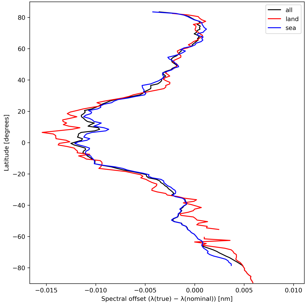
Figure 28: Zonal average of “Spectral offset ( \lambda(\text{true}) - \lambda(\text{nominal}) )” for 2023-10-06 to 2023-10-07.
