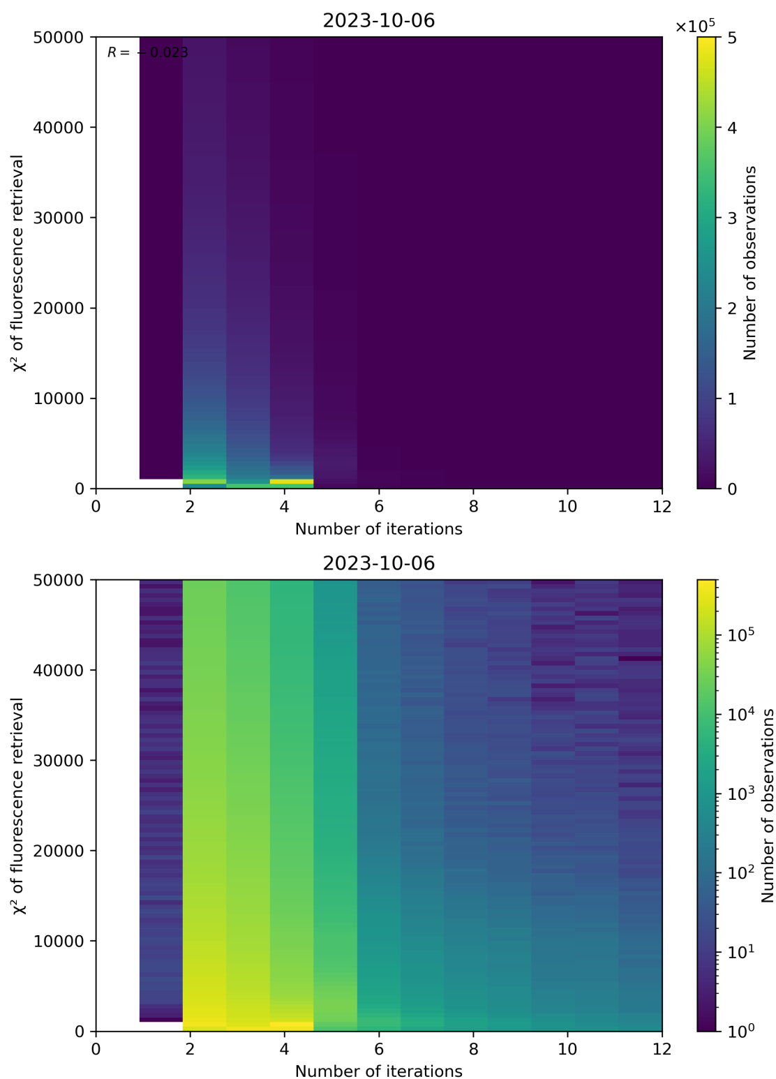
Figure 106: Scatter density plot of “Number of iterations” against “ \chi^2 of fluorescence retrieval” for 2023-10-06 to 2023-10-07.
