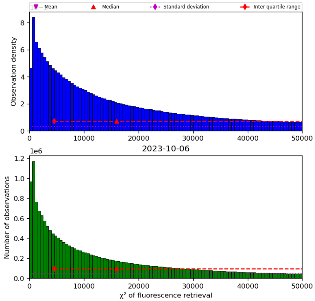
Figure 42: Histogram of “ \chi^2 of fluorescence retrieval” for 2023-10-06 to 2023-10-07
