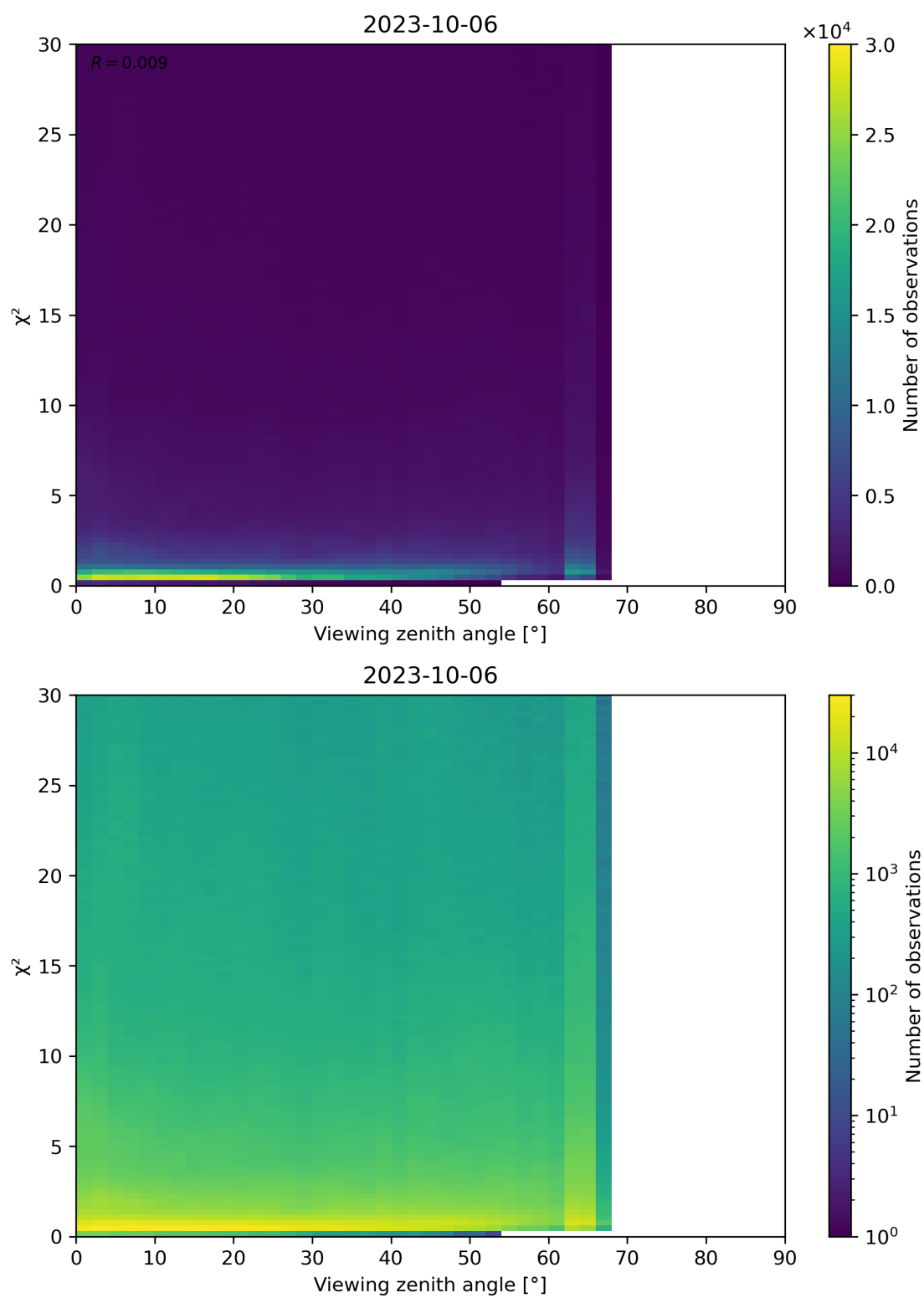
Figure 130: Scatter density plot of “Viewing zenith angle” against “ \chi^2 ” for 2023-10-06 to 2023-10-07.
