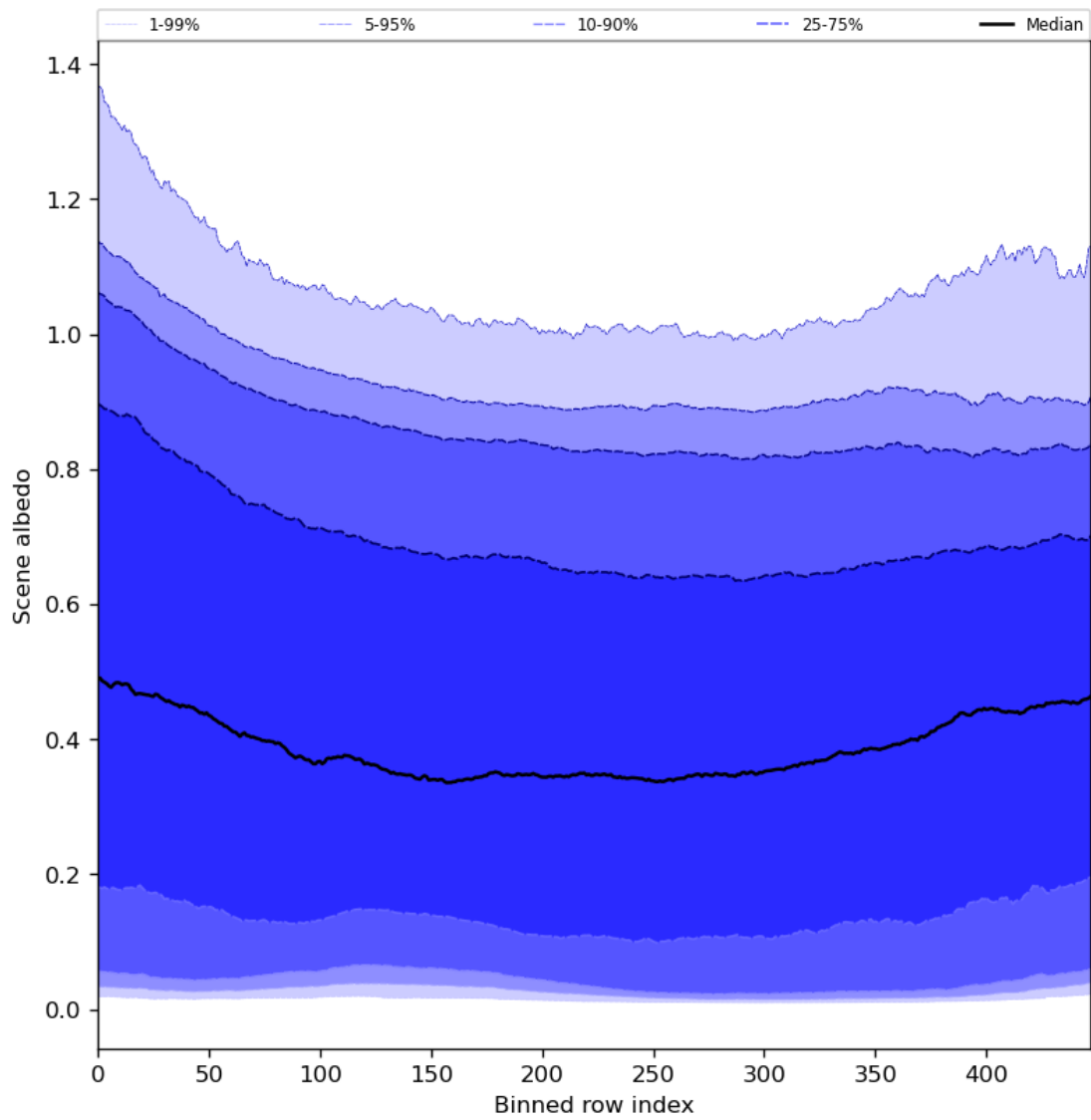
Figure 51: Along track statistics of “Scene albedo” for 2023-10-06 to 2023-10-07
