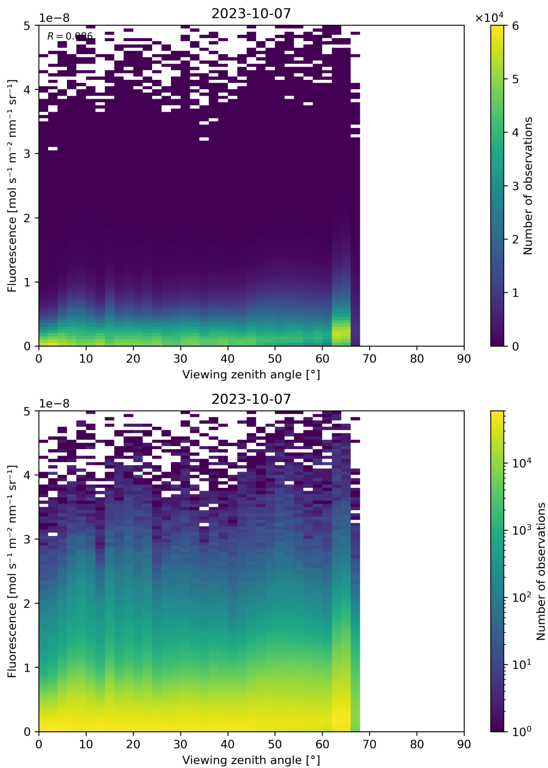
Figure 134: Scatter density plot of “Viewing zenith angle” against “Fluorescence” for 2023-10-06 to 2023-10-08.
