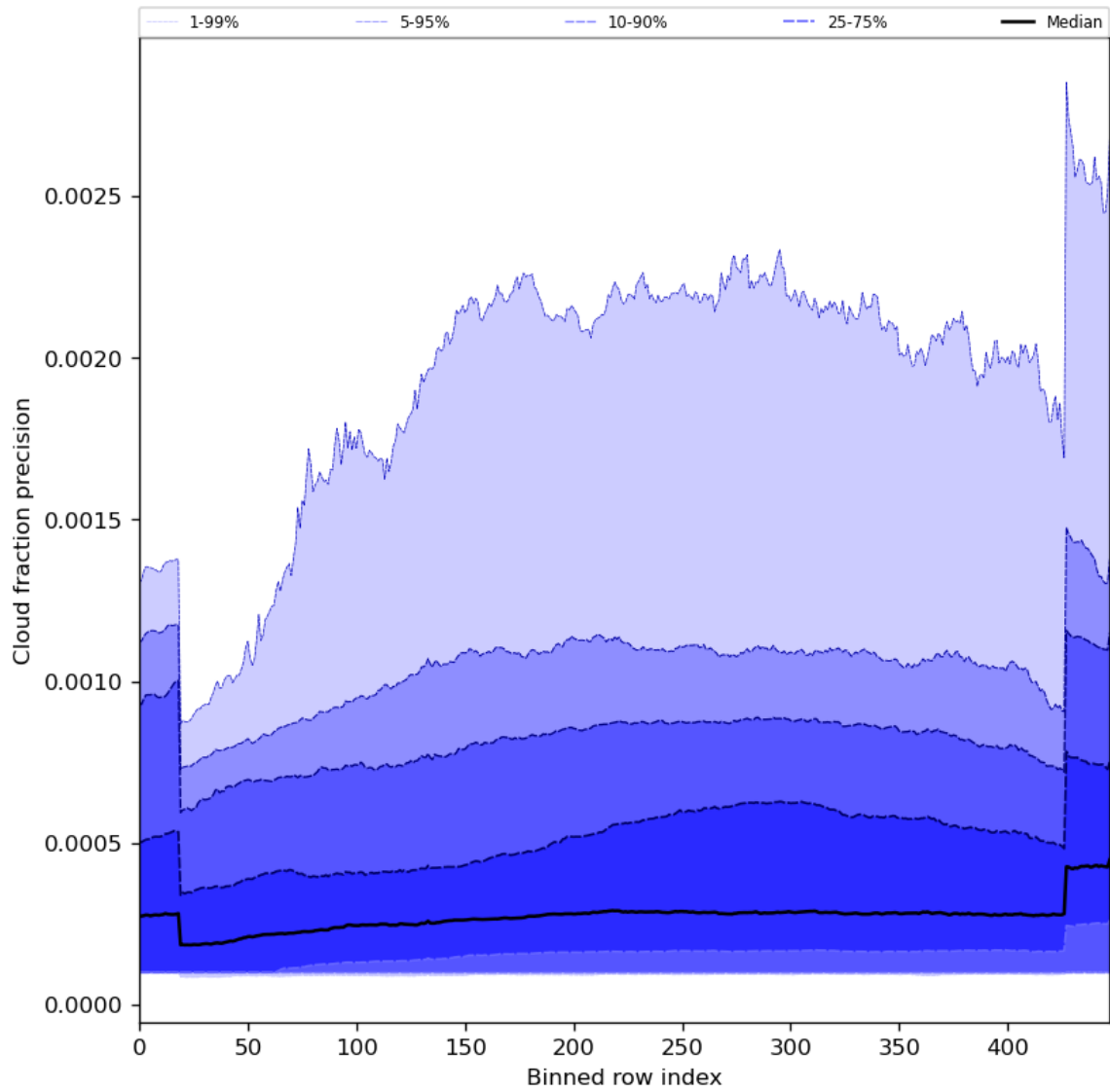
Figure 50: Along track statistics of “Cloud fraction precision” for 2023-10-06 to 2023-10-08
