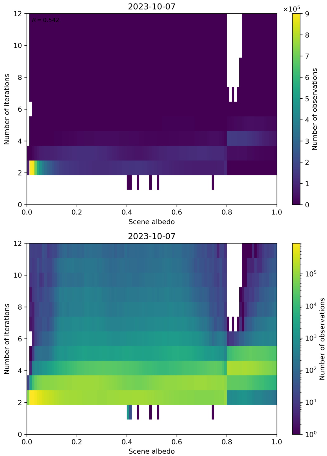
Figure 115: Scatter density plot of “Scene albedo” against “Number of iterations” for 2023-10-06 to 2023-10-08.
