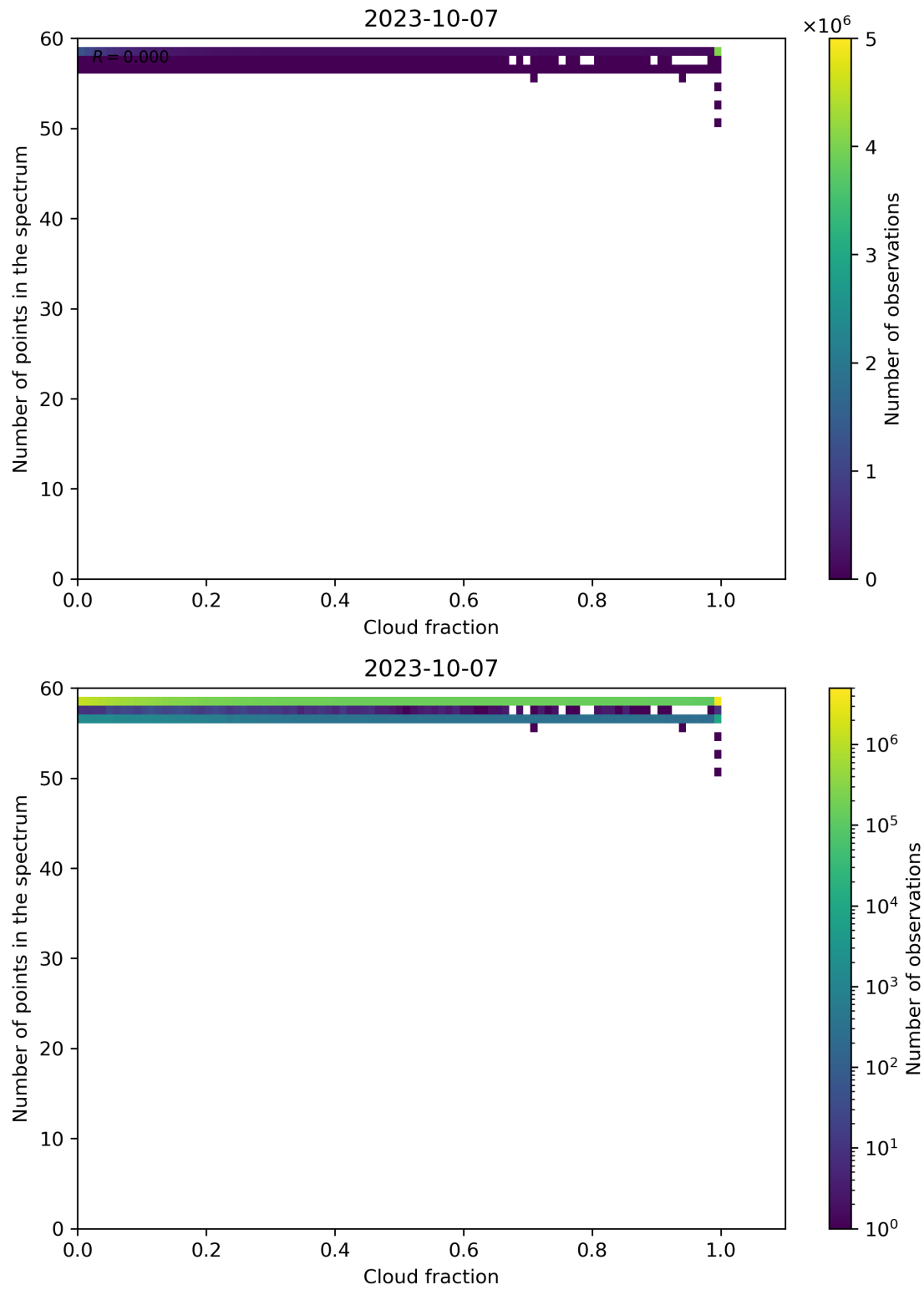
Figure 81: Scatter density plot of “Cloud fraction” against “Number of points in the spectrum” for 2023-10-06 to 2023-10-08.
