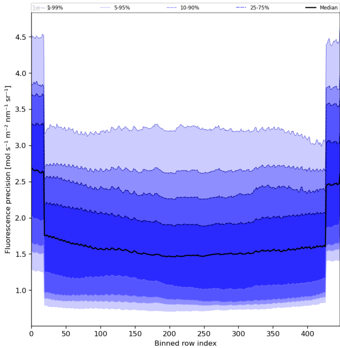
Figure 58: Along track statistics of “Fluorescence precision” for 2023-10-06 to 2023-10-08
