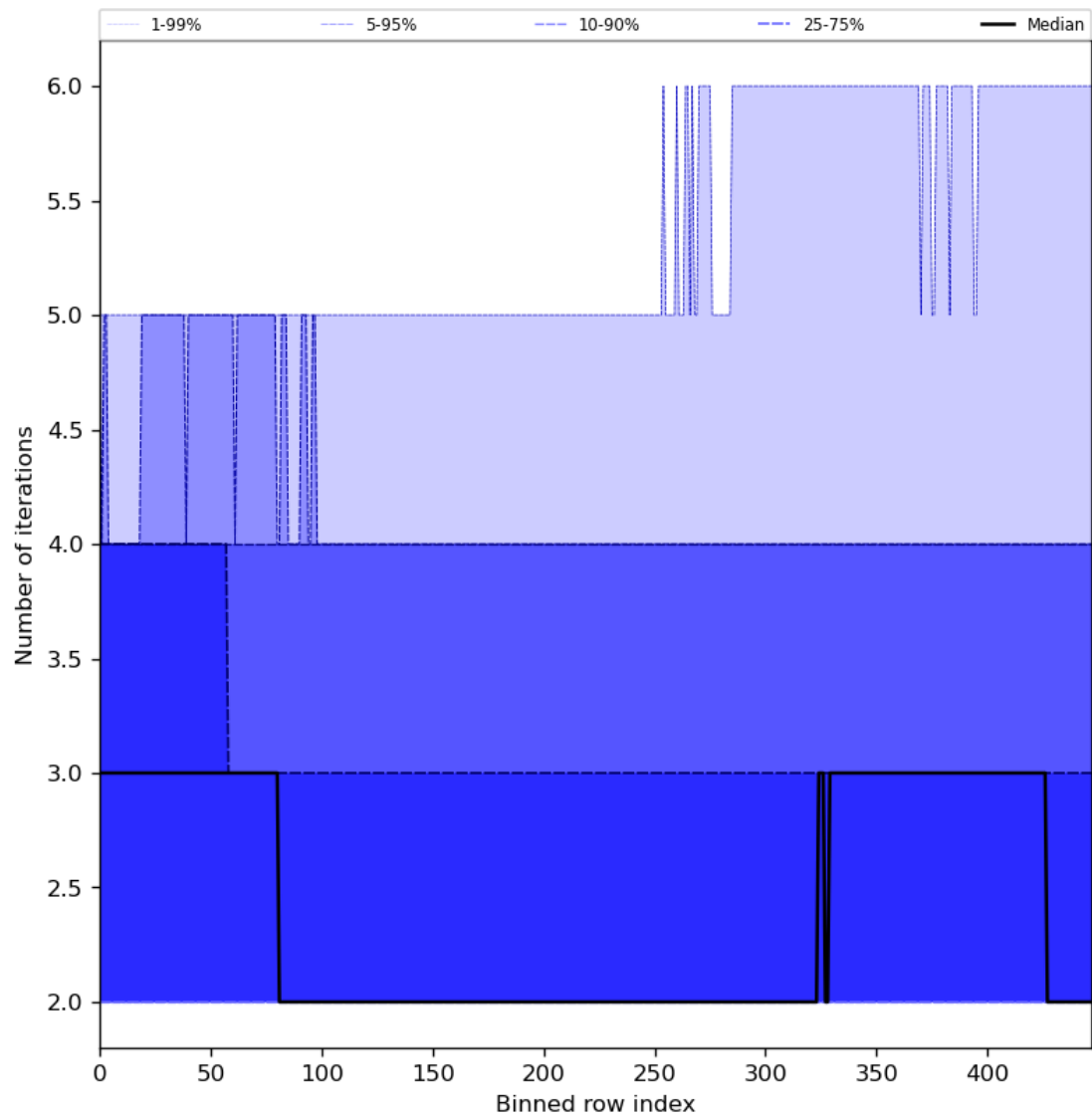
Figure 56: Along track statistics of “Number of iterations” for 2023-10-06 to 2023-10-08
