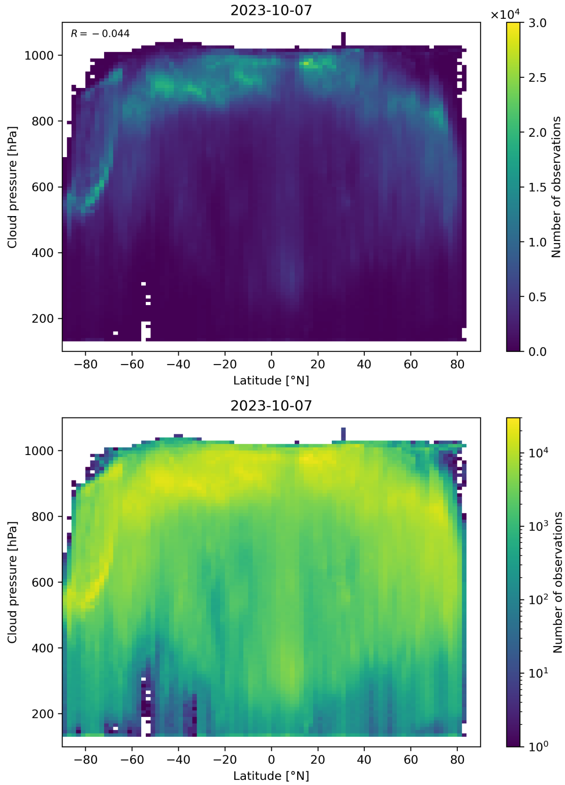
Figure 100: Scatter density plot of “Latitude” against “Cloud pressure” for 2023-10-06 to 2023-10-08.
