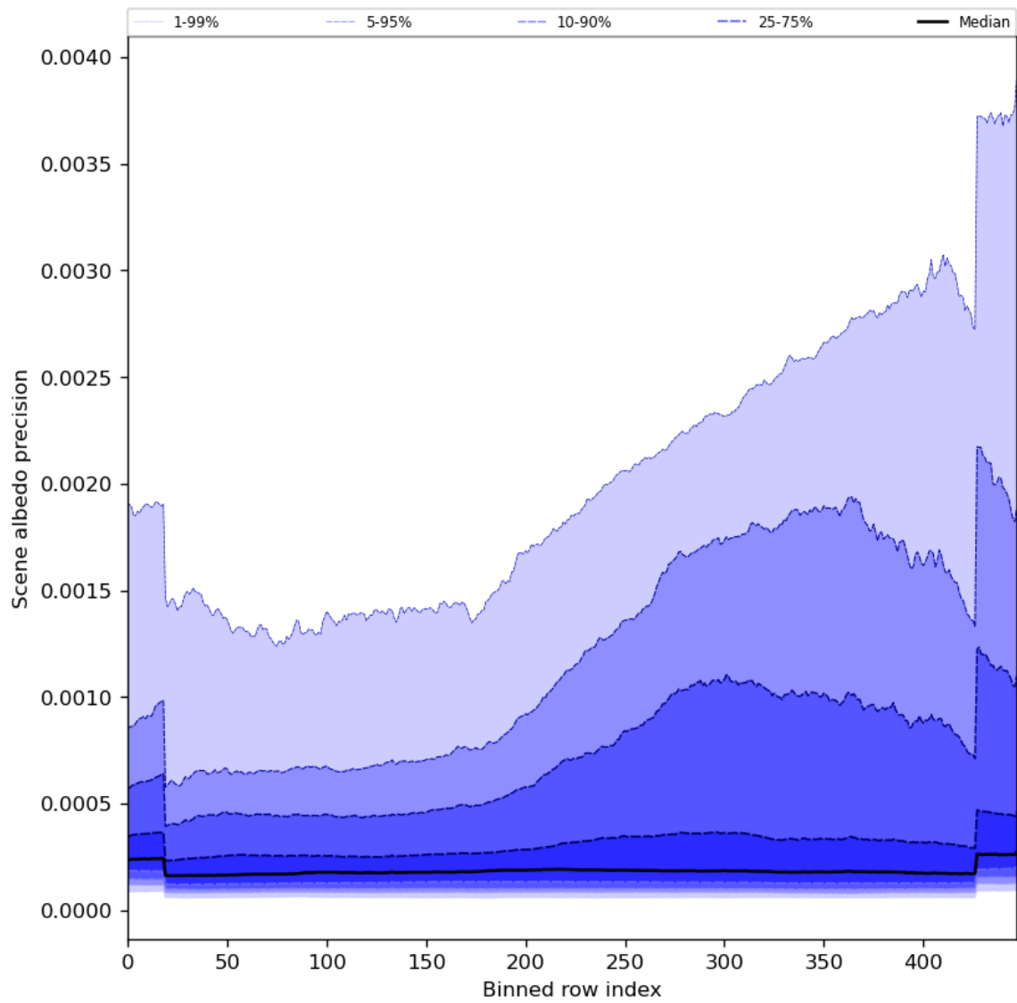
Figure 52: Along track statistics of “Scene albedo precision” for 2023-10-06 to 2023-10-08
