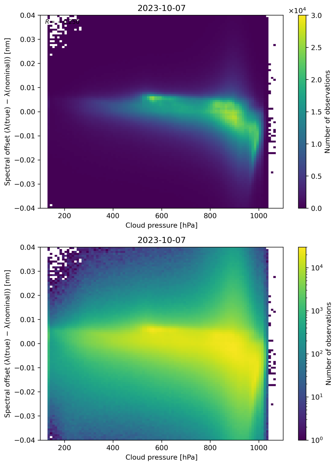
Figure 92: Scatter density plot of “Cloud pressure” against “Spectral offset ( \lambda(\text{true}) - \lambda(\text{nominal}) )” for 2023-10-06 to 2023-10-08.
