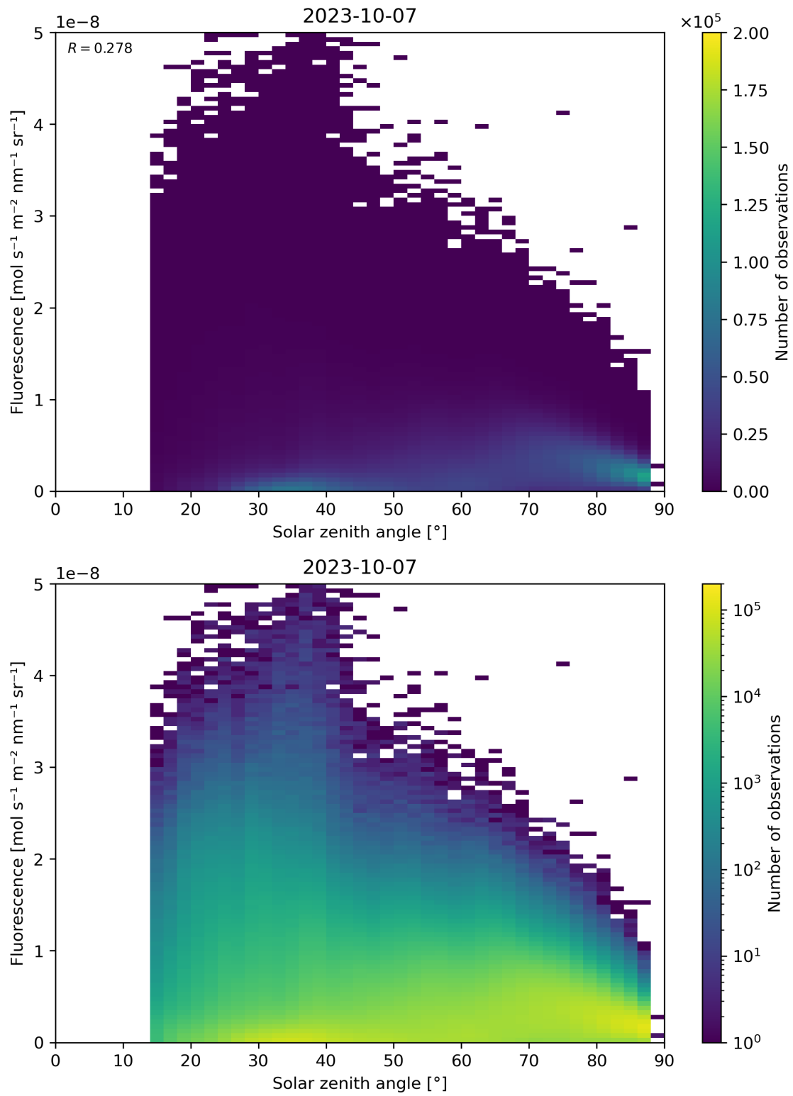
Figure 123: Scatter density plot of “Solar zenith angle” against “Fluorescence” for 2023-10-06 to 2023-10-08.
