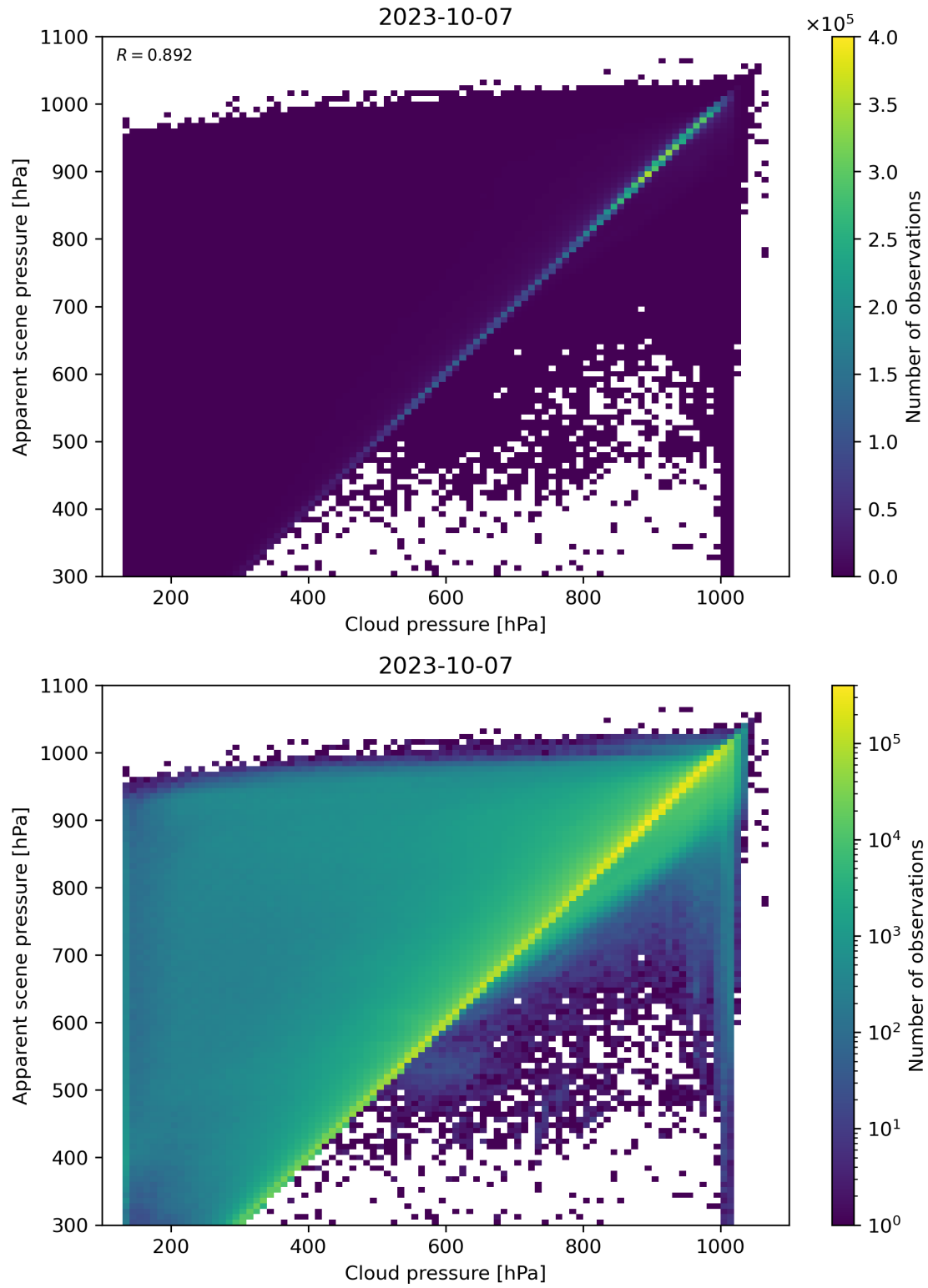
Figure 84: Scatter density plot of “Cloud pressure” against “Apparent scene pressure” for 2023-10-06 to 2023-10-08.
