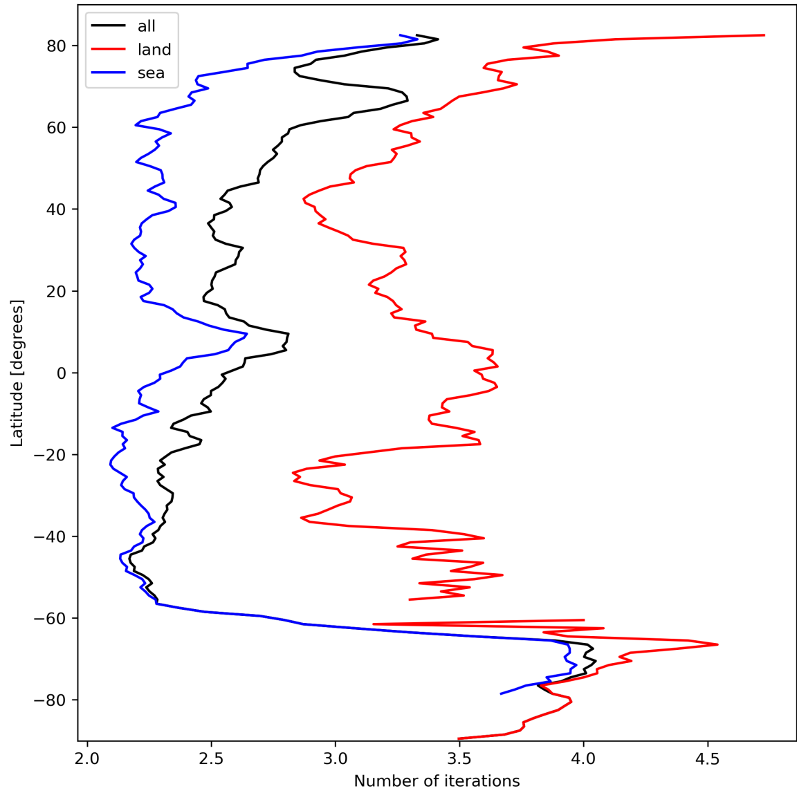
Figure 22: Zonal average of “Number of iterations” for 2023-10-06 to 2023-10-08.
