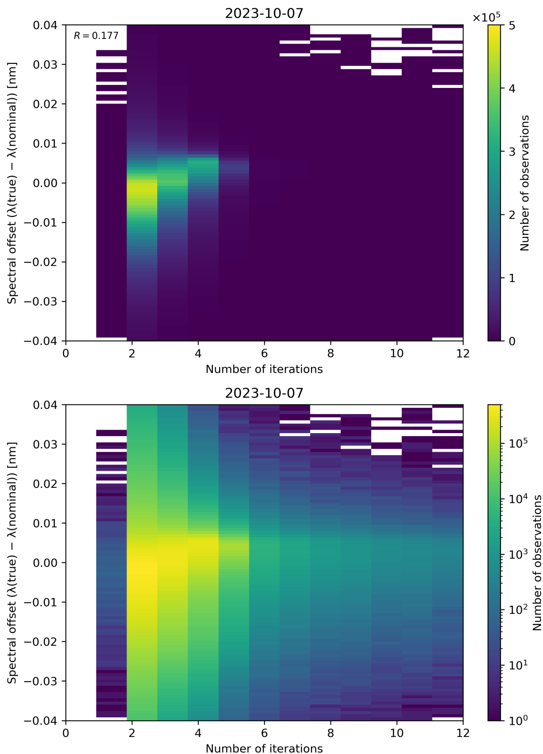
Figure 109: Scatter density plot of “Number of iterations” against “Spectral offset ( \lambda(\text{true}) - \lambda(\text{nominal}) )” for 2023-10-06 to 2023-10-08.
