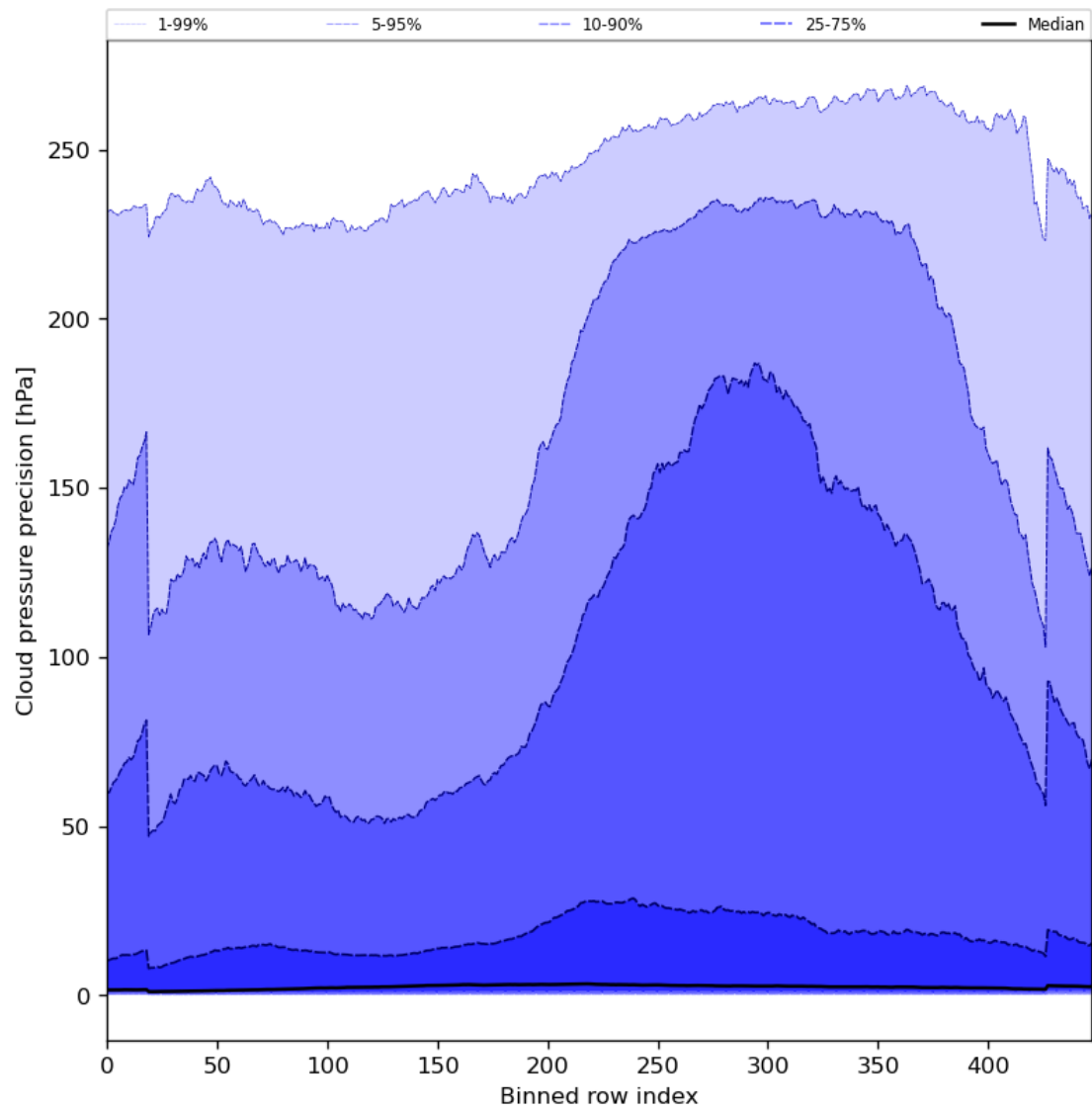
Figure 48: Along track statistics of “Cloud pressure precision” for 2023-10-06 to 2023-10-08
