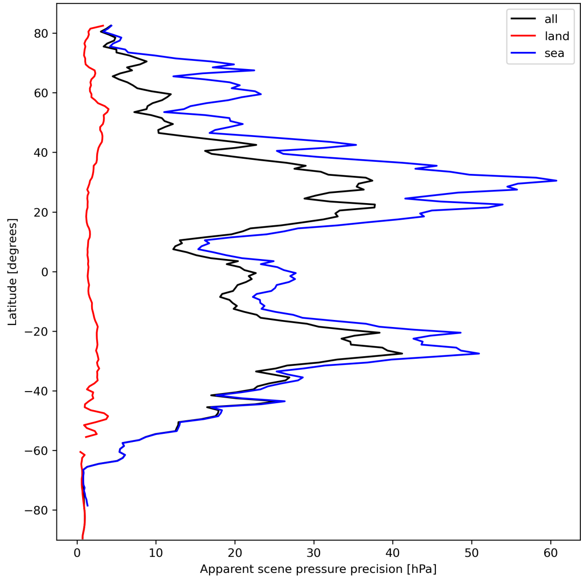
Figure 20: Zonal average of “Apparent scene pressure precision” for 2023-10-06 to 2023-10-08.
