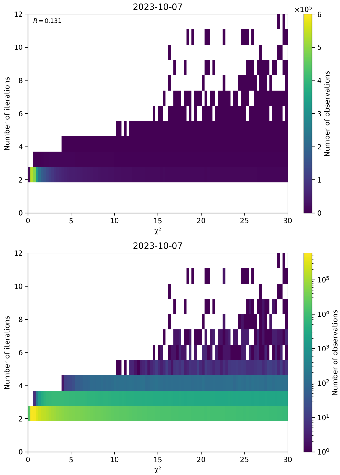
Figure 73: Scatter density plot of “ \chi^2 ” against “Number of iterations” for 2023-10-06 to 2023-10-08.
