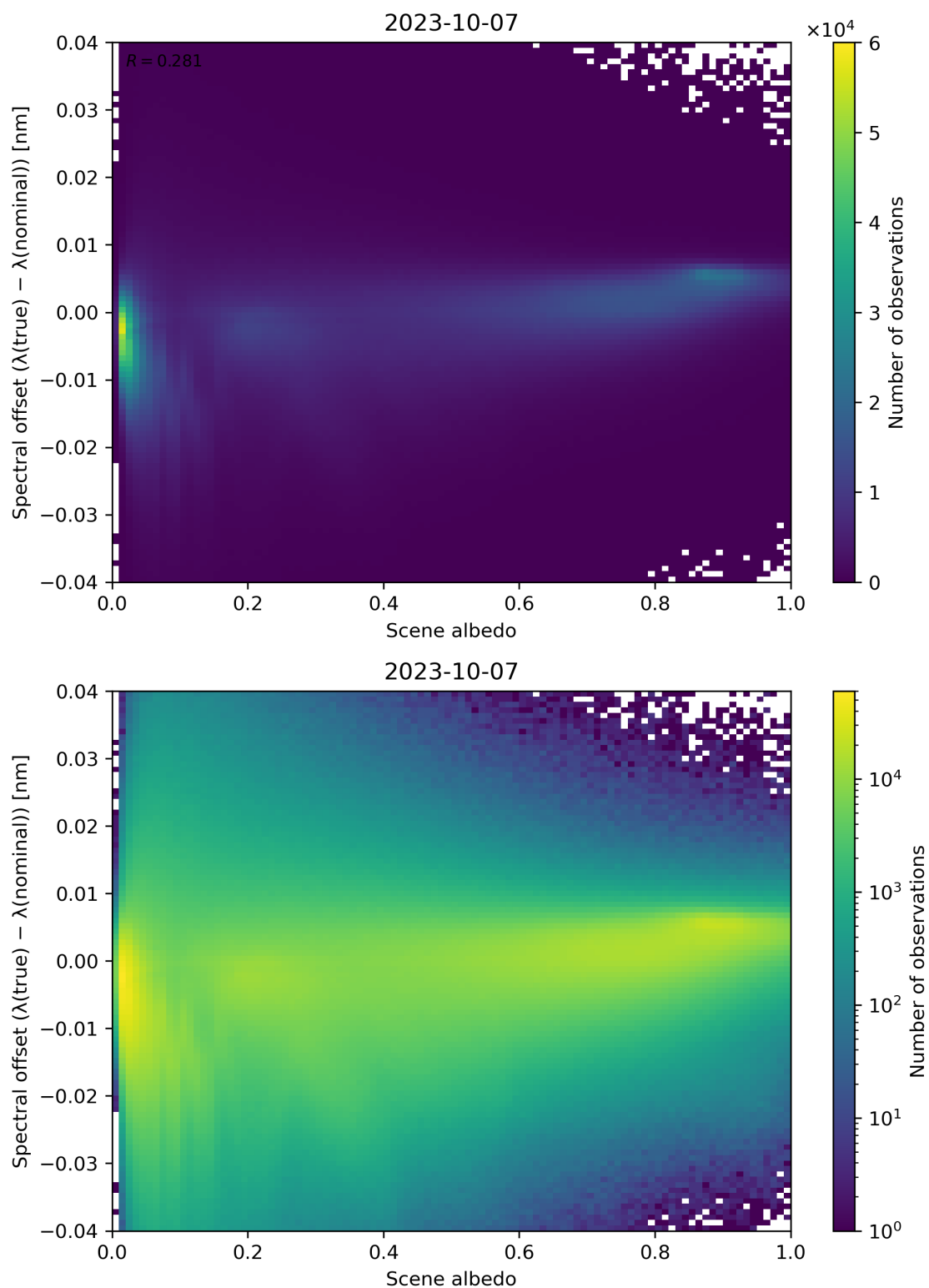
Figure 117: Scatter density plot of “Scene albedo” against “Spectral offset ( \lambda(\text{true}) - \lambda(\text{nominal}) )” for 2023-10-06 to 2023-10-08.
