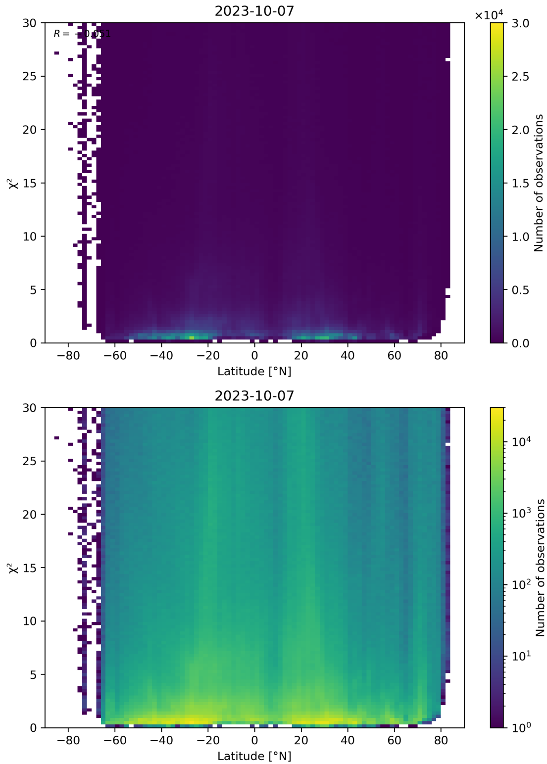
Figure 97: Scatter density plot of “Latitude” against “ \chi^2 ” for 2023-10-06 to 2023-10-08.
