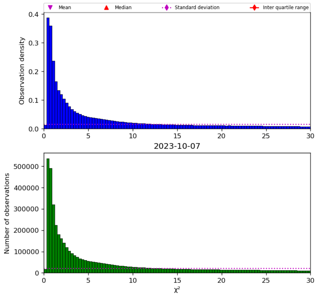
Figure 38: Histogram of " \chi^2 " for 2023-10-06 to 2023-10-08
