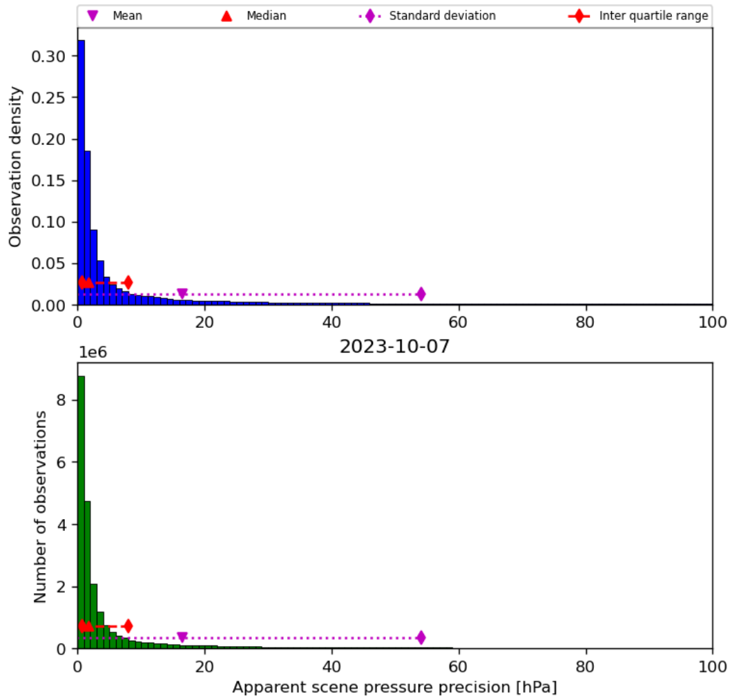
Figure 37: Histogram of “Apparent scene pressure precision” for 2023-10-06 to 2023-10-08
