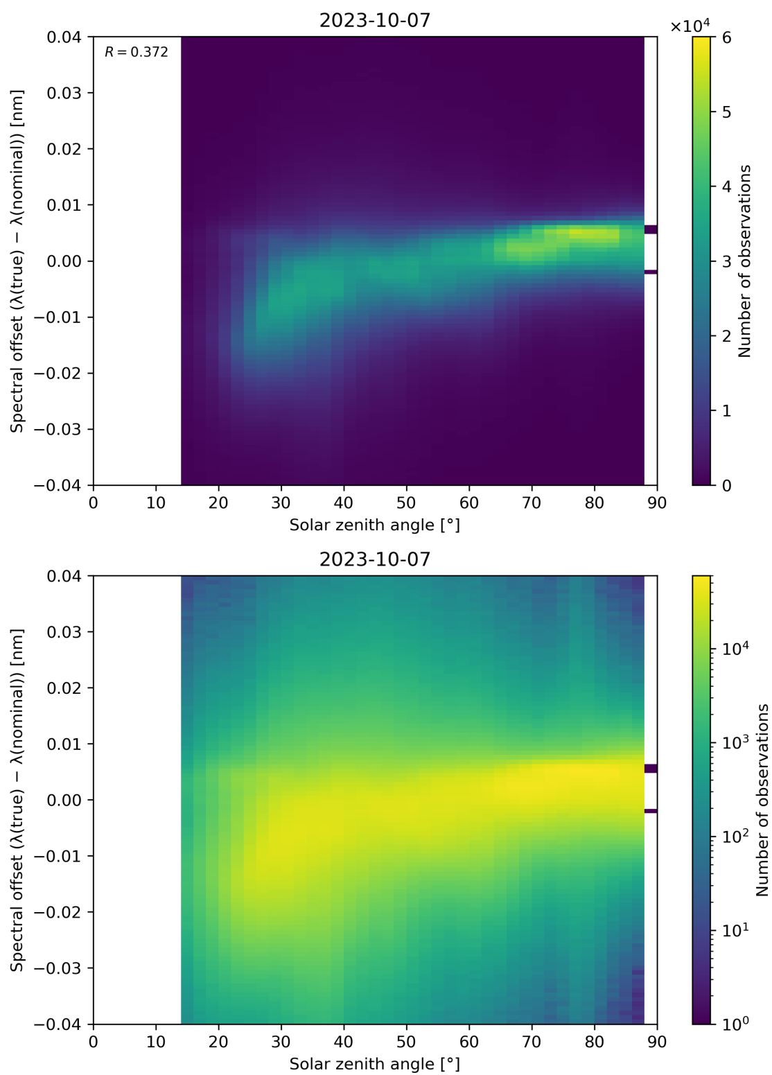
Figure 128: Scatter density plot of “Solar zenith angle” against “Spectral offset ( \lambda(\text{true}) - \lambda(\text{nominal}) )” for 2023-10-06 to 2023-10-08.
