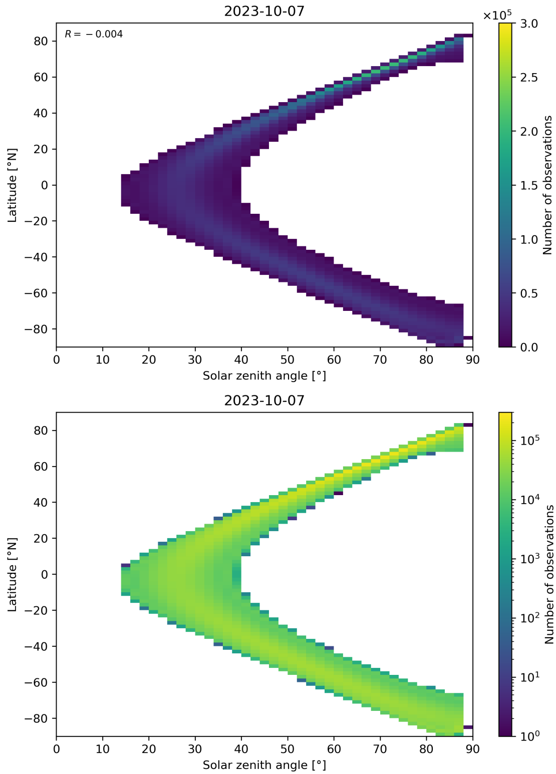
Figure 124: Scatter density plot of “Solar zenith angle” against “Latitude” for 2023-10-06 to 2023-10-08.
