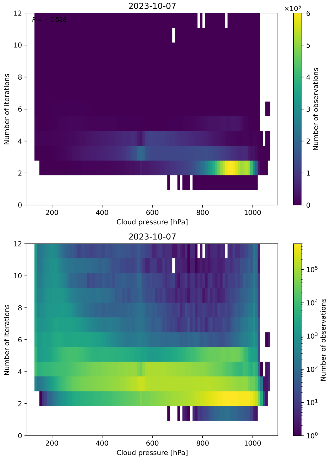
Figure 89: Scatter density plot of “Cloud pressure” against “Number of iterations” for 2023-10-06 to 2023-10-08.
