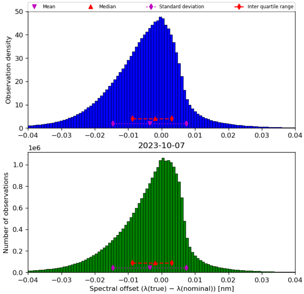
Figure 45: Histogram of “Spectral offset ( \lambda(\text{true}) - \lambda(\text{nominal}) )” for 2023-10-06 to 2023-10-08
