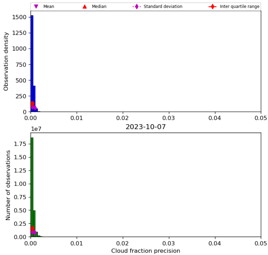
Figure 33: Histogram of “Cloud fraction precision” for 2023-10-06 to 2023-10-08
