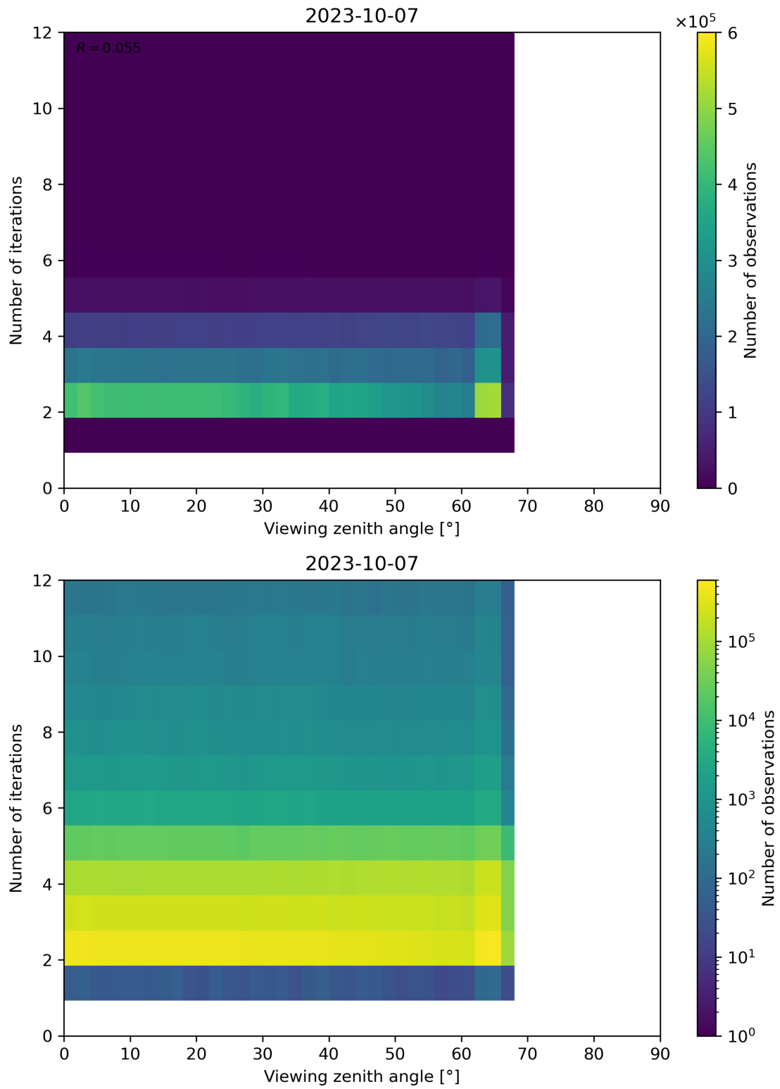
Figure 136: Scatter density plot of “Viewing zenith angle” against “Number of iterations” for 2023-10-06 to 2023-10-08.
