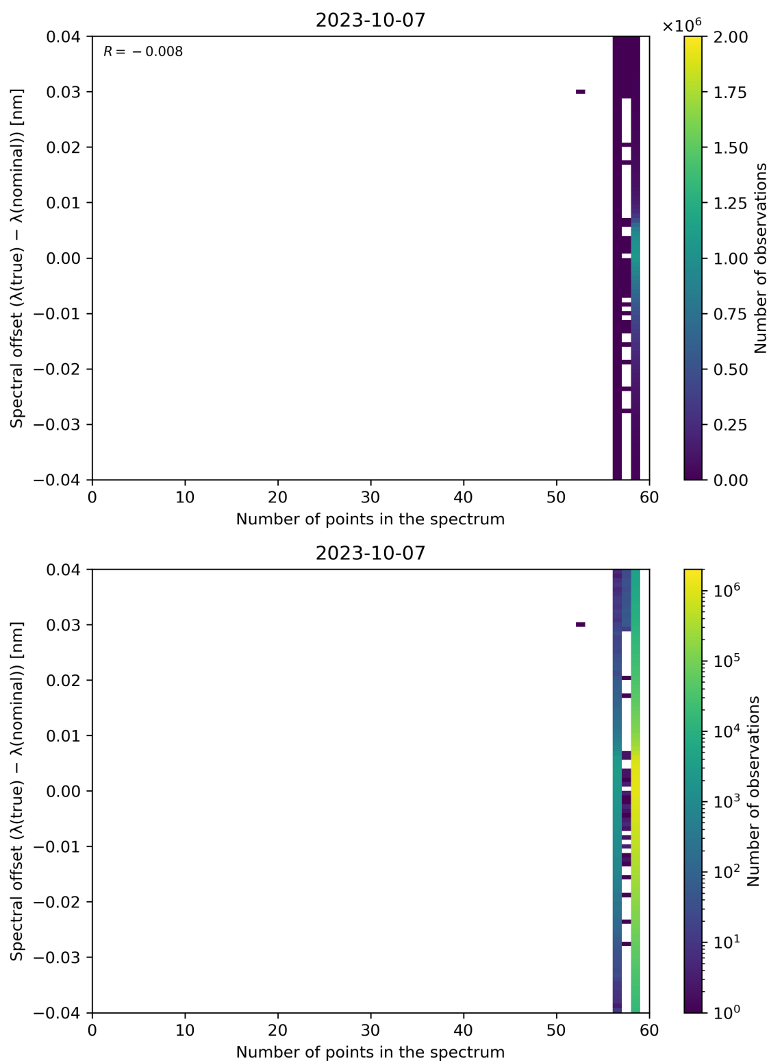
Figure 110: Scatter density plot of “Number of points in the spectrum” against “Spectral offset ( \lambda(\text{true}) - \lambda(\text{nominal}) )” for 2023-10-06 to 2023-10-08.
