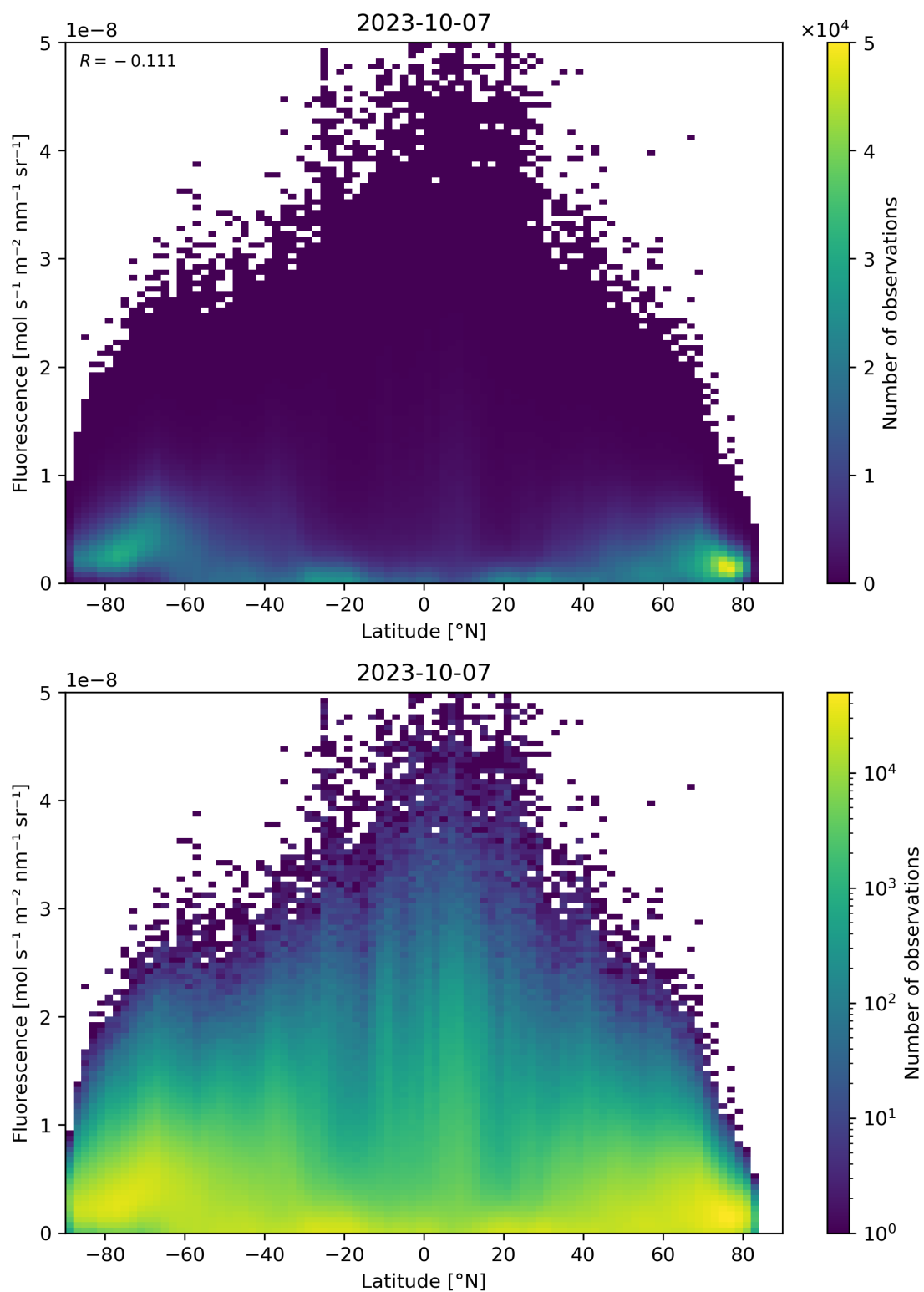
Figure 101: Scatter density plot of “Latitude” against “Fluorescence” for 2023-10-06 to 2023-10-08.
