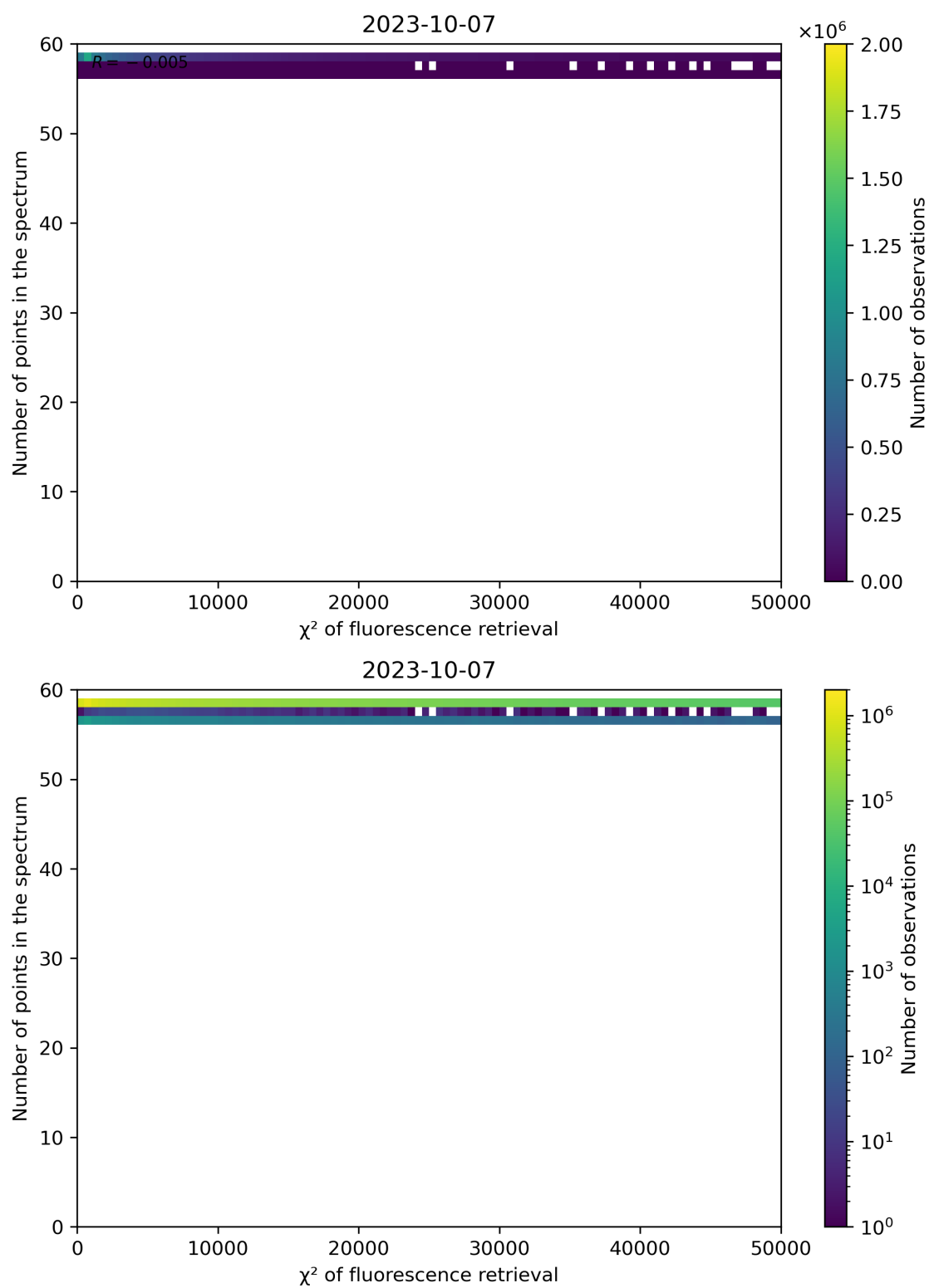
Figure 71: Scatter density plot of “ \chi^2 of fluorescence retrieval” against “Number of points in the spectrum” for 2023-10-06 to 2023-10-08.
