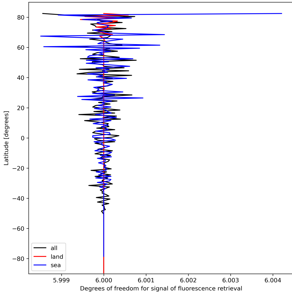
Figure 26: Zonal average of “Degrees of freedom for signal of fluorescence retrieval” for 2023-10-06 to 2023-10-08.
