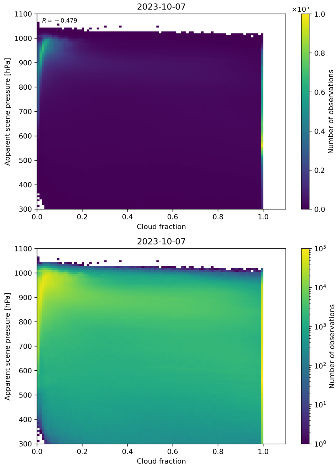
Figure 76: Scatter density plot of “Cloud fraction” against “Apparent scene pressure” for 2023-10-06 to 2023-10-08.
