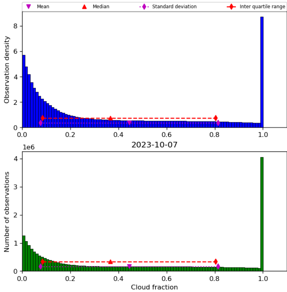
Figure 32: Histogram of “Cloud fraction” for 2023-10-06 to 2023-10-08
