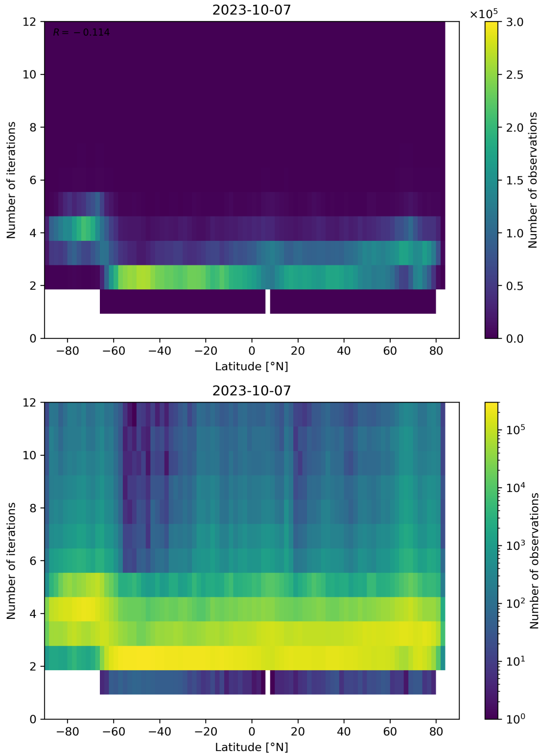
Figure 102: Scatter density plot of “Latitude” against “Number of iterations” for 2023-10-06 to 2023-10-08.
