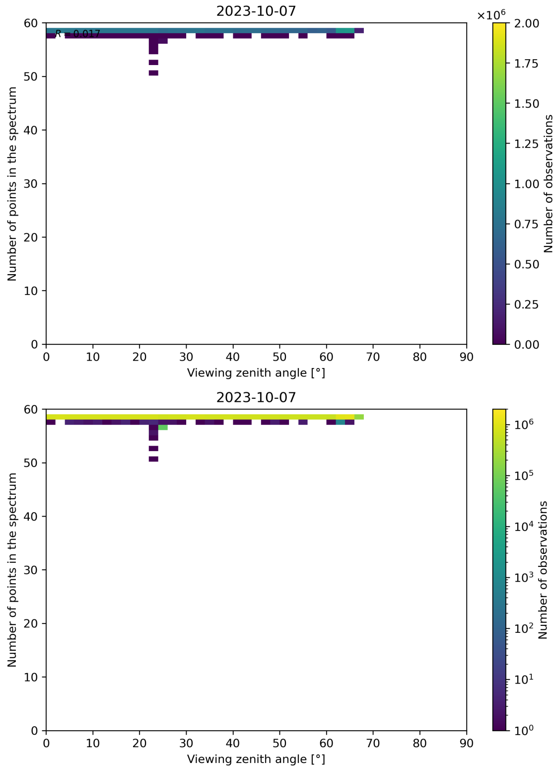
Figure 137: Scatter density plot of “Viewing zenith angle” against “Number of points in the spectrum” for 2023-10-06 to 2023-10-08.
