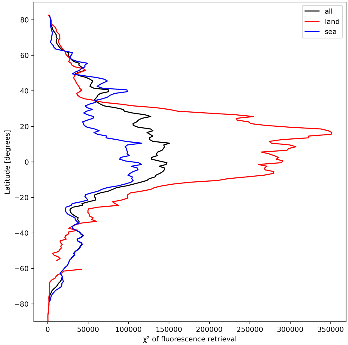
Figure 25: Zonal average of “ \chi^2 of fluorescence retrieval” for 2023-10-06 to 2023-10-08.
