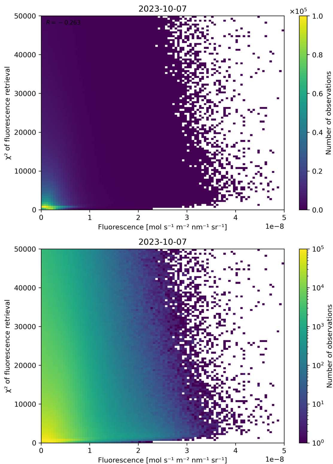
Figure 93: Scatter density plot of “Fluorescence” against “ \chi^2 of fluorescence retrieval” for 2023-10-06 to 2023-10-08.
