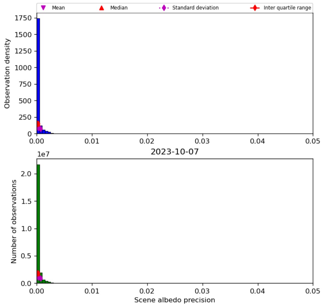
Figure 35: Histogram of “Scene albedo precision” for 2023-10-06 to 2023-10-08
