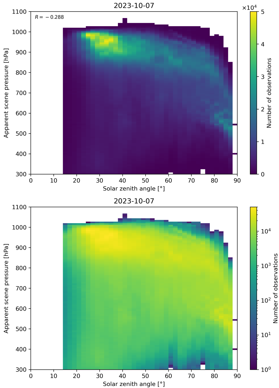
Figure 118: Scatter density plot of “Solar zenith angle” against “Apparent scene pressure” for 2023-10-06 to 2023-10-08.
