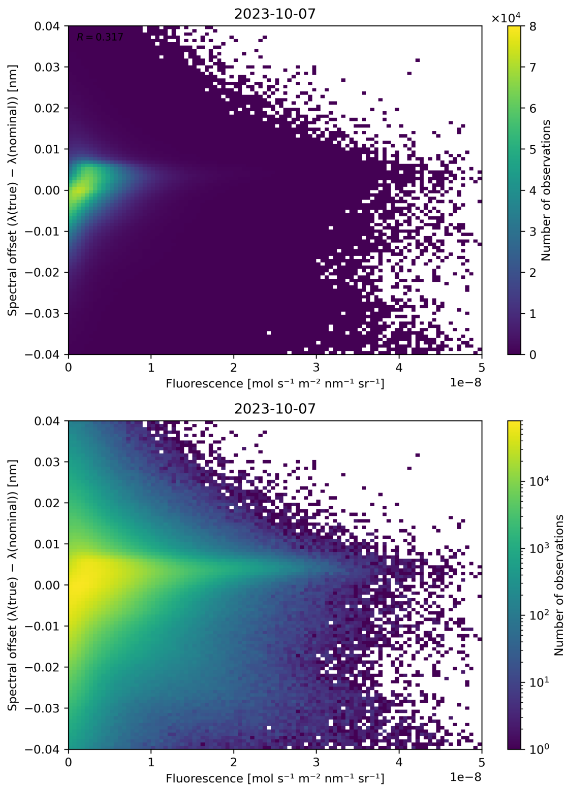
Figure 95: Scatter density plot of “Fluorescence” against “Spectral offset ( \lambda(\text{true}) - \lambda(\text{nominal}) )” for 2023-10-06 to 2023-10-08.
