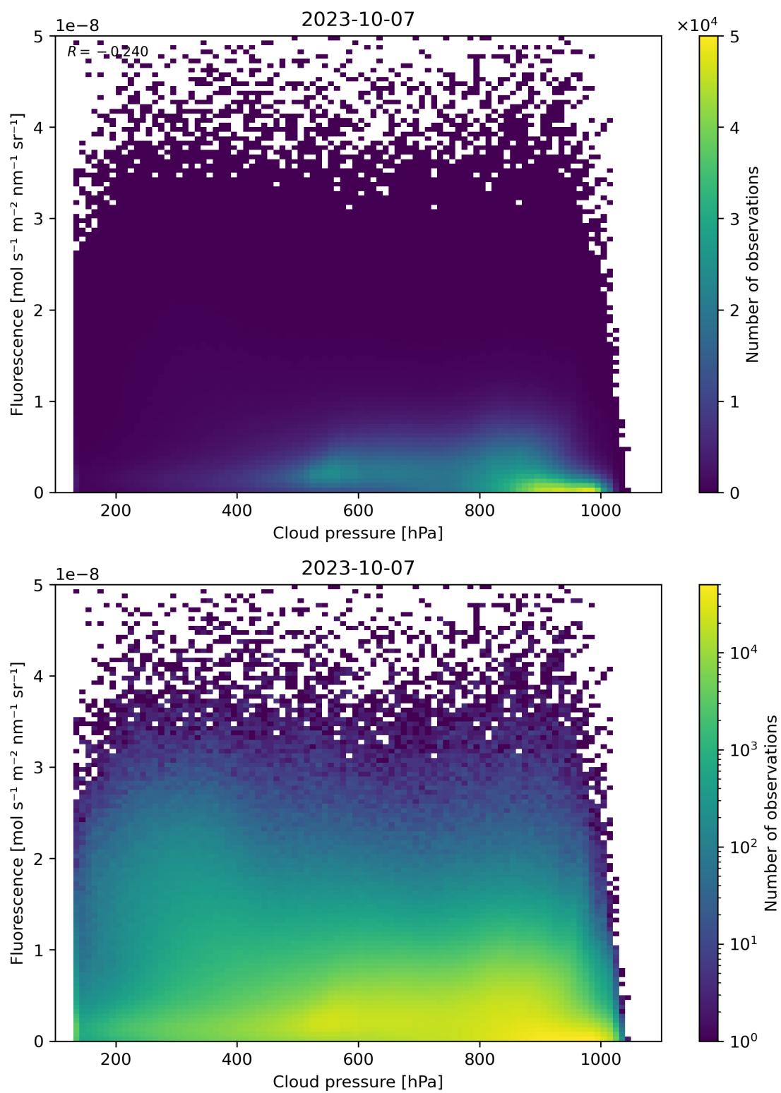
Figure 88: Scatter density plot of “Cloud pressure” against “Fluorescence” for 2023-10-06 to 2023-10-08.
