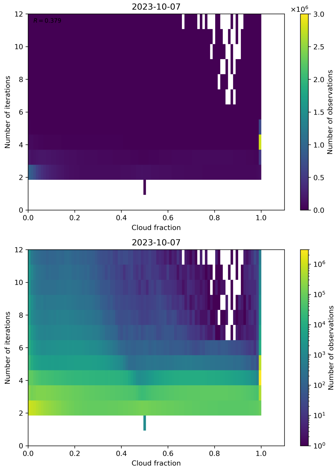
Figure 80: Scatter density plot of “Cloud fraction” against “Number of iterations” for 2023-10-06 to 2023-10-08.
