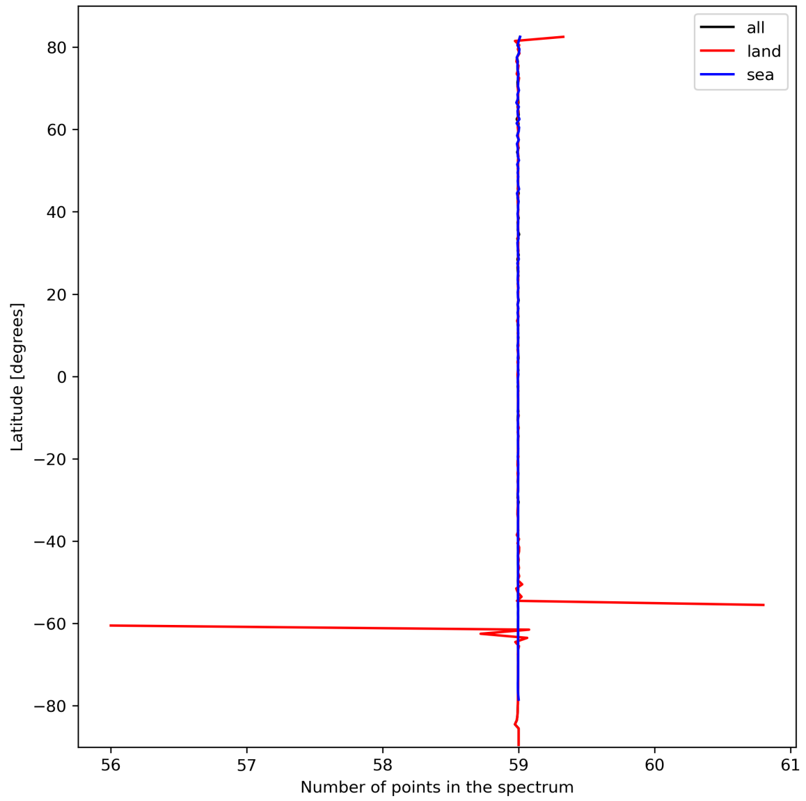
Figure 27: Zonal average of “Number of points in the spectrum” for 2023-10-06 to 2023-10-08.
