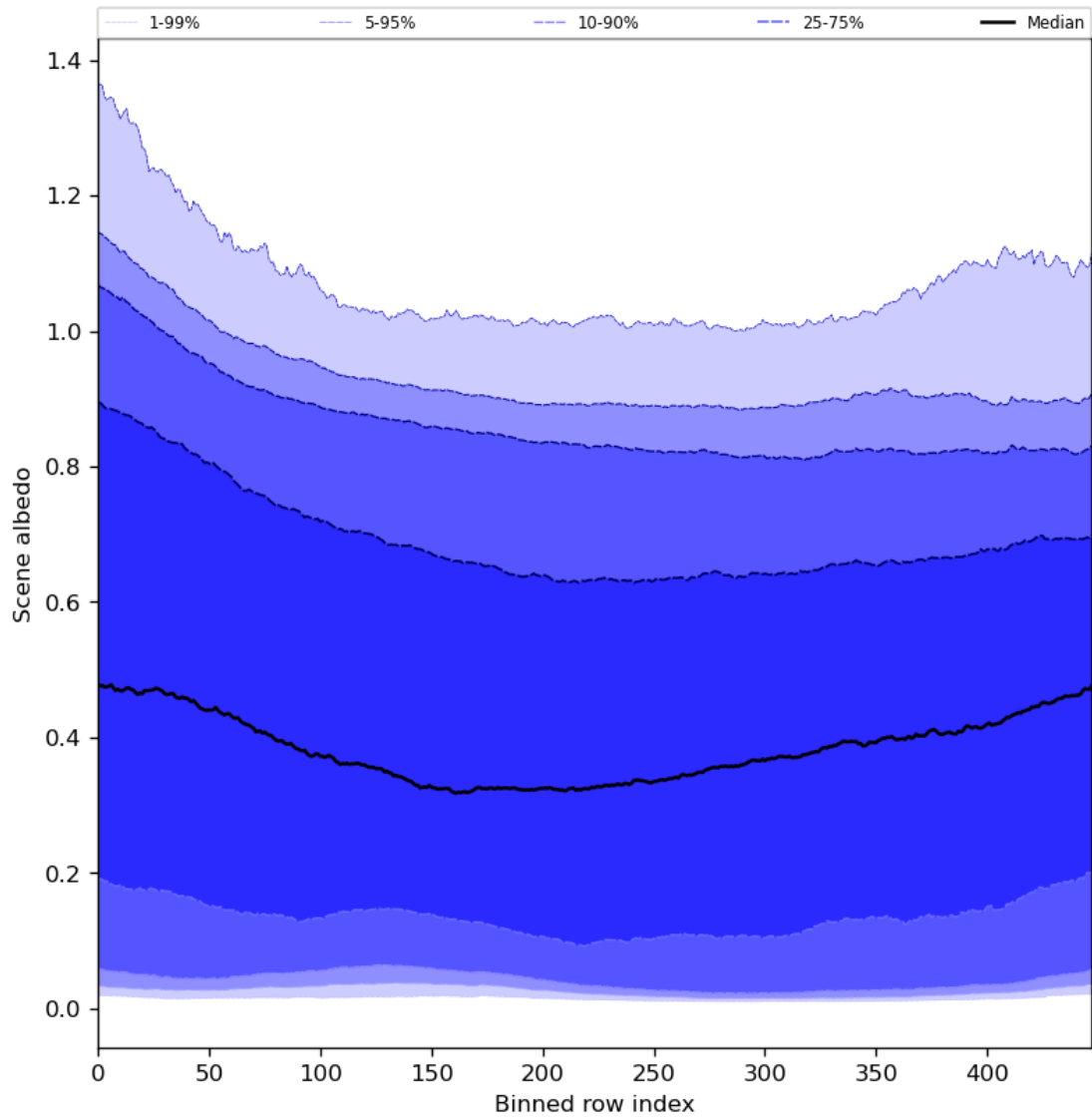
Figure 51: Along track statistics of “Scene albedo” for 2023-10-06 to 2023-10-08
