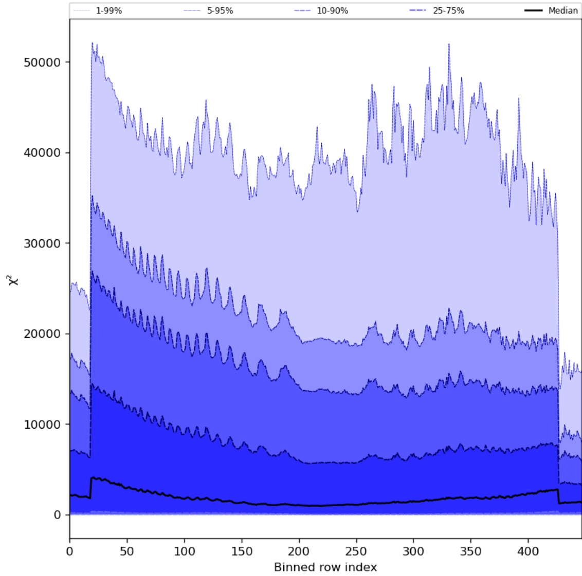
Figure 55: Along track statistics of “ \chi^2 ” for 2023-10-06 to 2023-10-08
