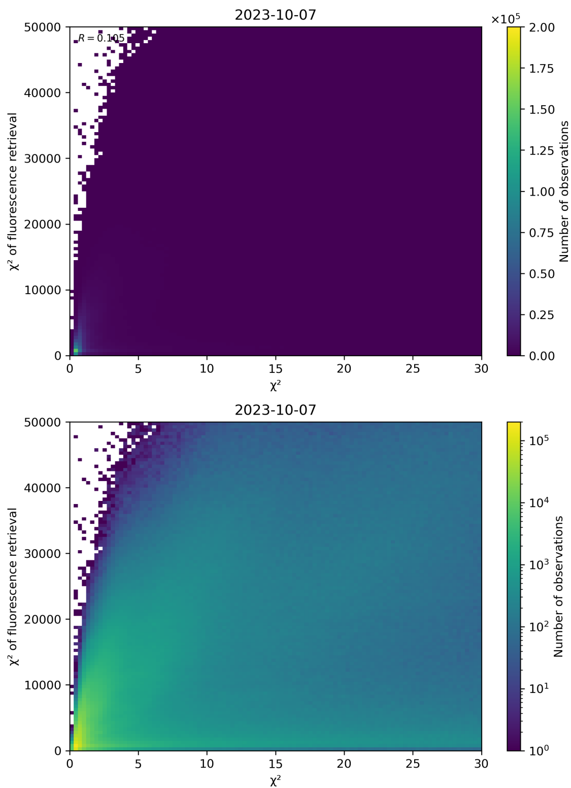
Figure 69: Scatter density plot of “ \chi^2 ” against “ \chi^2 of fluorescence retrieval” for 2023-10-06 to 2023-10-08.
