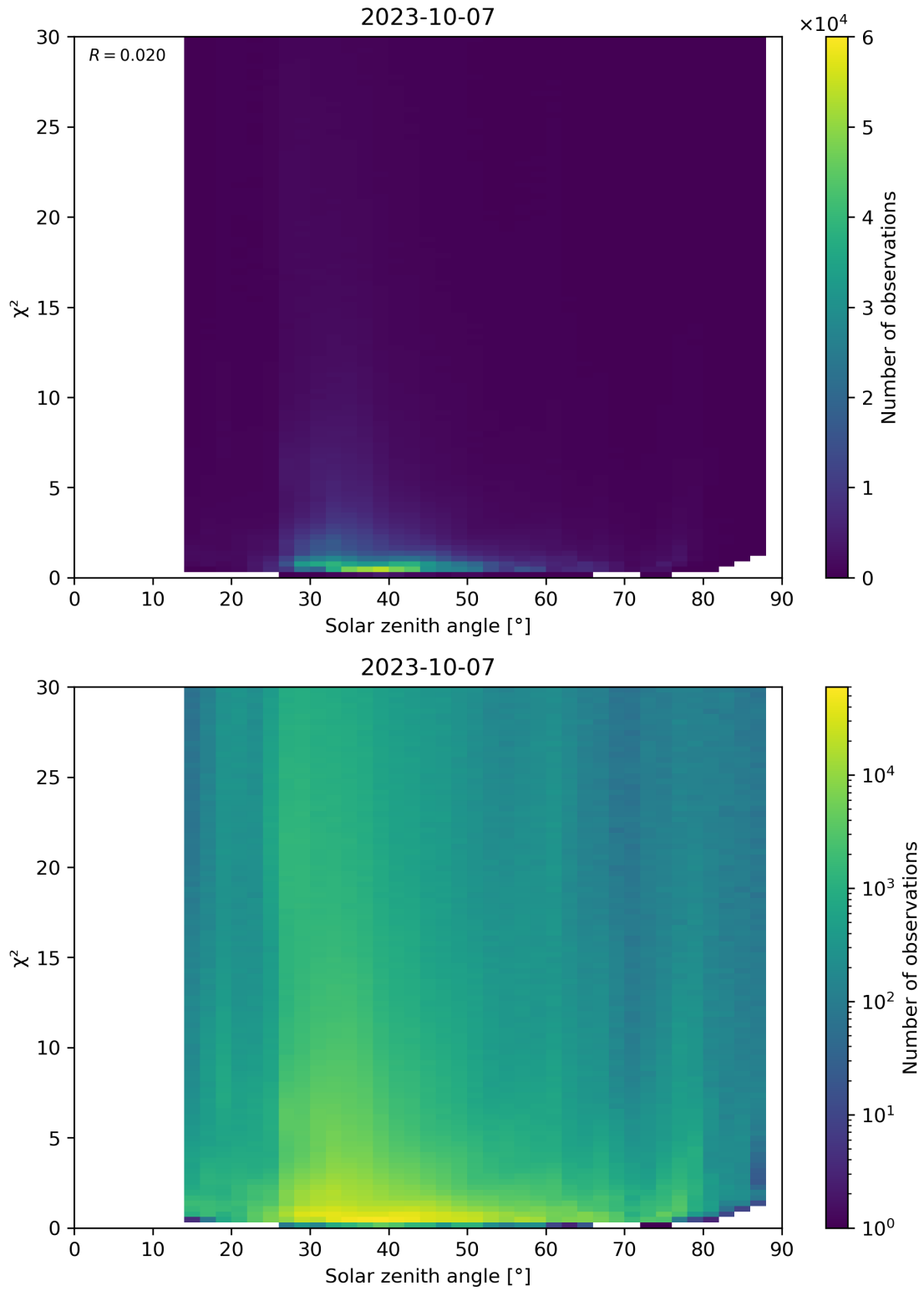
Figure 119: Scatter density plot of “Solar zenith angle” against “ \chi^2 ” for 2023-10-06 to 2023-10-08.
