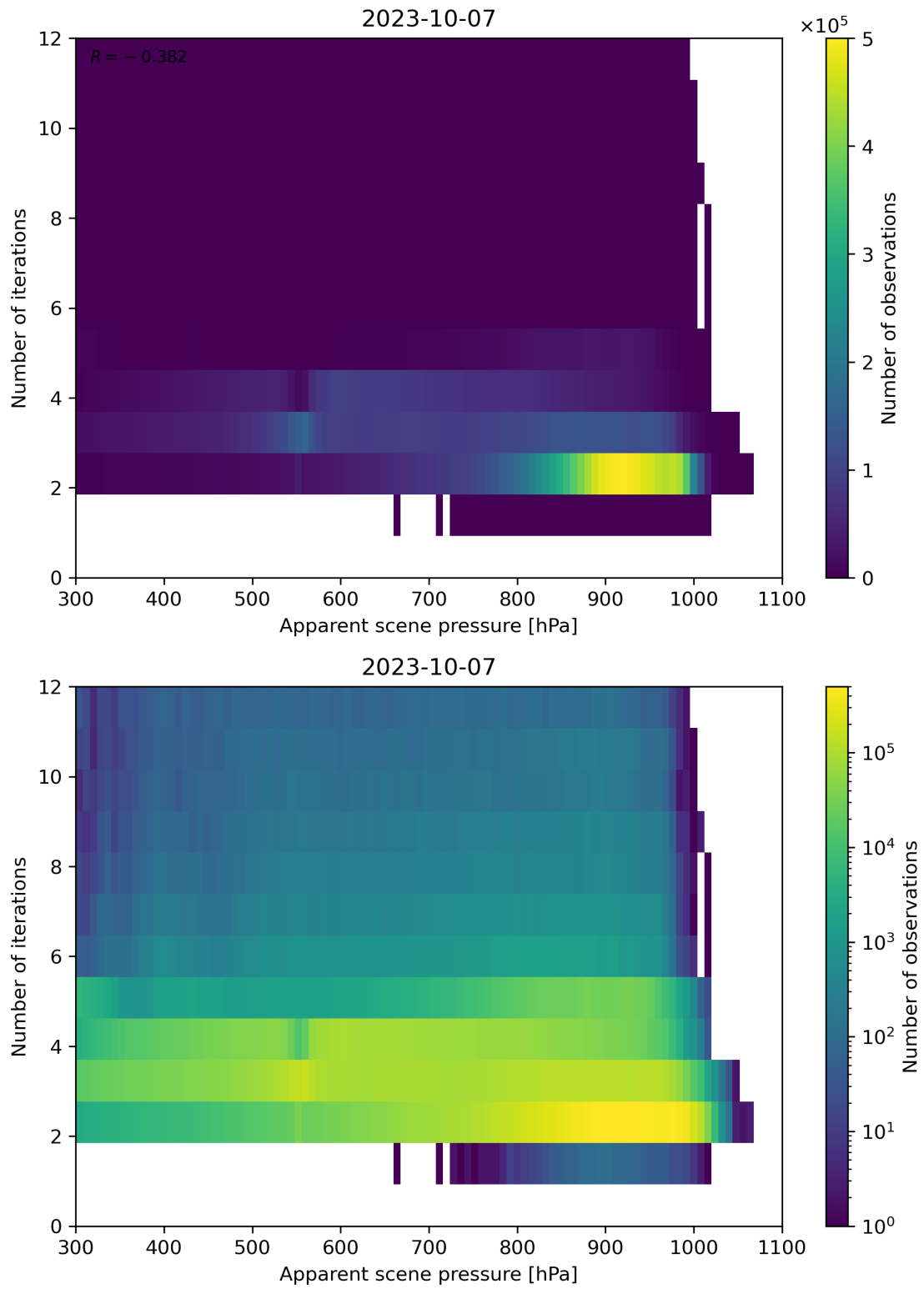
Figure 66: Scatter density plot of “Apparent scene pressure” against “Number of iterations” for 2023-10-06 to 2023-10-08.
