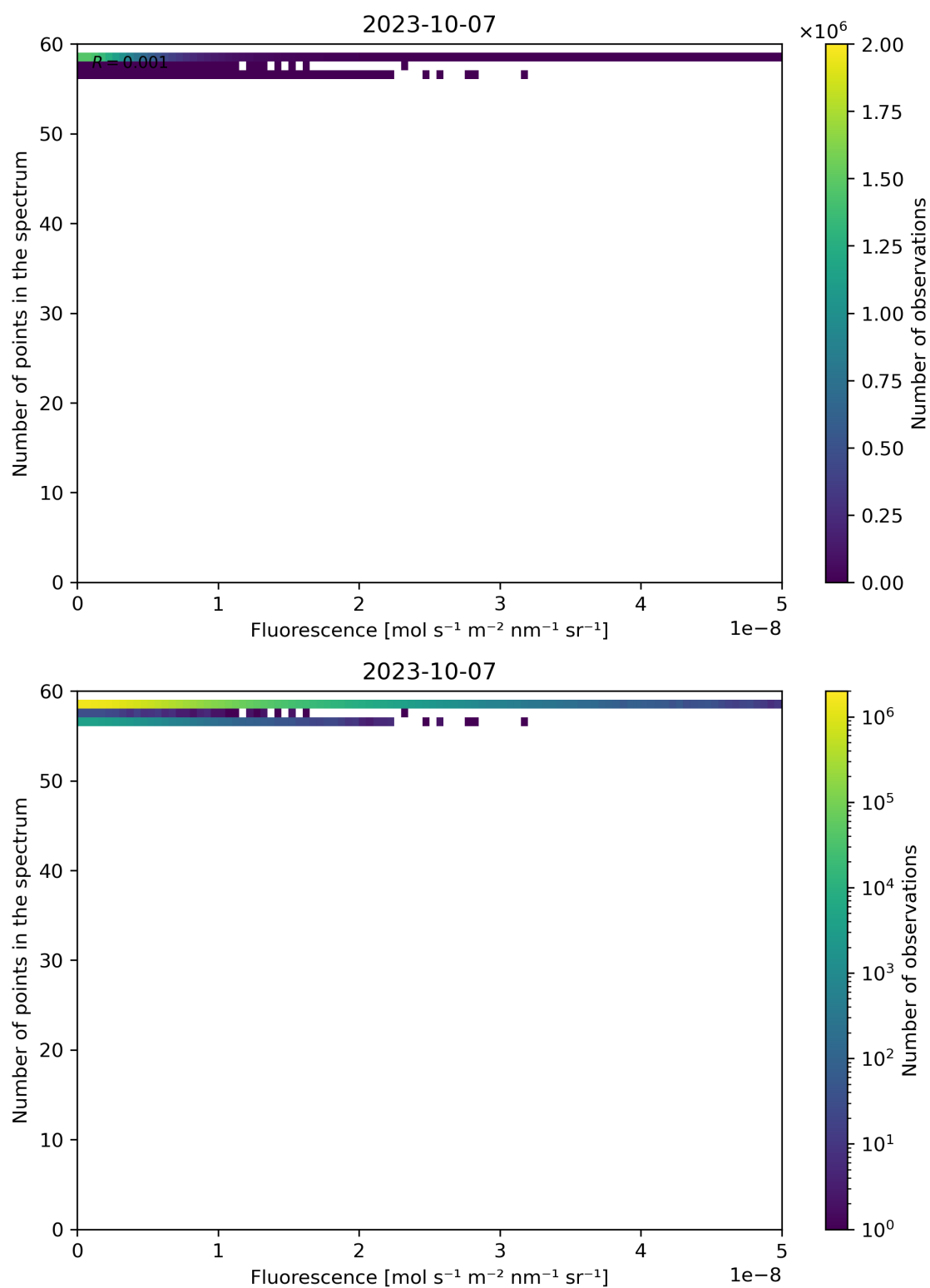
Figure 94: Scatter density plot of “Fluorescence” against “Number of points in the spectrum” for 2023-10-06 to 2023-10-08.
