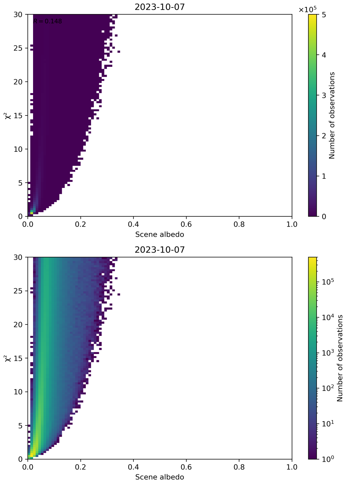
Figure 112: Scatter density plot of “Scene albedo” against “ \chi^2 ” for 2023-10-06 to 2023-10-08.
