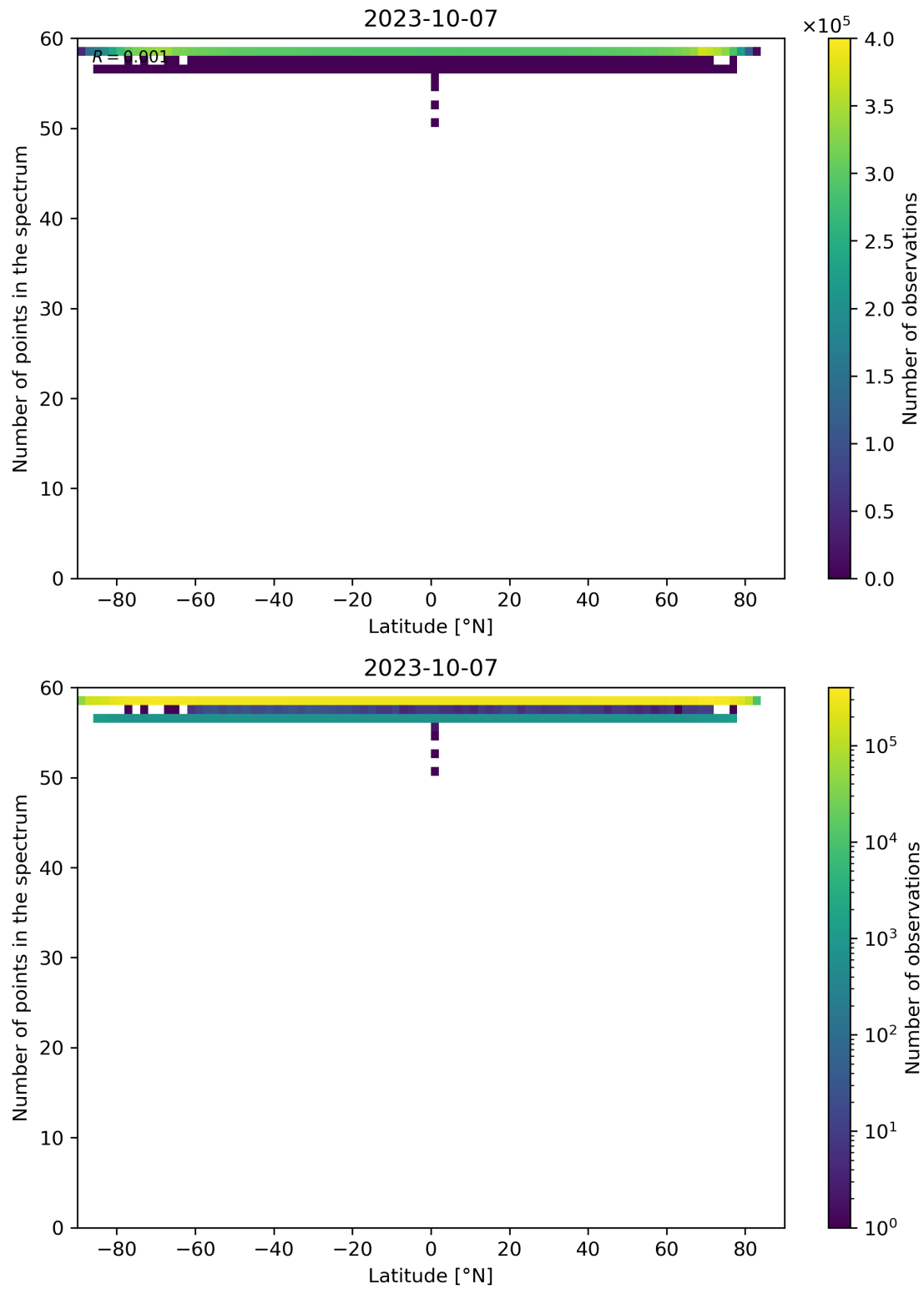
Figure 103: Scatter density plot of “Latitude” against “Number of points in the spectrum” for 2023-10-06 to 2023-10-08.
