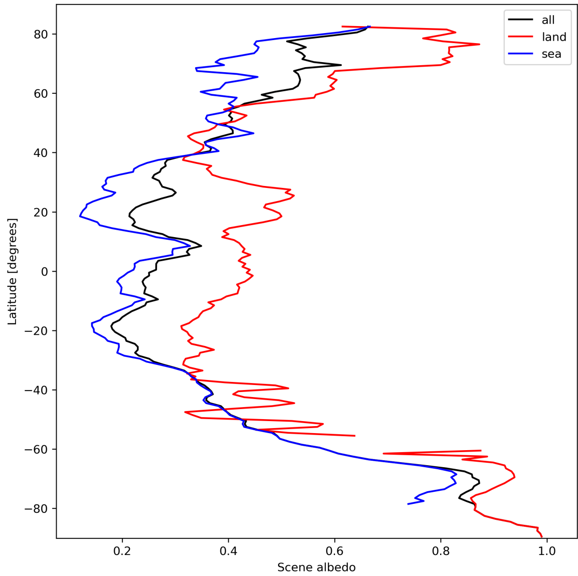
Figure 17: Zonal average of “Scene albedo” for 2023-10-06 to 2023-10-08.
