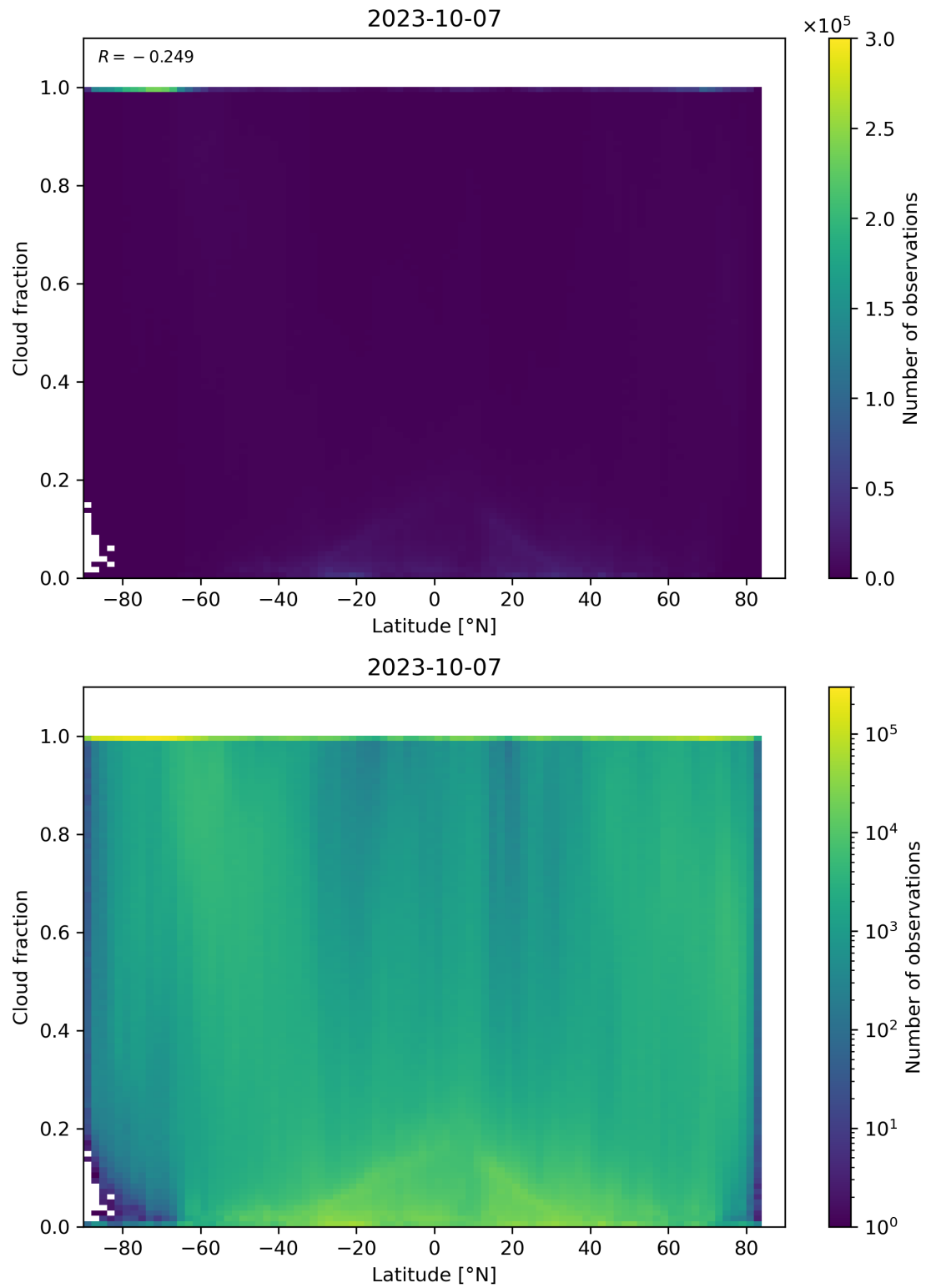
Figure 99: Scatter density plot of “Latitude” against “Cloud fraction” for 2023-10-06 to 2023-10-08.
