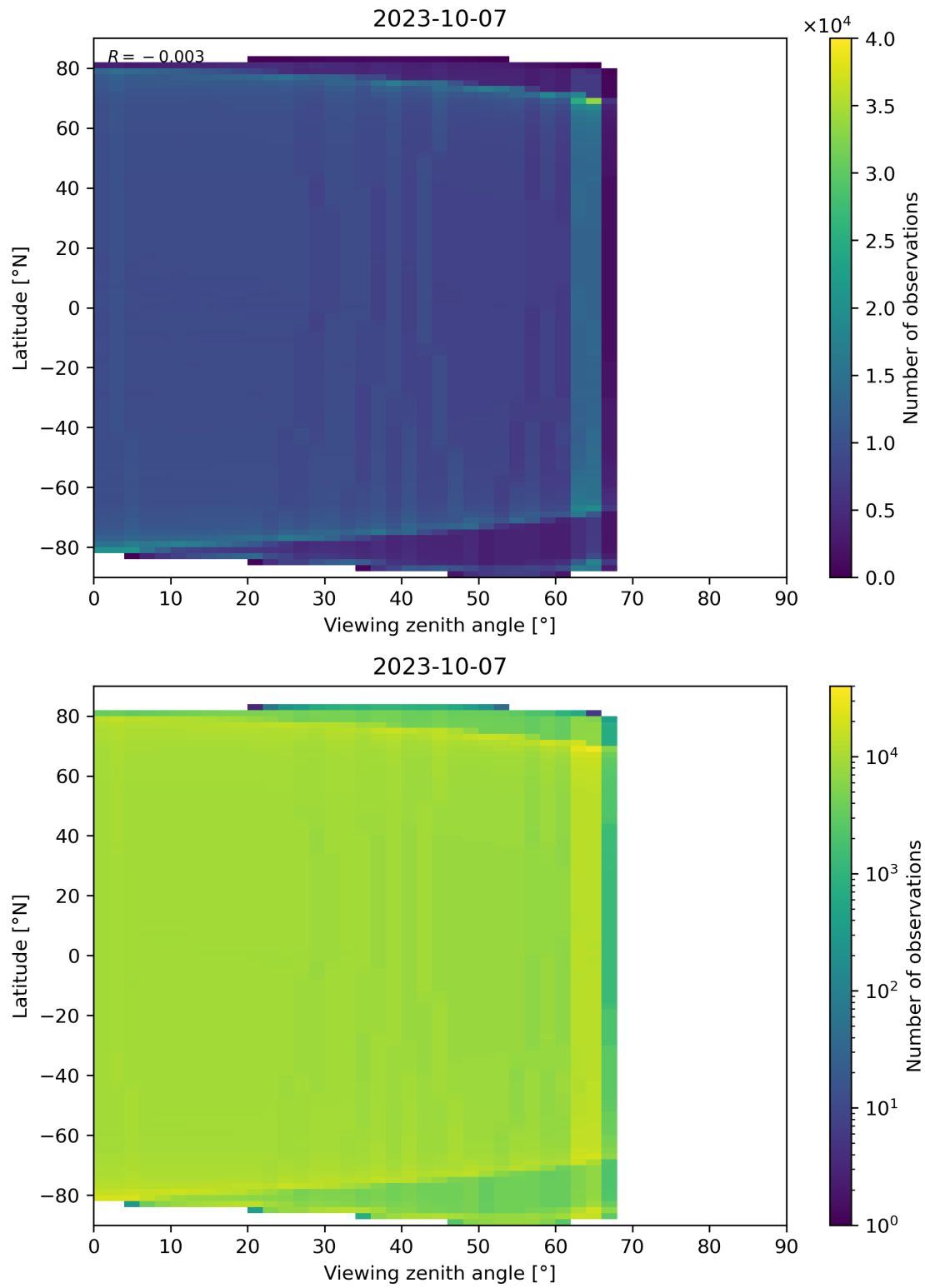
Figure 135: Scatter density plot of “Viewing zenith angle” against “Latitude” for 2023-10-06 to 2023-10-08.
