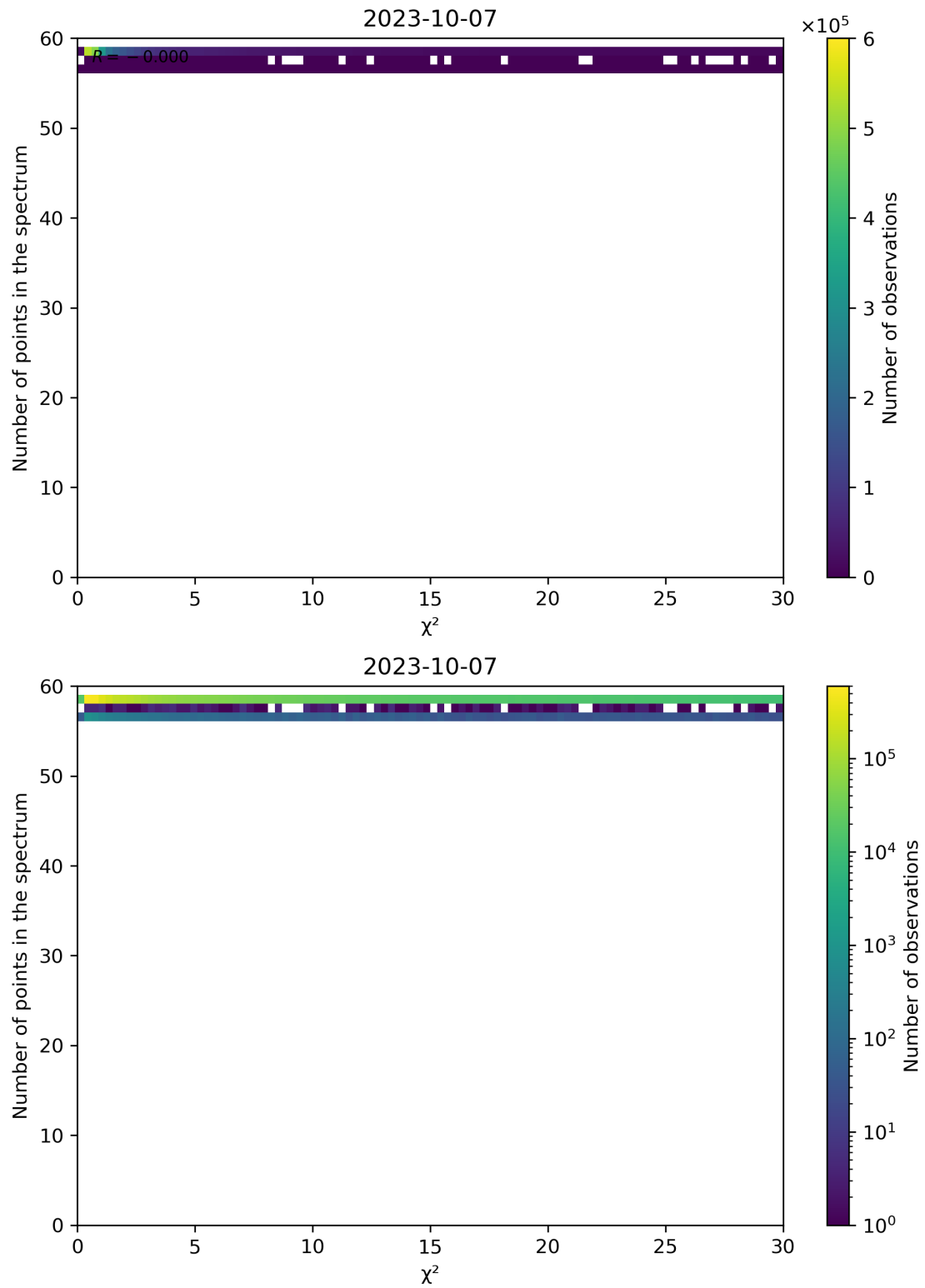
Figure 74: Scatter density plot of " \chi^2 " against "Number of points in the spectrum" for 2023-10-06 to 2023-10-08.
