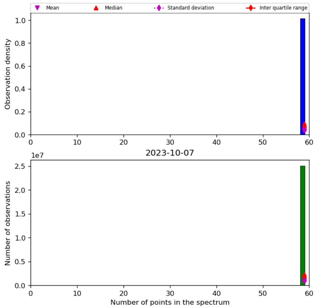
Figure 44: Histogram of “Number of points in the spectrum” for 2023-10-06 to 2023-10-08
