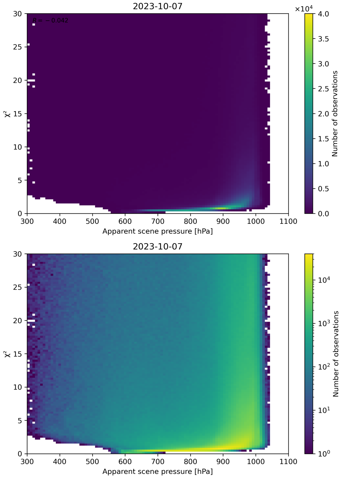
Figure 63: Scatter density plot of “Apparent scene pressure” against “ \chi^2 ” for 2023-10-06 to 2023-10-08.
