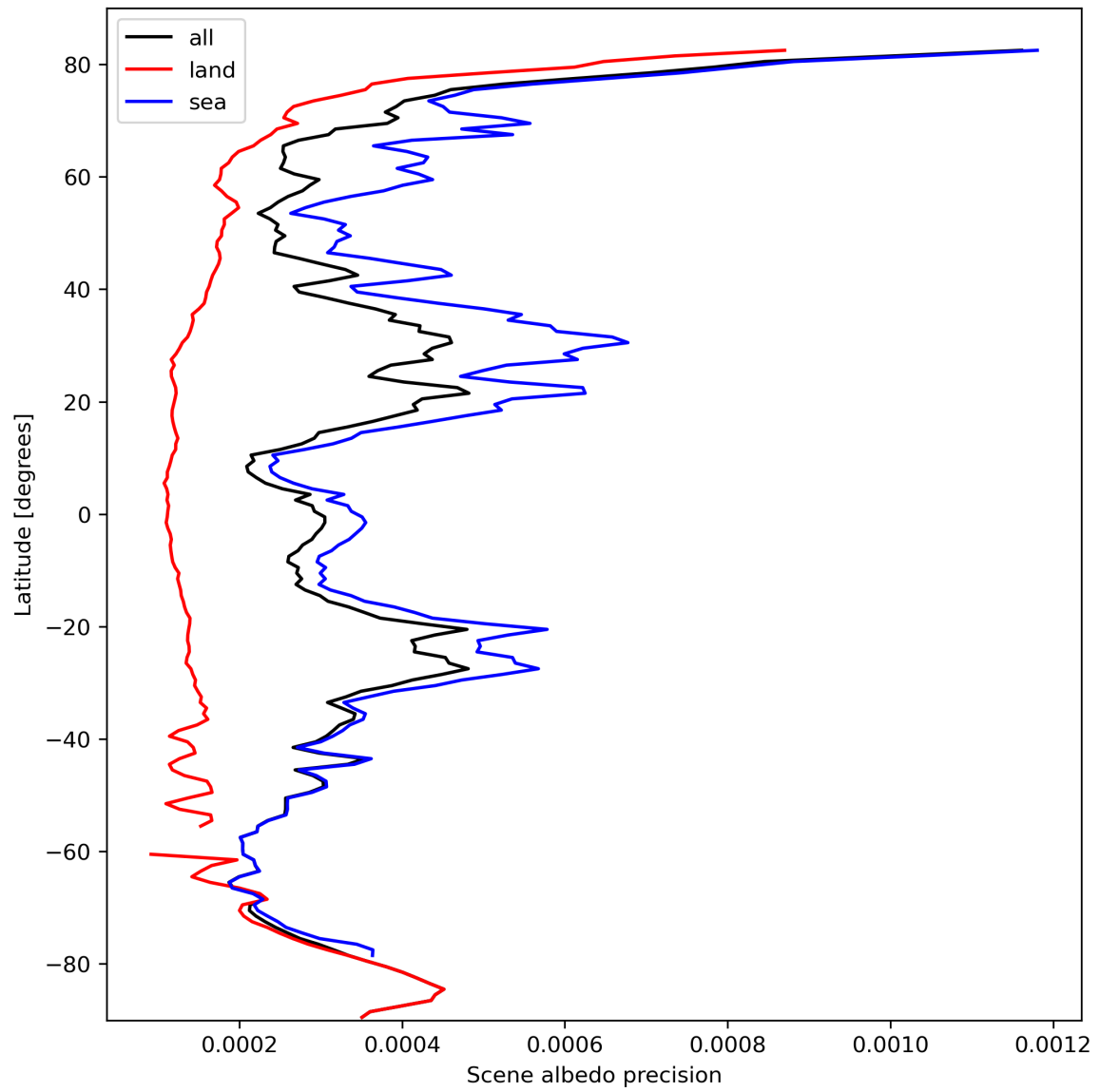
Figure 18: Zonal average of “Scene albedo precision” for 2023-10-06 to 2023-10-08.
