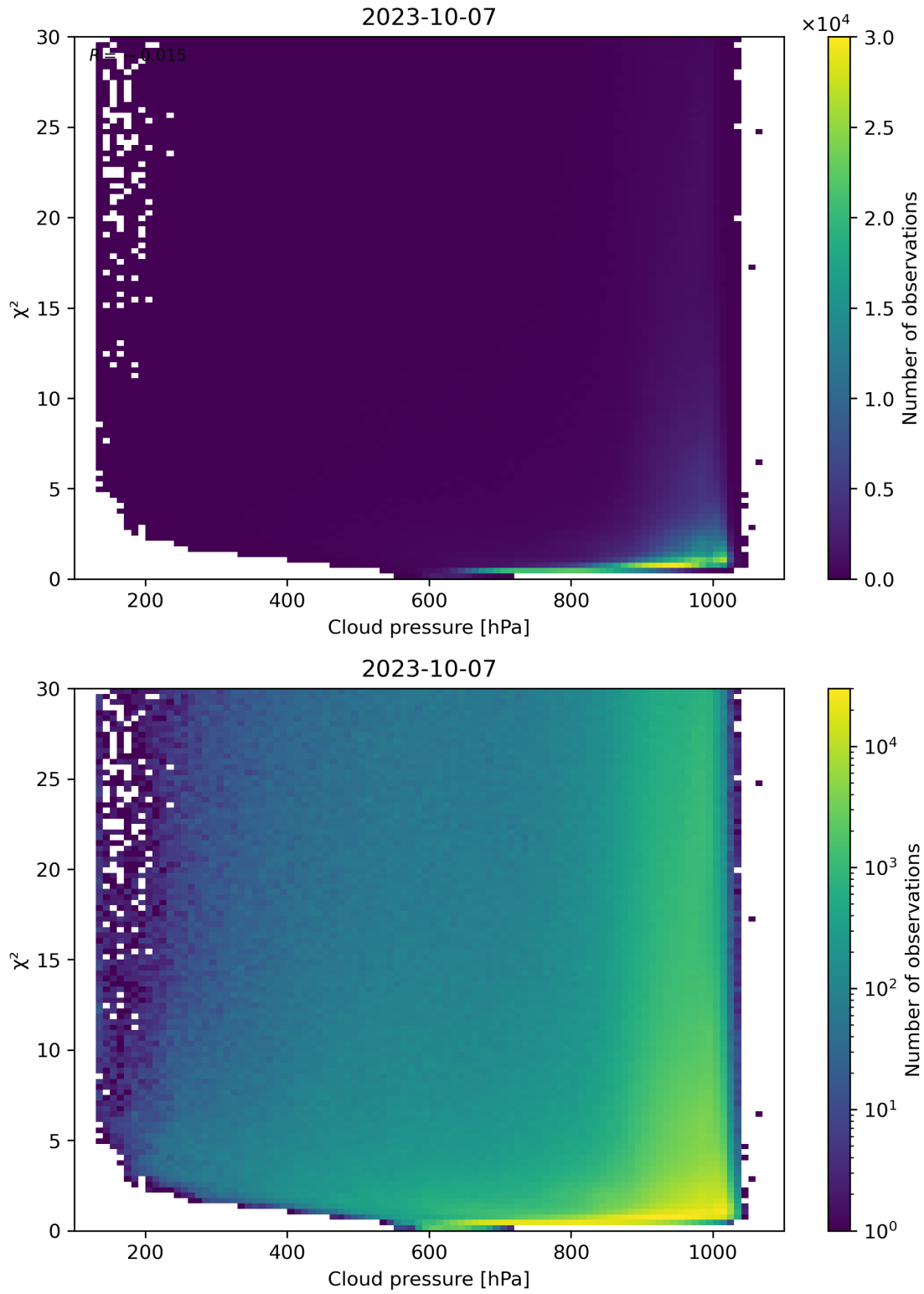
Figure 85: Scatter density plot of “Cloud pressure” against “ \chi^2 ” for 2023-10-06 to 2023-10-08.
