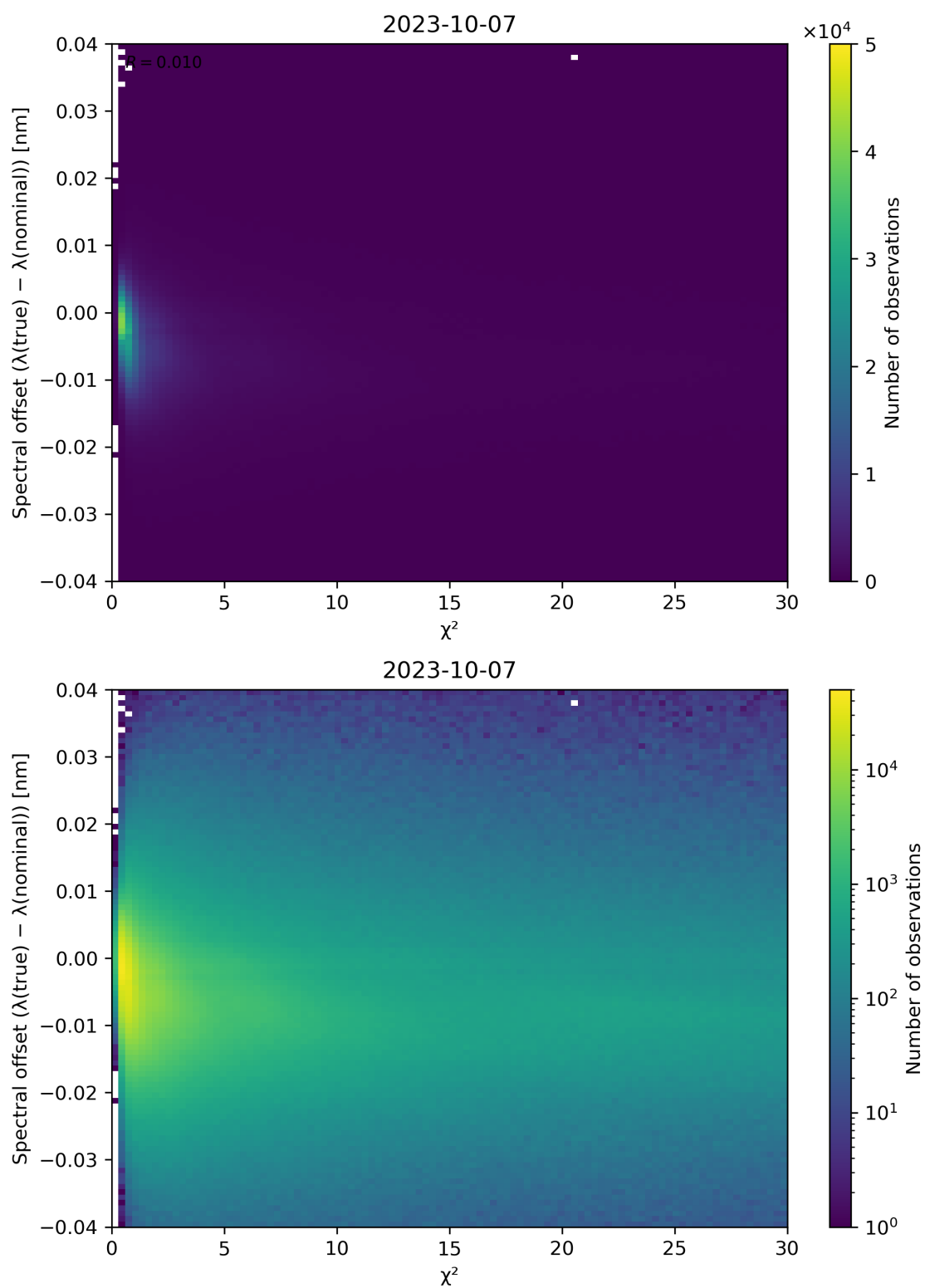
Figure 75: Scatter density plot of “ \chi^2 ” against “Spectral offset ( \lambda(\text{true}) - \lambda(\text{nominal}) )” for 2023-10-06 to 2023-10-08.
