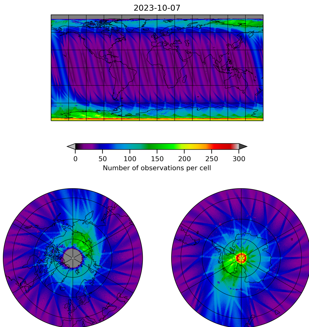
Figure 11: Map of the number of observations for 2023-10-06 to 2023-10-08
