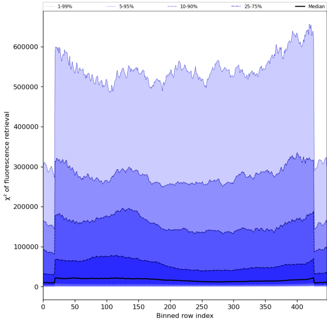
Figure 59: Along track statistics of “ \chi^2 of fluorescence retrieval” for 2023-10-06 to 2023-10-08
