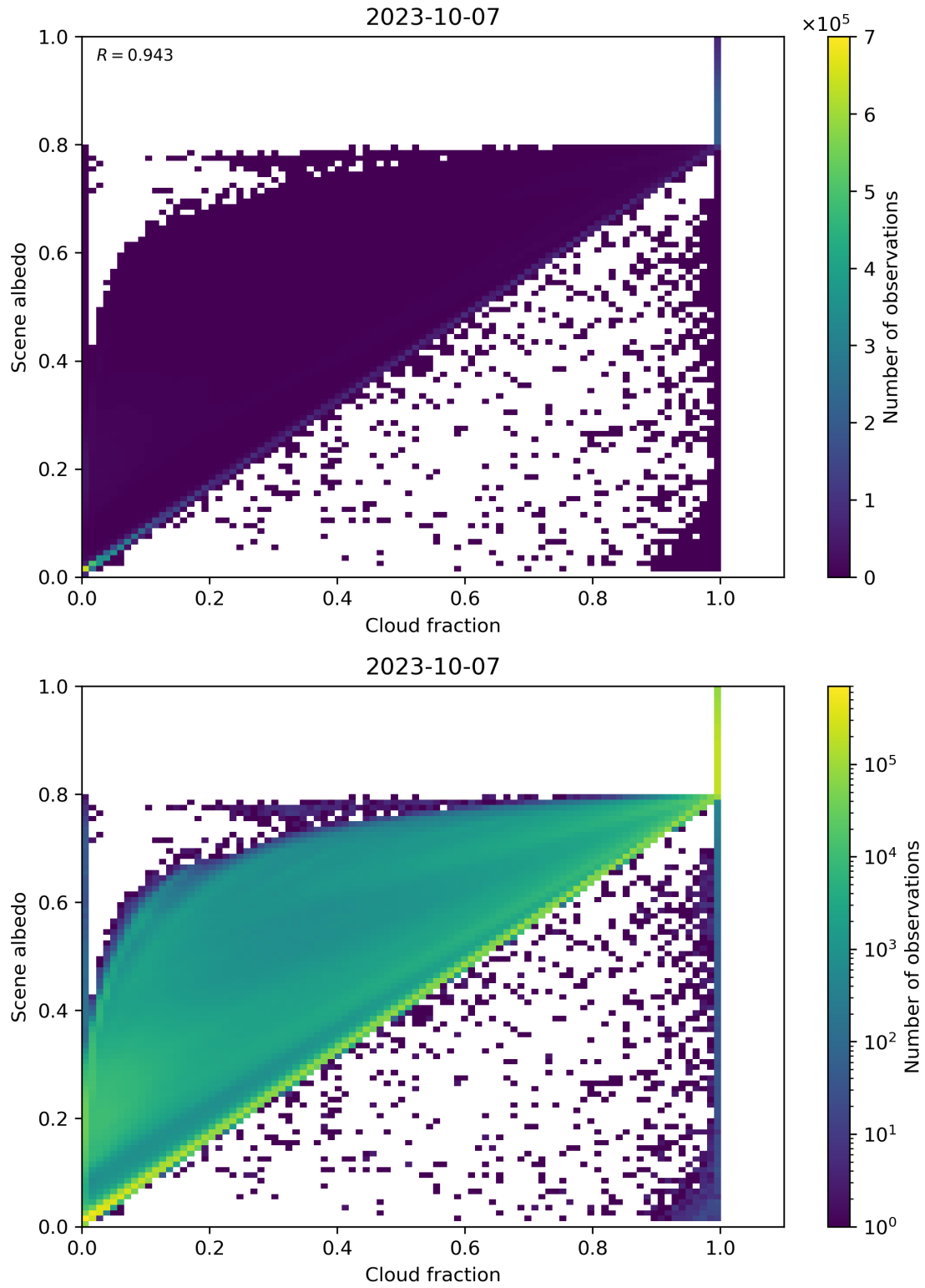
Figure 82: Scatter density plot of “Cloud fraction” against “Scene albedo” for 2023-10-06 to 2023-10-08.
