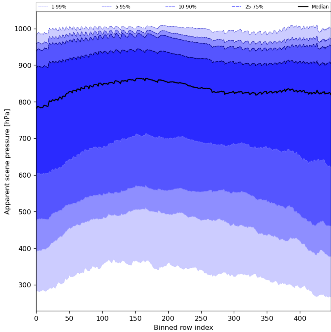
Figure 53: Along track statistics of “Apparent scene pressure” for 2023-10-06 to 2023-10-08
