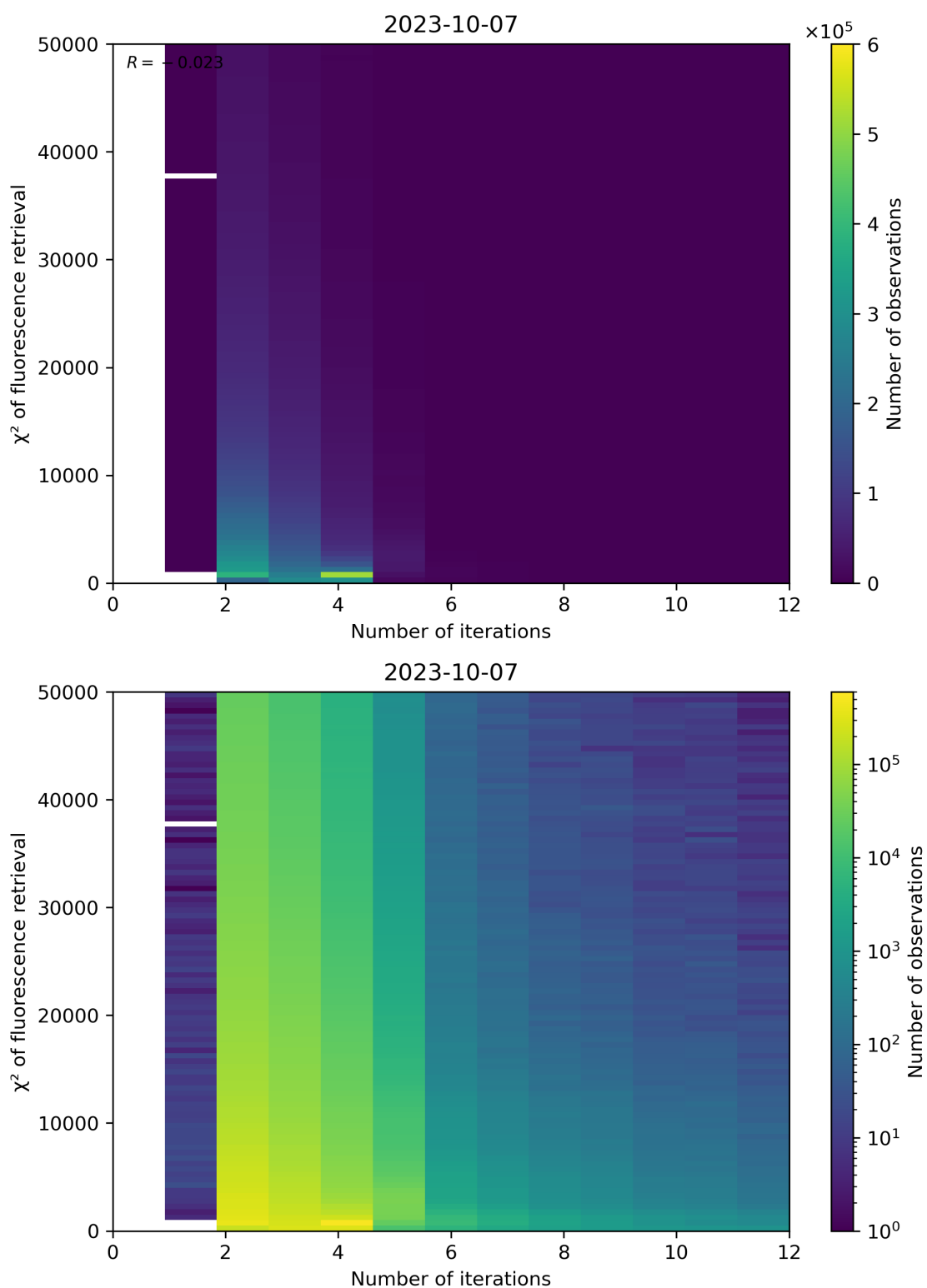
Figure 106: Scatter density plot of “Number of iterations” against “ \chi^2 of fluorescence retrieval” for 2023-10-06 to 2023-10-08.
