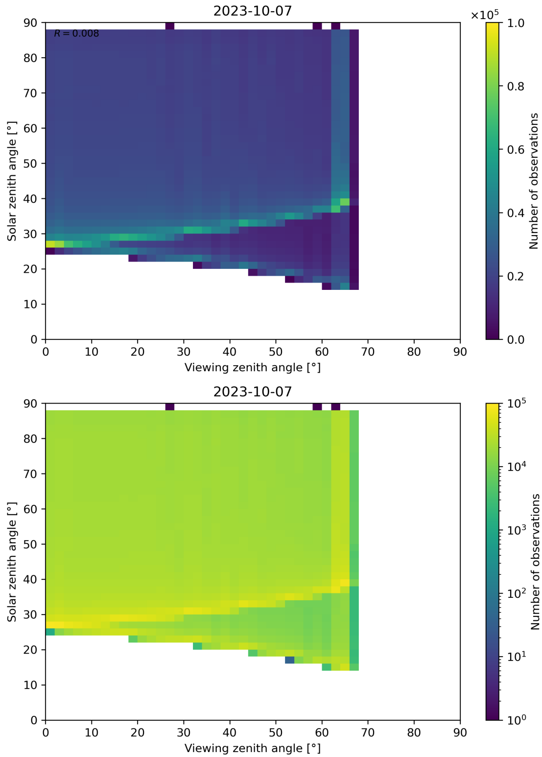
Figure 139: Scatter density plot of “Viewing zenith angle” against “Solar zenith angle” for 2023-10-06 to 2023-10-08.
