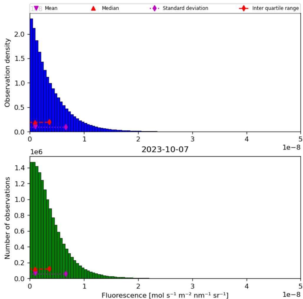
Figure 40: Histogram of “Fluorescence” for 2023-10-06 to 2023-10-08
