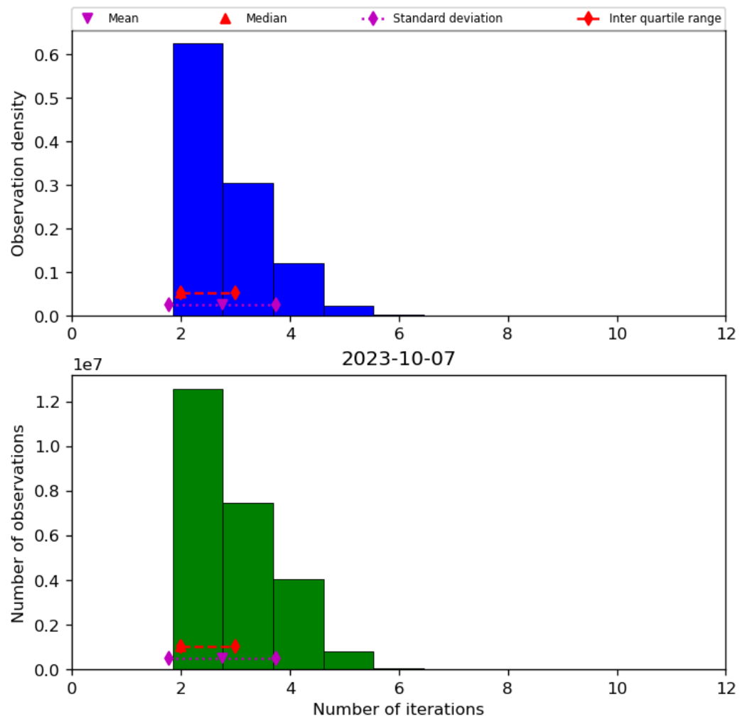
Figure 39: Histogram of “Number of iterations” for 2023-10-06 to 2023-10-08
