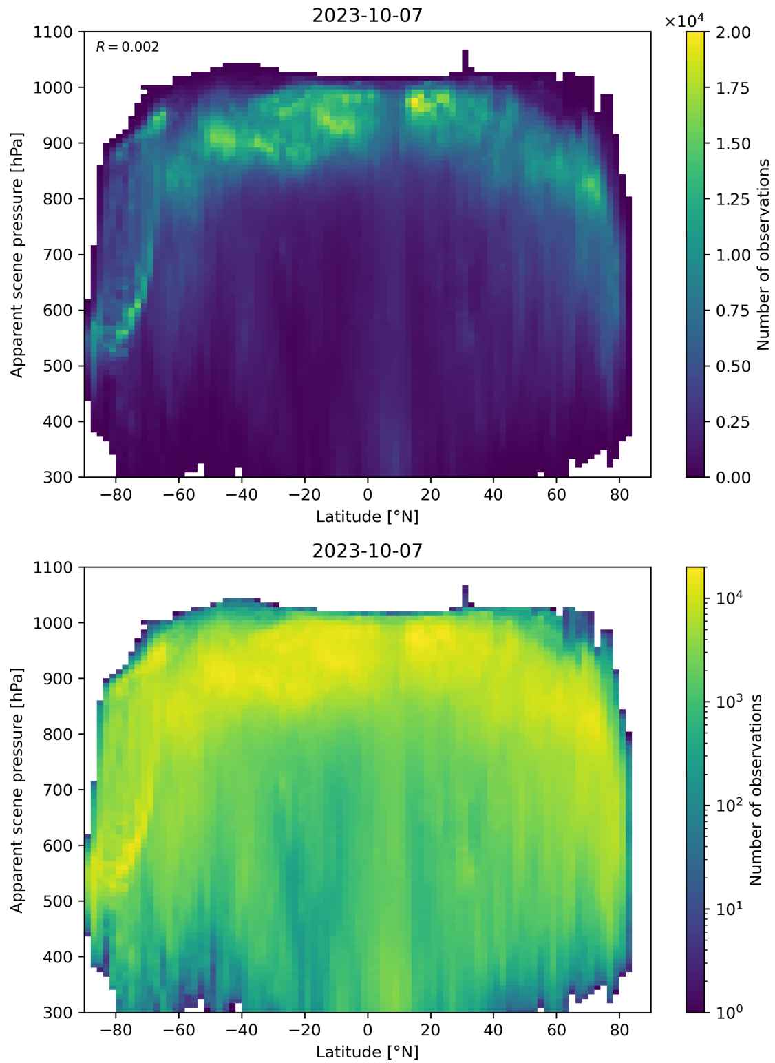
Figure 96: Scatter density plot of “Latitude” against “Apparent scene pressure” for 2023-10-06 to 2023-10-08.
