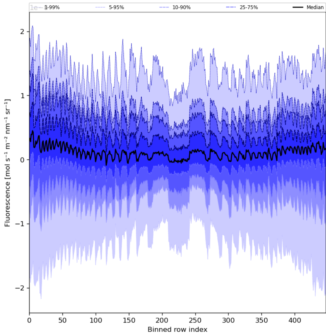
Figure 57: Along track statistics of “Fluorescence” for 2023-10-06 to 2023-10-08
