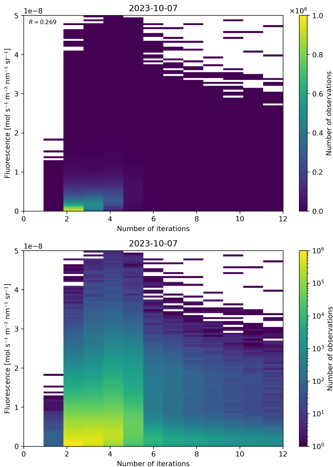
Figure 107: Scatter density plot of “Number of iterations” against “Fluorescence” for 2023-10-06 to 2023-10-08.
