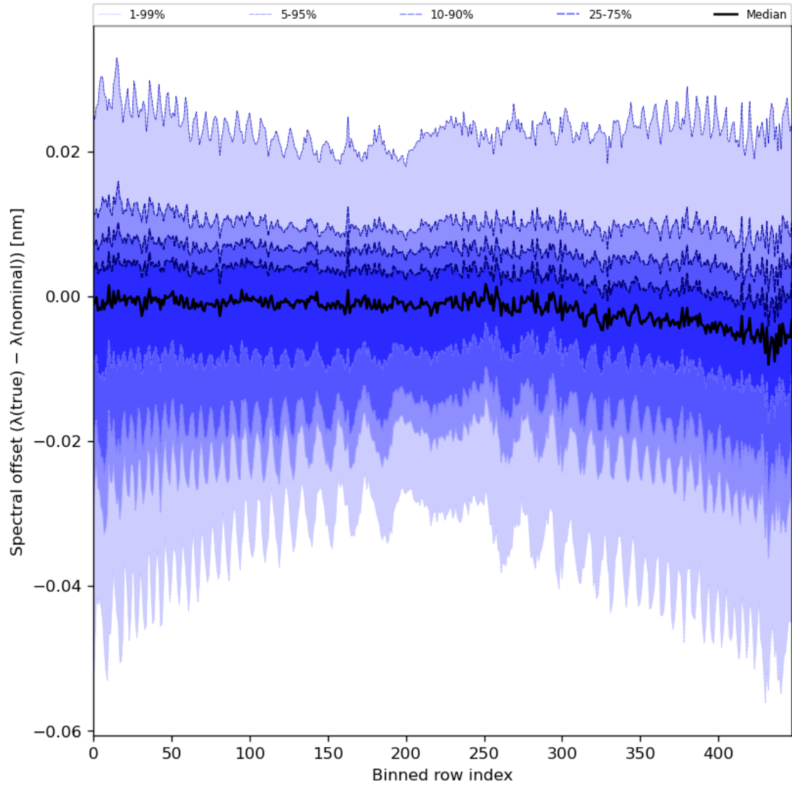
Figure 62: Along track statistics of “Spectral offset ( \lambda(\text{true}) - \lambda(\text{nominal}) )” for 2023-10-06 to 2023-10-08
