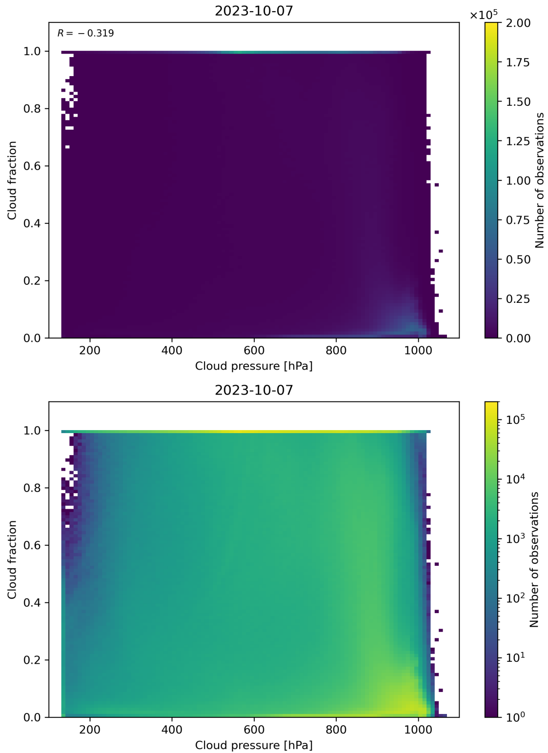
Figure 87: Scatter density plot of “Cloud pressure” against “Cloud fraction” for 2023-10-06 to 2023-10-08.
