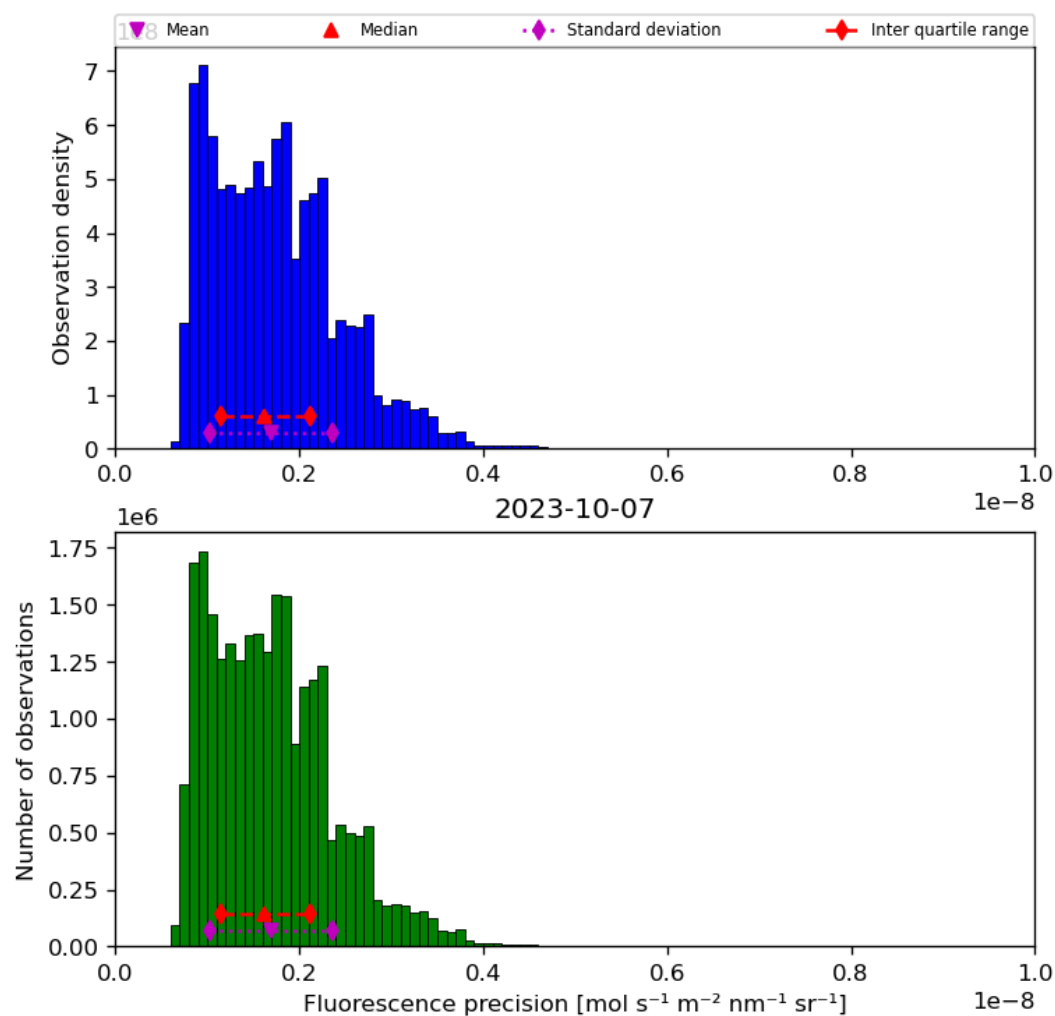
Figure 41: Histogram of “Fluorescence precision” for 2023-10-06 to 2023-10-08
