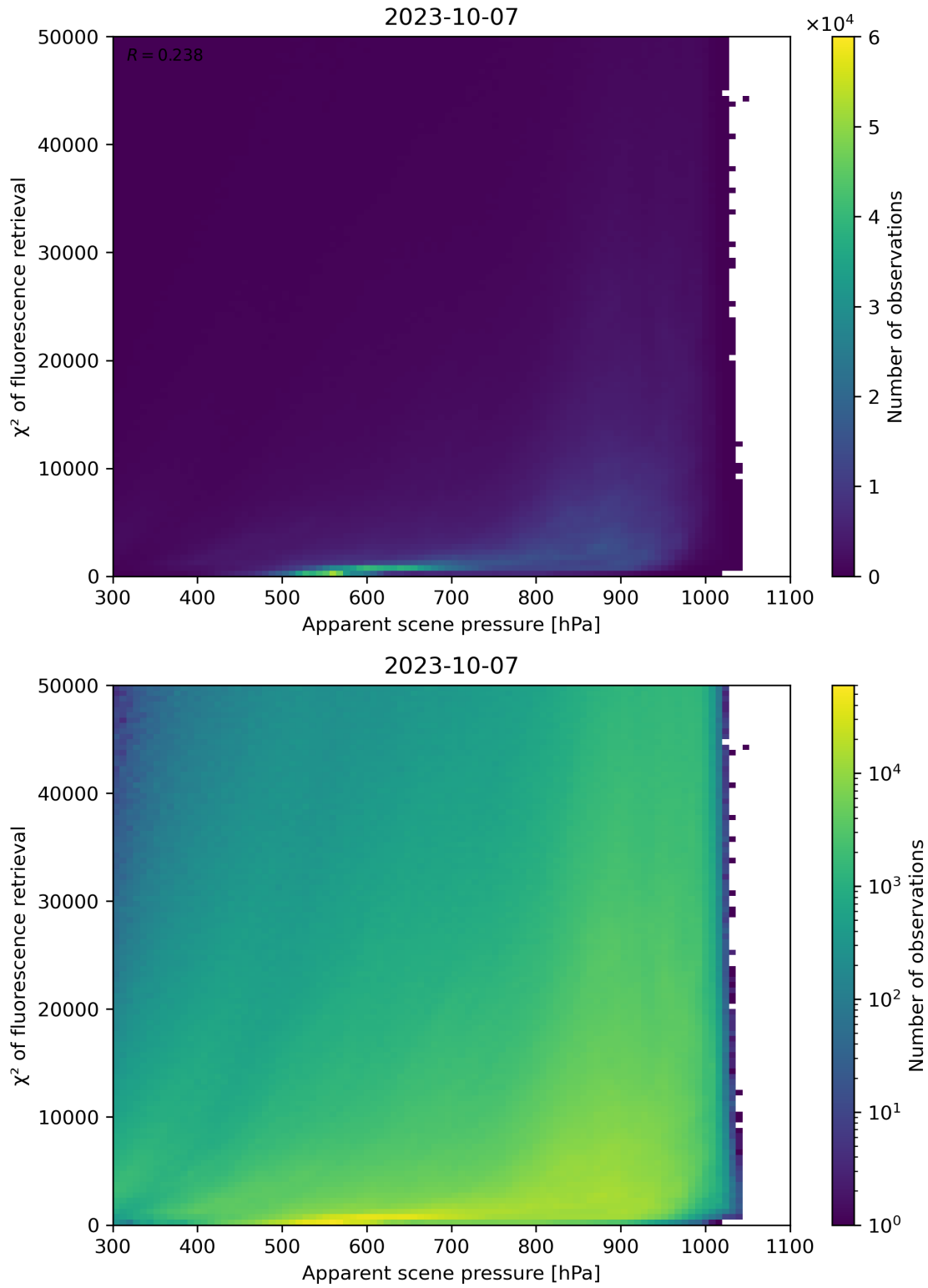
Figure 64: Scatter density plot of “Apparent scene pressure” against “ \chi^2 of fluorescence retrieval” for 2023-10-06 to 2023-10-08.
