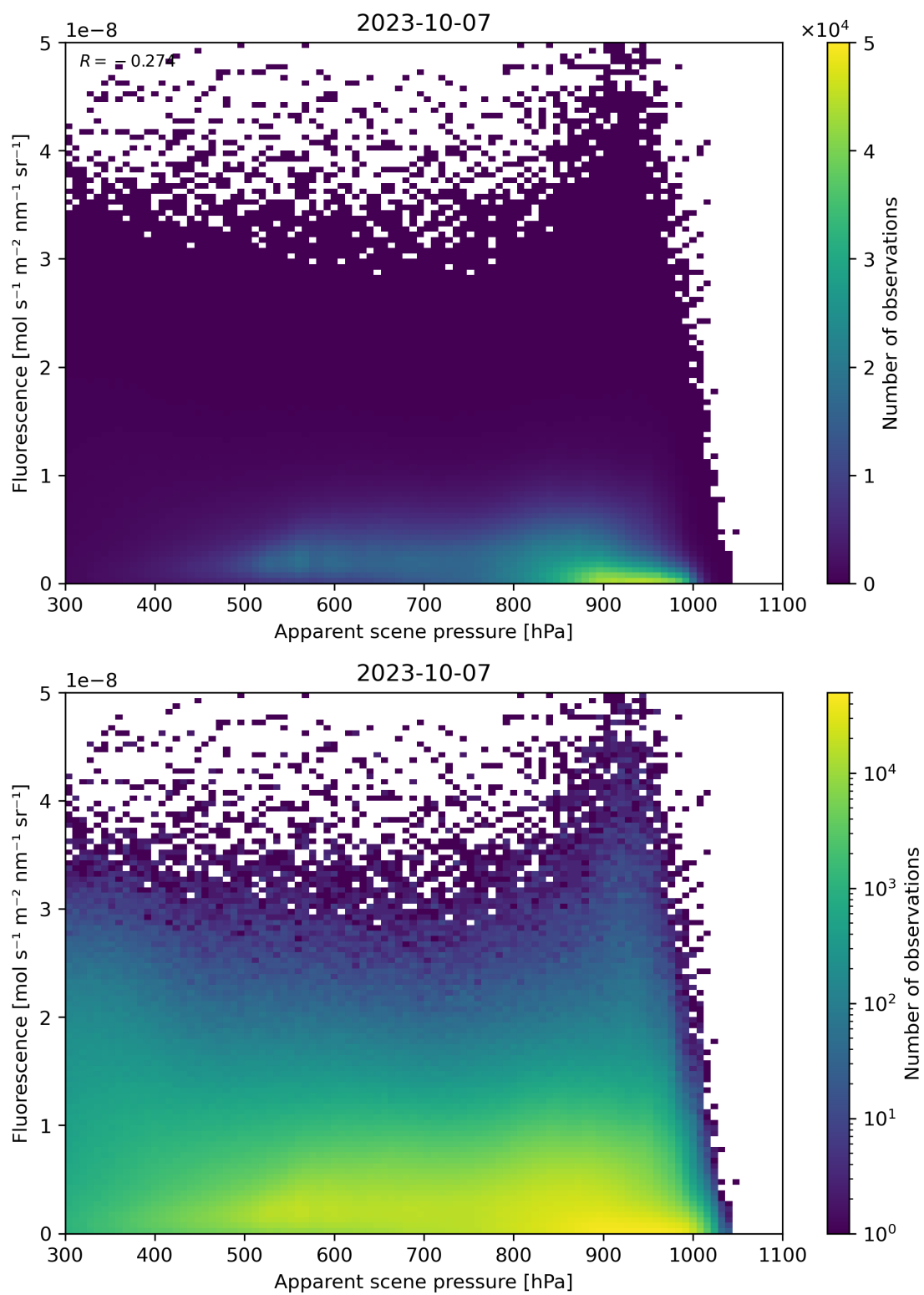
Figure 65: Scatter density plot of “Apparent scene pressure” against “Fluorescence” for 2023-10-06 to 2023-10-08.
