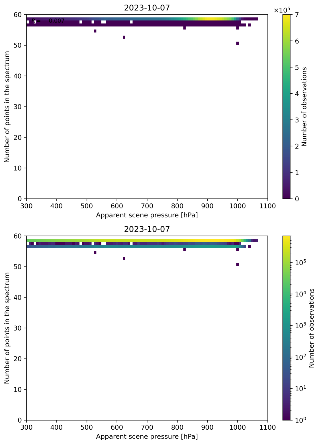
Figure 67: Scatter density plot of “Apparent scene pressure” against “Number of points in the spectrum” for 2023-10-06 to 2023-10-08.
