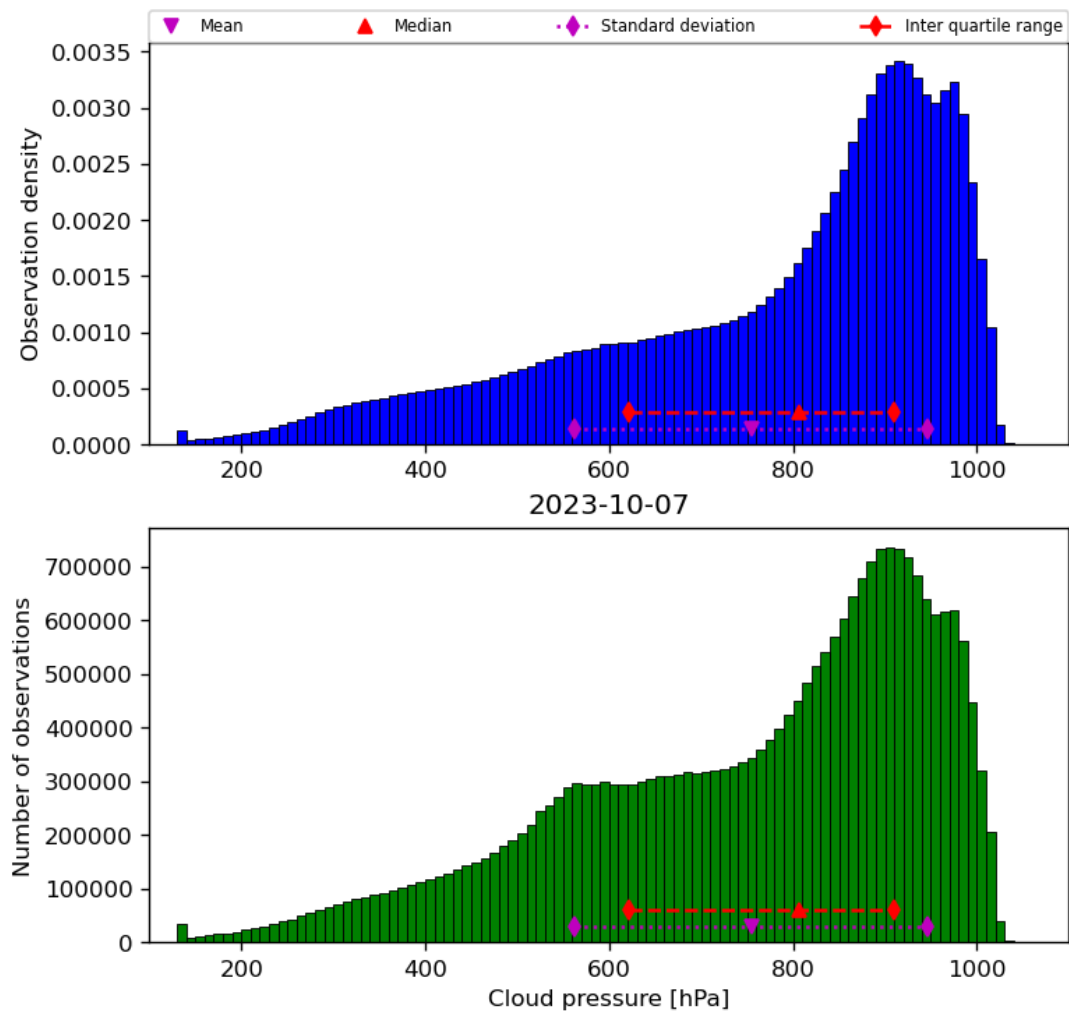
Figure 30: Histogram of “Cloud pressure” for 2023-10-06 to 2023-10-08
