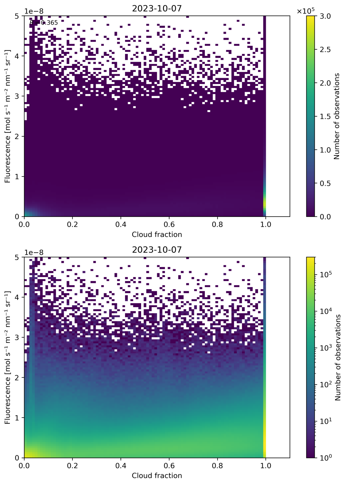
Figure 79: Scatter density plot of “Cloud fraction” against “Fluorescence” for 2023-10-06 to 2023-10-08.
