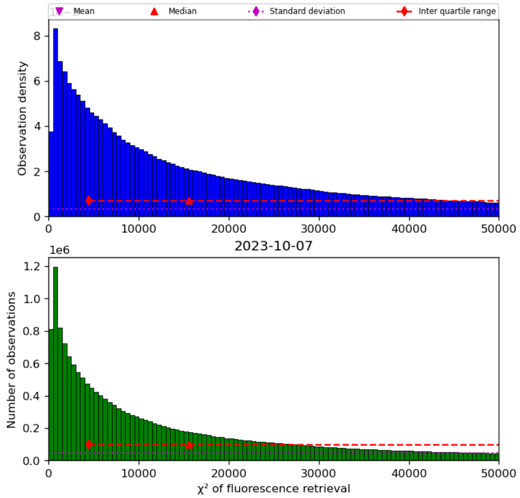
Figure 42: Histogram of “ \chi^2 of fluorescence retrieval” for 2023-10-06 to 2023-10-08
