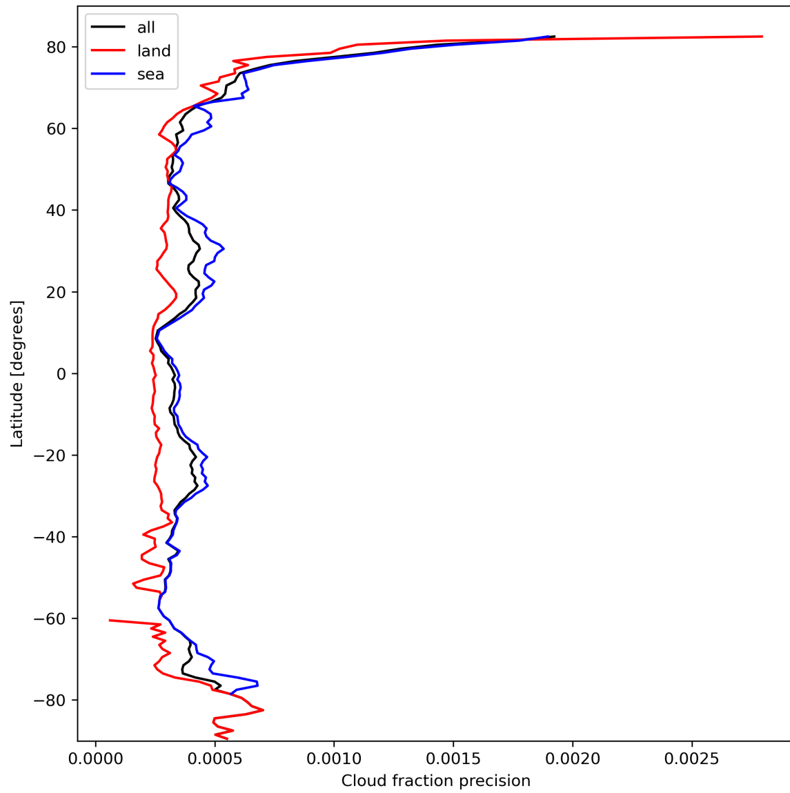
Figure 16: Zonal average of “Cloud fraction precision” for 2023-10-06 to 2023-10-08.
