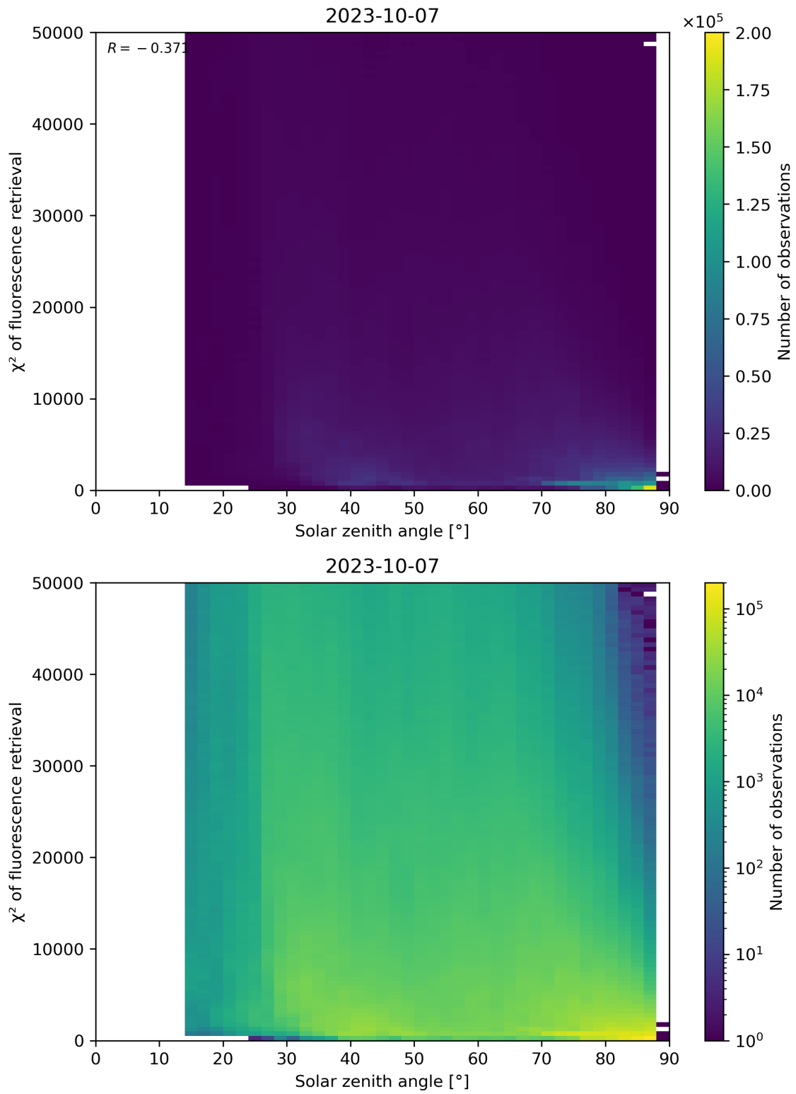
Figure 120: Scatter density plot of “Solar zenith angle” against “ \chi^2 of fluorescence retrieval” for 2023-10-06 to 2023-10-08.
