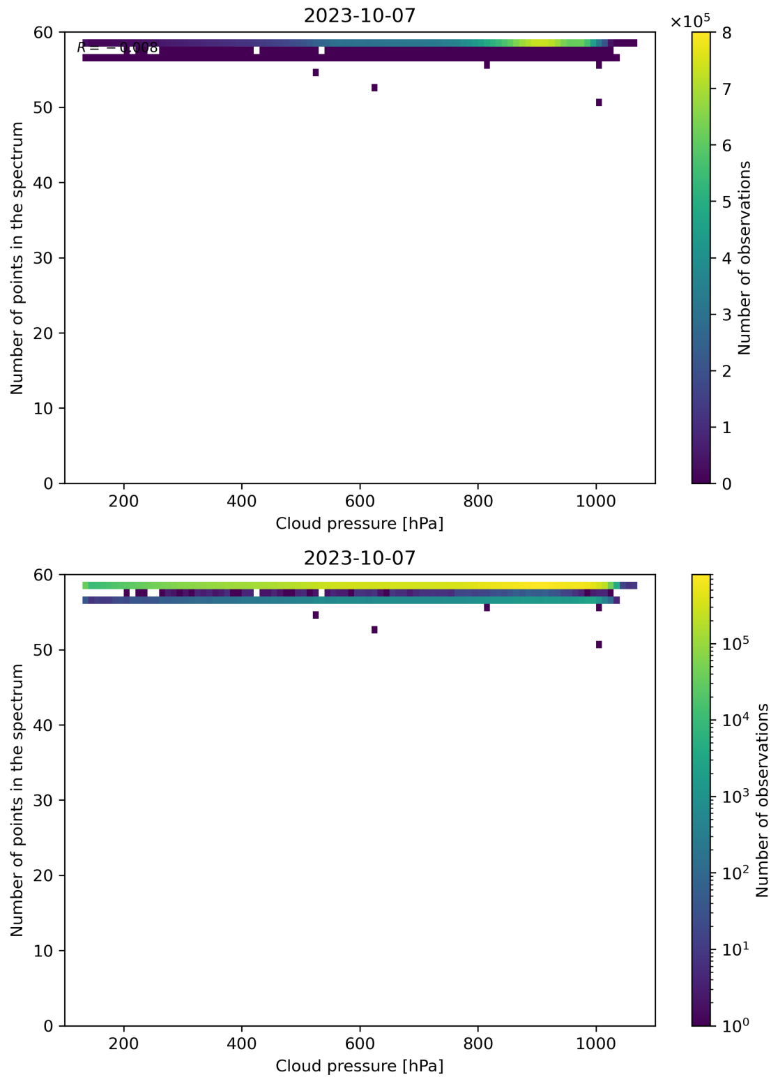
Figure 90: Scatter density plot of “Cloud pressure” against “Number of points in the spectrum” for 2023-10-06 to 2023-10-08.
