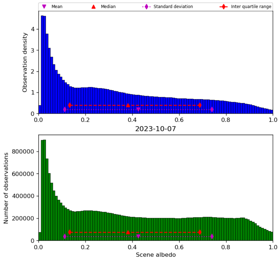
Figure 34: Histogram of “Scene albedo” for 2023-10-06 to 2023-10-08
