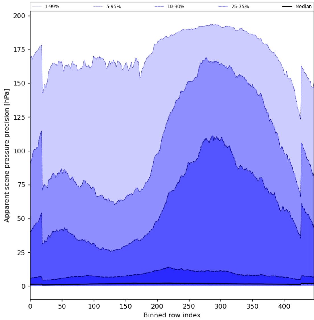
Figure 54: Along track statistics of “Apparent scene pressure precision” for 2023-10-06 to 2023-10-08
