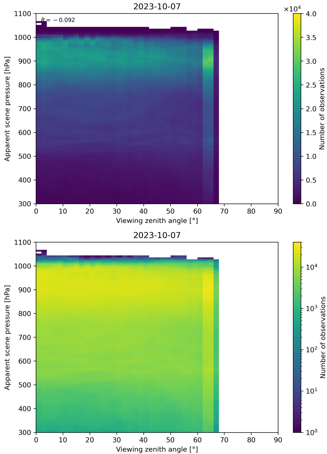
Figure 129: Scatter density plot of “Viewing zenith angle” against “Apparent scene pressure” for 2023-10-06 to 2023-10-08.
