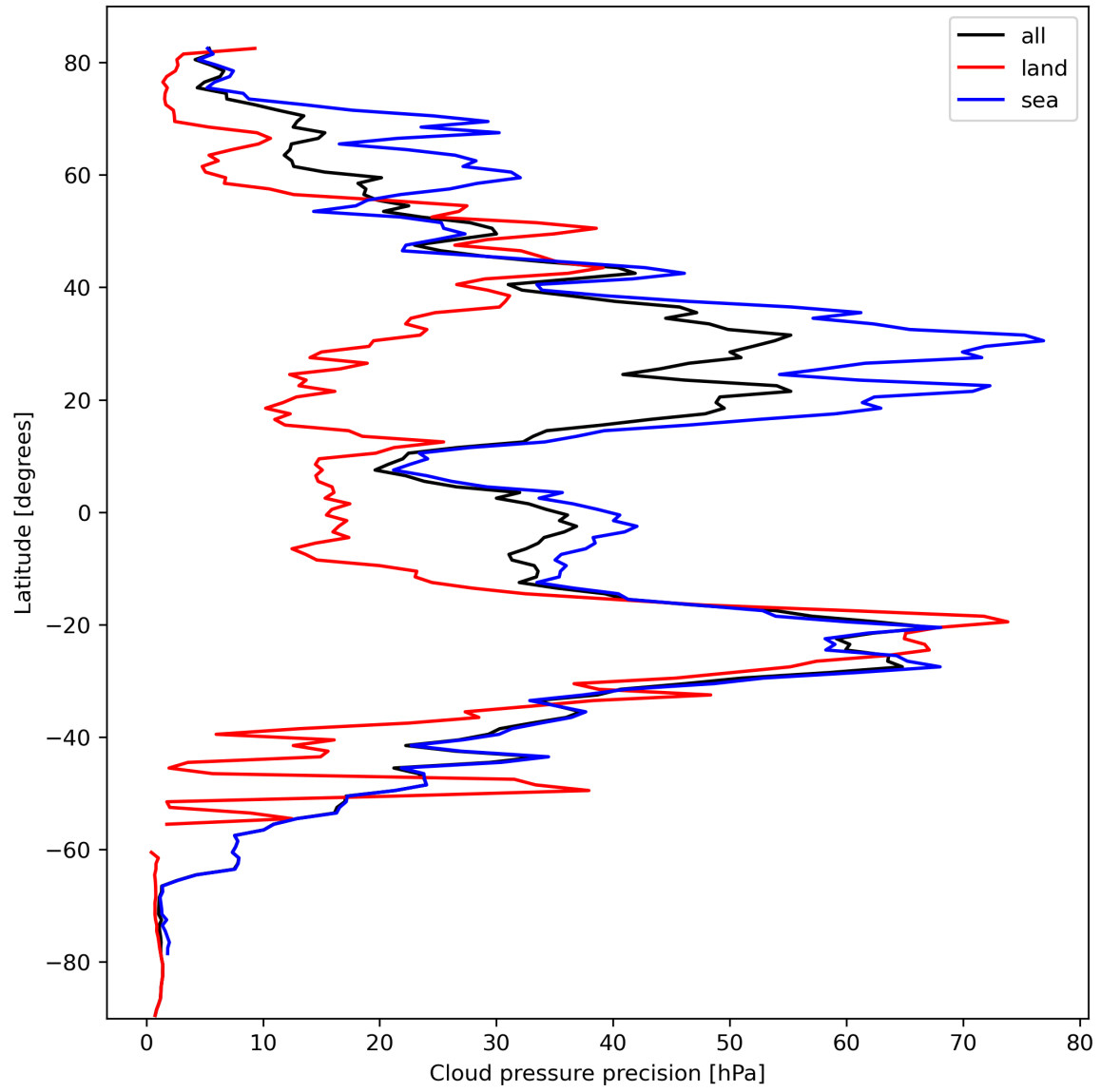
Figure 14: Zonal average of “Cloud pressure precision” for 2023-10-06 to 2023-10-08.
