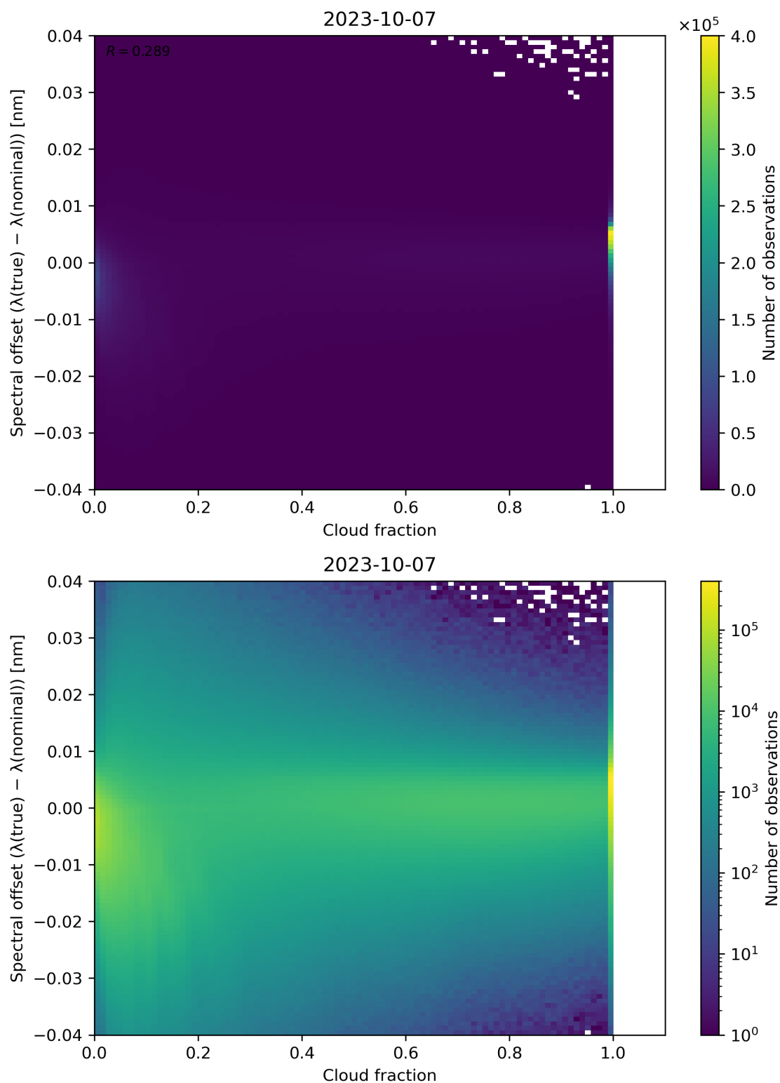
Figure 83: Scatter density plot of “Cloud fraction” against “Spectral offset ( \lambda(\text{true}) - \lambda(\text{nominal}) )” for 2023-10-06 to 2023-10-08.
