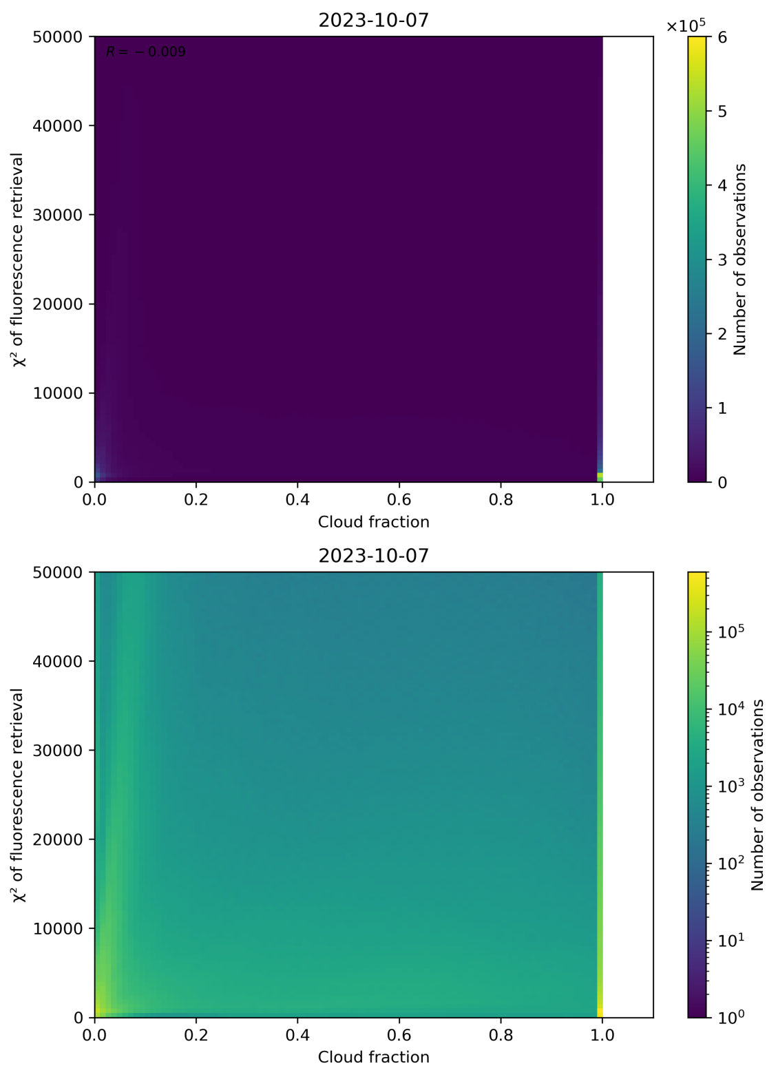
Figure 78: Scatter density plot of “Cloud fraction” against “ \chi^2 of fluorescence retrieval” for 2023-10-06 to 2023-10-08.
