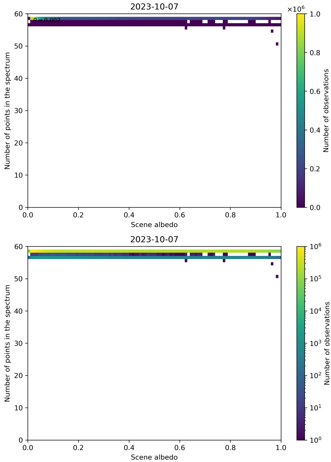
Figure 116: Scatter density plot of “Scene albedo” against “Number of points in the spectrum” for 2023-10-06 to 2023-10-08.
