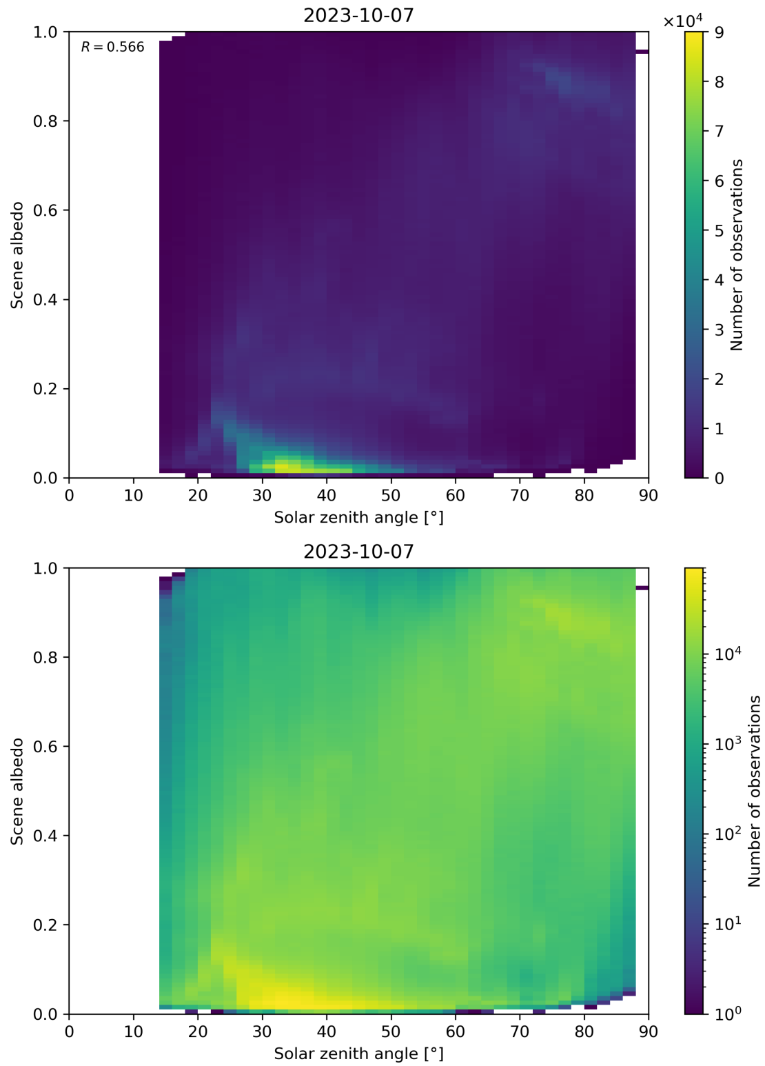
Figure 127: Scatter density plot of “Solar zenith angle” against “Scene albedo” for 2023-10-06 to 2023-10-08.
