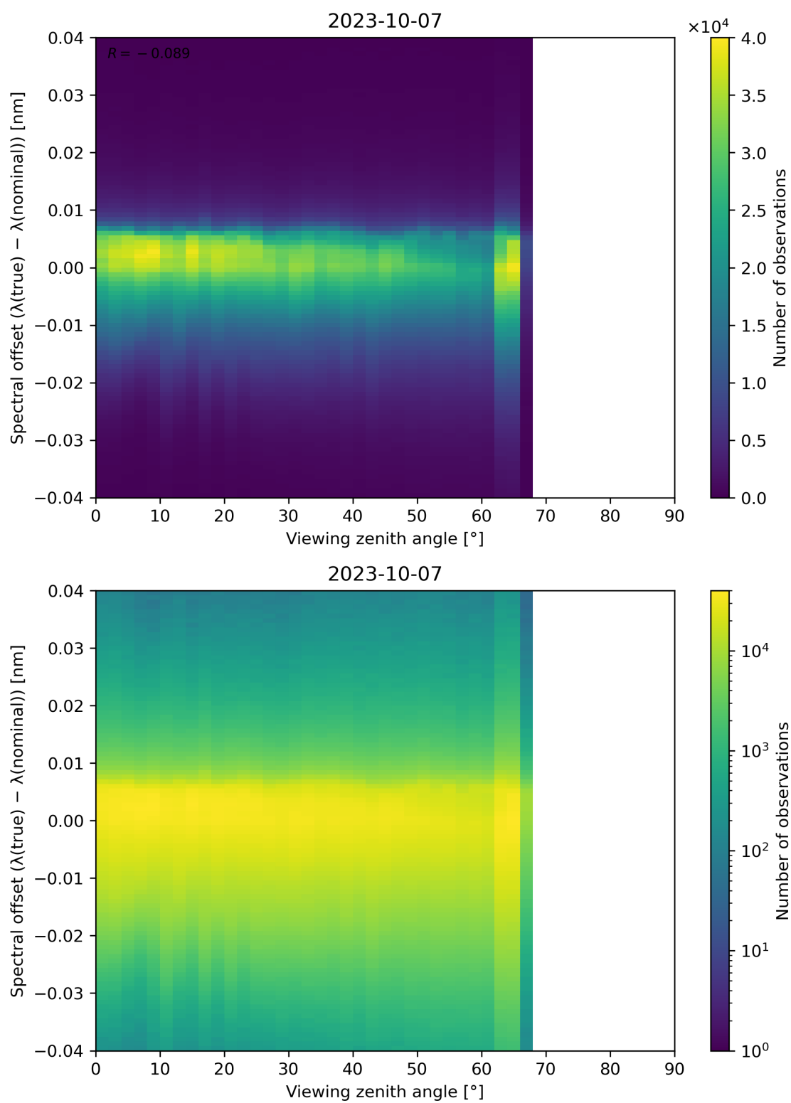
Figure 140: Scatter density plot of “Viewing zenith angle” against “Spectral offset ( \lambda(\text{true}) - \lambda(\text{nominal}) )” for 2023-10-06 to 2023-10-08.
