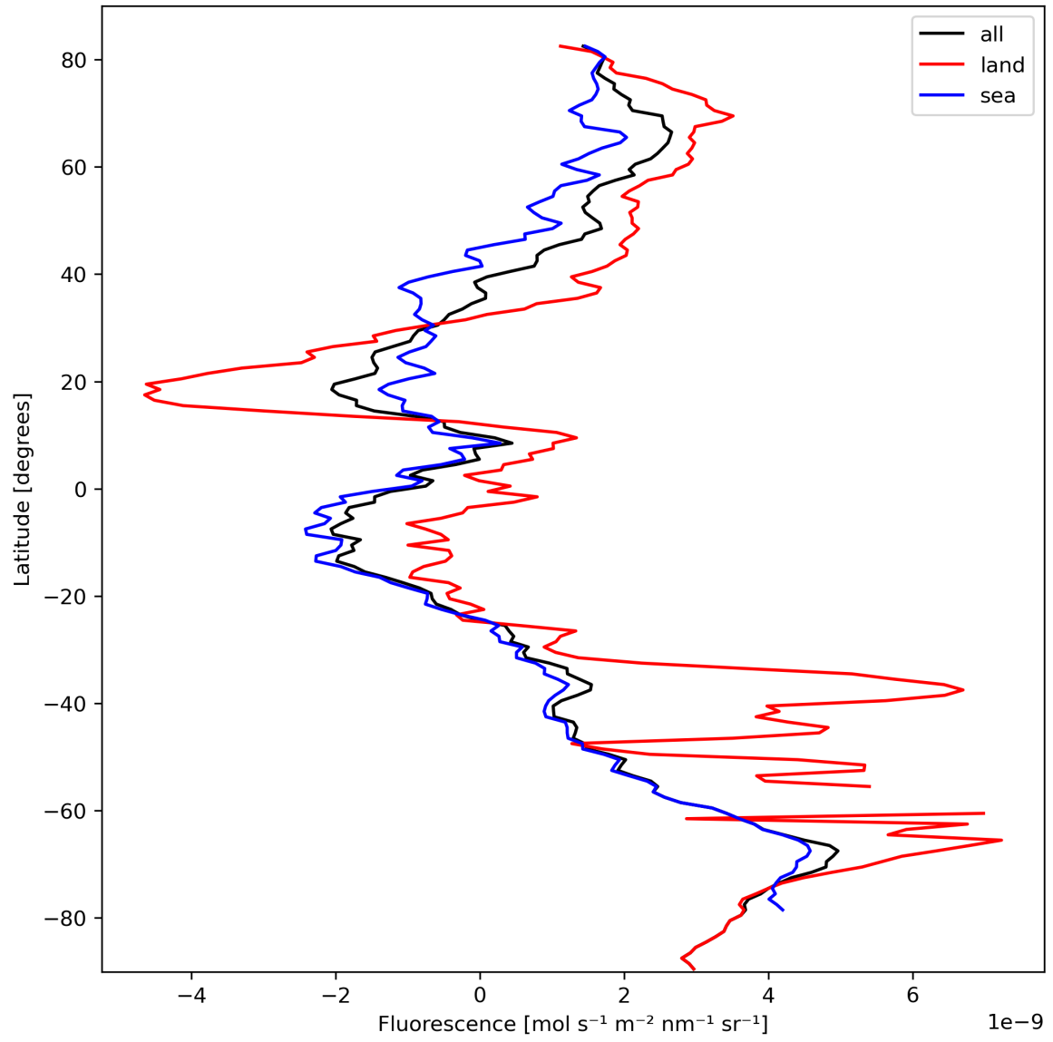
Figure 23: Zonal average of “Fluorescence” for 2023-10-06 to 2023-10-08.
