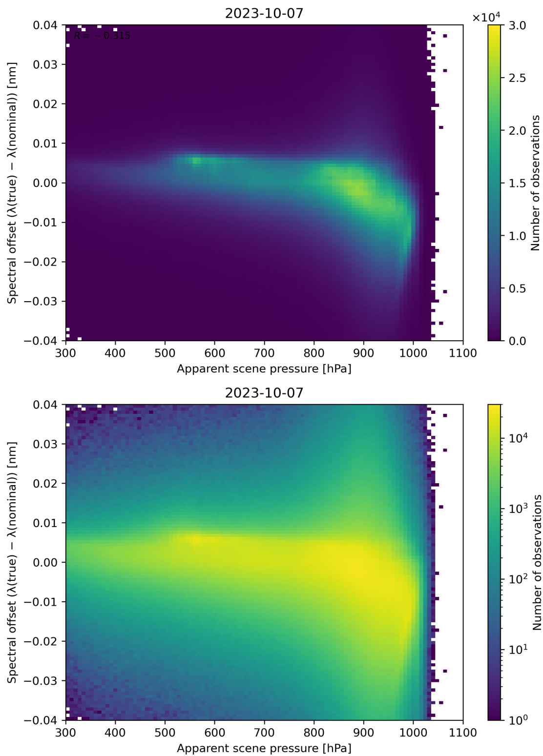
Figure 68: Scatter density plot of “Apparent scene pressure” against “Spectral offset ( \lambda(\text{true}) - \lambda(\text{nominal}) )” for 2023-10-06 to 2023-10-08.
