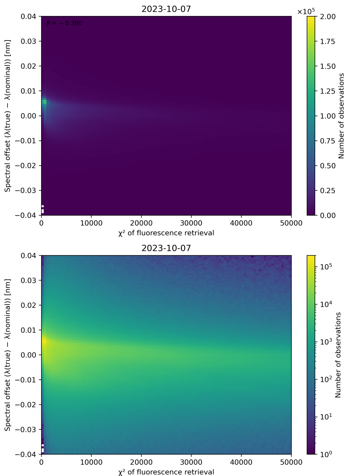
Figure 72: Scatter density plot of " \chi^2 of fluorescence retrieval" against "Spectral offset ( \lambda(\text{true}) - \lambda(\text{nominal}) )" for 2023-10-06 to 2023-10-08.
