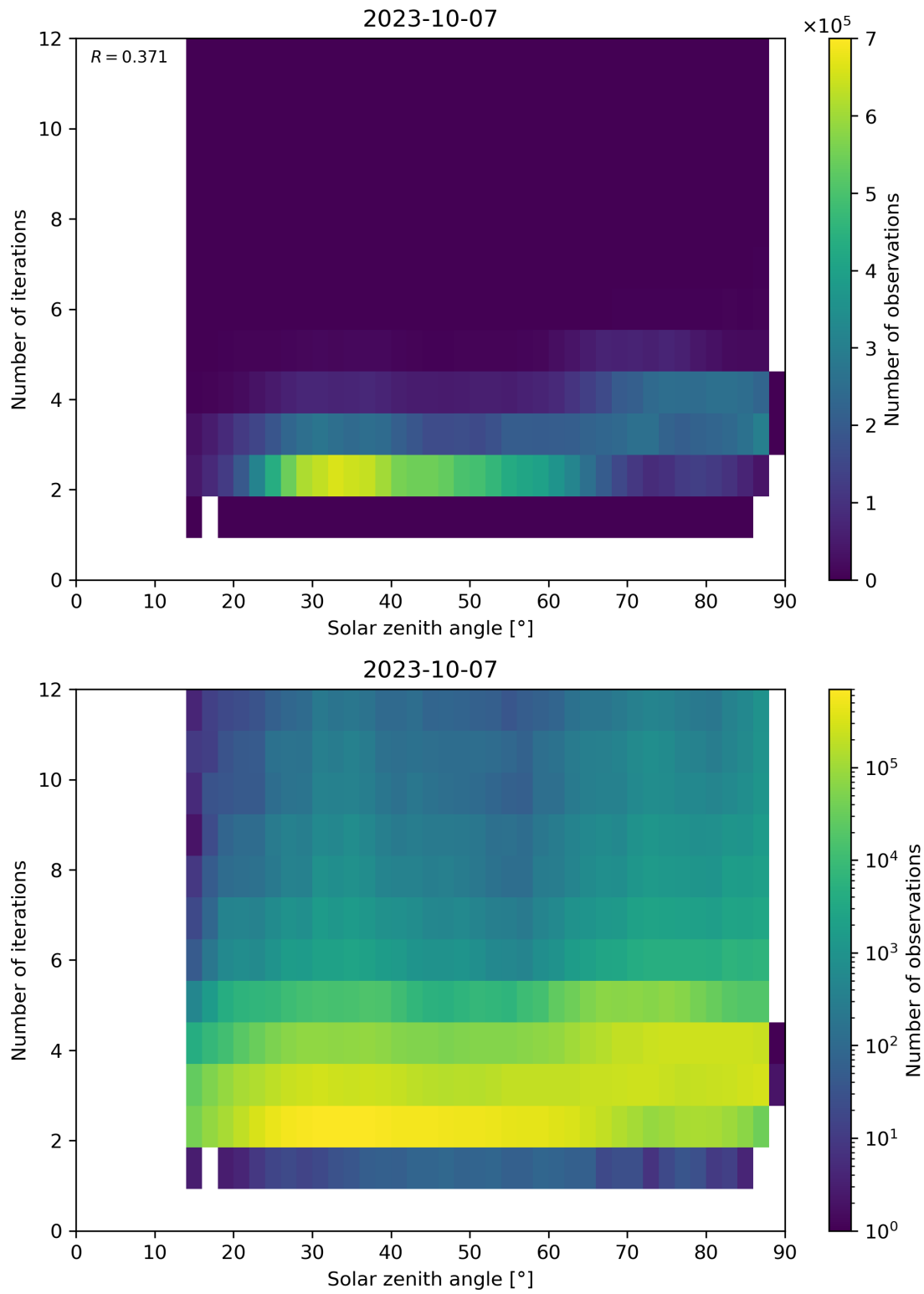
Figure 125: Scatter density plot of “Solar zenith angle” against “Number of iterations” for 2023-10-06 to 2023-10-08.
