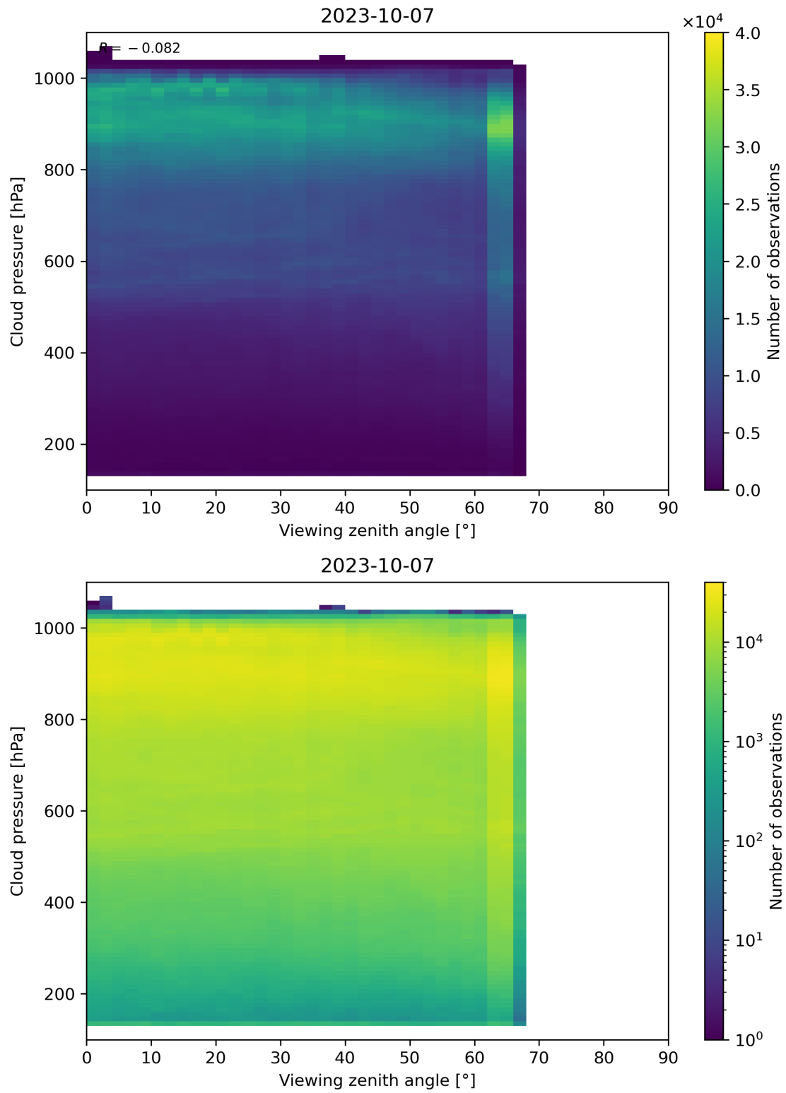
Figure 133: Scatter density plot of “Viewing zenith angle” against “Cloud pressure” for 2023-10-06 to 2023-10-08.
