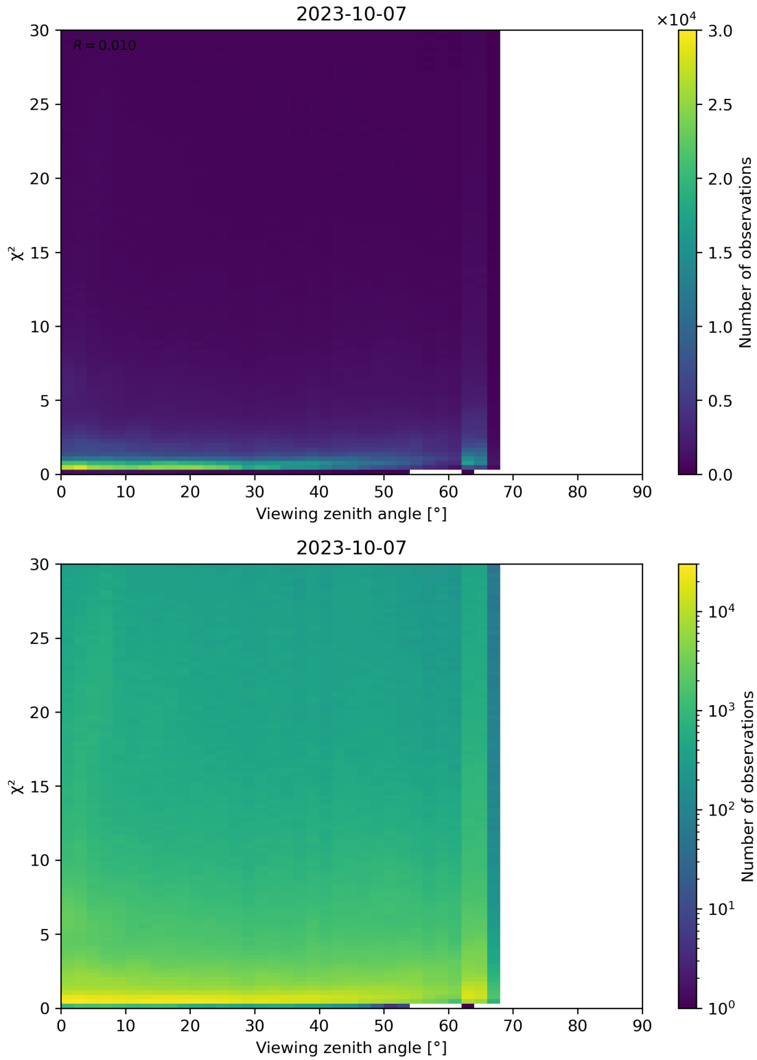
Figure 130: Scatter density plot of “Viewing zenith angle” against “ \chi^2 ” for 2023-10-06 to 2023-10-08.
