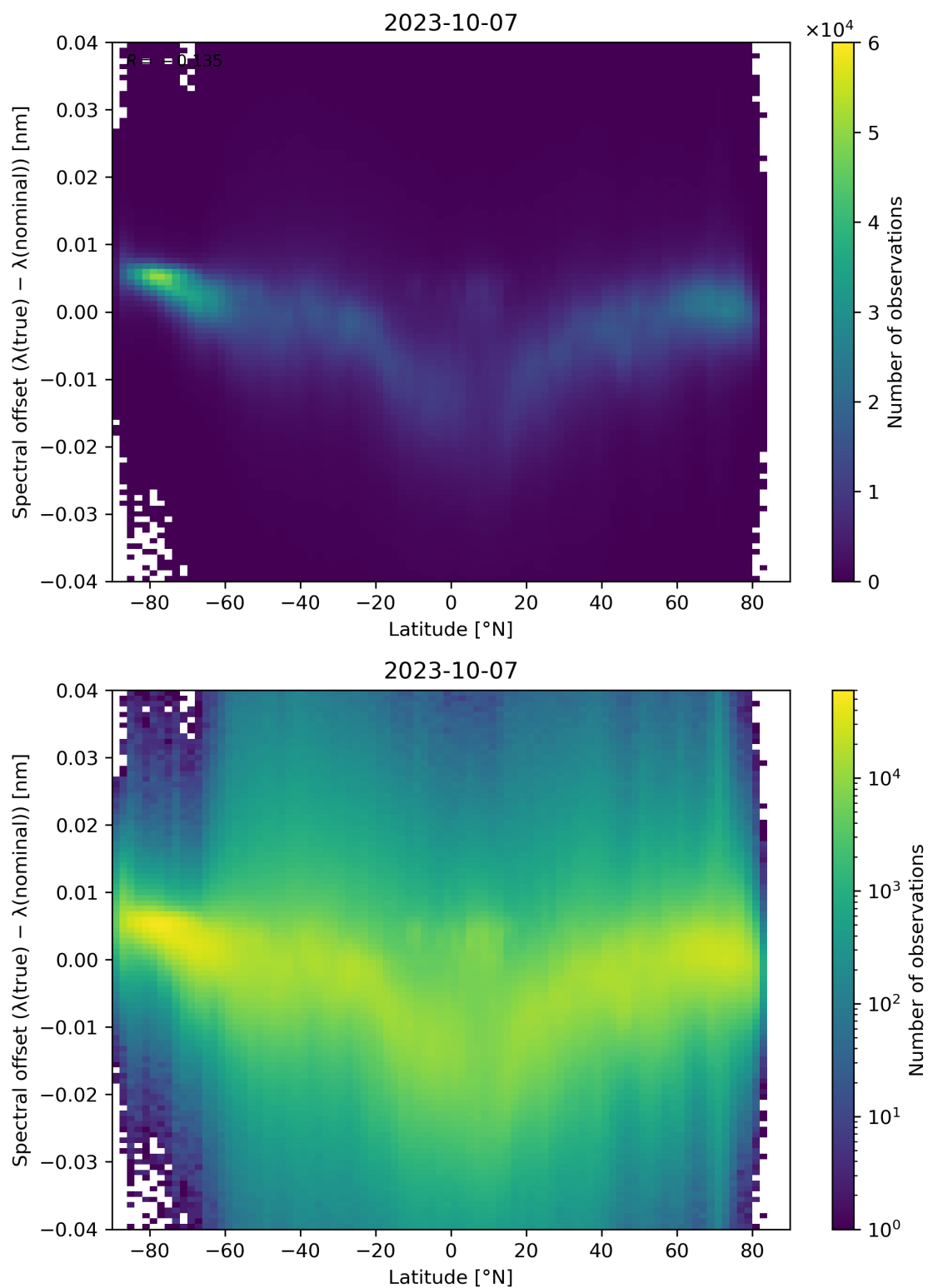
Figure 105: Scatter density plot of “Latitude” against “Spectral offset ( \lambda(\text{true}) - \lambda(\text{nominal}) )” for 2023-10-06 to 2023-10-08.
