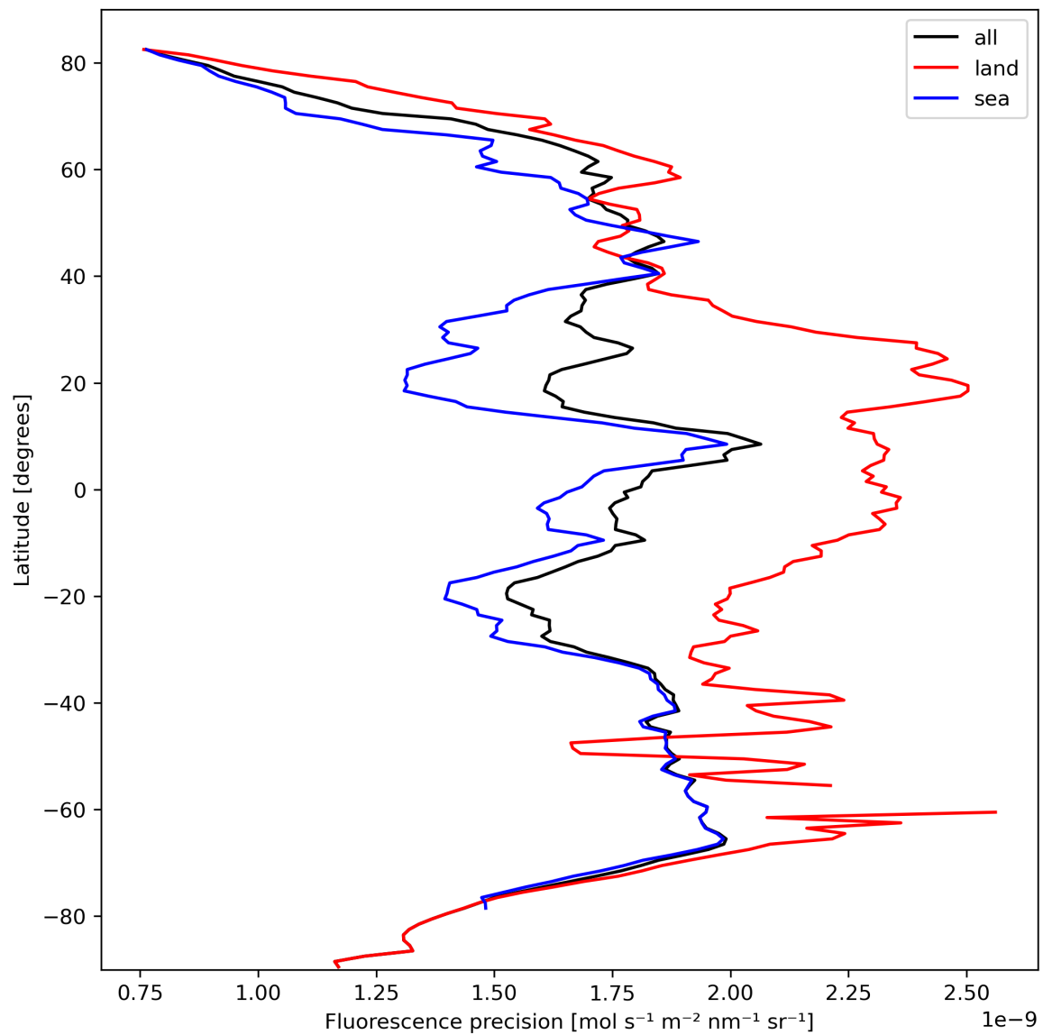
Figure 24: Zonal average of “Fluorescence precision” for 2023-10-06 to 2023-10-08.
