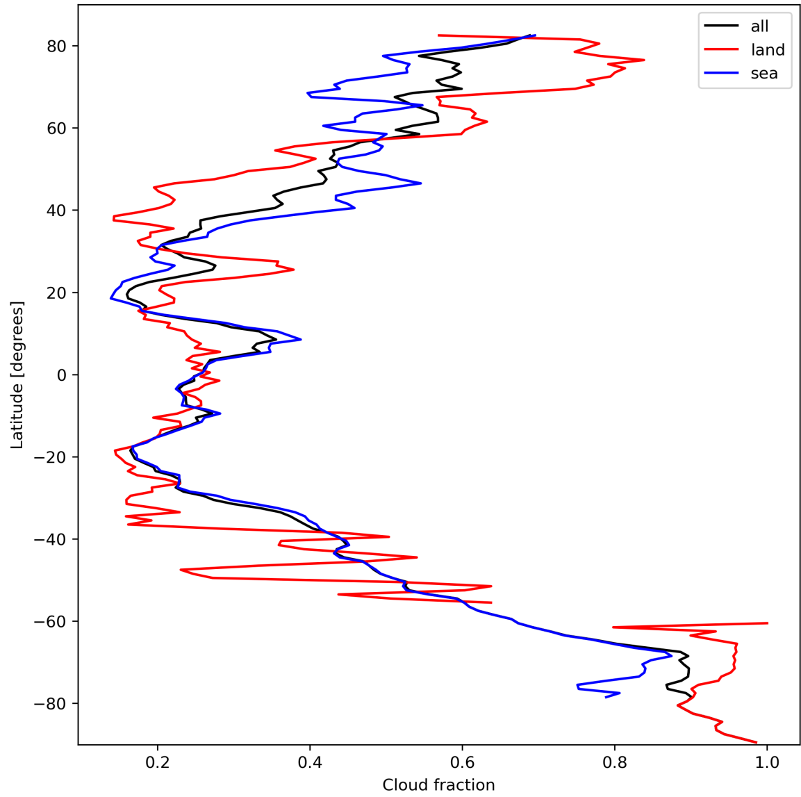
Figure 15: Zonal average of “Cloud fraction” for 2023-10-06 to 2023-10-08.
