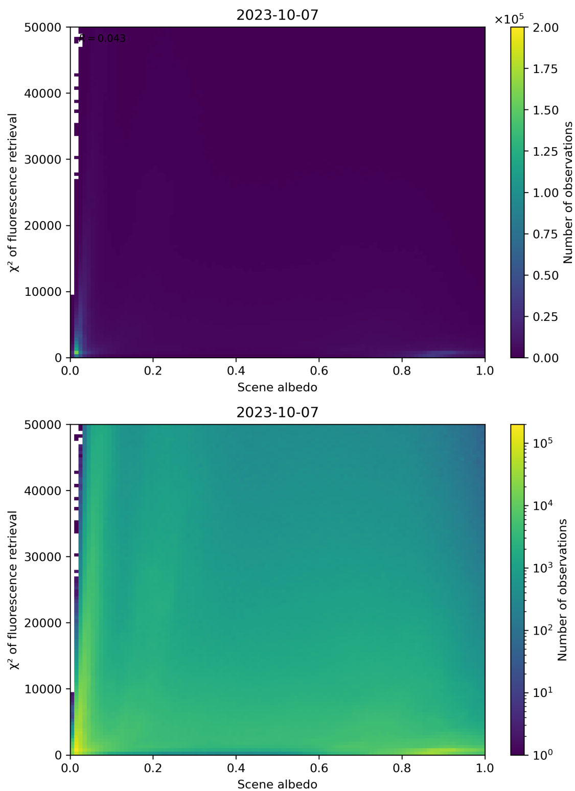
Figure 113: Scatter density plot of “Scene albedo” against “ \chi^2 of fluorescence retrieval” for 2023-10-06 to 2023-10-08.
