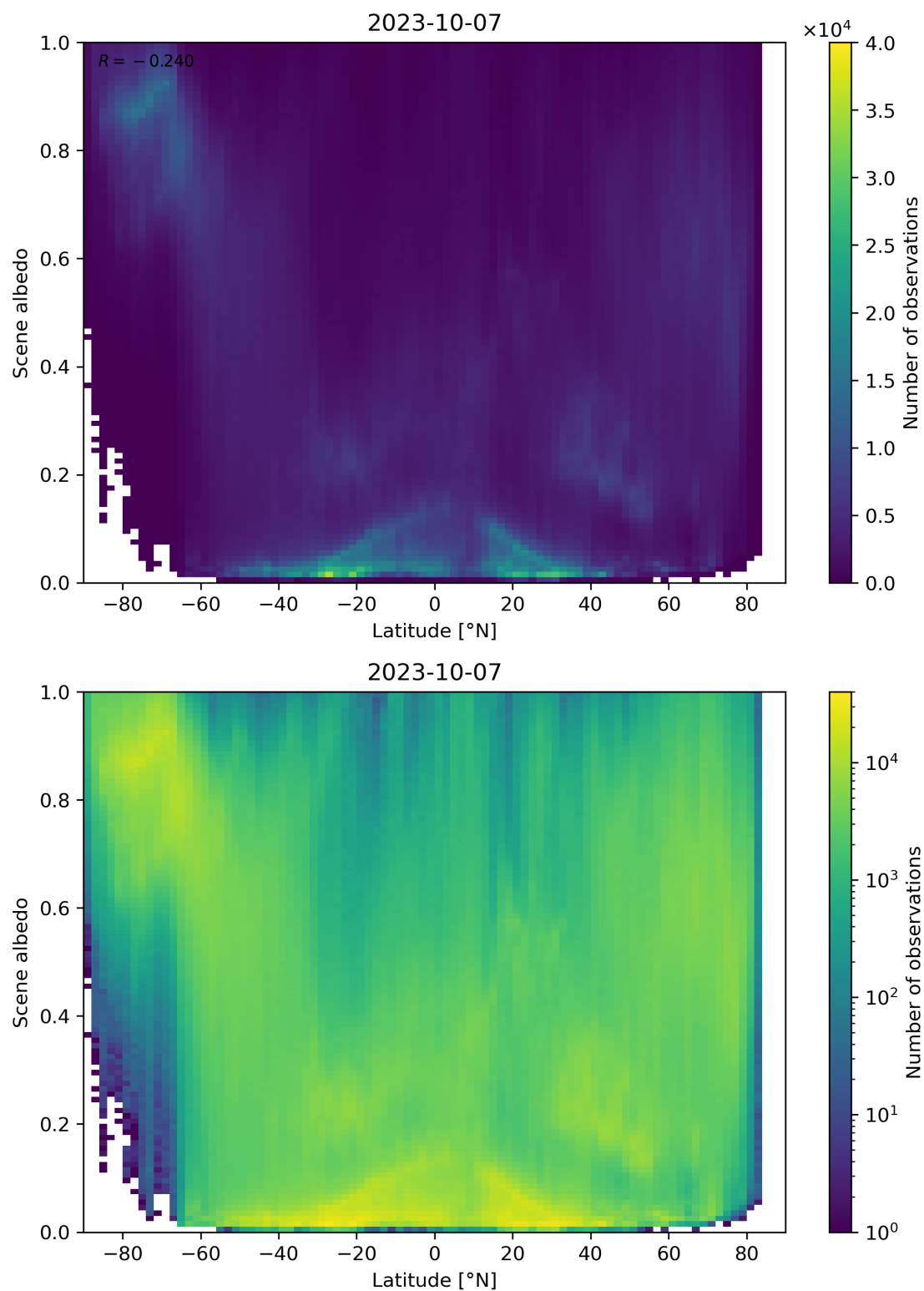
Figure 104: Scatter density plot of “Latitude” against “Scene albedo” for 2023-10-06 to 2023-10-08.
