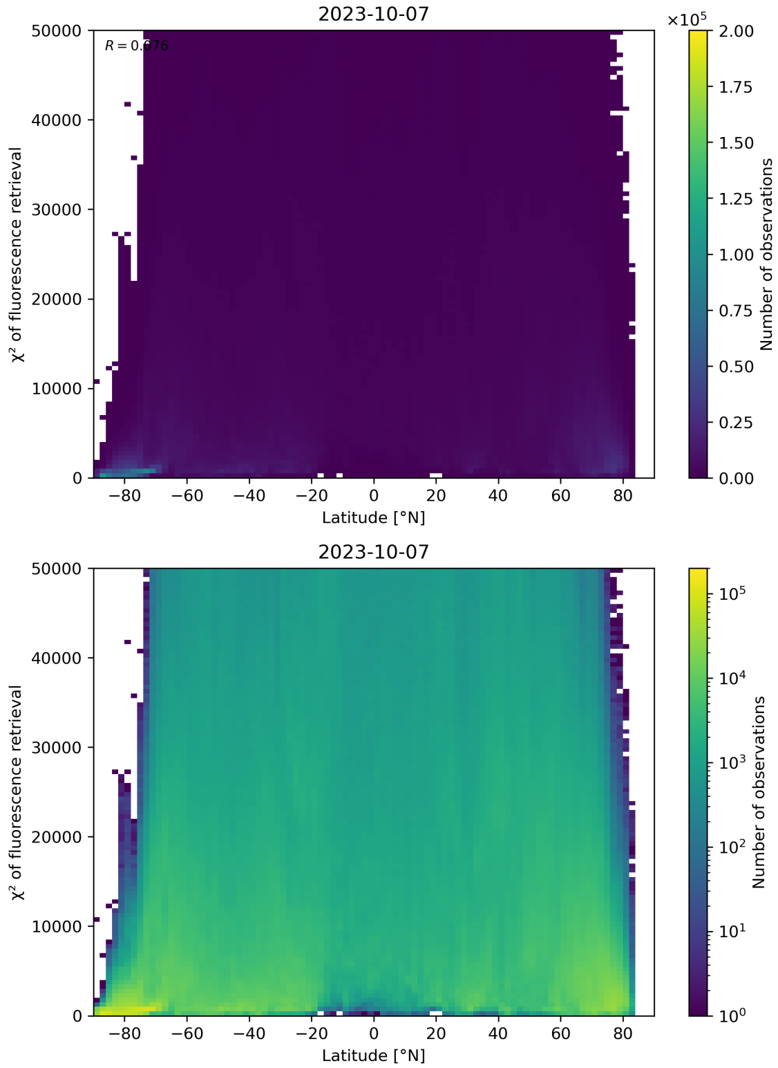
Figure 98: Scatter density plot of “Latitude” against “ \chi^2 of fluorescence retrieval” for 2023-10-06 to 2023-10-08.
