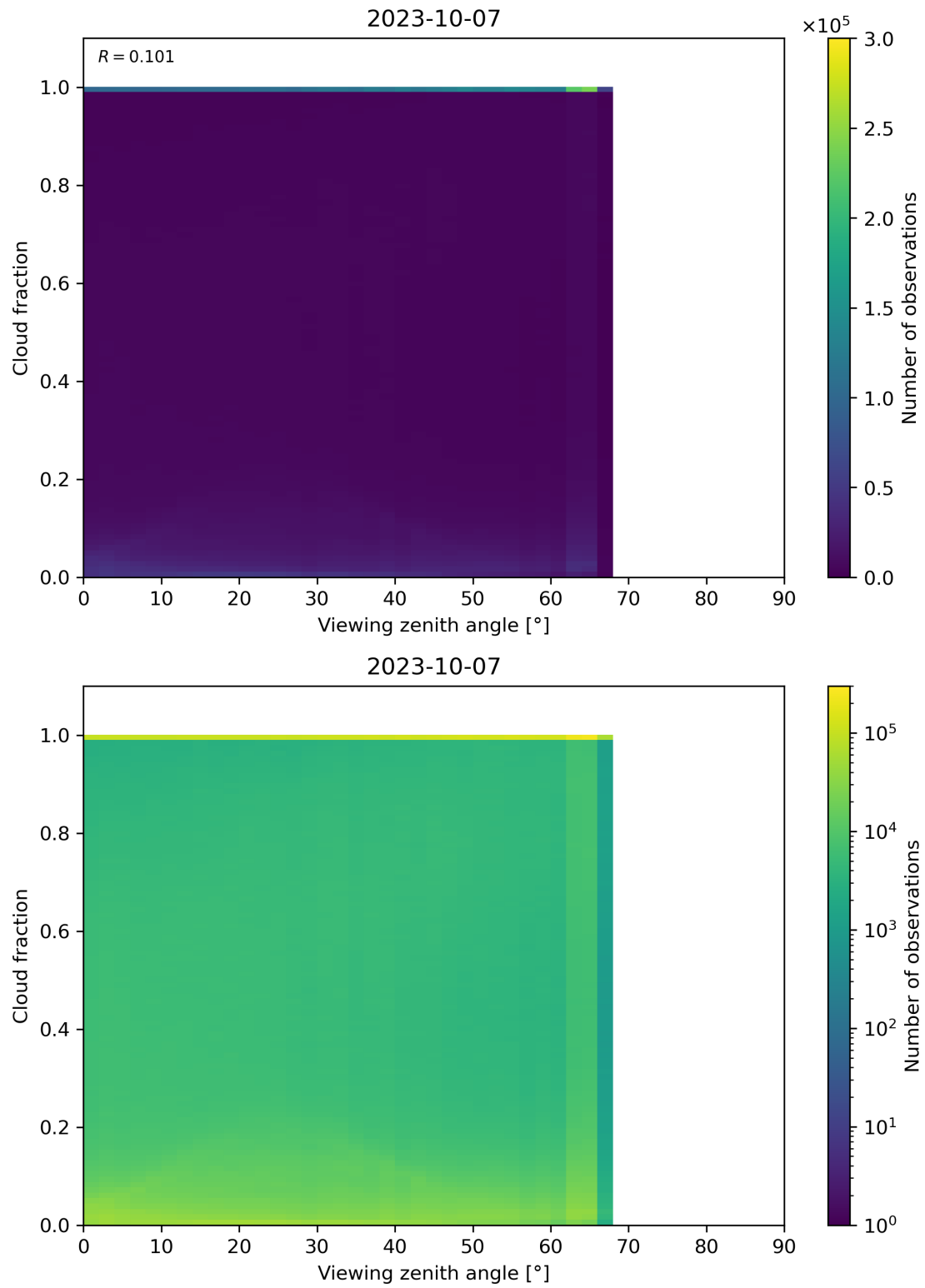
Figure 132: Scatter density plot of “Viewing zenith angle” against “Cloud fraction” for 2023-10-06 to 2023-10-08.
