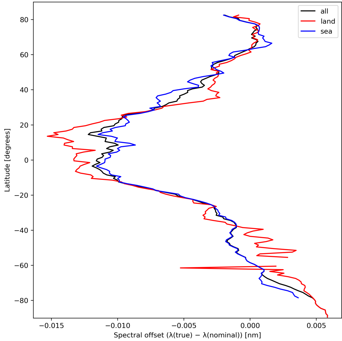
Figure 28: Zonal average of “Spectral offset ( \lambda(\text{true}) - \lambda(\text{nominal}) )” for 2023-10-06 to 2023-10-08.
