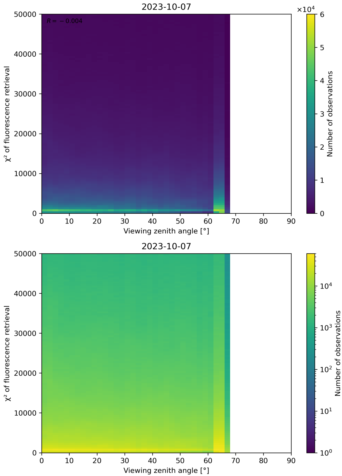
Figure 131: Scatter density plot of “Viewing zenith angle” against “ \chi^2 of fluorescence retrieval” for 2023-10-06 to 2023-10-08.
