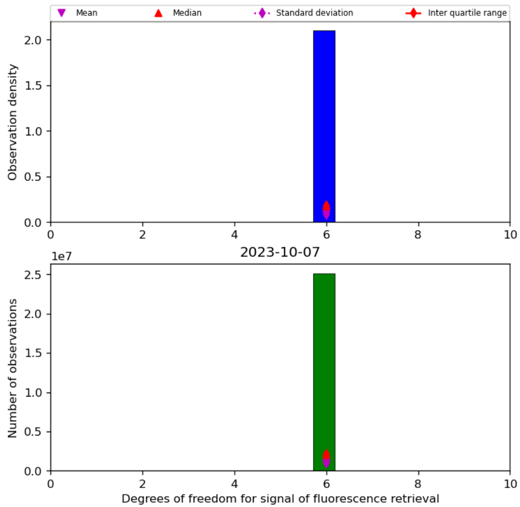
Figure 43: Histogram of “Degrees of freedom for signal of fluorescence retrieval” for 2023-10-06 to 2023-10-08
