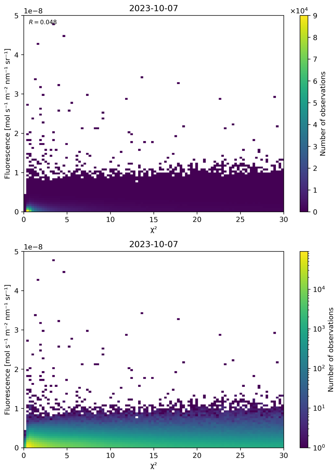
Figure 70: Scatter density plot of “ \chi^2 ” against “Fluorescence” for 2023-10-06 to 2023-10-08.
