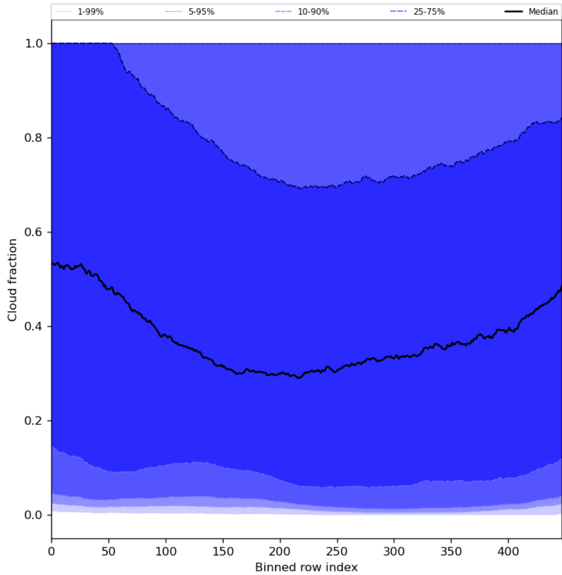
Figure 49: Along track statistics of “Cloud fraction” for 2023-10-06 to 2023-10-08
