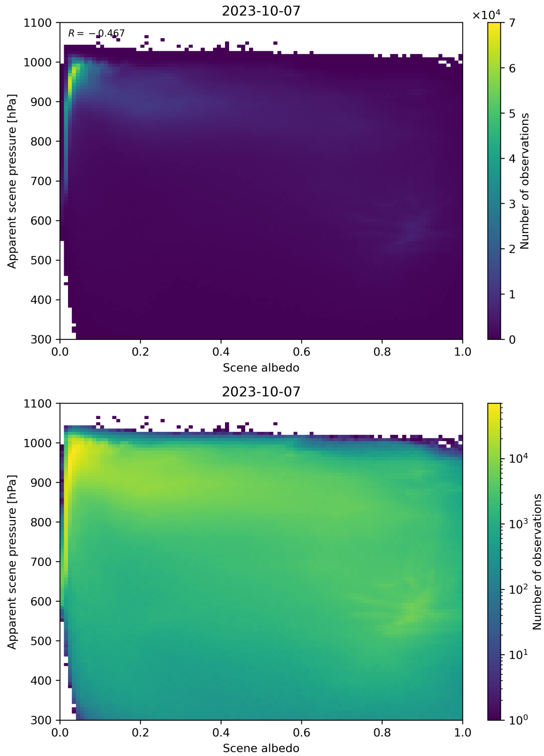
Figure 111: Scatter density plot of “Scene albedo” against “Apparent scene pressure” for 2023-10-06 to 2023-10-08.
