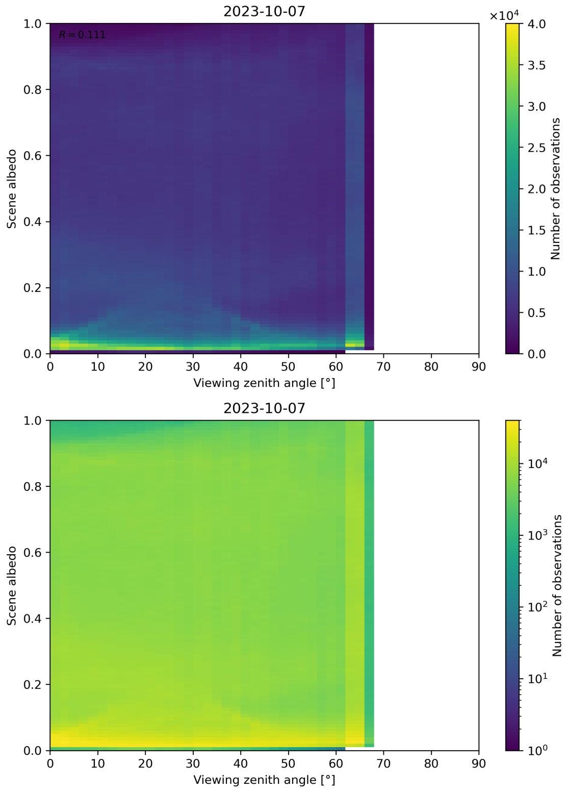
Figure 138: Scatter density plot of “Viewing zenith angle” against “Scene albedo” for 2023-10-06 to 2023-10-08.
