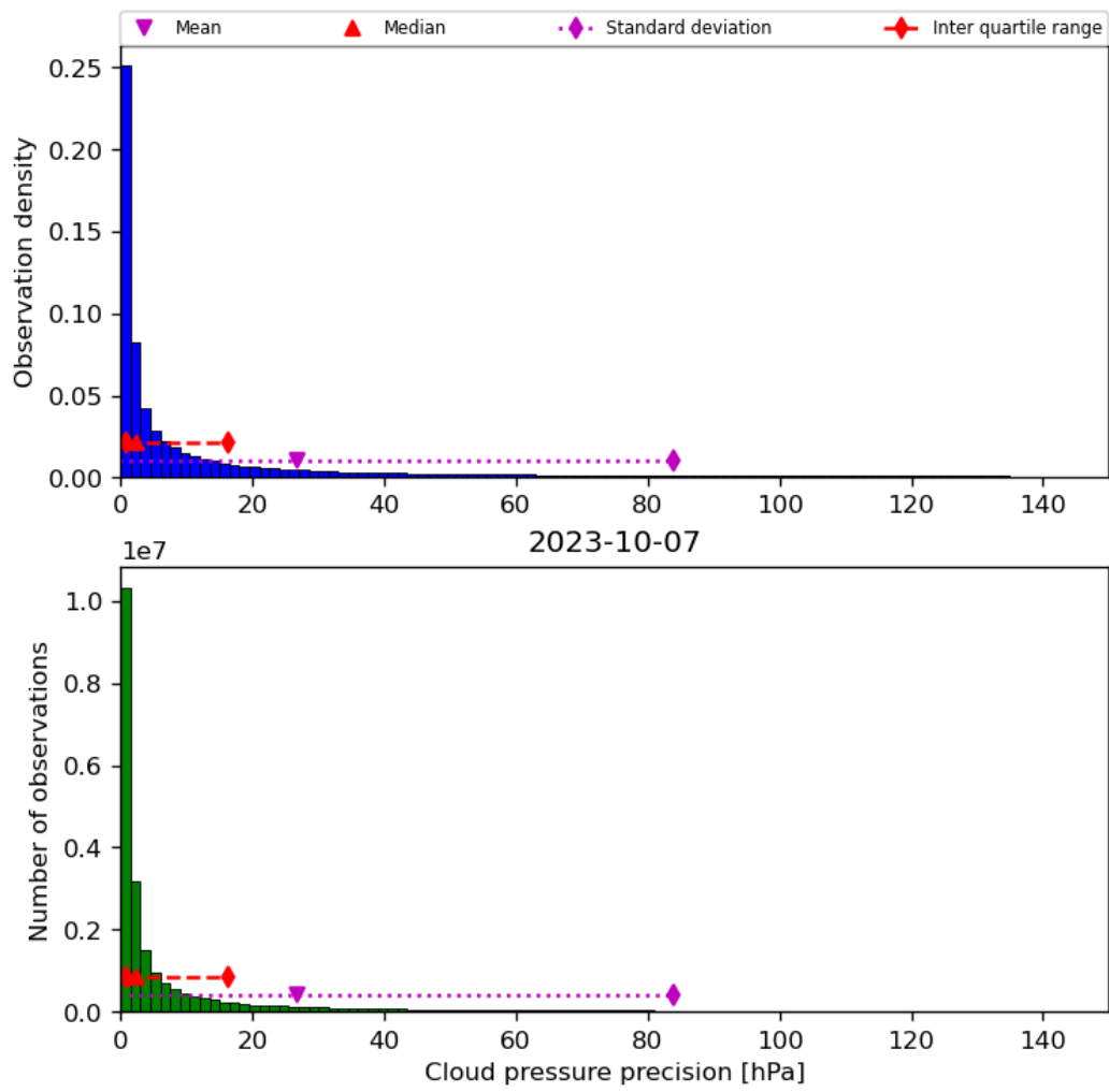
Figure 31: Histogram of “Cloud pressure precision” for 2023-10-06 to 2023-10-08
