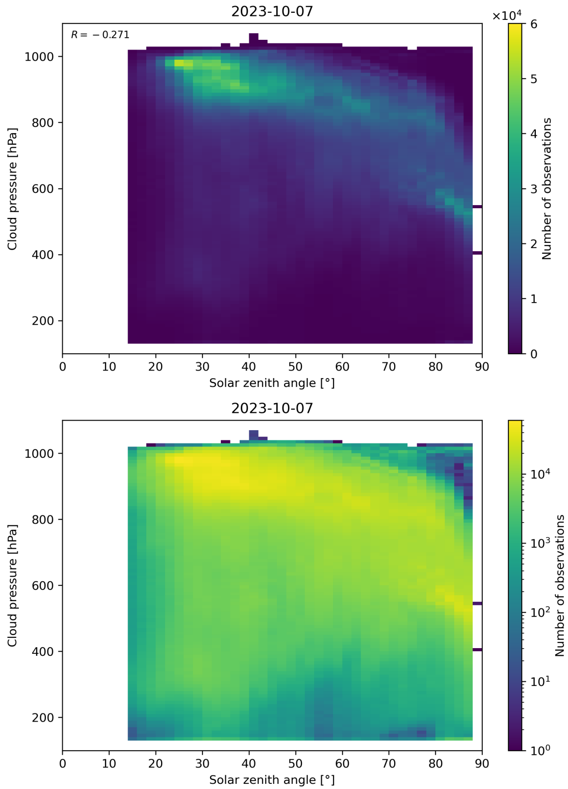
Figure 122: Scatter density plot of “Solar zenith angle” against “Cloud pressure” for 2023-10-06 to 2023-10-08.
