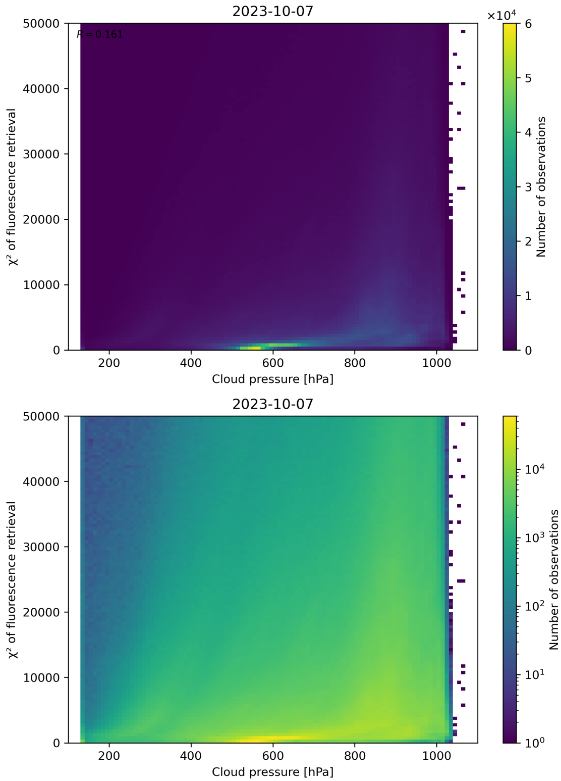
Figure 86: Scatter density plot of “Cloud pressure” against “ \chi^2 of fluorescence retrieval” for 2023-10-06 to 2023-10-08.
