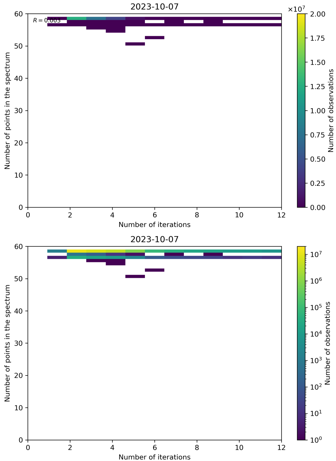
Figure 108: Scatter density plot of “Number of iterations” against “Number of points in the spectrum” for 2023-10-06 to 2023-10-08.
