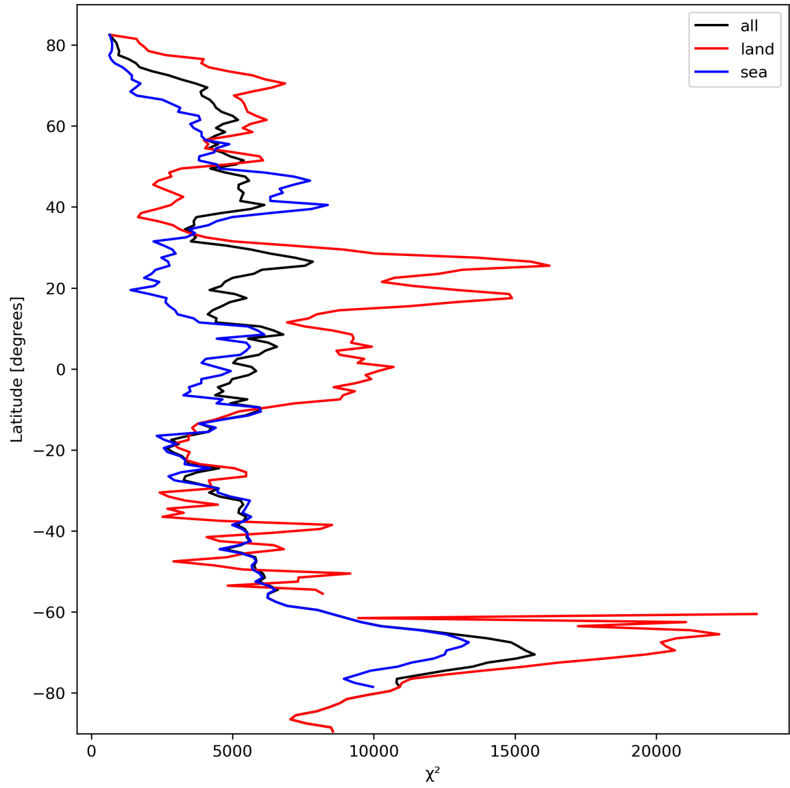
Figure 21: Zonal average of “ \chi^2 ” for 2023-10-06 to 2023-10-08.
