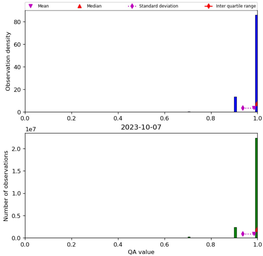
Figure 29: Histogram of “QA value” for 2023-10-06 to 2023-10-08
