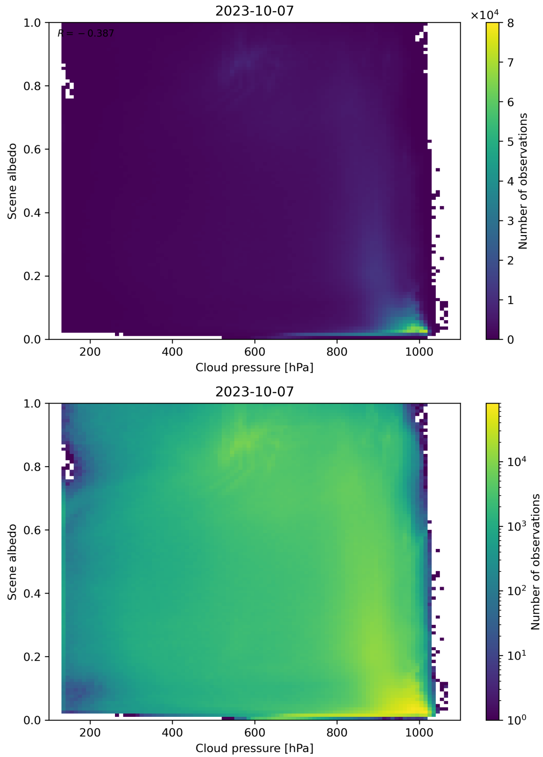
Figure 91: Scatter density plot of “Cloud pressure” against “Scene albedo” for 2023-10-06 to 2023-10-08.
