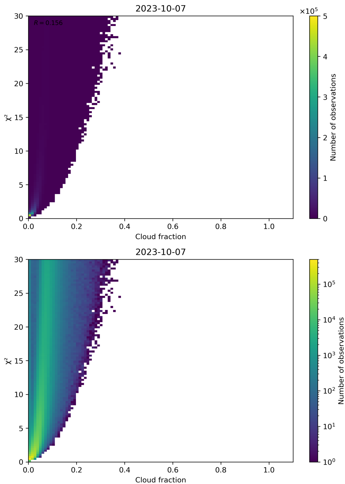
Figure 77: Scatter density plot of “Cloud fraction” against “ \chi^2 ” for 2023-10-06 to 2023-10-08.
