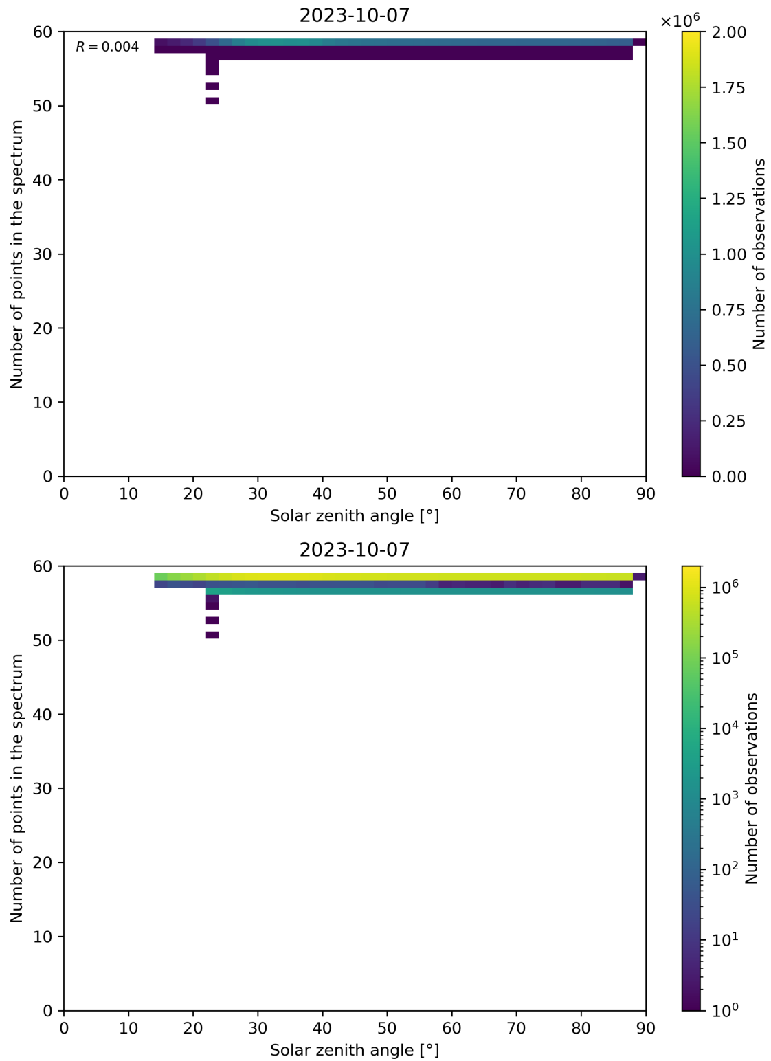
Figure 126: Scatter density plot of “Solar zenith angle” against “Number of points in the spectrum” for 2023-10-06 to 2023-10-08.
