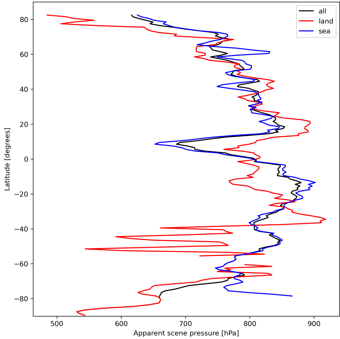
Figure 19: Zonal average of “Apparent scene pressure” for 2023-10-06 to 2023-10-08.
