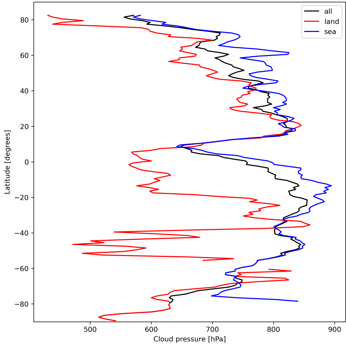
Figure 13: Zonal average of “Cloud pressure” for 2023-10-06 to 2023-10-08.
