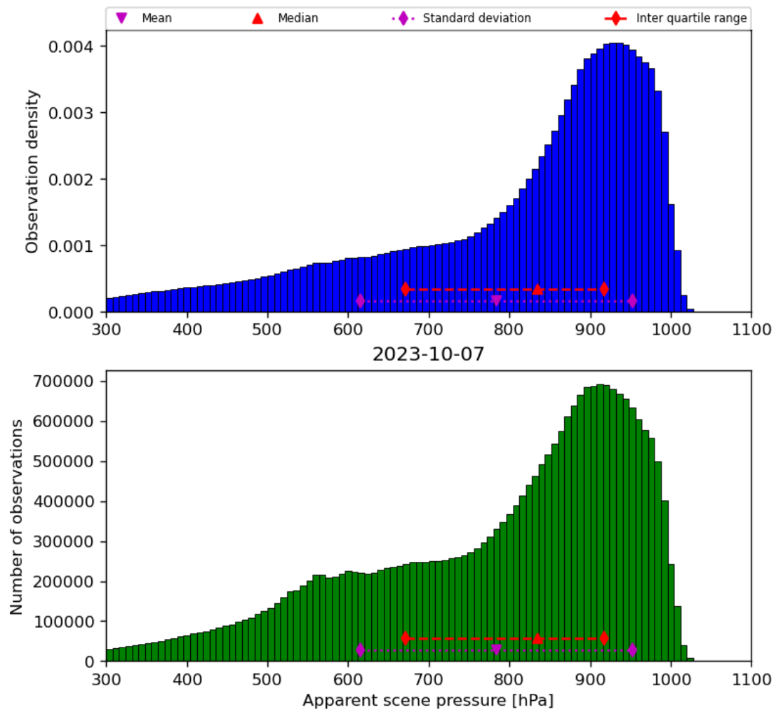
Figure 36: Histogram of “Apparent scene pressure” for 2023-10-06 to 2023-10-08
