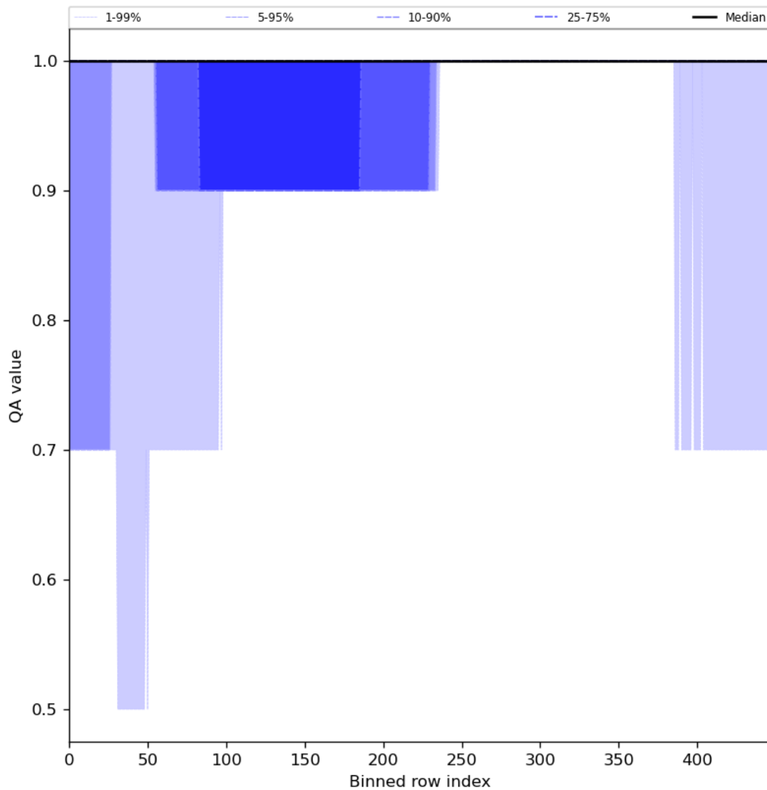
Figure 46: Along track statistics of “QA value” for 2023-10-06 to 2023-10-08
