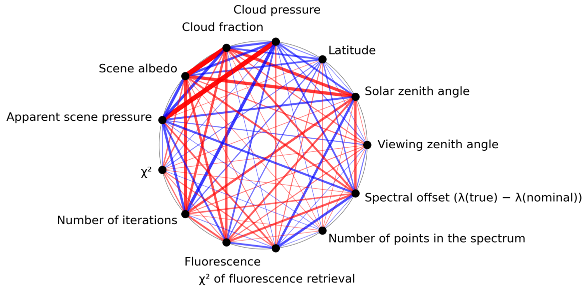
Figure 1: Map of correlation graph for 2023-10-06 to 2023-10-08.
