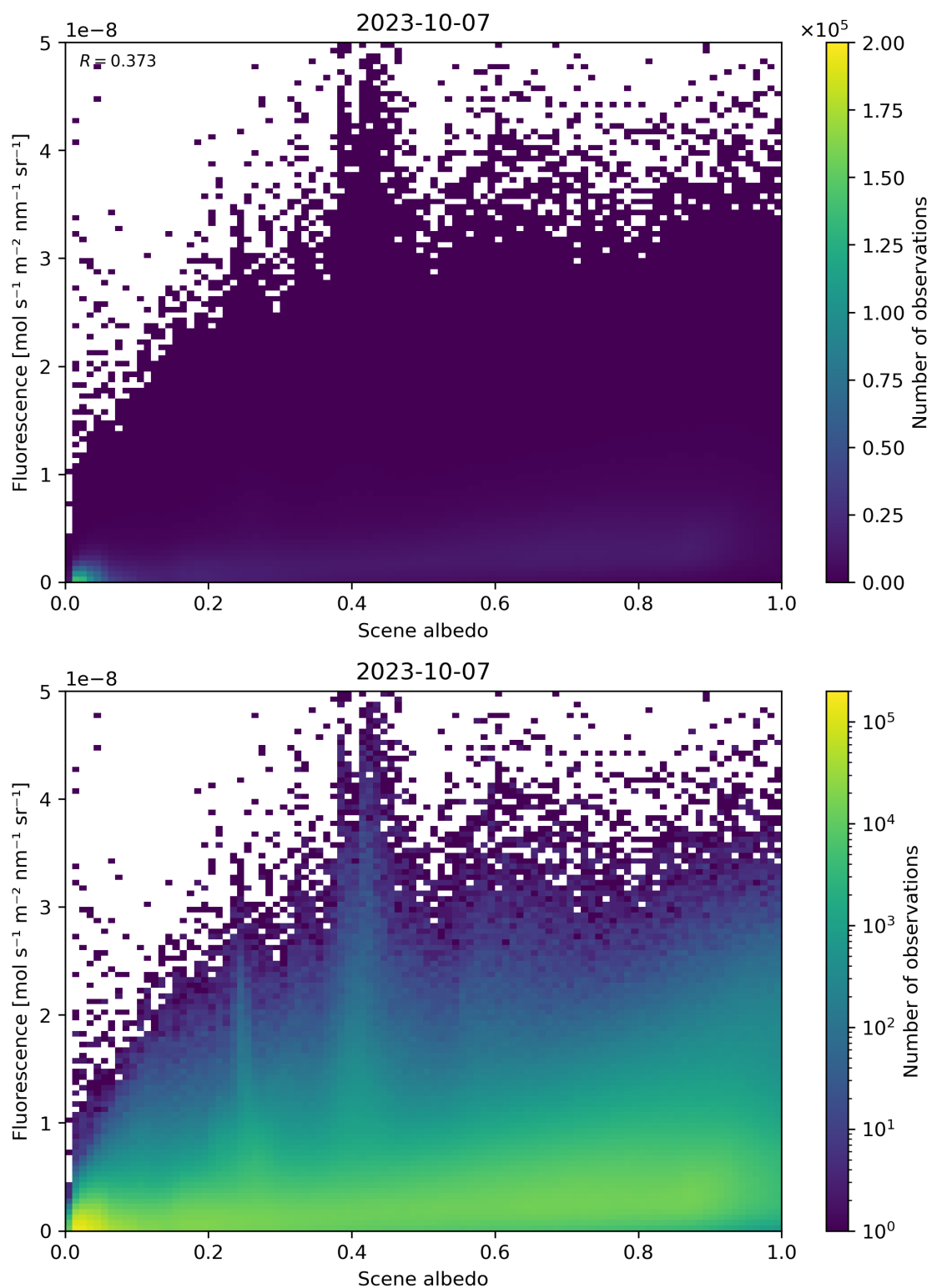
Figure 114: Scatter density plot of “Scene albedo” against “Fluorescence” for 2023-10-06 to 2023-10-08.
