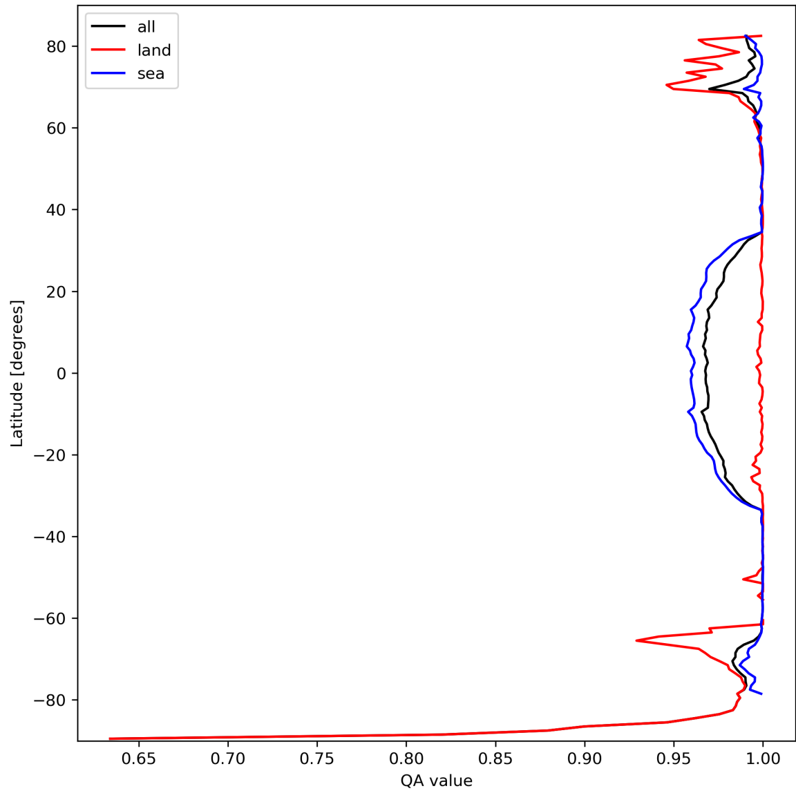
Figure 12: Zonal average of “QA value” for 2023-10-06 to 2023-10-08.
