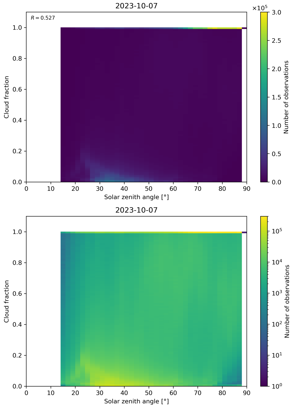
Figure 121: Scatter density plot of “Solar zenith angle” against “Cloud fraction” for 2023-10-06 to 2023-10-08.
