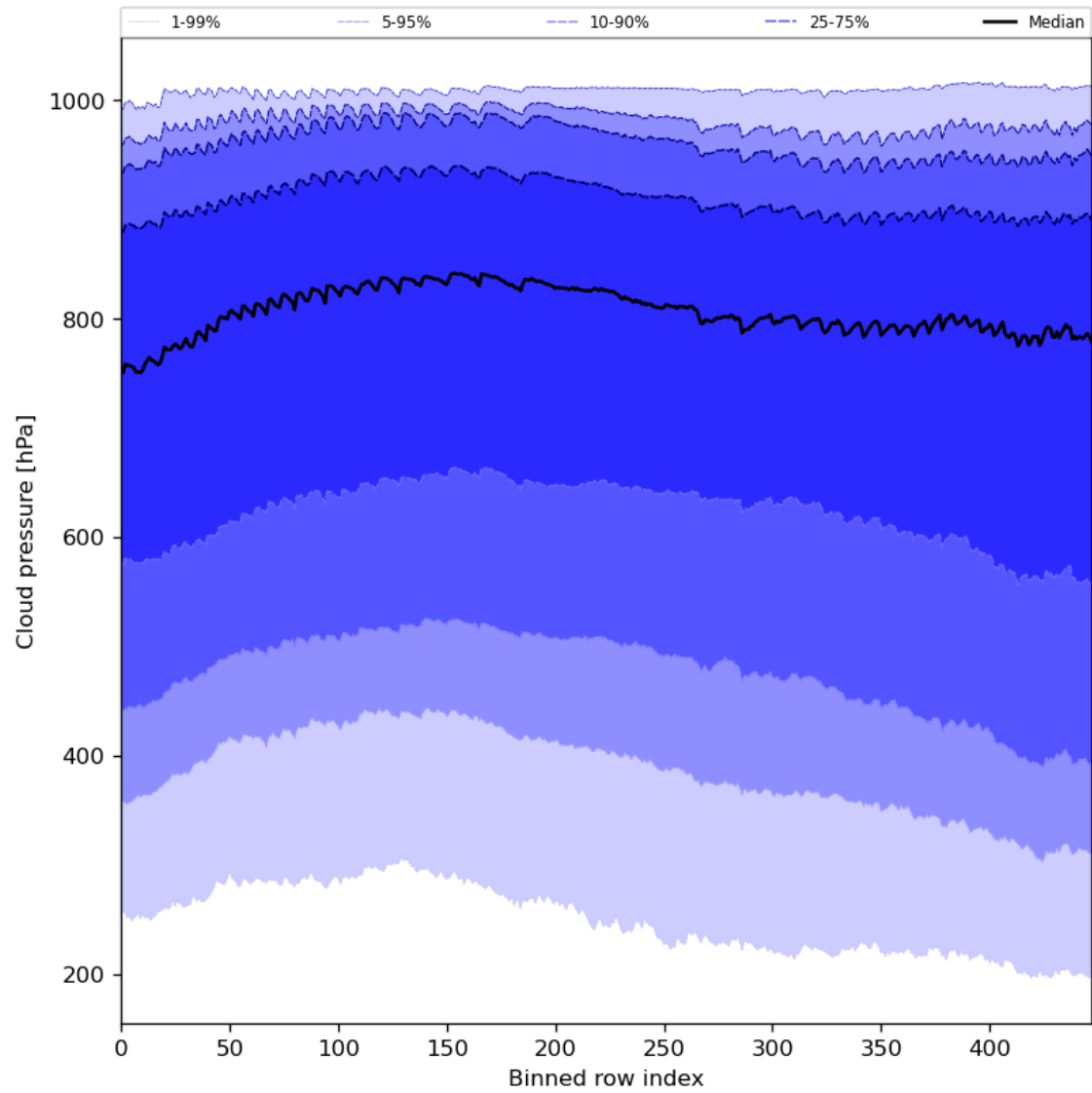
Figure 47: Along track statistics of “Cloud pressure” for 2023-10-06 to 2023-10-08
