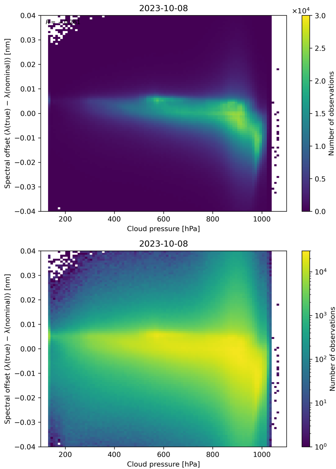
Figure 92: Scatter density plot of “Cloud pressure” against “Spectral offset ( \lambda(\text{true}) - \lambda(\text{nominal}) )” for 2023-10-07 to 2023-10-09.
