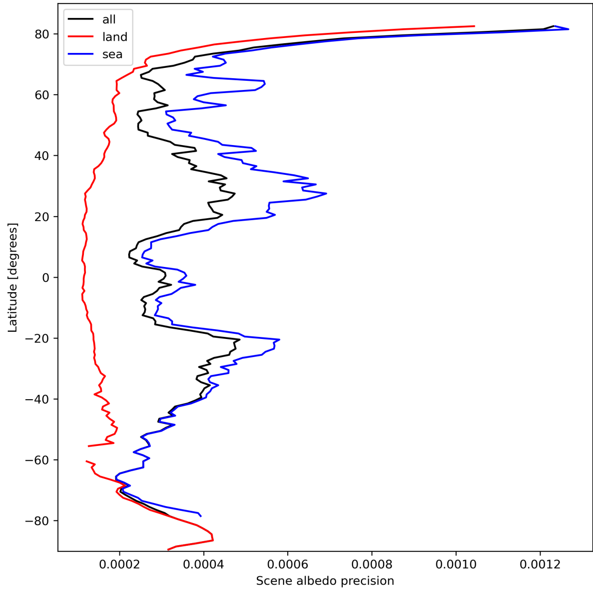
Figure 18: Zonal average of "Scene albedo precision" for 2023-10-07 to 2023-10-09.
