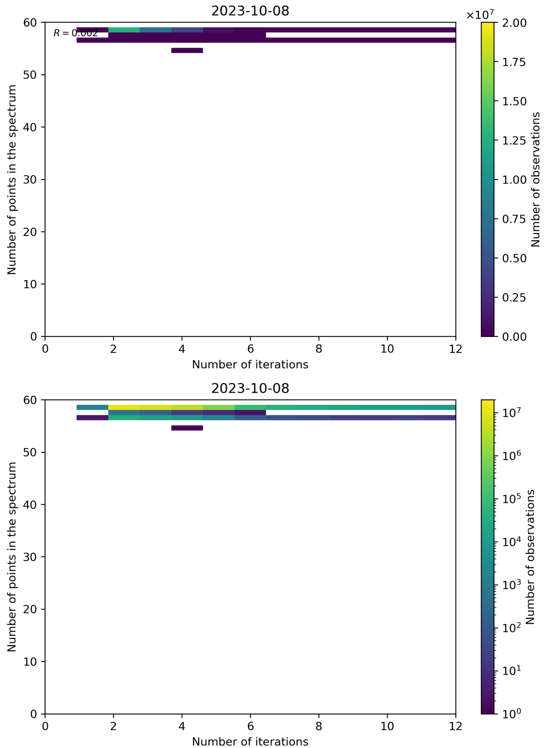
Figure 108: Scatter density plot of “Number of iterations” against “Number of points in the spectrum” for 2023-10-07 to 2023-10-09.
