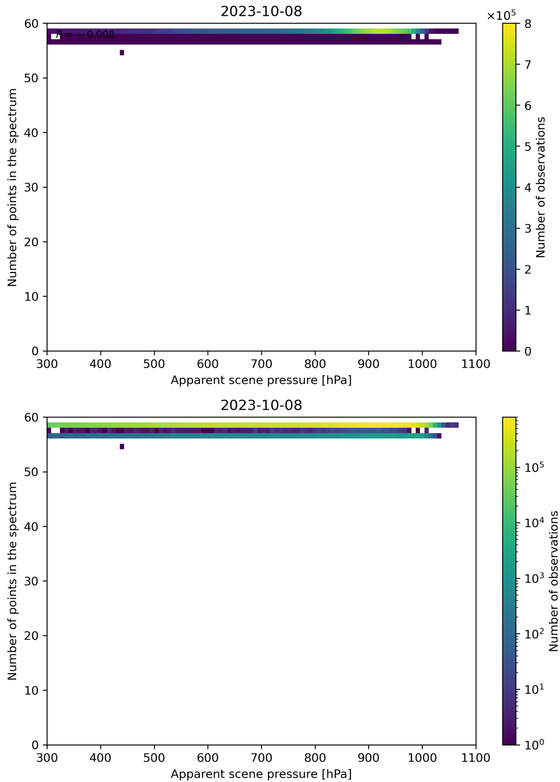
Figure 67: Scatter density plot of “Apparent scene pressure” against “Number of points in the spectrum” for 2023-10-07 to 2023-10-09.
