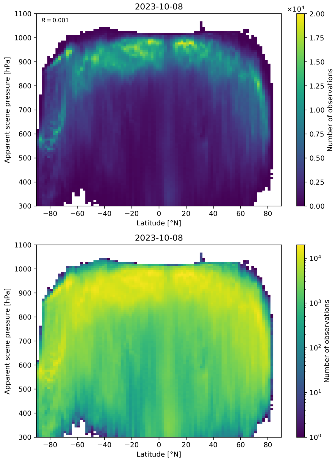
Figure 96: Scatter density plot of “Latitude” against “Apparent scene pressure” for 2023-10-07 to 2023-10-09.
