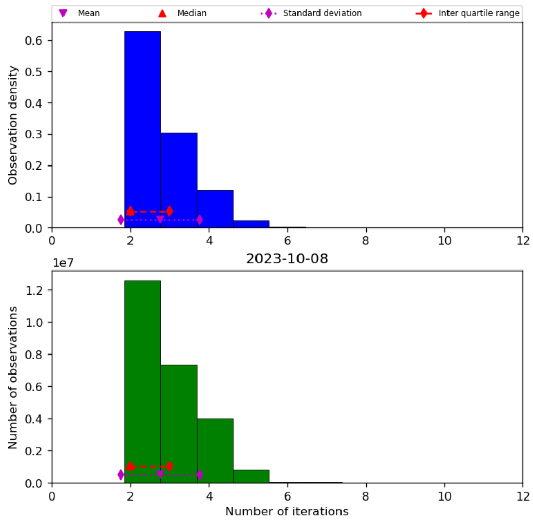
Figure 39: Histogram of “Number of iterations” for 2023-10-07 to 2023-10-09
