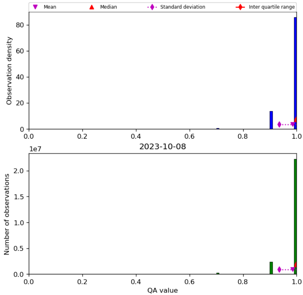
Figure 29: Histogram of “QA value” for 2023-10-07 to 2023-10-09
