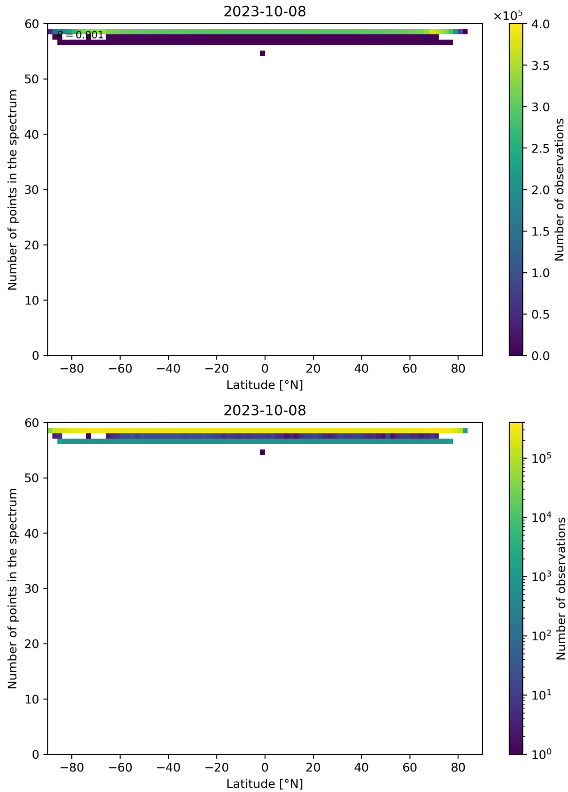
Figure 103: Scatter density plot of “Latitude” against “Number of points in the spectrum” for 2023-10-07 to 2023-10-09.
