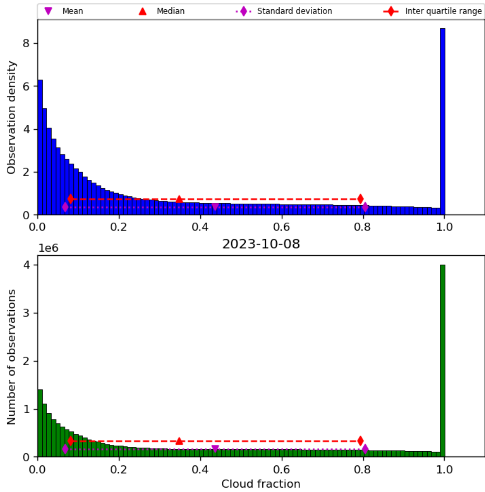
Figure 32: Histogram of “Cloud fraction” for 2023-10-07 to 2023-10-09
