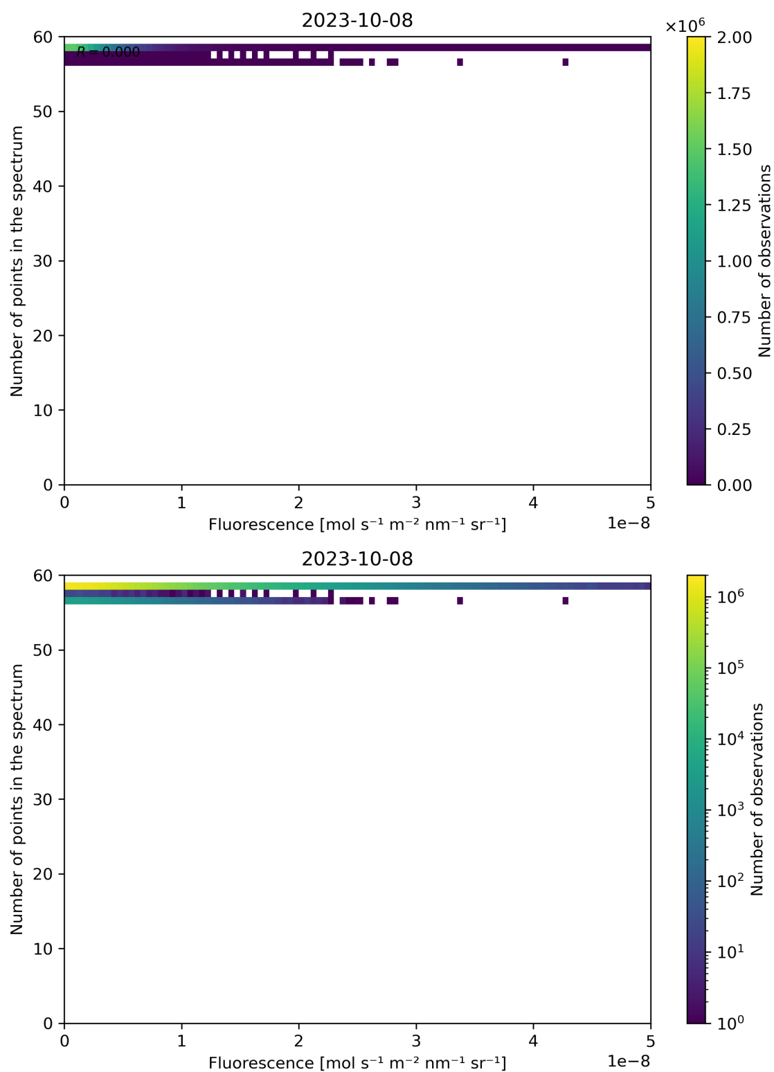
Figure 94: Scatter density plot of “Fluorescence” against “Number of points in the spectrum” for 2023-10-07 to 2023-10-09.
