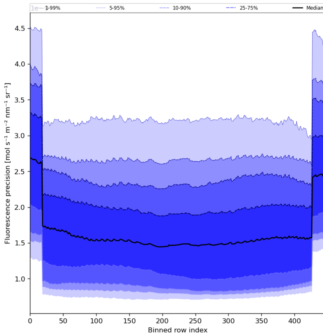
Figure 58: Along track statistics of “Fluorescence precision” for 2023-10-07 to 2023-10-09
