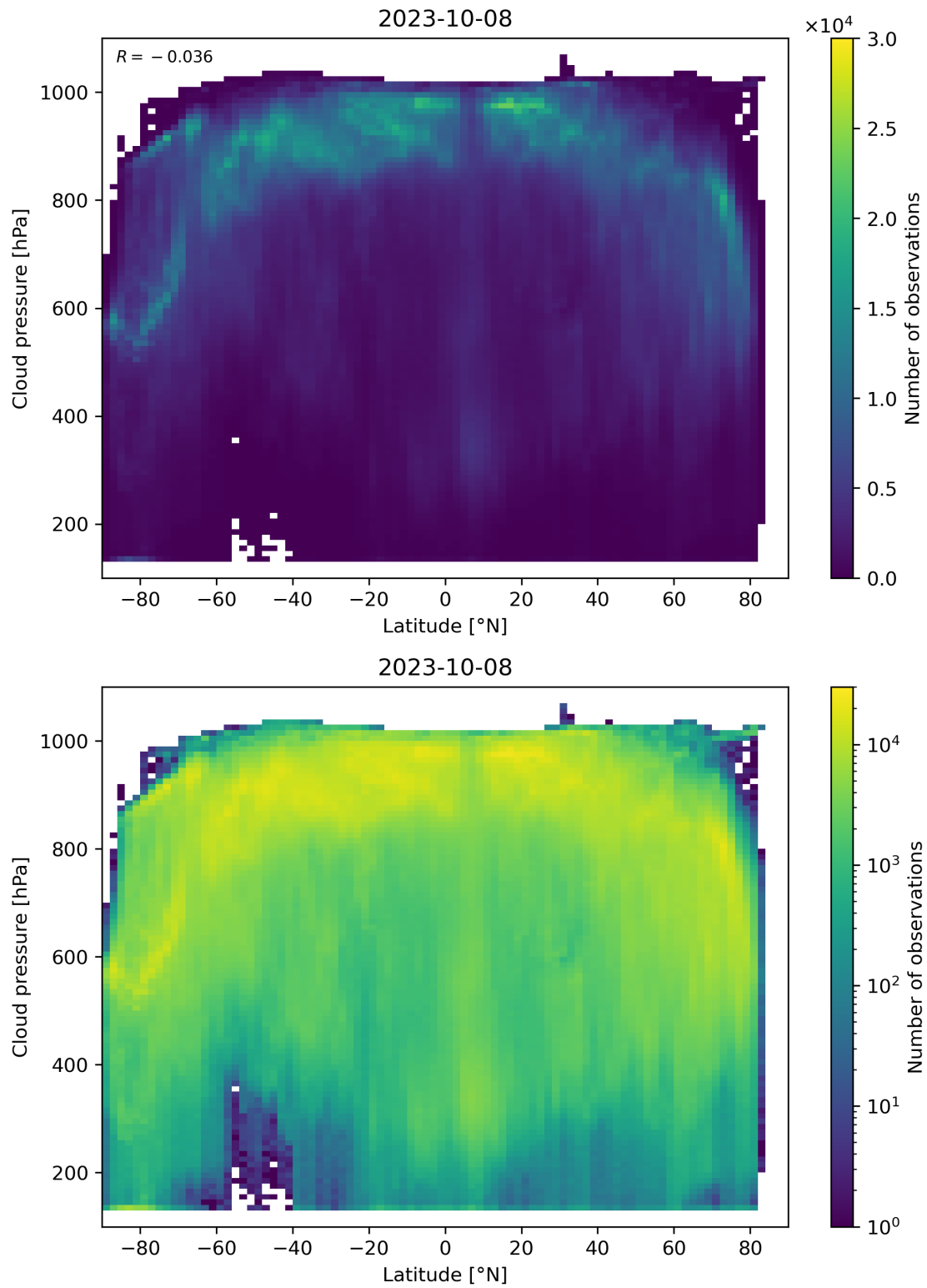
Figure 100: Scatter density plot of “Latitude” against “Cloud pressure” for 2023-10-07 to 2023-10-09.
