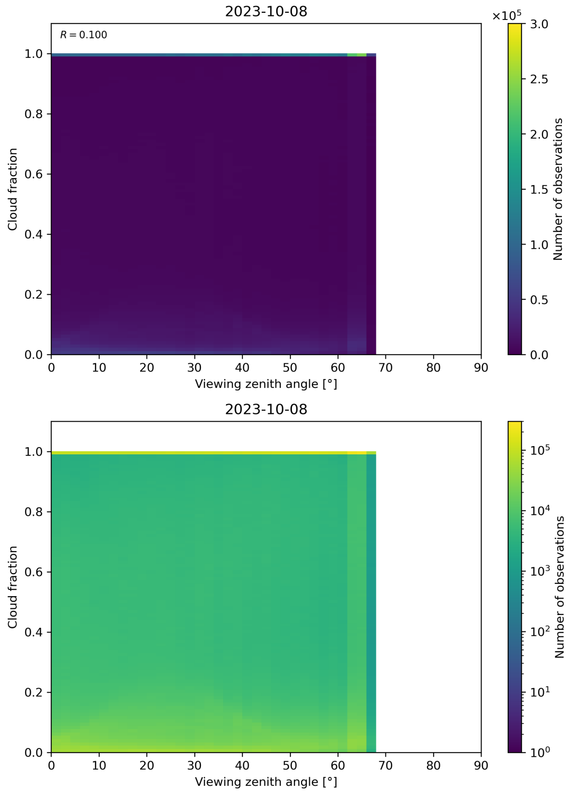
Figure 132: Scatter density plot of “Viewing zenith angle” against “Cloud fraction” for 2023-10-07 to 2023-10-09.
