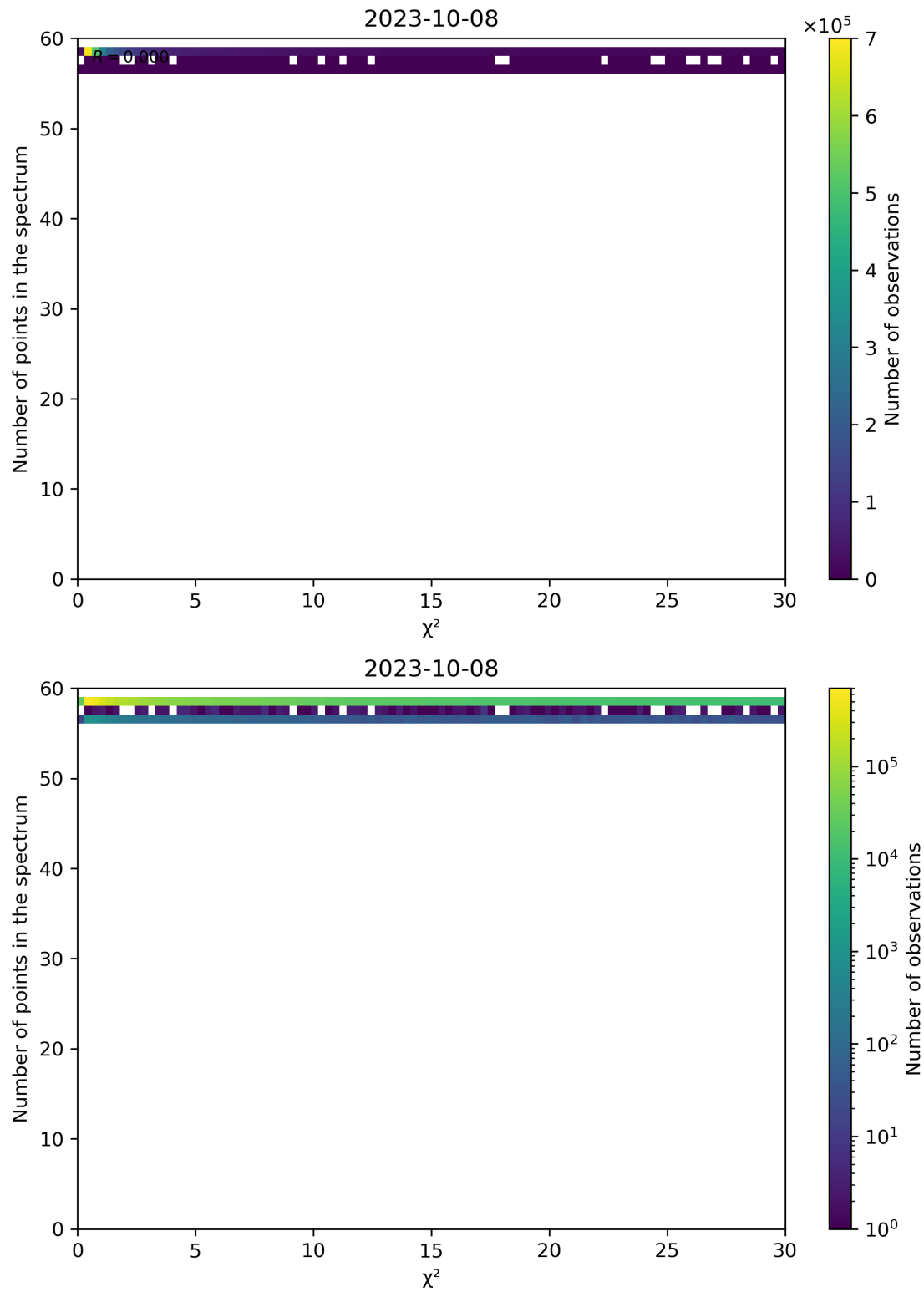
Figure 74: Scatter density plot of " \chi^2 " against "Number of points in the spectrum" for 2023-10-07 to 2023-10-09.
