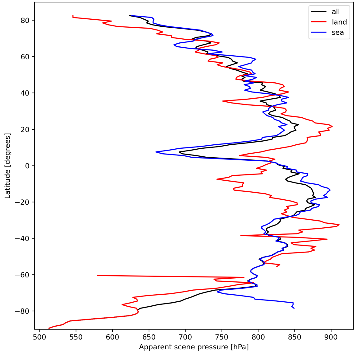
Figure 19: Zonal average of “Apparent scene pressure” for 2023-10-07 to 2023-10-09.
