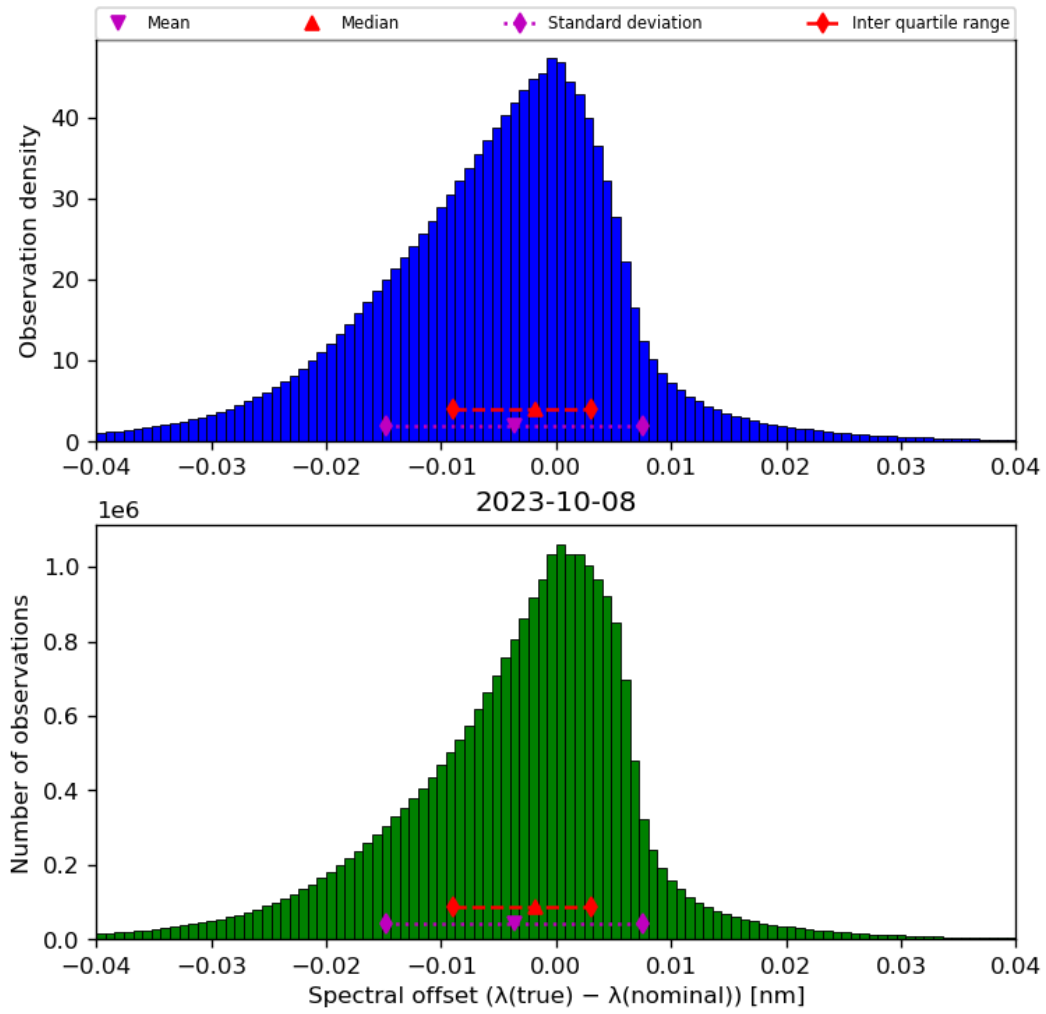
Figure 45: Histogram of “Spectral offset ( \lambda(\text{true}) - \lambda(\text{nominal}) )” for 2023-10-07 to 2023-10-09
