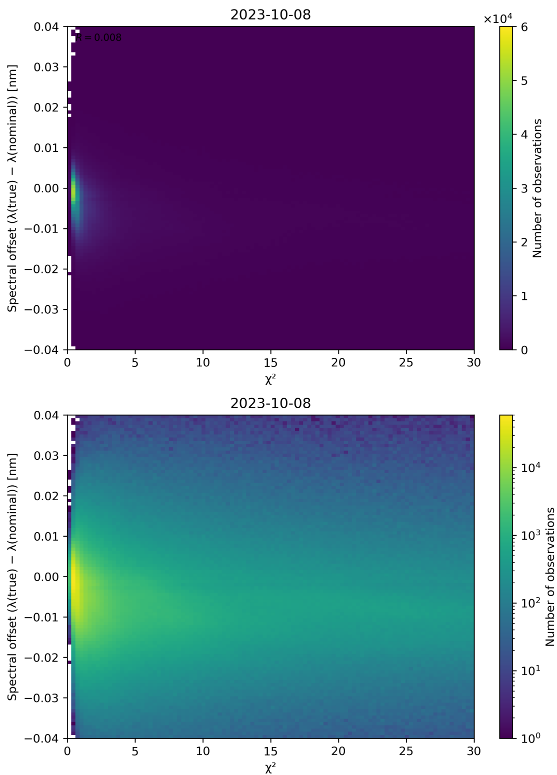
Figure 75: Scatter density plot of “ \chi^2 ” against “Spectral offset ( \lambda(\text{true}) - \lambda(\text{nominal}) )” for 2023-10-07 to 2023-10-09.
