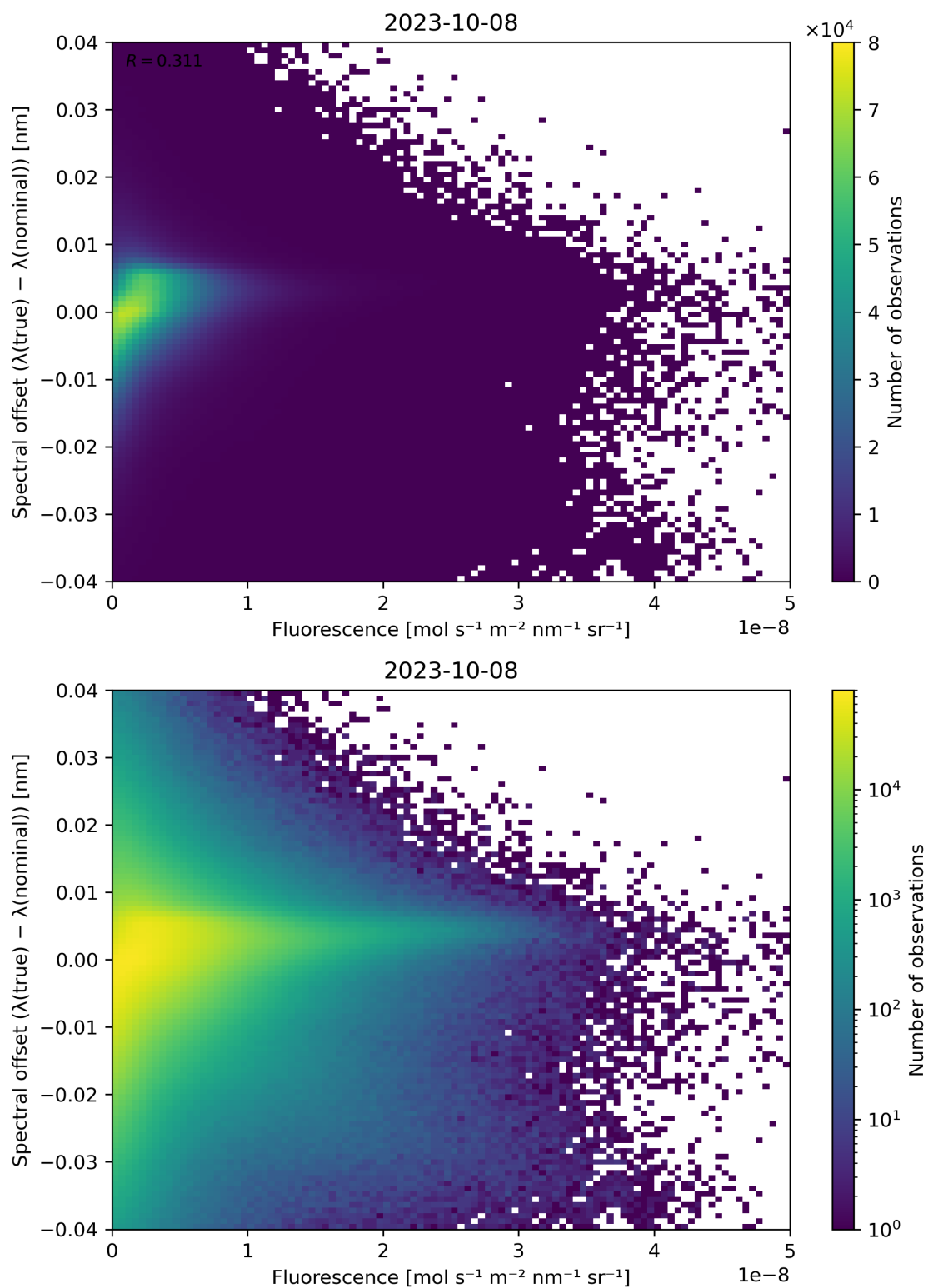
Figure 95: Scatter density plot of “Fluorescence” against “Spectral offset ( \lambda(\text{true}) - \lambda(\text{nominal}) )” for 2023-10-07 to 2023-10-09.
