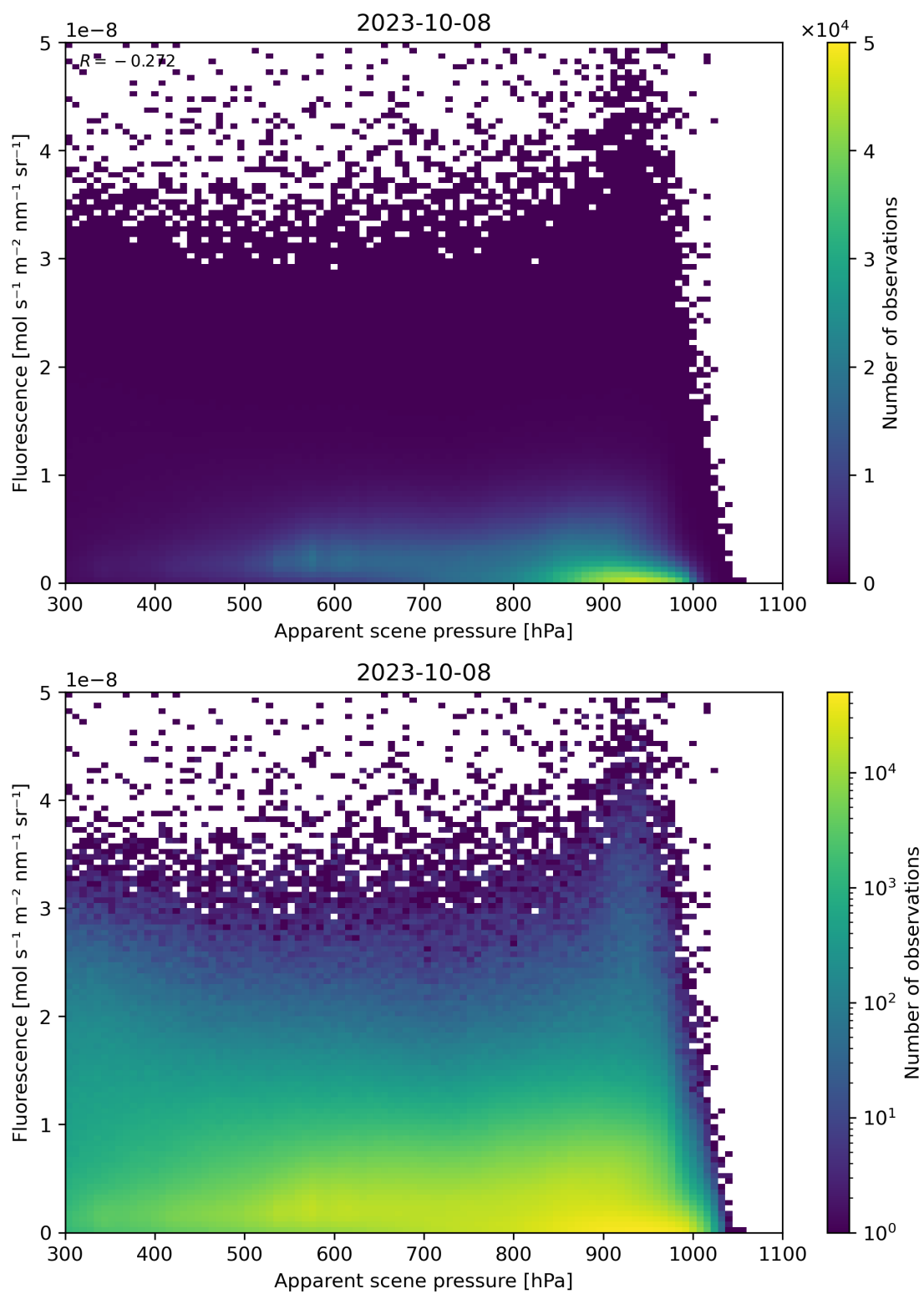
Figure 65: Scatter density plot of “Apparent scene pressure” against “Fluorescence” for 2023-10-07 to 2023-10-09.
