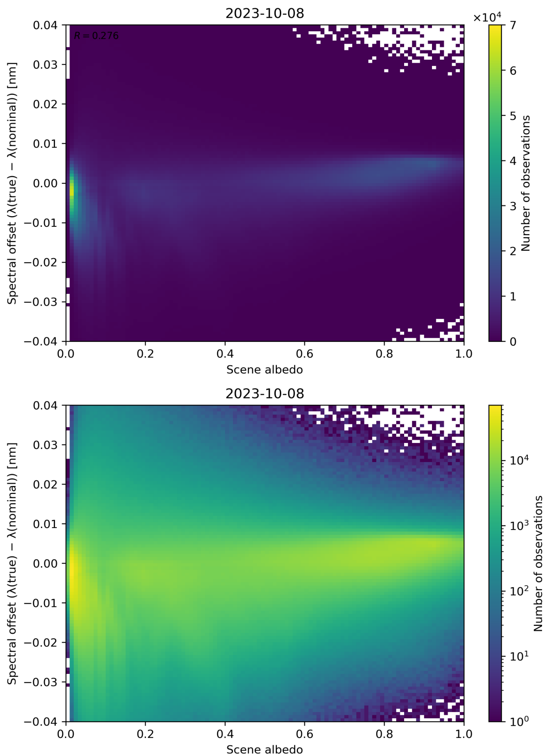
Figure 117: Scatter density plot of “Scene albedo” against “Spectral offset ( \lambda(\text{true}) - \lambda(\text{nominal}) )” for 2023-10-07 to 2023-10-09.
