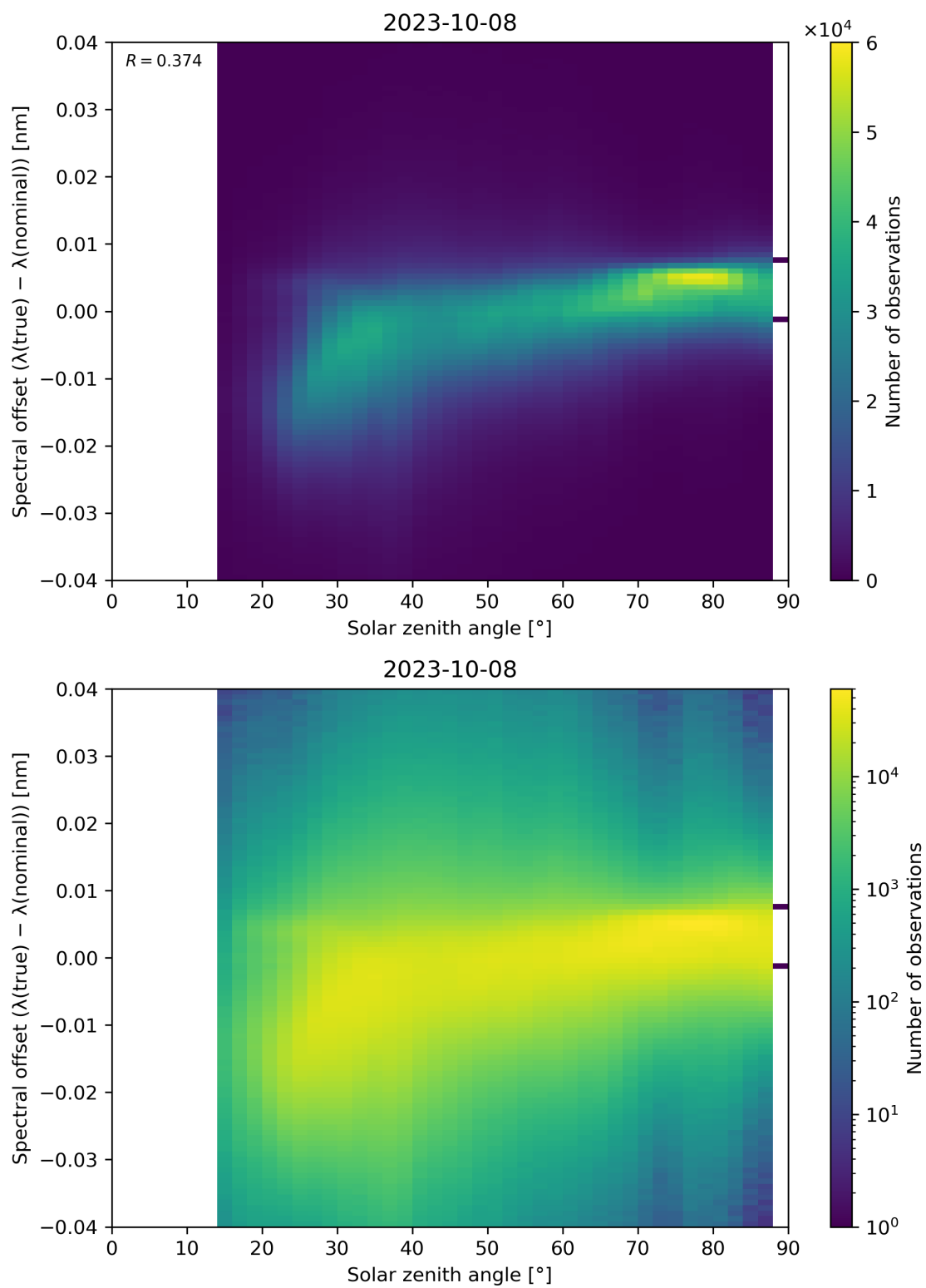
Figure 128: Scatter density plot of “Solar zenith angle” against “Spectral offset ( \lambda(\text{true}) - \lambda(\text{nominal}) )” for 2023-10-07 to 2023-10-09.
