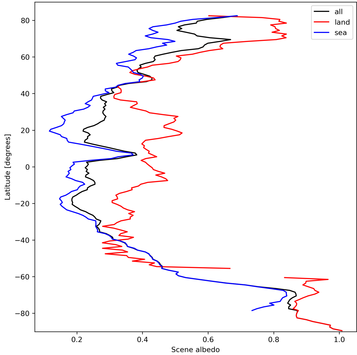
Figure 17: Zonal average of “Scene albedo” for 2023-10-07 to 2023-10-09.
