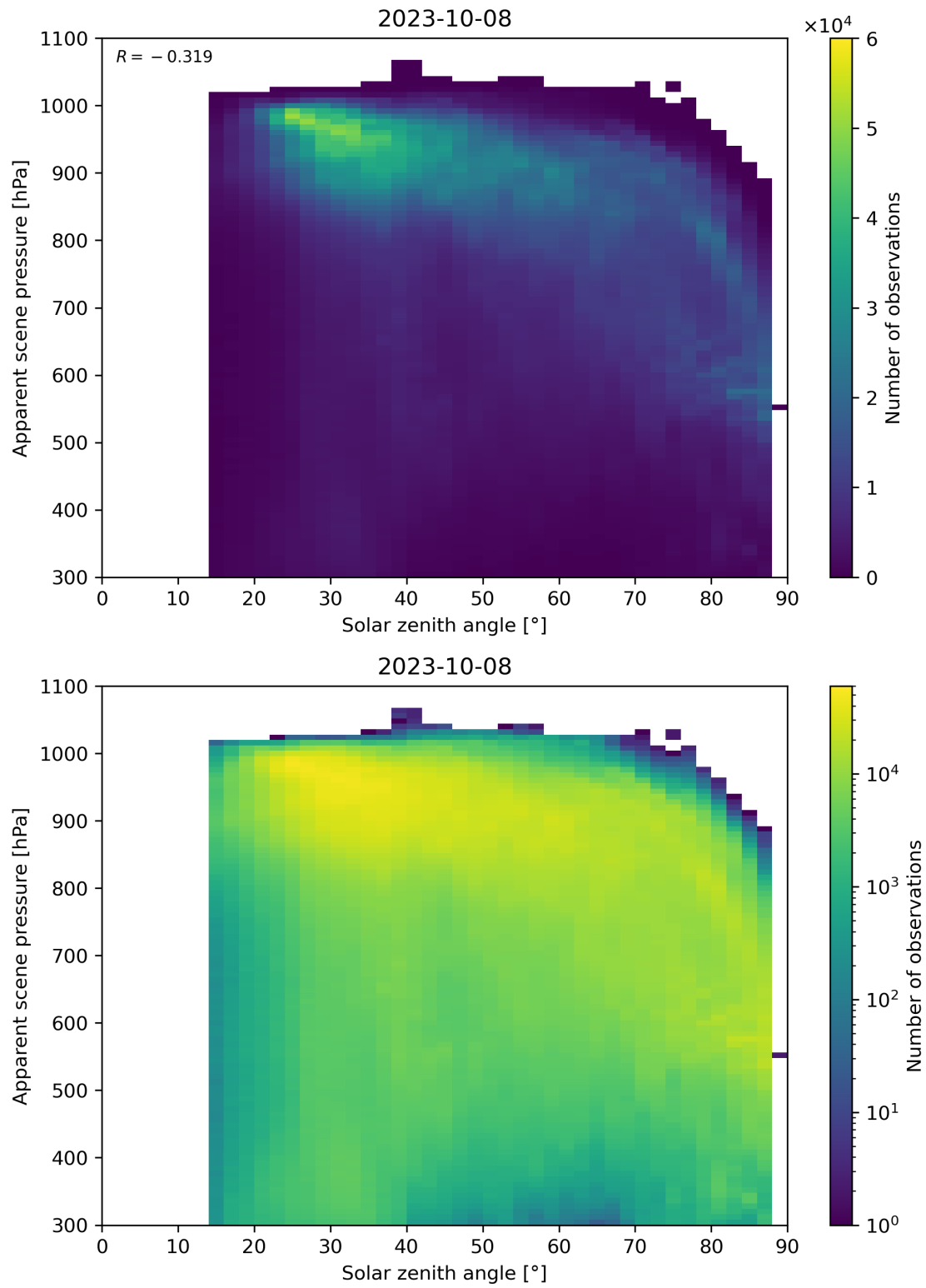
Figure 118: Scatter density plot of “Solar zenith angle” against “Apparent scene pressure” for 2023-10-07 to 2023-10-09.
