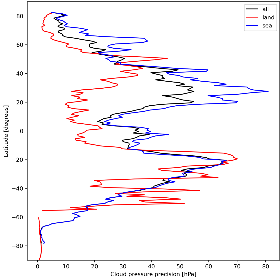
Figure 14: Zonal average of “Cloud pressure precision” for 2023-10-07 to 2023-10-09.
