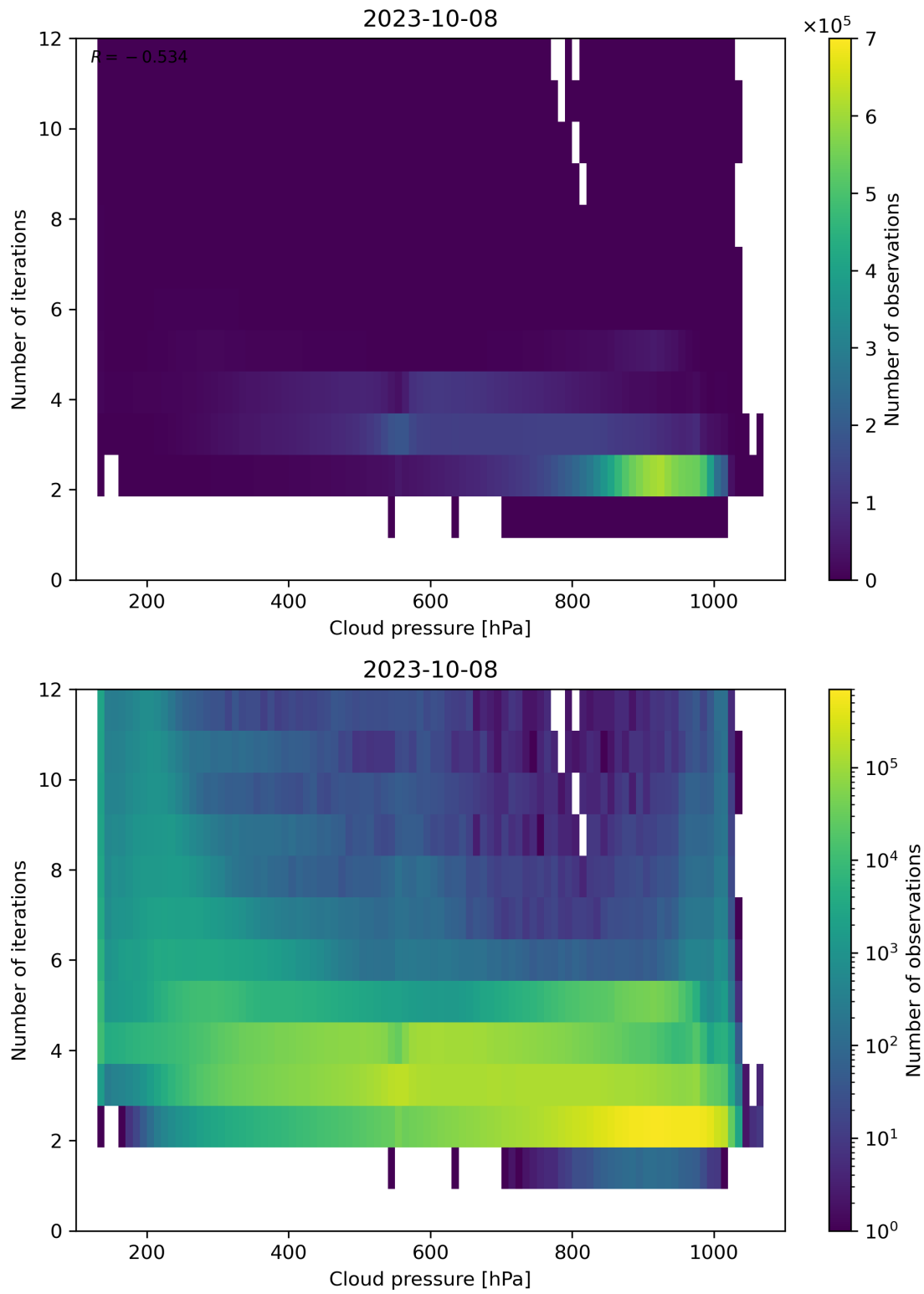
Figure 89: Scatter density plot of “Cloud pressure” against “Number of iterations” for 2023-10-07 to 2023-10-09.
