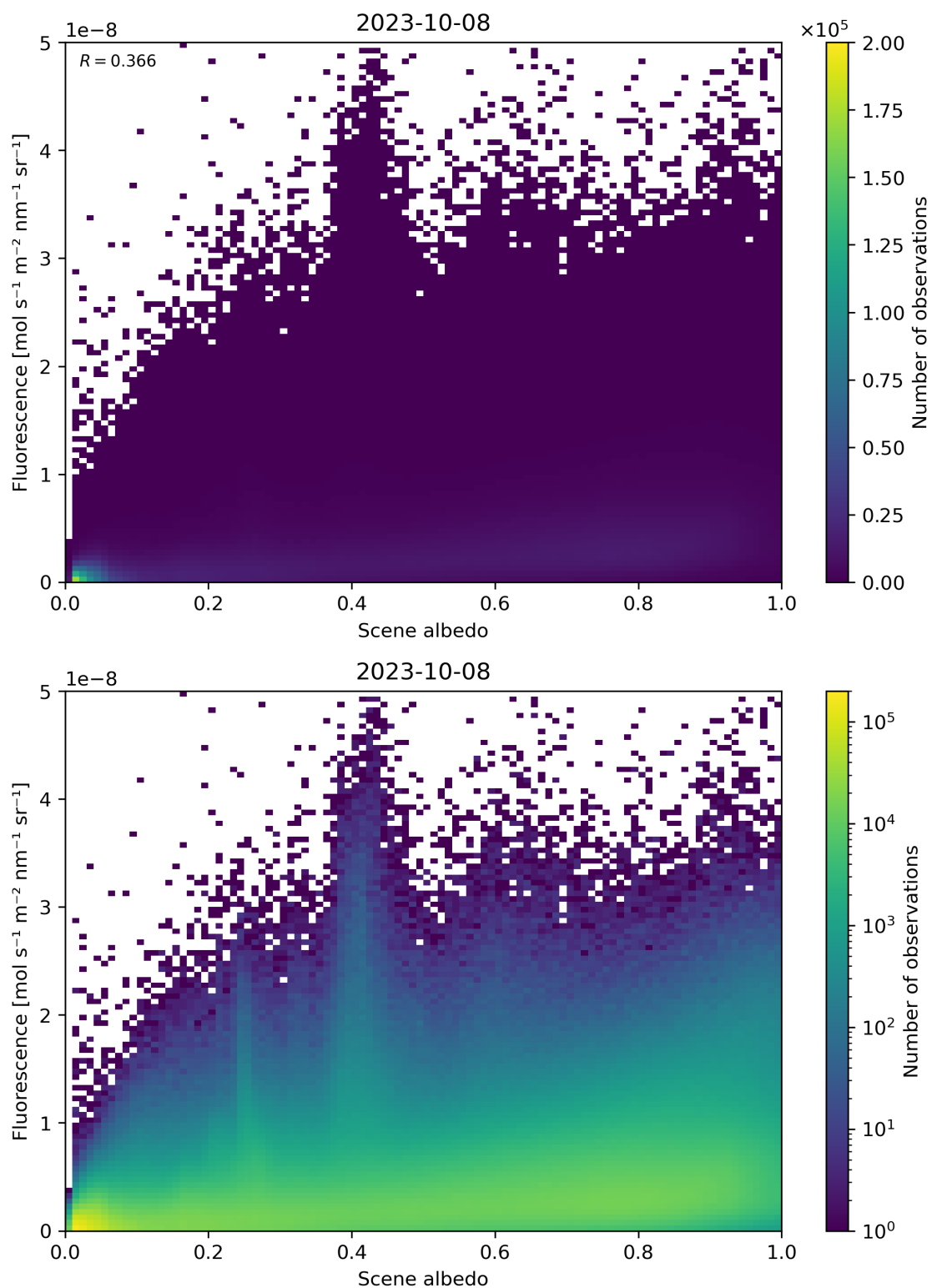
Figure 114: Scatter density plot of “Scene albedo” against “Fluorescence” for 2023-10-07 to 2023-10-09.
