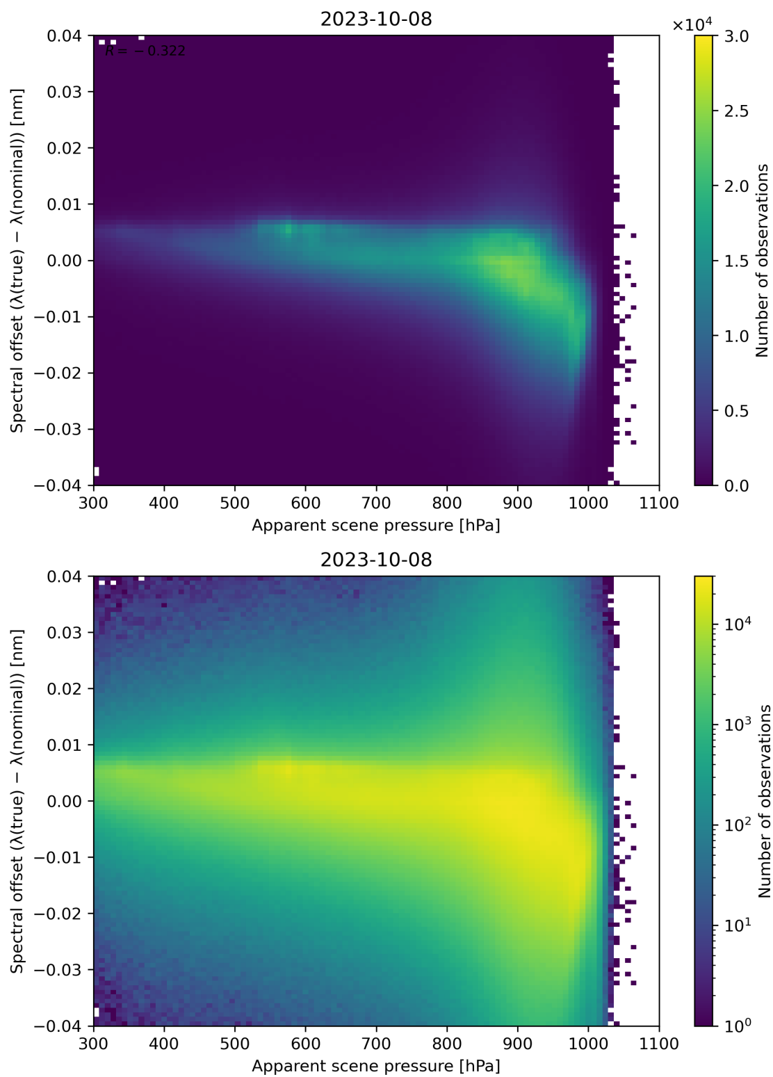
Figure 68: Scatter density plot of “Apparent scene pressure” against “Spectral offset ( \lambda(\text{true}) - \lambda(\text{nominal}) )” for 2023-10-07 to 2023-10-09.
