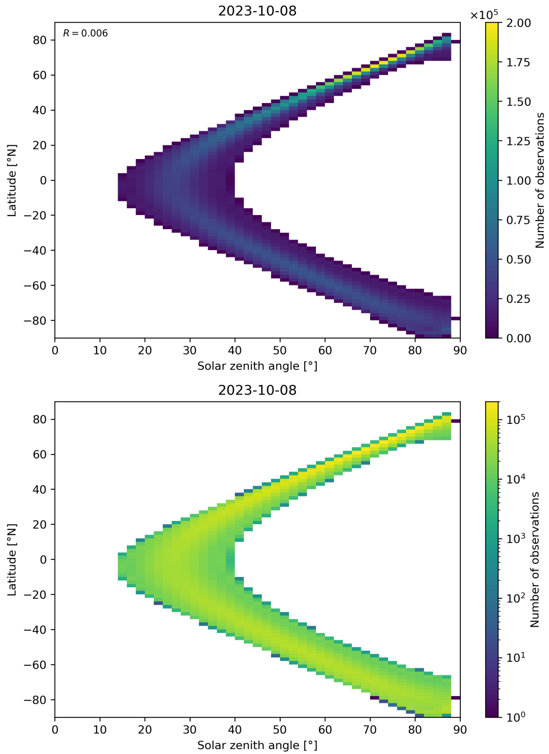
Figure 124: Scatter density plot of “Solar zenith angle” against “Latitude” for 2023-10-07 to 2023-10-09.
