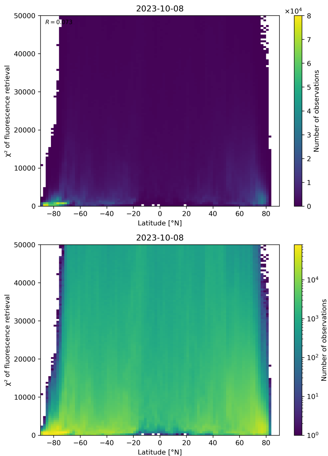
Figure 98: Scatter density plot of “Latitude” against “ \chi^2 of fluorescence retrieval” for 2023-10-07 to 2023-10-09.
