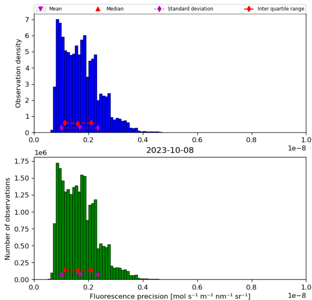
Figure 41: Histogram of “Fluorescence precision” for 2023-10-07 to 2023-10-09
