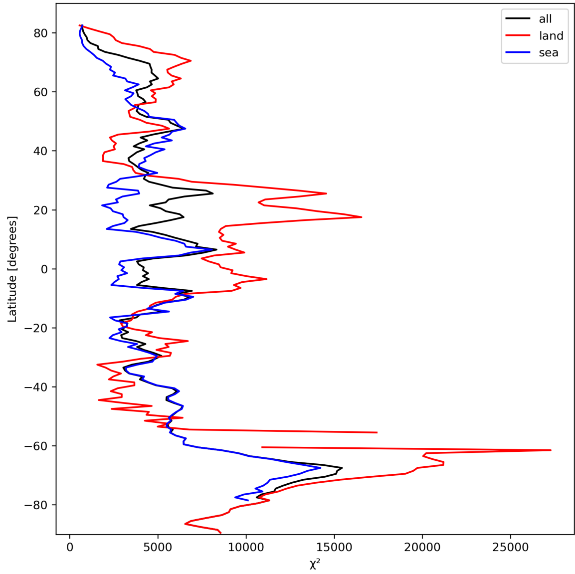
Figure 21: Zonal average of “ \chi^2 ” for 2023-10-07 to 2023-10-09.
