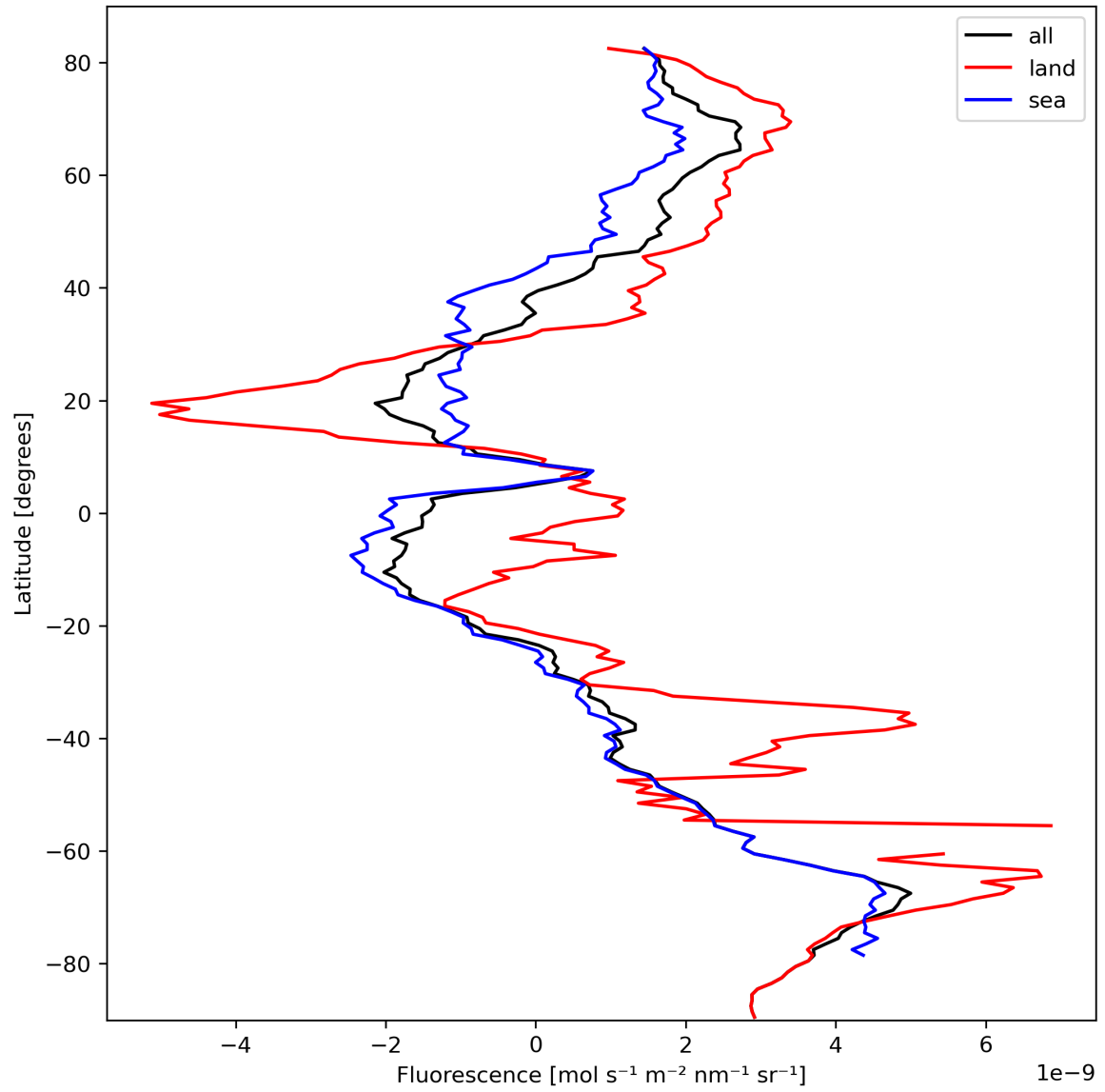
Figure 23: Zonal average of “Fluorescence” for 2023-10-07 to 2023-10-09.
