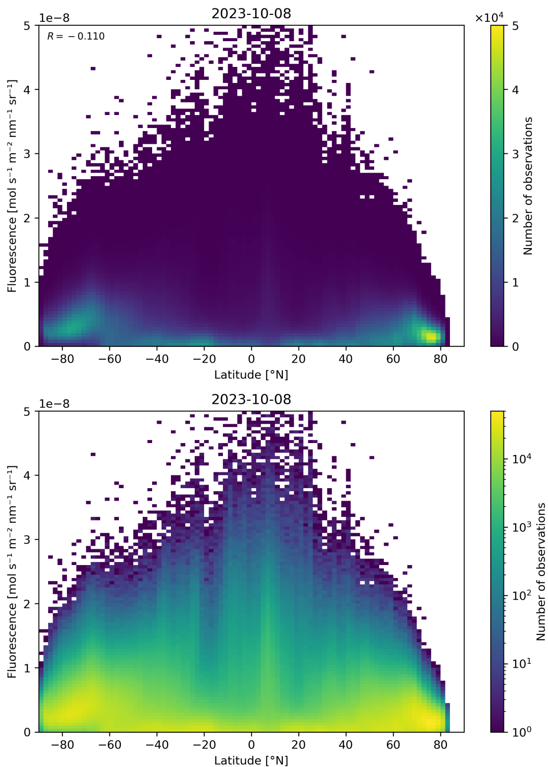
Figure 101: Scatter density plot of “Latitude” against “Fluorescence” for 2023-10-07 to 2023-10-09.
