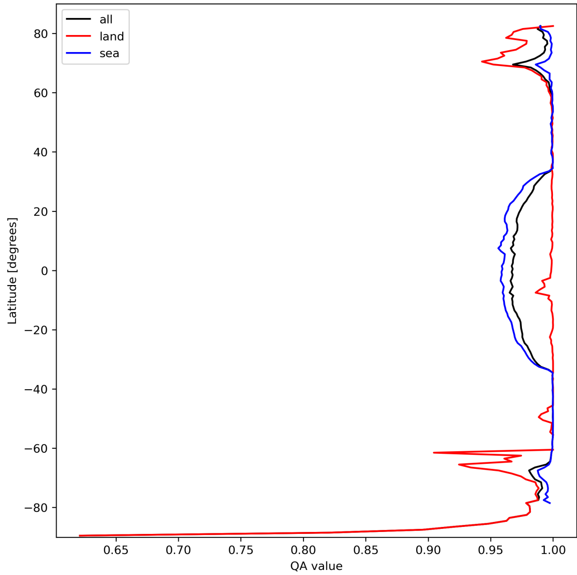
Figure 12: Zonal average of “QA value” for 2023-10-07 to 2023-10-09.
