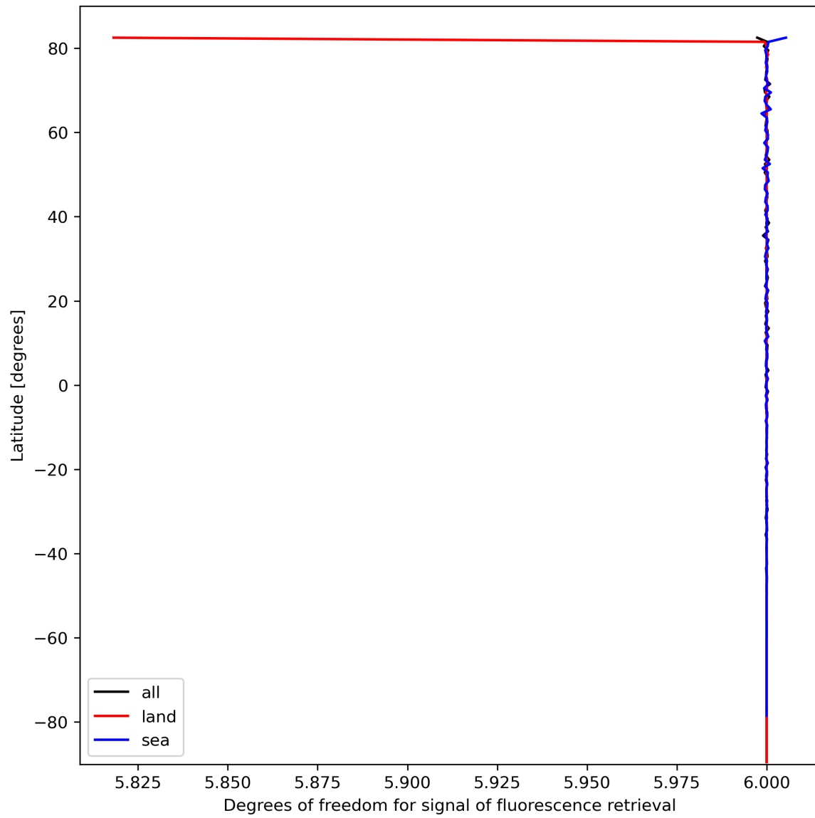
Figure 26: Zonal average of “Degrees of freedom for signal of fluorescence retrieval” for 2023-10-07 to 2023-10-09.
