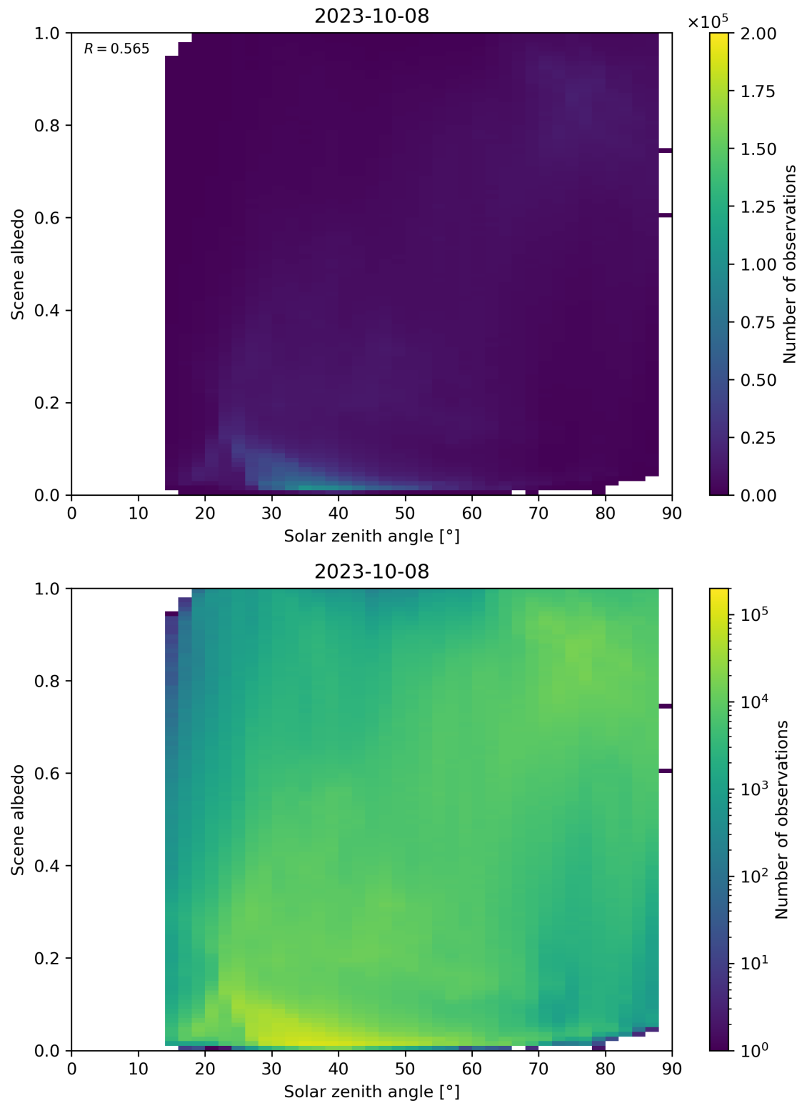
Figure 127: Scatter density plot of “Solar zenith angle” against “Scene albedo” for 2023-10-07 to 2023-10-09.
