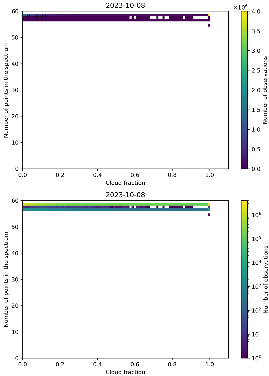
Figure 81: Scatter density plot of “Cloud fraction” against “Number of points in the spectrum” for 2023-10-07 to 2023-10-09.
