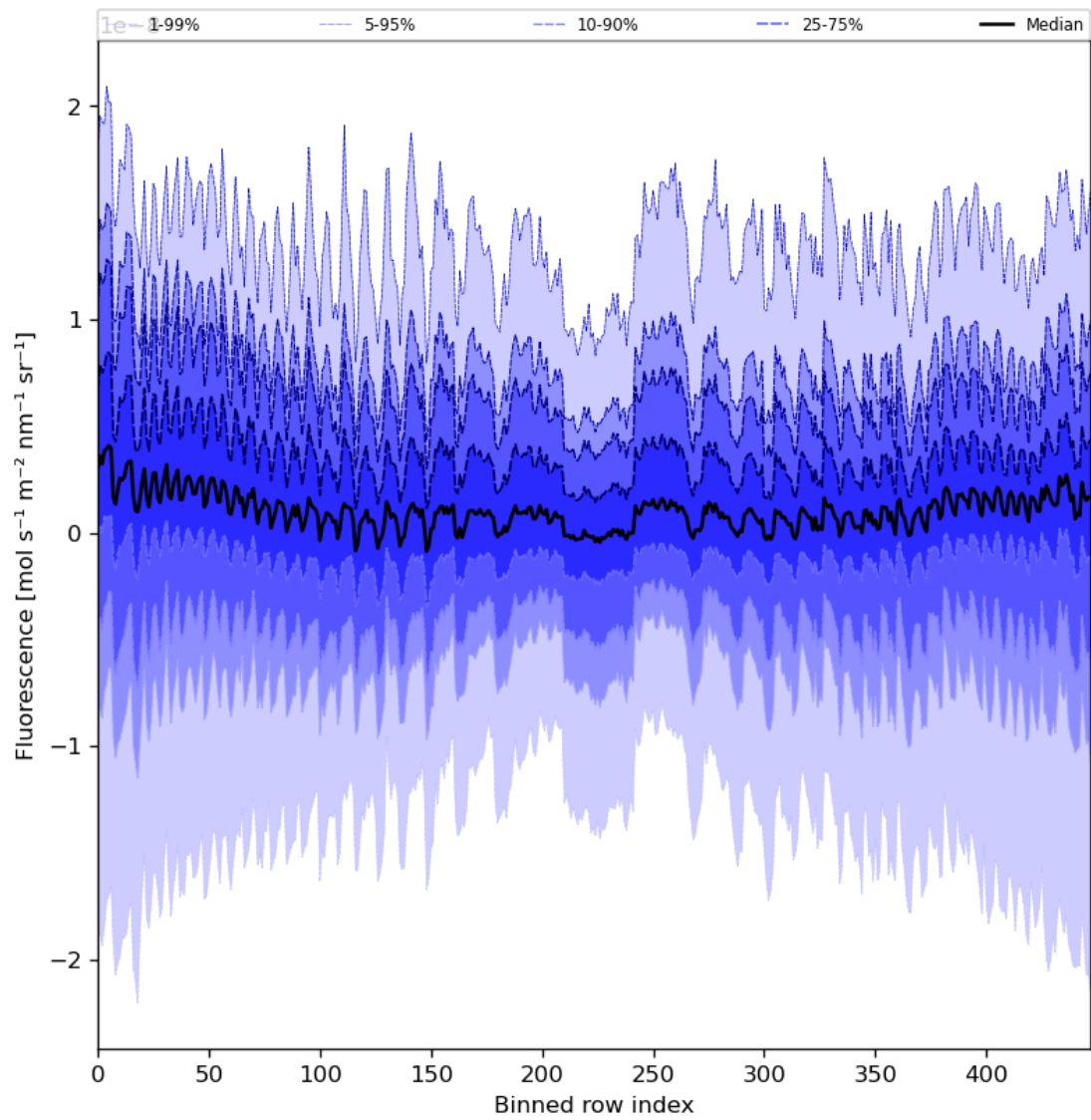
Figure 57: Along track statistics of “Fluorescence” for 2023-10-07 to 2023-10-09
