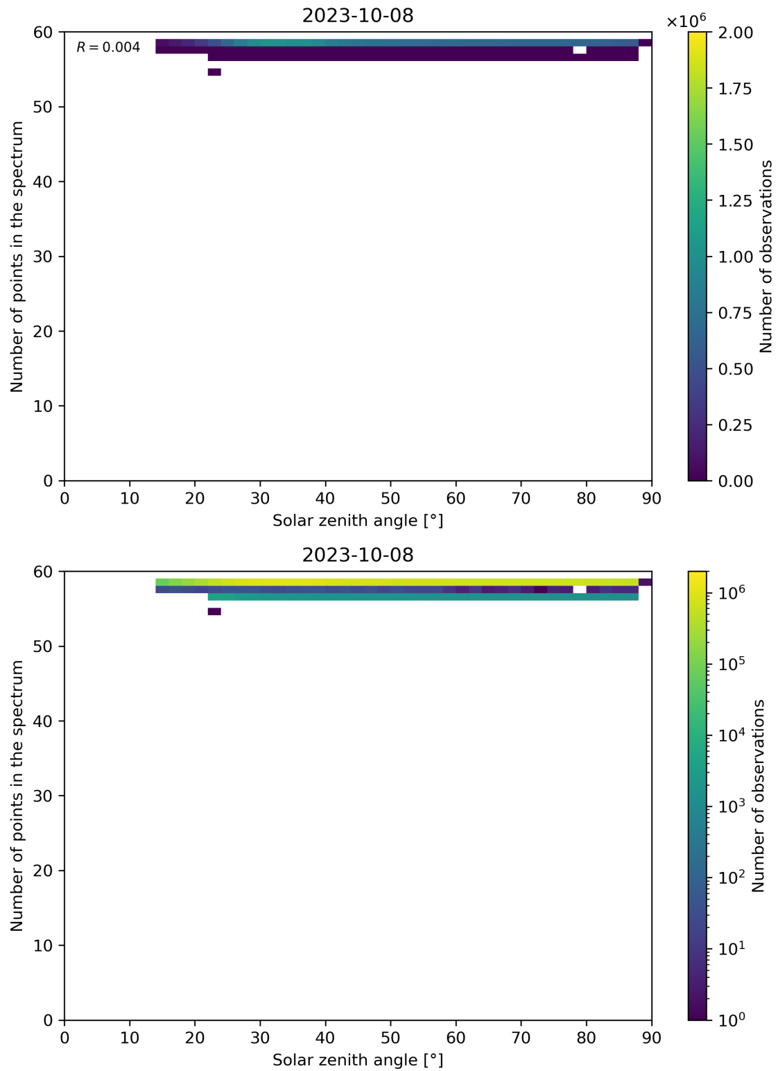
Figure 126: Scatter density plot of “Solar zenith angle” against “Number of points in the spectrum” for 2023-10-07 to 2023-10-09.
