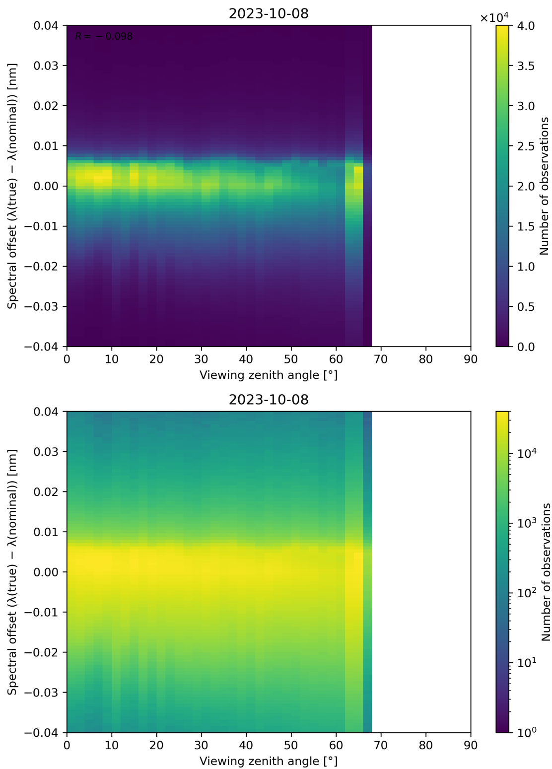
Figure 140: Scatter density plot of “Viewing zenith angle” against “Spectral offset ( \lambda(\text{true}) - \lambda(\text{nominal}) )” for 2023-10-07 to 2023-10-09.
