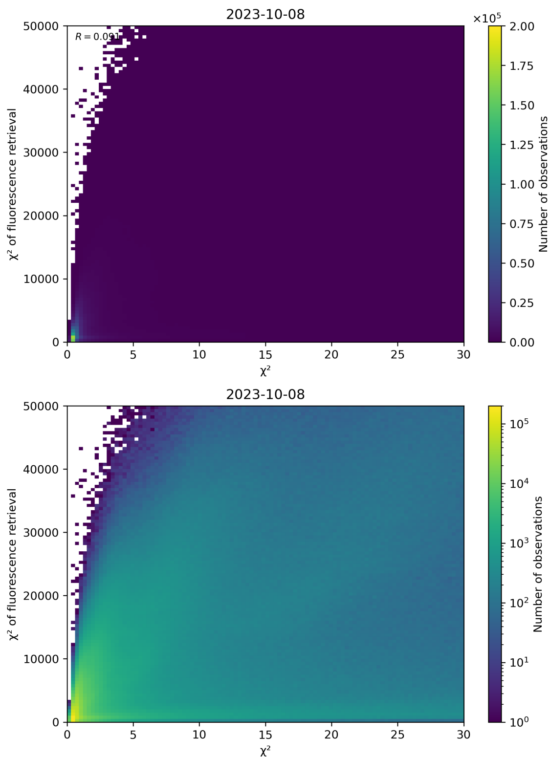
Figure 69: Scatter density plot of “ \chi^2 ” against “ \chi^2 of fluorescence retrieval” for 2023-10-07 to 2023-10-09.
