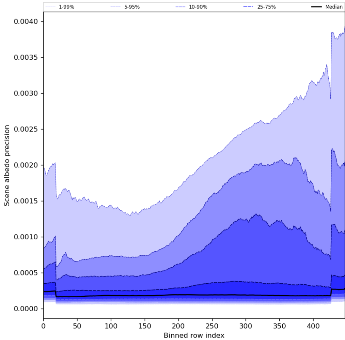
Figure 52: Along track statistics of “Scene albedo precision” for 2023-10-07 to 2023-10-09
