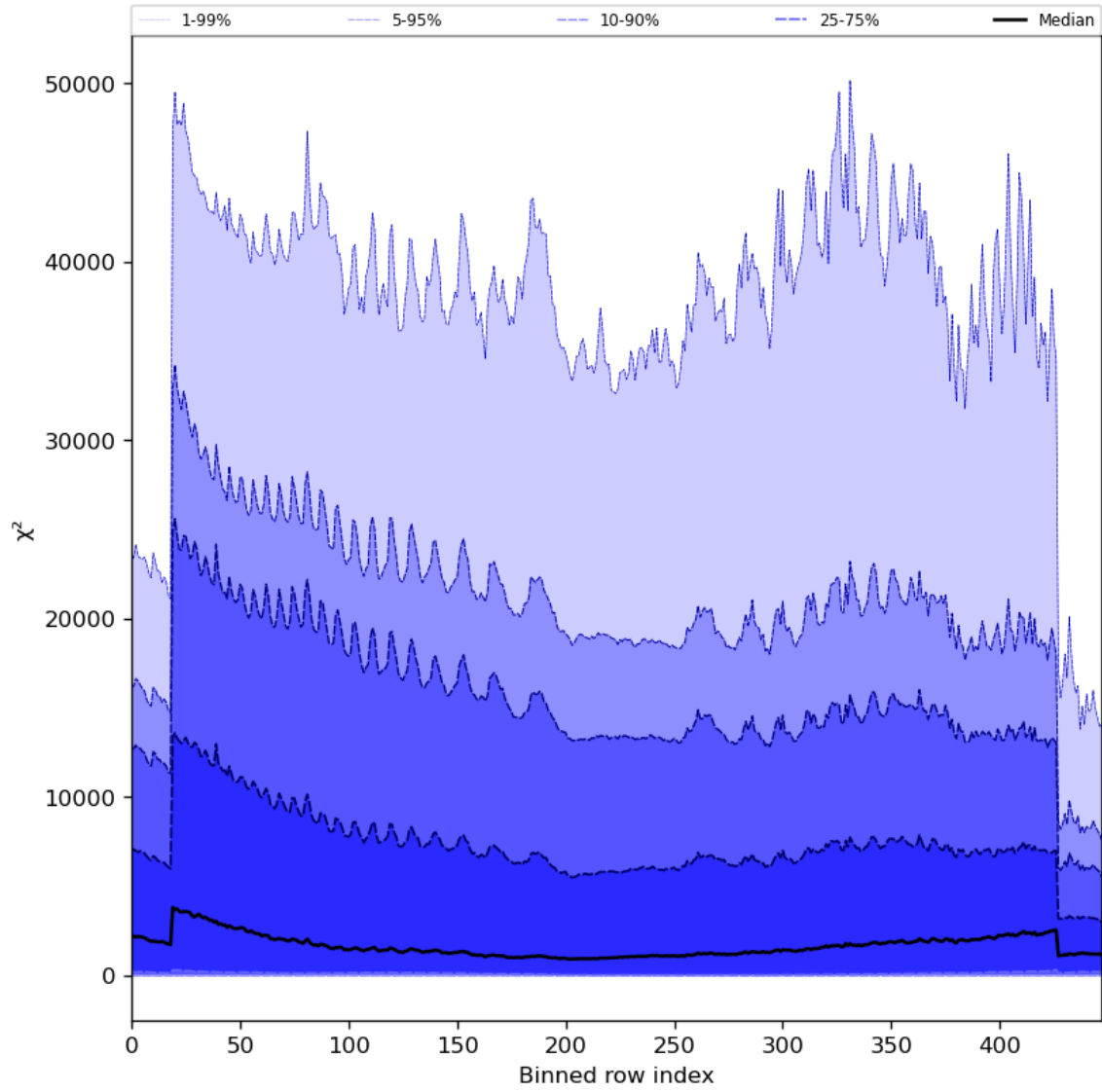
Figure 55: Along track statistics of “ \chi^2 ” for 2023-10-07 to 2023-10-09
