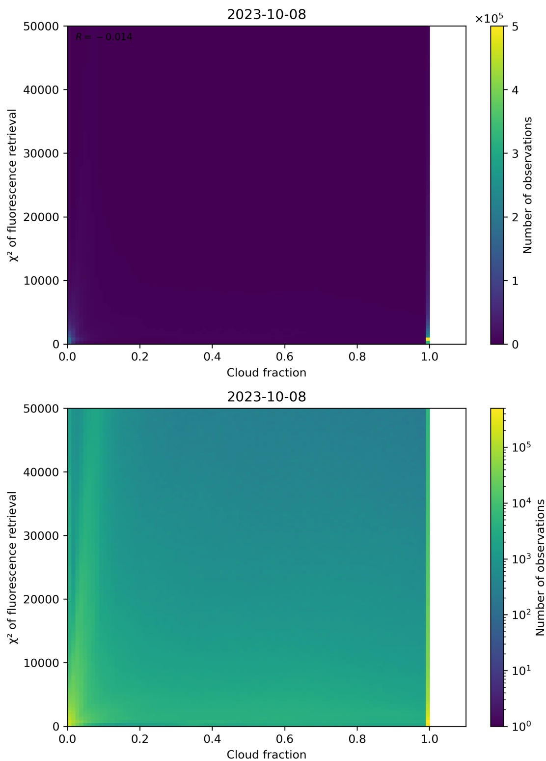
Figure 78: Scatter density plot of “Cloud fraction” against “ \chi^2 of fluorescence retrieval” for 2023-10-07 to 2023-10-09.
