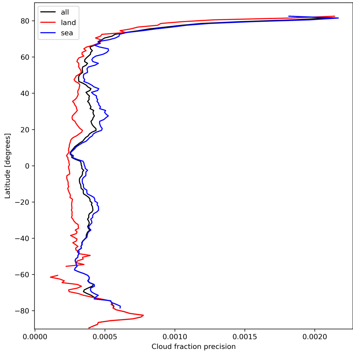
Figure 16: Zonal average of “Cloud fraction precision” for 2023-10-07 to 2023-10-09.
