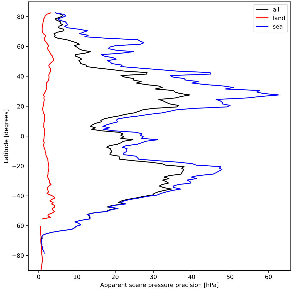
Figure 20: Zonal average of “Apparent scene pressure precision” for 2023-10-07 to 2023-10-09.
