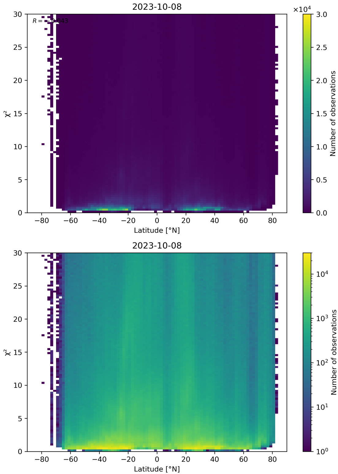
Figure 97: Scatter density plot of “Latitude” against “ \chi^2 ” for 2023-10-07 to 2023-10-09.
