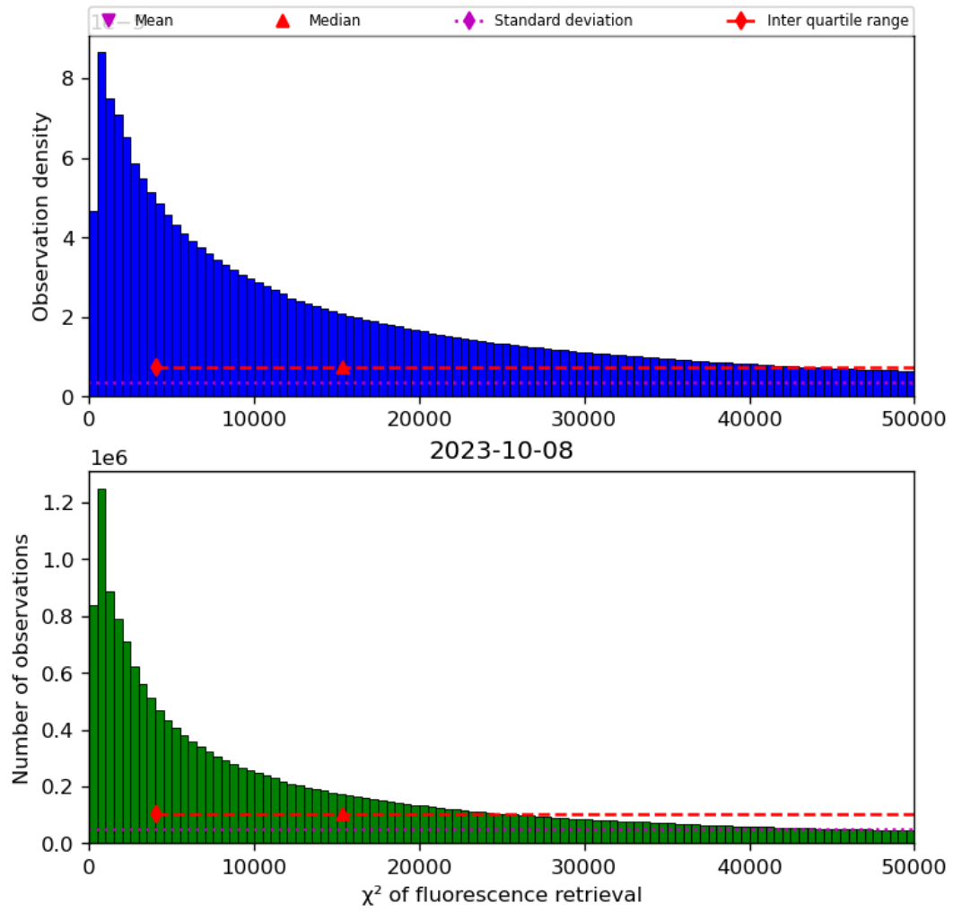
Figure 42: Histogram of “ \chi^2 of fluorescence retrieval” for 2023-10-07 to 2023-10-09
