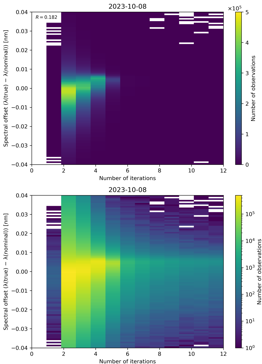
Figure 109: Scatter density plot of “Number of iterations” against “Spectral offset ( \lambda(\text{true}) - \lambda(\text{nominal}) )” for 2023-10-07 to 2023-10-09.
