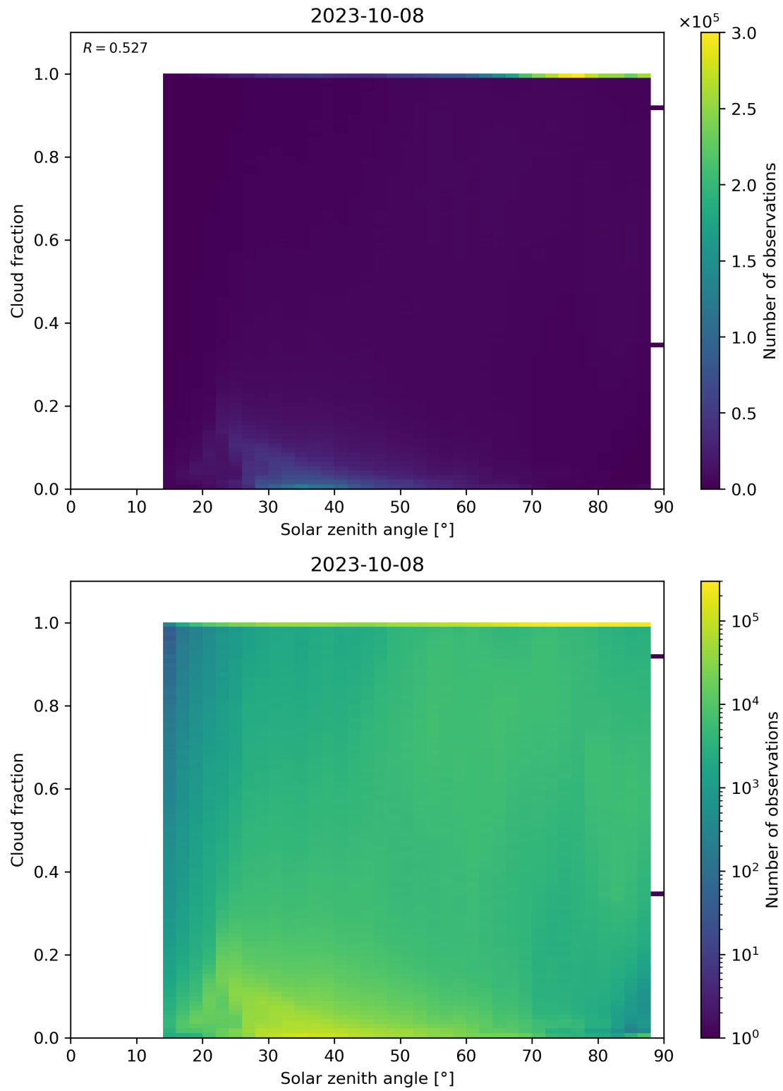
Figure 121: Scatter density plot of “Solar zenith angle” against “Cloud fraction” for 2023-10-07 to 2023-10-09.
