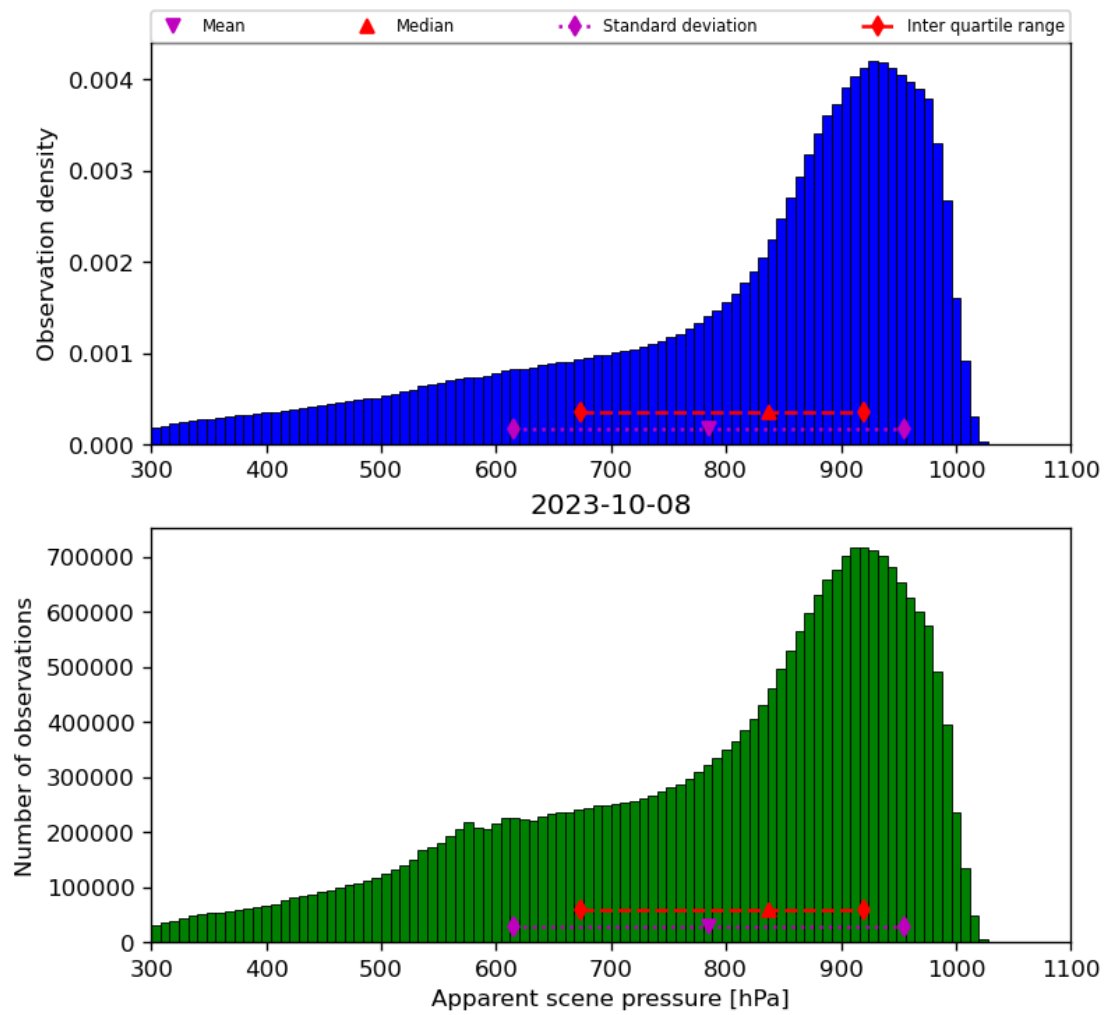
Figure 36: Histogram of “Apparent scene pressure” for 2023-10-07 to 2023-10-09
