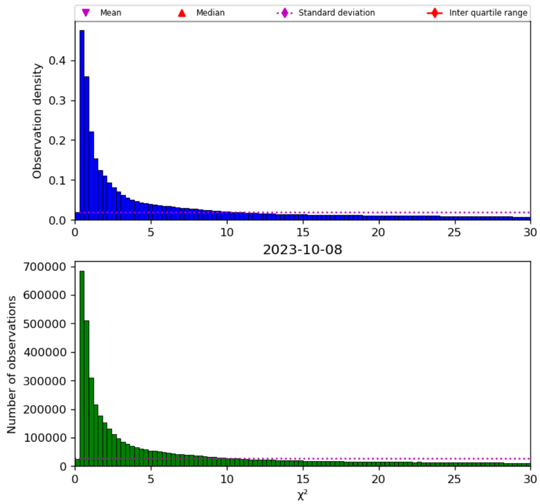
Figure 38: Histogram of “ \chi^2 ” for 2023-10-07 to 2023-10-09
