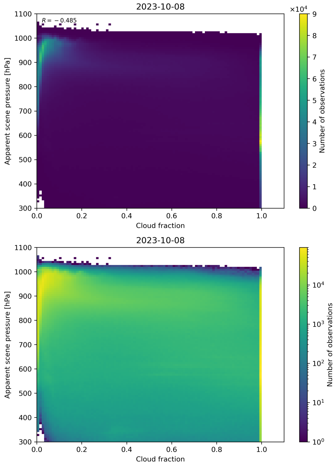
Figure 76: Scatter density plot of “Cloud fraction” against “Apparent scene pressure” for 2023-10-07 to 2023-10-09.
