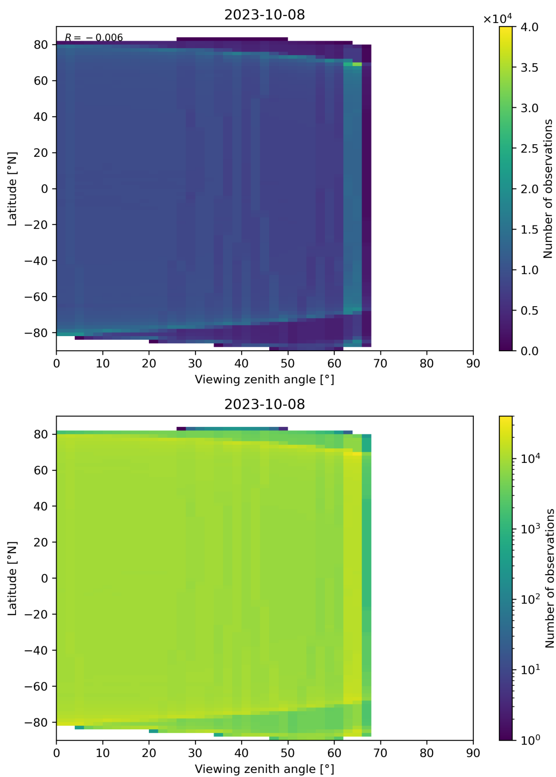
Figure 135: Scatter density plot of “Viewing zenith angle” against “Latitude” for 2023-10-07 to 2023-10-09.
