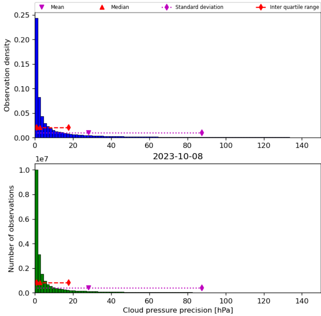
Figure 31: Histogram of “Cloud pressure precision” for 2023-10-07 to 2023-10-09
