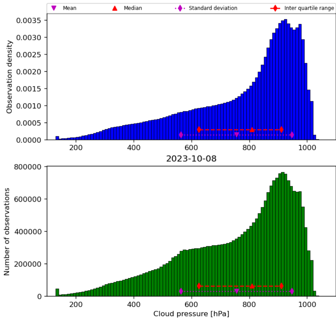
Figure 30: Histogram of “Cloud pressure” for 2023-10-07 to 2023-10-09
