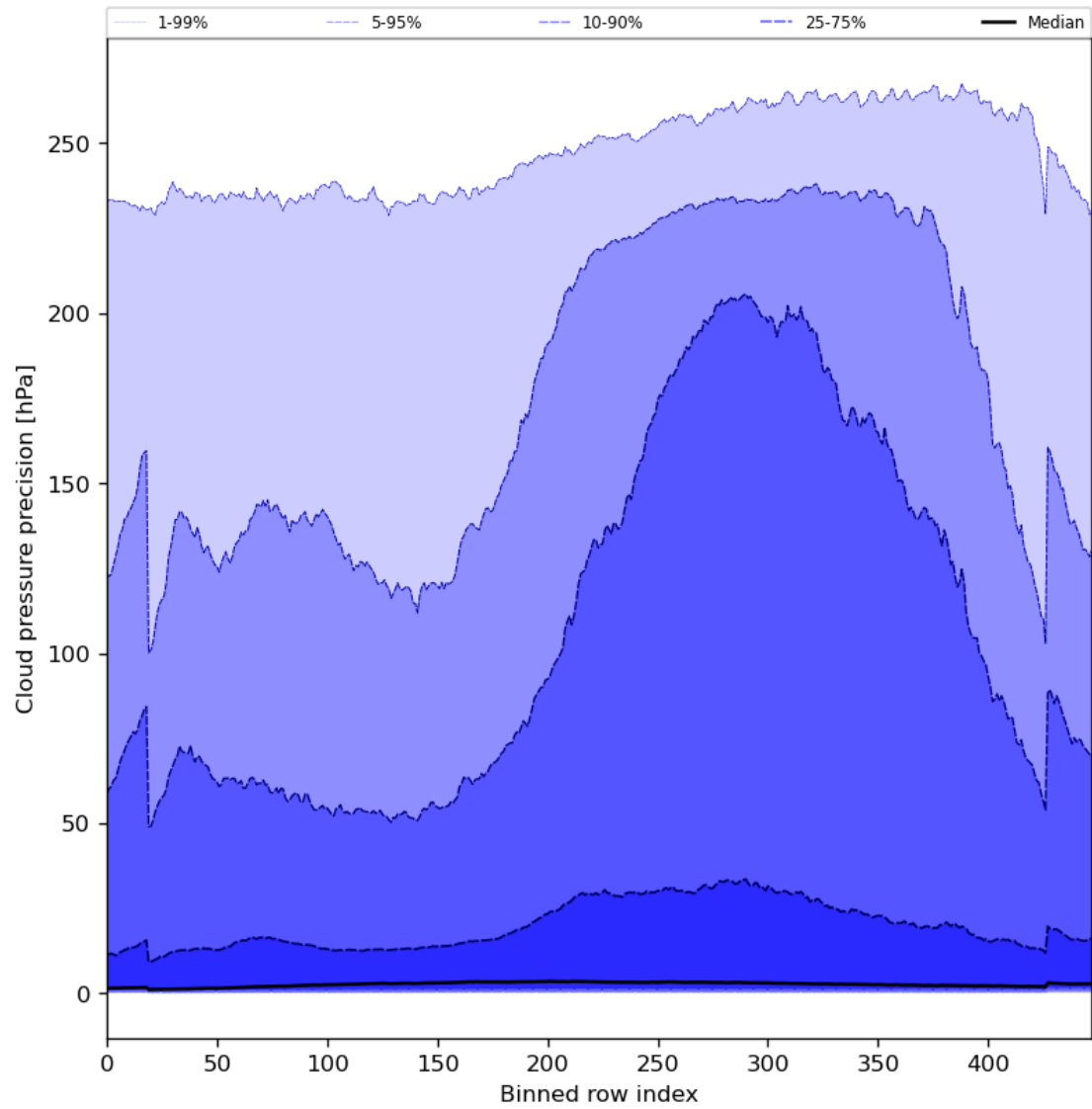
Figure 48: Along track statistics of “Cloud pressure precision” for 2023-10-07 to 2023-10-09
