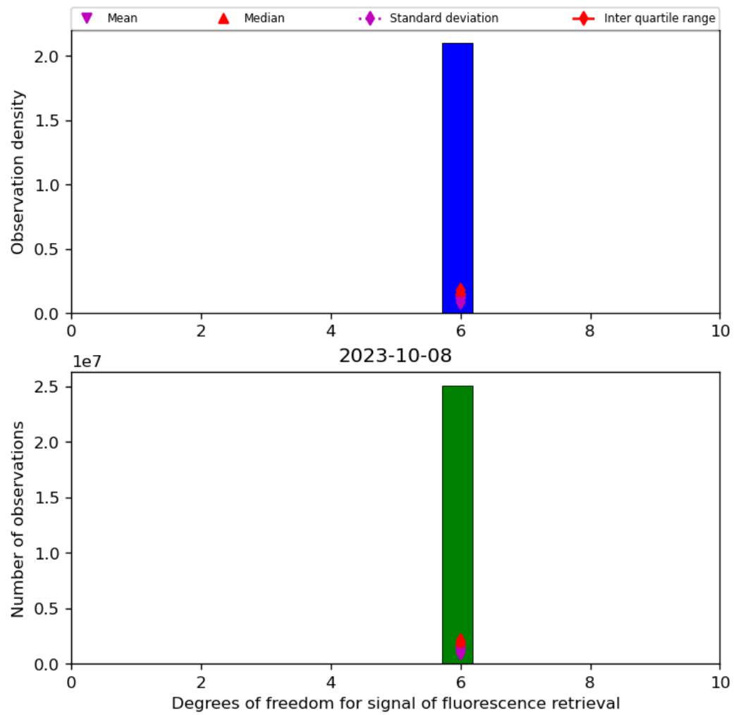
Figure 43: Histogram of “Degrees of freedom for signal of fluorescence retrieval” for 2023-10-07 to 2023-10-09
