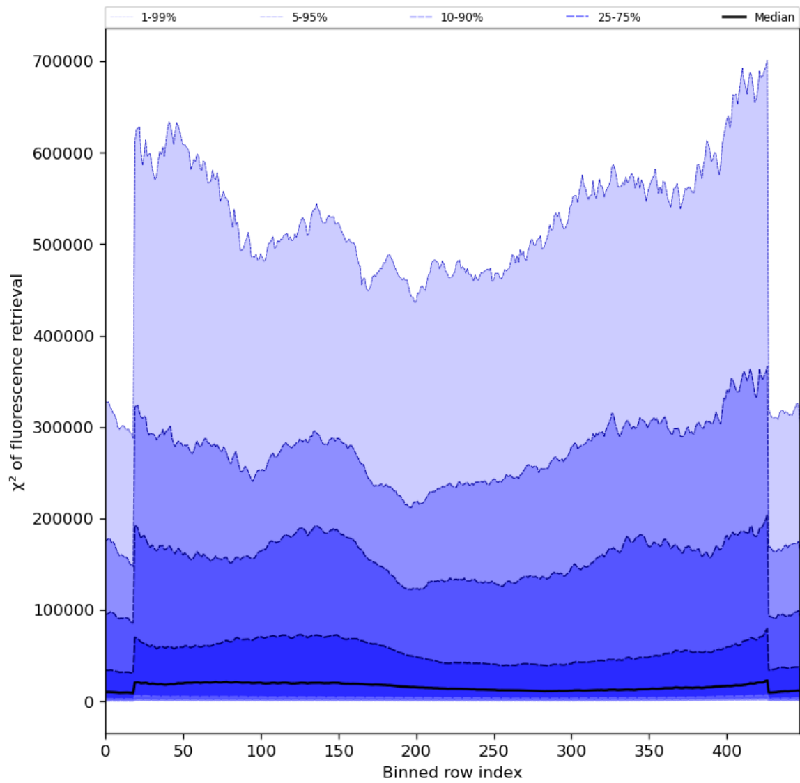
Figure 59: Along track statistics of “ \chi^2 of fluorescence retrieval” for 2023-10-07 to 2023-10-09
