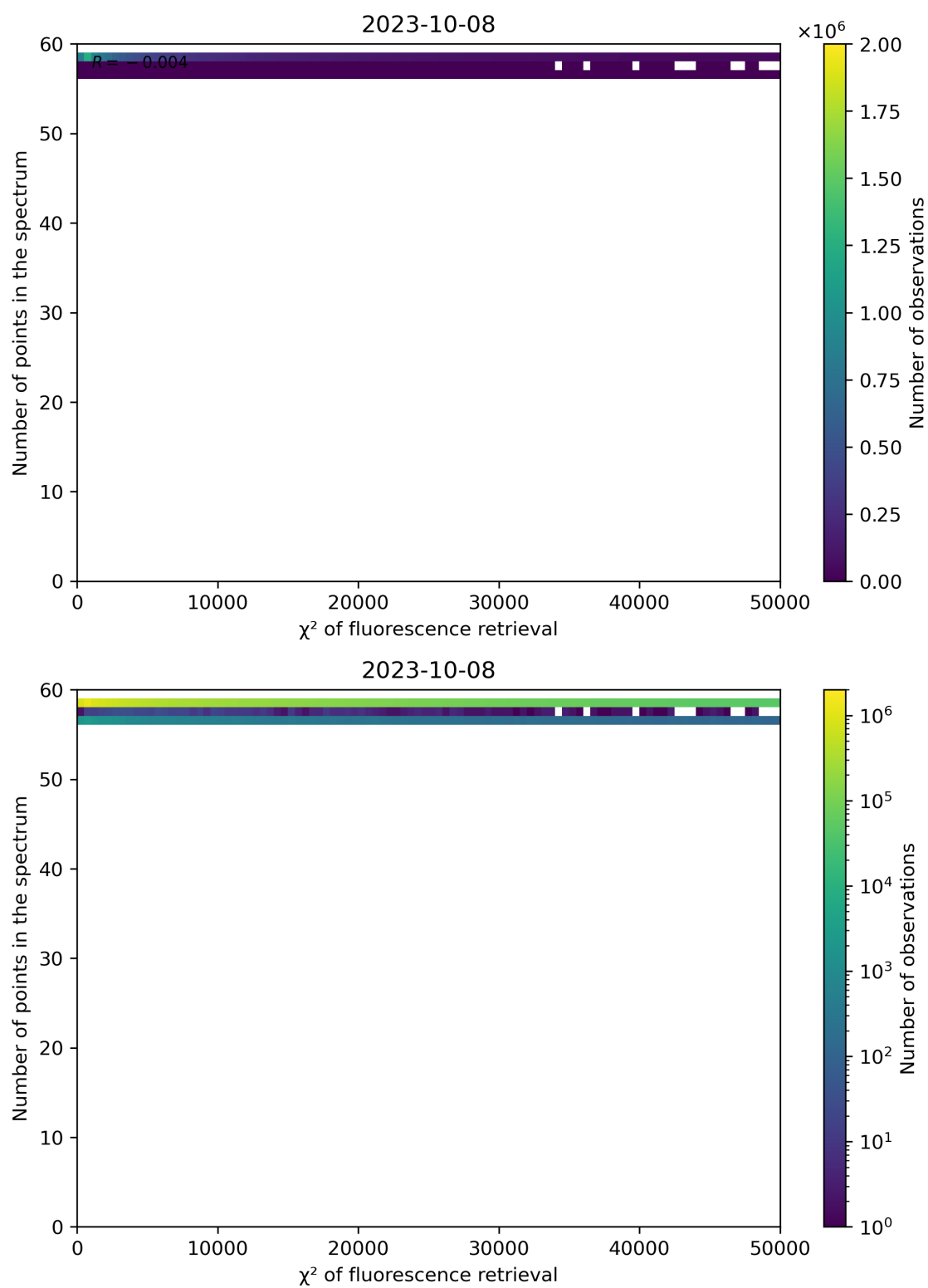
Figure 71: Scatter density plot of " \chi^2 of fluorescence retrieval" against "Number of points in the spectrum" for 2023-10-07 to 2023-10-09.
