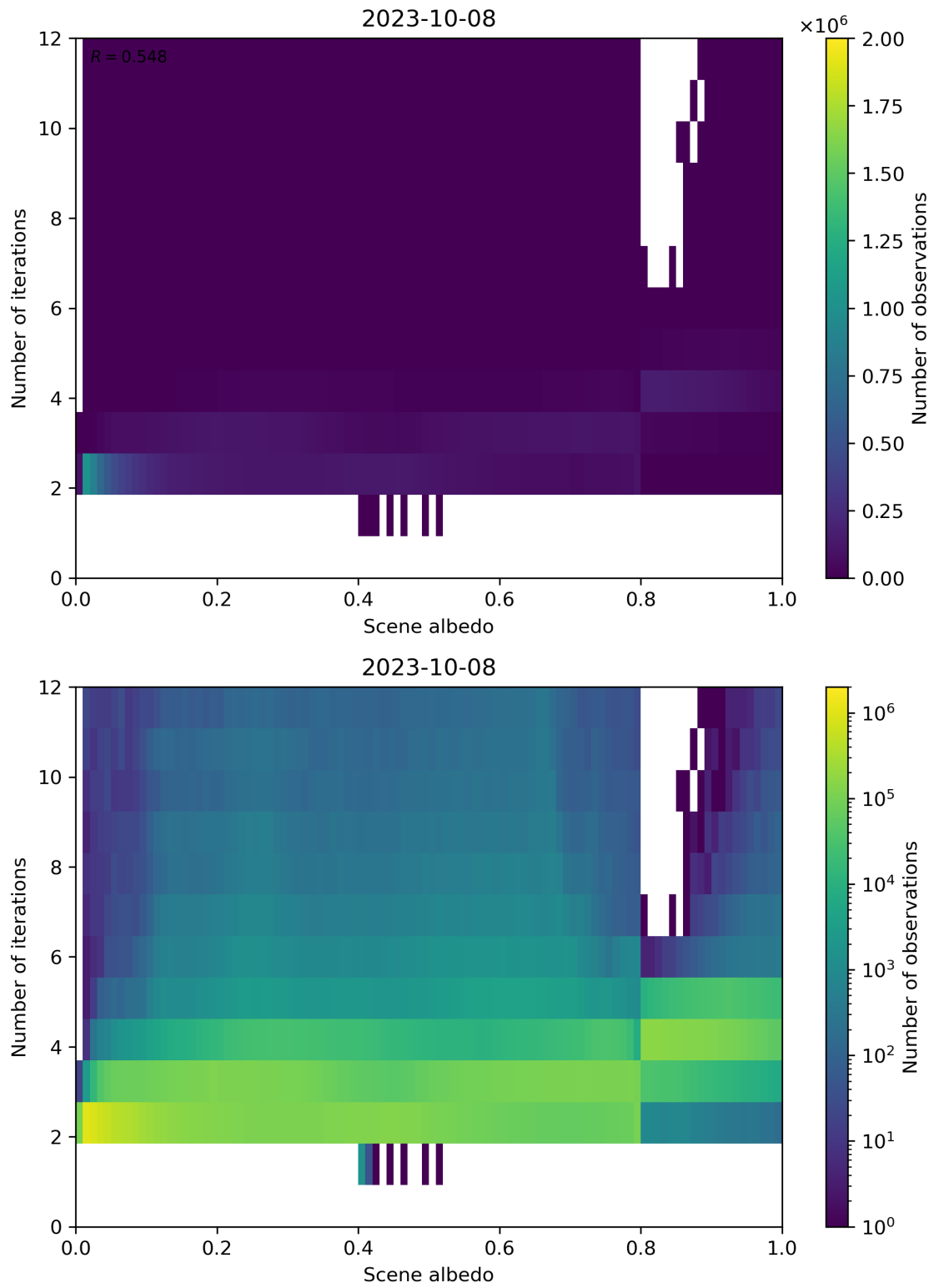
Figure 115: Scatter density plot of “Scene albedo” against “Number of iterations” for 2023-10-07 to 2023-10-09.
