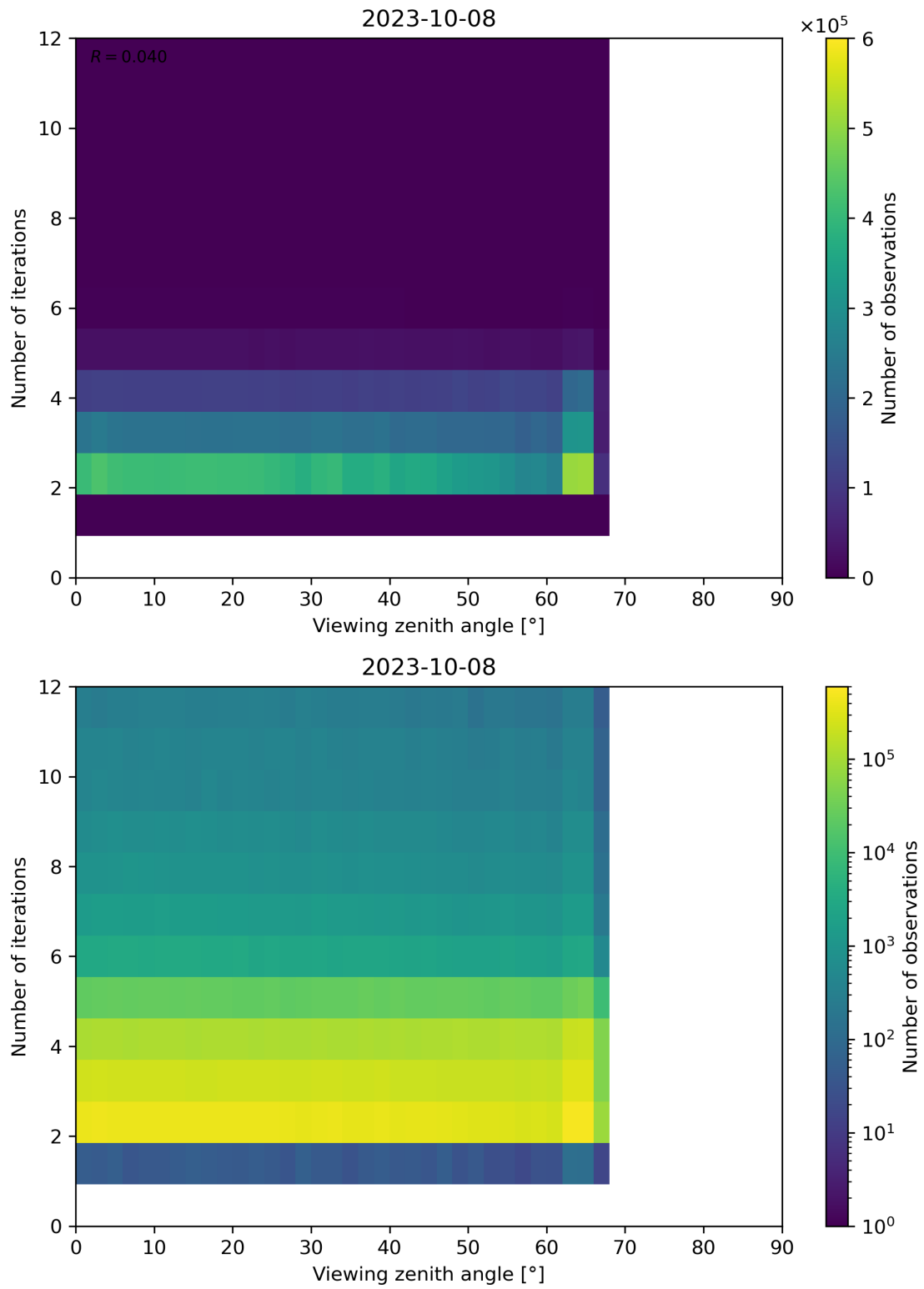
Figure 136: Scatter density plot of “Viewing zenith angle” against “Number of iterations” for 2023-10-07 to 2023-10-09.
