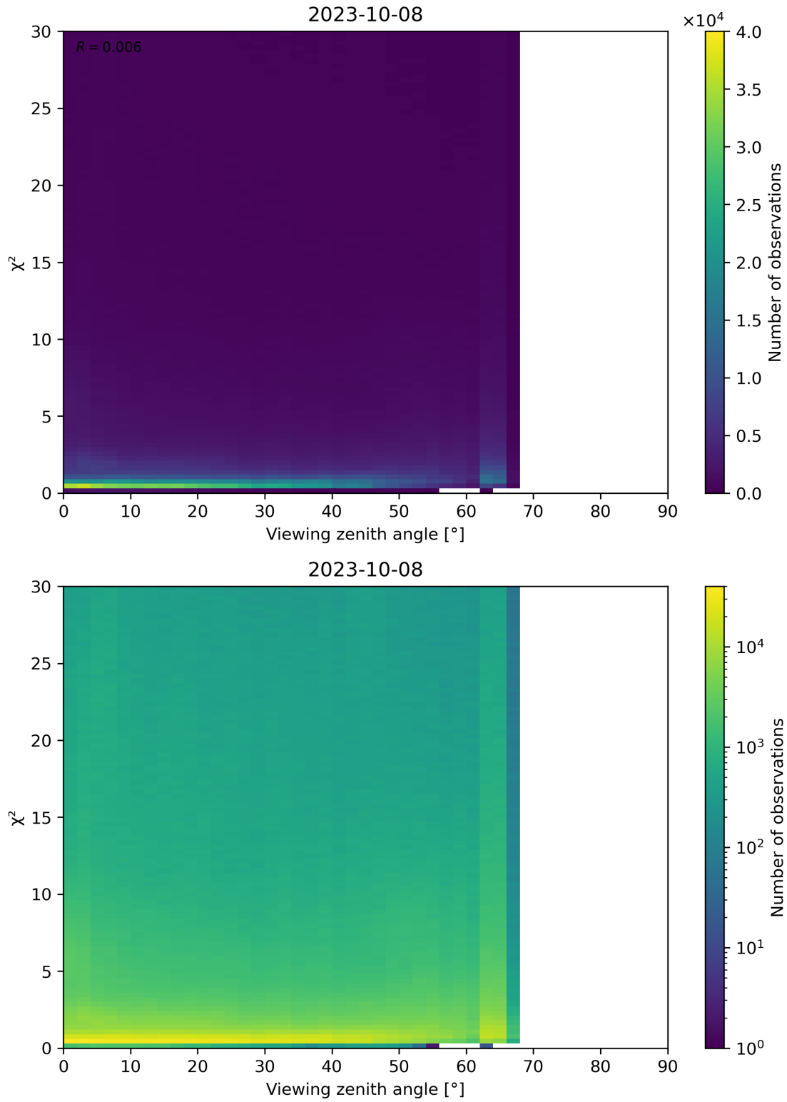
Figure 130: Scatter density plot of “Viewing zenith angle” against “ \chi^2 ” for 2023-10-07 to 2023-10-09.
