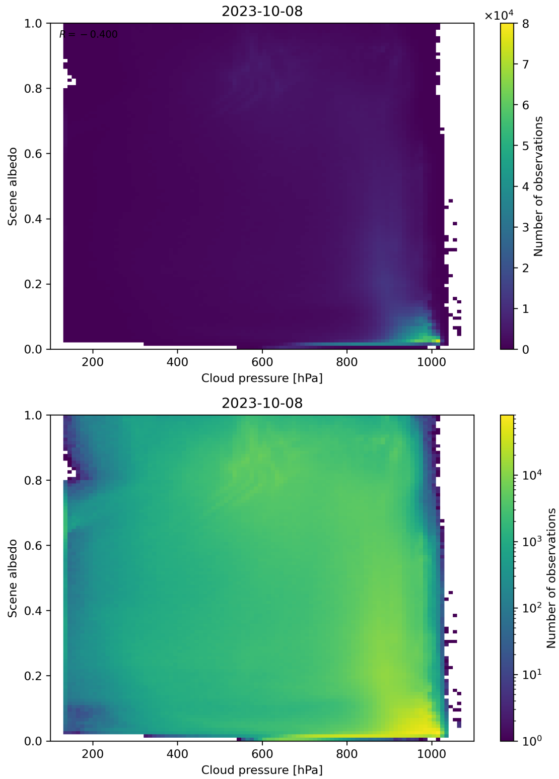
Figure 91: Scatter density plot of “Cloud pressure” against “Scene albedo” for 2023-10-07 to 2023-10-09.
