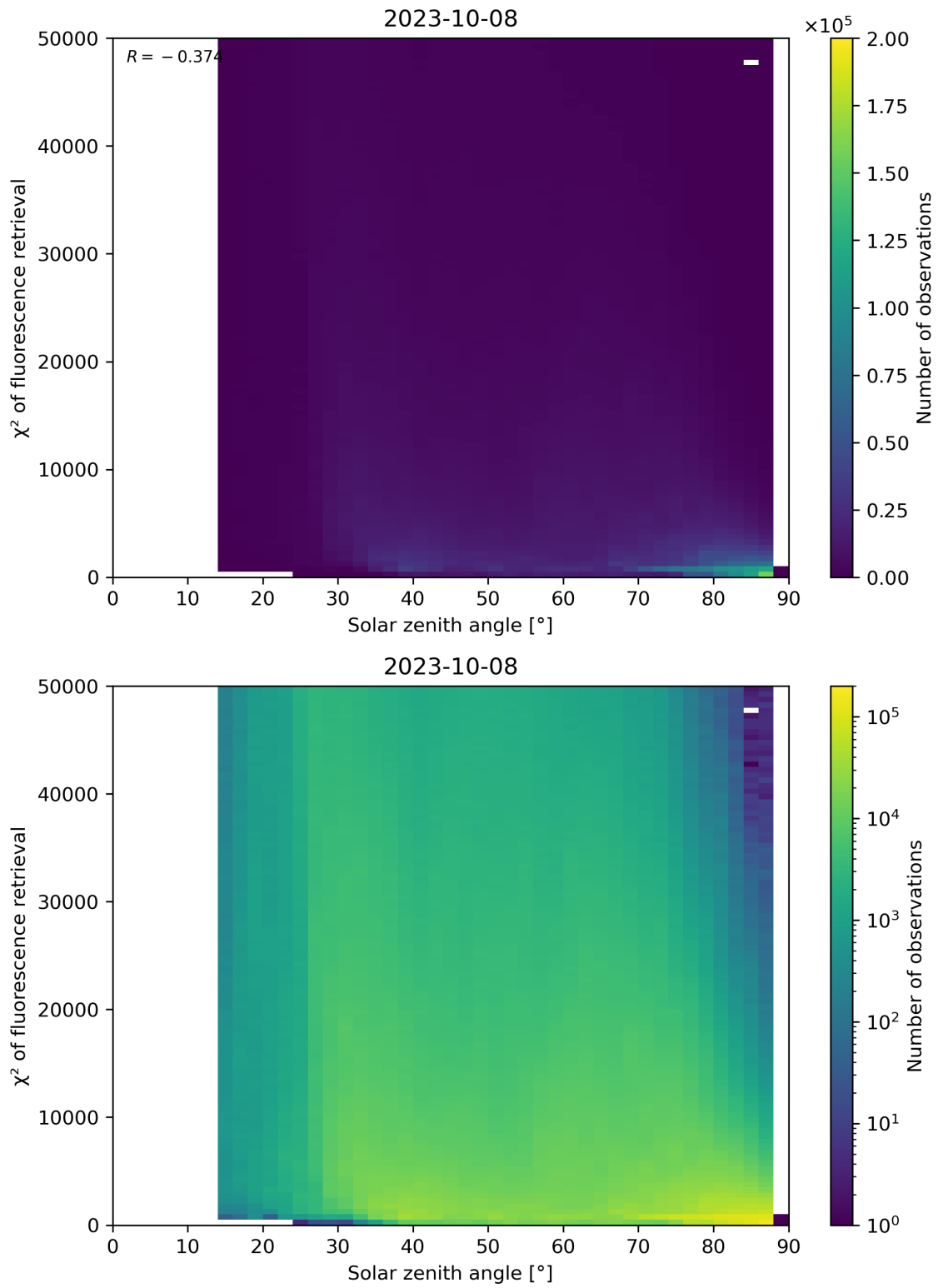
Figure 120: Scatter density plot of “Solar zenith angle” against “ \chi^2 of fluorescence retrieval” for 2023-10-07 to 2023-10-09.
