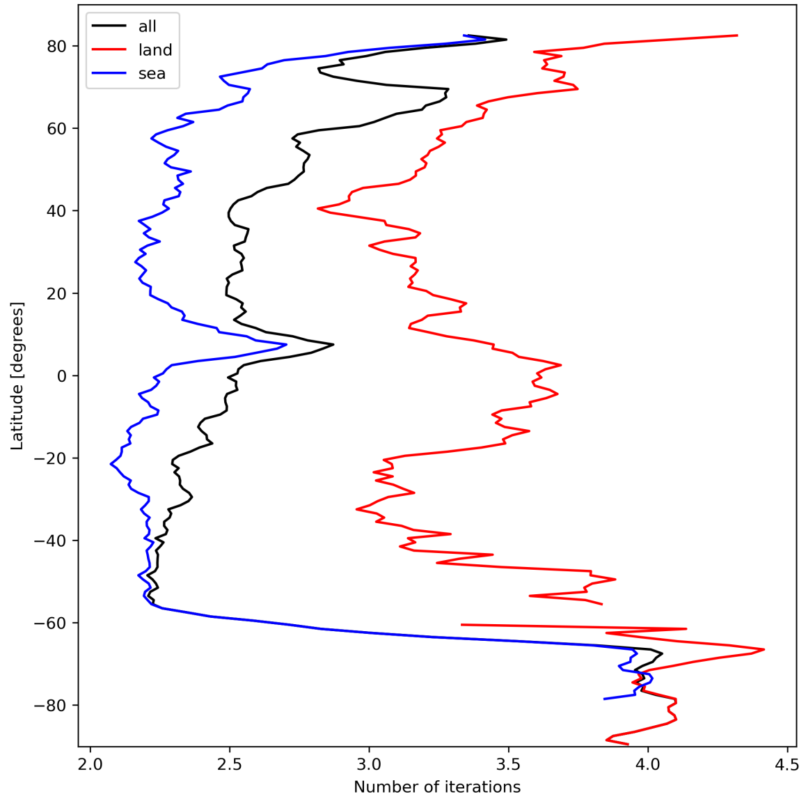
Figure 22: Zonal average of “Number of iterations” for 2023-10-07 to 2023-10-09.
