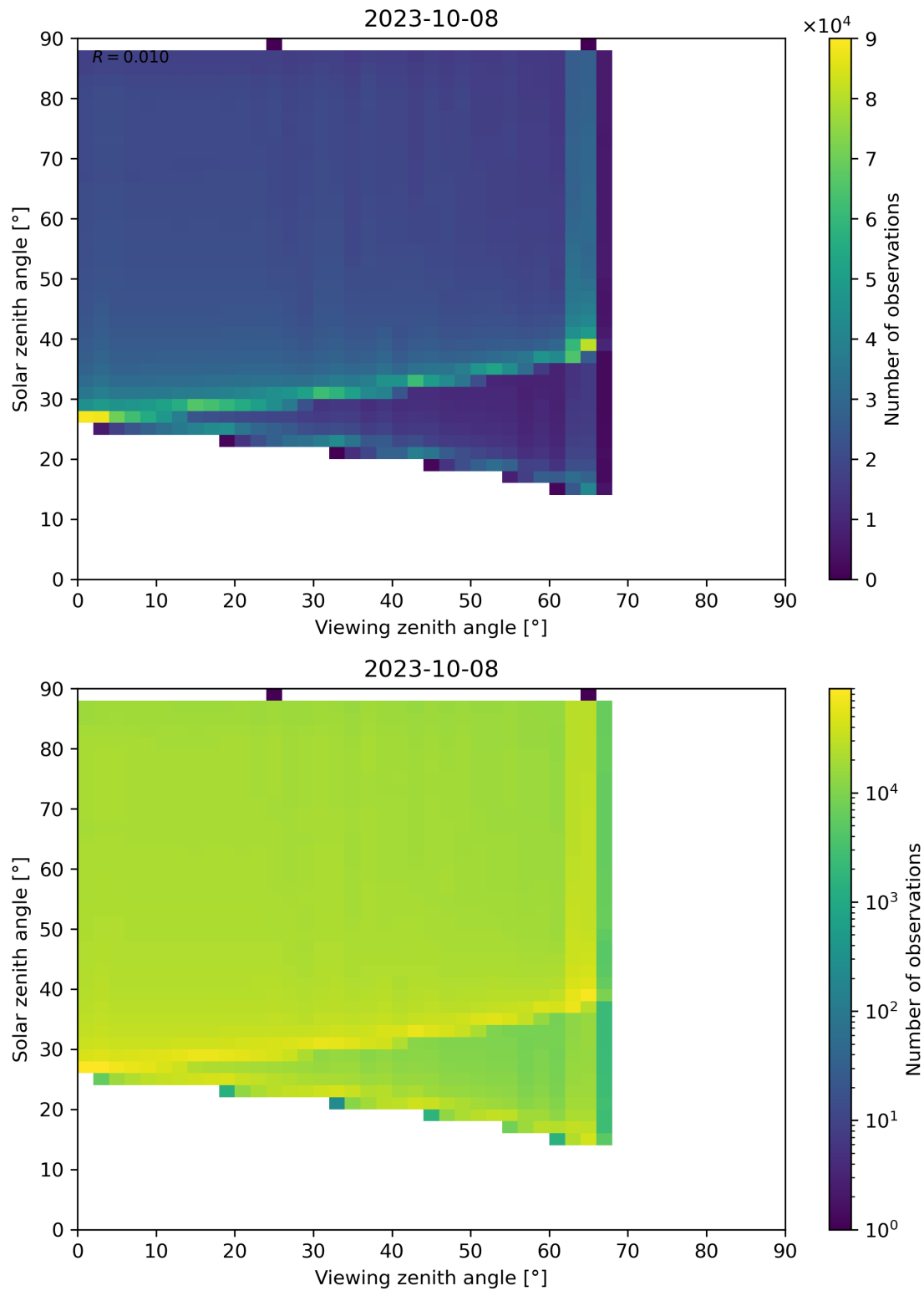
Figure 139: Scatter density plot of “Viewing zenith angle” against “Solar zenith angle” for 2023-10-07 to 2023-10-09.
