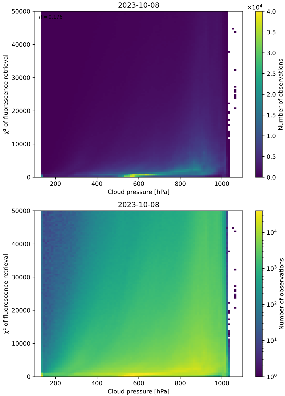
Figure 86: Scatter density plot of “Cloud pressure” against “ \chi^2 of fluorescence retrieval” for 2023-10-07 to 2023-10-09.
