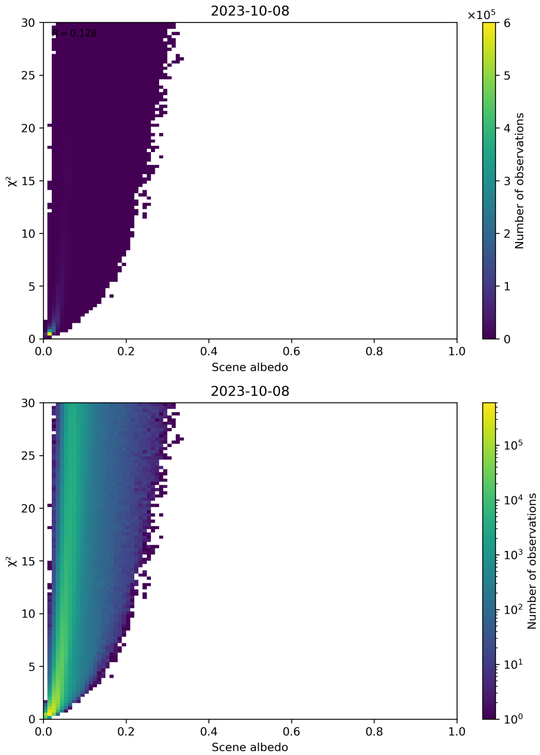
Figure 112: Scatter density plot of “Scene albedo” against “ \chi^2 ” for 2023-10-07 to 2023-10-09.
