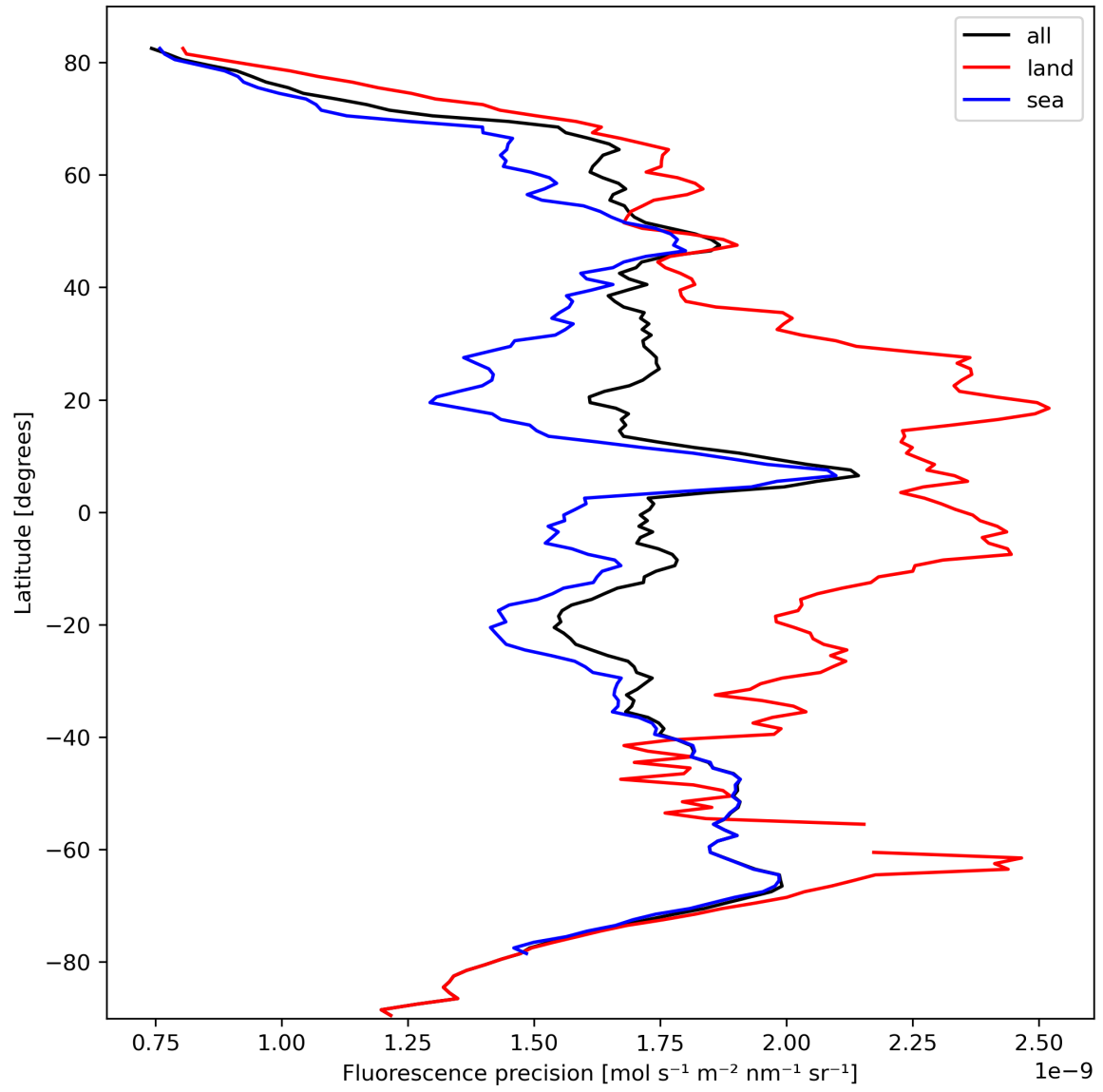
Figure 24: Zonal average of “Fluorescence precision” for 2023-10-07 to 2023-10-09.
