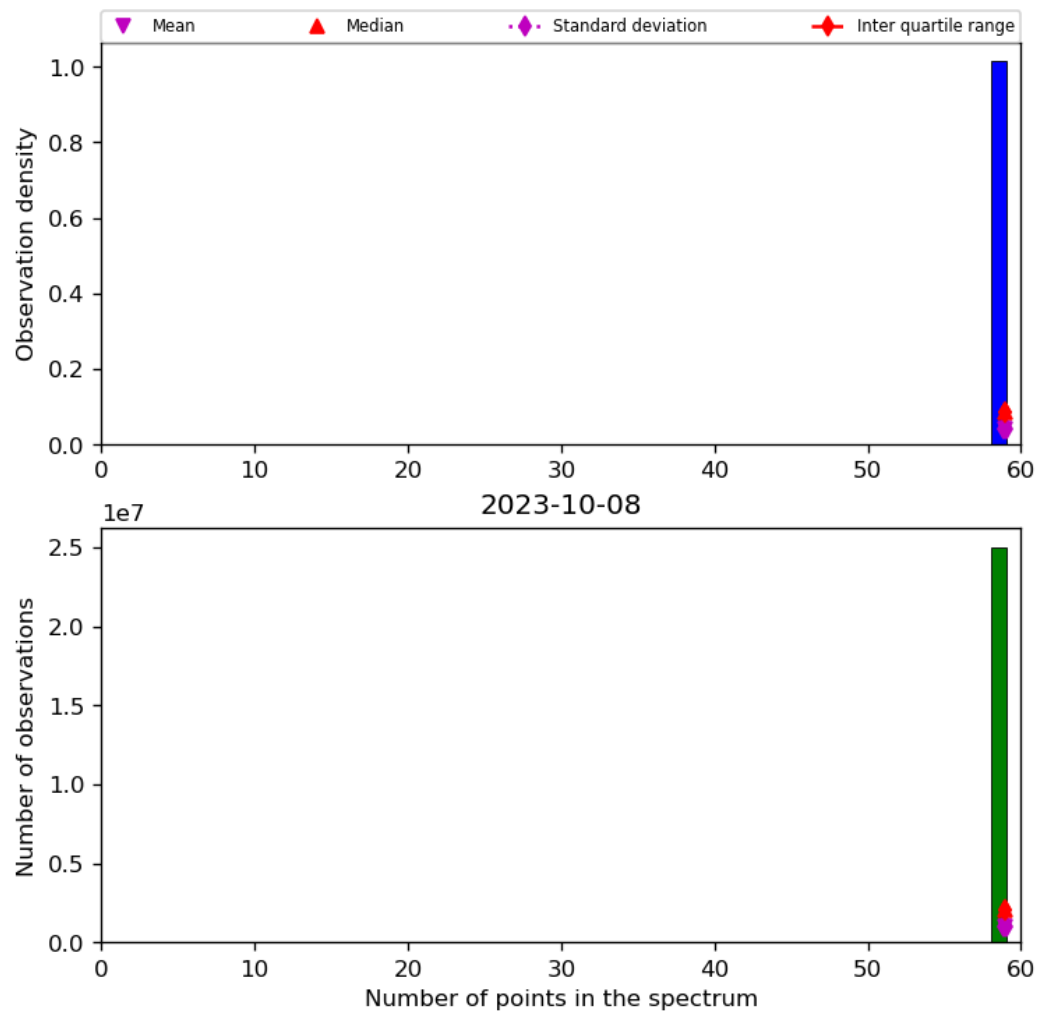
Figure 44: Histogram of “Number of points in the spectrum” for 2023-10-07 to 2023-10-09
