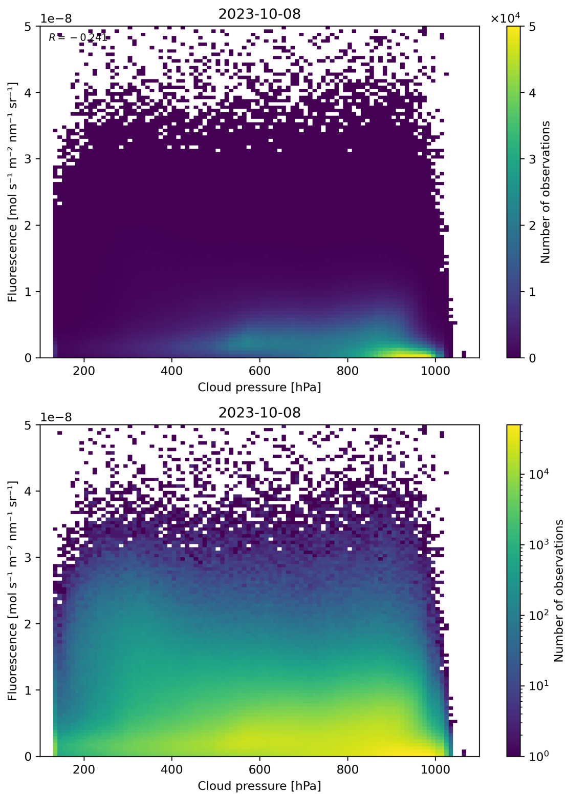
Figure 88: Scatter density plot of “Cloud pressure” against “Fluorescence” for 2023-10-07 to 2023-10-09.
