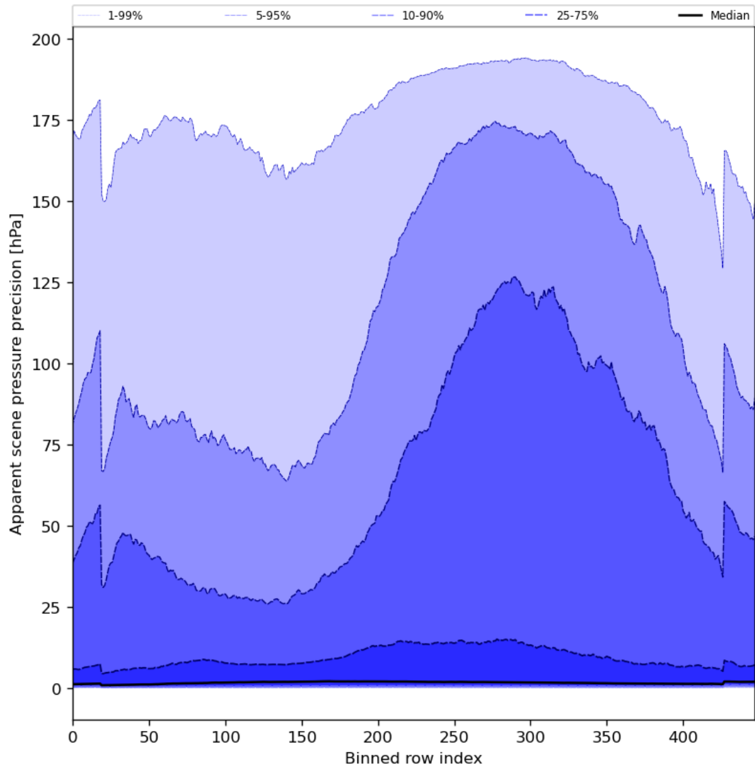
Figure 54: Along track statistics of “Apparent scene pressure precision” for 2023-10-07 to 2023-10-09
