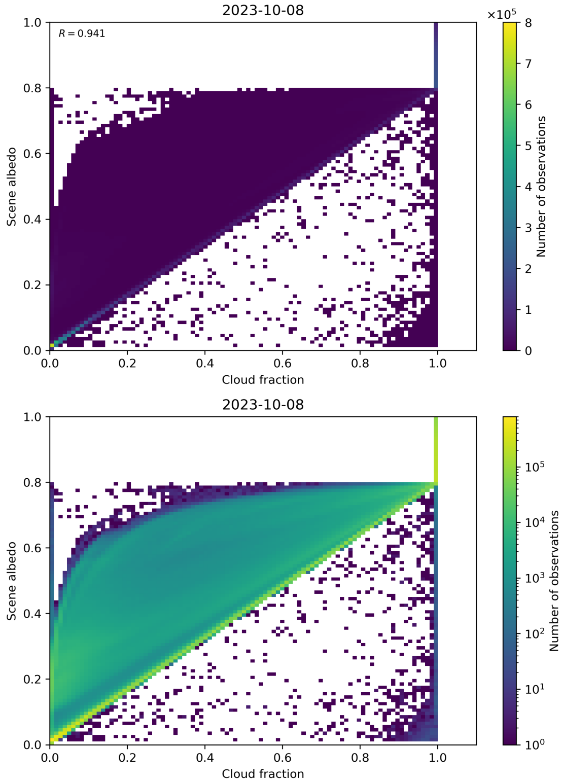
Figure 82: Scatter density plot of “Cloud fraction” against “Scene albedo” for 2023-10-07 to 2023-10-09.
