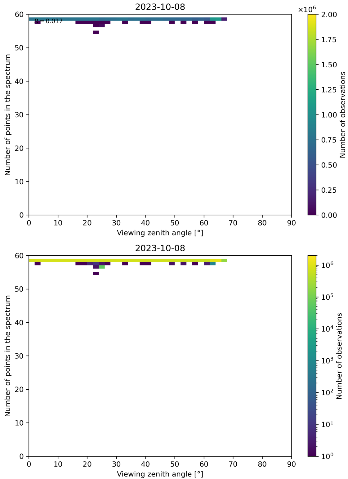
Figure 137: Scatter density plot of “Viewing zenith angle” against “Number of points in the spectrum” for 2023-10-07 to 2023-10-09.
