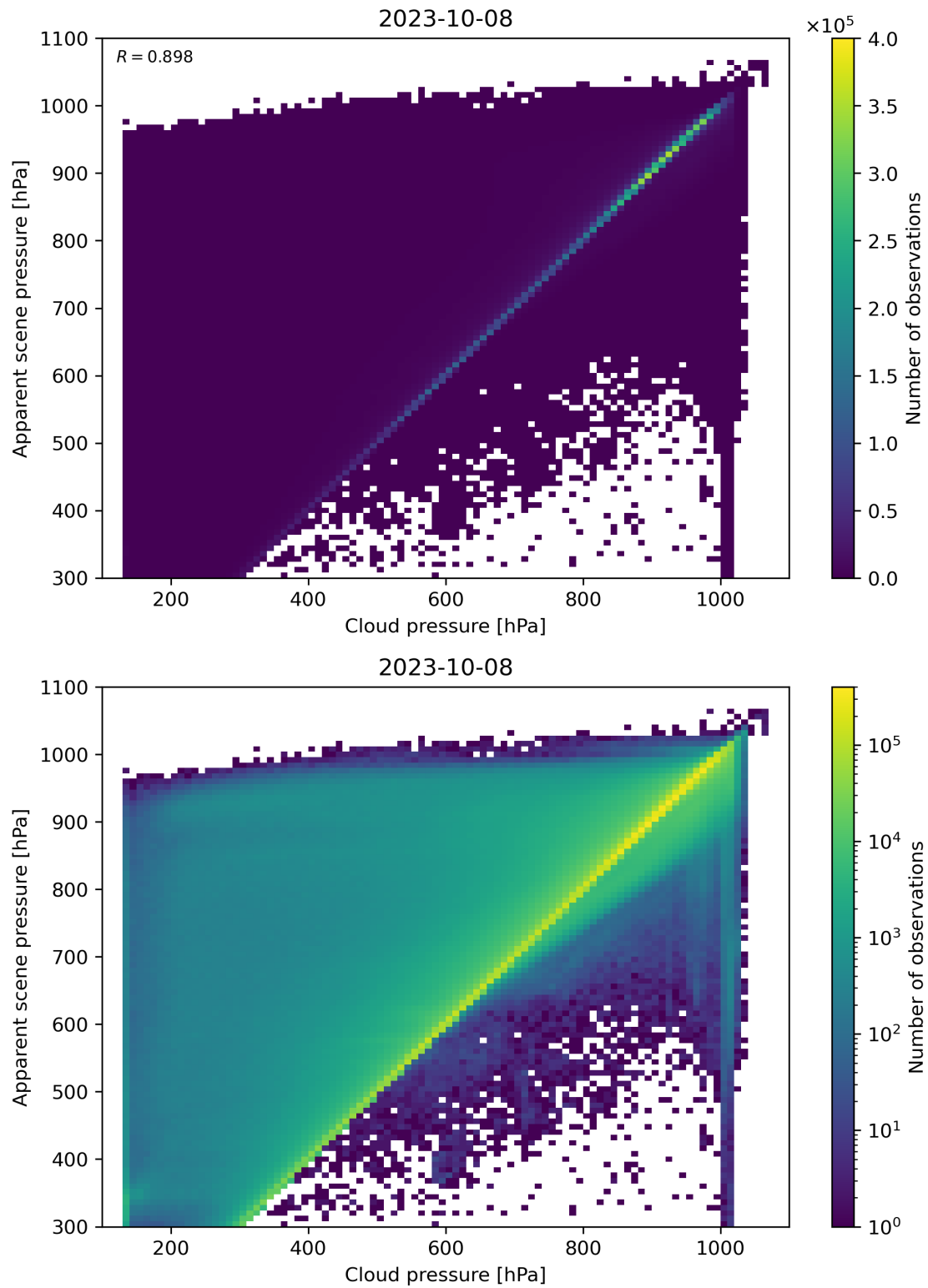
Figure 84: Scatter density plot of “Cloud pressure” against “Apparent scene pressure” for 2023-10-07 to 2023-10-09.
