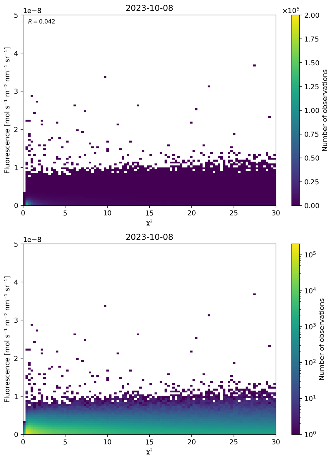
Figure 70: Scatter density plot of “ \chi^2 ” against “Fluorescence” for 2023-10-07 to 2023-10-09.
