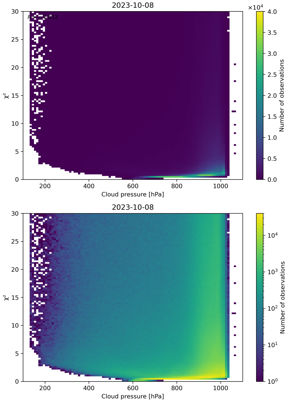
Figure 85: Scatter density plot of “Cloud pressure” against “ \chi^2 ” for 2023-10-07 to 2023-10-09.
