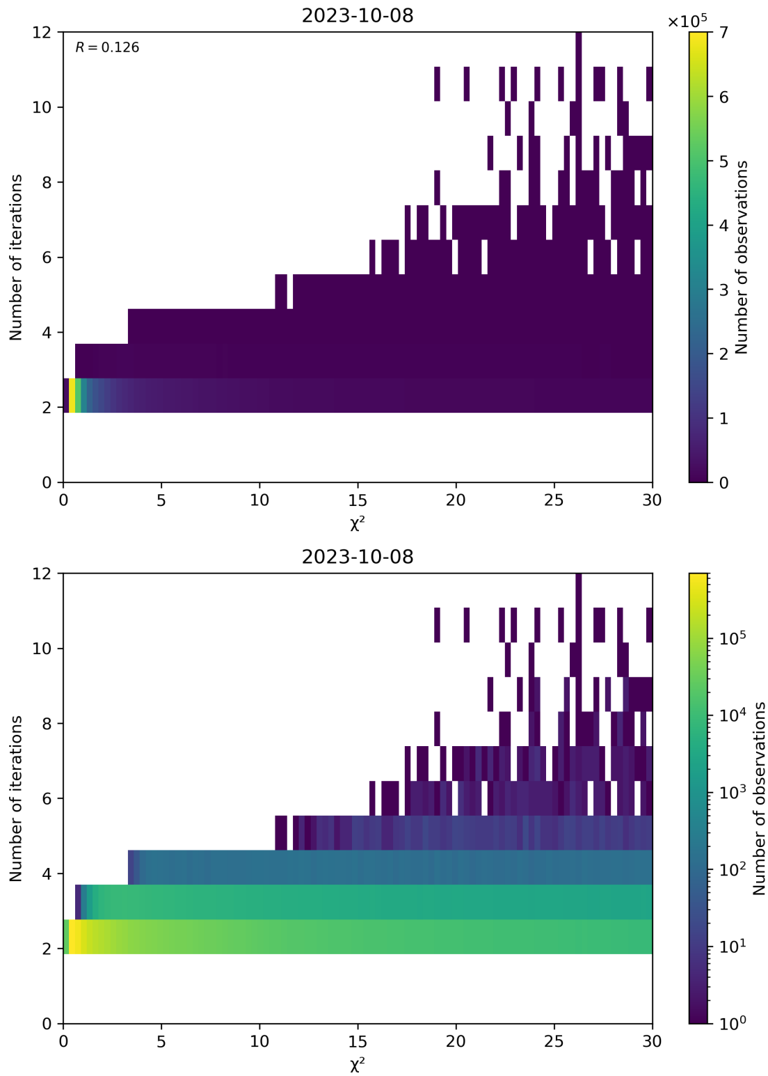
Figure 73: Scatter density plot of " \chi^2 " against "Number of iterations" for 2023-10-07 to 2023-10-09.
