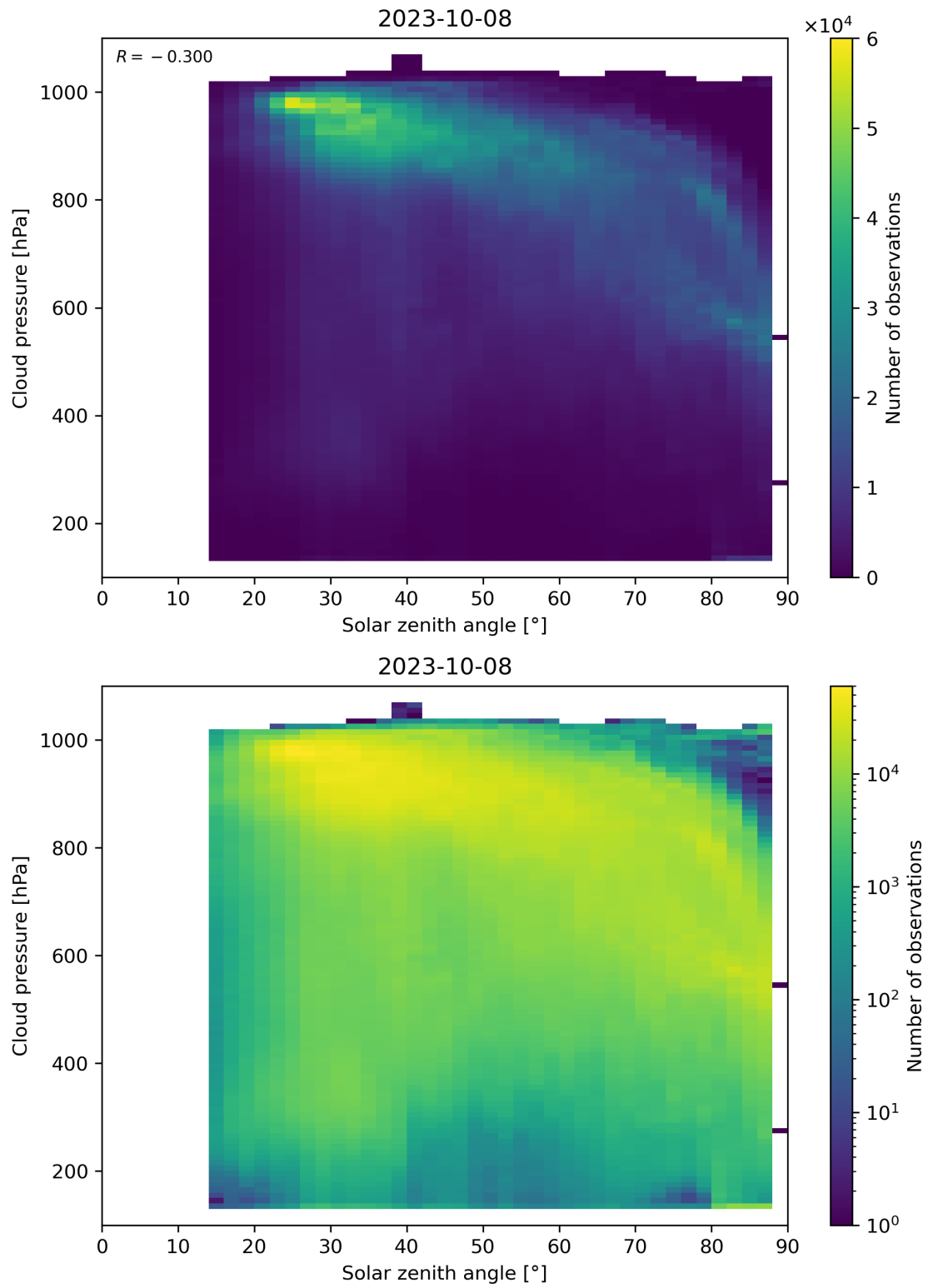
Figure 122: Scatter density plot of “Solar zenith angle” against “Cloud pressure” for 2023-10-07 to 2023-10-09.
