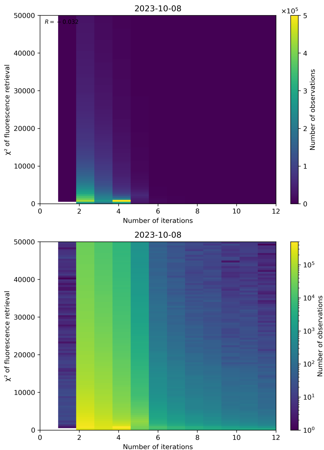
Figure 106: Scatter density plot of “Number of iterations” against “ \chi^2 of fluorescence retrieval” for 2023-10-07 to 2023-10-09.
