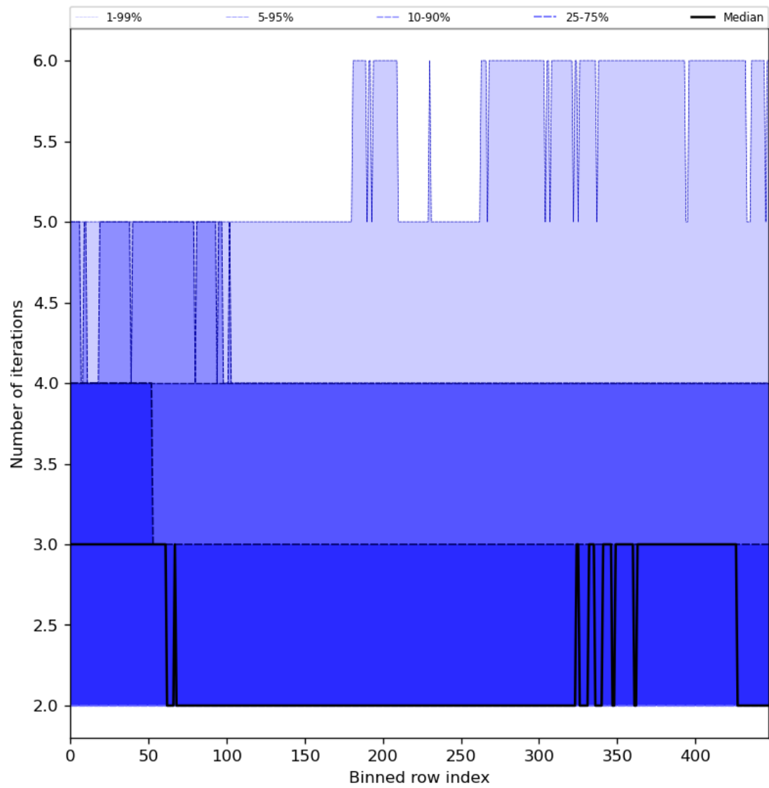
Figure 56: Along track statistics of “Number of iterations” for 2023-10-07 to 2023-10-09
