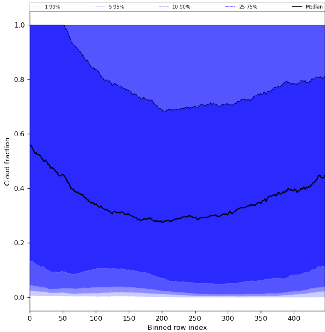
Figure 49: Along track statistics of “Cloud fraction” for 2023-10-07 to 2023-10-09
