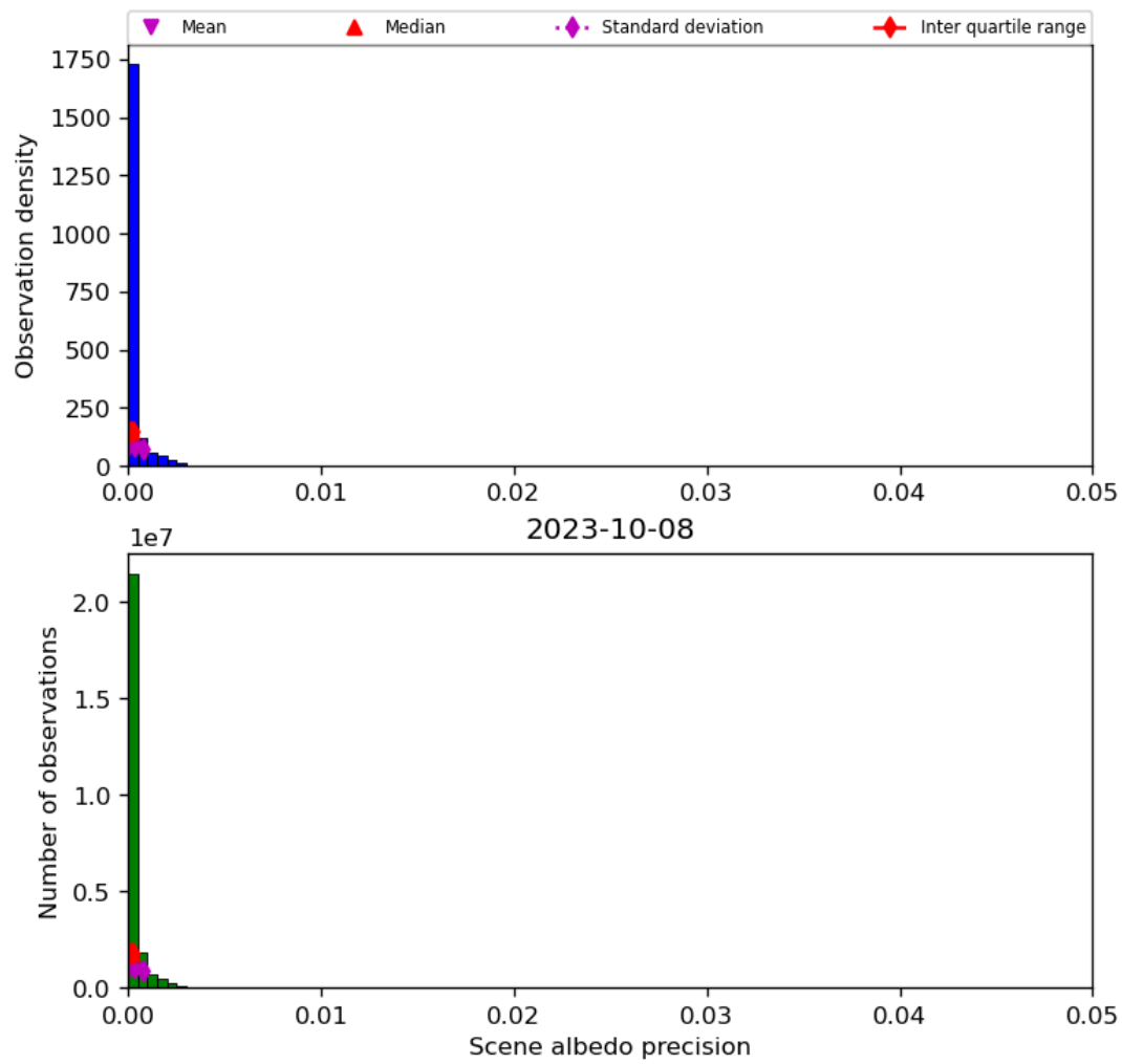
Figure 35: Histogram of “Scene albedo precision” for 2023-10-07 to 2023-10-09
