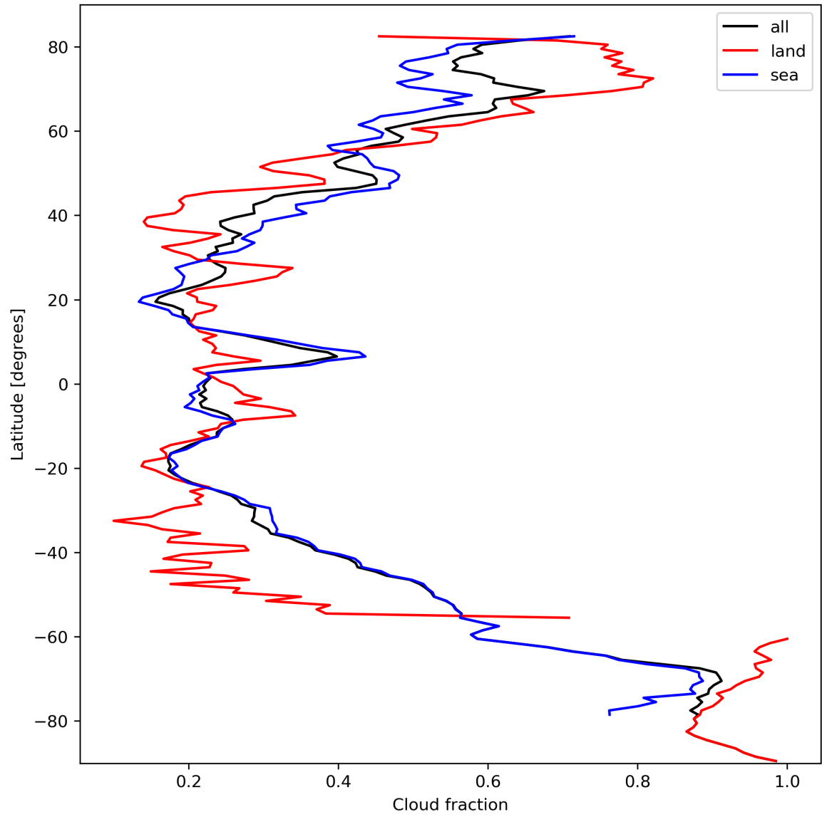
Figure 15: Zonal average of “Cloud fraction” for 2023-10-07 to 2023-10-09.
