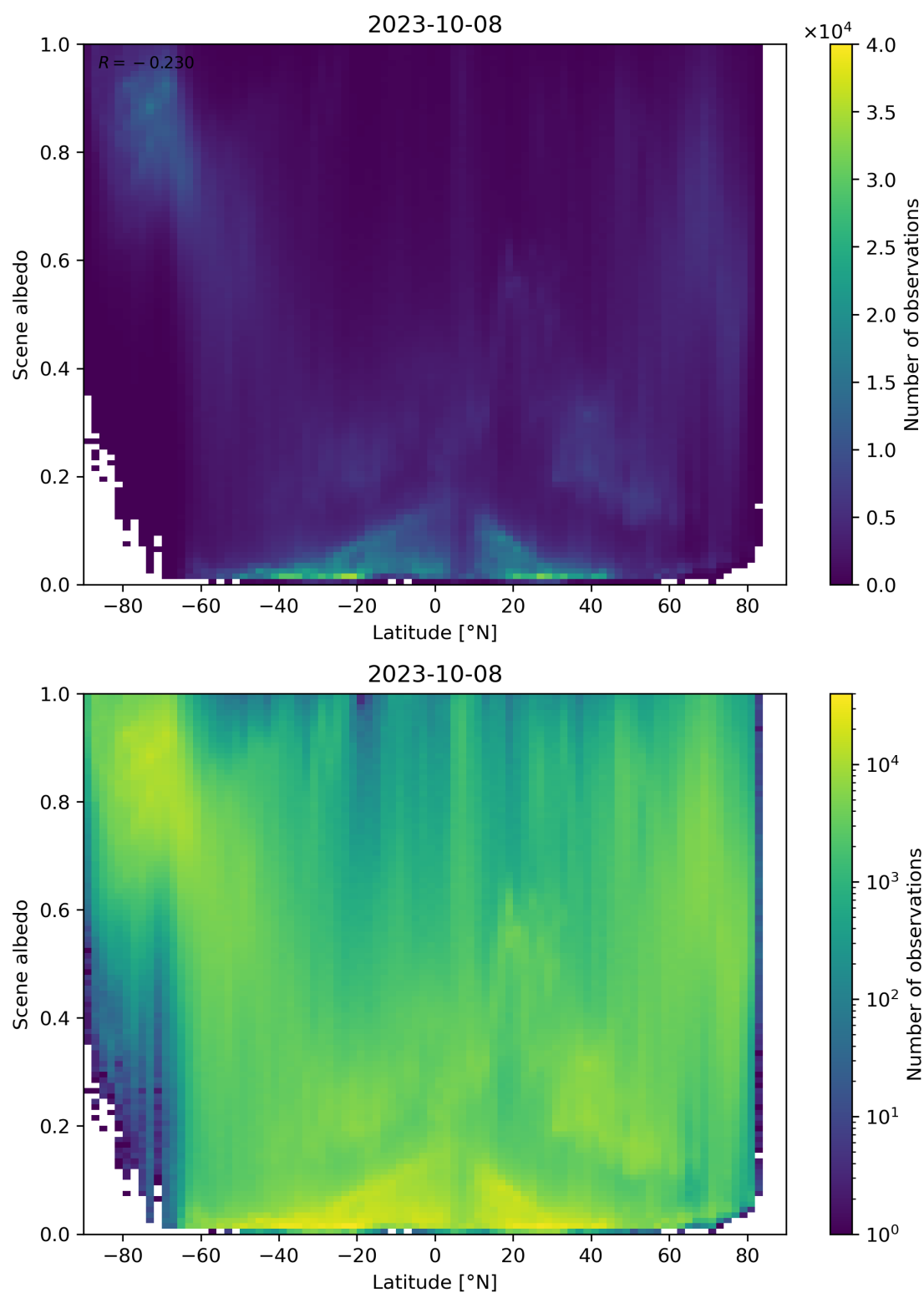
Figure 104: Scatter density plot of “Latitude” against “Scene albedo” for 2023-10-07 to 2023-10-09.
