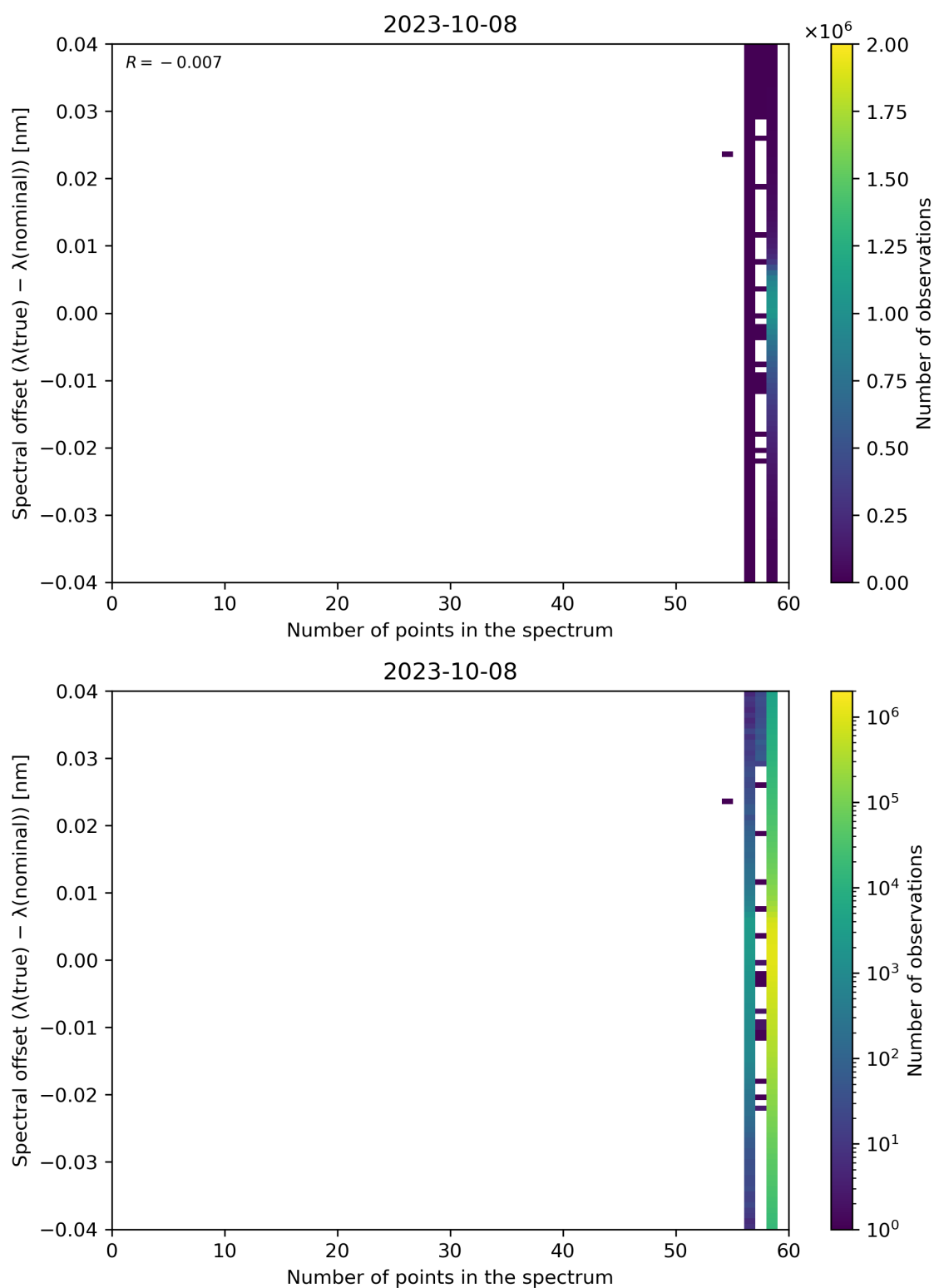
Figure 110: Scatter density plot of “Number of points in the spectrum” against “Spectral offset ( \lambda(\text{true}) - \lambda(\text{nominal}) )” for 2023-10-07 to 2023-10-09.
