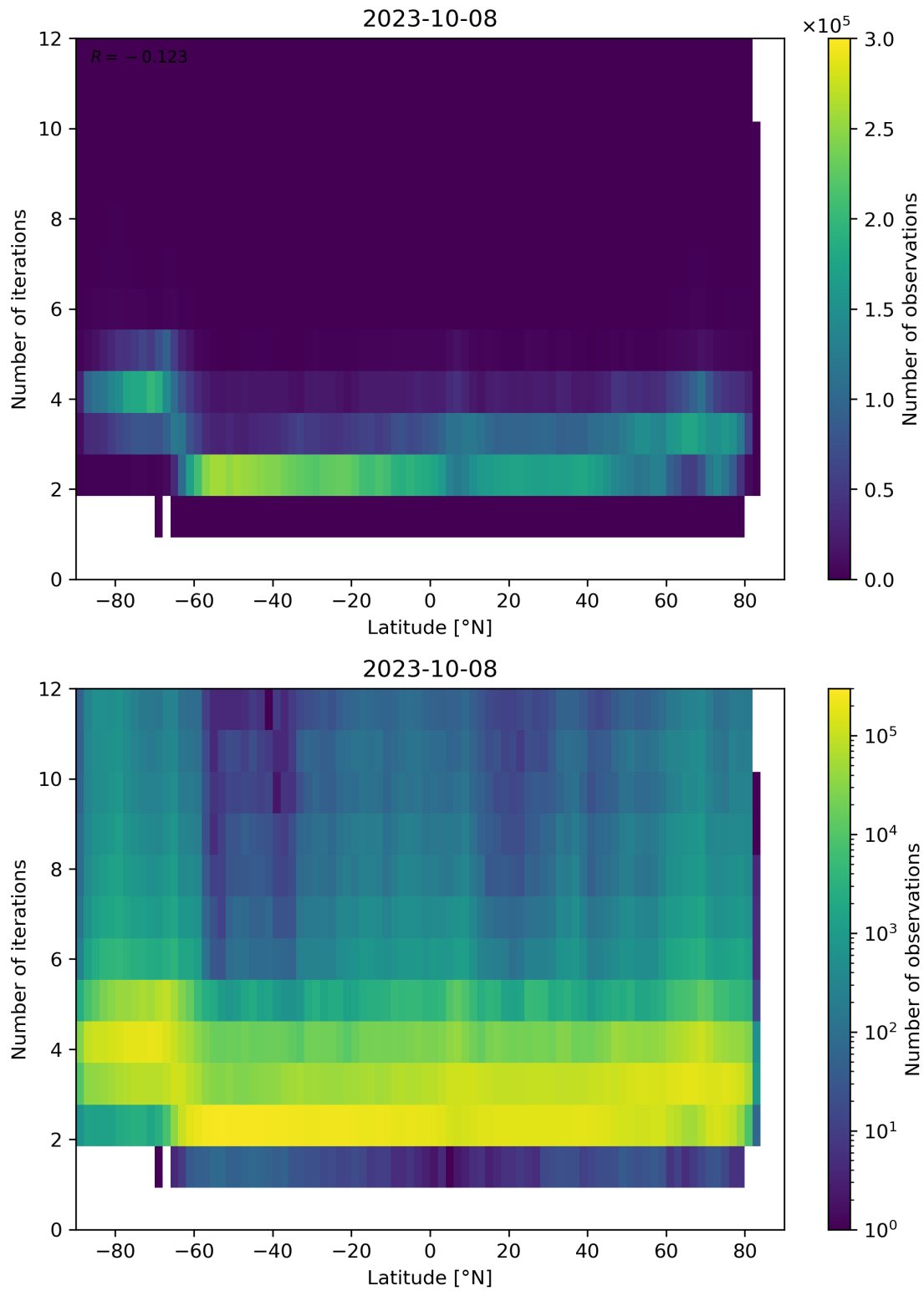
Figure 102: Scatter density plot of “Latitude” against “Number of iterations” for 2023-10-07 to 2023-10-09.
