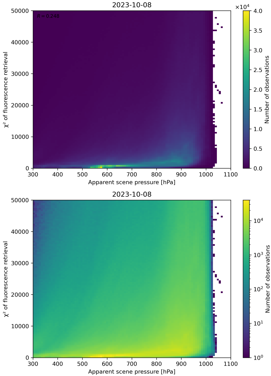
Figure 64: Scatter density plot of “Apparent scene pressure” against “ \chi^2 of fluorescence retrieval” for 2023-10-07 to 2023-10-09.
