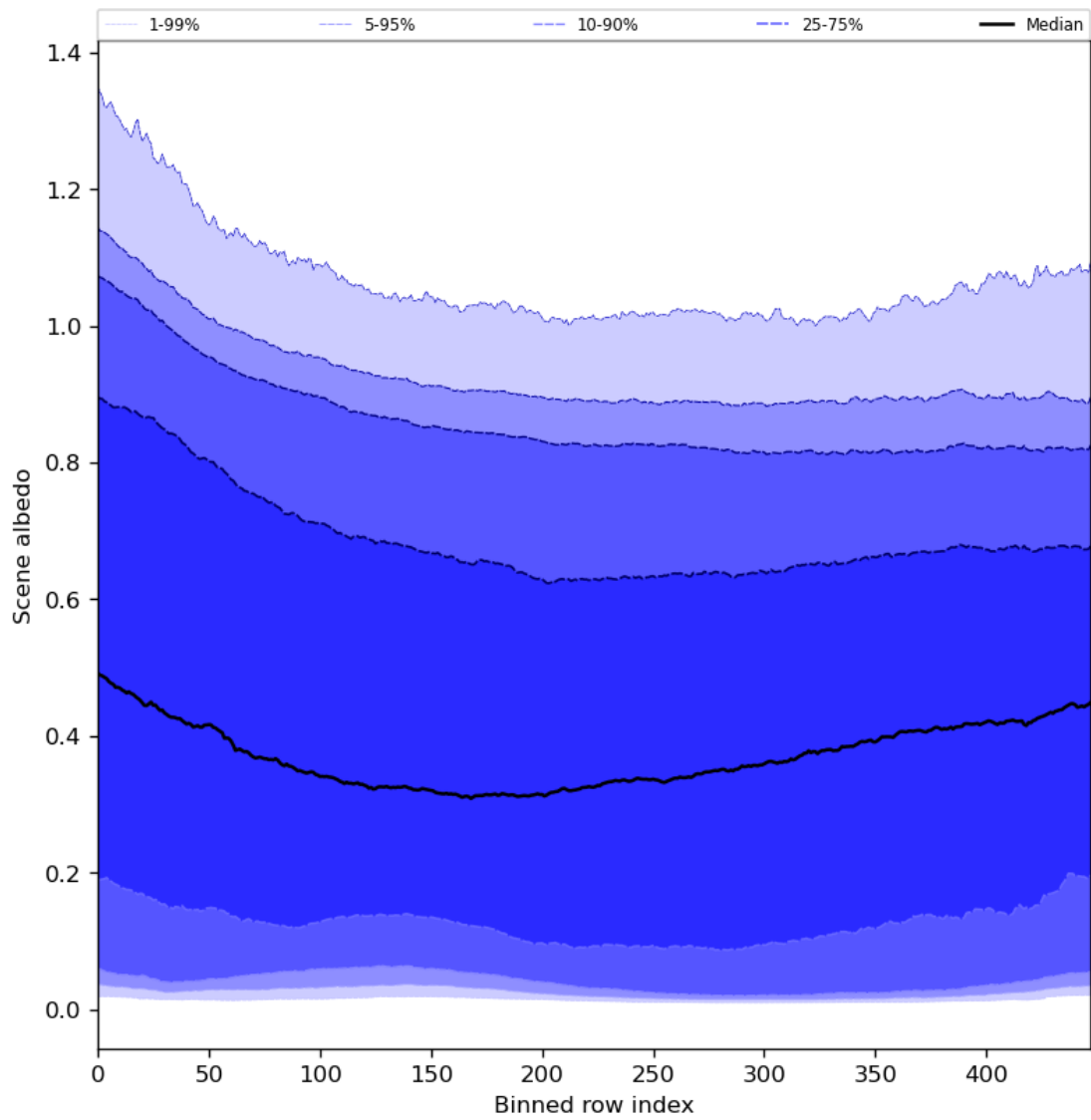
Figure 51: Along track statistics of “Scene albedo” for 2023-10-07 to 2023-10-09
