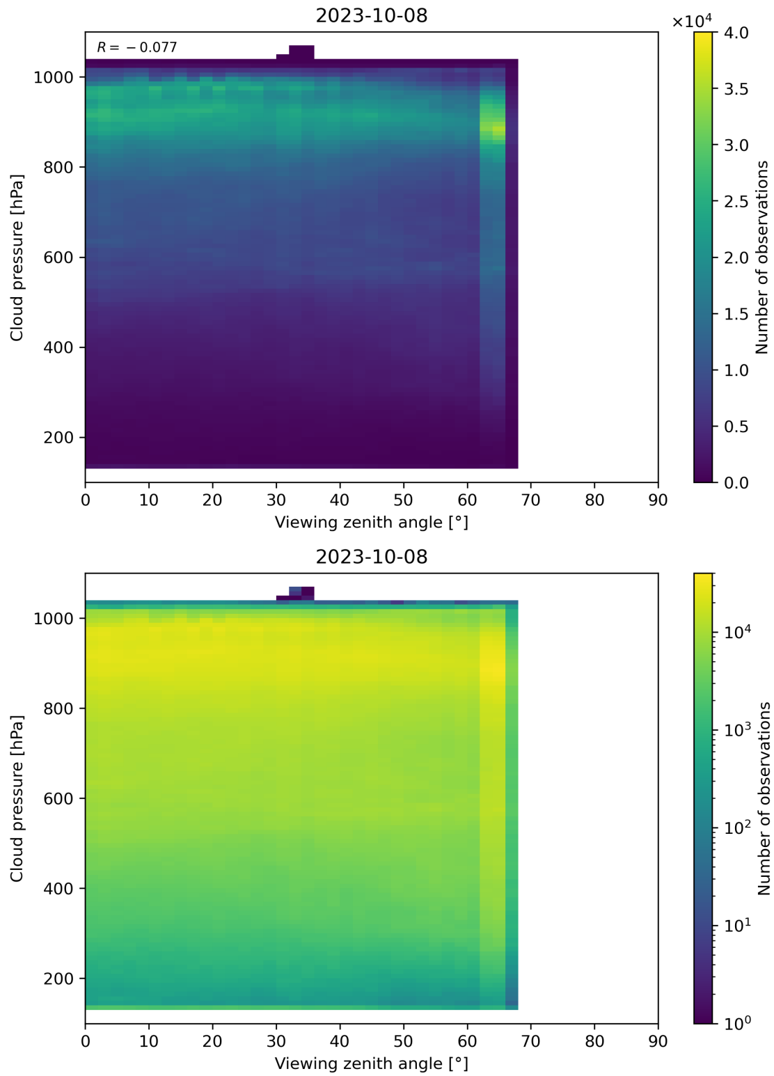
Figure 133: Scatter density plot of “Viewing zenith angle” against “Cloud pressure” for 2023-10-07 to 2023-10-09.
