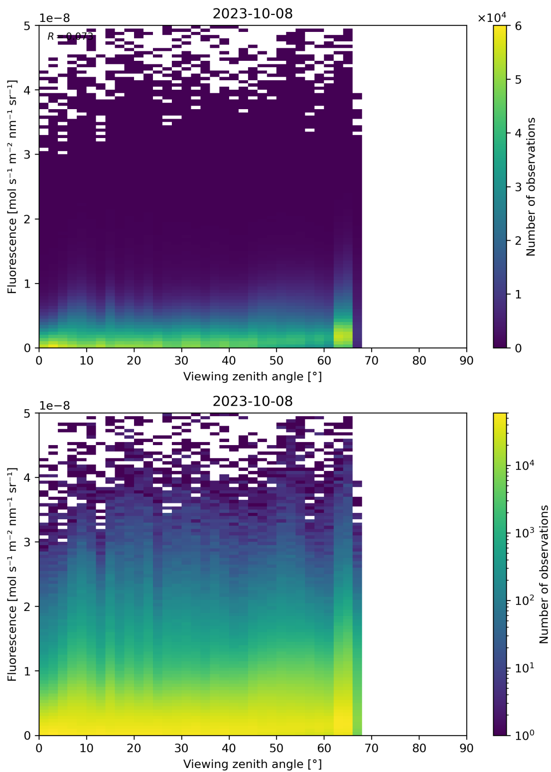
Figure 134: Scatter density plot of “Viewing zenith angle” against “Fluorescence” for 2023-10-07 to 2023-10-09.
