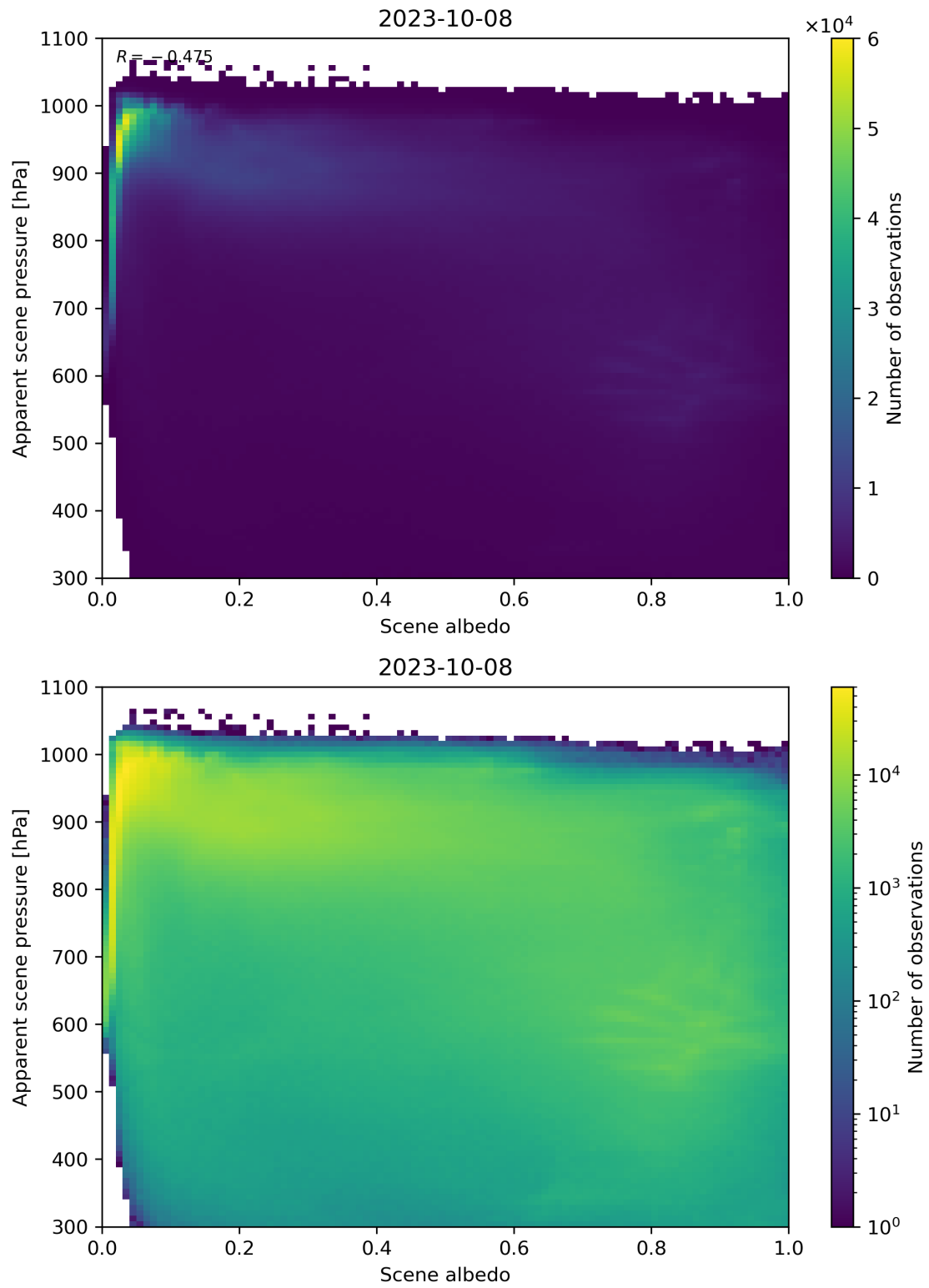
Figure 111: Scatter density plot of “Scene albedo” against “Apparent scene pressure” for 2023-10-07 to 2023-10-09.
