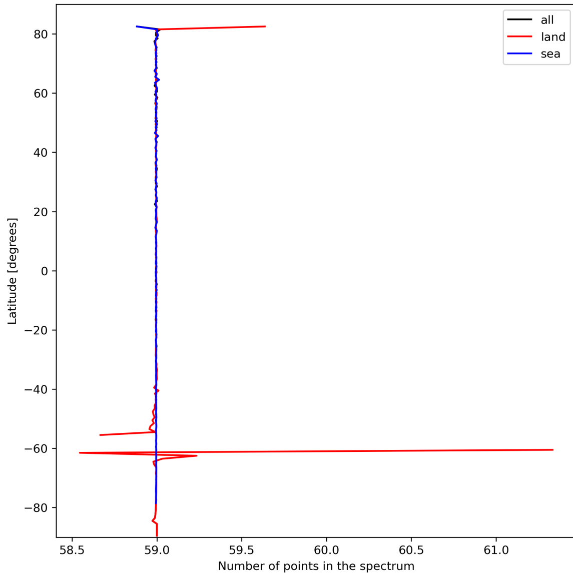
Figure 27: Zonal average of “Number of points in the spectrum” for 2023-10-07 to 2023-10-09.
