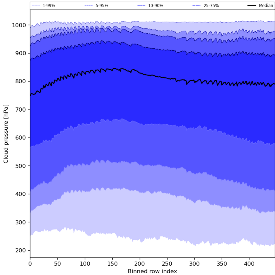
Figure 47: Along track statistics of “Cloud pressure” for 2023-10-07 to 2023-10-09
