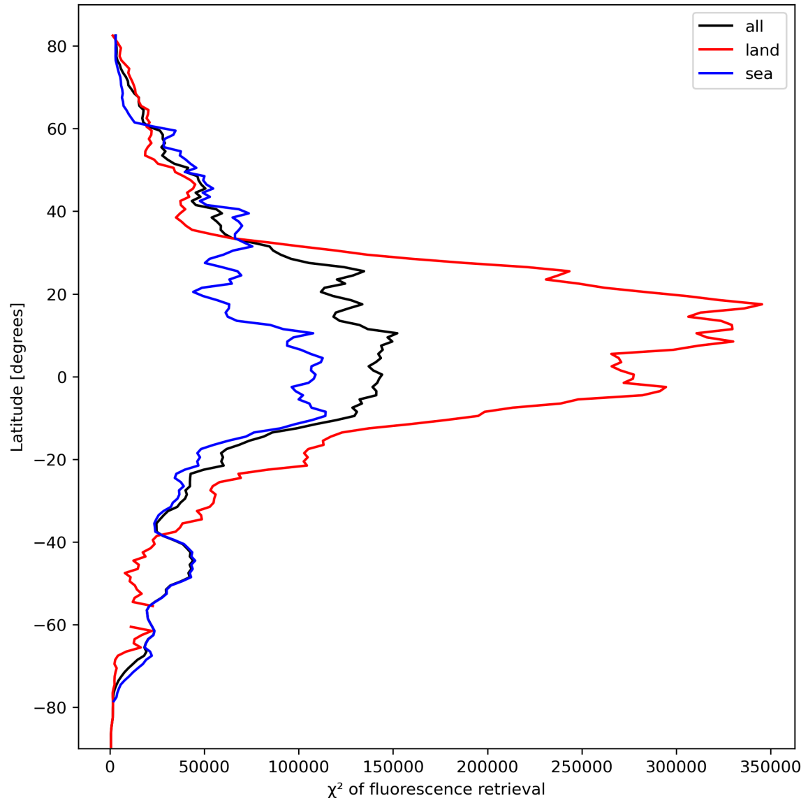
Figure 25: Zonal average of “ \chi^2 of fluorescence retrieval” for 2023-10-07 to 2023-10-09.
