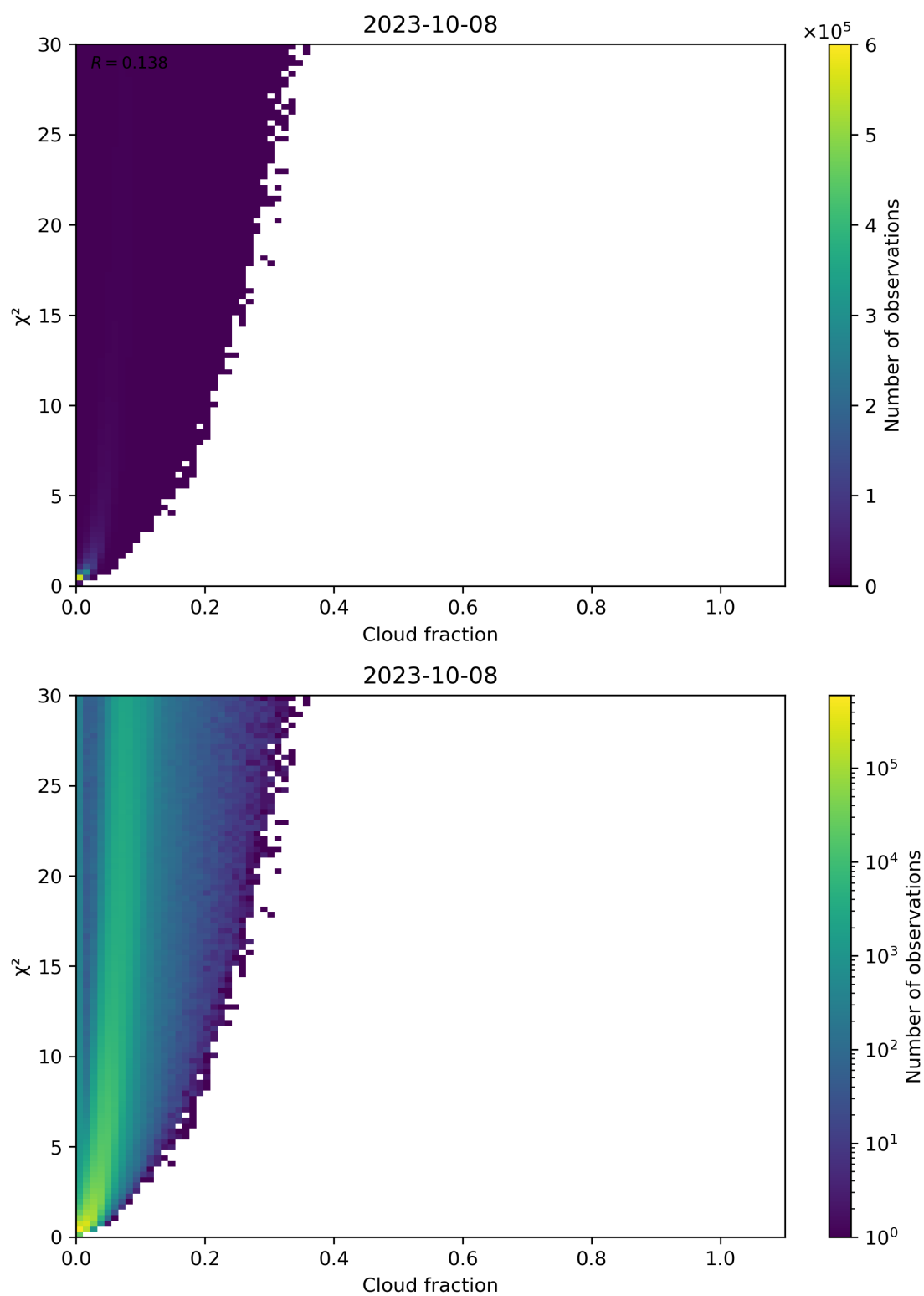
Figure 77: Scatter density plot of “Cloud fraction” against “ \chi^2 ” for 2023-10-07 to 2023-10-09.
