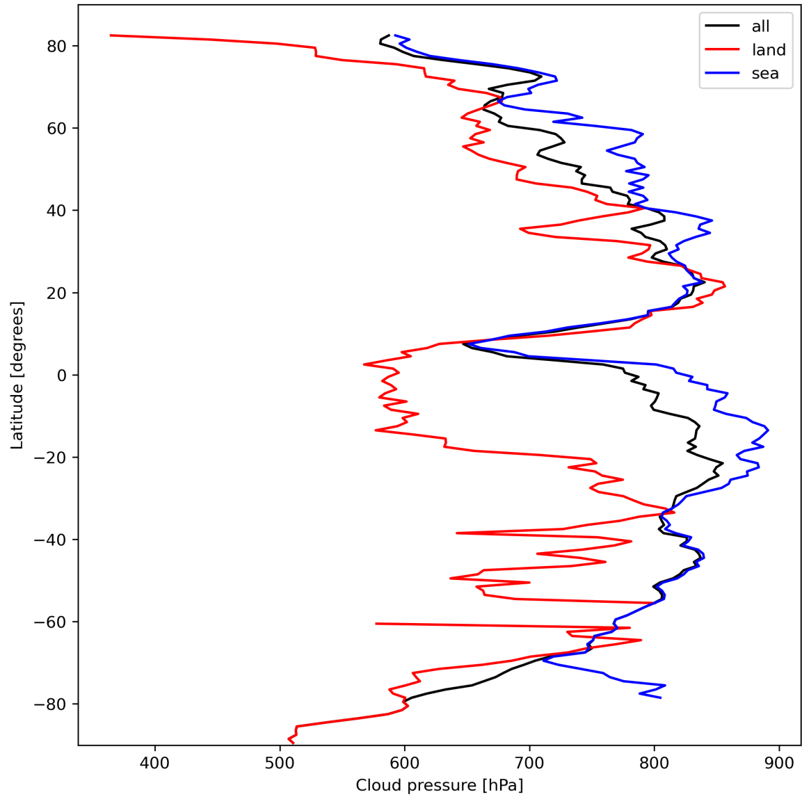
Figure 13: Zonal average of “Cloud pressure” for 2023-10-07 to 2023-10-09.
