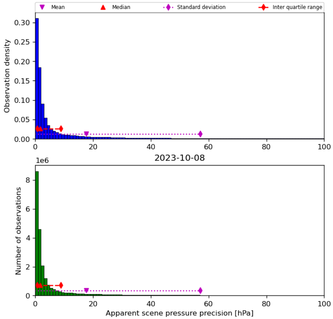
Figure 37: Histogram of “Apparent scene pressure precision” for 2023-10-07 to 2023-10-09
