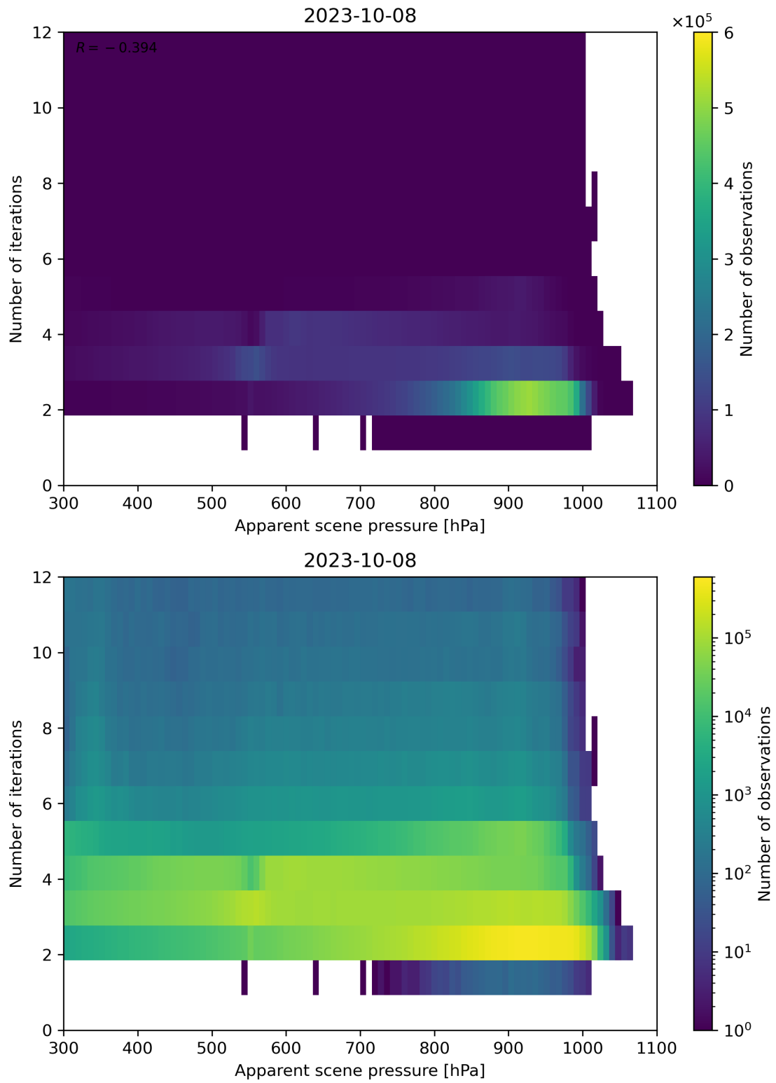
Figure 66: Scatter density plot of “Apparent scene pressure” against “Number of iterations” for 2023-10-07 to 2023-10-09.
