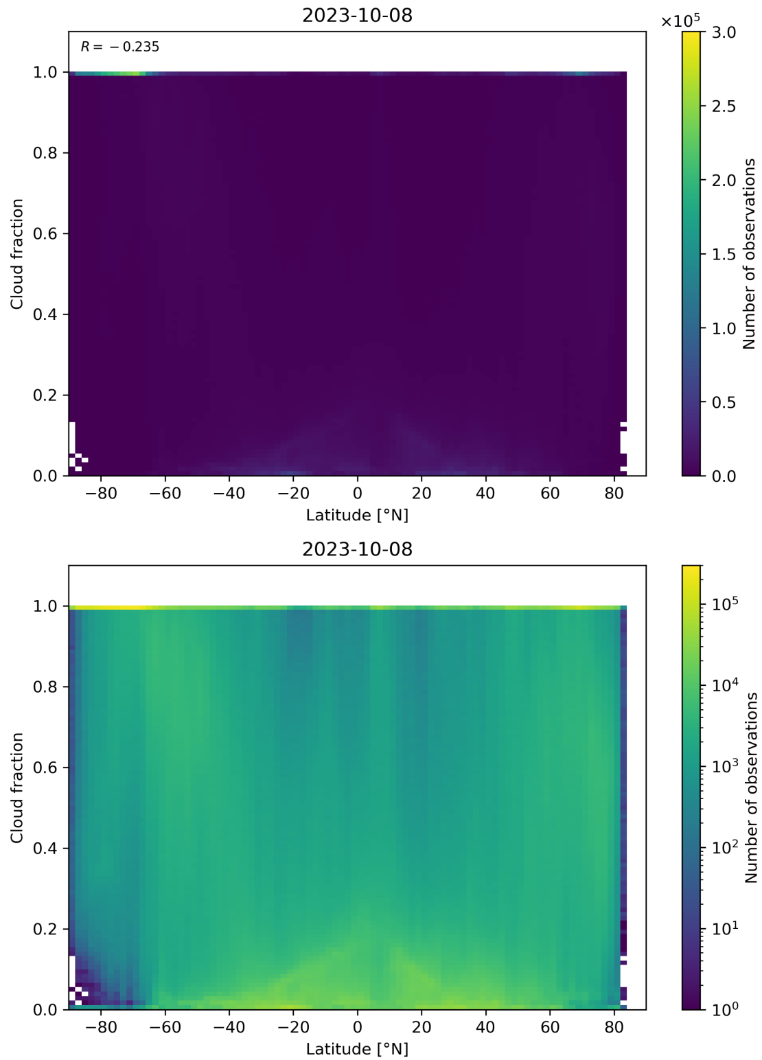
Figure 99: Scatter density plot of “Latitude” against “Cloud fraction” for 2023-10-07 to 2023-10-09.
