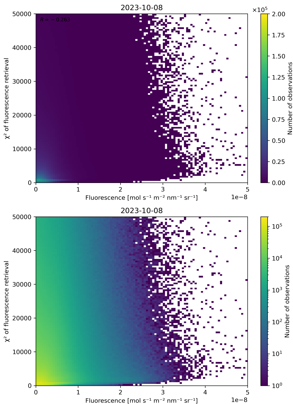
Figure 93: Scatter density plot of “Fluorescence” against “ \chi^2 of fluorescence retrieval” for 2023-10-07 to 2023-10-09.
