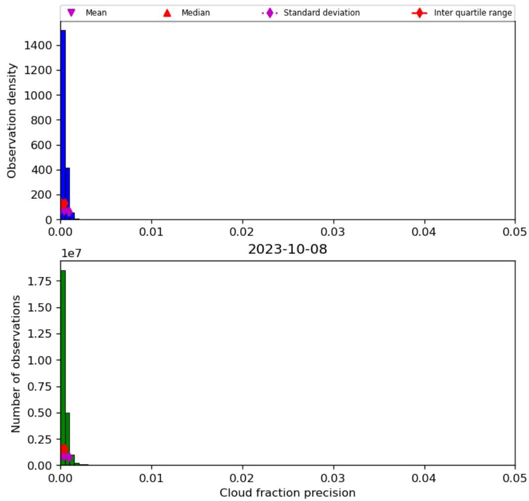
Figure 33: Histogram of “Cloud fraction precision” for 2023-10-07 to 2023-10-09
