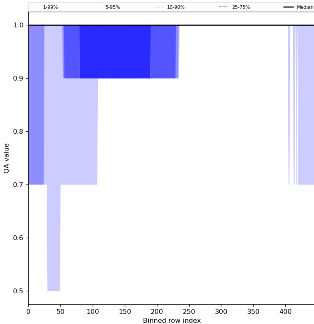
Figure 46: Along track statistics of “QA value” for 2023-10-07 to 2023-10-09
