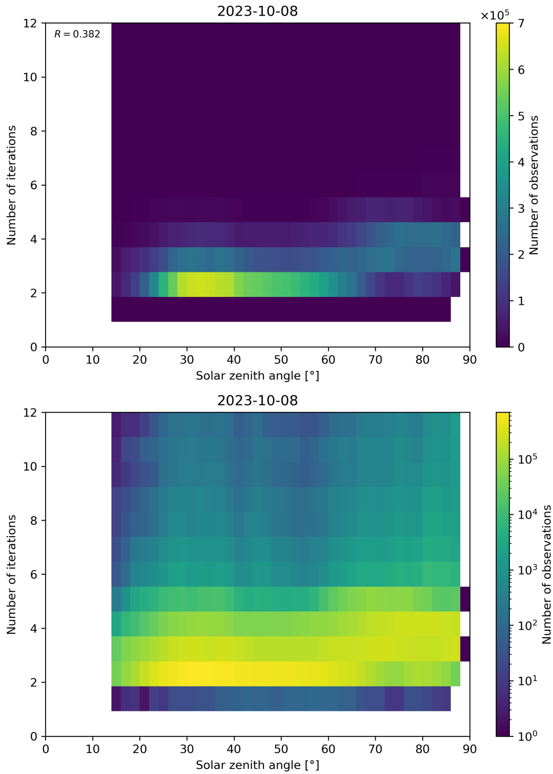
Figure 125: Scatter density plot of “Solar zenith angle” against “Number of iterations” for 2023-10-07 to 2023-10-09.
