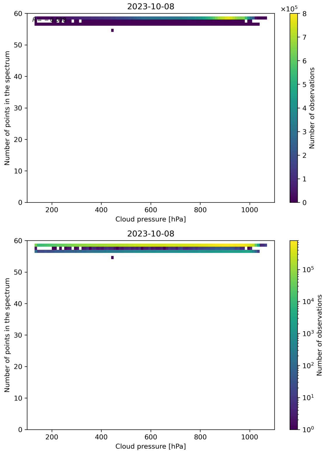
Figure 90: Scatter density plot of “Cloud pressure” against “Number of points in the spectrum” for 2023-10-07 to 2023-10-09.
