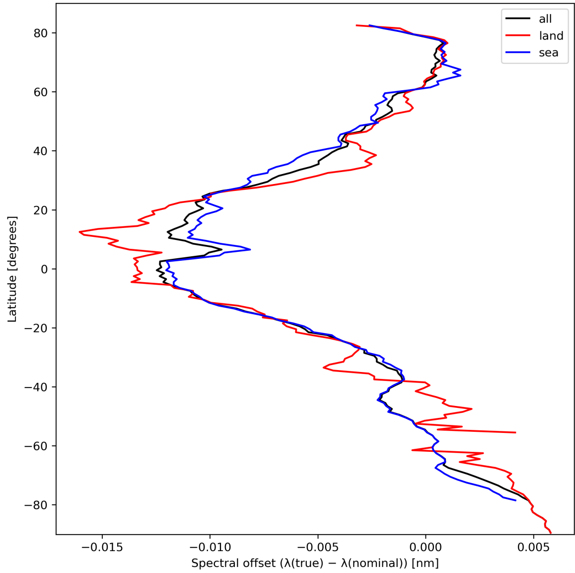
Figure 28: Zonal average of “Spectral offset ( \lambda(\text{true}) - \lambda(\text{nominal}) )” for 2023-10-07 to 2023-10-09.
