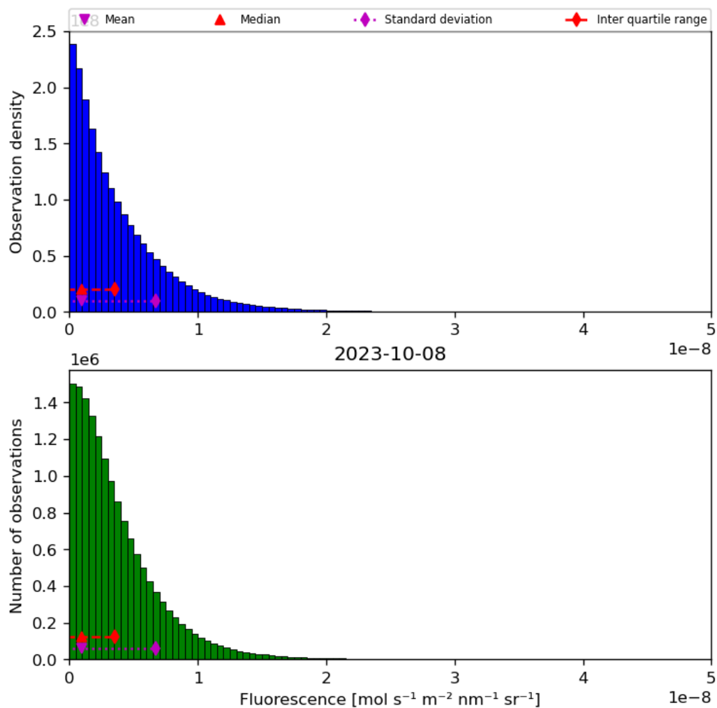
Figure 40: Histogram of “Fluorescence” for 2023-10-07 to 2023-10-09
