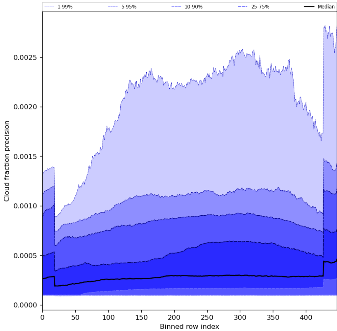
Figure 50: Along track statistics of “Cloud fraction precision” for 2023-10-07 to 2023-10-09
