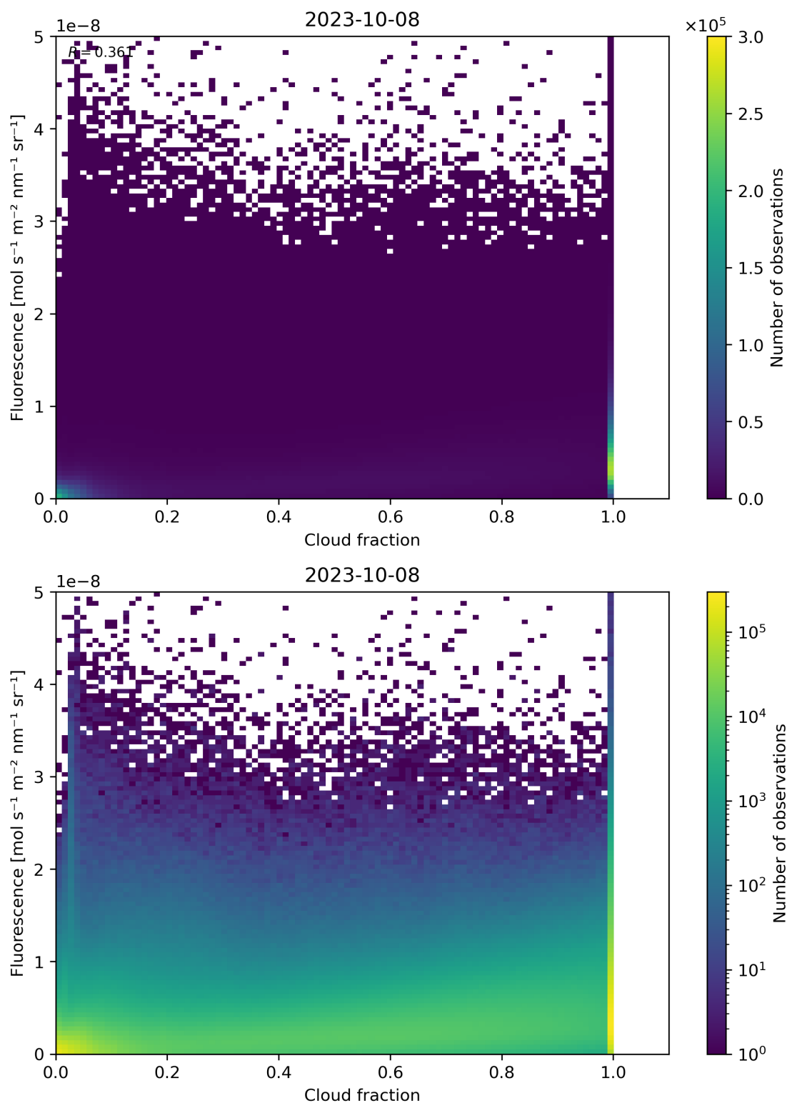
Figure 79: Scatter density plot of “Cloud fraction” against “Fluorescence” for 2023-10-07 to 2023-10-09.
