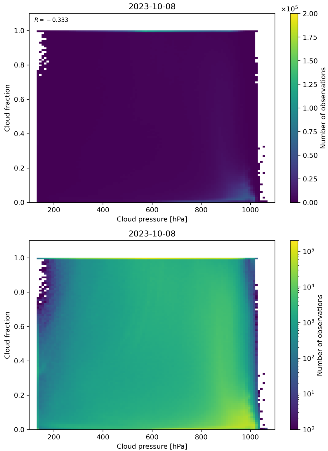
Figure 87: Scatter density plot of “Cloud pressure” against “Cloud fraction” for 2023-10-07 to 2023-10-09.
