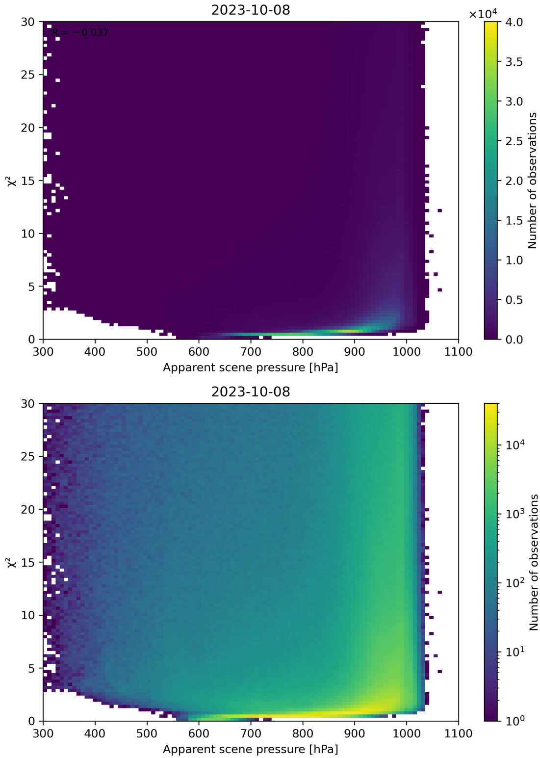
Figure 63: Scatter density plot of “Apparent scene pressure” against “ \chi^2 ” for 2023-10-07 to 2023-10-09.
