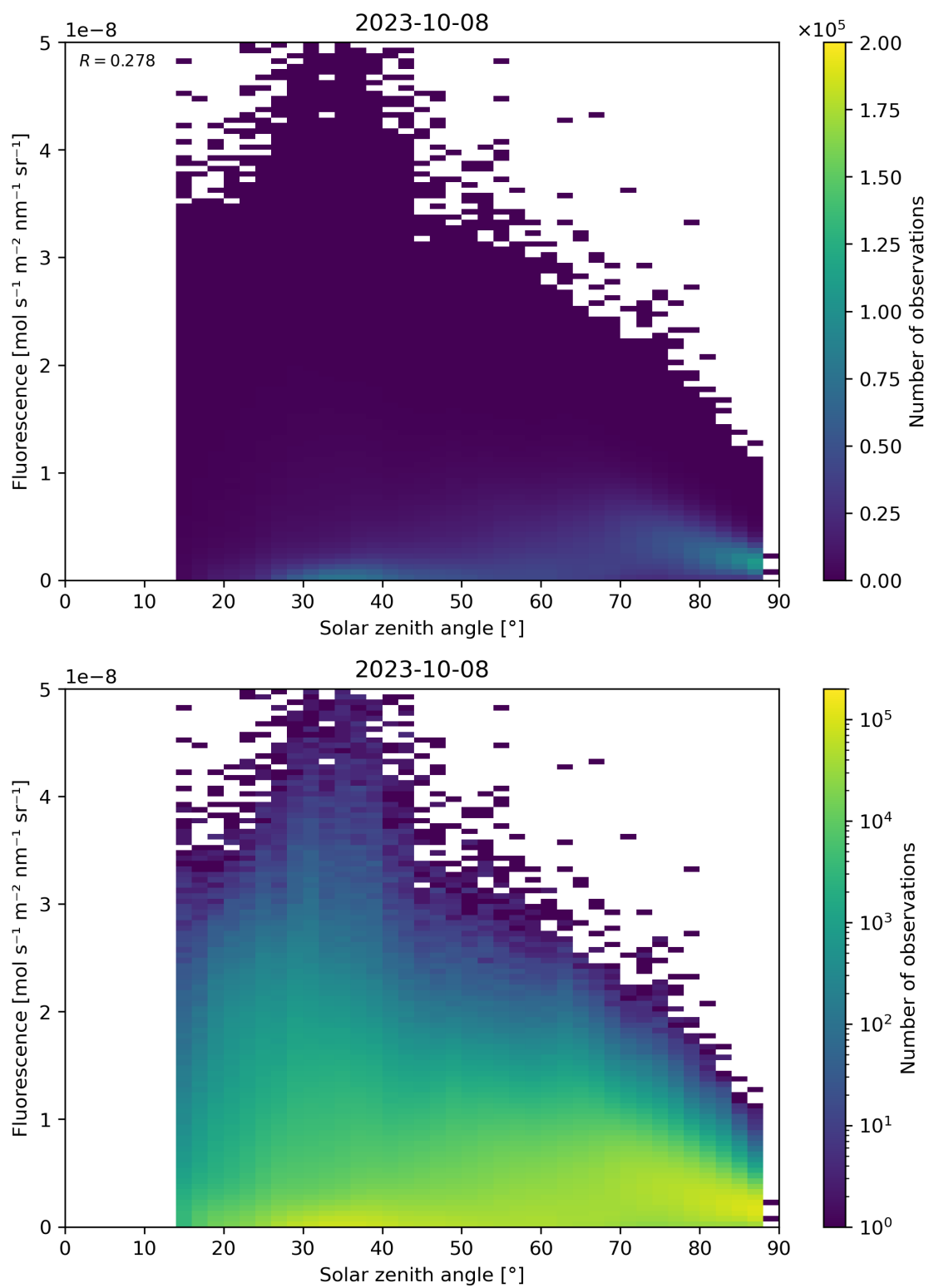
Figure 123: Scatter density plot of “Solar zenith angle” against “Fluorescence” for 2023-10-07 to 2023-10-09.
