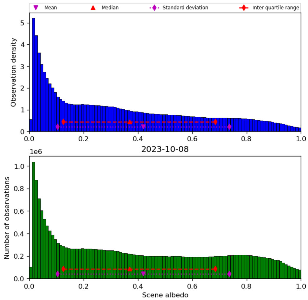
Figure 34: Histogram of “Scene albedo” for 2023-10-07 to 2023-10-09
