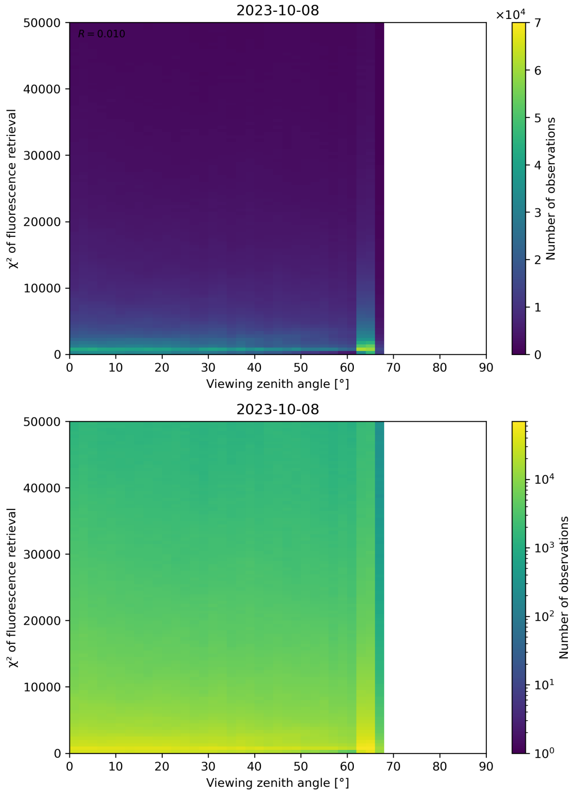
Figure 131: Scatter density plot of “Viewing zenith angle” against “ \chi^2 of fluorescence retrieval” for 2023-10-07 to 2023-10-09.
