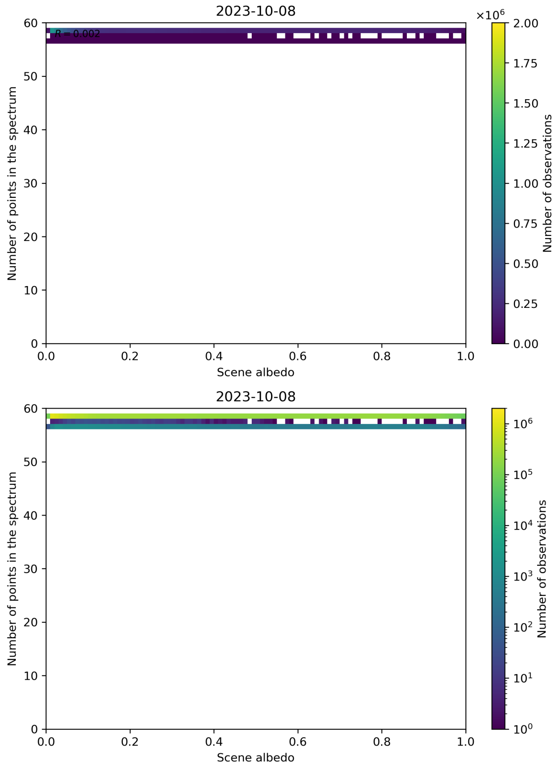
Figure 116: Scatter density plot of “Scene albedo” against “Number of points in the spectrum” for 2023-10-07 to 2023-10-09.
