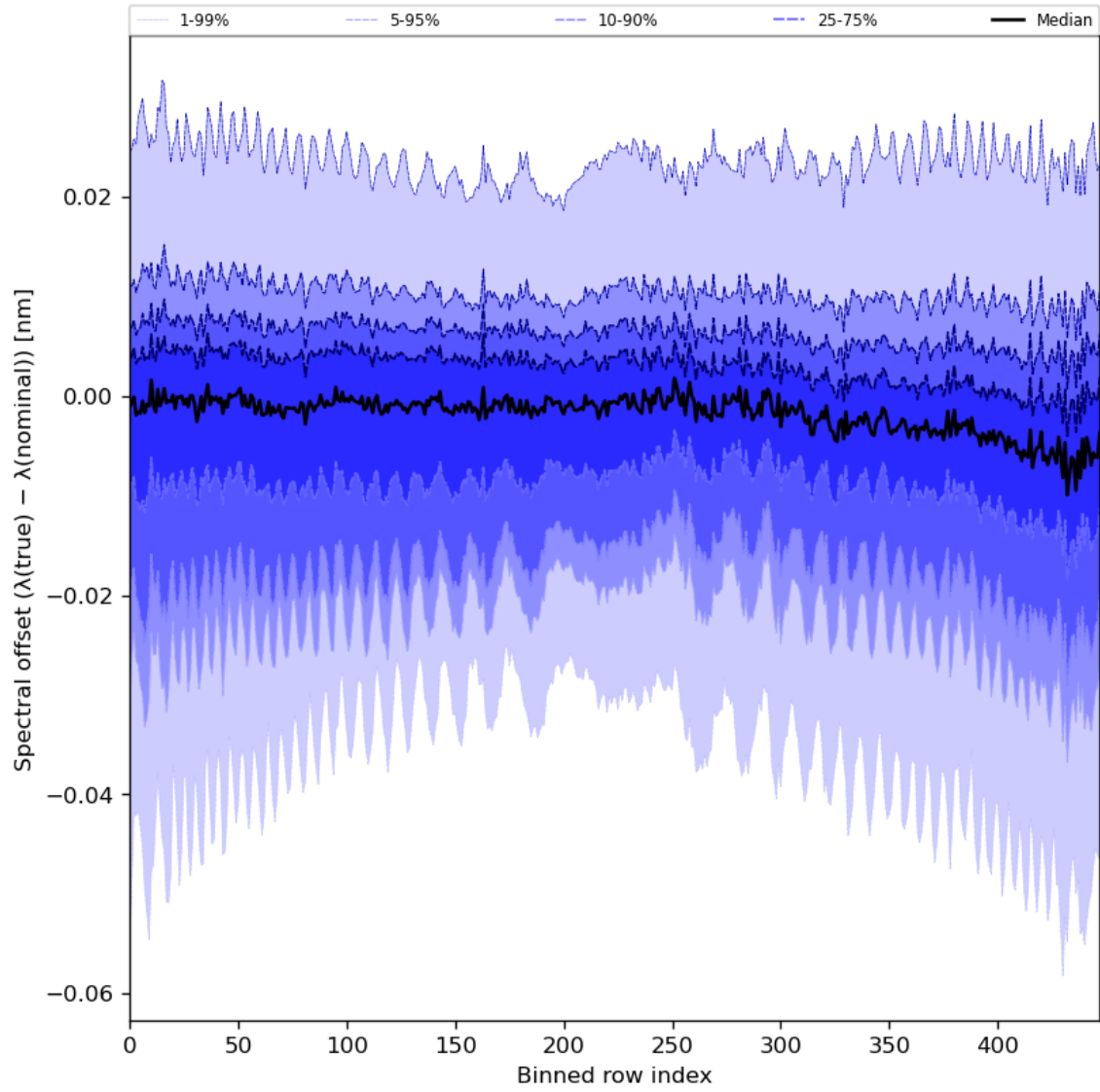
Figure 62: Along track statistics of “Spectral offset ( \lambda(\text{true}) - \lambda(\text{nominal}) )” for 2023-10-07 to 2023-10-09
