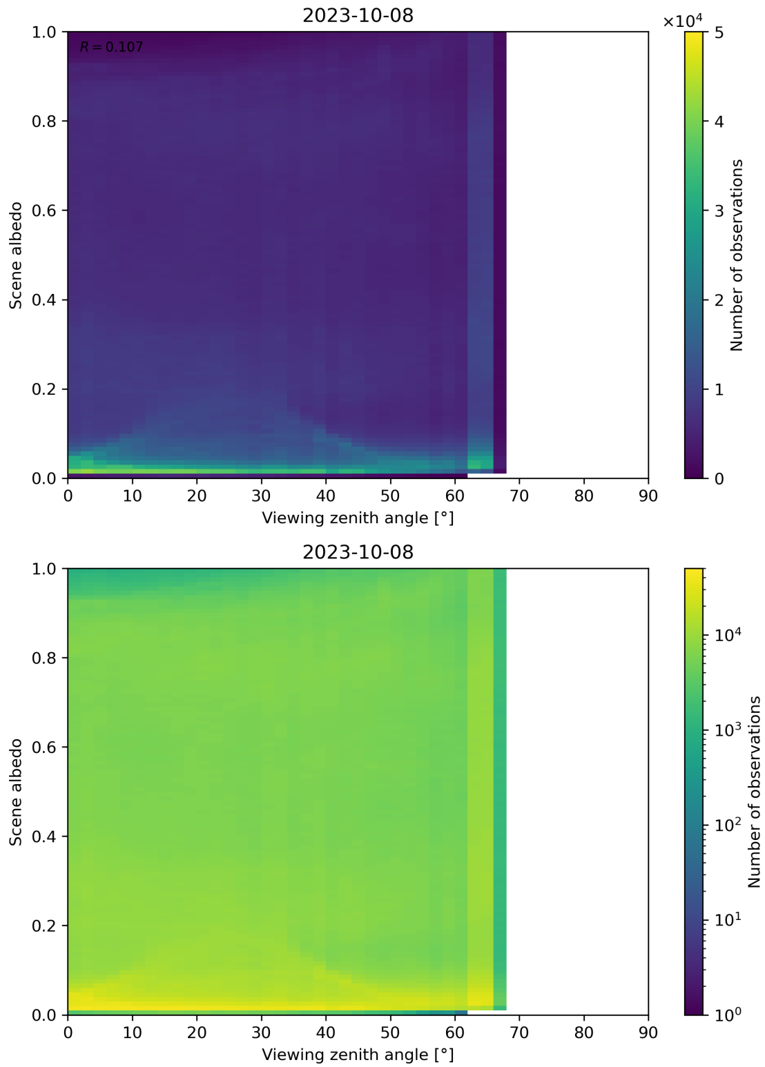
Figure 138: Scatter density plot of “Viewing zenith angle” against “Scene albedo” for 2023-10-07 to 2023-10-09.
