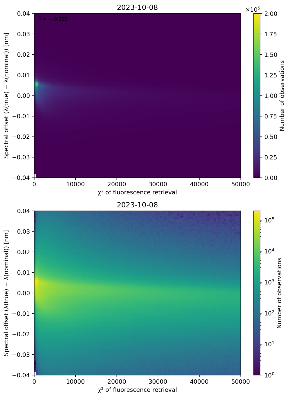
Figure 72: Scatter density plot of " \chi^2 of fluorescence retrieval" against "Spectral offset ( \lambda(\text{true}) - \lambda(\text{nominal}) )" for 2023-10-07 to 2023-10-09.
