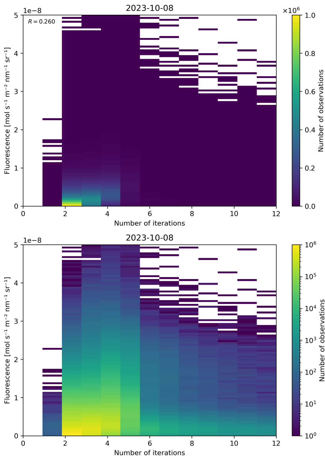
Figure 107: Scatter density plot of “Number of iterations” against “Fluorescence” for 2023-10-07 to 2023-10-09.
