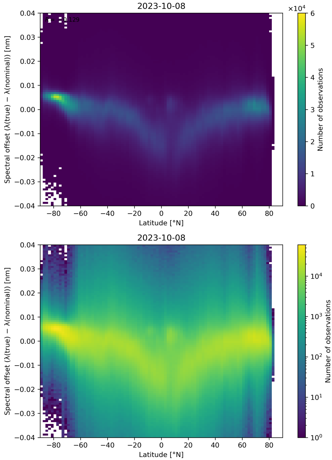
Figure 105: Scatter density plot of “Latitude” against “Spectral offset ( \lambda(\text{true}) - \lambda(\text{nominal}) )” for 2023-10-07 to 2023-10-09.
