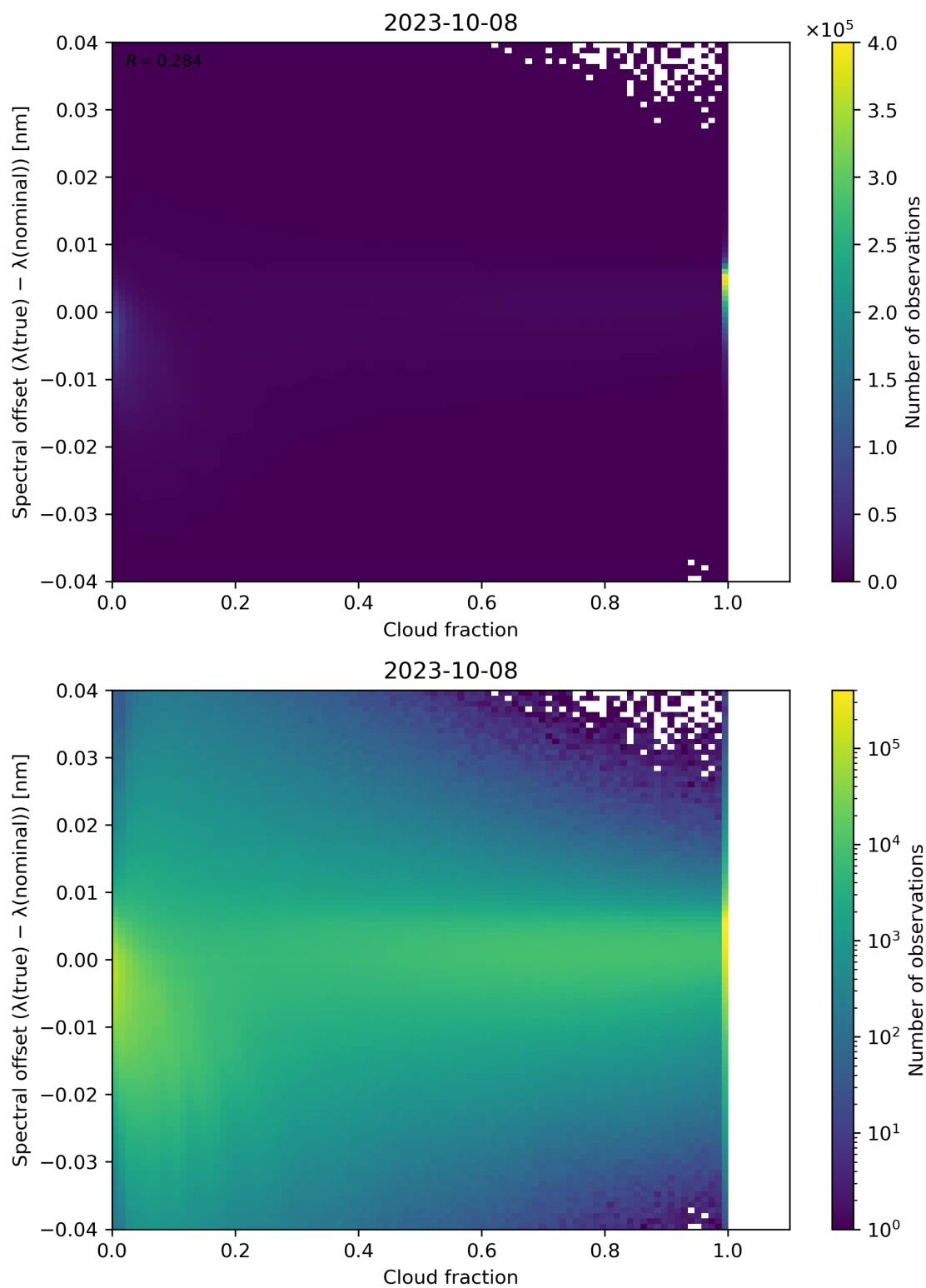
Figure 83: Scatter density plot of “Cloud fraction” against “Spectral offset ( \lambda(\text{true}) - \lambda(\text{nominal}) )” for 2023-10-07 to 2023-10-09.
