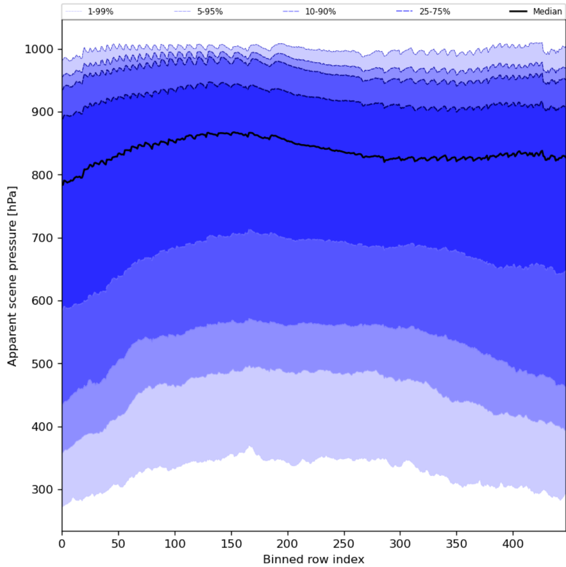
Figure 53: Along track statistics of “Apparent scene pressure” for 2023-10-07 to 2023-10-09
