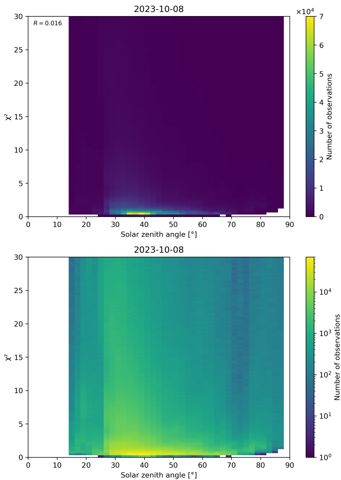
Figure 119: Scatter density plot of “Solar zenith angle” against “ \chi^2 ” for 2023-10-07 to 2023-10-09.
