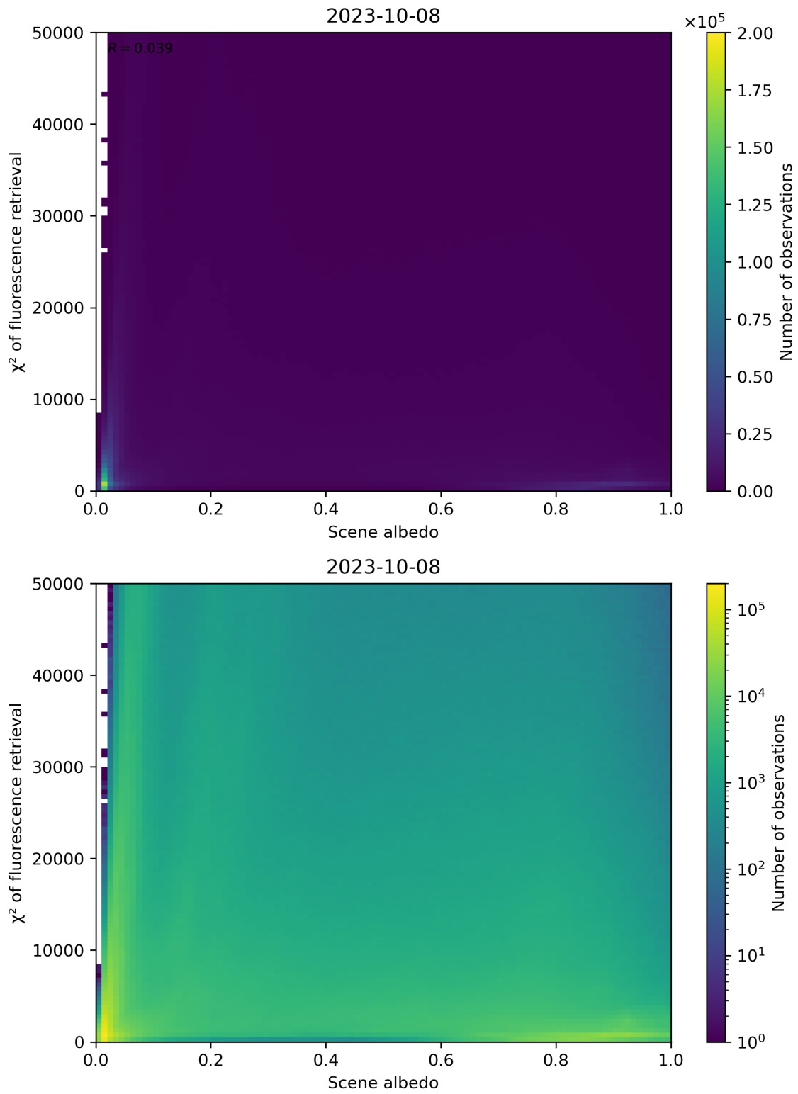
Figure 113: Scatter density plot of “Scene albedo” against “ \chi^2 of fluorescence retrieval” for 2023-10-07 to 2023-10-09.
