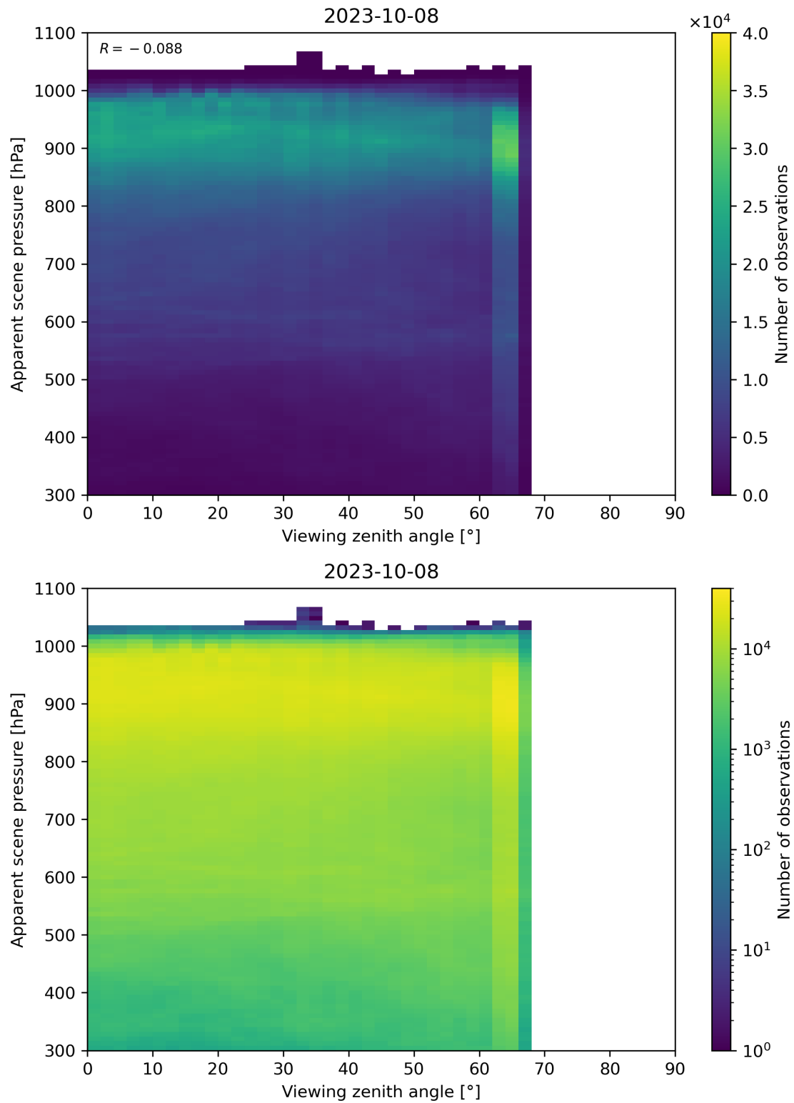
Figure 129: Scatter density plot of “Viewing zenith angle” against “Apparent scene pressure” for 2023-10-07 to 2023-10-09.
