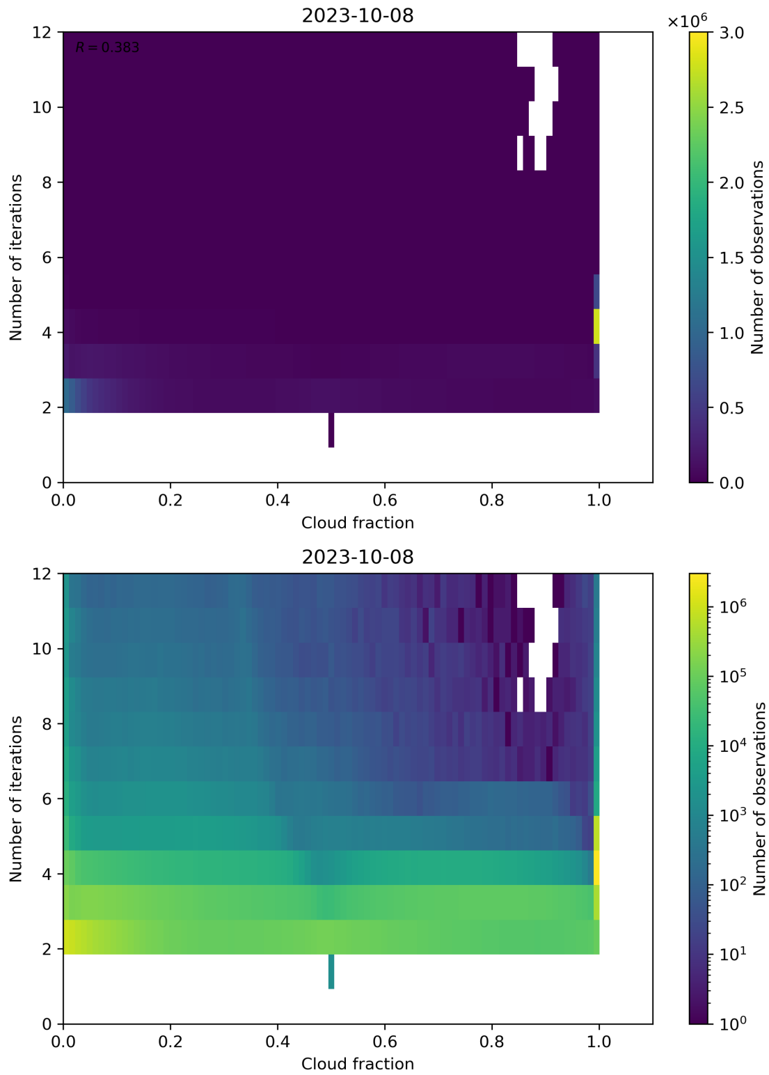
Figure 80: Scatter density plot of “Cloud fraction” against “Number of iterations” for 2023-10-07 to 2023-10-09.
