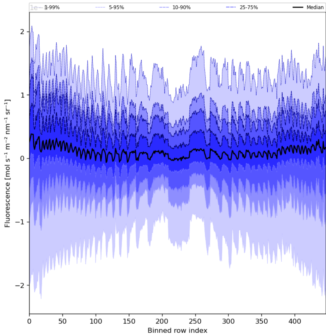
Figure 57: Along track statistics of “Fluorescence” for 2023-10-08 to 2023-10-10
