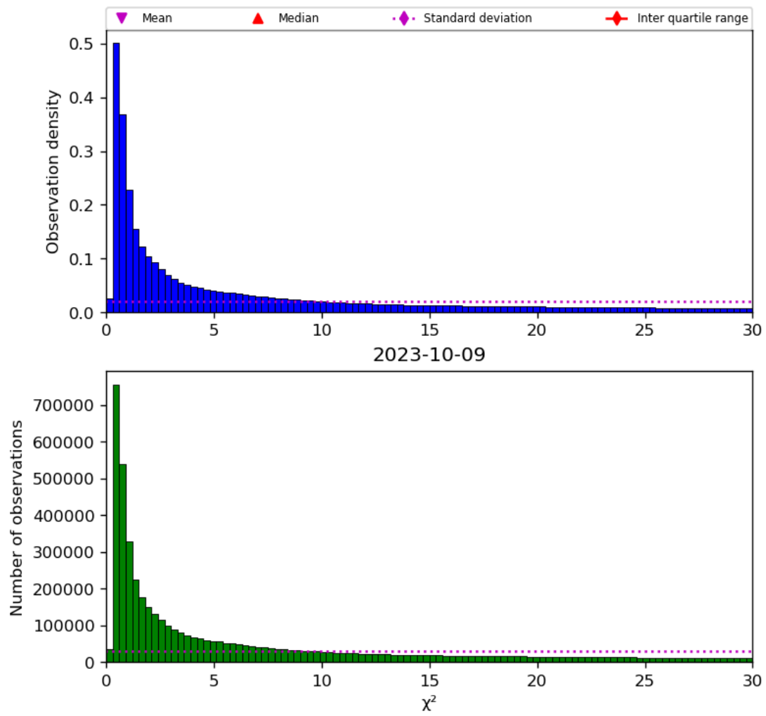
Figure 38: Histogram of “ \chi^2 ” for 2023-10-08 to 2023-10-10
