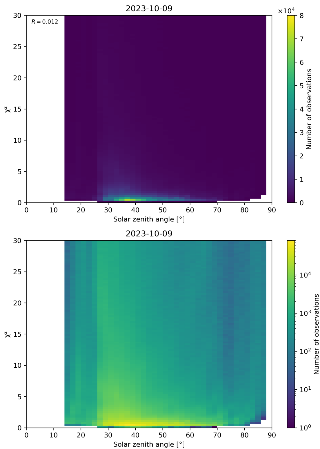
Figure 119: Scatter density plot of “Solar zenith angle” against “ \chi^2 ” for 2023-10-08 to 2023-10-10.
