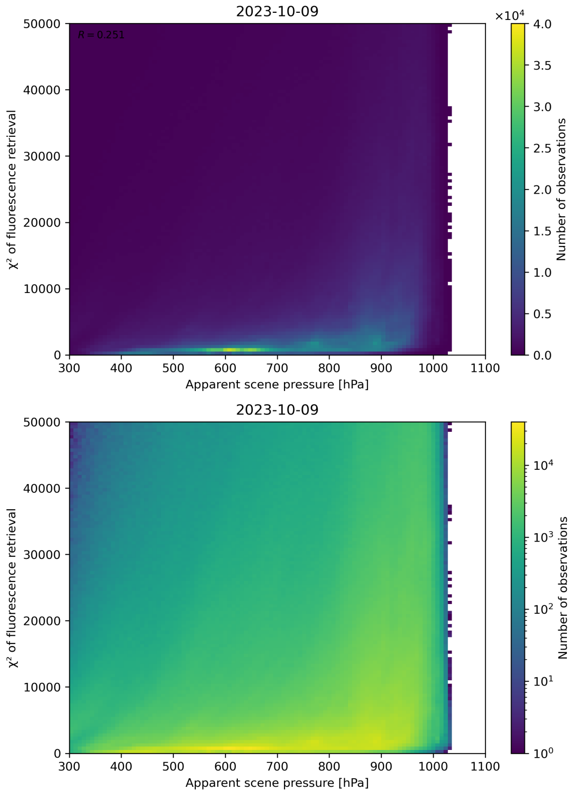
Figure 64: Scatter density plot of “Apparent scene pressure” against “ \chi^2 of fluorescence retrieval” for 2023-10-08 to 2023-10-10.
