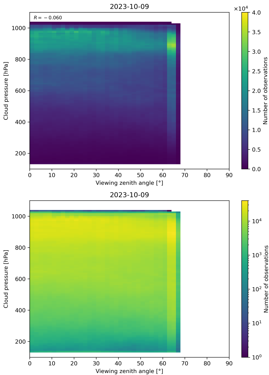
Figure 133: Scatter density plot of “Viewing zenith angle” against “Cloud pressure” for 2023-10-08 to 2023-10-10.
