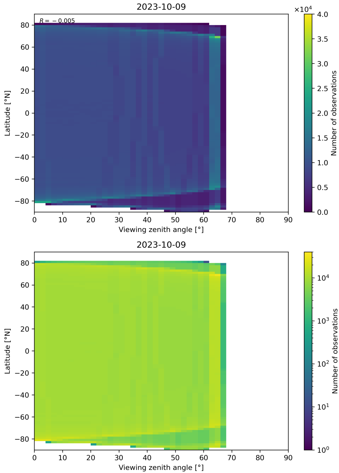
Figure 135: Scatter density plot of “Viewing zenith angle” against “Latitude” for 2023-10-08 to 2023-10-10.
