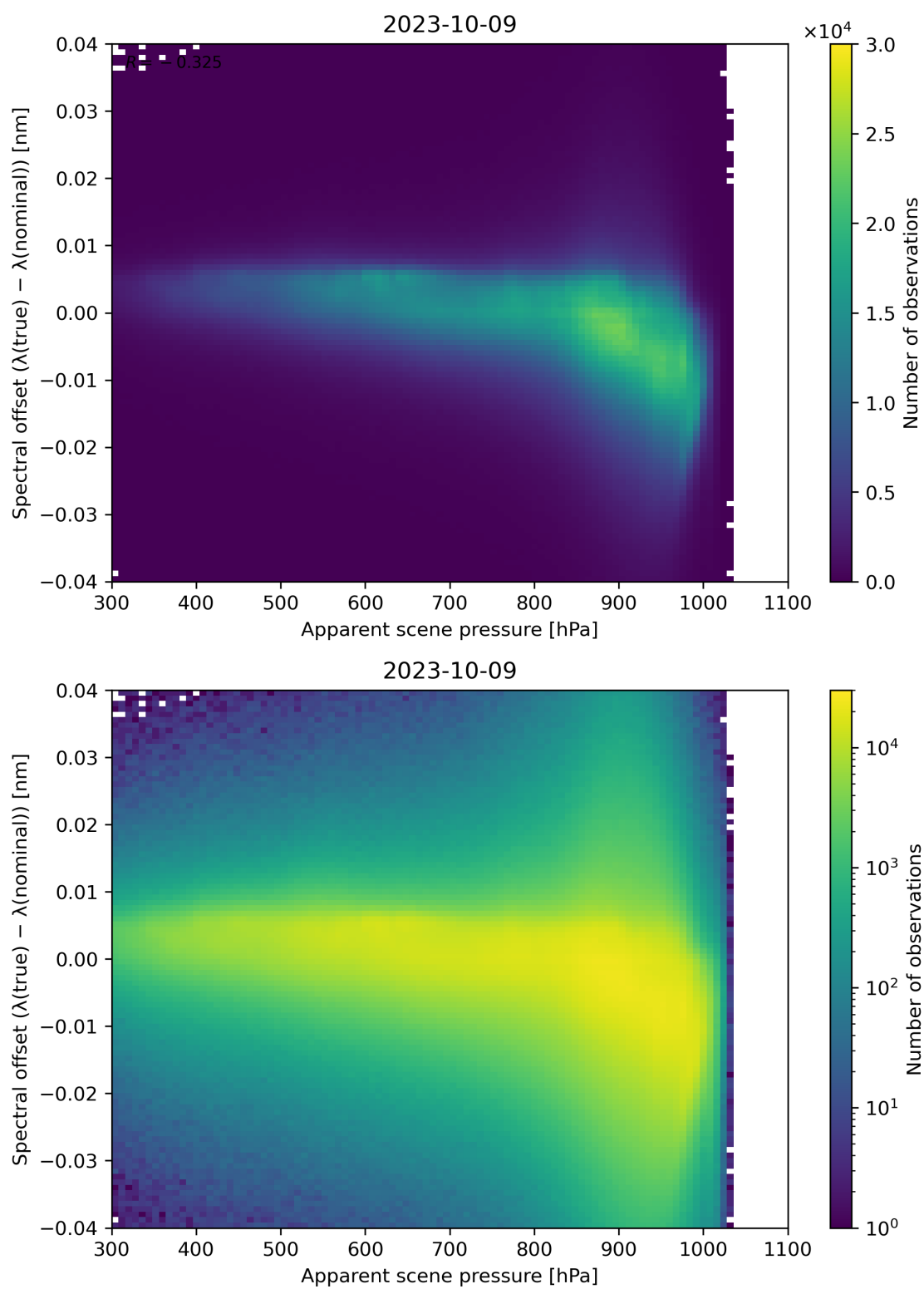
Figure 68: Scatter density plot of “Apparent scene pressure” against “Spectral offset ( \lambda(\text{true}) - \lambda(\text{nominal}) )” for 2023-10-08 to 2023-10-10.
