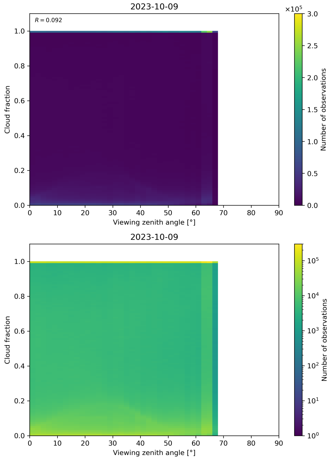
Figure 132: Scatter density plot of “Viewing zenith angle” against “Cloud fraction” for 2023-10-08 to 2023-10-10.
