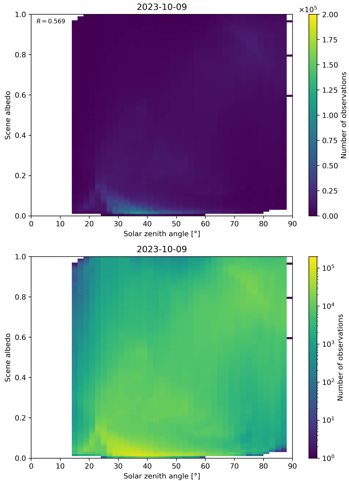
Figure 127: Scatter density plot of “Solar zenith angle” against “Scene albedo” for 2023-10-08 to 2023-10-10.
