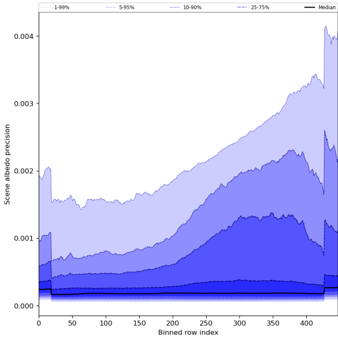
Figure 52: Along track statistics of “Scene albedo precision” for 2023-10-08 to 2023-10-10
