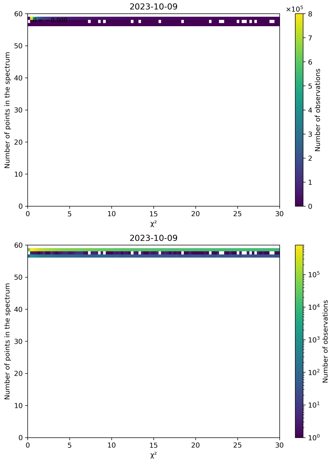
Figure 74: Scatter density plot of " \chi^2 " against "Number of points in the spectrum" for 2023-10-08 to 2023-10-10.
