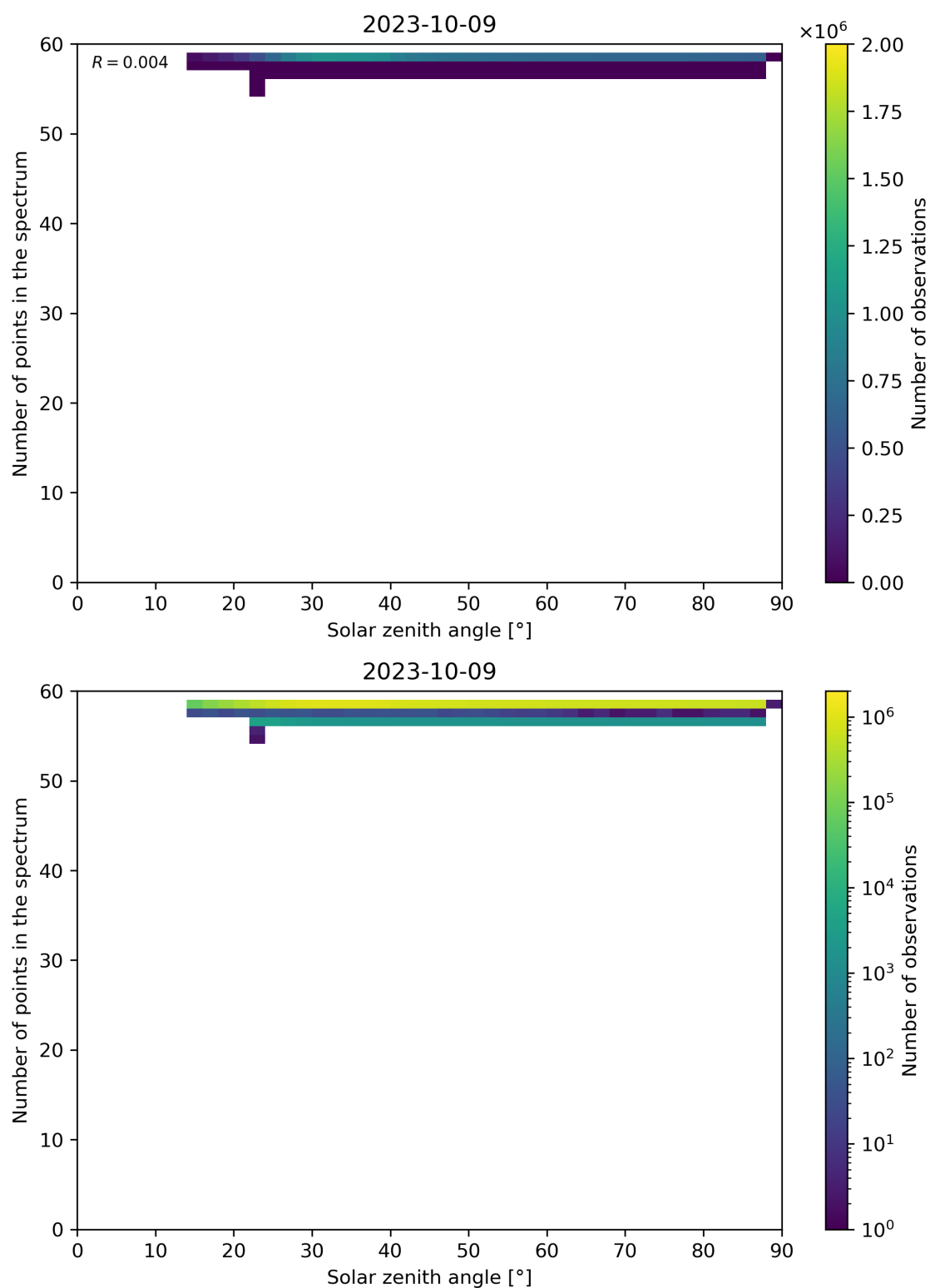
Figure 126: Scatter density plot of “Solar zenith angle” against “Number of points in the spectrum” for 2023-10-08 to 2023-10-10.
