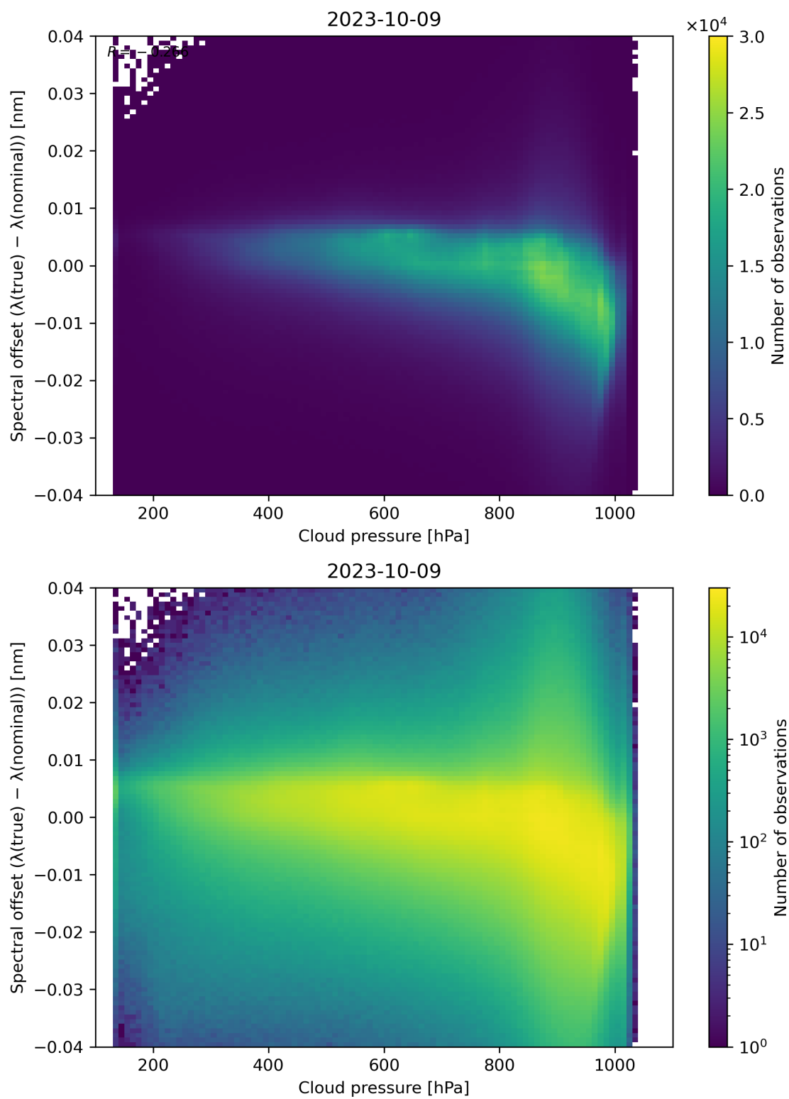
Figure 92: Scatter density plot of “Cloud pressure” against “Spectral offset ( \lambda(\text{true}) - \lambda(\text{nominal}) )” for 2023-10-08 to 2023-10-10.
