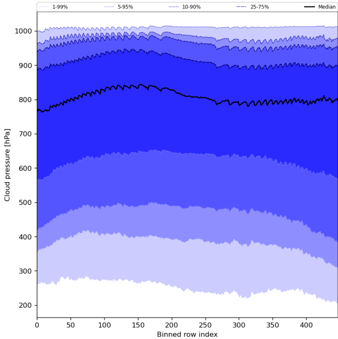
Figure 47: Along track statistics of “Cloud pressure” for 2023-10-08 to 2023-10-10
