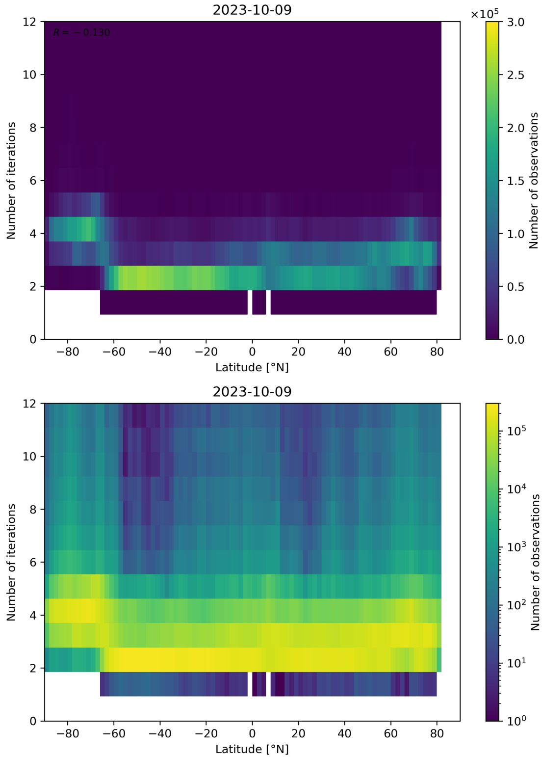
Figure 102: Scatter density plot of “Latitude” against “Number of iterations” for 2023-10-08 to 2023-10-10.
