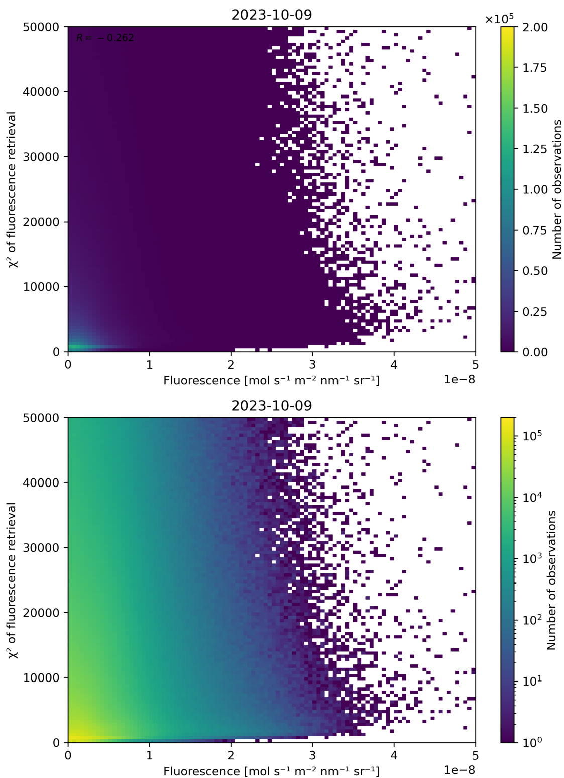
Figure 93: Scatter density plot of “Fluorescence” against “ \chi^2 of fluorescence retrieval” for 2023-10-08 to 2023-10-10.
