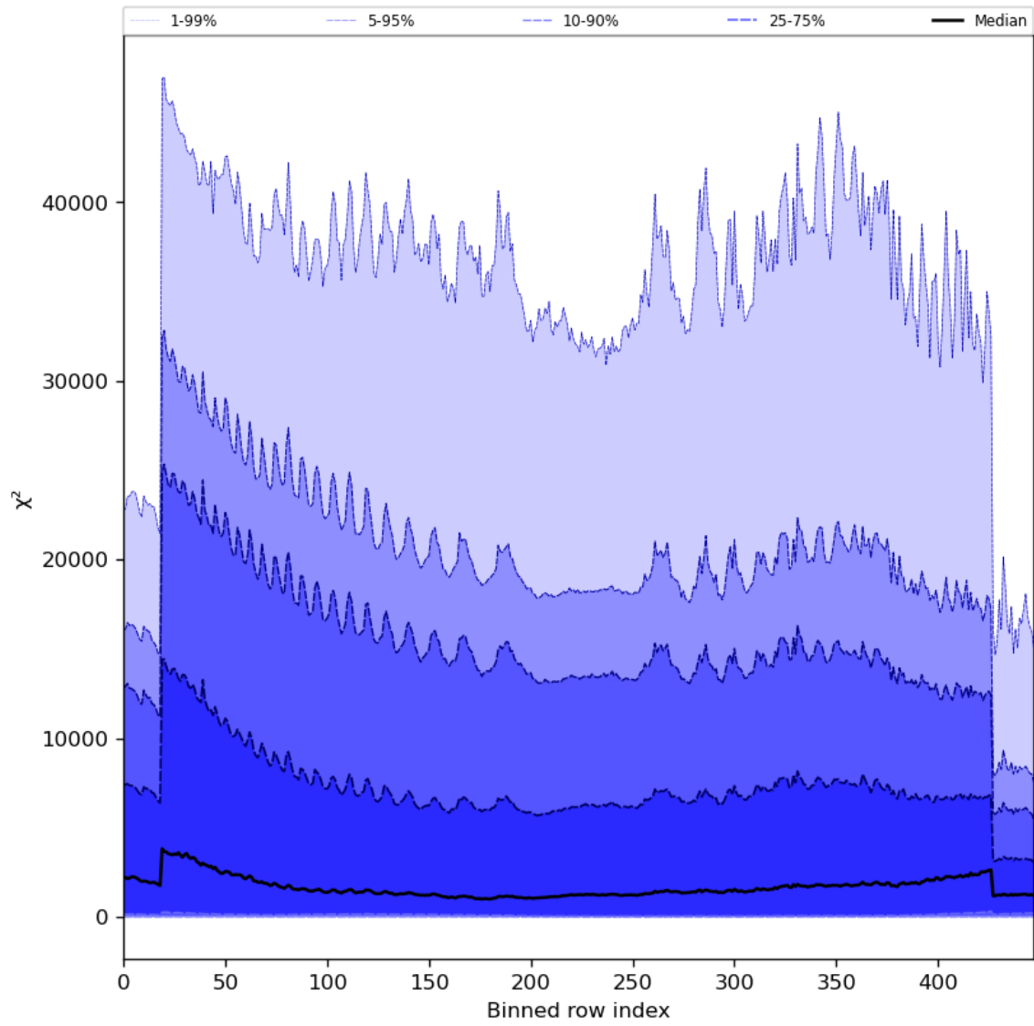
Figure 55: Along track statistics of “ \chi^2 ” for 2023-10-08 to 2023-10-10
