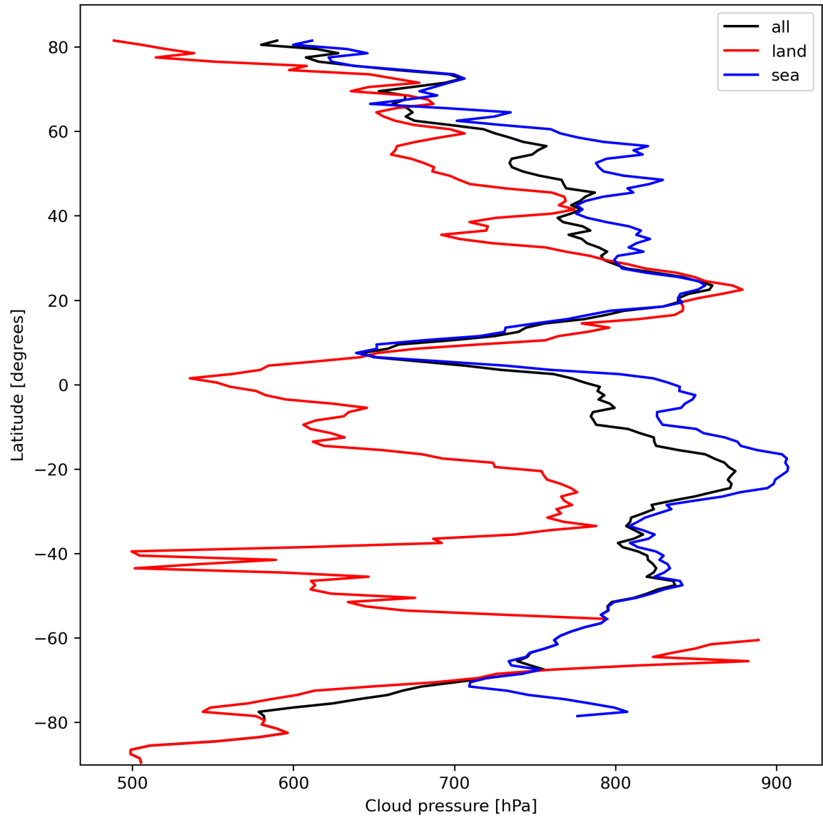
Figure 13: Zonal average of “Cloud pressure” for 2023-10-08 to 2023-10-10.
