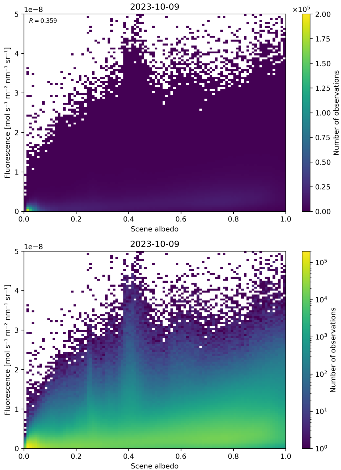
Figure 114: Scatter density plot of “Scene albedo” against “Fluorescence” for 2023-10-08 to 2023-10-10.
