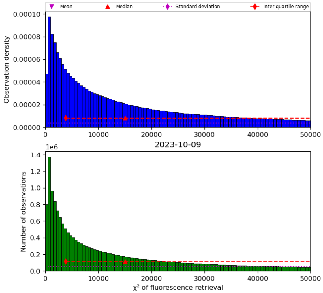
Figure 42: Histogram of “ \chi^2 of fluorescence retrieval” for 2023-10-08 to 2023-10-10
