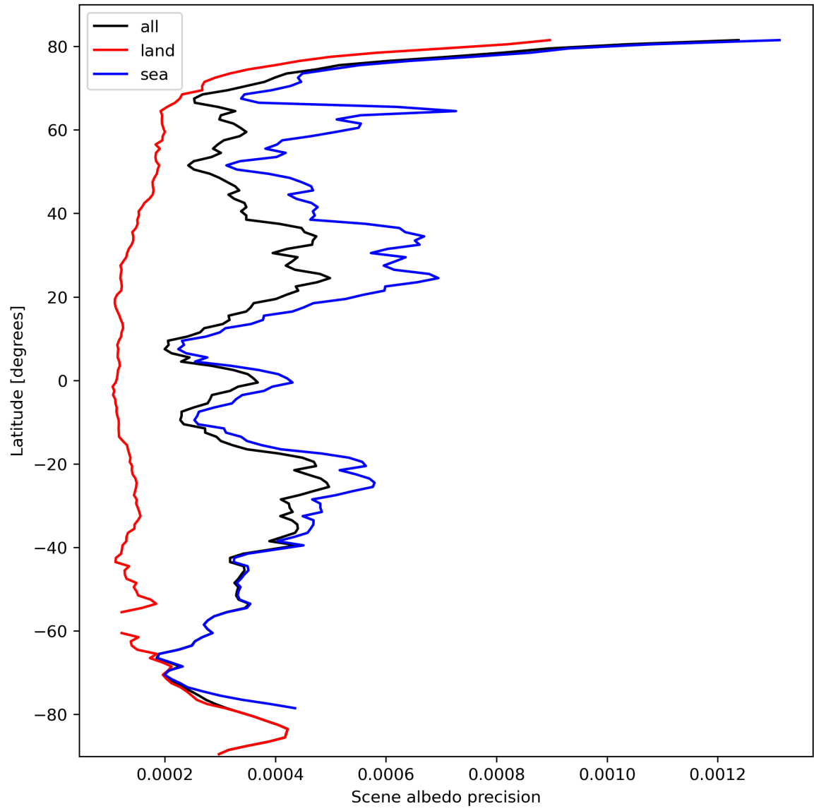
Figure 18: Zonal average of “Scene albedo precision” for 2023-10-08 to 2023-10-10.
