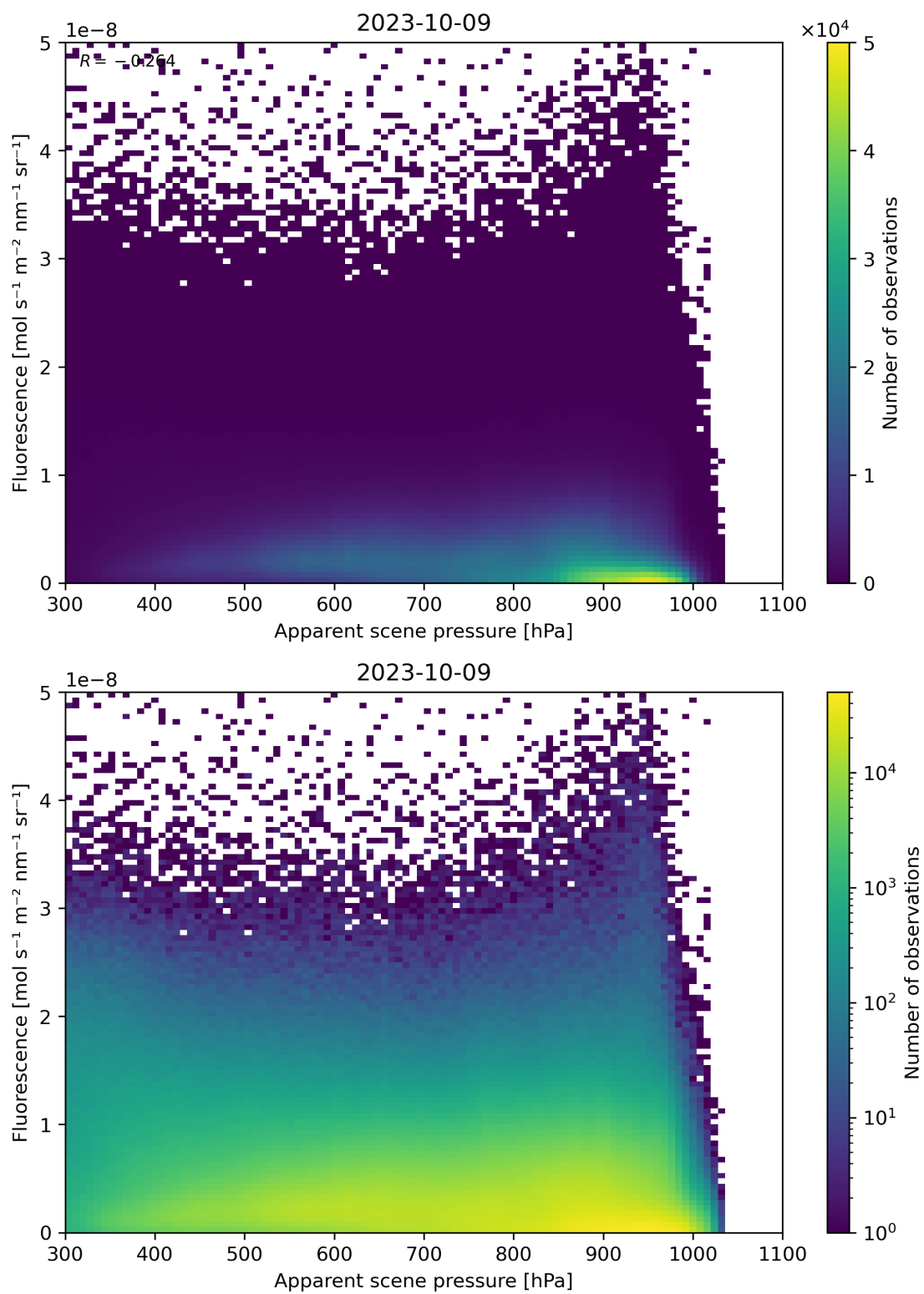
Figure 65: Scatter density plot of “Apparent scene pressure” against “Fluorescence” for 2023-10-08 to 2023-10-10.
