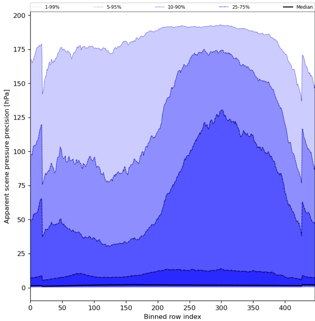
Figure 54: Along track statistics of “Apparent scene pressure precision” for 2023-10-08 to 2023-10-10
