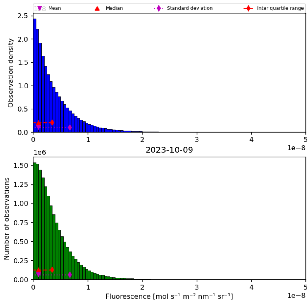
Figure 40: Histogram of “Fluorescence” for 2023-10-08 to 2023-10-10
