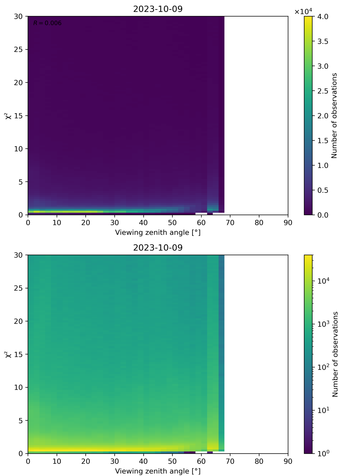
Figure 130: Scatter density plot of “Viewing zenith angle” against “ \chi^2 ” for 2023-10-08 to 2023-10-10.
