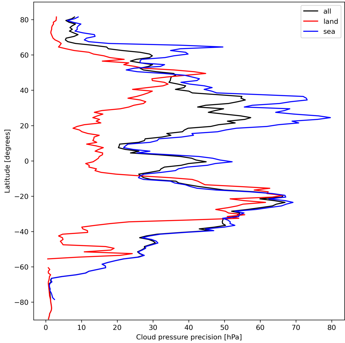
Figure 14: Zonal average of “Cloud pressure precision” for 2023-10-08 to 2023-10-10.
