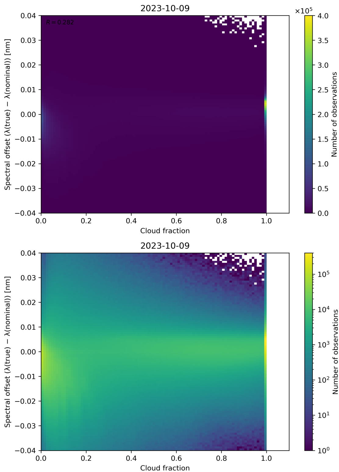
Figure 83: Scatter density plot of “Cloud fraction” against “Spectral offset ( \lambda(\text{true}) - \lambda(\text{nominal}) )” for 2023-10-08 to 2023-10-10.
