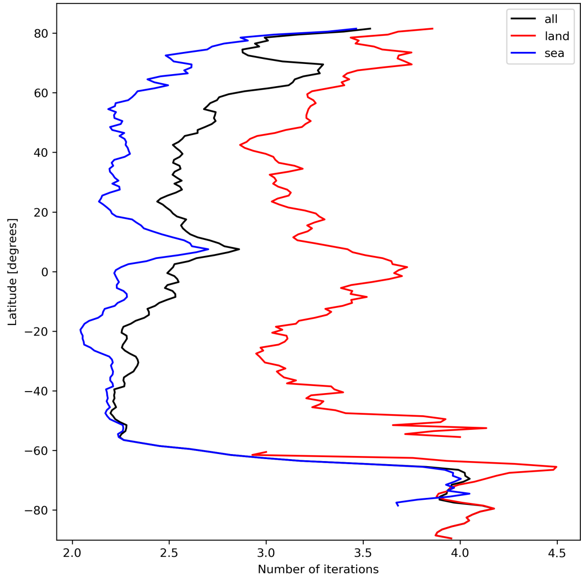
Figure 22: Zonal average of “Number of iterations” for 2023-10-08 to 2023-10-10.
