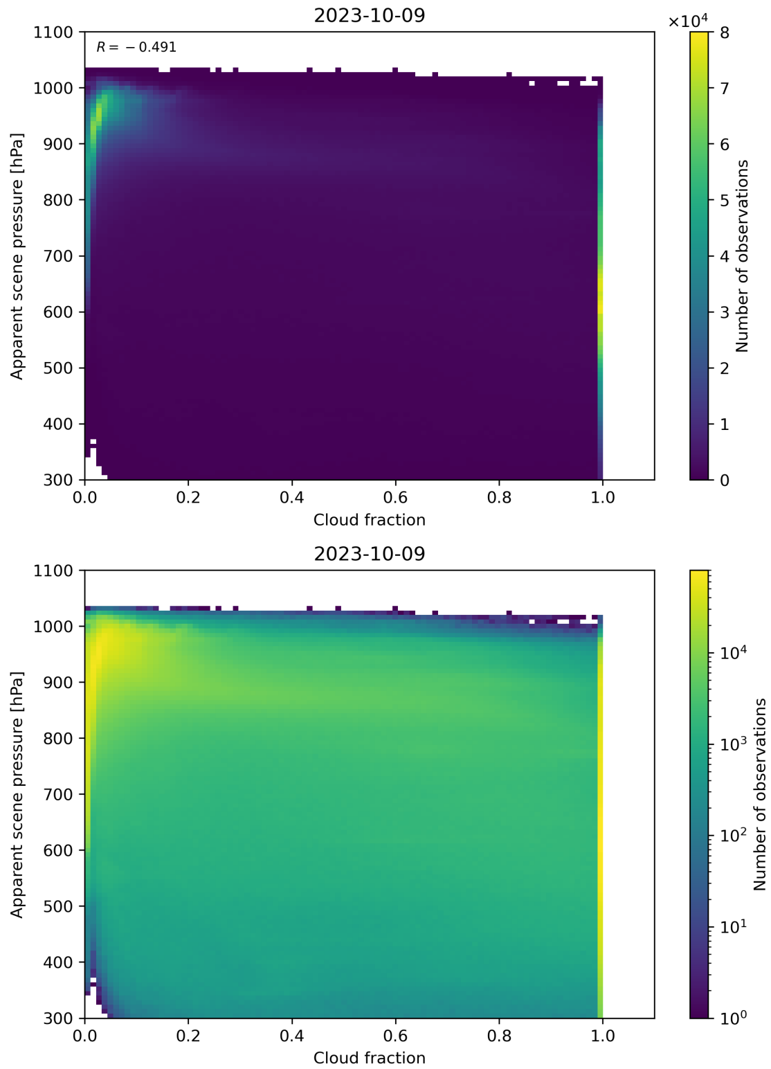
Figure 76: Scatter density plot of “Cloud fraction” against “Apparent scene pressure” for 2023-10-08 to 2023-10-10.
