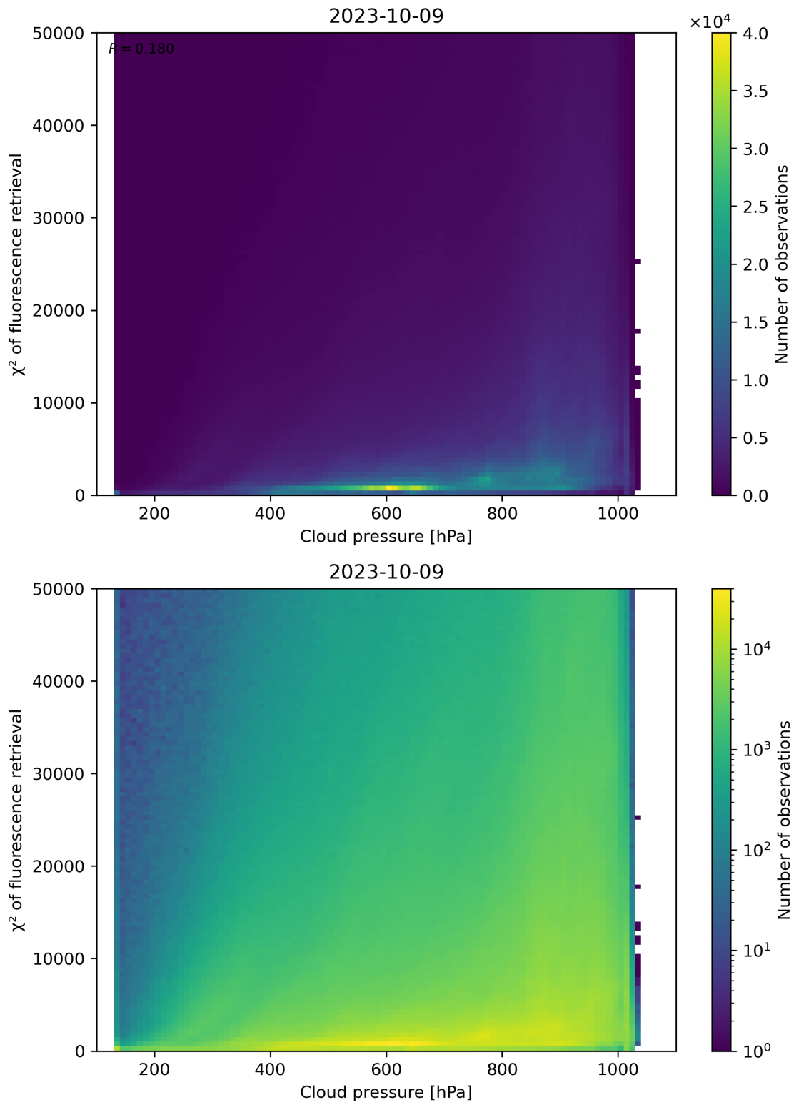
Figure 86: Scatter density plot of “Cloud pressure” against “ \chi^2 of fluorescence retrieval” for 2023-10-08 to 2023-10-10.
