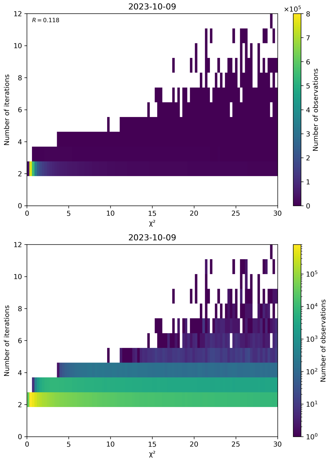
Figure 73: Scatter density plot of “ \chi^2 ” against “Number of iterations” for 2023-10-08 to 2023-10-10.
