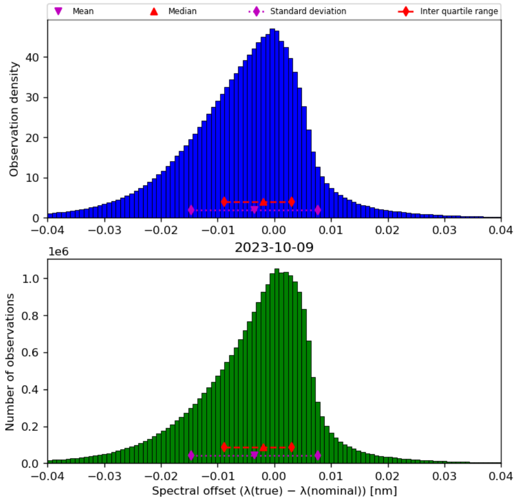
Figure 45: Histogram of “Spectral offset ( \lambda(\text{true}) - \lambda(\text{nominal}) )” for 2023-10-08 to 2023-10-10
