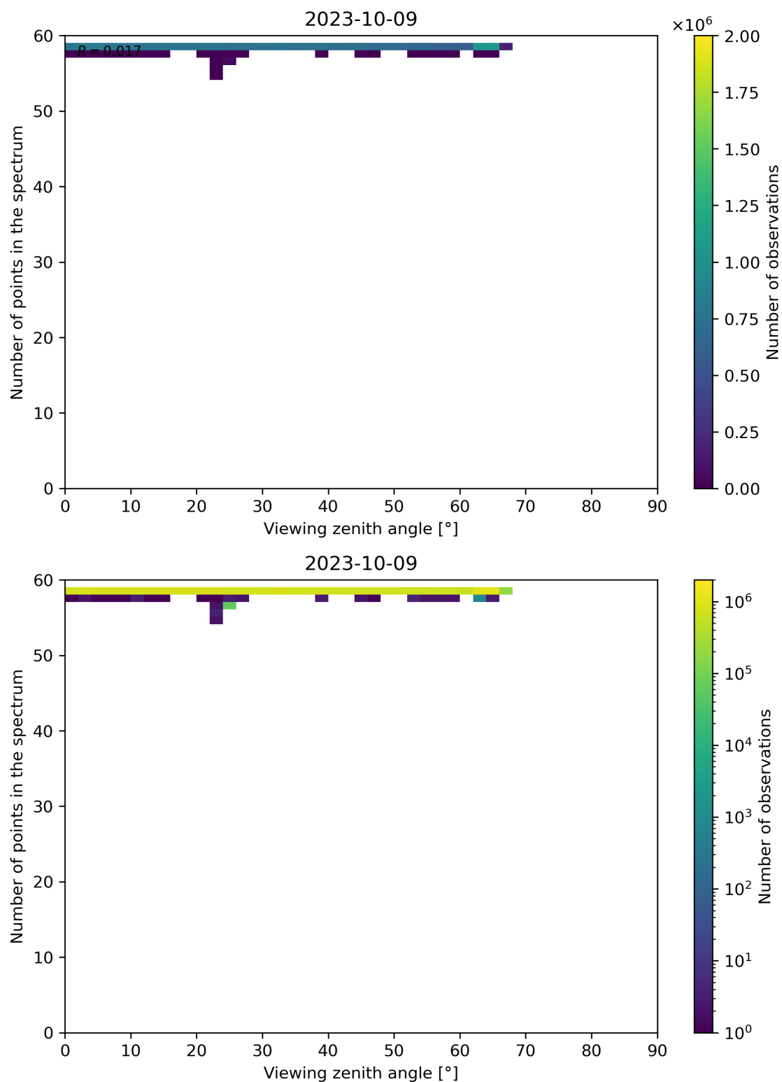
Figure 137: Scatter density plot of “Viewing zenith angle” against “Number of points in the spectrum” for 2023-10-08 to 2023-10-10.
