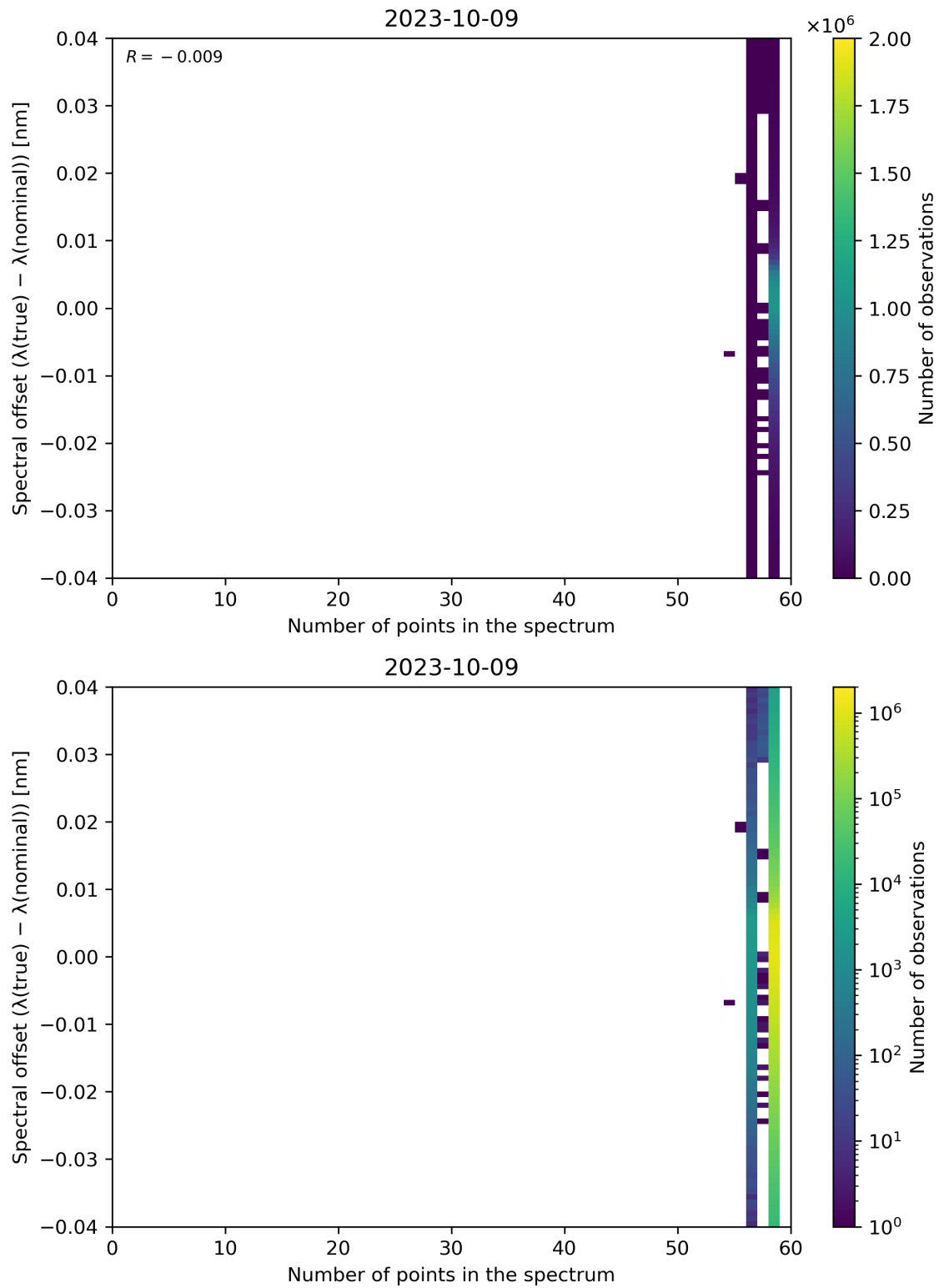
Figure 110: Scatter density plot of “Number of points in the spectrum” against “Spectral offset ( \lambda(\text{true}) - \lambda(\text{nominal}) )” for 2023-10-08 to 2023-10-10.
