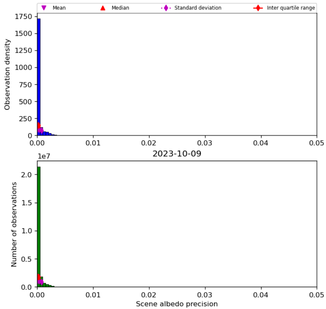
Figure 35: Histogram of “Scene albedo precision” for 2023-10-08 to 2023-10-10
