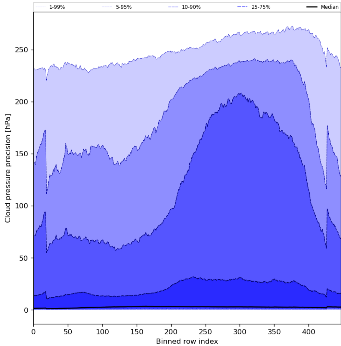
Figure 48: Along track statistics of “Cloud pressure precision” for 2023-10-08 to 2023-10-10
