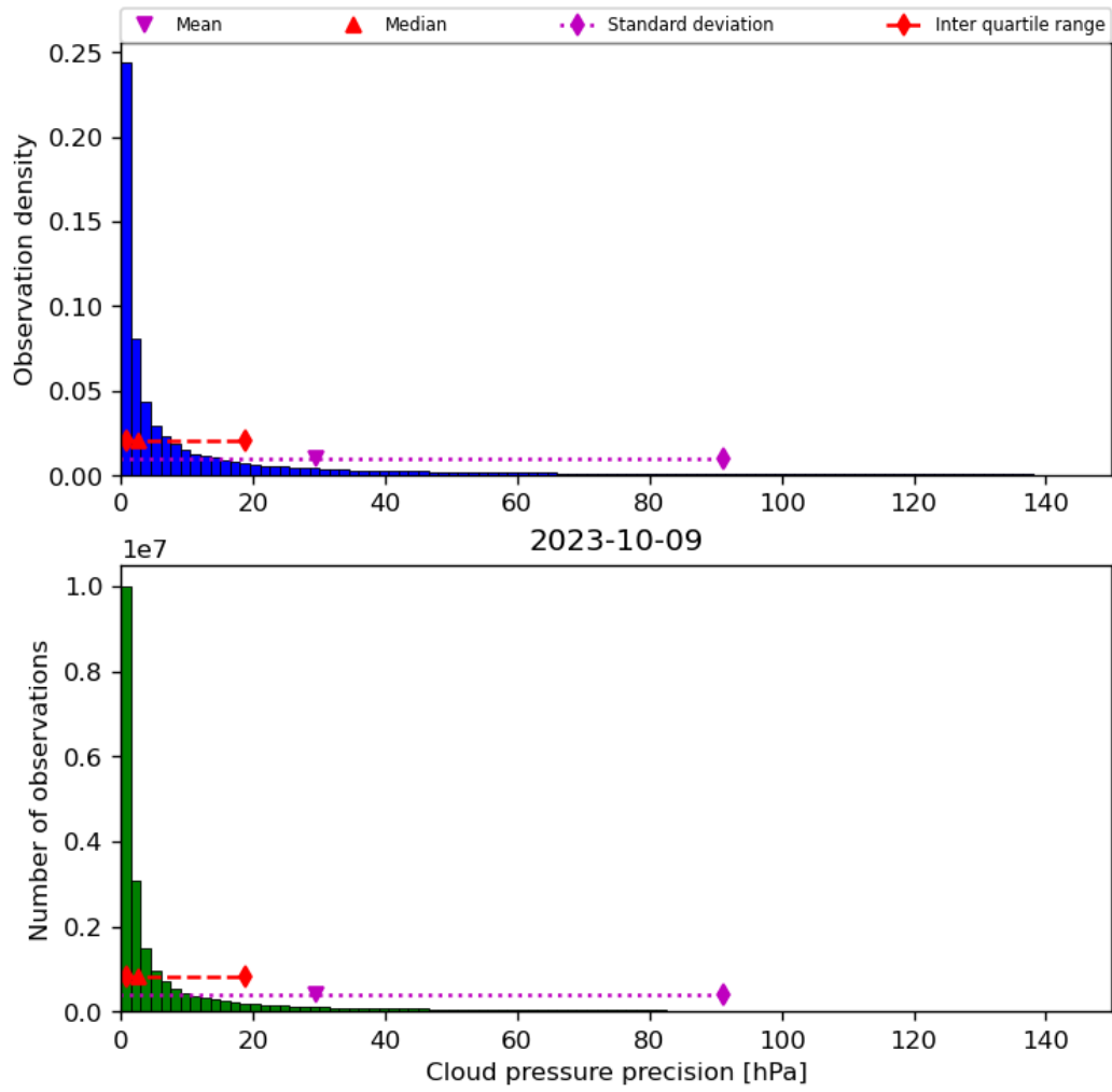
Figure 31: Histogram of “Cloud pressure precision” for 2023-10-08 to 2023-10-10
