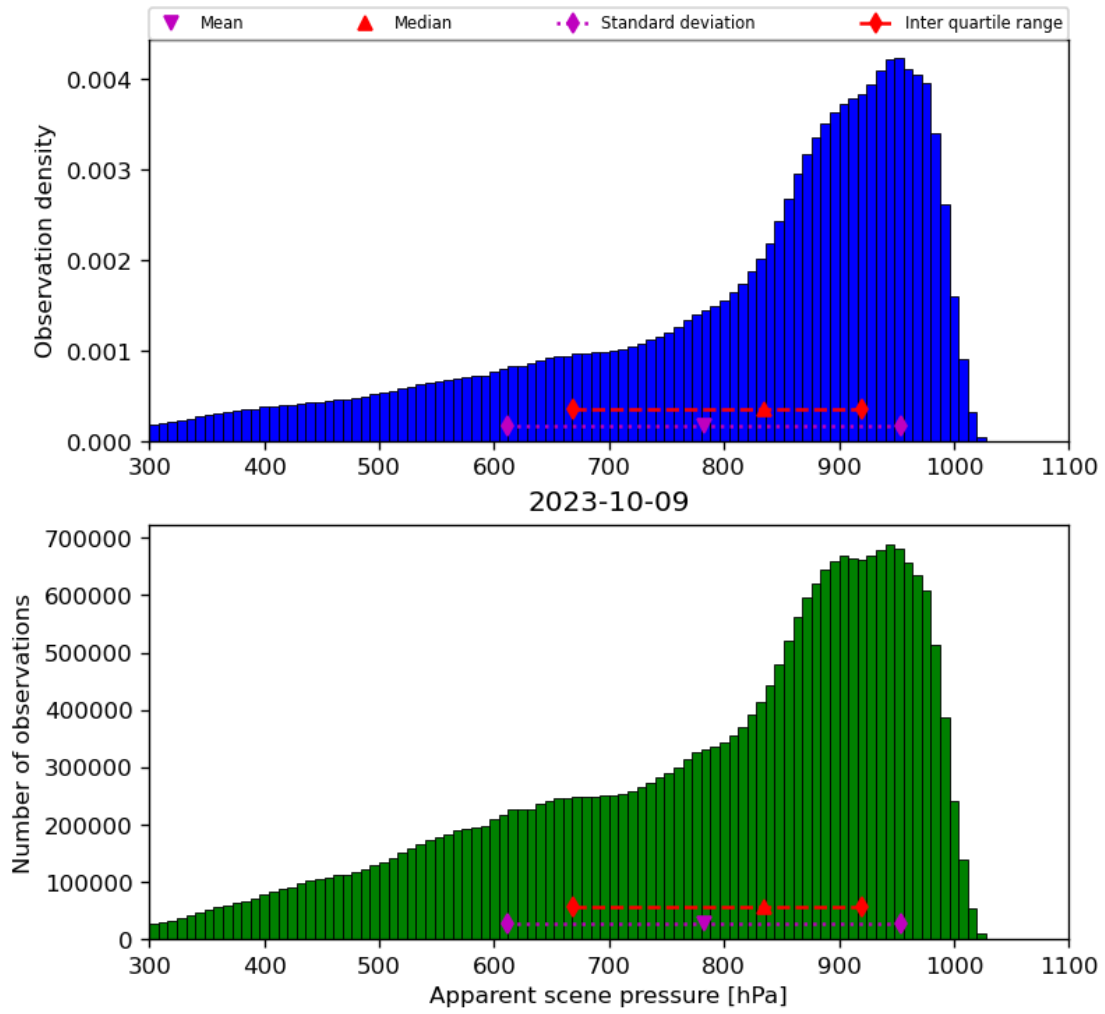
Figure 36: Histogram of “Apparent scene pressure” for 2023-10-08 to 2023-10-10
