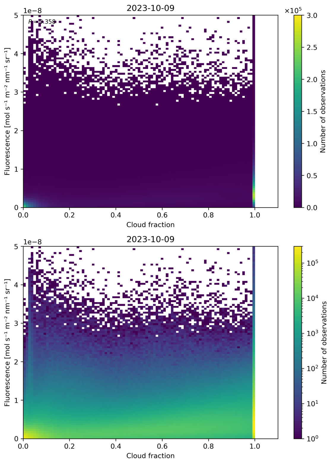
Figure 79: Scatter density plot of “Cloud fraction” against “Fluorescence” for 2023-10-08 to 2023-10-10.
