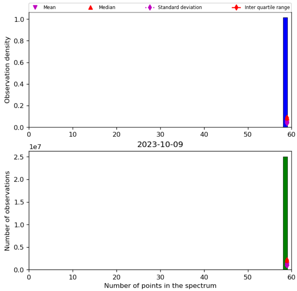
Figure 44: Histogram of “Number of points in the spectrum” for 2023-10-08 to 2023-10-10
