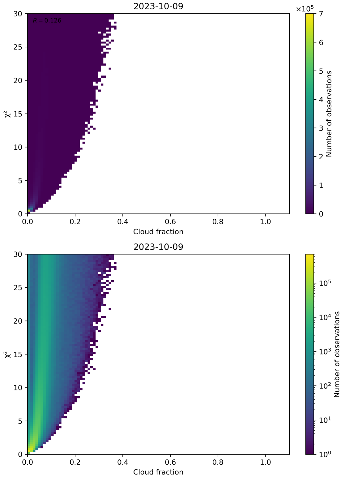
Figure 77: Scatter density plot of “Cloud fraction” against “ \chi^2 ” for 2023-10-08 to 2023-10-10.
