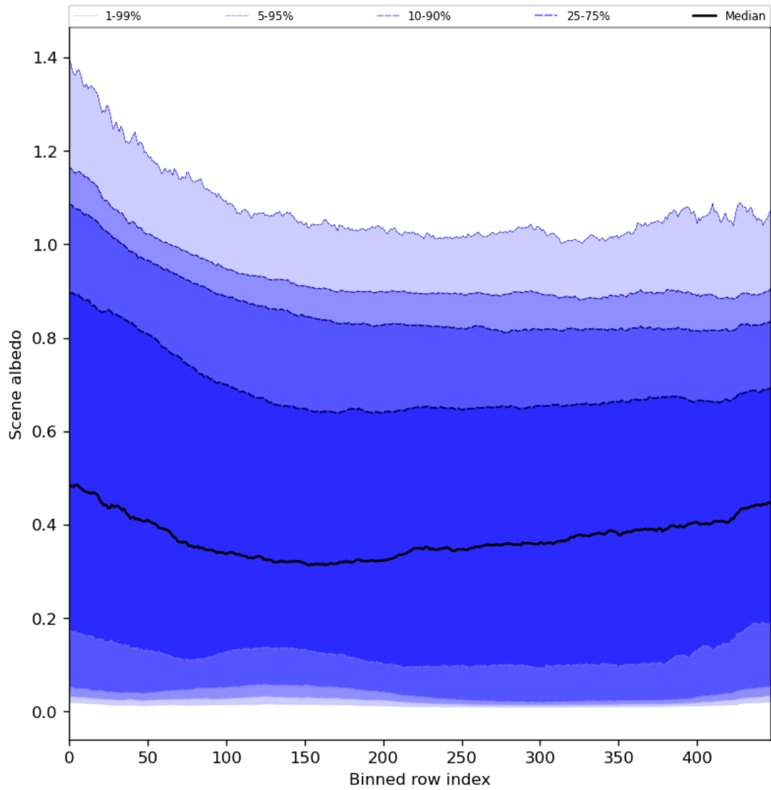
Figure 51: Along track statistics of “Scene albedo” for 2023-10-08 to 2023-10-10
