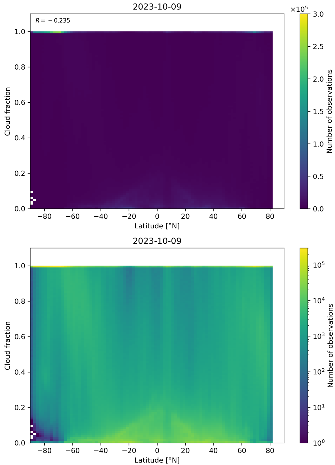
Figure 99: Scatter density plot of “Latitude” against “Cloud fraction” for 2023-10-08 to 2023-10-10.
