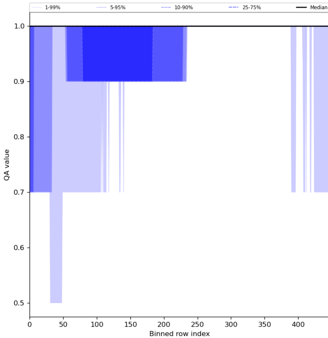
Figure 46: Along track statistics of “QA value” for 2023-10-08 to 2023-10-10
