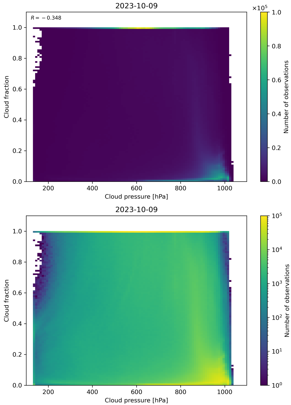
Figure 87: Scatter density plot of “Cloud pressure” against “Cloud fraction” for 2023-10-08 to 2023-10-10.
