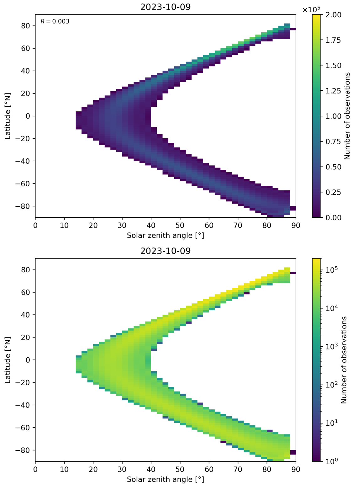
Figure 124: Scatter density plot of “Solar zenith angle” against “Latitude” for 2023-10-08 to 2023-10-10.
