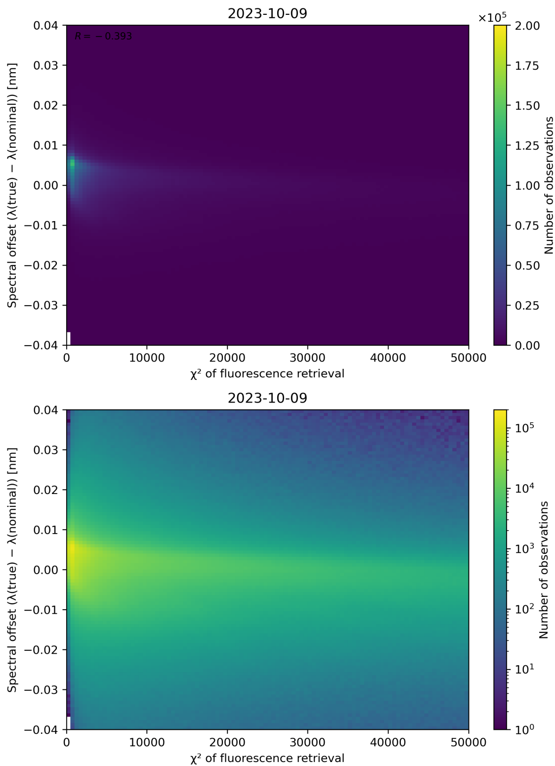
Figure 72: Scatter density plot of " \chi^2 of fluorescence retrieval" against "Spectral offset ( \lambda(\text{true}) - \lambda(\text{nominal}) )" for 2023-10-08 to 2023-10-10.
