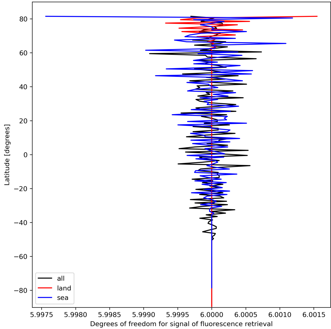
Figure 26: Zonal average of “Degrees of freedom for signal of fluorescence retrieval” for 2023-10-08 to 2023-10-10.
