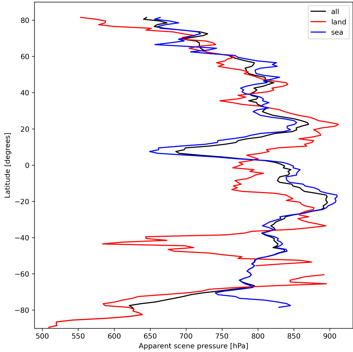
Figure 19: Zonal average of “Apparent scene pressure” for 2023-10-08 to 2023-10-10.
