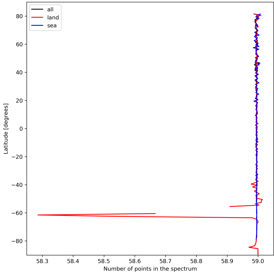
Figure 27: Zonal average of “Number of points in the spectrum” for 2023-10-08 to 2023-10-10.
