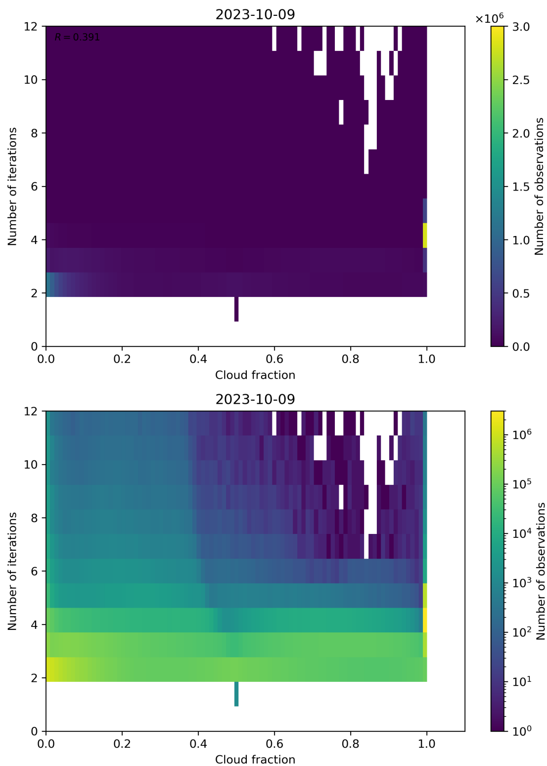
Figure 80: Scatter density plot of “Cloud fraction” against “Number of iterations” for 2023-10-08 to 2023-10-10.
