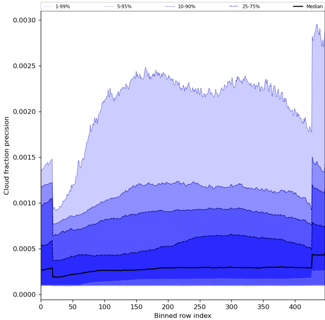
Figure 50: Along track statistics of “Cloud fraction precision” for 2023-10-08 to 2023-10-10
