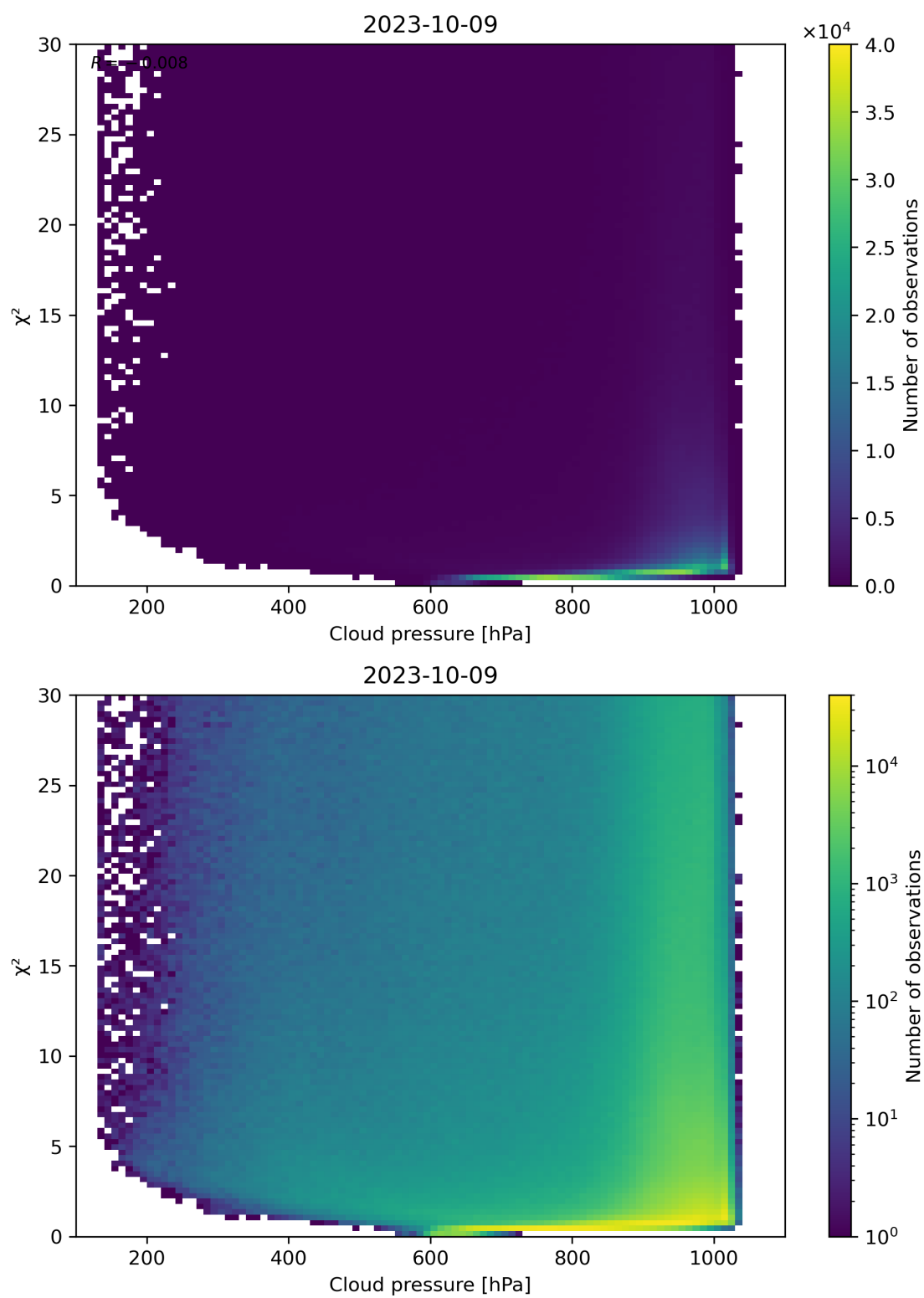
Figure 85: Scatter density plot of “Cloud pressure” against “ \chi^2 ” for 2023-10-08 to 2023-10-10.
