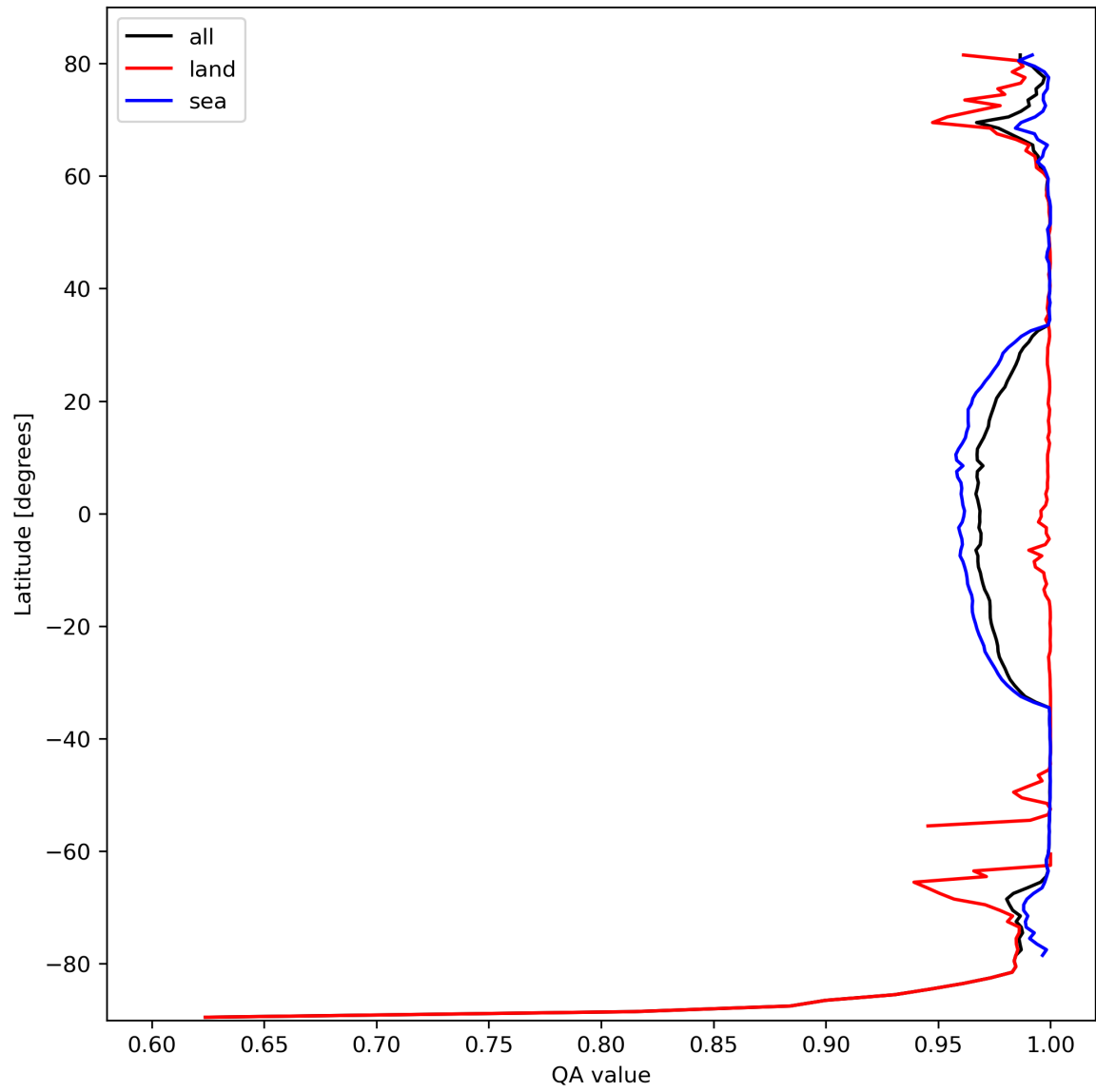
Figure 12: Zonal average of “QA value” for 2023-10-08 to 2023-10-10.
