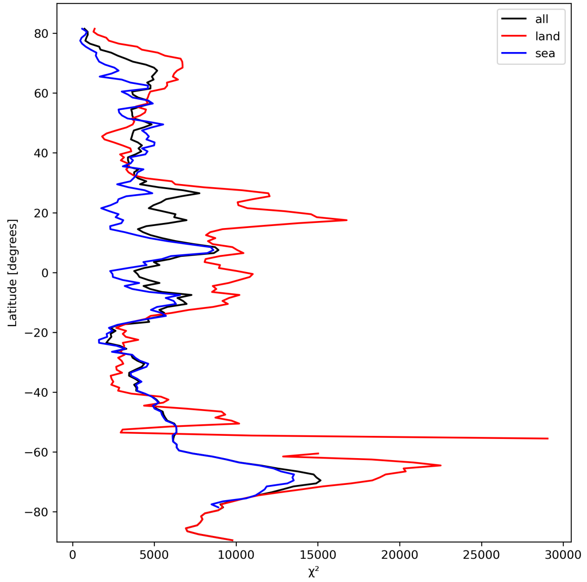
Figure 21: Zonal average of “ \chi^2 ” for 2023-10-08 to 2023-10-10.
