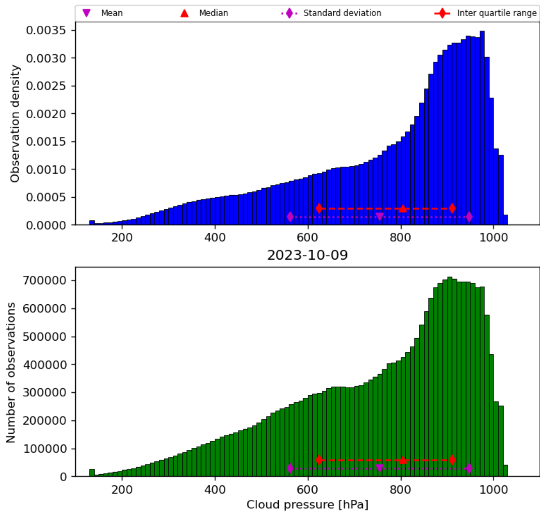
Figure 30: Histogram of “Cloud pressure” for 2023-10-08 to 2023-10-10
