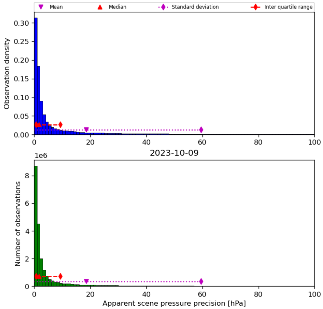
Figure 37: Histogram of “Apparent scene pressure precision” for 2023-10-08 to 2023-10-10
