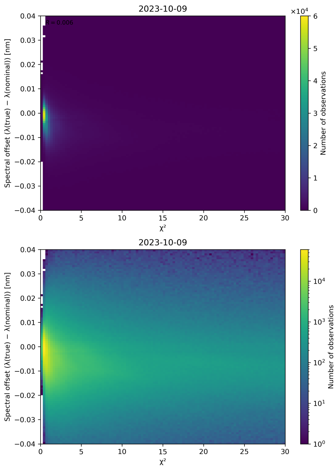
Figure 75: Scatter density plot of “ \chi^2 ” against “Spectral offset ( \lambda(\text{true}) - \lambda(\text{nominal}) )” for 2023-10-08 to 2023-10-10.
