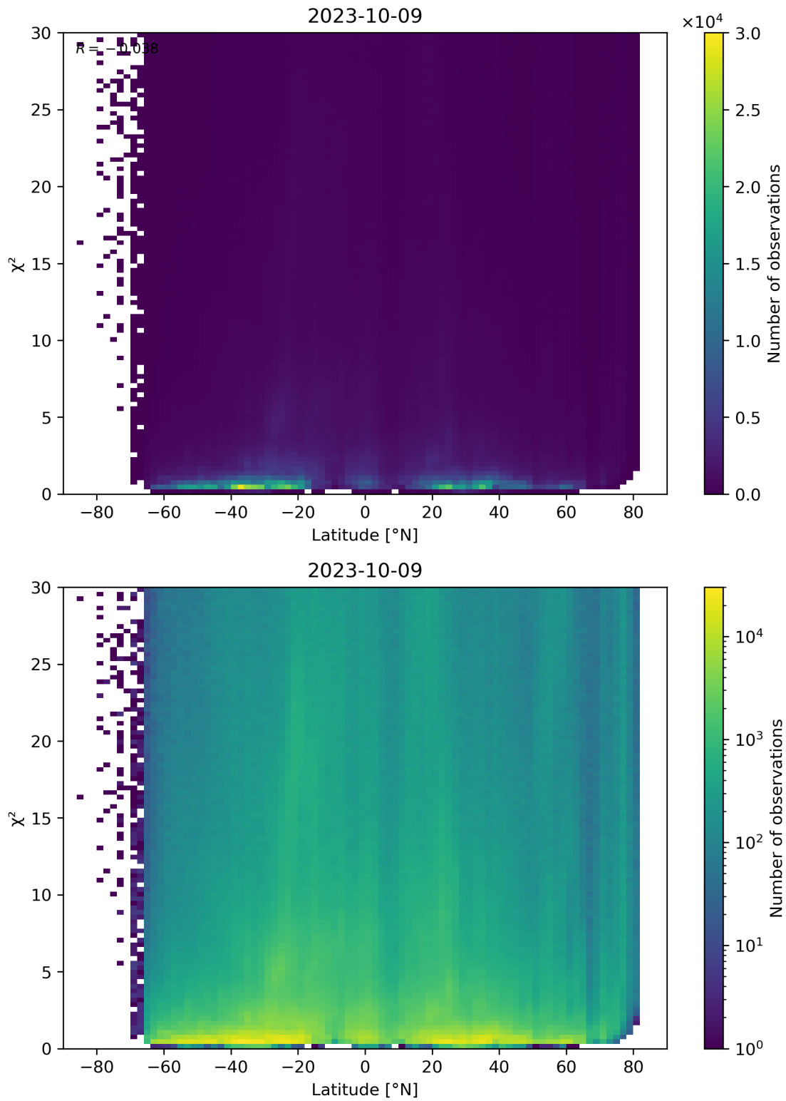
Figure 97: Scatter density plot of “Latitude” against “ \chi^2 ” for 2023-10-08 to 2023-10-10.
