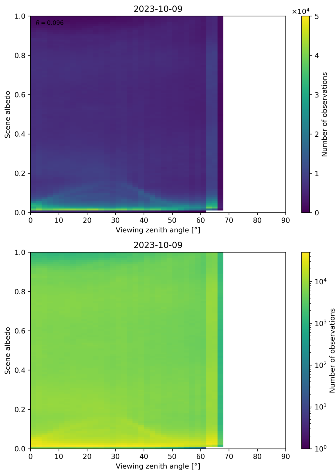
Figure 138: Scatter density plot of “Viewing zenith angle” against “Scene albedo” for 2023-10-08 to 2023-10-10.
