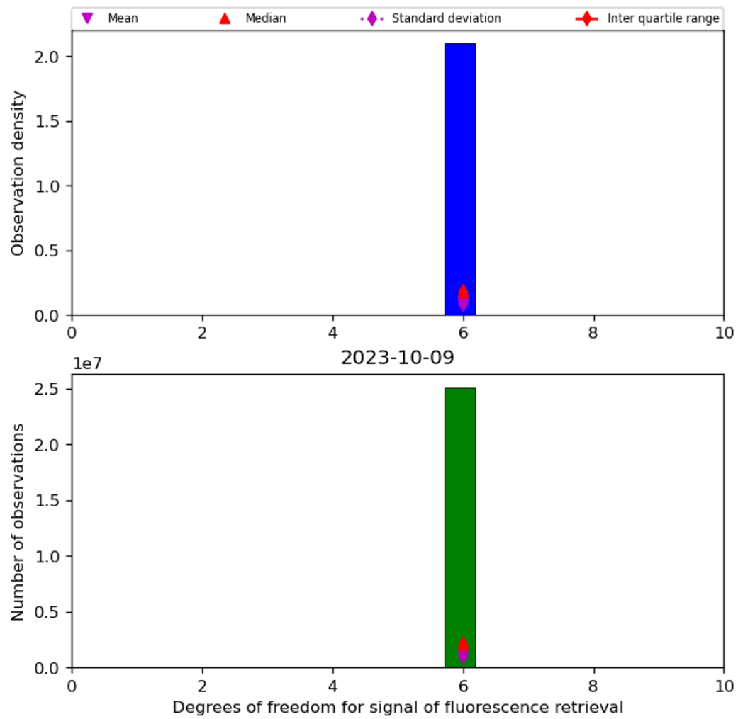
Figure 43: Histogram of “Degrees of freedom for signal of fluorescence retrieval” for 2023-10-08 to 2023-10-10
