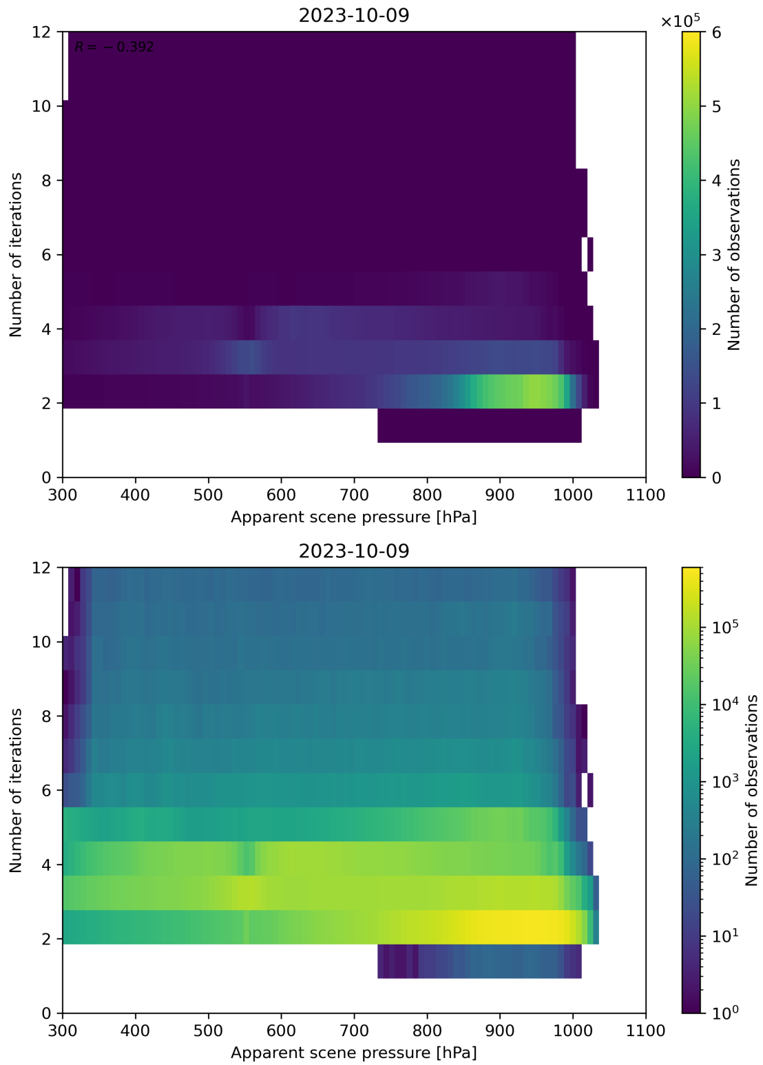
Figure 66: Scatter density plot of “Apparent scene pressure” against “Number of iterations” for 2023-10-08 to 2023-10-10.
