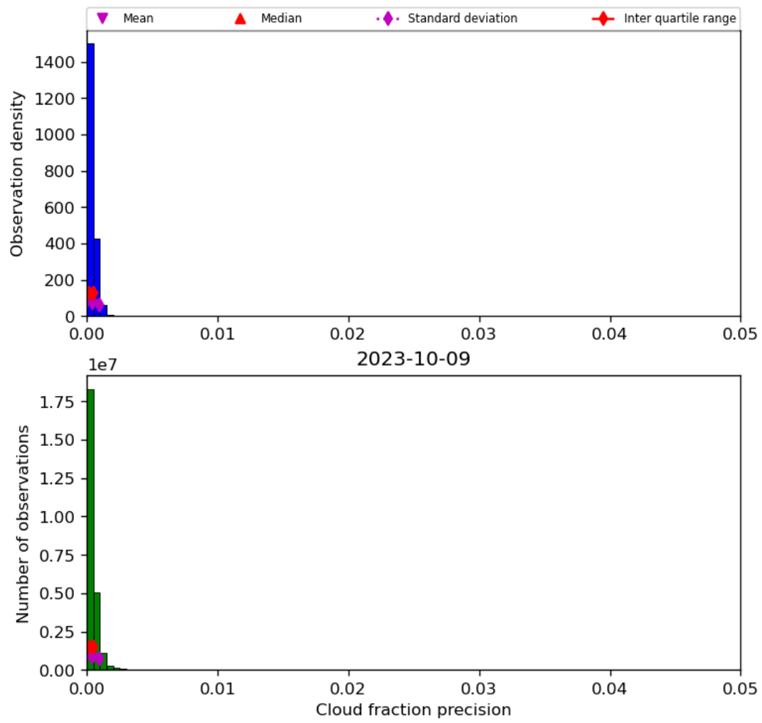
Figure 33: Histogram of “Cloud fraction precision” for 2023-10-08 to 2023-10-10
