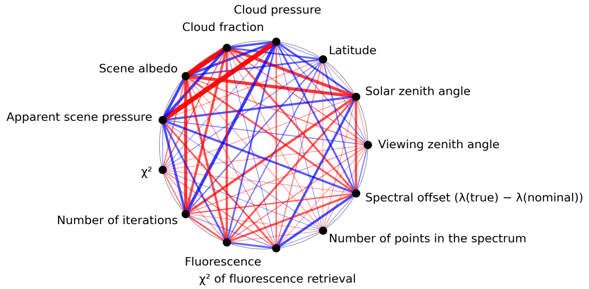
Figure 1: Map of correlation graph for 2023-10-08 to 2023-10-10.
