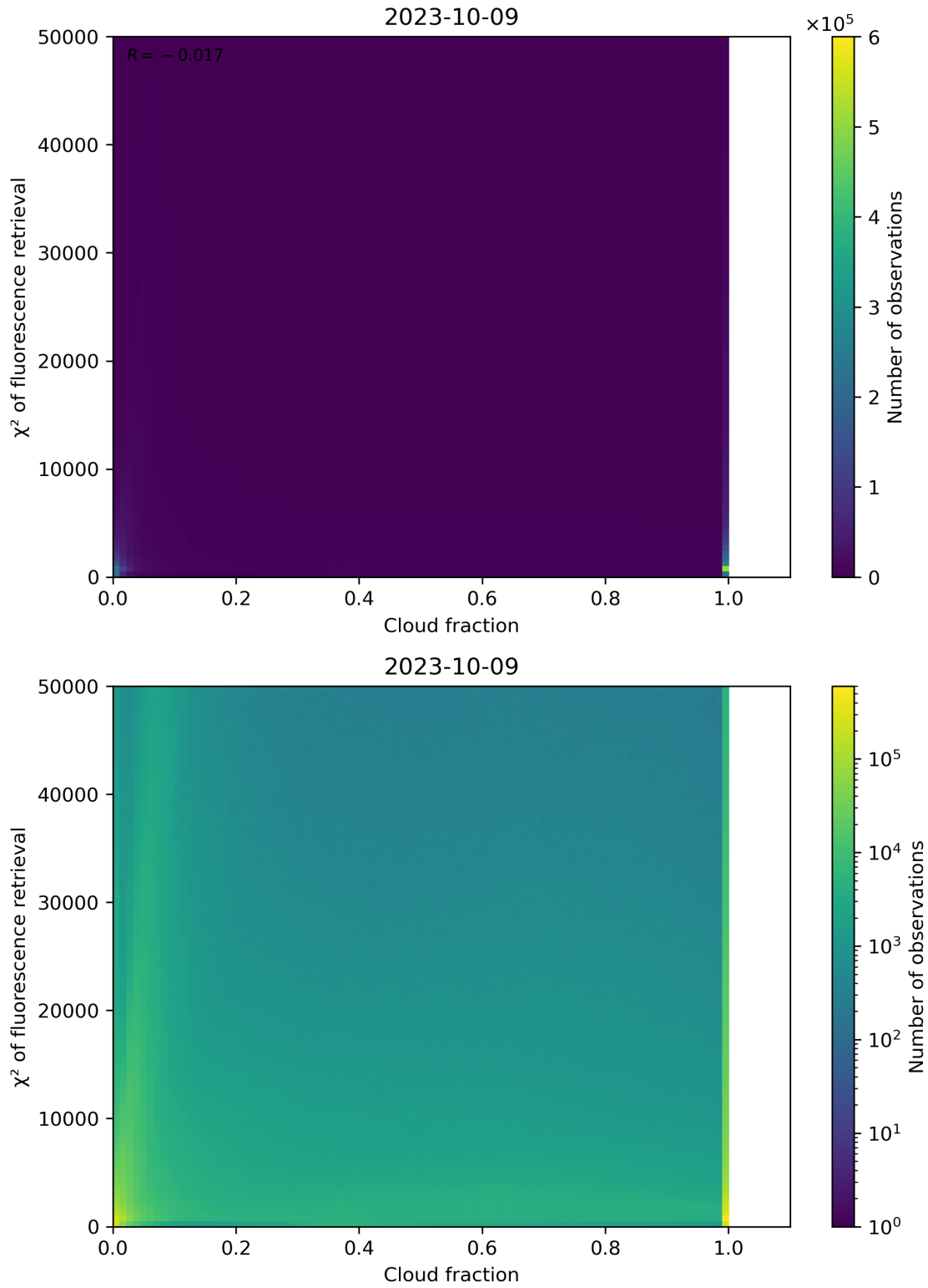
Figure 78: Scatter density plot of “Cloud fraction” against “ \chi^2 of fluorescence retrieval” for 2023-10-08 to 2023-10-10.
