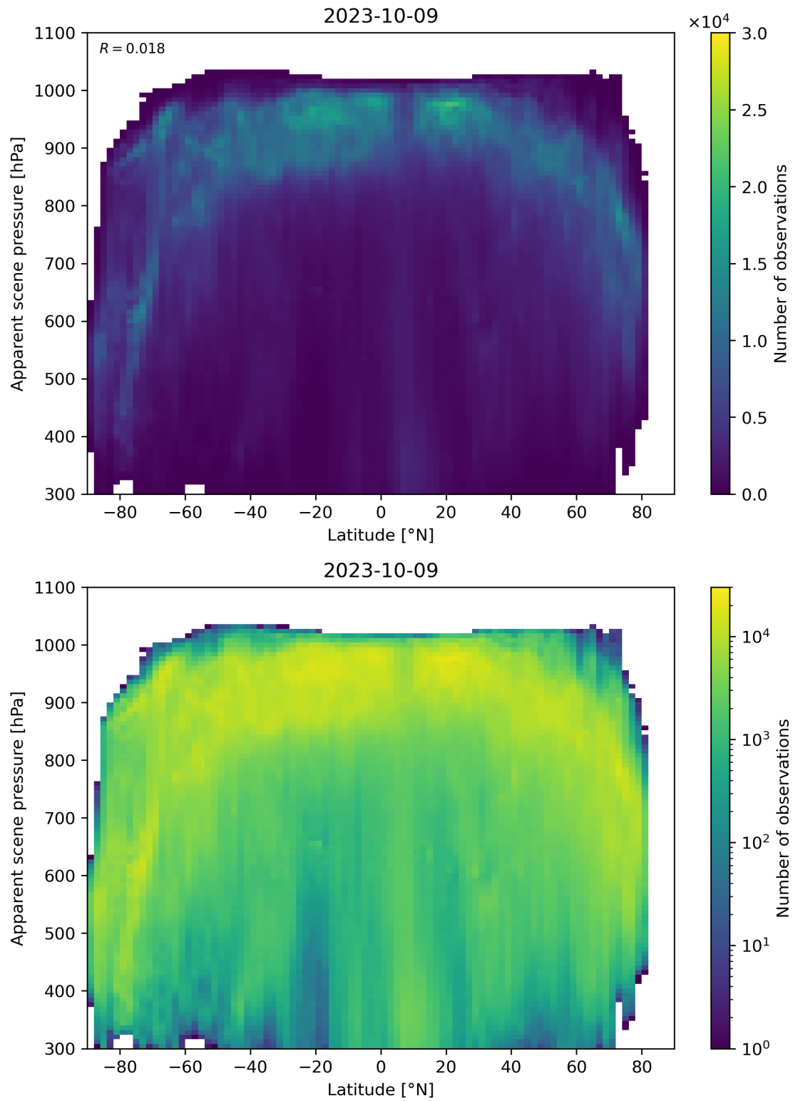
Figure 96: Scatter density plot of “Latitude” against “Apparent scene pressure” for 2023-10-08 to 2023-10-10.
