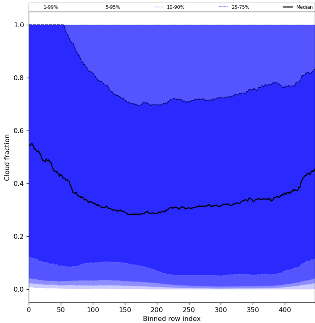
Figure 49: Along track statistics of “Cloud fraction” for 2023-10-08 to 2023-10-10
