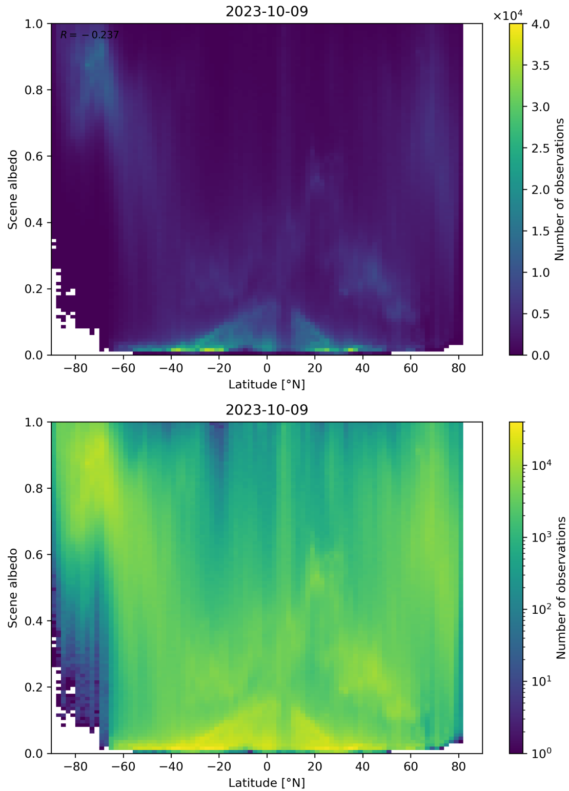
Figure 104: Scatter density plot of “Latitude” against “Scene albedo” for 2023-10-08 to 2023-10-10.
