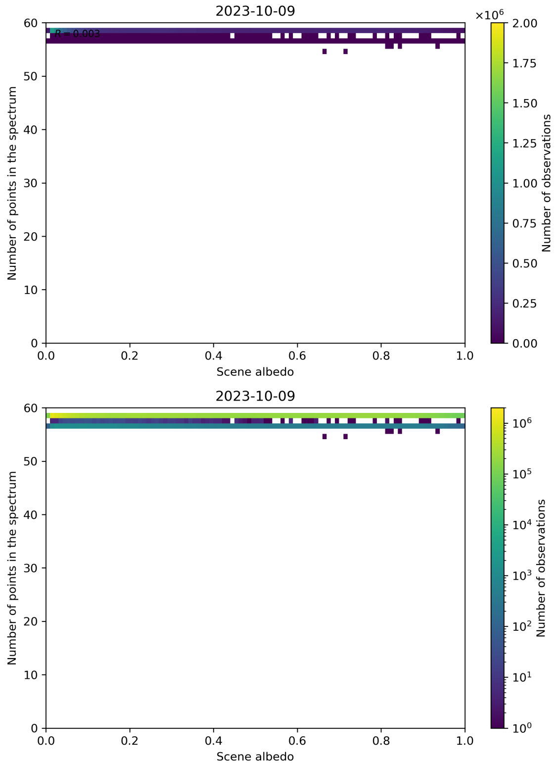
Figure 116: Scatter density plot of “Scene albedo” against “Number of points in the spectrum” for 2023-10-08 to 2023-10-10.
