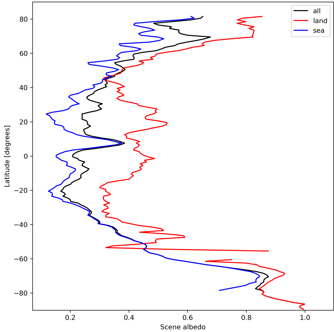
Figure 17: Zonal average of “Scene albedo” for 2023-10-08 to 2023-10-10.
