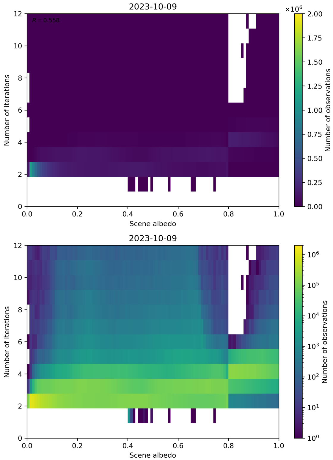
Figure 115: Scatter density plot of “Scene albedo” against “Number of iterations” for 2023-10-08 to 2023-10-10.
