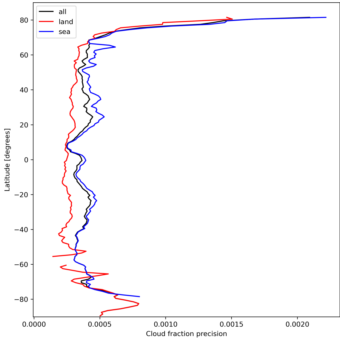
Figure 16: Zonal average of “Cloud fraction precision” for 2023-10-08 to 2023-10-10.
