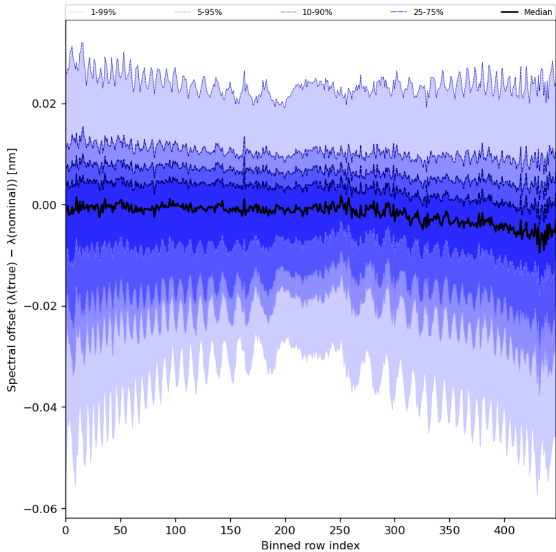
Figure 62: Along track statistics of “Spectral offset ( \lambda(\text{true}) - \lambda(\text{nominal}) )” for 2023-10-08 to 2023-10-10
