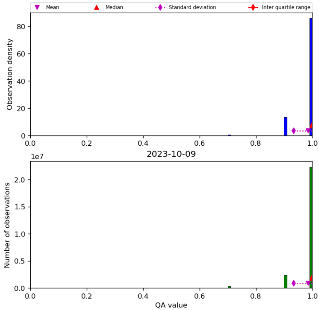
Figure 29: Histogram of “QA value” for 2023-10-08 to 2023-10-10
