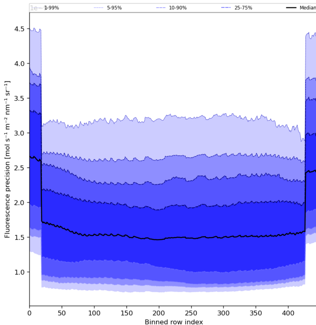
Figure 58: Along track statistics of “Fluorescence precision” for 2023-10-08 to 2023-10-10
