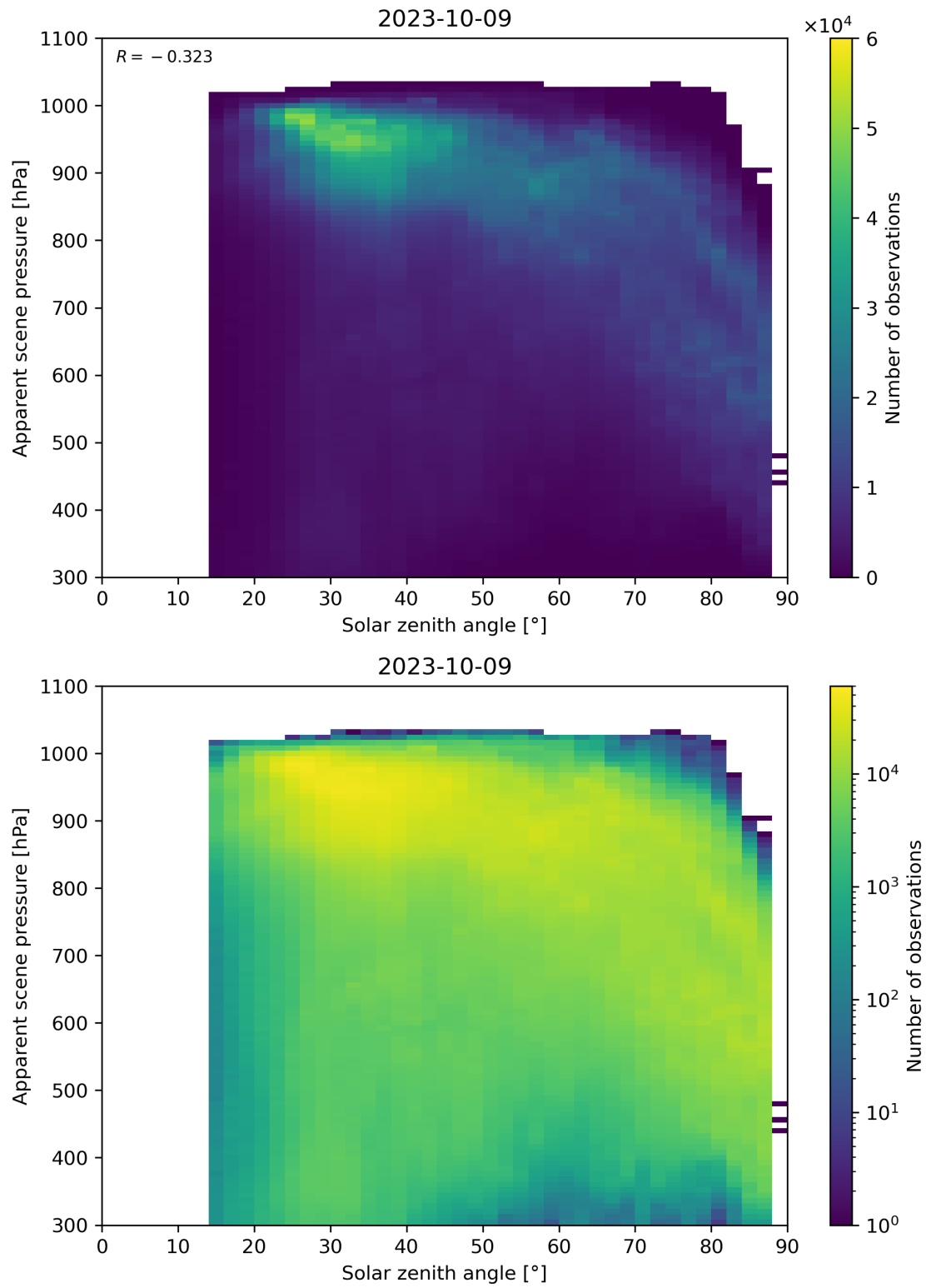
Figure 118: Scatter density plot of “Solar zenith angle” against “Apparent scene pressure” for 2023-10-08 to 2023-10-10.
