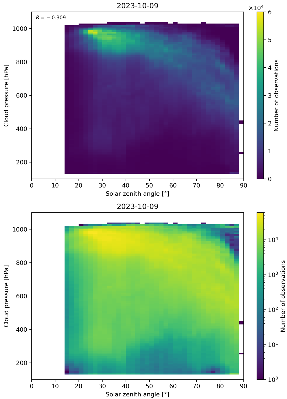
Figure 122: Scatter density plot of “Solar zenith angle” against “Cloud pressure” for 2023-10-08 to 2023-10-10.
