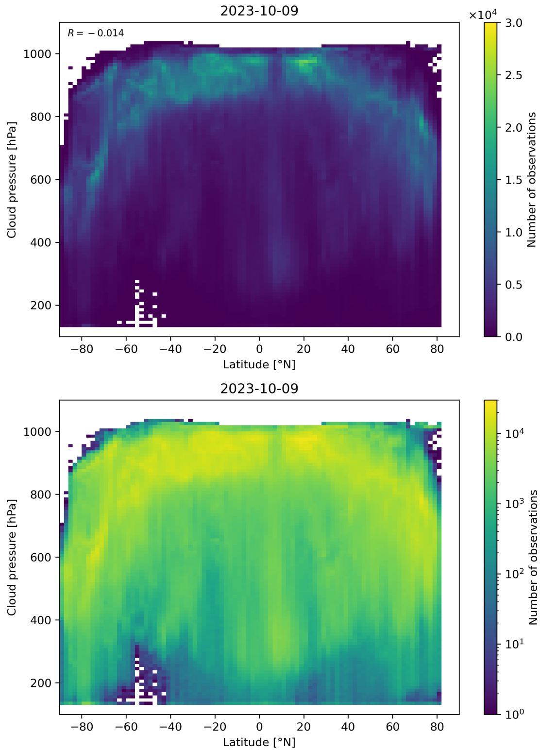
Figure 100: Scatter density plot of “Latitude” against “Cloud pressure” for 2023-10-08 to 2023-10-10.
