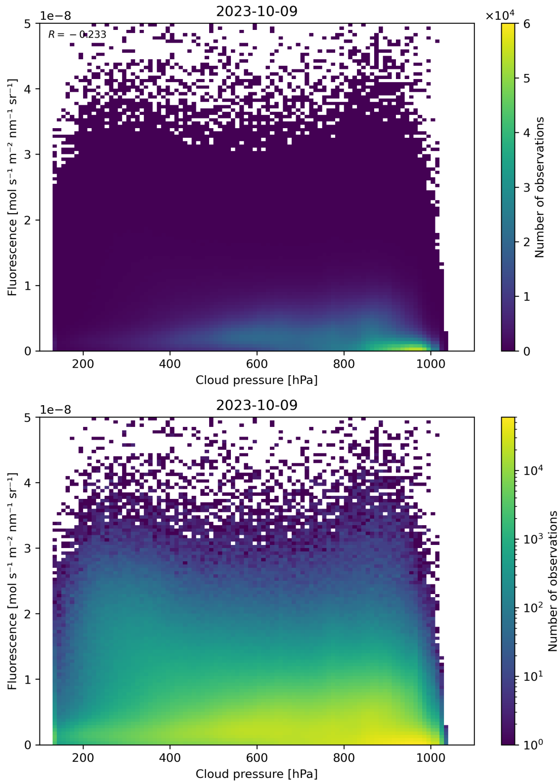
Figure 88: Scatter density plot of “Cloud pressure” against “Fluorescence” for 2023-10-08 to 2023-10-10.
