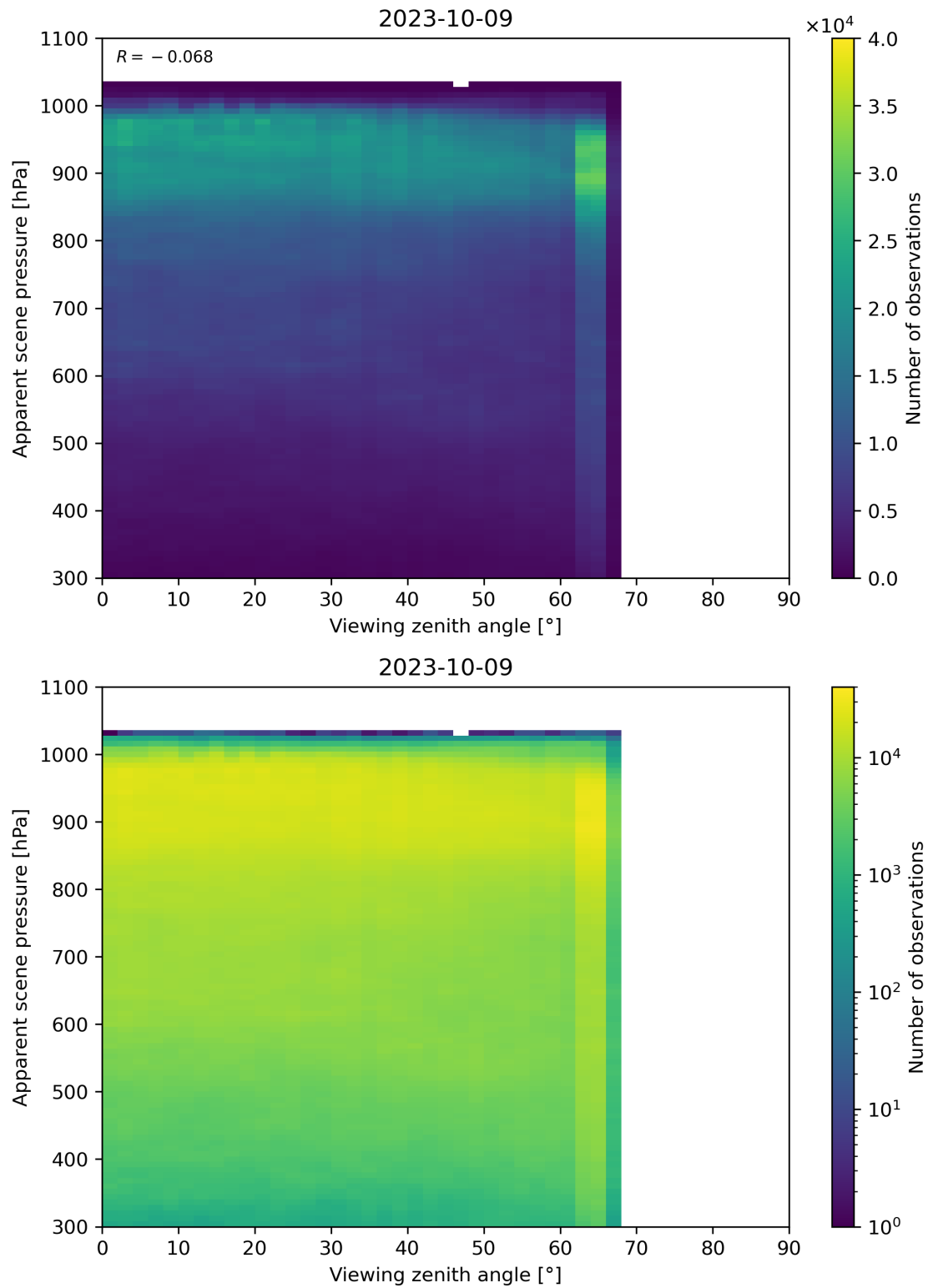
Figure 129: Scatter density plot of “Viewing zenith angle” against “Apparent scene pressure” for 2023-10-08 to 2023-10-10.
