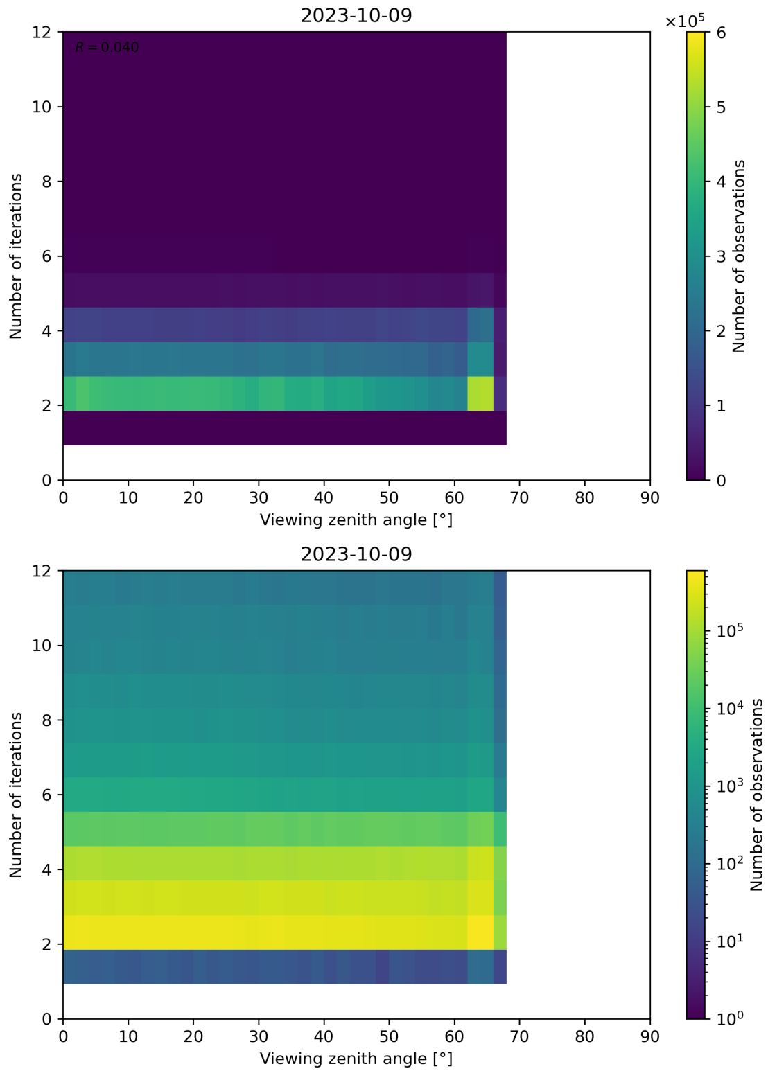
Figure 136: Scatter density plot of “Viewing zenith angle” against “Number of iterations” for 2023-10-08 to 2023-10-10.
