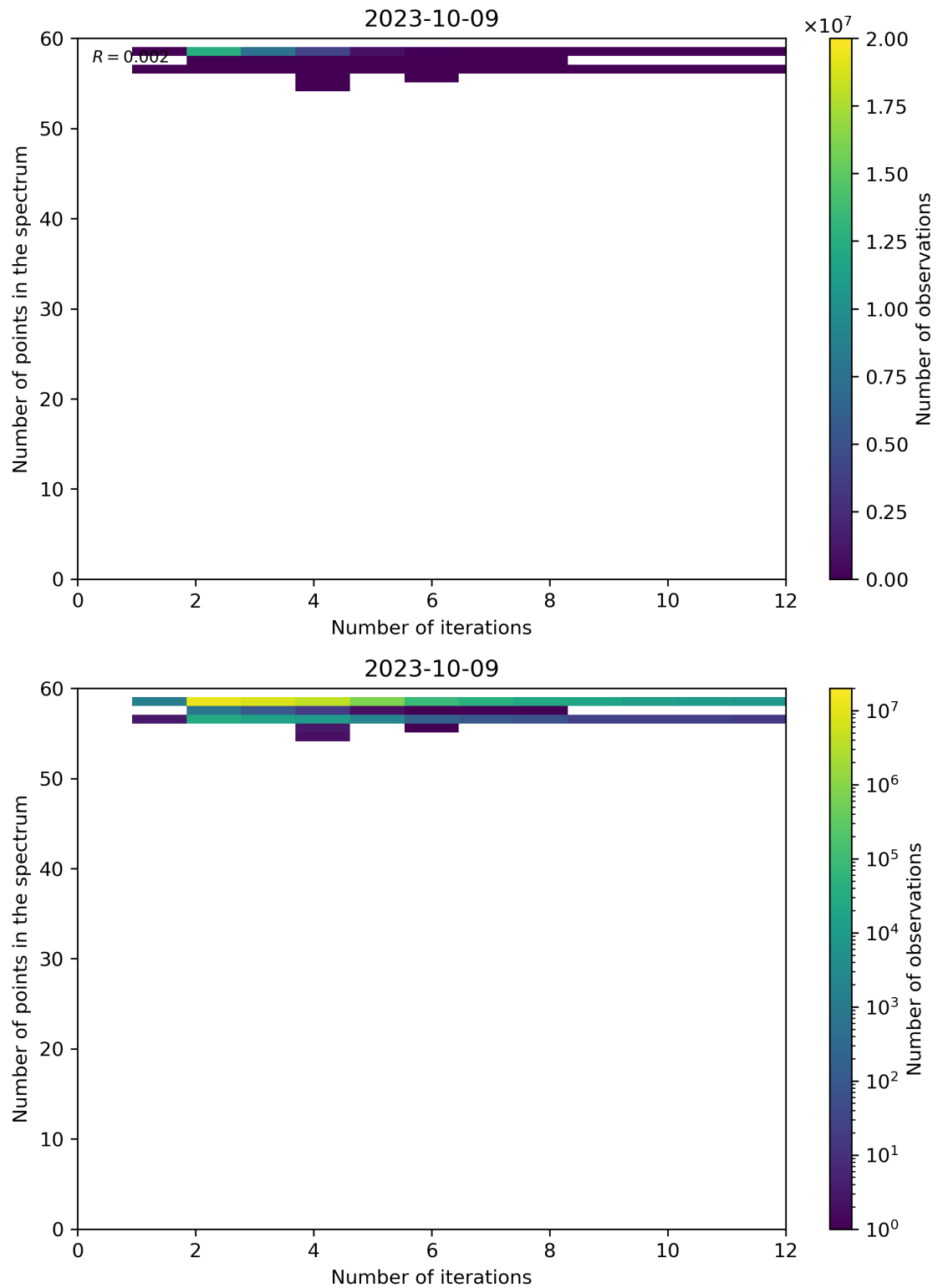
Figure 108: Scatter density plot of “Number of iterations” against “Number of points in the spectrum” for 2023-10-08 to 2023-10-10.
