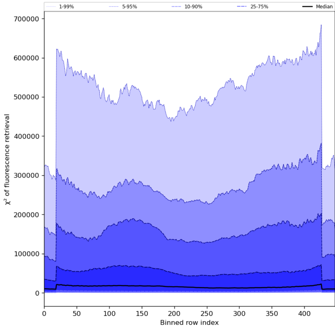
Figure 59: Along track statistics of “ \chi^2 of fluorescence retrieval” for 2023-10-08 to 2023-10-10
