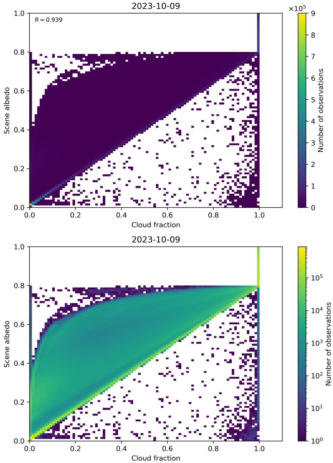
Figure 82: Scatter density plot of “Cloud fraction” against “Scene albedo” for 2023-10-08 to 2023-10-10.
