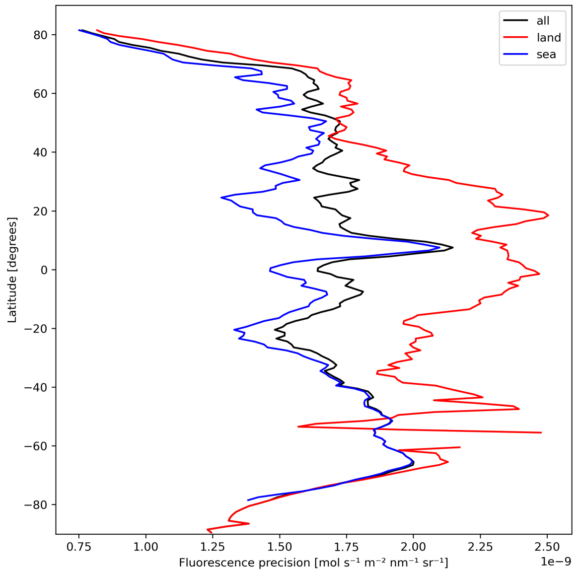
Figure 24: Zonal average of “Fluorescence precision” for 2023-10-08 to 2023-10-10.
