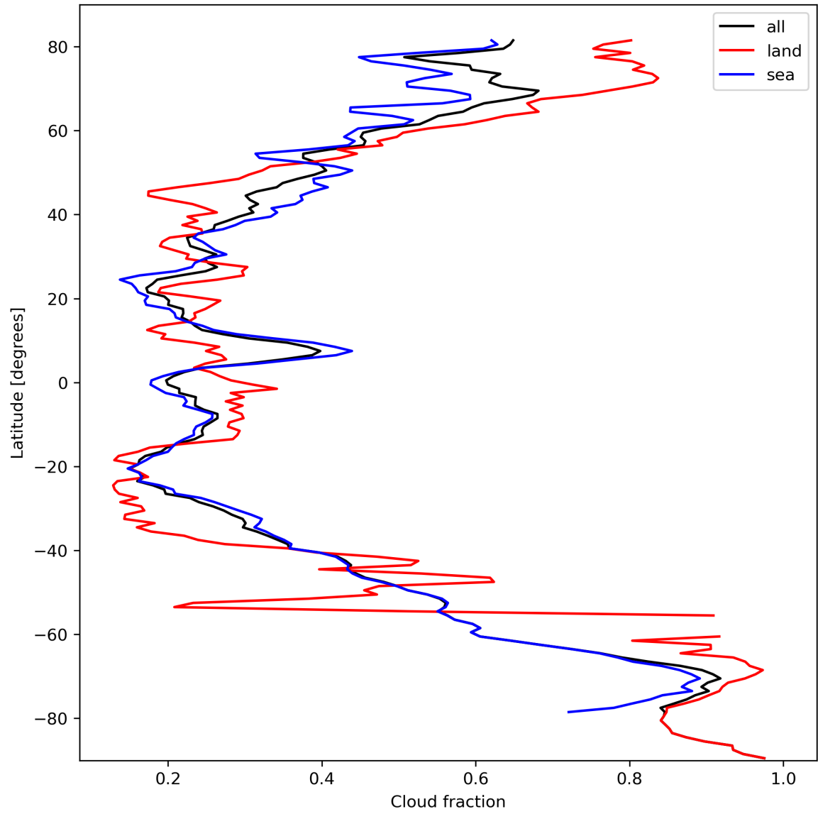
Figure 15: Zonal average of “Cloud fraction” for 2023-10-08 to 2023-10-10.
