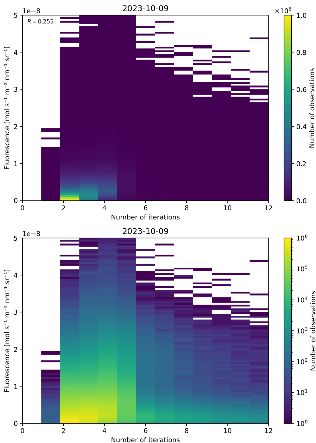
Figure 107: Scatter density plot of “Number of iterations” against “Fluorescence” for 2023-10-08 to 2023-10-10.
