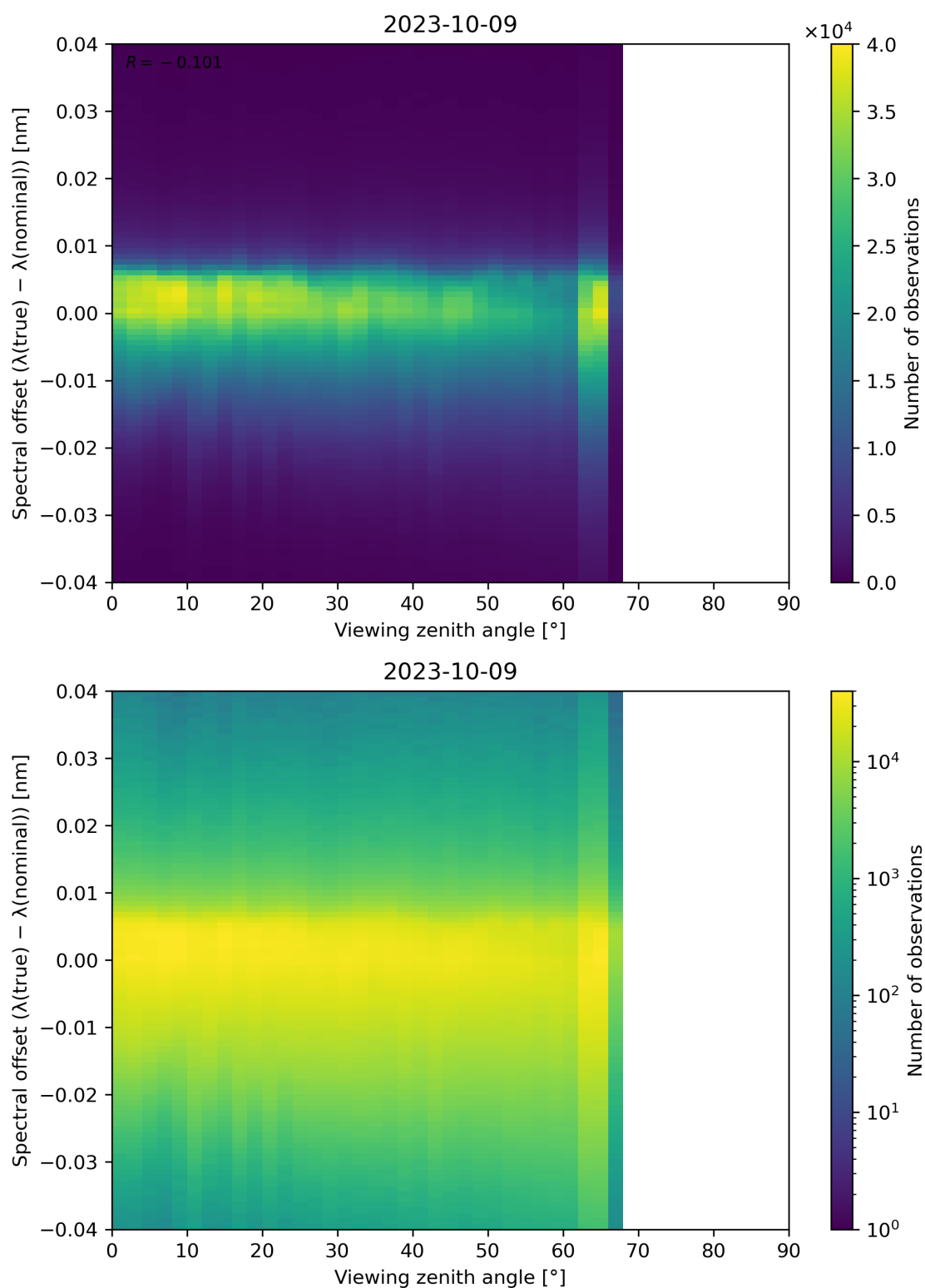
Figure 140: Scatter density plot of “Viewing zenith angle” against “Spectral offset ( \lambda(\text{true}) - \lambda(\text{nominal}) )” for 2023-10-08 to 2023-10-10.
