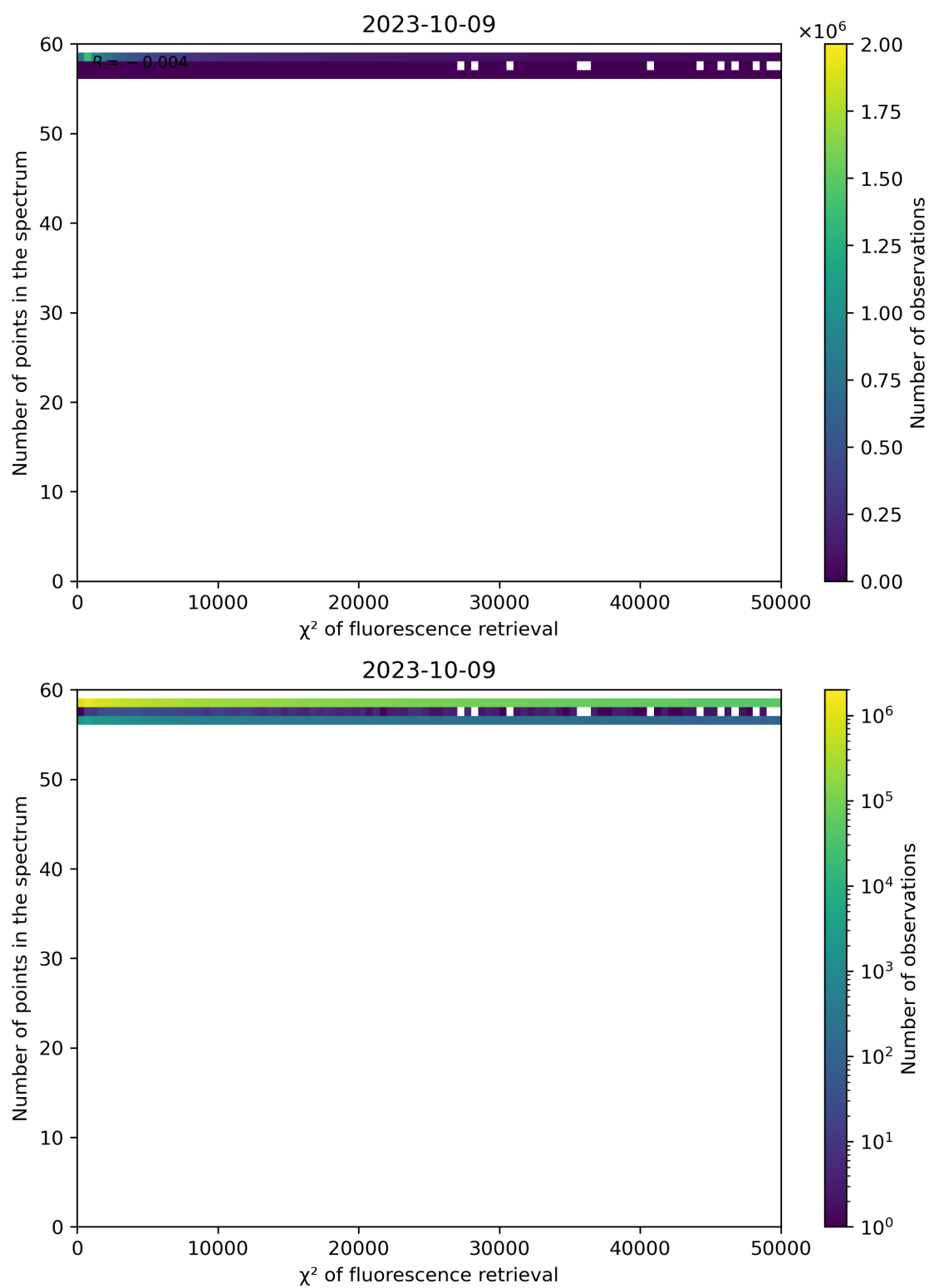
Figure 71: Scatter density plot of " \chi^2 of fluorescence retrieval" against "Number of points in the spectrum" for 2023-10-08 to 2023-10-10.
