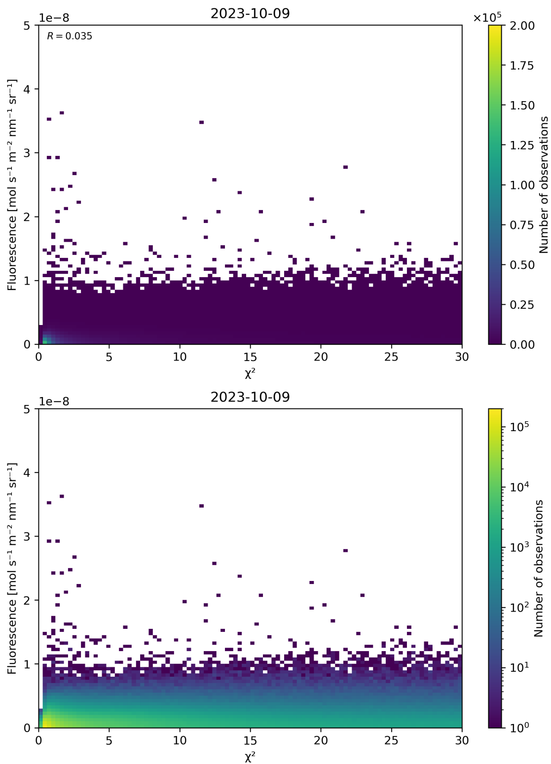
Figure 70: Scatter density plot of “ \chi^2 ” against “Fluorescence” for 2023-10-08 to 2023-10-10.
