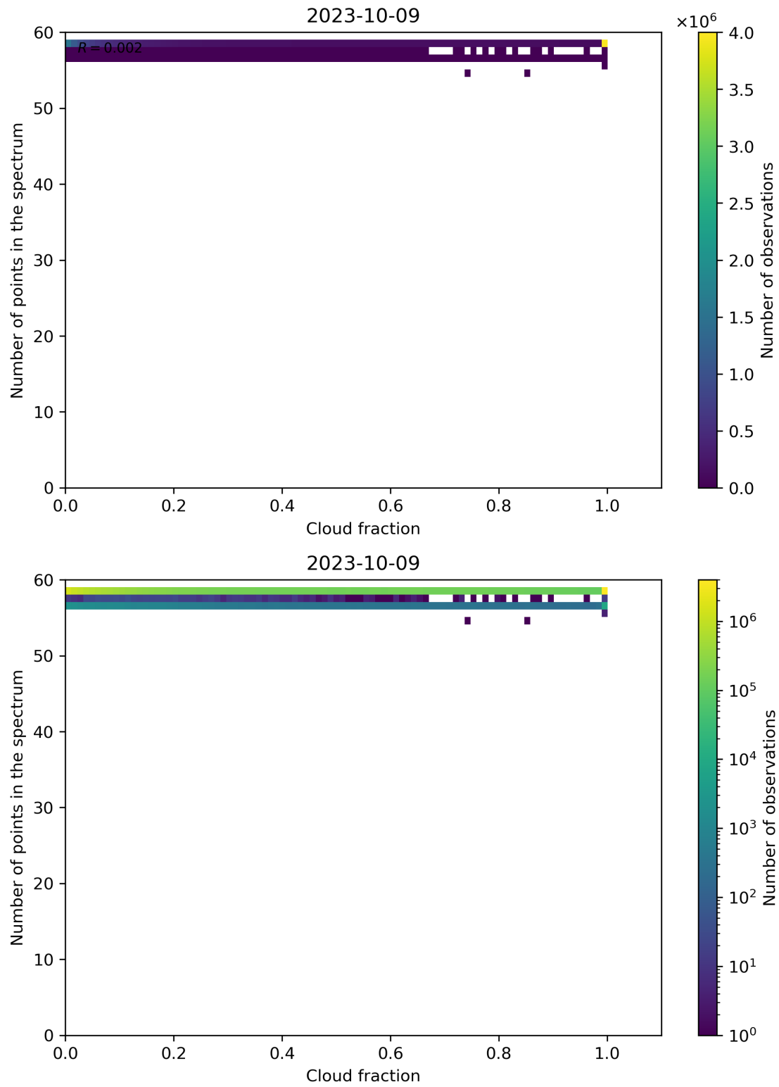
Figure 81: Scatter density plot of “Cloud fraction” against “Number of points in the spectrum” for 2023-10-08 to 2023-10-10.
