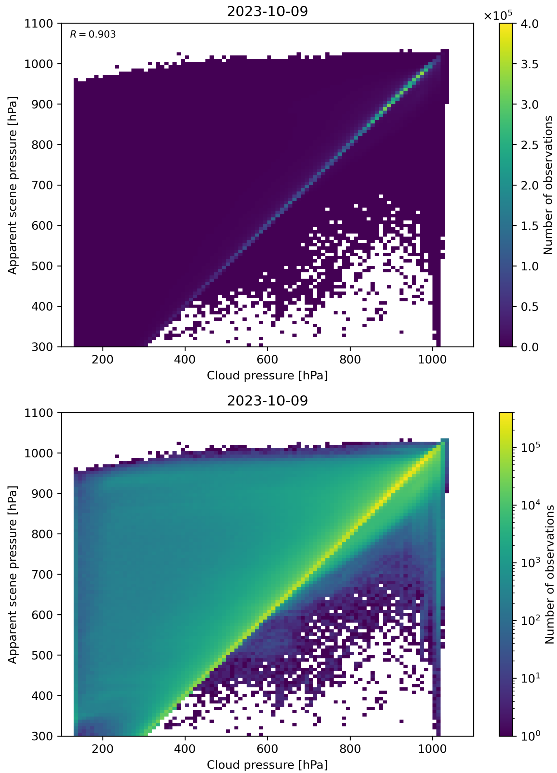
Figure 84: Scatter density plot of “Cloud pressure” against “Apparent scene pressure” for 2023-10-08 to 2023-10-10.
