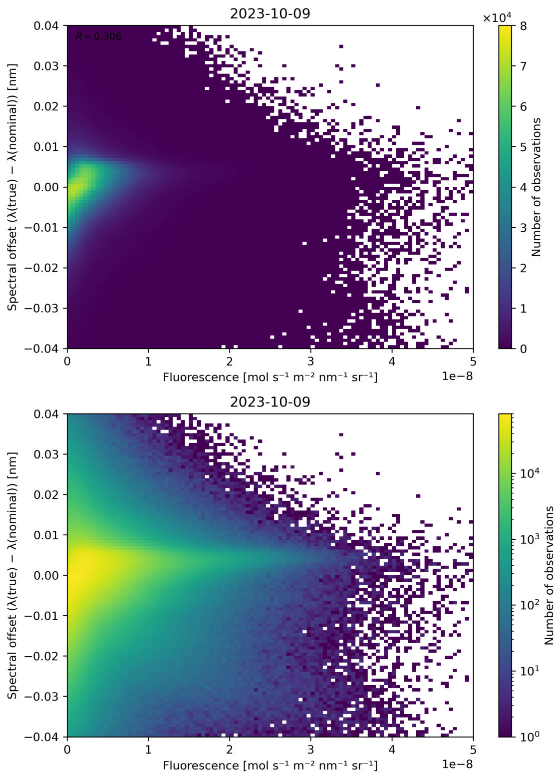
Figure 95: Scatter density plot of “Fluorescence” against “Spectral offset ( \lambda(\text{true}) - \lambda(\text{nominal}) )” for 2023-10-08 to 2023-10-10.
