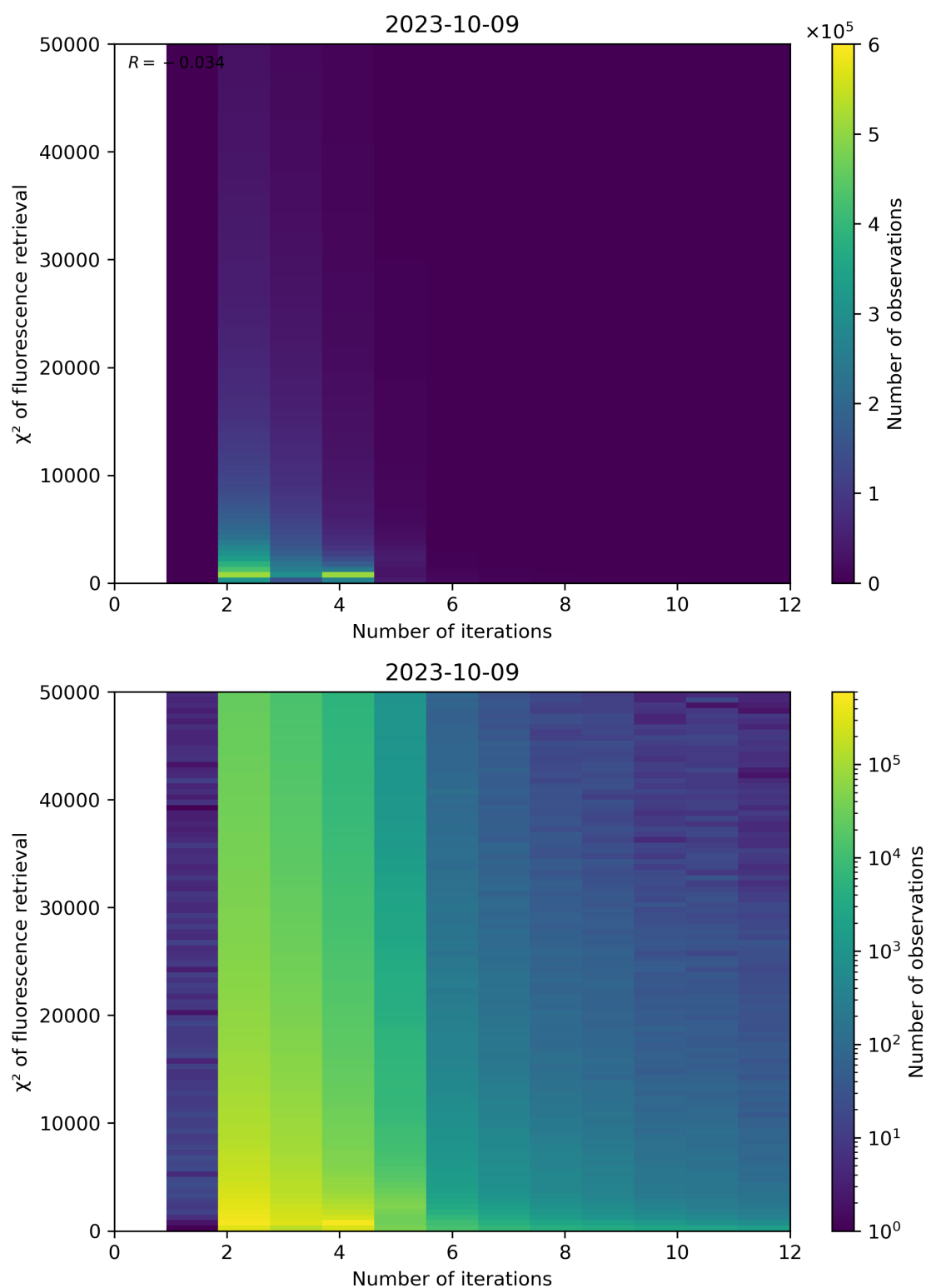
Figure 106: Scatter density plot of “Number of iterations” against “ \chi^2 of fluorescence retrieval” for 2023-10-08 to 2023-10-10.
