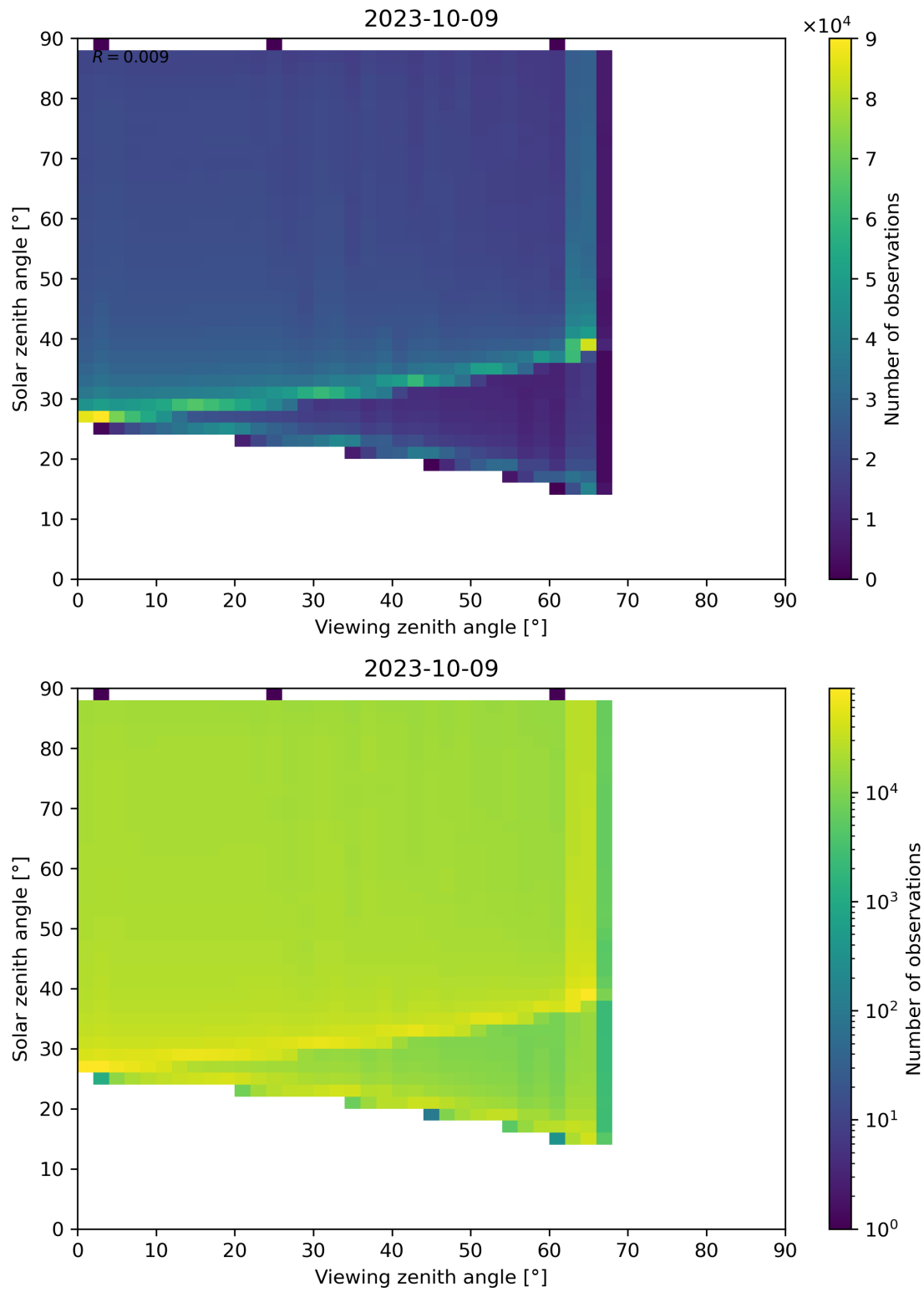
Figure 139: Scatter density plot of “Viewing zenith angle” against “Solar zenith angle” for 2023-10-08 to 2023-10-10.
