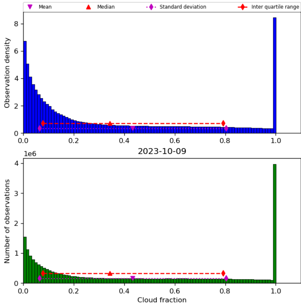
Figure 32: Histogram of “Cloud fraction” for 2023-10-08 to 2023-10-10
