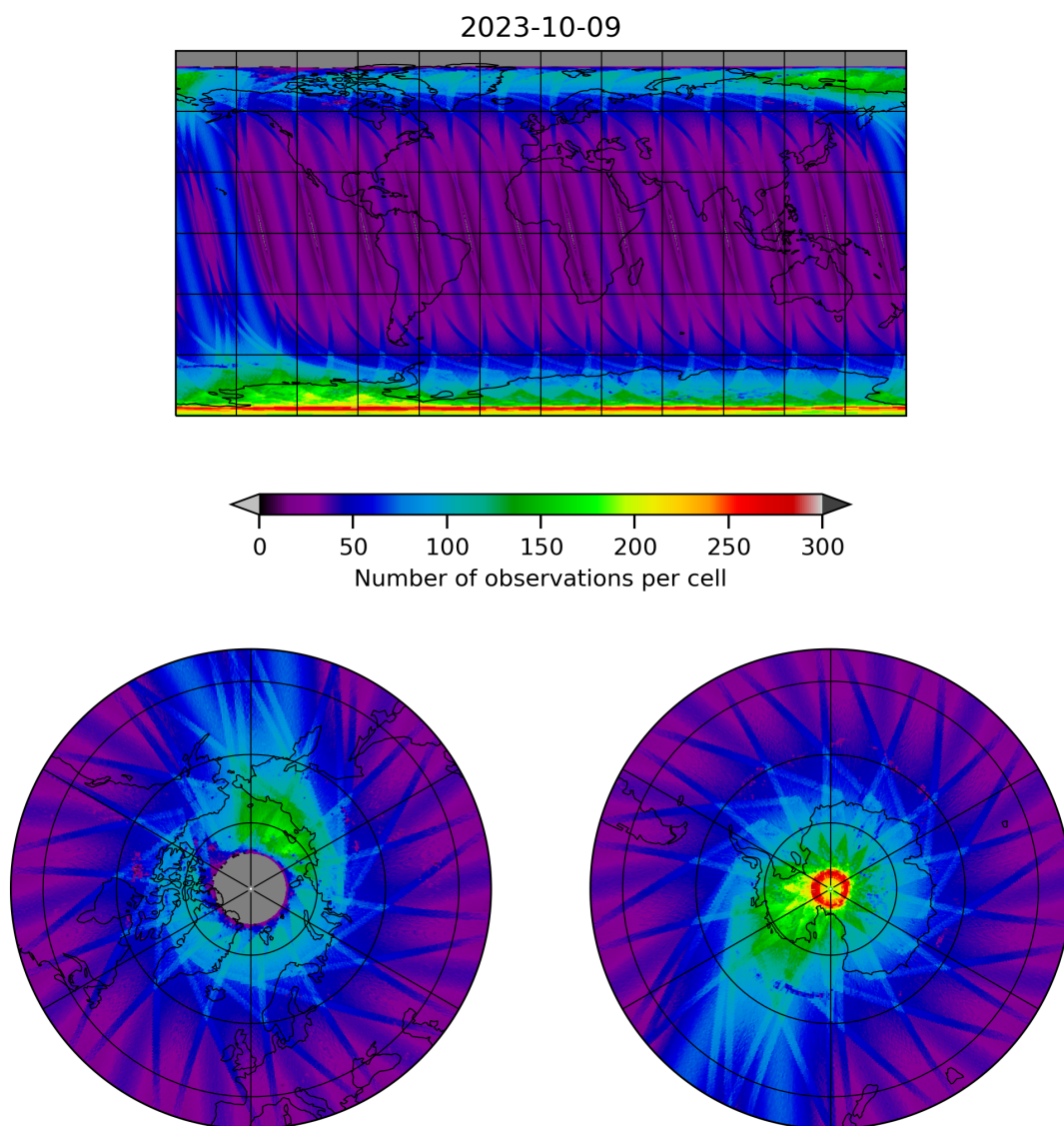
Figure 11: Map of the number of observations for 2023-10-08 to 2023-10-10
