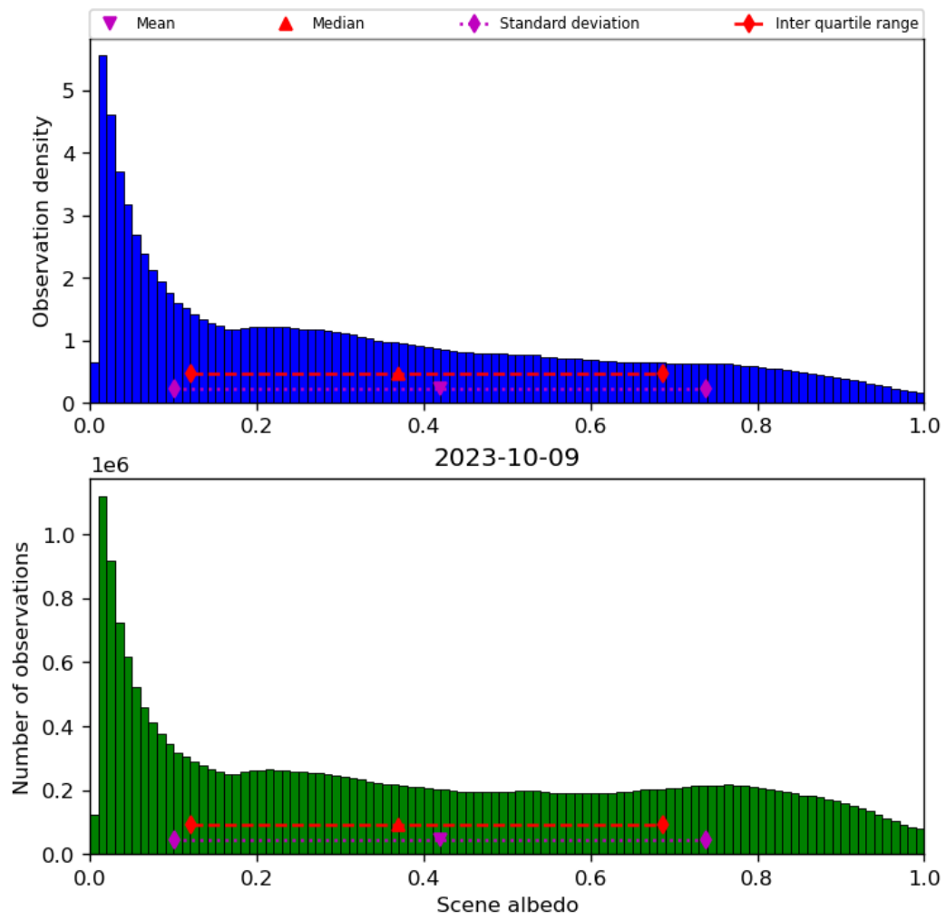
Figure 34: Histogram of “Scene albedo” for 2023-10-08 to 2023-10-10
