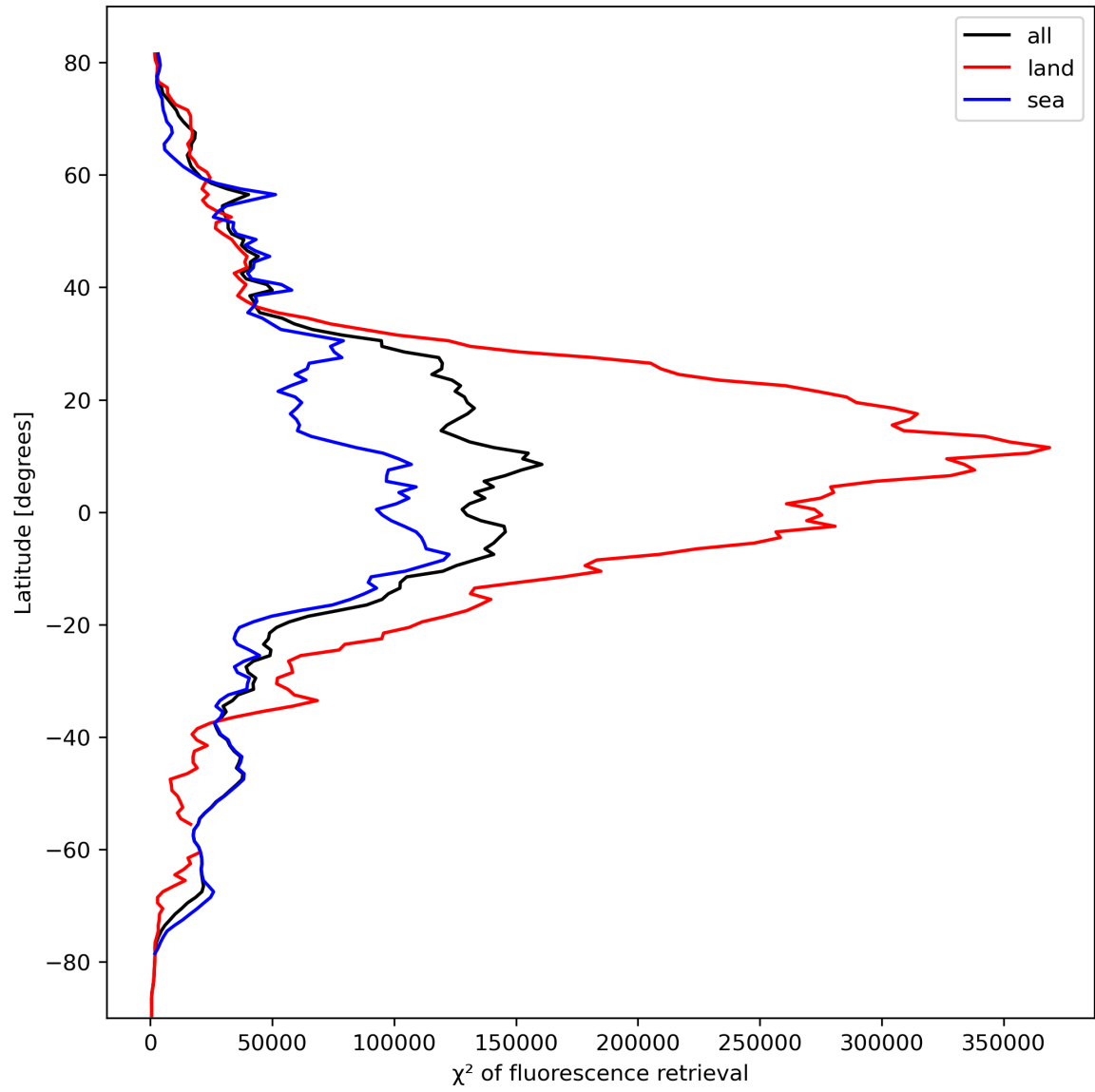
Figure 25: Zonal average of “ \chi^2 of fluorescence retrieval” for 2023-10-08 to 2023-10-10.
