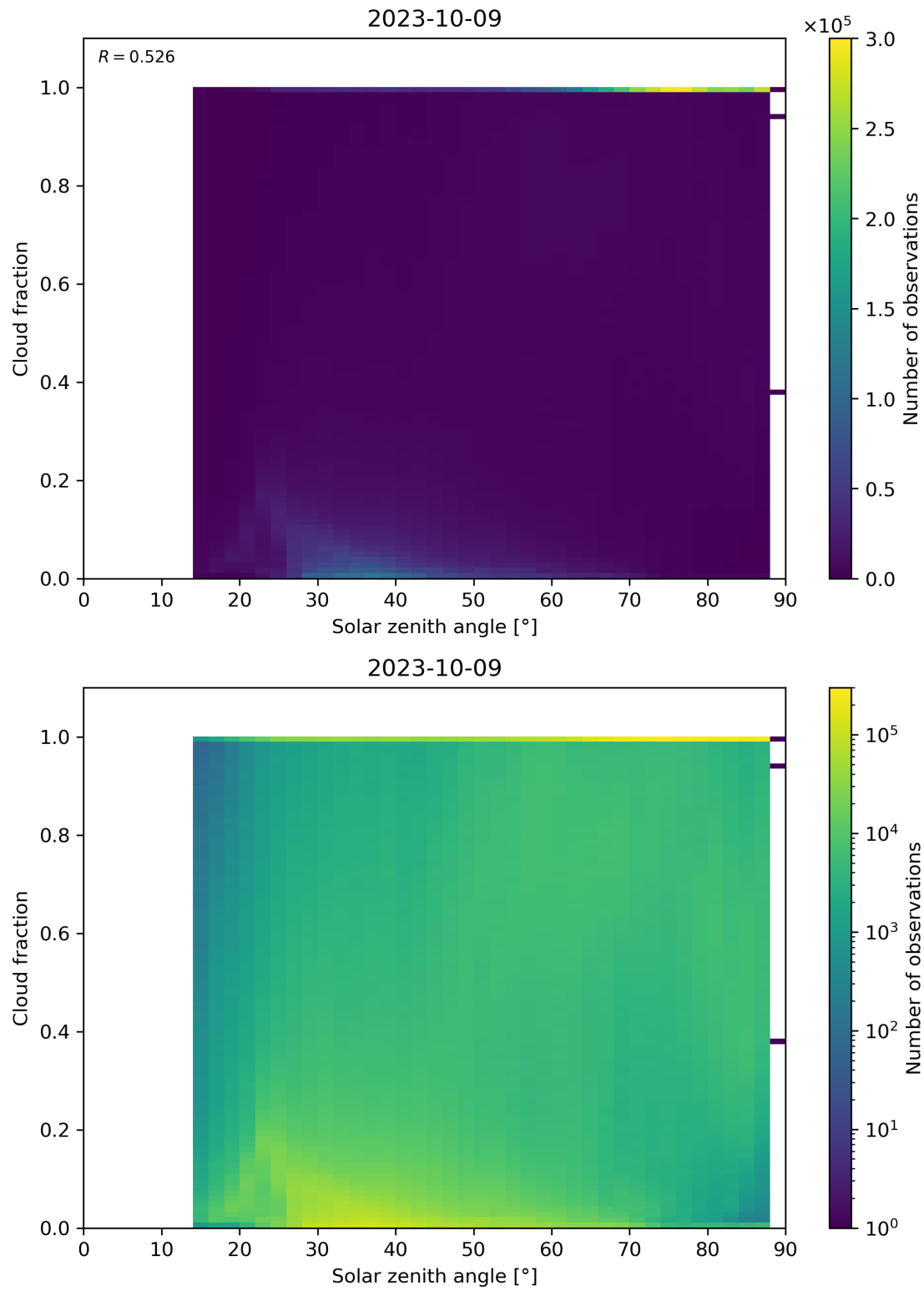
Figure 121: Scatter density plot of “Solar zenith angle” against “Cloud fraction” for 2023-10-08 to 2023-10-10.
