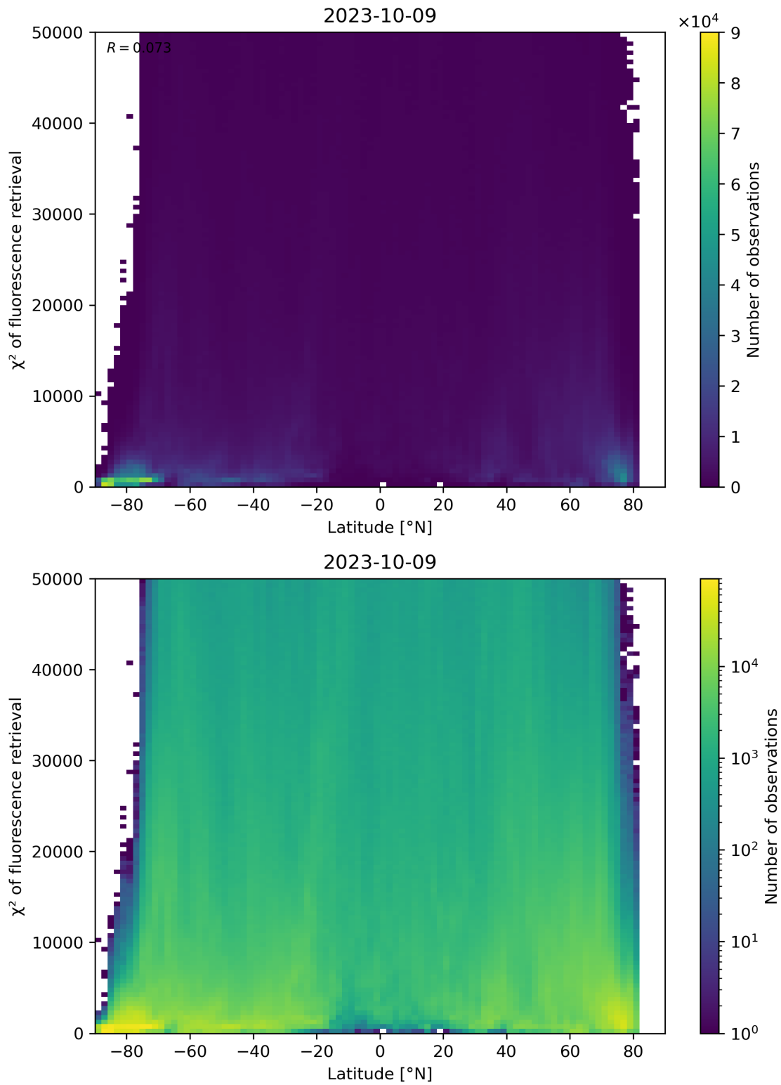
Figure 98: Scatter density plot of “Latitude” against “ \chi^2 of fluorescence retrieval” for 2023-10-08 to 2023-10-10.
