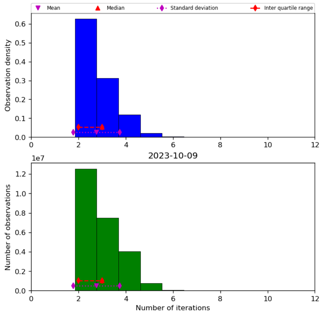
Figure 39: Histogram of “Number of iterations” for 2023-10-08 to 2023-10-10
