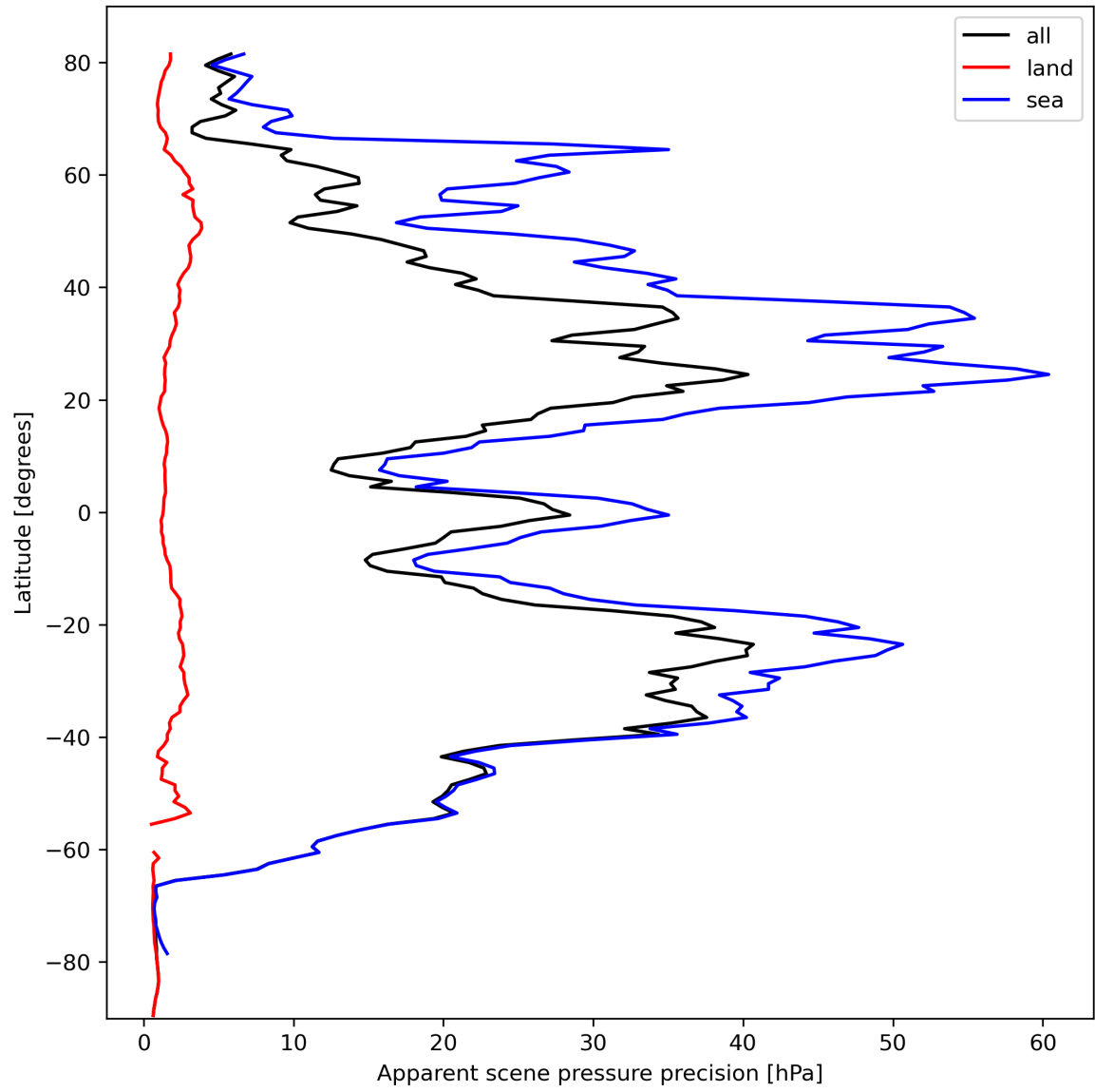
Figure 20: Zonal average of “Apparent scene pressure precision” for 2023-10-08 to 2023-10-10.
