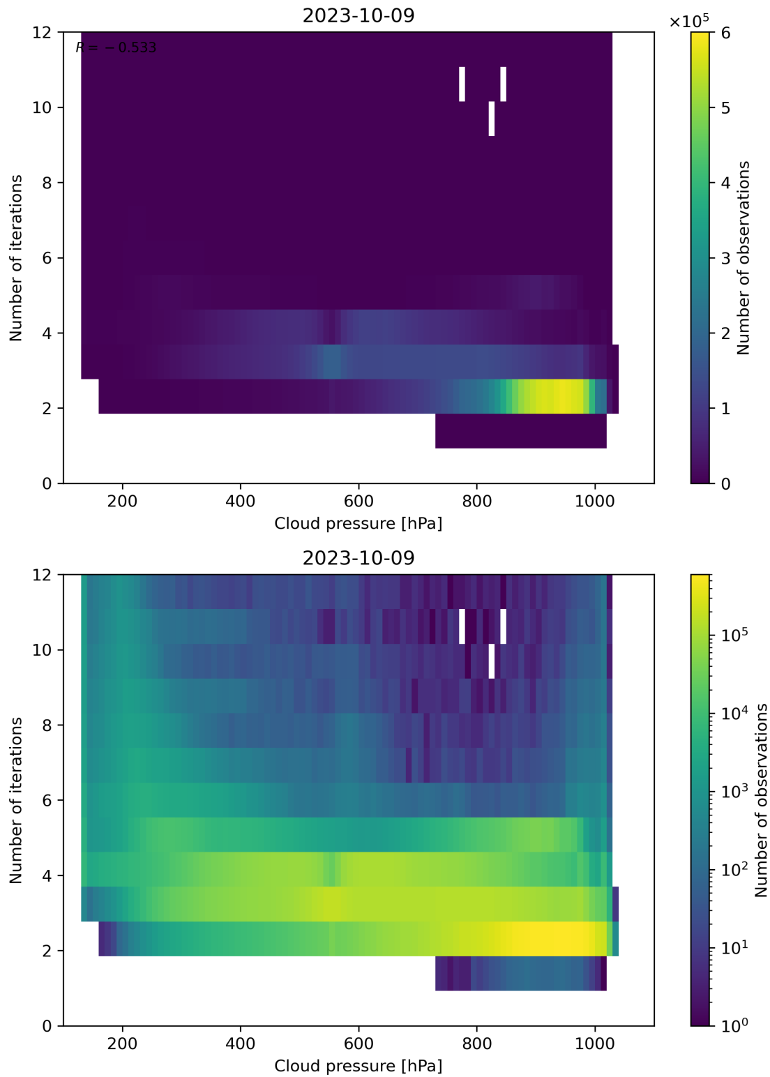
Figure 89: Scatter density plot of “Cloud pressure” against “Number of iterations” for 2023-10-08 to 2023-10-10.
