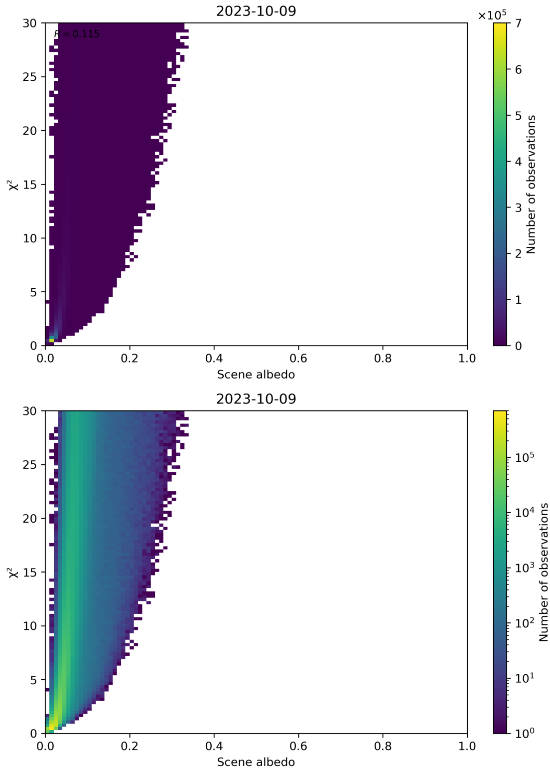
Figure 112: Scatter density plot of “Scene albedo” against “ \chi^2 ” for 2023-10-08 to 2023-10-10.
