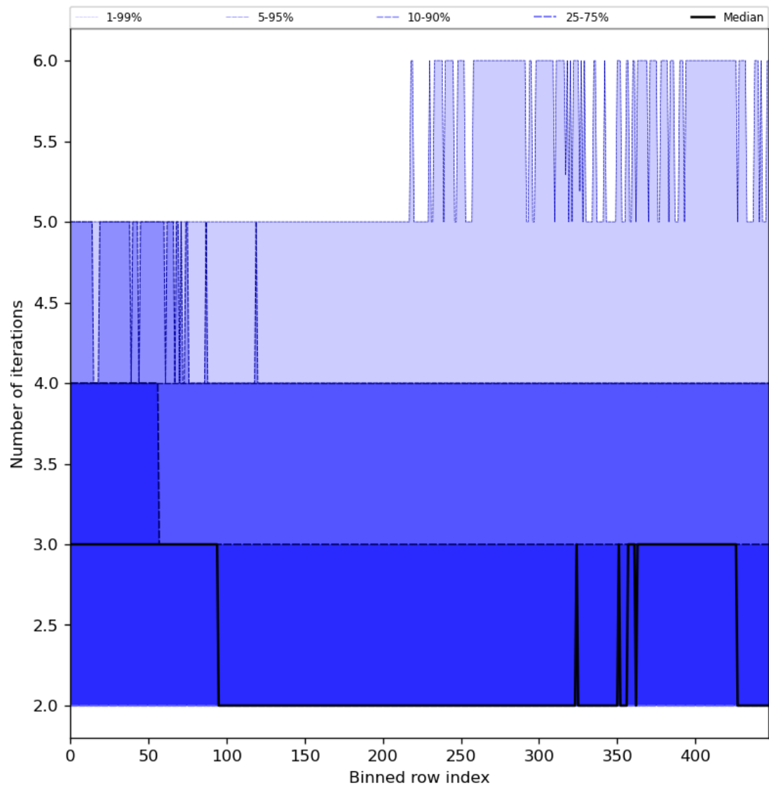
Figure 56: Along track statistics of “Number of iterations” for 2023-10-08 to 2023-10-10
