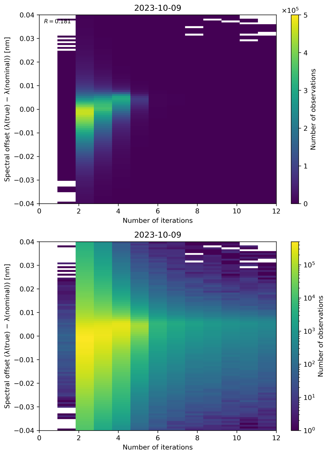
Figure 109: Scatter density plot of “Number of iterations” against “Spectral offset ( \lambda(\text{true}) - \lambda(\text{nominal}) )” for 2023-10-08 to 2023-10-10.
