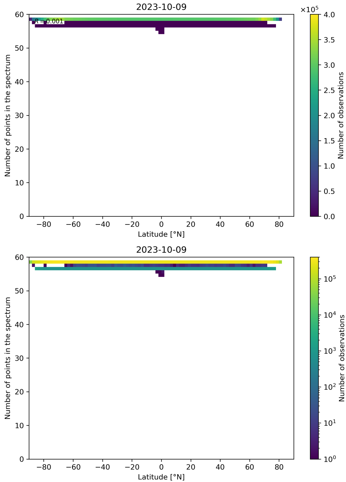
Figure 103: Scatter density plot of “Latitude” against “Number of points in the spectrum” for 2023-10-08 to 2023-10-10.
