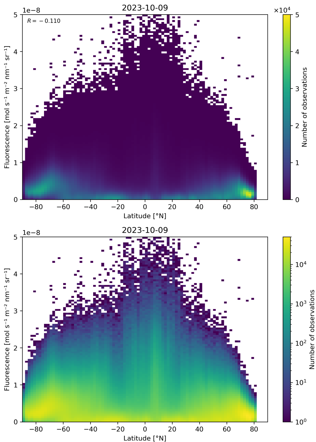
Figure 101: Scatter density plot of “Latitude” against “Fluorescence” for 2023-10-08 to 2023-10-10.
