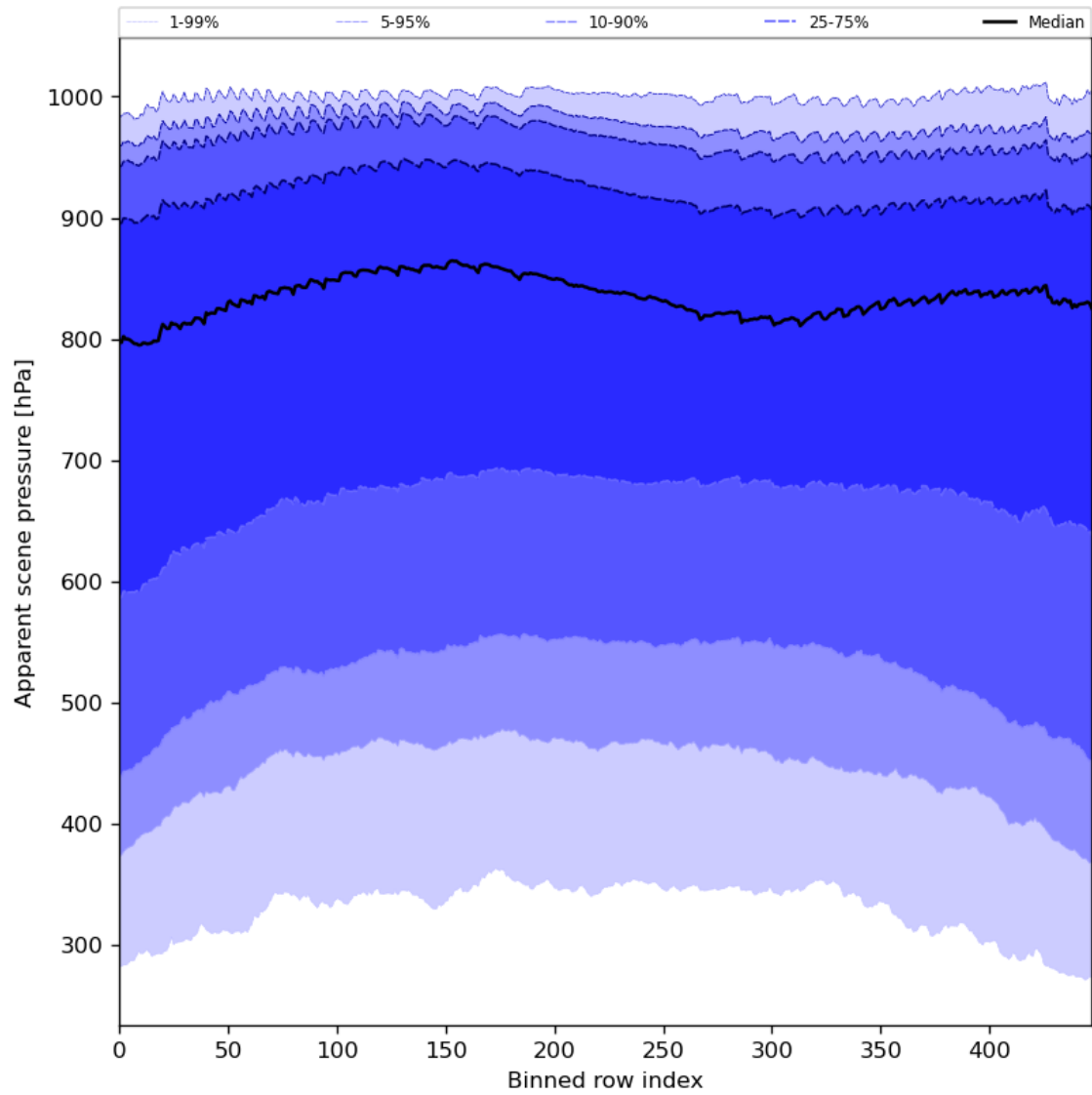
Figure 53: Along track statistics of “Apparent scene pressure” for 2023-10-08 to 2023-10-10
