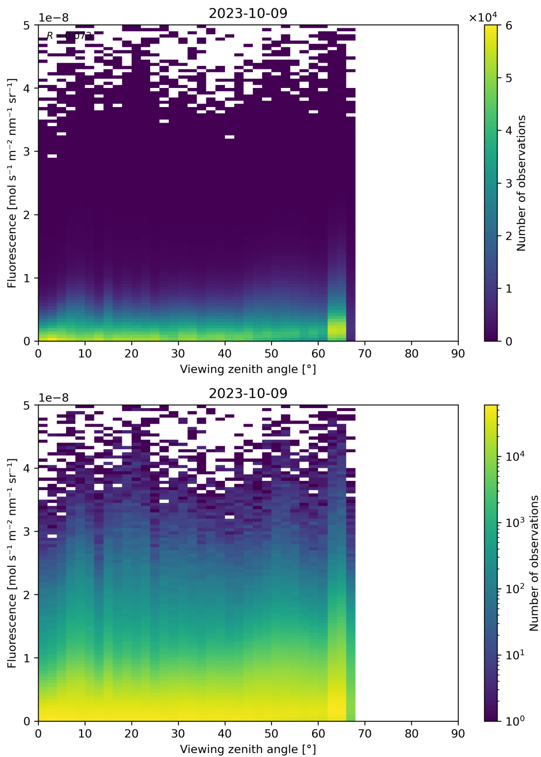
Figure 134: Scatter density plot of “Viewing zenith angle” against “Fluorescence” for 2023-10-08 to 2023-10-10.
