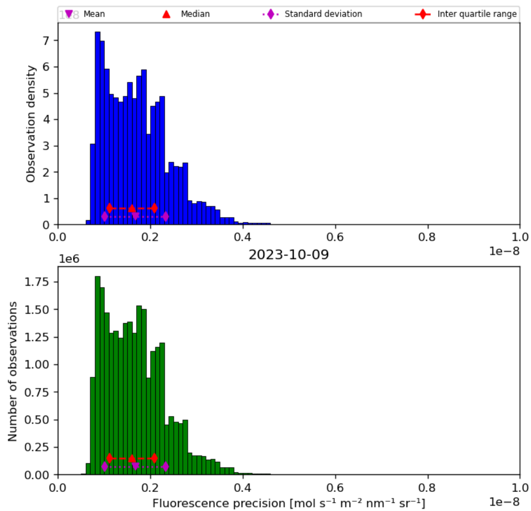
Figure 41: Histogram of “Fluorescence precision” for 2023-10-08 to 2023-10-10
