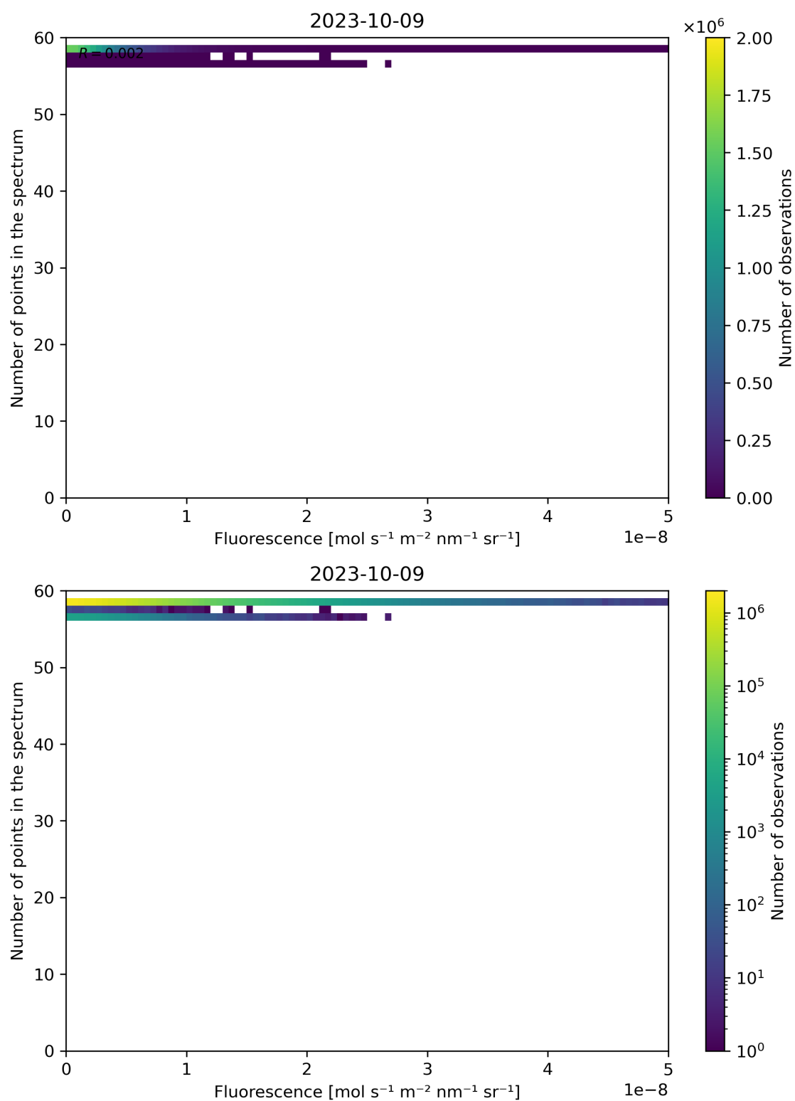
Figure 94: Scatter density plot of “Fluorescence” against “Number of points in the spectrum” for 2023-10-08 to 2023-10-10.
