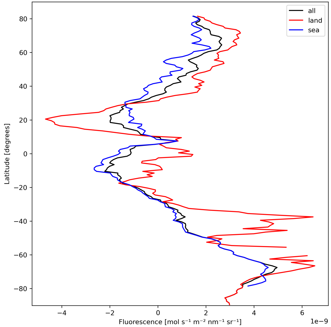
Figure 23: Zonal average of “Fluorescence” for 2023-10-08 to 2023-10-10.
