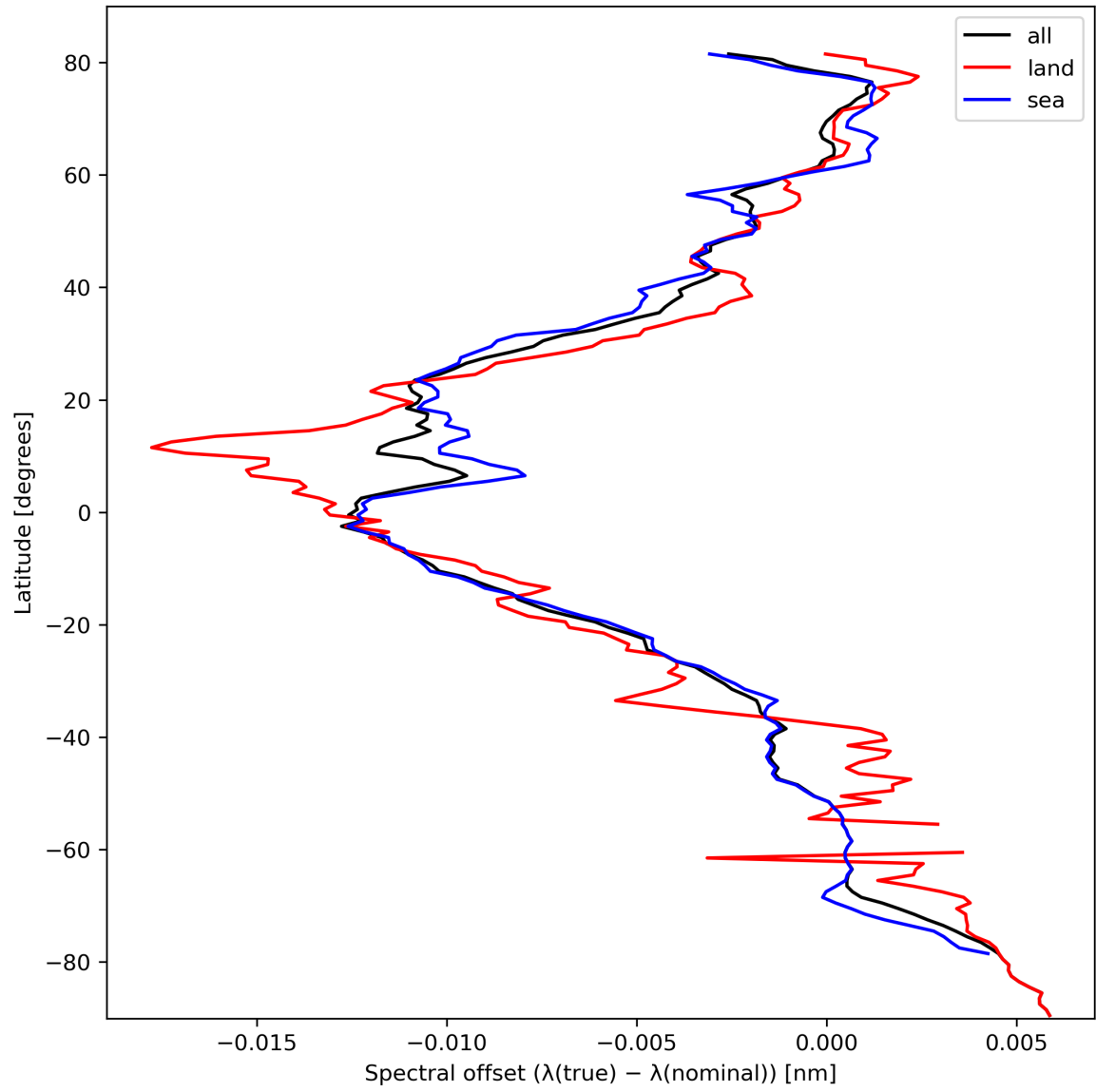
Figure 28: Zonal average of “Spectral offset ( \lambda(\text{true}) - \lambda(\text{nominal}) )” for 2023-10-08 to 2023-10-10.
