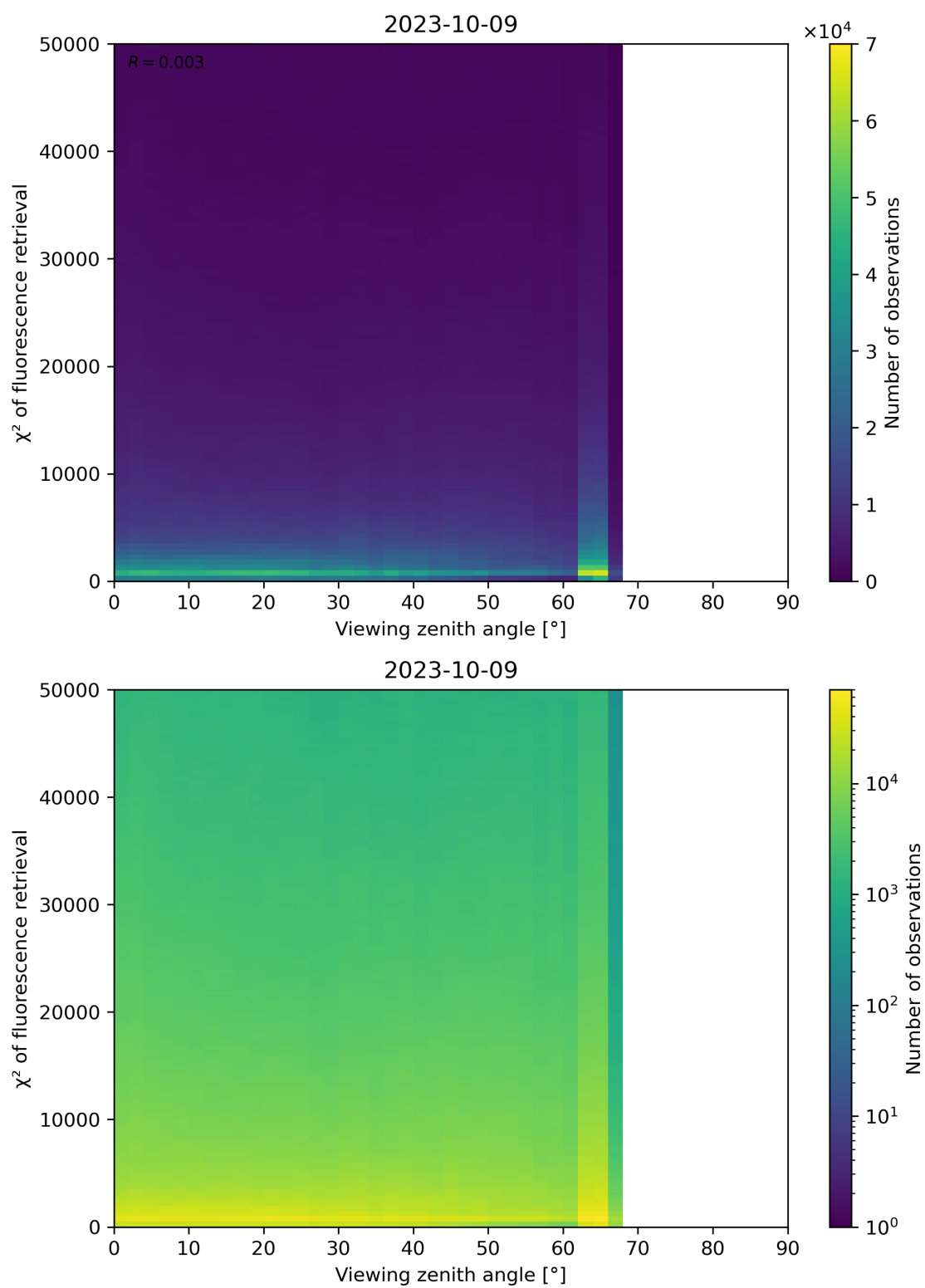
Figure 131: Scatter density plot of “Viewing zenith angle” against “ \chi^2 of fluorescence retrieval” for 2023-10-08 to 2023-10-10.
