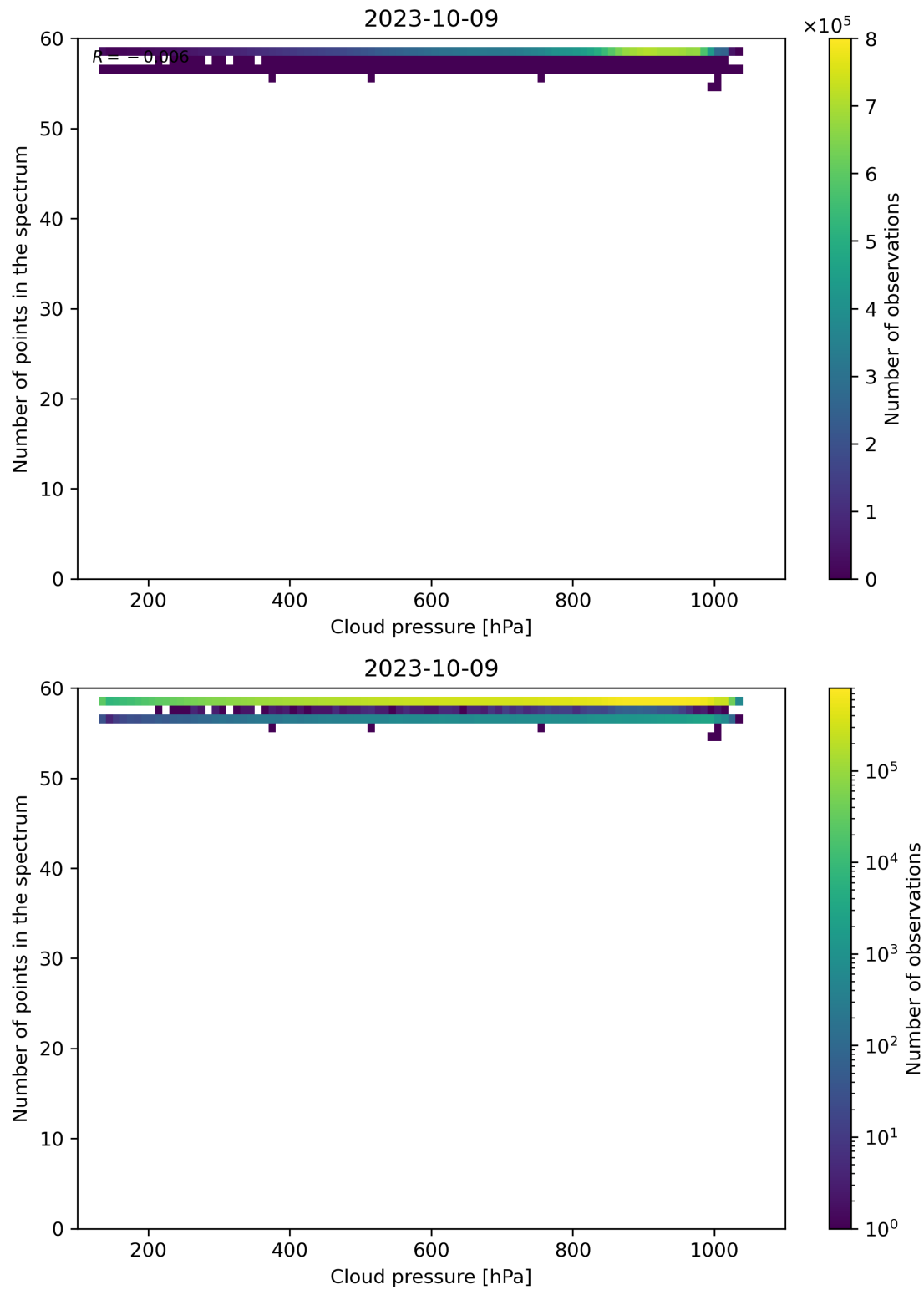
Figure 90: Scatter density plot of “Cloud pressure” against “Number of points in the spectrum” for 2023-10-08 to 2023-10-10.
