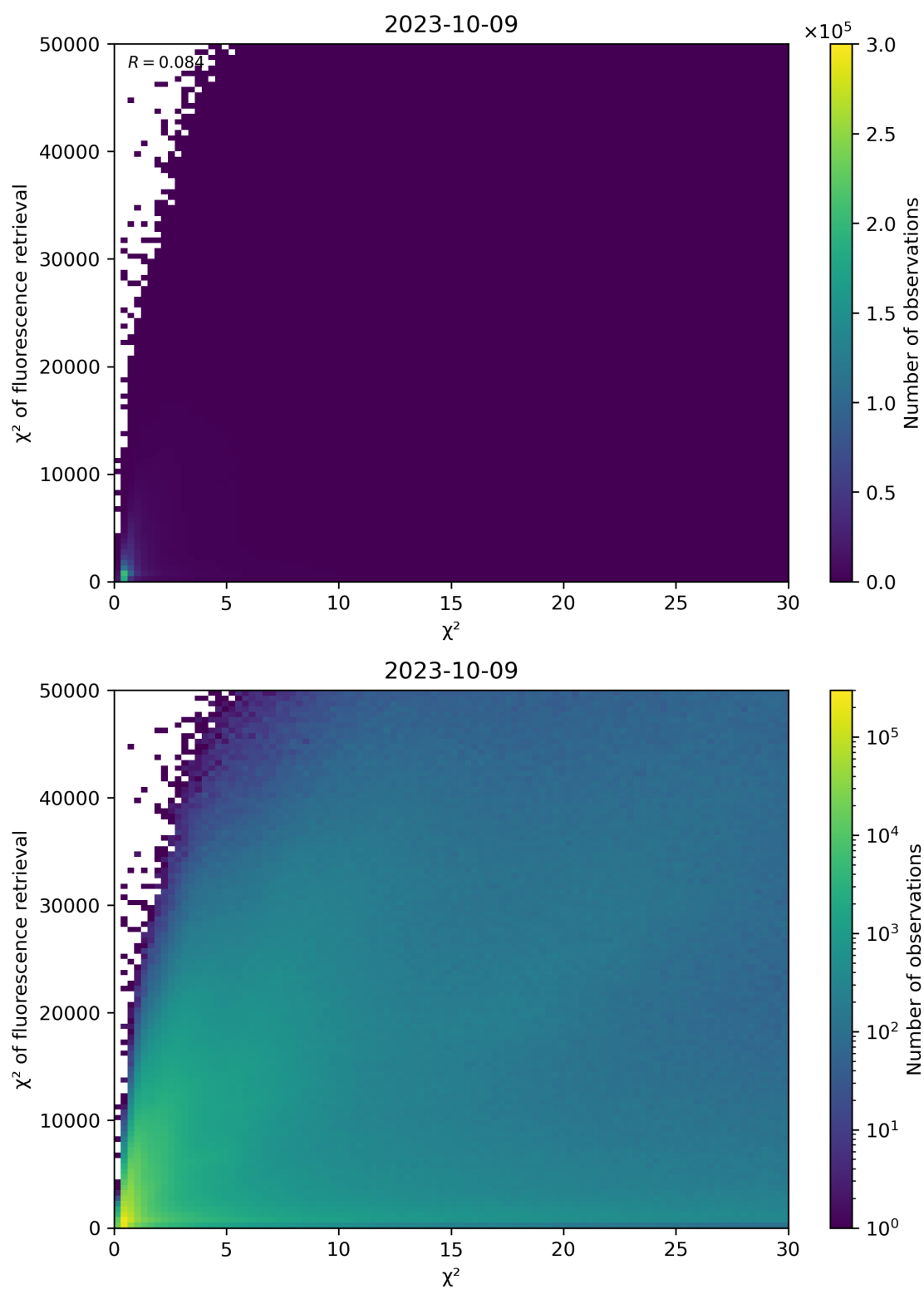
Figure 69: Scatter density plot of “ \chi^2 ” against “ \chi^2 of fluorescence retrieval” for 2023-10-08 to 2023-10-10.
