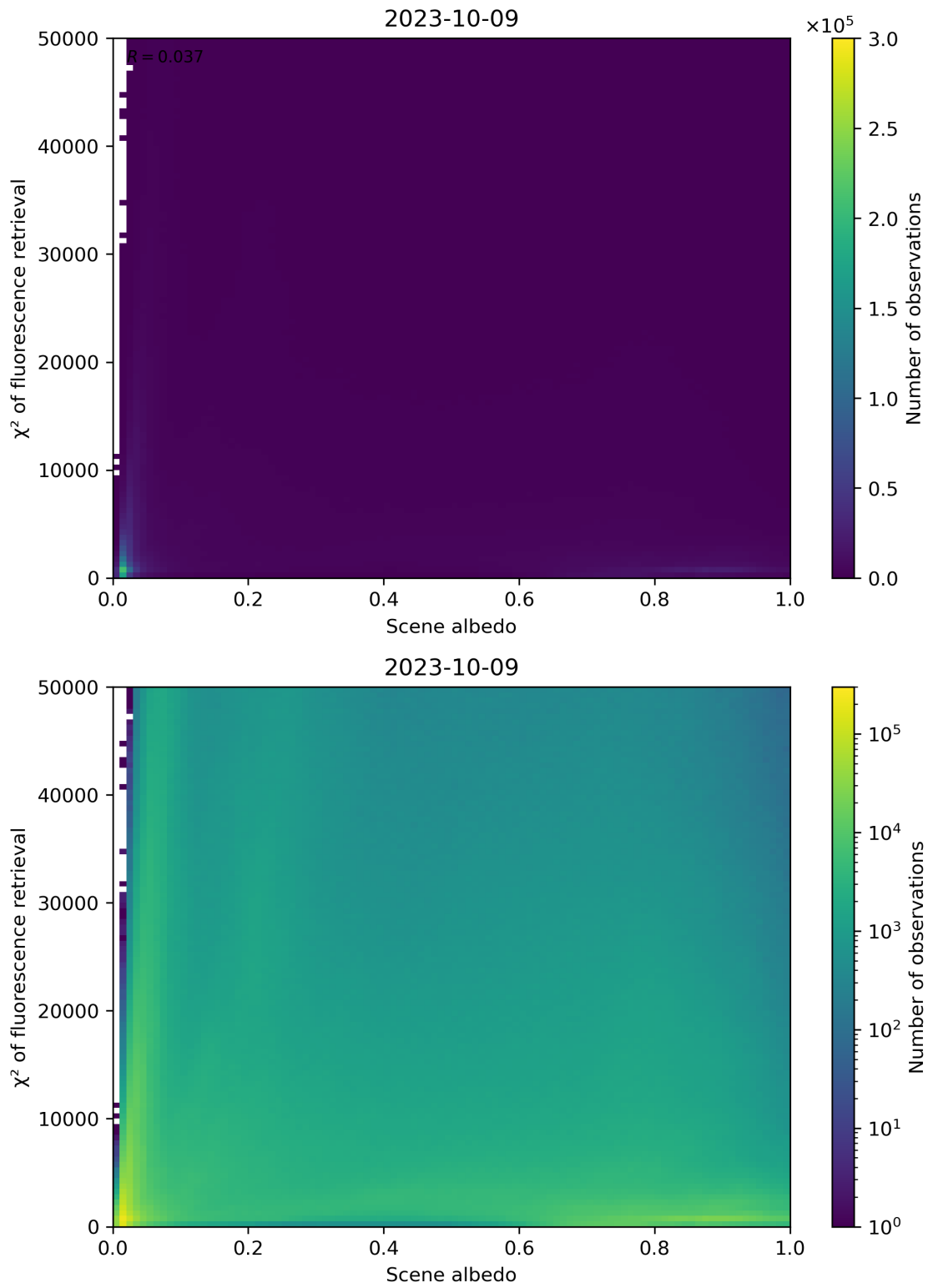
Figure 113: Scatter density plot of “Scene albedo” against “ \chi^2 of fluorescence retrieval” for 2023-10-08 to 2023-10-10.
