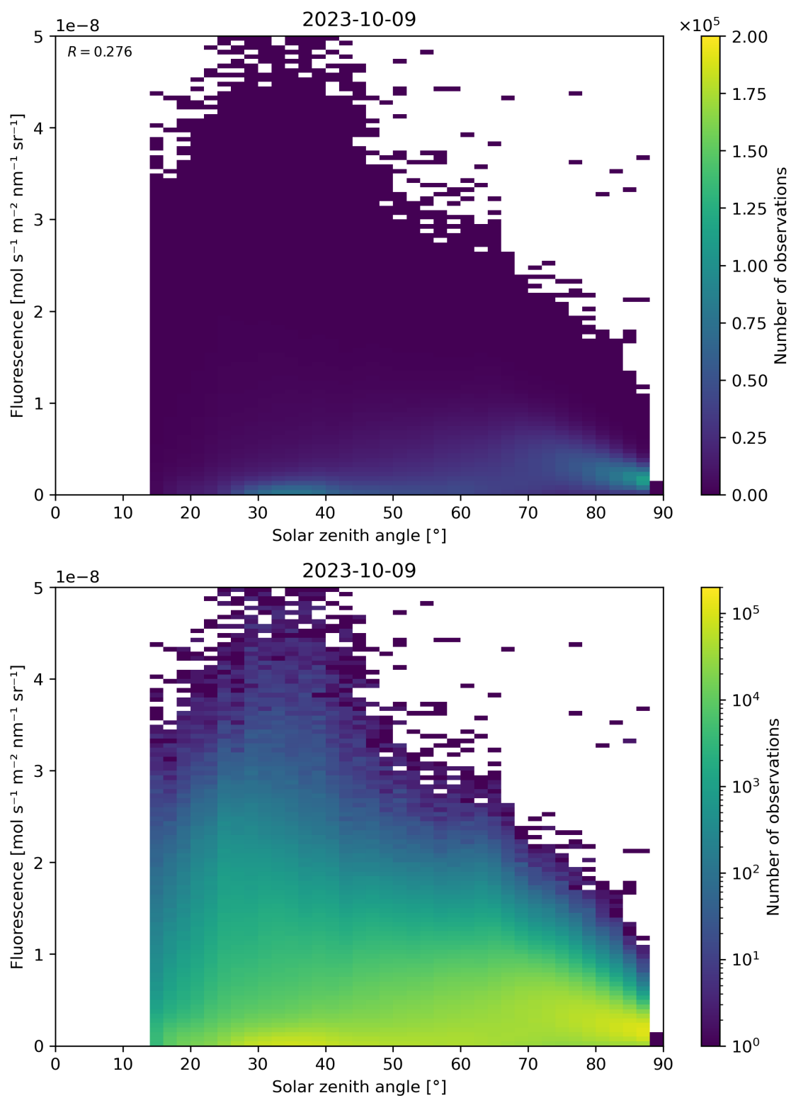
Figure 123: Scatter density plot of “Solar zenith angle” against “Fluorescence” for 2023-10-08 to 2023-10-10.
