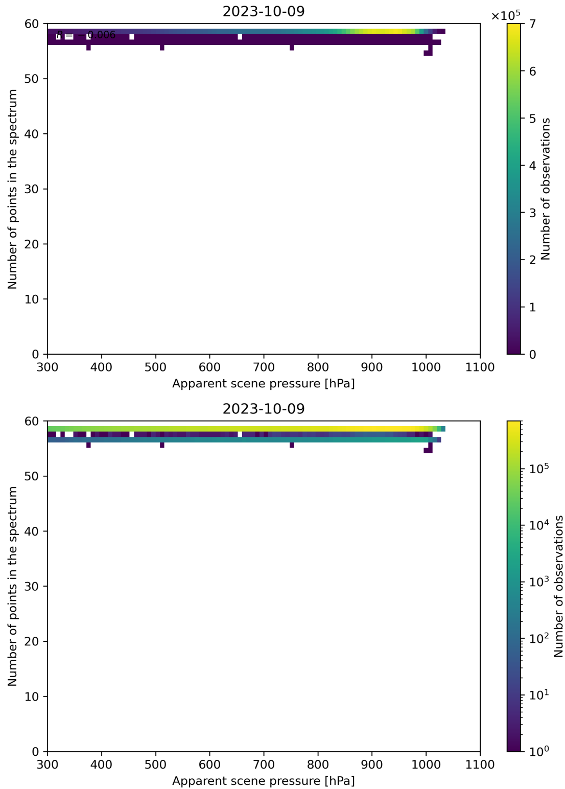
Figure 67: Scatter density plot of “Apparent scene pressure” against “Number of points in the spectrum” for 2023-10-08 to 2023-10-10.
