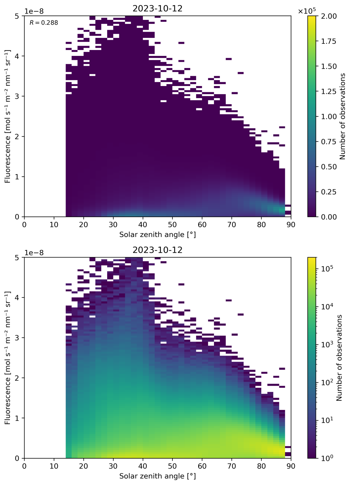
Figure 123: Scatter density plot of “Solar zenith angle” against “Fluorescence” for 2023-10-12 to 2023-10-13.
