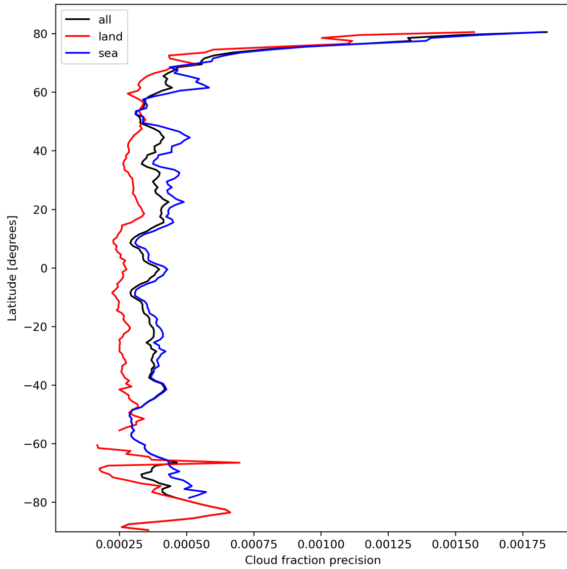
Figure 16: Zonal average of “Cloud fraction precision” for 2023-10-12 to 2023-10-13.
