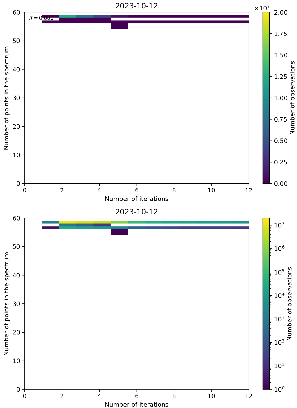
Figure 108: Scatter density plot of “Number of iterations” against “Number of points in the spectrum” for 2023-10-12 to 2023-10-13.
