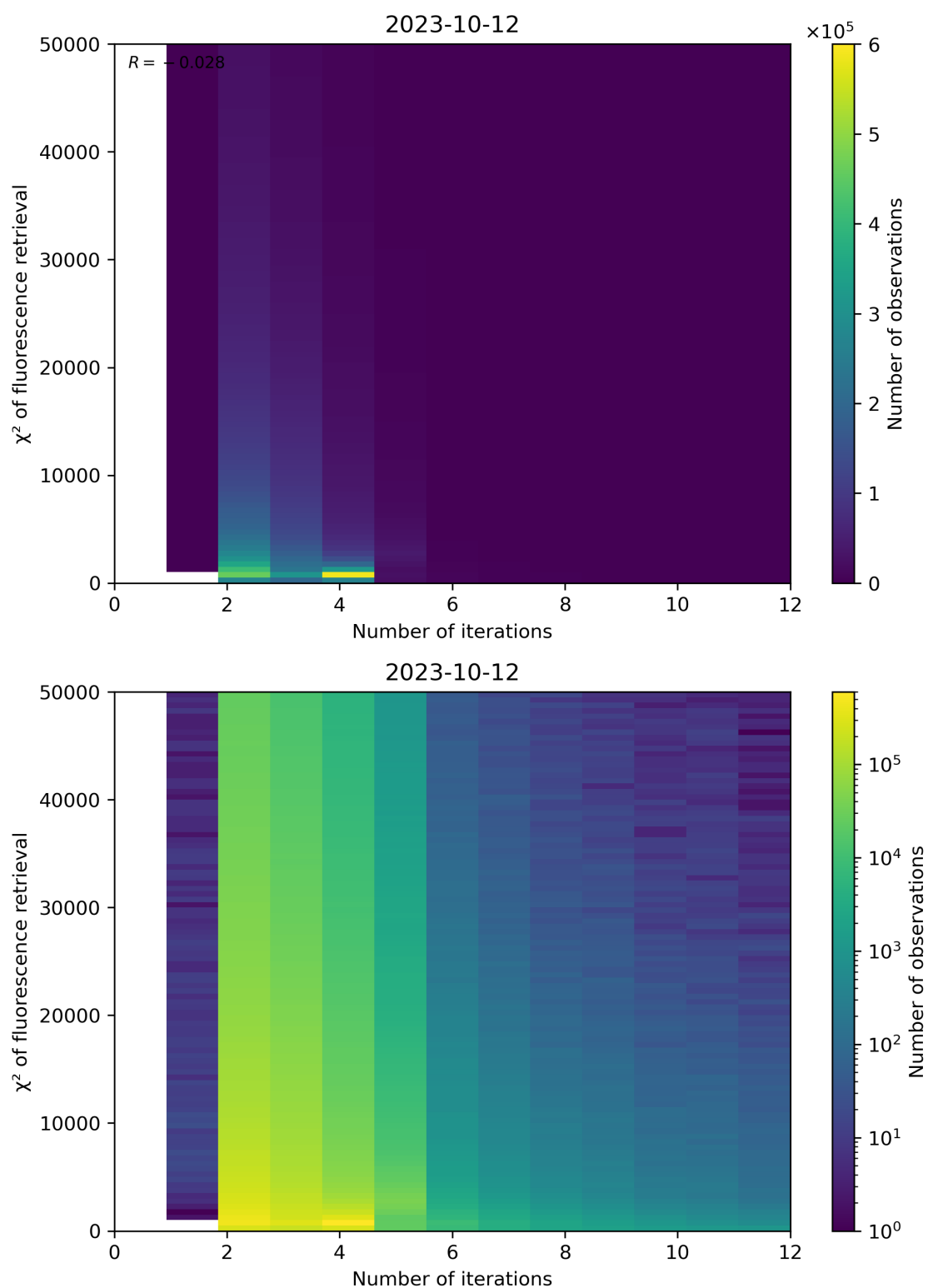
Figure 106: Scatter density plot of “Number of iterations” against “ \chi^2 of fluorescence retrieval” for 2023-10-12 to 2023-10-13.
