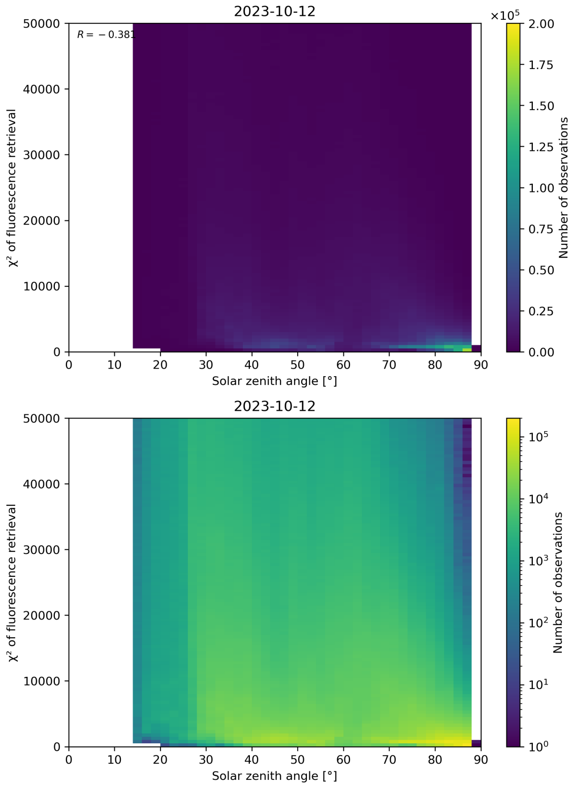
Figure 120: Scatter density plot of “Solar zenith angle” against “ \chi^2 of fluorescence retrieval” for 2023-10-12 to 2023-10-13.
