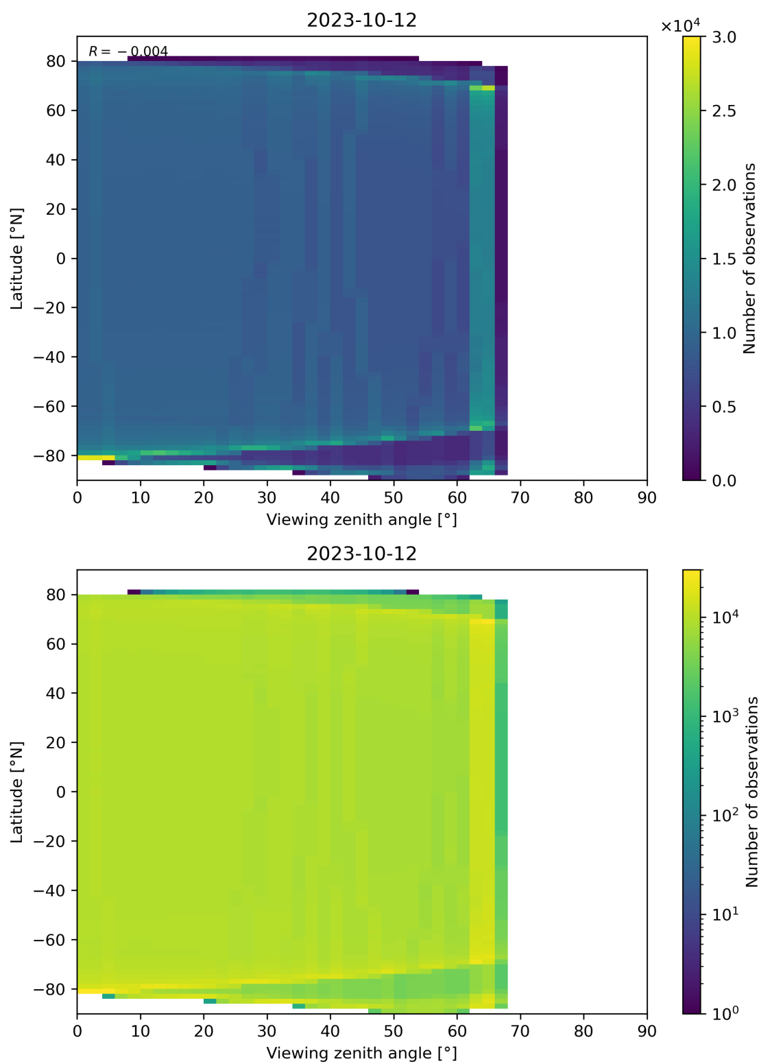
Figure 135: Scatter density plot of “Viewing zenith angle” against “Latitude” for 2023-10-12 to 2023-10-13.
