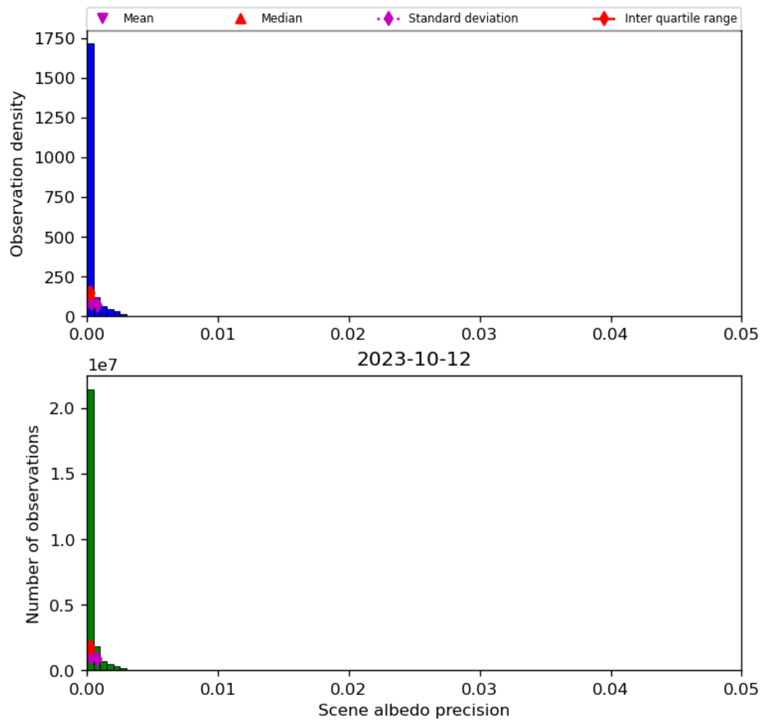
Figure 35: Histogram of “Scene albedo precision” for 2023-10-12 to 2023-10-13
