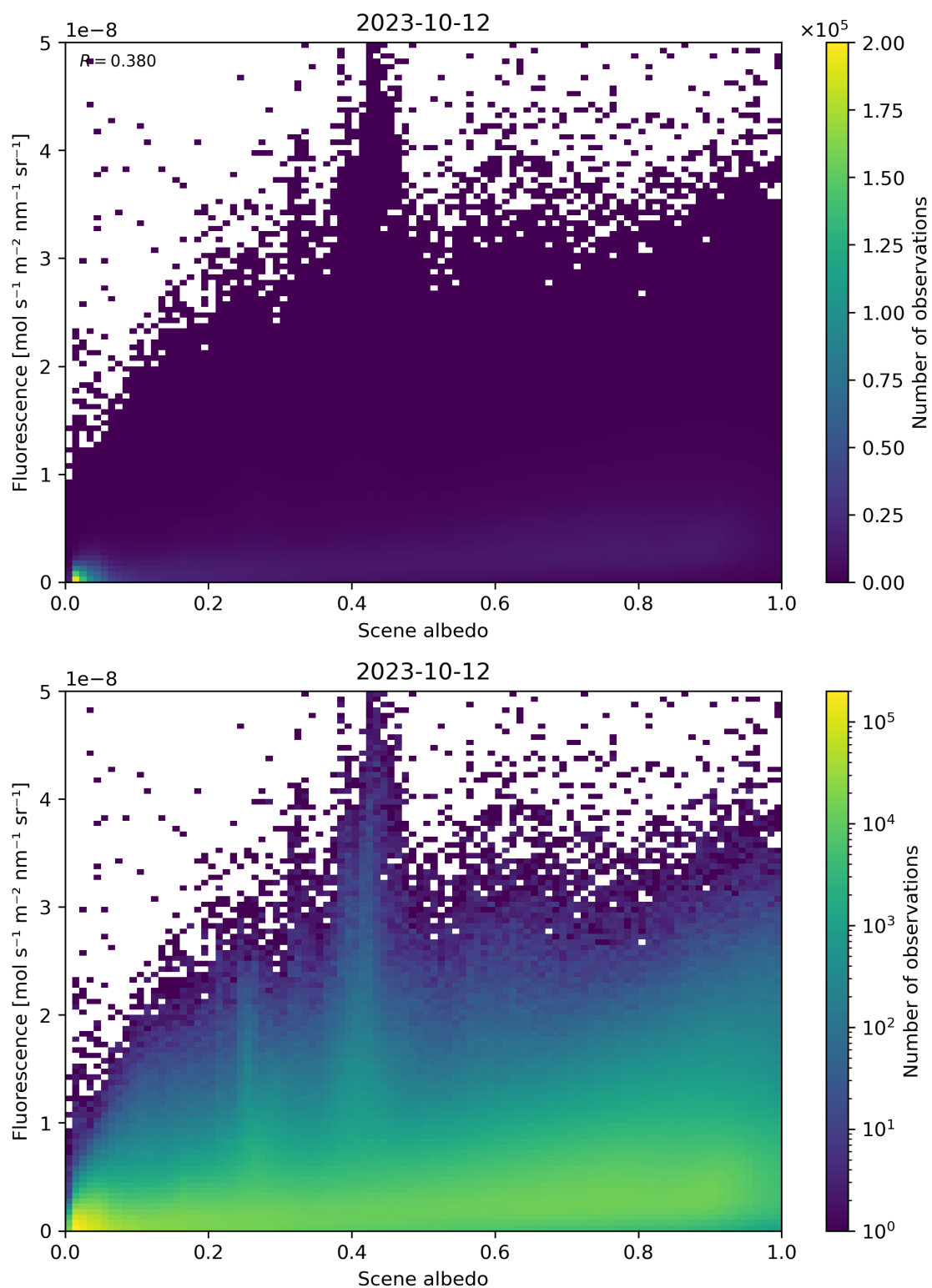
Figure 114: Scatter density plot of “Scene albedo” against “Fluorescence” for 2023-10-12 to 2023-10-13.
