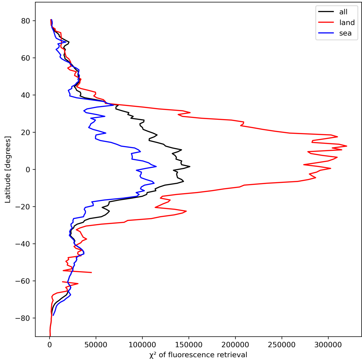
Figure 25: Zonal average of “ \chi^2 of fluorescence retrieval” for 2023-10-12 to 2023-10-13.
