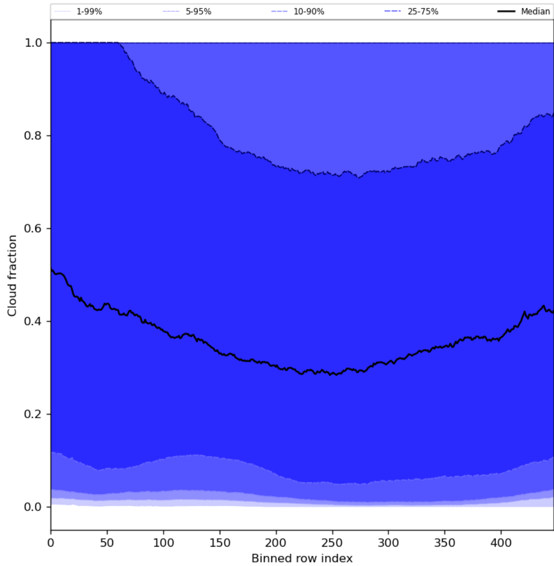
Figure 49: Along track statistics of “Cloud fraction” for 2023-10-12 to 2023-10-13
