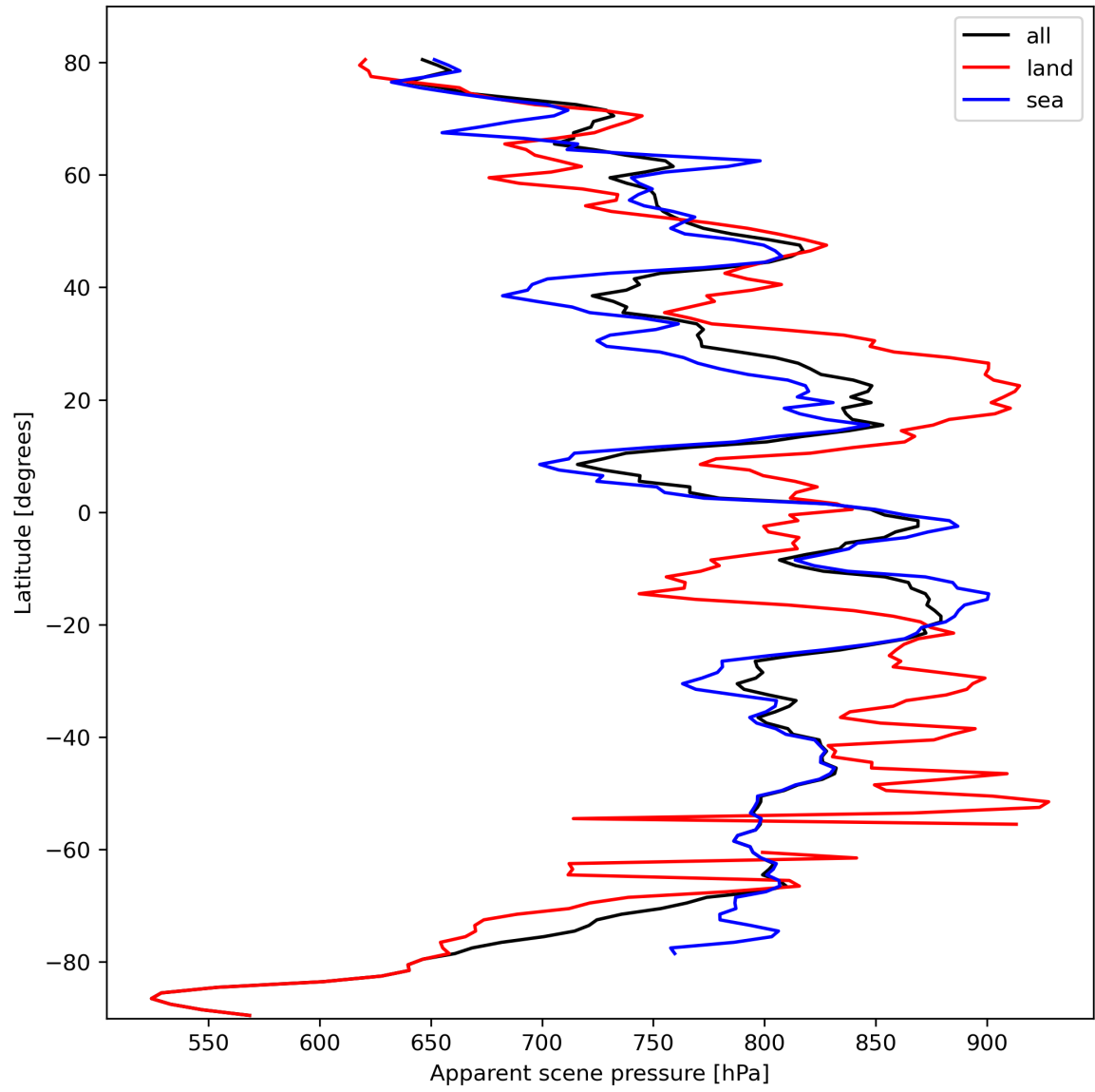
Figure 19: Zonal average of “Apparent scene pressure” for 2023-10-12 to 2023-10-13.
