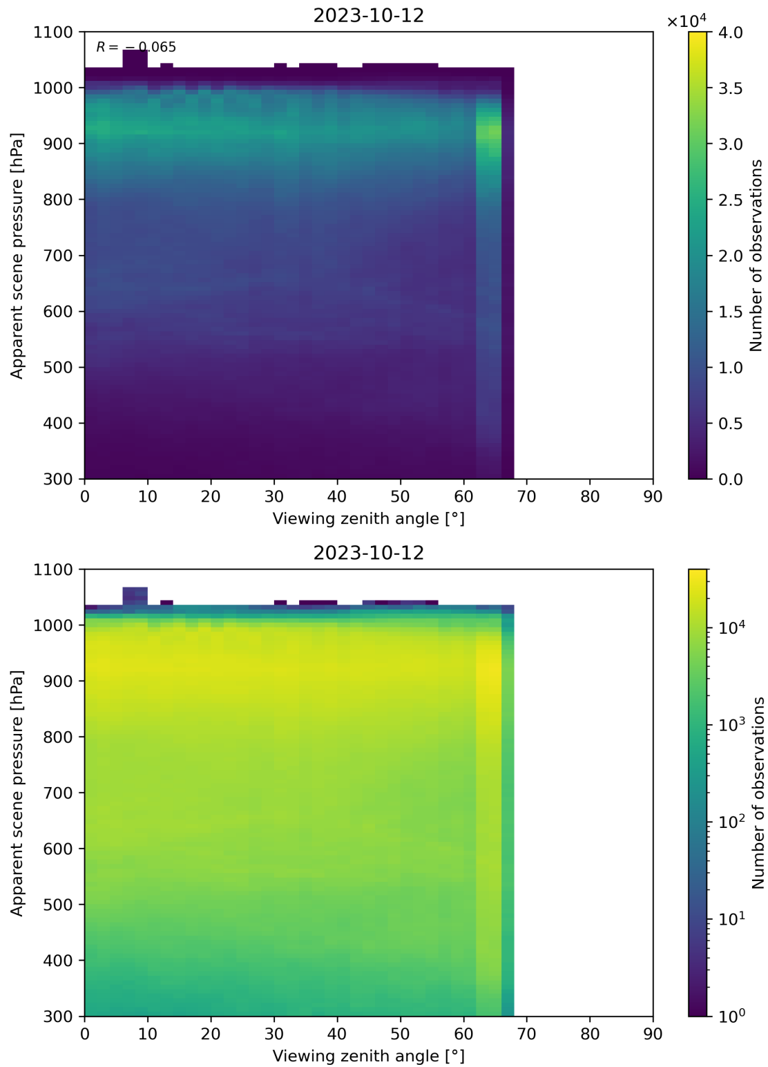
Figure 129: Scatter density plot of “Viewing zenith angle” against “Apparent scene pressure” for 2023-10-12 to 2023-10-13.
