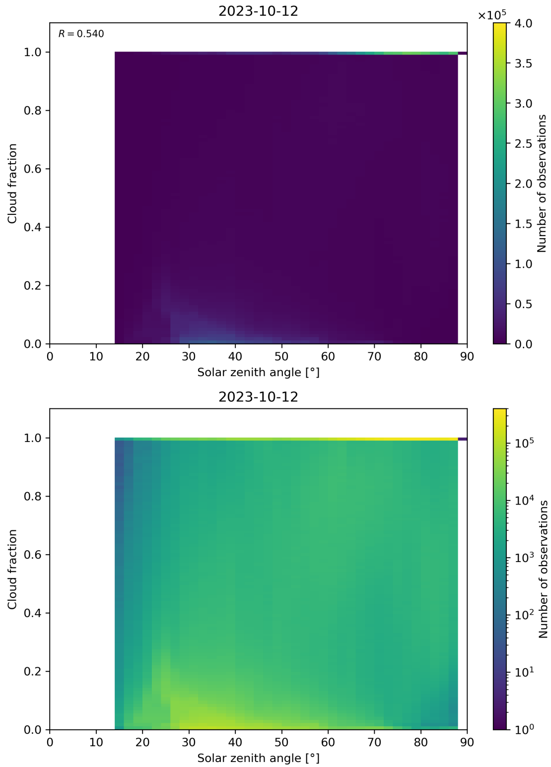
Figure 121: Scatter density plot of “Solar zenith angle” against “Cloud fraction” for 2023-10-12 to 2023-10-13.
