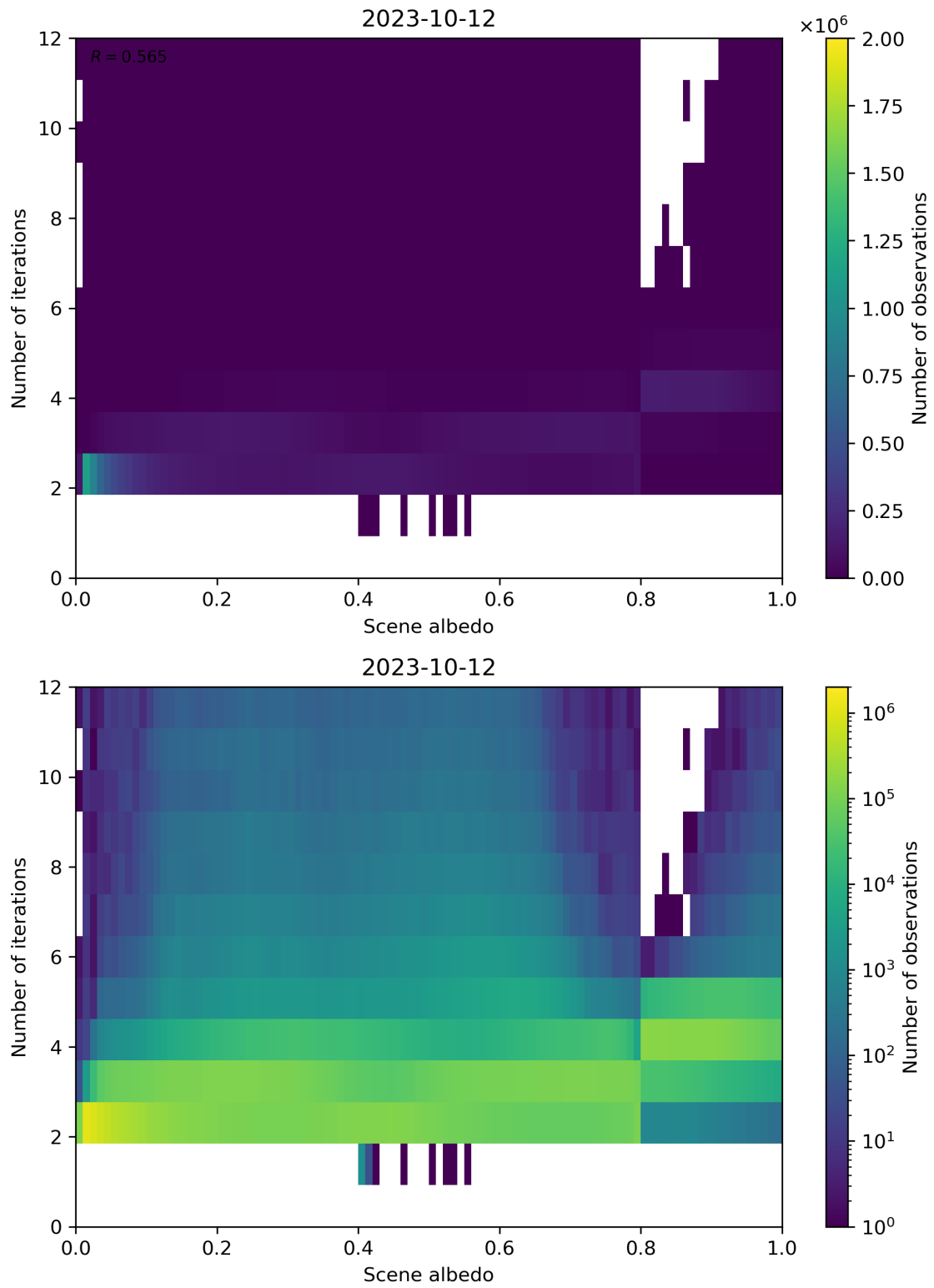
Figure 115: Scatter density plot of “Scene albedo” against “Number of iterations” for 2023-10-12 to 2023-10-13.
