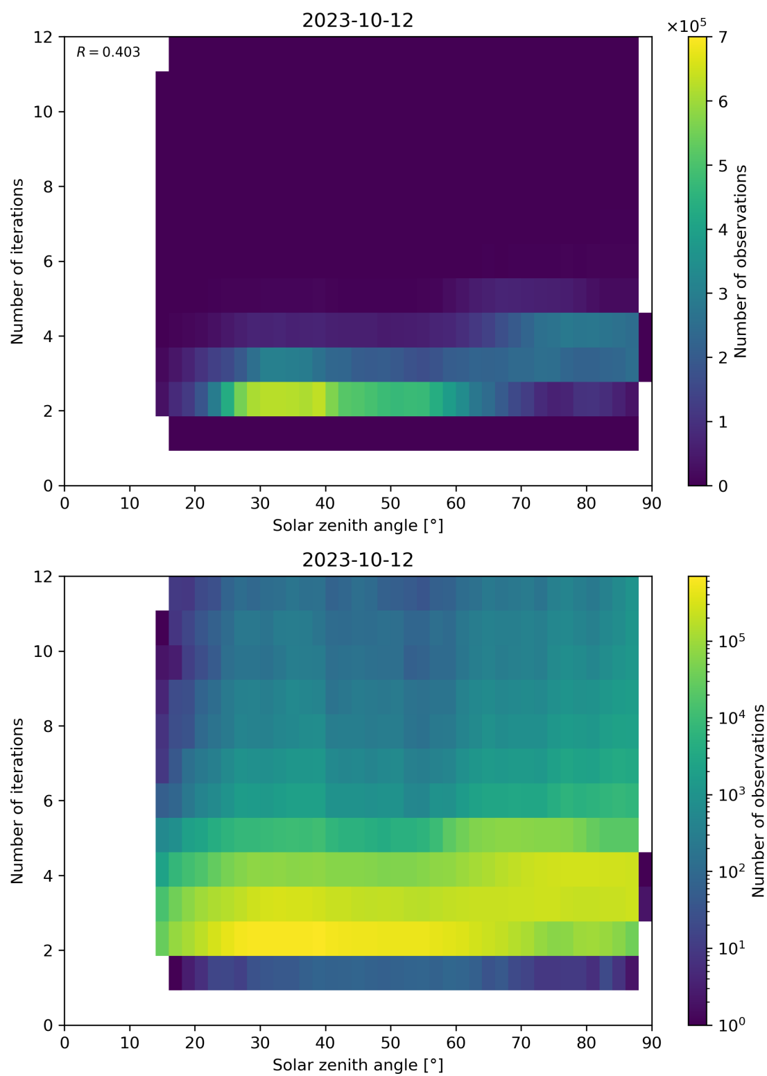
Figure 125: Scatter density plot of “Solar zenith angle” against “Number of iterations” for 2023-10-12 to 2023-10-13.
