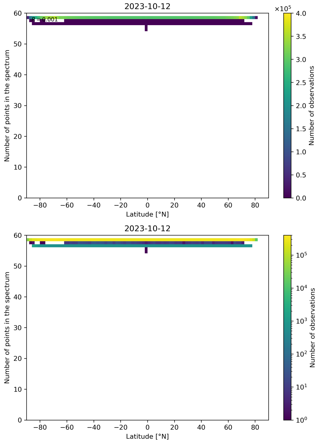
Figure 103: Scatter density plot of “Latitude” against “Number of points in the spectrum” for 2023-10-12 to 2023-10-13.
