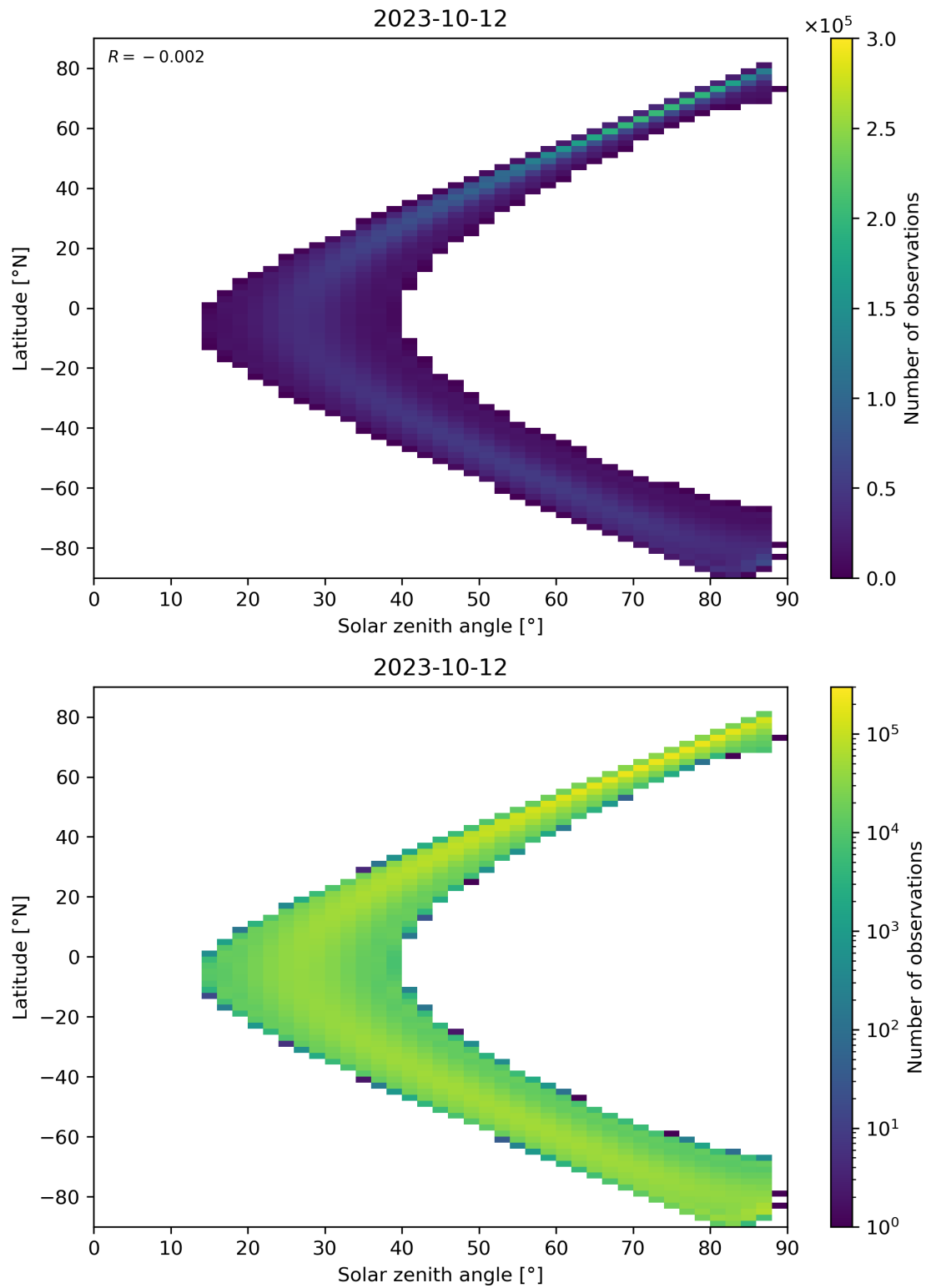
Figure 124: Scatter density plot of “Solar zenith angle” against “Latitude” for 2023-10-12 to 2023-10-13.
