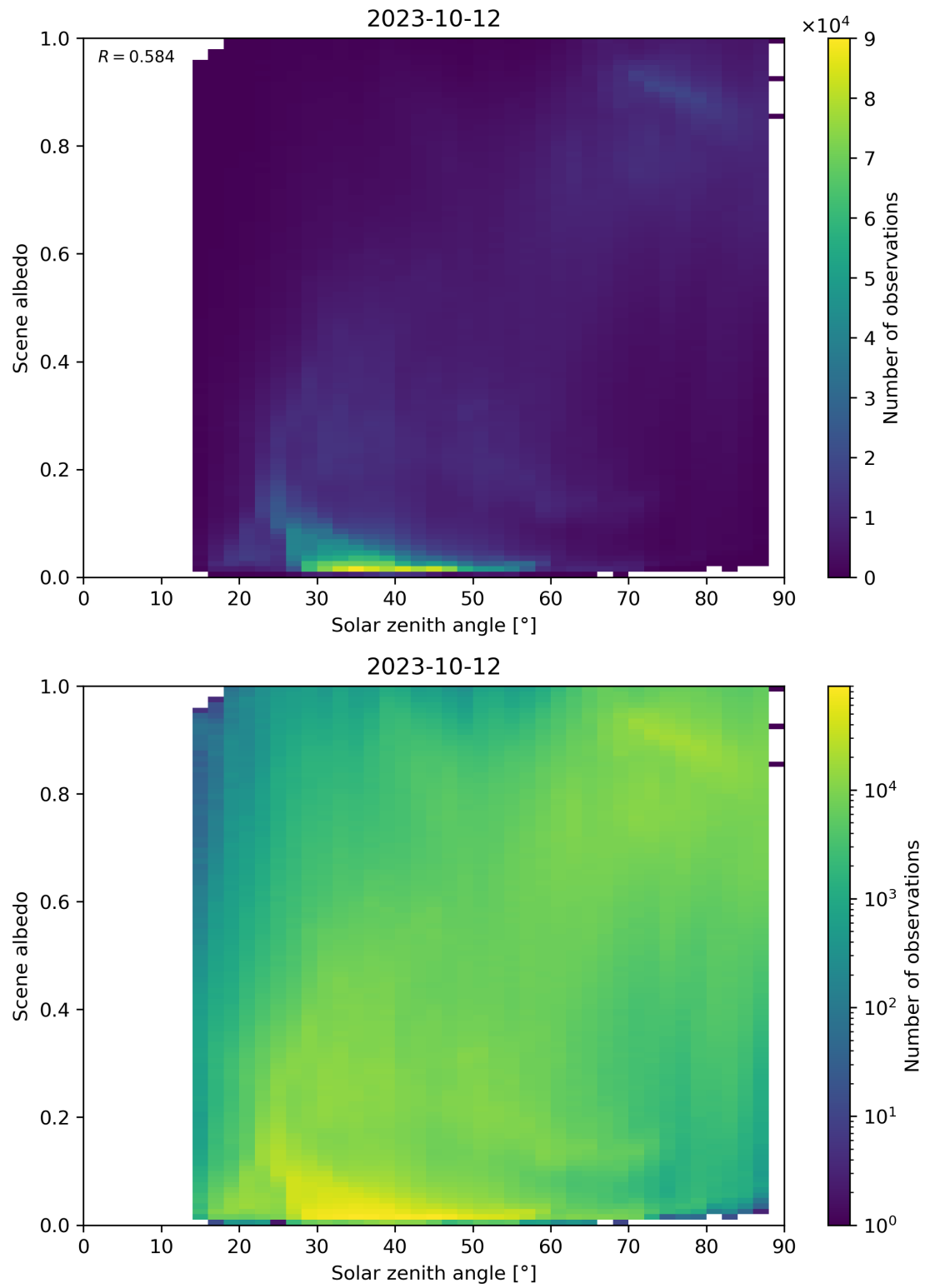
Figure 127: Scatter density plot of “Solar zenith angle” against “Scene albedo” for 2023-10-12 to 2023-10-13.
