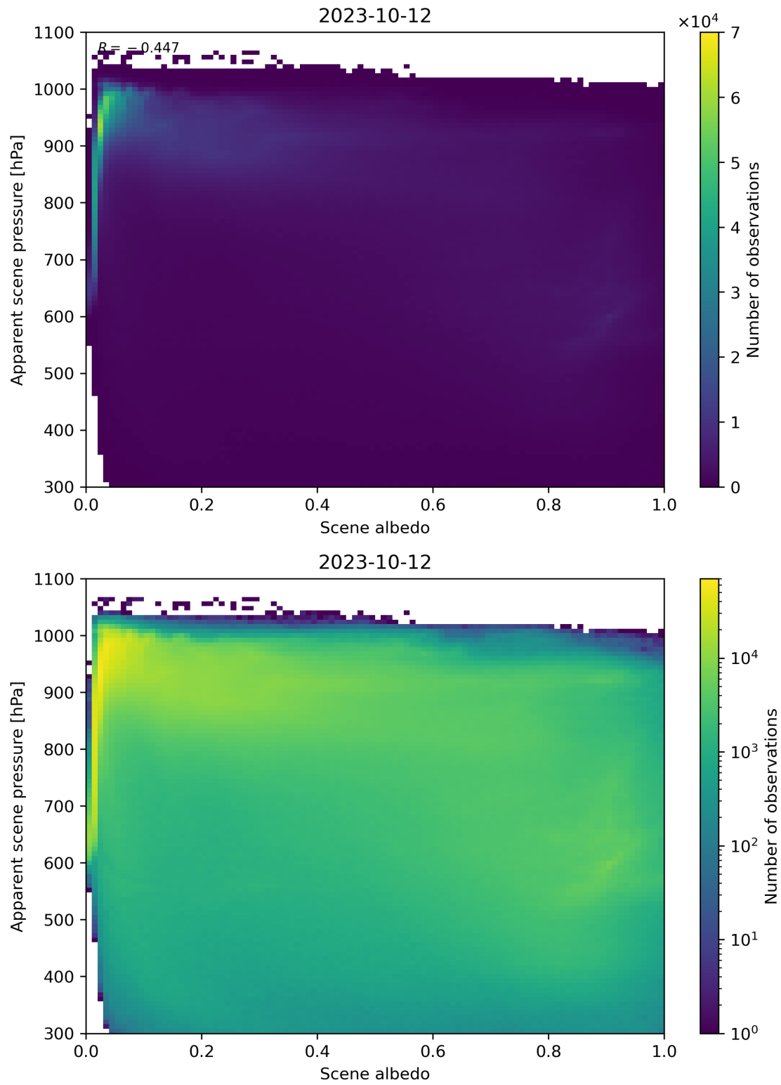
Figure 111: Scatter density plot of “Scene albedo” against “Apparent scene pressure” for 2023-10-12 to 2023-10-13.
