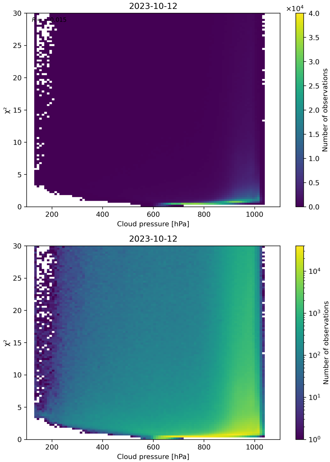
Figure 85: Scatter density plot of “Cloud pressure” against “ \chi^2 ” for 2023-10-12 to 2023-10-13.
