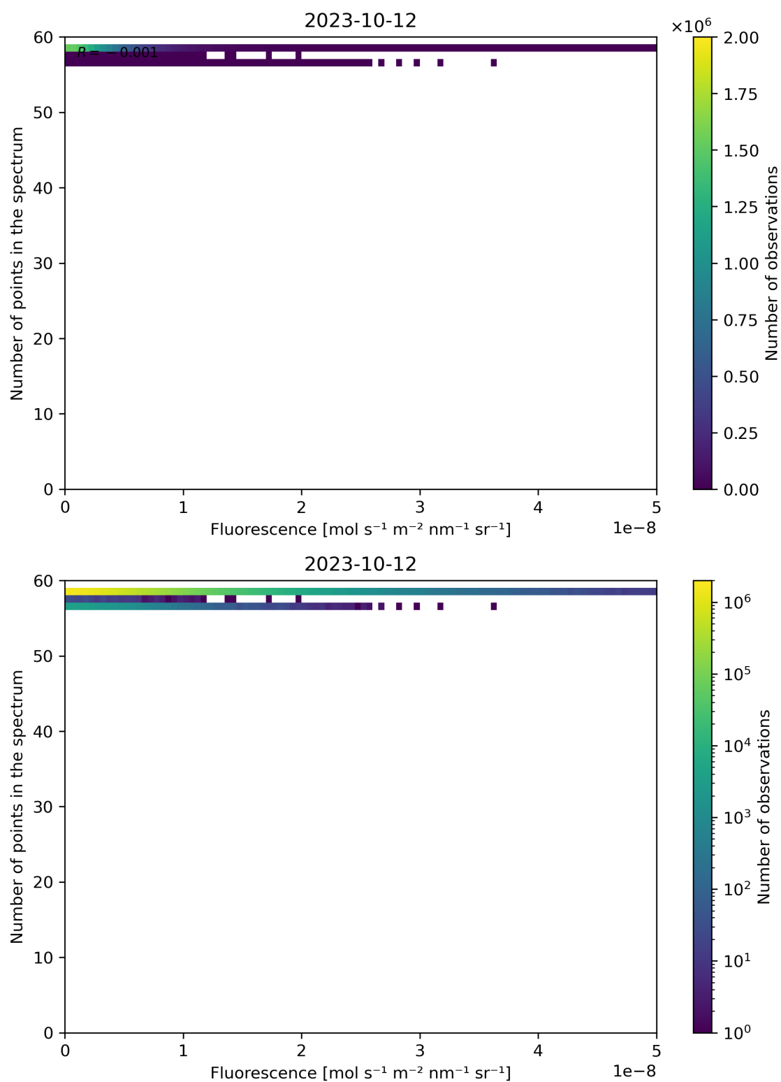
Figure 94: Scatter density plot of “Fluorescence” against “Number of points in the spectrum” for 2023-10-12 to 2023-10-13.
