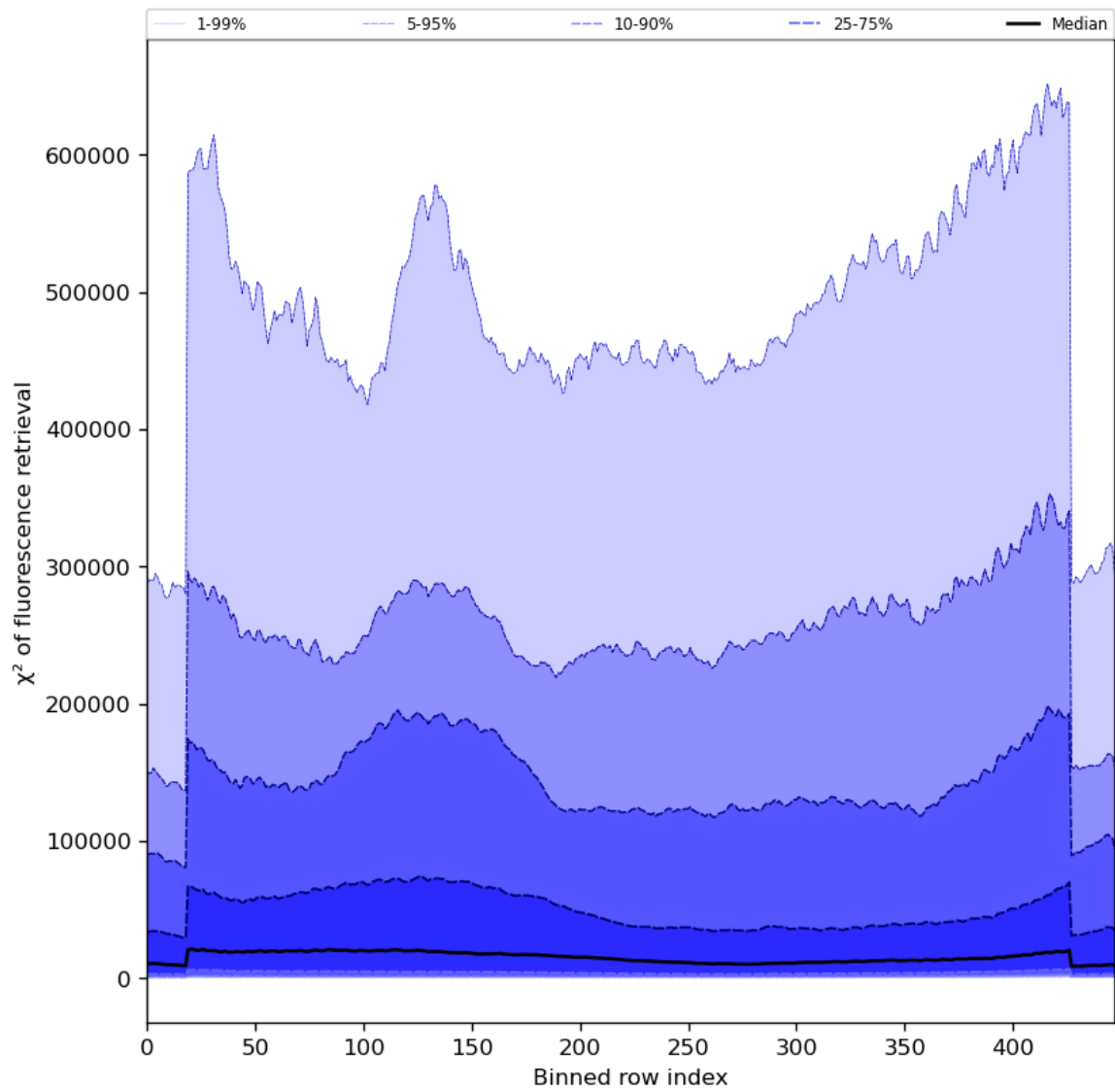
Figure 59: Along track statistics of “ \chi^2 of fluorescence retrieval” for 2023-10-12 to 2023-10-13
