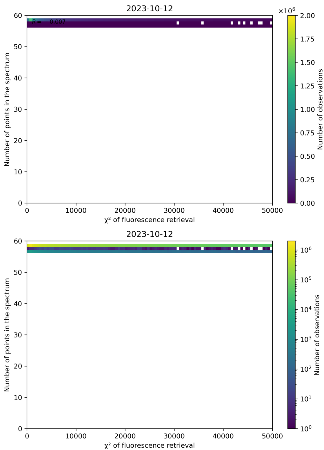
Figure 71: Scatter density plot of " \chi^2 of fluorescence retrieval" against "Number of points in the spectrum" for 2023-10-12 to 2023-10-13.
