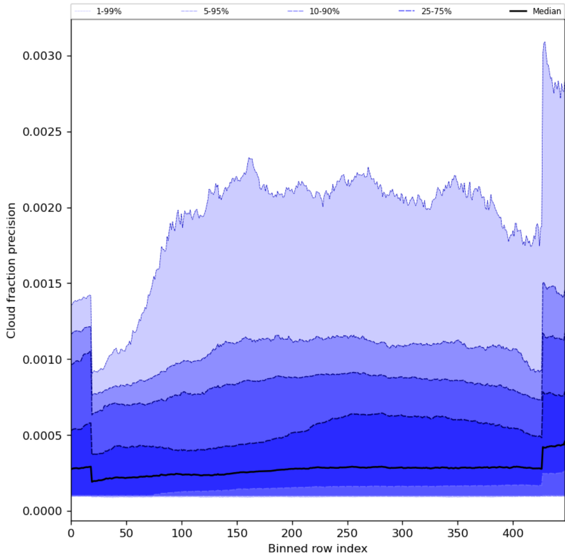
Figure 50: Along track statistics of “Cloud fraction precision” for 2023-10-12 to 2023-10-13
