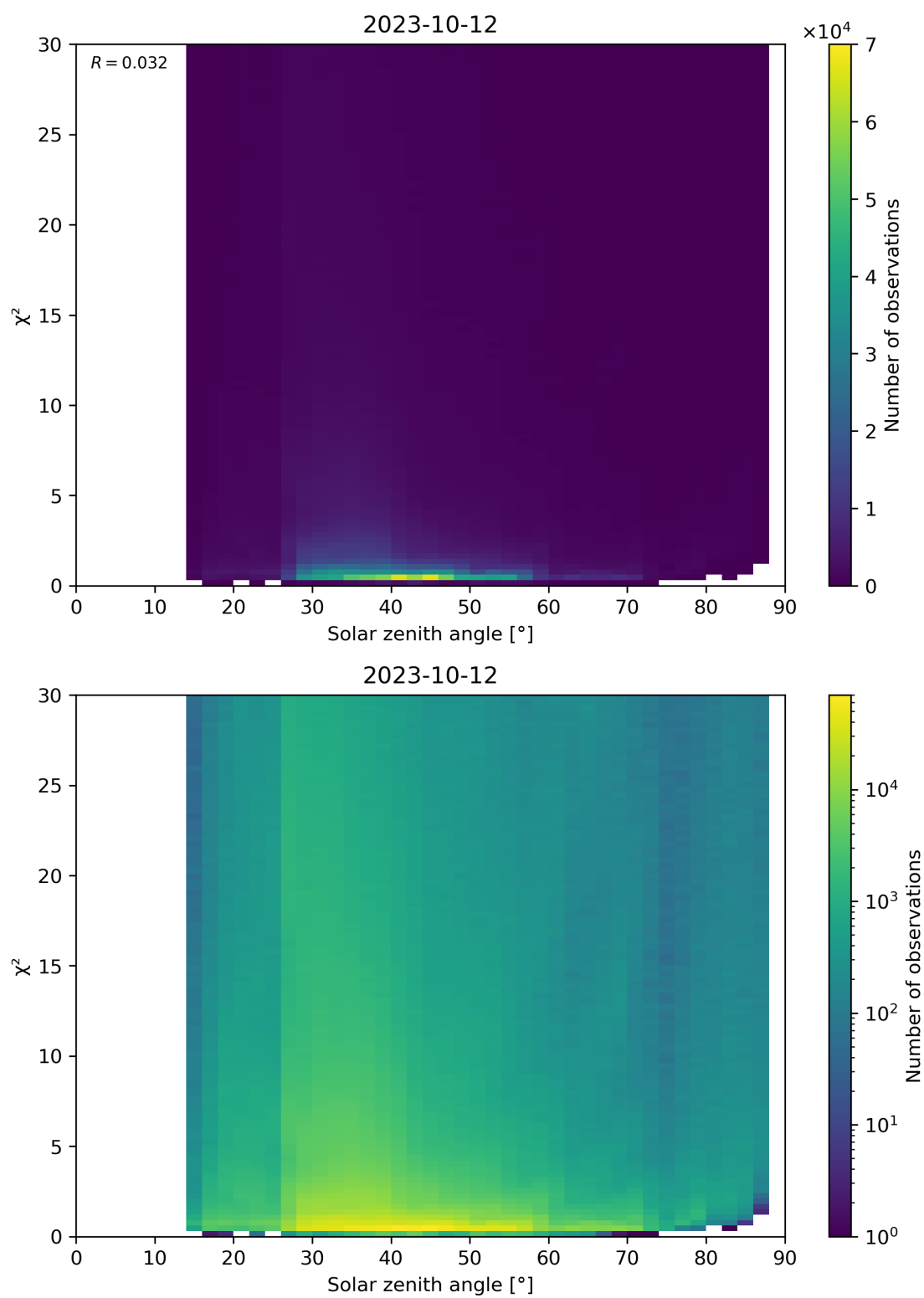
Figure 119: Scatter density plot of “Solar zenith angle” against “ \chi^2 ” for 2023-10-12 to 2023-10-13.
