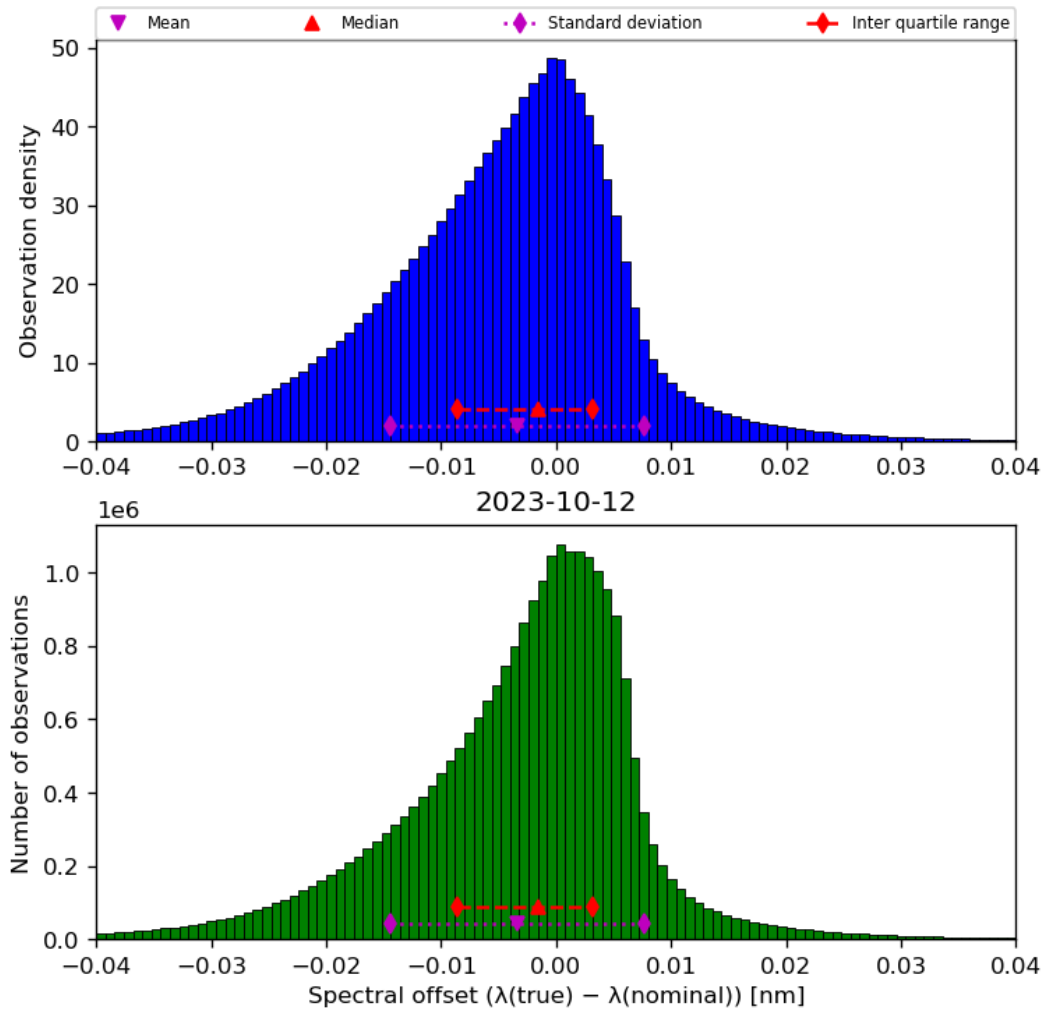
Figure 45: Histogram of “Spectral offset ( \lambda(\text{true}) - \lambda(\text{nominal}) )” for 2023-10-12 to 2023-10-13
