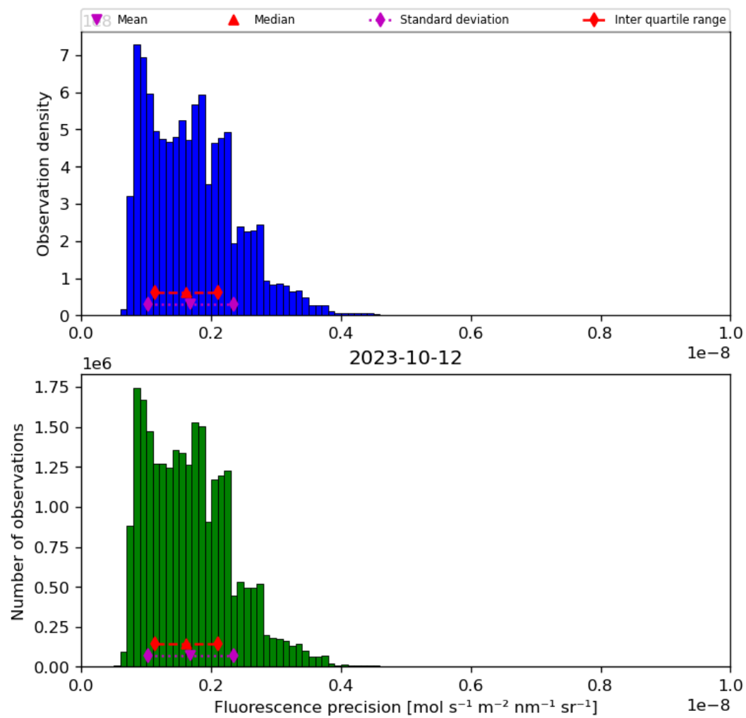
Figure 41: Histogram of “Fluorescence precision” for 2023-10-12 to 2023-10-13
