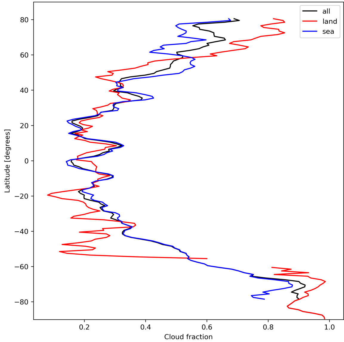
Figure 15: Zonal average of “Cloud fraction” for 2023-10-12 to 2023-10-13.
