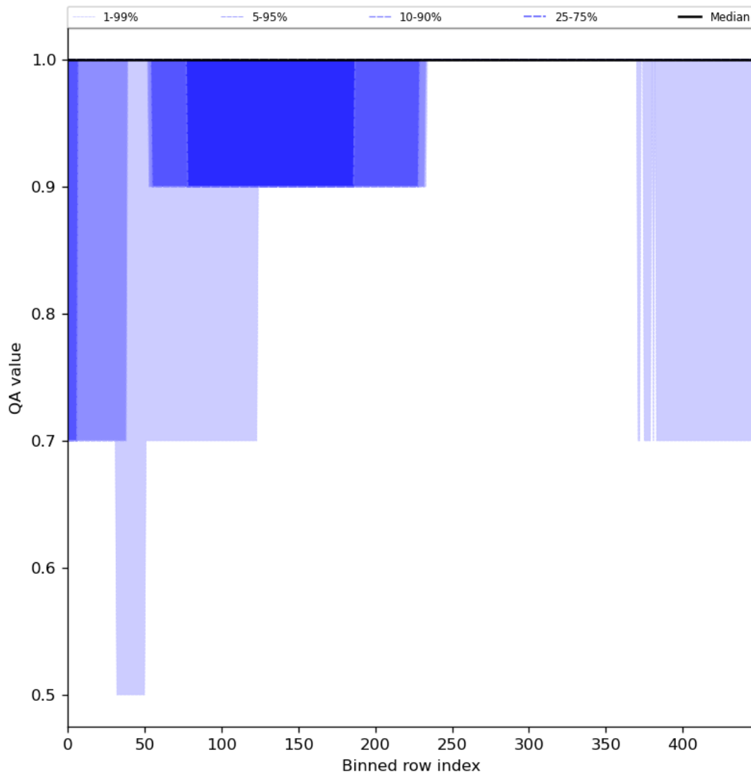
Figure 46: Along track statistics of “QA value” for 2023-10-12 to 2023-10-13
