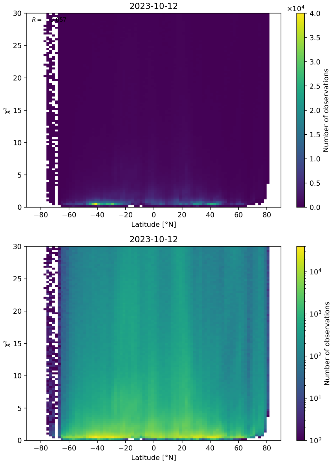
Figure 97: Scatter density plot of “Latitude” against “ \chi^2 ” for 2023-10-12 to 2023-10-13.
