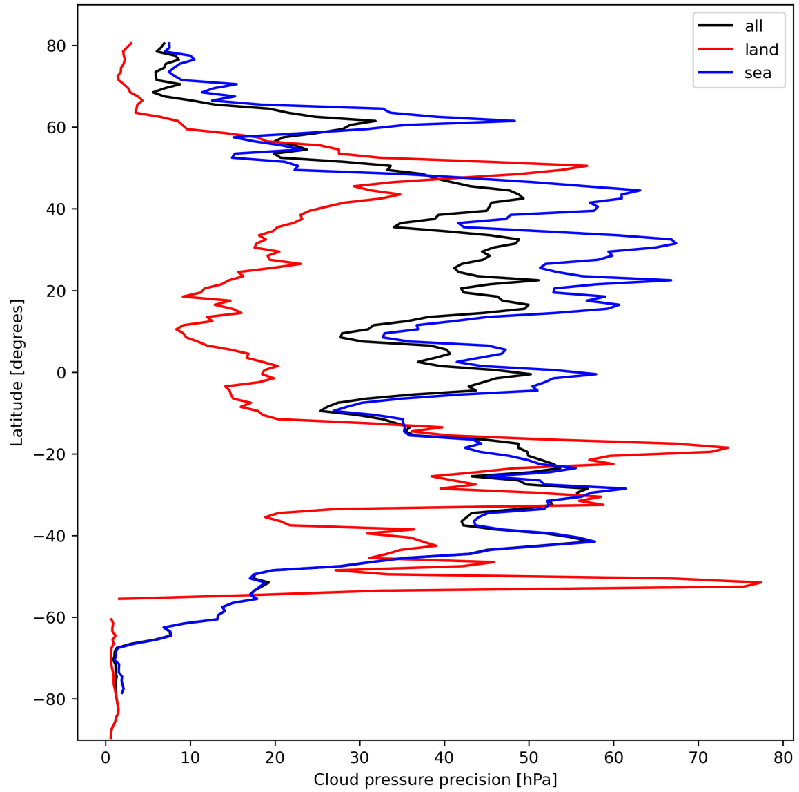
Figure 14: Zonal average of “Cloud pressure precision” for 2023-10-12 to 2023-10-13.
