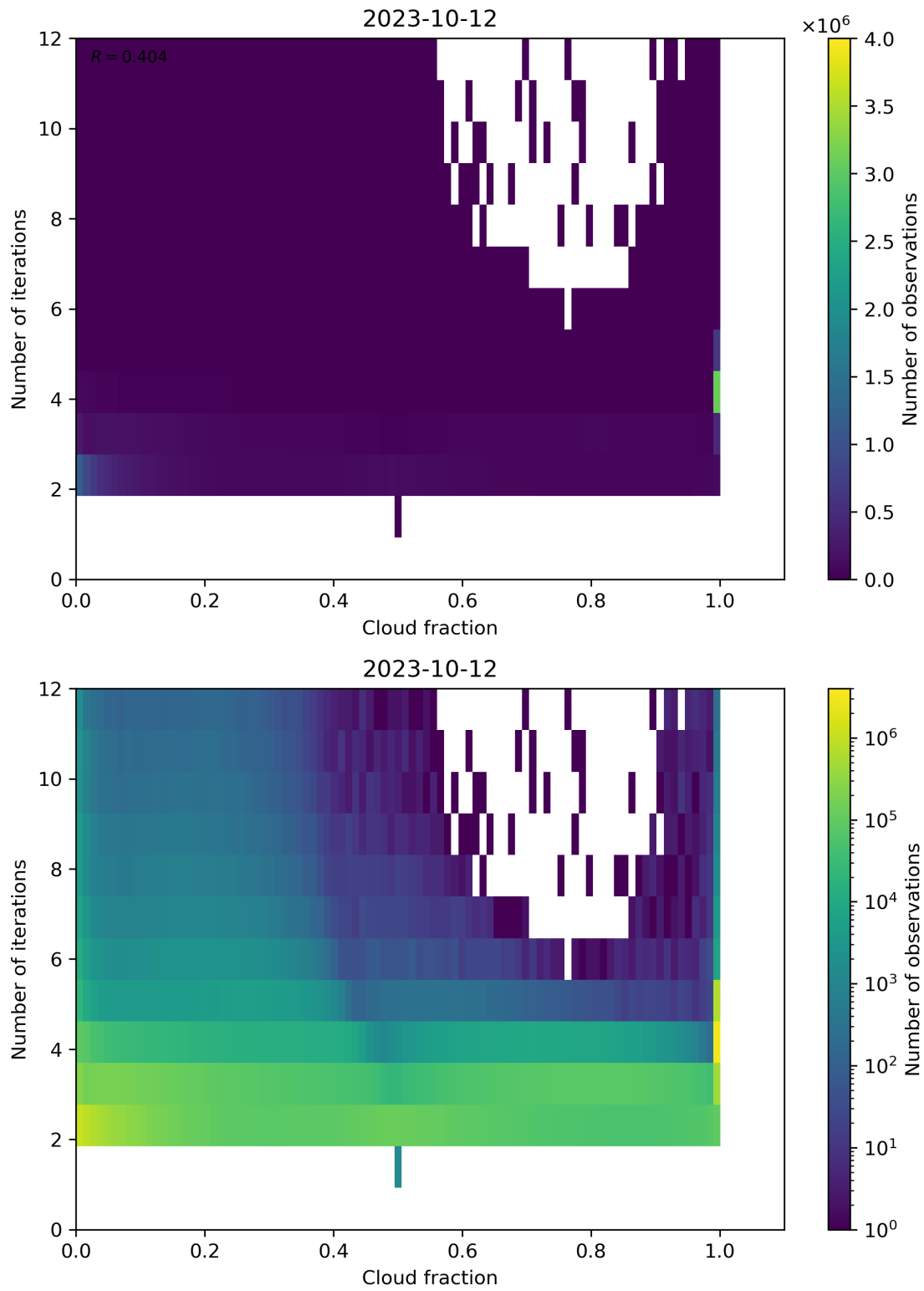
Figure 80: Scatter density plot of “Cloud fraction” against “Number of iterations” for 2023-10-12 to 2023-10-13.
