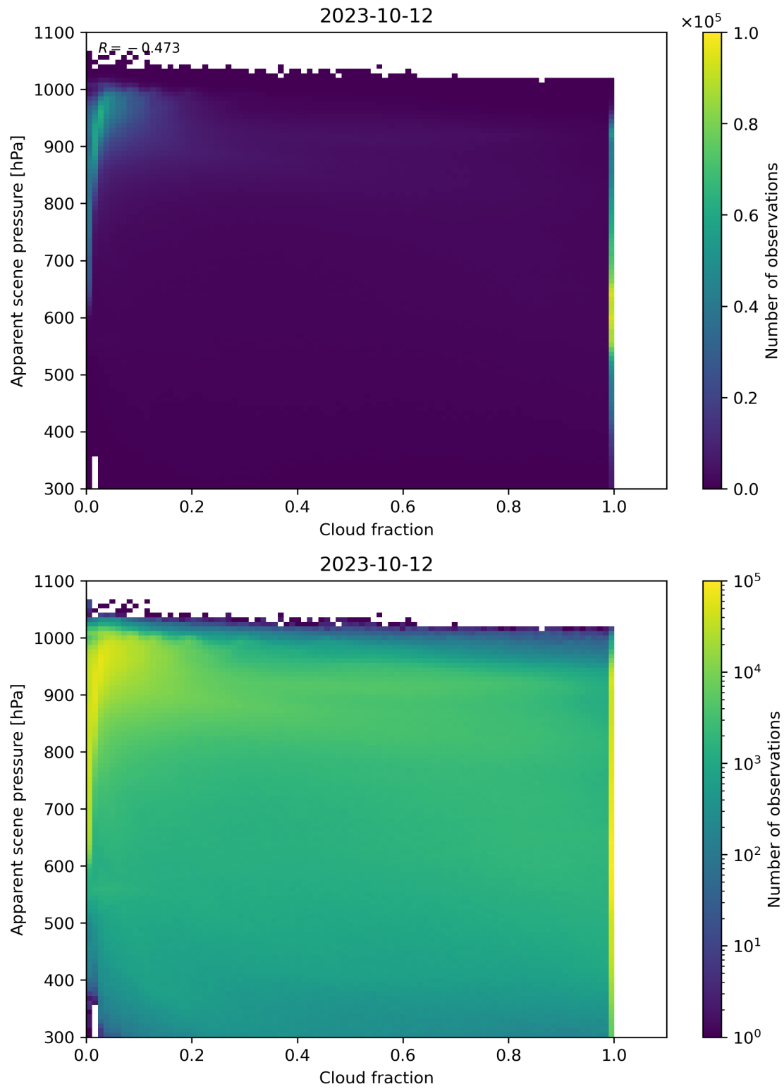
Figure 76: Scatter density plot of “Cloud fraction” against “Apparent scene pressure” for 2023-10-12 to 2023-10-13.
