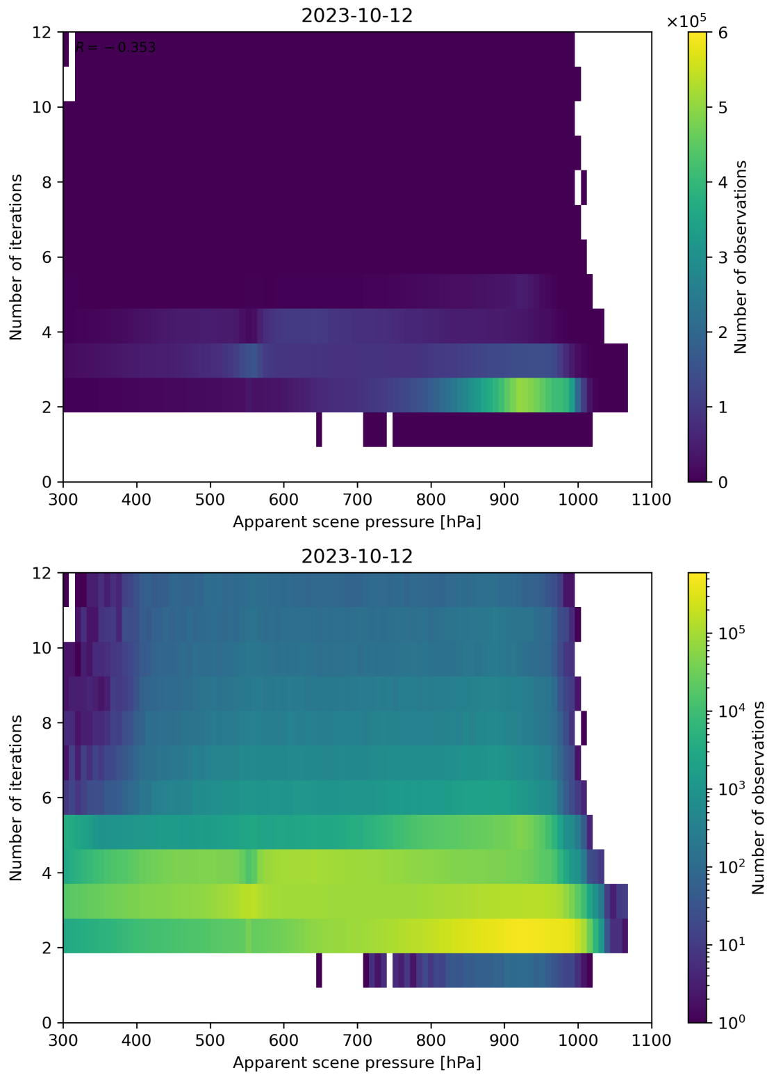
Figure 66: Scatter density plot of “Apparent scene pressure” against “Number of iterations” for 2023-10-12 to 2023-10-13.
