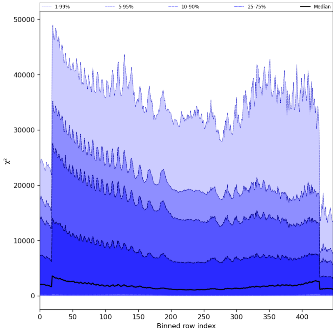
Figure 55: Along track statistics of “ \chi^2 ” for 2023-10-12 to 2023-10-13
