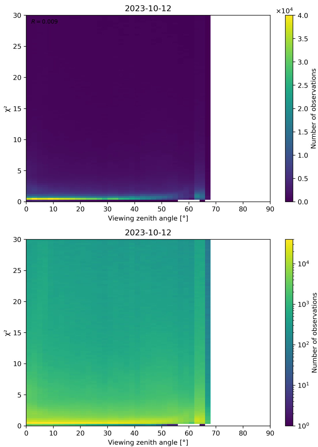
Figure 130: Scatter density plot of “Viewing zenith angle” against “ \chi^2 ” for 2023-10-12 to 2023-10-13.
