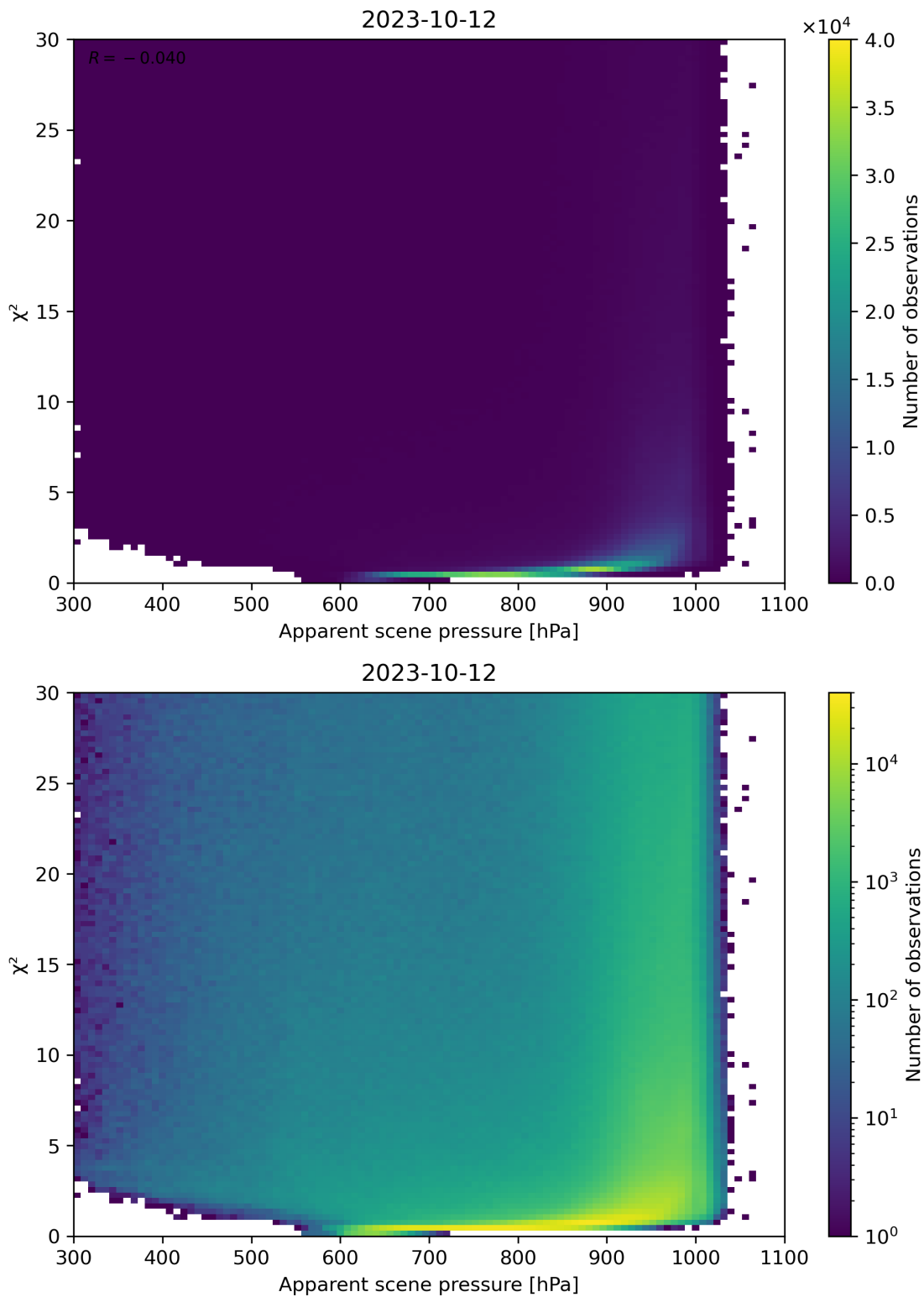
Figure 63: Scatter density plot of “Apparent scene pressure” against “ \chi^2 ” for 2023-10-12 to 2023-10-13.
