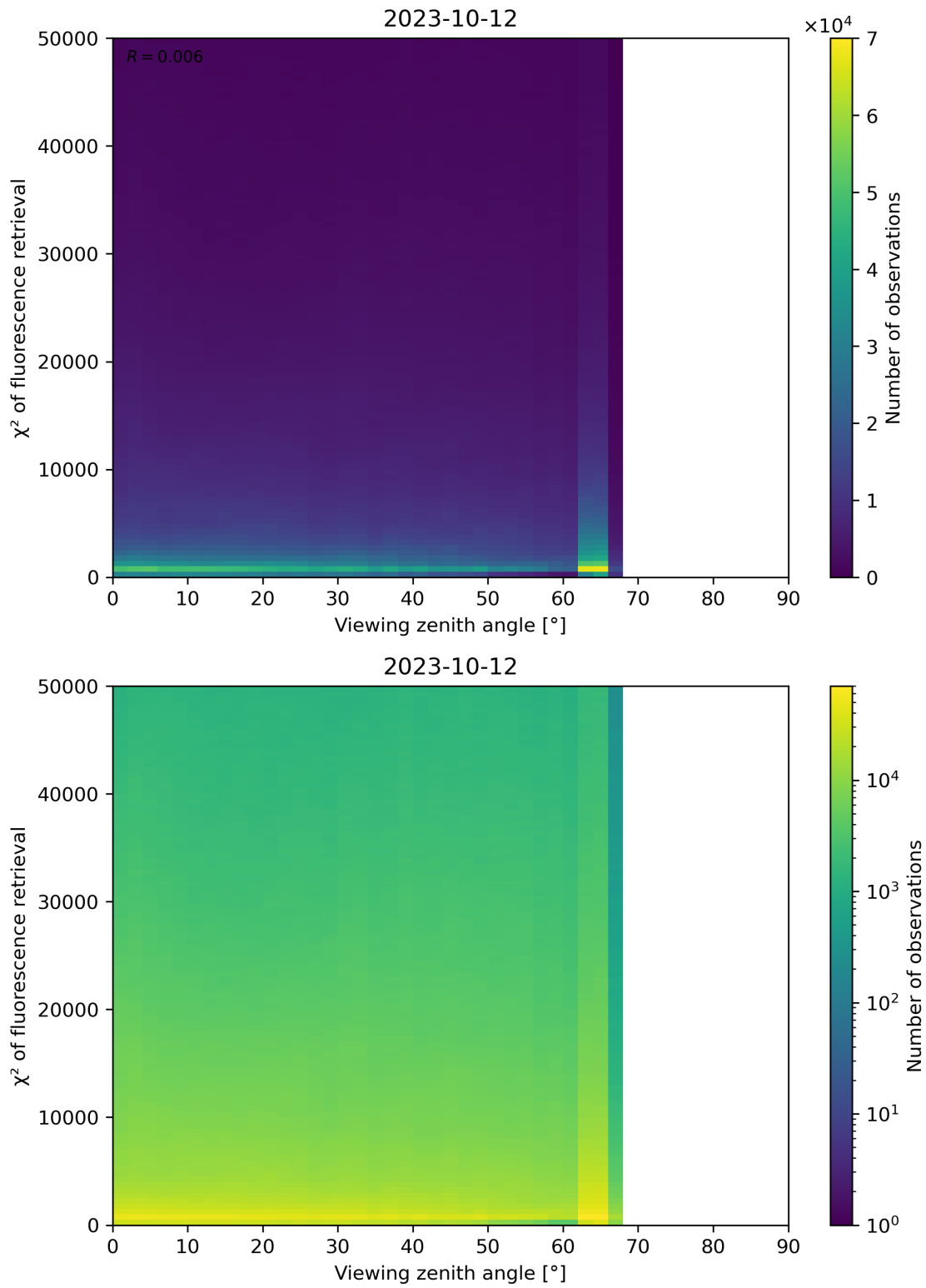
Figure 131: Scatter density plot of “Viewing zenith angle” against “ \chi^2 of fluorescence retrieval” for 2023-10-12 to 2023-10-13.
