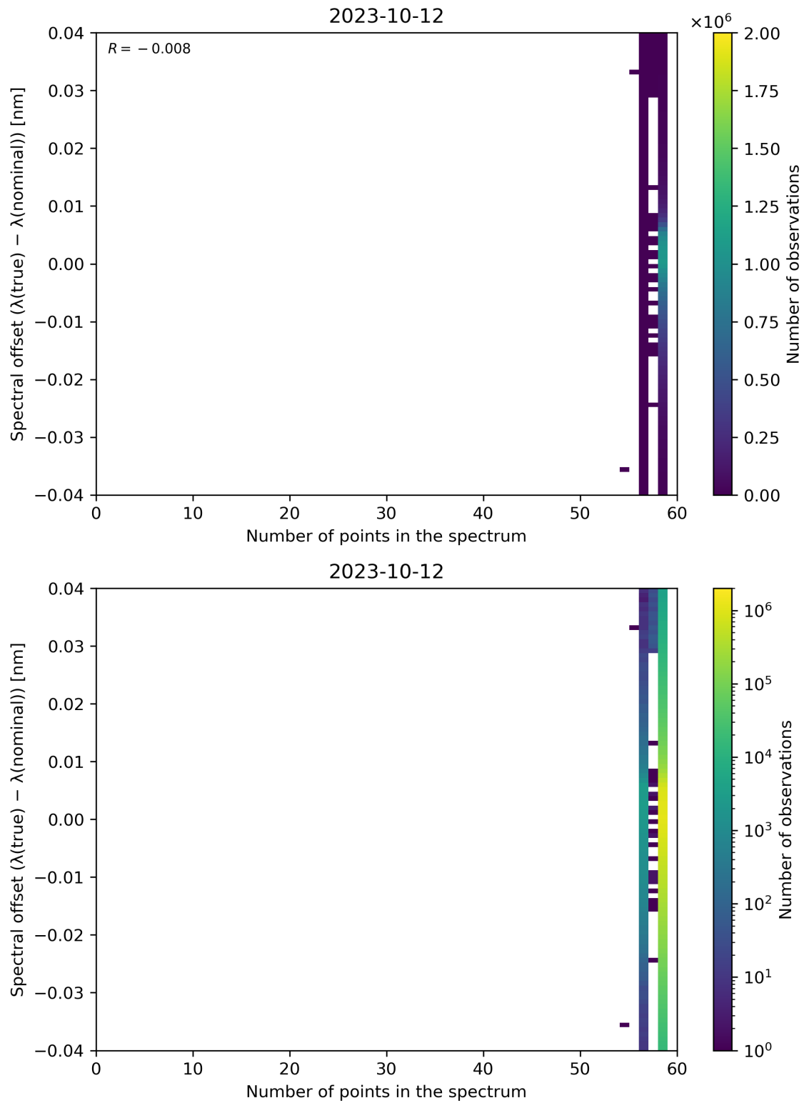
Figure 110: Scatter density plot of “Number of points in the spectrum” against “Spectral offset ( \lambda(\text{true}) - \lambda(\text{nominal}) )” for 2023-10-12 to 2023-10-13.
