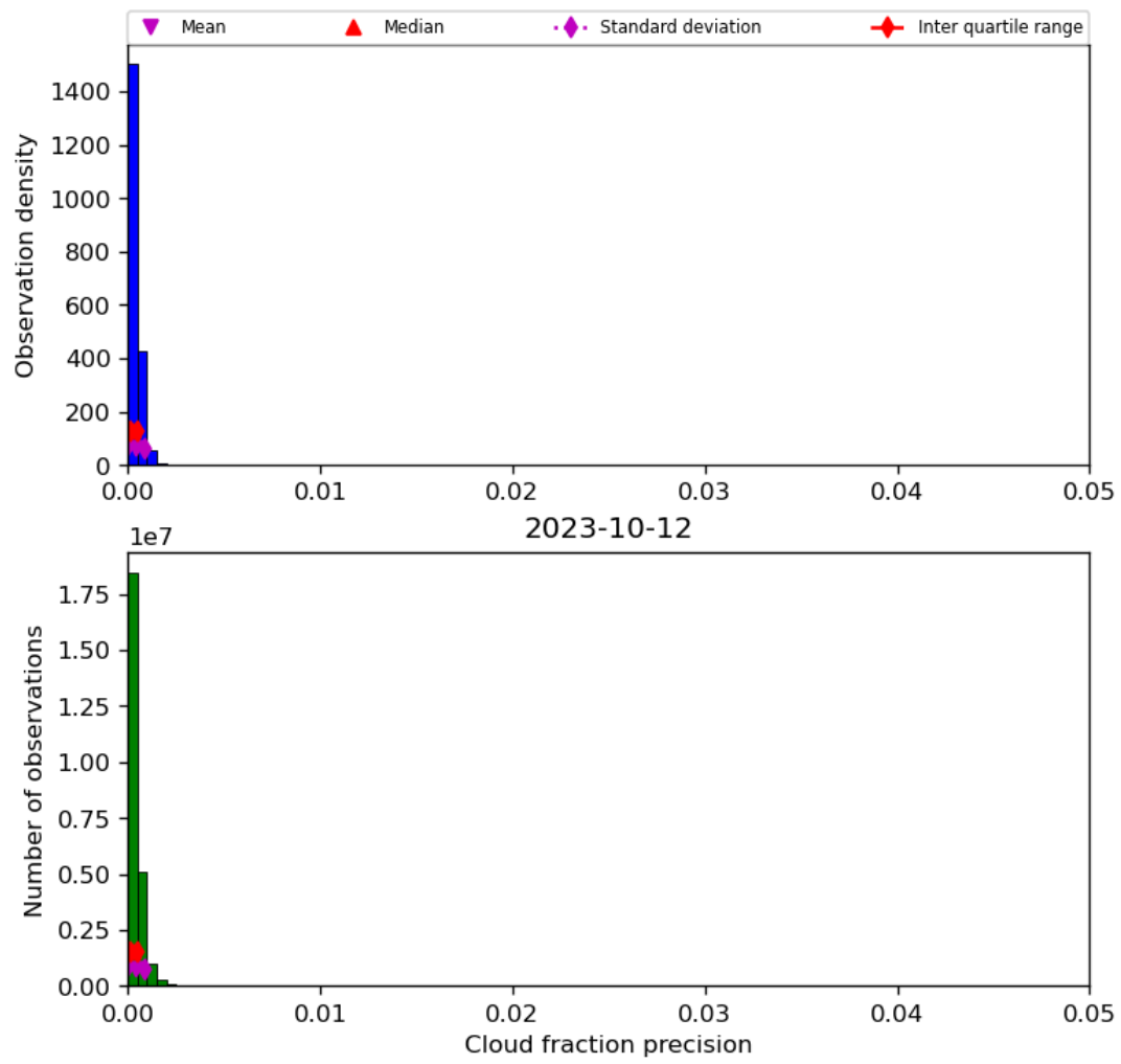
Figure 33: Histogram of “Cloud fraction precision” for 2023-10-12 to 2023-10-13
