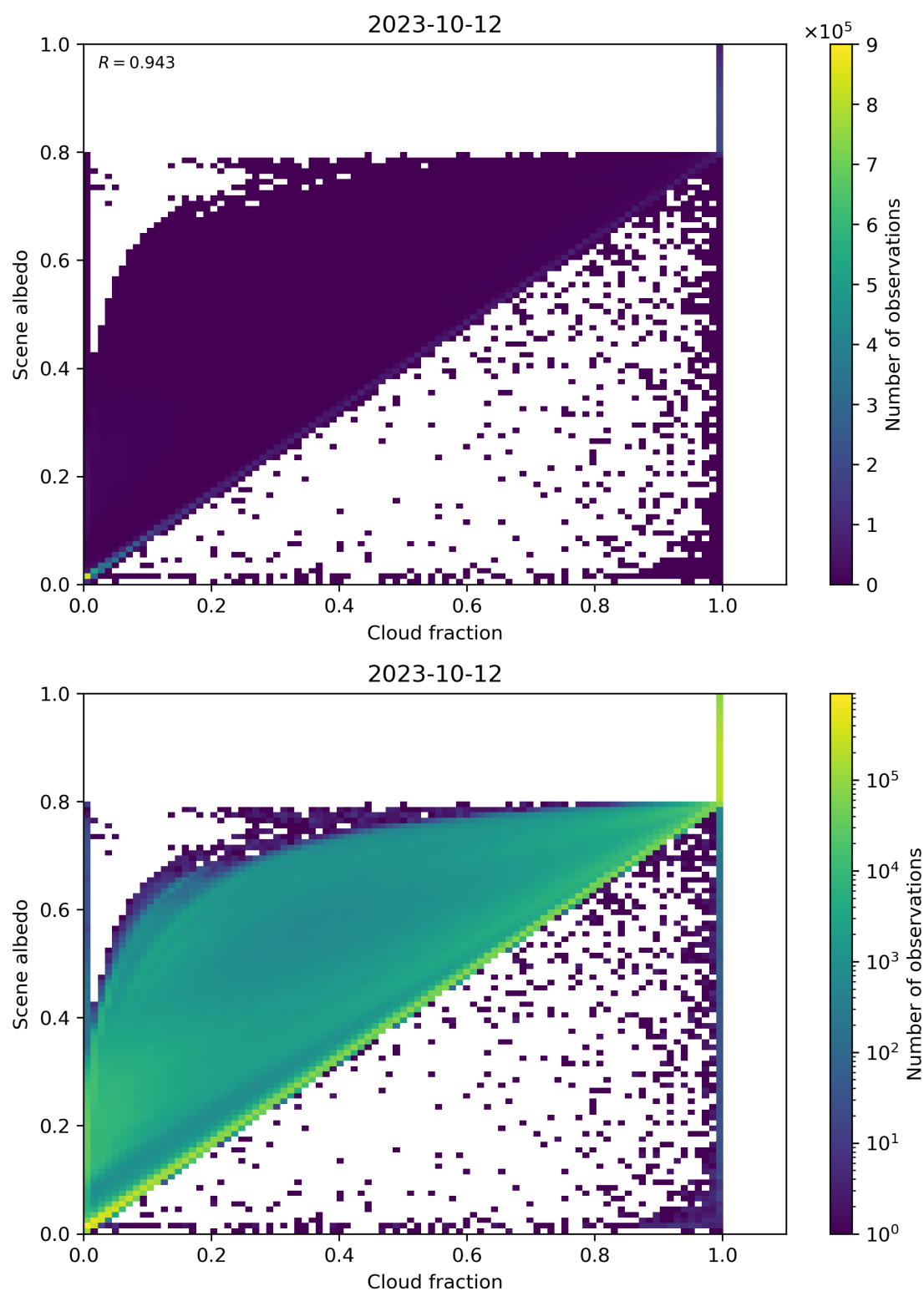
Figure 82: Scatter density plot of “Cloud fraction” against “Scene albedo” for 2023-10-12 to 2023-10-13.
