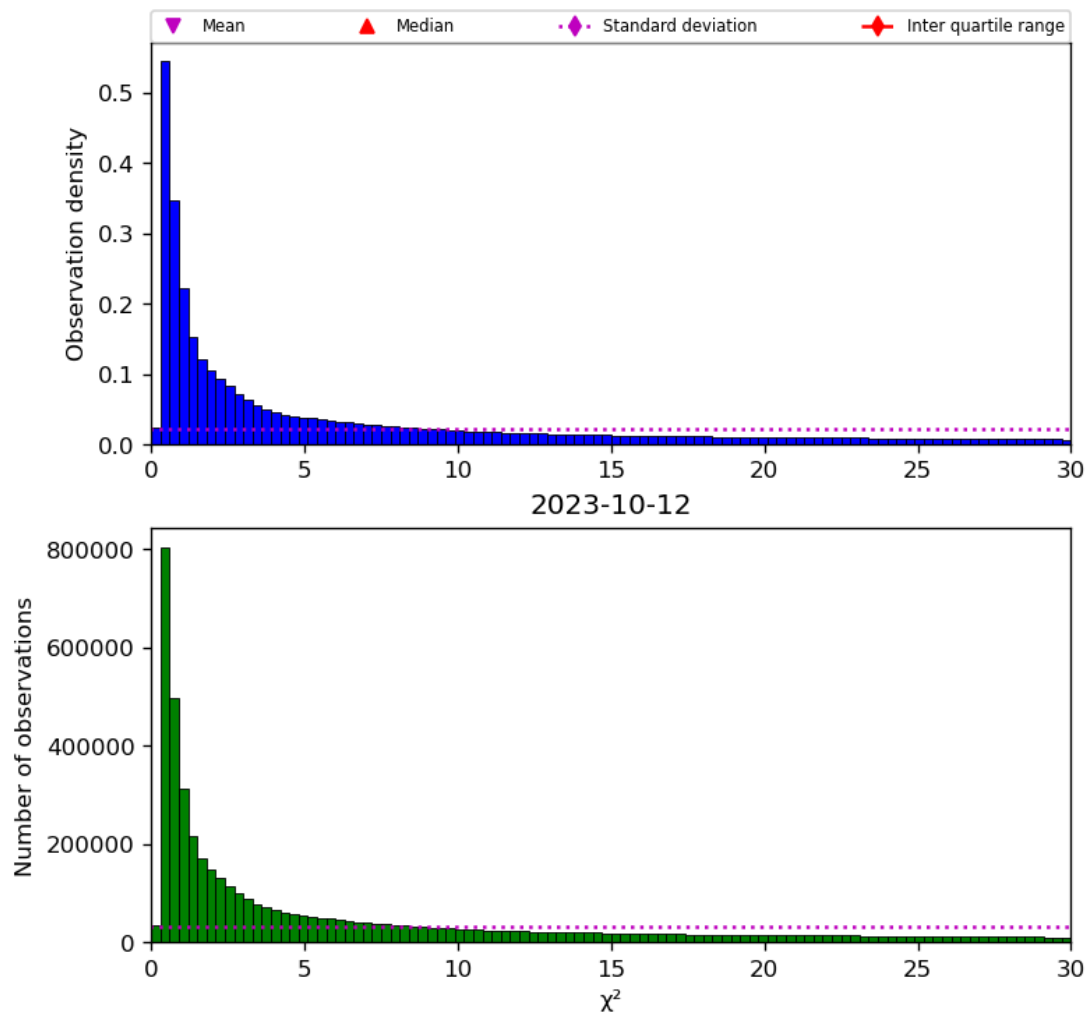
Figure 38: Histogram of “ \chi^2 ” for 2023-10-12 to 2023-10-13
