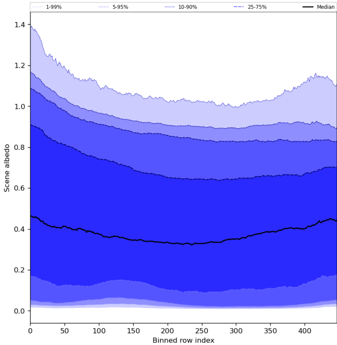
Figure 51: Along track statistics of “Scene albedo” for 2023-10-12 to 2023-10-13
