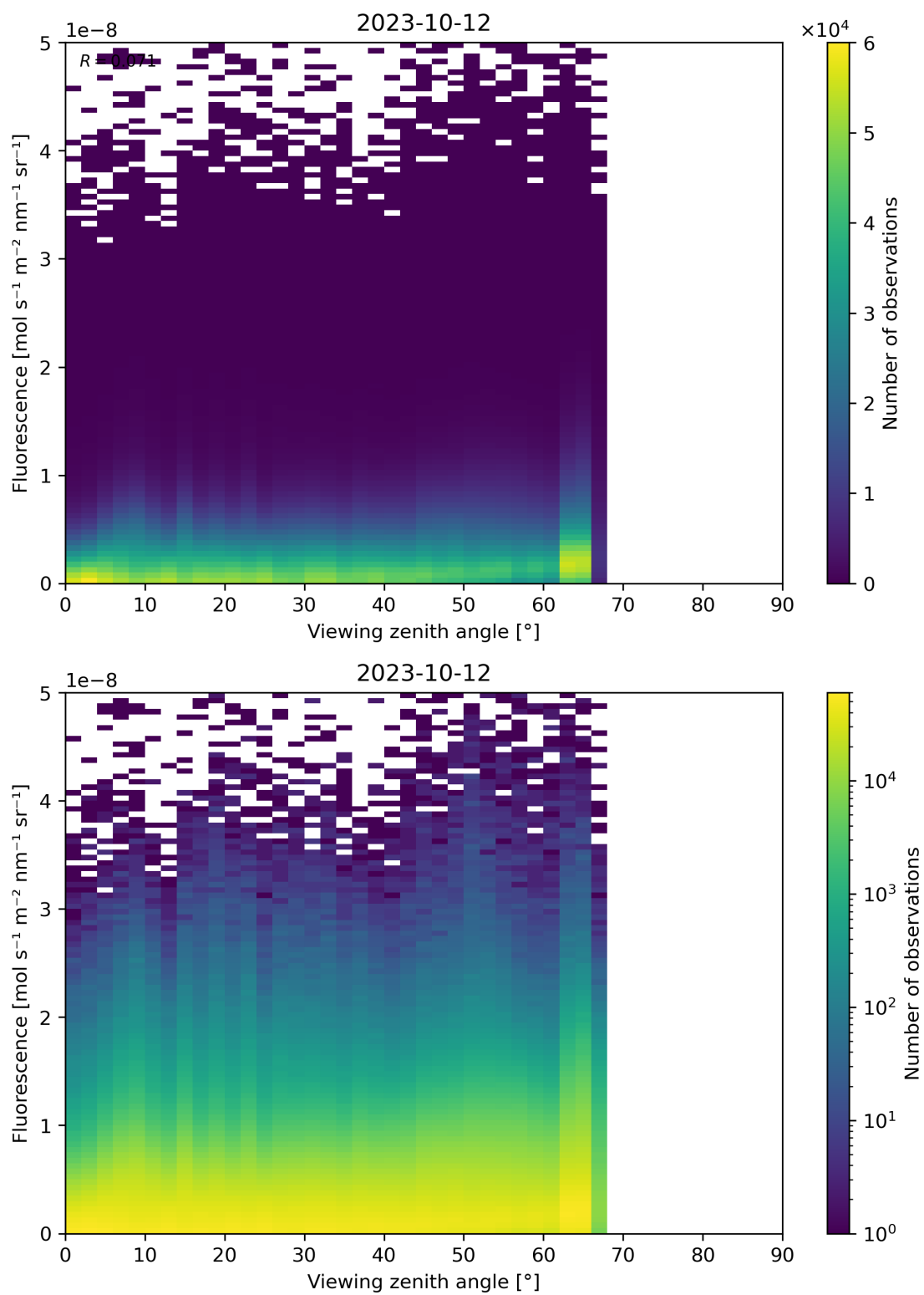
Figure 134: Scatter density plot of “Viewing zenith angle” against “Fluorescence” for 2023-10-12 to 2023-10-13.
