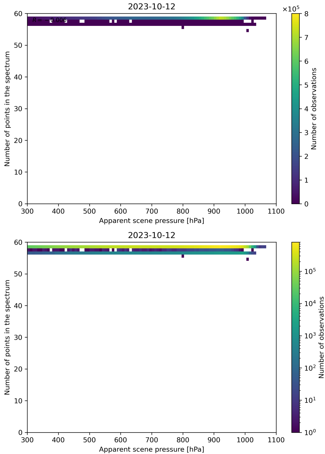
Figure 67: Scatter density plot of “Apparent scene pressure” against “Number of points in the spectrum” for 2023-10-12 to 2023-10-13.
