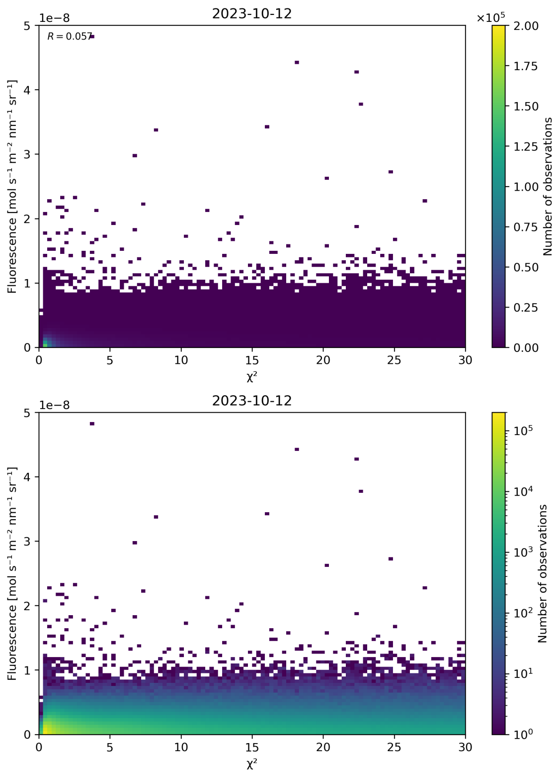
Figure 70: Scatter density plot of “ \chi^2 ” against “Fluorescence” for 2023-10-12 to 2023-10-13.
