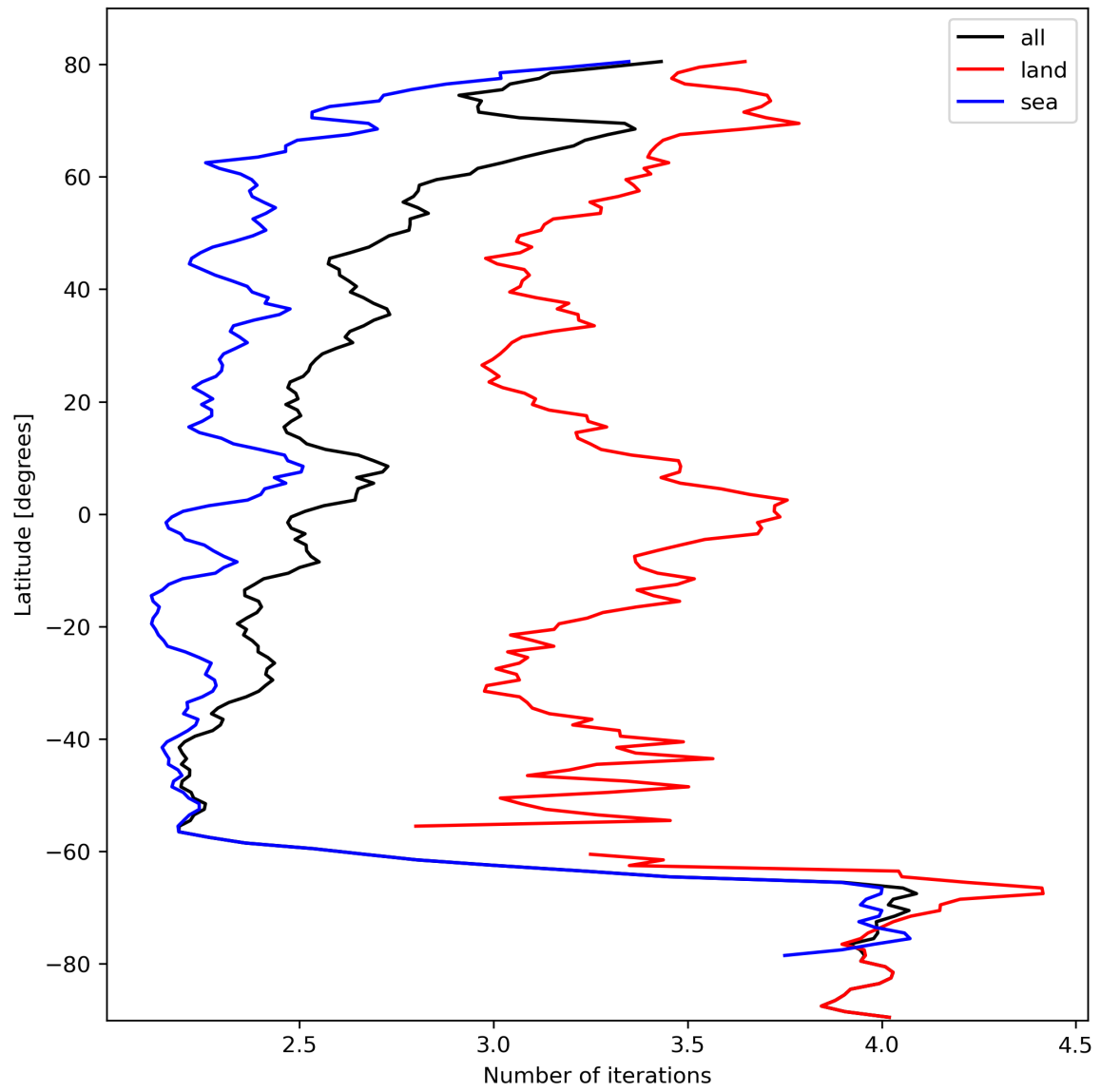
Figure 22: Zonal average of “Number of iterations” for 2023-10-12 to 2023-10-13.
