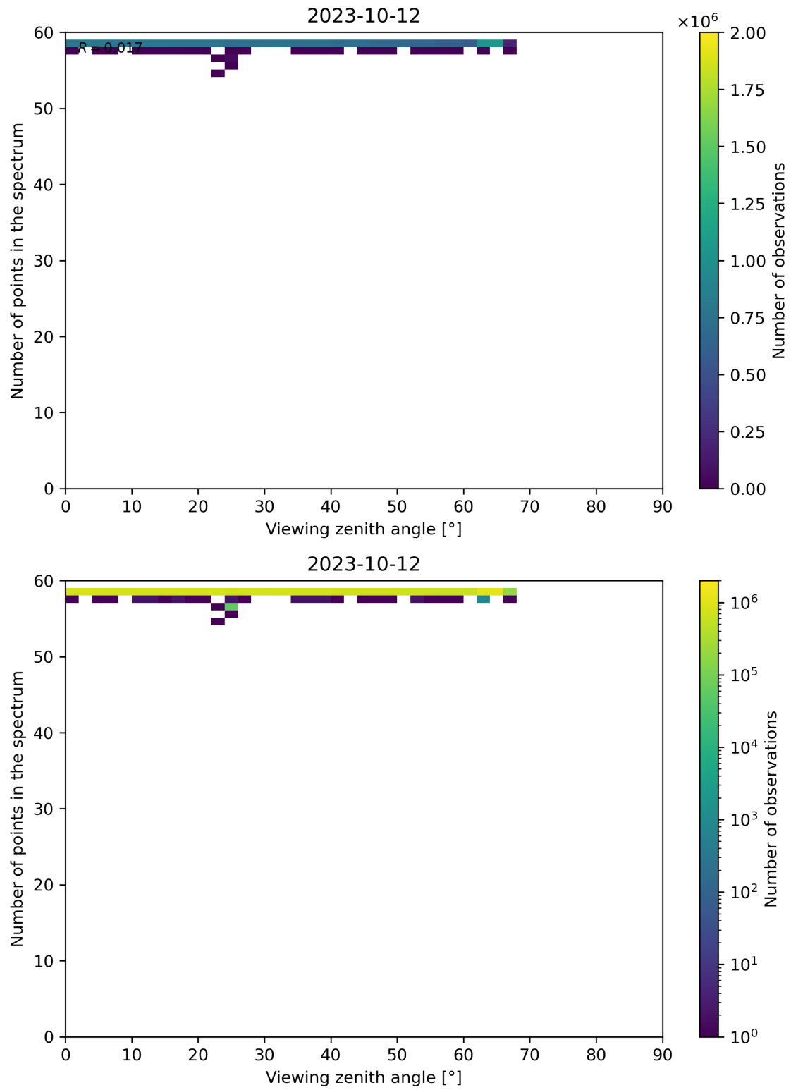
Figure 137: Scatter density plot of “Viewing zenith angle” against “Number of points in the spectrum” for 2023-10-12 to 2023-10-13.
