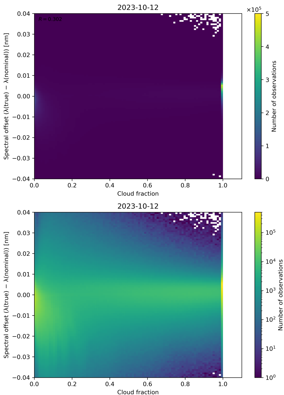
Figure 83: Scatter density plot of “Cloud fraction” against “Spectral offset ( \lambda(\text{true}) - \lambda(\text{nominal}) )” for 2023-10-12 to 2023-10-13.
