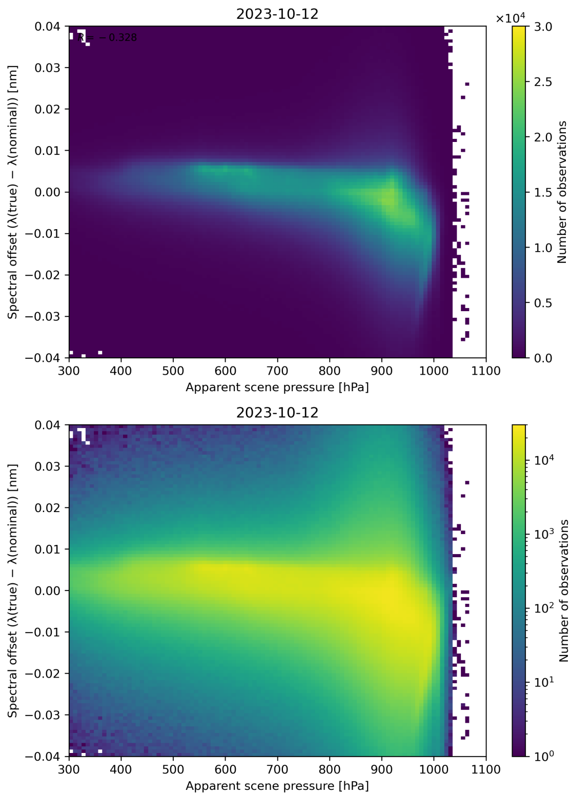
Figure 68: Scatter density plot of “Apparent scene pressure” against “Spectral offset ( \lambda(\text{true}) - \lambda(\text{nominal}) )” for 2023-10-12 to 2023-10-13.
