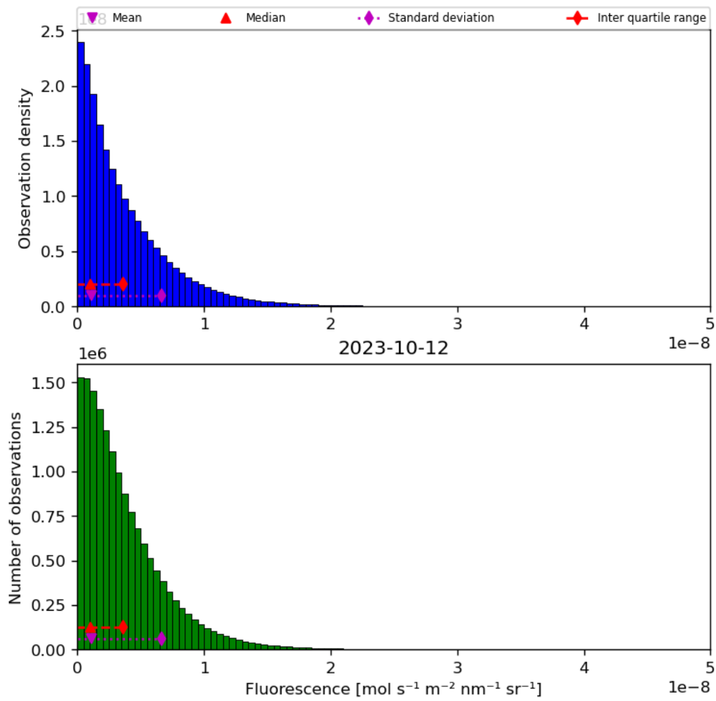
Figure 40: Histogram of “Fluorescence” for 2023-10-12 to 2023-10-13
