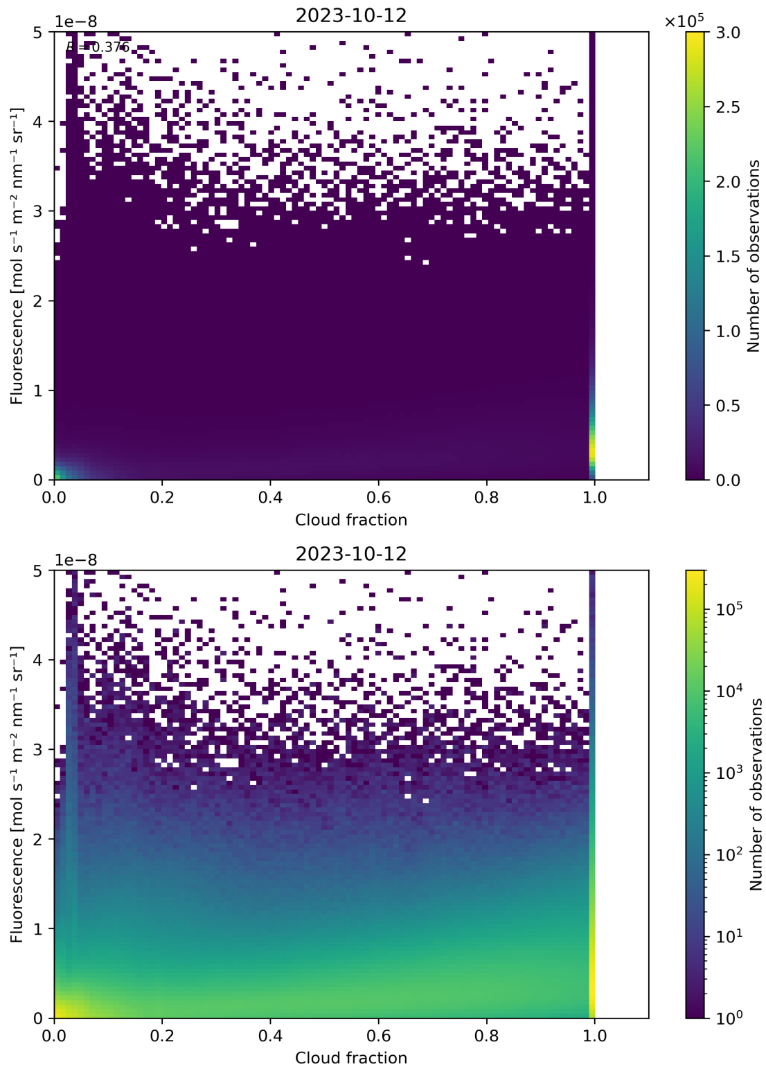
Figure 79: Scatter density plot of “Cloud fraction” against “Fluorescence” for 2023-10-12 to 2023-10-13.
