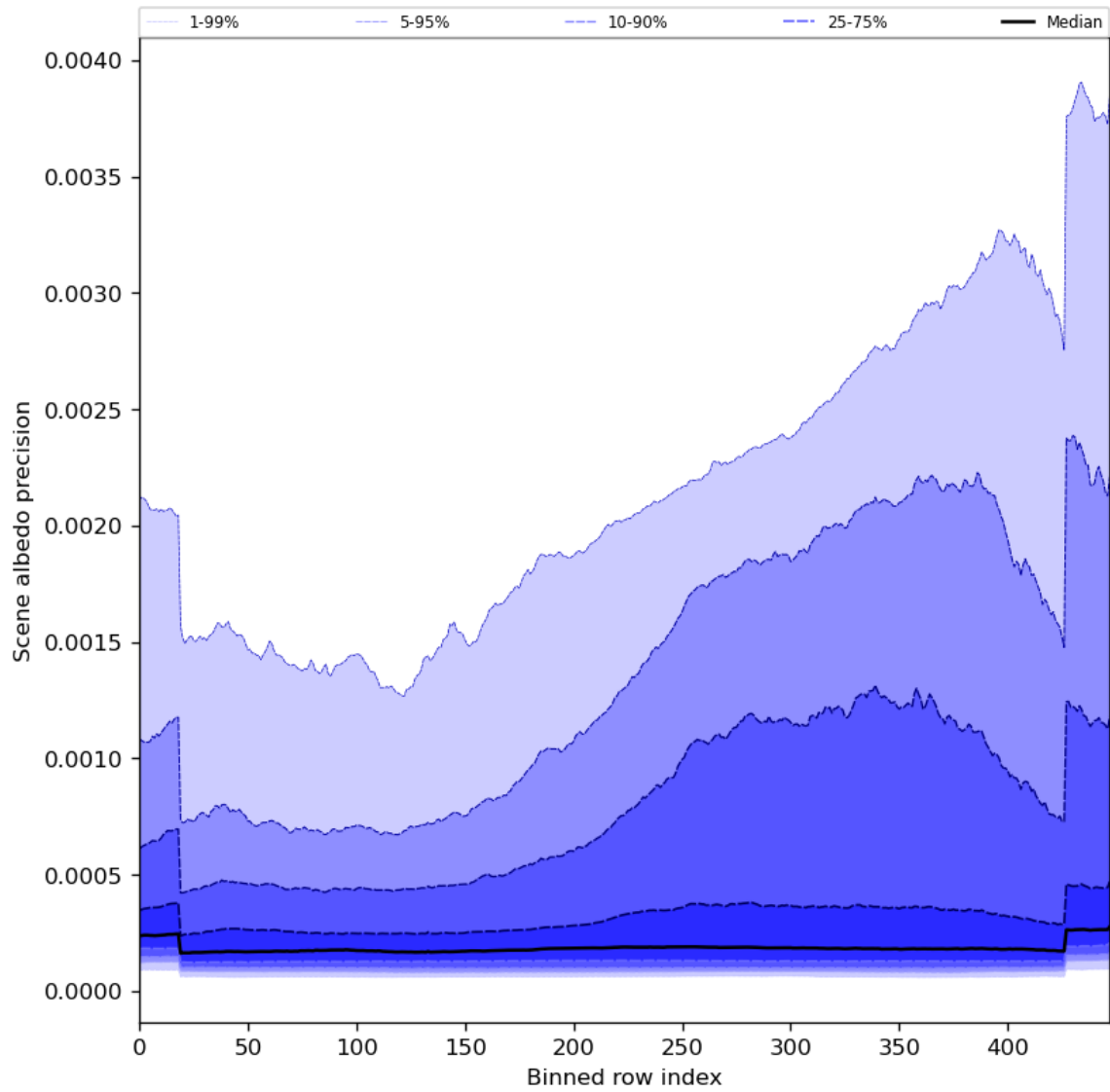
Figure 52: Along track statistics of “Scene albedo precision” for 2023-10-12 to 2023-10-13
