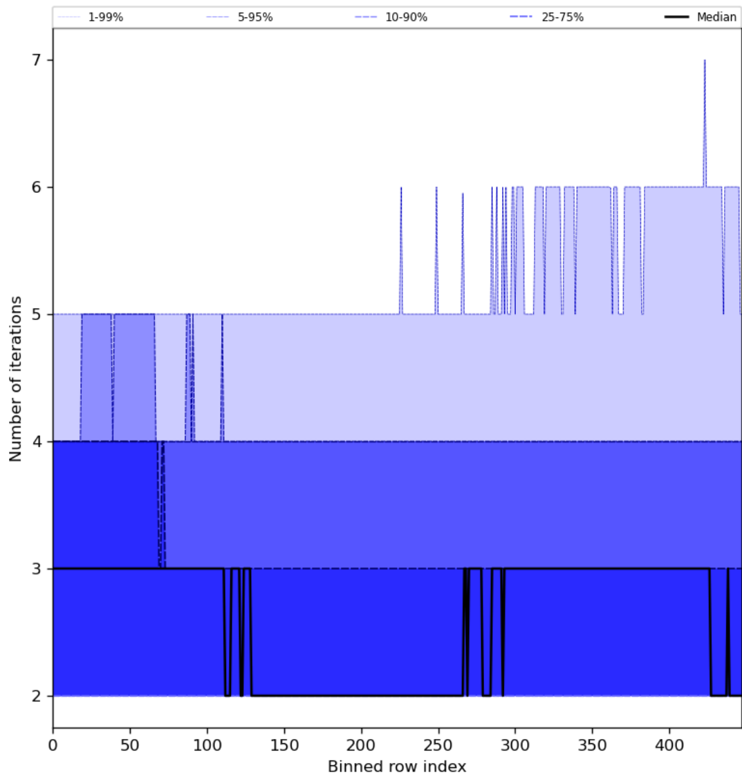
Figure 56: Along track statistics of “Number of iterations” for 2023-10-12 to 2023-10-13
