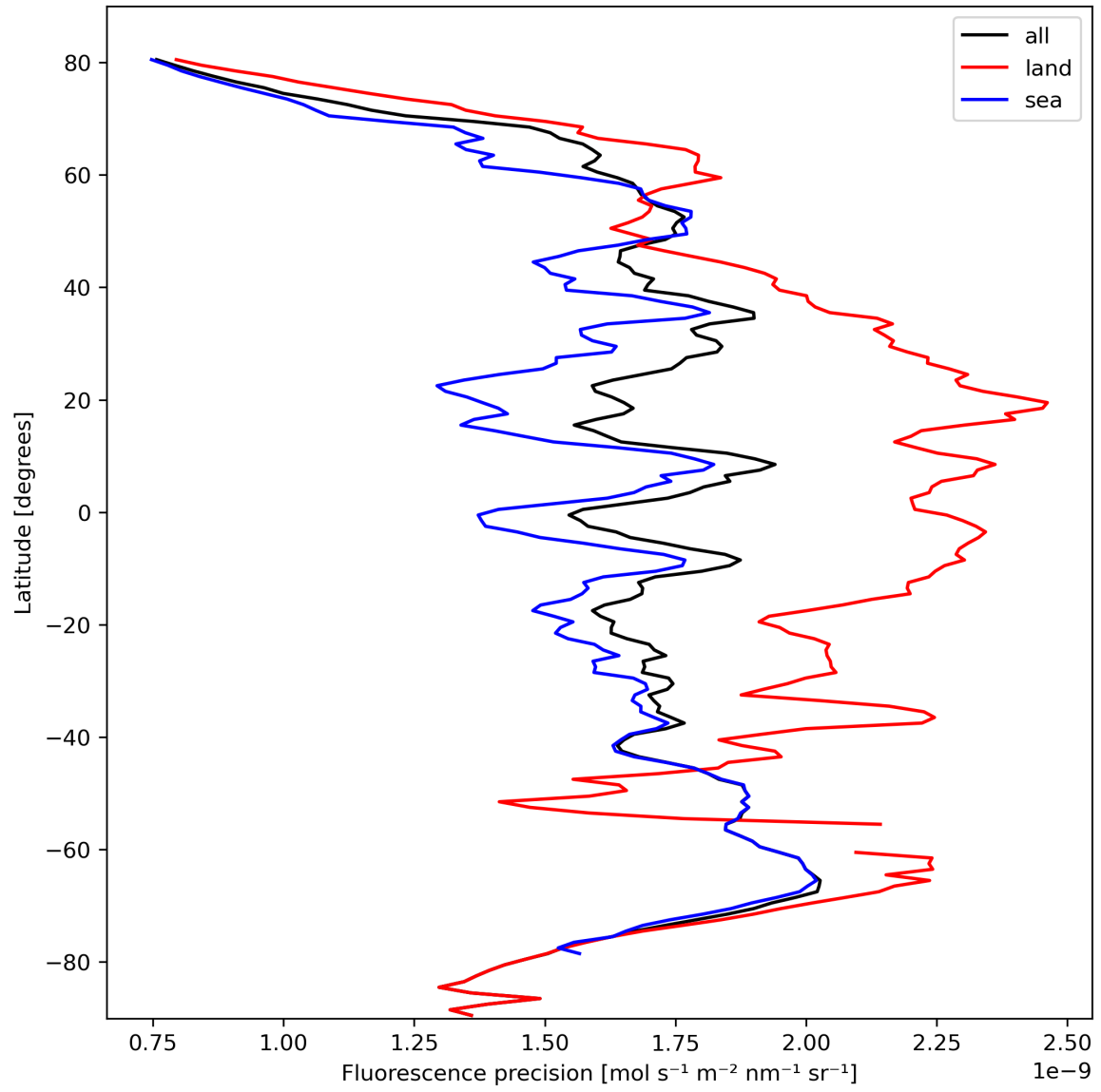
Figure 24: Zonal average of “Fluorescence precision” for 2023-10-12 to 2023-10-13.
