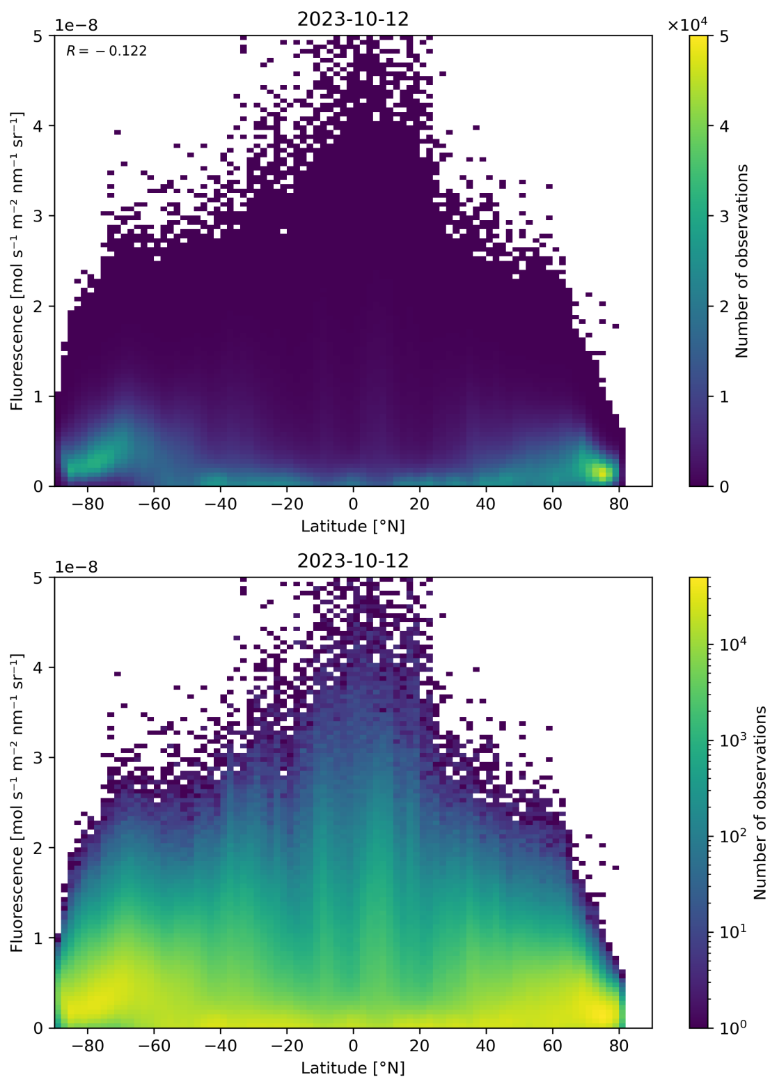
Figure 101: Scatter density plot of “Latitude” against “Fluorescence” for 2023-10-12 to 2023-10-13.
