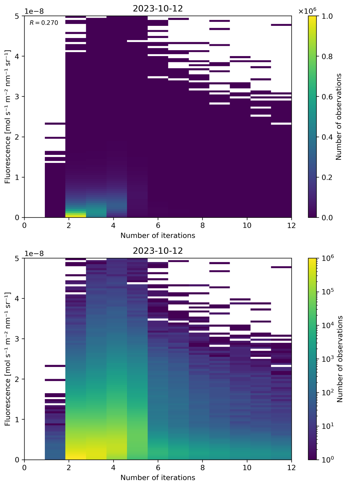
Figure 107: Scatter density plot of “Number of iterations” against “Fluorescence” for 2023-10-12 to 2023-10-13.
