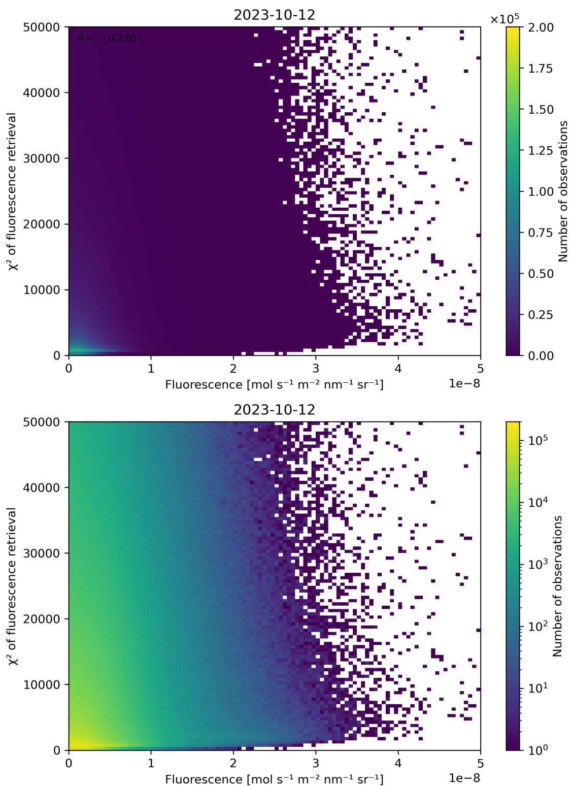
Figure 93: Scatter density plot of “Fluorescence” against “ \chi^2 of fluorescence retrieval” for 2023-10-12 to 2023-10-13.
