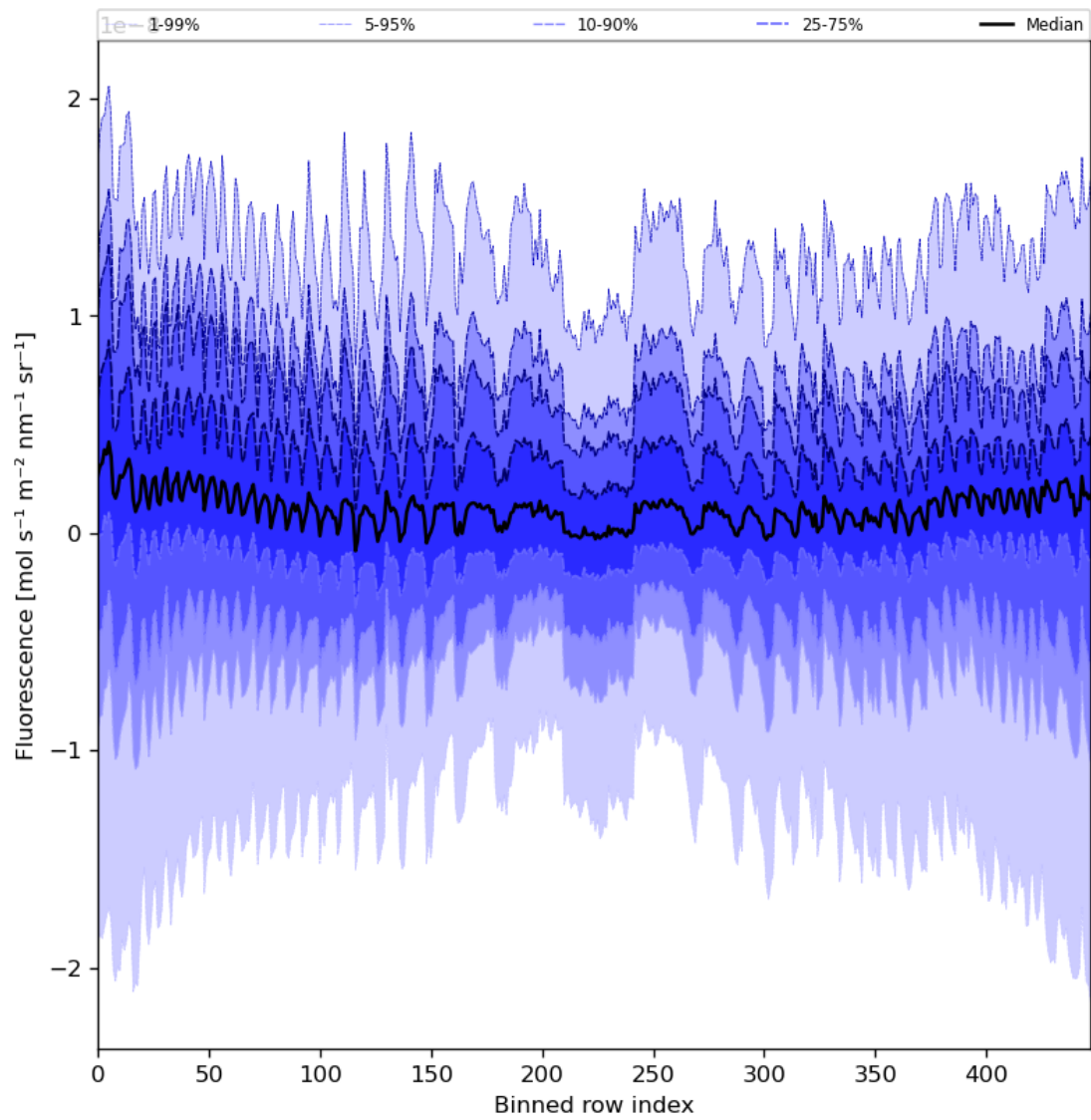
Figure 57: Along track statistics of "Fluorescence" for 2023-10-12 to 2023-10-13
