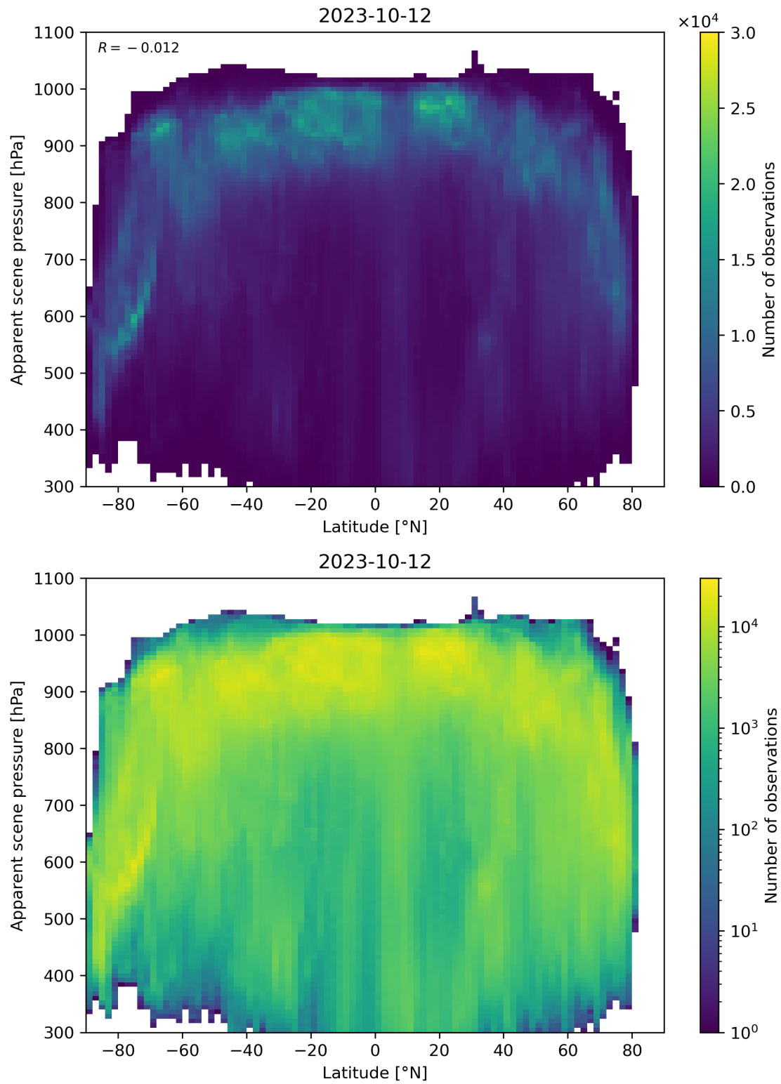
Figure 96: Scatter density plot of “Latitude” against “Apparent scene pressure” for 2023-10-12 to 2023-10-13.
