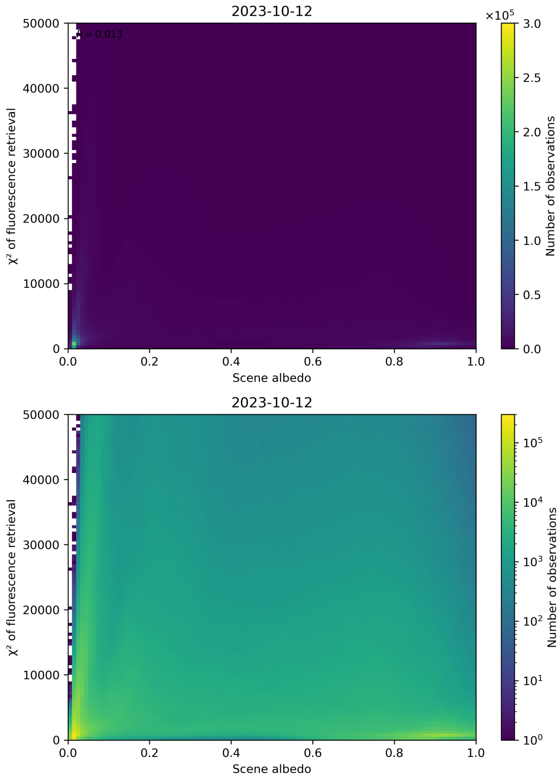
Figure 113: Scatter density plot of “Scene albedo” against “ \chi^2 of fluorescence retrieval” for 2023-10-12 to 2023-10-13.
