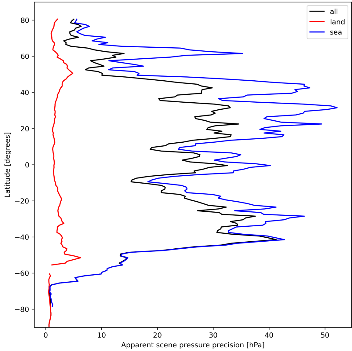
Figure 20: Zonal average of “Apparent scene pressure precision” for 2023-10-12 to 2023-10-13.
