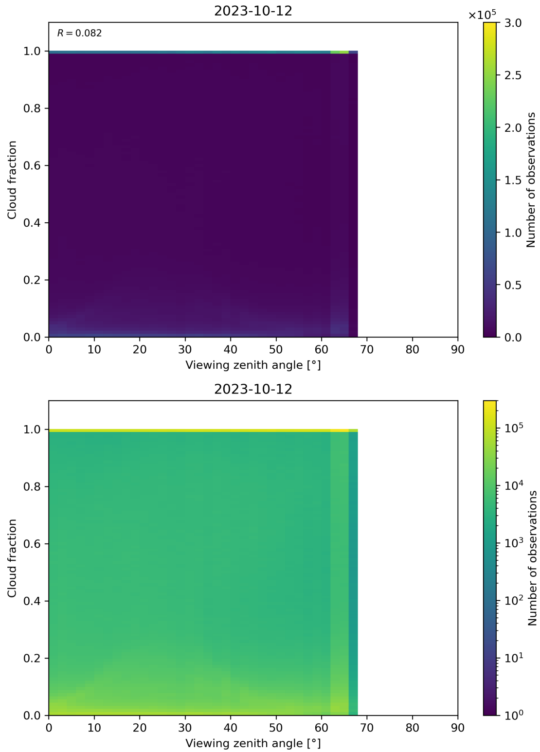
Figure 132: Scatter density plot of “Viewing zenith angle” against “Cloud fraction” for 2023-10-12 to 2023-10-13.
