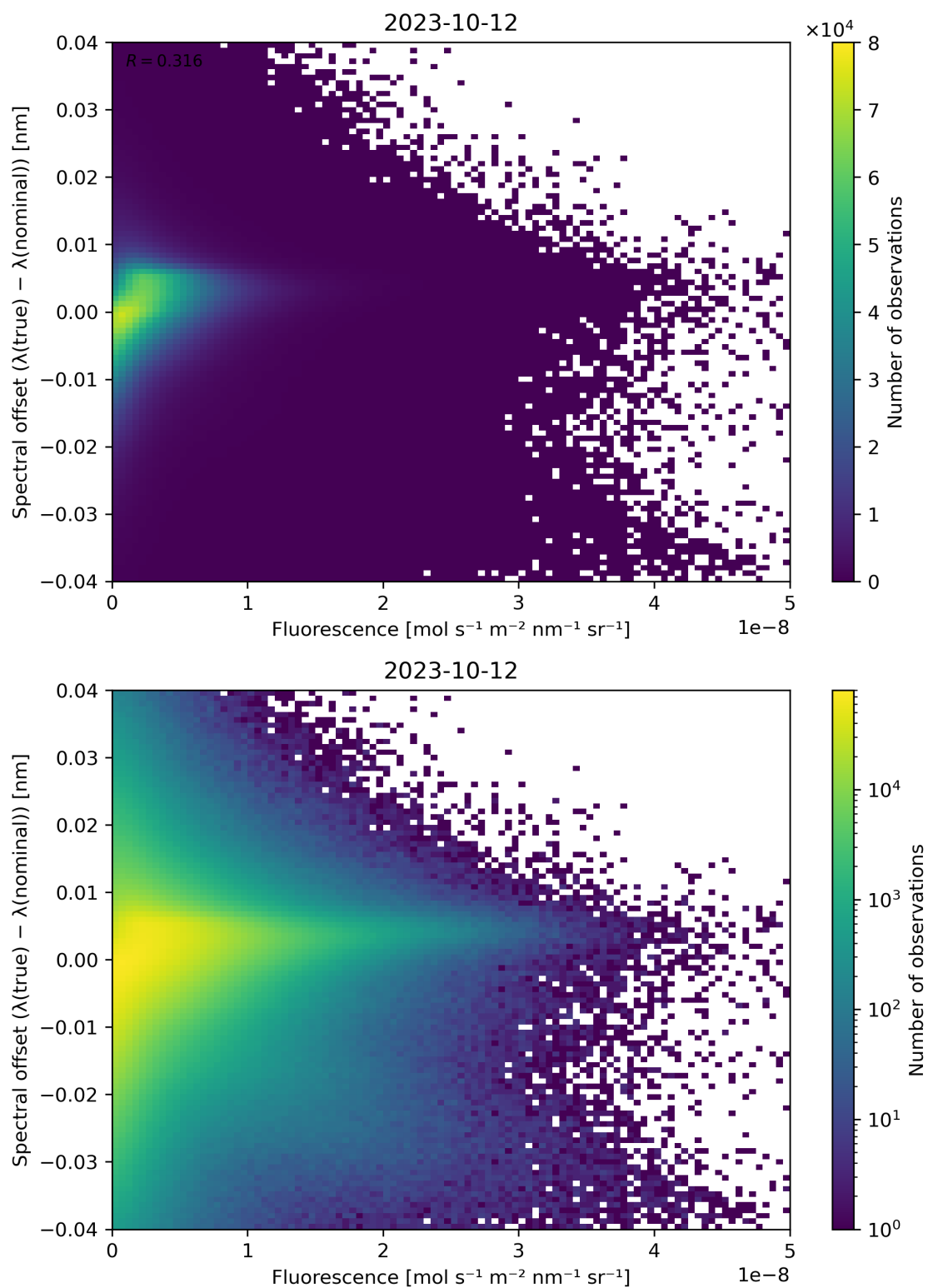
Figure 95: Scatter density plot of “Fluorescence” against “Spectral offset ( \lambda(\text{true}) - \lambda(\text{nominal}) )” for 2023-10-12 to 2023-10-13.
