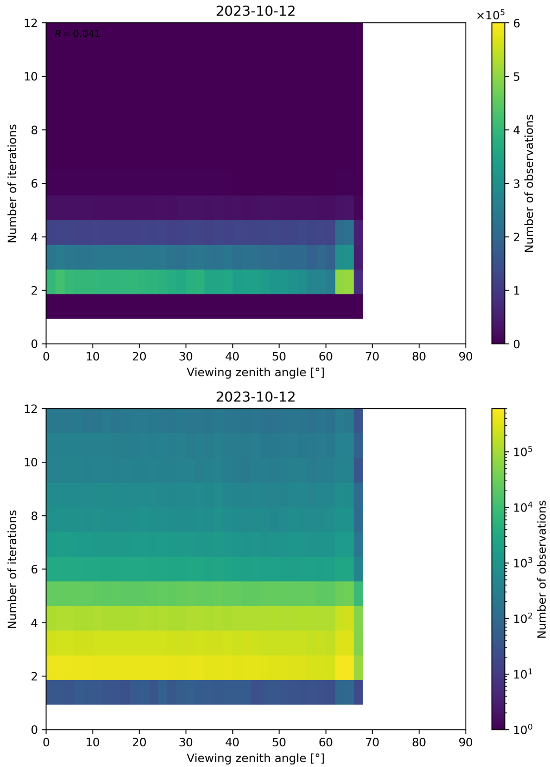
Figure 136: Scatter density plot of “Viewing zenith angle” against “Number of iterations” for 2023-10-12 to 2023-10-13.
