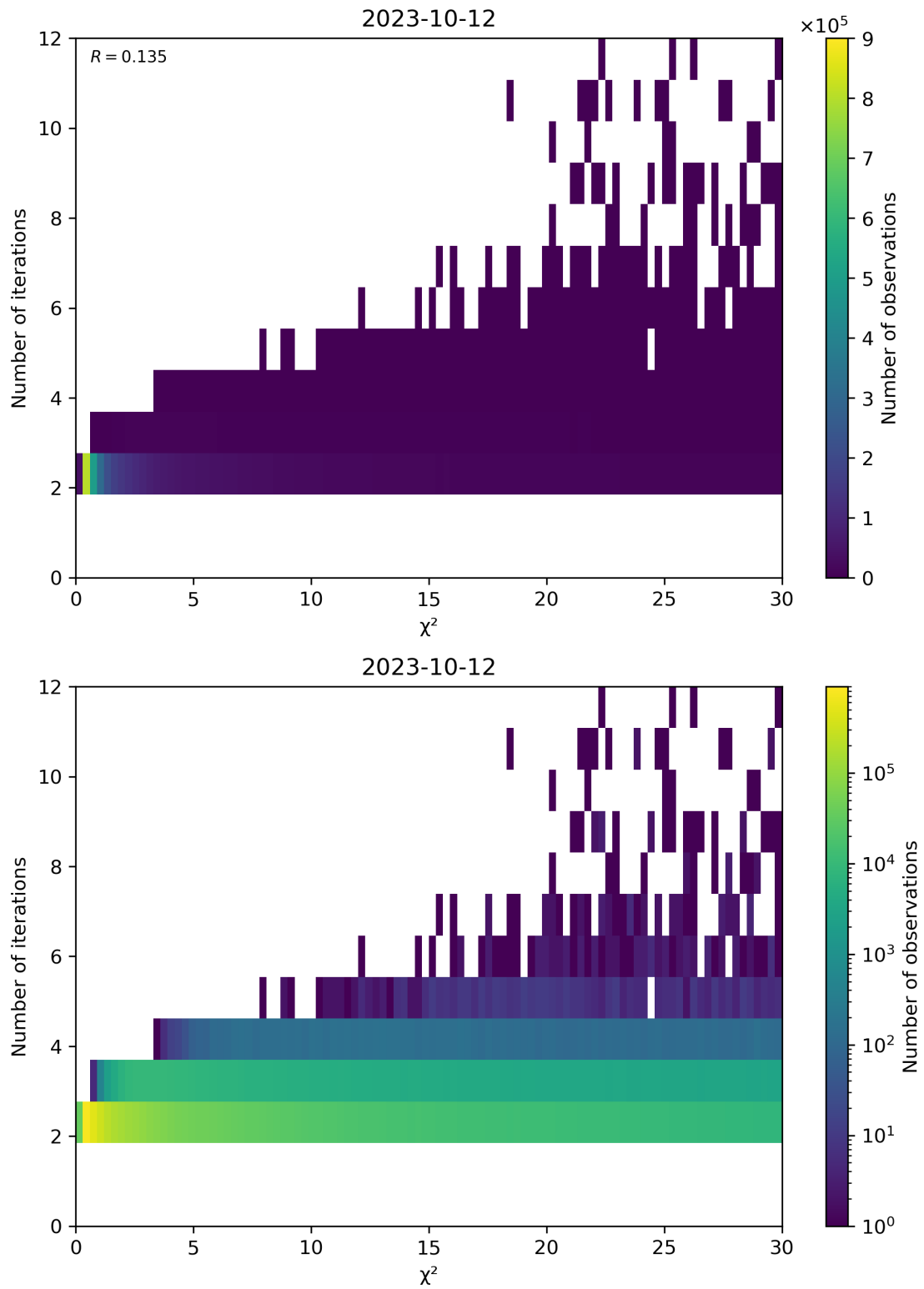
Figure 73: Scatter density plot of " \chi^2 " against "Number of iterations" for 2023-10-12 to 2023-10-13.
