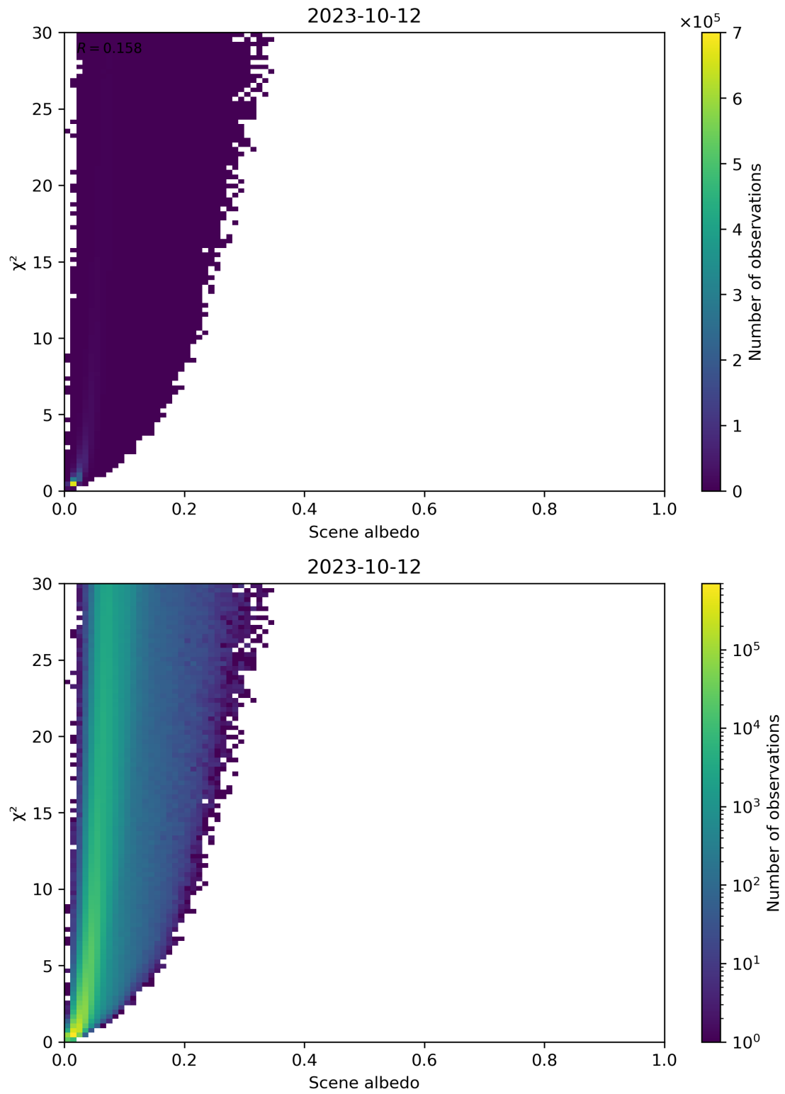
Figure 112: Scatter density plot of “Scene albedo” against “ \chi^2 ” for 2023-10-12 to 2023-10-13.
