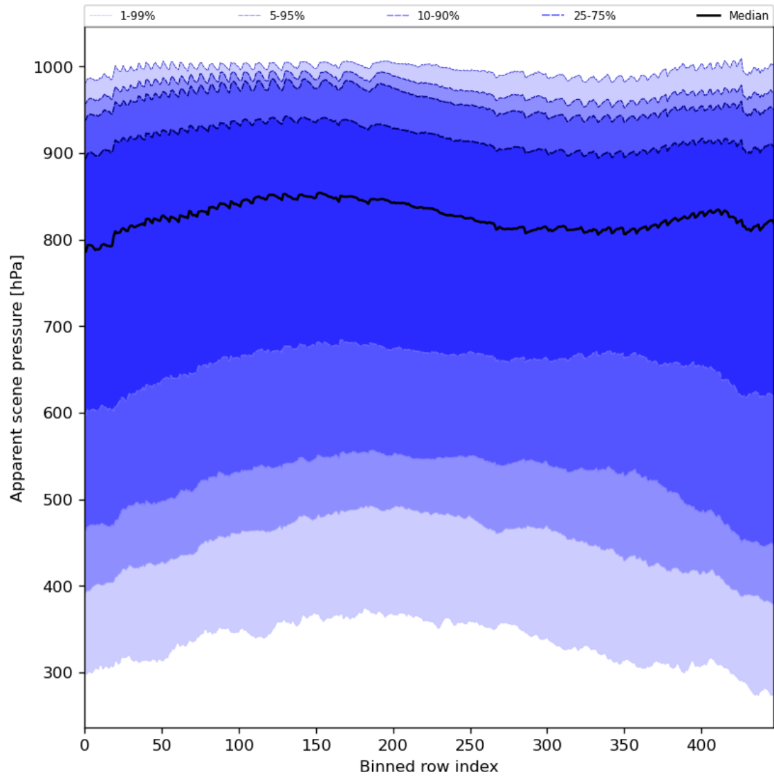
Figure 53: Along track statistics of “Apparent scene pressure” for 2023-10-12 to 2023-10-13
