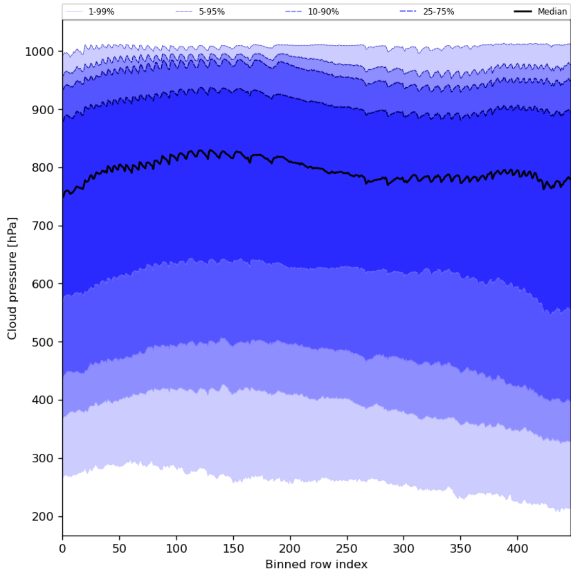
Figure 47: Along track statistics of “Cloud pressure” for 2023-10-12 to 2023-10-13
