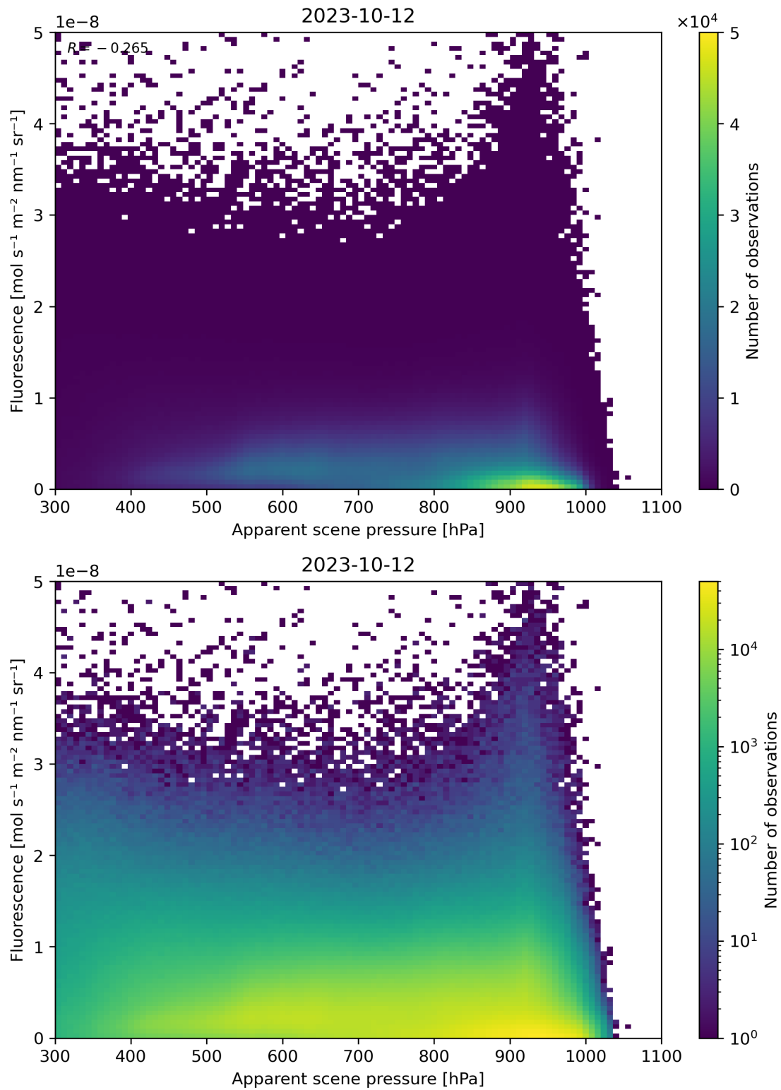
Figure 65: Scatter density plot of “Apparent scene pressure” against “Fluorescence” for 2023-10-12 to 2023-10-13.
