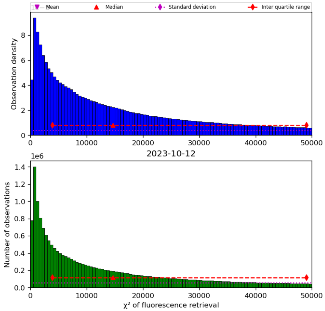
Figure 42: Histogram of “ \chi^2 of fluorescence retrieval” for 2023-10-12 to 2023-10-13
