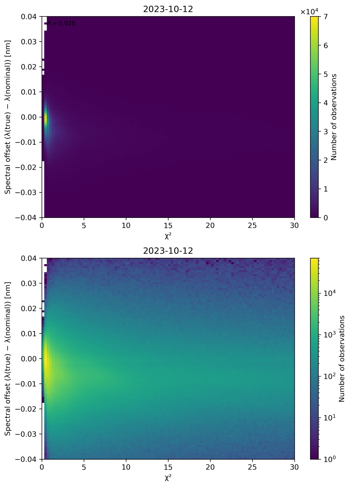
Figure 75: Scatter density plot of " \chi^2 " against "Spectral offset ( \lambda(\text{true}) - \lambda(\text{nominal}) )" for 2023-10-12 to 2023-10-13.
