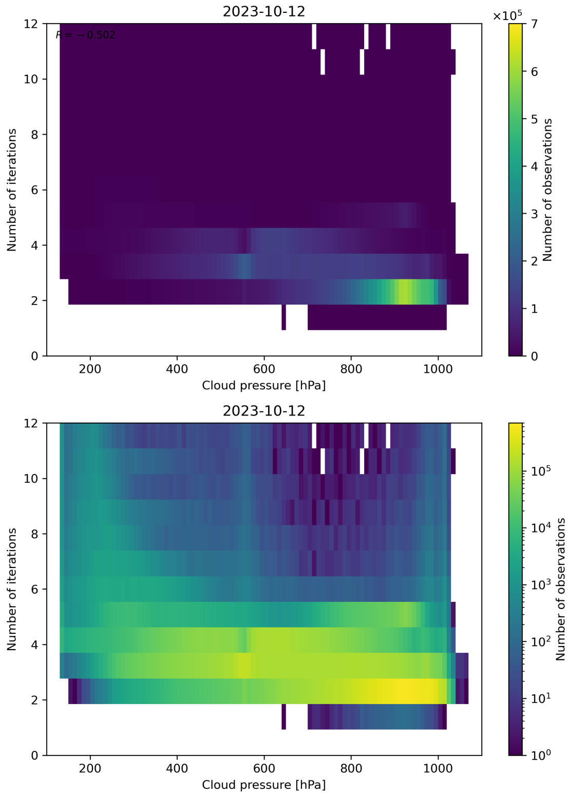
Figure 89: Scatter density plot of “Cloud pressure” against “Number of iterations” for 2023-10-12 to 2023-10-13.
