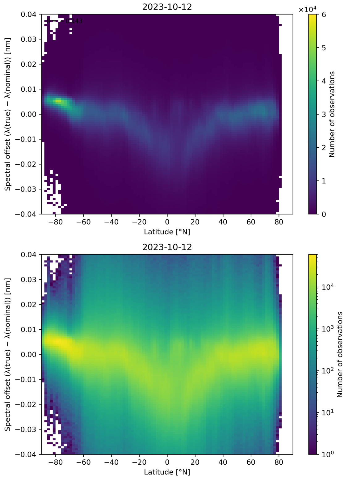
Figure 105: Scatter density plot of “Latitude” against “Spectral offset ( \lambda(\text{true}) - \lambda(\text{nominal}) )” for 2023-10-12 to 2023-10-13.
