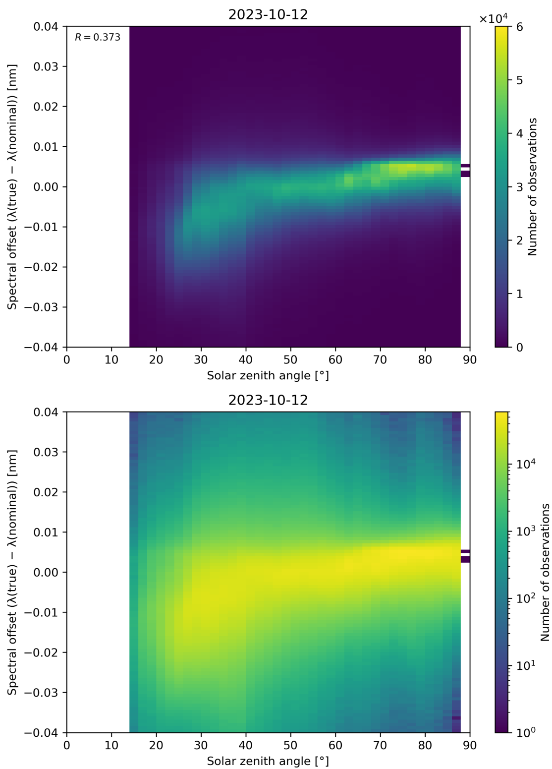
Figure 128: Scatter density plot of “Solar zenith angle” against “Spectral offset ( \lambda(\text{true}) - \lambda(\text{nominal}) )” for 2023-10-12 to 2023-10-13.
