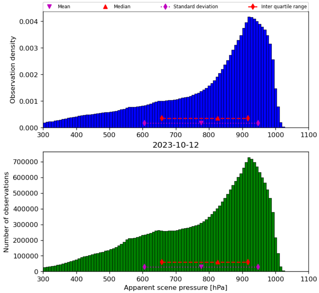
Figure 36: Histogram of “Apparent scene pressure” for 2023-10-12 to 2023-10-13
