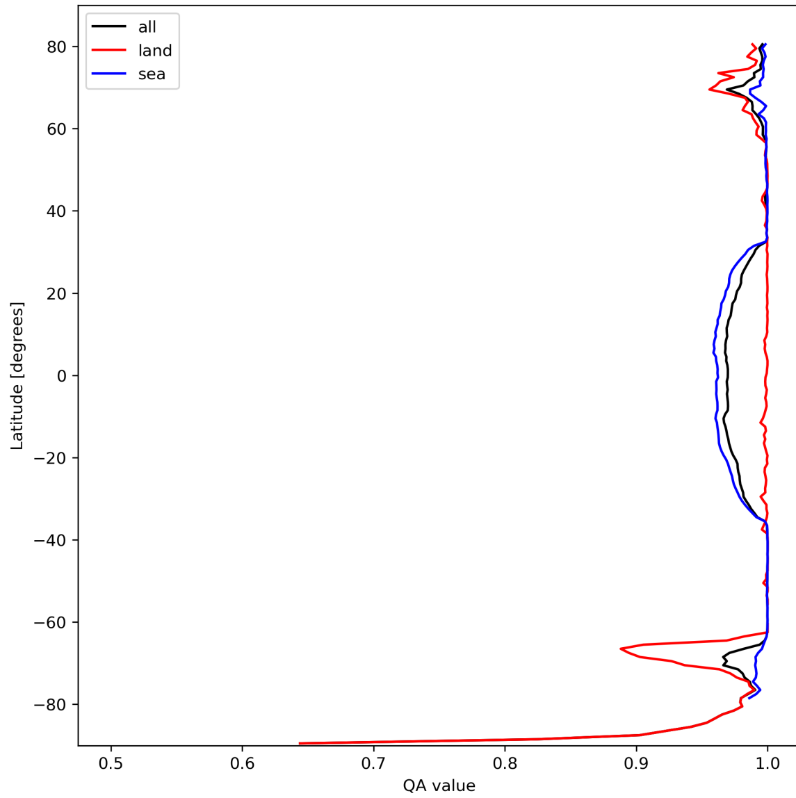
Figure 12: Zonal average of “QA value” for 2023-10-12 to 2023-10-13.
