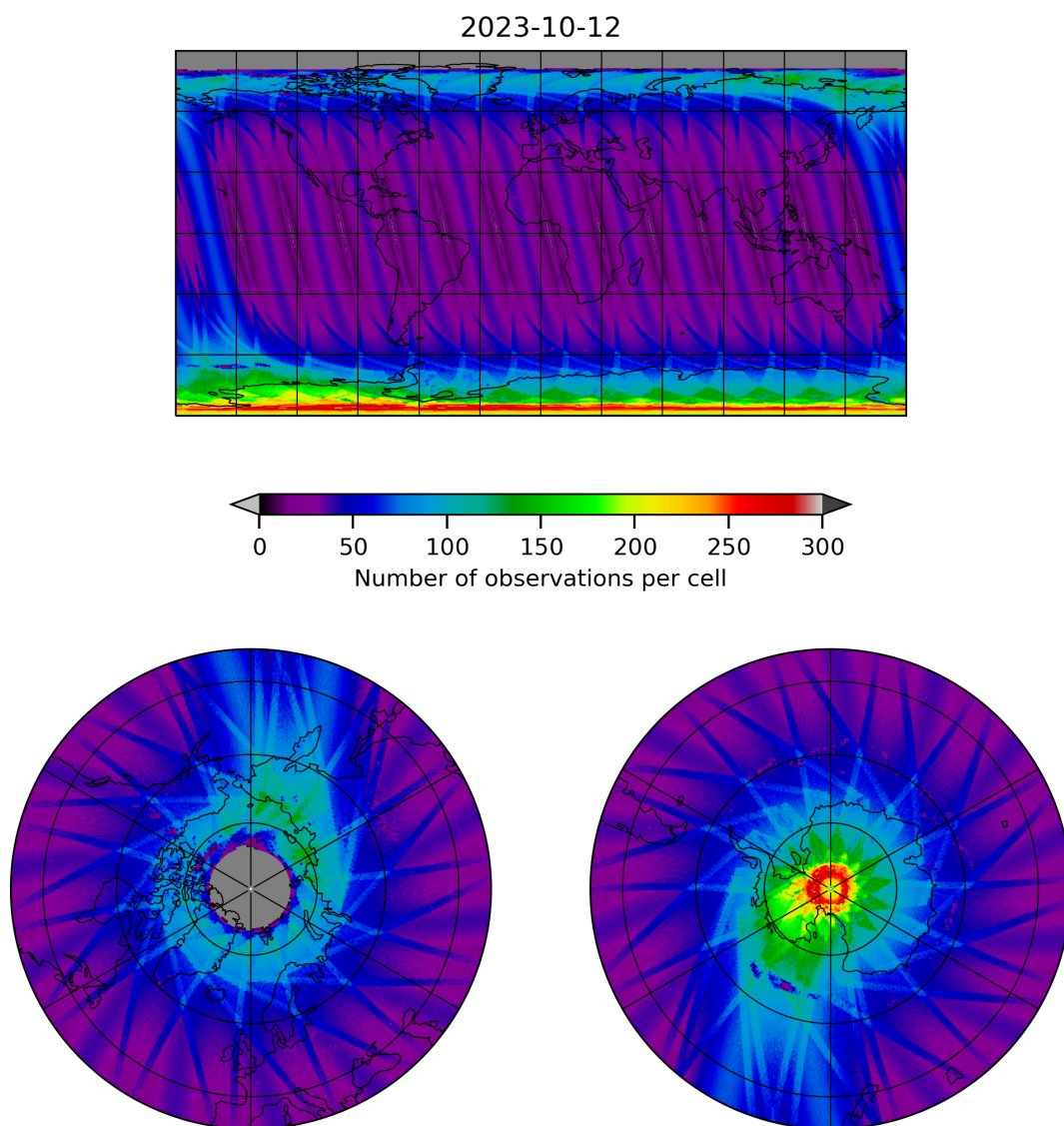
Figure 11: Map of the number of observations for 2023-10-12 to 2023-10-13
