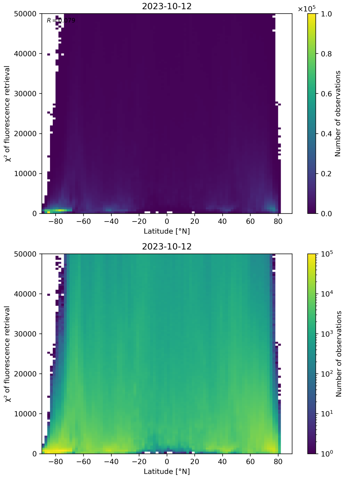
Figure 98: Scatter density plot of “Latitude” against “ \chi^2 of fluorescence retrieval” for 2023-10-12 to 2023-10-13.
