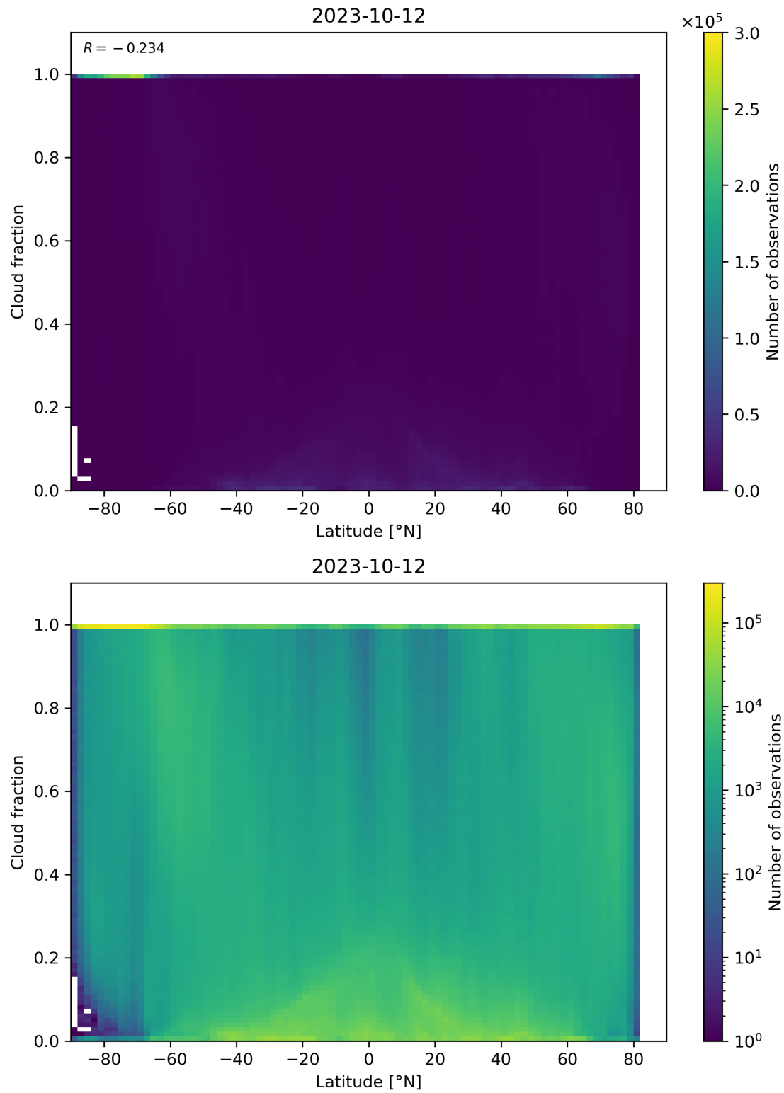
Figure 99: Scatter density plot of “Latitude” against “Cloud fraction” for 2023-10-12 to 2023-10-13.
