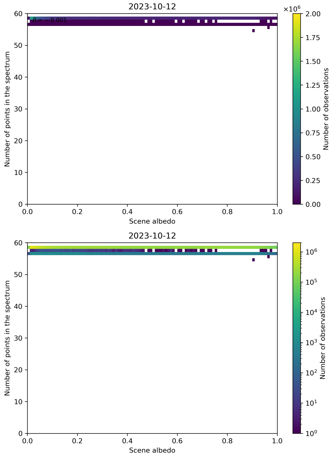
Figure 116: Scatter density plot of “Scene albedo” against “Number of points in the spectrum” for 2023-10-12 to 2023-10-13.
