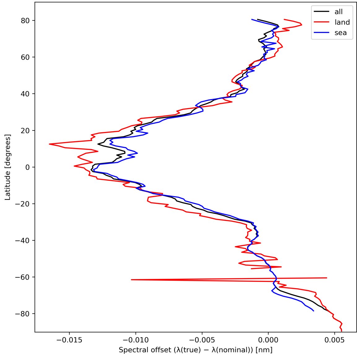
Figure 28: Zonal average of “Spectral offset ( \lambda(\text{true}) - \lambda(\text{nominal}) )” for 2023-10-12 to 2023-10-13.
