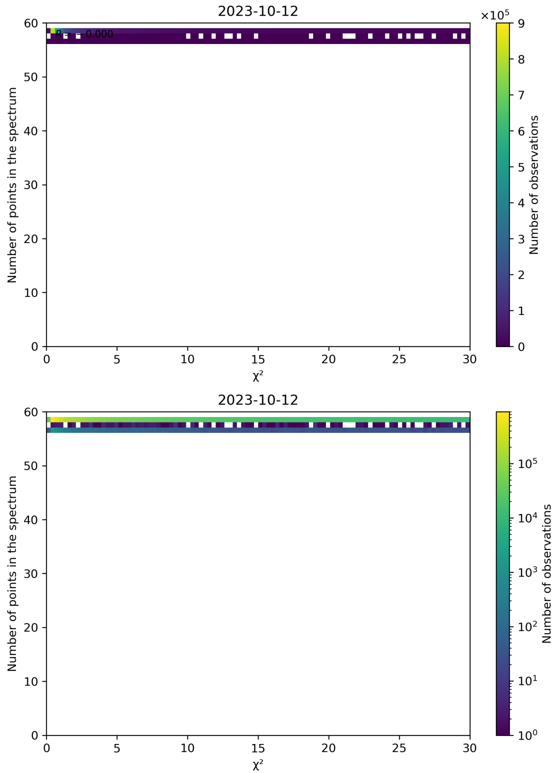
Figure 74: Scatter density plot of " \chi^2 " against "Number of points in the spectrum" for 2023-10-12 to 2023-10-13.
