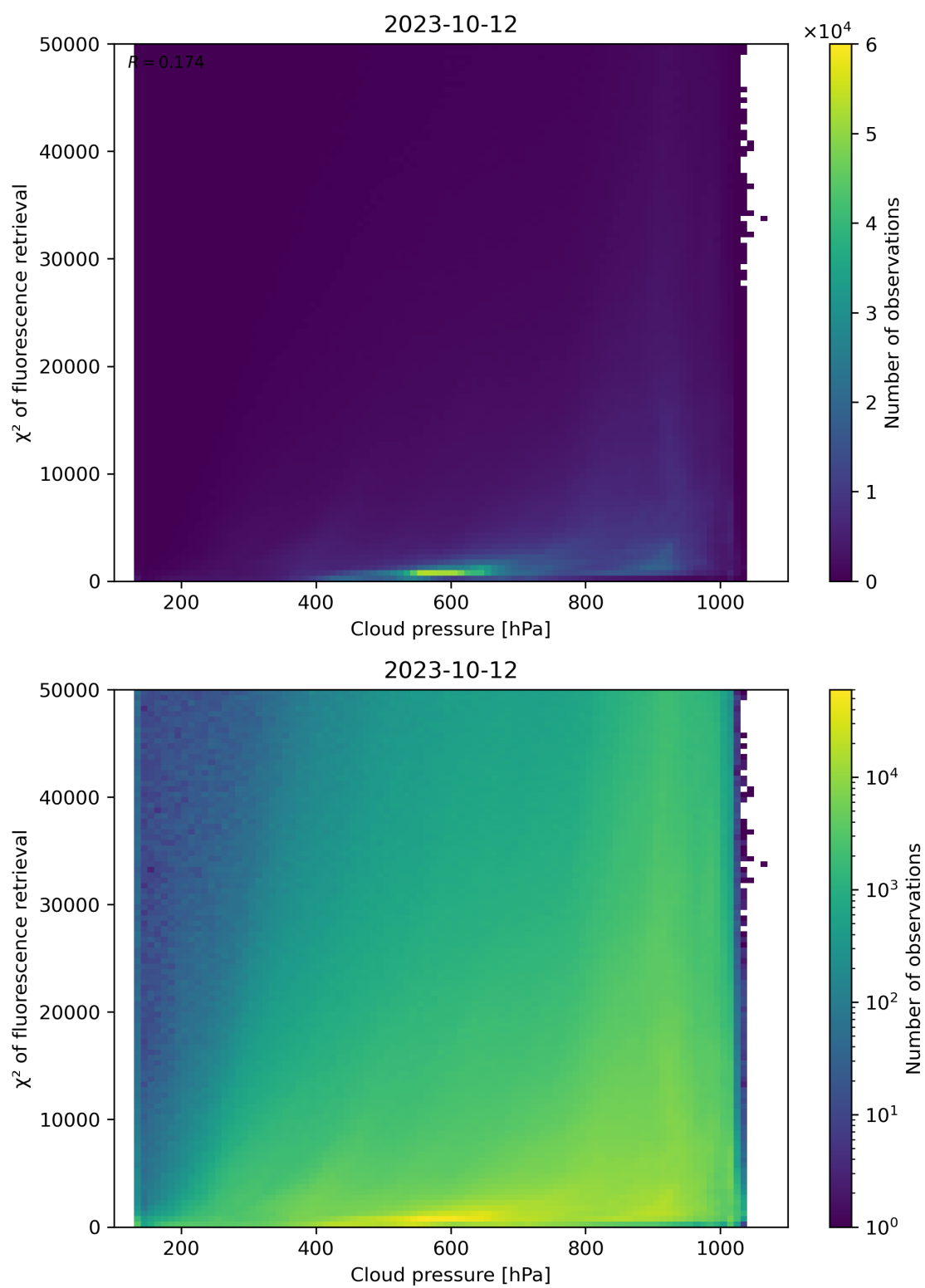
Figure 86: Scatter density plot of “Cloud pressure” against “ \chi^2 of fluorescence retrieval” for 2023-10-12 to 2023-10-13.
