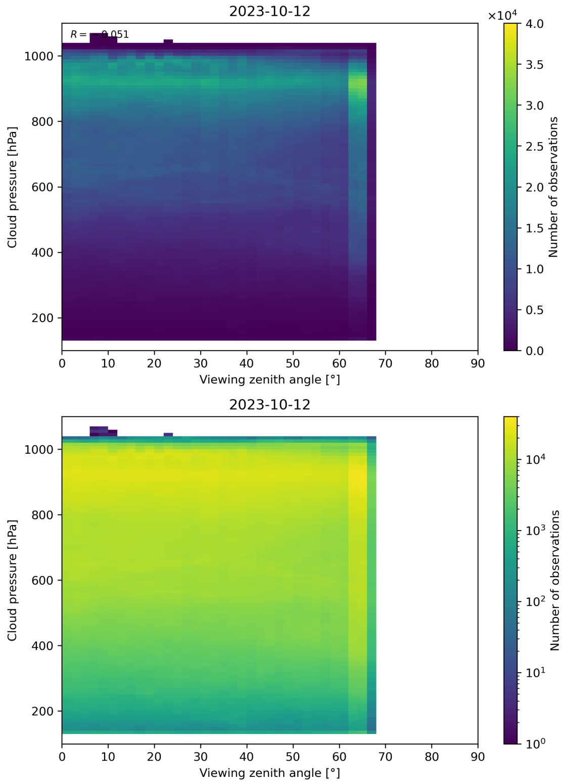
Figure 133: Scatter density plot of “Viewing zenith angle” against “Cloud pressure” for 2023-10-12 to 2023-10-13.
