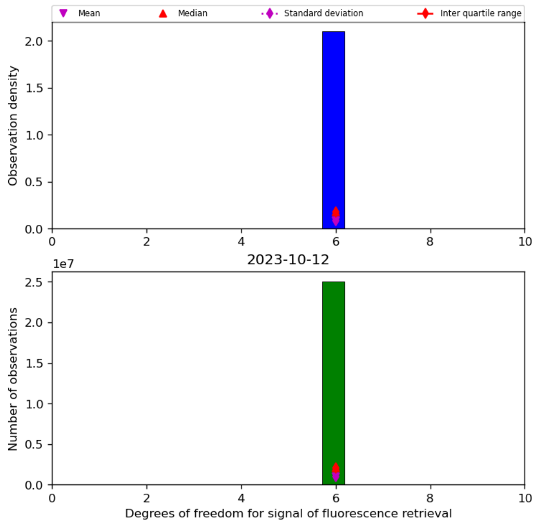
Figure 43: Histogram of “Degrees of freedom for signal of fluorescence retrieval” for 2023-10-12 to 2023-10-13
