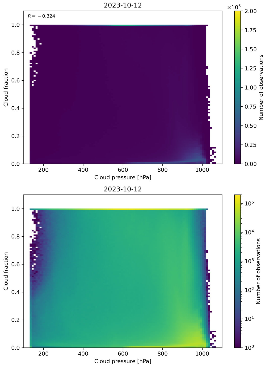
Figure 87: Scatter density plot of “Cloud pressure” against “Cloud fraction” for 2023-10-12 to 2023-10-13.
