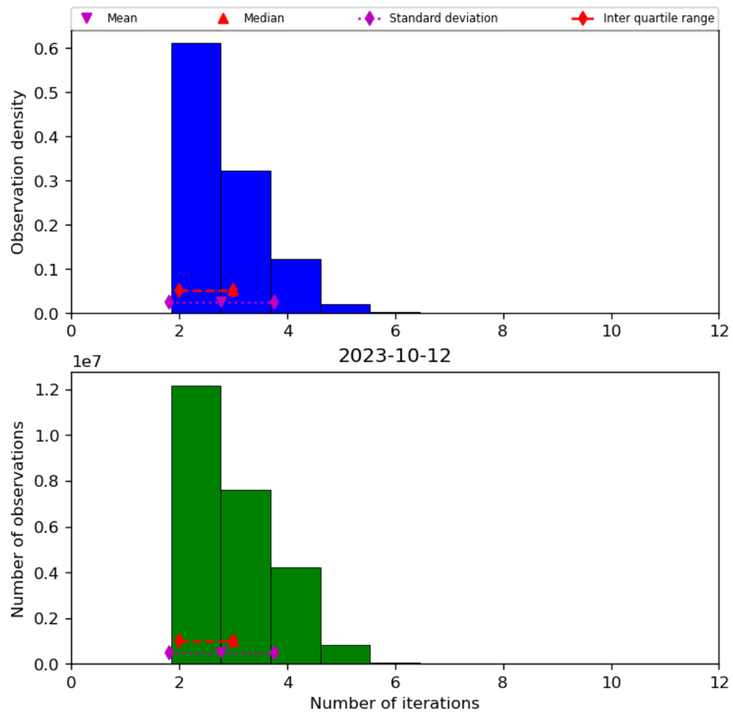
Figure 39: Histogram of “Number of iterations” for 2023-10-12 to 2023-10-13
