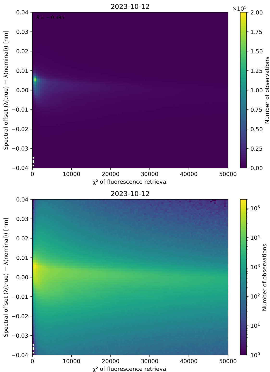
Figure 72: Scatter density plot of " \chi^2 of fluorescence retrieval" against "Spectral offset ( \lambda(\text{true}) - \lambda(\text{nominal})) " for 2023-10-12 to 2023-10-13.
