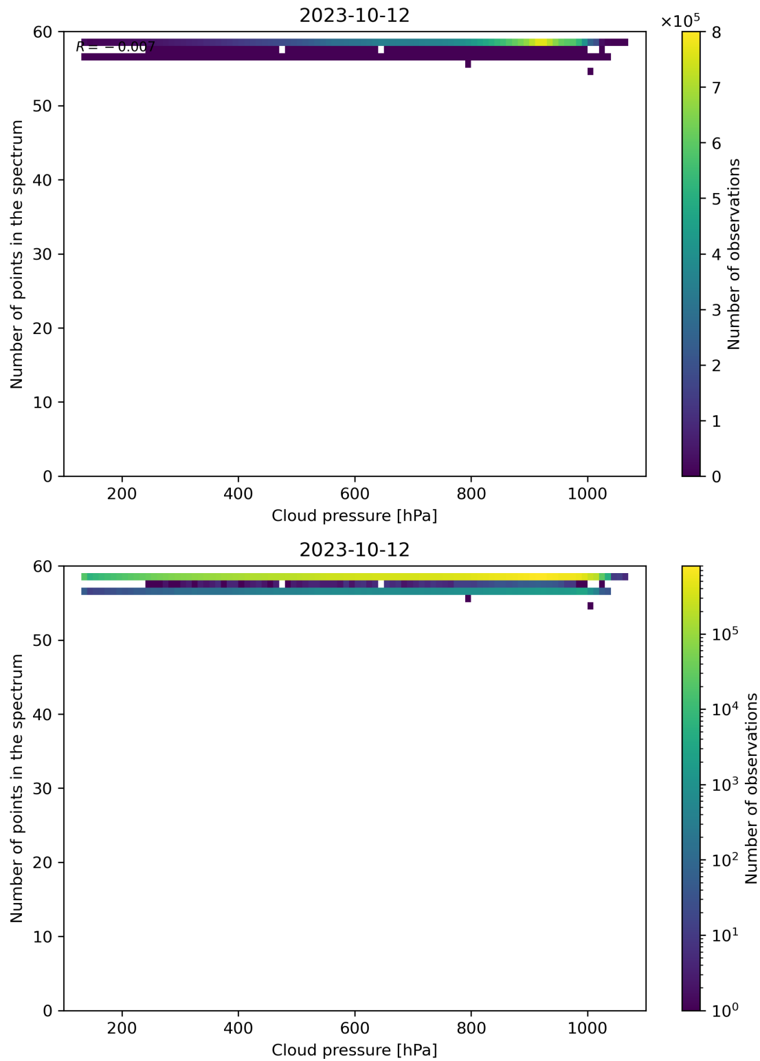
Figure 90: Scatter density plot of “Cloud pressure” against “Number of points in the spectrum” for 2023-10-12 to 2023-10-13.
