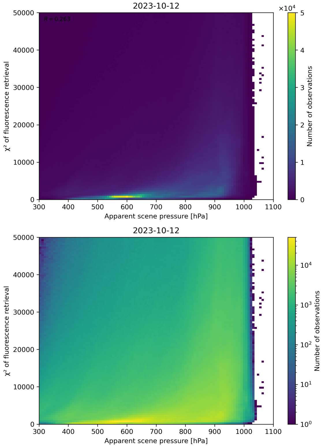
Figure 64: Scatter density plot of “Apparent scene pressure” against “ \chi^2 of fluorescence retrieval” for 2023-10-12 to 2023-10-13.
