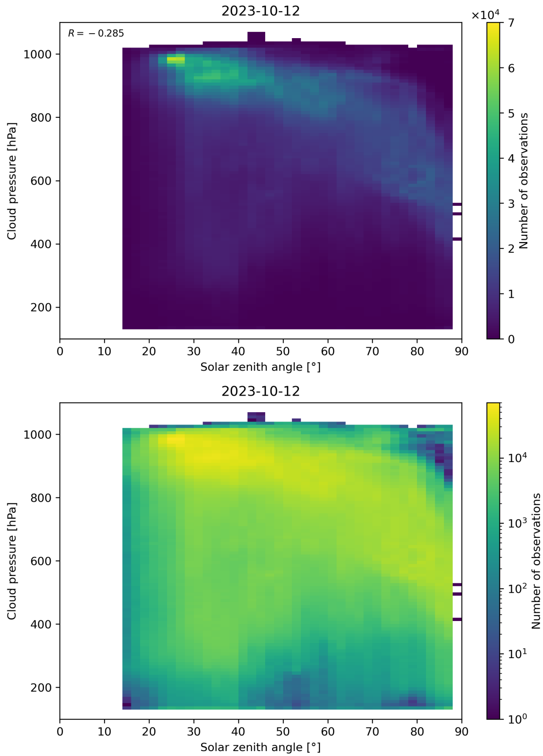
Figure 122: Scatter density plot of “Solar zenith angle” against “Cloud pressure” for 2023-10-12 to 2023-10-13.
