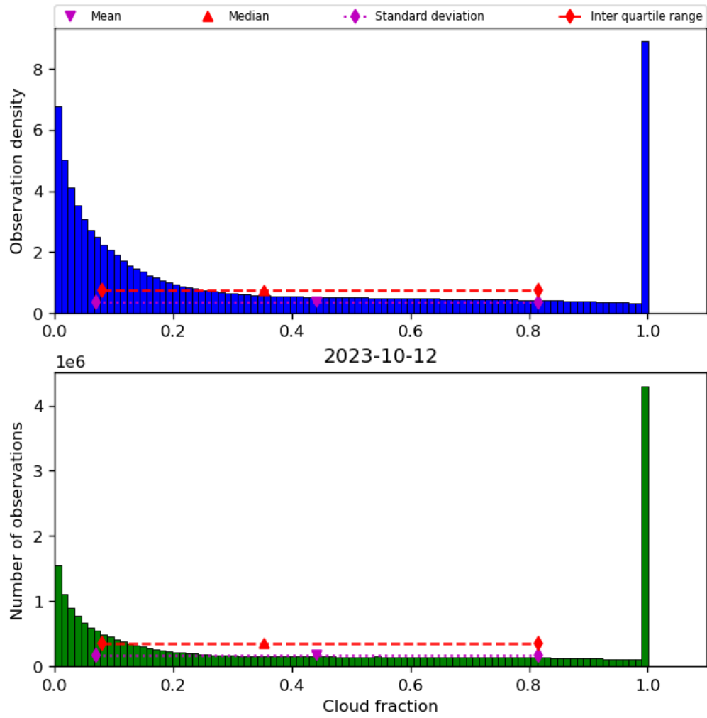
Figure 32: Histogram of “Cloud fraction” for 2023-10-12 to 2023-10-13
