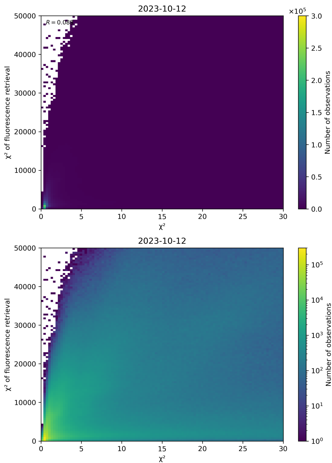
Figure 69: Scatter density plot of “ \chi^2 ” against “ \chi^2 of fluorescence retrieval” for 2023-10-12 to 2023-10-13.
