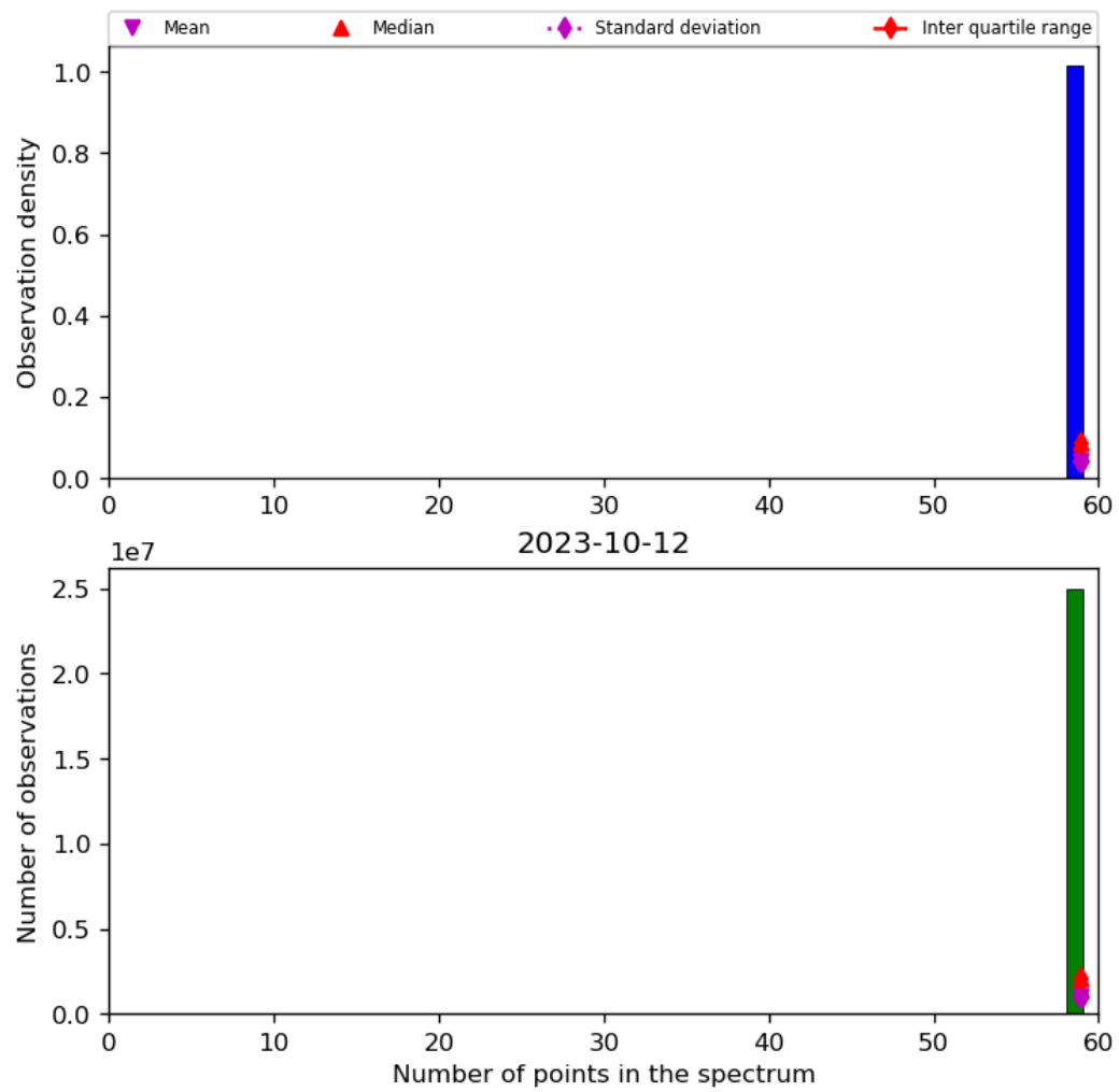
Figure 44: Histogram of “Number of points in the spectrum” for 2023-10-12 to 2023-10-13
