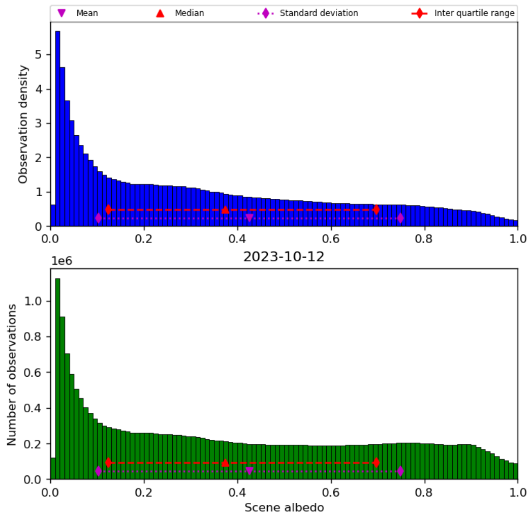
Figure 34: Histogram of “Scene albedo” for 2023-10-12 to 2023-10-13
