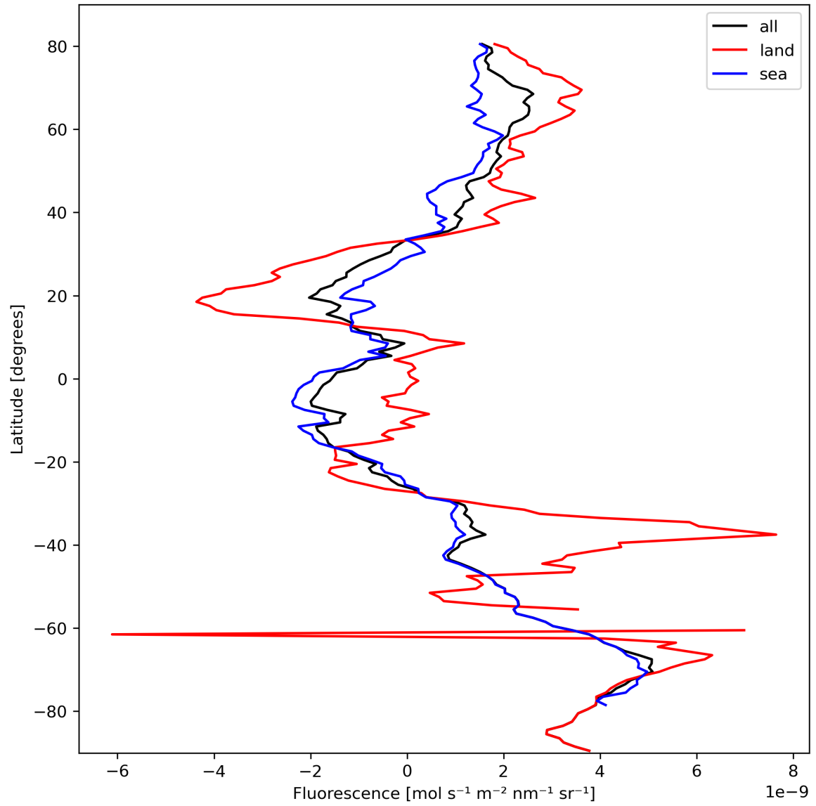
Figure 23: Zonal average of “Fluorescence” for 2023-10-12 to 2023-10-13.
