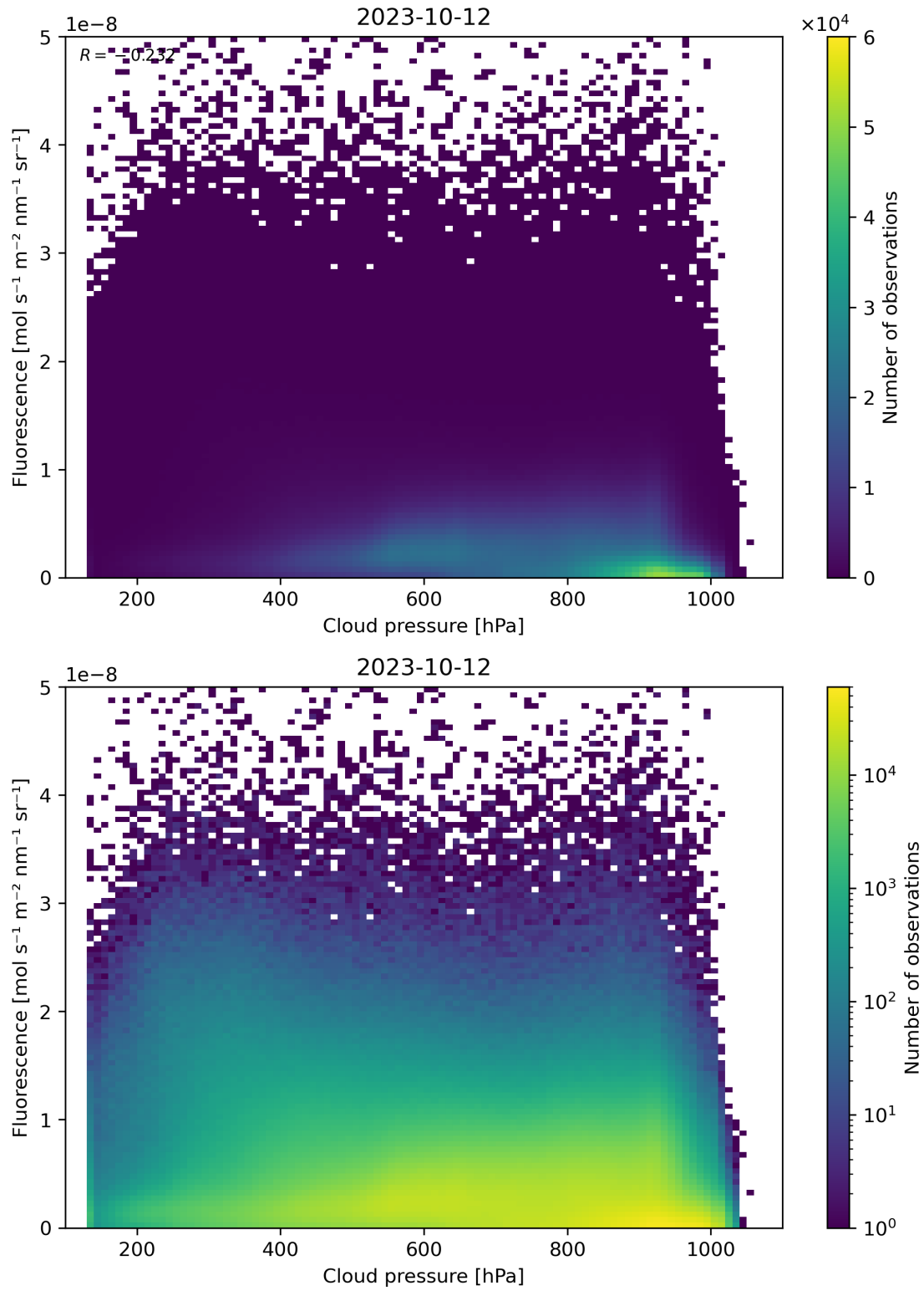
Figure 88: Scatter density plot of “Cloud pressure” against “Fluorescence” for 2023-10-12 to 2023-10-13.
