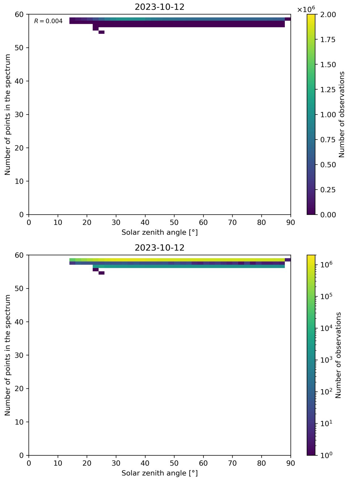
Figure 126: Scatter density plot of “Solar zenith angle” against “Number of points in the spectrum” for 2023-10-12 to 2023-10-13.
