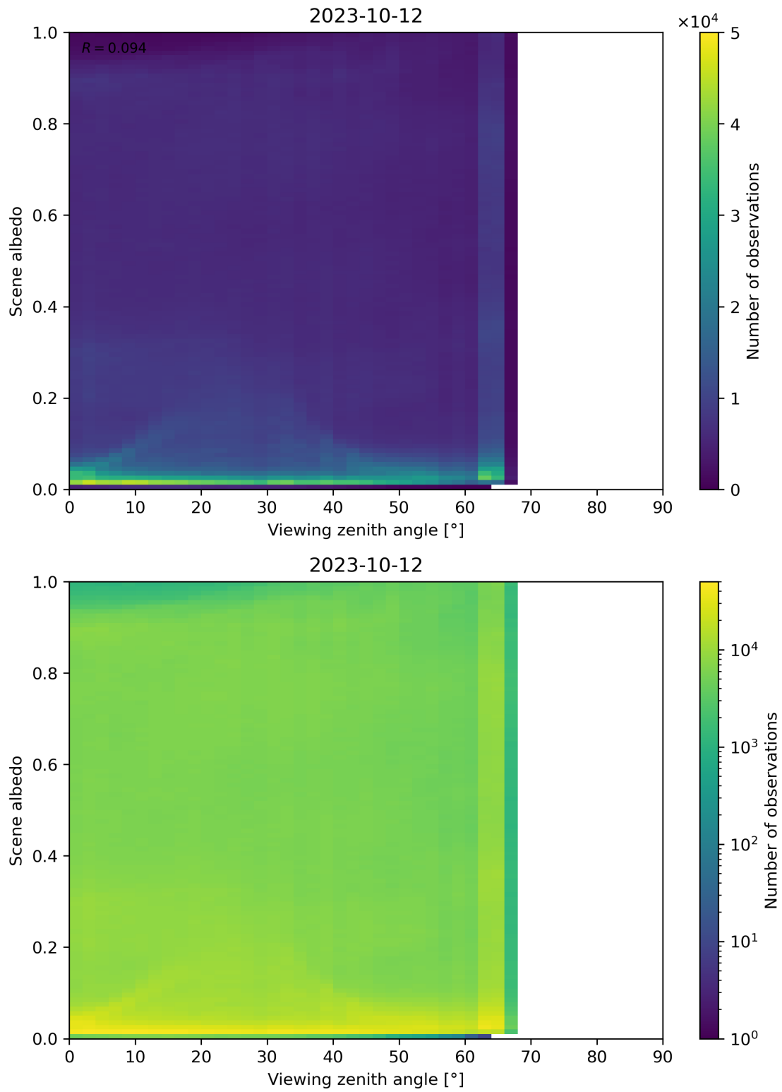
Figure 138: Scatter density plot of “Viewing zenith angle” against “Scene albedo” for 2023-10-12 to 2023-10-13.
