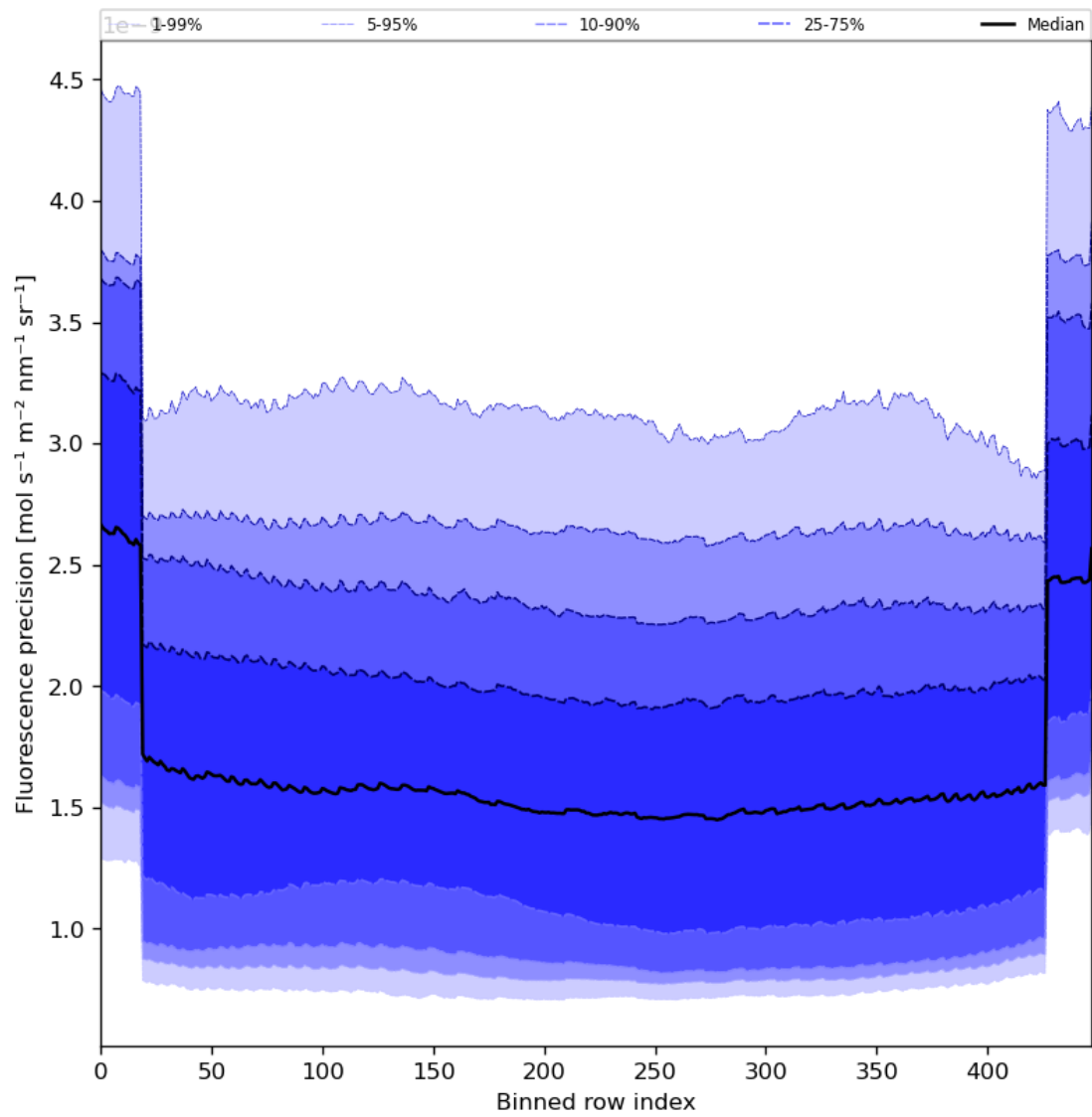
Figure 58: Along track statistics of “Fluorescence precision” for 2023-10-12 to 2023-10-13
