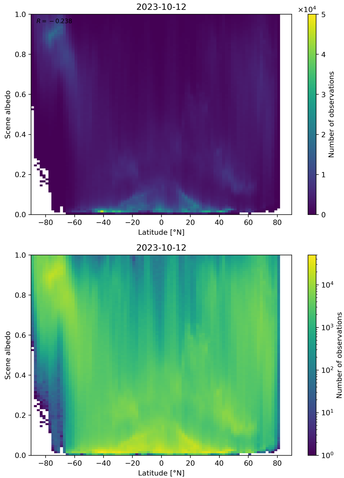
Figure 104: Scatter density plot of “Latitude” against “Scene albedo” for 2023-10-12 to 2023-10-13.
