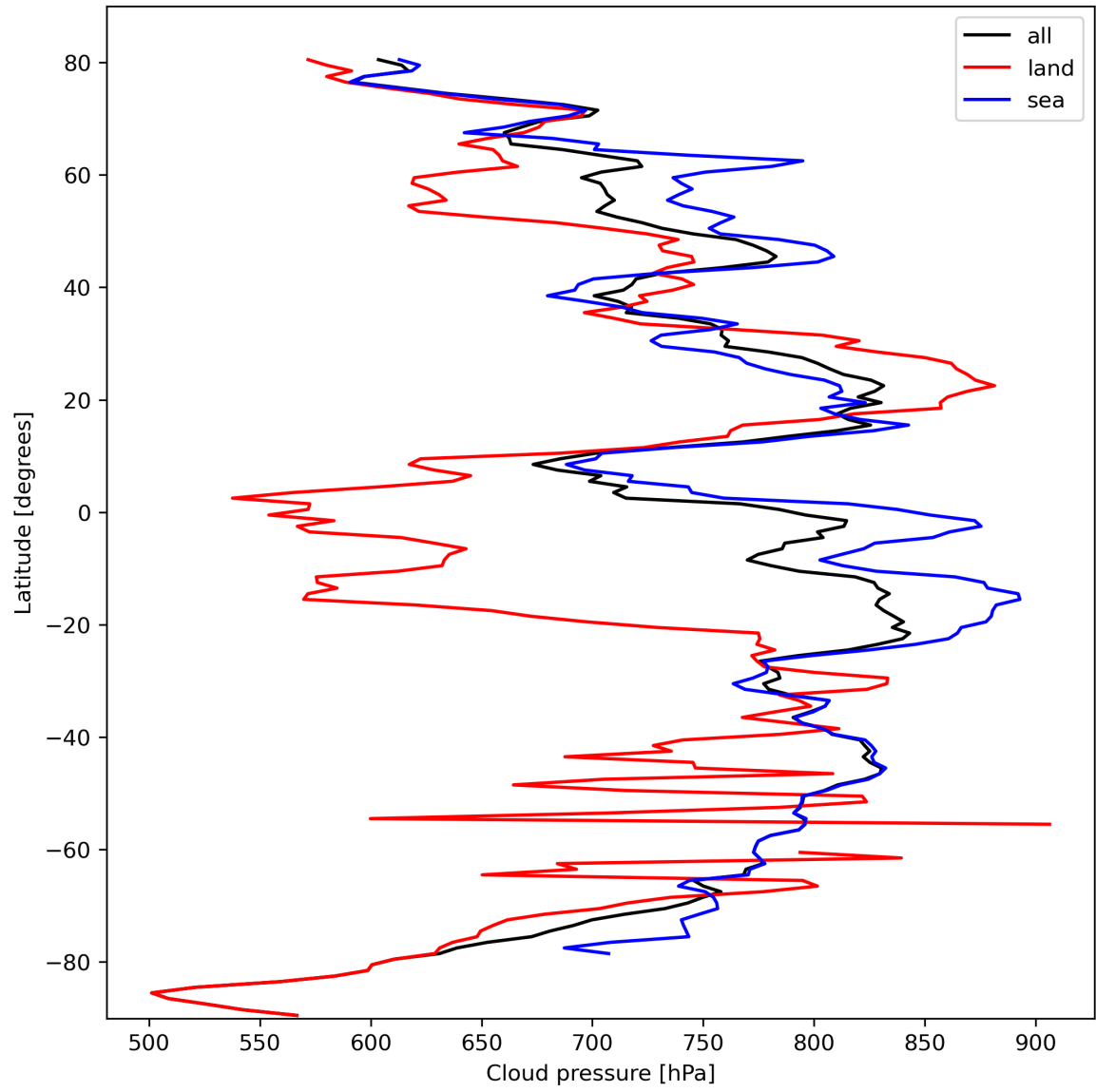
Figure 13: Zonal average of “Cloud pressure” for 2023-10-12 to 2023-10-13.
