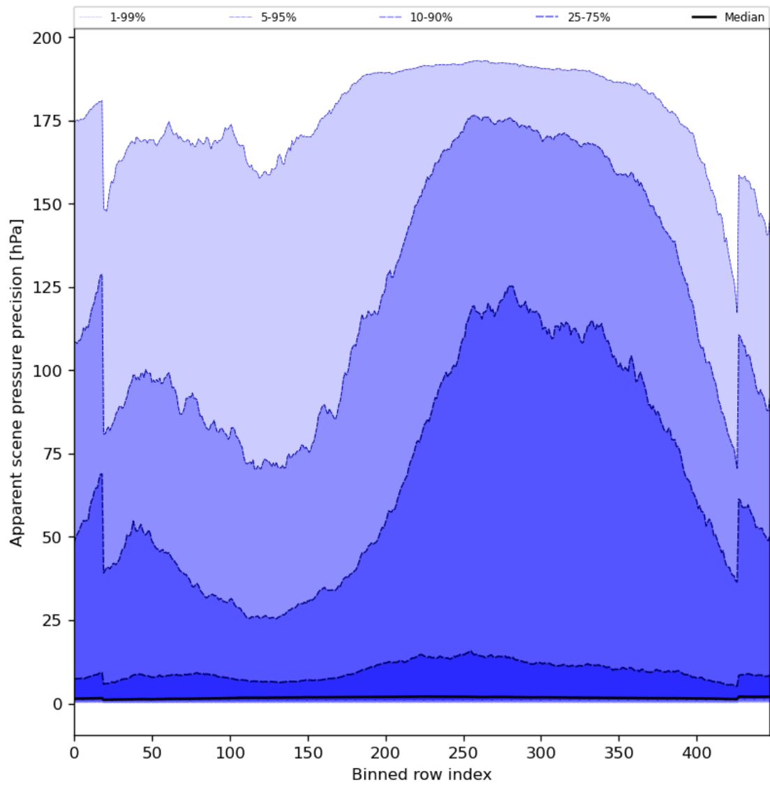
Figure 54: Along track statistics of “Apparent scene pressure precision” for 2023-10-12 to 2023-10-13
