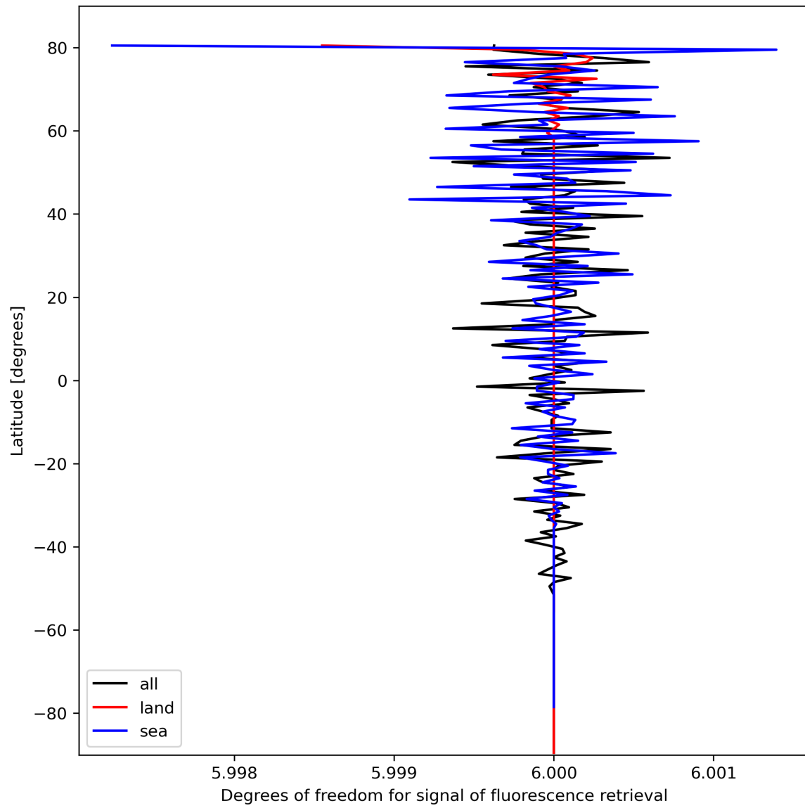
Figure 26: Zonal average of “Degrees of freedom for signal of fluorescence retrieval” for 2023-10-12 to 2023-10-13.
