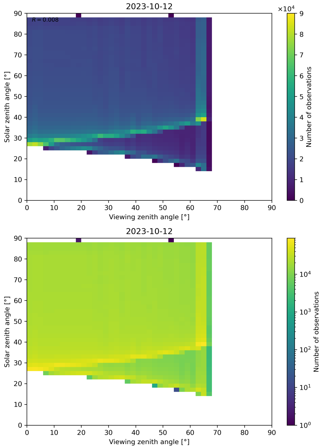
Figure 139: Scatter density plot of “Viewing zenith angle” against “Solar zenith angle” for 2023-10-12 to 2023-10-13.
