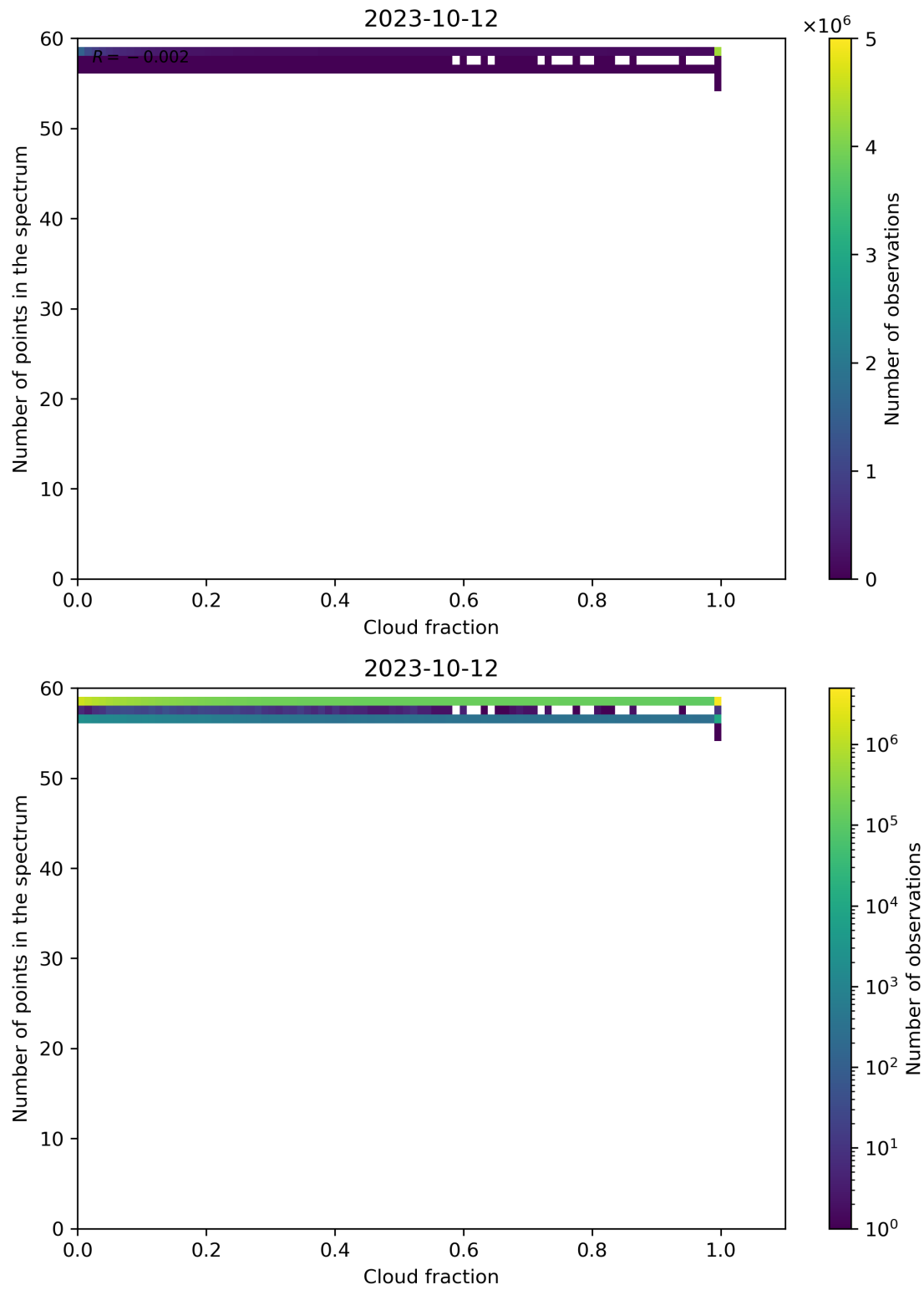
Figure 81: Scatter density plot of “Cloud fraction” against “Number of points in the spectrum” for 2023-10-12 to 2023-10-13.
