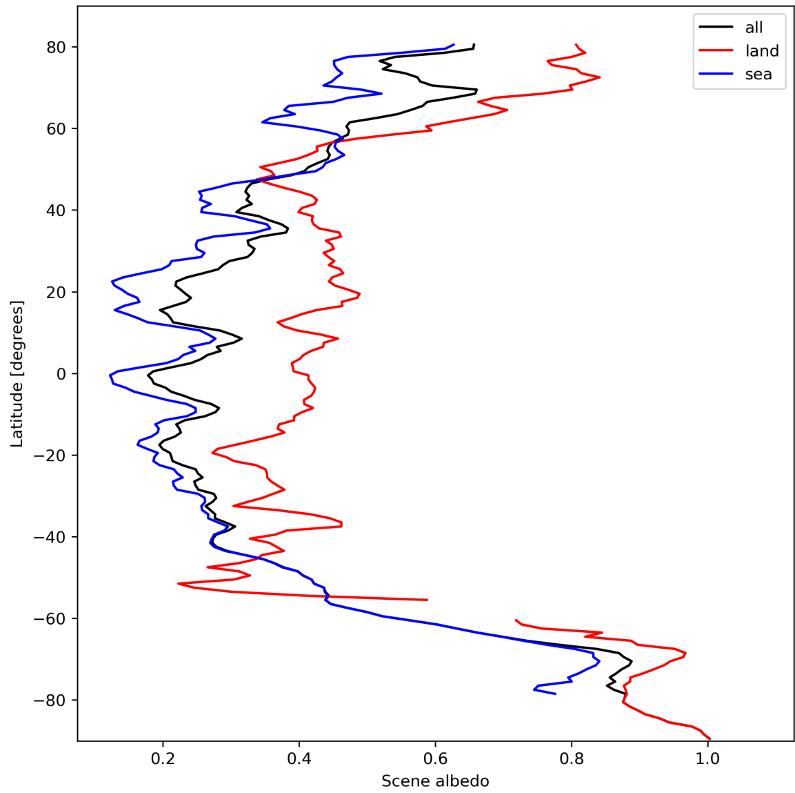
Figure 17: Zonal average of “Scene albedo” for 2023-10-12 to 2023-10-13.
