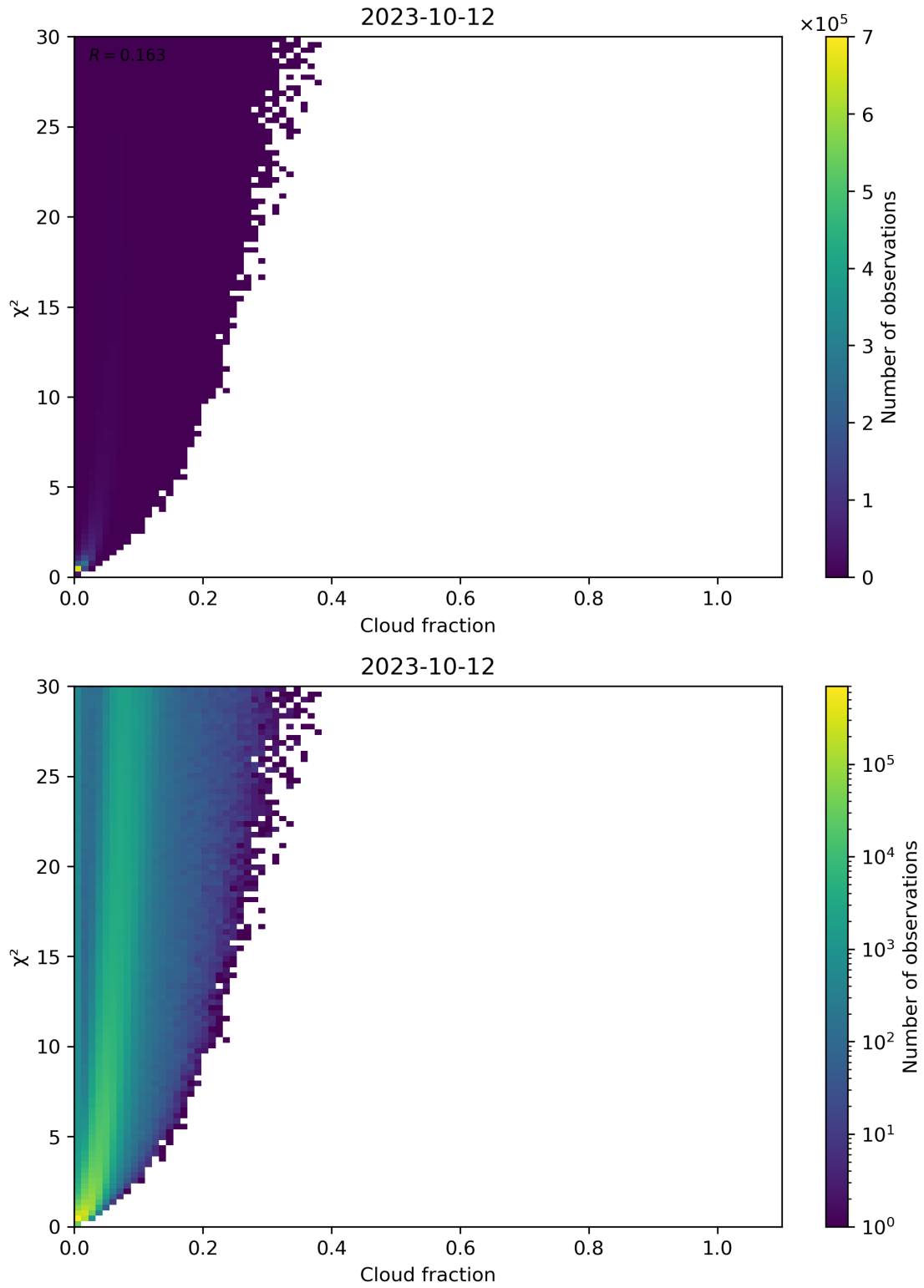
Figure 77: Scatter density plot of “Cloud fraction” against “ \chi^2 ” for 2023-10-12 to 2023-10-13.
