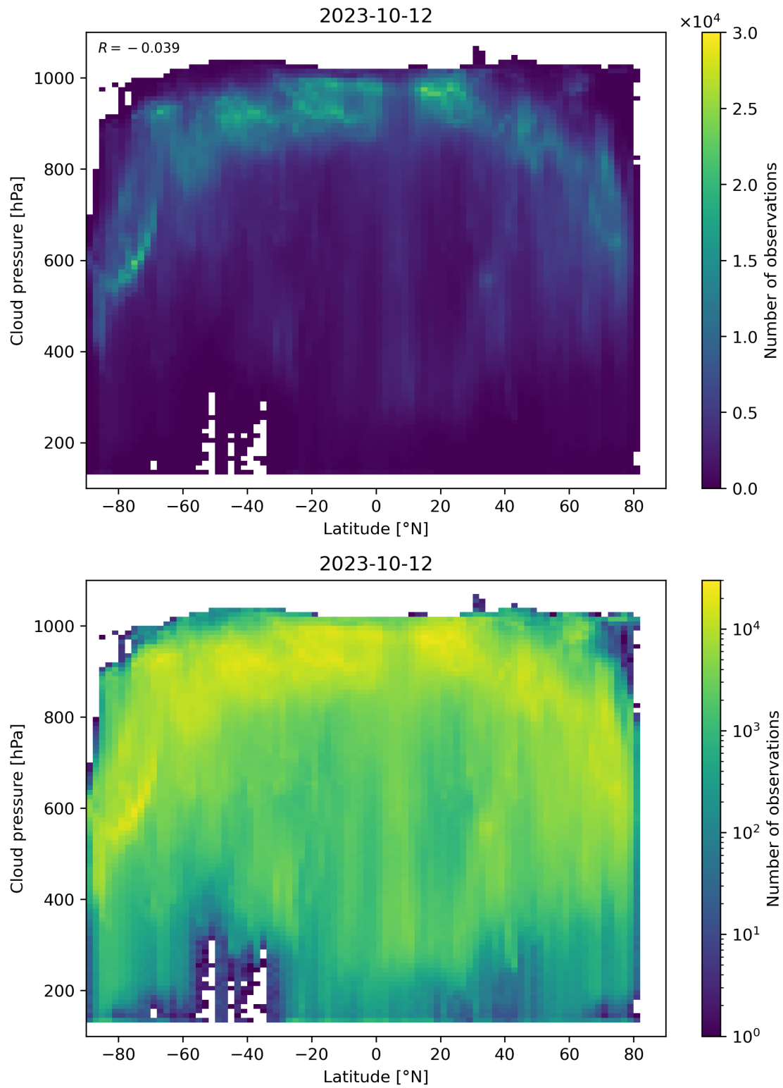
Figure 100: Scatter density plot of “Latitude” against “Cloud pressure” for 2023-10-12 to 2023-10-13.
