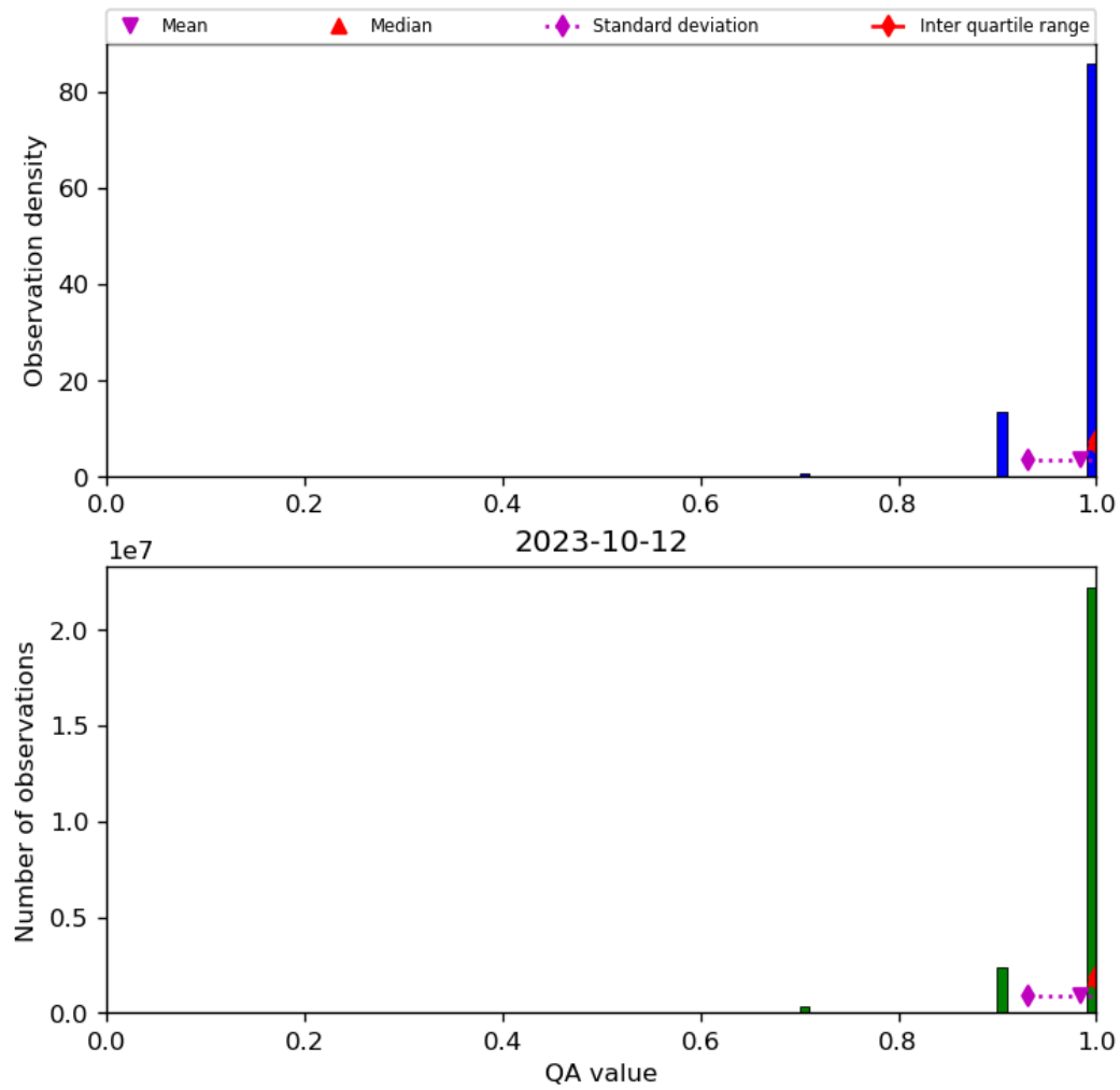
Figure 29: Histogram of “QA value” for 2023-10-12 to 2023-10-13
