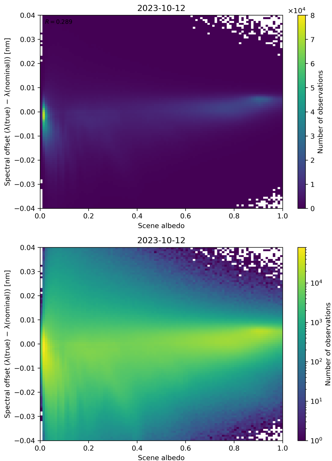
Figure 117: Scatter density plot of “Scene albedo” against “Spectral offset ( \lambda(\text{true}) - \lambda(\text{nominal}) )” for 2023-10-12 to 2023-10-13.
