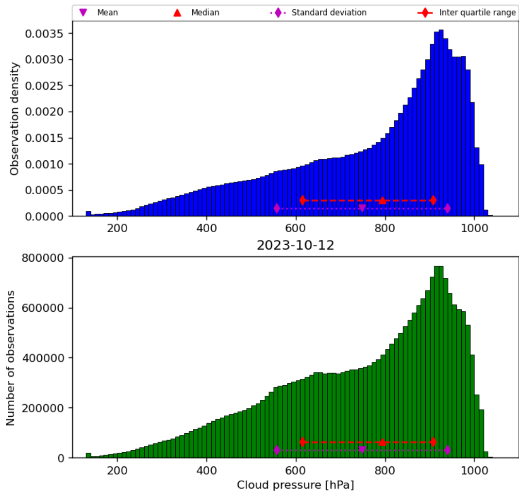
Figure 30: Histogram of “Cloud pressure” for 2023-10-12 to 2023-10-13
