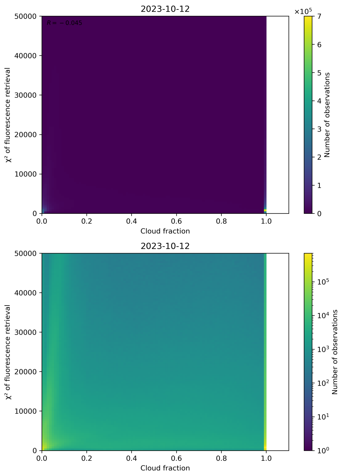
Figure 78: Scatter density plot of “Cloud fraction” against “ \chi^2 of fluorescence retrieval” for 2023-10-12 to 2023-10-13.
