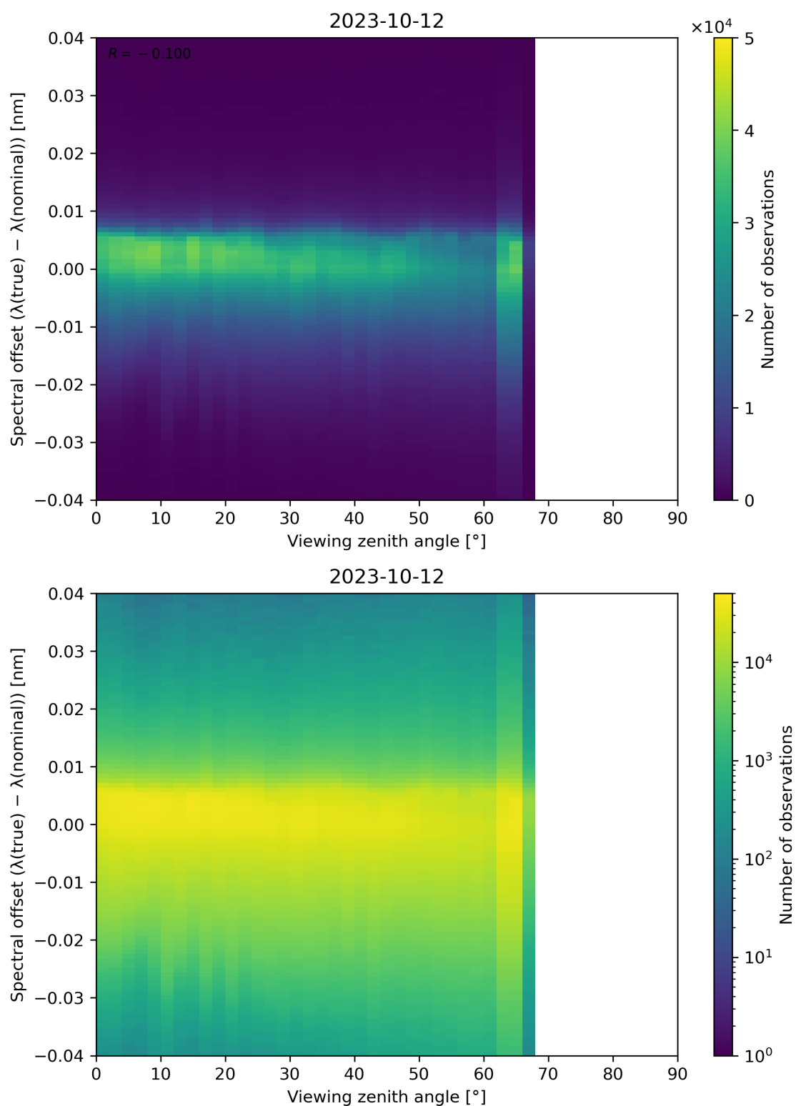
Figure 140: Scatter density plot of “Viewing zenith angle” against “Spectral offset ( \lambda(\text{true}) - \lambda(\text{nominal}) )” for 2023-10-12 to 2023-10-13.
