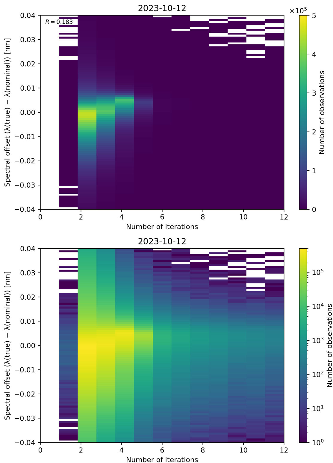
Figure 109: Scatter density plot of “Number of iterations” against “Spectral offset ( \lambda(\text{true}) - \lambda(\text{nominal}) )” for 2023-10-12 to 2023-10-13.
