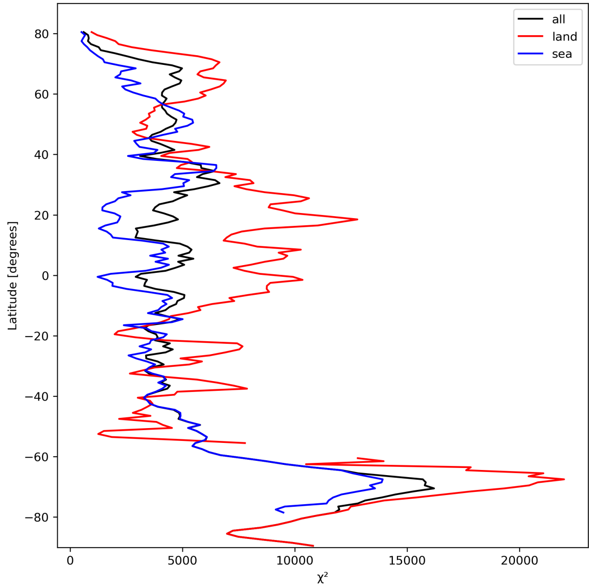
Figure 21: Zonal average of “ \chi^2 ” for 2023-10-12 to 2023-10-13.
