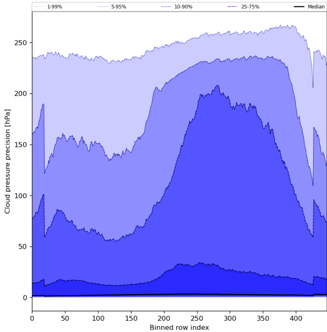
Figure 48: Along track statistics of “Cloud pressure precision” for 2023-10-12 to 2023-10-13
