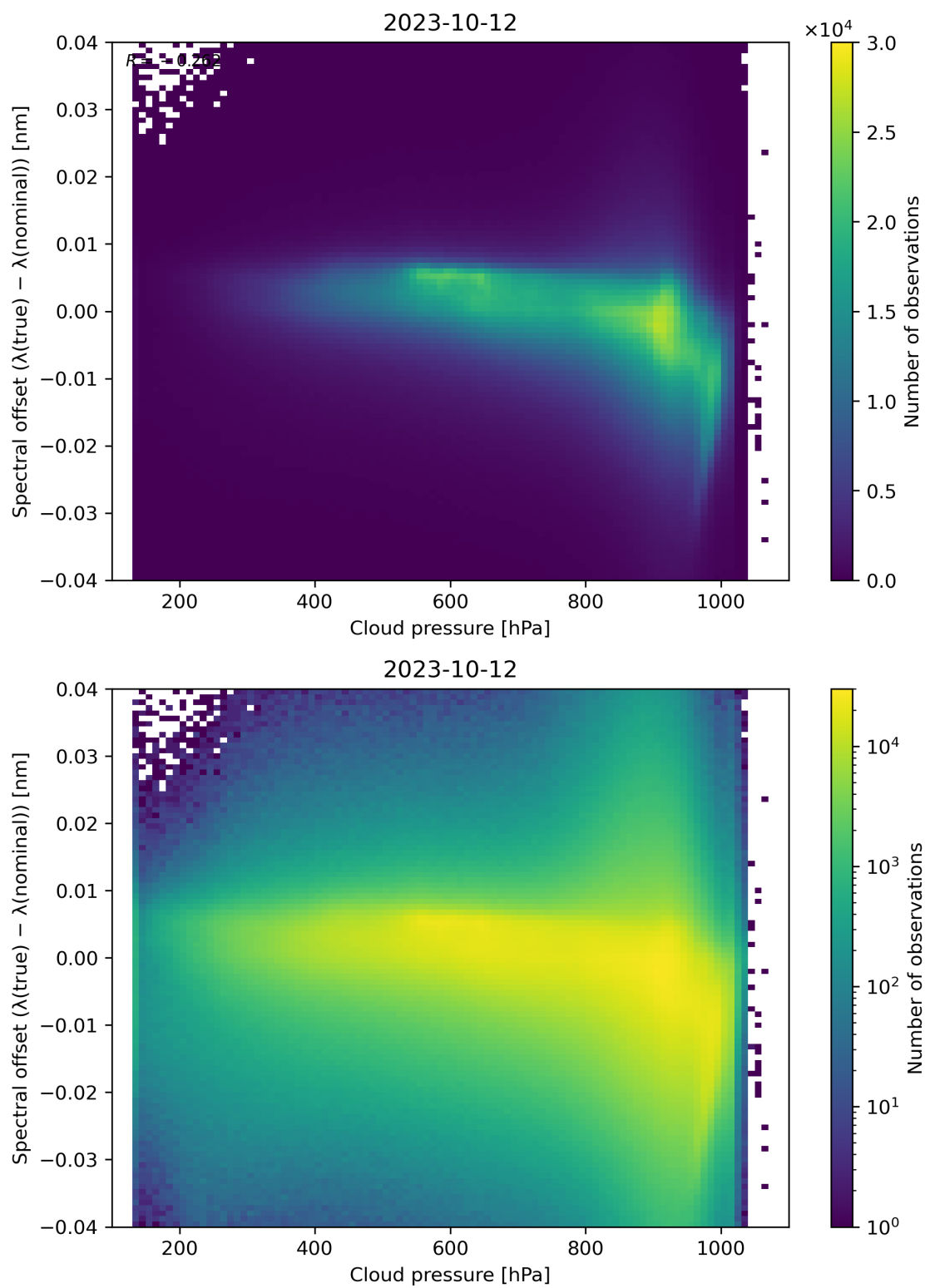
Figure 92: Scatter density plot of “Cloud pressure” against “Spectral offset ( \lambda(\text{true}) - \lambda(\text{nominal}) )” for 2023-10-12 to 2023-10-13.
