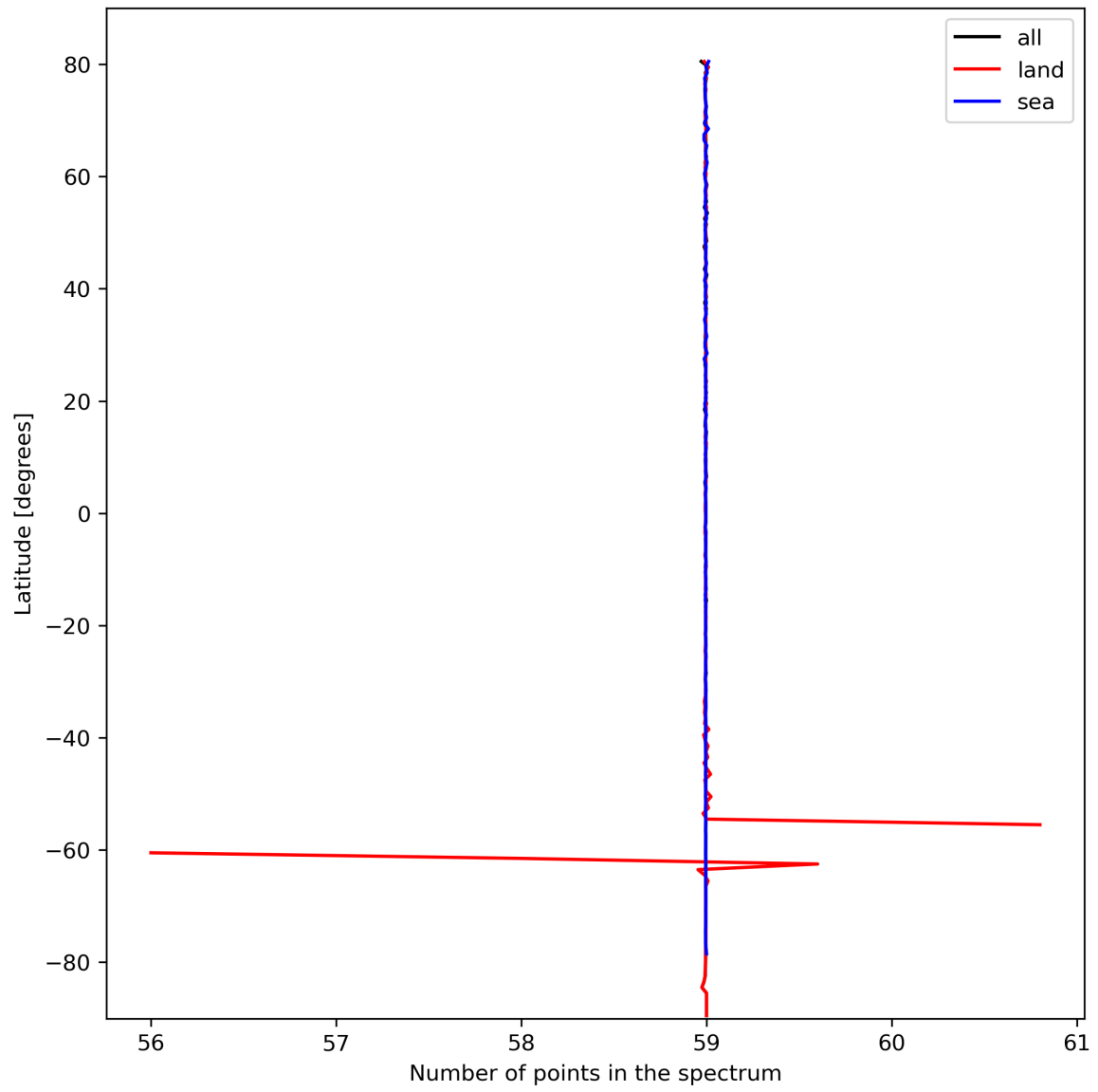
Figure 27: Zonal average of “Number of points in the spectrum” for 2023-10-12 to 2023-10-13.
