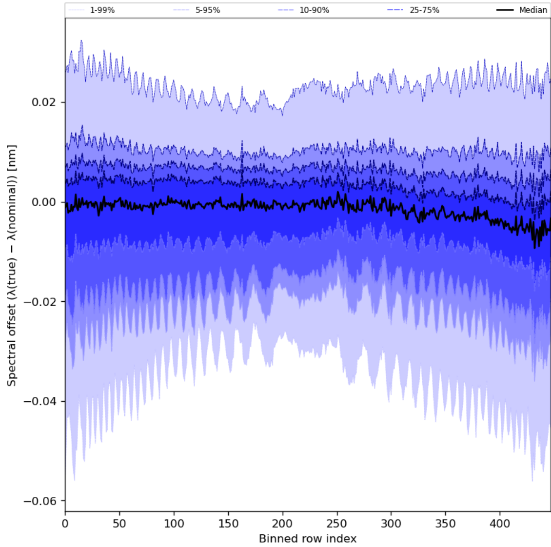
Figure 62: Along track statistics of “Spectral offset ( \lambda(\text{true}) - \lambda(\text{nominal}) )” for 2023-10-12 to 2023-10-13
