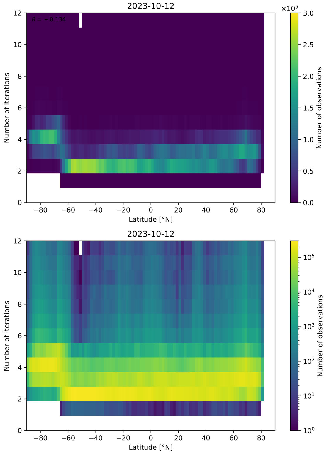
Figure 102: Scatter density plot of “Latitude” against “Number of iterations” for 2023-10-12 to 2023-10-13.
