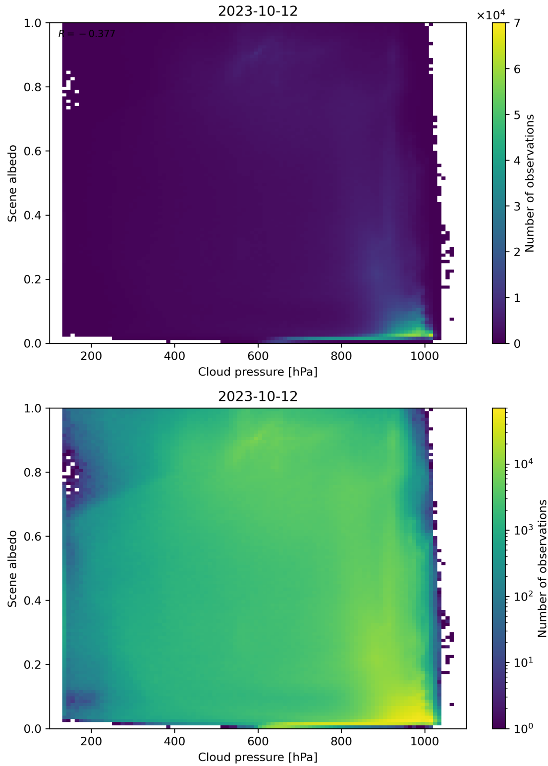
Figure 91: Scatter density plot of “Cloud pressure” against “Scene albedo” for 2023-10-12 to 2023-10-13.
