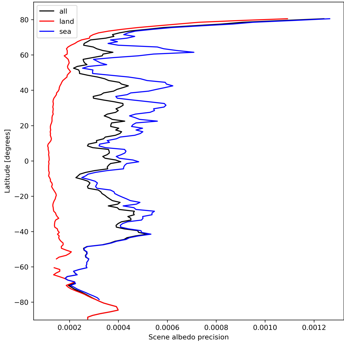
Figure 18: Zonal average of “Scene albedo precision” for 2023-10-12 to 2023-10-13.
