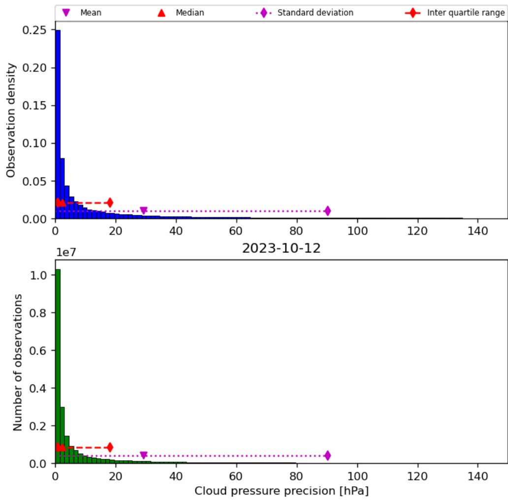
Figure 31: Histogram of “Cloud pressure precision” for 2023-10-12 to 2023-10-13
