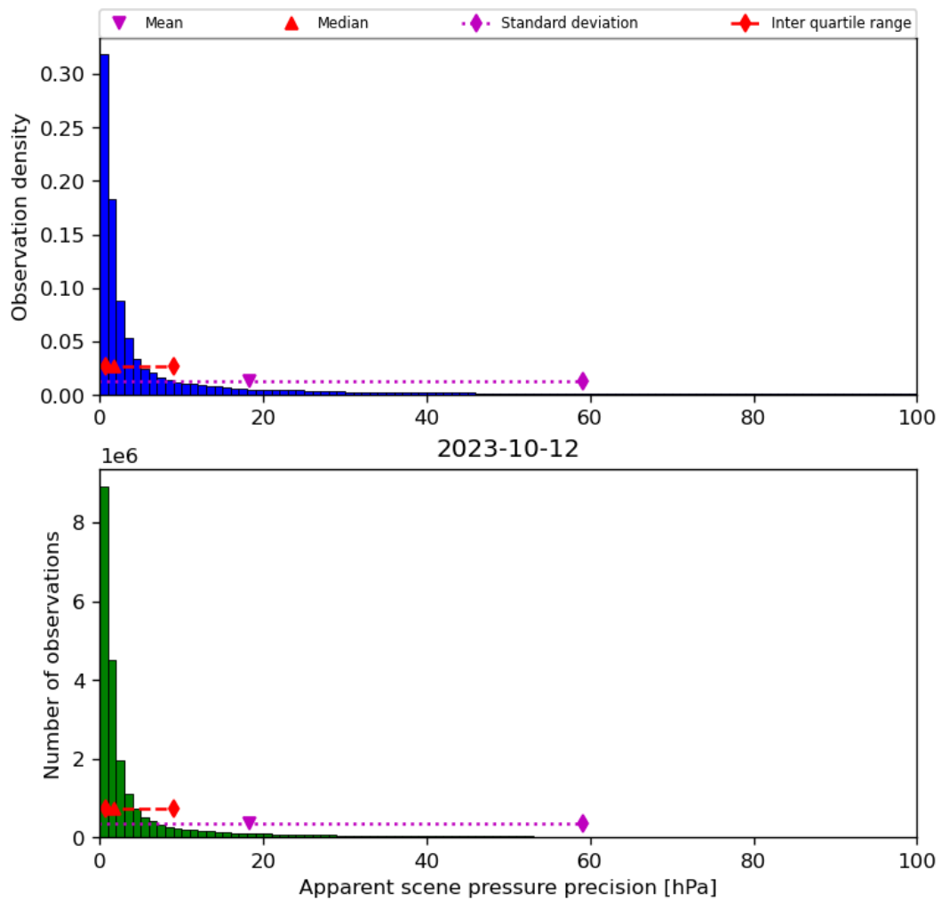
Figure 37: Histogram of “Apparent scene pressure precision” for 2023-10-12 to 2023-10-13
