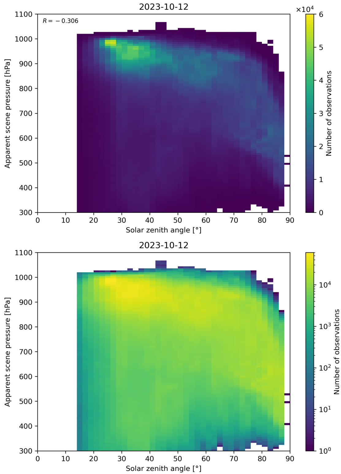
Figure 118: Scatter density plot of “Solar zenith angle” against “Apparent scene pressure” for 2023-10-12 to 2023-10-13.
