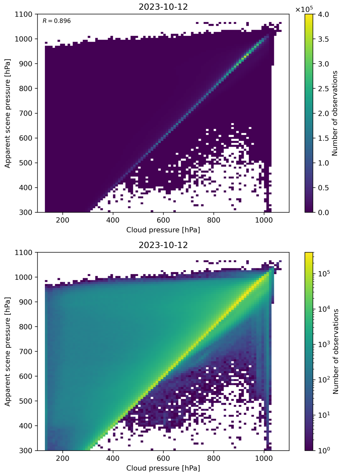
Figure 84: Scatter density plot of “Cloud pressure” against “Apparent scene pressure” for 2023-10-12 to 2023-10-13.
