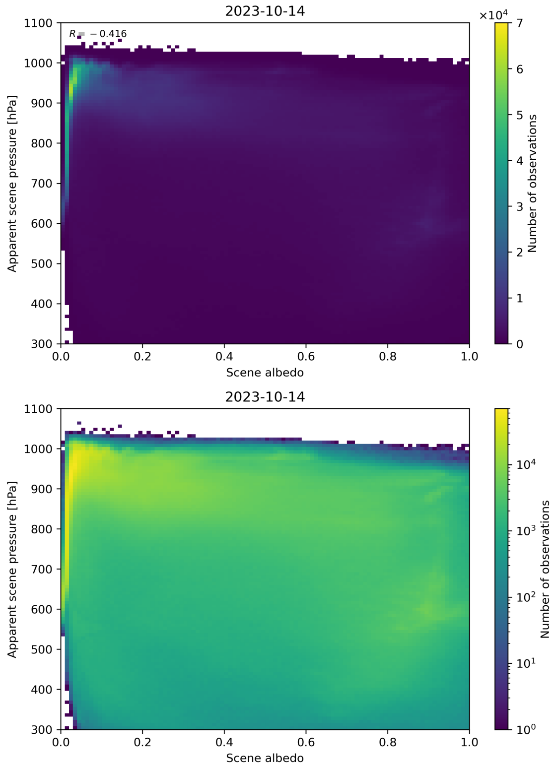
Figure 111: Scatter density plot of “Scene albedo” against “Apparent scene pressure” for 2023-10-13 to 2023-10-15.
