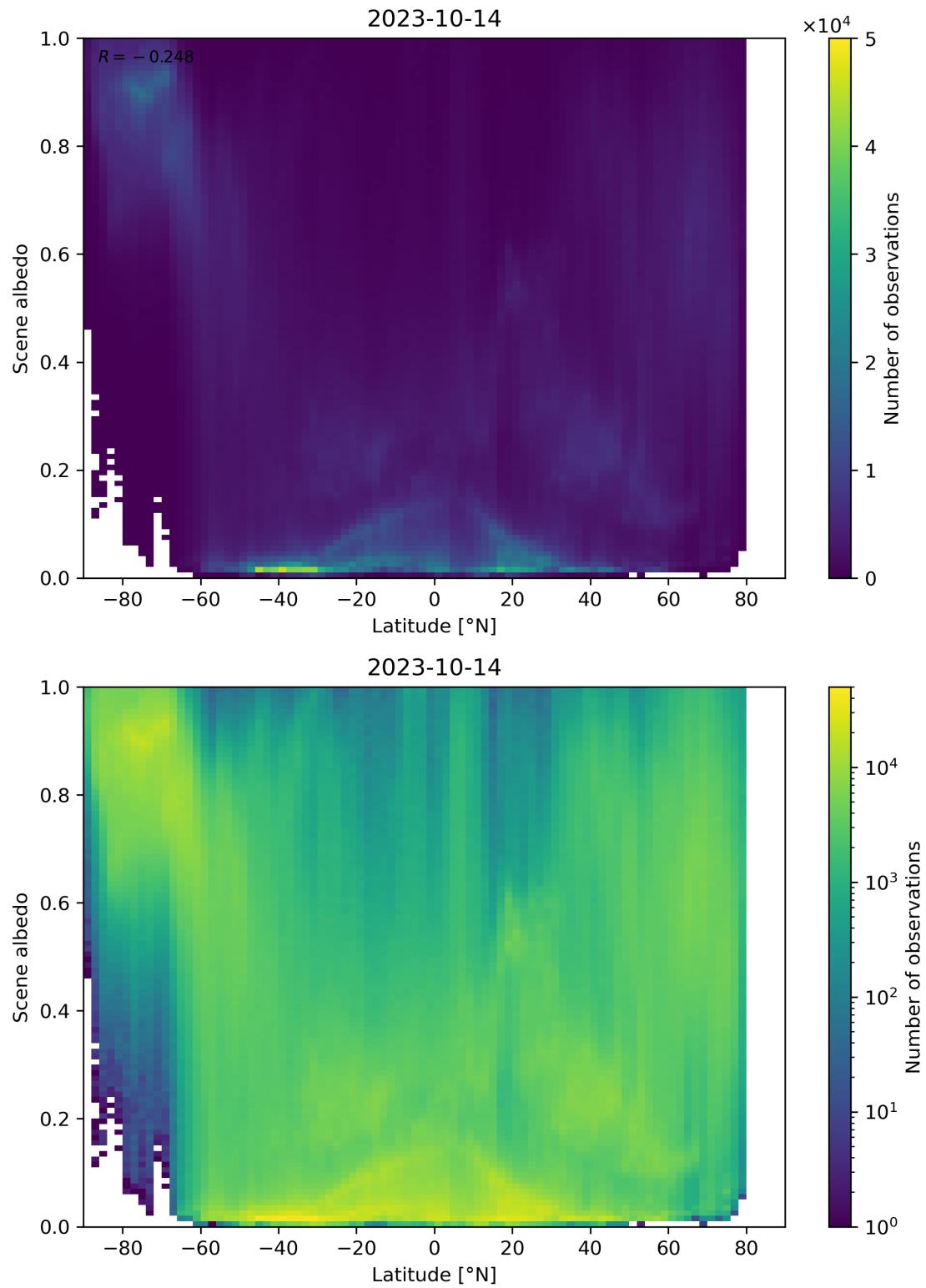
Figure 104: Scatter density plot of “Latitude” against “Scene albedo” for 2023-10-13 to 2023-10-15.
