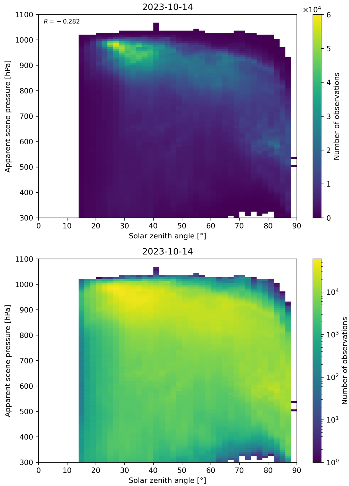
Figure 118: Scatter density plot of “Solar zenith angle” against “Apparent scene pressure” for 2023-10-13 to 2023-10-15.
