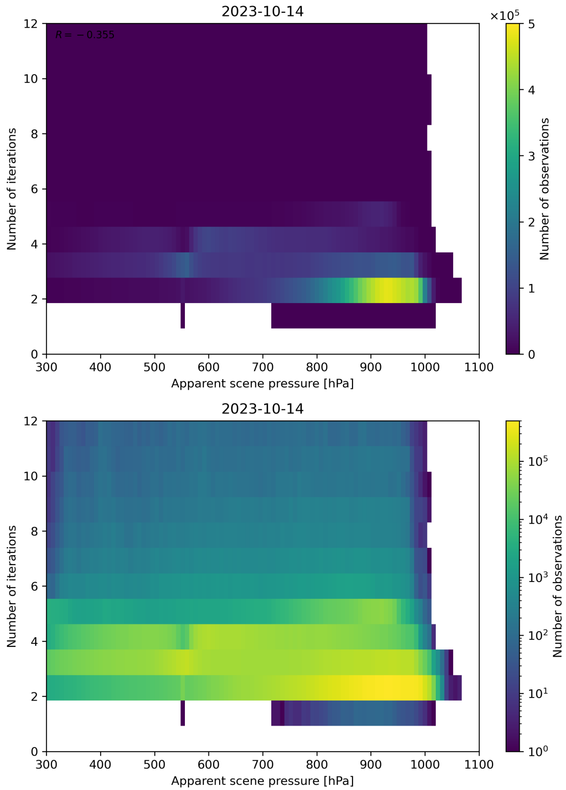
Figure 66: Scatter density plot of “Apparent scene pressure” against “Number of iterations” for 2023-10-13 to 2023-10-15.
