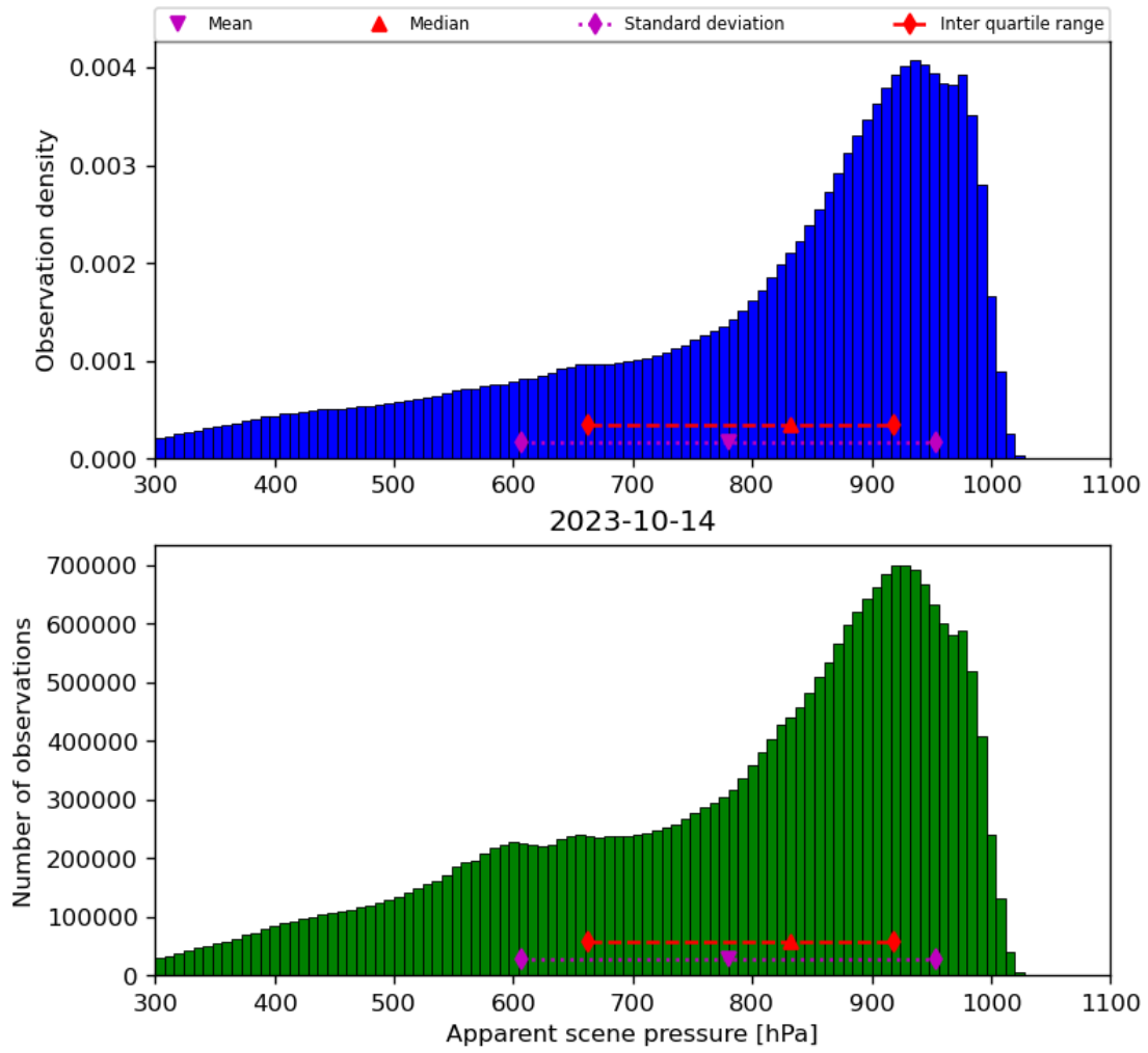
Figure 36: Histogram of “Apparent scene pressure” for 2023-10-13 to 2023-10-15
