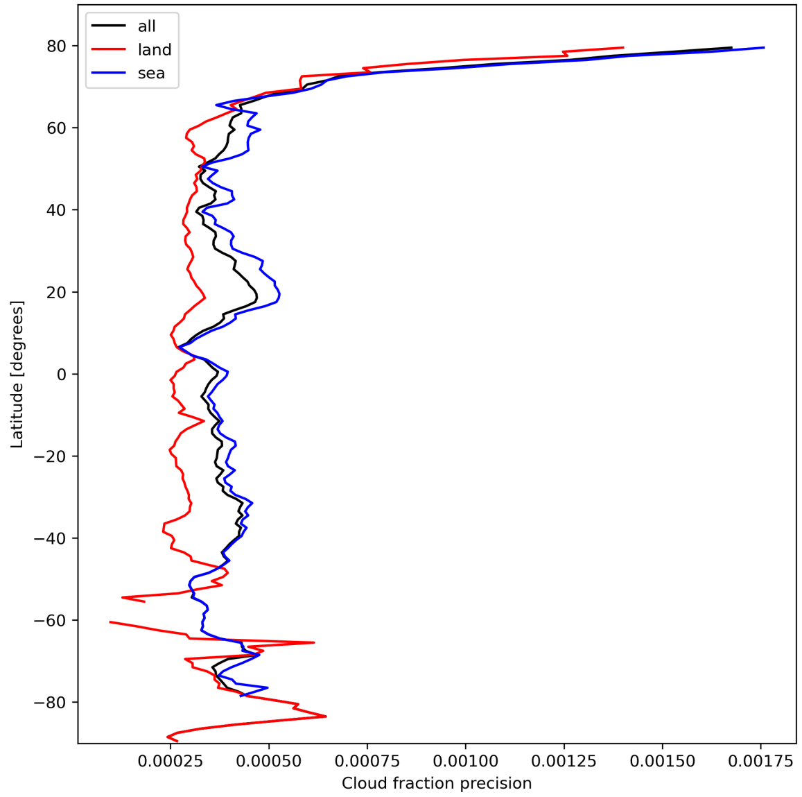
Figure 16: Zonal average of “Cloud fraction precision” for 2023-10-13 to 2023-10-15.
