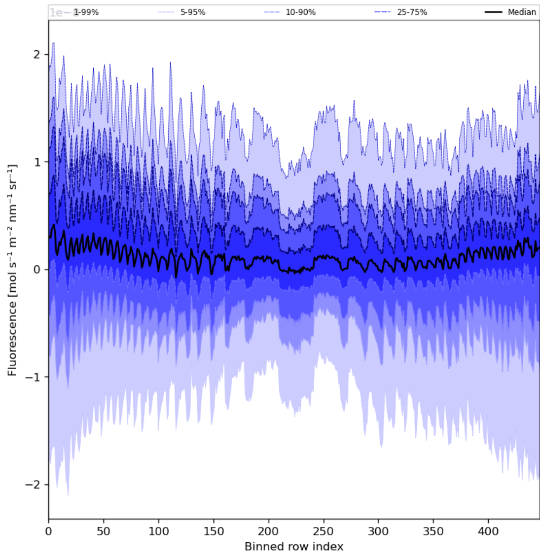
Figure 57: Along track statistics of “Fluorescence” for 2023-10-13 to 2023-10-15
