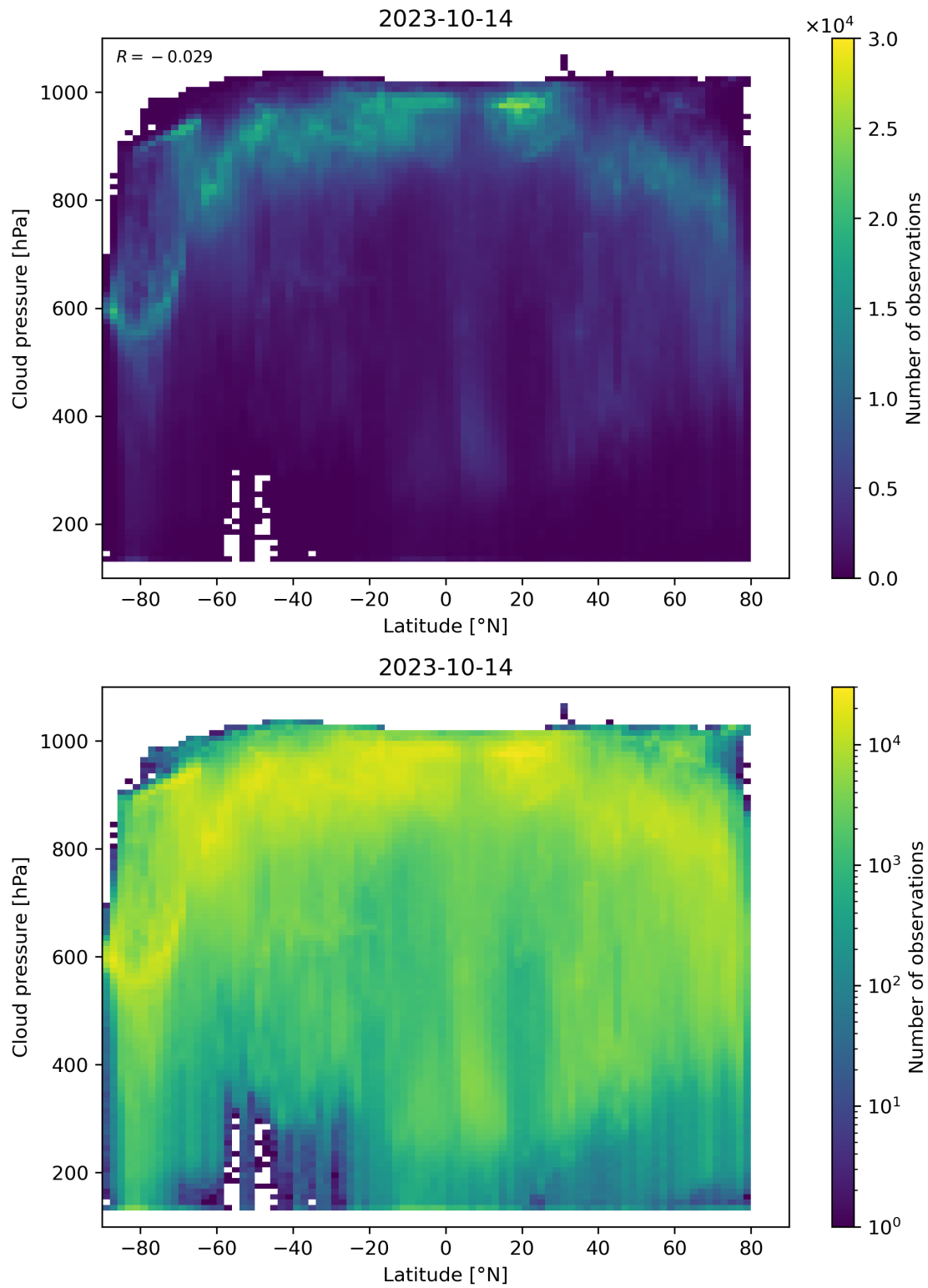
Figure 100: Scatter density plot of “Latitude” against “Cloud pressure” for 2023-10-13 to 2023-10-15.
