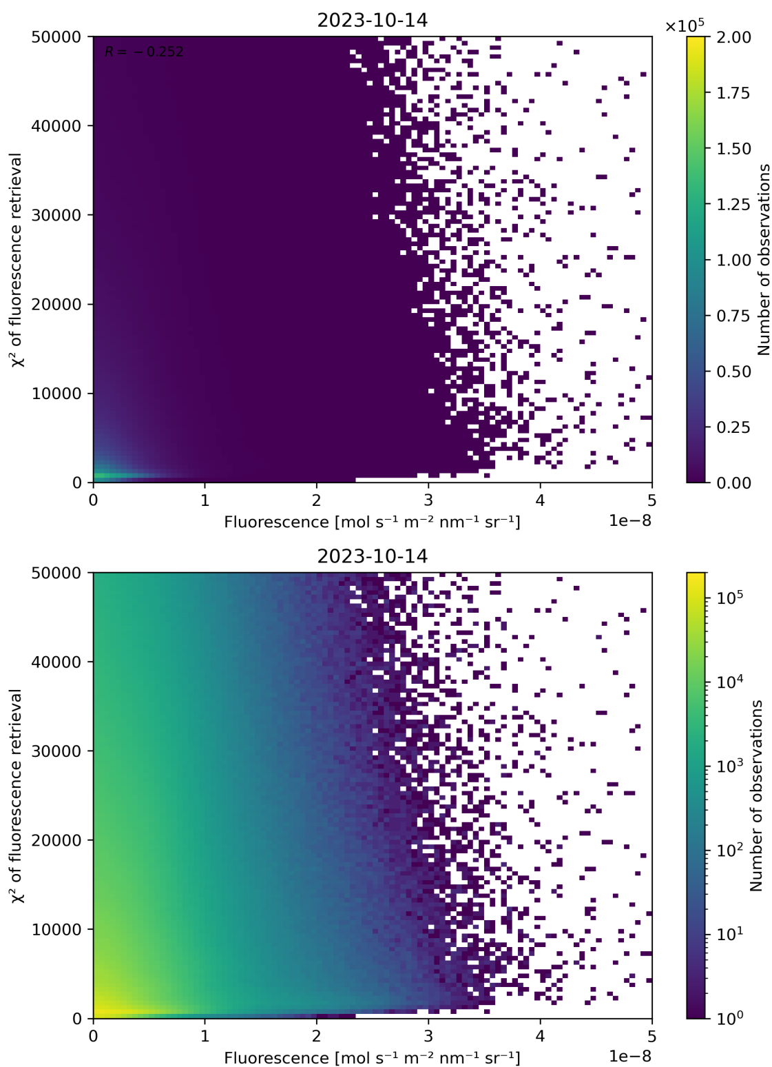
Figure 93: Scatter density plot of “Fluorescence” against “ \chi^2 of fluorescence retrieval” for 2023-10-13 to 2023-10-15.
