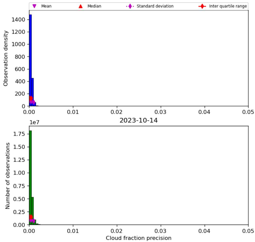
Figure 33: Histogram of “Cloud fraction precision” for 2023-10-13 to 2023-10-15
