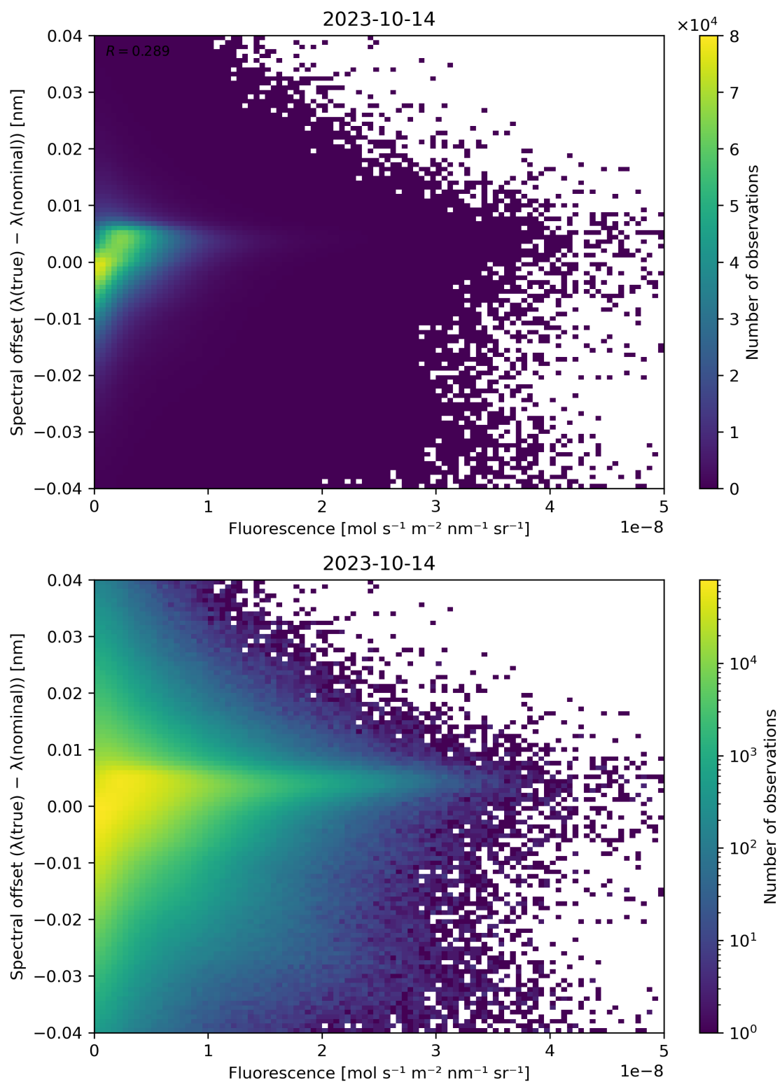
Figure 95: Scatter density plot of “Fluorescence” against “Spectral offset ( \lambda(\text{true}) - \lambda(\text{nominal}) )” for 2023-10-13 to 2023-10-15.
