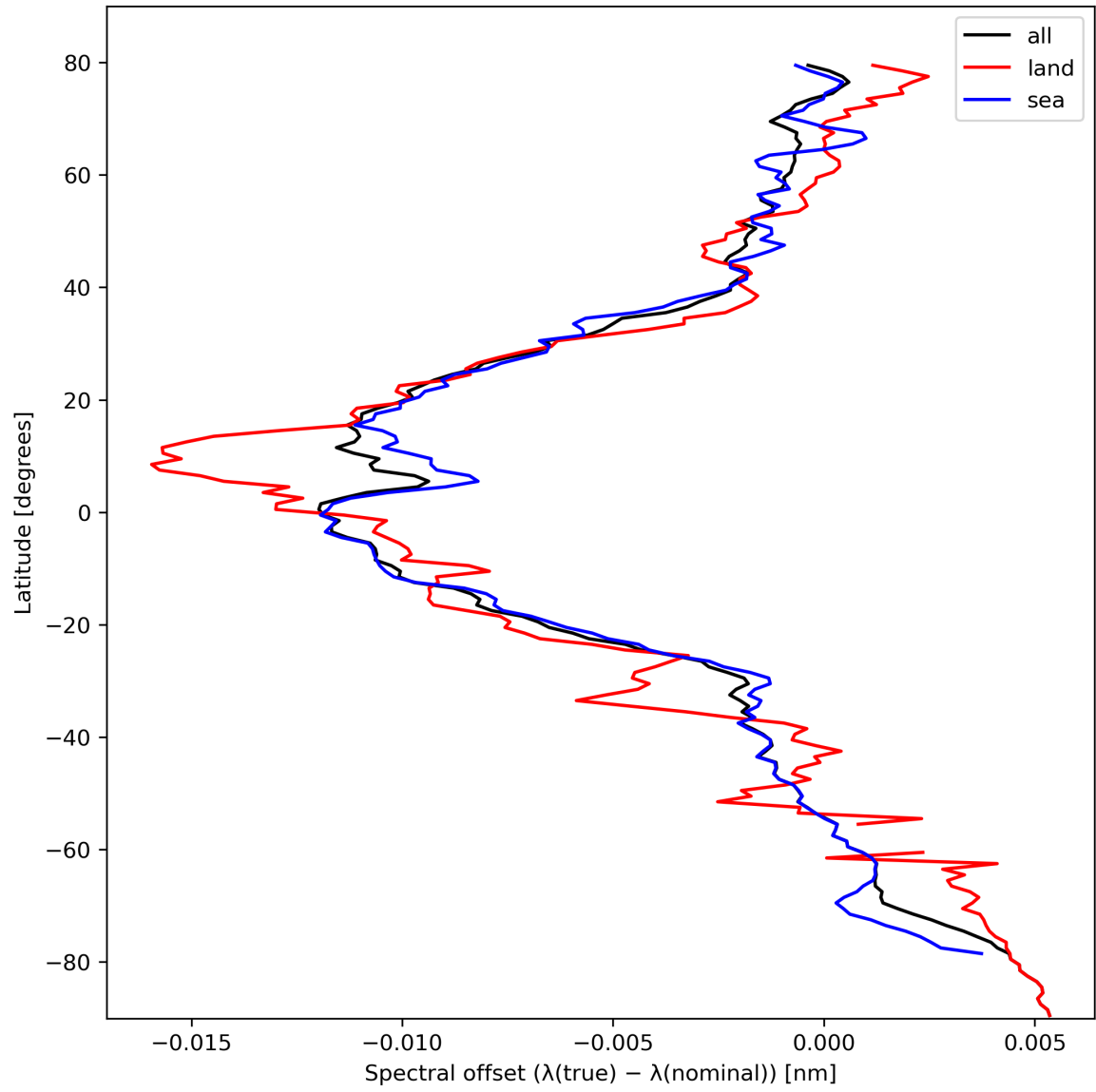
Figure 28: Zonal average of “Spectral offset ( \lambda(\text{true}) - \lambda(\text{nominal}) )” for 2023-10-13 to 2023-10-15.
