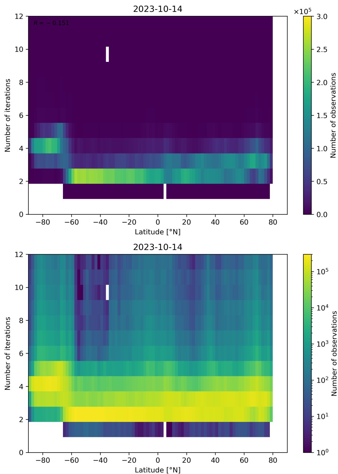
Figure 102: Scatter density plot of “Latitude” against “Number of iterations” for 2023-10-13 to 2023-10-15.
