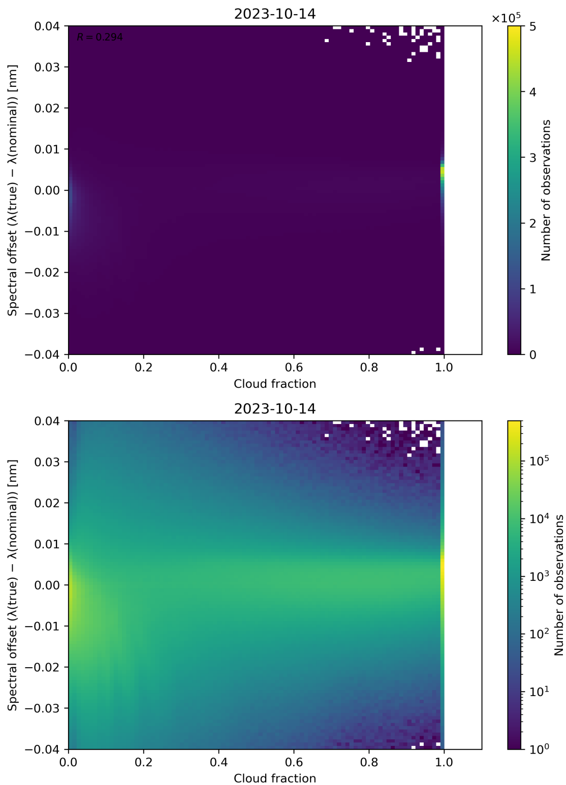
Figure 83: Scatter density plot of “Cloud fraction” against “Spectral offset ( \lambda(\text{true}) - \lambda(\text{nominal}) )” for 2023-10-13 to 2023-10-15.
