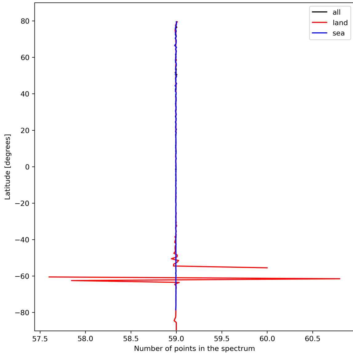
Figure 27: Zonal average of “Number of points in the spectrum” for 2023-10-13 to 2023-10-15.
