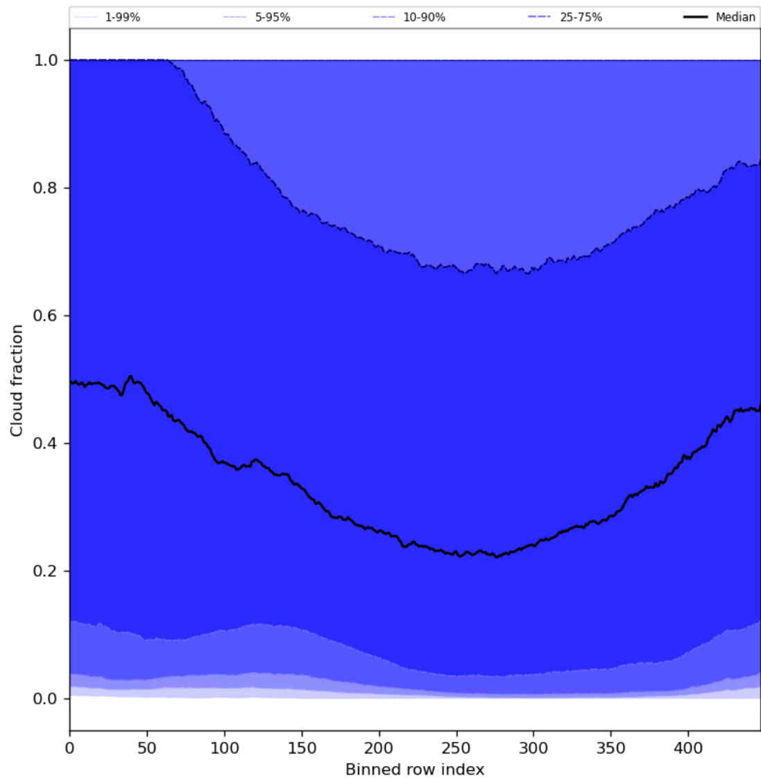
Figure 49: Along track statistics of “Cloud fraction” for 2023-10-13 to 2023-10-15
