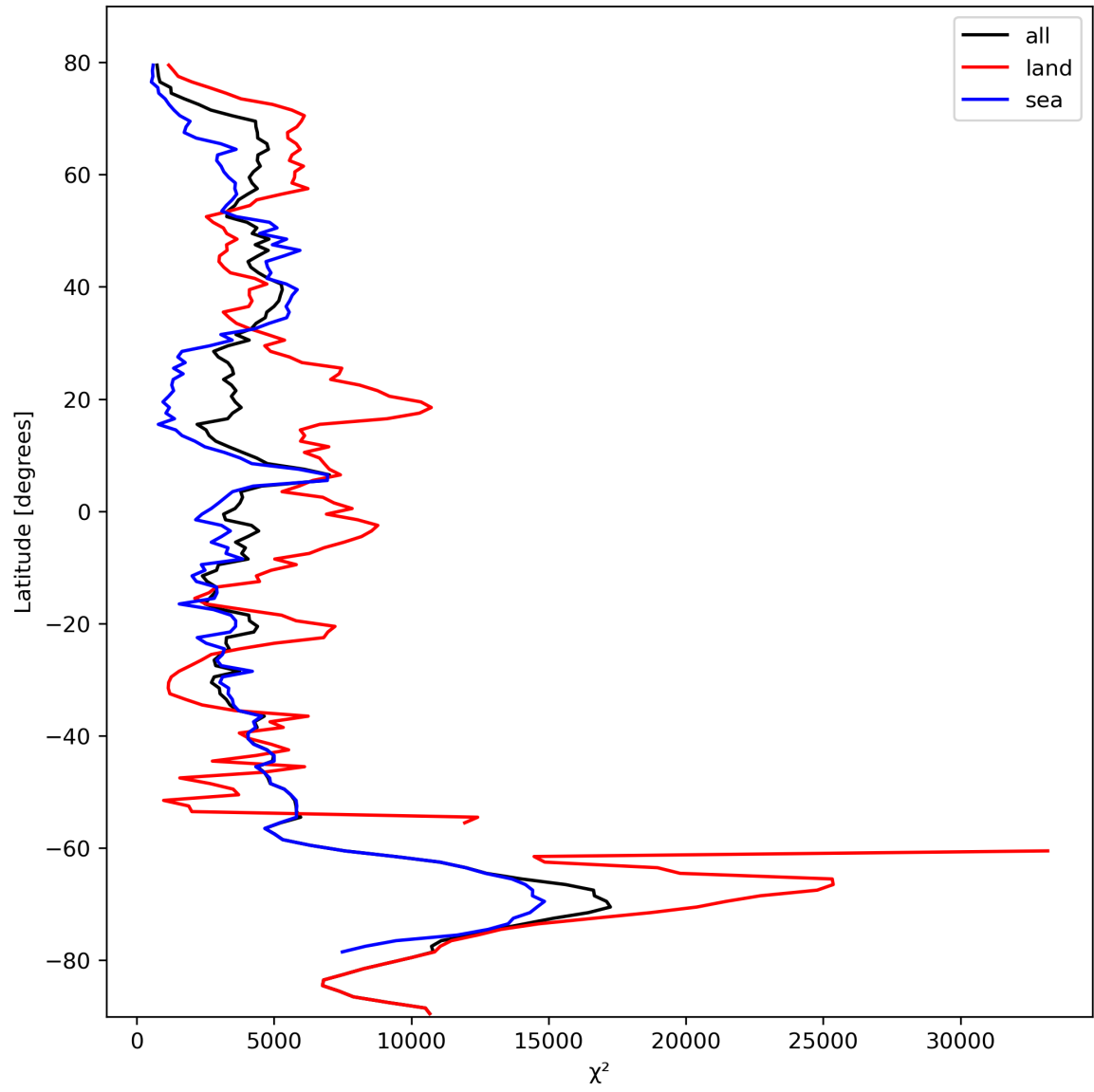
Figure 21: Zonal average of “ \chi^2 ” for 2023-10-13 to 2023-10-15.
