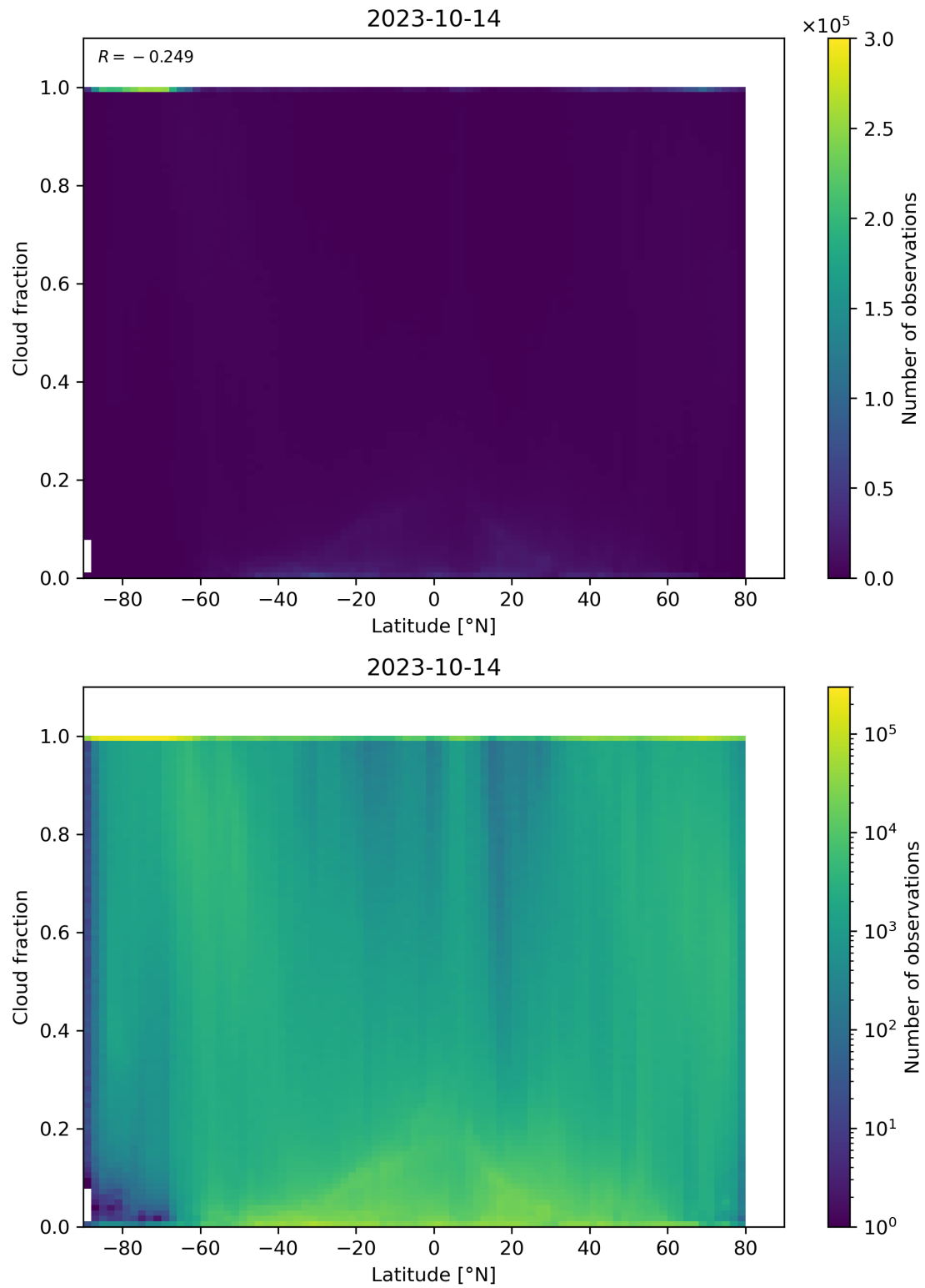
Figure 99: Scatter density plot of “Latitude” against “Cloud fraction” for 2023-10-13 to 2023-10-15.
