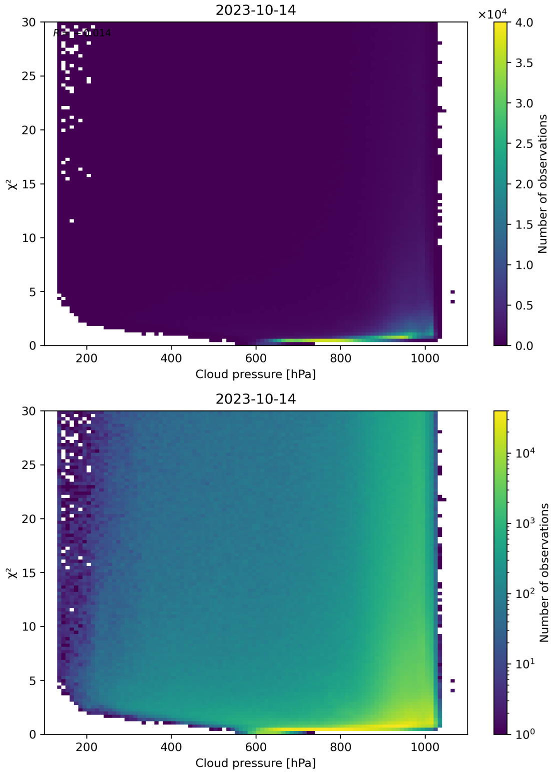
Figure 85: Scatter density plot of “Cloud pressure” against “ \chi^2 ” for 2023-10-13 to 2023-10-15.
