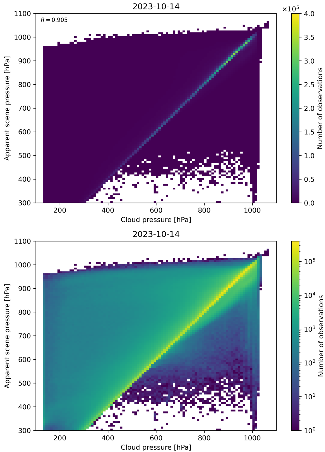
Figure 84: Scatter density plot of “Cloud pressure” against “Apparent scene pressure” for 2023-10-13 to 2023-10-15.
