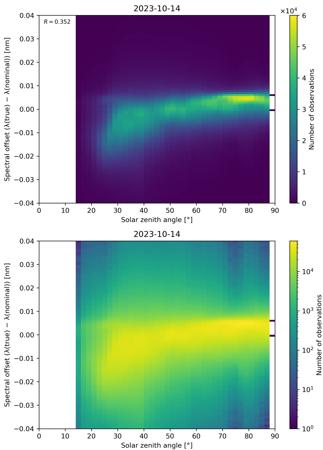
Figure 128: Scatter density plot of “Solar zenith angle” against “Spectral offset ( \lambda(\text{true}) - \lambda(\text{nominal}) )” for 2023-10-13 to 2023-10-15.
