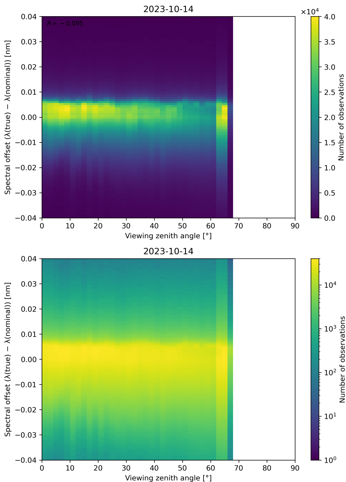
Figure 140: Scatter density plot of “Viewing zenith angle” against “Spectral offset ( \lambda(\text{true}) - \lambda(\text{nominal}) )” for 2023-10-13 to 2023-10-15.
