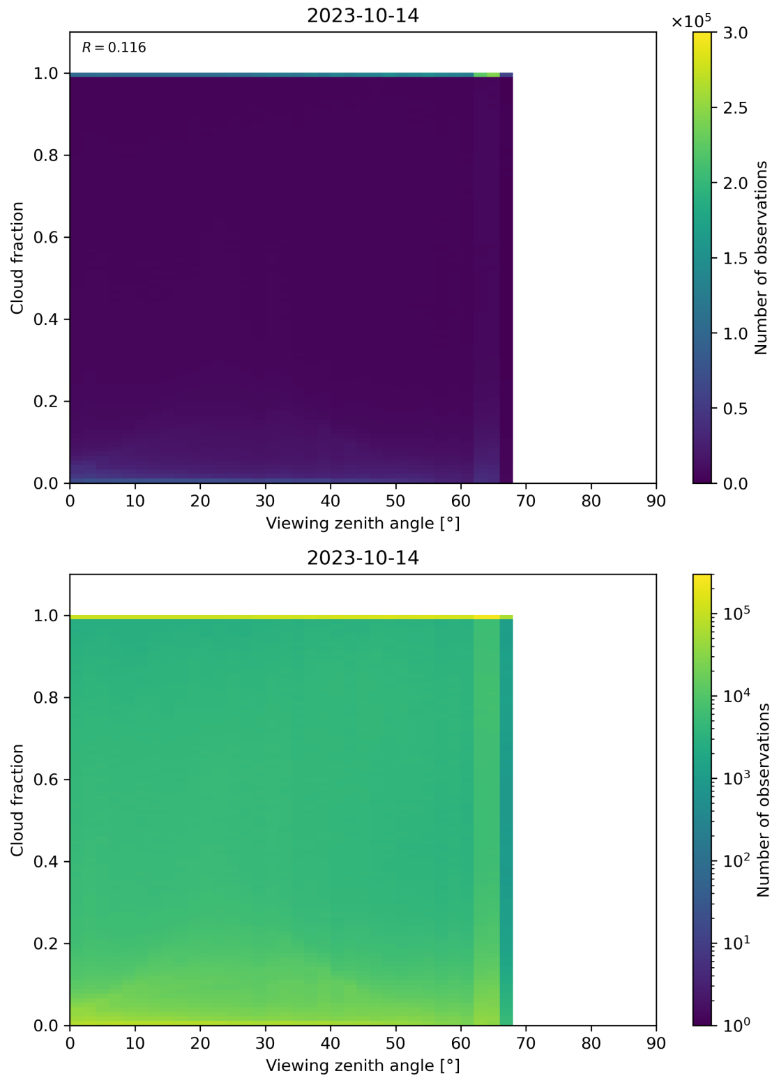
Figure 132: Scatter density plot of “Viewing zenith angle” against “Cloud fraction” for 2023-10-13 to 2023-10-15.
