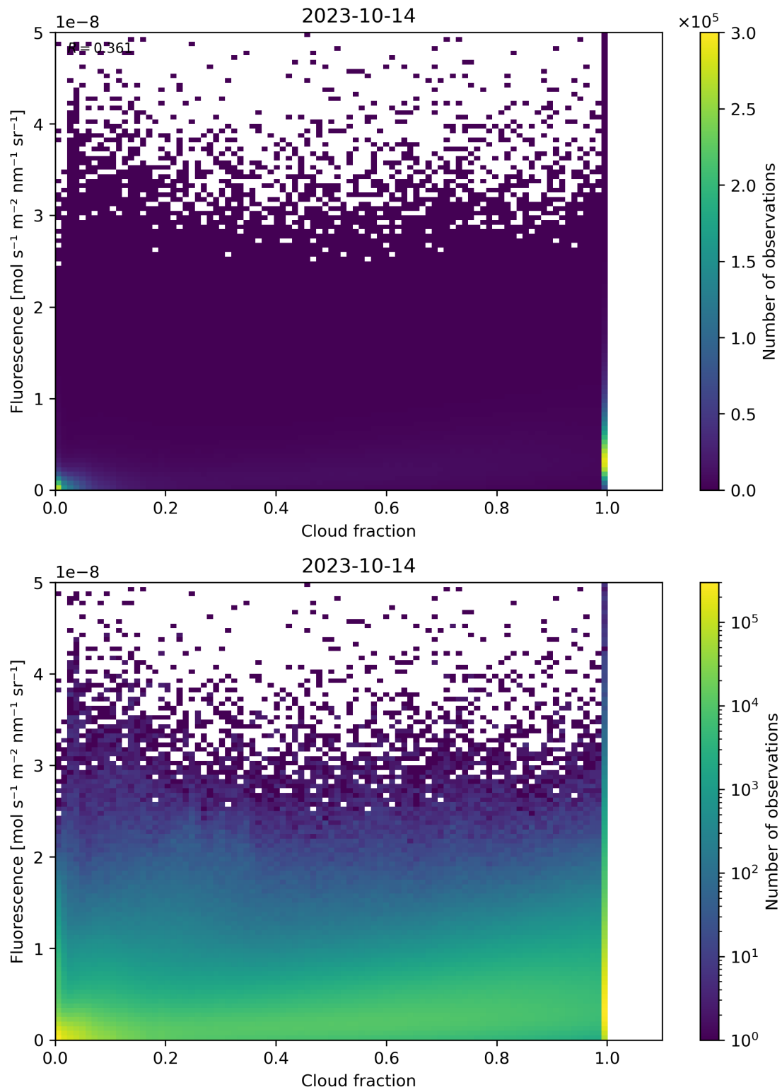
Figure 79: Scatter density plot of “Cloud fraction” against “Fluorescence” for 2023-10-13 to 2023-10-15.
