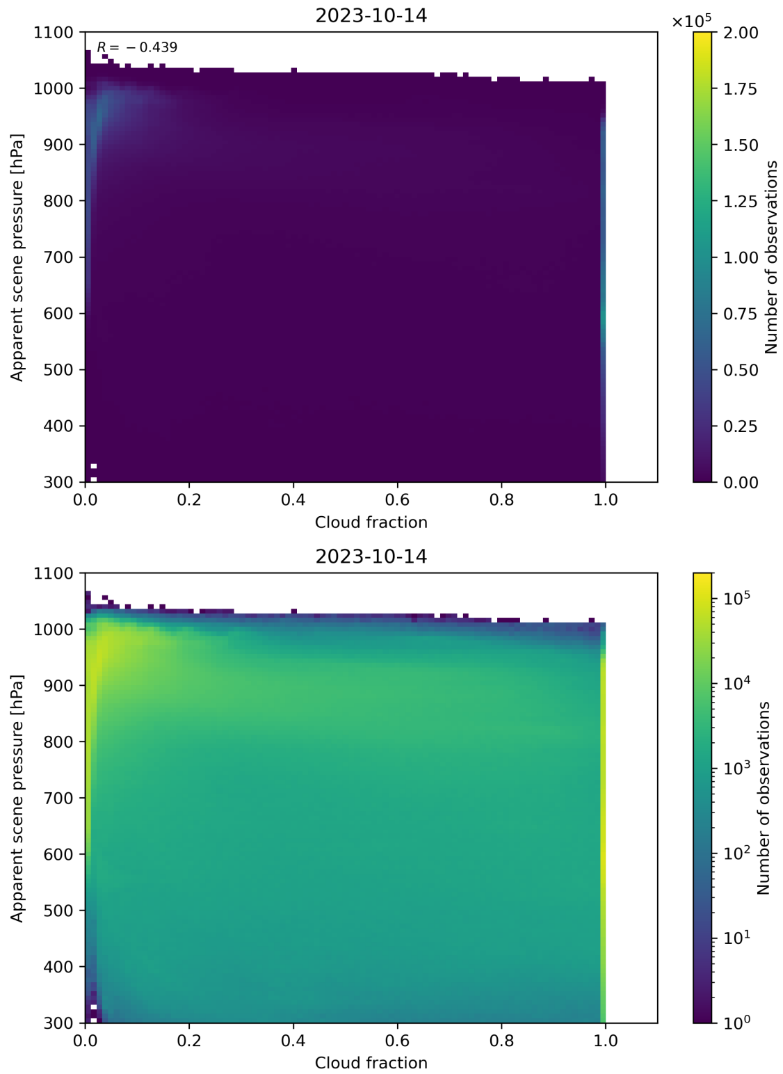
Figure 76: Scatter density plot of “Cloud fraction” against “Apparent scene pressure” for 2023-10-13 to 2023-10-15.
