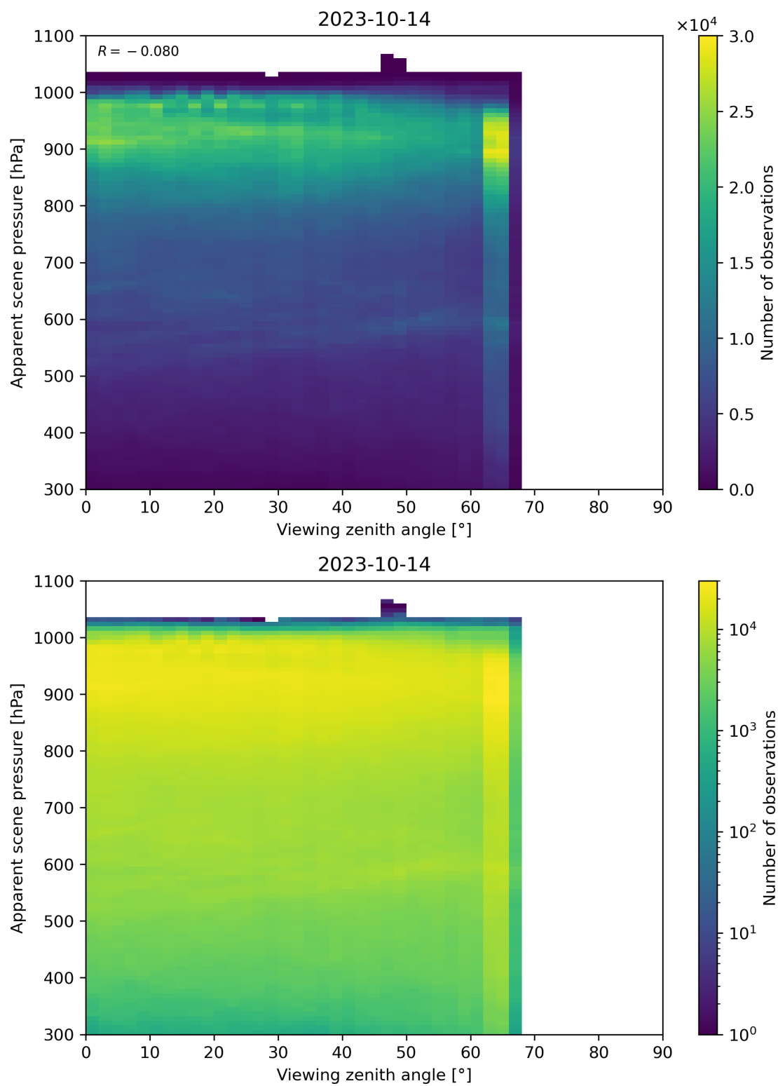
Figure 129: Scatter density plot of “Viewing zenith angle” against “Apparent scene pressure” for 2023-10-13 to 2023-10-15.
