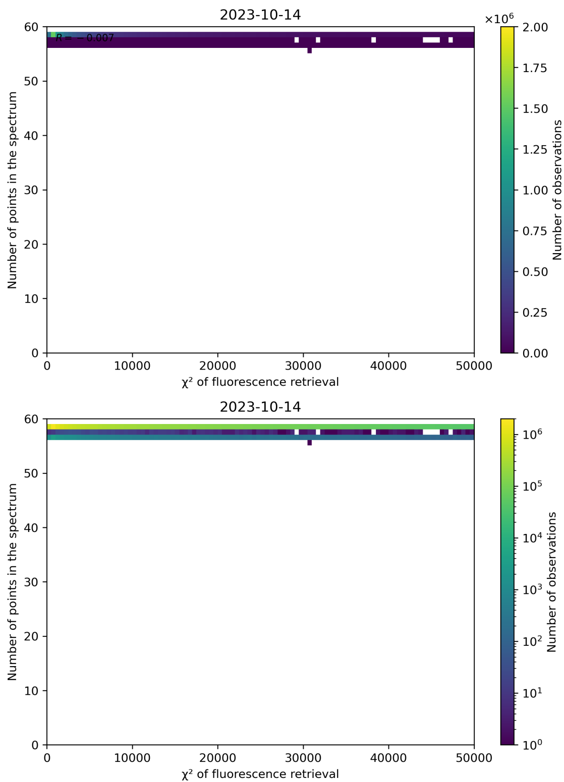
Figure 71: Scatter density plot of “ \chi^2 of fluorescence retrieval” against “Number of points in the spectrum” for 2023-10-13 to 2023-10-15.
