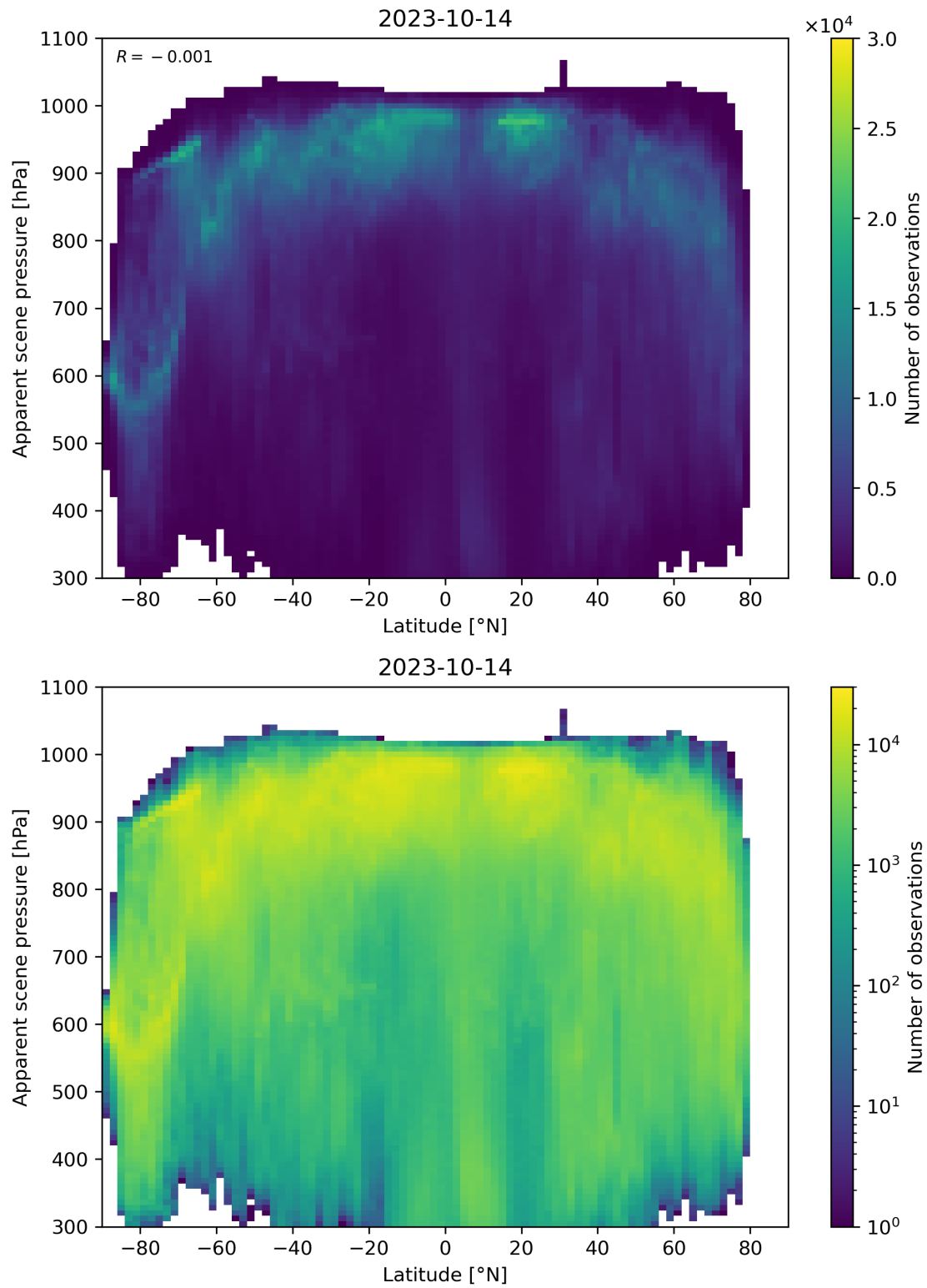
Figure 96: Scatter density plot of “Latitude” against “Apparent scene pressure” for 2023-10-13 to 2023-10-15.
