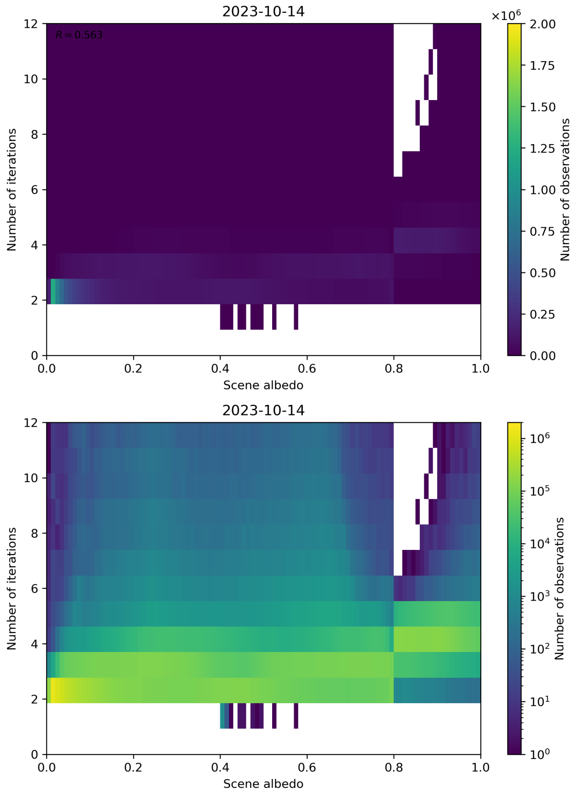
Figure 115: Scatter density plot of “Scene albedo” against “Number of iterations” for 2023-10-13 to 2023-10-15.
