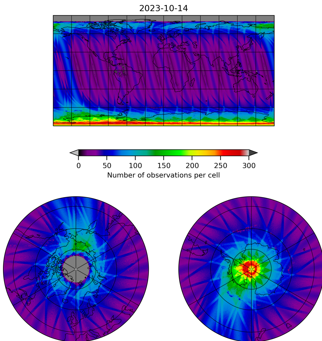
Figure 11: Map of the number of observations for 2023-10-13 to 2023-10-15
