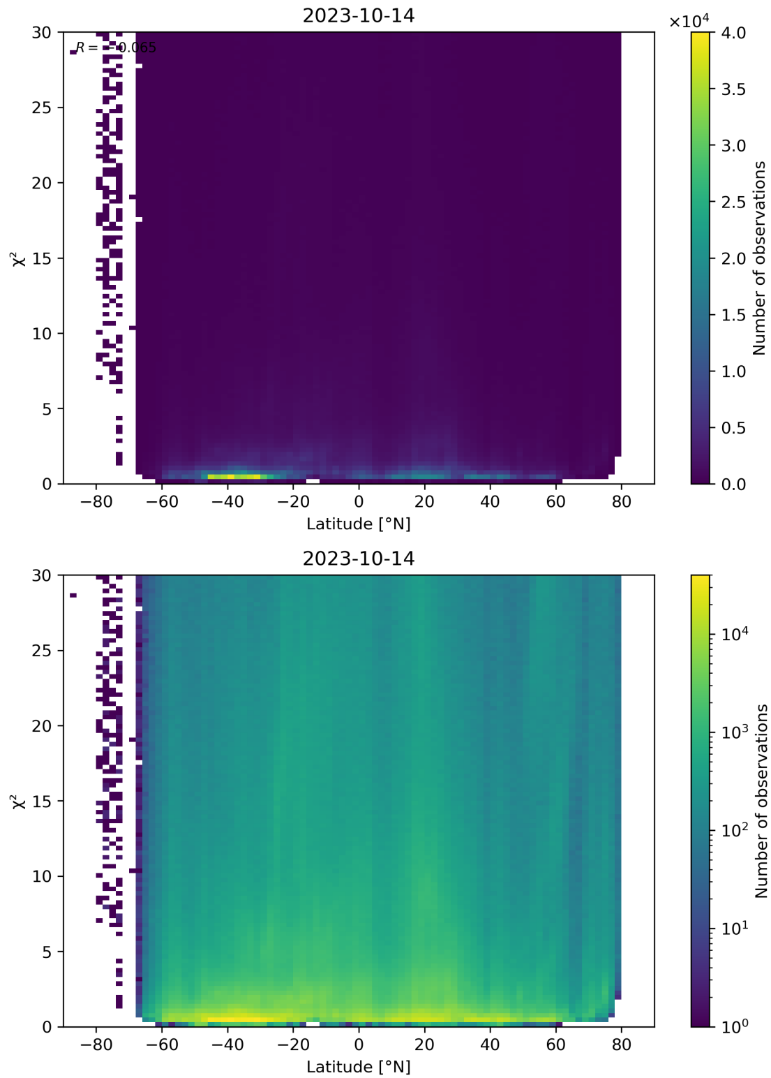
Figure 97: Scatter density plot of “Latitude” against “ \chi^2 ” for 2023-10-13 to 2023-10-15.
