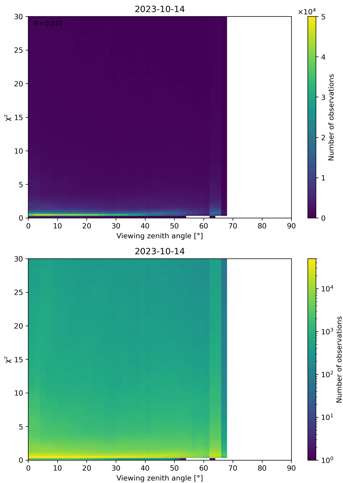
Figure 130: Scatter density plot of “Viewing zenith angle” against “ \chi^2 ” for 2023-10-13 to 2023-10-15.
