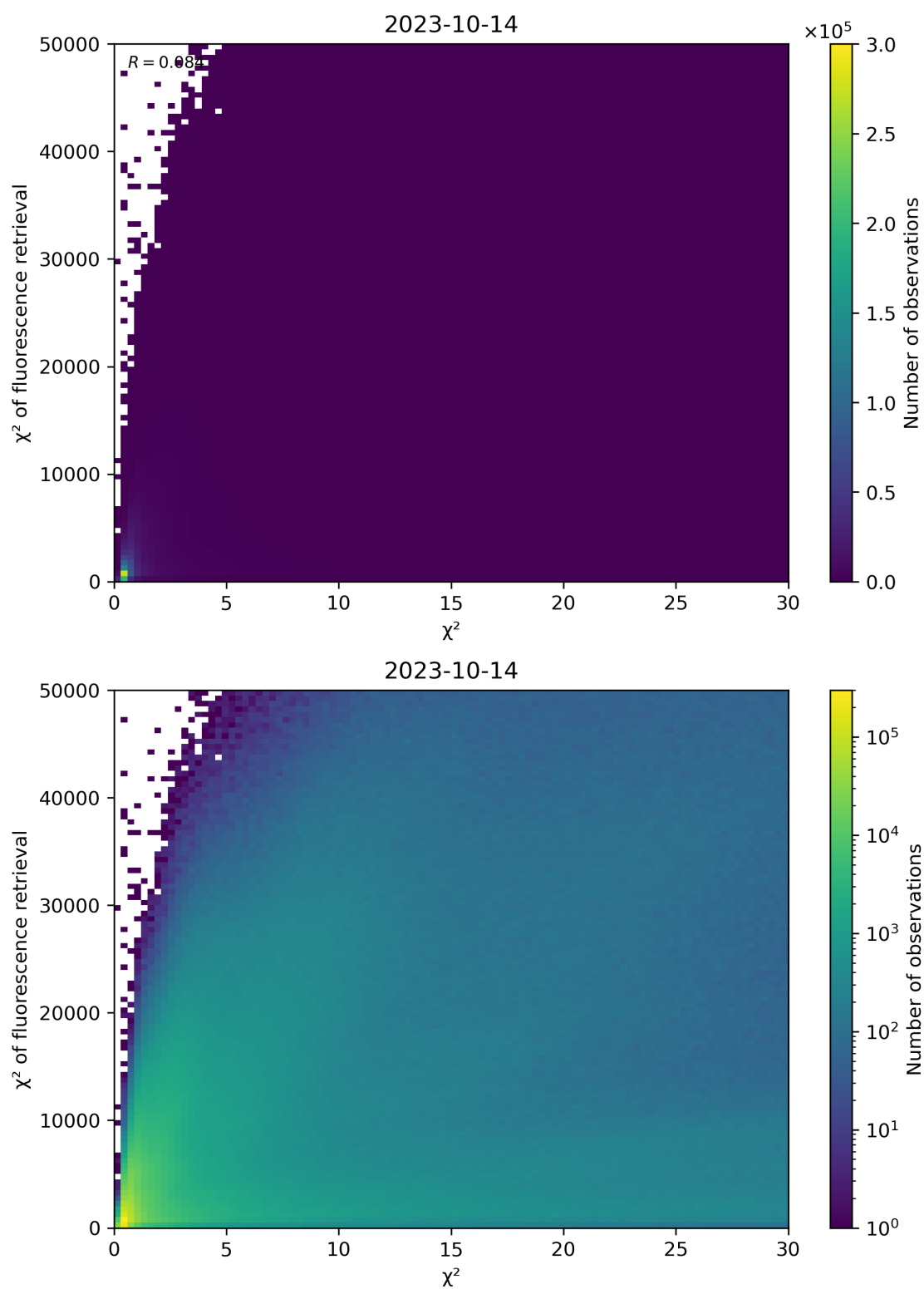
Figure 69: Scatter density plot of “ \chi^2 ” against “ \chi^2 of fluorescence retrieval” for 2023-10-13 to 2023-10-15.
