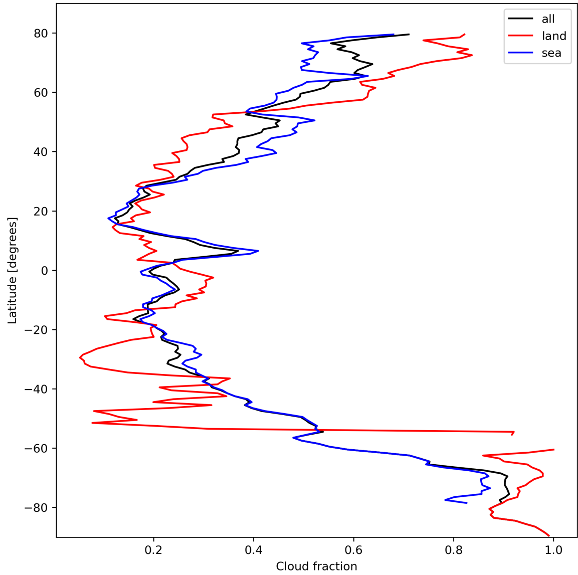
Figure 15: Zonal average of “Cloud fraction” for 2023-10-13 to 2023-10-15.
