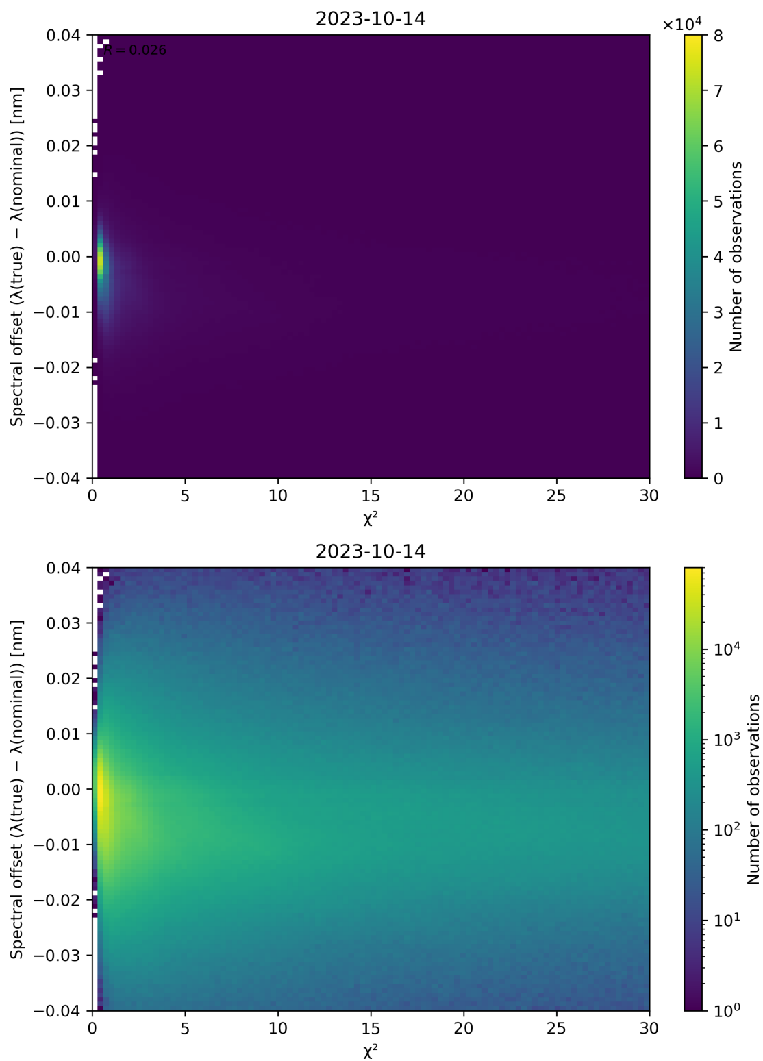
Figure 75: Scatter density plot of " \chi^2 " against "Spectral offset ( \lambda(\text{true}) - \lambda(\text{nominal}) )" for 2023-10-13 to 2023-10-15.
