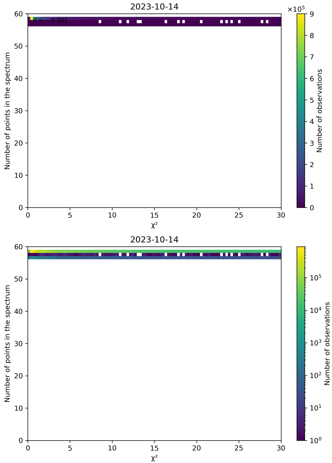
Figure 74: Scatter density plot of " \chi^2 " against "Number of points in the spectrum" for 2023-10-13 to 2023-10-15.
