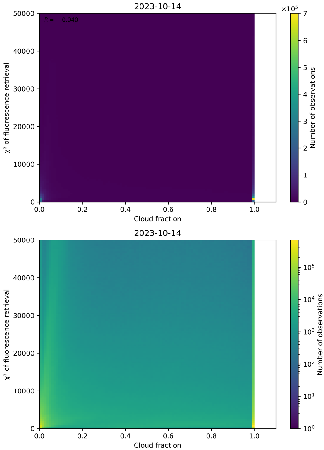
Figure 78: Scatter density plot of “Cloud fraction” against “ \chi^2 of fluorescence retrieval” for 2023-10-13 to 2023-10-15.
