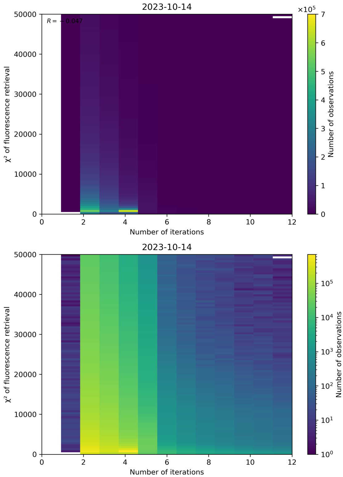
Figure 106: Scatter density plot of “Number of iterations” against “ \chi^2 of fluorescence retrieval” for 2023-10-13 to 2023-10-15.
