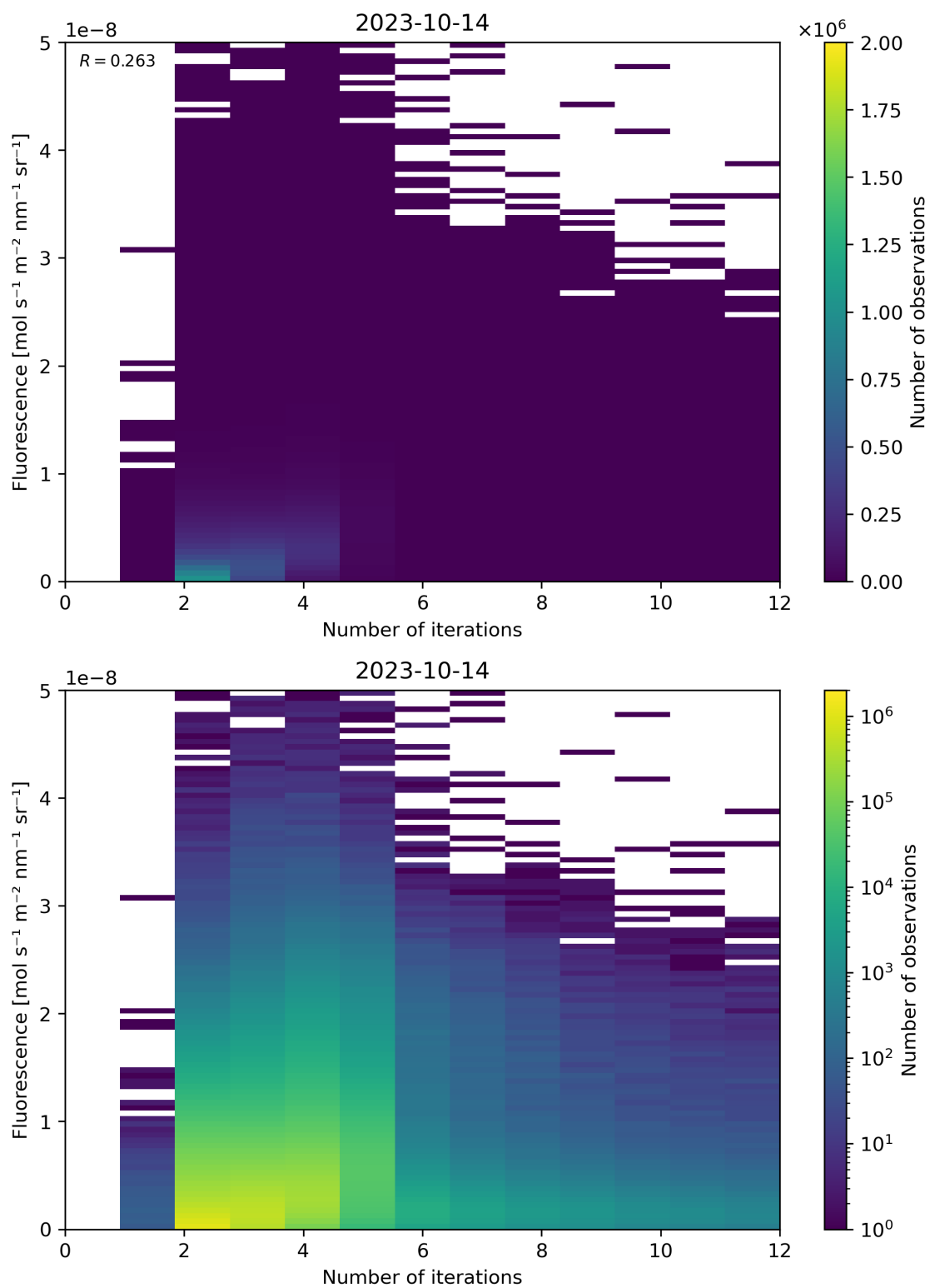
Figure 107: Scatter density plot of “Number of iterations” against “Fluorescence” for 2023-10-13 to 2023-10-15.
