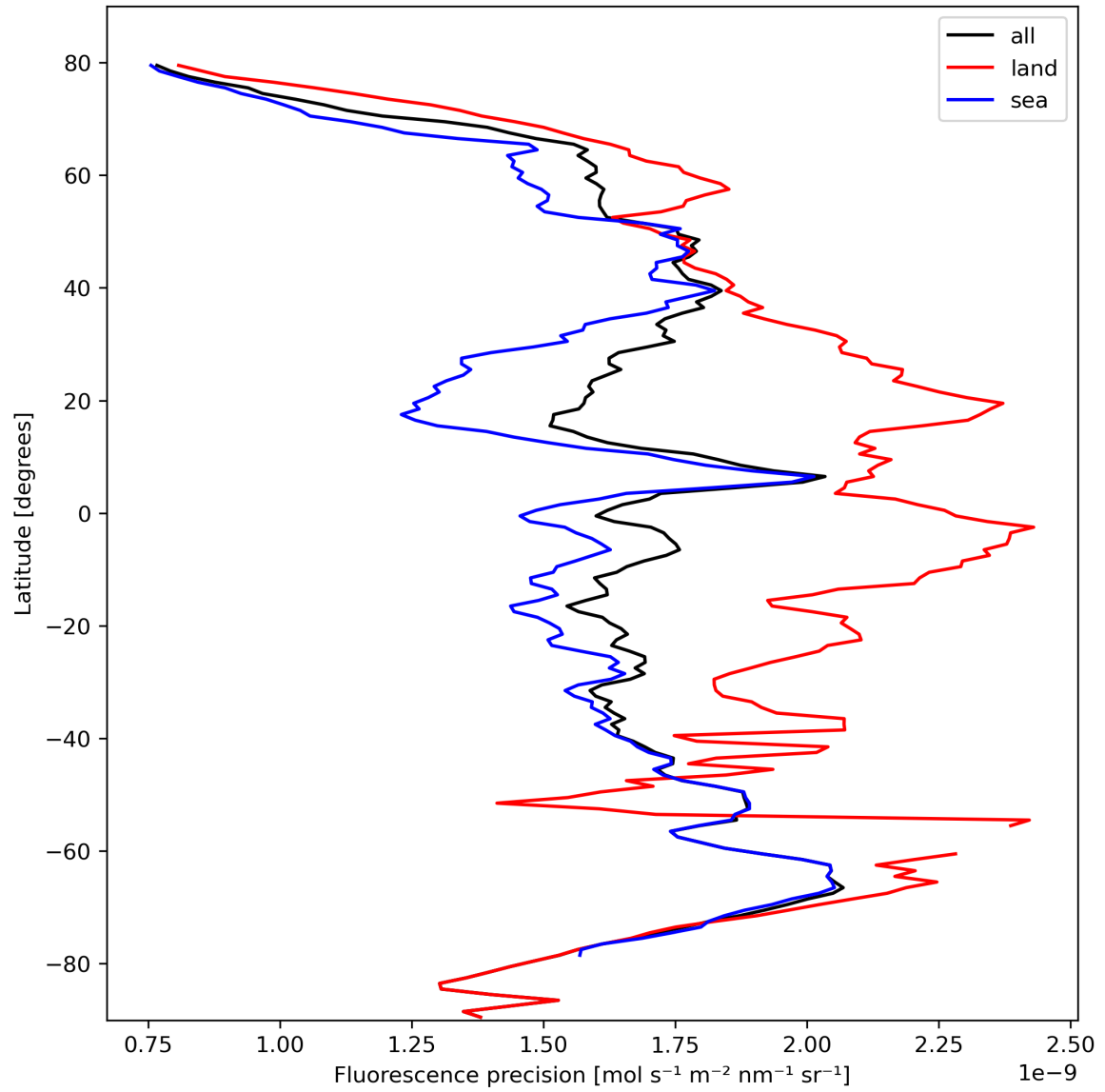
Figure 24: Zonal average of “Fluorescence precision” for 2023-10-13 to 2023-10-15.
