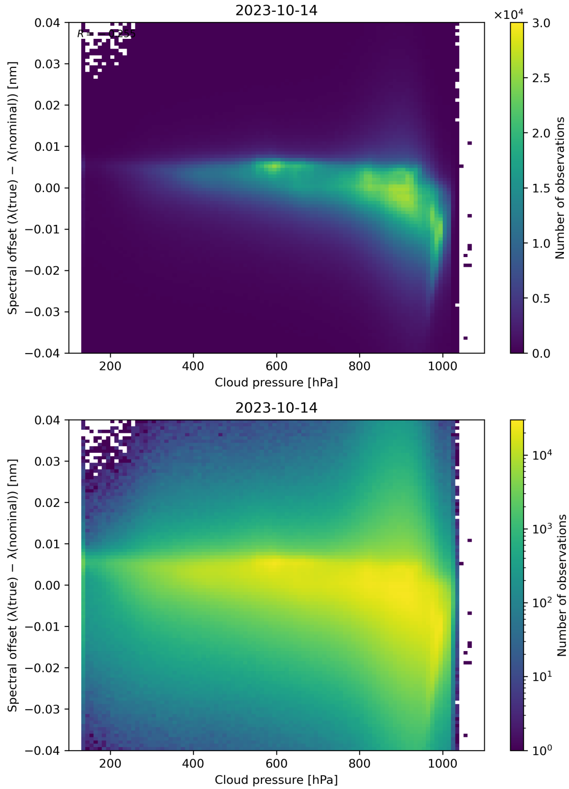
Figure 92: Scatter density plot of “Cloud pressure” against “Spectral offset ( \lambda(\text{true}) - \lambda(\text{nominal}) )” for 2023-10-13 to 2023-10-15.
