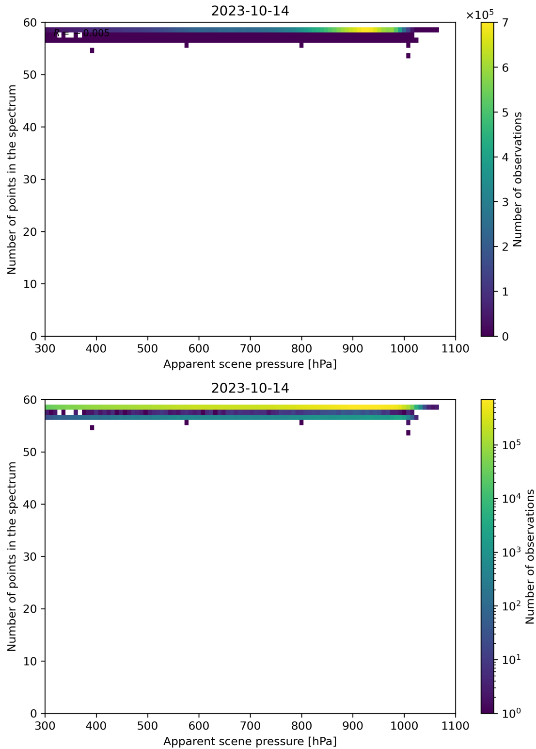
Figure 67: Scatter density plot of “Apparent scene pressure” against “Number of points in the spectrum” for 2023-10-13 to 2023-10-15.
