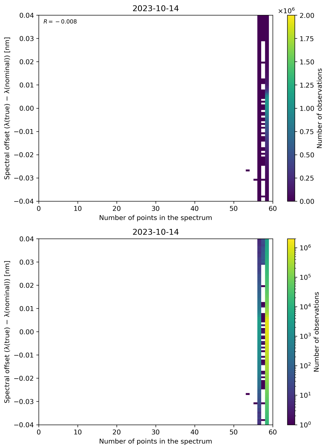
Figure 110: Scatter density plot of “Number of points in the spectrum” against “Spectral offset ( \lambda(\text{true}) - \lambda(\text{nominal}) )” for 2023-10-13 to 2023-10-15.
