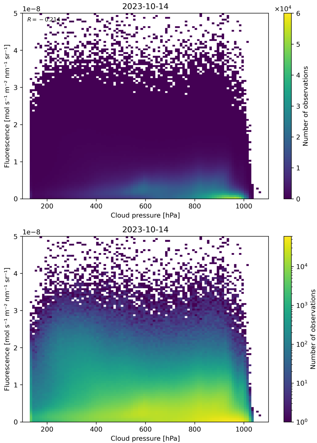
Figure 88: Scatter density plot of “Cloud pressure” against “Fluorescence” for 2023-10-13 to 2023-10-15.
