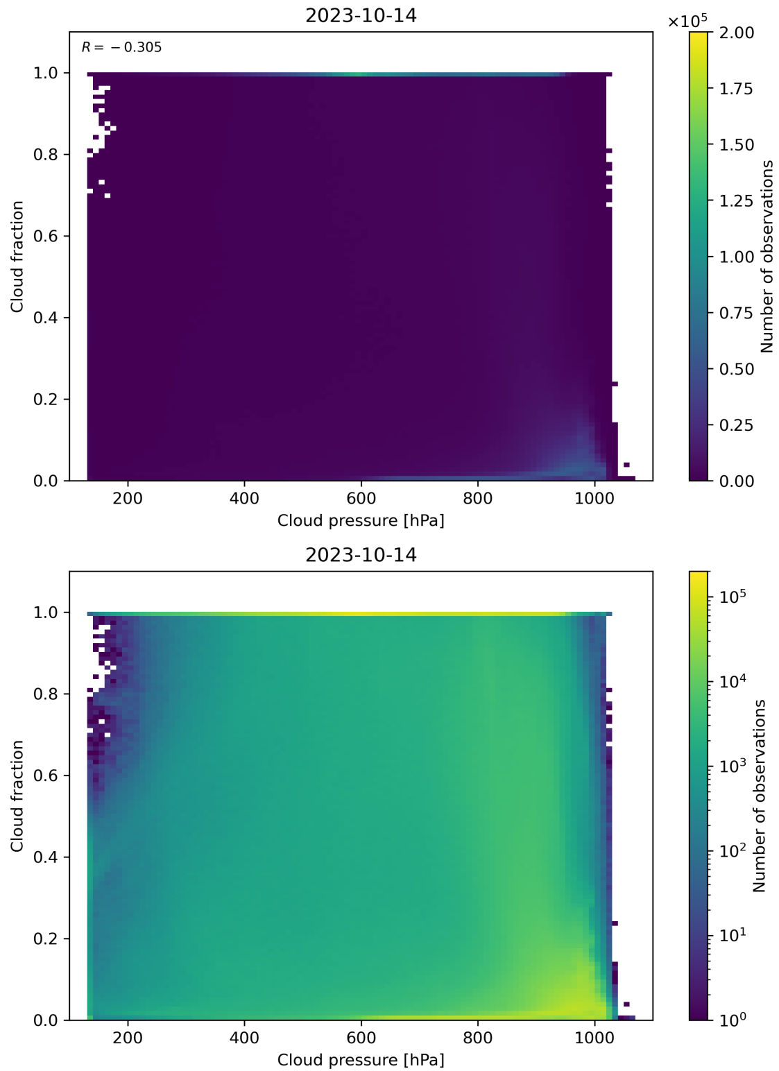
Figure 87: Scatter density plot of “Cloud pressure” against “Cloud fraction” for 2023-10-13 to 2023-10-15.
