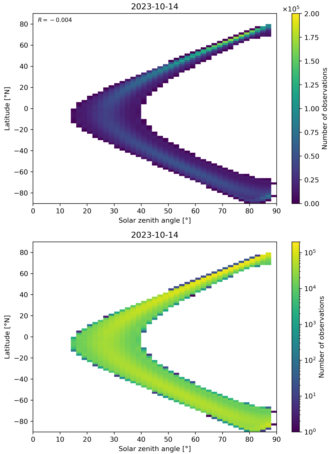
Figure 124: Scatter density plot of “Solar zenith angle” against “Latitude” for 2023-10-13 to 2023-10-15.
