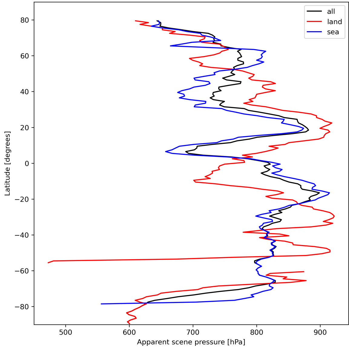
Figure 19: Zonal average of “Apparent scene pressure” for 2023-10-13 to 2023-10-15.
