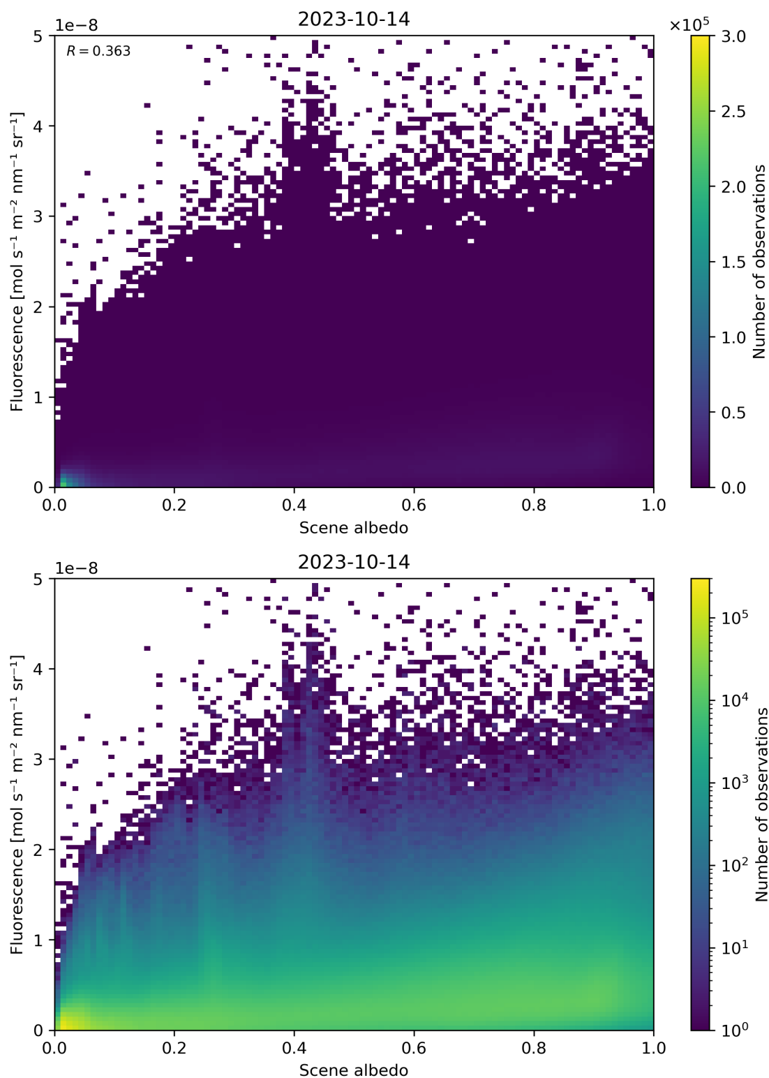
Figure 114: Scatter density plot of “Scene albedo” against “Fluorescence” for 2023-10-13 to 2023-10-15.
