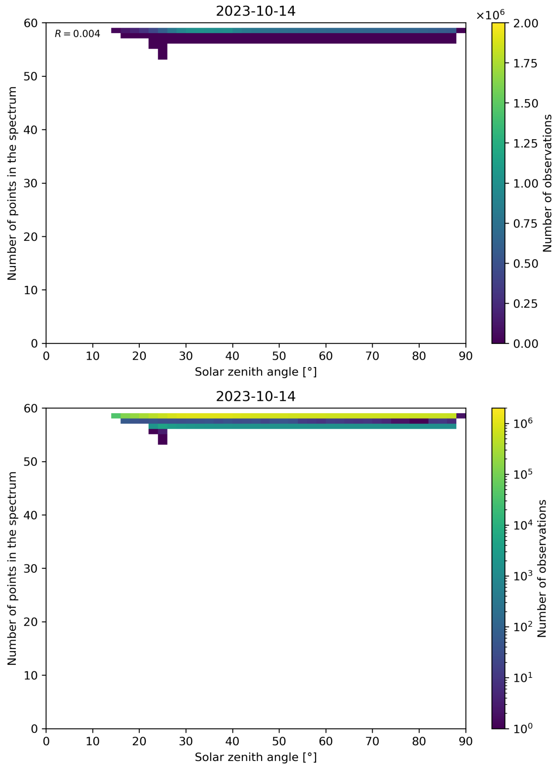
Figure 126: Scatter density plot of “Solar zenith angle” against “Number of points in the spectrum” for 2023-10-13 to 2023-10-15.
