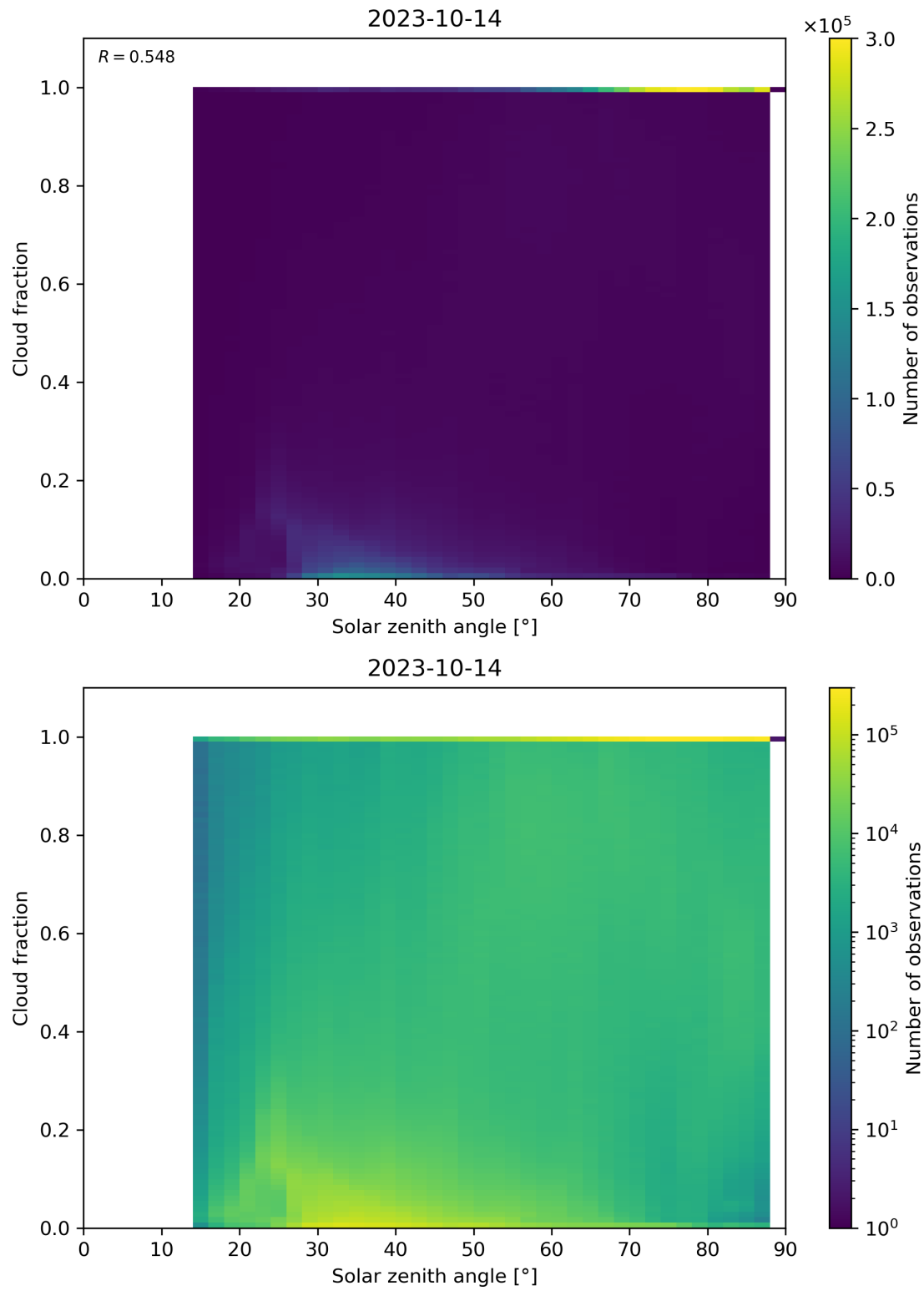
Figure 121: Scatter density plot of “Solar zenith angle” against “Cloud fraction” for 2023-10-13 to 2023-10-15.
