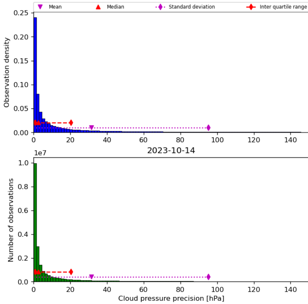
Figure 31: Histogram of “Cloud pressure precision” for 2023-10-13 to 2023-10-15
