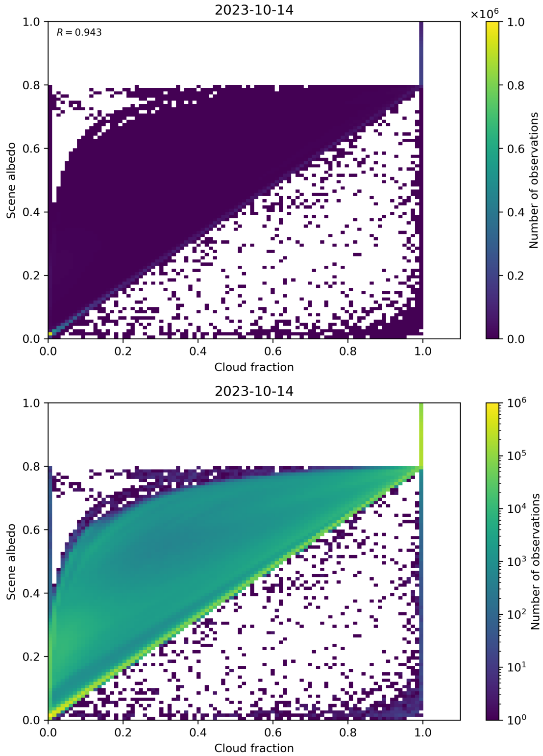
Figure 82: Scatter density plot of “Cloud fraction” against “Scene albedo” for 2023-10-13 to 2023-10-15.
