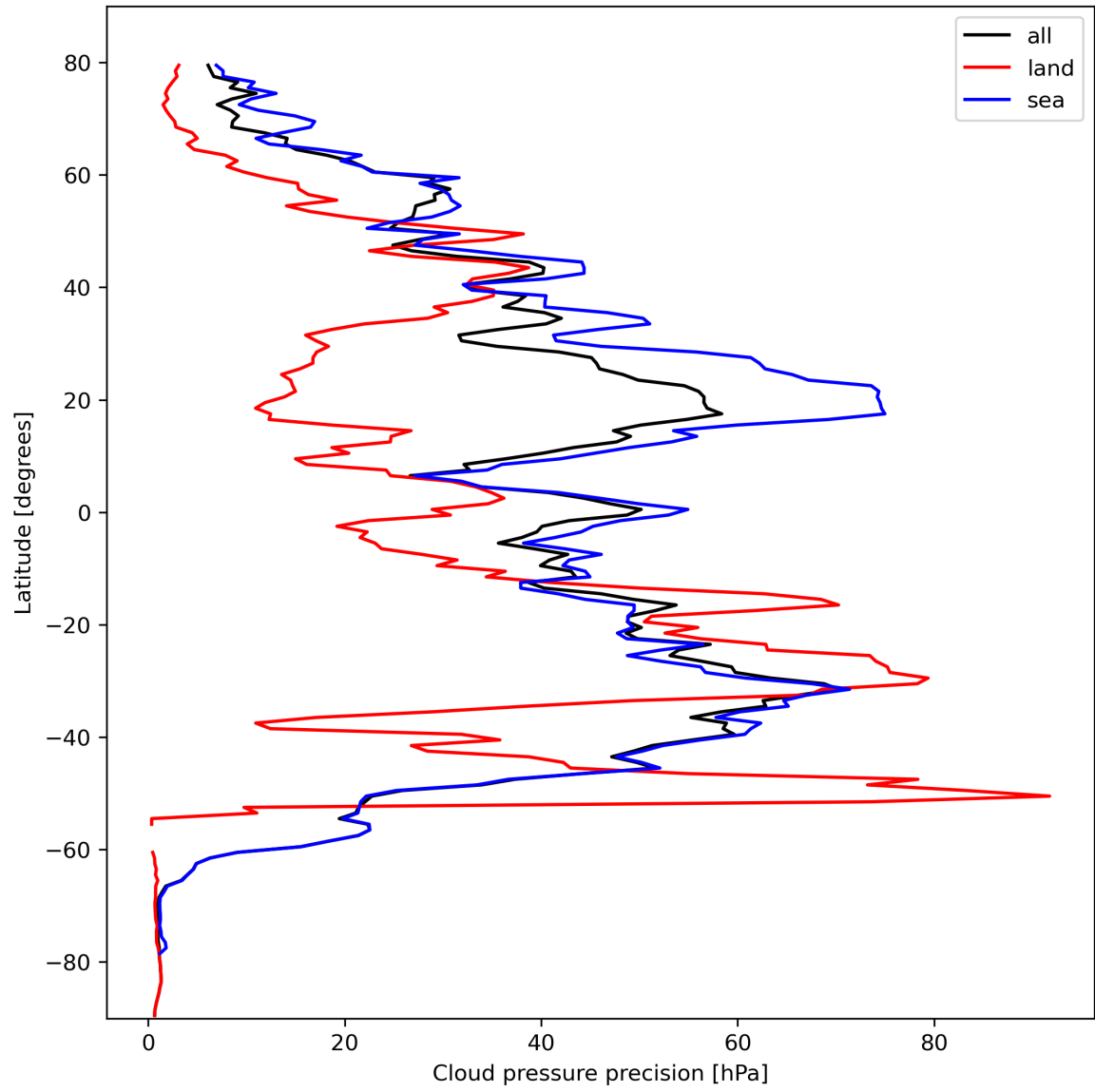
Figure 14: Zonal average of “Cloud pressure precision” for 2023-10-13 to 2023-10-15.
