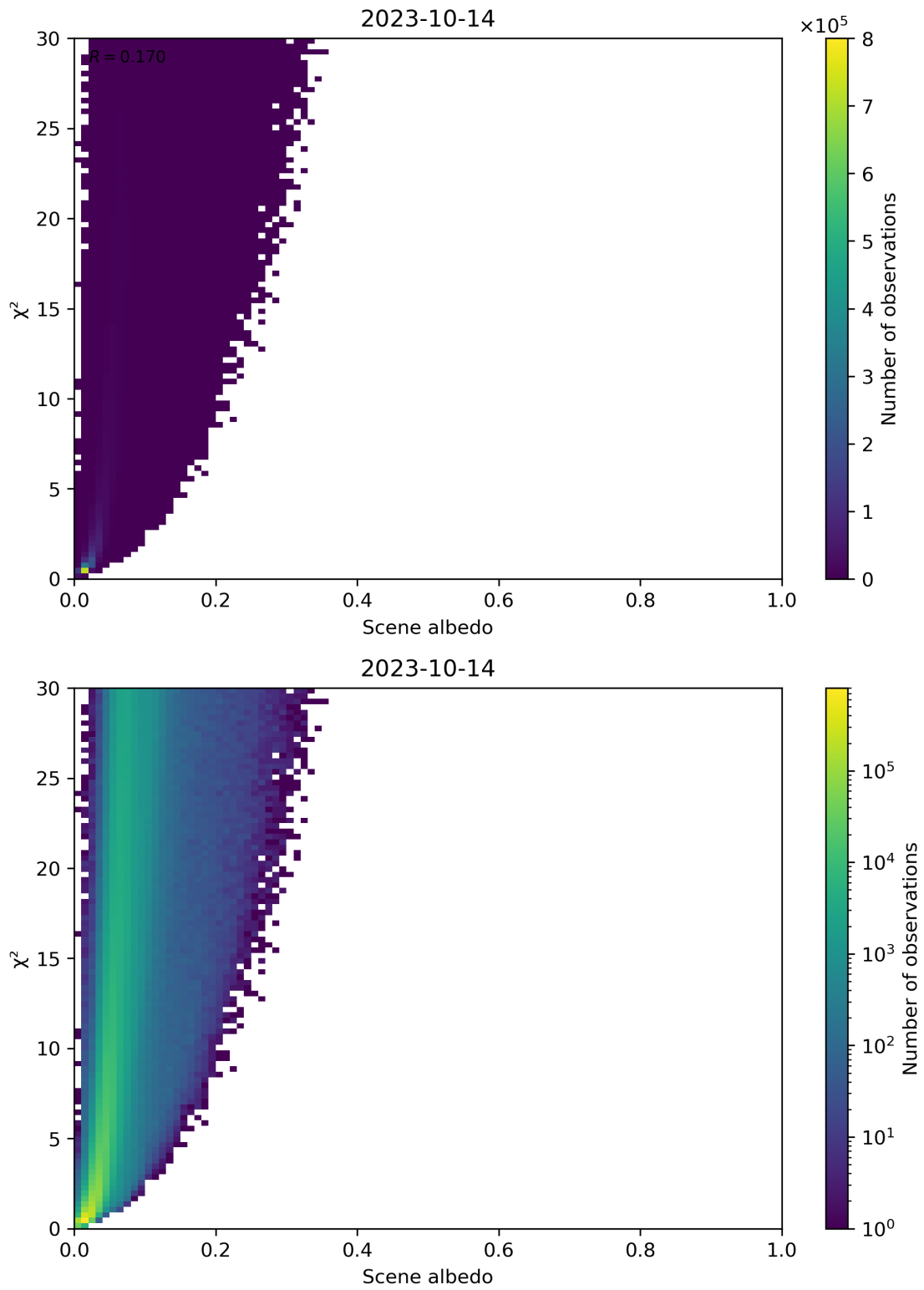
Figure 112: Scatter density plot of “Scene albedo” against “ \chi^2 ” for 2023-10-13 to 2023-10-15.
