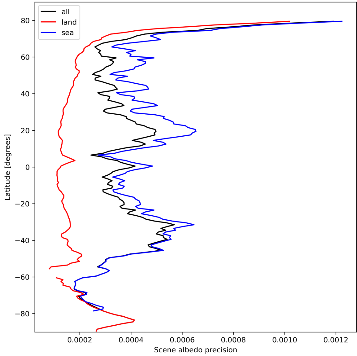
Figure 18: Zonal average of “Scene albedo precision” for 2023-10-13 to 2023-10-15.
