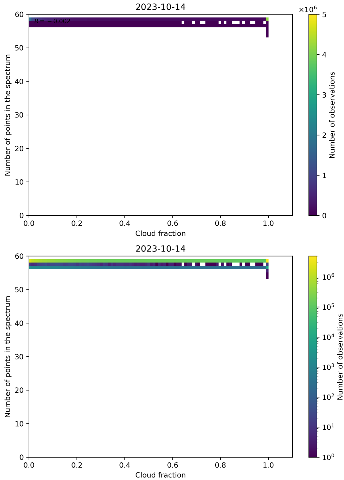
Figure 81: Scatter density plot of “Cloud fraction” against “Number of points in the spectrum” for 2023-10-13 to 2023-10-15.
