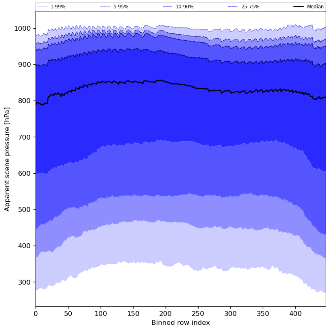
Figure 53: Along track statistics of “Apparent scene pressure” for 2023-10-13 to 2023-10-15
