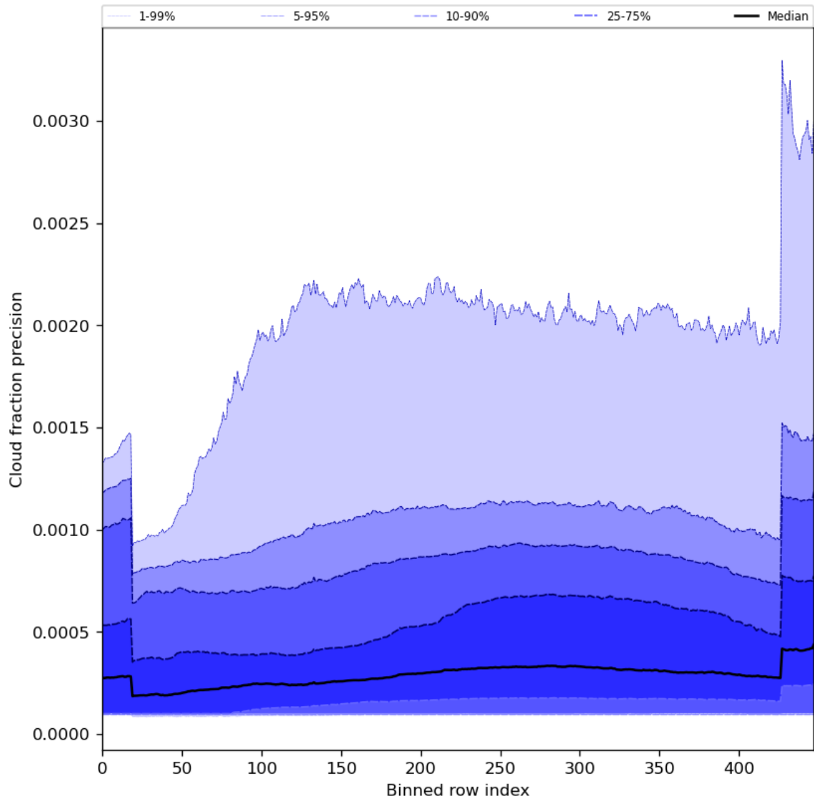
Figure 50: Along track statistics of “Cloud fraction precision” for 2023-10-13 to 2023-10-15
