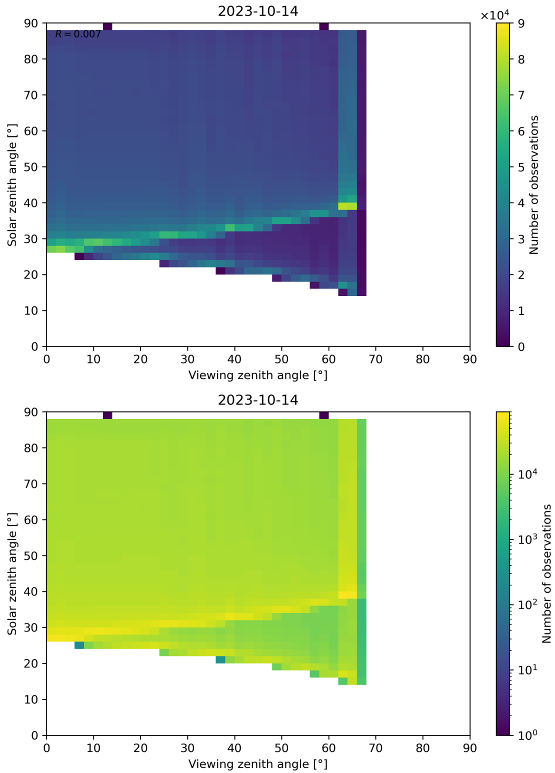
Figure 139: Scatter density plot of “Viewing zenith angle” against “Solar zenith angle” for 2023-10-13 to 2023-10-15.
