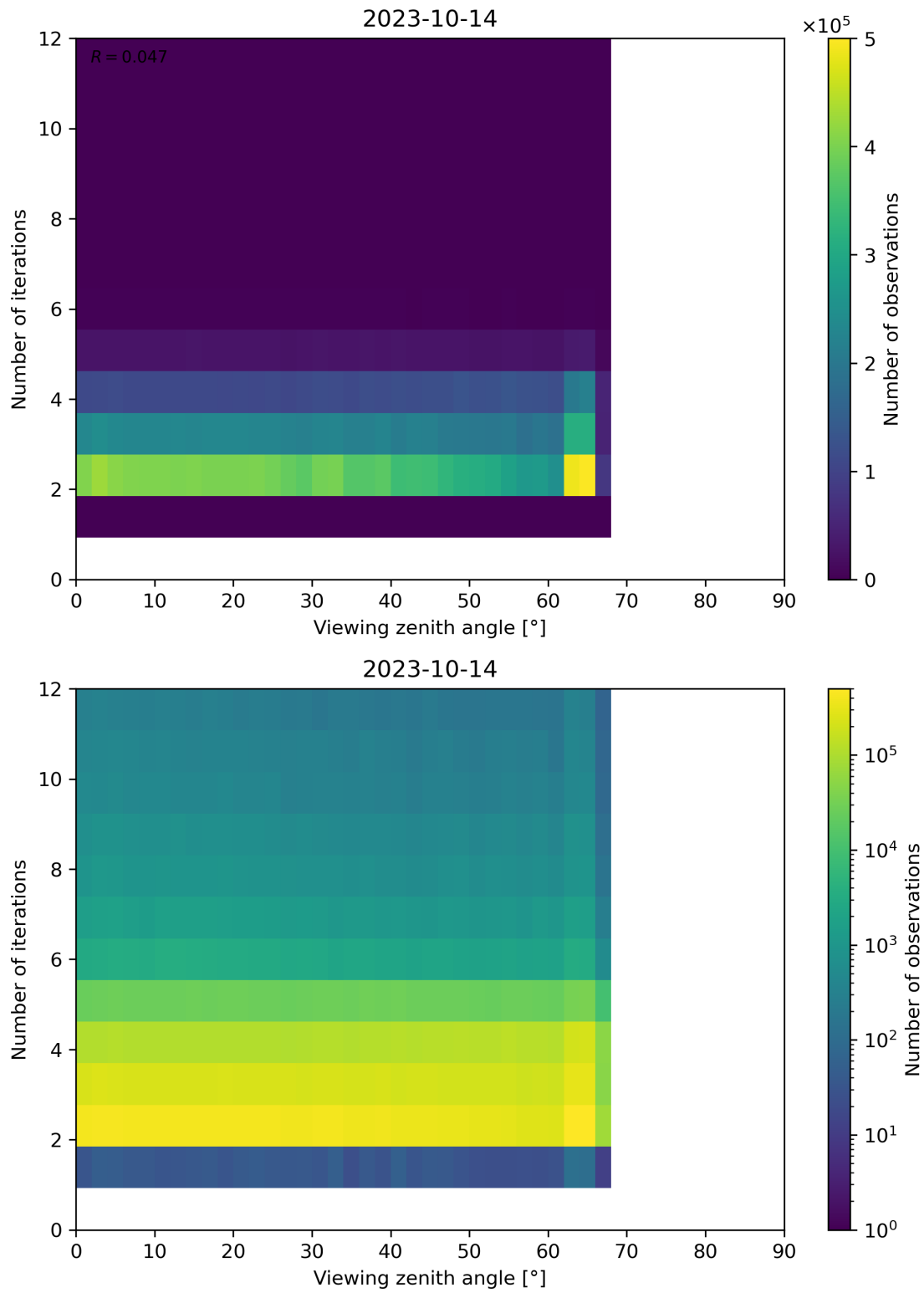
Figure 136: Scatter density plot of “Viewing zenith angle” against “Number of iterations” for 2023-10-13 to 2023-10-15.
