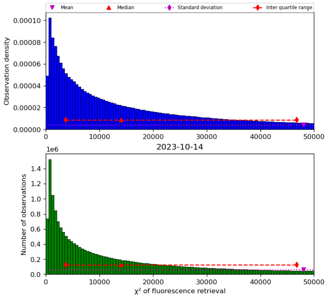
Figure 42: Histogram of “ \chi^2 of fluorescence retrieval” for 2023-10-13 to 2023-10-15
