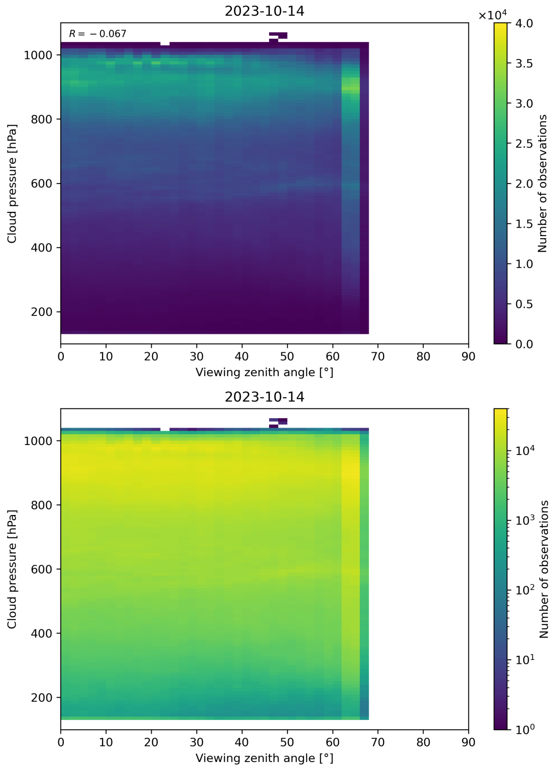
Figure 133: Scatter density plot of “Viewing zenith angle” against “Cloud pressure” for 2023-10-13 to 2023-10-15.
