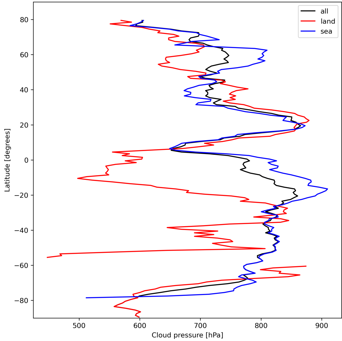
Figure 13: Zonal average of “Cloud pressure” for 2023-10-13 to 2023-10-15.
