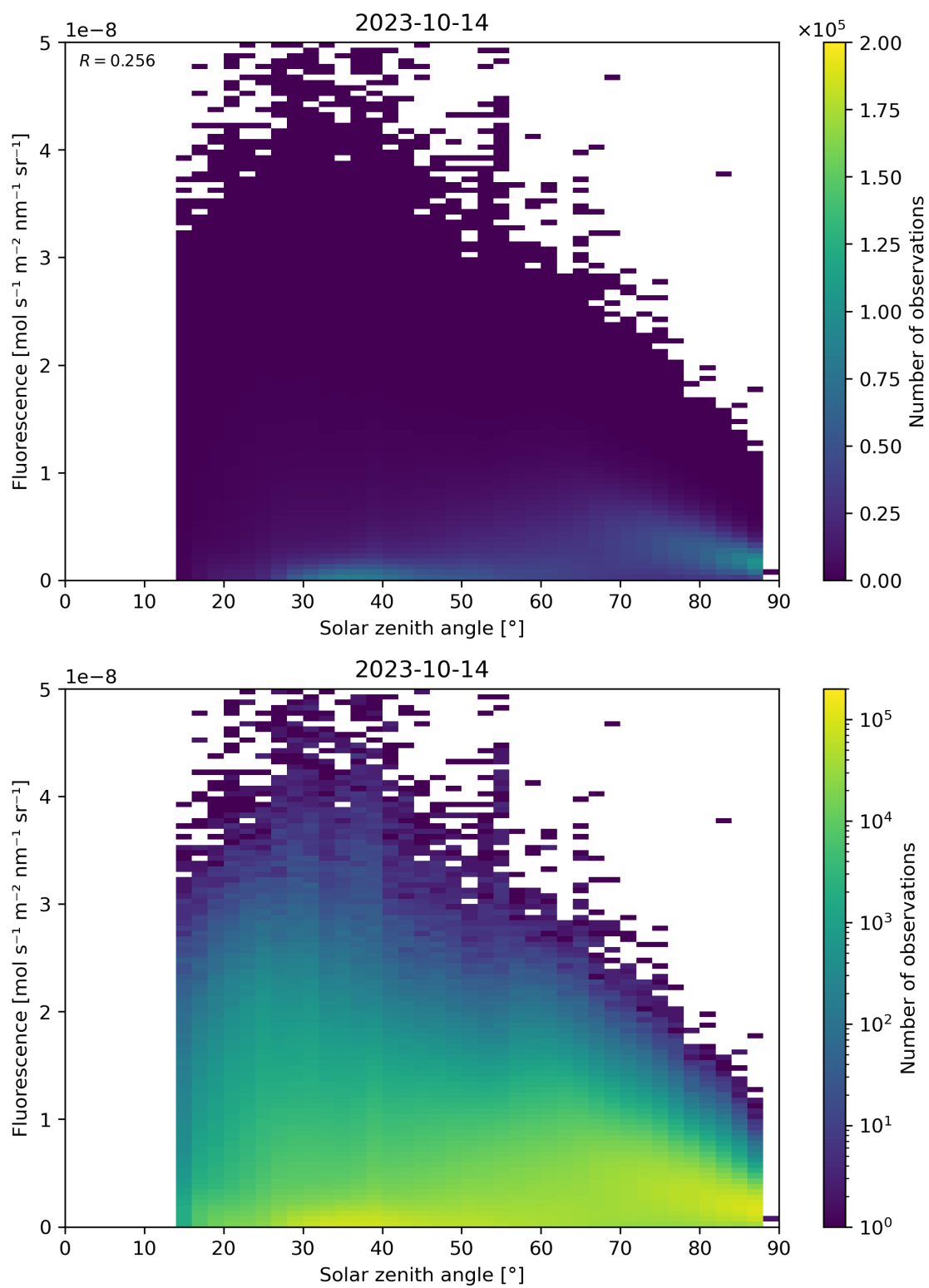
Figure 123: Scatter density plot of “Solar zenith angle” against “Fluorescence” for 2023-10-13 to 2023-10-15.
