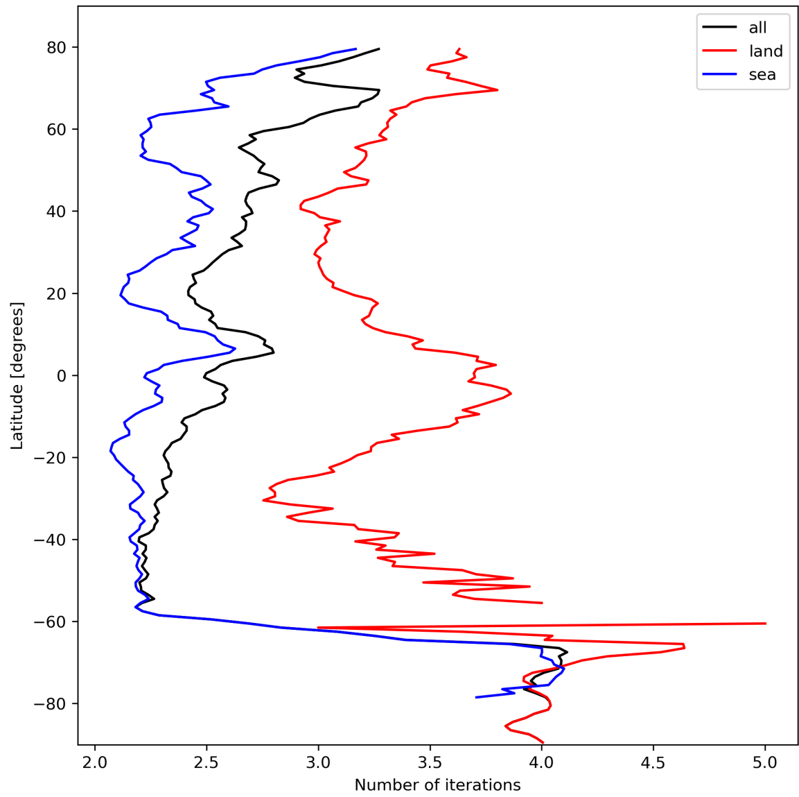
Figure 22: Zonal average of “Number of iterations” for 2023-10-13 to 2023-10-15.
