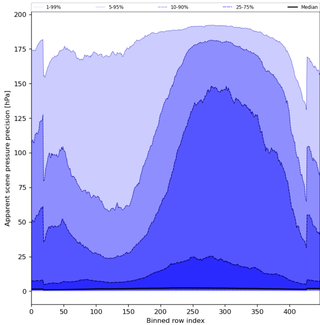
Figure 54: Along track statistics of “Apparent scene pressure precision” for 2023-10-13 to 2023-10-15
