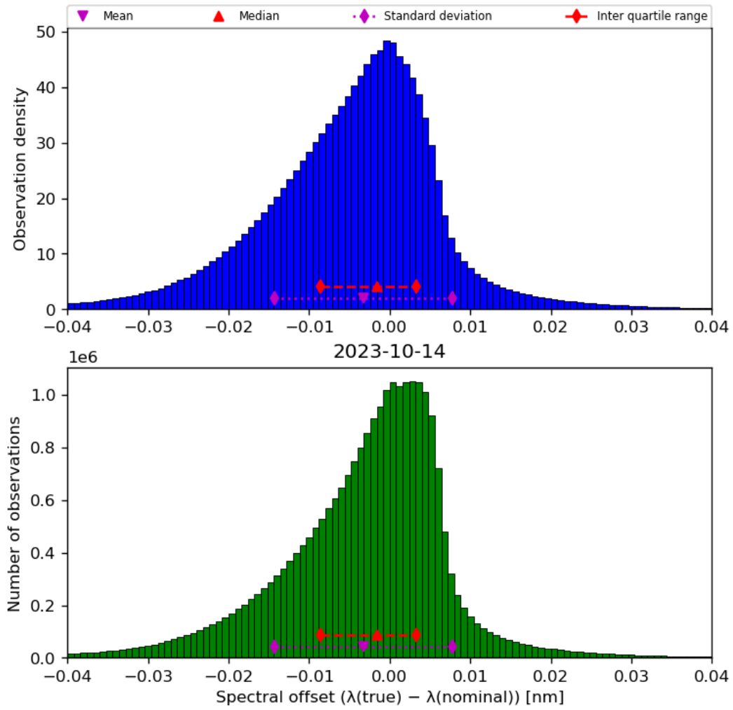
Figure 45: Histogram of “Spectral offset ( \lambda(\text{true}) - \lambda(\text{nominal}) )” for 2023-10-13 to 2023-10-15
