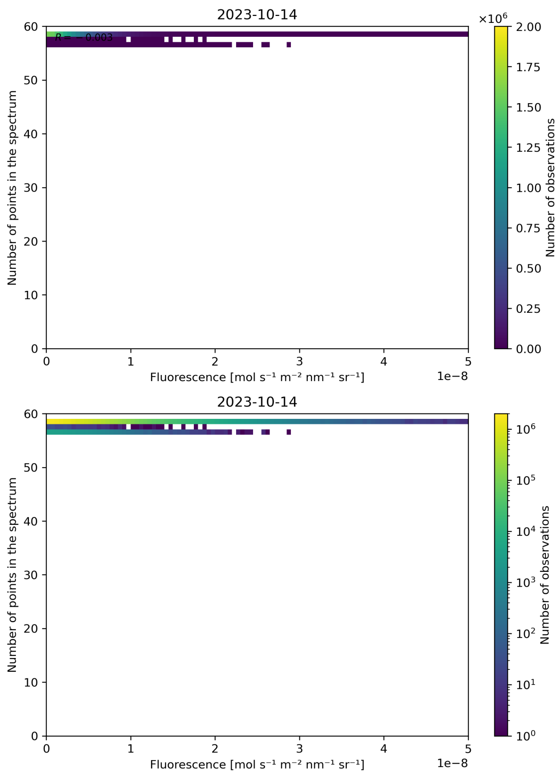
Figure 94: Scatter density plot of “Fluorescence” against “Number of points in the spectrum” for 2023-10-13 to 2023-10-15.
