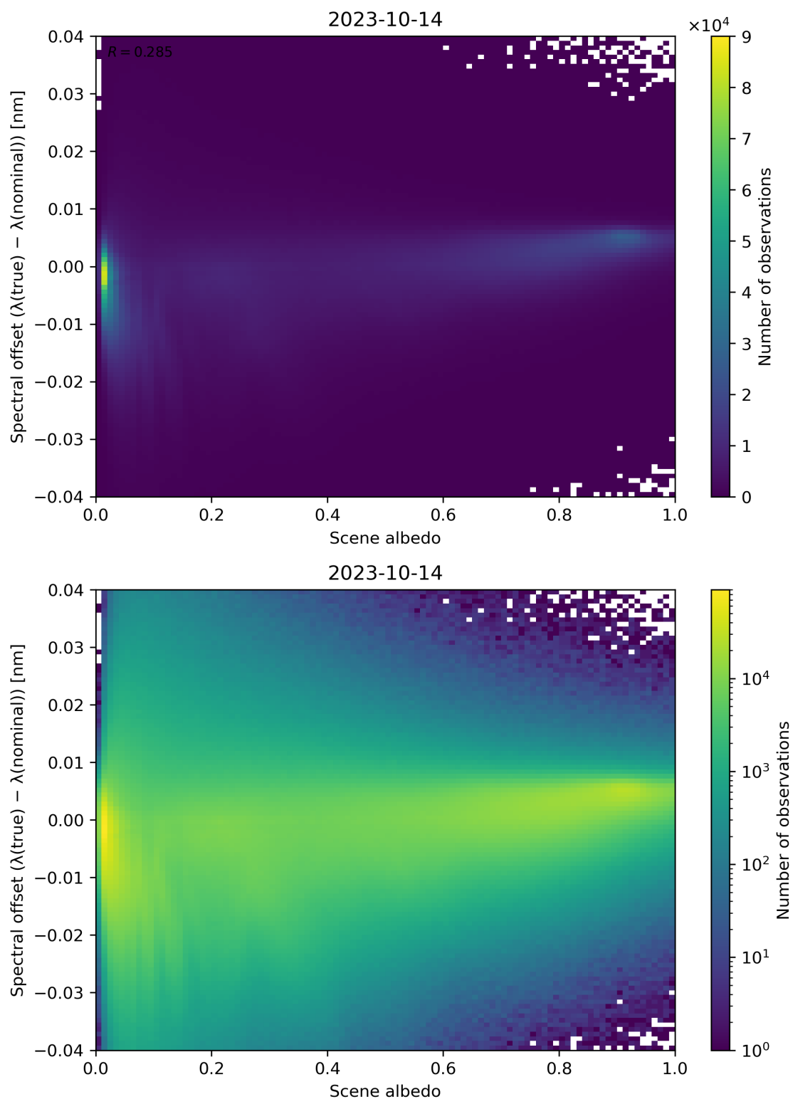
Figure 117: Scatter density plot of “Scene albedo” against “Spectral offset ( \lambda(\text{true}) - \lambda(\text{nominal}) )” for 2023-10-13 to 2023-10-15.
