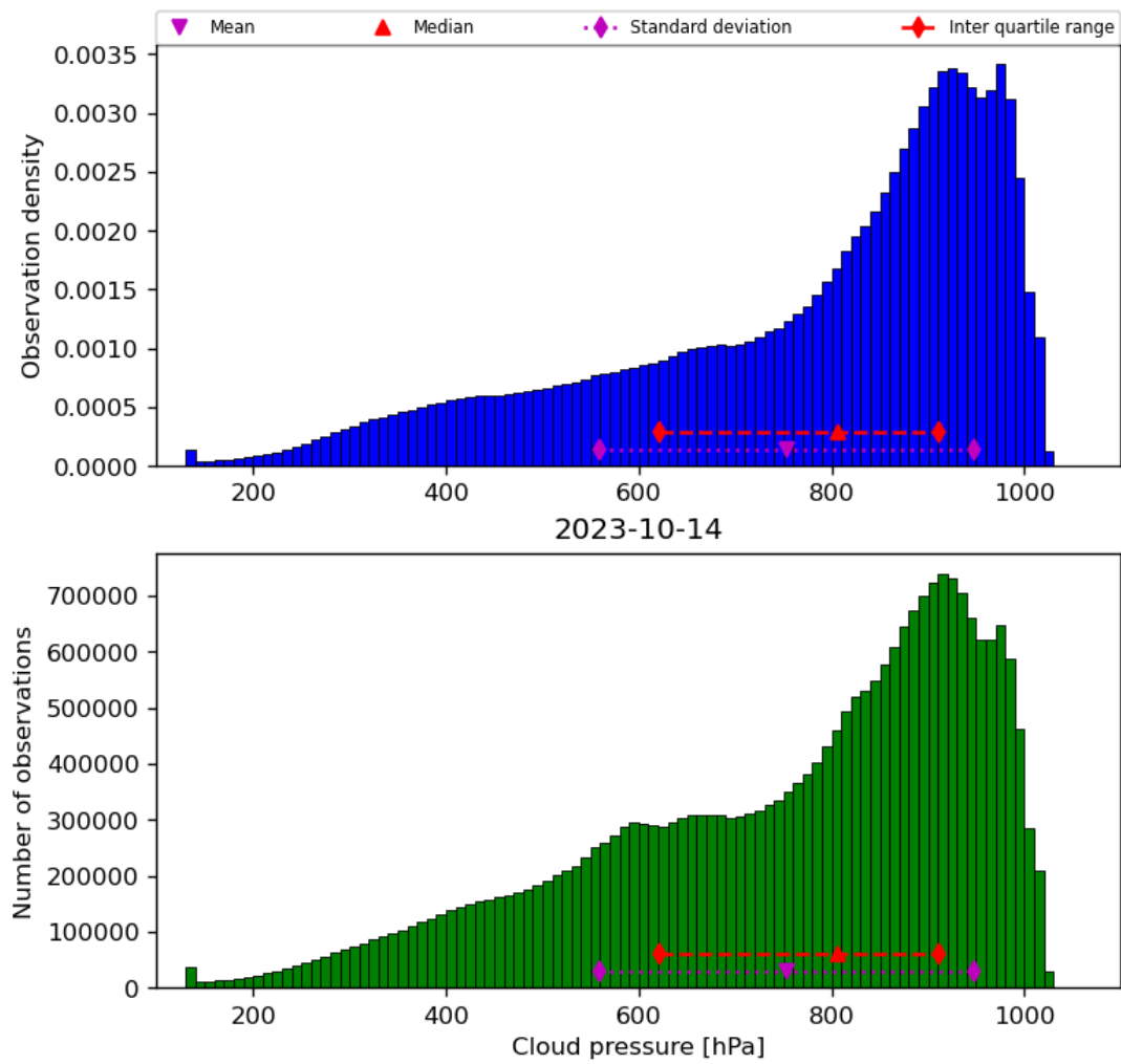
Figure 30: Histogram of “Cloud pressure” for 2023-10-13 to 2023-10-15
