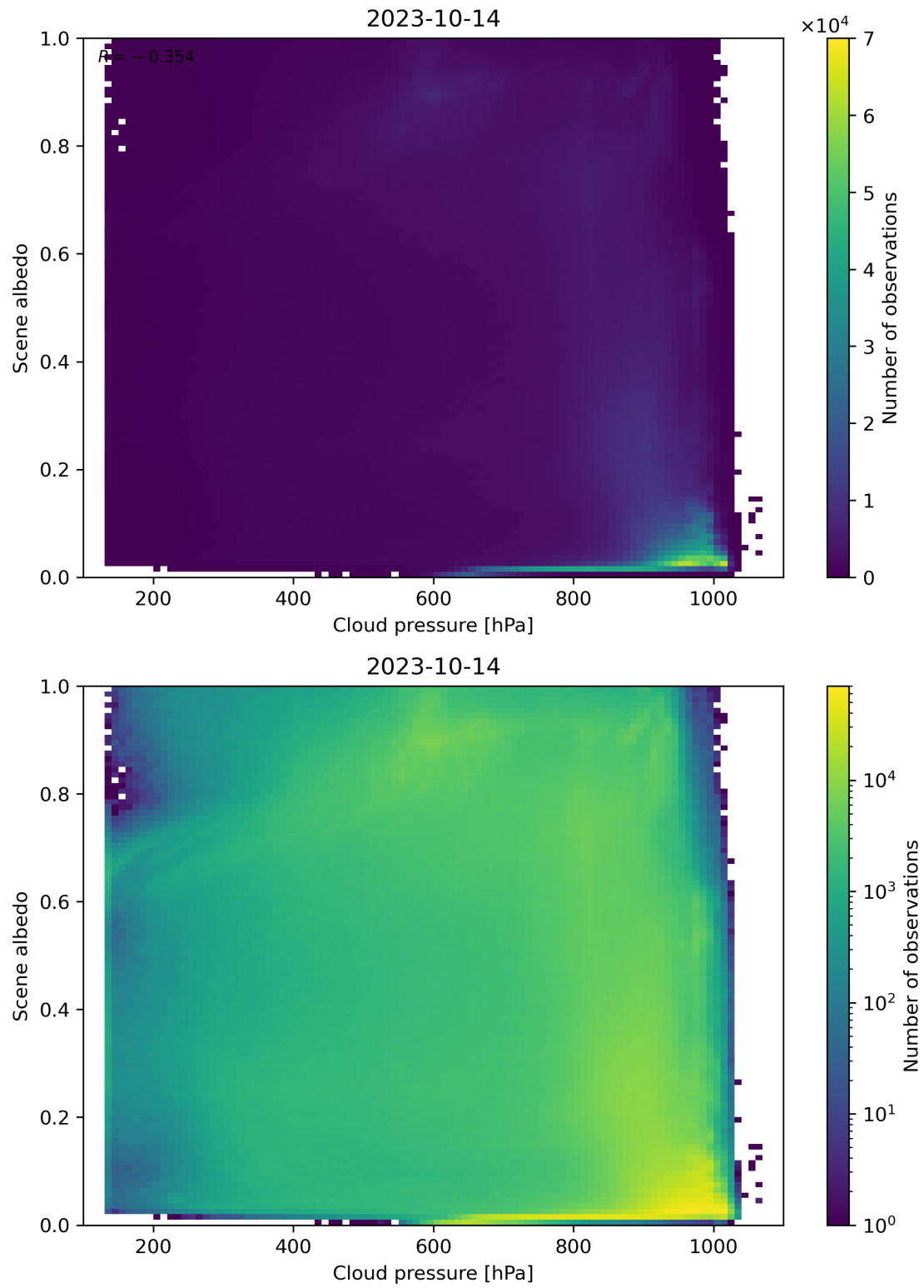
Figure 91: Scatter density plot of “Cloud pressure” against “Scene albedo” for 2023-10-13 to 2023-10-15.
