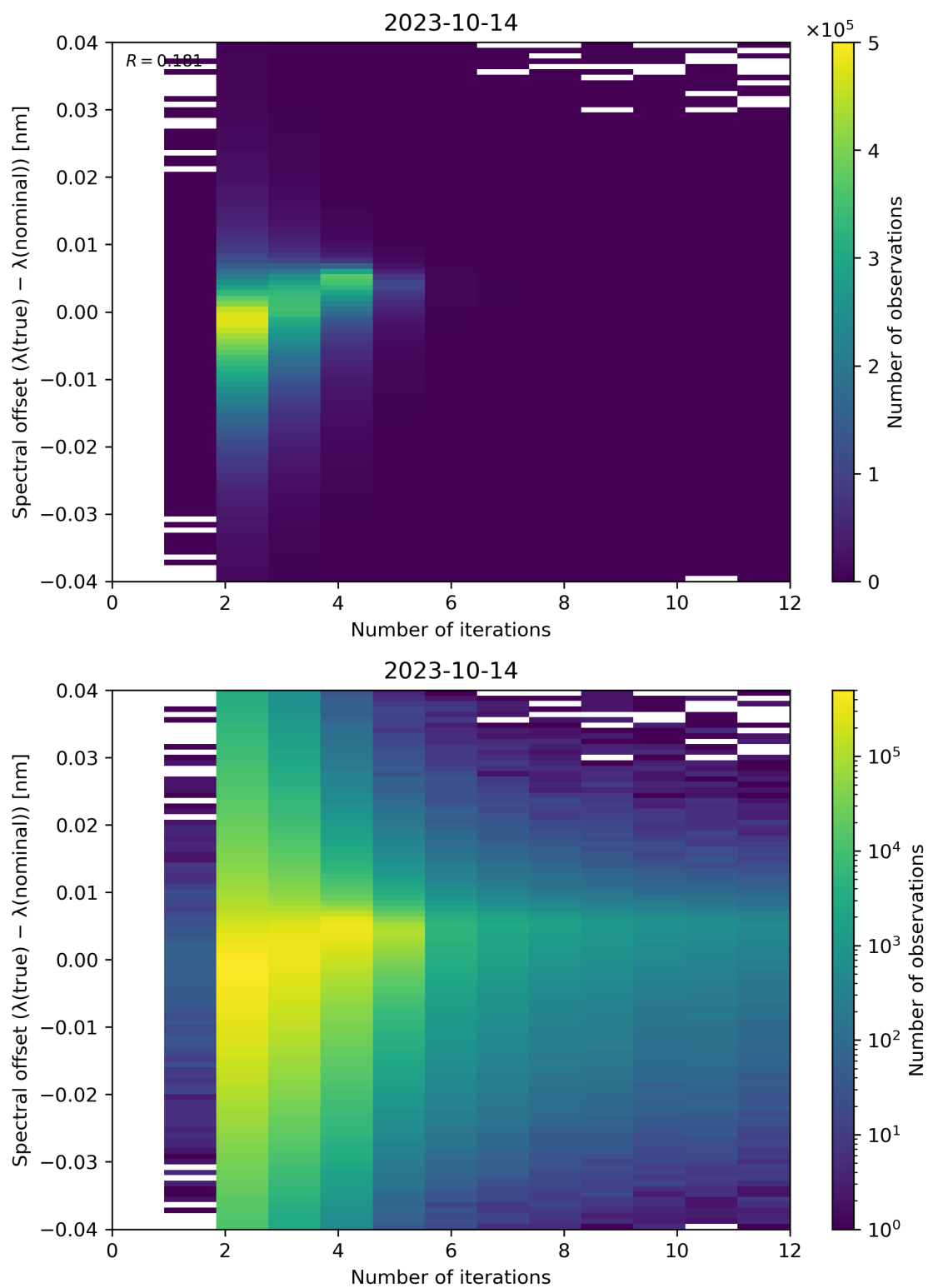
Figure 109: Scatter density plot of “Number of iterations” against “Spectral offset ( \lambda(\text{true}) - \lambda(\text{nominal}) )” for 2023-10-13 to 2023-10-15.
