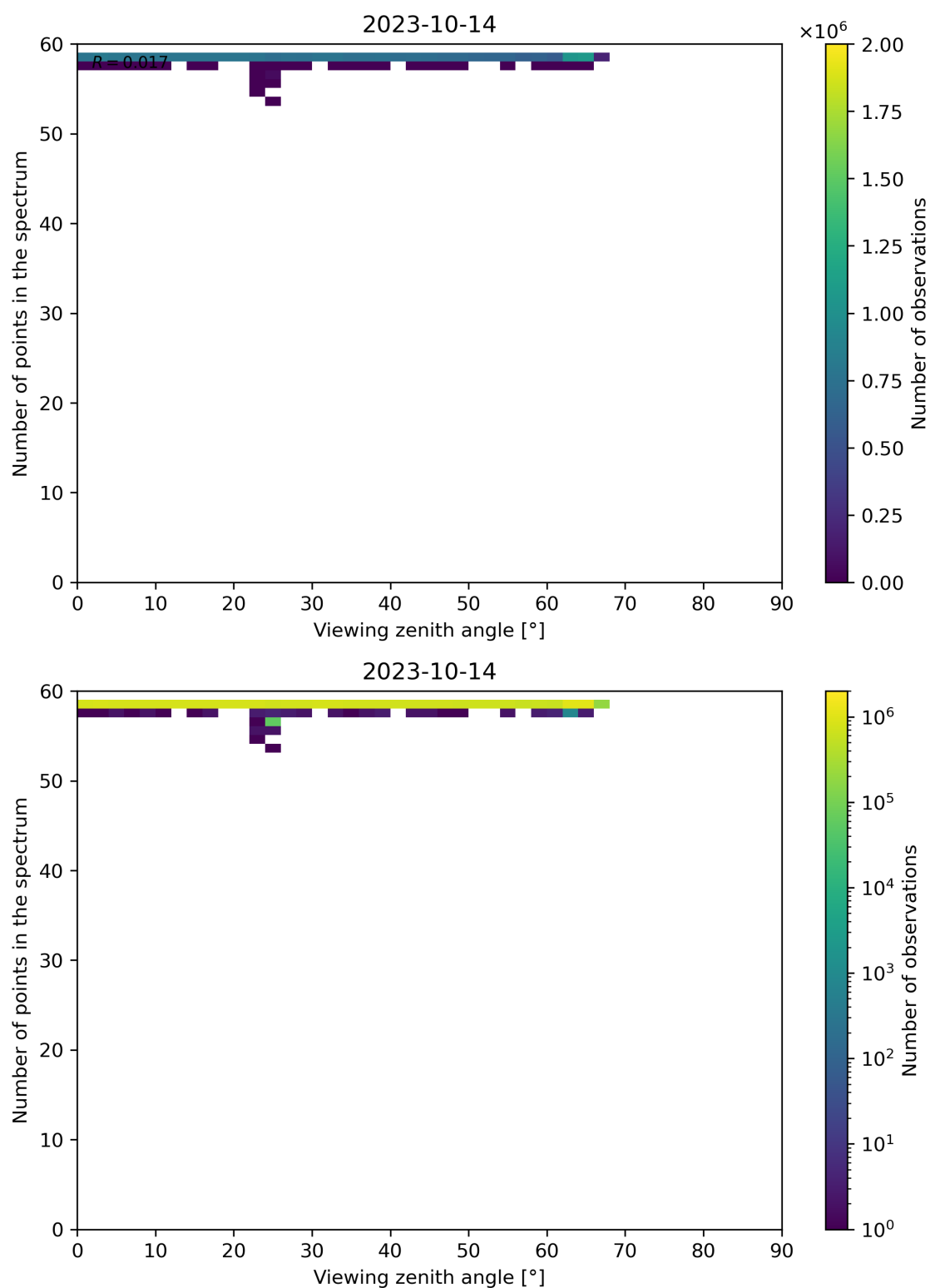
Figure 137: Scatter density plot of “Viewing zenith angle” against “Number of points in the spectrum” for 2023-10-13 to 2023-10-15.
