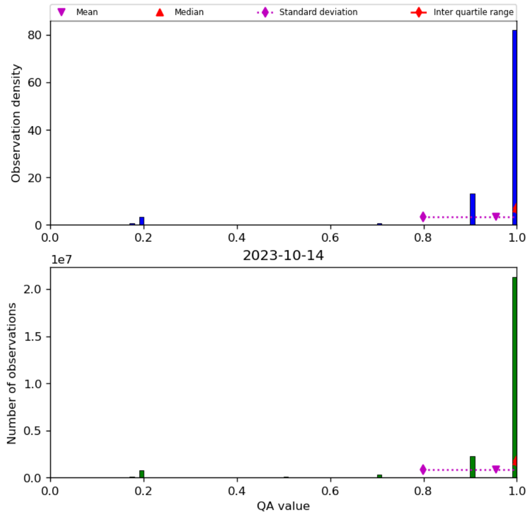
Figure 29: Histogram of “QA value” for 2023-10-13 to 2023-10-15
