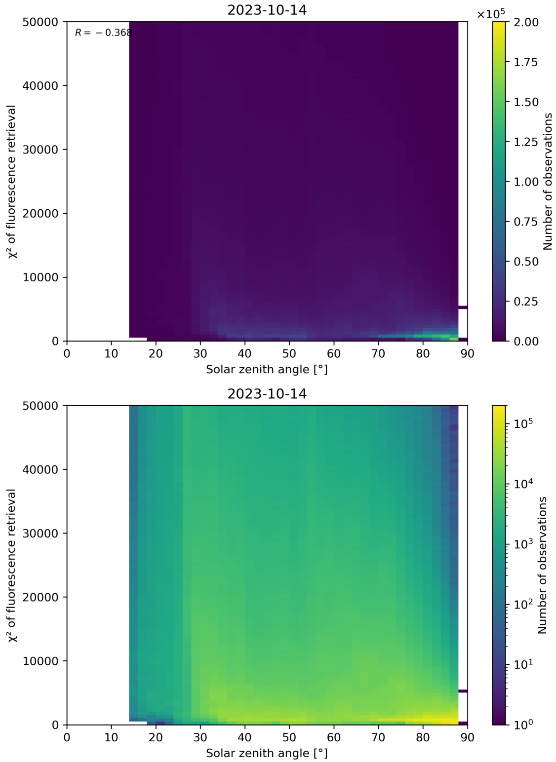
Figure 120: Scatter density plot of “Solar zenith angle” against “ \chi^2 of fluorescence retrieval” for 2023-10-13 to 2023-10-15.
