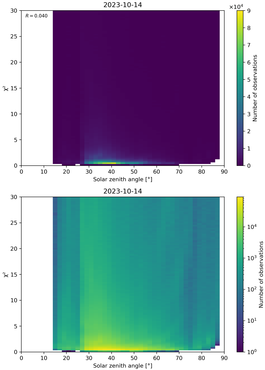
Figure 119: Scatter density plot of “Solar zenith angle” against “ \chi^2 ” for 2023-10-13 to 2023-10-15.
