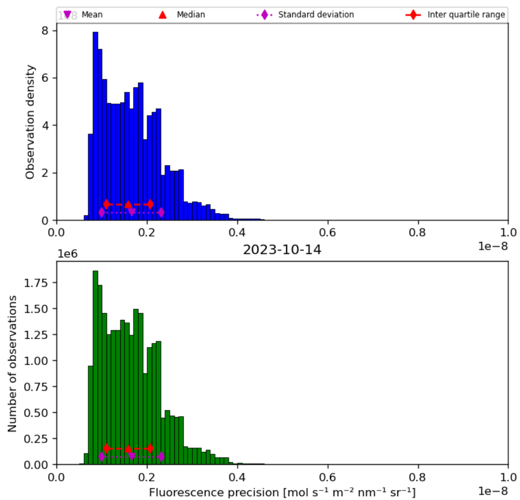
Figure 41: Histogram of “Fluorescence precision” for 2023-10-13 to 2023-10-15
