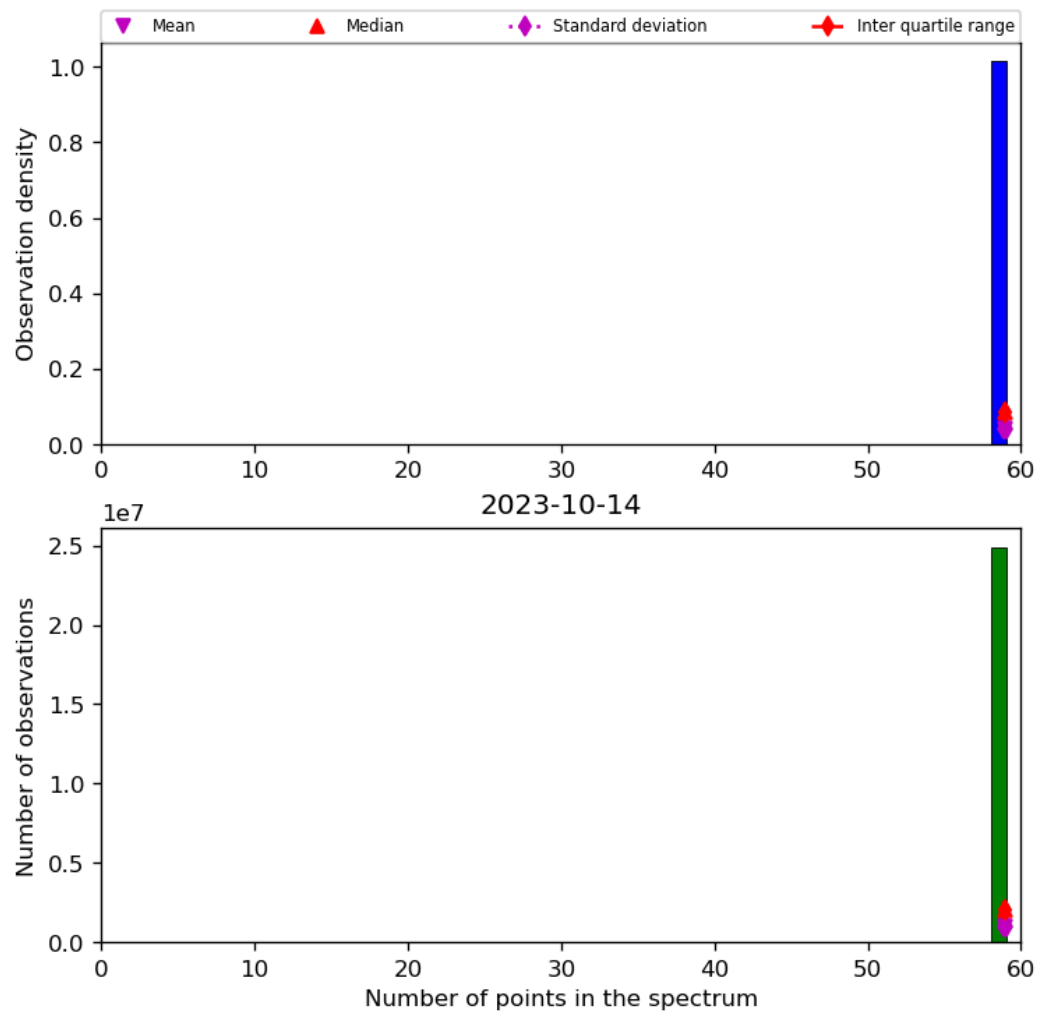
Figure 44: Histogram of “Number of points in the spectrum” for 2023-10-13 to 2023-10-15
