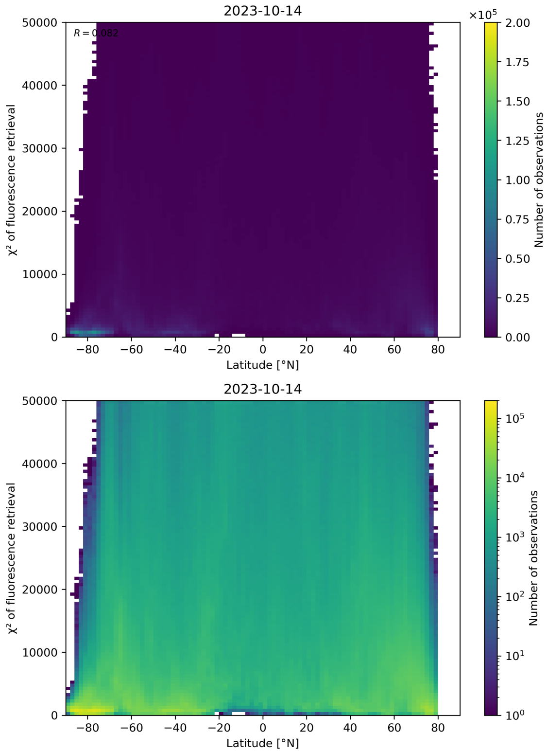
Figure 98: Scatter density plot of “Latitude” against “ \chi^2 of fluorescence retrieval” for 2023-10-13 to 2023-10-15.
