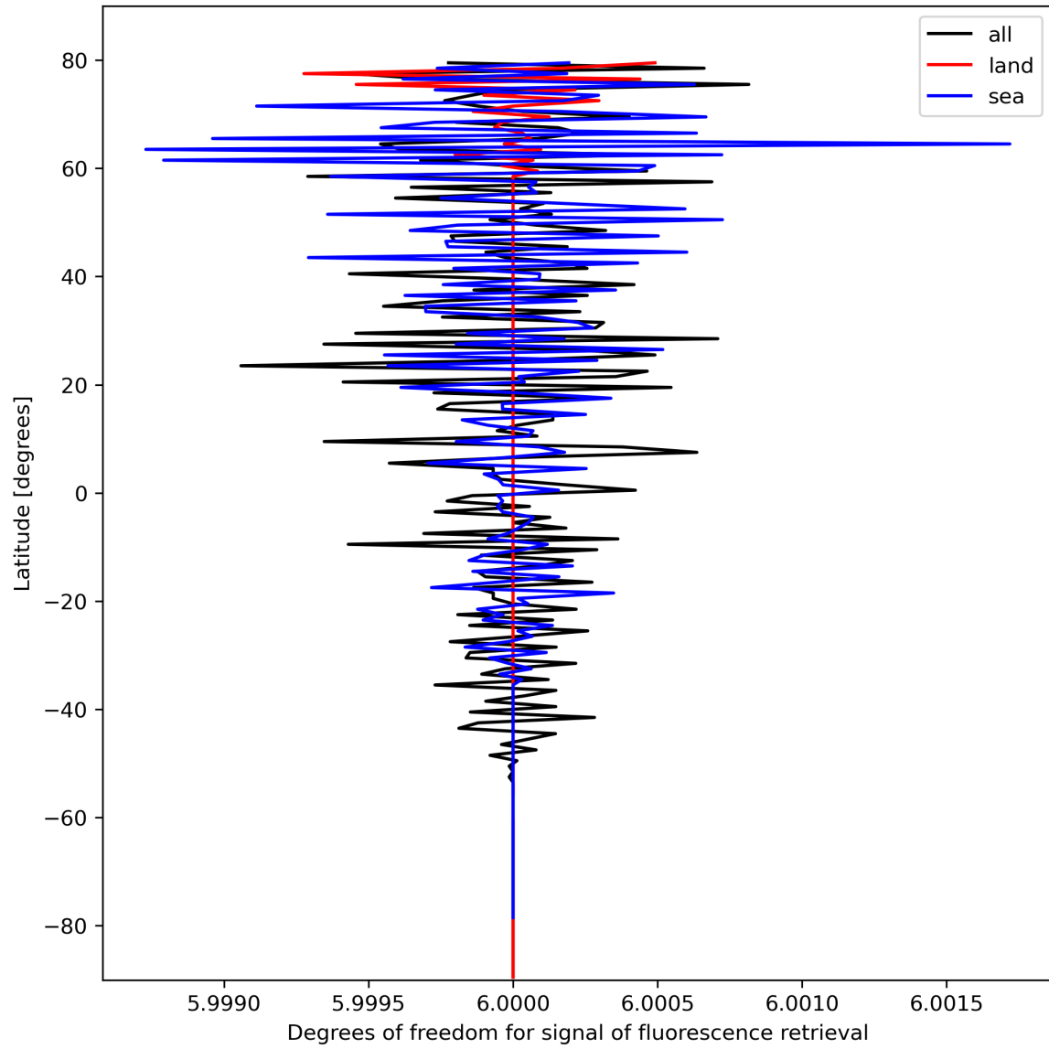
Figure 26: Zonal average of “Degrees of freedom for signal of fluorescence retrieval” for 2023-10-13 to 2023-10-15.
