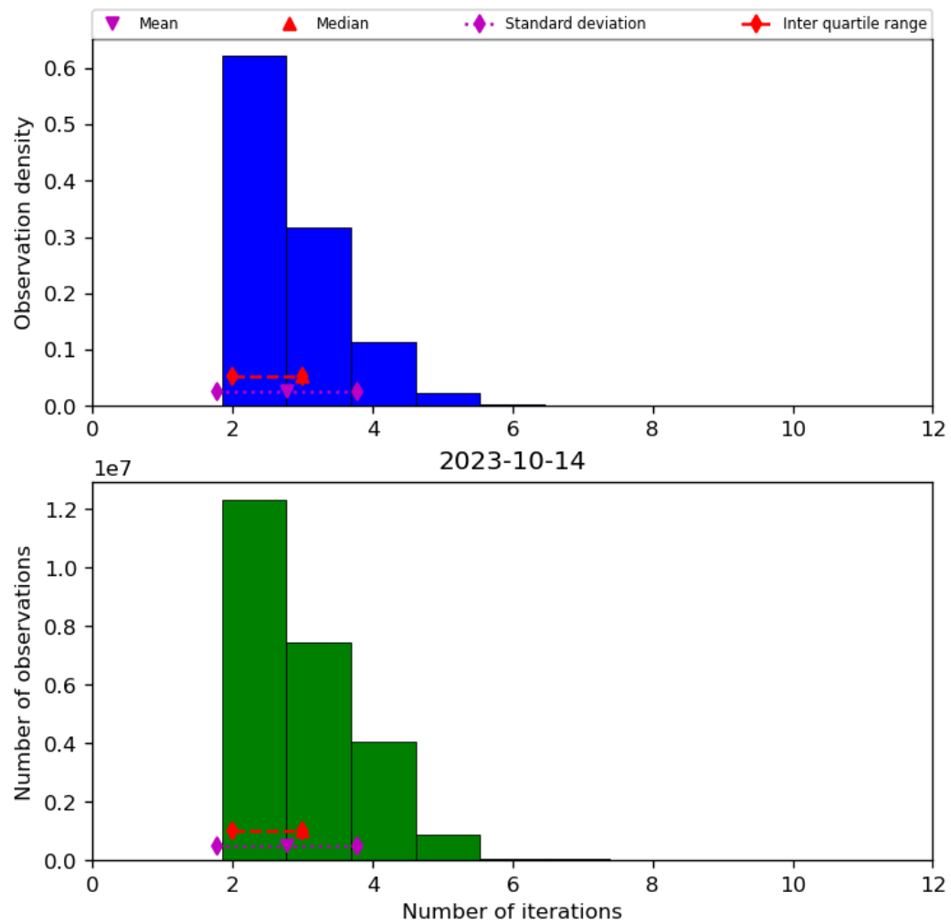
Figure 39: Histogram of “Number of iterations” for 2023-10-13 to 2023-10-15
