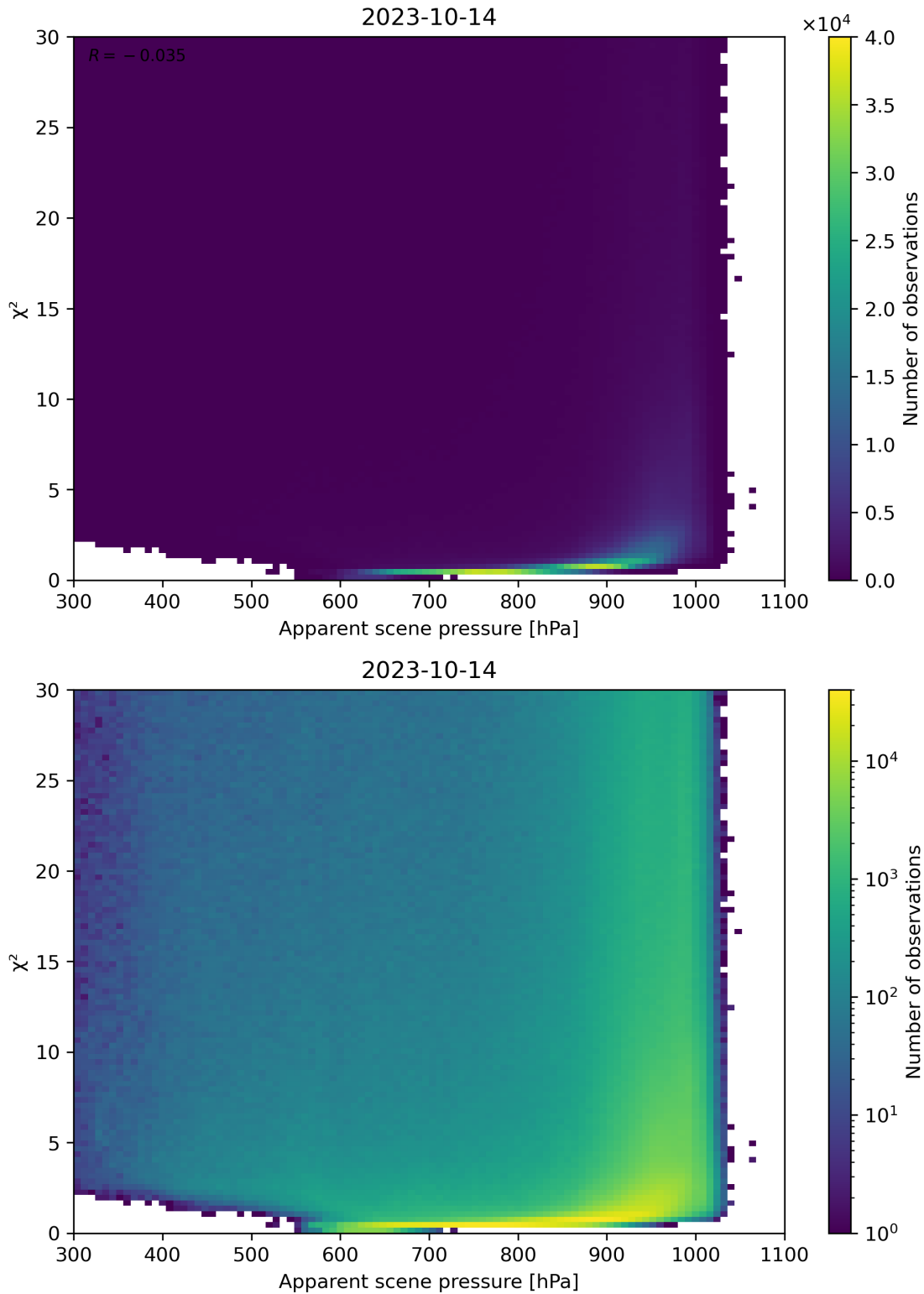
Figure 63: Scatter density plot of “Apparent scene pressure” against “ \chi^2 ” for 2023-10-13 to 2023-10-15.
