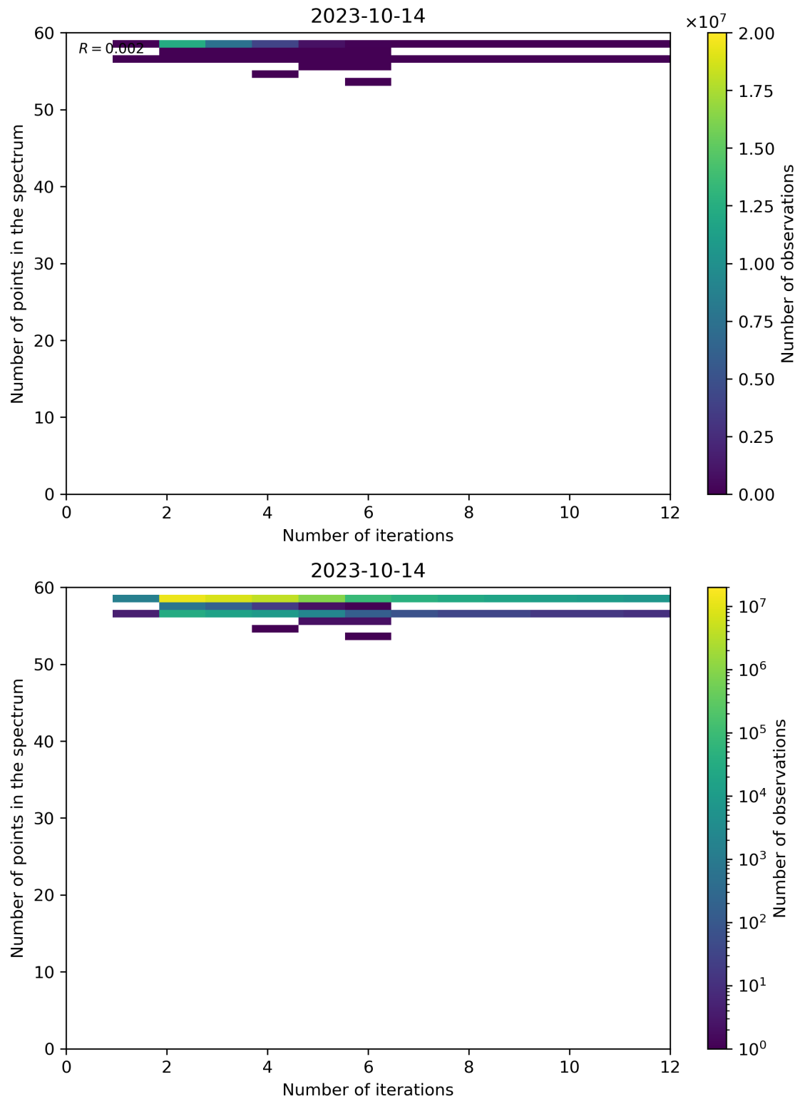
Figure 108: Scatter density plot of “Number of iterations” against “Number of points in the spectrum” for 2023-10-13 to 2023-10-15.
