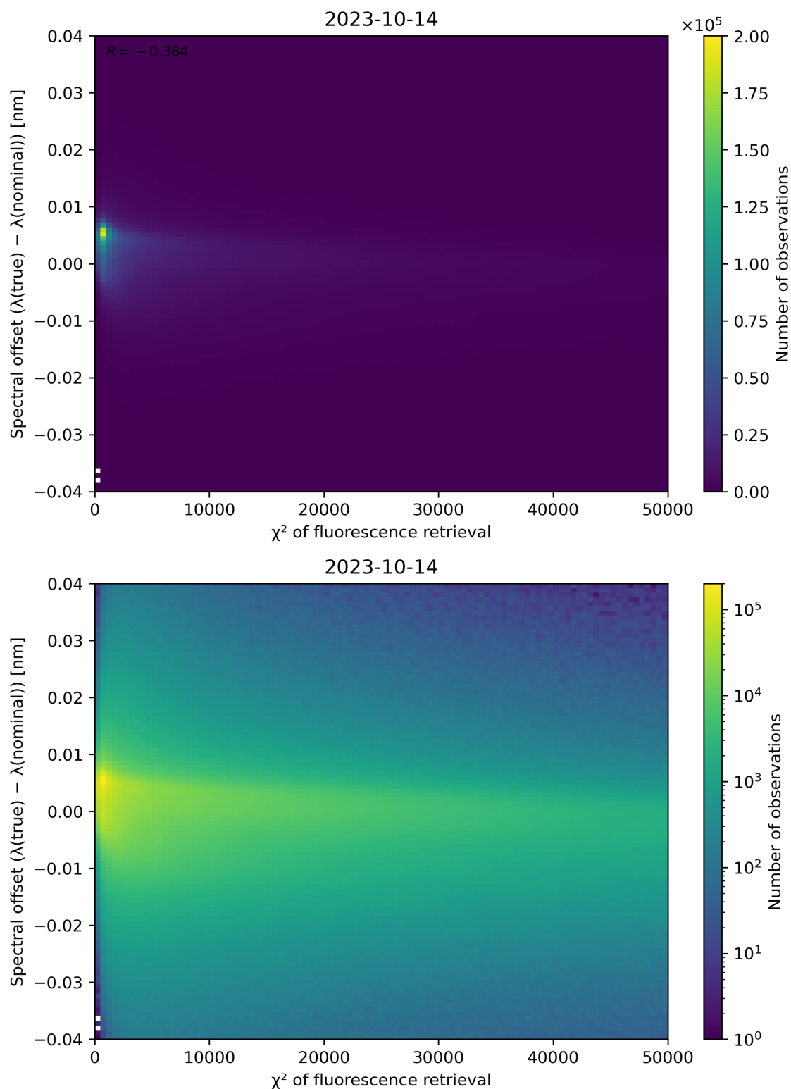
Figure 72: Scatter density plot of " \chi^2 of fluorescence retrieval" against "Spectral offset ( \lambda(\text{true}) - \lambda(\text{nominal})) " for 2023-10-13 to 2023-10-15.
