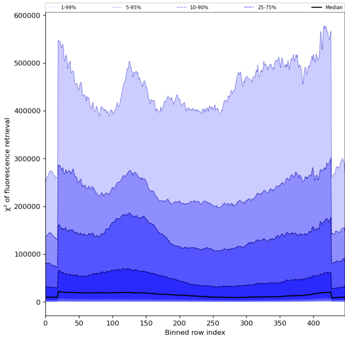
Figure 59: Along track statistics of “ \chi^2 of fluorescence retrieval” for 2023-10-13 to 2023-10-15
