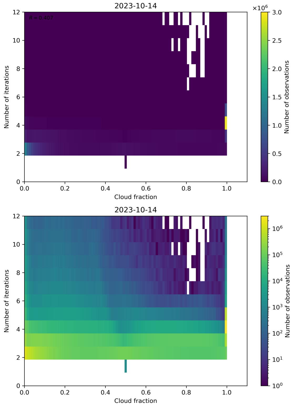
Figure 80: Scatter density plot of “Cloud fraction” against “Number of iterations” for 2023-10-13 to 2023-10-15.
