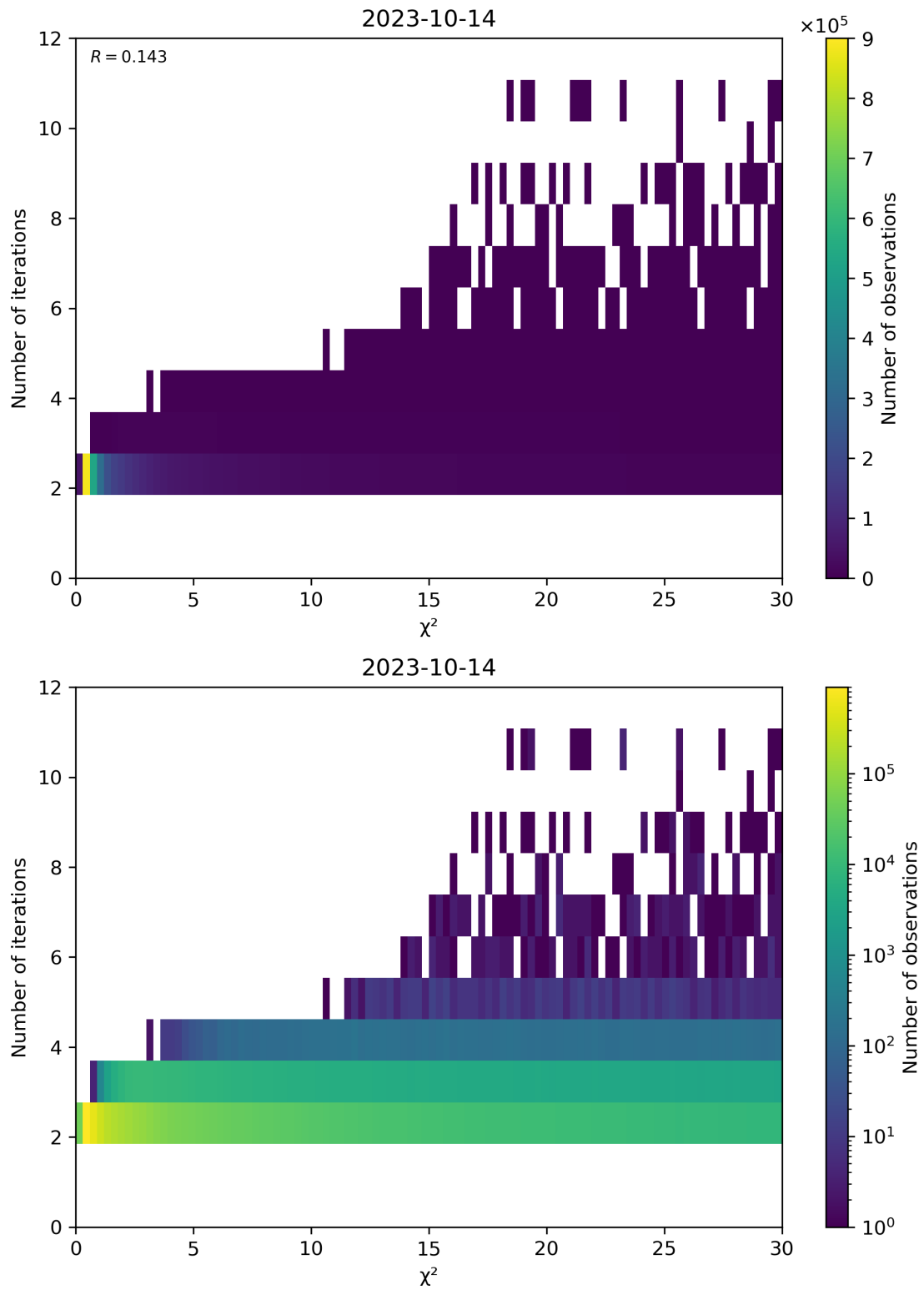
Figure 73: Scatter density plot of “ \chi^2 ” against “Number of iterations” for 2023-10-13 to 2023-10-15.
