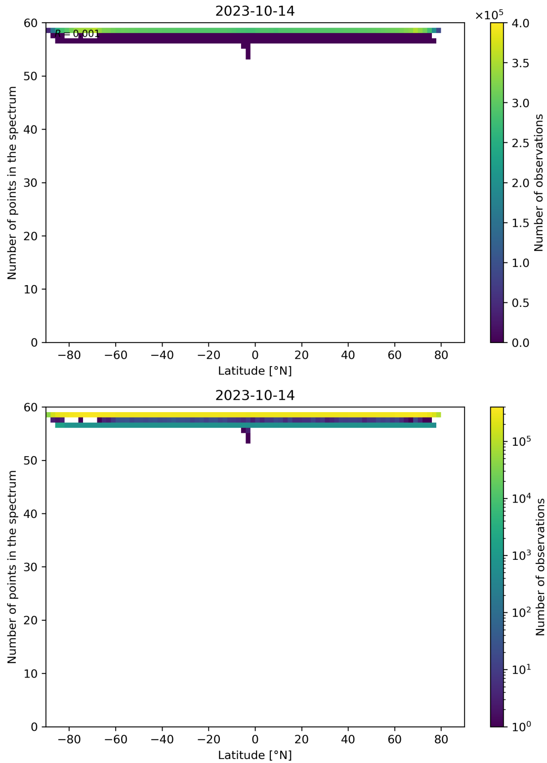
Figure 103: Scatter density plot of “Latitude” against “Number of points in the spectrum” for 2023-10-13 to 2023-10-15.
