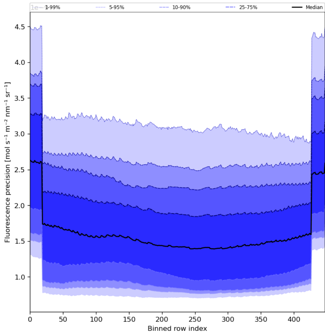
Figure 58: Along track statistics of “Fluorescence precision” for 2023-10-13 to 2023-10-15
