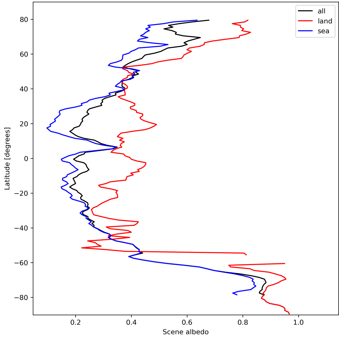
Figure 17: Zonal average of “Scene albedo” for 2023-10-13 to 2023-10-15.
