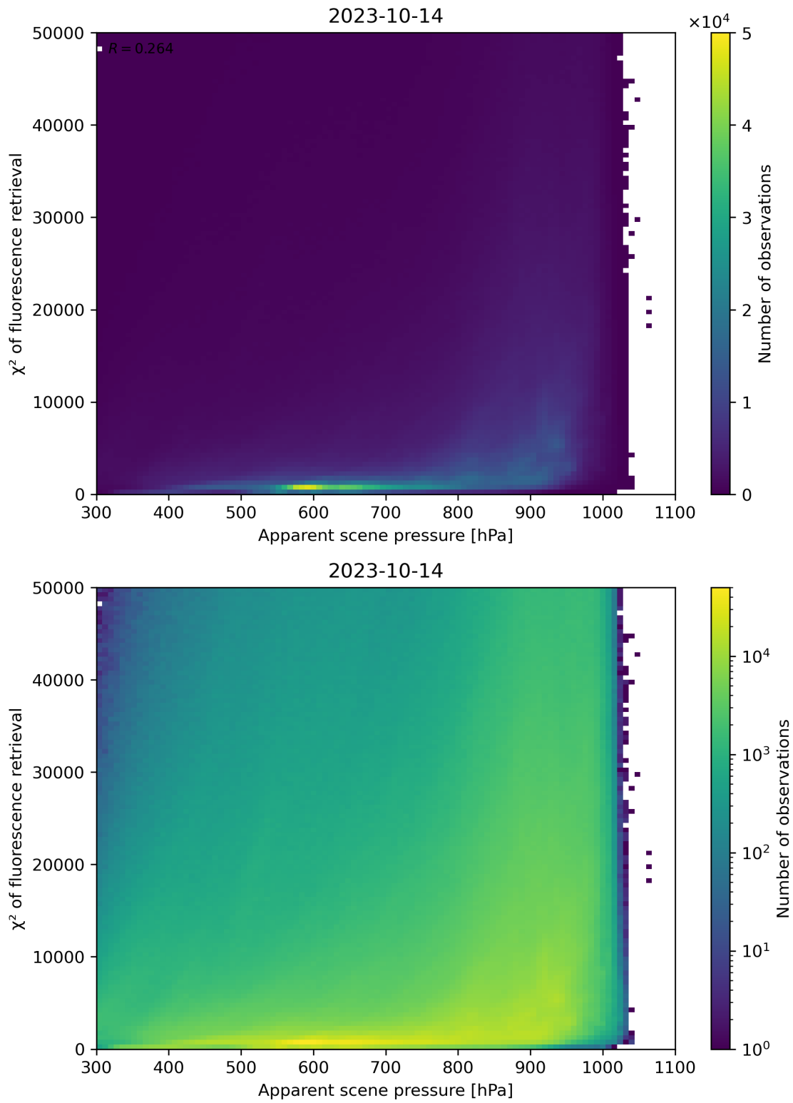
Figure 64: Scatter density plot of “Apparent scene pressure” against “ \chi^2 of fluorescence retrieval” for 2023-10-13 to 2023-10-15.
