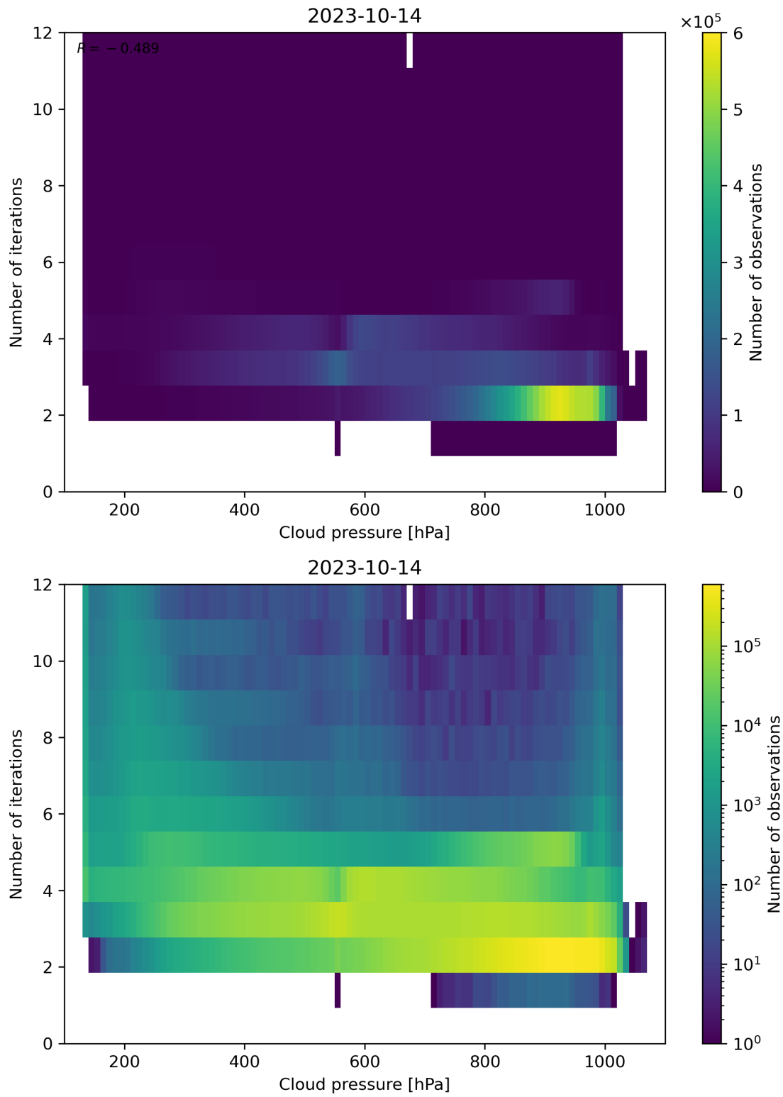
Figure 89: Scatter density plot of “Cloud pressure” against “Number of iterations” for 2023-10-13 to 2023-10-15.
