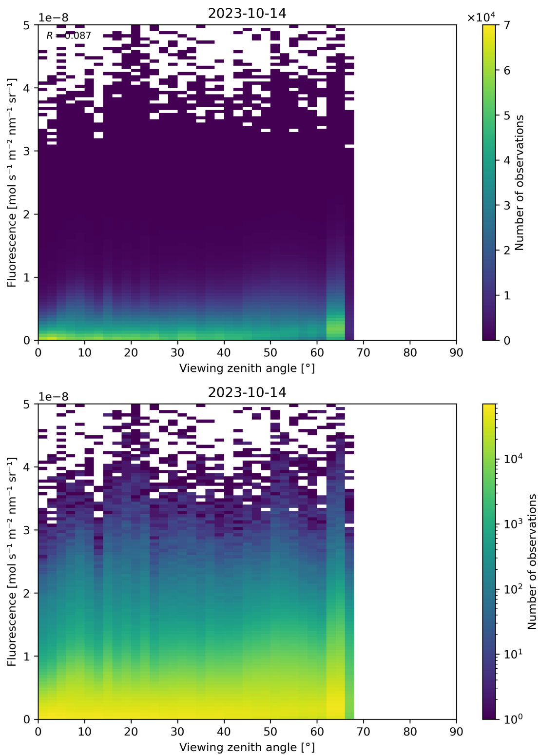
Figure 134: Scatter density plot of “Viewing zenith angle” against “Fluorescence” for 2023-10-13 to 2023-10-15.
