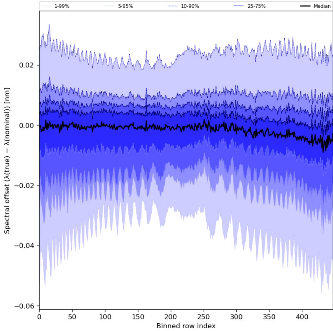
Figure 62: Along track statistics of “Spectral offset ( \lambda(\text{true}) - \lambda(\text{nominal}) )” for 2023-10-13 to 2023-10-15
