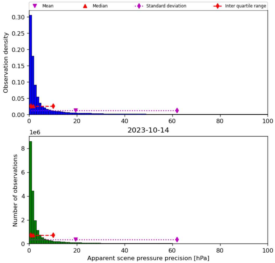
Figure 37: Histogram of “Apparent scene pressure precision” for 2023-10-13 to 2023-10-15
