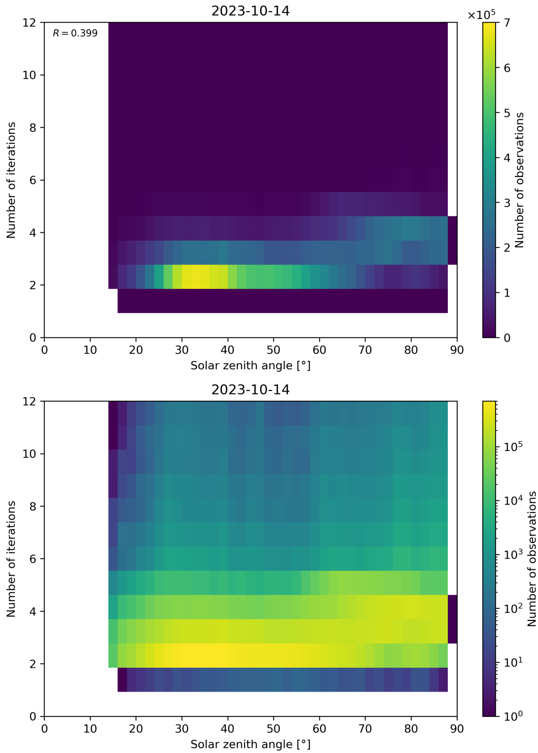
Figure 125: Scatter density plot of “Solar zenith angle” against “Number of iterations” for 2023-10-13 to 2023-10-15.
