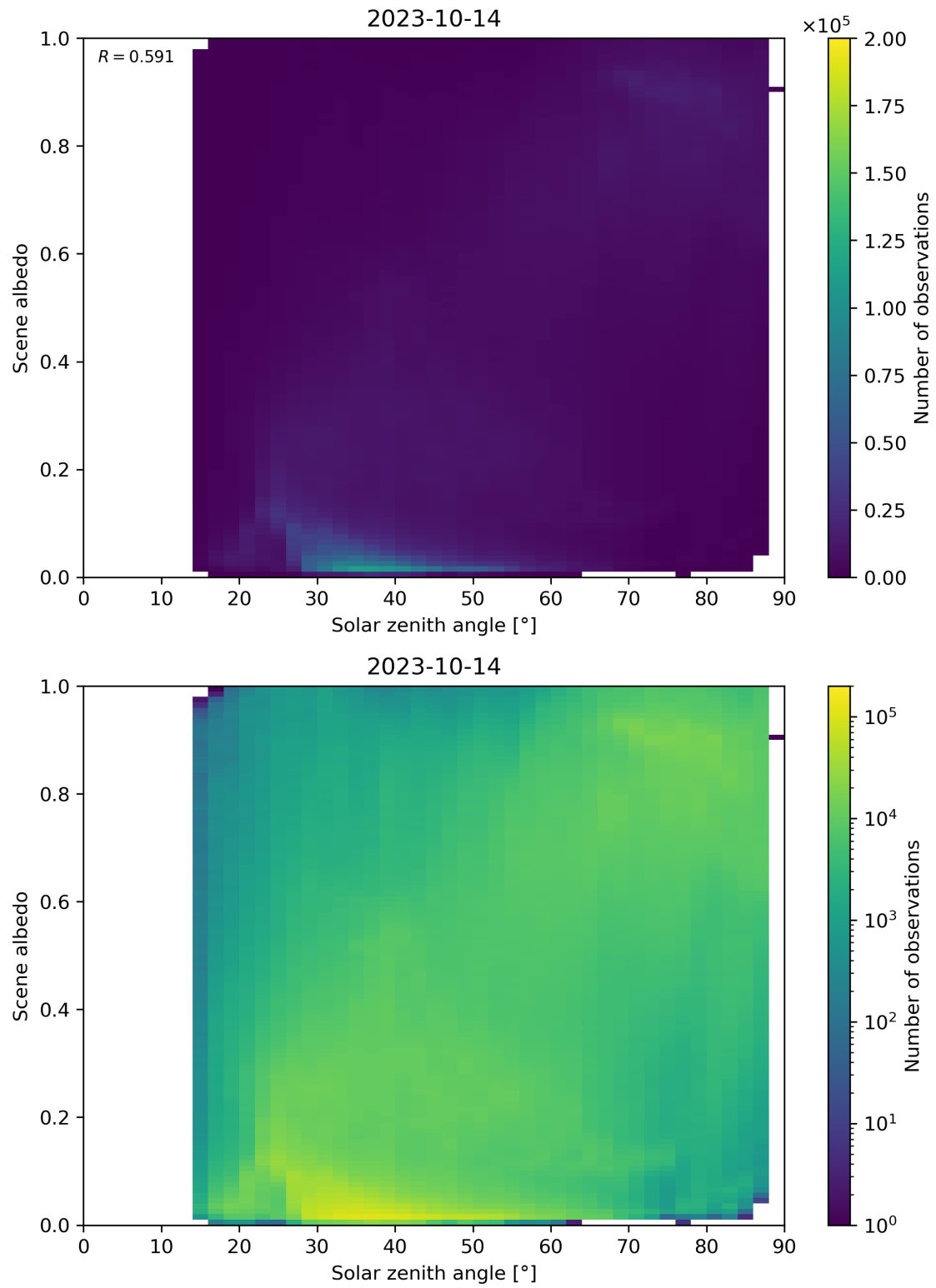
Figure 127: Scatter density plot of “Solar zenith angle” against “Scene albedo” for 2023-10-13 to 2023-10-15.
