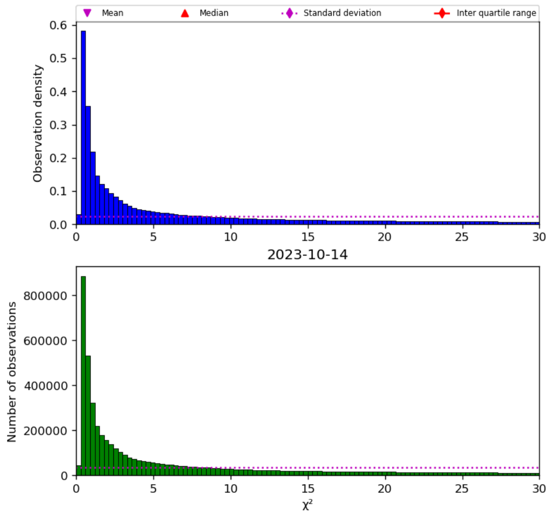
Figure 38: Histogram of “ \chi^2 ” for 2023-10-13 to 2023-10-15
