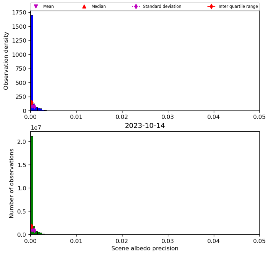
Figure 35: Histogram of “Scene albedo precision” for 2023-10-13 to 2023-10-15
