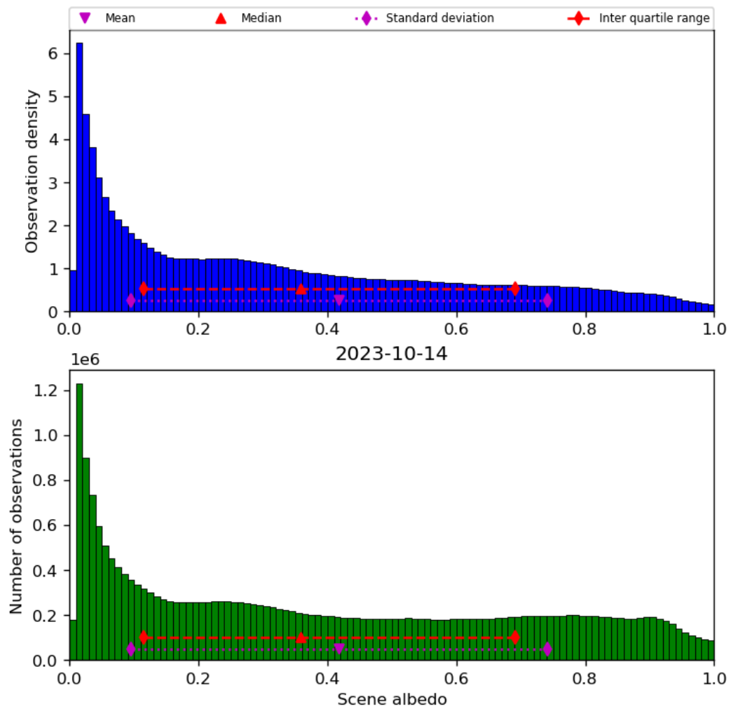
Figure 34: Histogram of “Scene albedo” for 2023-10-13 to 2023-10-15
