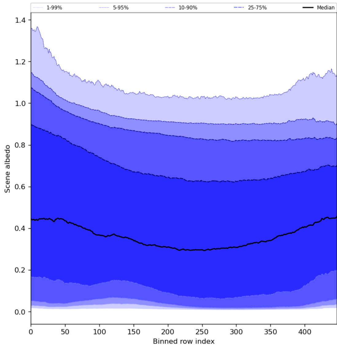
Figure 51: Along track statistics of “Scene albedo” for 2023-10-13 to 2023-10-15
