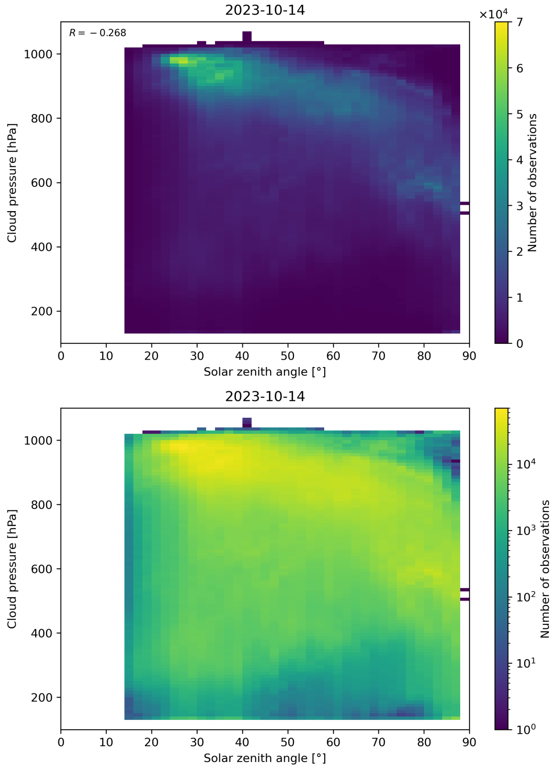
Figure 122: Scatter density plot of “Solar zenith angle” against “Cloud pressure” for 2023-10-13 to 2023-10-15.
