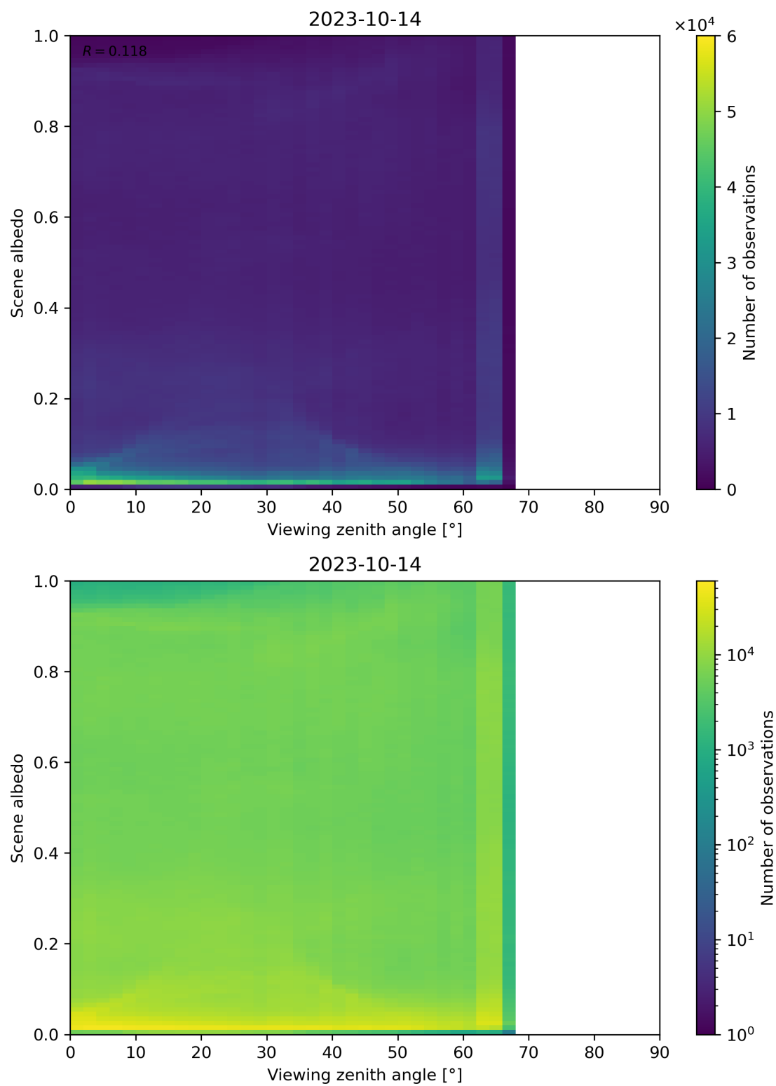
Figure 138: Scatter density plot of “Viewing zenith angle” against “Scene albedo” for 2023-10-13 to 2023-10-15.
