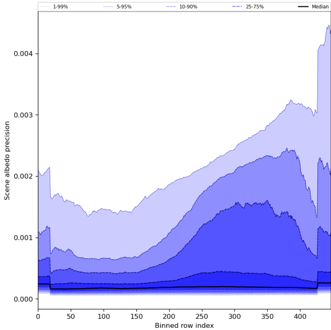
Figure 52: Along track statistics of “Scene albedo precision” for 2023-10-13 to 2023-10-15
