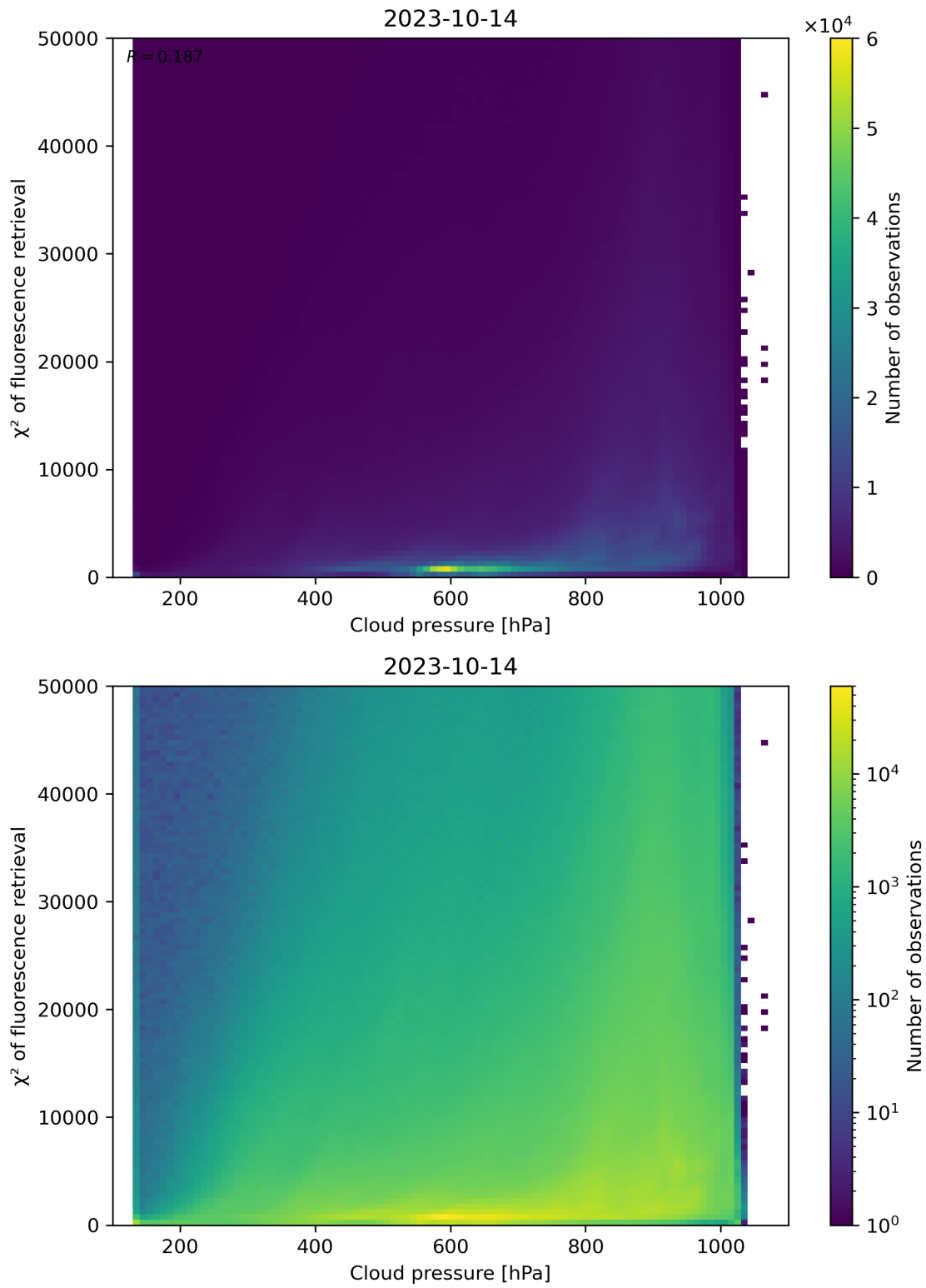
Figure 86: Scatter density plot of “Cloud pressure” against “ \chi^2 of fluorescence retrieval” for 2023-10-13 to 2023-10-15.
