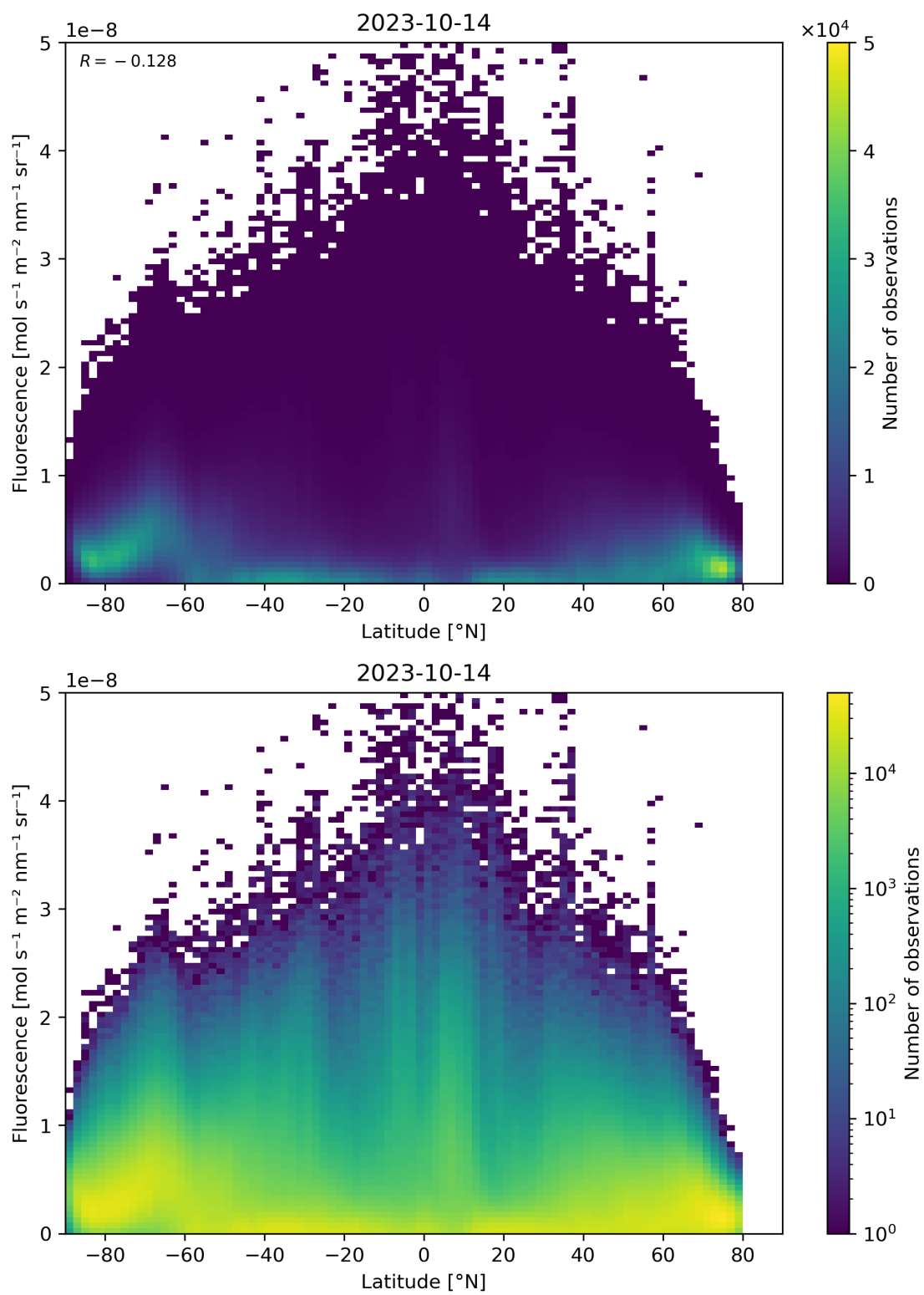
Figure 101: Scatter density plot of “Latitude” against “Fluorescence” for 2023-10-13 to 2023-10-15.
