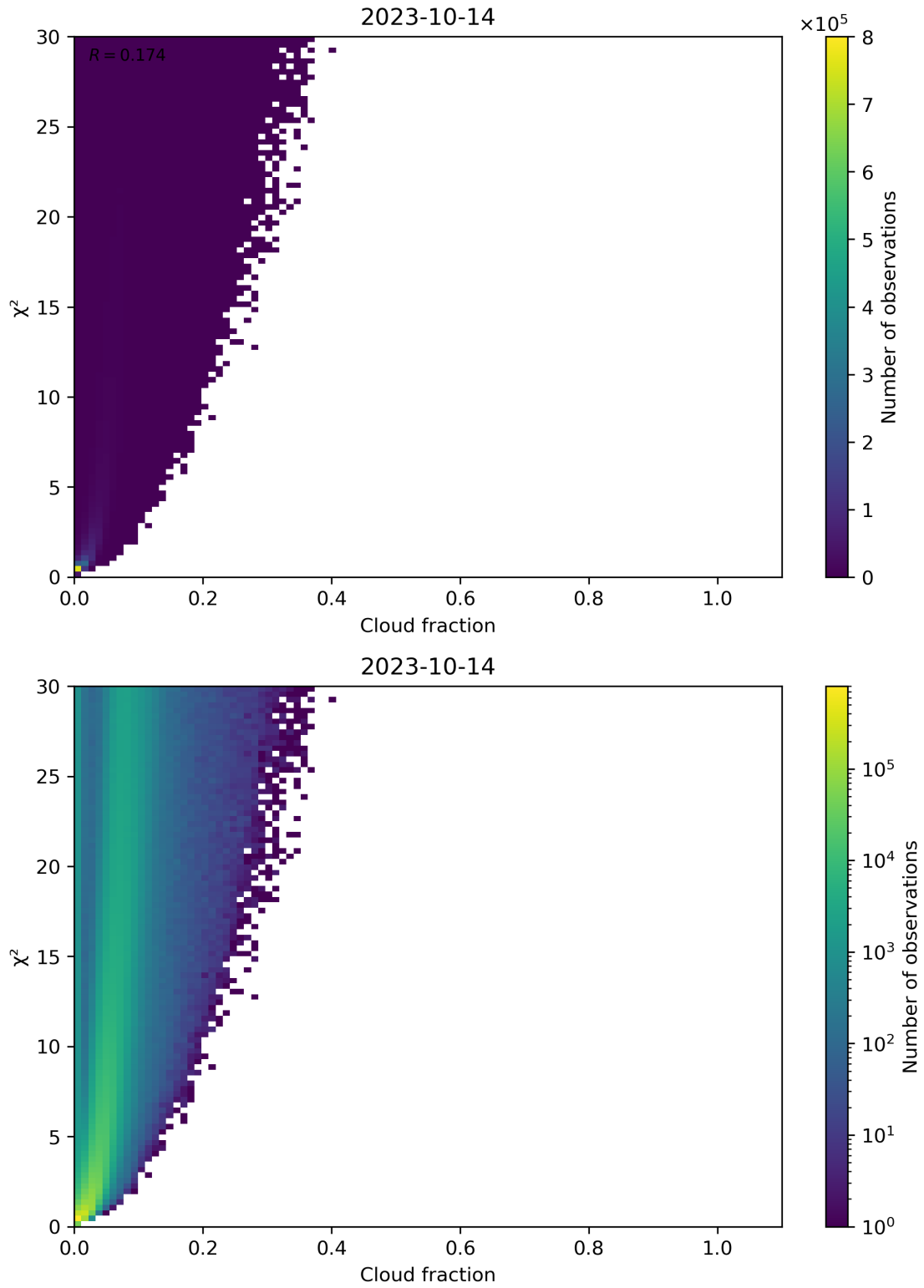
Figure 77: Scatter density plot of “Cloud fraction” against “ \chi^2 ” for 2023-10-13 to 2023-10-15.
