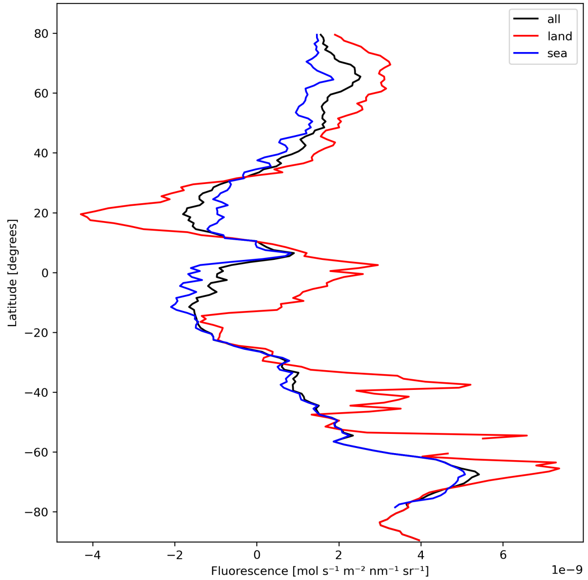
Figure 23: Zonal average of “Fluorescence” for 2023-10-13 to 2023-10-15.
