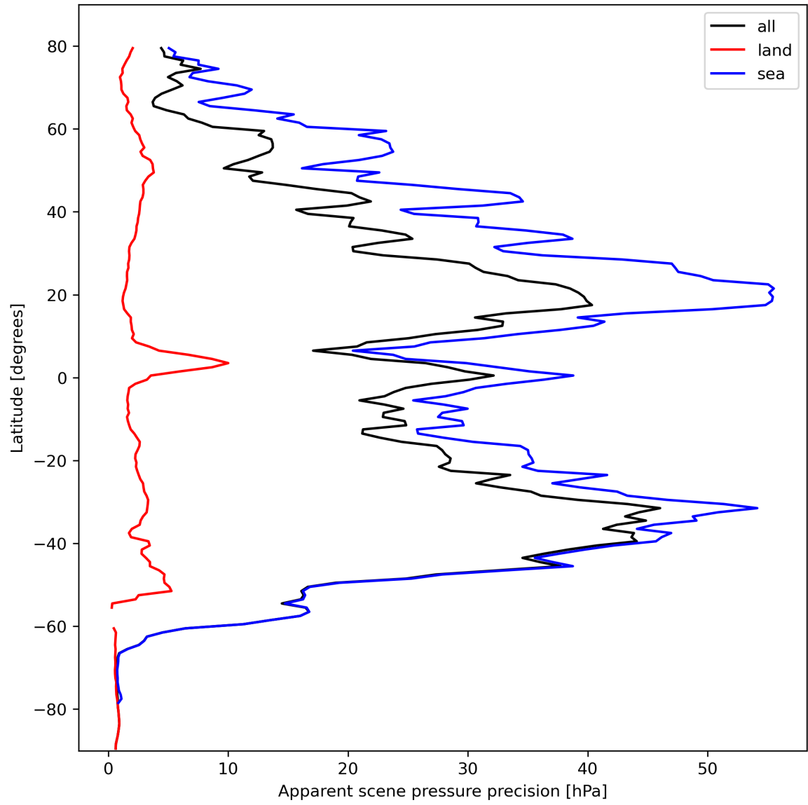
Figure 20: Zonal average of “Apparent scene pressure precision” for 2023-10-13 to 2023-10-15.
