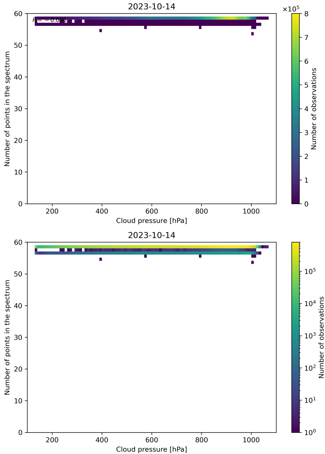
Figure 90: Scatter density plot of “Cloud pressure” against “Number of points in the spectrum” for 2023-10-13 to 2023-10-15.
