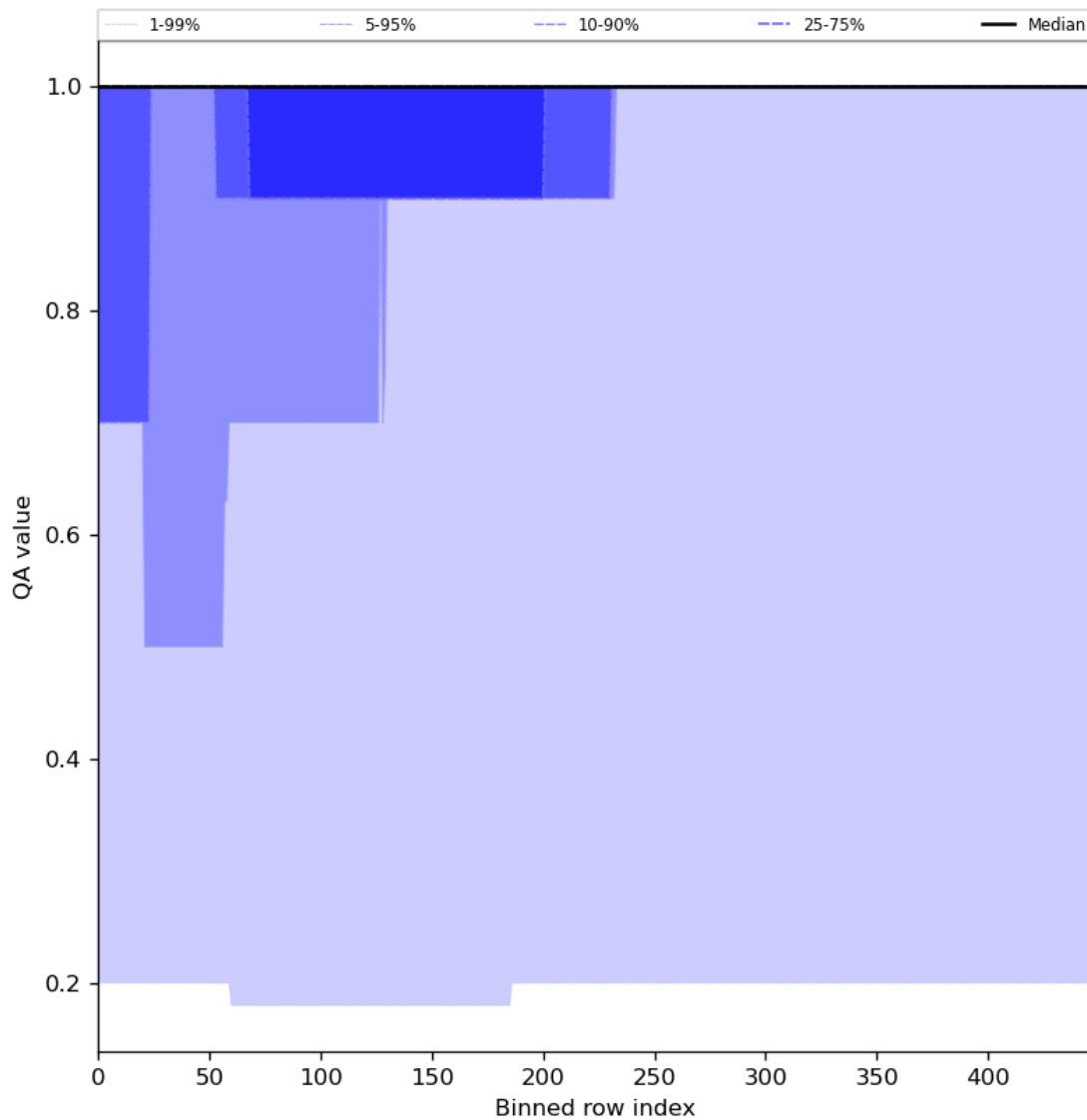
Figure 46: Along track statistics of “QA value” for 2023-10-13 to 2023-10-15
