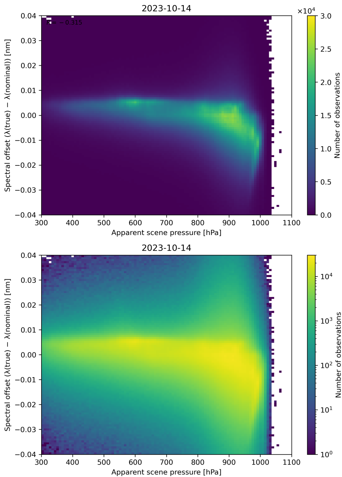
Figure 68: Scatter density plot of “Apparent scene pressure” against “Spectral offset ( \lambda(\text{true}) - \lambda(\text{nominal}) )” for 2023-10-13 to 2023-10-15.
