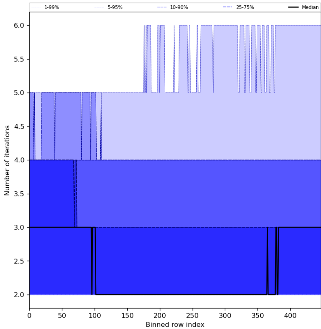
Figure 56: Along track statistics of “Number of iterations” for 2023-10-13 to 2023-10-15
