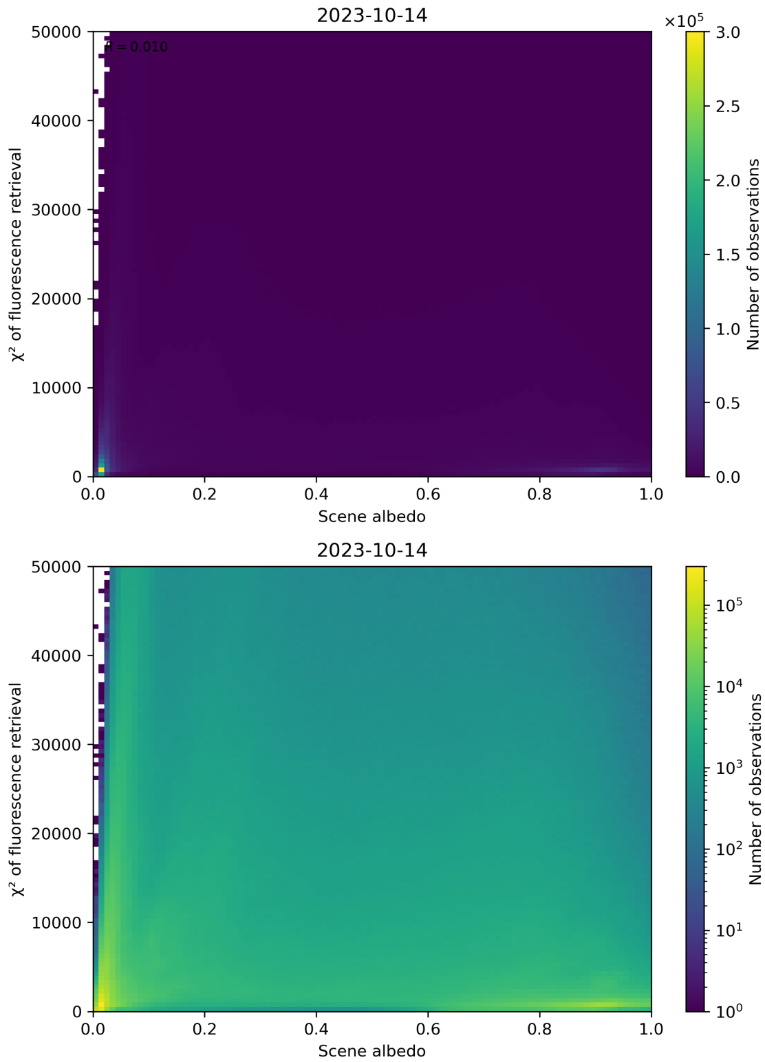
Figure 113: Scatter density plot of “Scene albedo” against “ \chi^2 of fluorescence retrieval” for 2023-10-13 to 2023-10-15.
