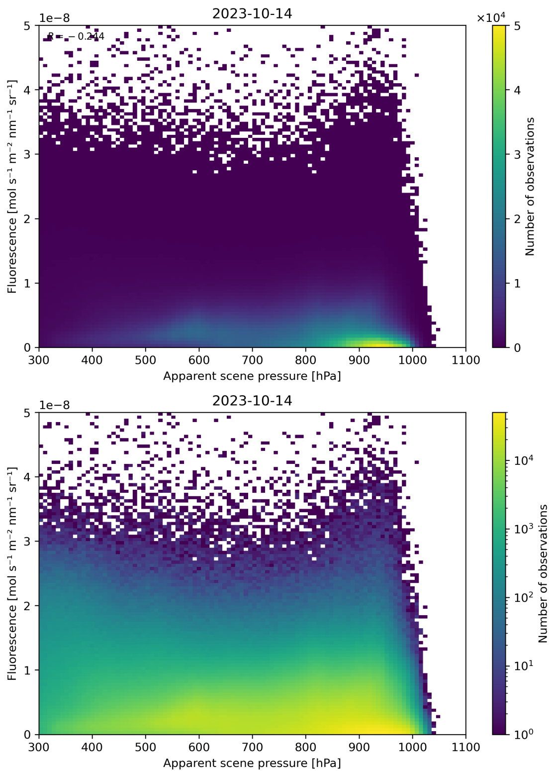
Figure 65: Scatter density plot of “Apparent scene pressure” against “Fluorescence” for 2023-10-13 to 2023-10-15.
