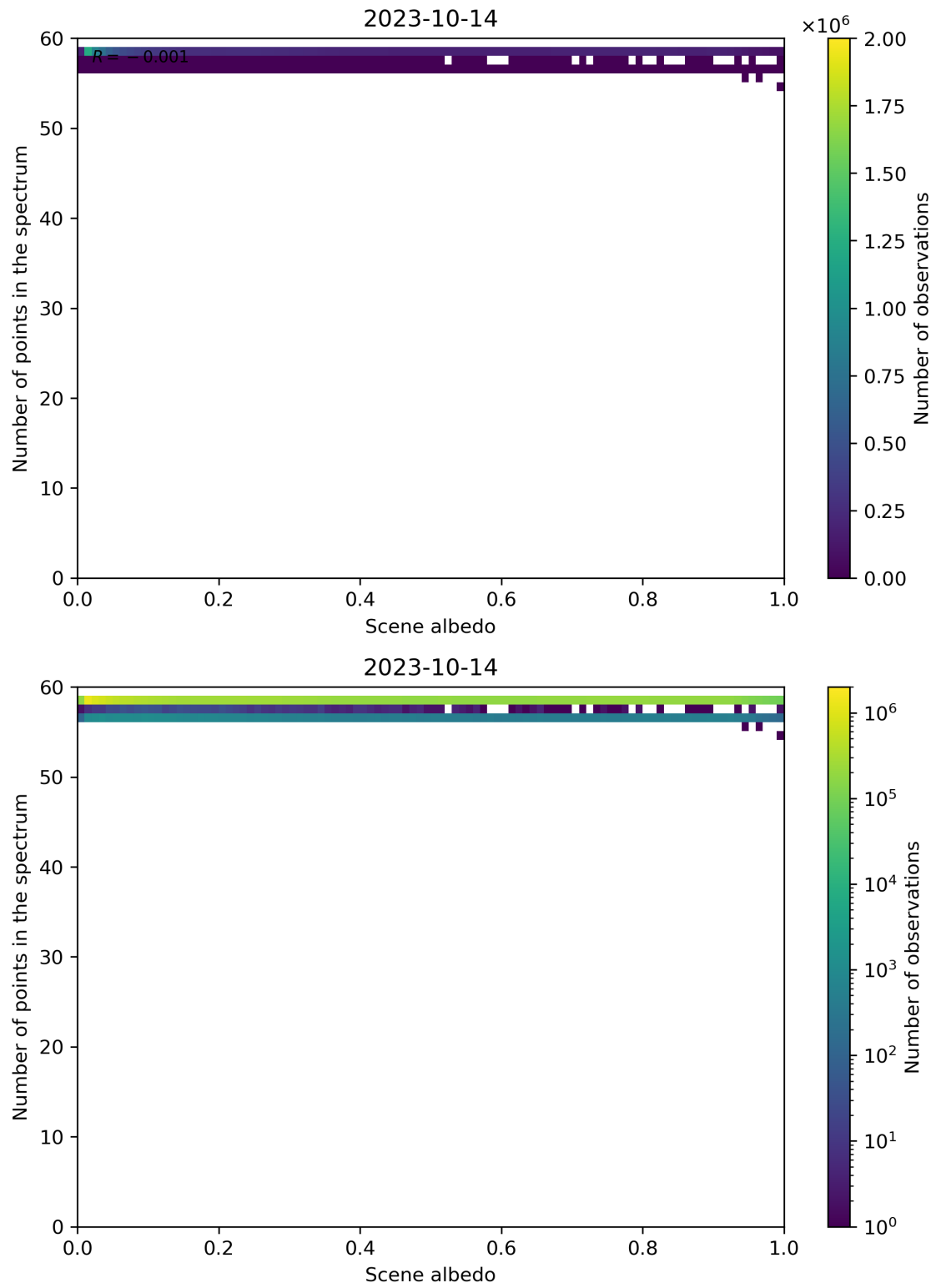
Figure 116: Scatter density plot of “Scene albedo” against “Number of points in the spectrum” for 2023-10-13 to 2023-10-15.
