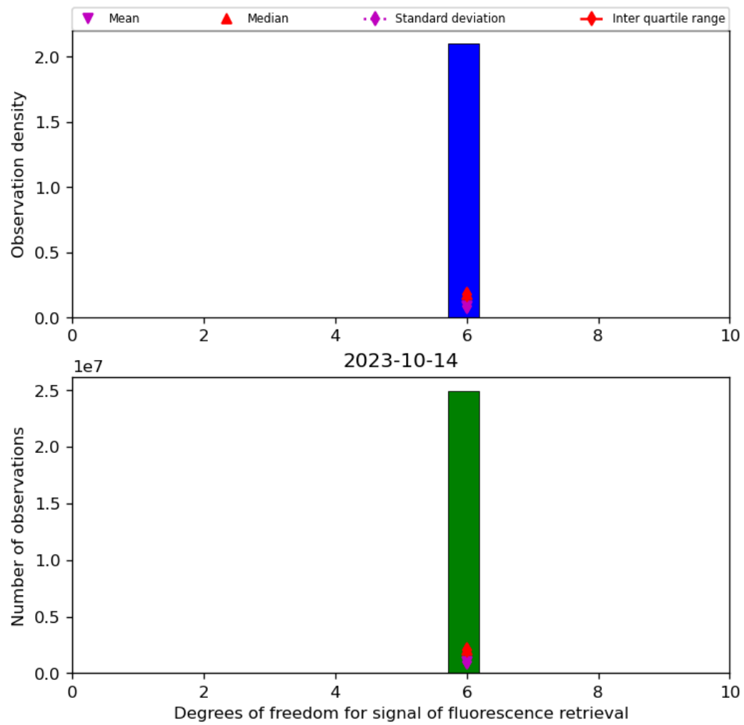
Figure 43: Histogram of “Degrees of freedom for signal of fluorescence retrieval” for 2023-10-13 to 2023-10-15
