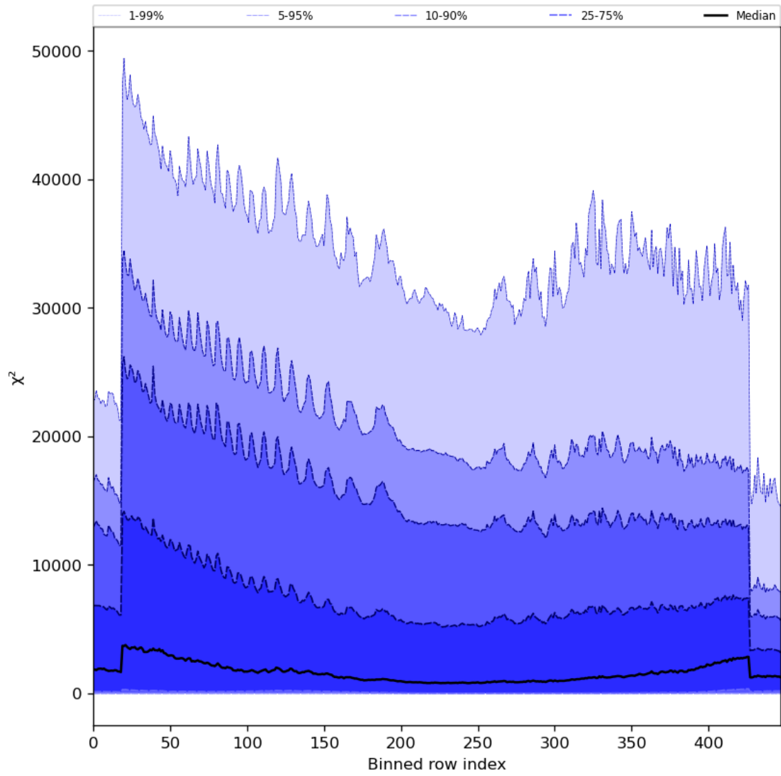
Figure 55: Along track statistics of “ \chi^2 ” for 2023-10-13 to 2023-10-15
