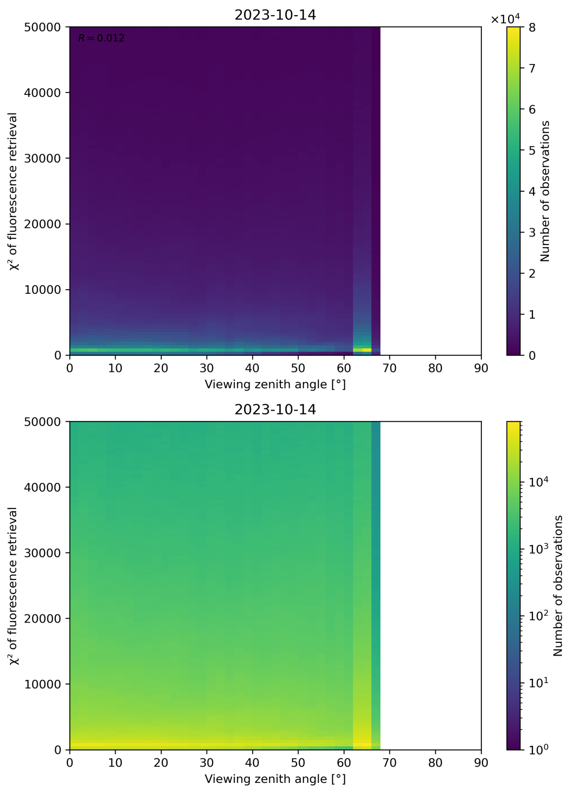
Figure 131: Scatter density plot of “Viewing zenith angle” against “ \chi^2 of fluorescence retrieval” for 2023-10-13 to 2023-10-15.
