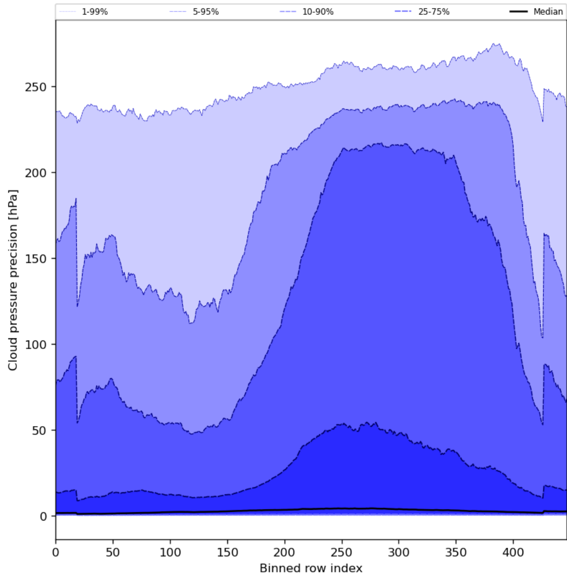
Figure 48: Along track statistics of “Cloud pressure precision” for 2023-10-13 to 2023-10-15
