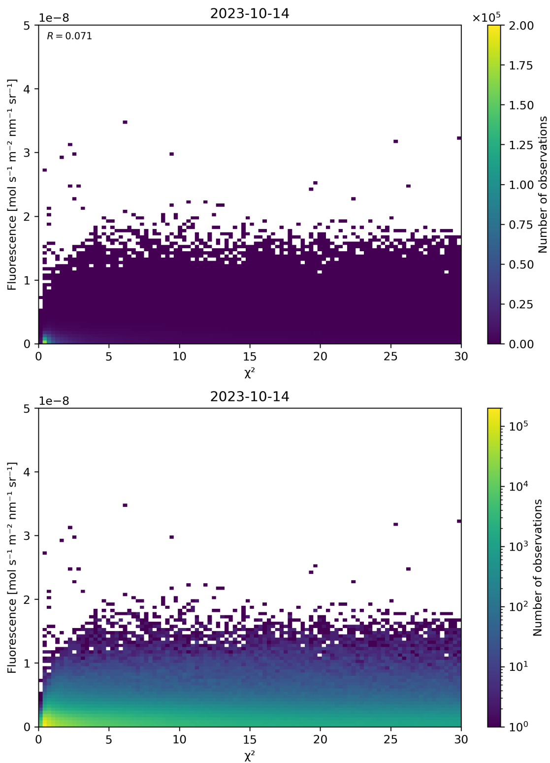
Figure 70: Scatter density plot of “ \chi^2 ” against “Fluorescence” for 2023-10-13 to 2023-10-15.
