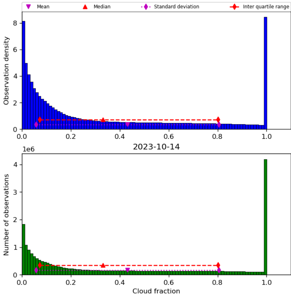
Figure 32: Histogram of “Cloud fraction” for 2023-10-13 to 2023-10-15
