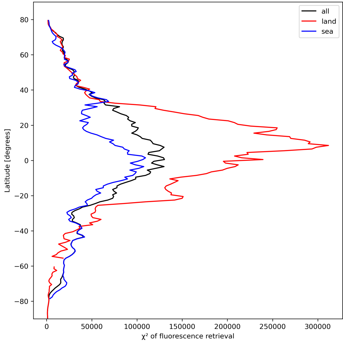
Figure 25: Zonal average of “ \chi^2 of fluorescence retrieval” for 2023-10-13 to 2023-10-15.
