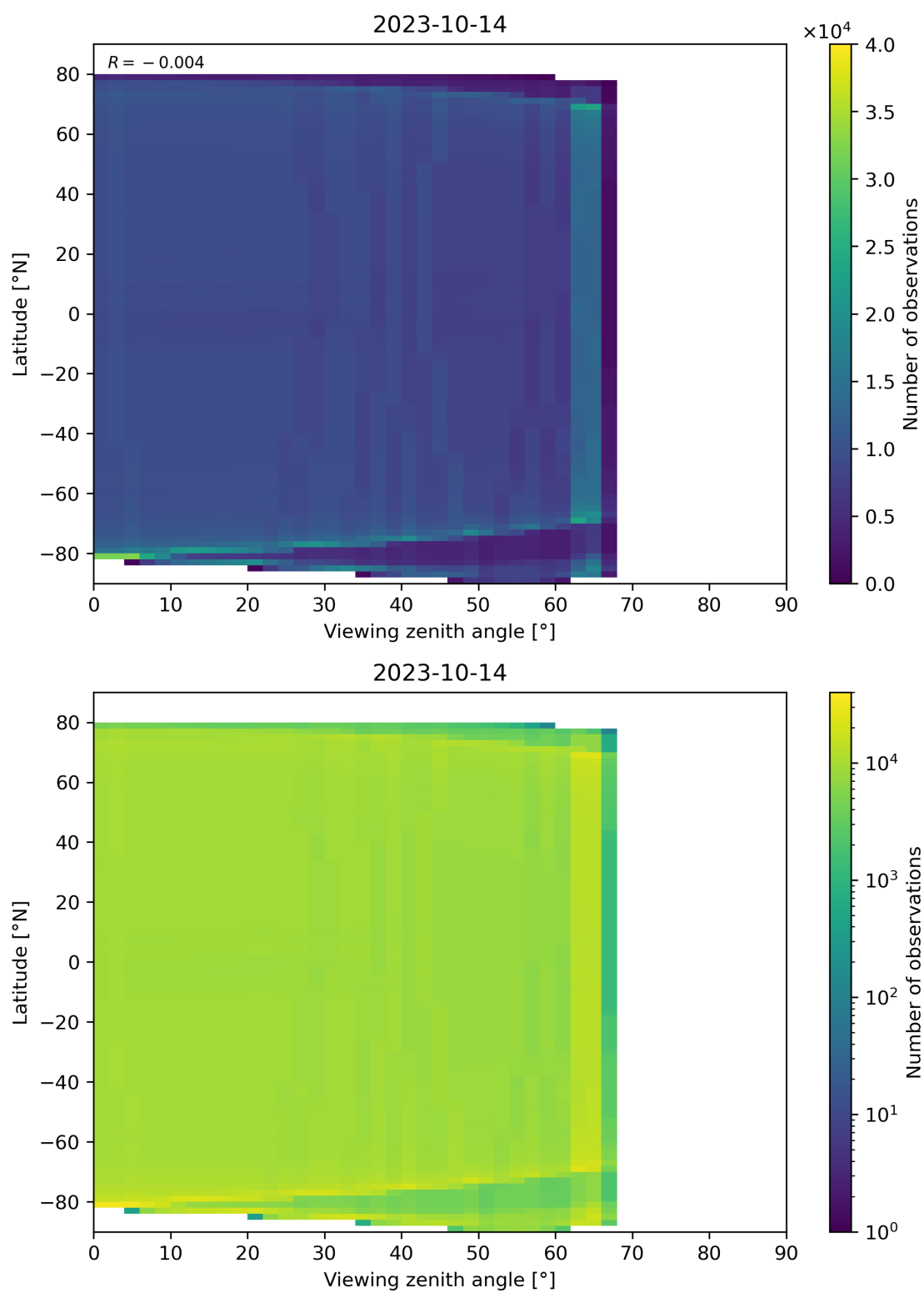
Figure 135: Scatter density plot of “Viewing zenith angle” against “Latitude” for 2023-10-13 to 2023-10-15.
