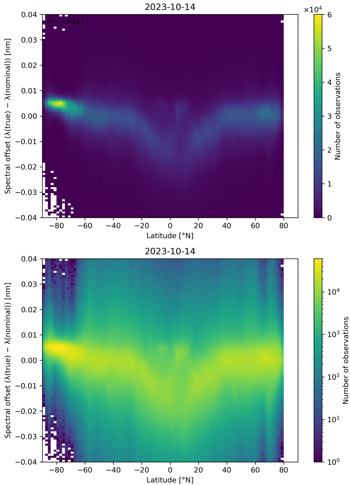
Figure 105: Scatter density plot of “Latitude” against “Spectral offset ( \lambda(\text{true}) - \lambda(\text{nominal}) )” for 2023-10-13 to 2023-10-15.
