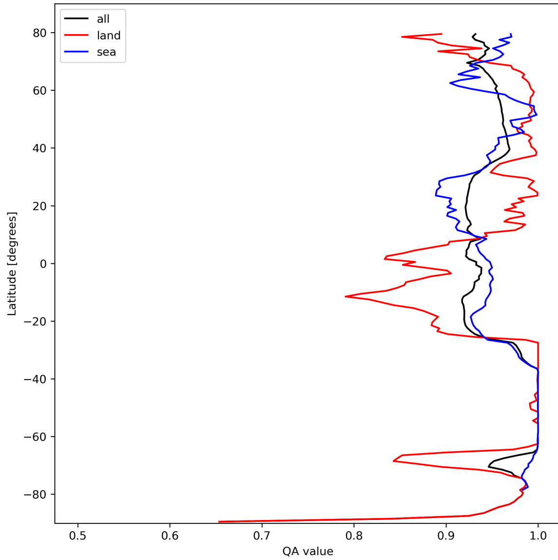
Figure 12: Zonal average of “QA value” for 2023-10-13 to 2023-10-15.
