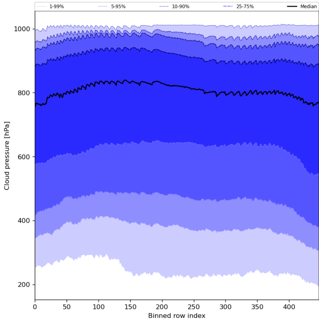
Figure 47: Along track statistics of “Cloud pressure” for 2023-10-13 to 2023-10-15
