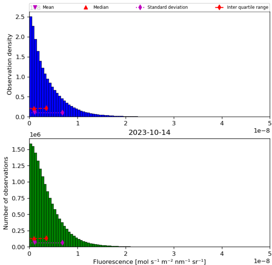
Figure 40: Histogram of “Fluorescence” for 2023-10-13 to 2023-10-15
