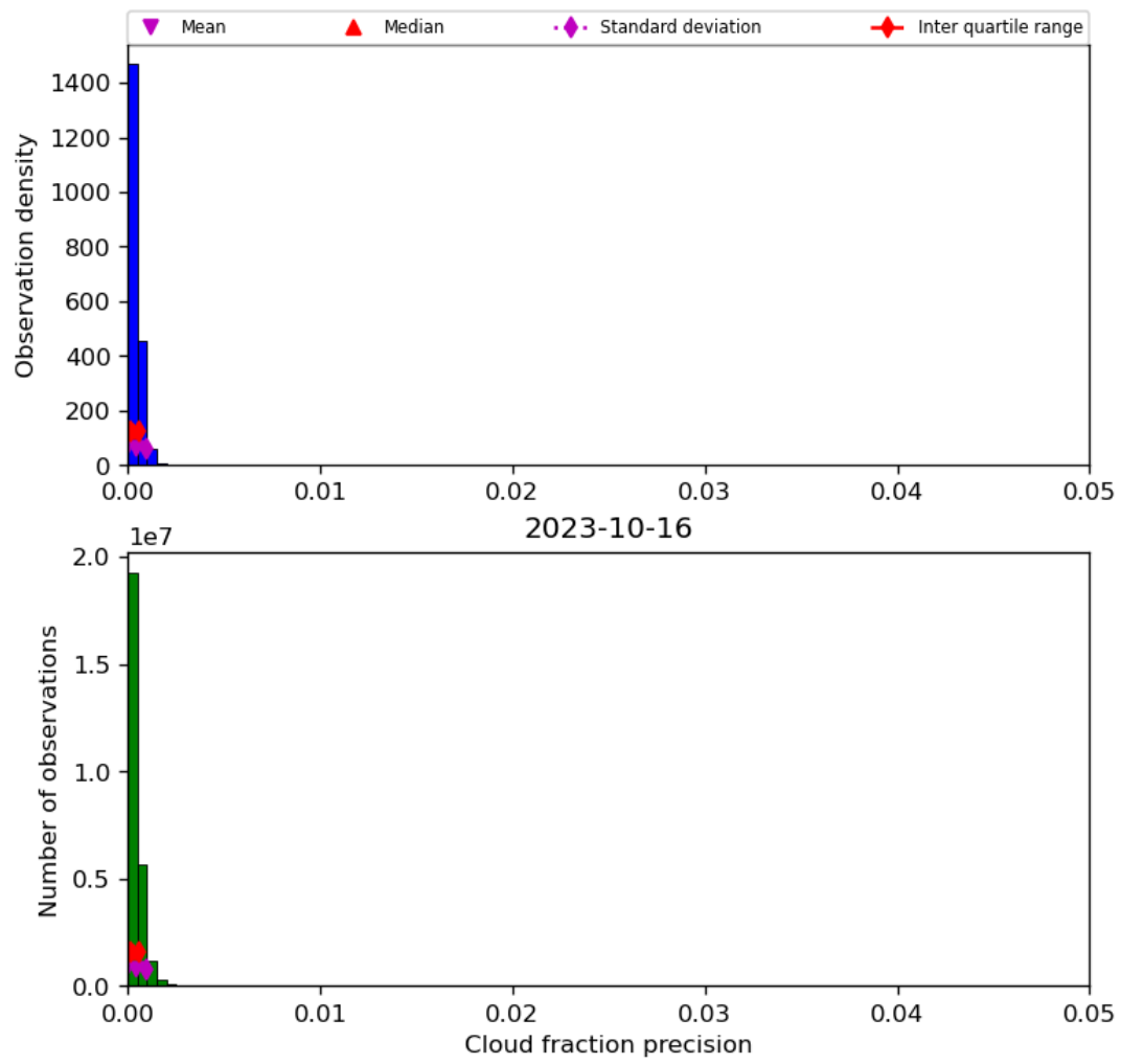
Figure 33: Histogram of “Cloud fraction precision” for 2023-10-15 to 2023-10-17
