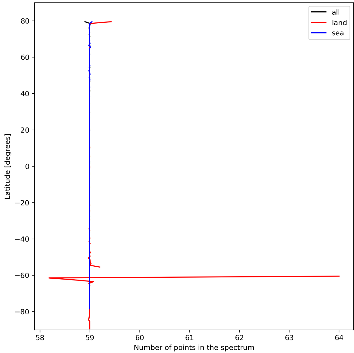
Figure 27: Zonal average of “Number of points in the spectrum” for 2023-10-15 to 2023-10-17.
