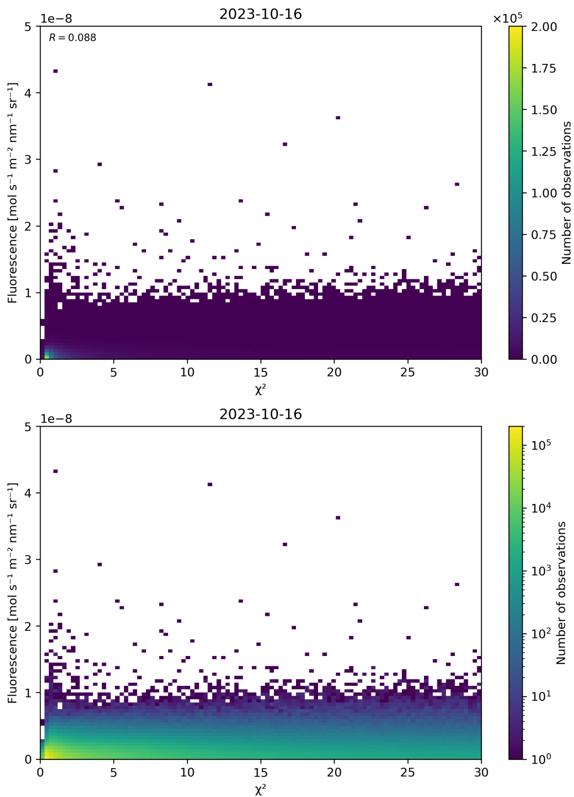
Figure 70: Scatter density plot of “ \chi^2 ” against “Fluorescence” for 2023-10-15 to 2023-10-17.
