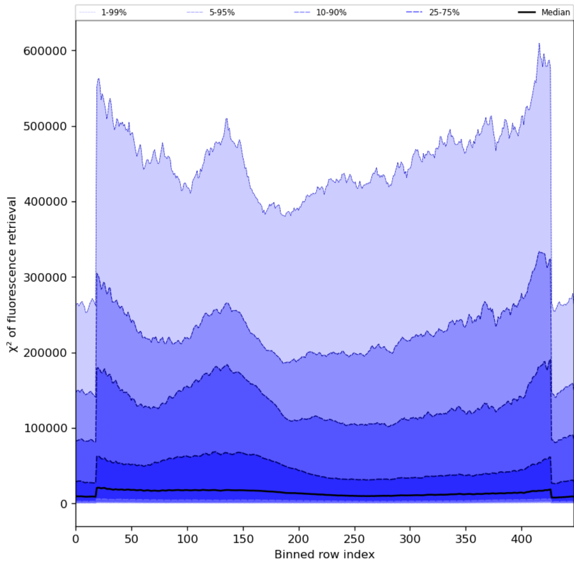
Figure 59: Along track statistics of “ \chi^2 of fluorescence retrieval” for 2023-10-15 to 2023-10-17
