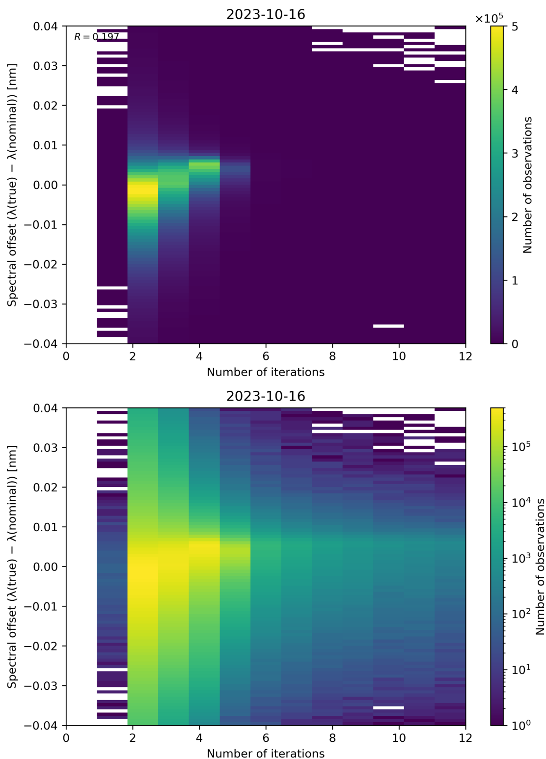
Figure 109: Scatter density plot of “Number of iterations” against “Spectral offset ( \lambda(\text{true}) - \lambda(\text{nominal}) )” for 2023-10-15 to 2023-10-17.
