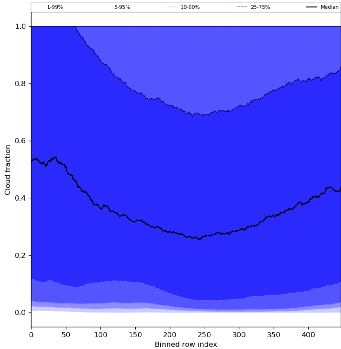
Figure 49: Along track statistics of “Cloud fraction” for 2023-10-15 to 2023-10-17
