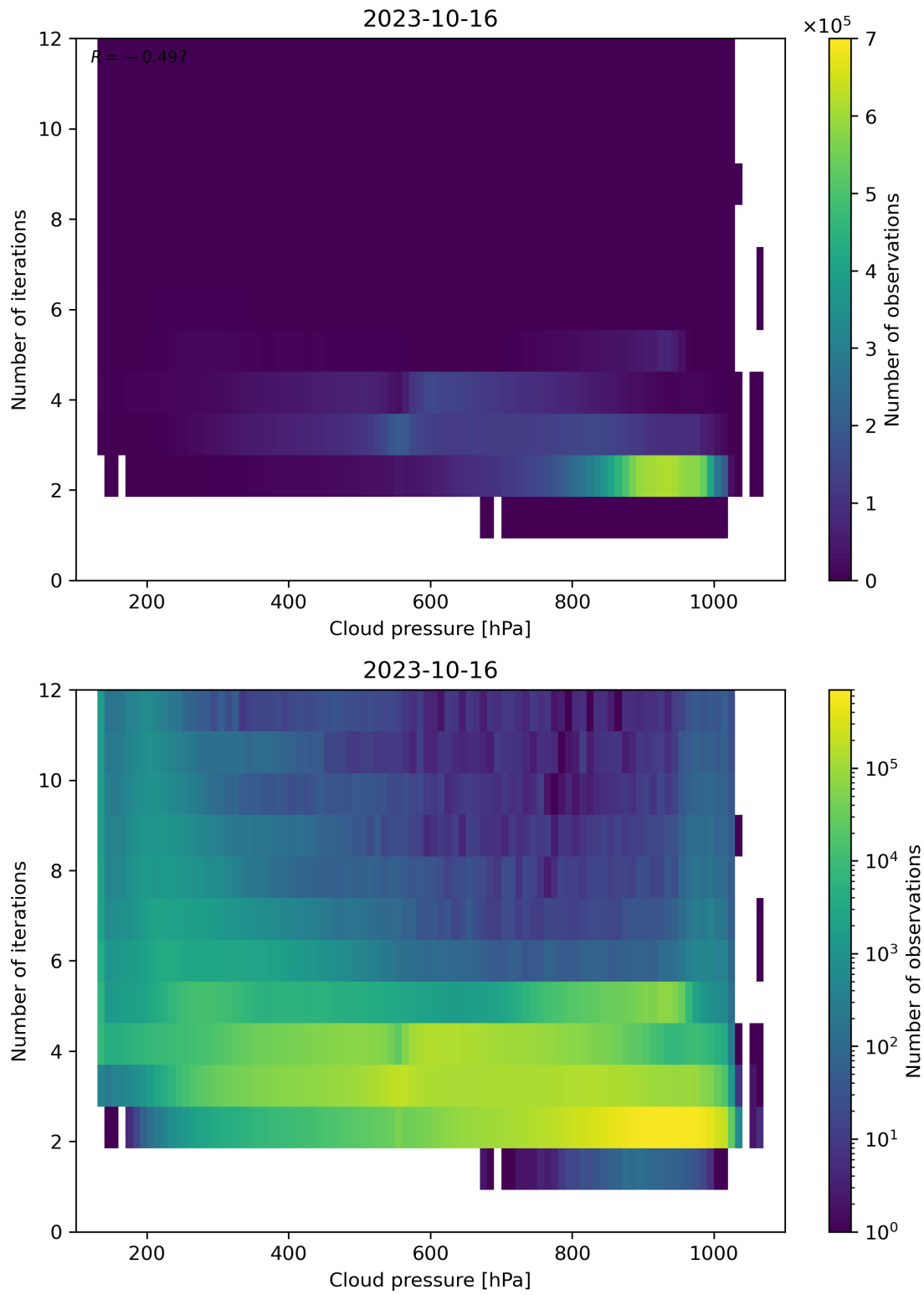
Figure 89: Scatter density plot of “Cloud pressure” against “Number of iterations” for 2023-10-15 to 2023-10-17.
