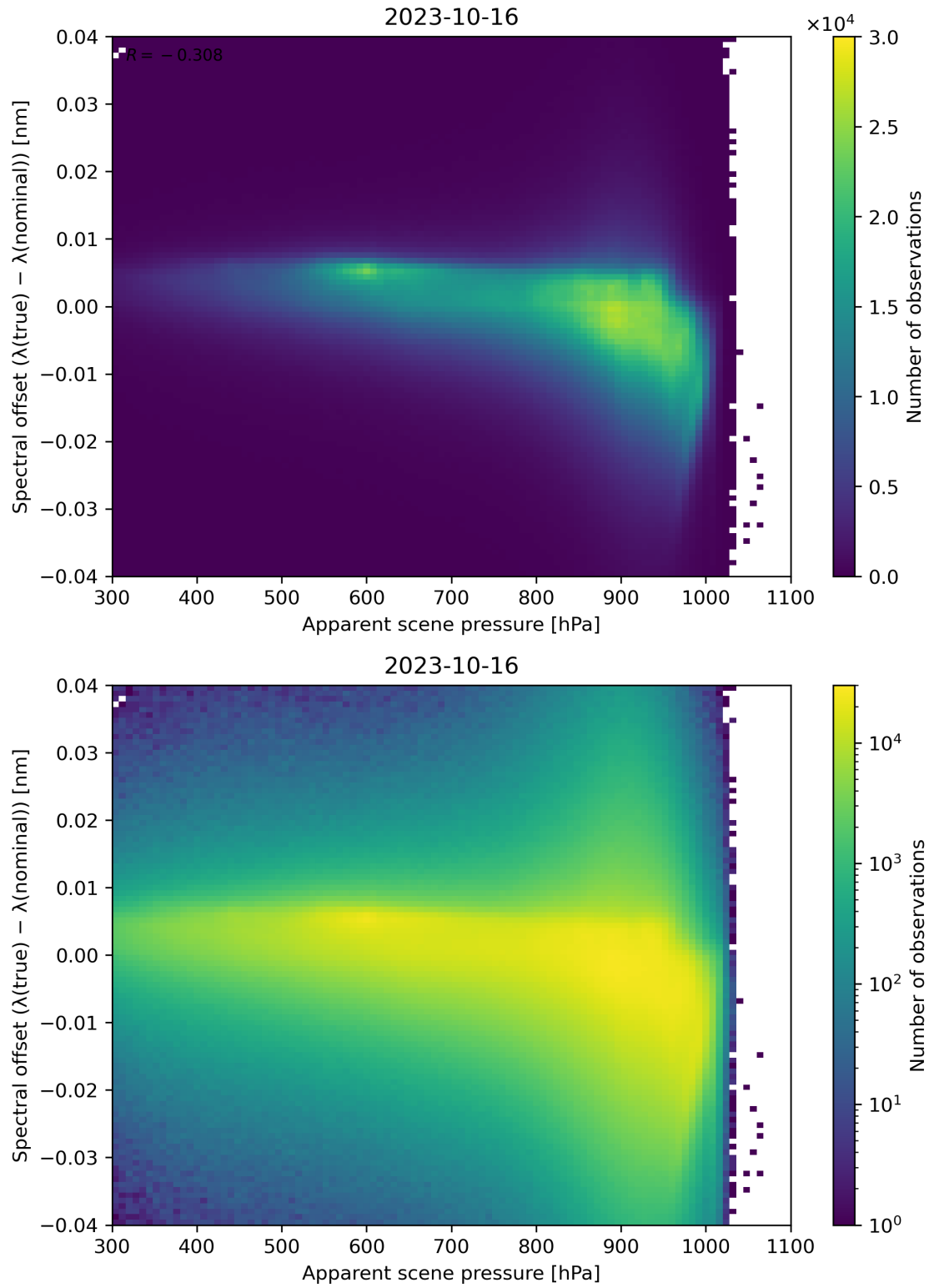
Figure 68: Scatter density plot of “Apparent scene pressure” against “Spectral offset ( \lambda(\text{true}) - \lambda(\text{nominal}) )” for 2023-10-15 to 2023-10-17.
