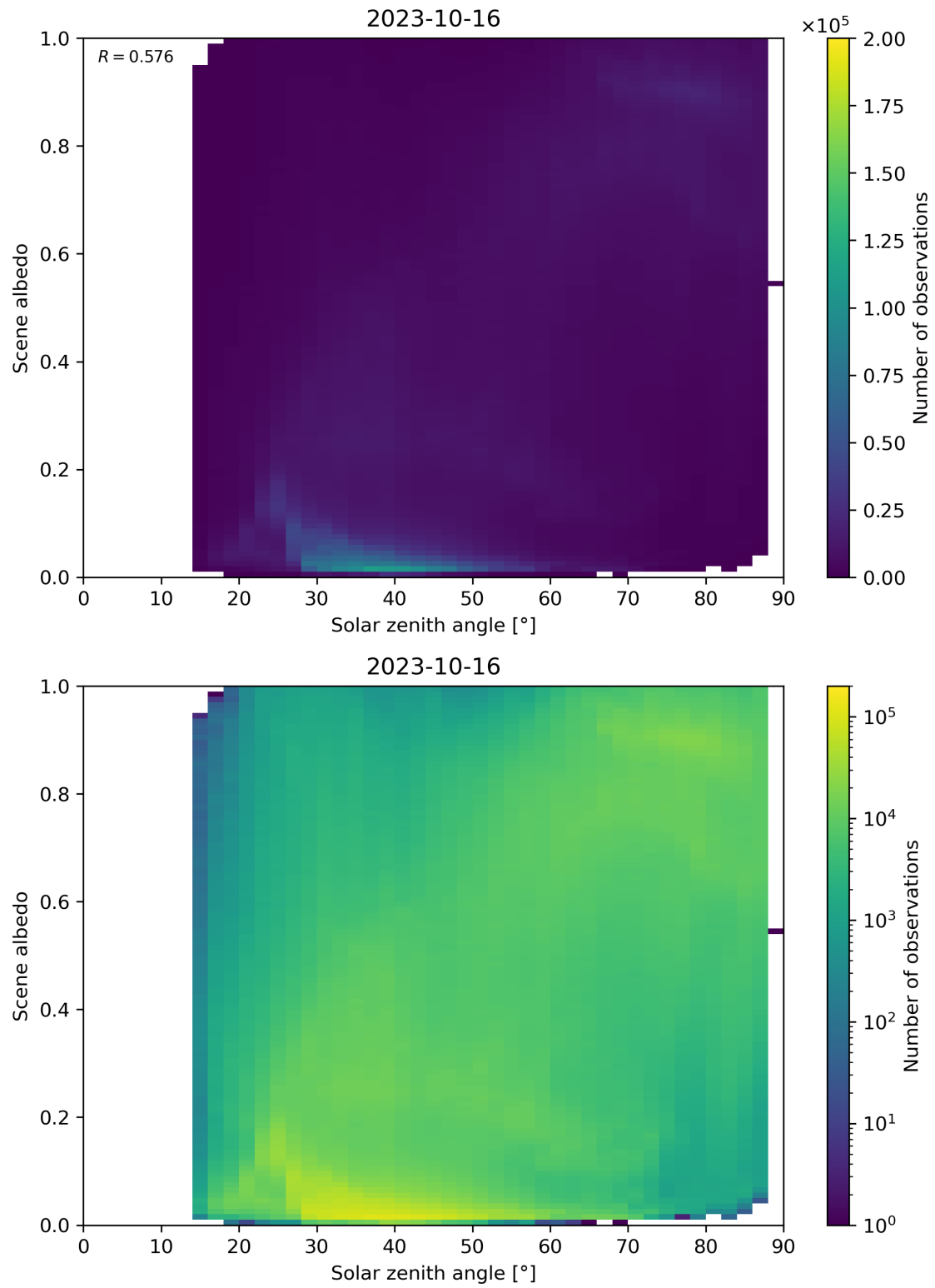
Figure 127: Scatter density plot of “Solar zenith angle” against “Scene albedo” for 2023-10-15 to 2023-10-17.
