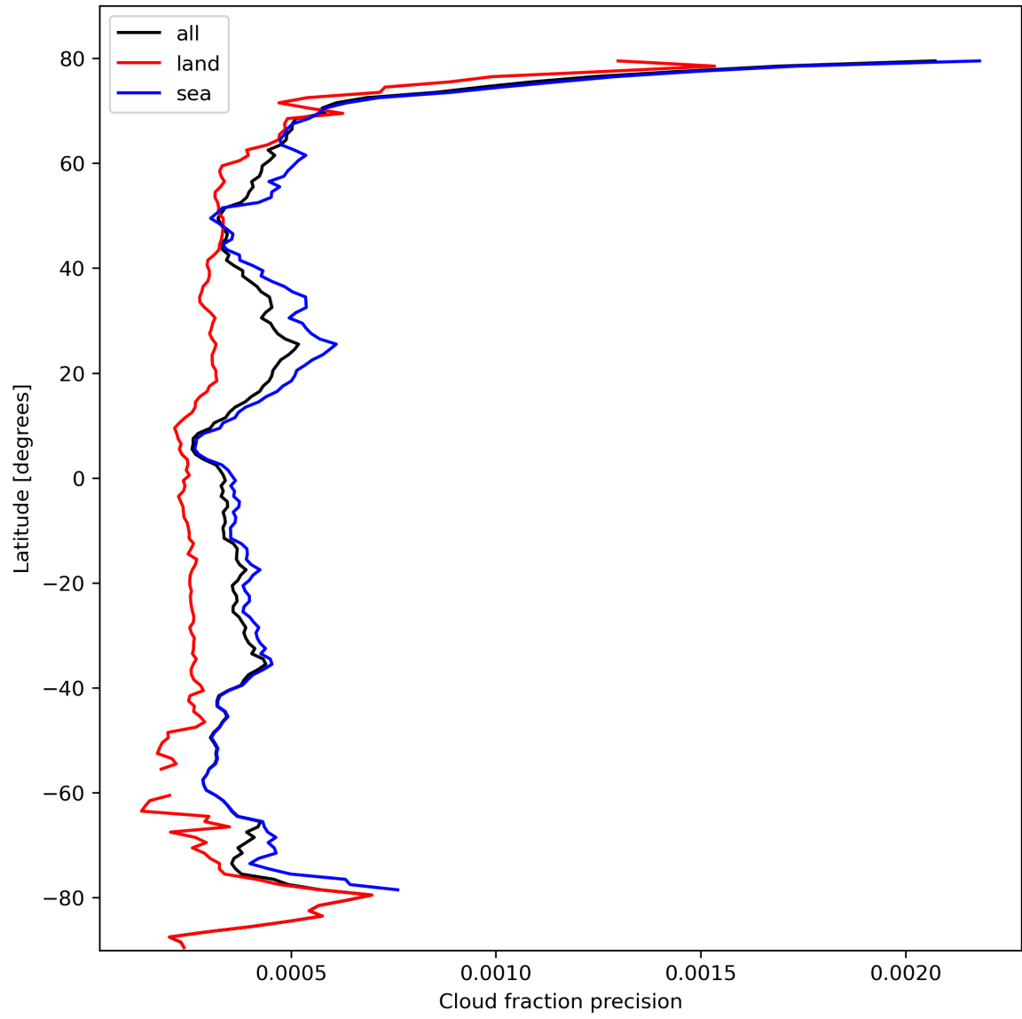
Figure 16: Zonal average of “Cloud fraction precision” for 2023-10-15 to 2023-10-17.
