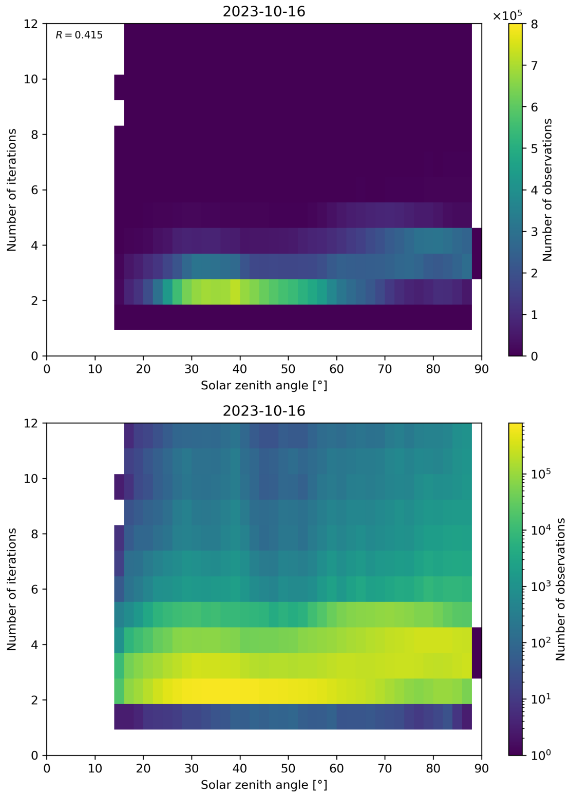
Figure 125: Scatter density plot of “Solar zenith angle” against “Number of iterations” for 2023-10-15 to 2023-10-17.
