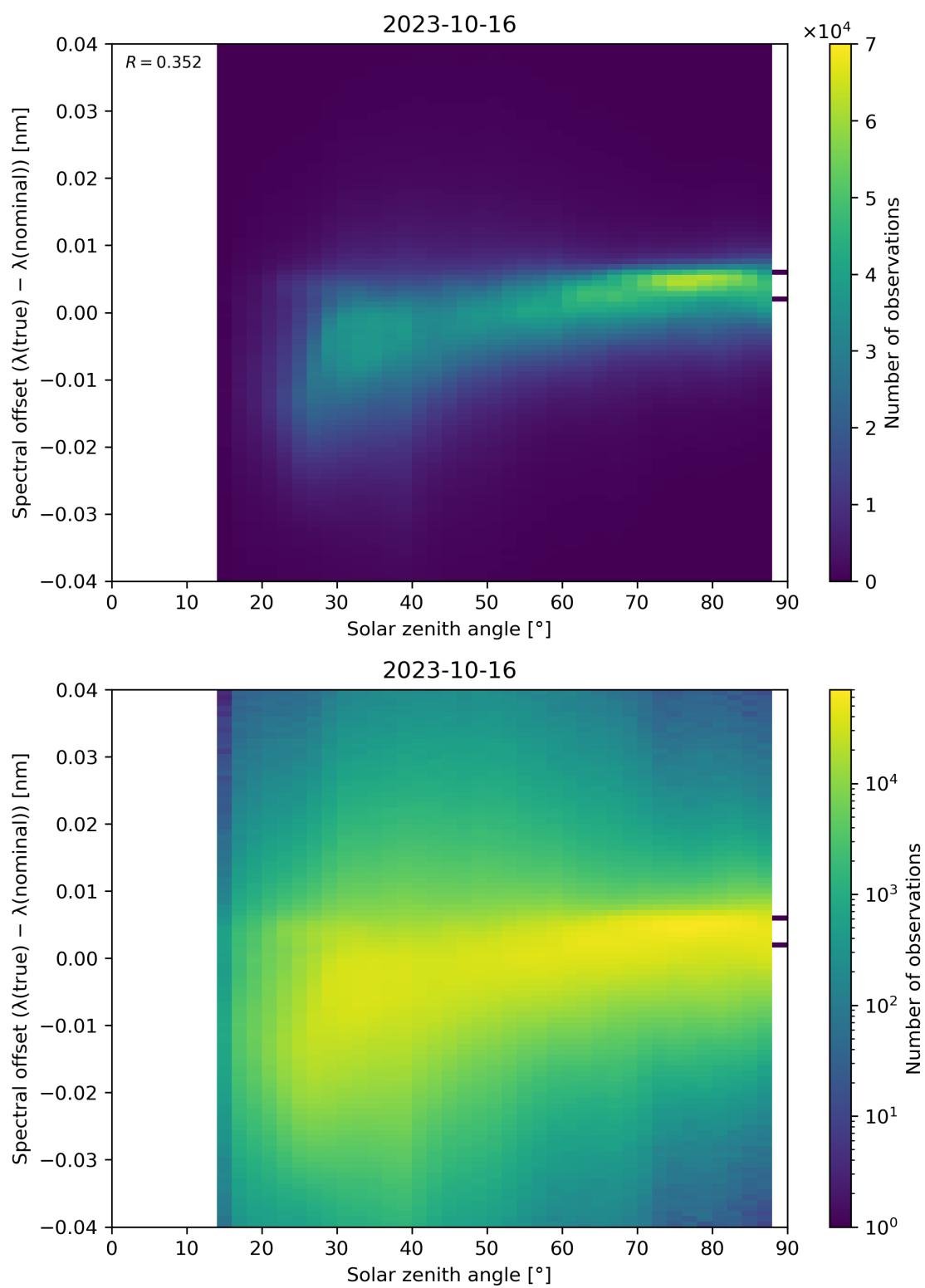
Figure 128: Scatter density plot of “Solar zenith angle” against “Spectral offset ( \lambda(\text{true}) - \lambda(\text{nominal}) )” for 2023-10-15 to 2023-10-17.
