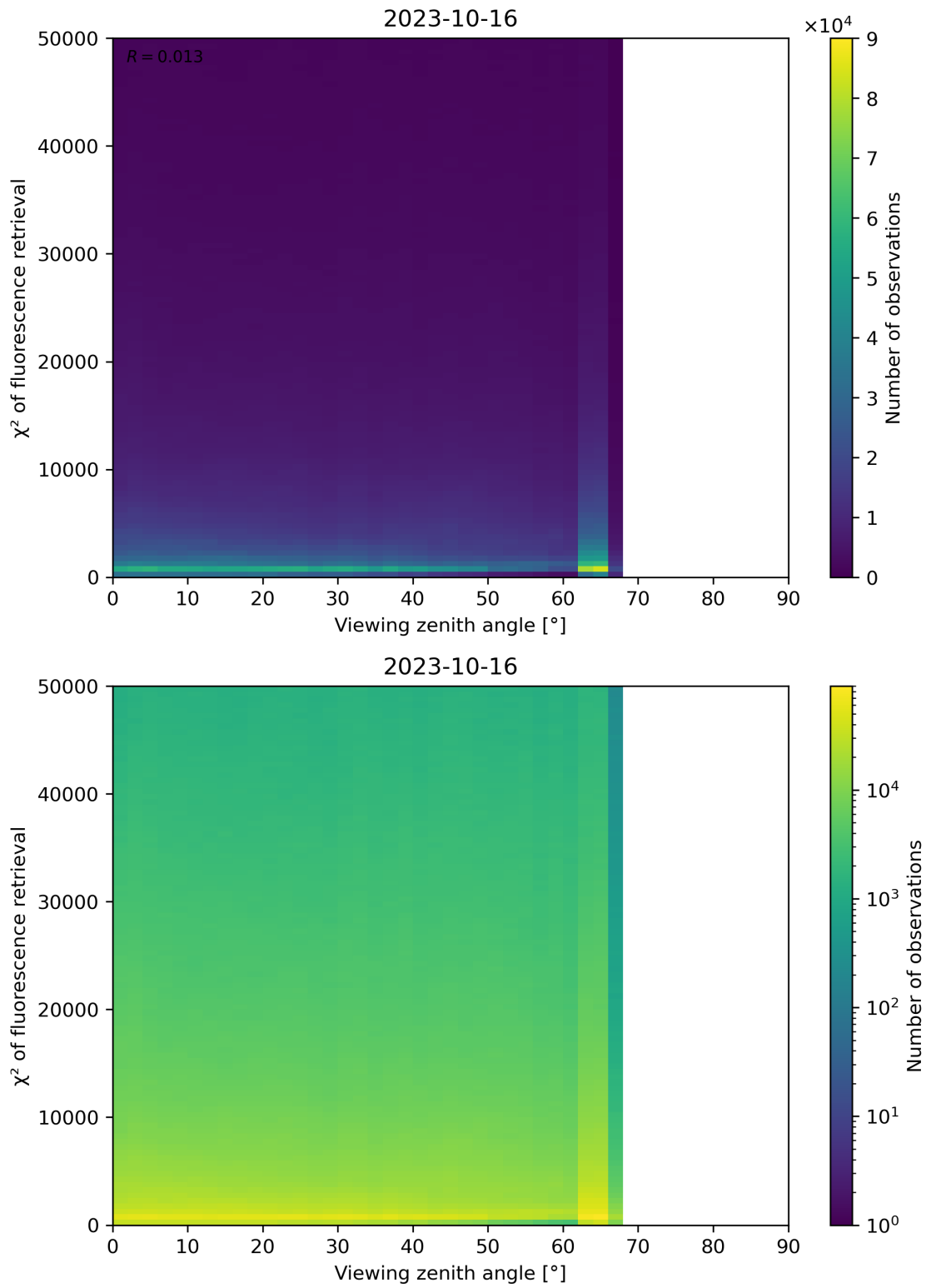
Figure 131: Scatter density plot of “Viewing zenith angle” against “ \chi^2 of fluorescence retrieval” for 2023-10-15 to 2023-10-17.
