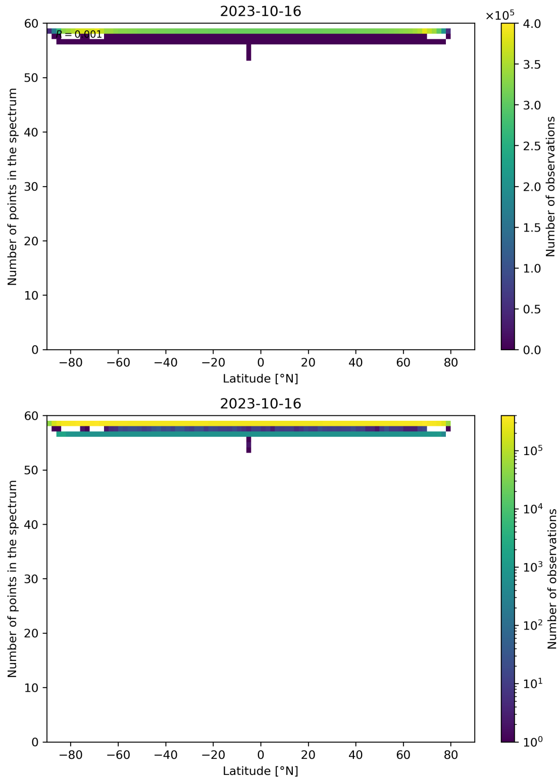
Figure 103: Scatter density plot of “Latitude” against “Number of points in the spectrum” for 2023-10-15 to 2023-10-17.
