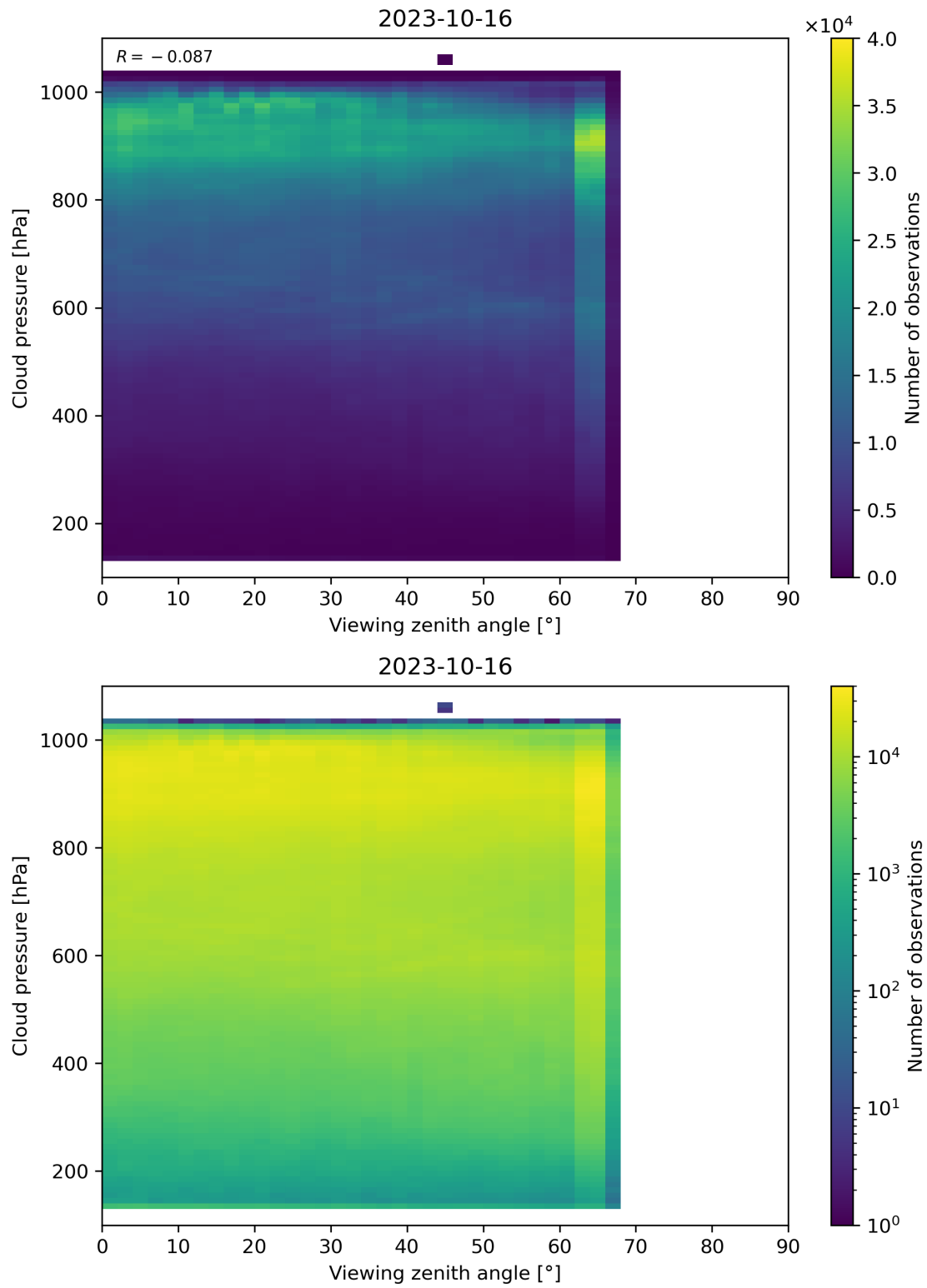
Figure 133: Scatter density plot of “Viewing zenith angle” against “Cloud pressure” for 2023-10-15 to 2023-10-17.
