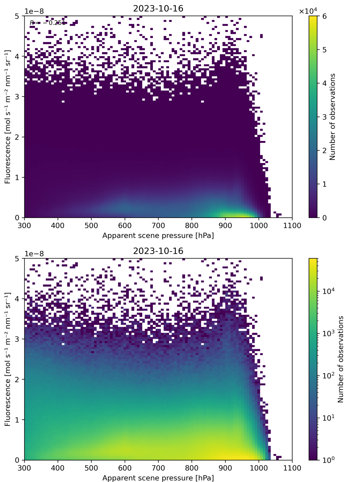
Figure 65: Scatter density plot of “Apparent scene pressure” against “Fluorescence” for 2023-10-15 to 2023-10-17.
