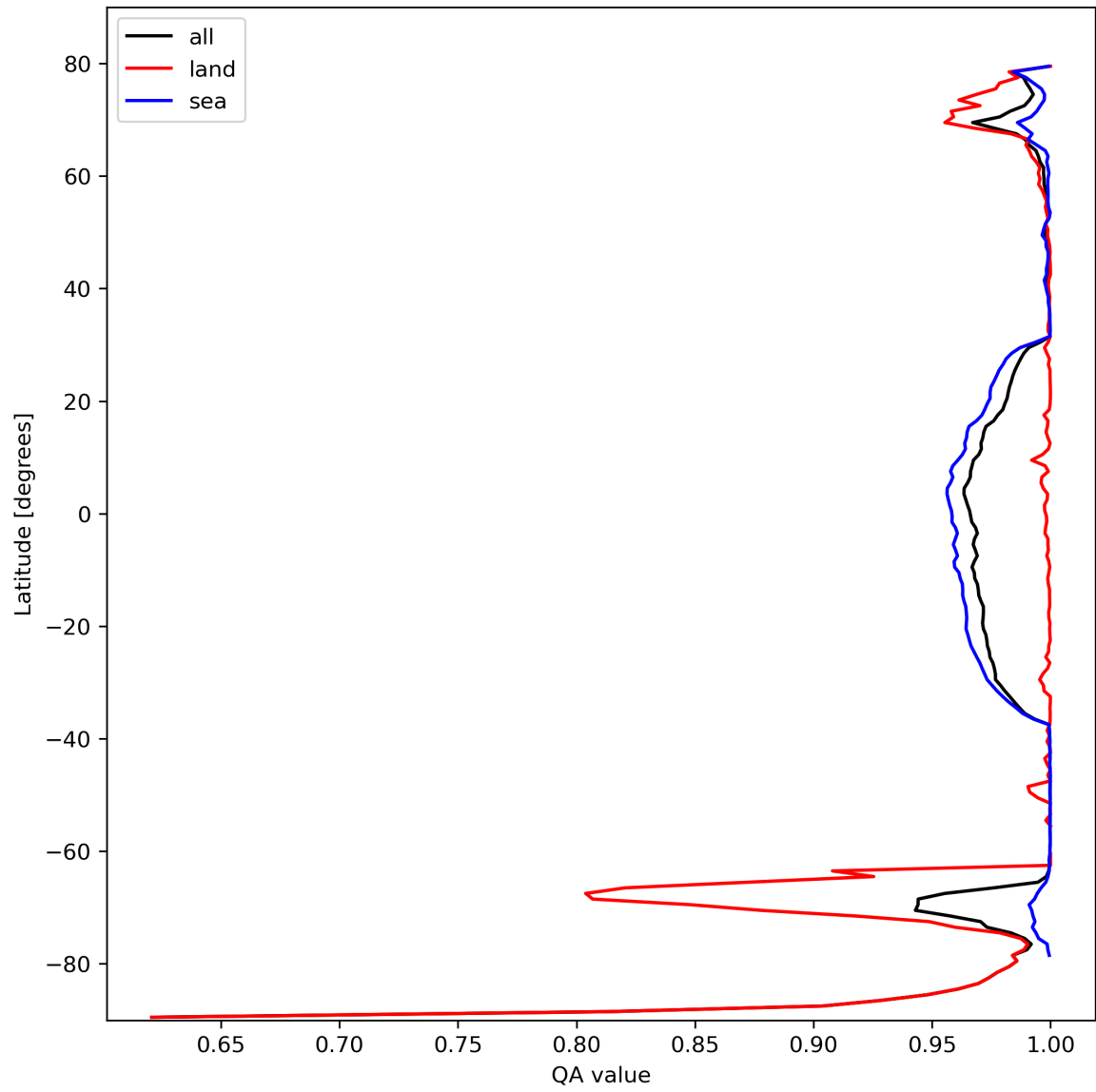
Figure 12: Zonal average of "QA value" for 2023-10-15 to 2023-10-17.
