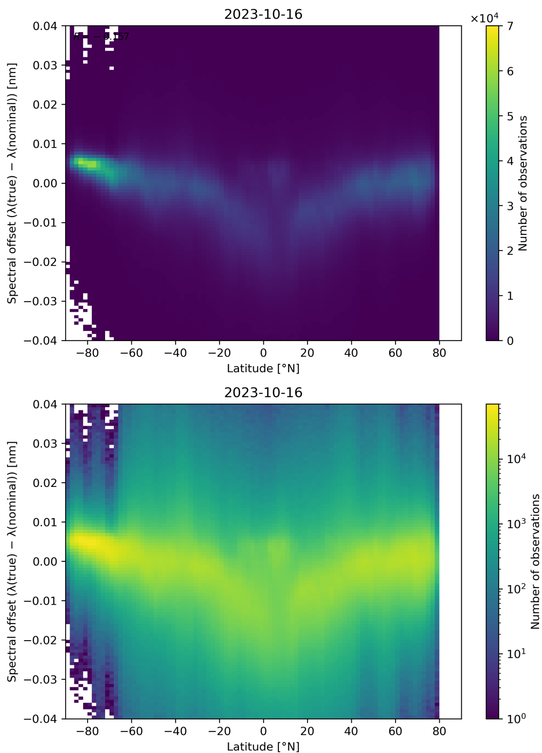
Figure 105: Scatter density plot of “Latitude” against “Spectral offset ( \lambda(\text{true}) - \lambda(\text{nominal}) )” for 2023-10-15 to 2023-10-17.
