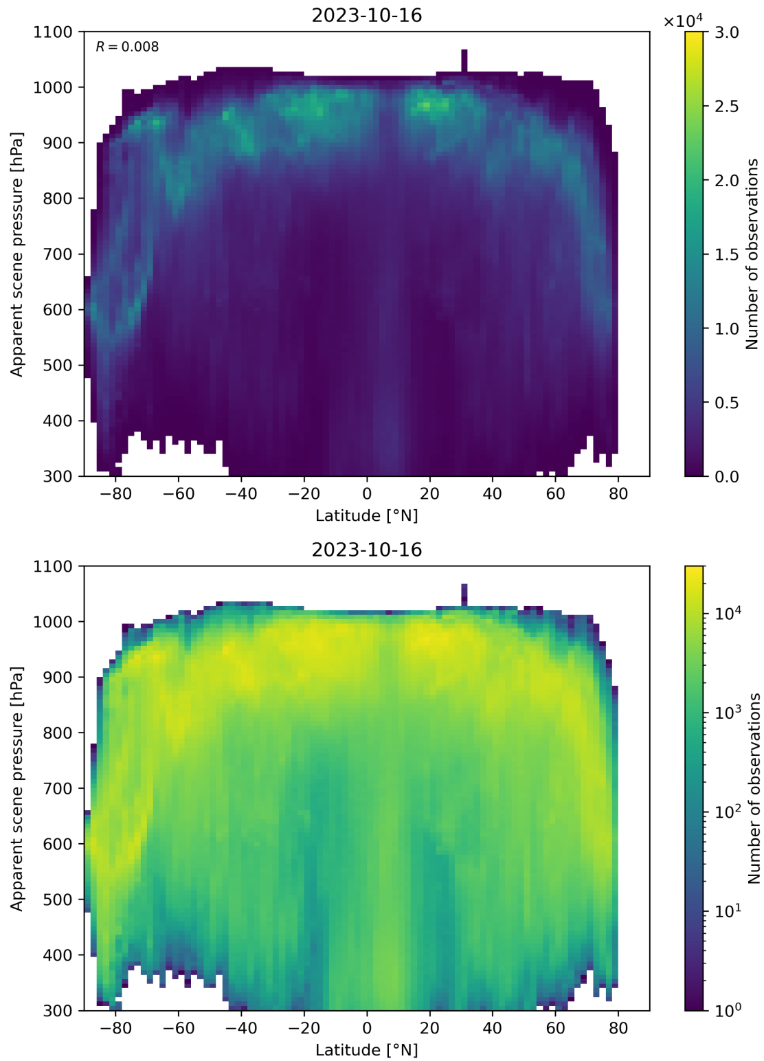
Figure 96: Scatter density plot of “Latitude” against “Apparent scene pressure” for 2023-10-15 to 2023-10-17.
