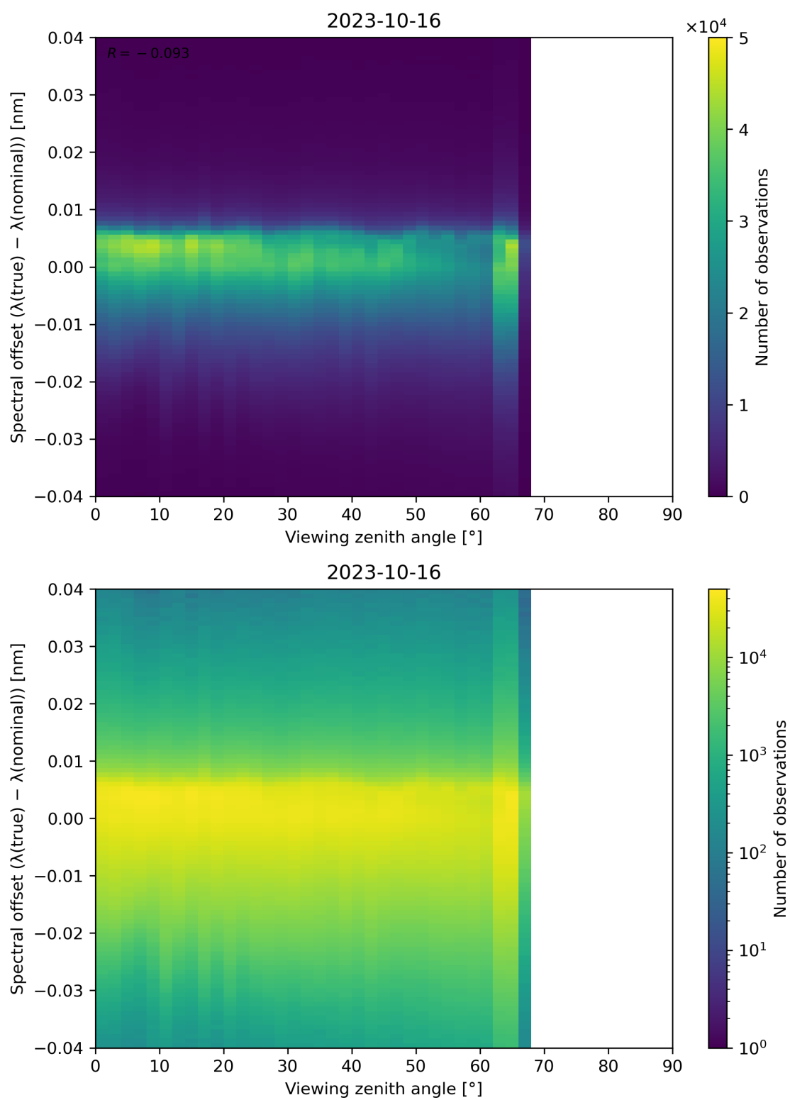
Figure 140: Scatter density plot of “Viewing zenith angle” against “Spectral offset ( \lambda(\text{true}) - \lambda(\text{nominal}) )” for 2023-10-15 to 2023-10-17.
