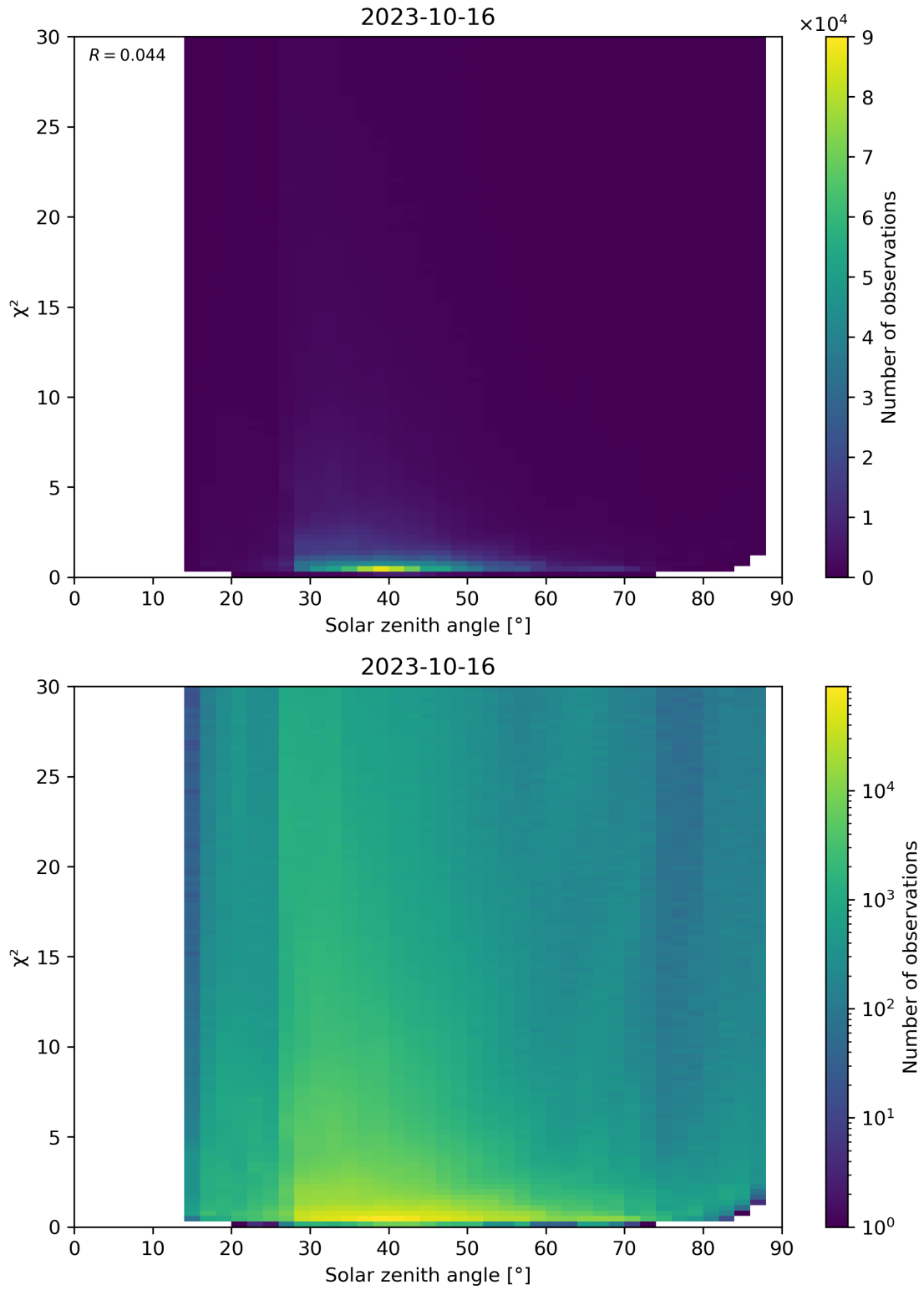
Figure 119: Scatter density plot of “Solar zenith angle” against “ \chi^2 ” for 2023-10-15 to 2023-10-17.
