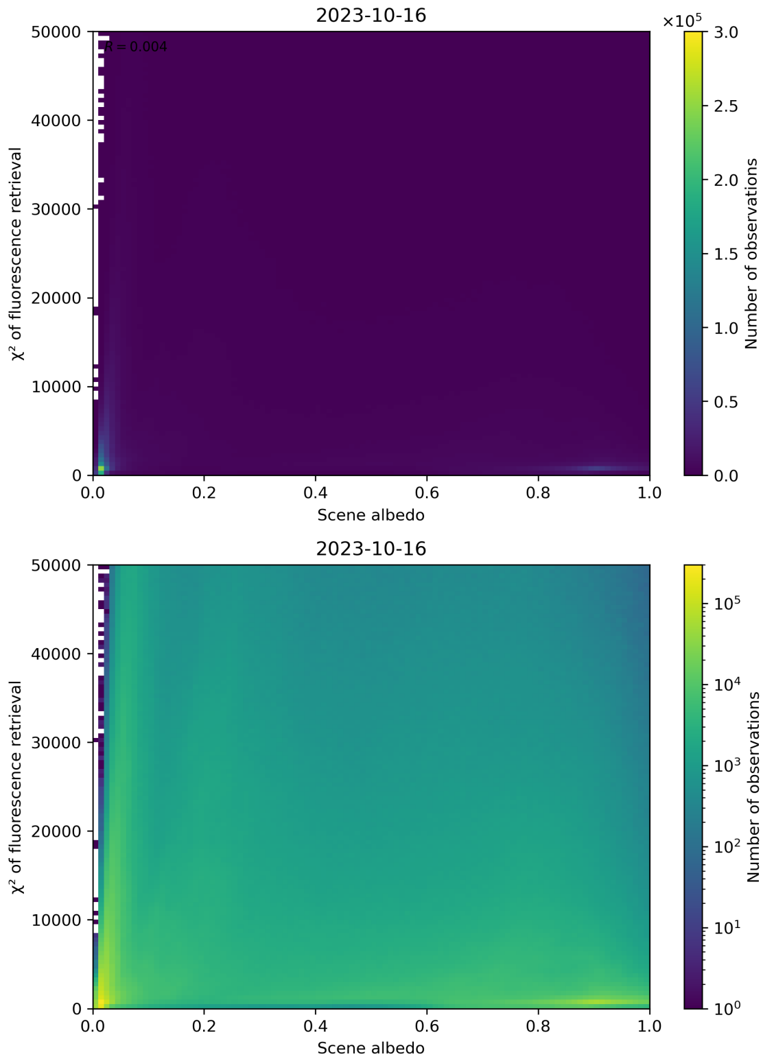
Figure 113: Scatter density plot of “Scene albedo” against “ \chi^2 of fluorescence retrieval” for 2023-10-15 to 2023-10-17.
