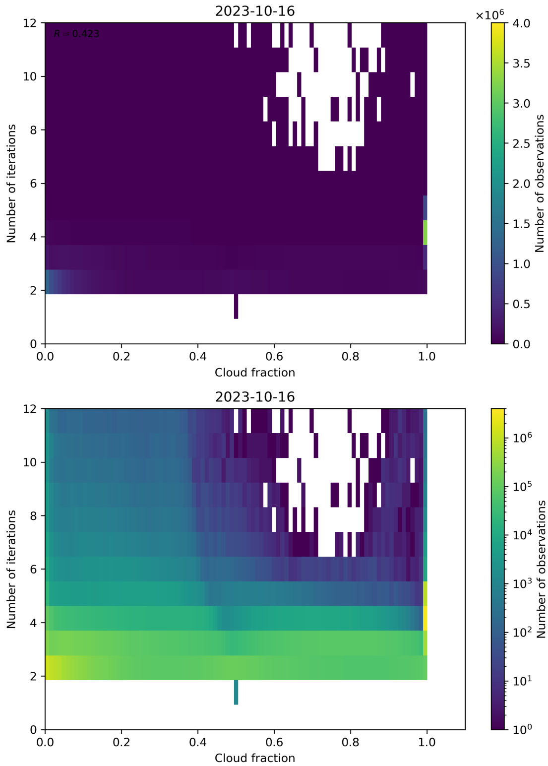
Figure 80: Scatter density plot of “Cloud fraction” against “Number of iterations” for 2023-10-15 to 2023-10-17.
