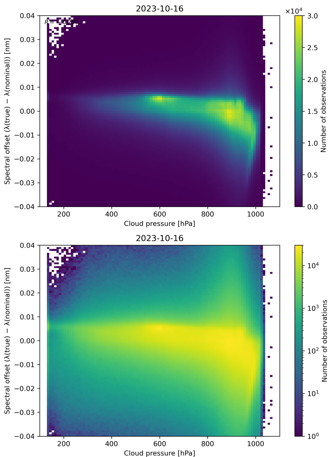
Figure 92: Scatter density plot of “Cloud pressure” against “Spectral offset ( \lambda(\text{true}) - \lambda(\text{nominal}) )” for 2023-10-15 to 2023-10-17.
