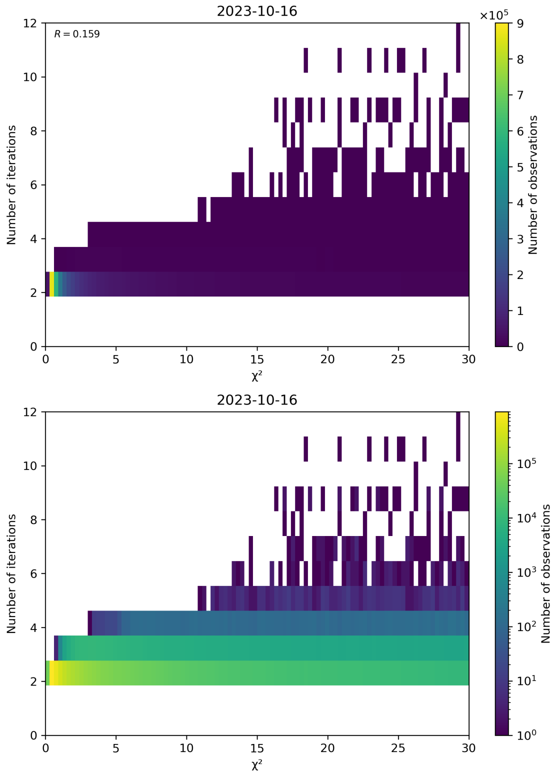
Figure 73: Scatter density plot of “ \chi^2 ” against “Number of iterations” for 2023-10-15 to 2023-10-17.
