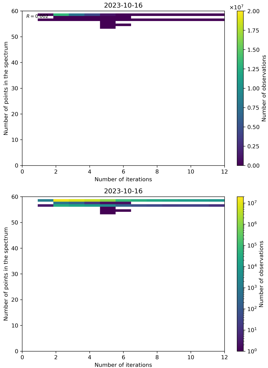
Figure 108: Scatter density plot of “Number of iterations” against “Number of points in the spectrum” for 2023-10-15 to 2023-10-17.
