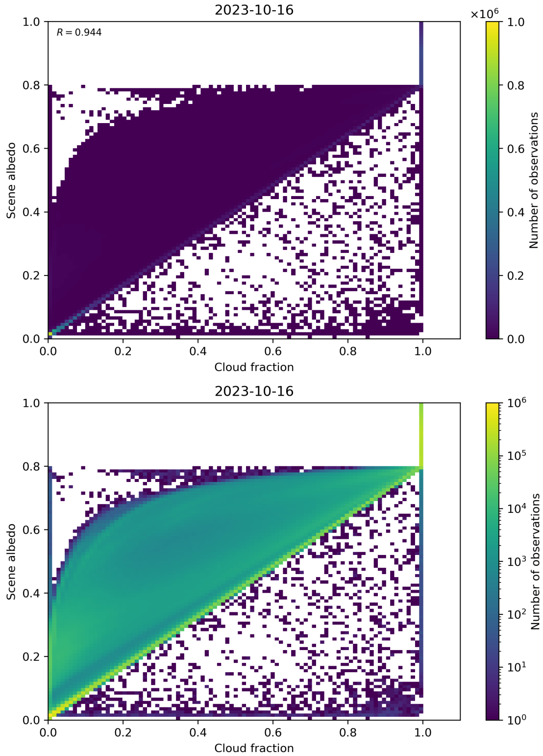
Figure 82: Scatter density plot of “Cloud fraction” against “Scene albedo” for 2023-10-15 to 2023-10-17.
