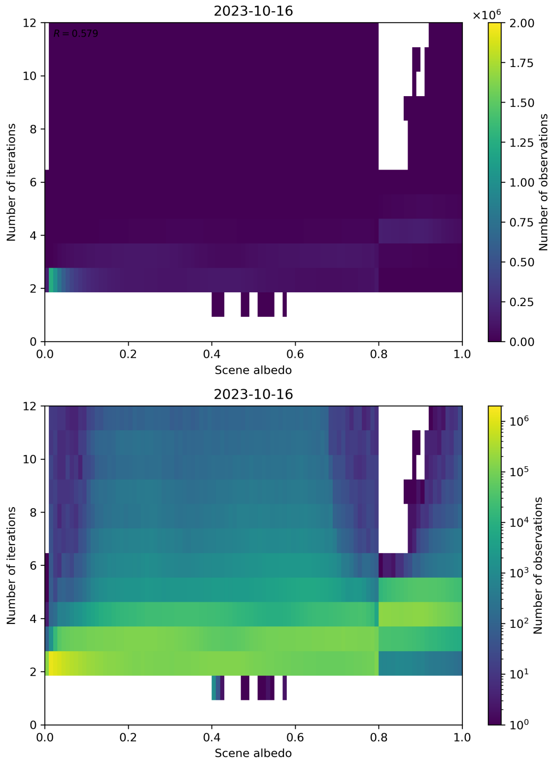
Figure 115: Scatter density plot of “Scene albedo” against “Number of iterations” for 2023-10-15 to 2023-10-17.
