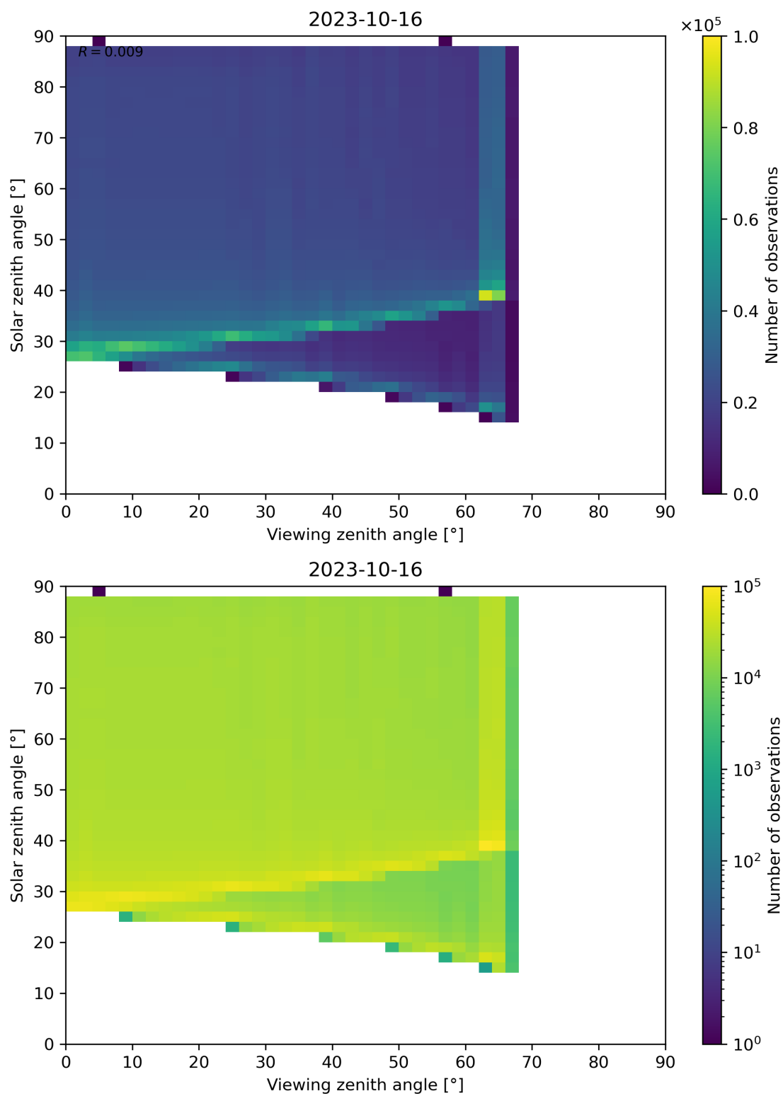
Figure 139: Scatter density plot of “Viewing zenith angle” against “Solar zenith angle” for 2023-10-15 to 2023-10-17.
