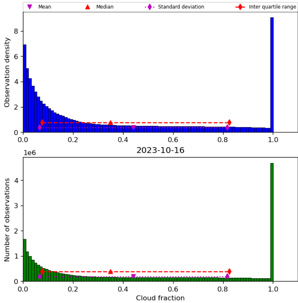
Figure 32: Histogram of “Cloud fraction” for 2023-10-15 to 2023-10-17
