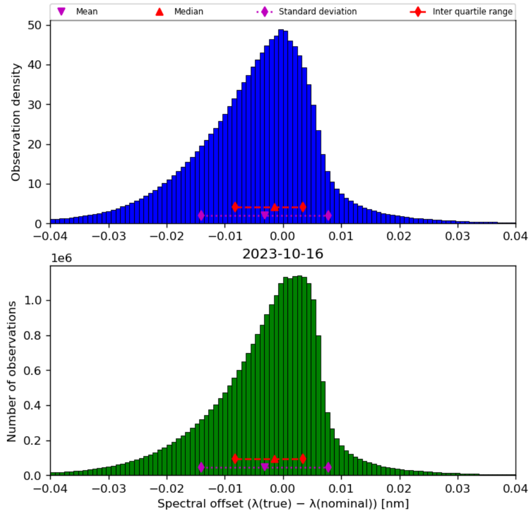
Figure 45: Histogram of “Spectral offset ( \lambda(\text{true}) - \lambda(\text{nominal}) )” for 2023-10-15 to 2023-10-17
