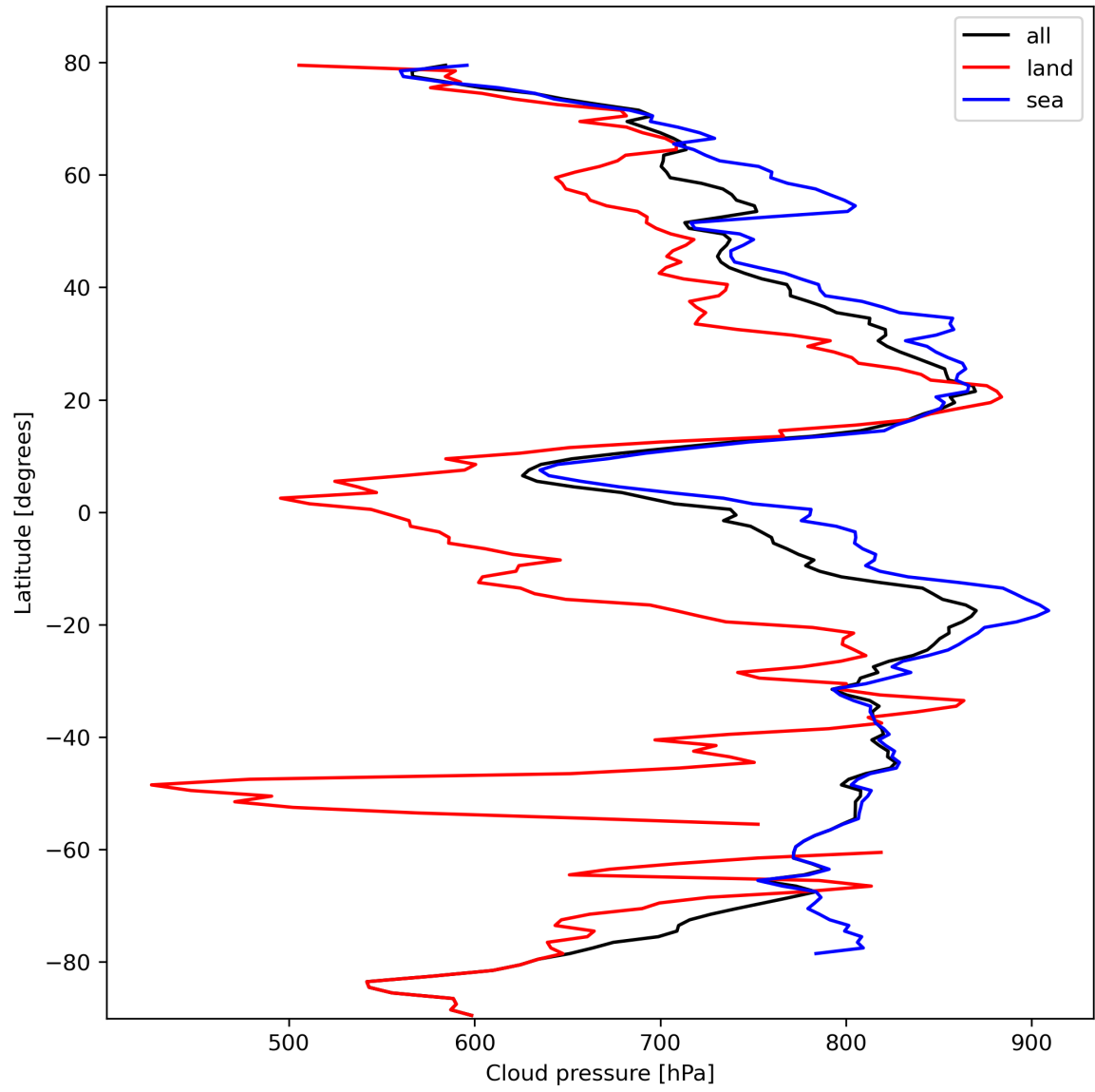
Figure 13: Zonal average of “Cloud pressure” for 2023-10-15 to 2023-10-17.
