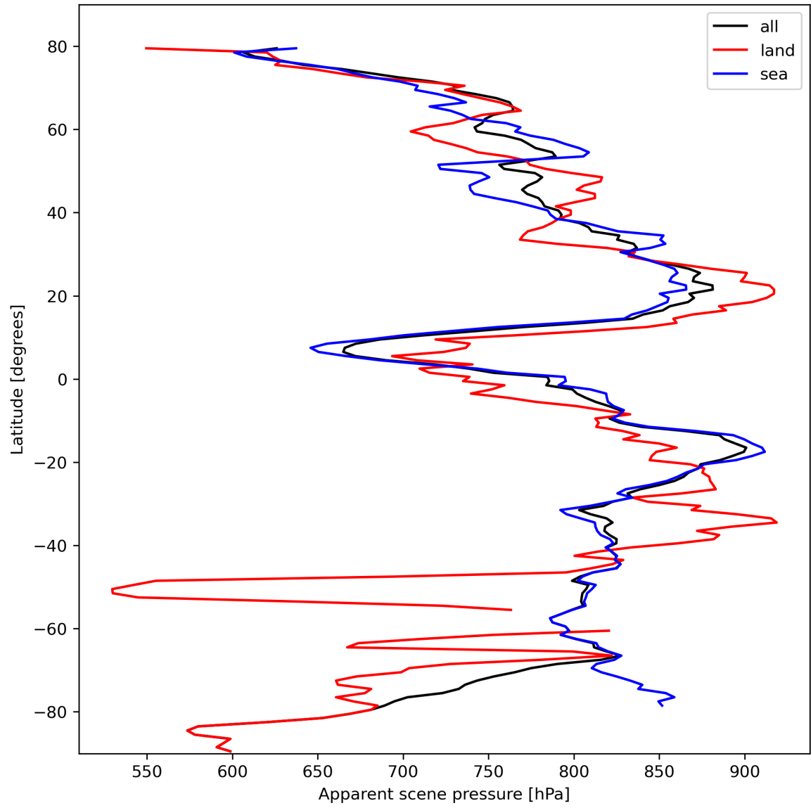
Figure 19: Zonal average of “Apparent scene pressure” for 2023-10-15 to 2023-10-17.
