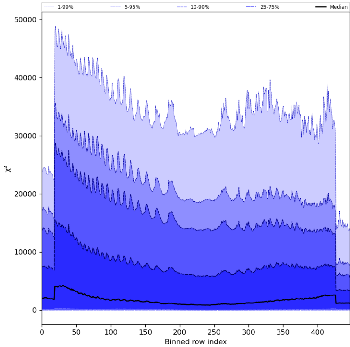
Figure 55: Along track statistics of “ \chi^2 ” for 2023-10-15 to 2023-10-17
