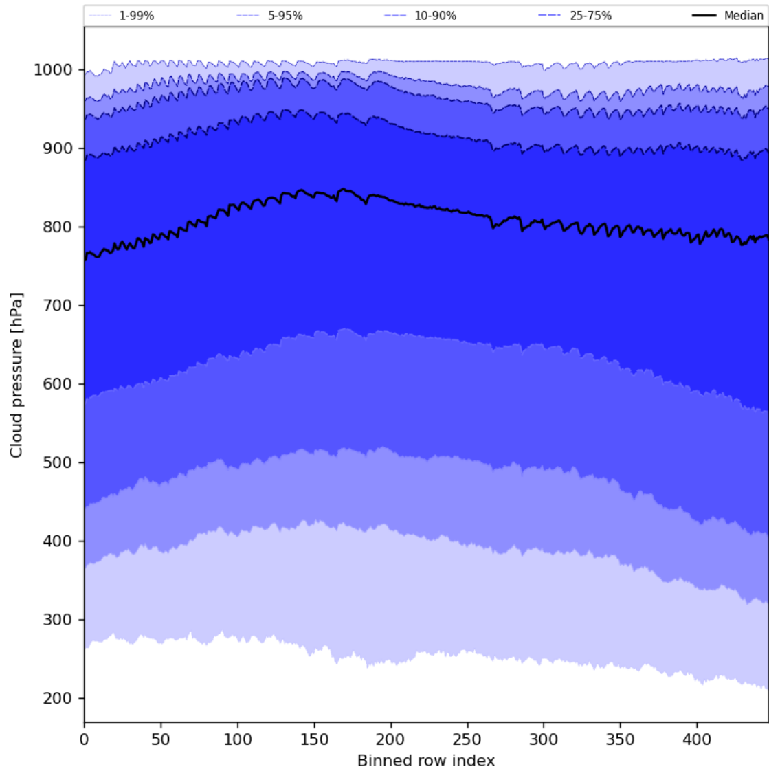
Figure 47: Along track statistics of “Cloud pressure” for 2023-10-15 to 2023-10-17
