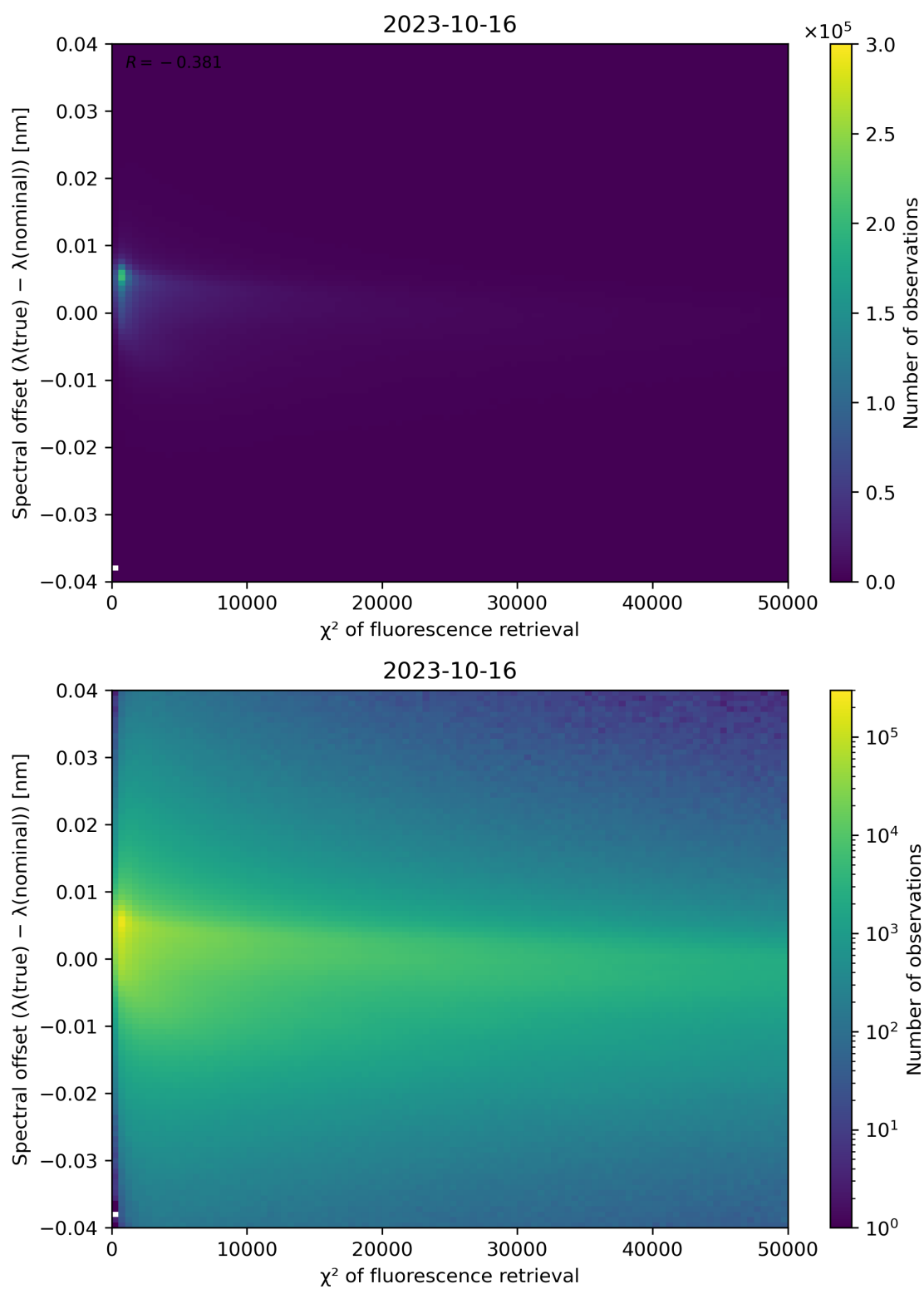
Figure 72: Scatter density plot of “ \chi^2 of fluorescence retrieval” against “Spectral offset ( \lambda(\text{true}) - \lambda(\text{nominal}) )” for 2023-10-15 to 2023-10-17.
