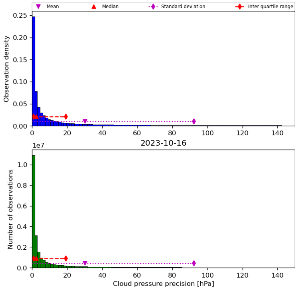
Figure 31: Histogram of “Cloud pressure precision” for 2023-10-15 to 2023-10-17
