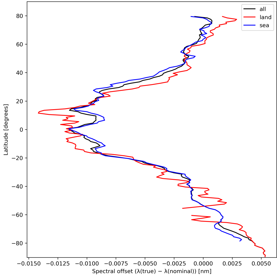
Figure 28: Zonal average of “Spectral offset ( \lambda(\text{true}) - \lambda(\text{nominal}) )” for 2023-10-15 to 2023-10-17.
