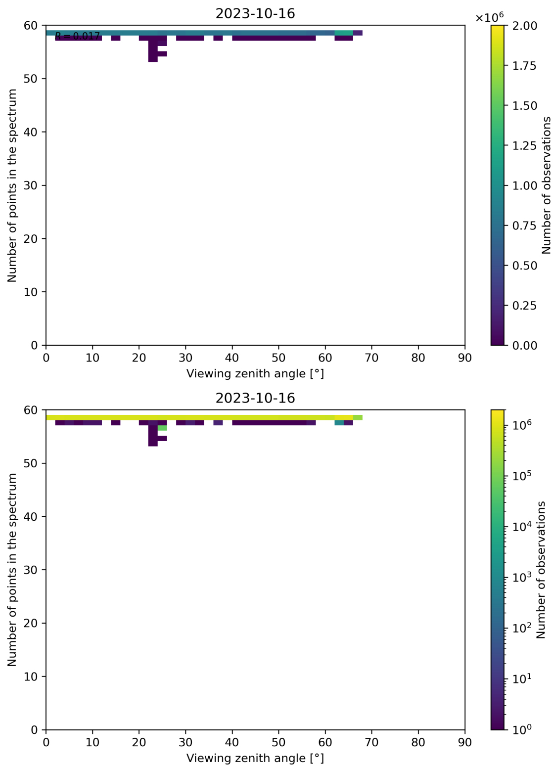
Figure 137: Scatter density plot of “Viewing zenith angle” against “Number of points in the spectrum” for 2023-10-15 to 2023-10-17.
