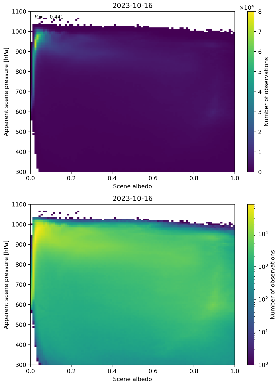
Figure 111: Scatter density plot of “Scene albedo” against “Apparent scene pressure” for 2023-10-15 to 2023-10-17.
