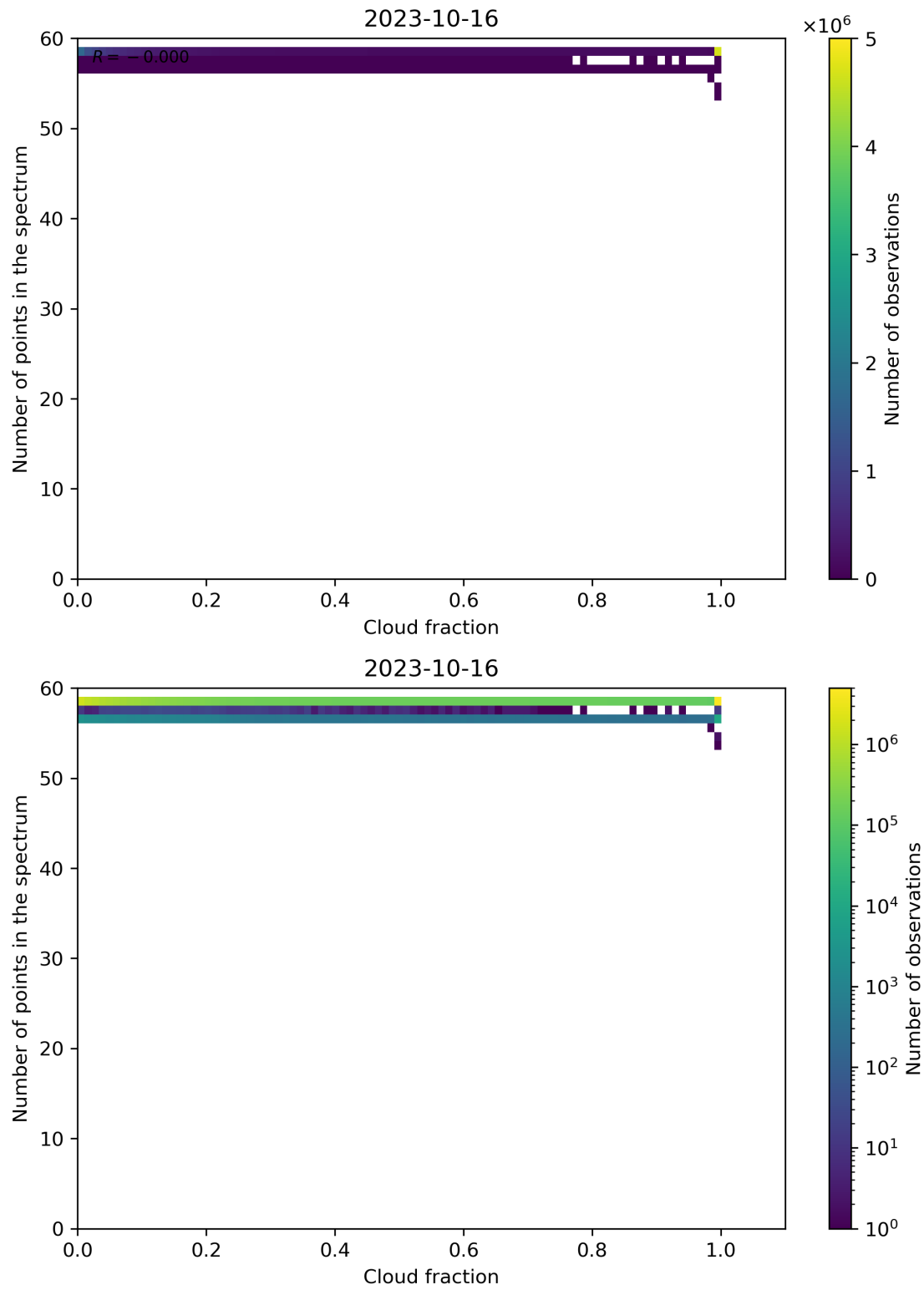
Figure 81: Scatter density plot of “Cloud fraction” against “Number of points in the spectrum” for 2023-10-15 to 2023-10-17.
