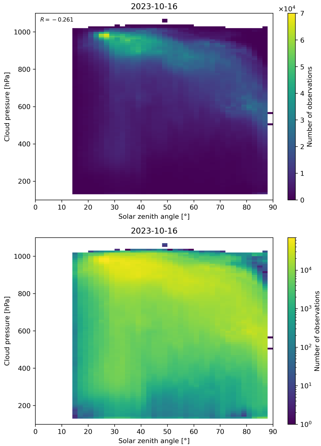
Figure 122: Scatter density plot of “Solar zenith angle” against “Cloud pressure” for 2023-10-15 to 2023-10-17.
