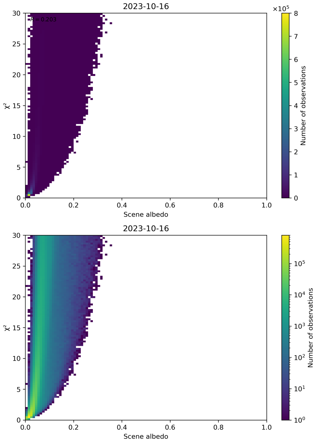
Figure 112: Scatter density plot of “Scene albedo” against “ \chi^2 ” for 2023-10-15 to 2023-10-17.
