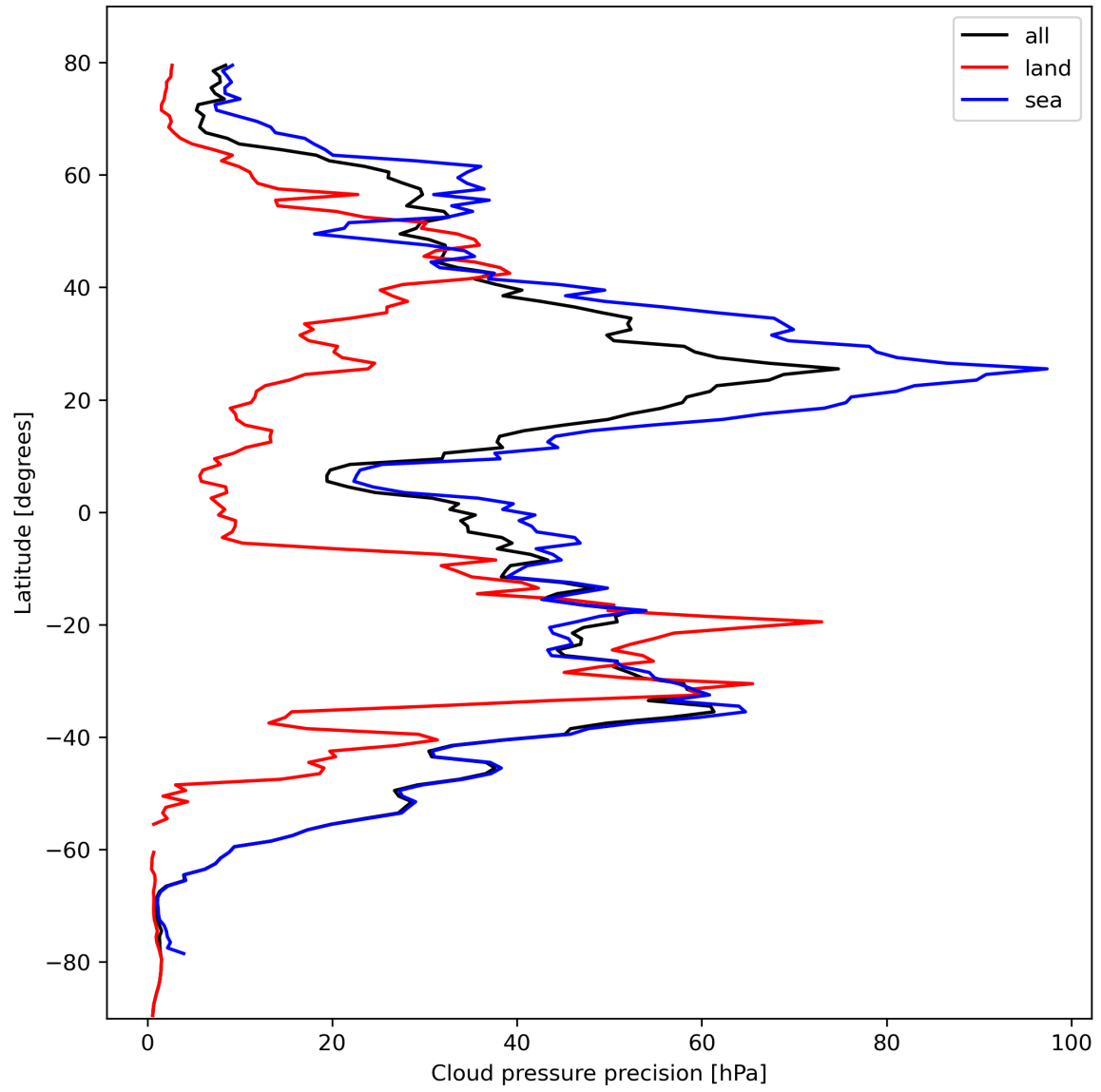
Figure 14: Zonal average of “Cloud pressure precision” for 2023-10-15 to 2023-10-17.
