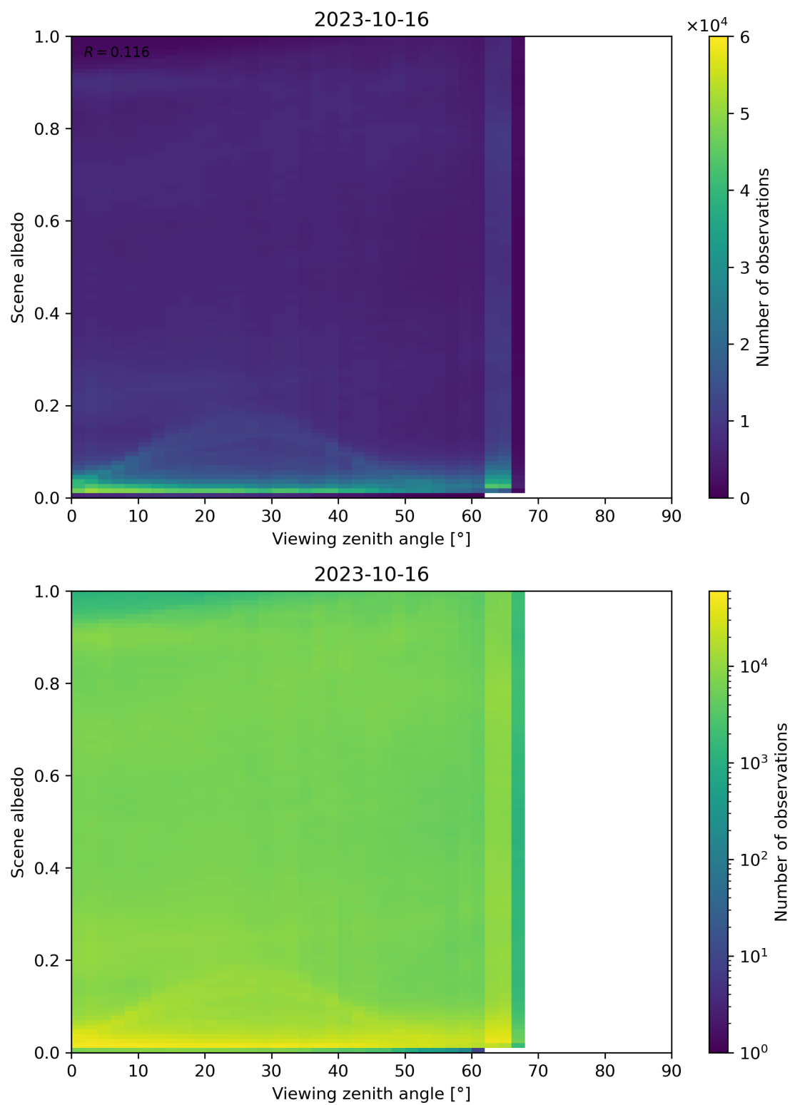
Figure 138: Scatter density plot of “Viewing zenith angle” against “Scene albedo” for 2023-10-15 to 2023-10-17.
