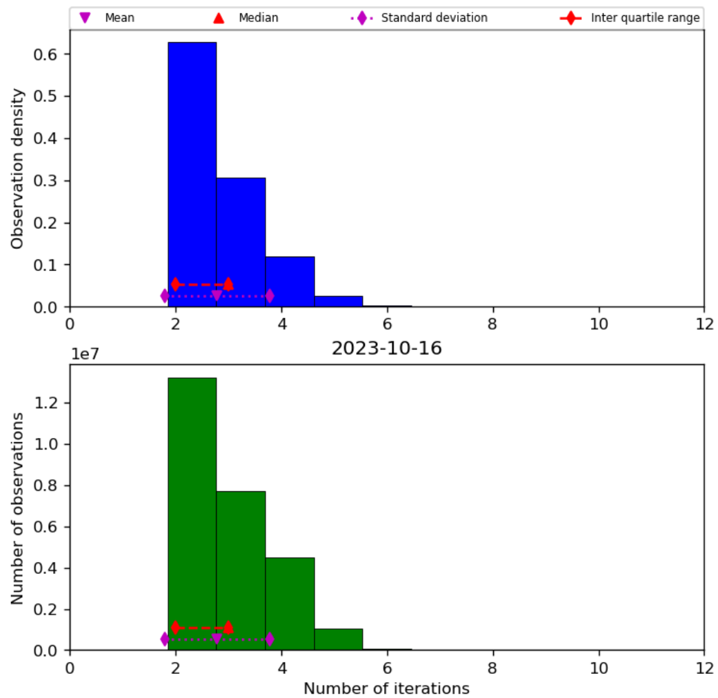
Figure 39: Histogram of “Number of iterations” for 2023-10-15 to 2023-10-17
