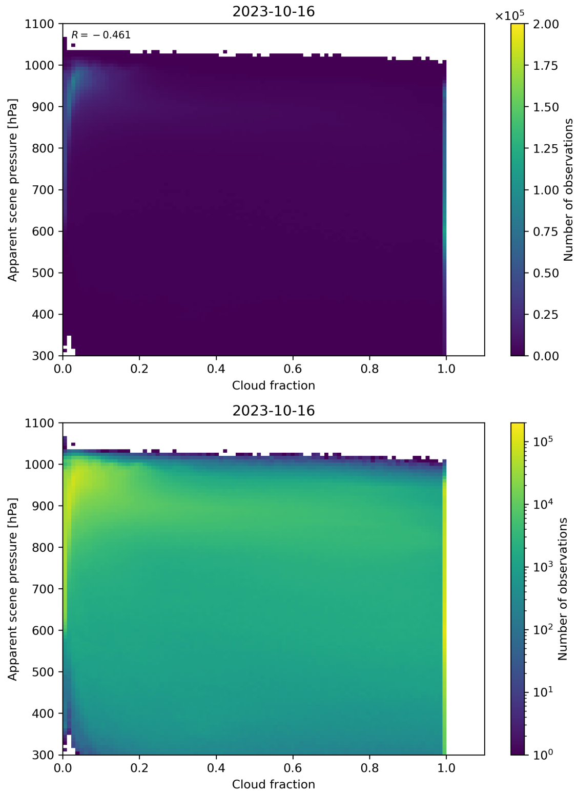
Figure 76: Scatter density plot of “Cloud fraction” against “Apparent scene pressure” for 2023-10-15 to 2023-10-17.
