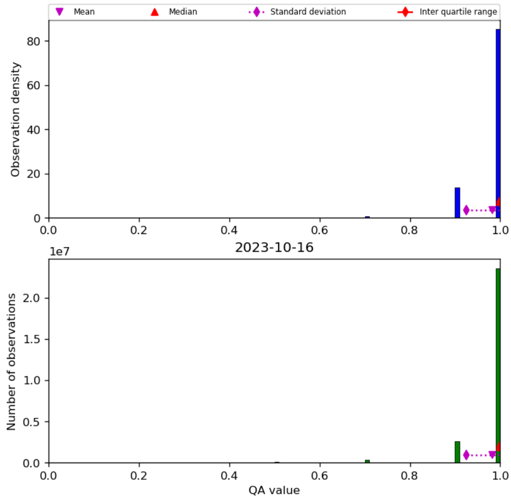
Figure 29: Histogram of “QA value” for 2023-10-15 to 2023-10-17
