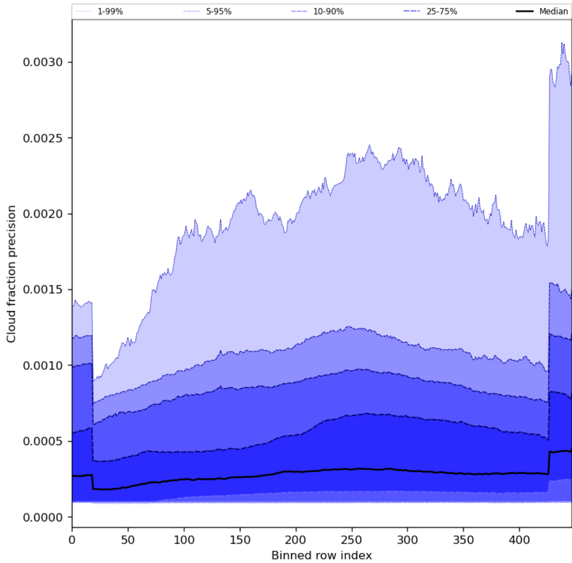
Figure 50: Along track statistics of “Cloud fraction precision” for 2023-10-15 to 2023-10-17
