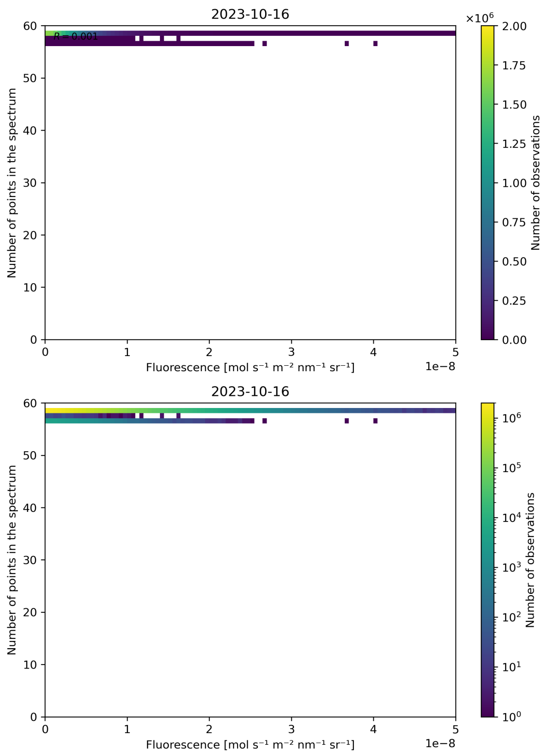
Figure 94: Scatter density plot of “Fluorescence” against “Number of points in the spectrum” for 2023-10-15 to 2023-10-17.
