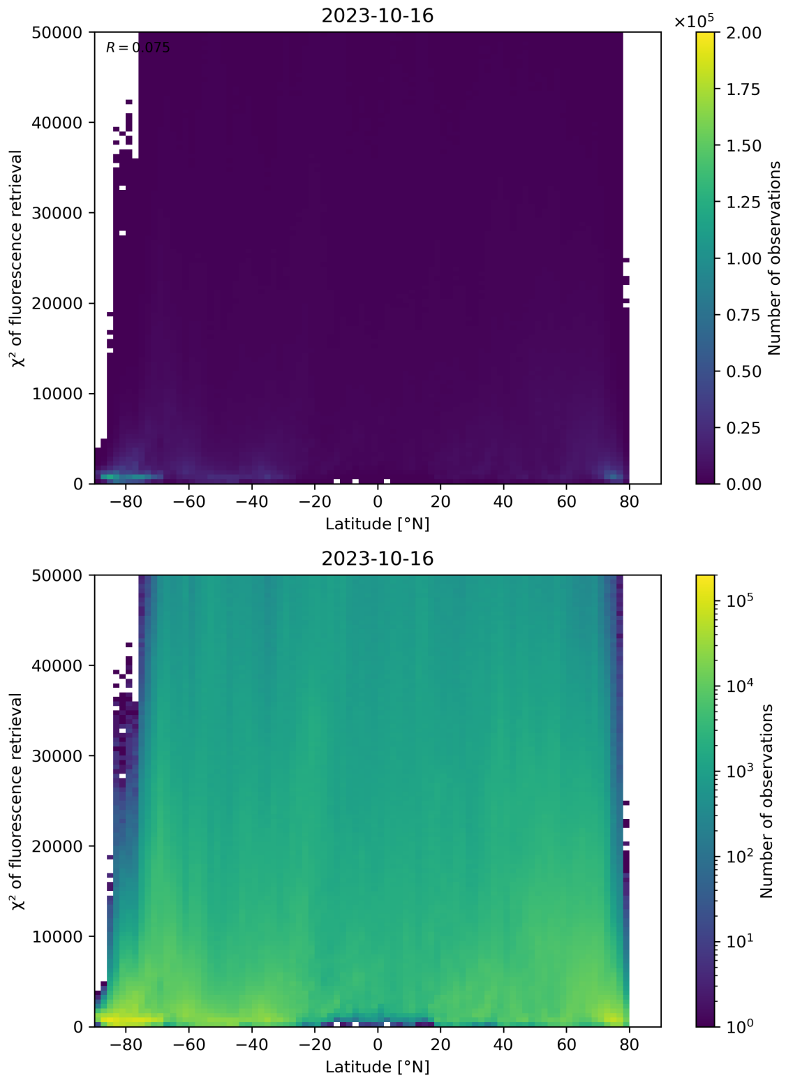
Figure 98: Scatter density plot of “Latitude” against “ \chi^2 of fluorescence retrieval” for 2023-10-15 to 2023-10-17.
