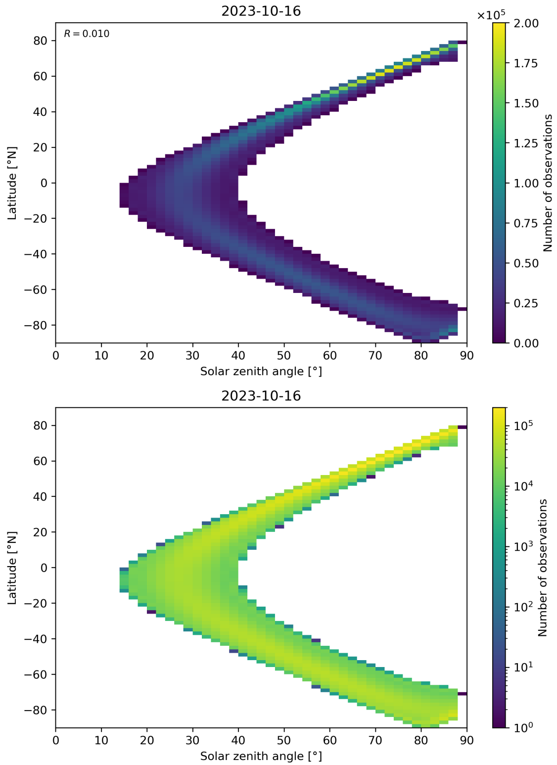
Figure 124: Scatter density plot of “Solar zenith angle” against “Latitude” for 2023-10-15 to 2023-10-17.
