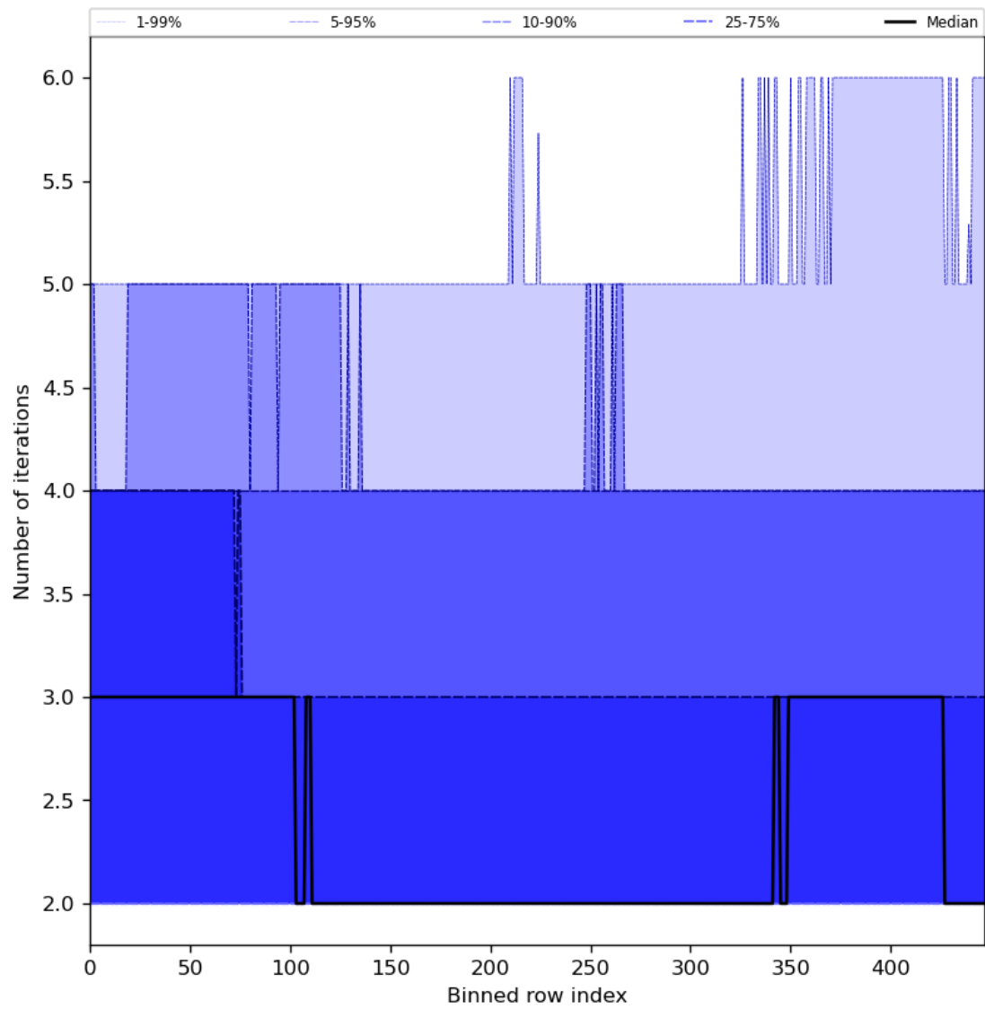
Figure 56: Along track statistics of “Number of iterations” for 2023-10-15 to 2023-10-17
