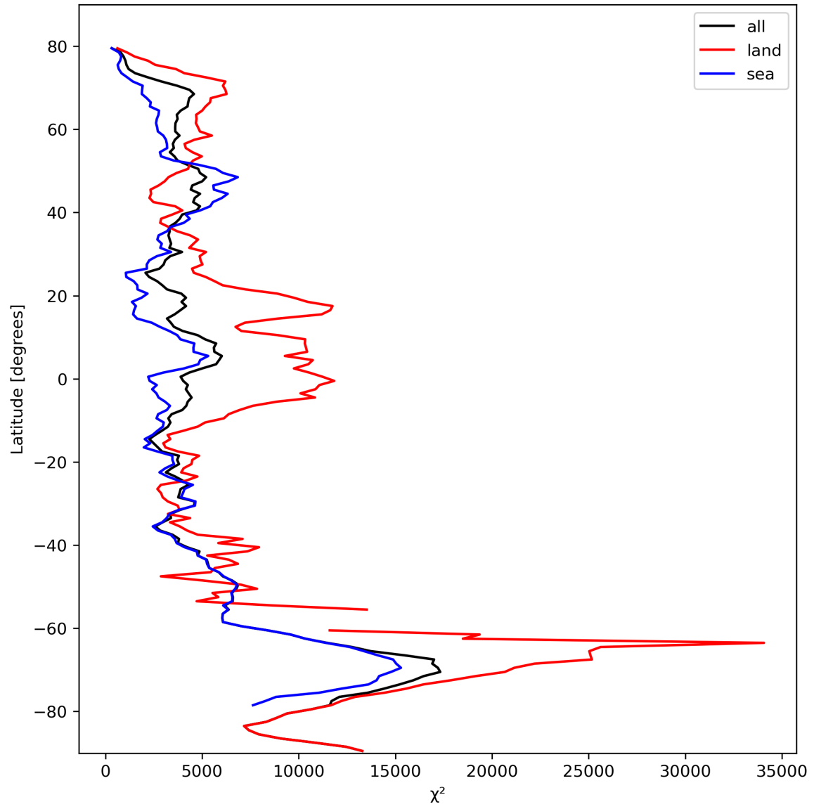
Figure 21: Zonal average of “ \chi^2 ” for 2023-10-15 to 2023-10-17.
