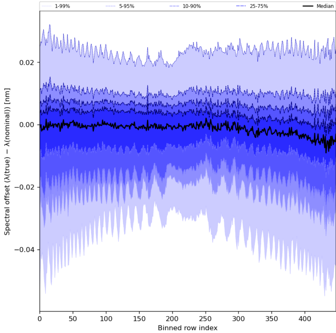
Figure 62: Along track statistics of “Spectral offset ( \lambda(\text{true}) - \lambda(\text{nominal}) )” for 2023-10-15 to 2023-10-17
