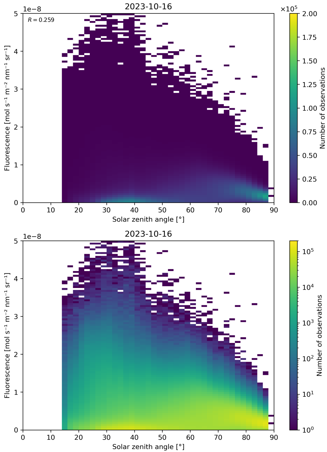
Figure 123: Scatter density plot of “Solar zenith angle” against “Fluorescence” for 2023-10-15 to 2023-10-17.
