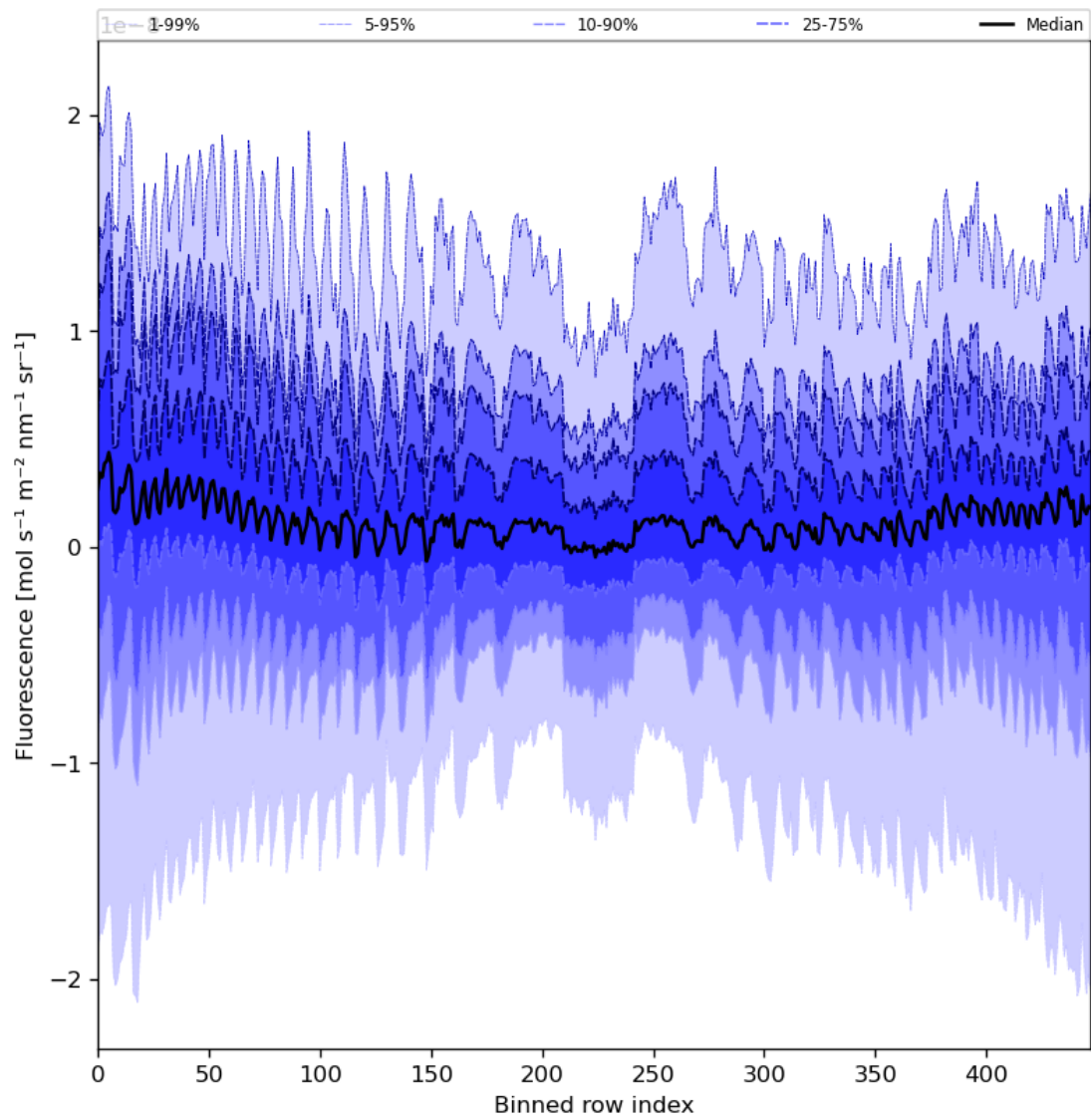
Figure 57: Along track statistics of “Fluorescence” for 2023-10-15 to 2023-10-17
