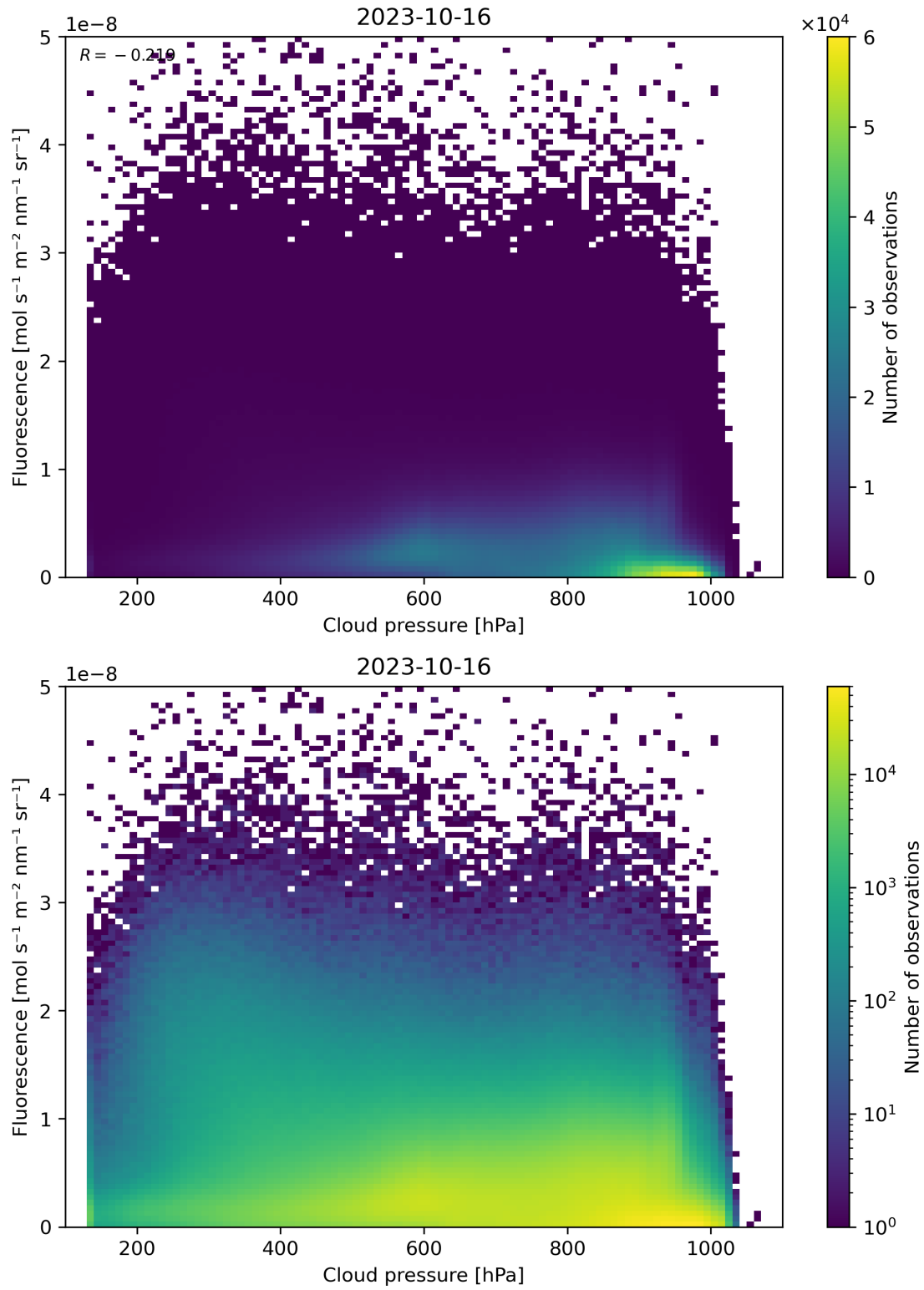
Figure 88: Scatter density plot of “Cloud pressure” against “Fluorescence” for 2023-10-15 to 2023-10-17.
