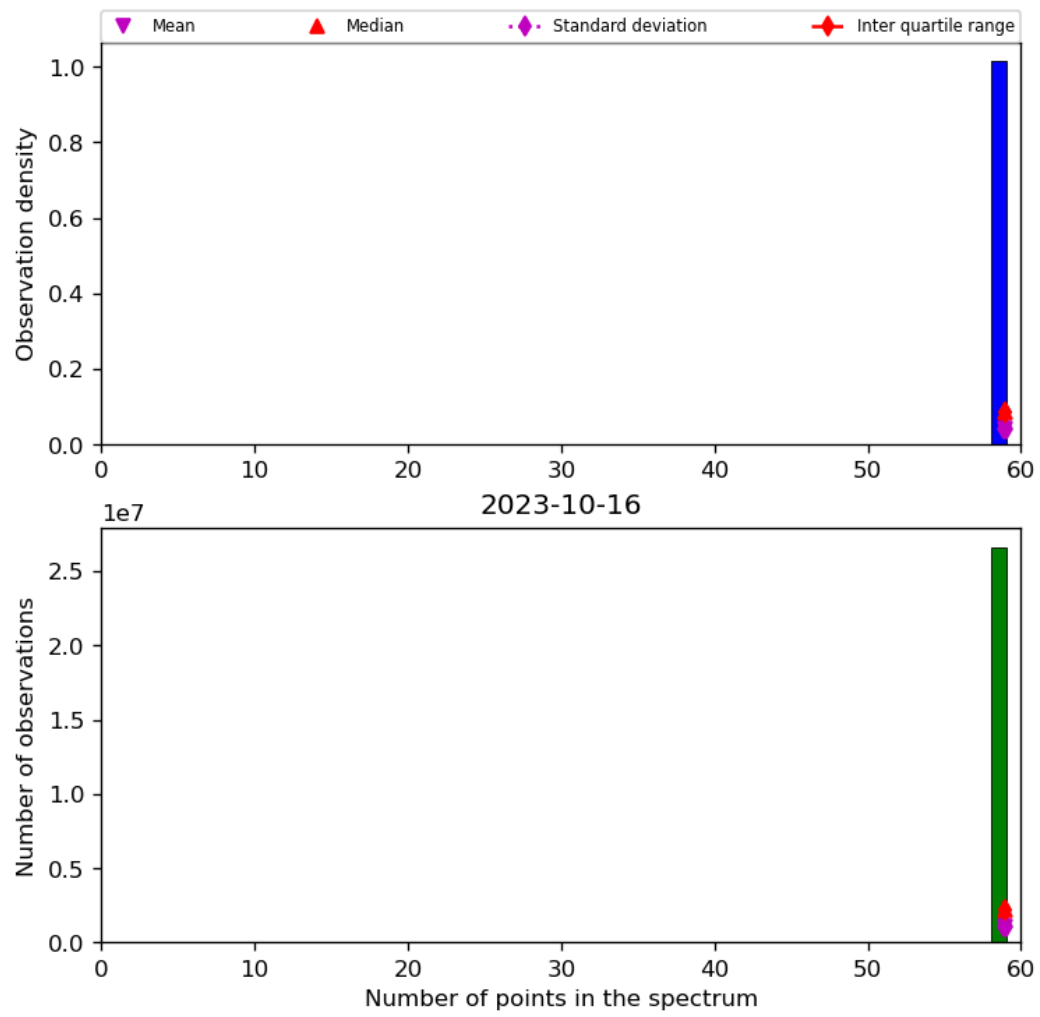
Figure 44: Histogram of “Number of points in the spectrum” for 2023-10-15 to 2023-10-17
