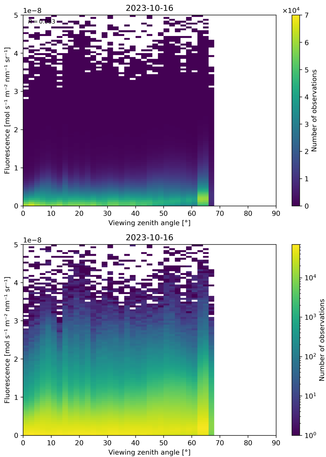
Figure 134: Scatter density plot of “Viewing zenith angle” against “Fluorescence” for 2023-10-15 to 2023-10-17.
