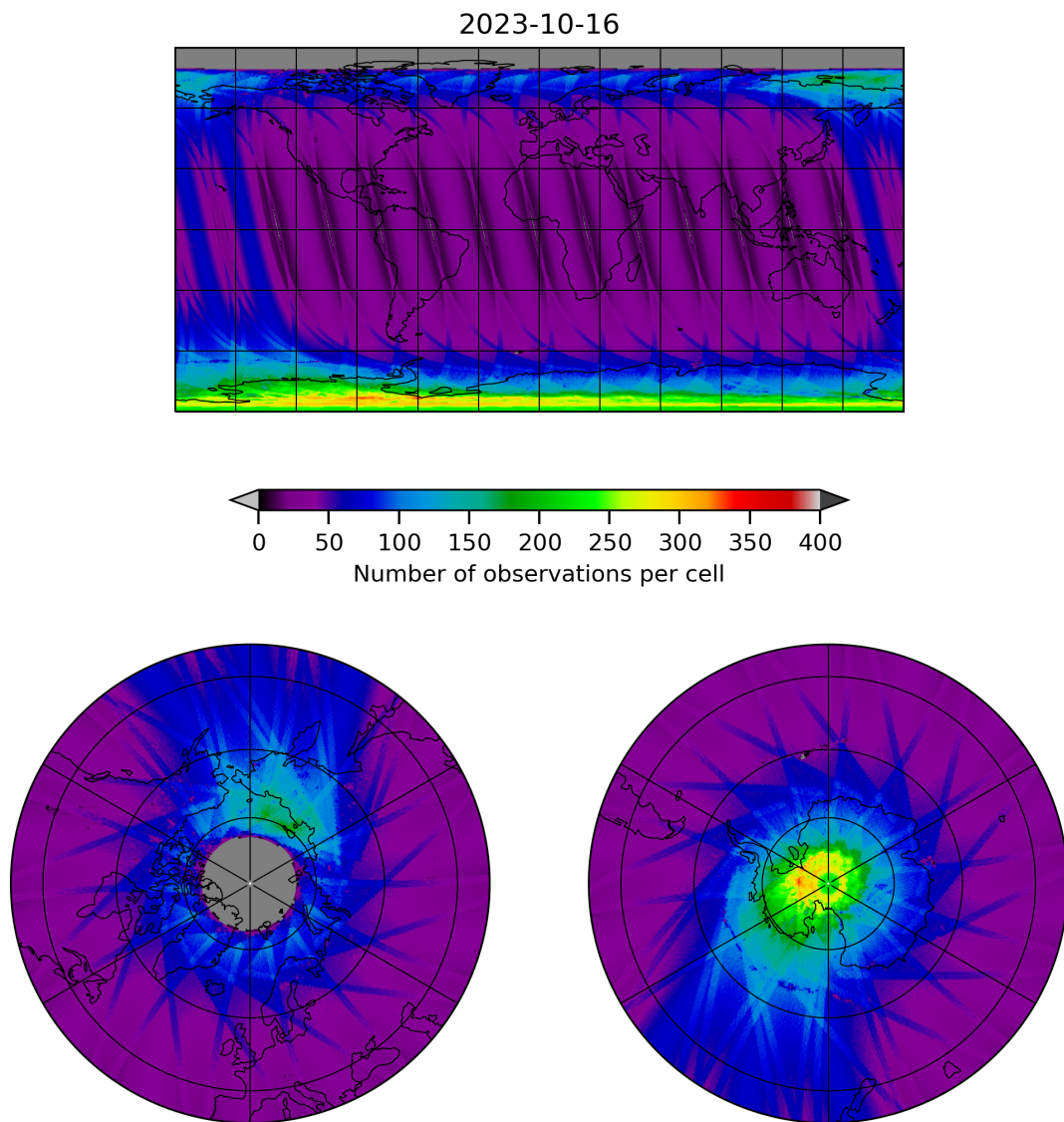
Figure 11: Map of the number of observations for 2023-10-15 to 2023-10-17
