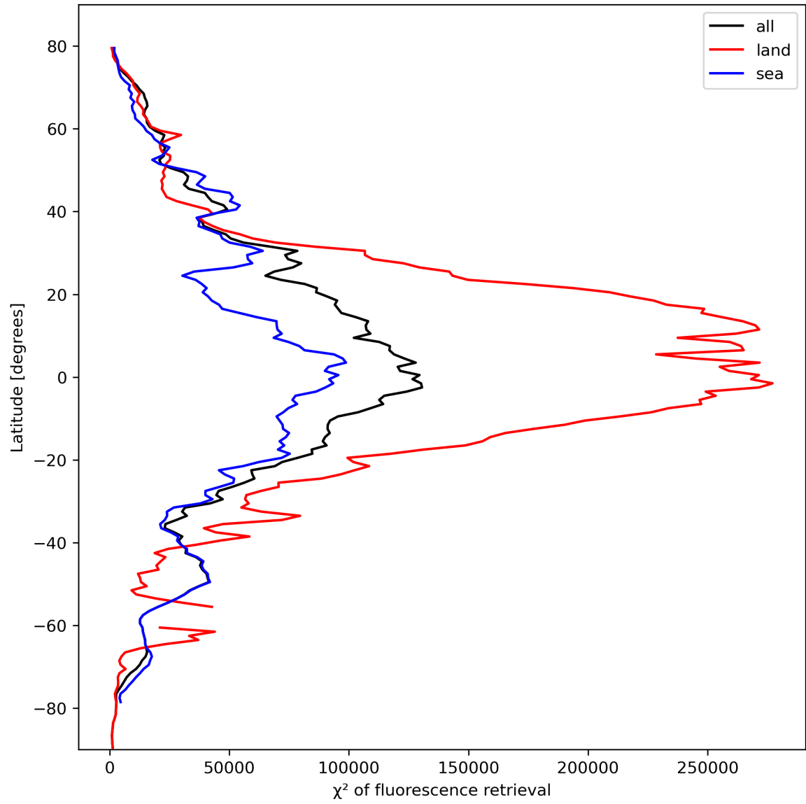
Figure 25: Zonal average of “ \chi^2 of fluorescence retrieval” for 2023-10-15 to 2023-10-17.
