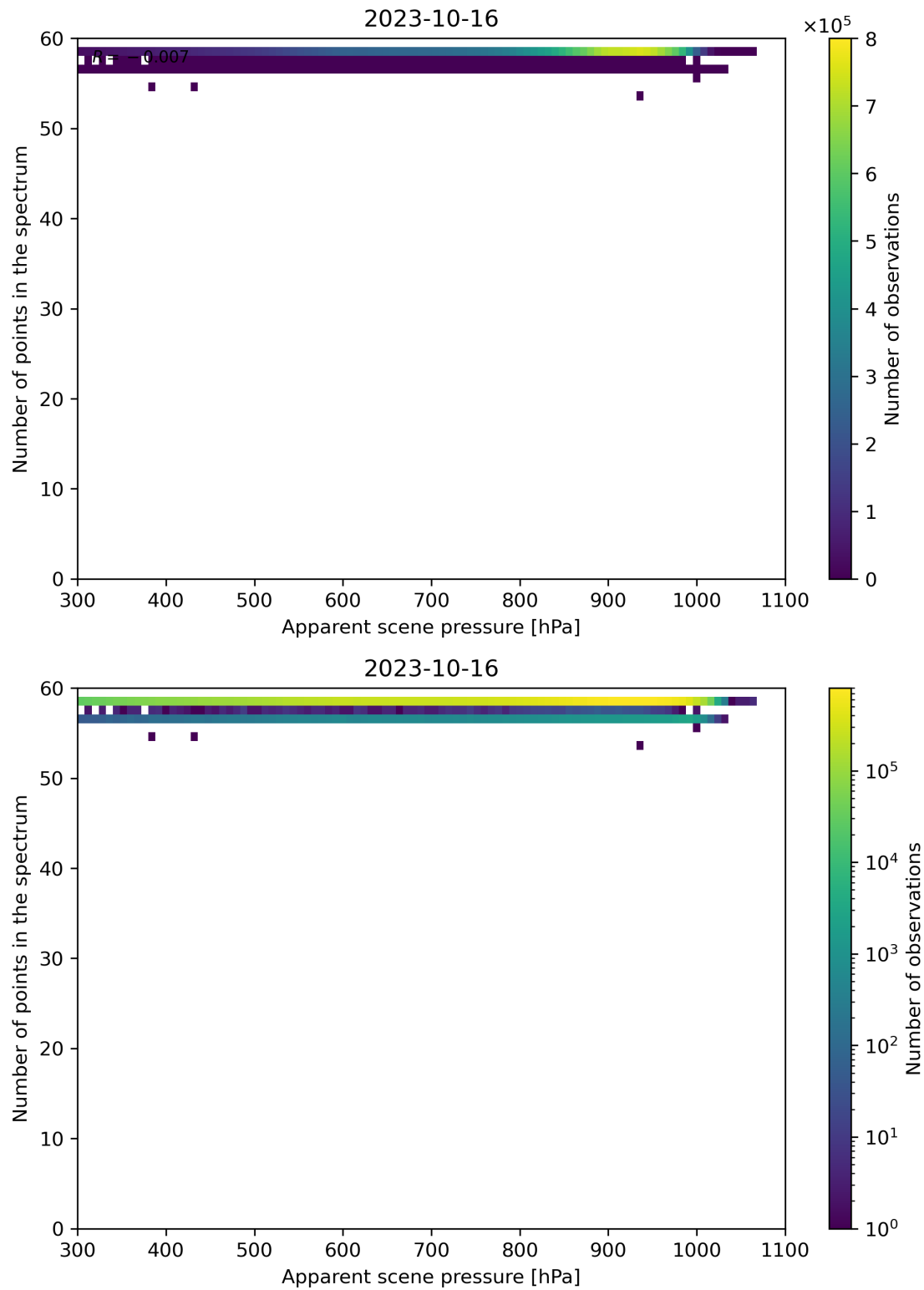
Figure 67: Scatter density plot of “Apparent scene pressure” against “Number of points in the spectrum” for 2023-10-15 to 2023-10-17.
