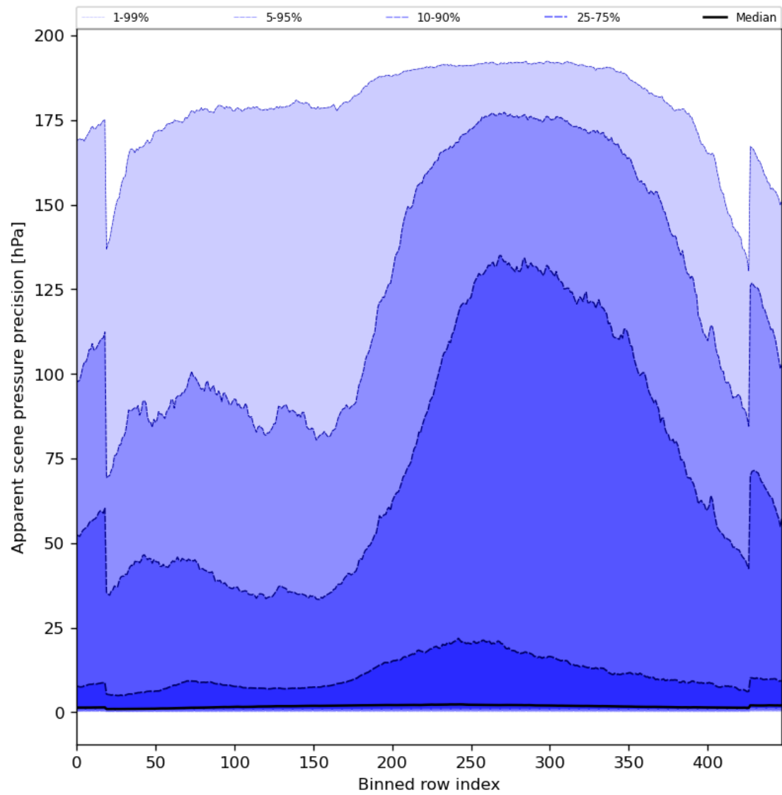
Figure 54: Along track statistics of “Apparent scene pressure precision” for 2023-10-15 to 2023-10-17
