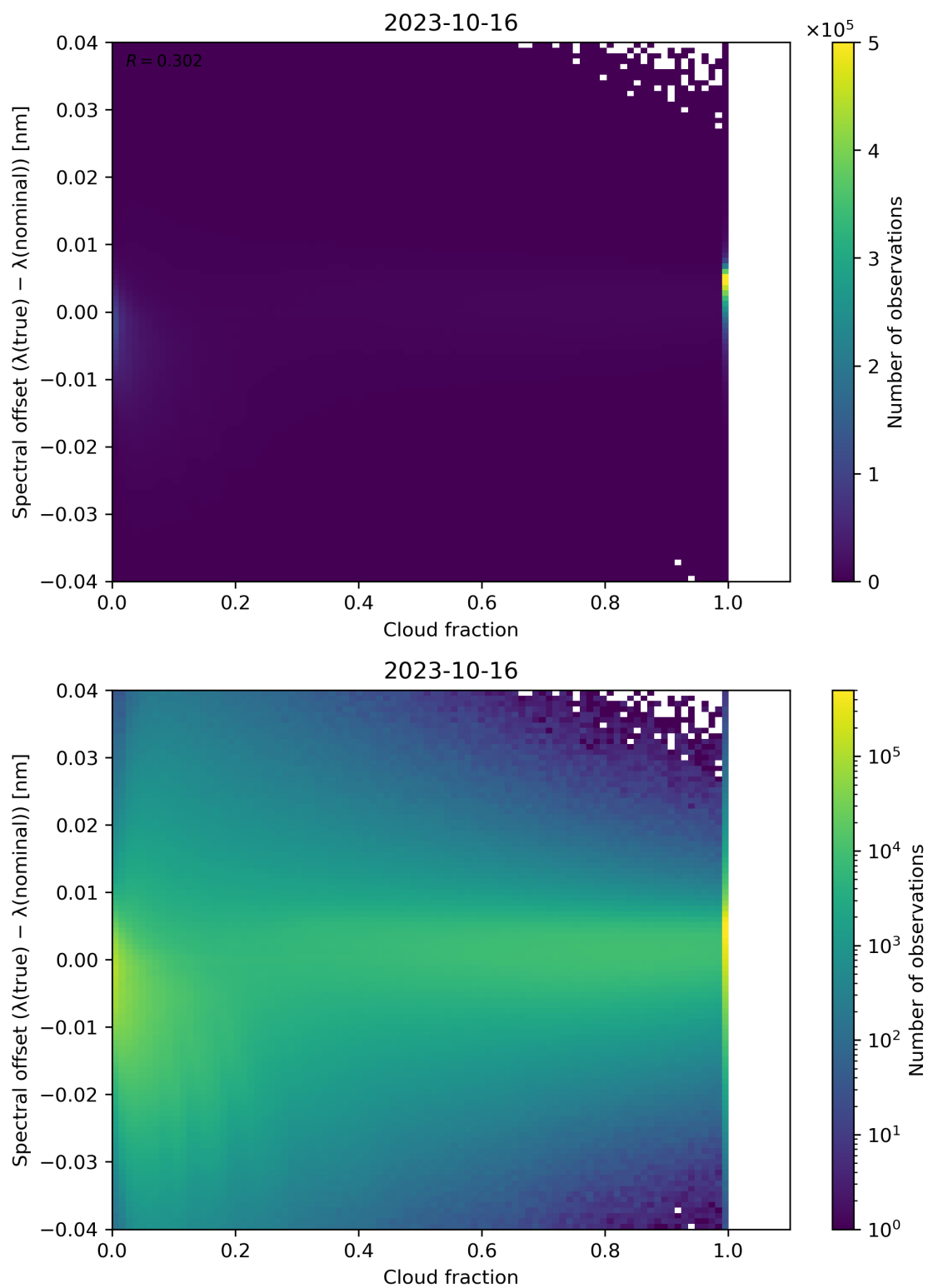
Figure 83: Scatter density plot of “Cloud fraction” against “Spectral offset ( \lambda(\text{true}) - \lambda(\text{nominal}) )” for 2023-10-15 to 2023-10-17.
