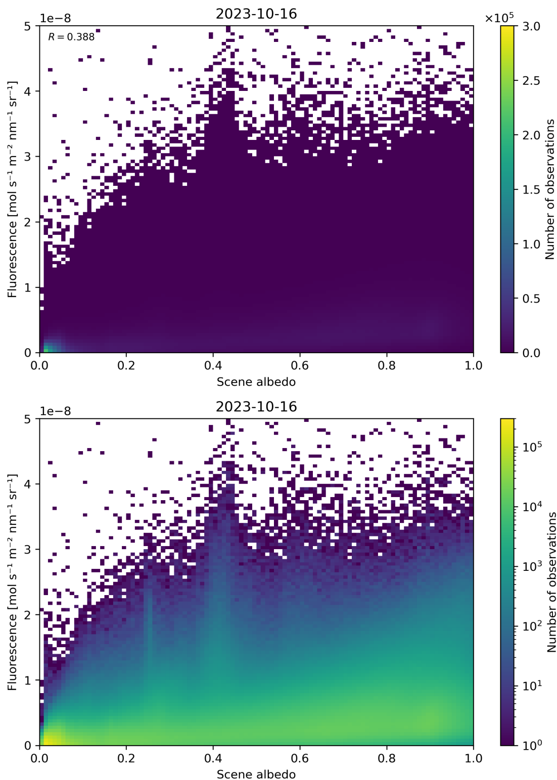
Figure 114: Scatter density plot of “Scene albedo” against “Fluorescence” for 2023-10-15 to 2023-10-17.
