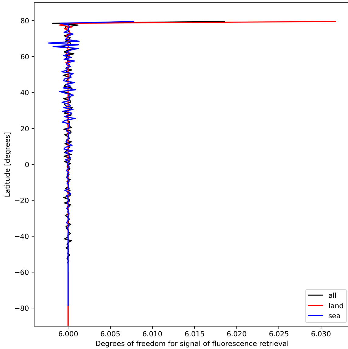
Figure 26: Zonal average of “Degrees of freedom for signal of fluorescence retrieval” for 2023-10-15 to 2023-10-17.
