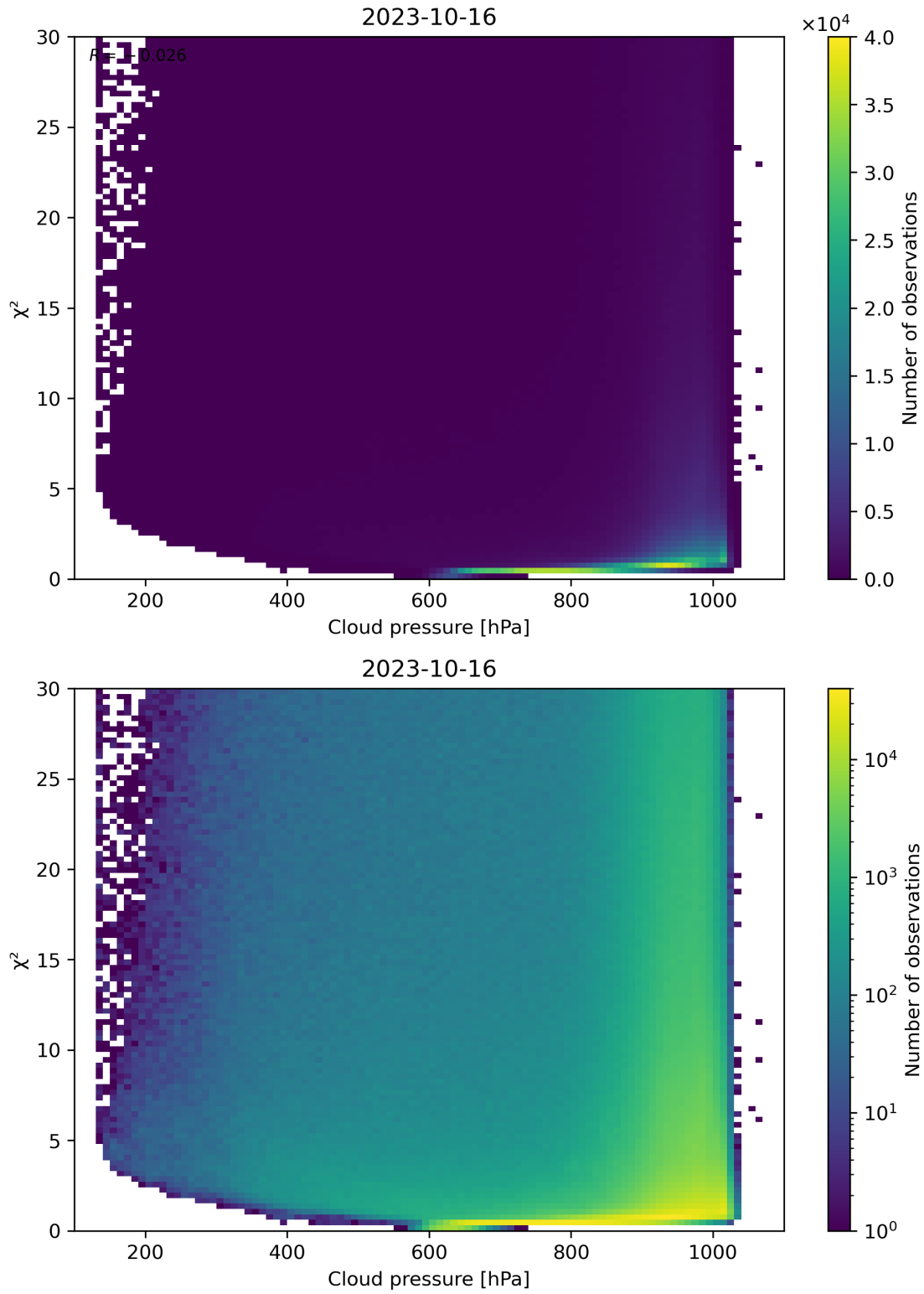
Figure 85: Scatter density plot of “Cloud pressure” against “ \chi^2 ” for 2023-10-15 to 2023-10-17.
