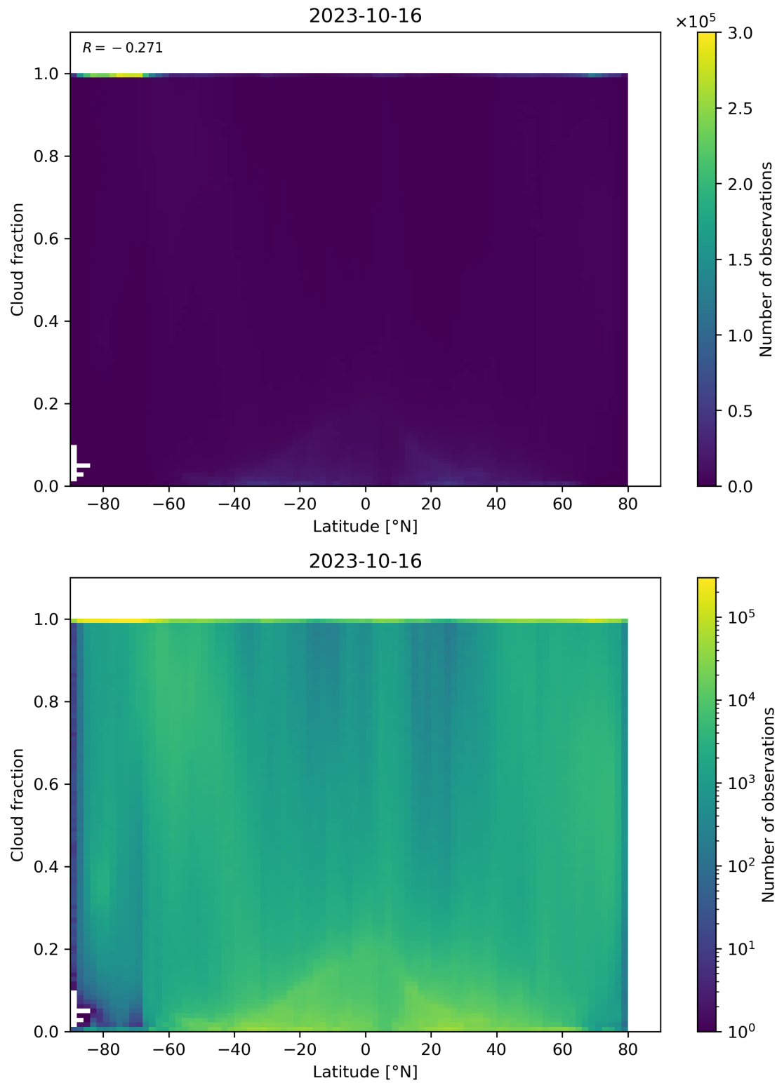
Figure 99: Scatter density plot of “Latitude” against “Cloud fraction” for 2023-10-15 to 2023-10-17.
