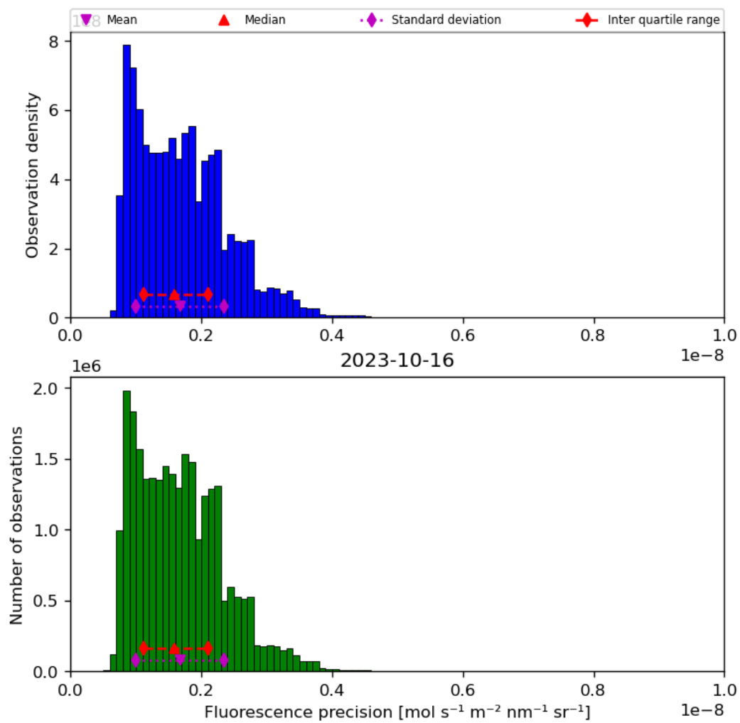
Figure 41: Histogram of “Fluorescence precision” for 2023-10-15 to 2023-10-17
