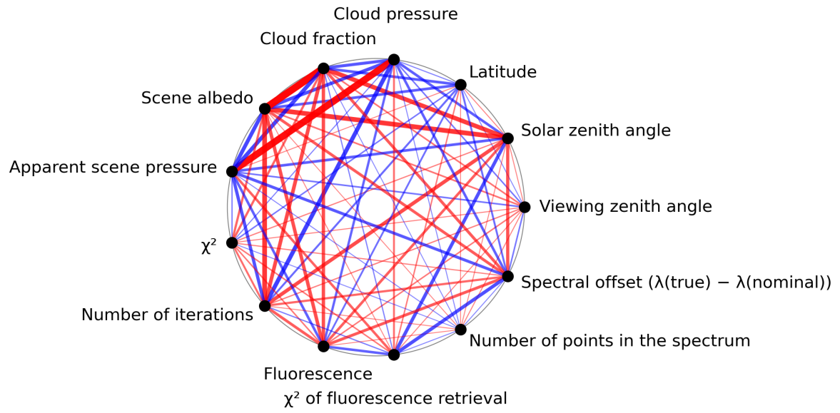
Figure 1: Map of correlation graph for 2023-10-15 to 2023-10-17.
