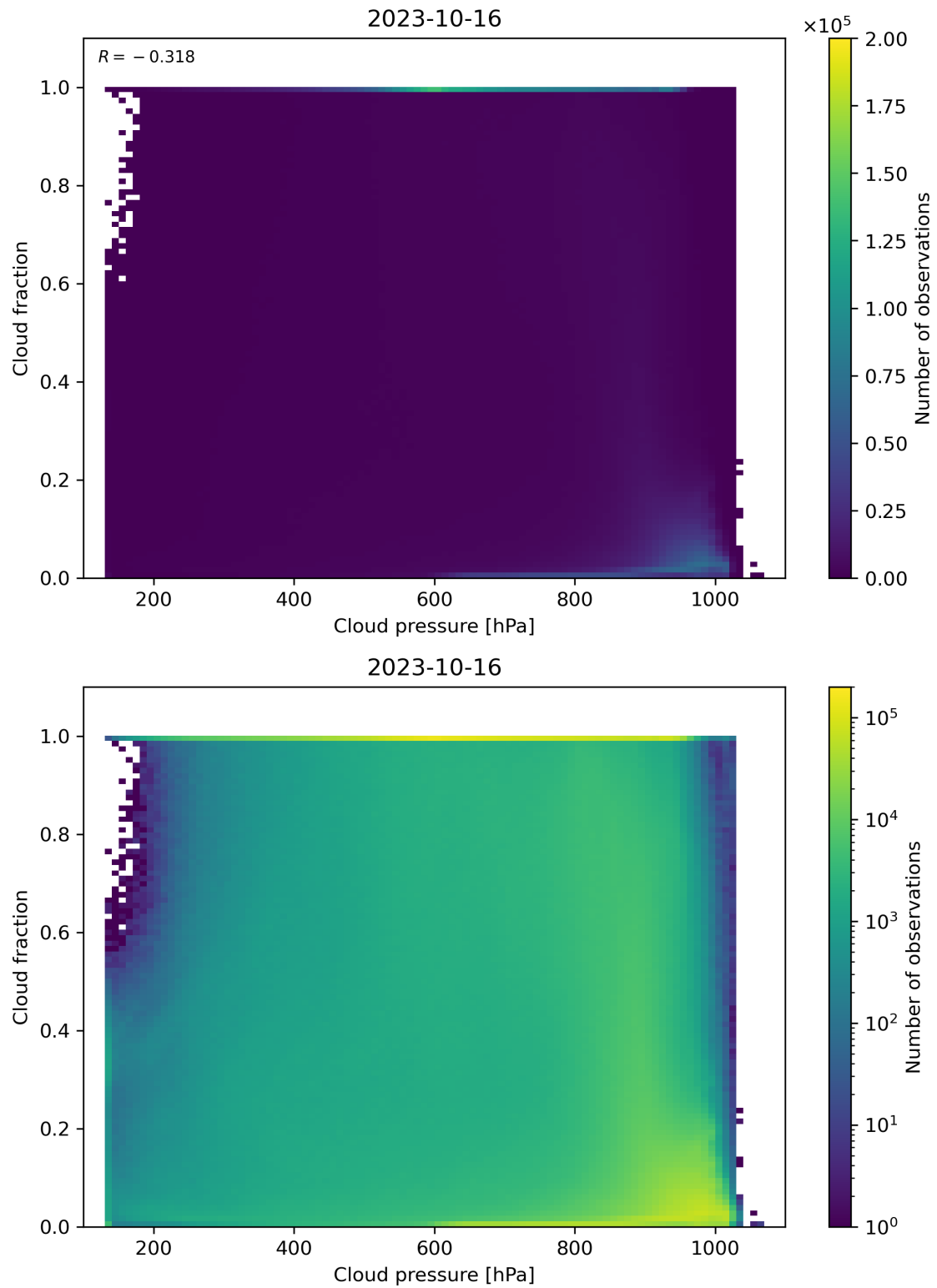
Figure 87: Scatter density plot of “Cloud pressure” against “Cloud fraction” for 2023-10-15 to 2023-10-17.
