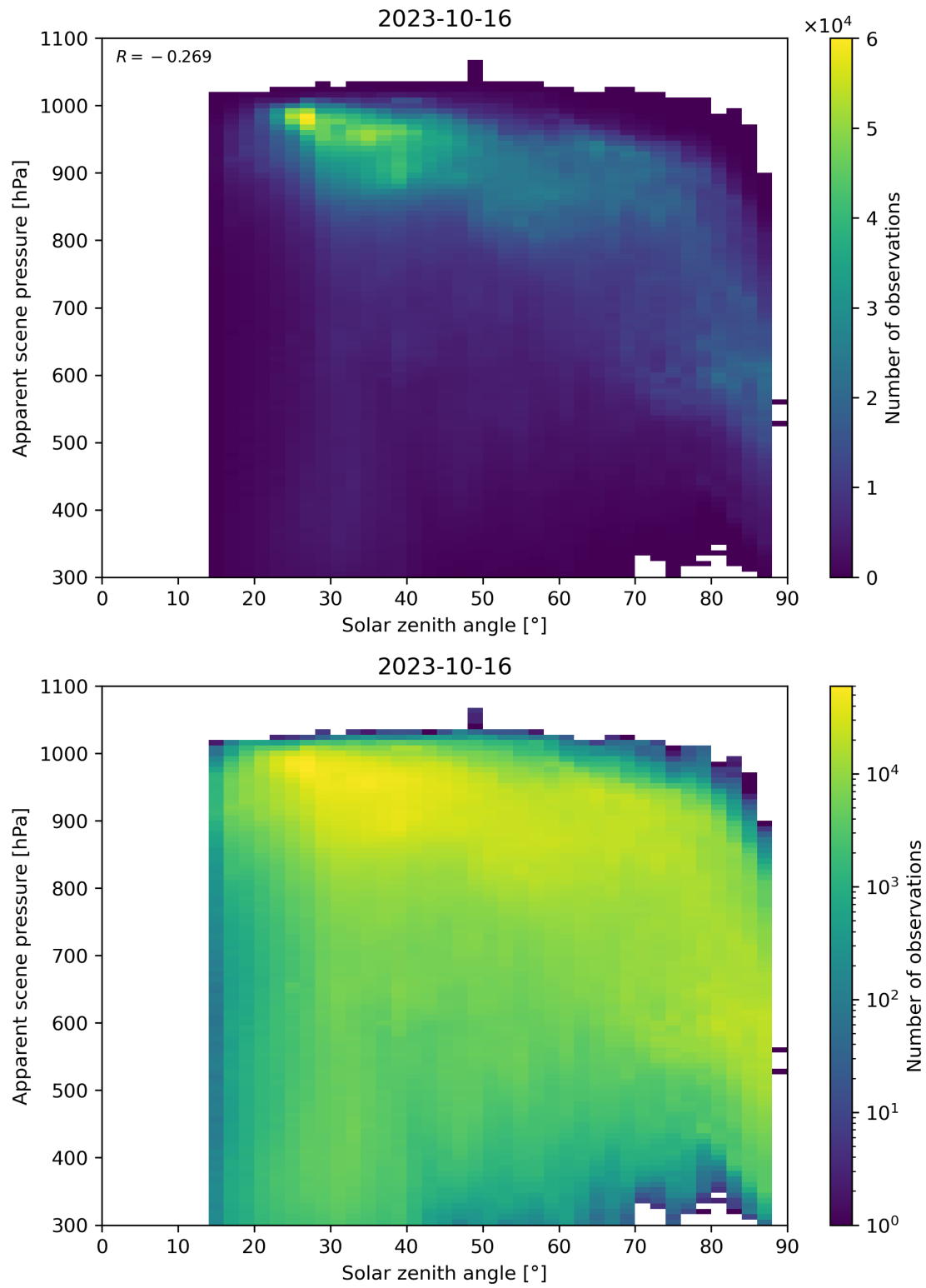
Figure 118: Scatter density plot of “Solar zenith angle” against “Apparent scene pressure” for 2023-10-15 to 2023-10-17.
