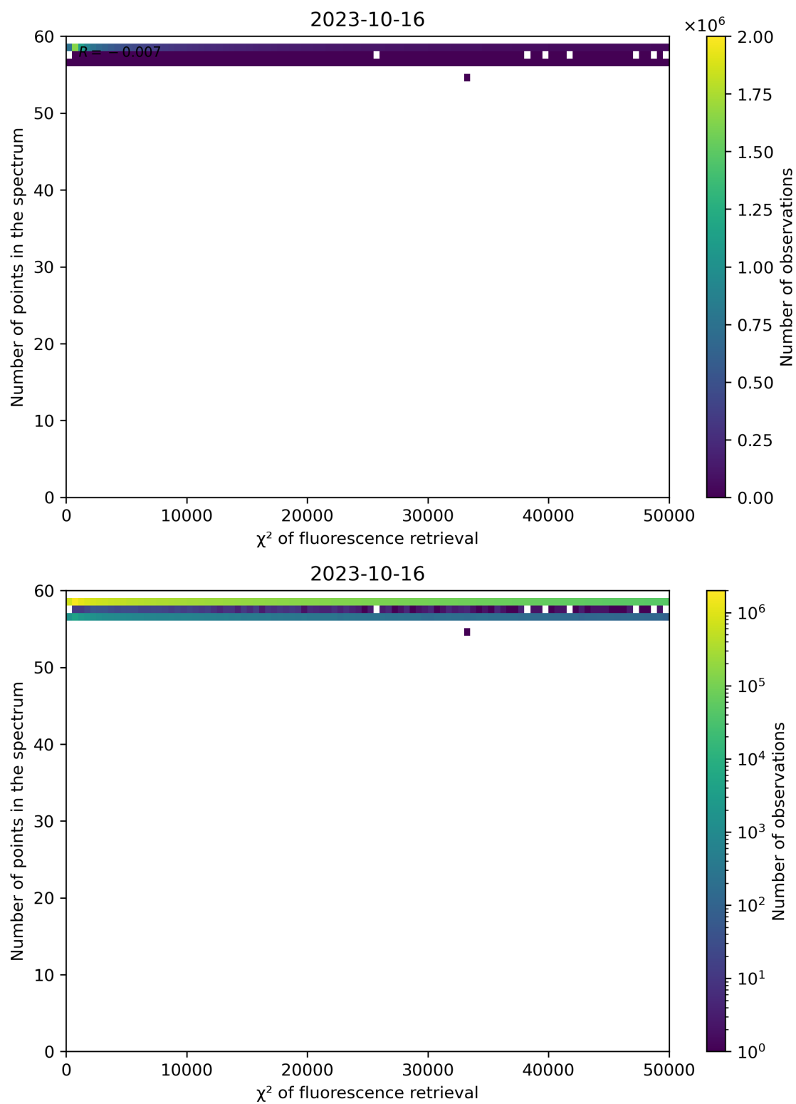
Figure 71: Scatter density plot of “ \chi^2 of fluorescence retrieval” against “Number of points in the spectrum” for 2023-10-15 to 2023-10-17.
