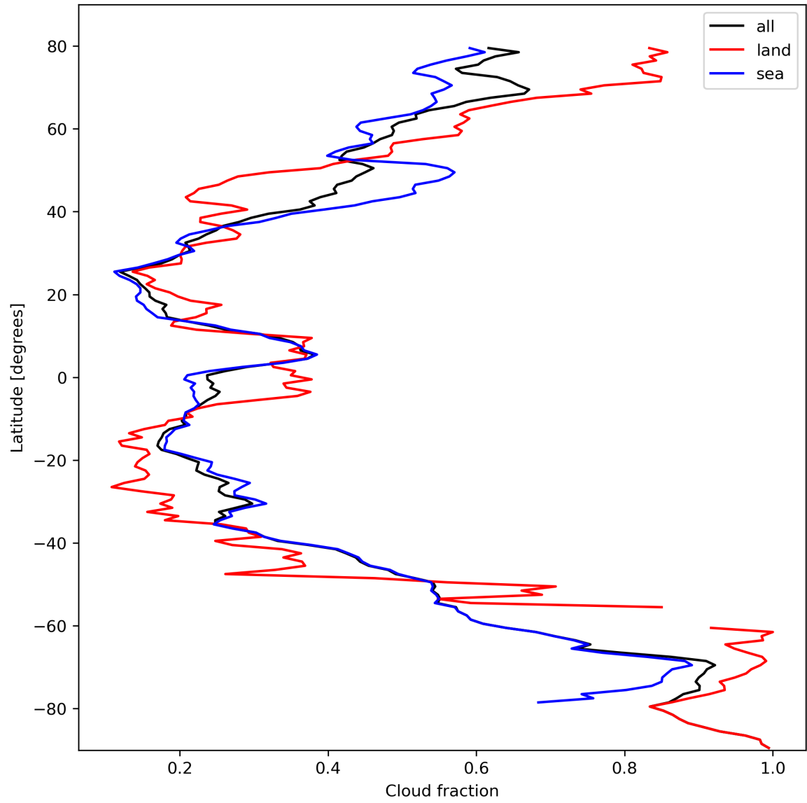
Figure 15: Zonal average of “Cloud fraction” for 2023-10-15 to 2023-10-17.
