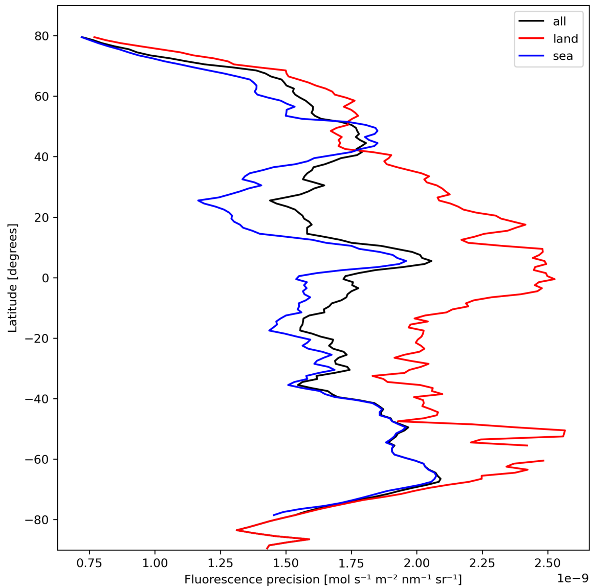
Figure 24: Zonal average of “Fluorescence precision” for 2023-10-15 to 2023-10-17.
