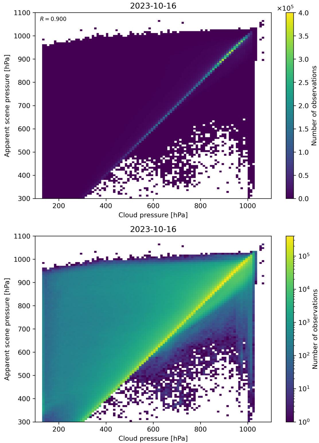
Figure 84: Scatter density plot of “Cloud pressure” against “Apparent scene pressure” for 2023-10-15 to 2023-10-17.
