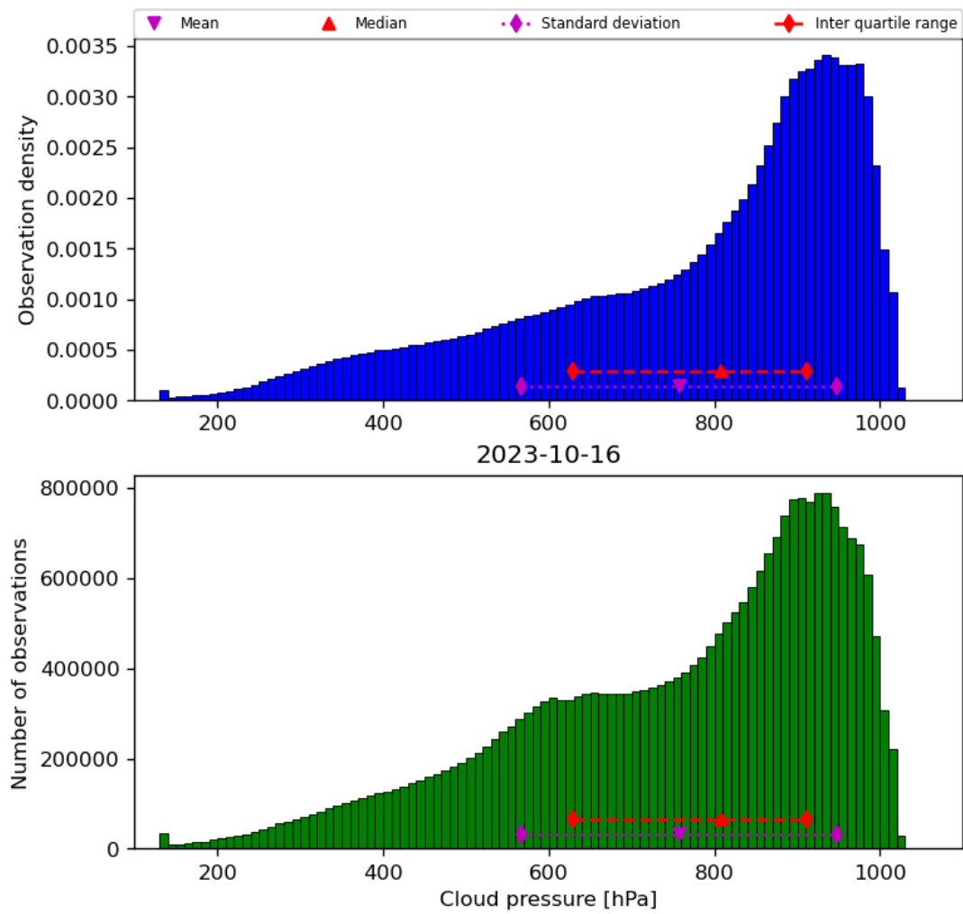
Figure 30: Histogram of “Cloud pressure” for 2023-10-15 to 2023-10-17
