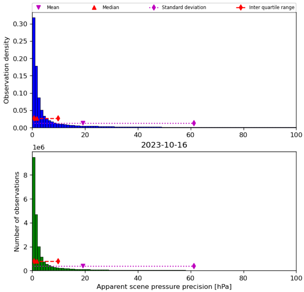
Figure 37: Histogram of “Apparent scene pressure precision” for 2023-10-15 to 2023-10-17
