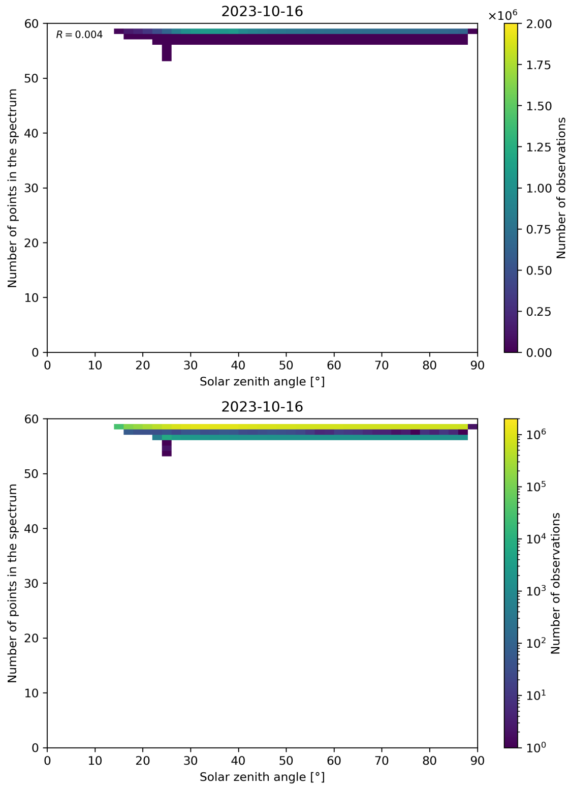
Figure 126: Scatter density plot of “Solar zenith angle” against “Number of points in the spectrum” for 2023-10-15 to 2023-10-17.
