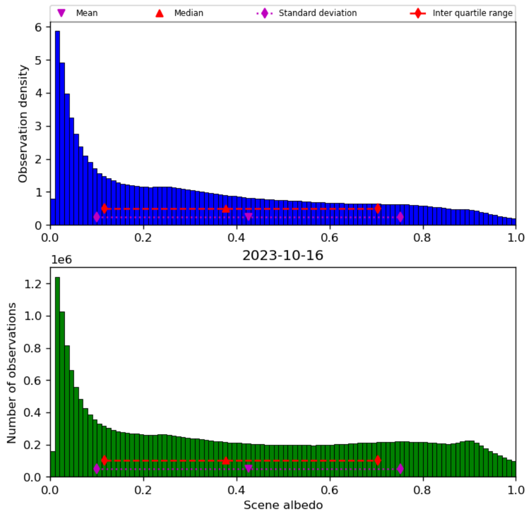
Figure 34: Histogram of “Scene albedo” for 2023-10-15 to 2023-10-17
