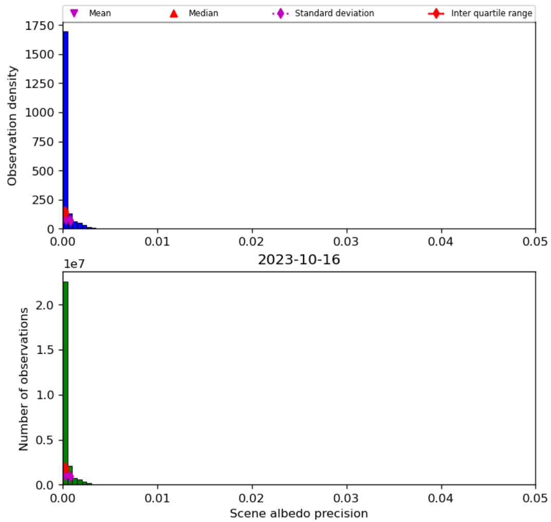
Figure 35: Histogram of “Scene albedo precision” for 2023-10-15 to 2023-10-17
