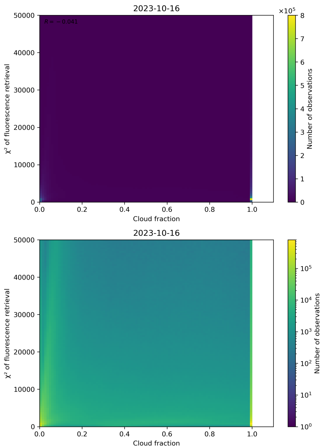
Figure 78: Scatter density plot of “Cloud fraction” against “ \chi^2 of fluorescence retrieval” for 2023-10-15 to 2023-10-17.
