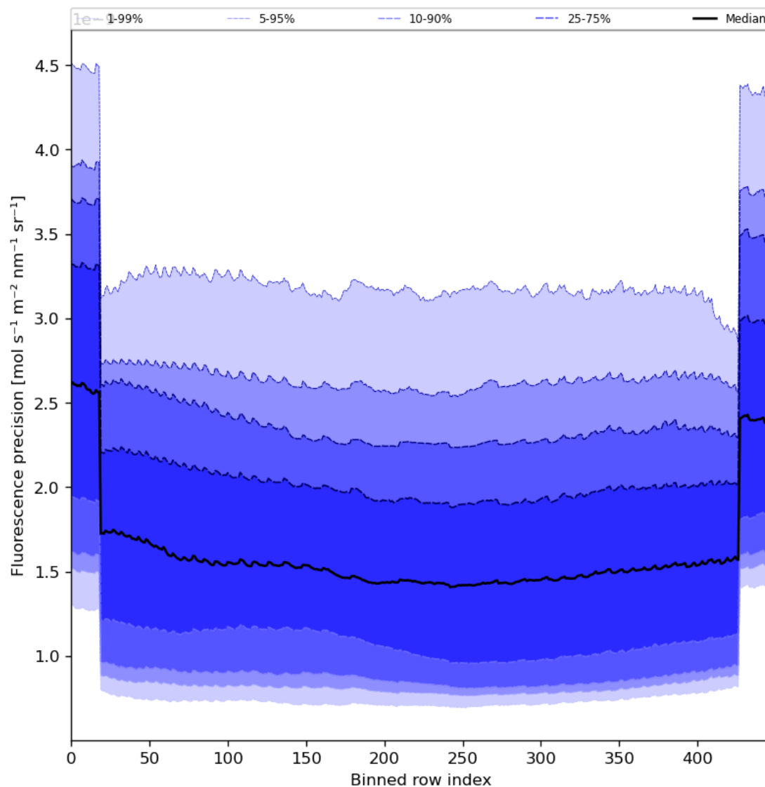
Figure 58: Along track statistics of “Fluorescence precision” for 2023-10-15 to 2023-10-17
