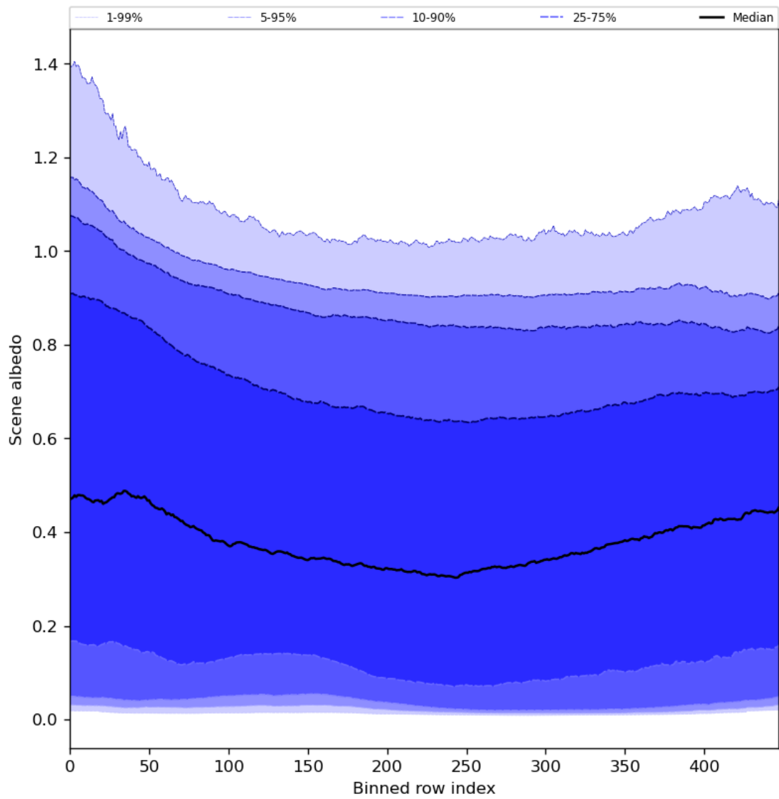
Figure 51: Along track statistics of “Scene albedo” for 2023-10-15 to 2023-10-17
