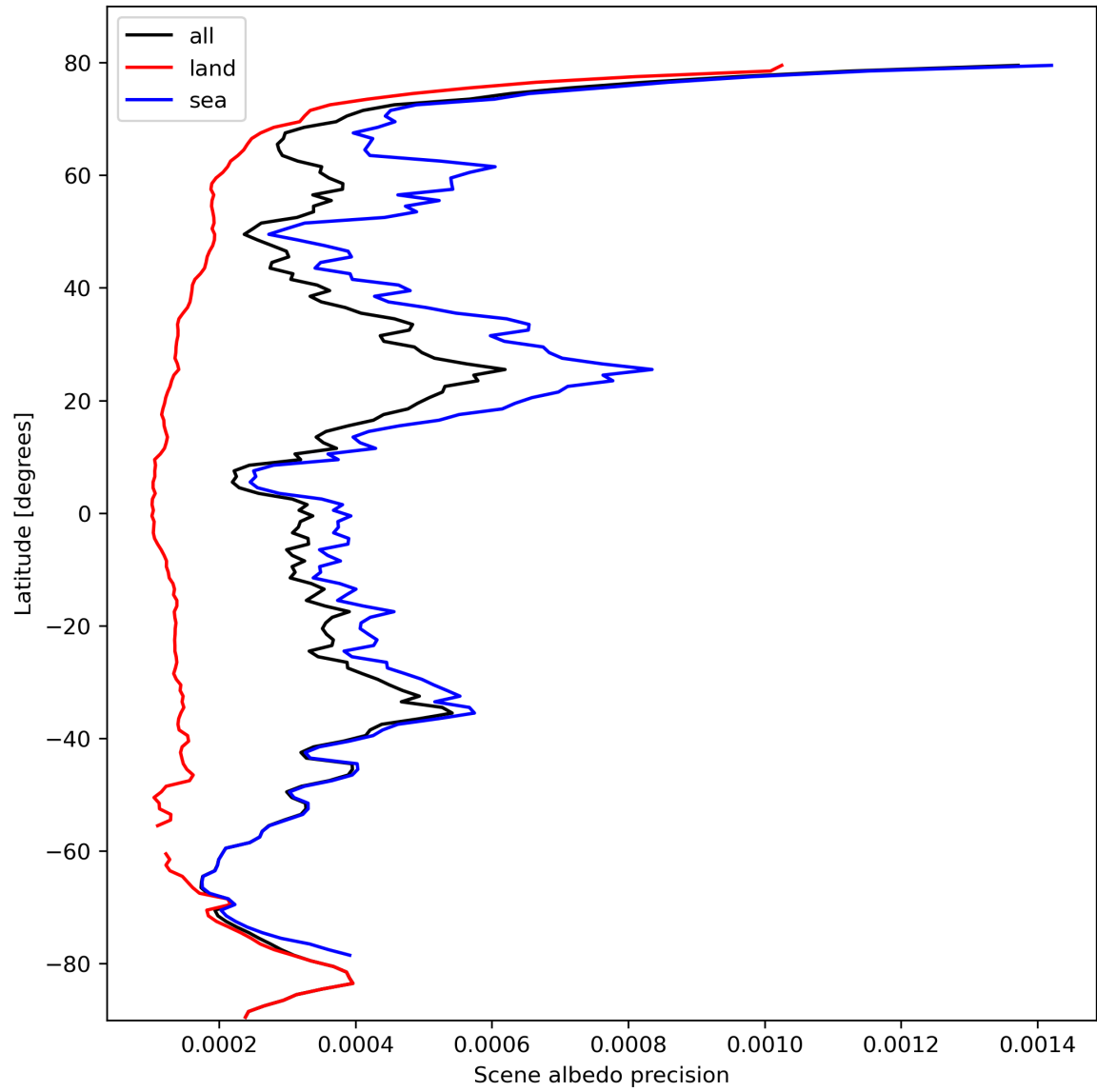
Figure 18: Zonal average of “Scene albedo precision” for 2023-10-15 to 2023-10-17.
