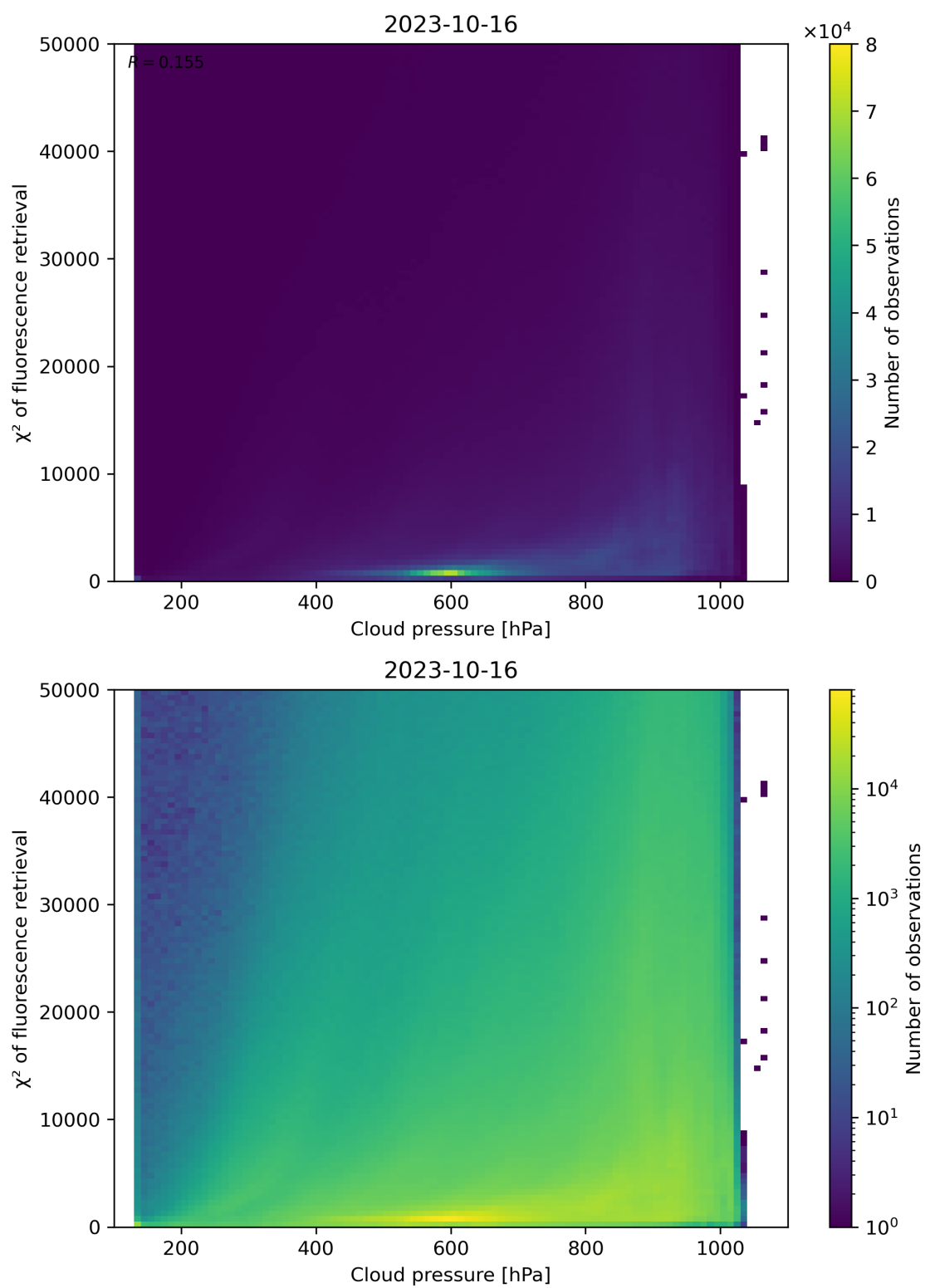
Figure 86: Scatter density plot of “Cloud pressure” against “ \chi^2 of fluorescence retrieval” for 2023-10-15 to 2023-10-17.
