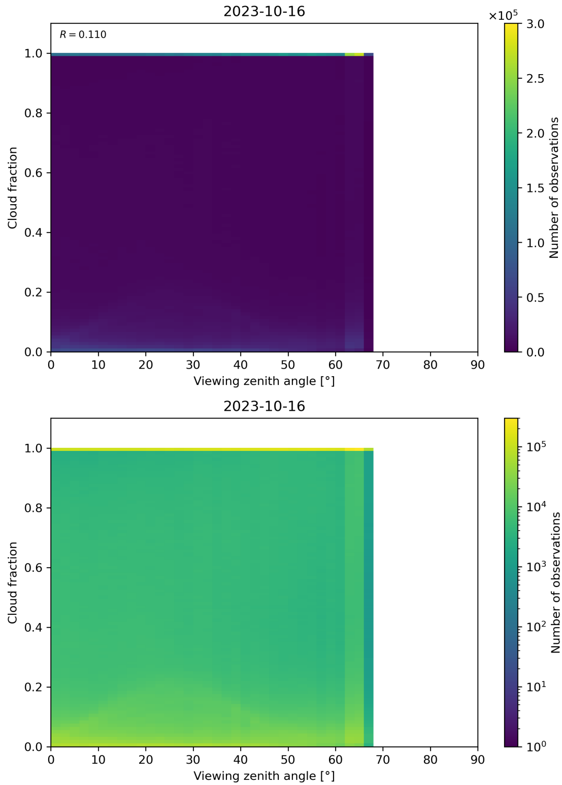
Figure 132: Scatter density plot of “Viewing zenith angle” against “Cloud fraction” for 2023-10-15 to 2023-10-17.
