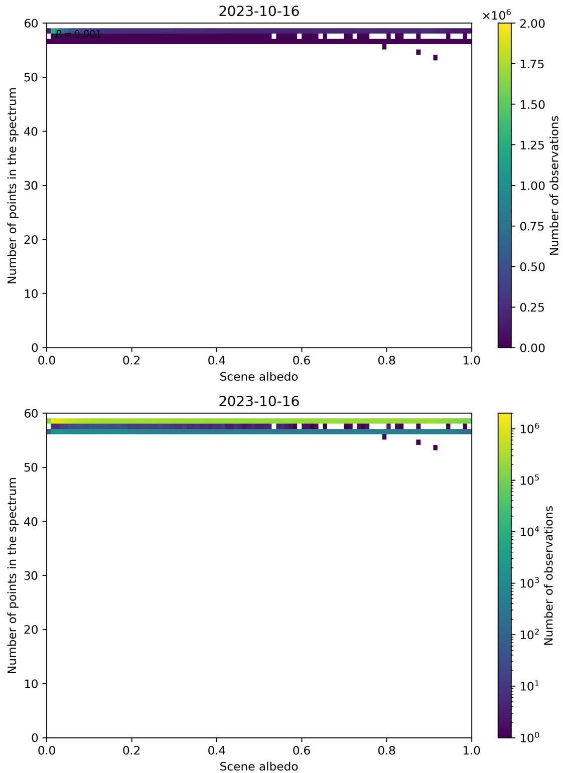
Figure 116: Scatter density plot of “Scene albedo” against “Number of points in the spectrum” for 2023-10-15 to 2023-10-17.
