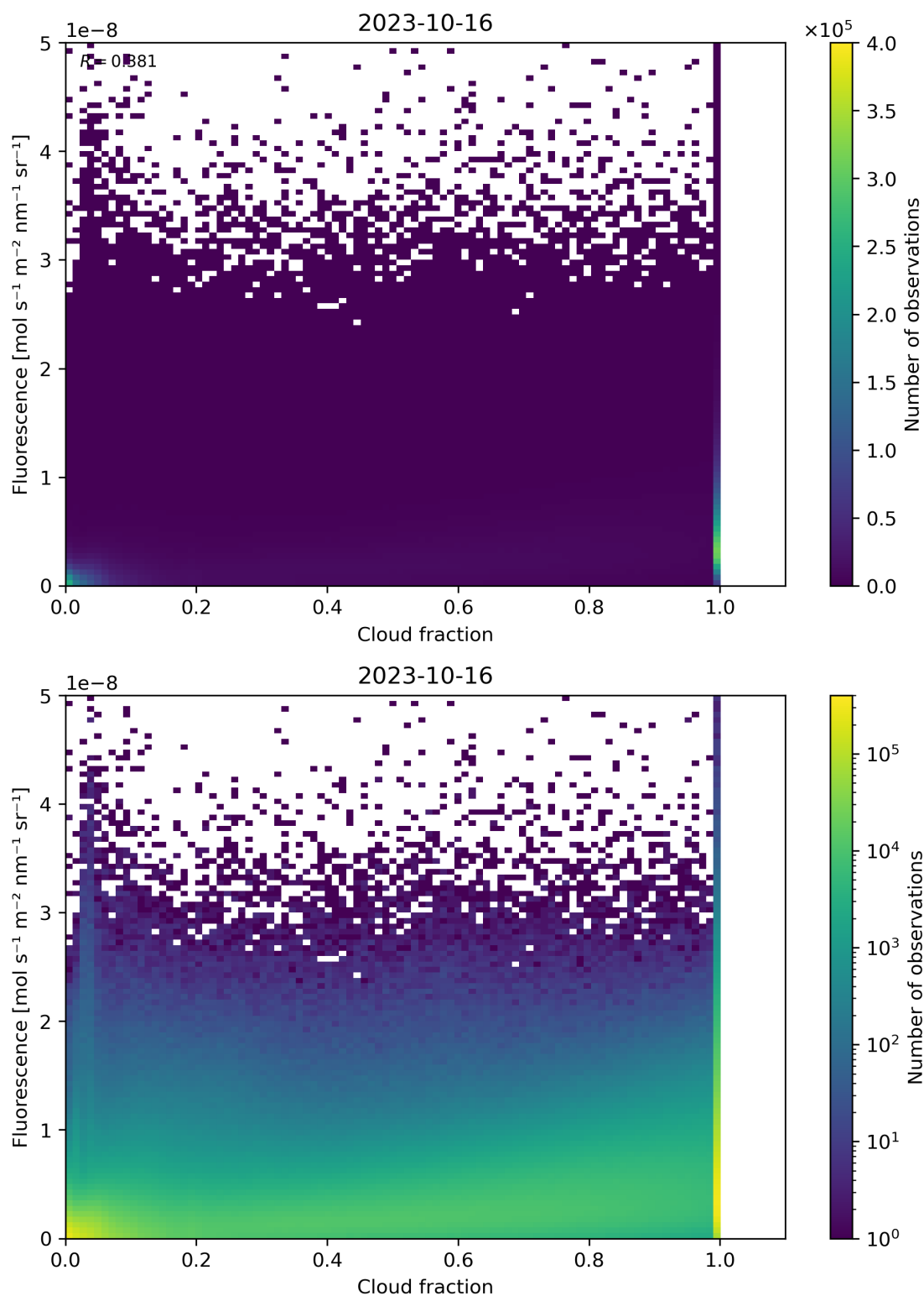
Figure 79: Scatter density plot of “Cloud fraction” against “Fluorescence” for 2023-10-15 to 2023-10-17.
