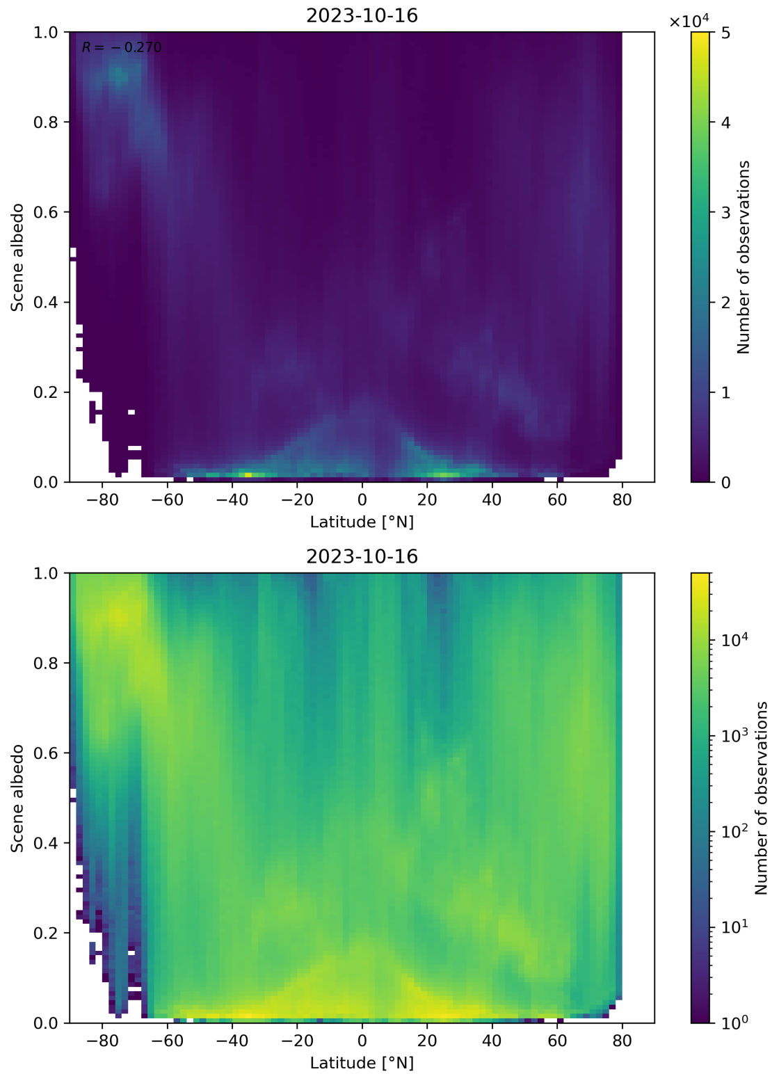
Figure 104: Scatter density plot of “Latitude” against “Scene albedo” for 2023-10-15 to 2023-10-17.
