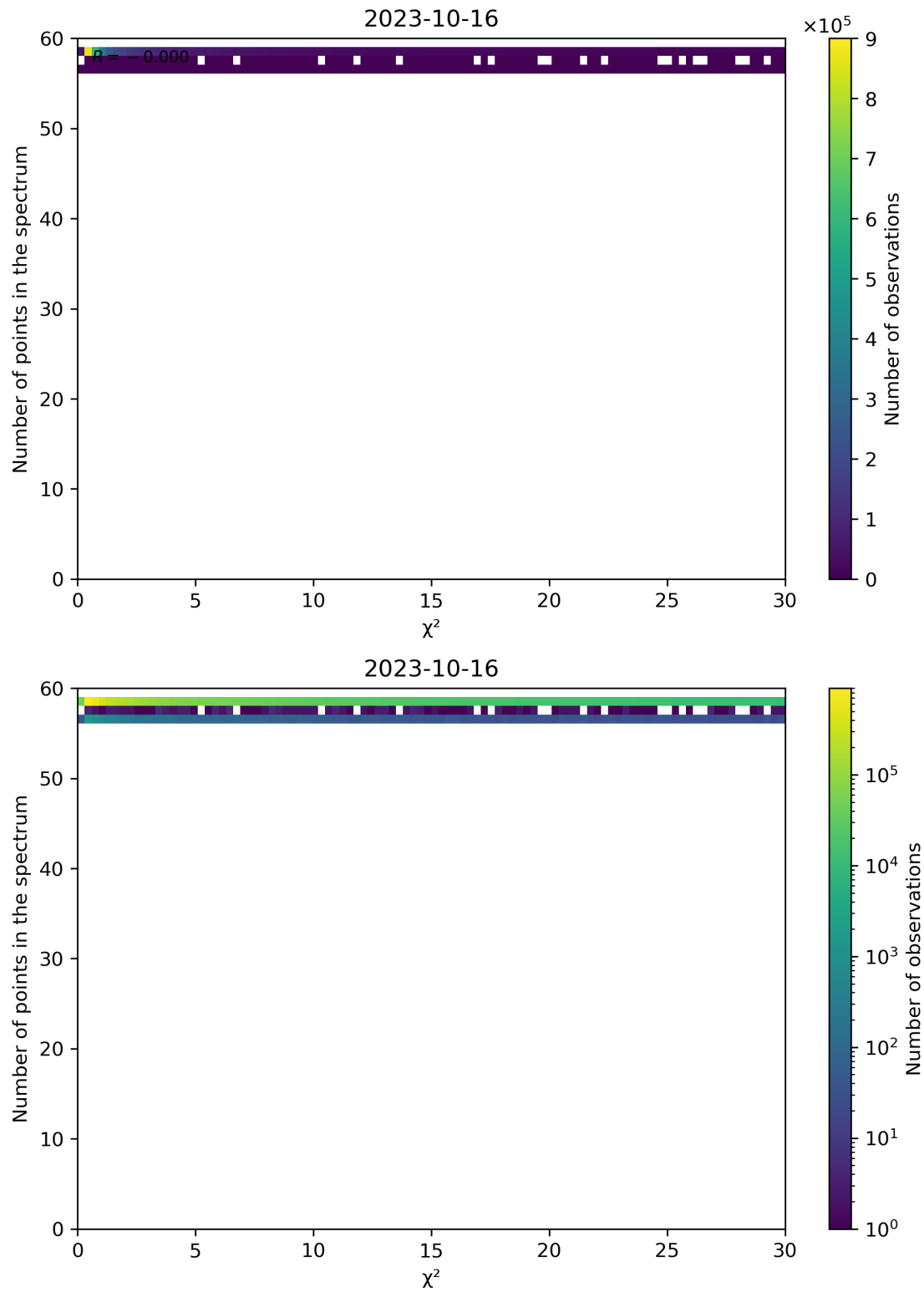
Figure 74: Scatter density plot of " \chi^2 " against "Number of points in the spectrum" for 2023-10-15 to 2023-10-17.
