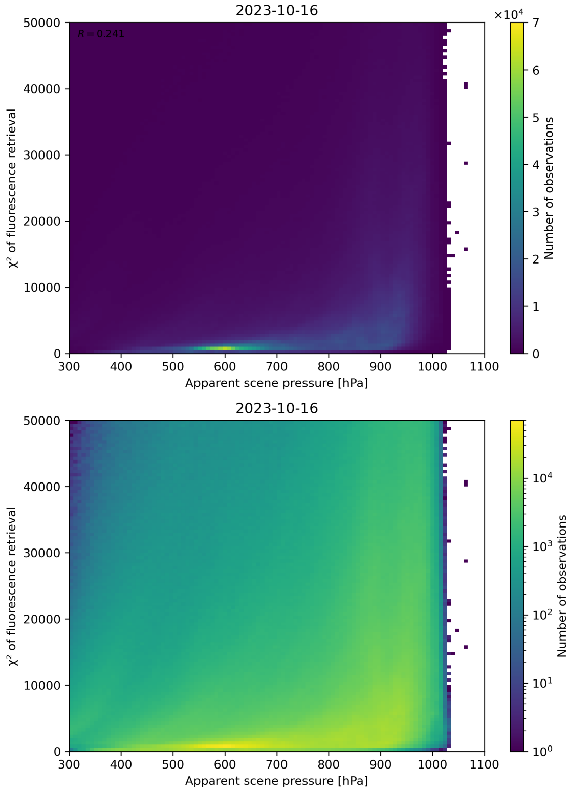
Figure 64: Scatter density plot of “Apparent scene pressure” against “ \chi^2 of fluorescence retrieval” for 2023-10-15 to 2023-10-17.
