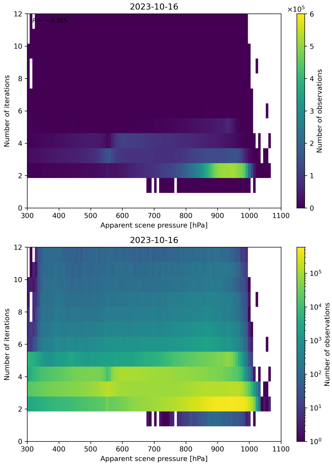
Figure 66: Scatter density plot of “Apparent scene pressure” against “Number of iterations” for 2023-10-15 to 2023-10-17.
