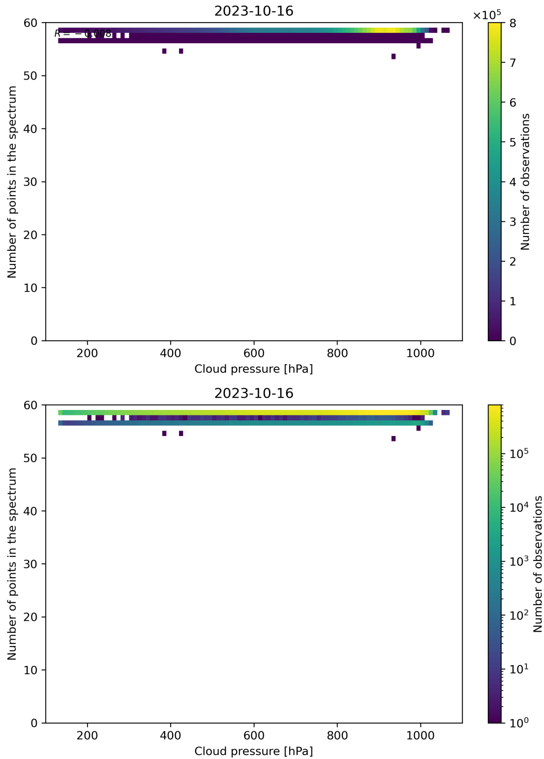
Figure 90: Scatter density plot of “Cloud pressure” against “Number of points in the spectrum” for 2023-10-15 to 2023-10-17.
