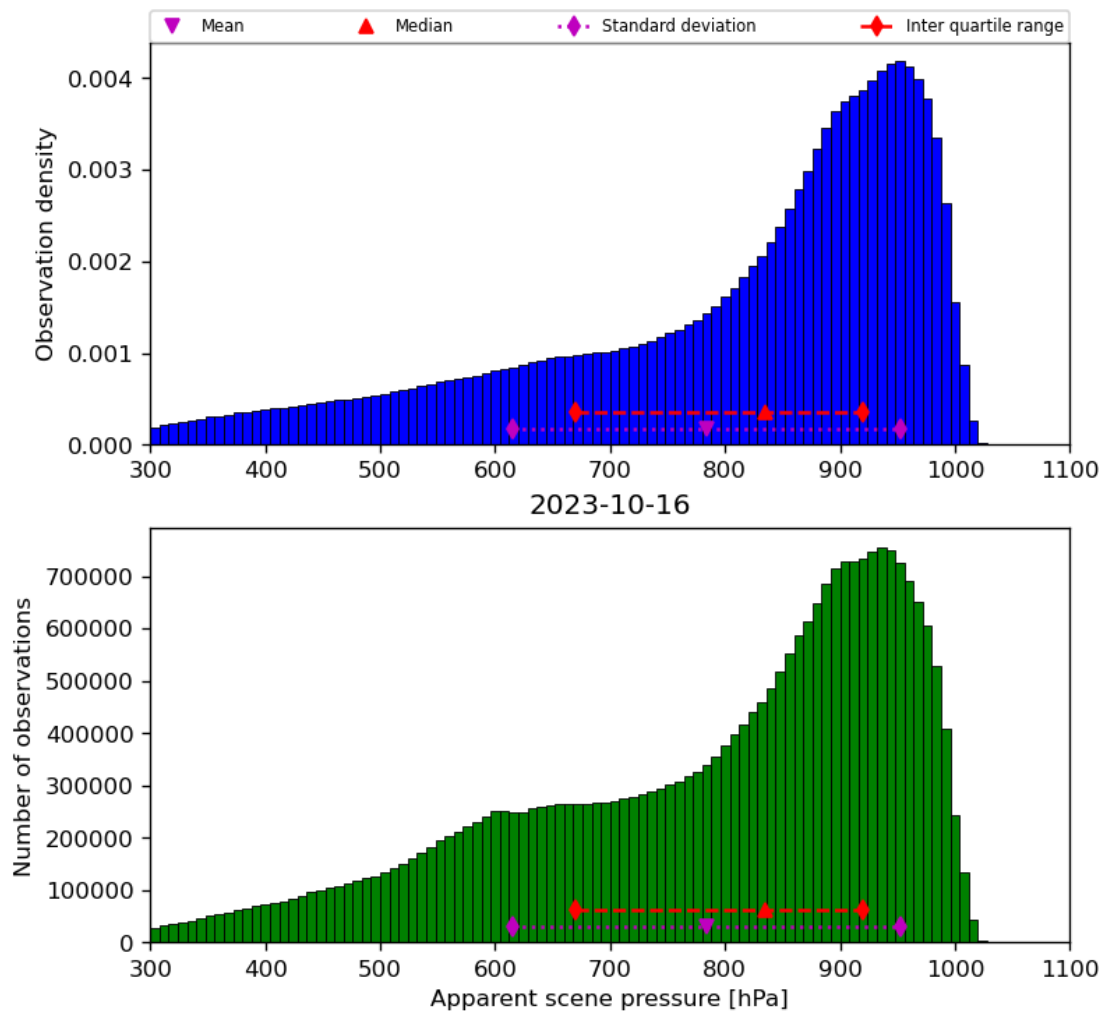
Figure 36: Histogram of “Apparent scene pressure” for 2023-10-15 to 2023-10-17
