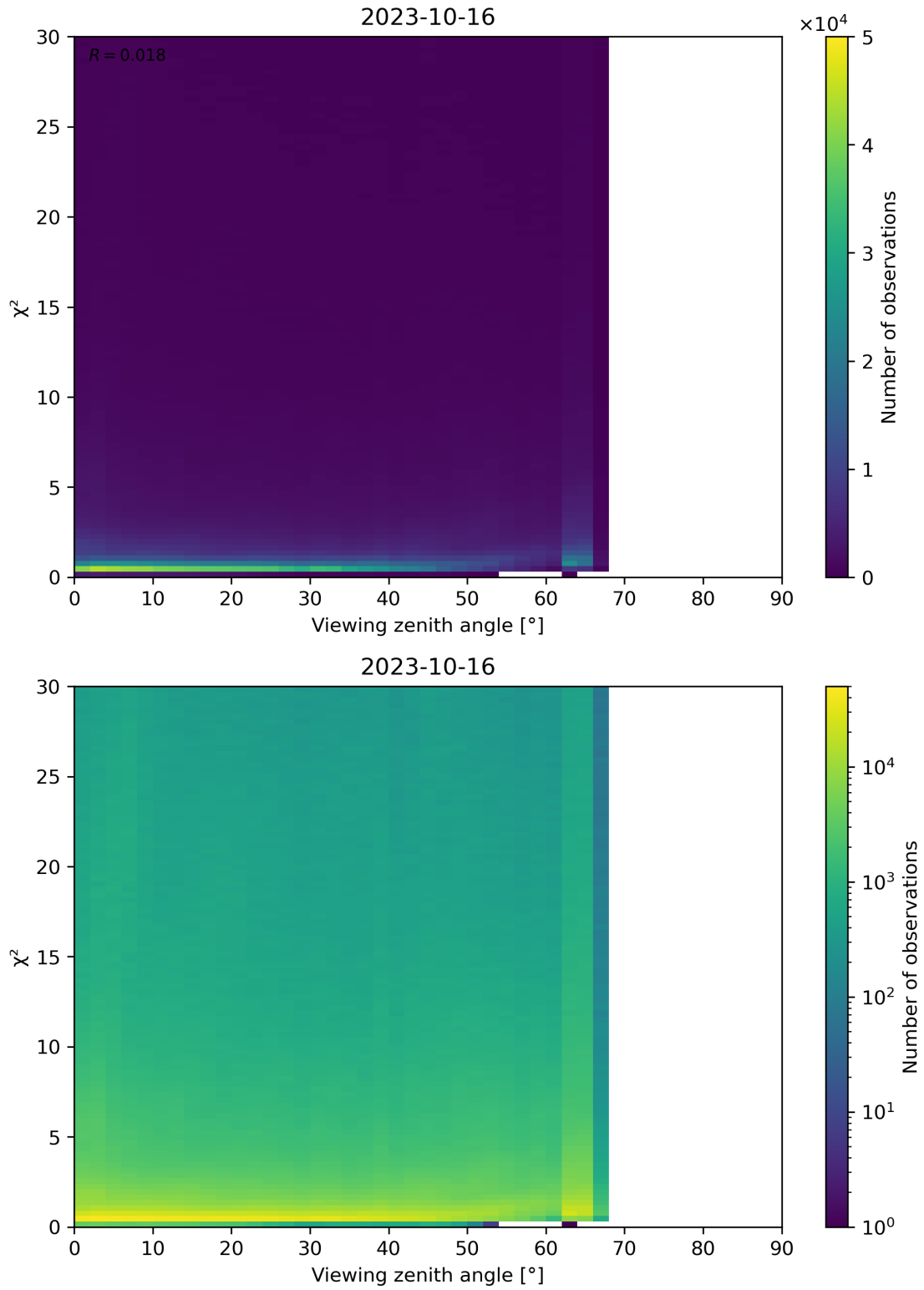
Figure 130: Scatter density plot of “Viewing zenith angle” against “ \chi^2 ” for 2023-10-15 to 2023-10-17.
