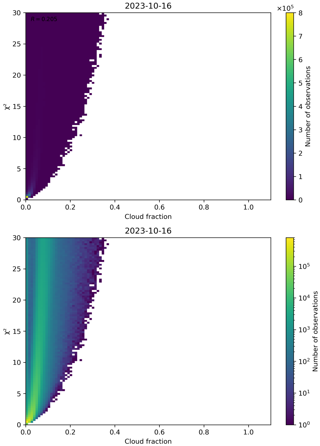
Figure 77: Scatter density plot of “Cloud fraction” against “ \chi^2 ” for 2023-10-15 to 2023-10-17.
