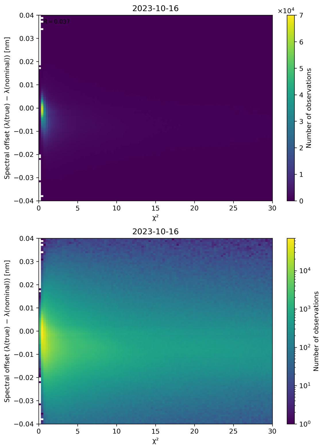
Figure 75: Scatter density plot of “ \chi^2 ” against “Spectral offset ( \lambda(\text{true}) - \lambda(\text{nominal}) )” for 2023-10-15 to 2023-10-17.
