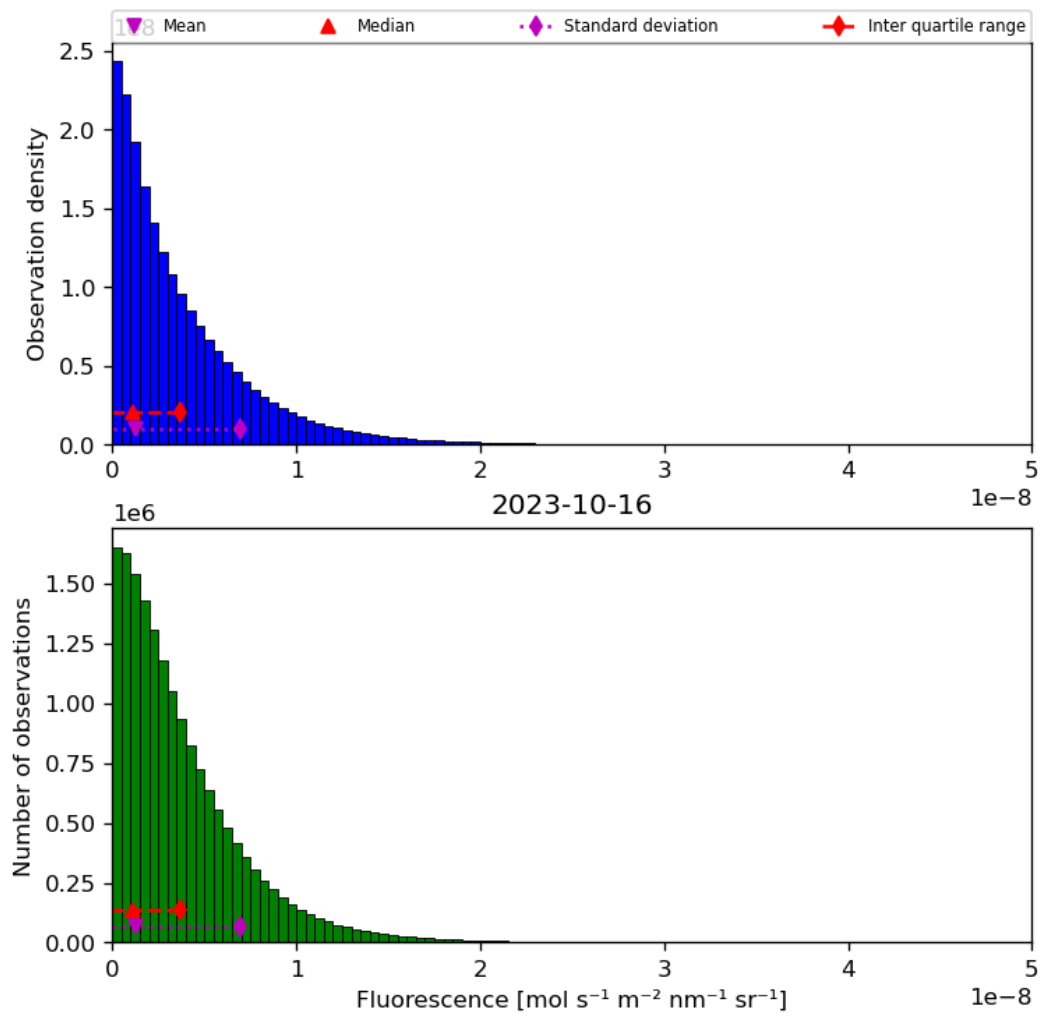
Figure 40: Histogram of “Fluorescence” for 2023-10-15 to 2023-10-17
