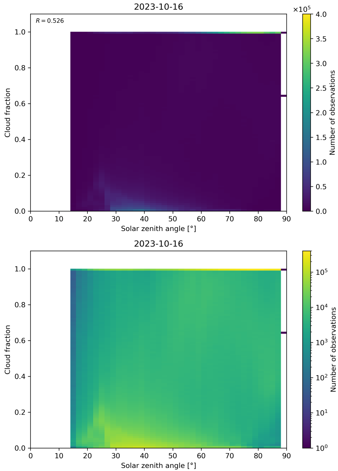
Figure 121: Scatter density plot of “Solar zenith angle” against “Cloud fraction” for 2023-10-15 to 2023-10-17.
