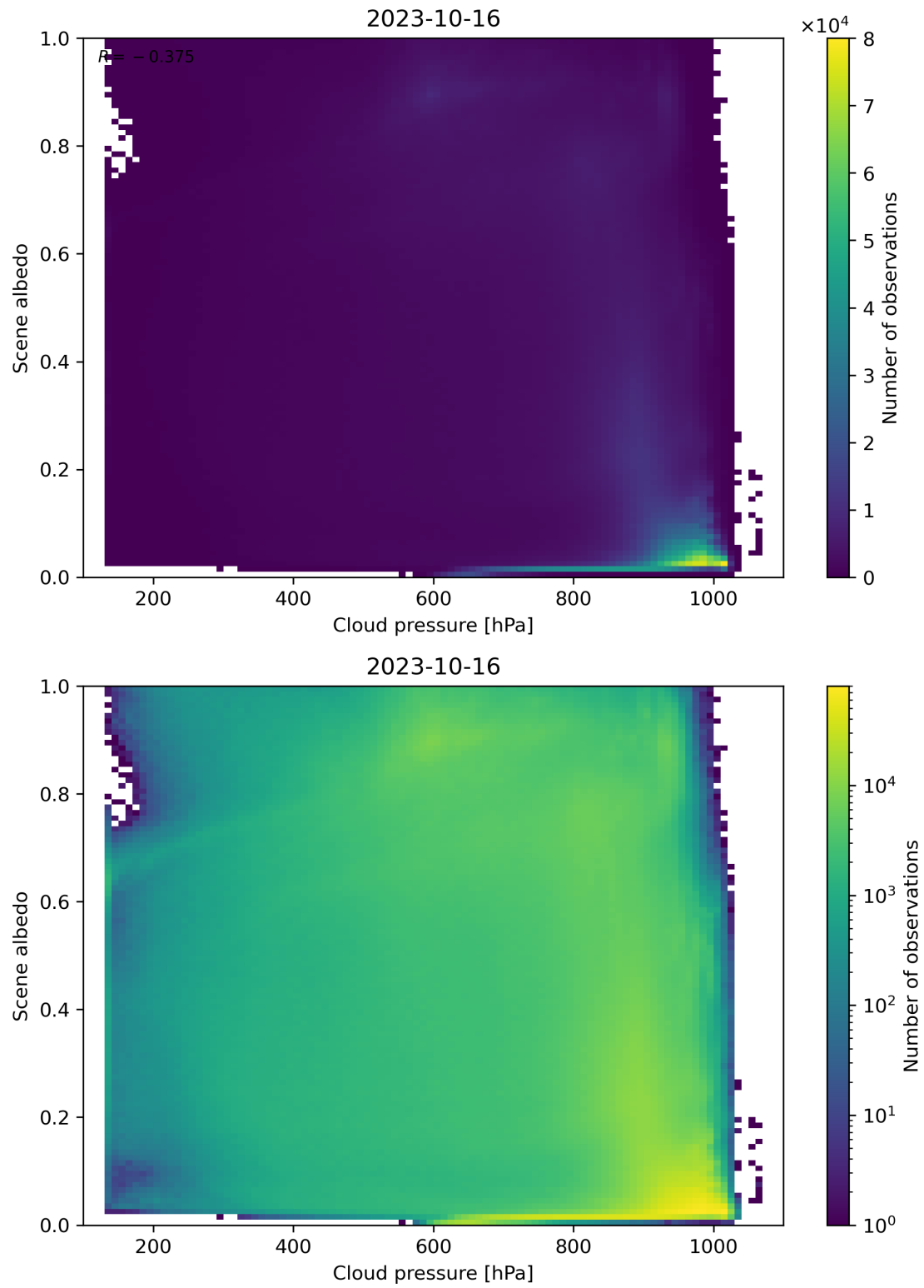
Figure 91: Scatter density plot of “Cloud pressure” against “Scene albedo” for 2023-10-15 to 2023-10-17.
