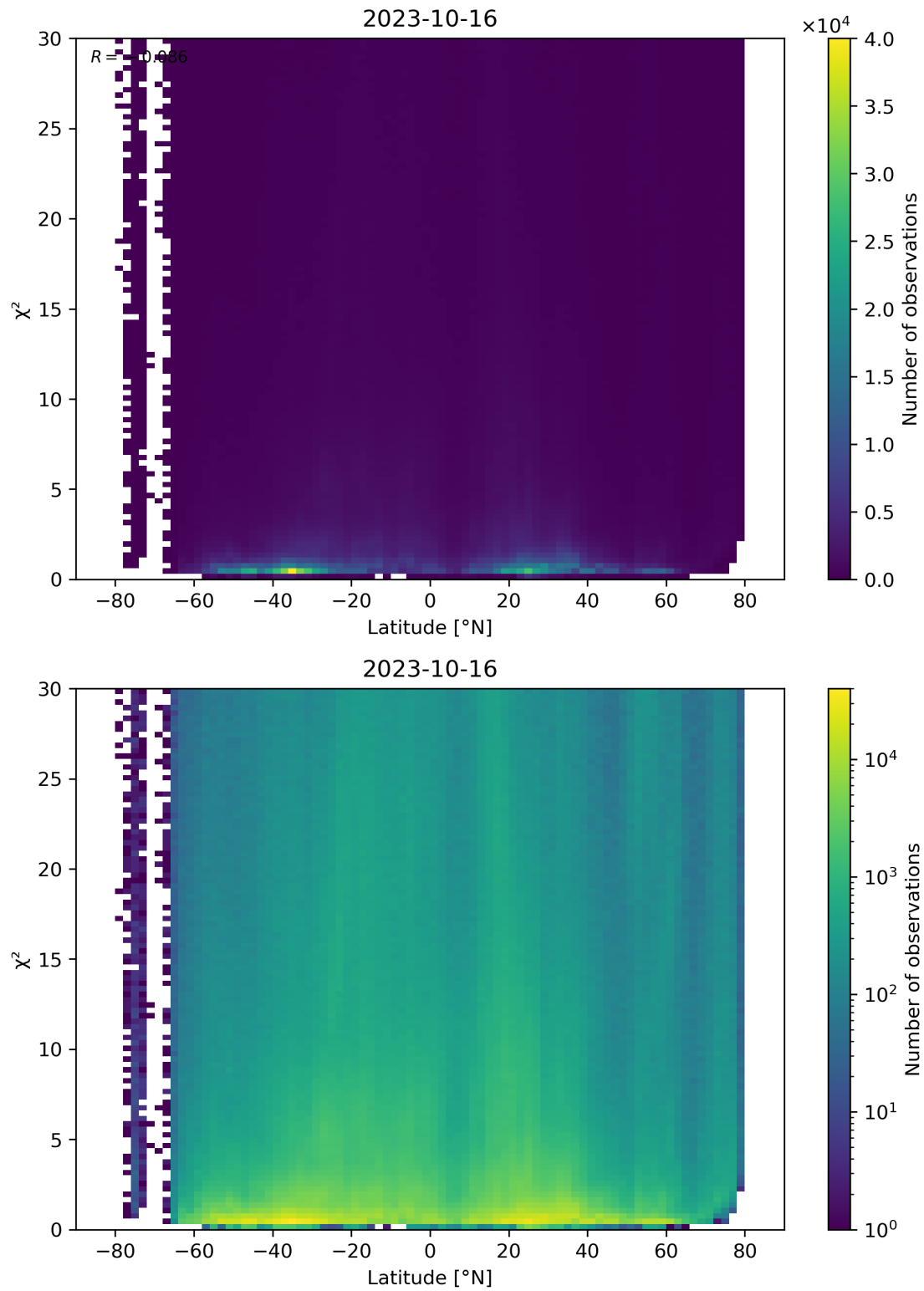
Figure 97: Scatter density plot of “Latitude” against “ \chi^2 ” for 2023-10-15 to 2023-10-17.
