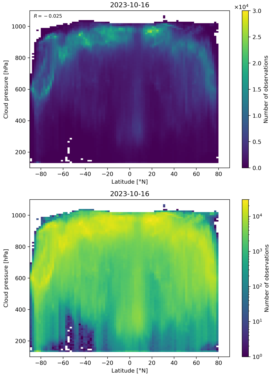
Figure 100: Scatter density plot of “Latitude” against “Cloud pressure” for 2023-10-15 to 2023-10-17.
