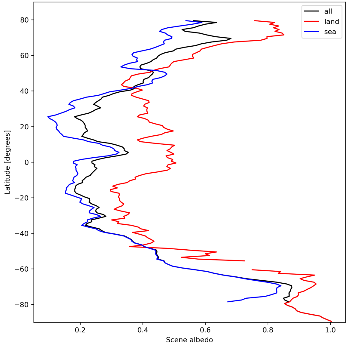
Figure 17: Zonal average of “Scene albedo” for 2023-10-15 to 2023-10-17.
