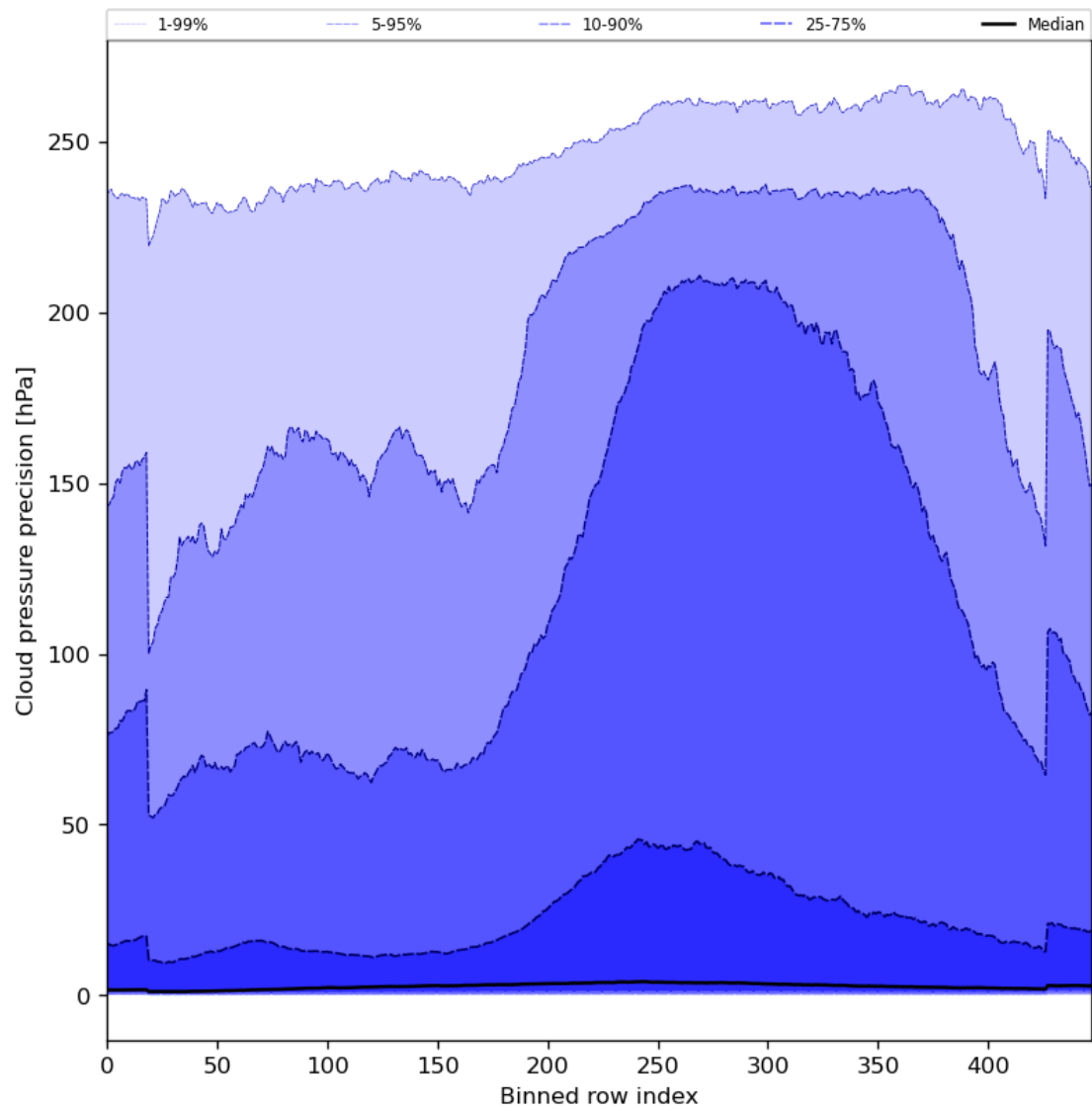
Figure 48: Along track statistics of “Cloud pressure precision” for 2023-10-15 to 2023-10-17
