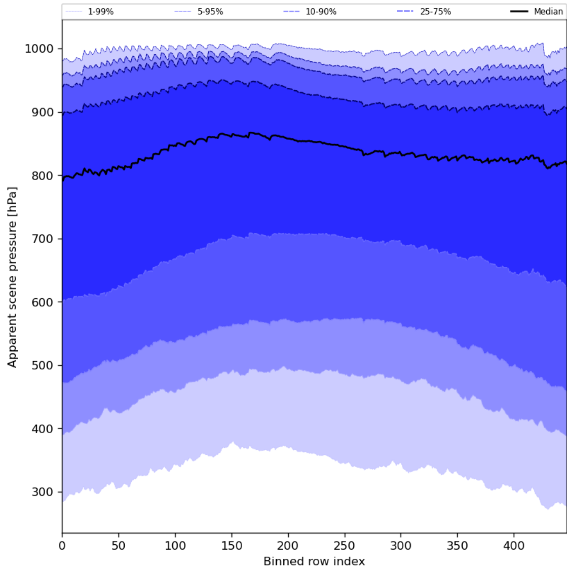
Figure 53: Along track statistics of “Apparent scene pressure” for 2023-10-15 to 2023-10-17
