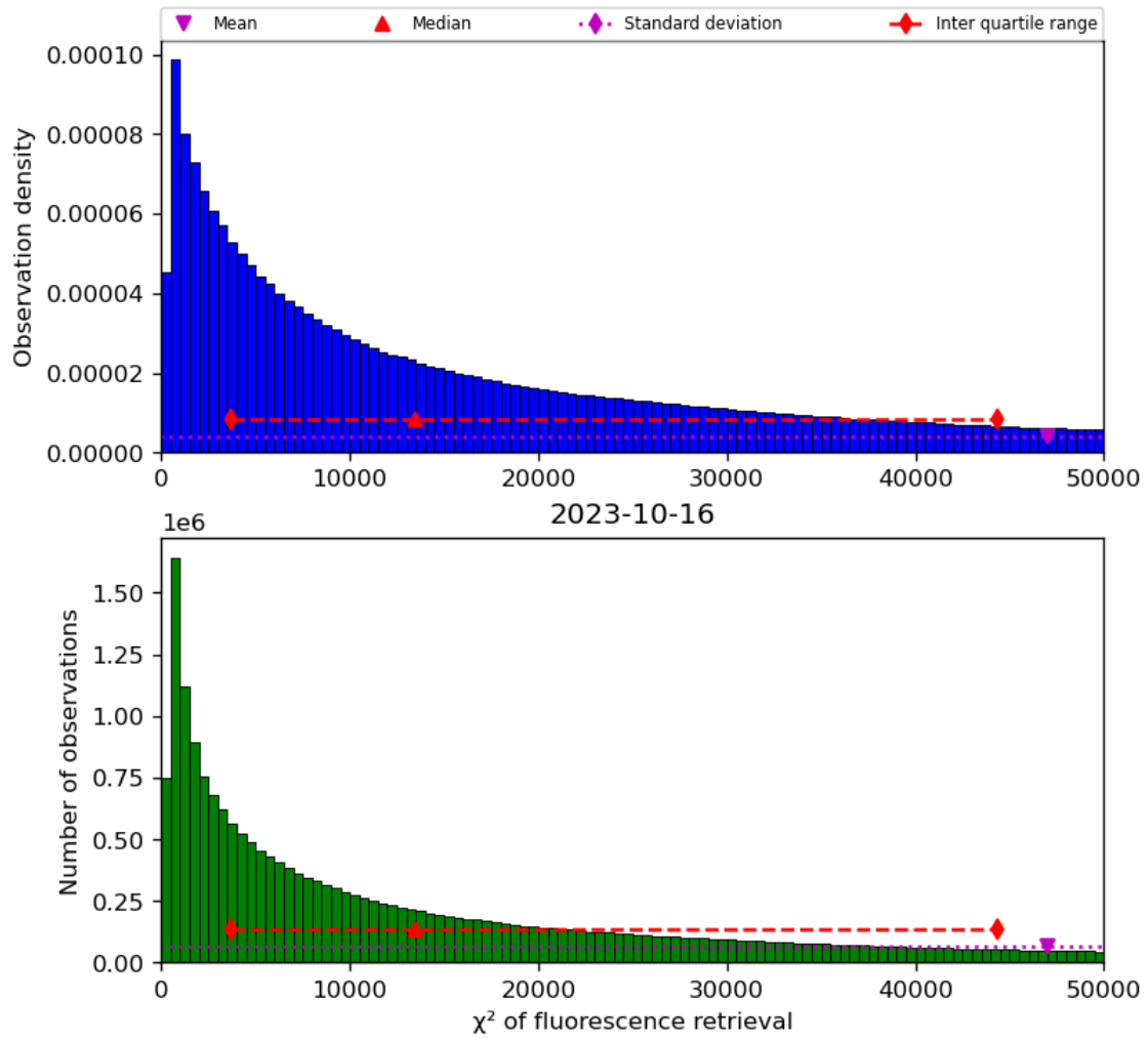
Figure 42: Histogram of “ \chi^2 of fluorescence retrieval” for 2023-10-15 to 2023-10-17
