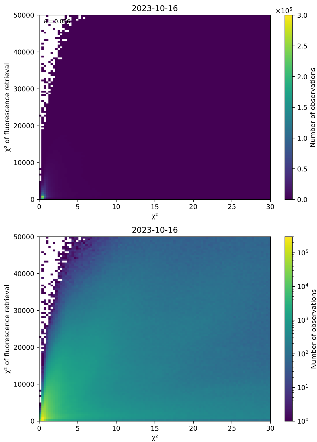
Figure 69: Scatter density plot of “ \chi^2 ” against “ \chi^2 of fluorescence retrieval” for 2023-10-15 to 2023-10-17.
