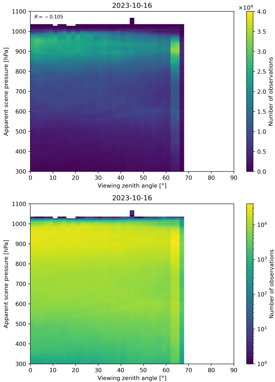
Figure 129: Scatter density plot of “Viewing zenith angle” against “Apparent scene pressure” for 2023-10-15 to 2023-10-17.
