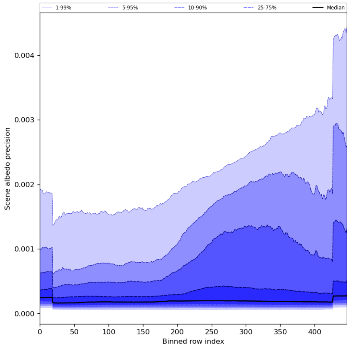
Figure 52: Along track statistics of “Scene albedo precision” for 2023-10-15 to 2023-10-17
