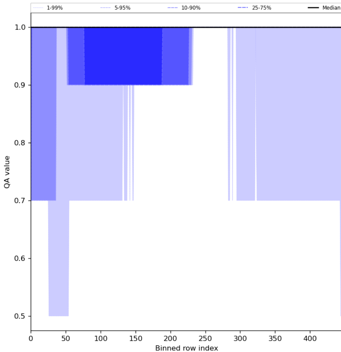
Figure 46: Along track statistics of “QA value” for 2023-10-15 to 2023-10-17
