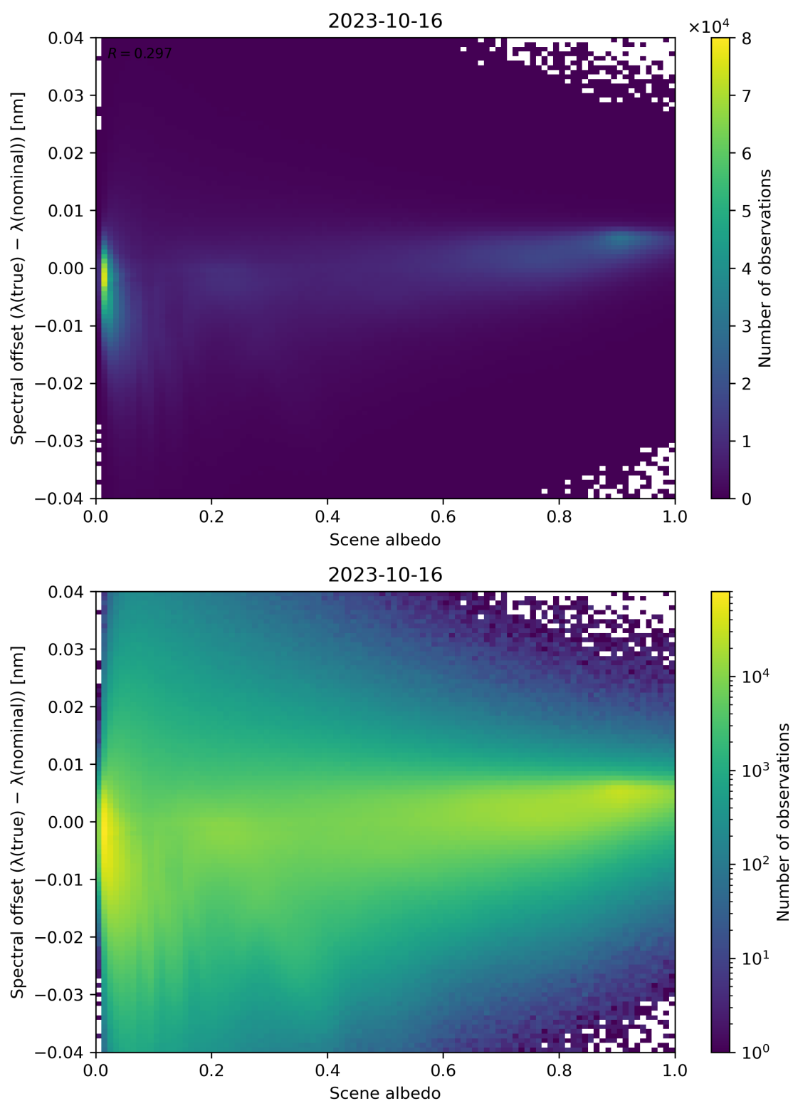
Figure 117: Scatter density plot of “Scene albedo” against “Spectral offset ( \lambda(\text{true}) - \lambda(\text{nominal}) )” for 2023-10-15 to 2023-10-17.
