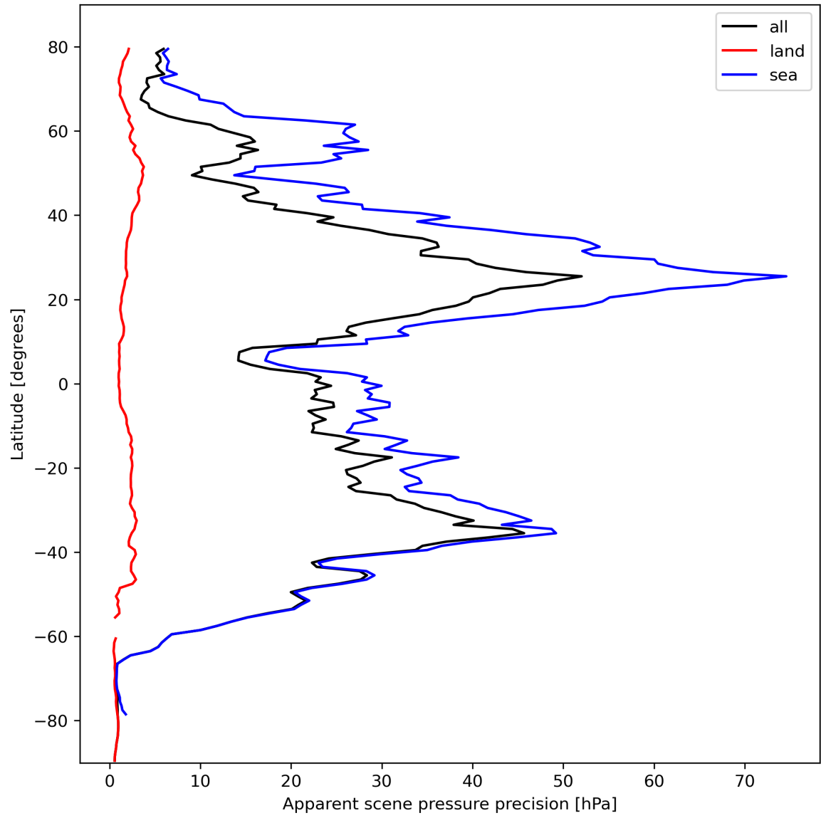
Figure 20: Zonal average of “Apparent scene pressure precision” for 2023-10-15 to 2023-10-17.
