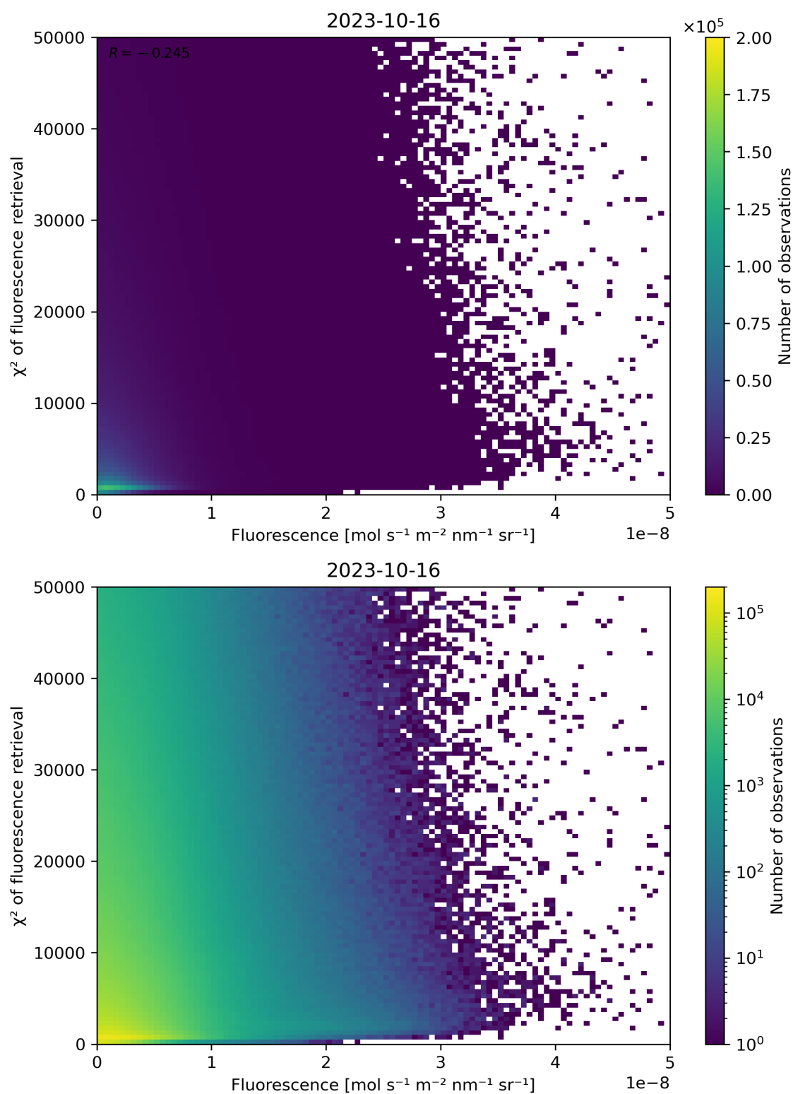
Figure 93: Scatter density plot of “Fluorescence” against “ \chi^2 of fluorescence retrieval” for 2023-10-15 to 2023-10-17.
