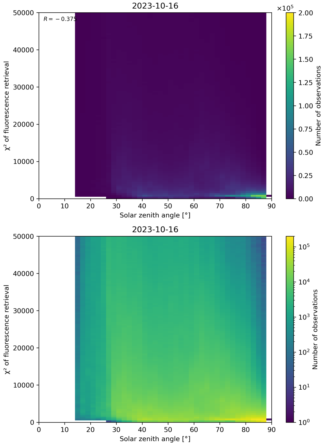
Figure 120: Scatter density plot of “Solar zenith angle” against “ \chi^2 of fluorescence retrieval” for 2023-10-15 to 2023-10-17.
