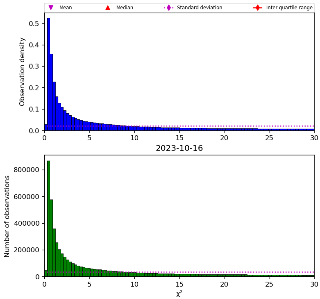
Figure 38: Histogram of “ \chi^2 ” for 2023-10-15 to 2023-10-17
