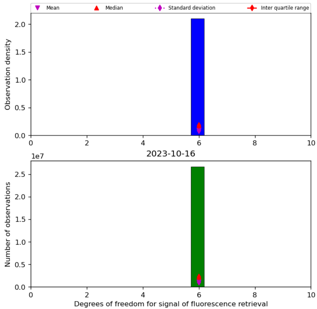
Figure 43: Histogram of “Degrees of freedom for signal of fluorescence retrieval” for 2023-10-15 to 2023-10-17
