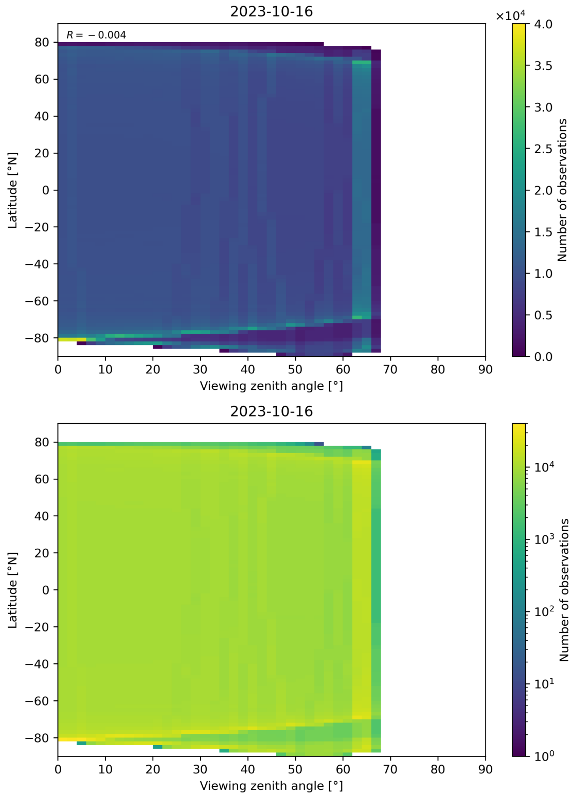
Figure 135: Scatter density plot of “Viewing zenith angle” against “Latitude” for 2023-10-15 to 2023-10-17.
