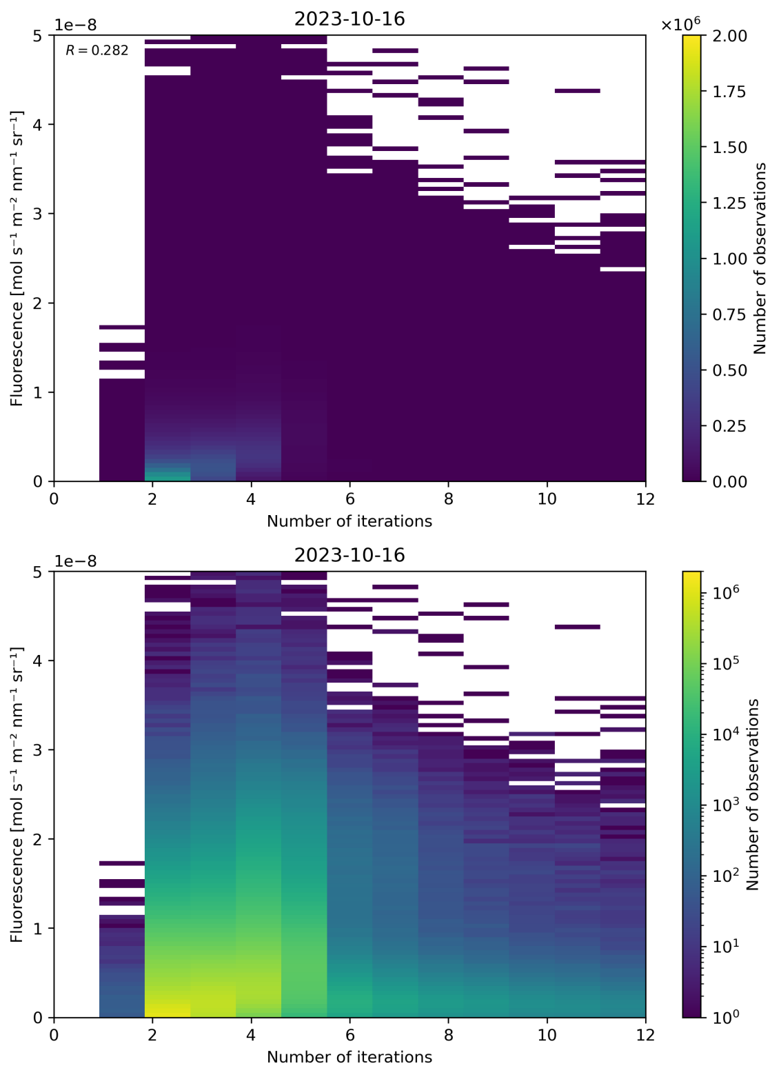
Figure 107: Scatter density plot of “Number of iterations” against “Fluorescence” for 2023-10-15 to 2023-10-17.
