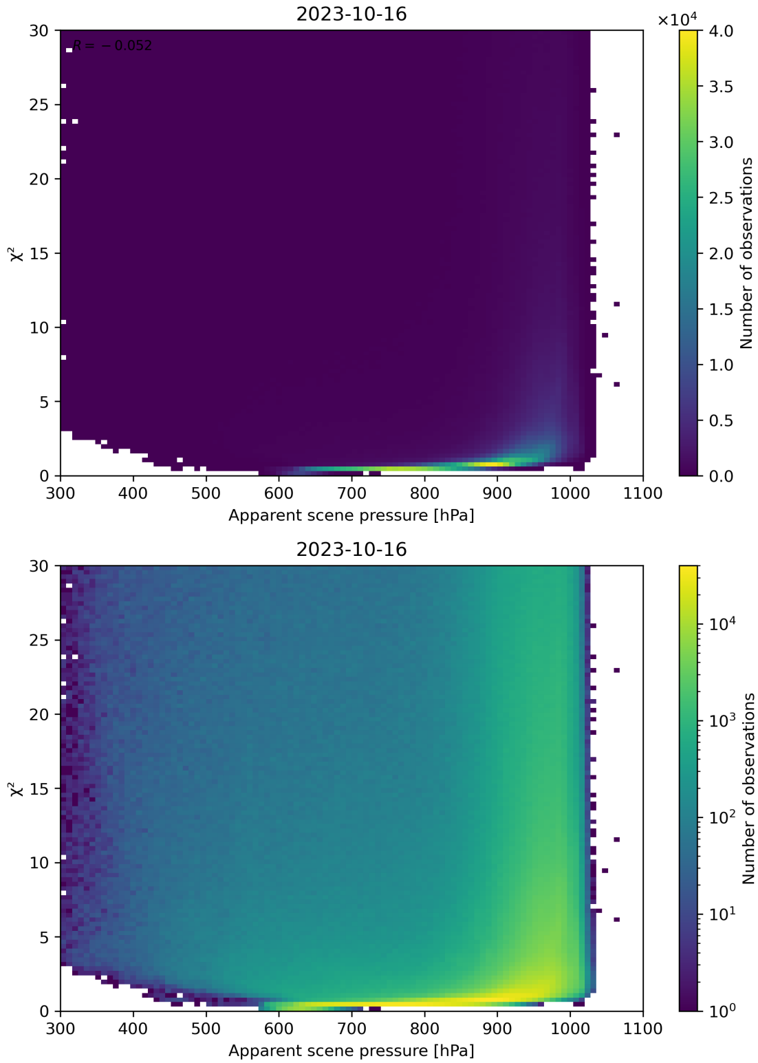
Figure 63: Scatter density plot of “Apparent scene pressure” against “ \chi^2 ” for 2023-10-15 to 2023-10-17.
