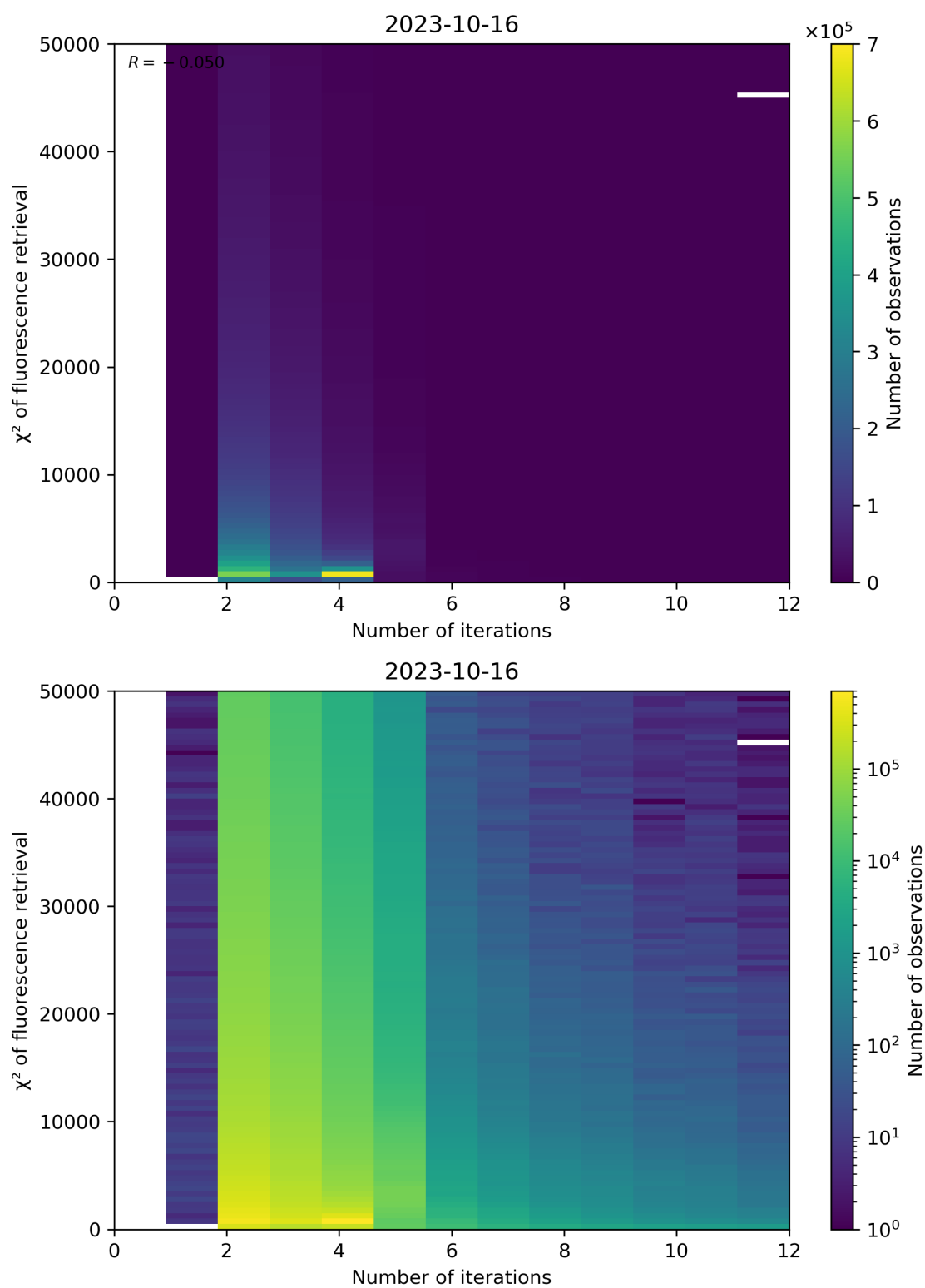
Figure 106: Scatter density plot of “Number of iterations” against “ \chi^2 of fluorescence retrieval” for 2023-10-15 to 2023-10-17.
