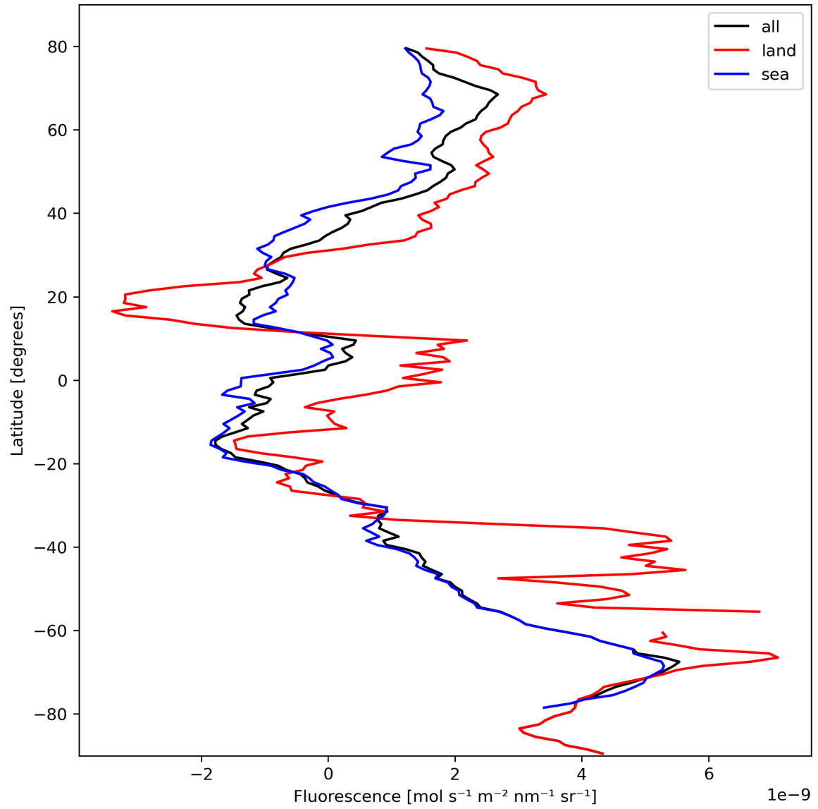
Figure 23: Zonal average of “Fluorescence” for 2023-10-15 to 2023-10-17.
