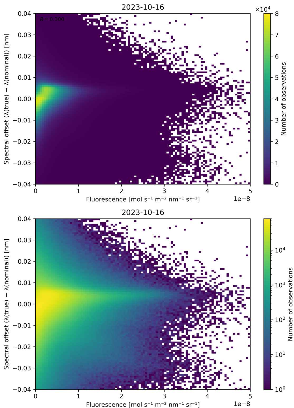
Figure 95: Scatter density plot of “Fluorescence” against “Spectral offset ( \lambda(\text{true}) - \lambda(\text{nominal}) )” for 2023-10-15 to 2023-10-17.
