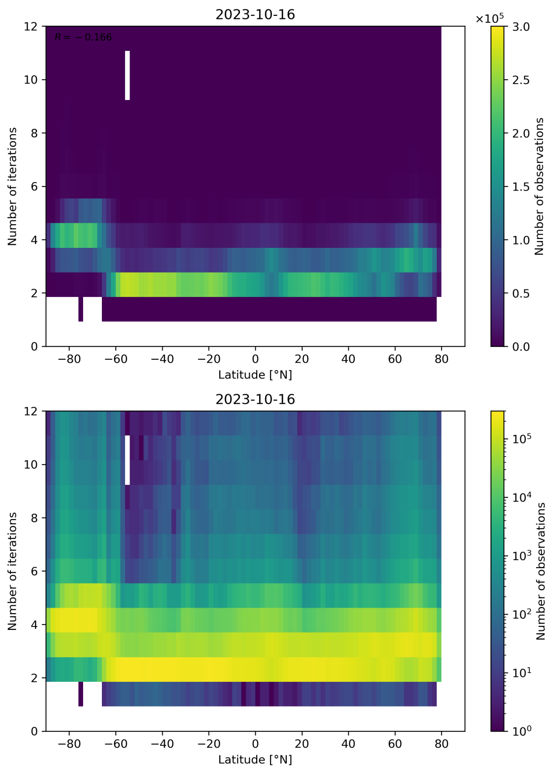
Figure 102: Scatter density plot of “Latitude” against “Number of iterations” for 2023-10-15 to 2023-10-17.
