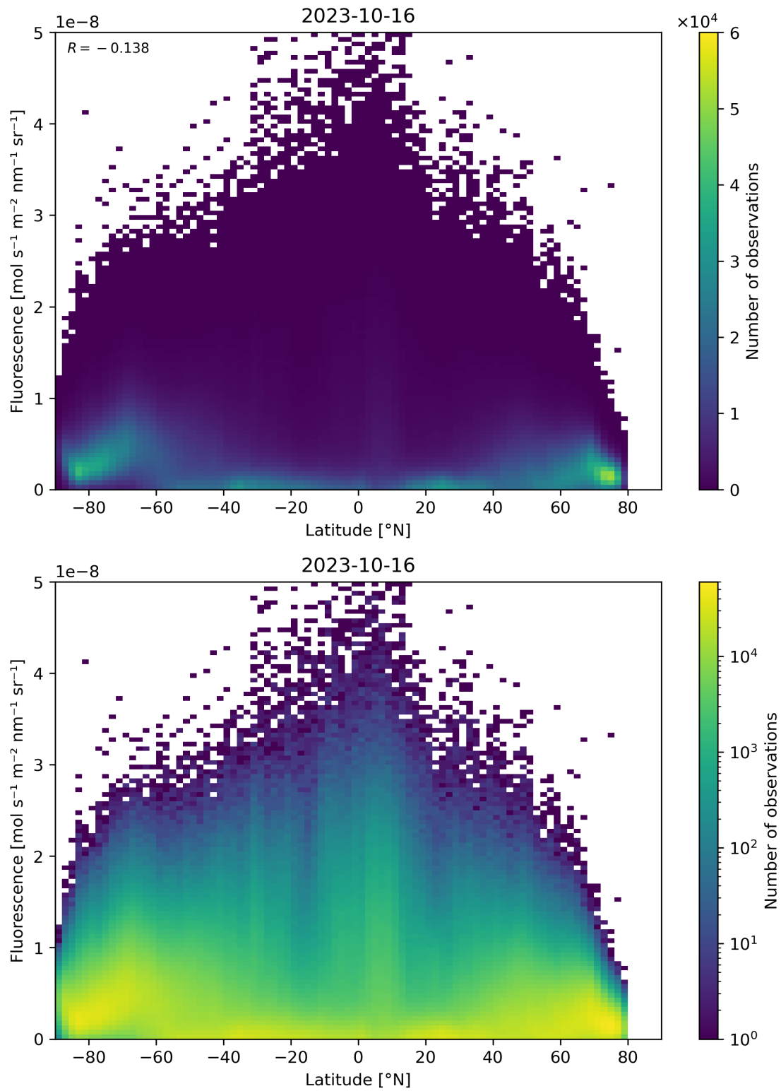
Figure 101: Scatter density plot of “Latitude” against “Fluorescence” for 2023-10-15 to 2023-10-17.
