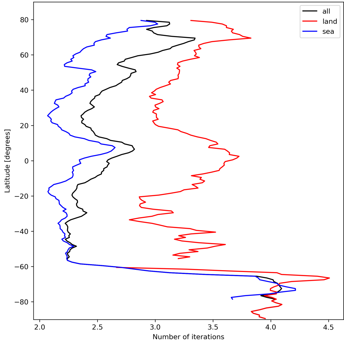
Figure 22: Zonal average of “Number of iterations” for 2023-10-15 to 2023-10-17.
