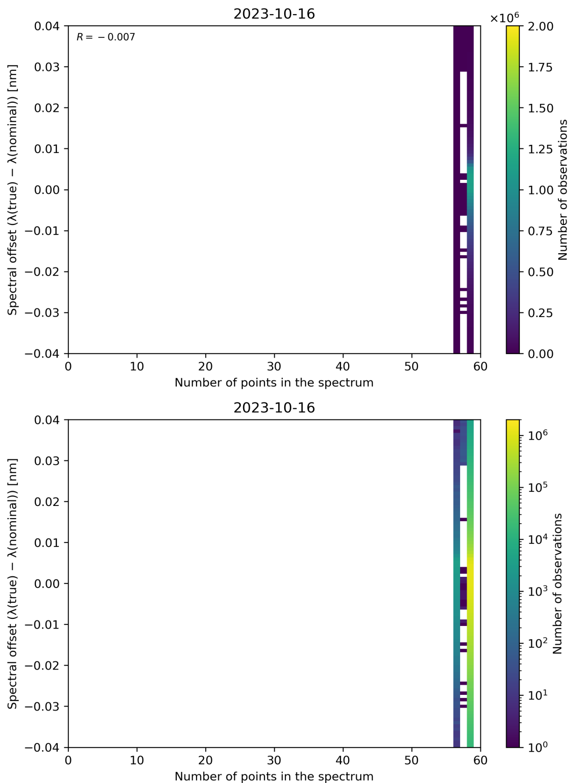
Figure 110: Scatter density plot of “Number of points in the spectrum” against “Spectral offset ( \lambda(\text{true}) - \lambda(\text{nominal}) )” for 2023-10-15 to 2023-10-17.
