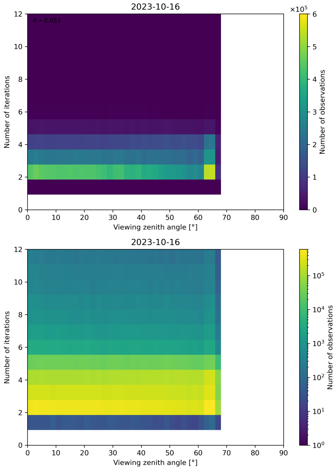
Figure 136: Scatter density plot of “Viewing zenith angle” against “Number of iterations” for 2023-10-15 to 2023-10-17.
