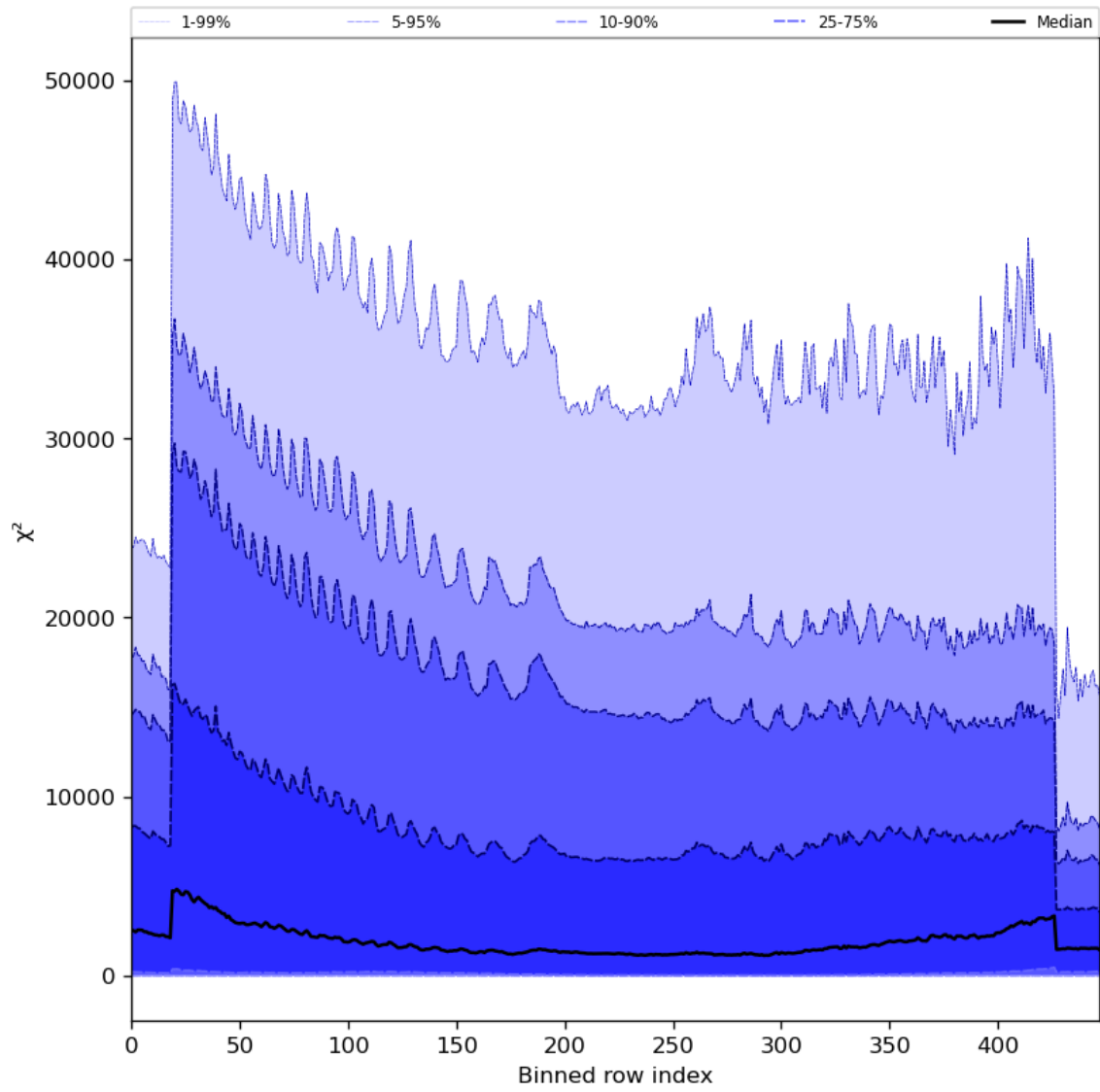
Figure 55: Along track statistics of " \chi^2 " for 2023-10-17 to 2023-10-18
