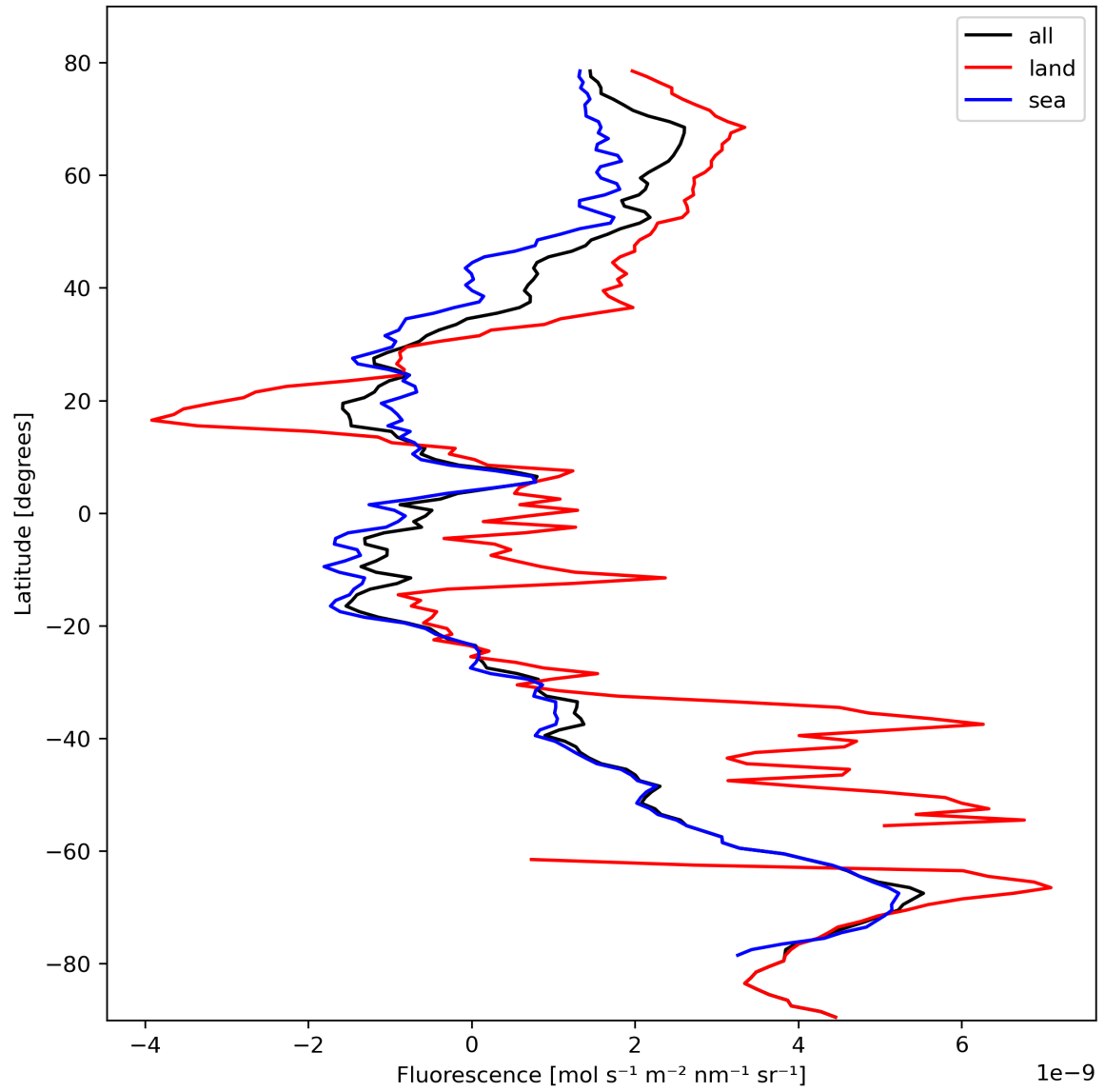
Figure 23: Zonal average of “Fluorescence” for 2023-10-17 to 2023-10-18.
