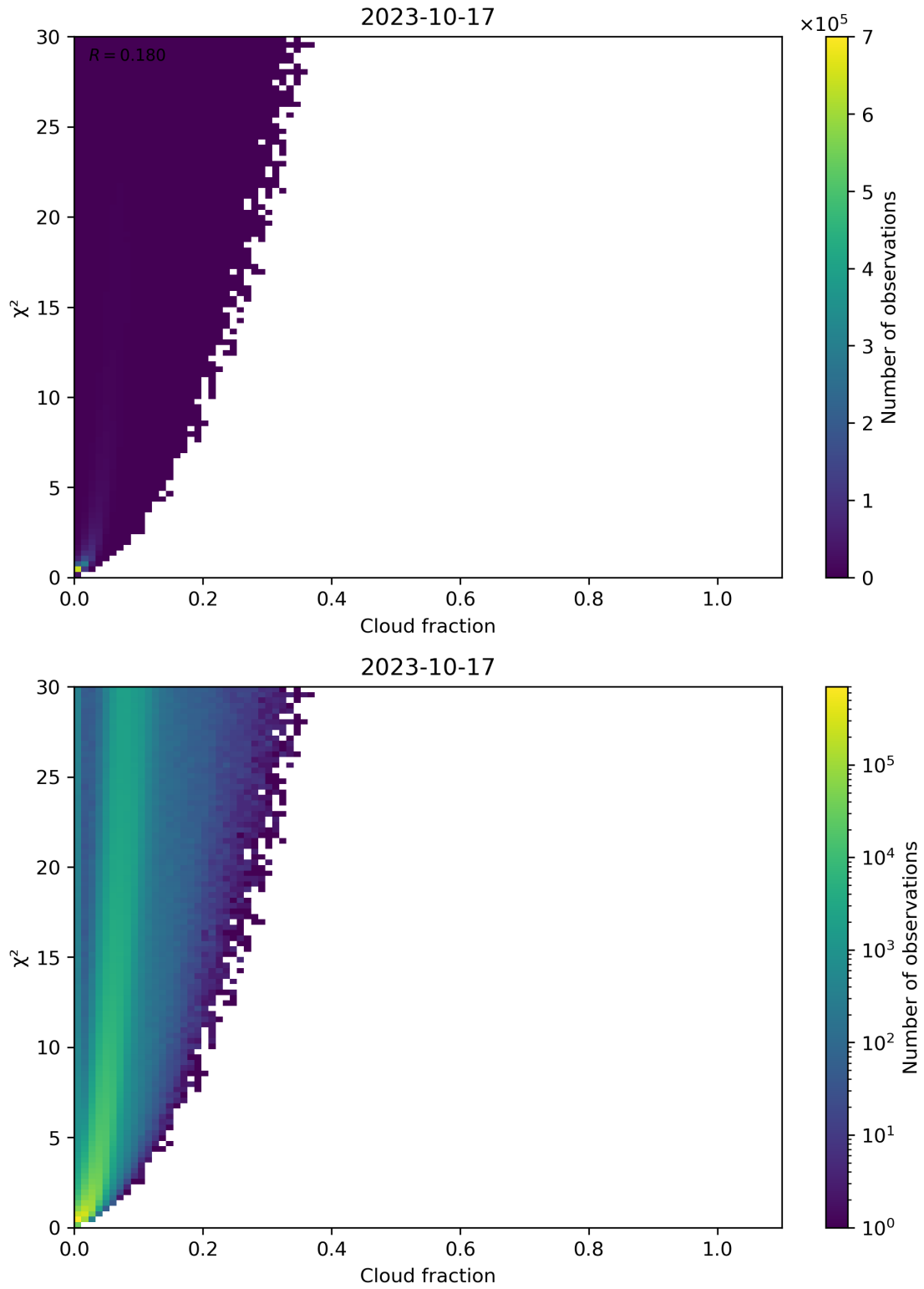
Figure 77: Scatter density plot of “Cloud fraction” against “ \chi^2 ” for 2023-10-17 to 2023-10-18.
