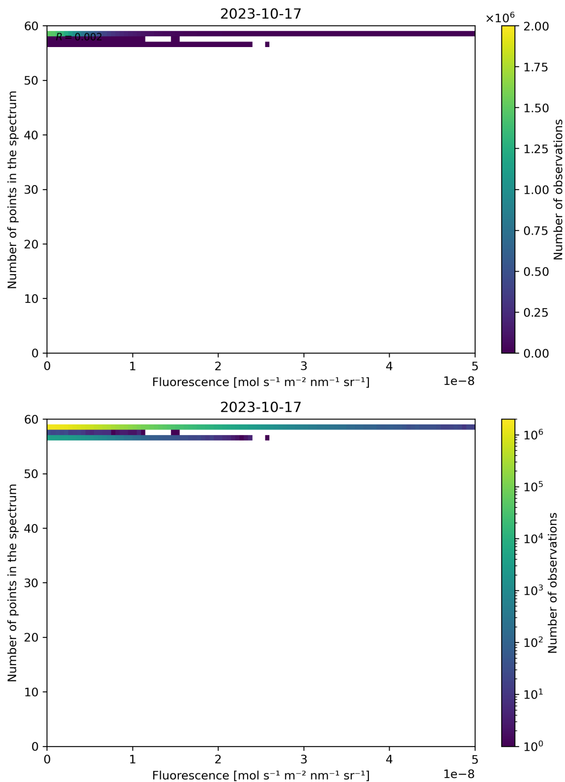
Figure 94: Scatter density plot of “Fluorescence” against “Number of points in the spectrum” for 2023-10-17 to 2023-10-18.
