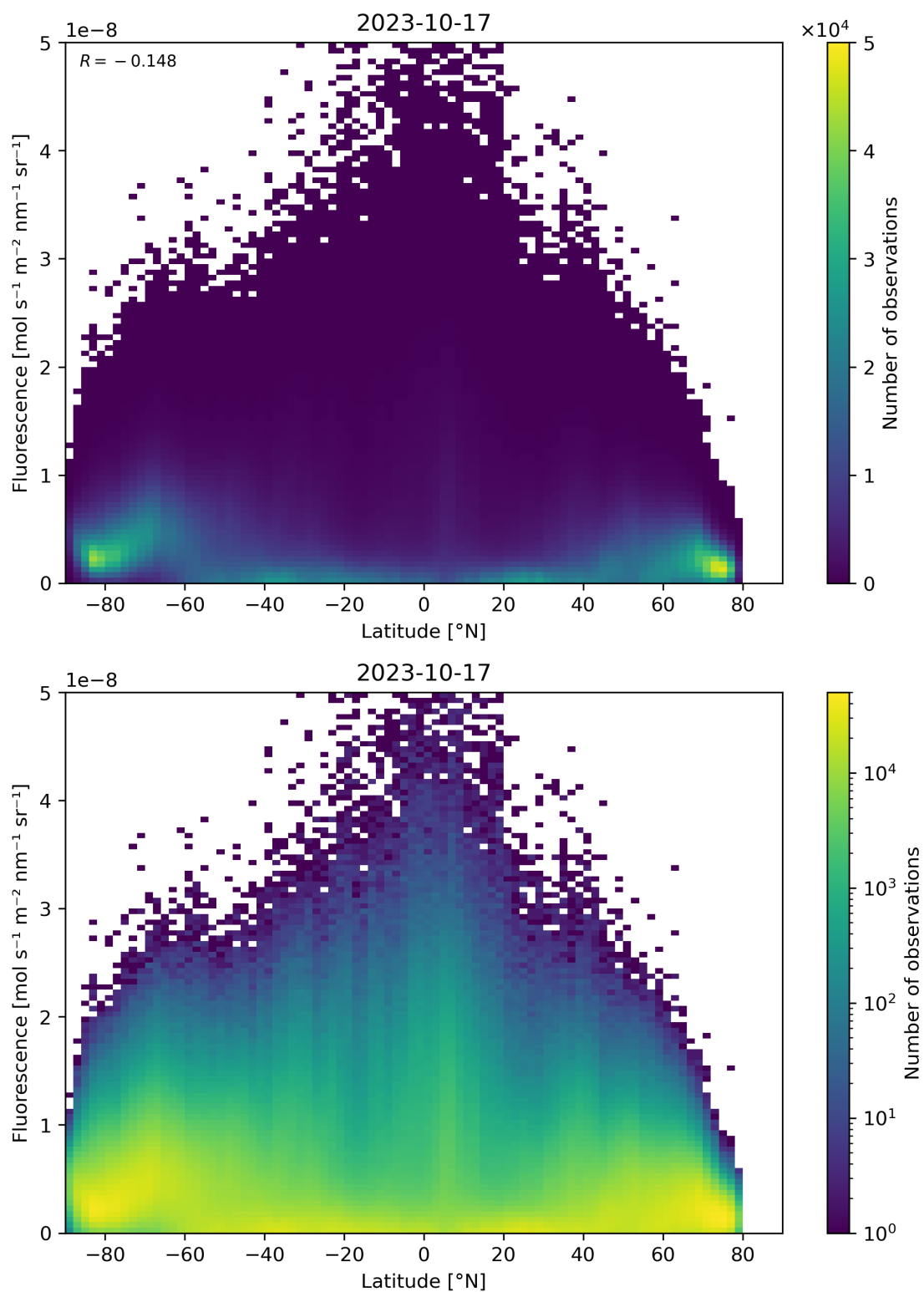
Figure 101: Scatter density plot of “Latitude” against “Fluorescence” for 2023-10-17 to 2023-10-18.
