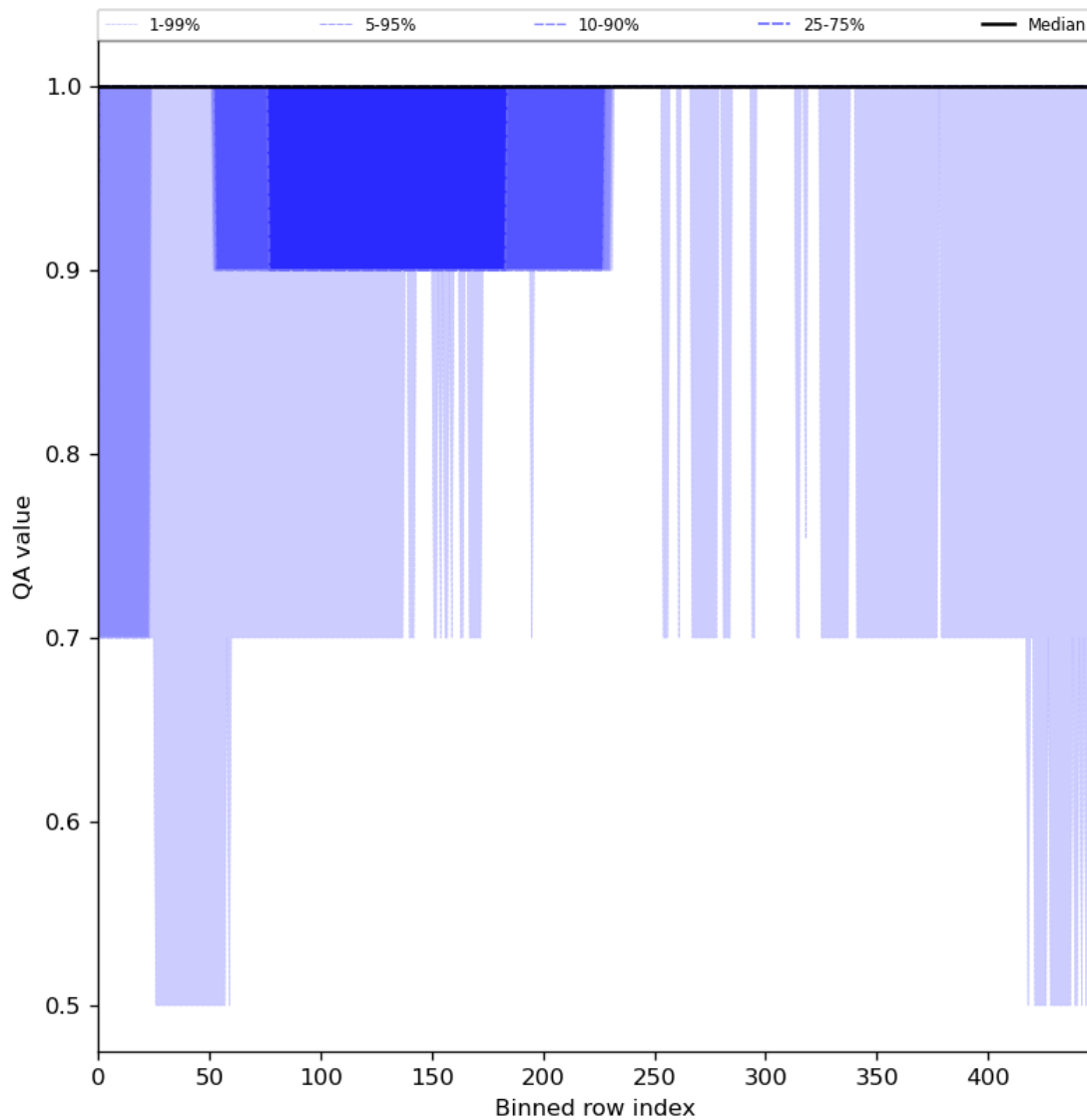
Figure 46: Along track statistics of “QA value” for 2023-10-17 to 2023-10-18
