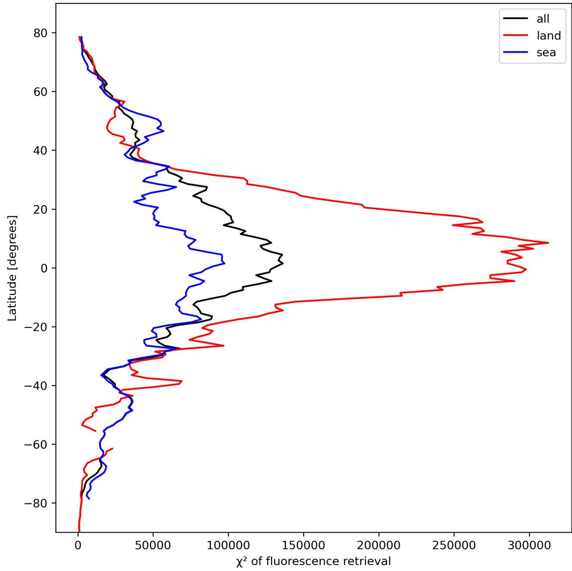
Figure 25: Zonal average of “ \chi^2 of fluorescence retrieval” for 2023-10-17 to 2023-10-18.
