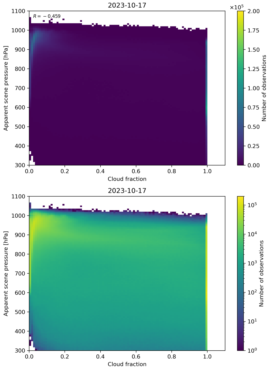
Figure 76: Scatter density plot of “Cloud fraction” against “Apparent scene pressure” for 2023-10-17 to 2023-10-18.
