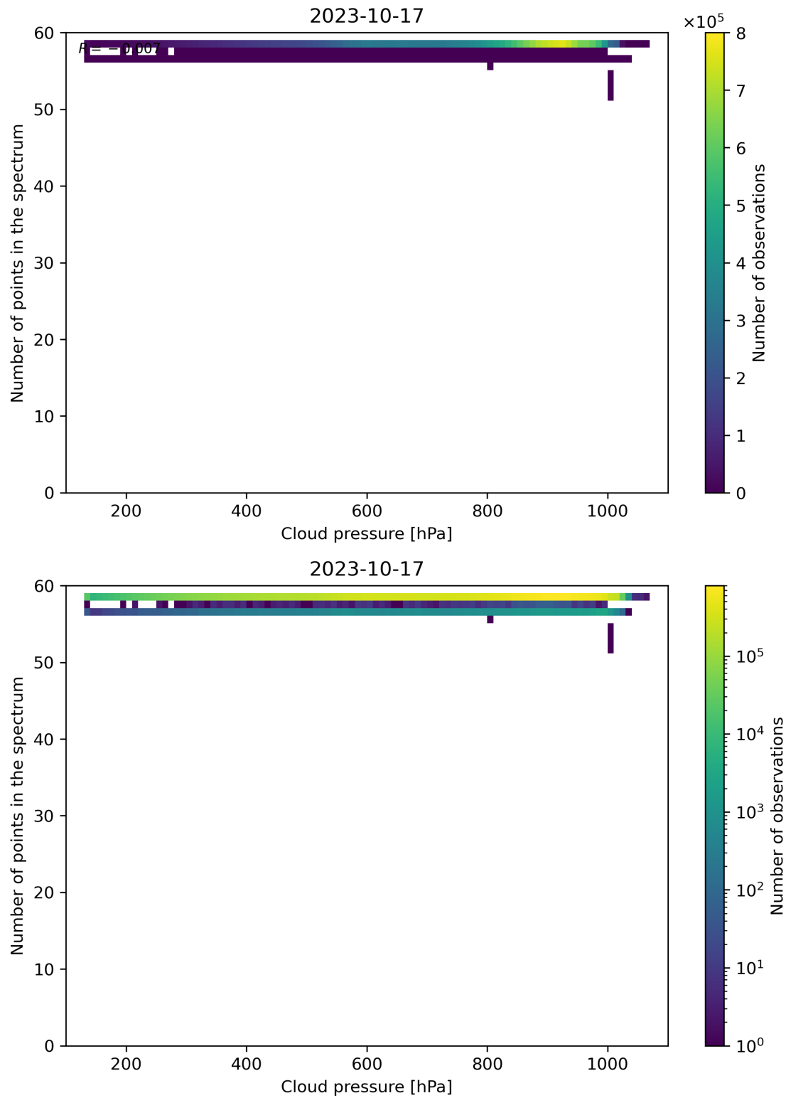
Figure 90: Scatter density plot of “Cloud pressure” against “Number of points in the spectrum” for 2023-10-17 to 2023-10-18.
