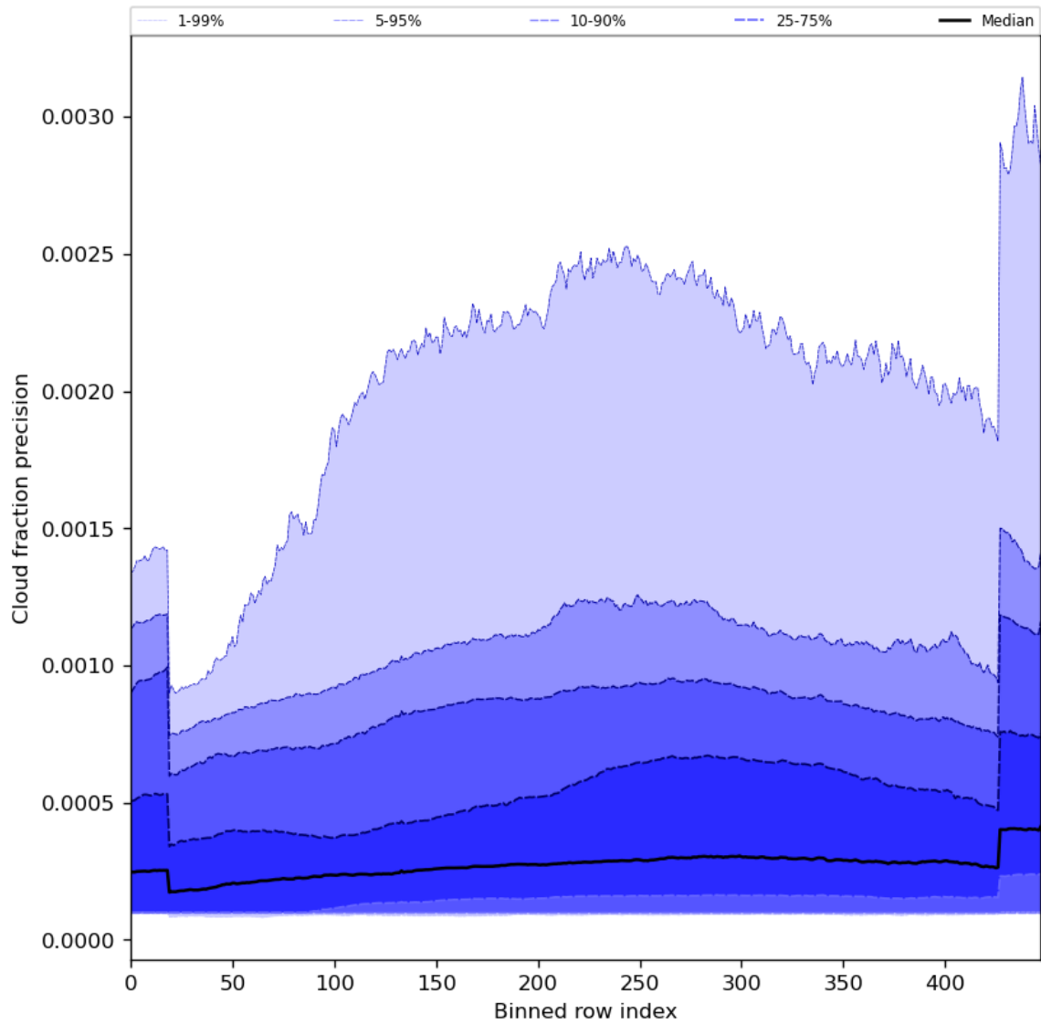
Figure 50: Along track statistics of “Cloud fraction precision” for 2023-10-17 to 2023-10-18
