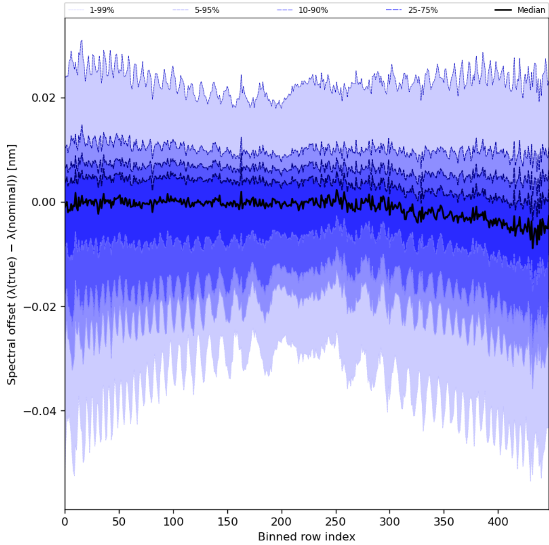
Figure 62: Along track statistics of “Spectral offset ( \lambda(\text{true}) - \lambda(\text{nominal}) )” for 2023-10-17 to 2023-10-18
