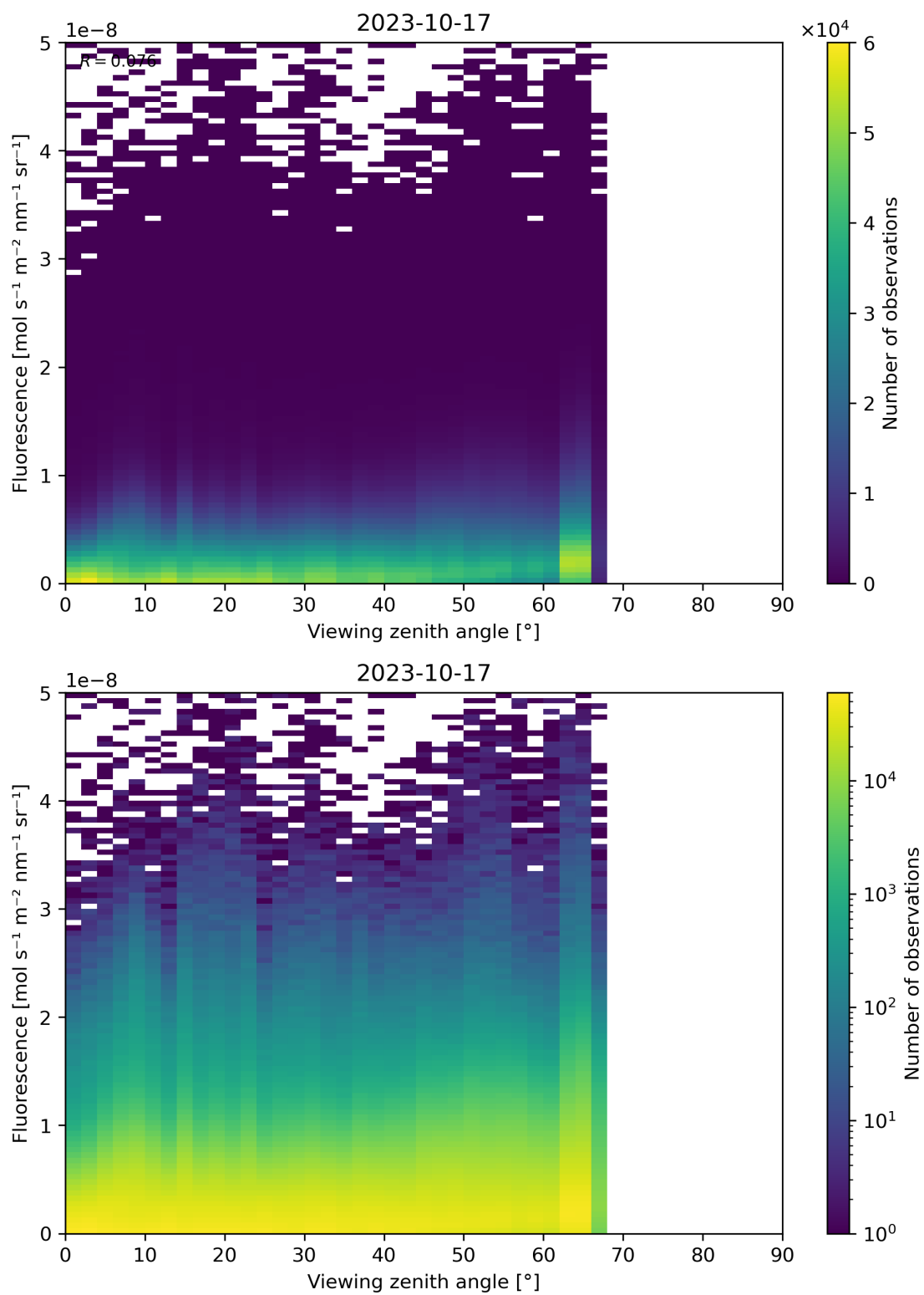
Figure 134: Scatter density plot of “Viewing zenith angle” against “Fluorescence” for 2023-10-17 to 2023-10-18.
