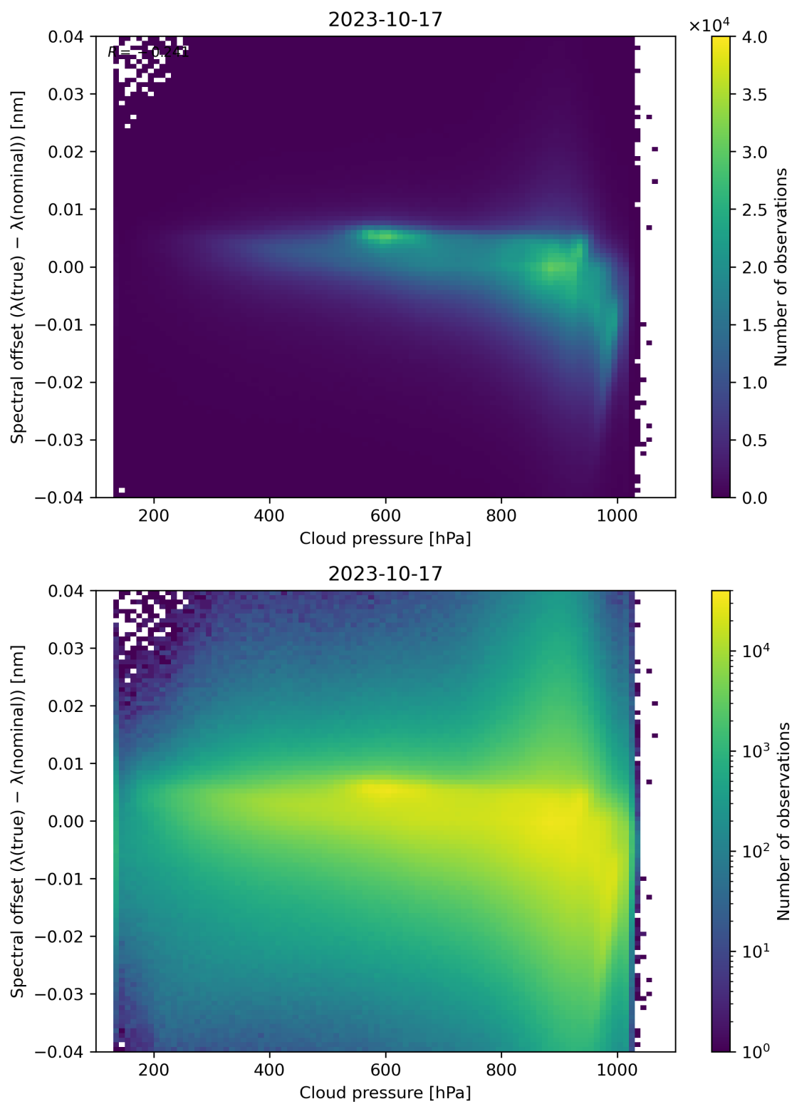
Figure 92: Scatter density plot of “Cloud pressure” against “Spectral offset ( \lambda(\text{true}) - \lambda(\text{nominal}) )” for 2023-10-17 to 2023-10-18.
