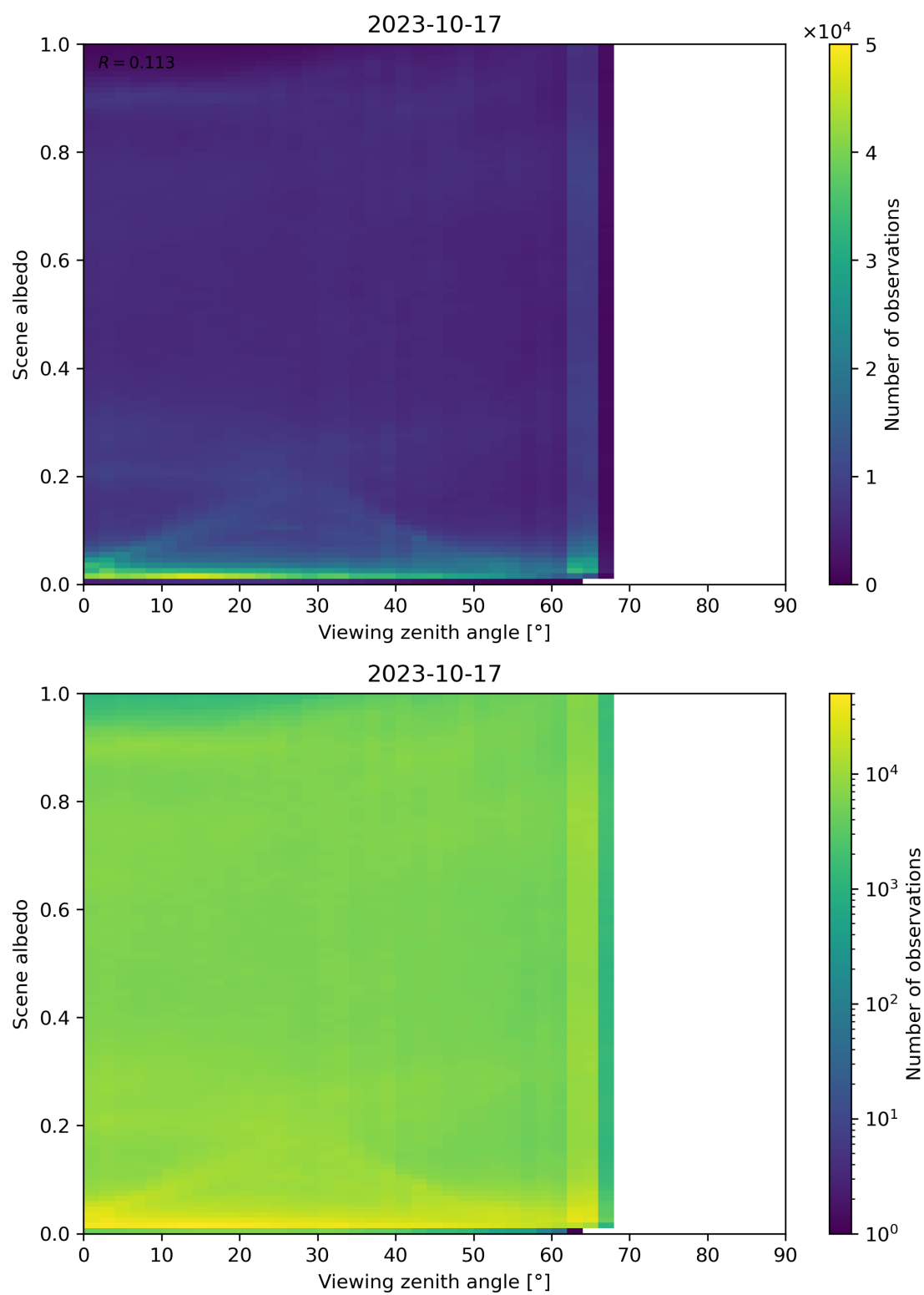
Figure 138: Scatter density plot of “Viewing zenith angle” against “Scene albedo” for 2023-10-17 to 2023-10-18.
