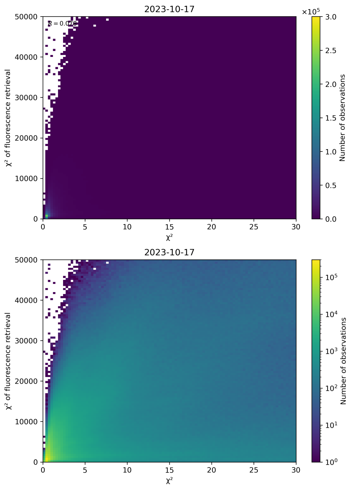
Figure 69: Scatter density plot of “ \chi^2 ” against “ \chi^2 of fluorescence retrieval” for 2023-10-17 to 2023-10-18.
