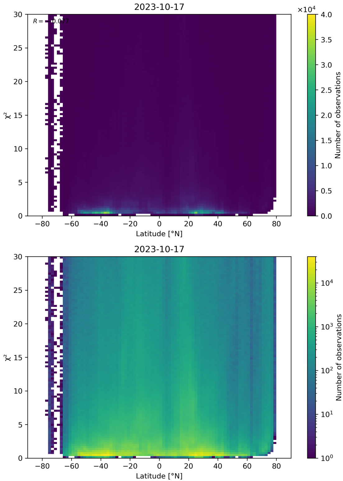
Figure 97: Scatter density plot of “Latitude” against “ \chi^2 ” for 2023-10-17 to 2023-10-18.
