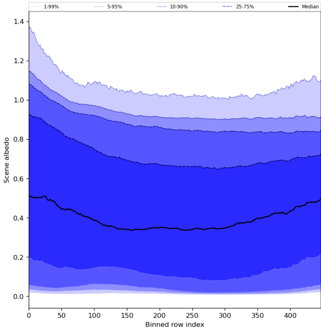
Figure 51: Along track statistics of “Scene albedo” for 2023-10-17 to 2023-10-18
