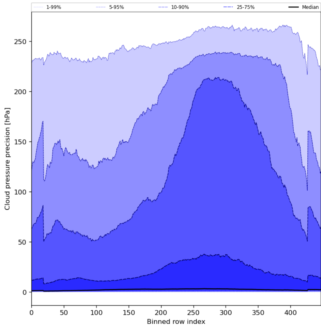
Figure 48: Along track statistics of “Cloud pressure precision” for 2023-10-17 to 2023-10-18
