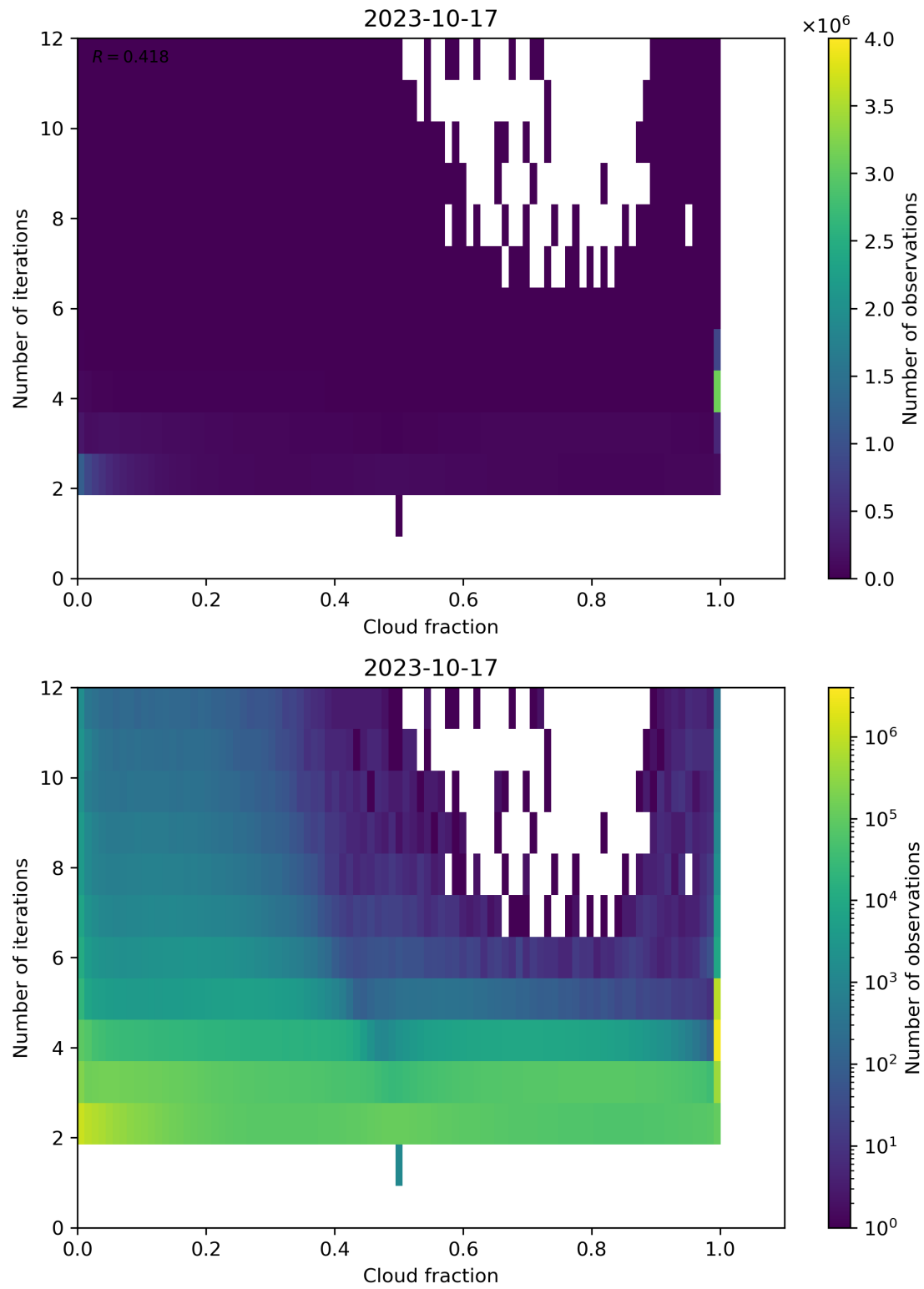
Figure 80: Scatter density plot of “Cloud fraction” against “Number of iterations” for 2023-10-17 to 2023-10-18.
