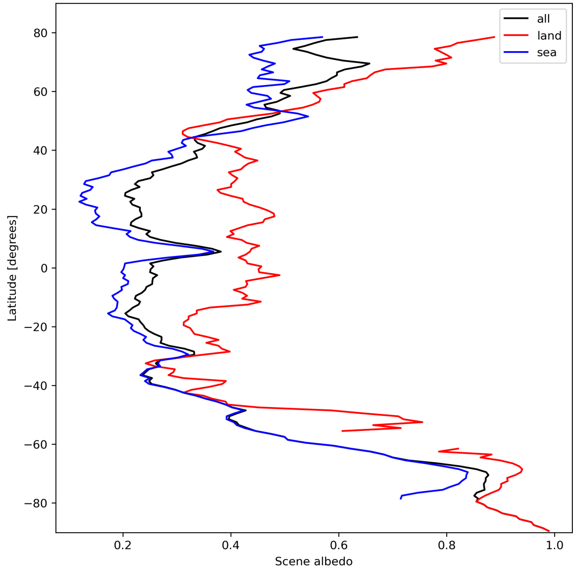
Figure 17: Zonal average of “Scene albedo” for 2023-10-17 to 2023-10-18.
