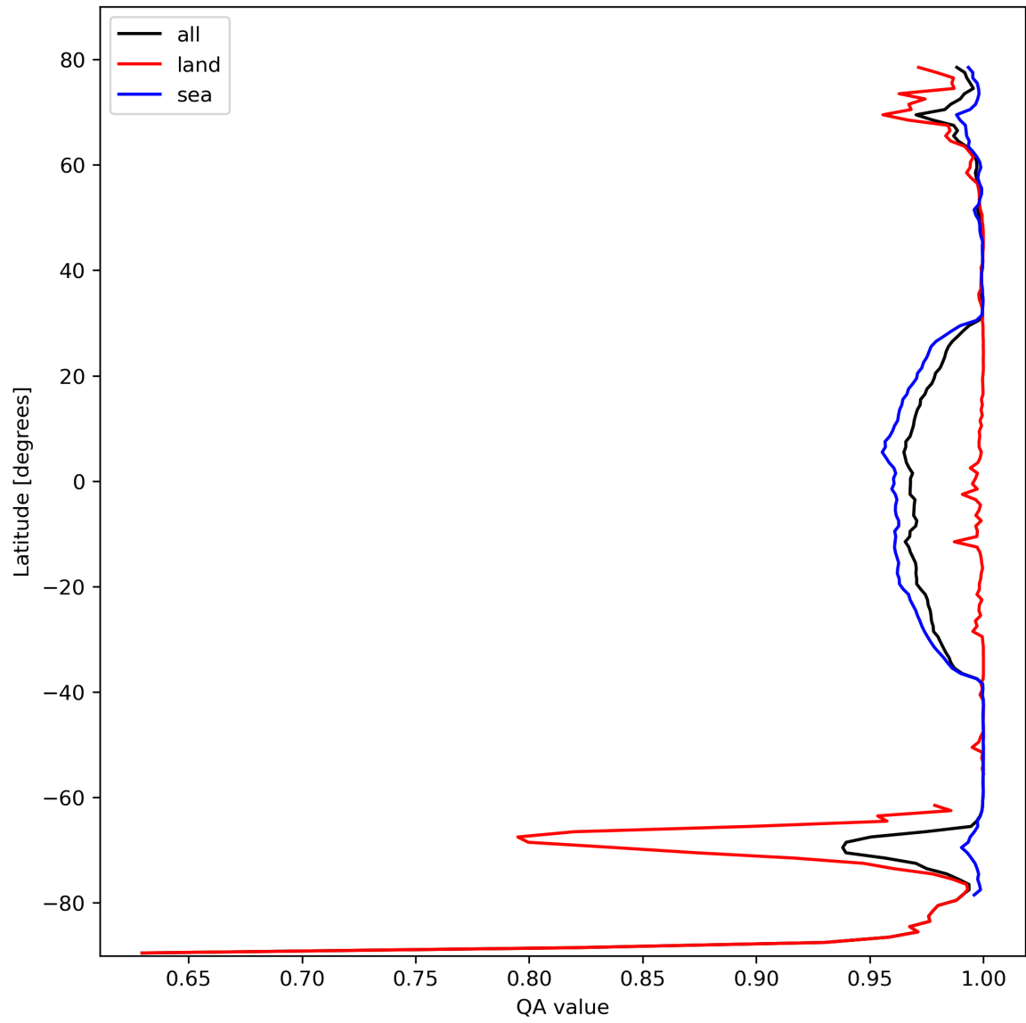
Figure 12: Zonal average of “QA value” for 2023-10-17 to 2023-10-18.
