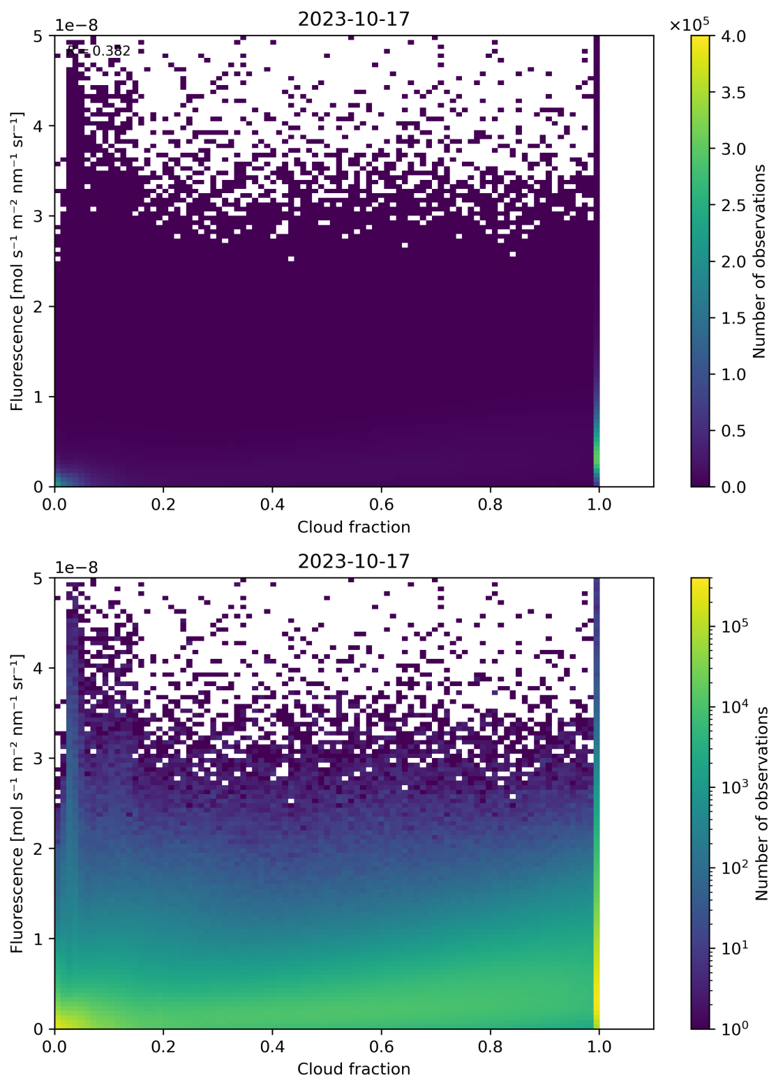
Figure 79: Scatter density plot of “Cloud fraction” against “Fluorescence” for 2023-10-17 to 2023-10-18.
