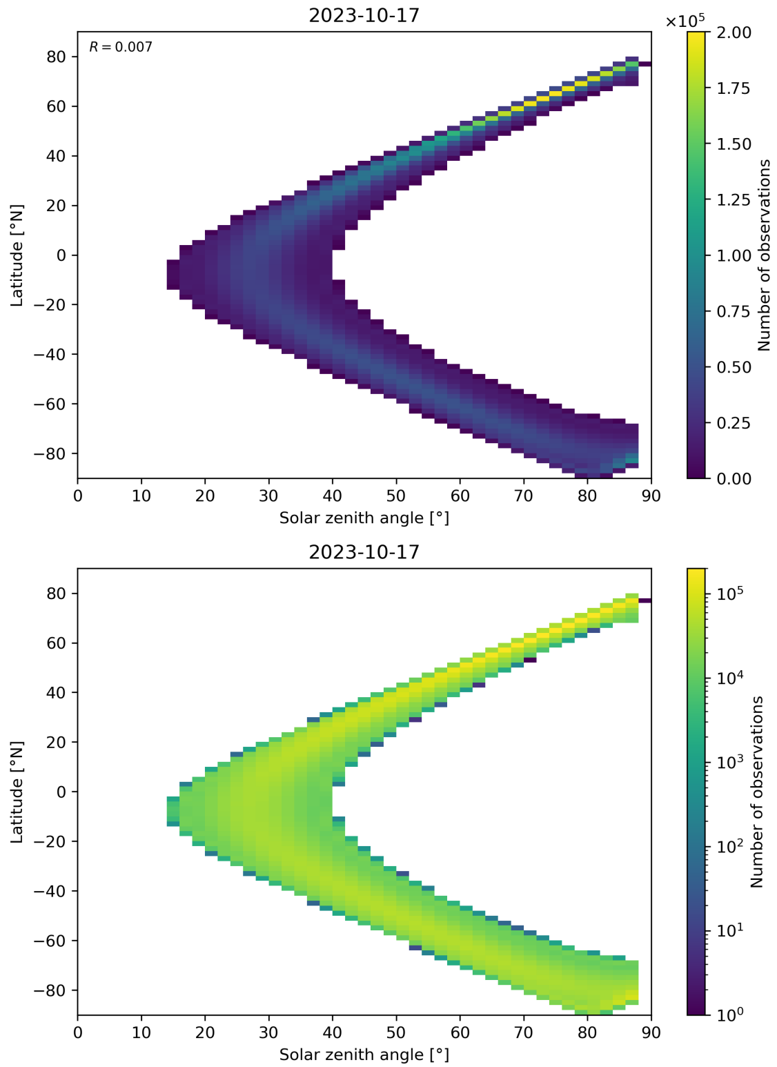
Figure 124: Scatter density plot of “Solar zenith angle” against “Latitude” for 2023-10-17 to 2023-10-18.
