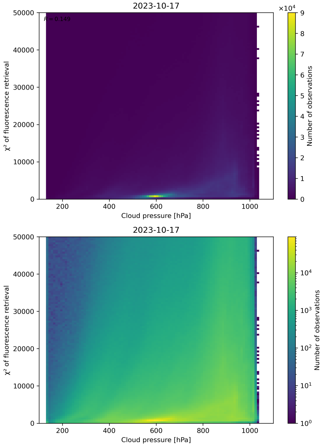
Figure 86: Scatter density plot of “Cloud pressure” against “ \chi^2 of fluorescence retrieval” for 2023-10-17 to 2023-10-18.
