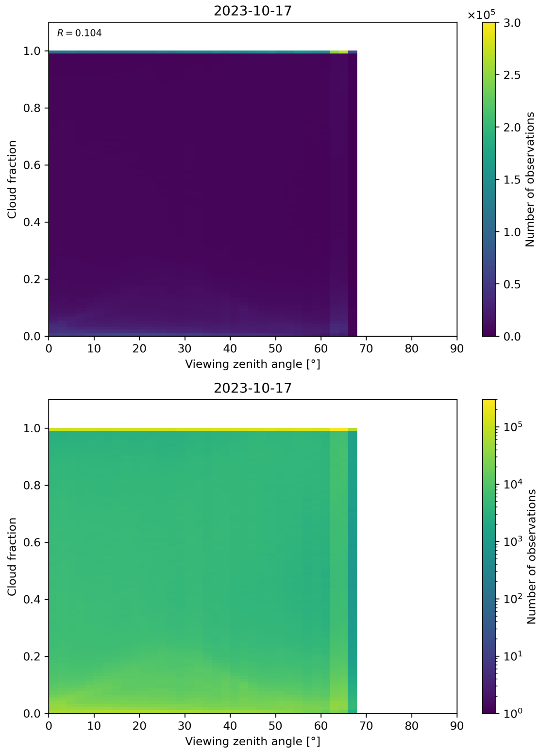
Figure 132: Scatter density plot of “Viewing zenith angle” against “Cloud fraction” for 2023-10-17 to 2023-10-18.
