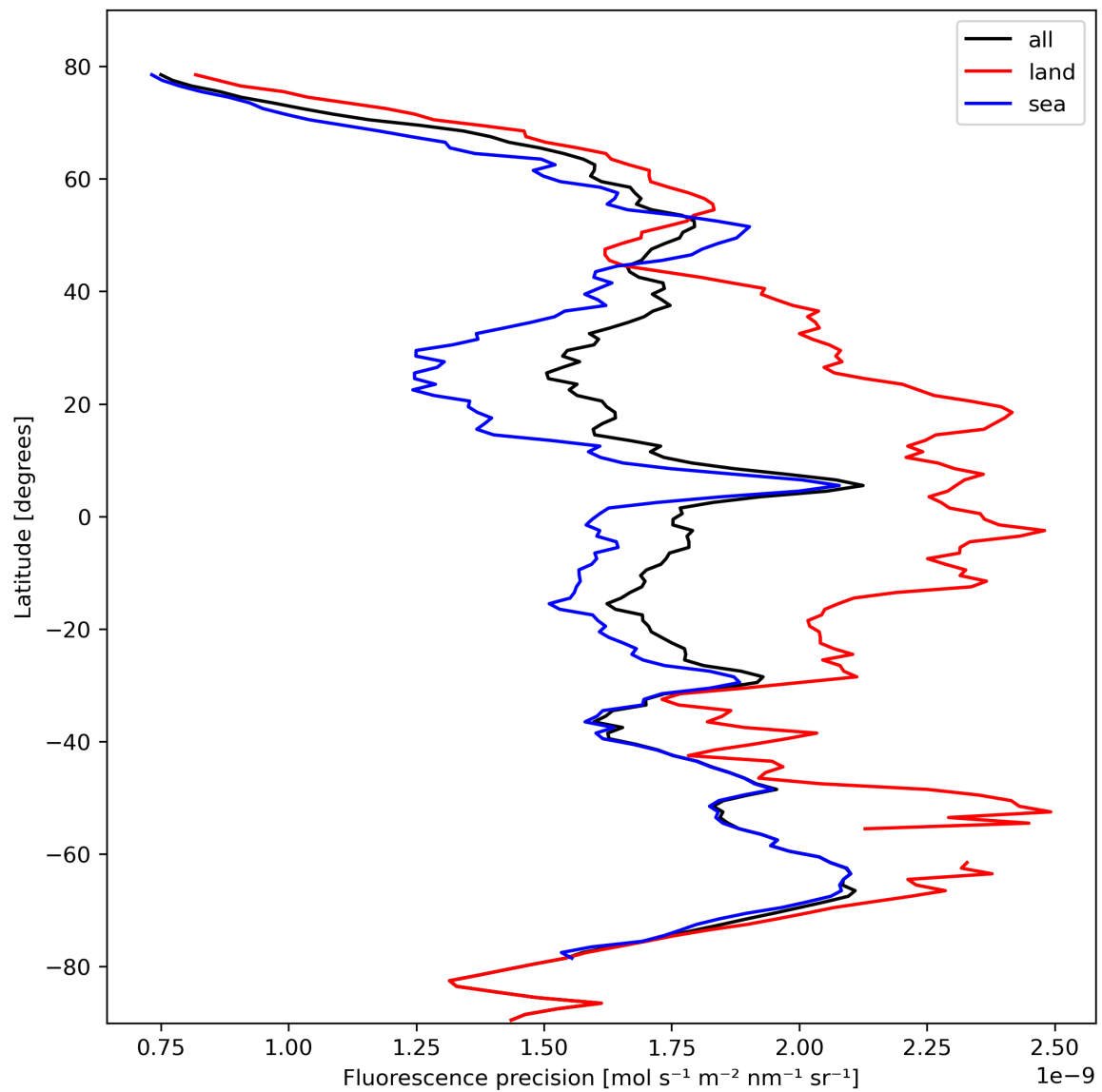
Figure 24: Zonal average of “Fluorescence precision” for 2023-10-17 to 2023-10-18.
