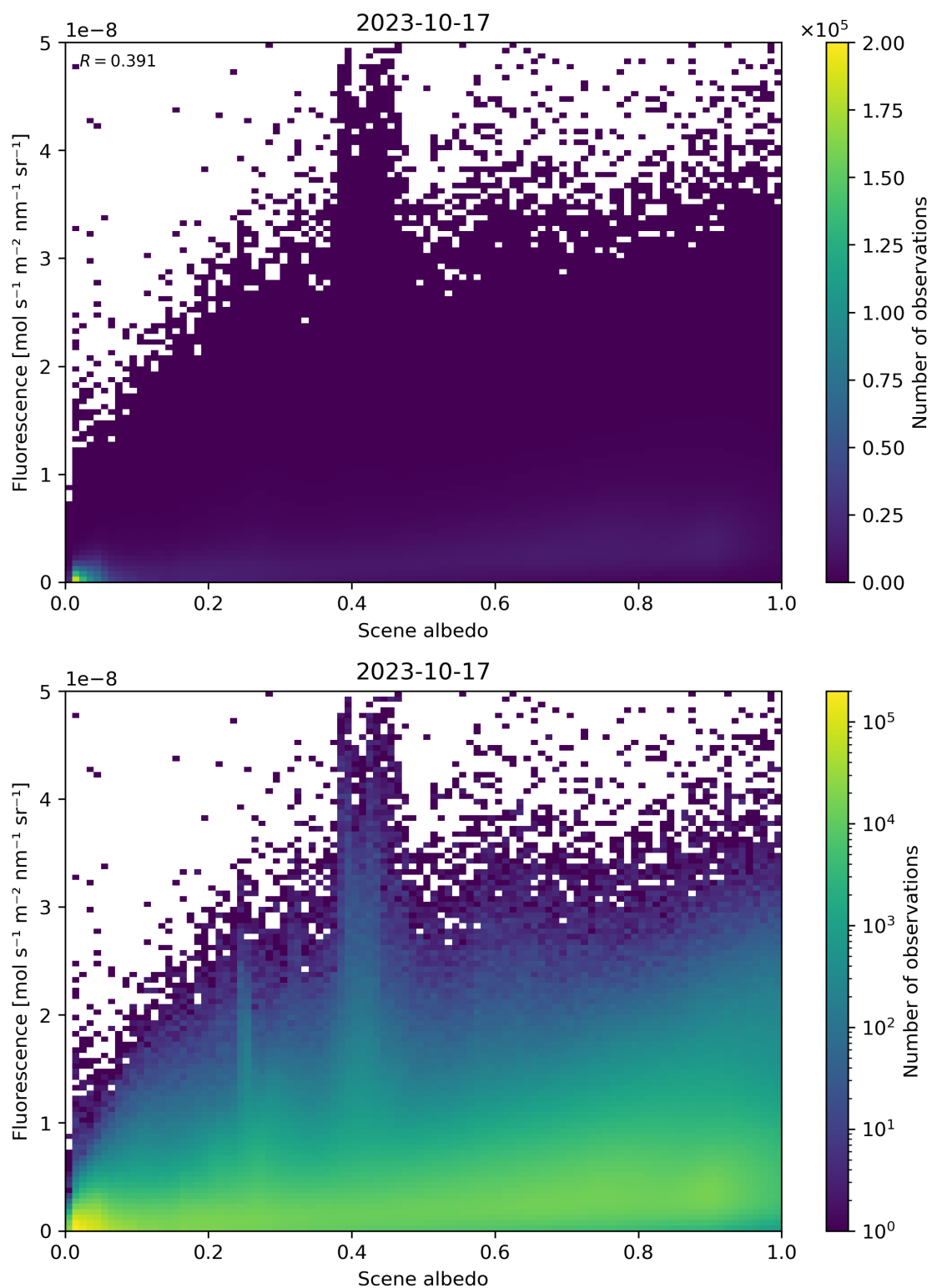
Figure 114: Scatter density plot of “Scene albedo” against “Fluorescence” for 2023-10-17 to 2023-10-18.
