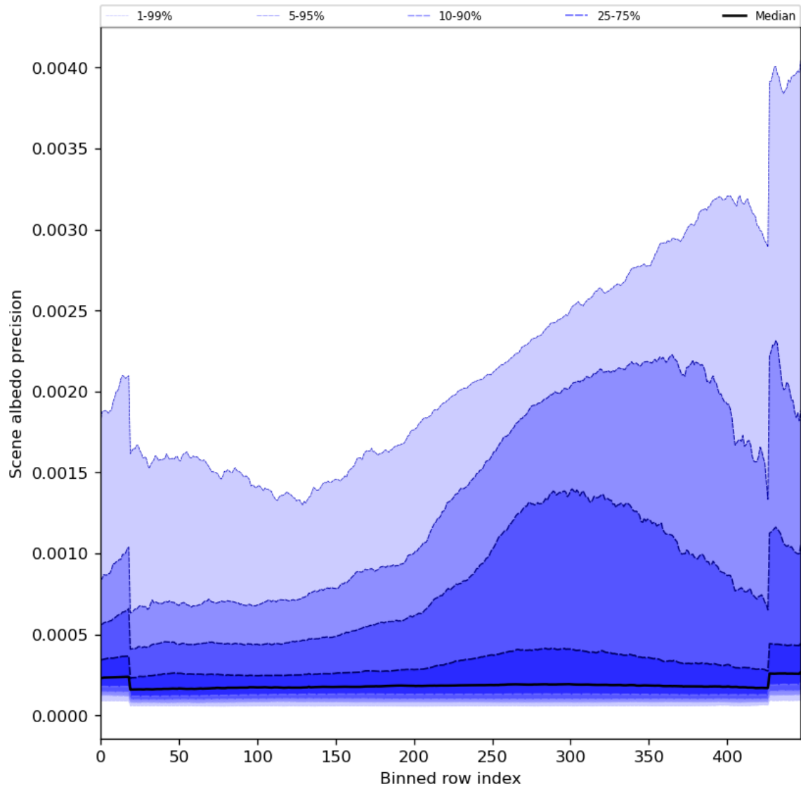
Figure 52: Along track statistics of “Scene albedo precision” for 2023-10-17 to 2023-10-18
