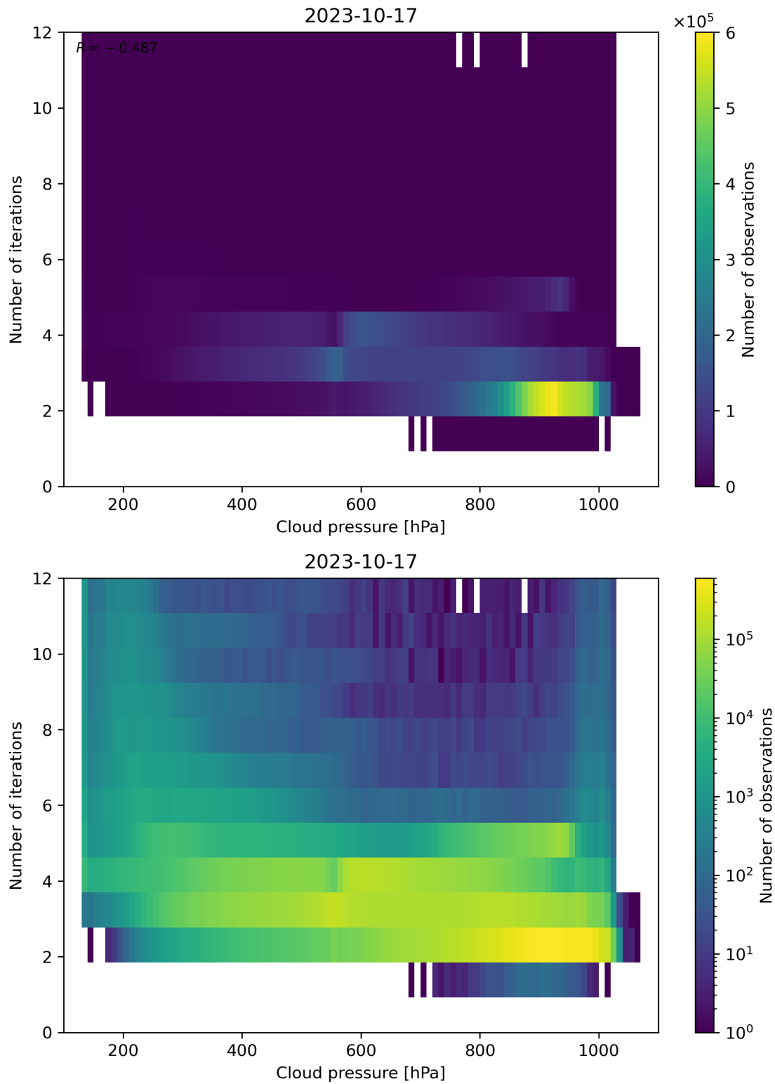
Figure 89: Scatter density plot of “Cloud pressure” against “Number of iterations” for 2023-10-17 to 2023-10-18.
