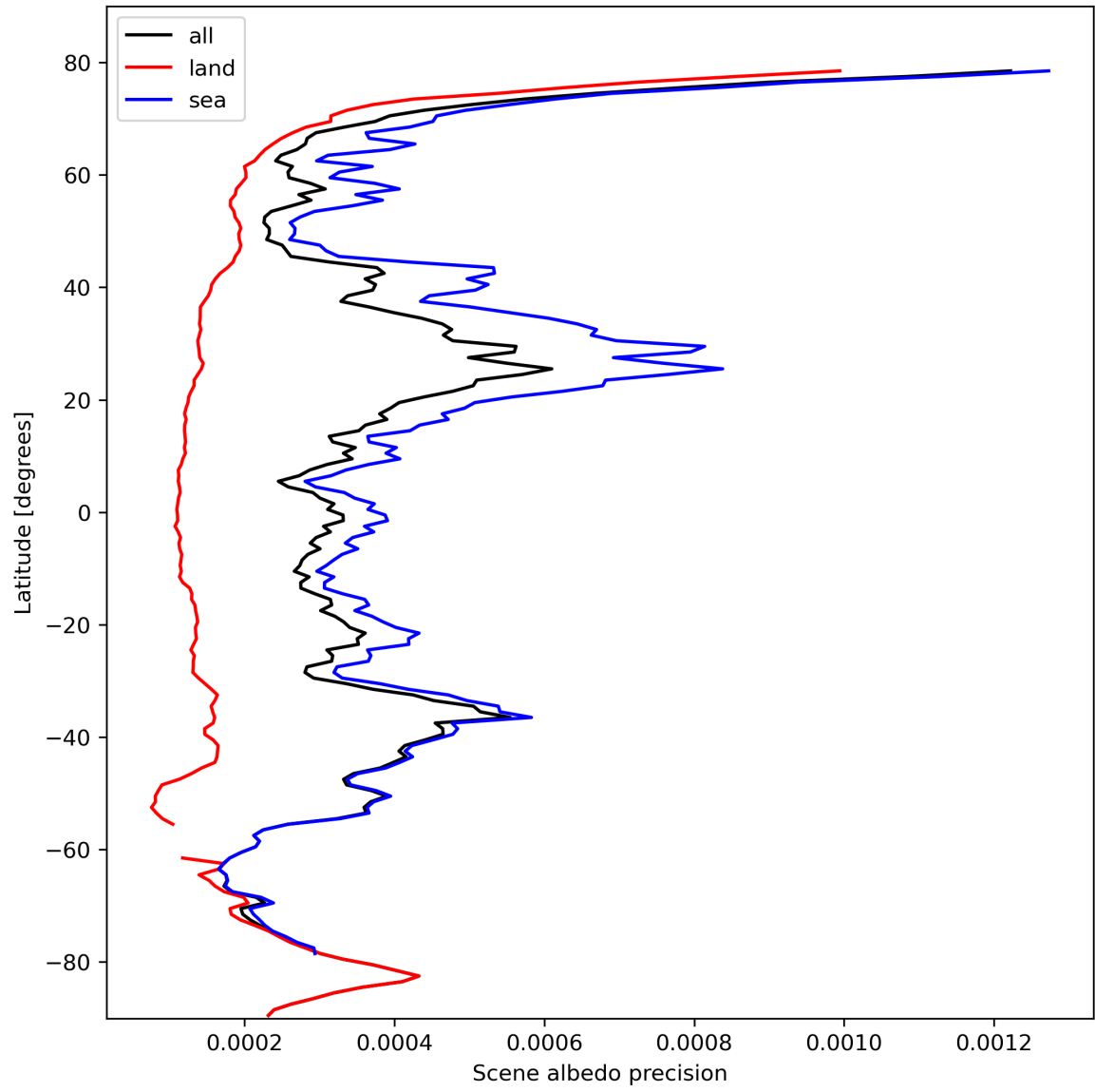
Figure 18: Zonal average of “Scene albedo precision” for 2023-10-17 to 2023-10-18.
