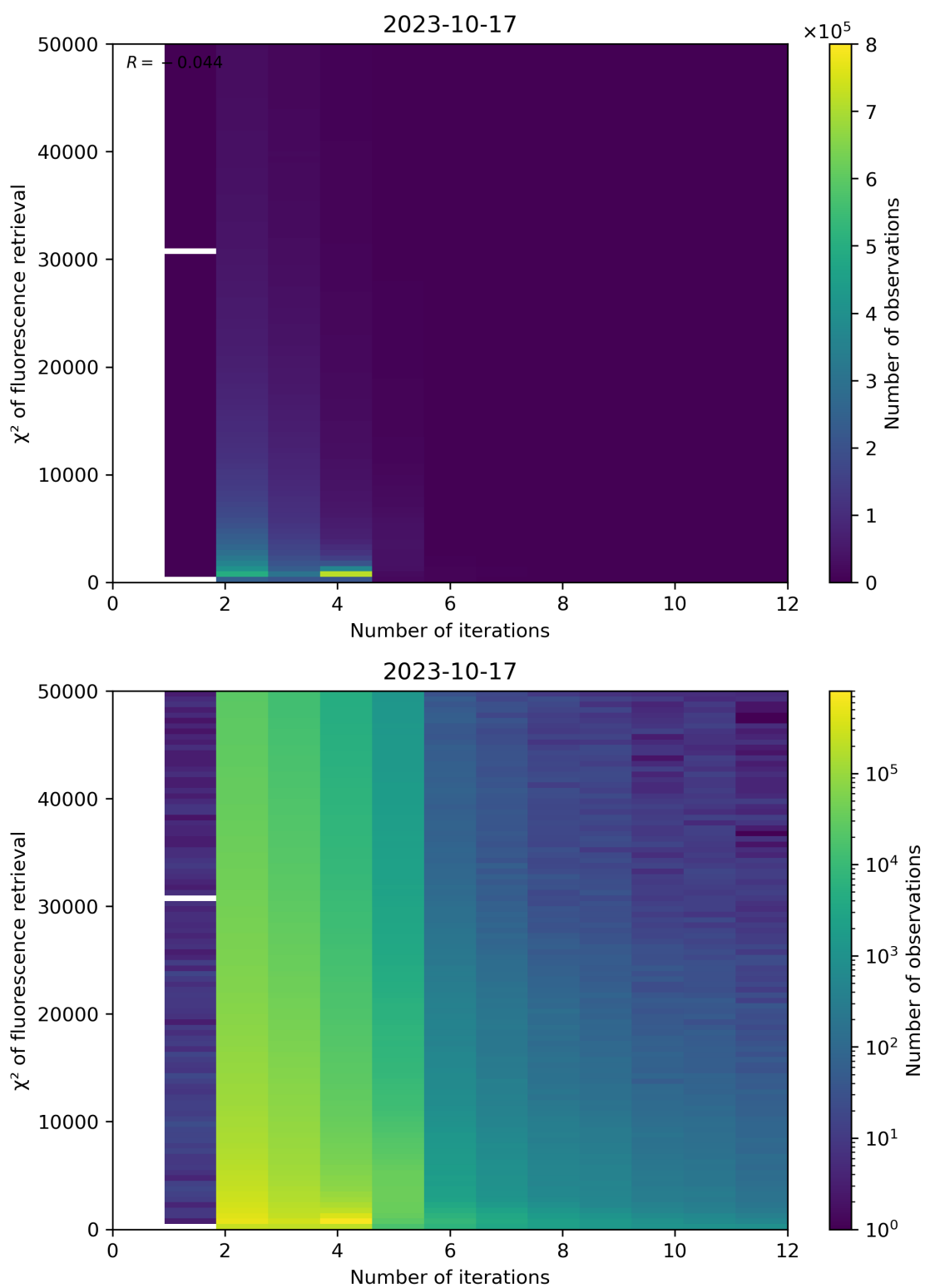
Figure 106: Scatter density plot of “Number of iterations” against “ \chi^2 of fluorescence retrieval” for 2023-10-17 to 2023-10-18.
