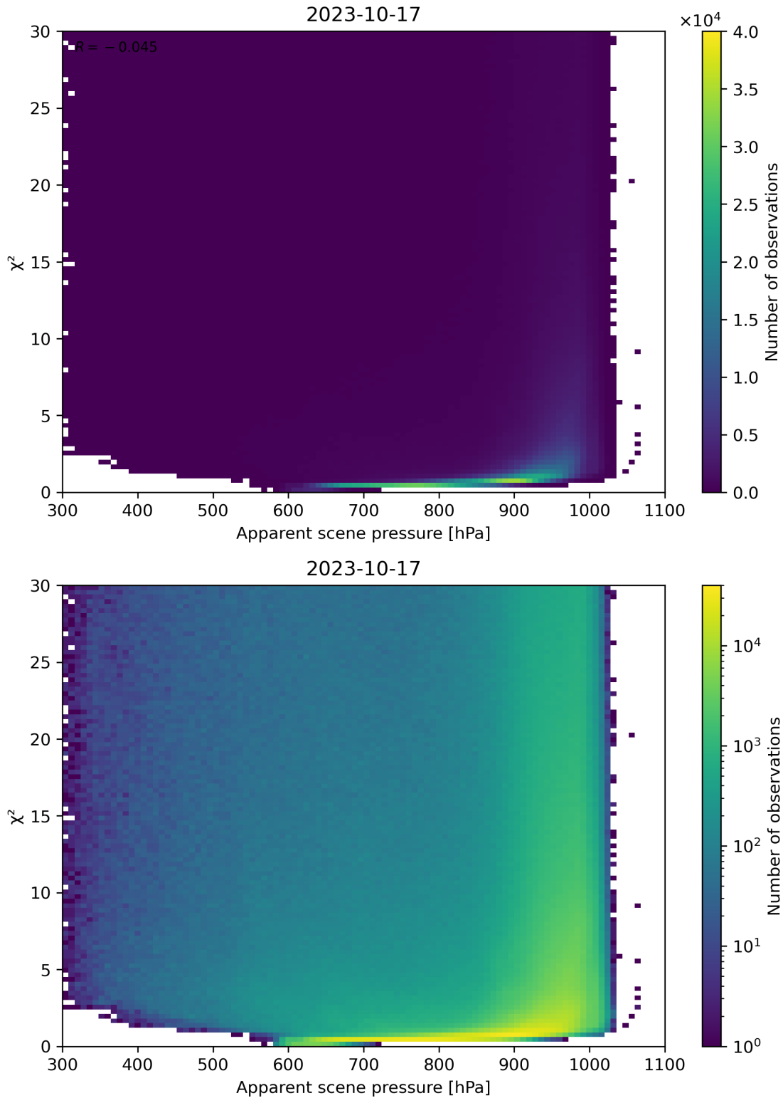
Figure 63: Scatter density plot of “Apparent scene pressure” against “ \chi^2 ” for 2023-10-17 to 2023-10-18.
