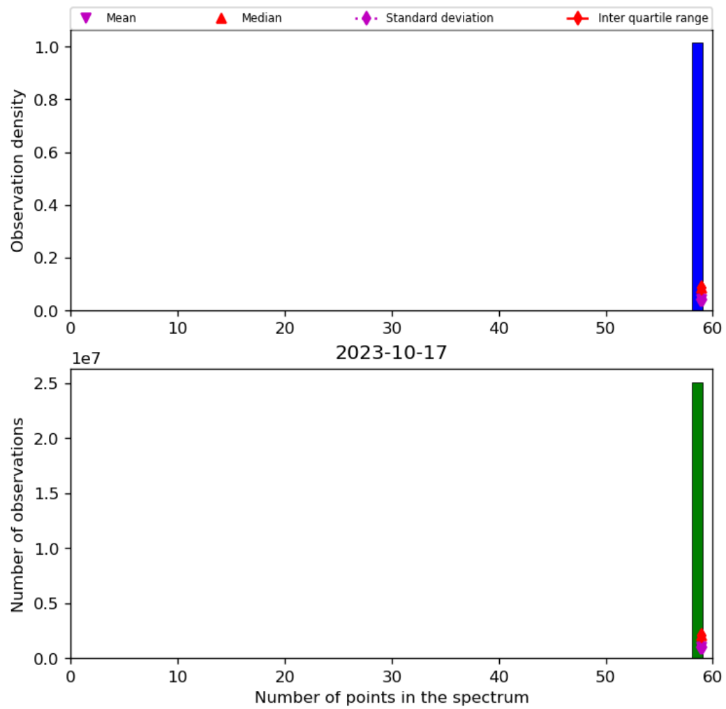
Figure 44: Histogram of “Number of points in the spectrum” for 2023-10-17 to 2023-10-18
