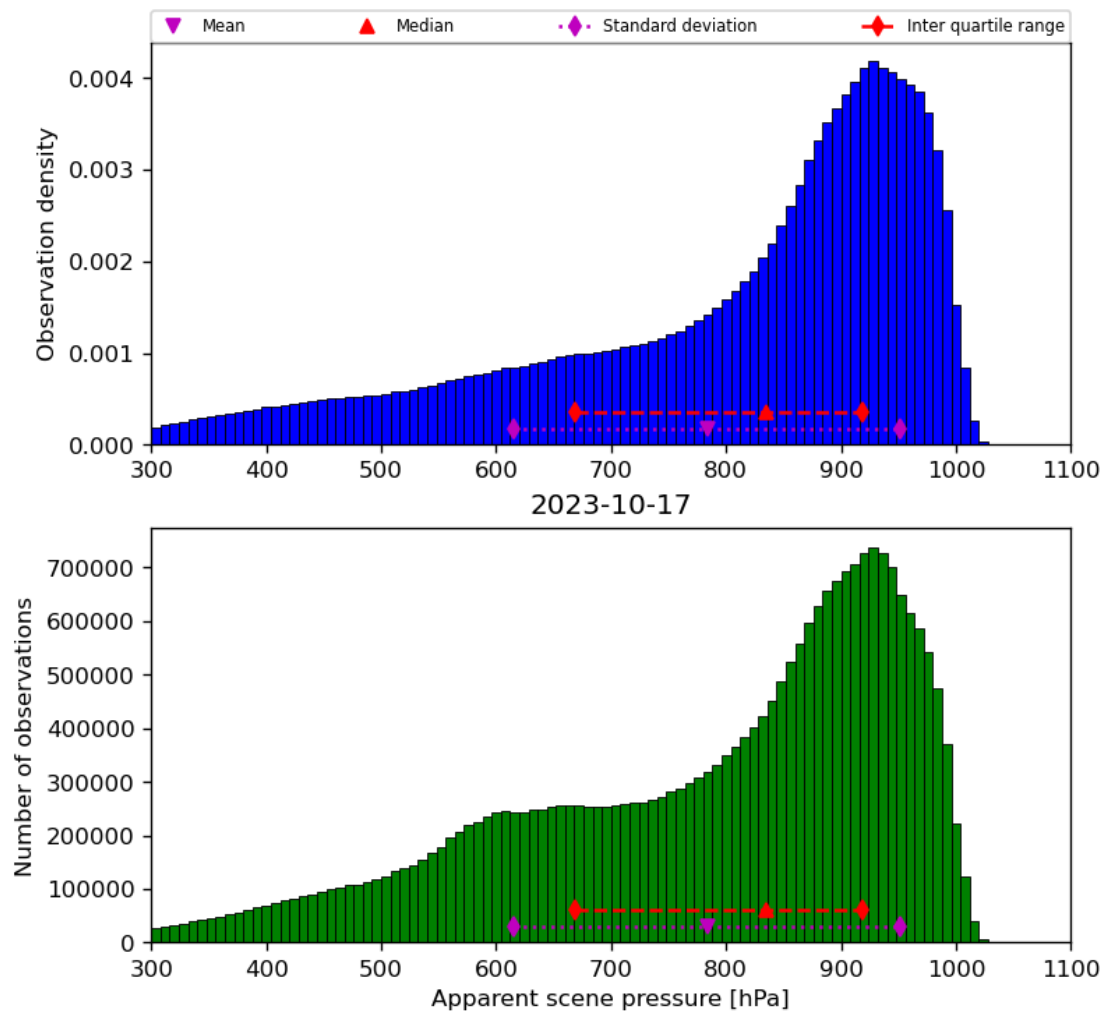
Figure 36: Histogram of “Apparent scene pressure” for 2023-10-17 to 2023-10-18
