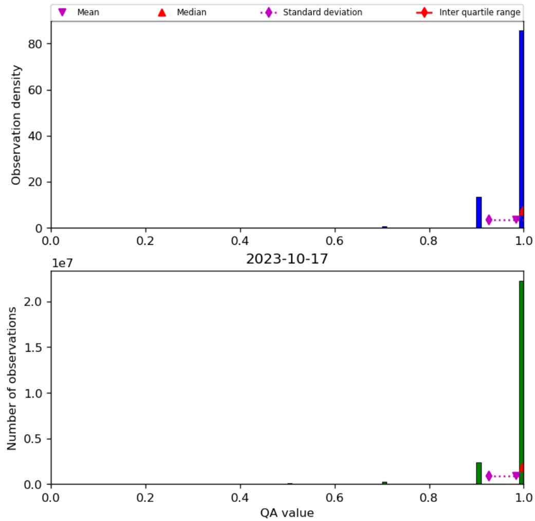
Figure 29: Histogram of “QA value” for 2023-10-17 to 2023-10-18
