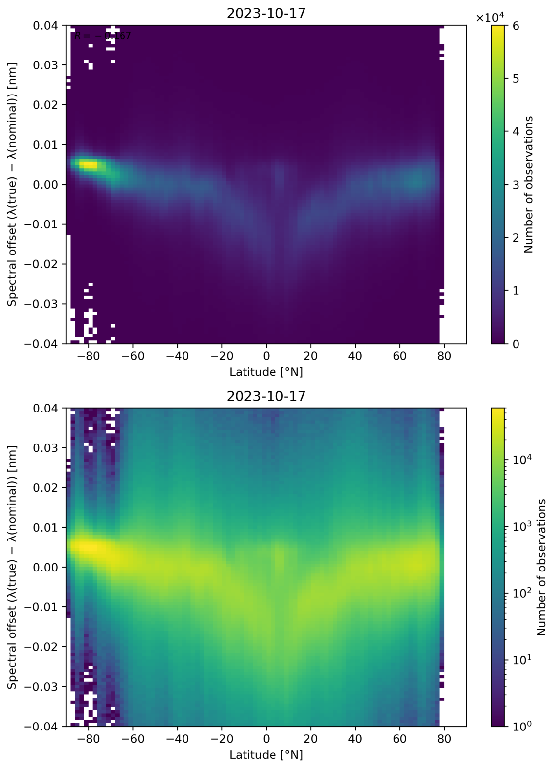
Figure 105: Scatter density plot of “Latitude” against “Spectral offset ( \lambda(\text{true}) - \lambda(\text{nominal}) )” for 2023-10-17 to 2023-10-18.
