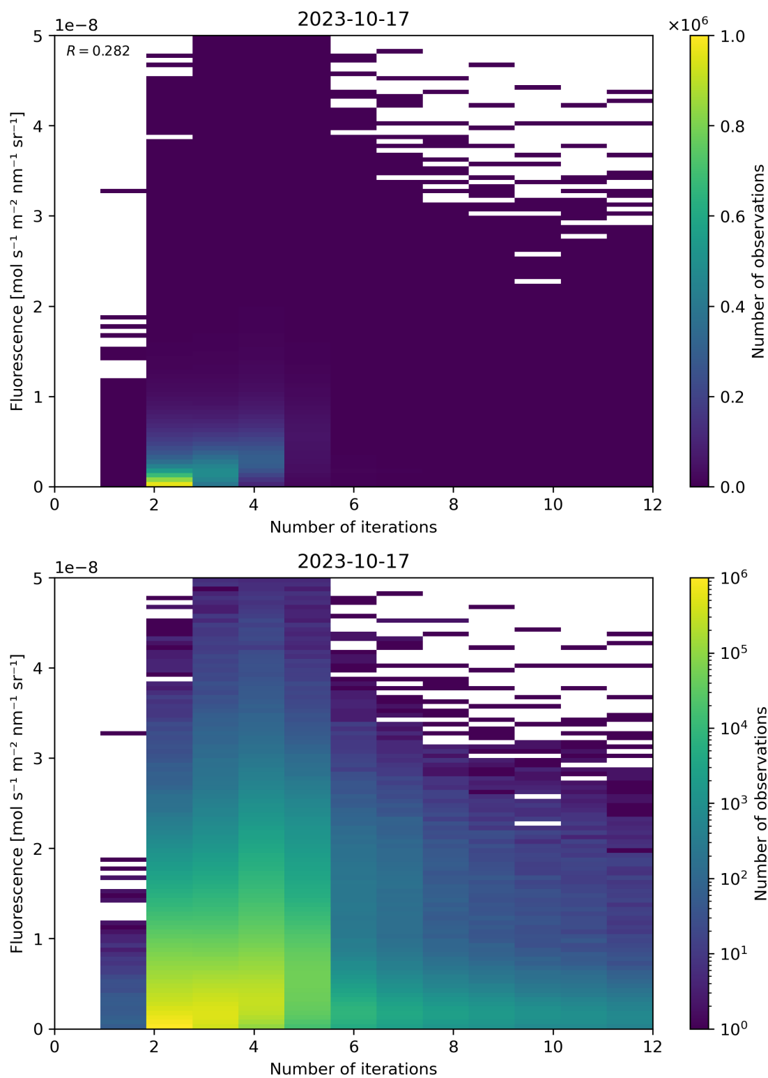
Figure 107: Scatter density plot of “Number of iterations” against “Fluorescence” for 2023-10-17 to 2023-10-18.
