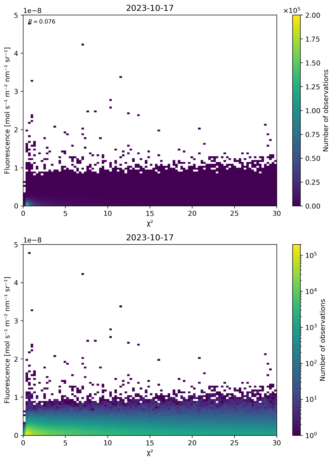
Figure 70: Scatter density plot of “ \chi^2 ” against “Fluorescence” for 2023-10-17 to 2023-10-18.
