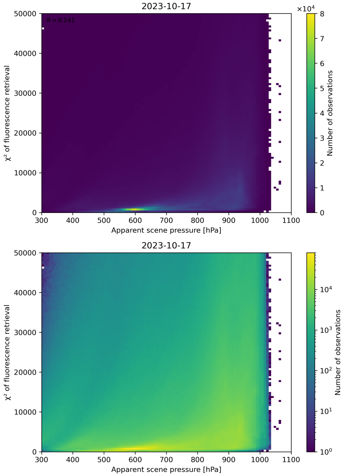
Figure 64: Scatter density plot of “Apparent scene pressure” against “ \chi^2 of fluorescence retrieval” for 2023-10-17 to 2023-10-18.
