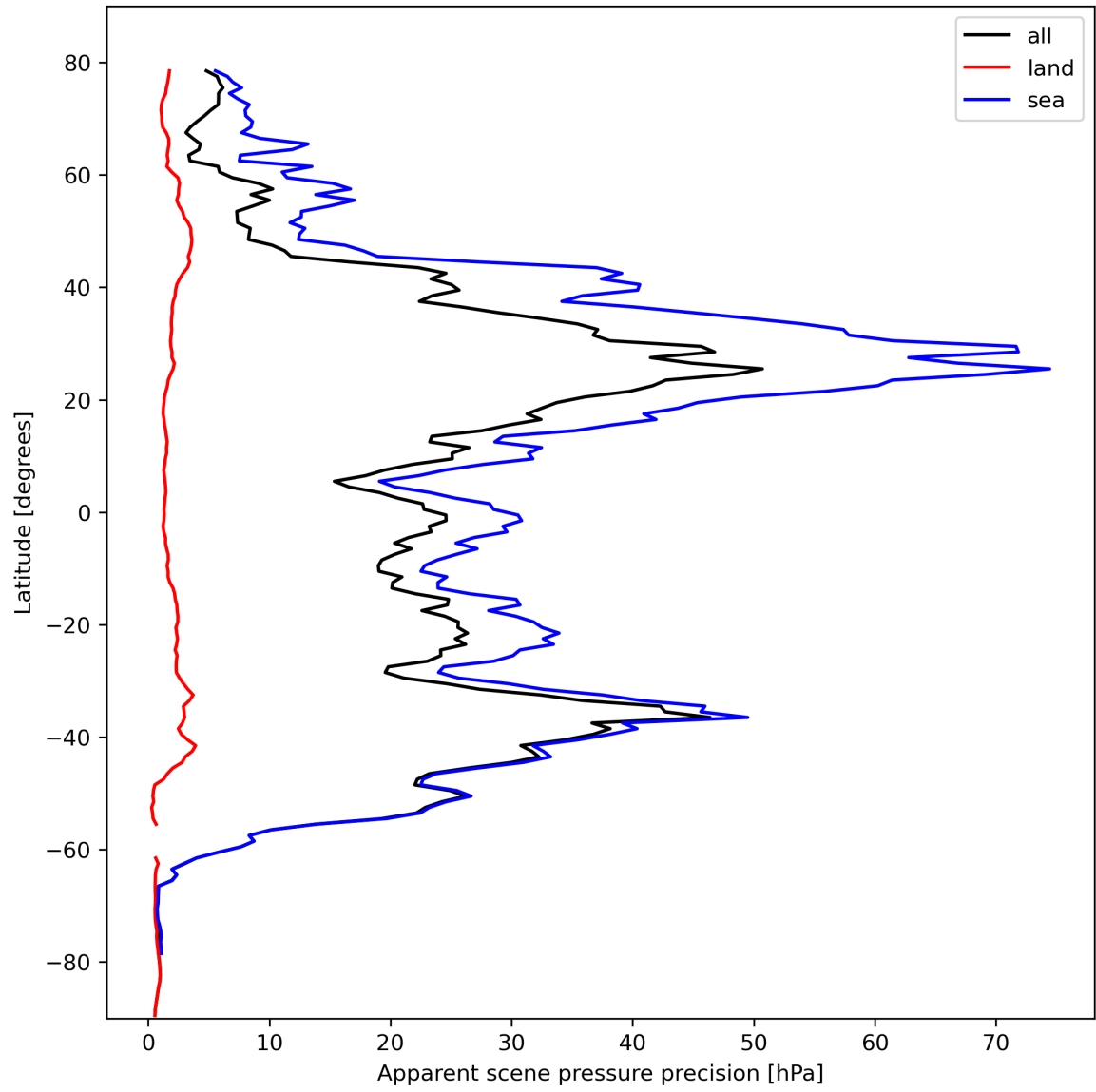
Figure 20: Zonal average of “Apparent scene pressure precision” for 2023-10-17 to 2023-10-18.
