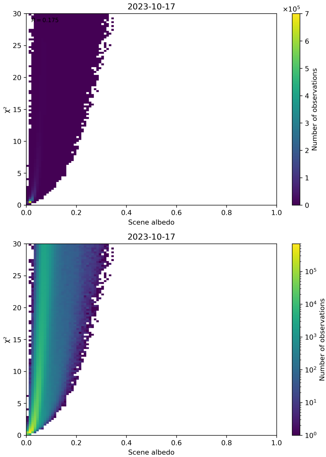
Figure 112: Scatter density plot of “Scene albedo” against “ \chi^2 ” for 2023-10-17 to 2023-10-18.
