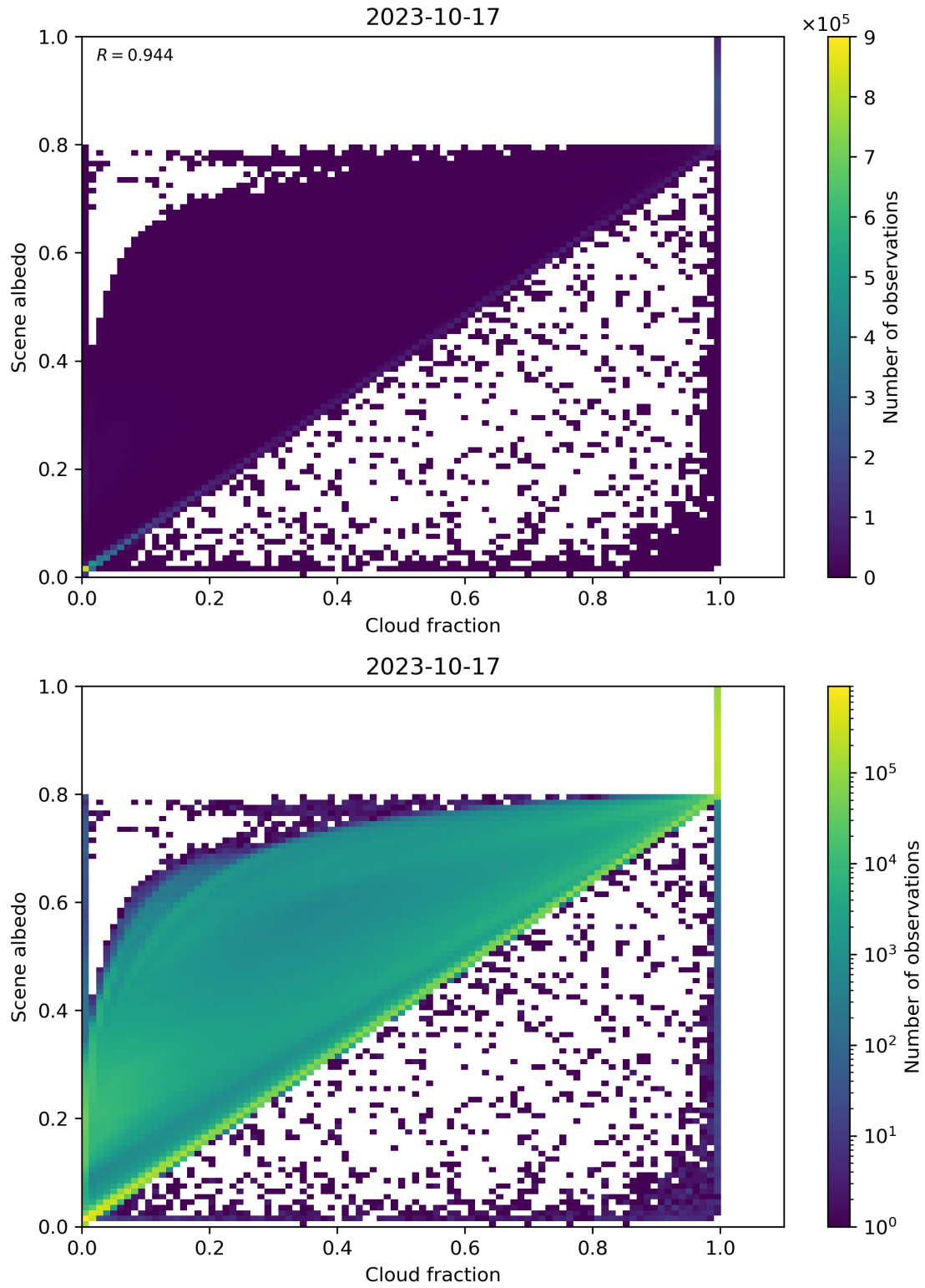
Figure 82: Scatter density plot of “Cloud fraction” against “Scene albedo” for 2023-10-17 to 2023-10-18.
