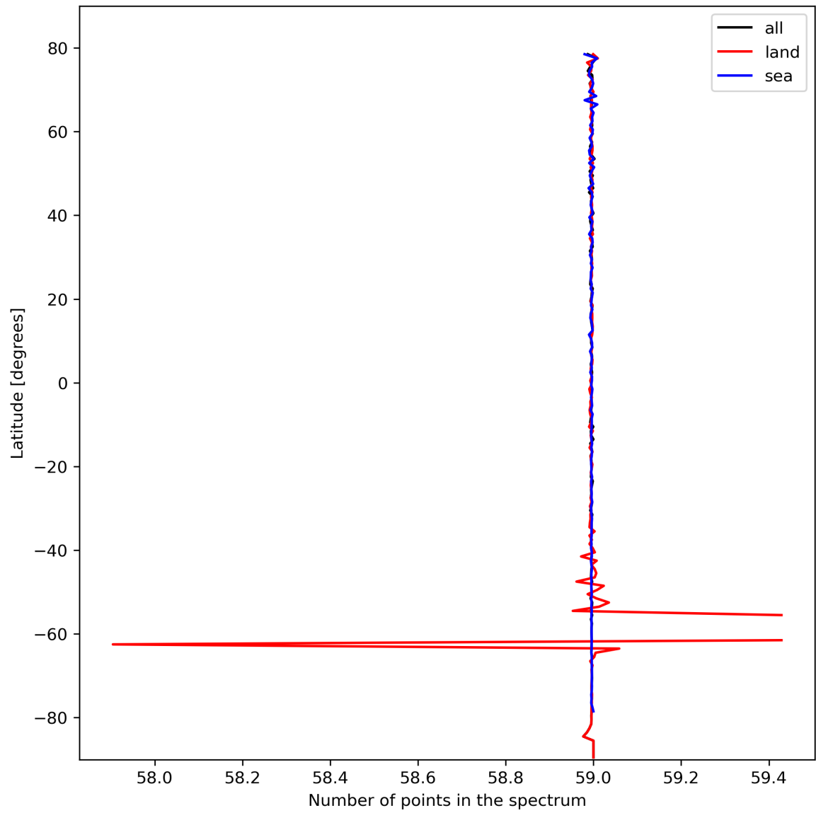
Figure 27: Zonal average of “Number of points in the spectrum” for 2023-10-17 to 2023-10-18.
