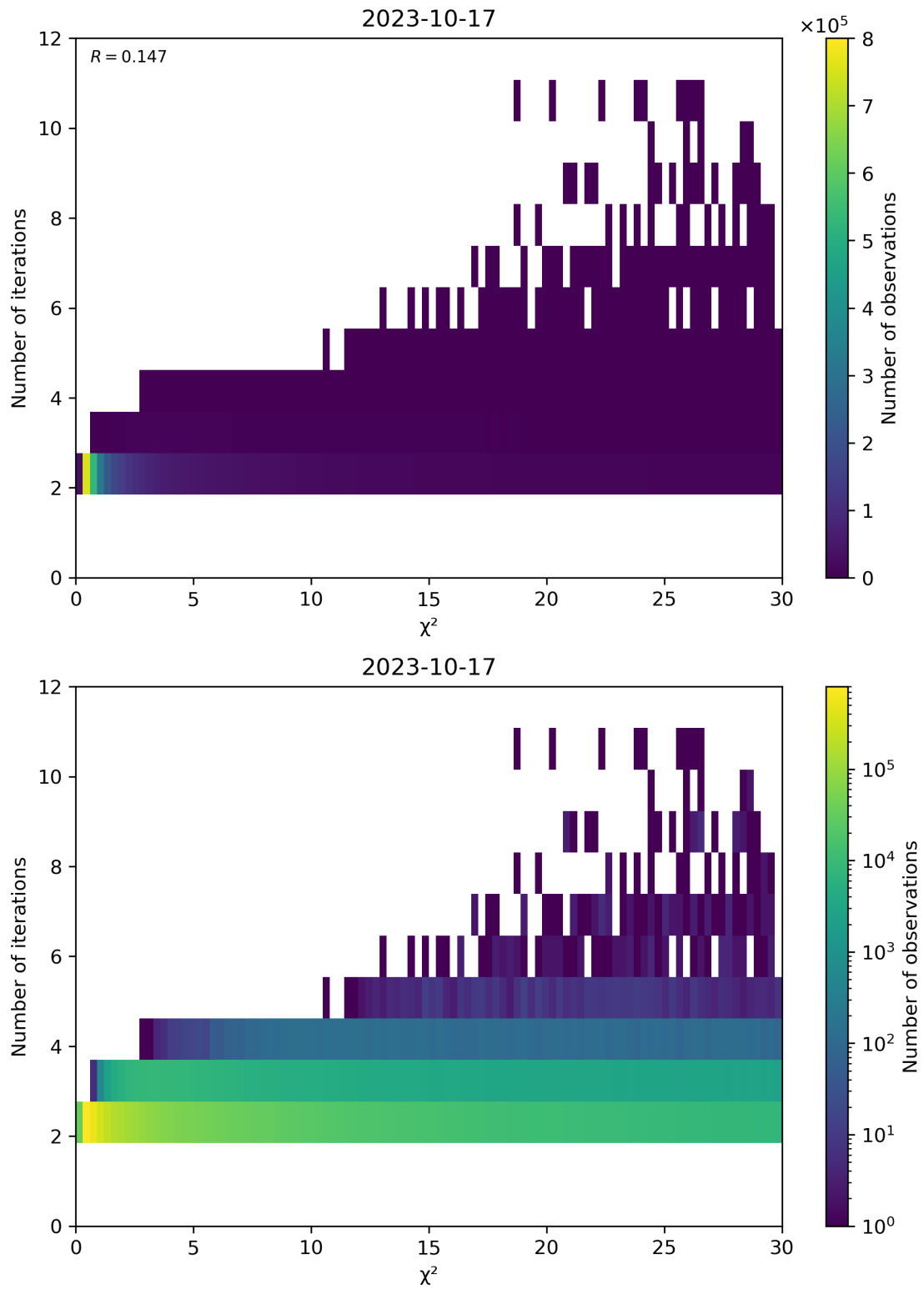
Figure 73: Scatter density plot of “ \chi^2 ” against “Number of iterations” for 2023-10-17 to 2023-10-18.
