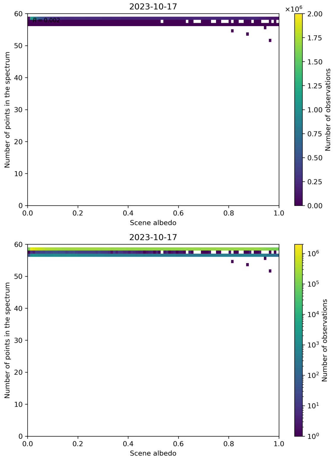
Figure 116: Scatter density plot of “Scene albedo” against “Number of points in the spectrum” for 2023-10-17 to 2023-10-18.
