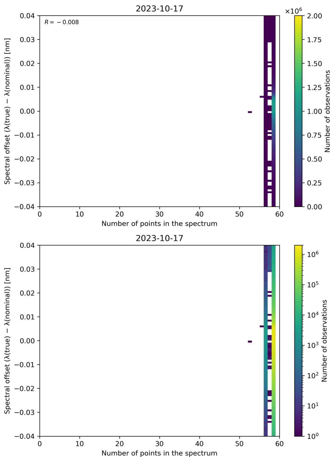
Figure 110: Scatter density plot of “Number of points in the spectrum” against “Spectral offset ( \lambda(\text{true}) - \lambda(\text{nominal}) )” for 2023-10-17 to 2023-10-18.
