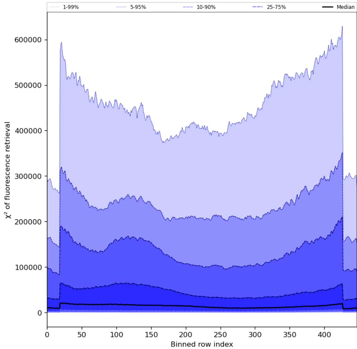
Figure 59: Along track statistics of “ \chi^2 of fluorescence retrieval” for 2023-10-17 to 2023-10-18
