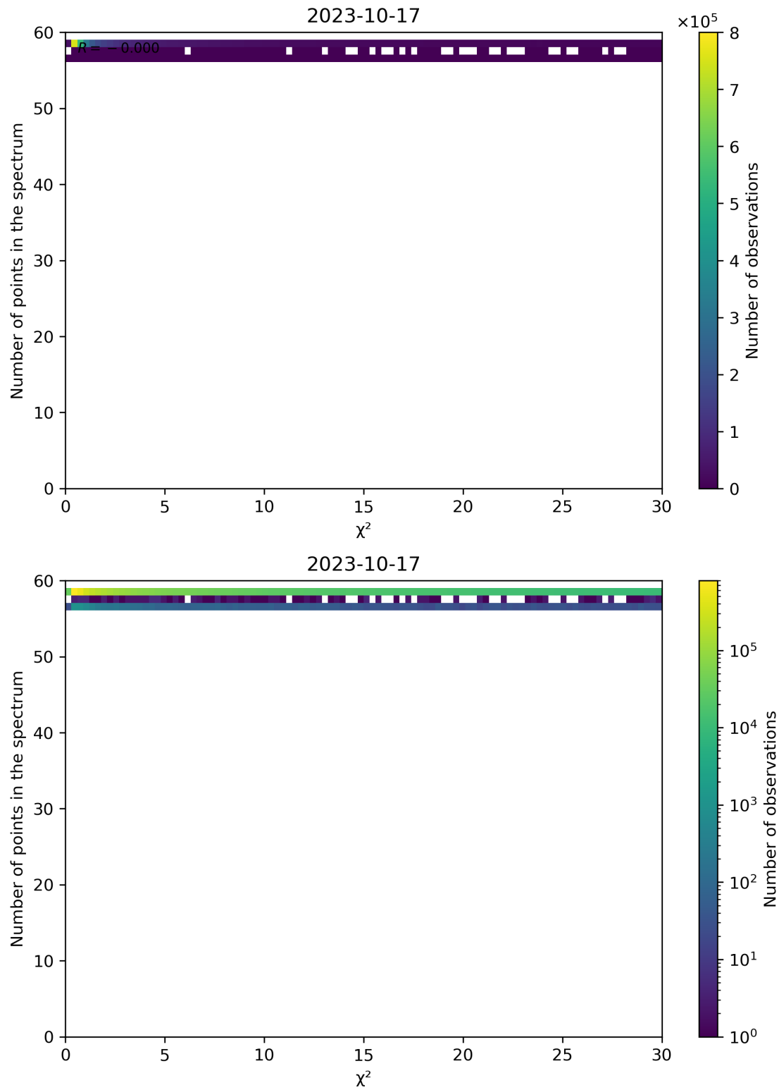
Figure 74: Scatter density plot of " \chi^2 " against "Number of points in the spectrum" for 2023-10-17 to 2023-10-18.
