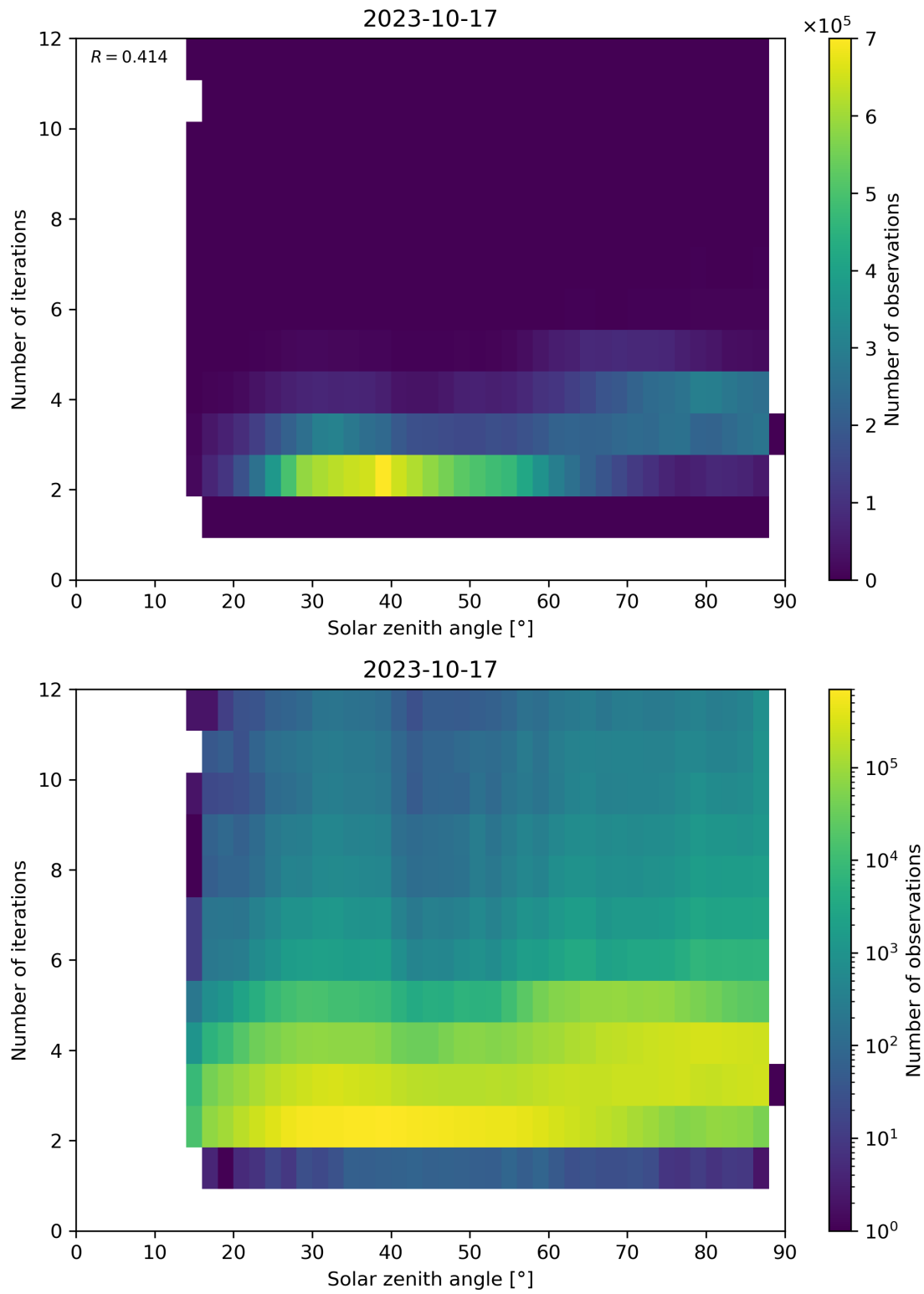
Figure 125: Scatter density plot of “Solar zenith angle” against “Number of iterations” for 2023-10-17 to 2023-10-18.
