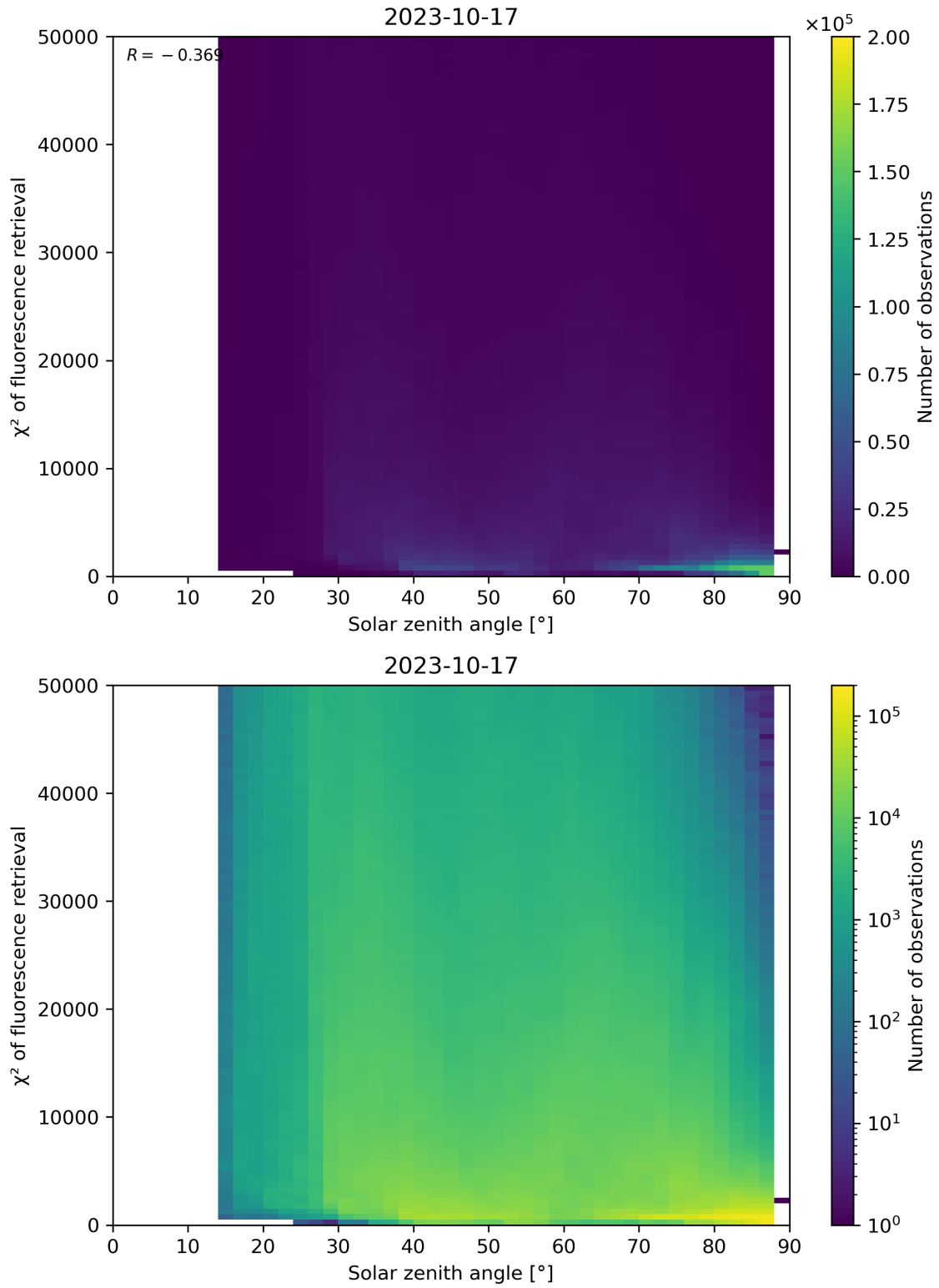
Figure 120: Scatter density plot of “Solar zenith angle” against “ \chi^2 of fluorescence retrieval” for 2023-10-17 to 2023-10-18.
