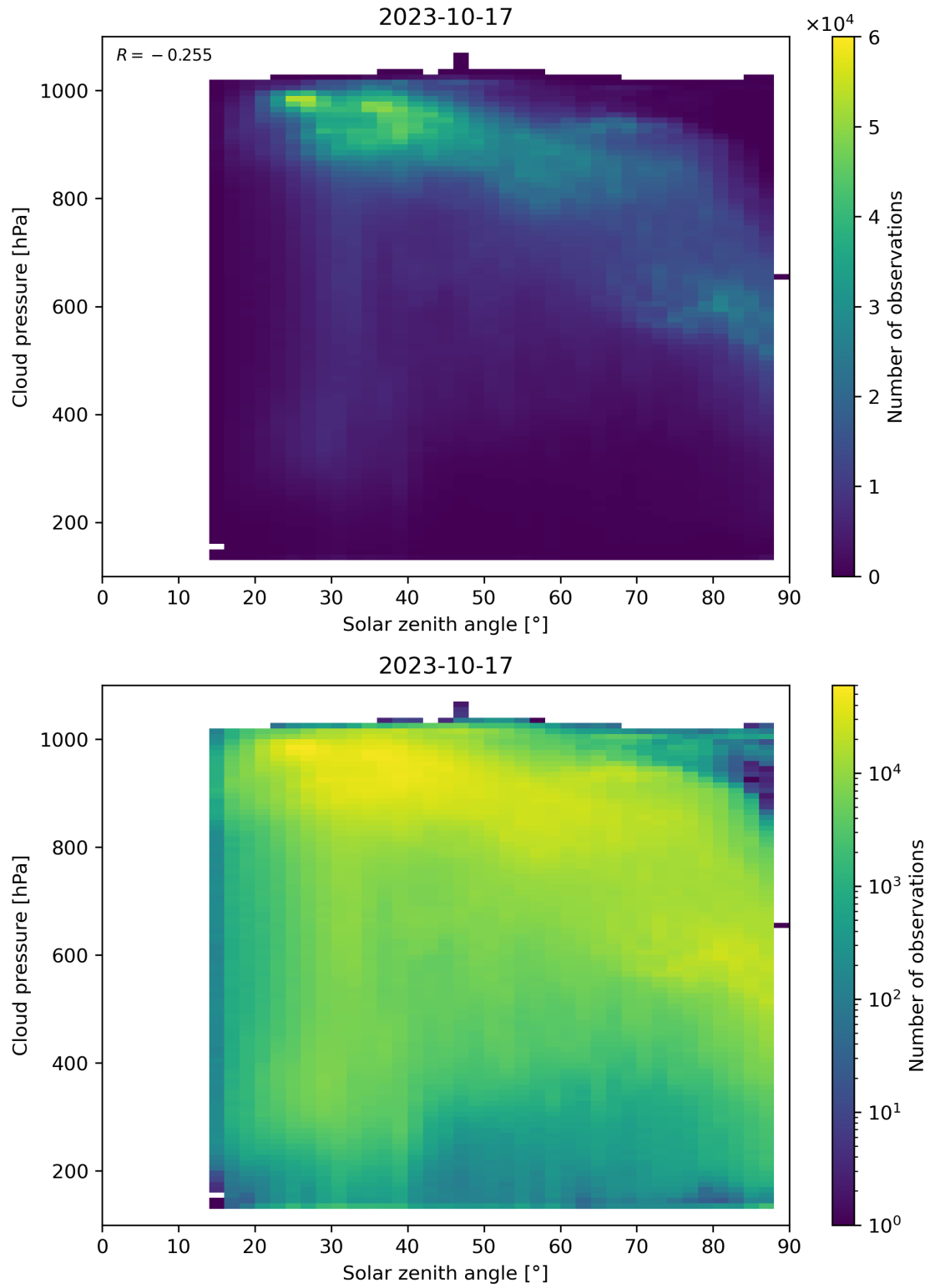
Figure 122: Scatter density plot of “Solar zenith angle” against “Cloud pressure” for 2023-10-17 to 2023-10-18.
