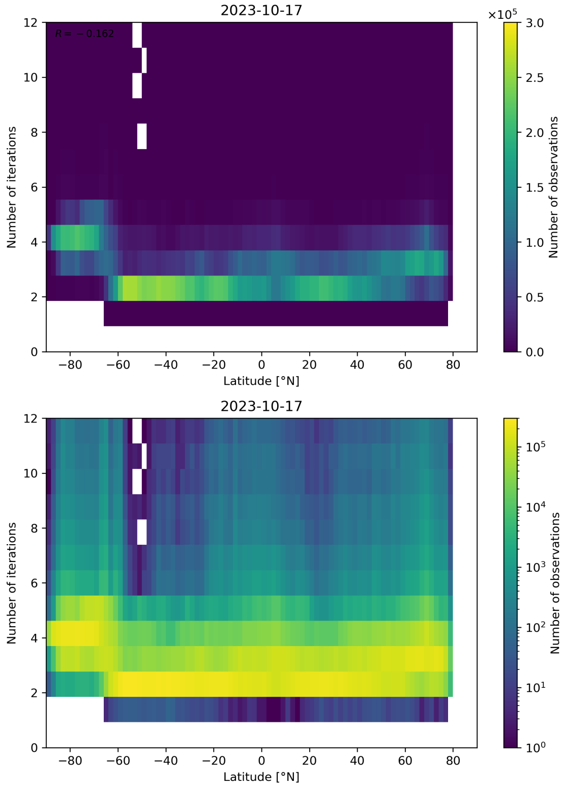
Figure 102: Scatter density plot of “Latitude” against “Number of iterations” for 2023-10-17 to 2023-10-18.
