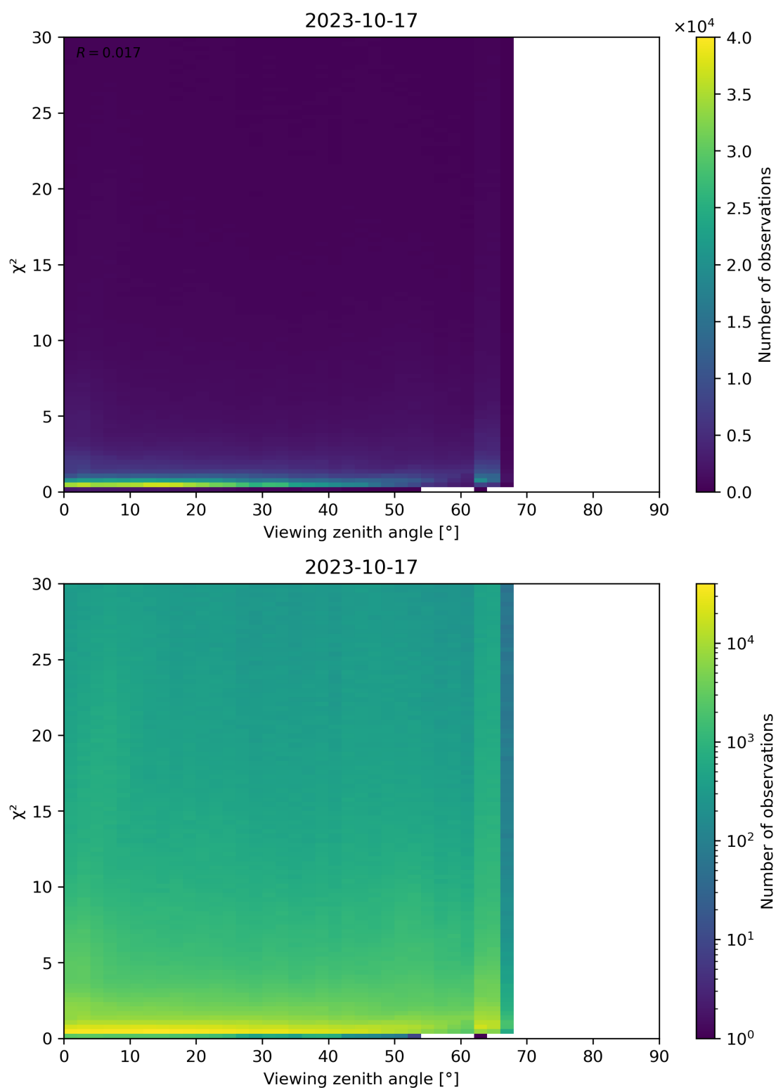
Figure 130: Scatter density plot of “Viewing zenith angle” against “ \chi^2 ” for 2023-10-17 to 2023-10-18.
