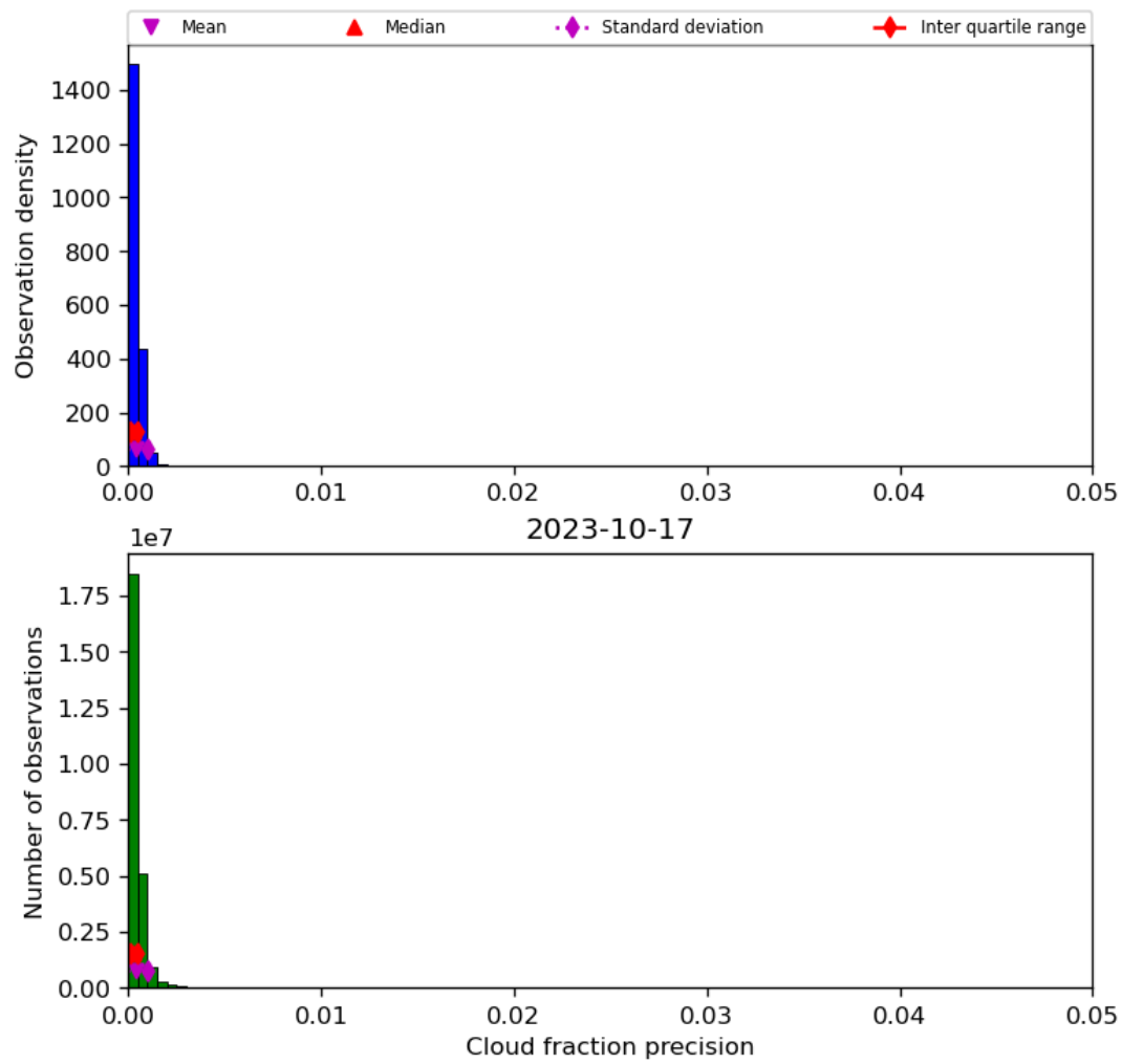
Figure 33: Histogram of “Cloud fraction precision” for 2023-10-17 to 2023-10-18
