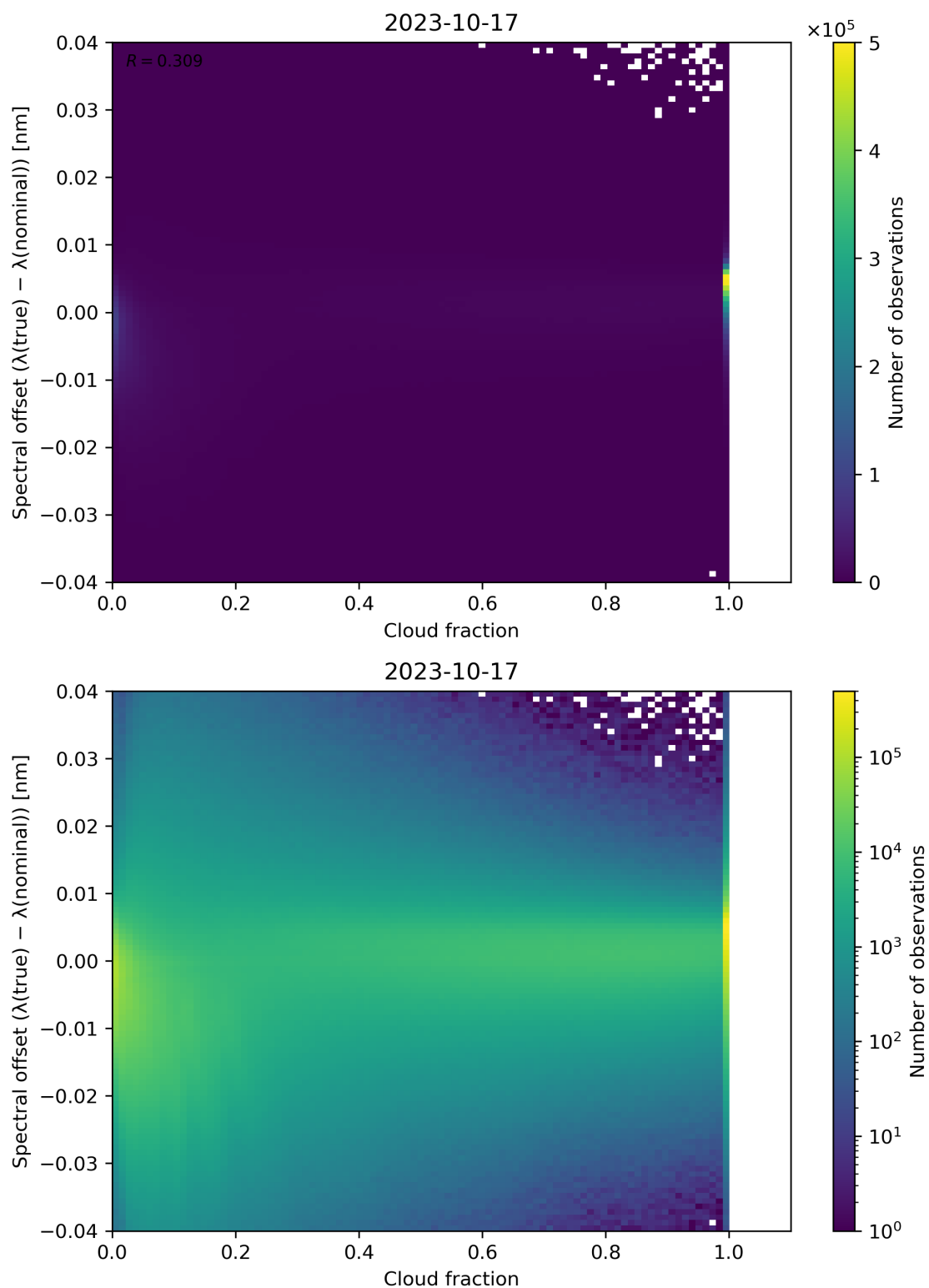
Figure 83: Scatter density plot of “Cloud fraction” against “Spectral offset ( \lambda(\text{true}) - \lambda(\text{nominal}) )” for 2023-10-17 to 2023-10-18.
