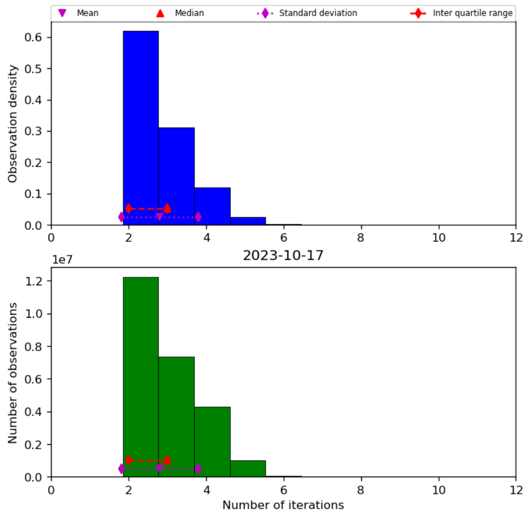
Figure 39: Histogram of “Number of iterations” for 2023-10-17 to 2023-10-18
