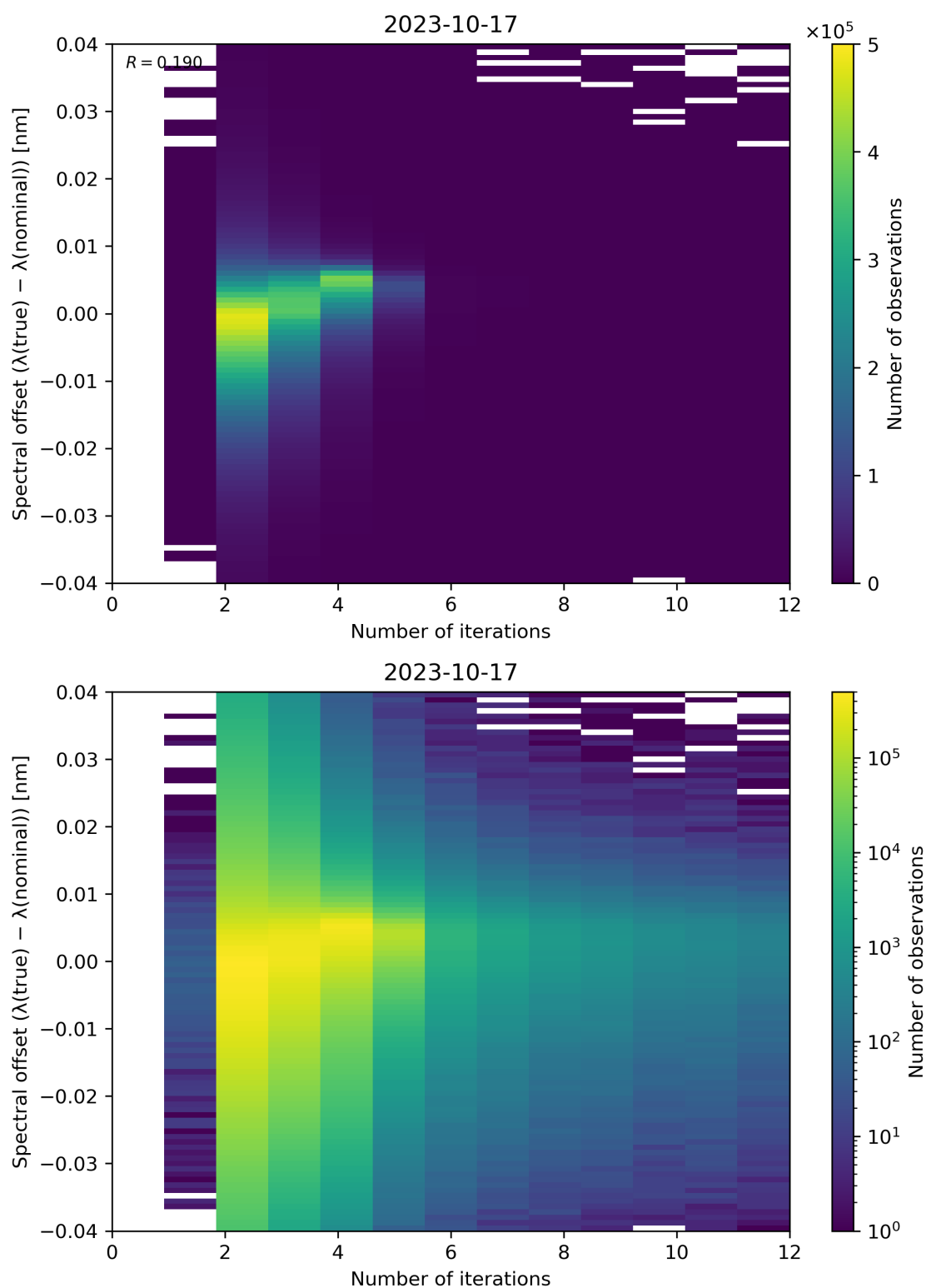
Figure 109: Scatter density plot of “Number of iterations” against “Spectral offset ( \lambda(\text{true}) - \lambda(\text{nominal}) )” for 2023-10-17 to 2023-10-18.
