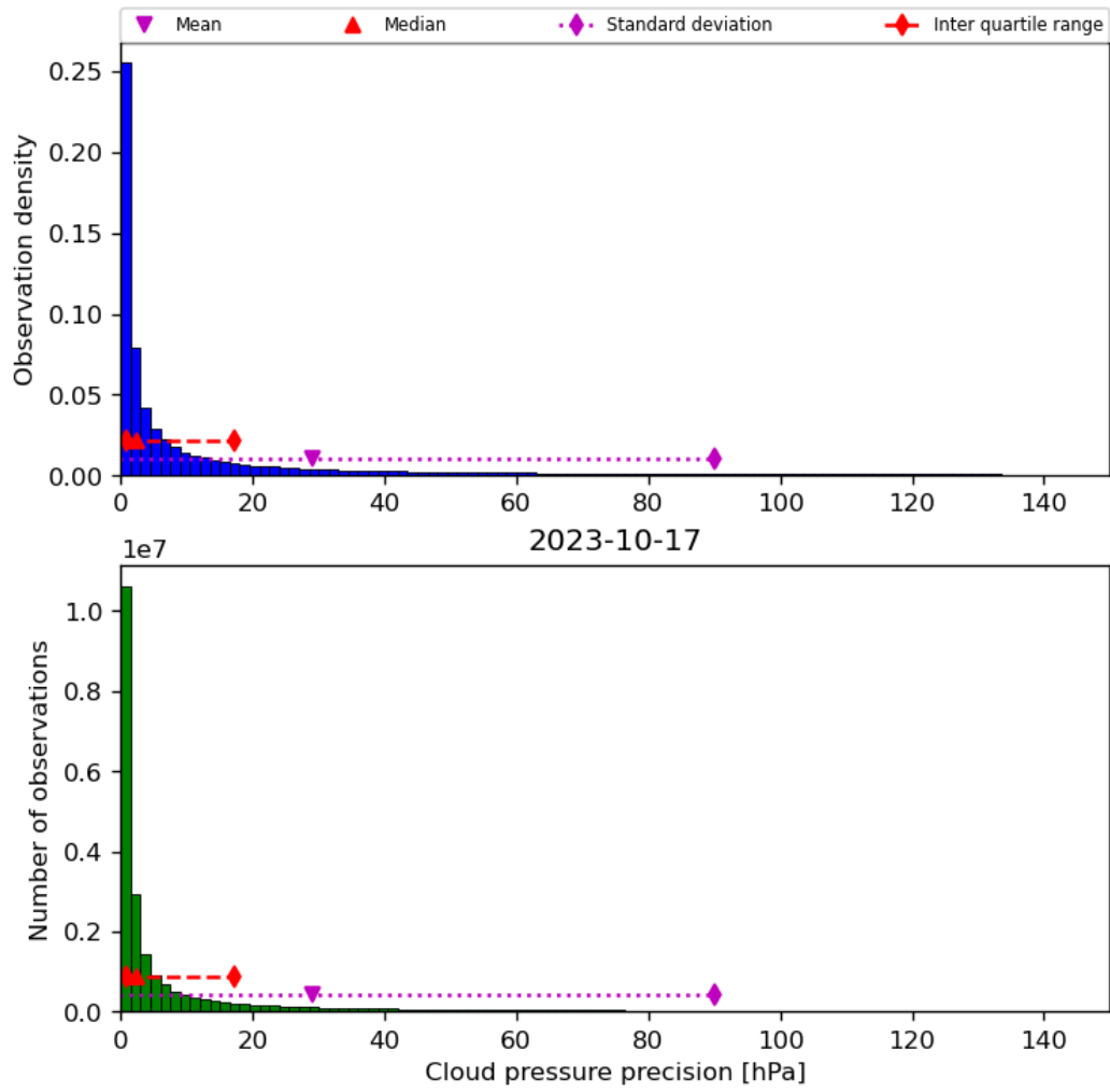
Figure 31: Histogram of “Cloud pressure precision” for 2023-10-17 to 2023-10-18
