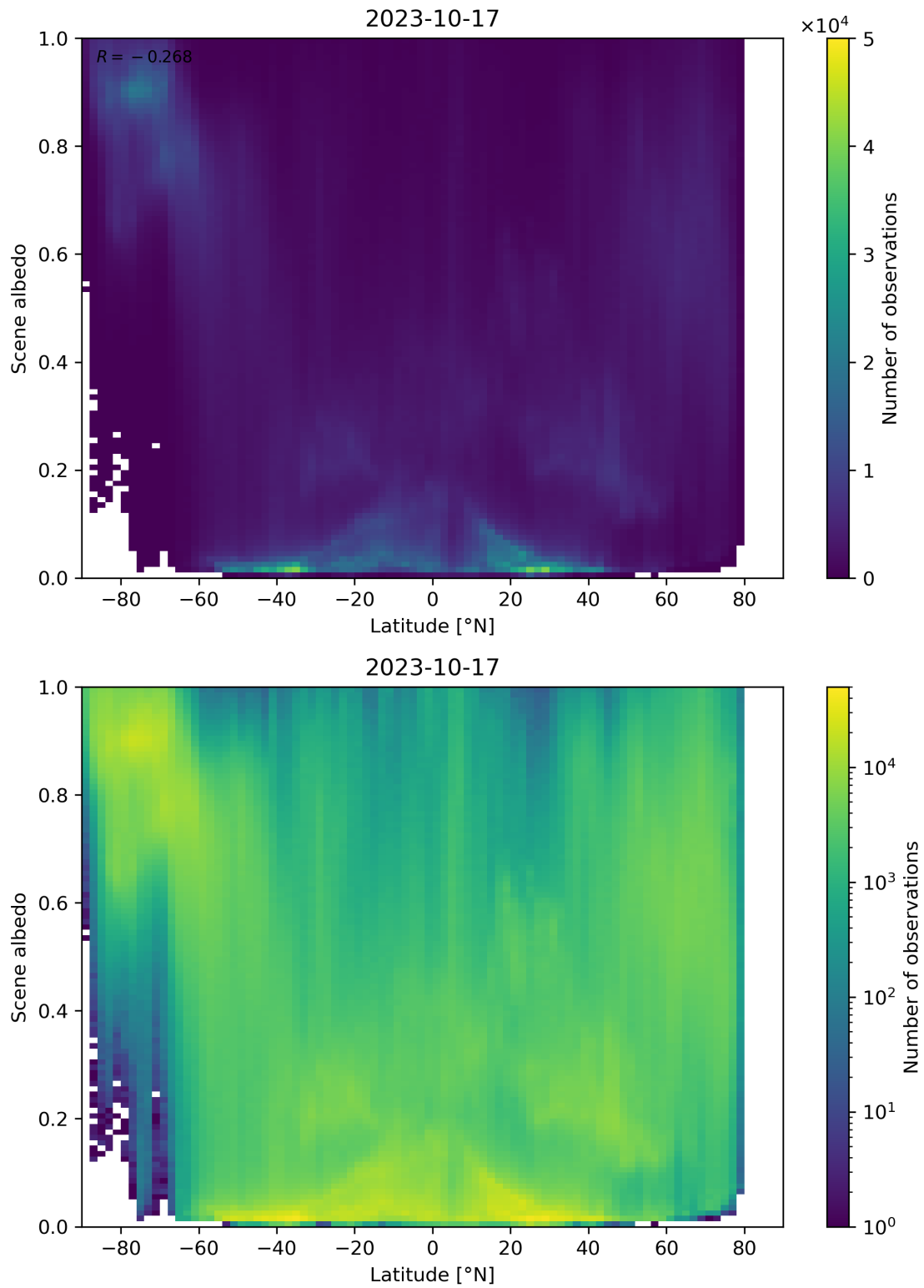
Figure 104: Scatter density plot of “Latitude” against “Scene albedo” for 2023-10-17 to 2023-10-18.
