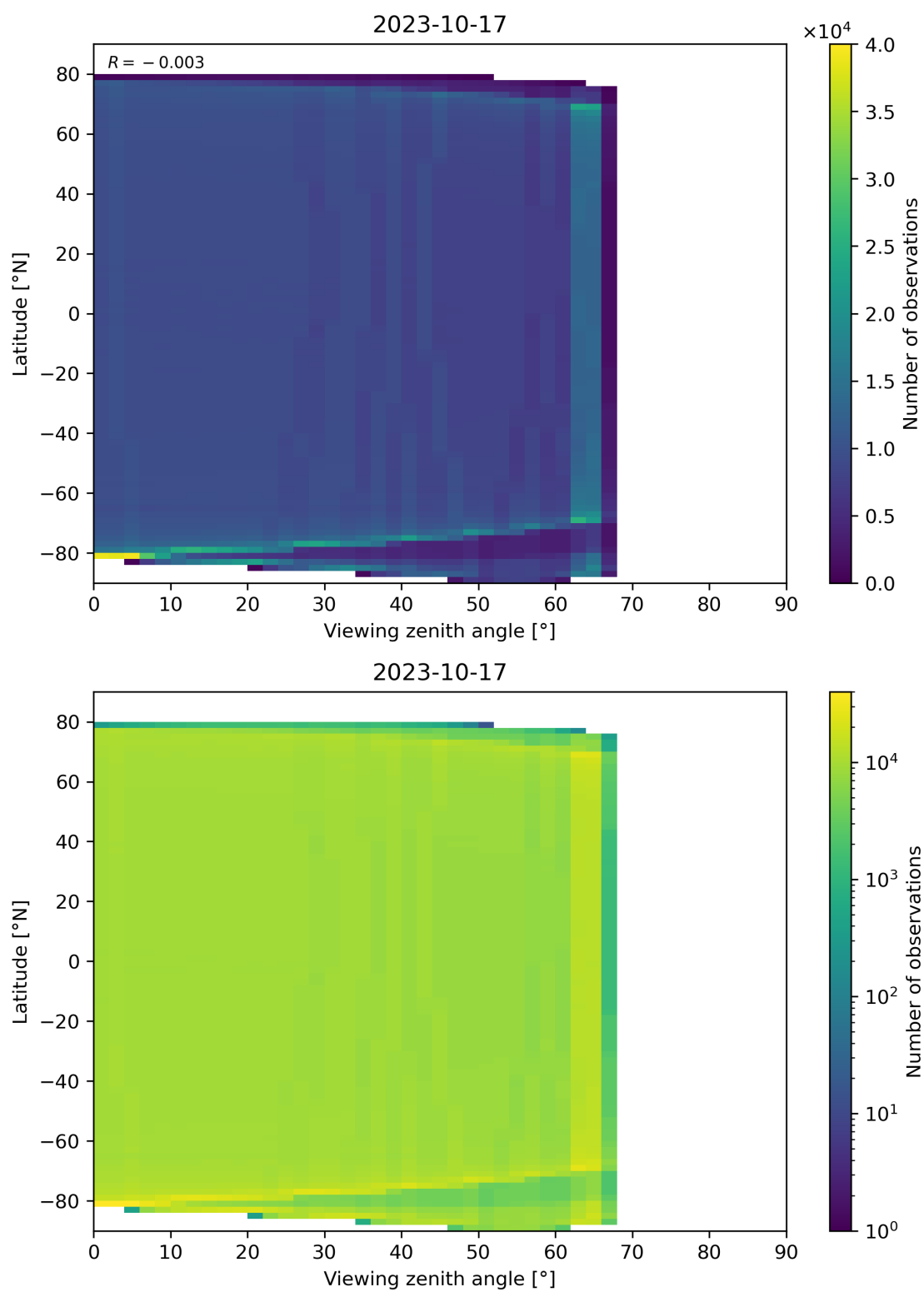
Figure 135: Scatter density plot of “Viewing zenith angle” against “Latitude” for 2023-10-17 to 2023-10-18.
