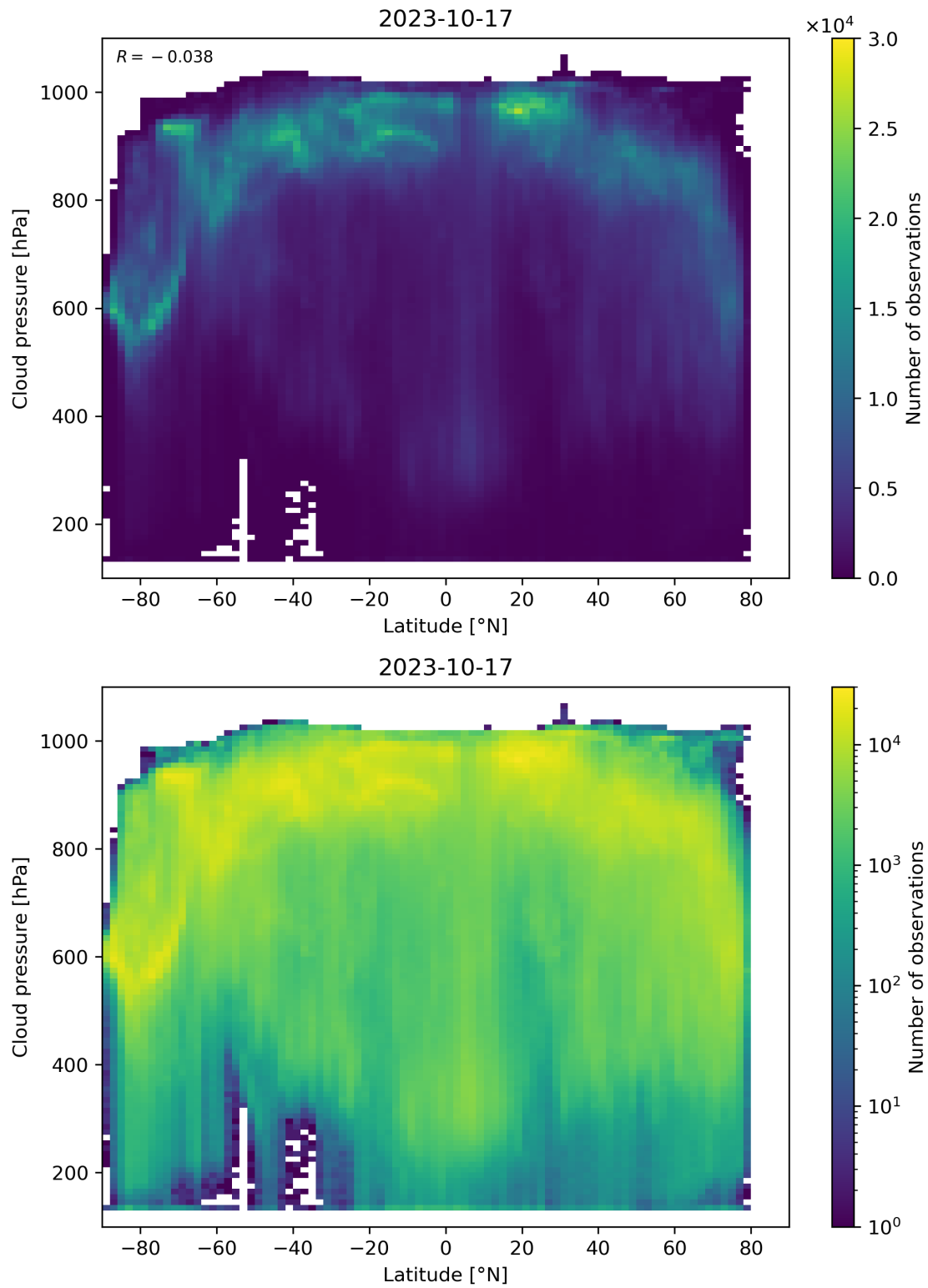
Figure 100: Scatter density plot of “Latitude” against “Cloud pressure” for 2023-10-17 to 2023-10-18.
