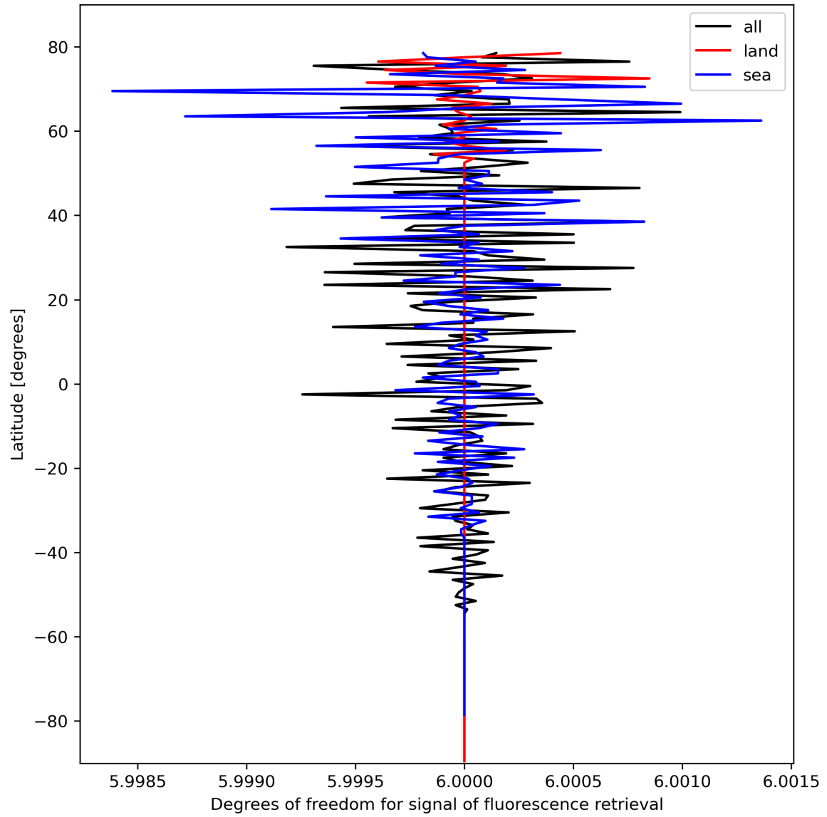
Figure 26: Zonal average of “Degrees of freedom for signal of fluorescence retrieval” for 2023-10-17 to 2023-10-18.
