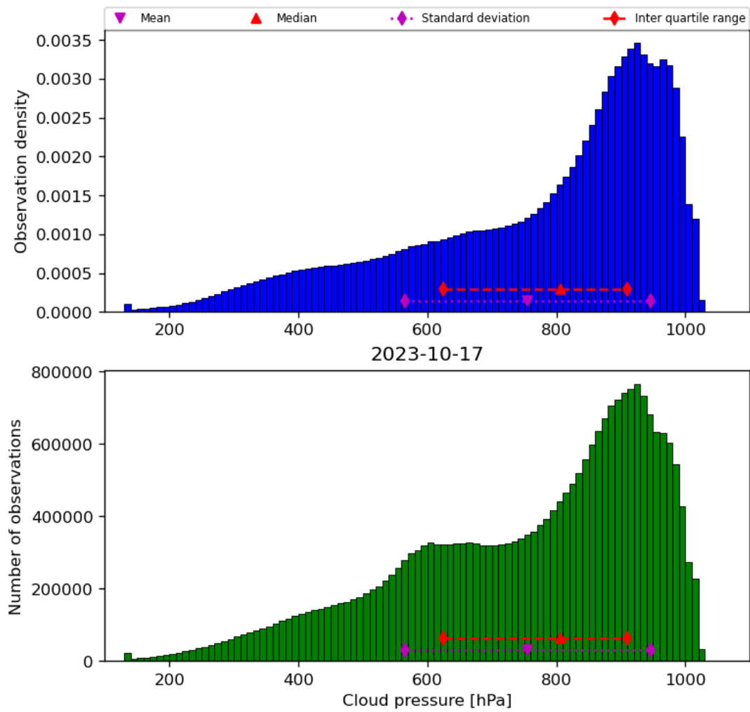
Figure 30: Histogram of “Cloud pressure” for 2023-10-17 to 2023-10-18
