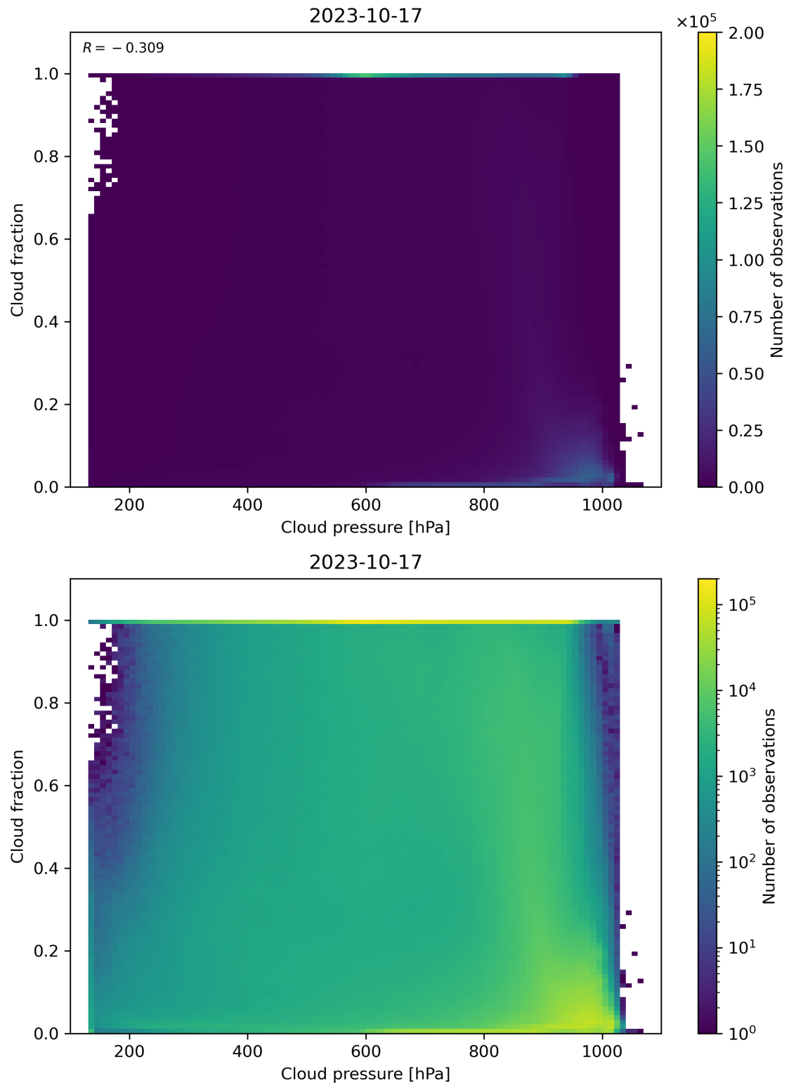
Figure 87: Scatter density plot of “Cloud pressure” against “Cloud fraction” for 2023-10-17 to 2023-10-18.
