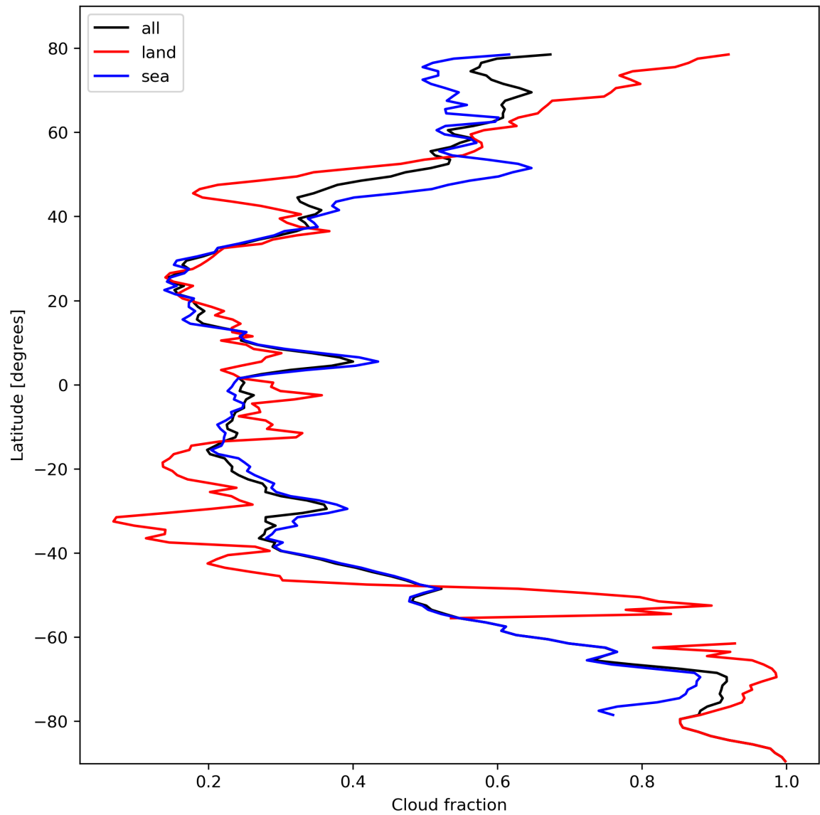
Figure 15: Zonal average of “Cloud fraction” for 2023-10-17 to 2023-10-18.
