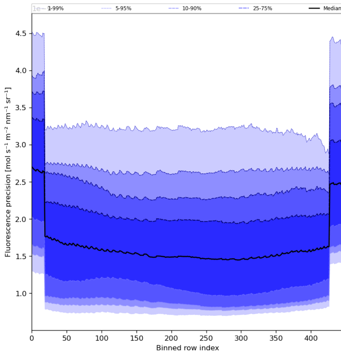
Figure 58: Along track statistics of “Fluorescence precision” for 2023-10-17 to 2023-10-18
