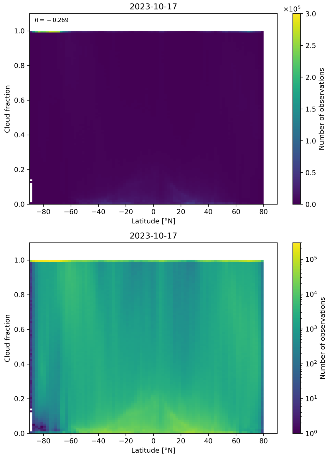
Figure 99: Scatter density plot of “Latitude” against “Cloud fraction” for 2023-10-17 to 2023-10-18.
