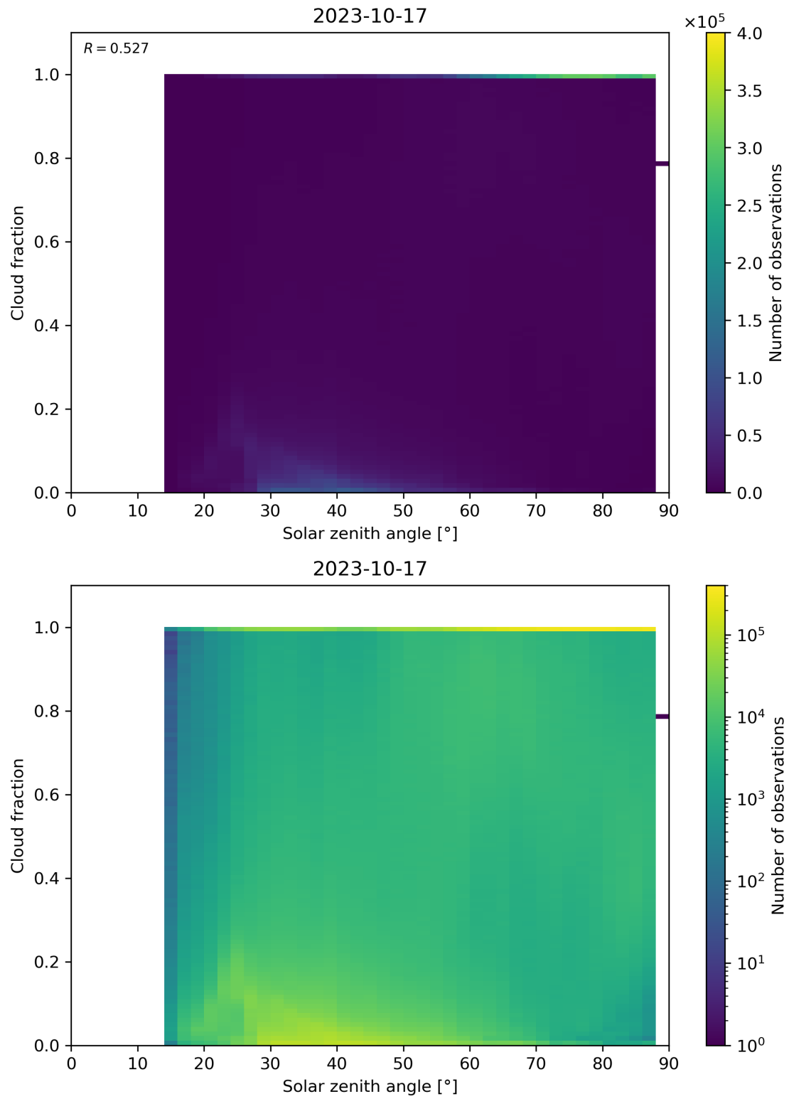
Figure 121: Scatter density plot of “Solar zenith angle” against “Cloud fraction” for 2023-10-17 to 2023-10-18.
