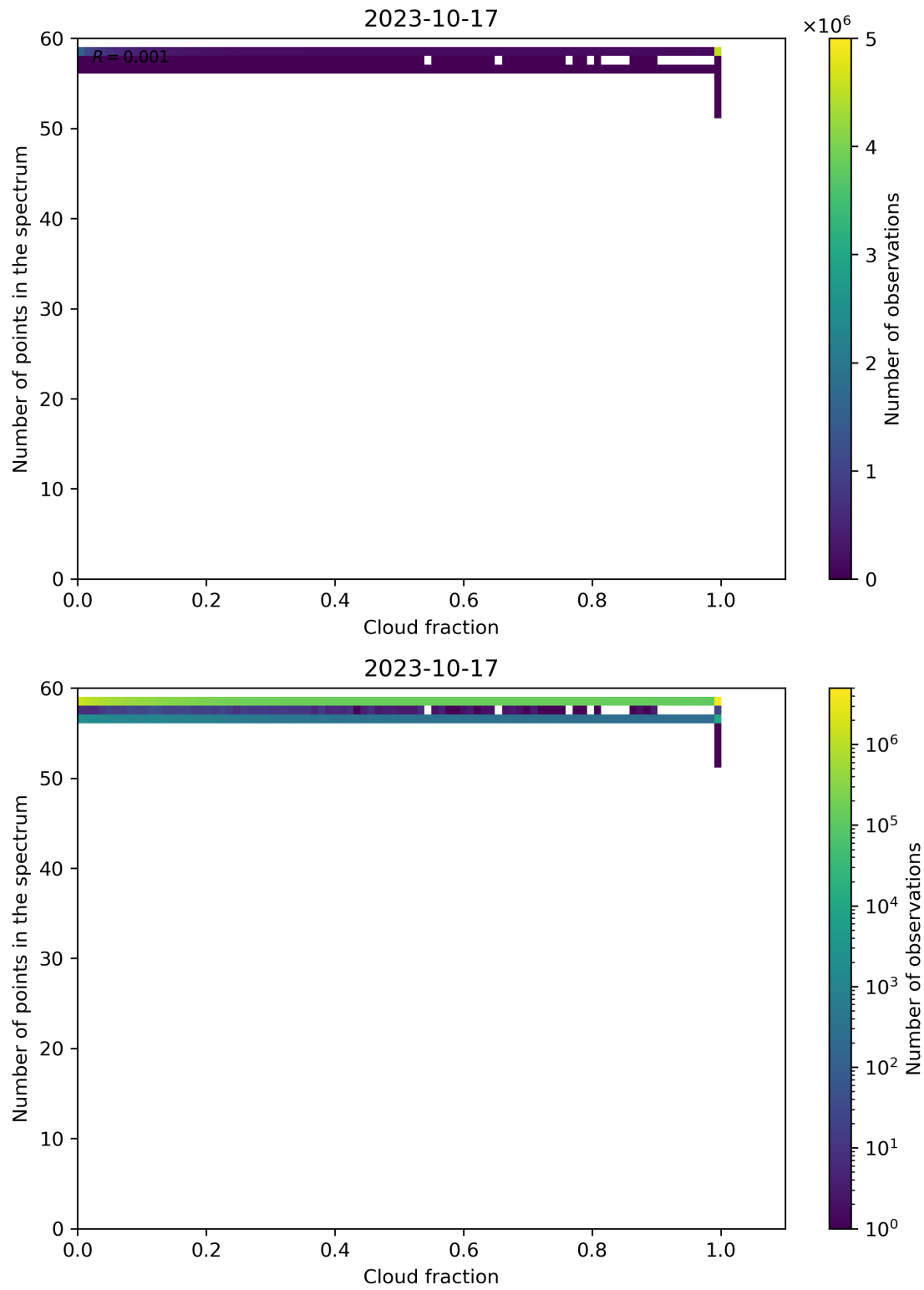
Figure 81: Scatter density plot of “Cloud fraction” against “Number of points in the spectrum” for 2023-10-17 to 2023-10-18.
