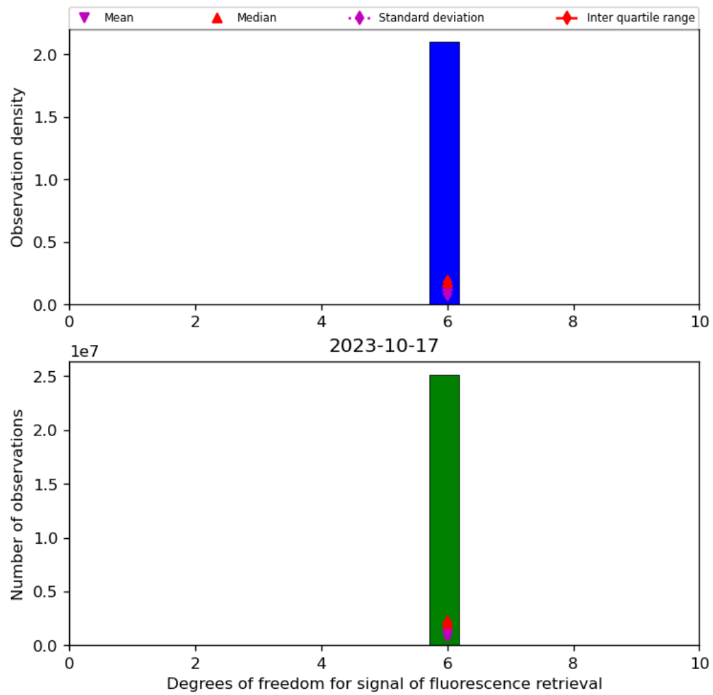
Figure 43: Histogram of “Degrees of freedom for signal of fluorescence retrieval” for 2023-10-17 to 2023-10-18
