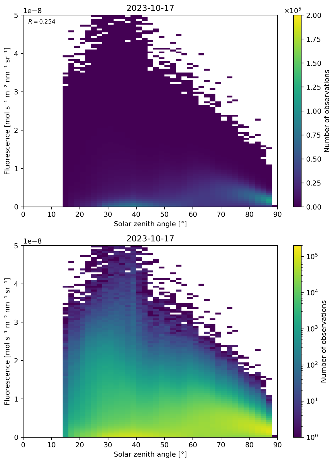
Figure 123: Scatter density plot of “Solar zenith angle” against “Fluorescence” for 2023-10-17 to 2023-10-18.
