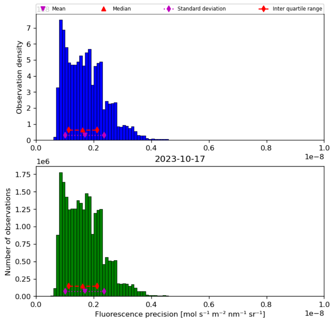
Figure 41: Histogram of “Fluorescence precision” for 2023-10-17 to 2023-10-18
