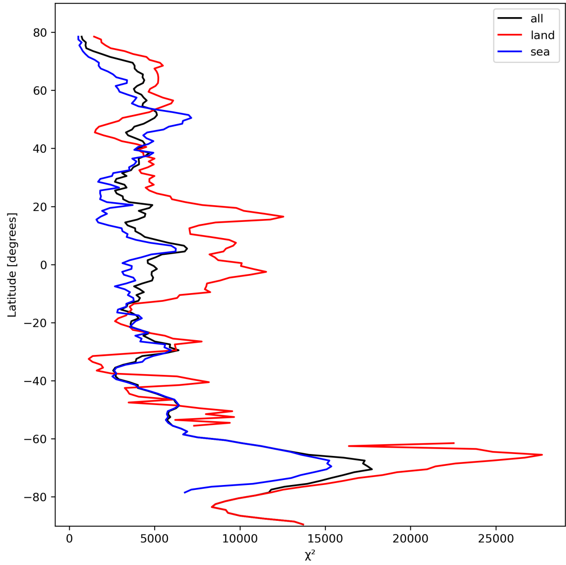
Figure 21: Zonal average of “ \chi^2 ” for 2023-10-17 to 2023-10-18.
