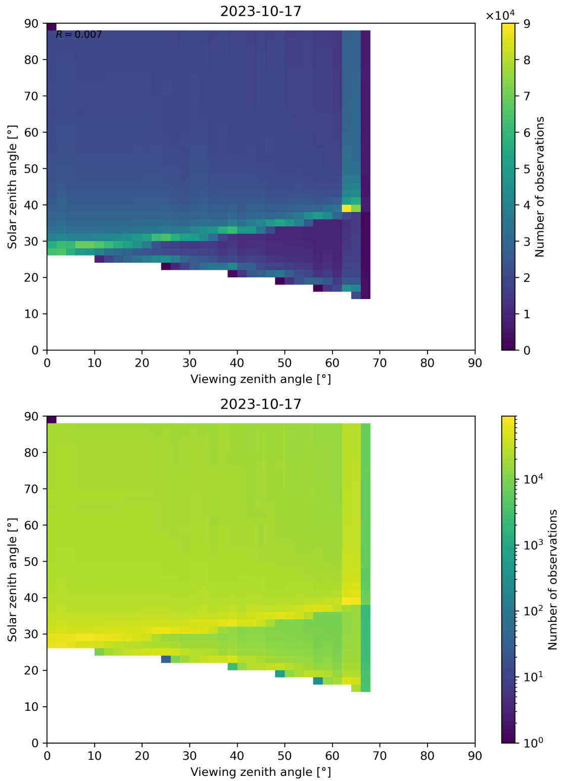
Figure 139: Scatter density plot of “Viewing zenith angle” against “Solar zenith angle” for 2023-10-17 to 2023-10-18.
