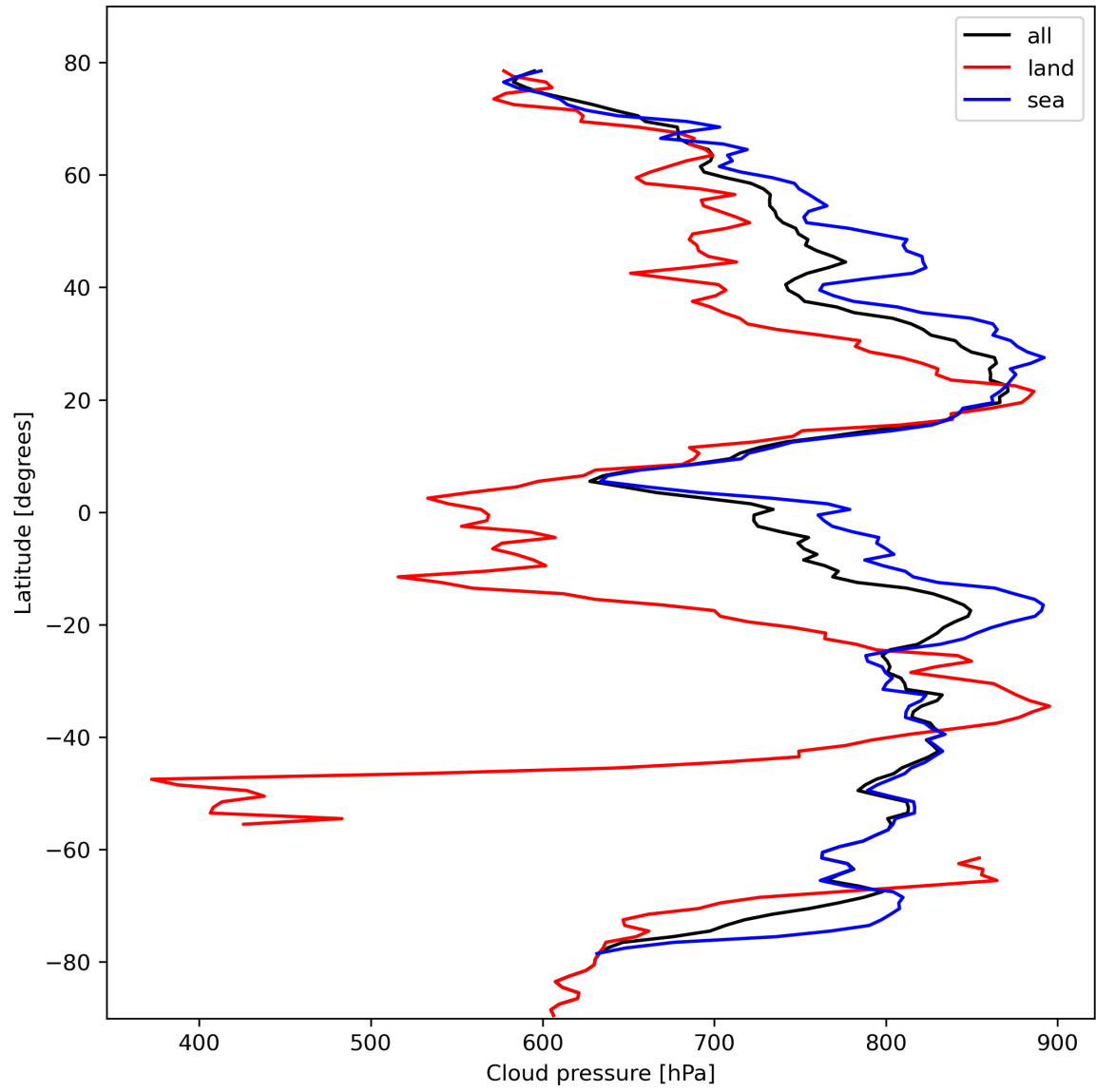
Figure 13: Zonal average of “Cloud pressure” for 2023-10-17 to 2023-10-18.
