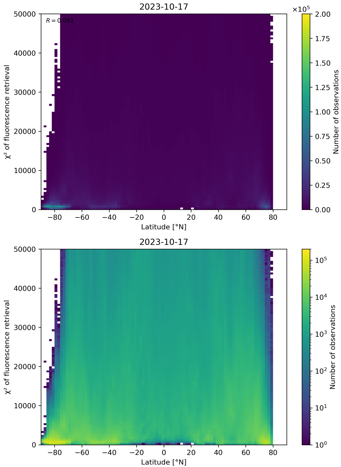
Figure 98: Scatter density plot of “Latitude” against “ \chi^2 of fluorescence retrieval” for 2023-10-17 to 2023-10-18.
