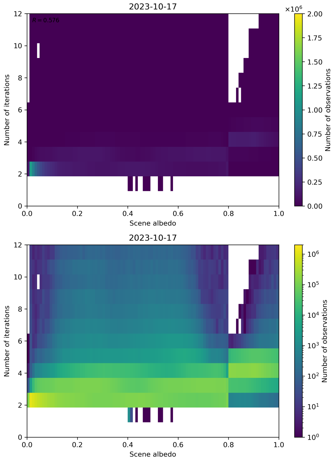
Figure 115: Scatter density plot of “Scene albedo” against “Number of iterations” for 2023-10-17 to 2023-10-18.
