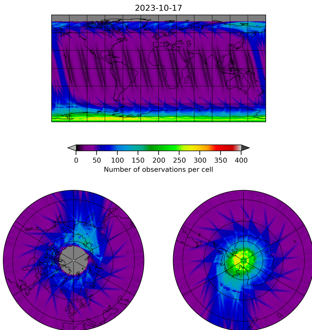
Figure 11: Map of the number of observations for 2023-10-17 to 2023-10-18
