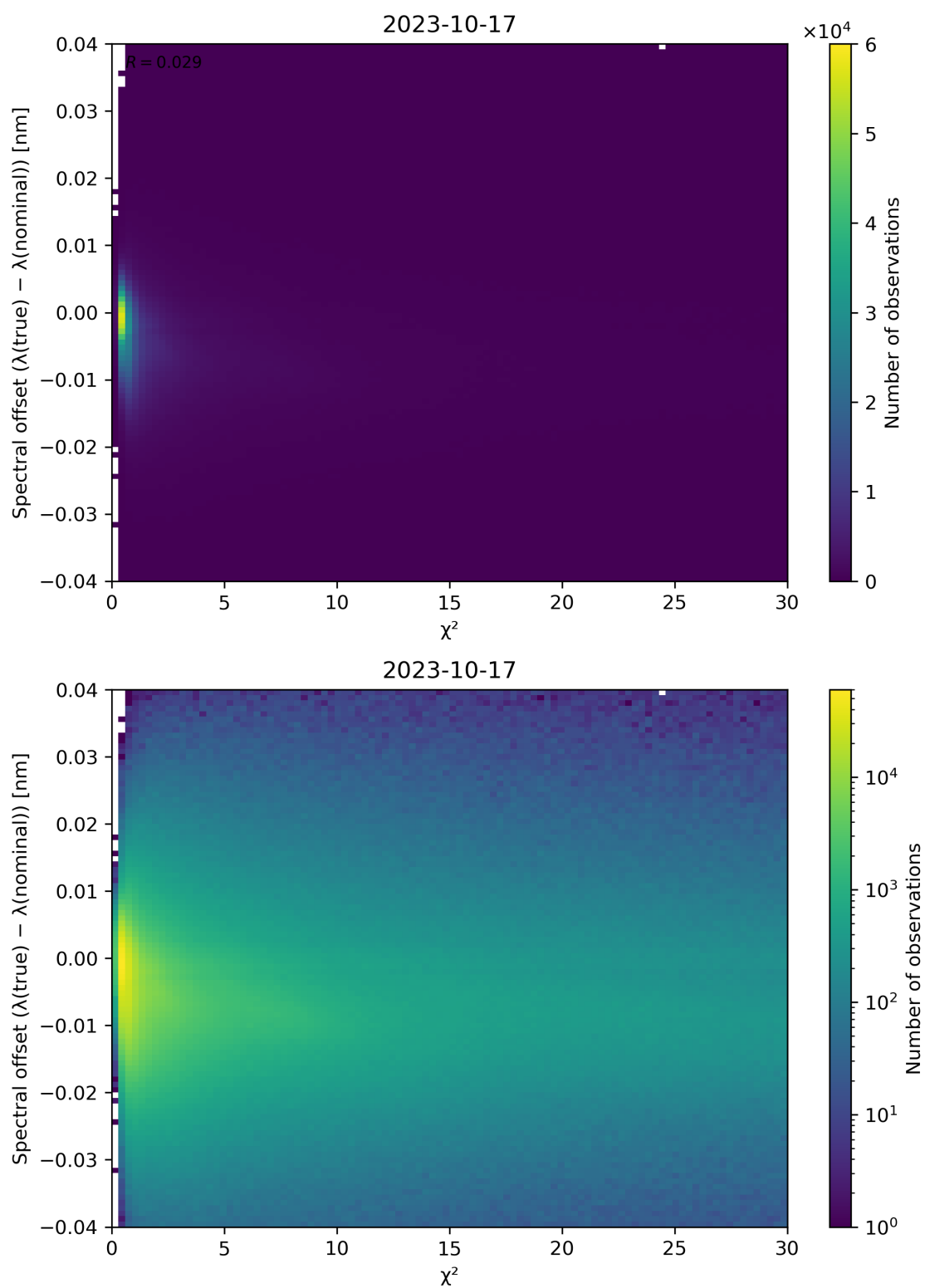
Figure 75: Scatter density plot of “ \chi^2 ” against “Spectral offset ( \lambda(\text{true}) - \lambda(\text{nominal}) )” for 2023-10-17 to 2023-10-18.
