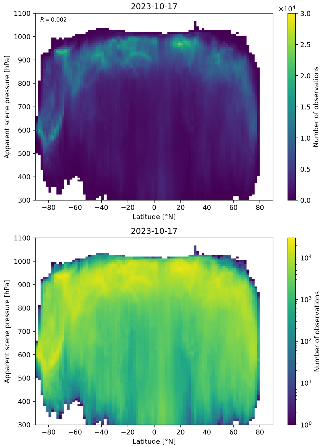
Figure 96: Scatter density plot of “Latitude” against “Apparent scene pressure” for 2023-10-17 to 2023-10-18.
