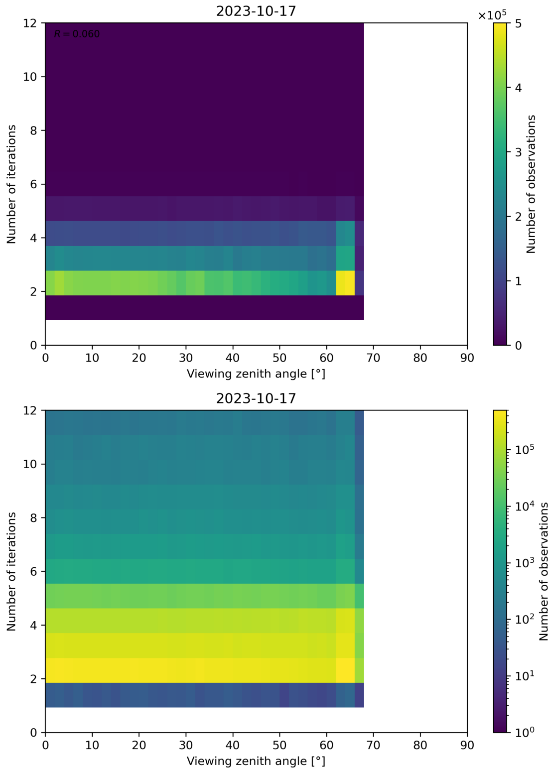
Figure 136: Scatter density plot of “Viewing zenith angle” against “Number of iterations” for 2023-10-17 to 2023-10-18.
