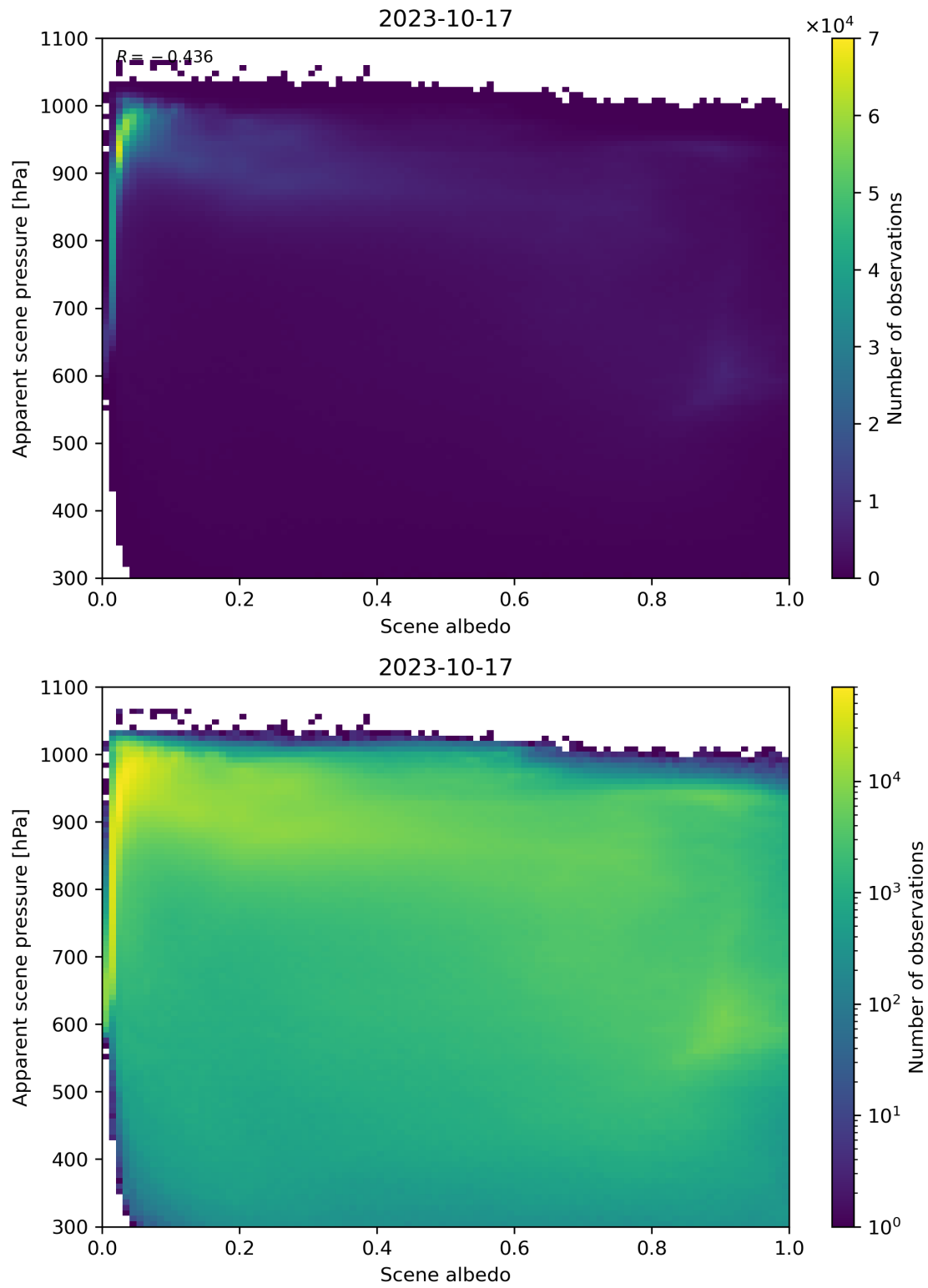
Figure 111: Scatter density plot of “Scene albedo” against “Apparent scene pressure” for 2023-10-17 to 2023-10-18.
