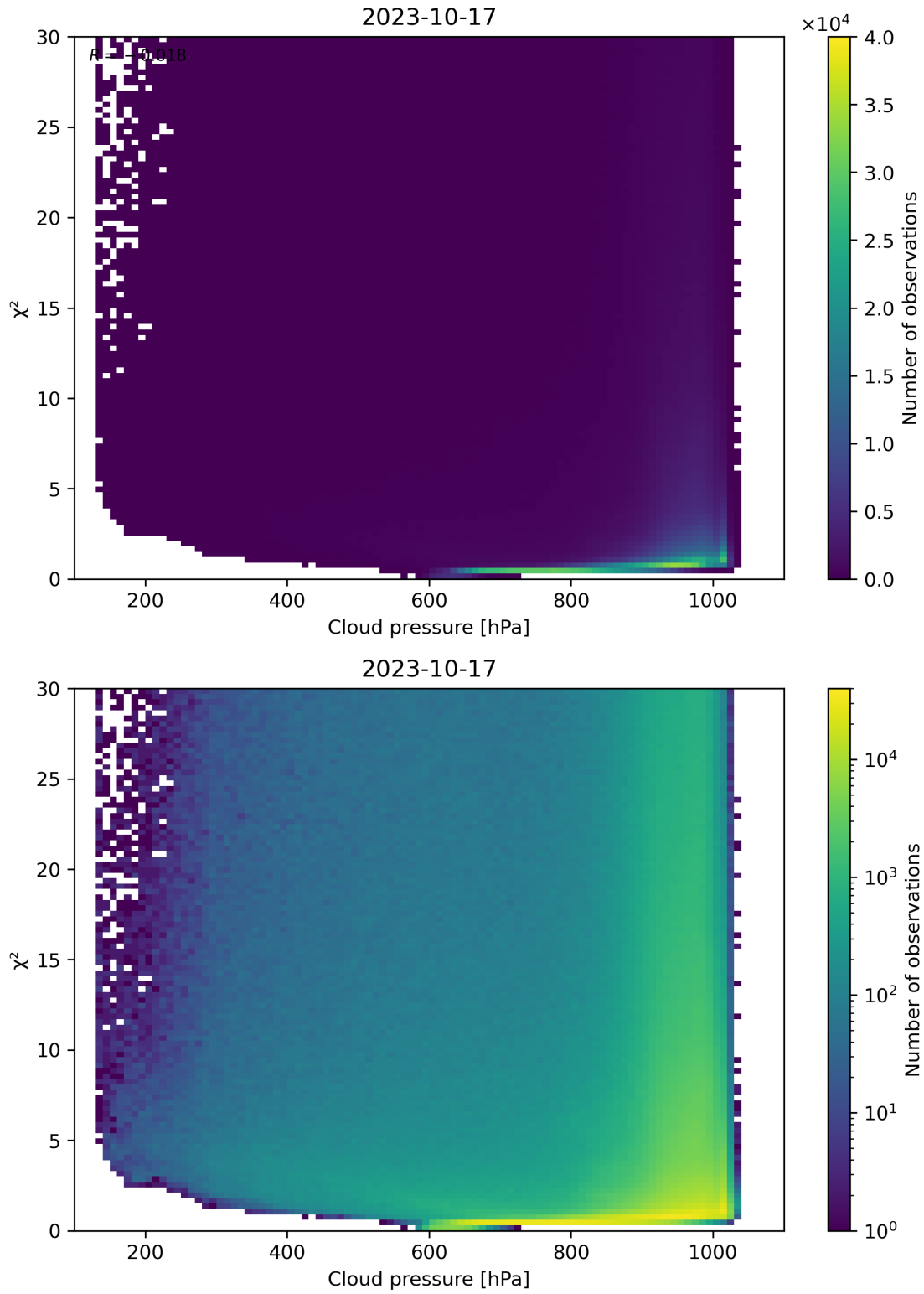
Figure 85: Scatter density plot of “Cloud pressure” against “ \chi^2 ” for 2023-10-17 to 2023-10-18.
