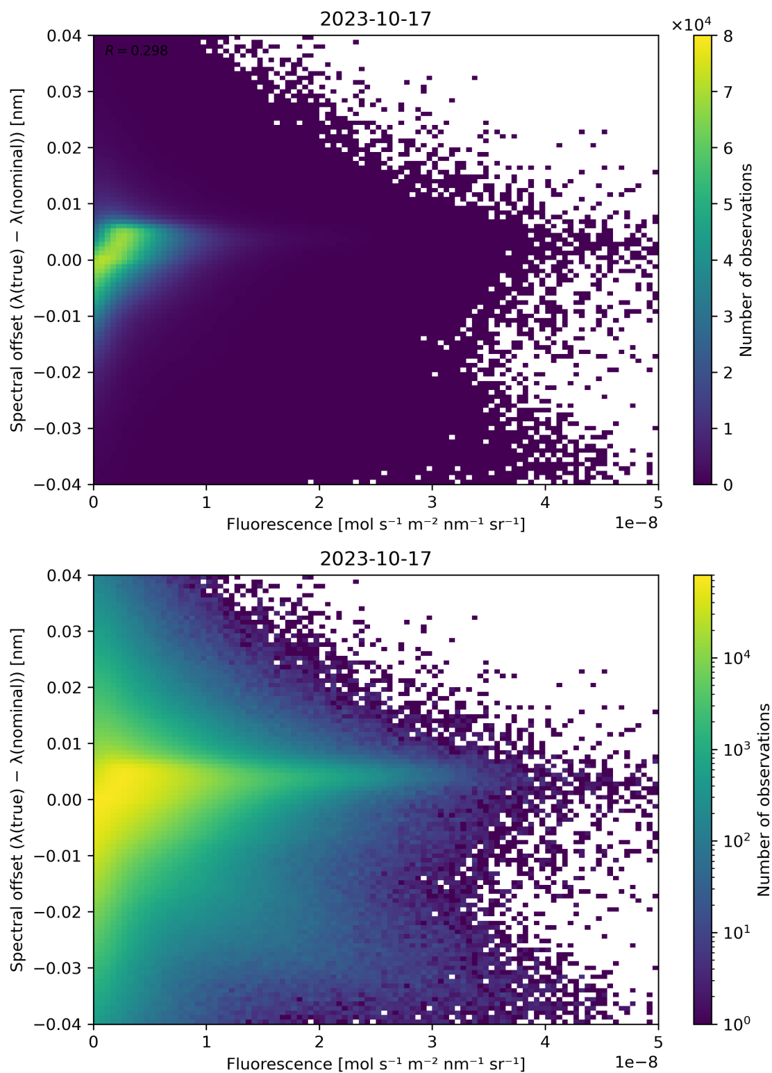
Figure 95: Scatter density plot of “Fluorescence” against “Spectral offset ( \lambda(\text{true}) - \lambda(\text{nominal}) )” for 2023-10-17 to 2023-10-18.
