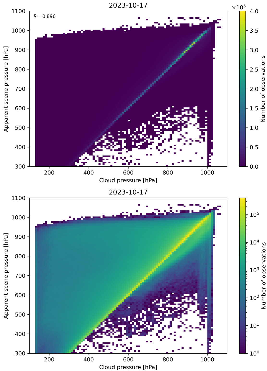
Figure 84: Scatter density plot of “Cloud pressure” against “Apparent scene pressure” for 2023-10-17 to 2023-10-18.
