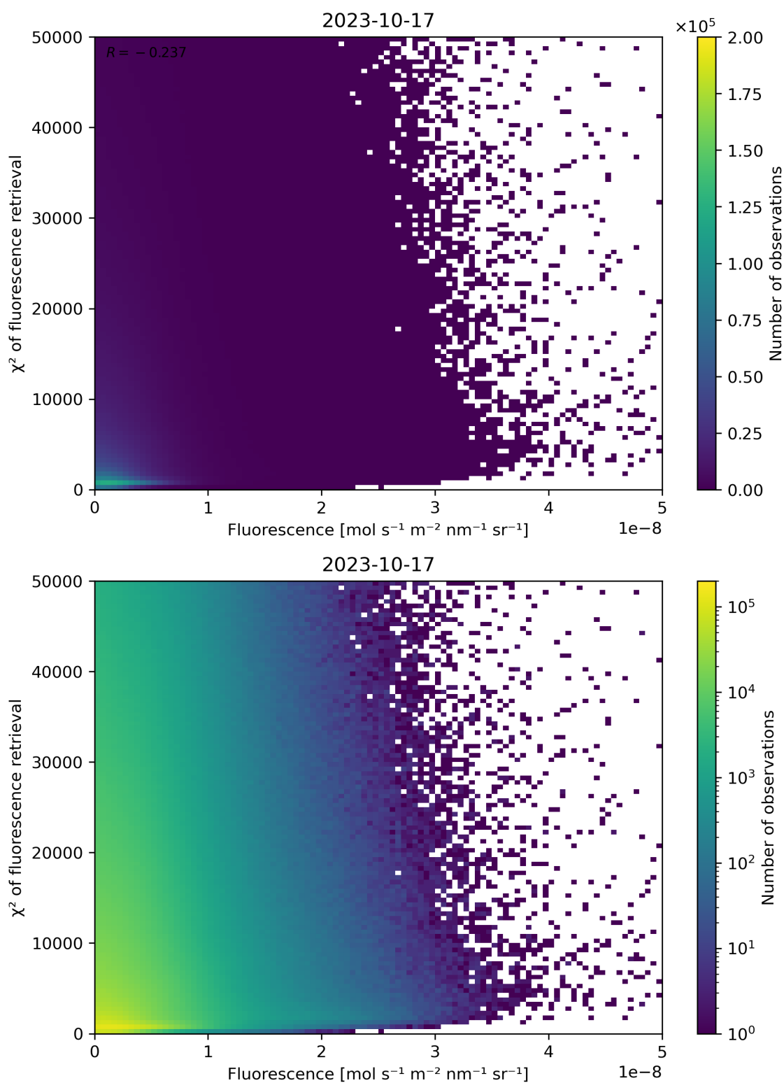
Figure 93: Scatter density plot of “Fluorescence” against “ \chi^2 of fluorescence retrieval” for 2023-10-17 to 2023-10-18.
