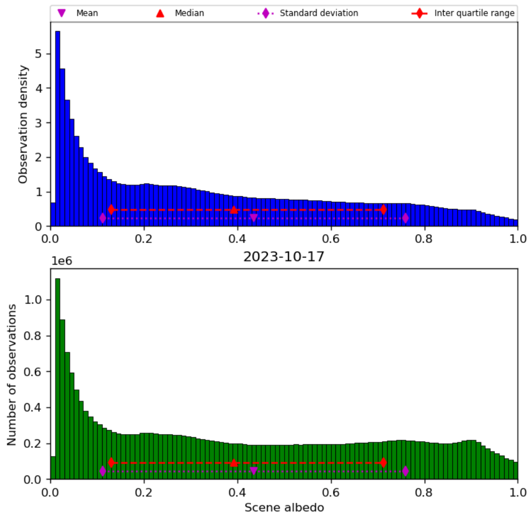
Figure 34: Histogram of “Scene albedo” for 2023-10-17 to 2023-10-18
