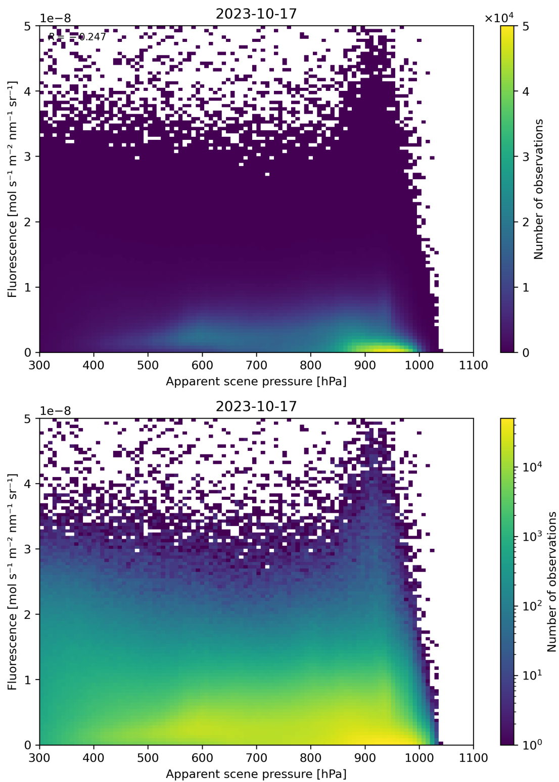
Figure 65: Scatter density plot of “Apparent scene pressure” against “Fluorescence” for 2023-10-17 to 2023-10-18.
