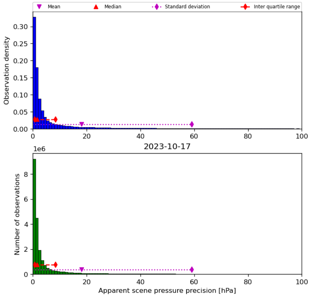
Figure 37: Histogram of “Apparent scene pressure precision” for 2023-10-17 to 2023-10-18
