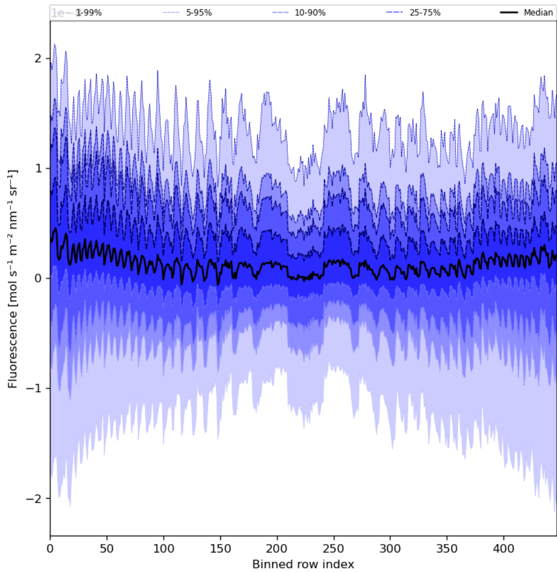
Figure 57: Along track statistics of “Fluorescence” for 2023-10-17 to 2023-10-18
