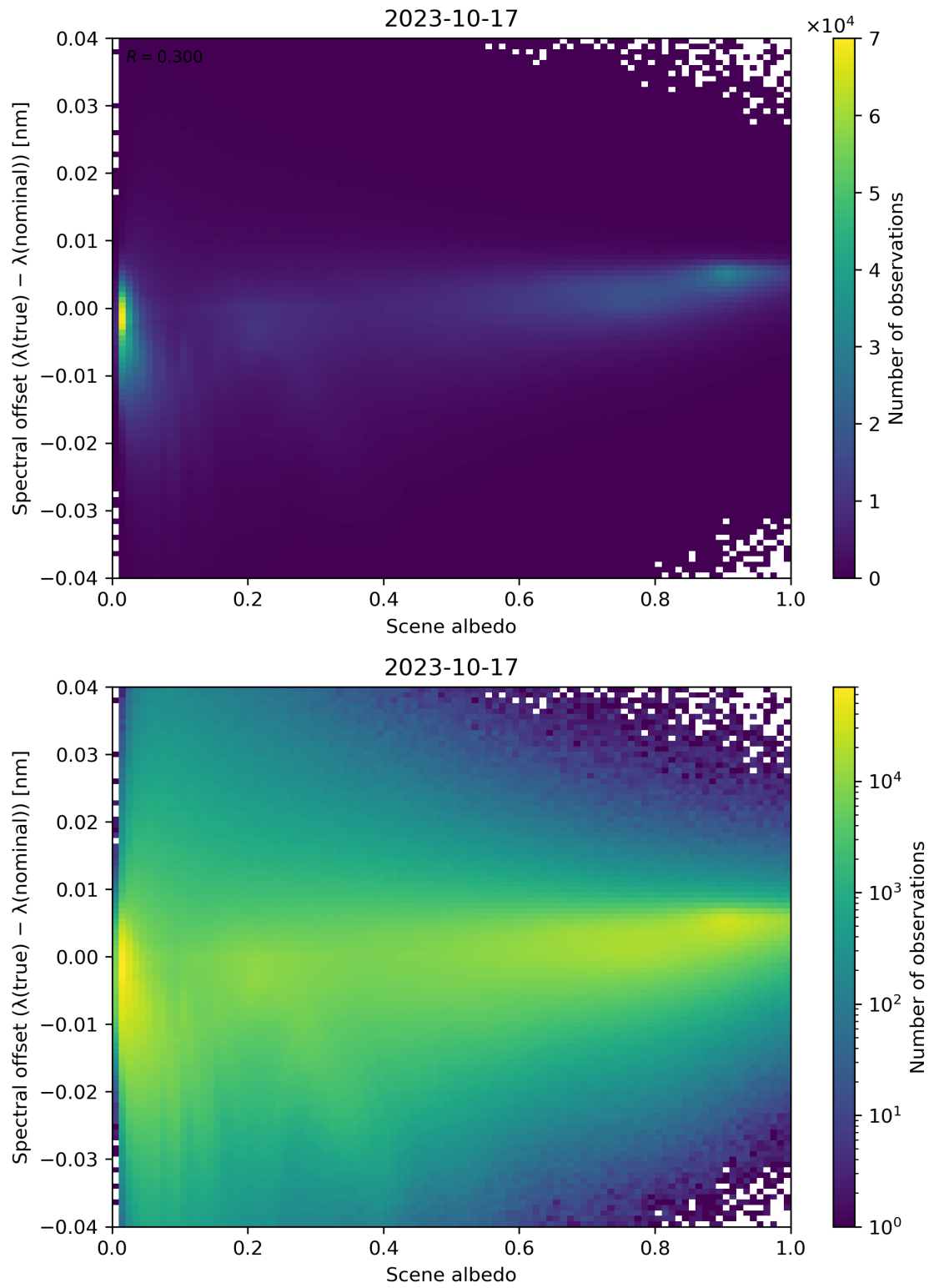
Figure 117: Scatter density plot of “Scene albedo” against “Spectral offset ( \lambda(\text{true}) - \lambda(\text{nominal}) )” for 2023-10-17 to 2023-10-18.
