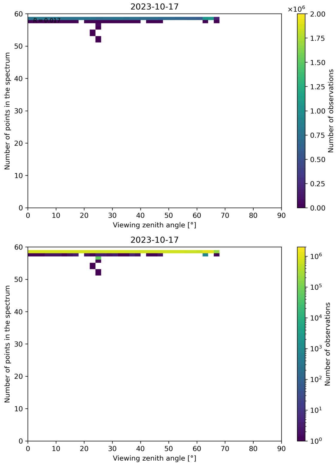
Figure 137: Scatter density plot of “Viewing zenith angle” against “Number of points in the spectrum” for 2023-10-17 to 2023-10-18.
