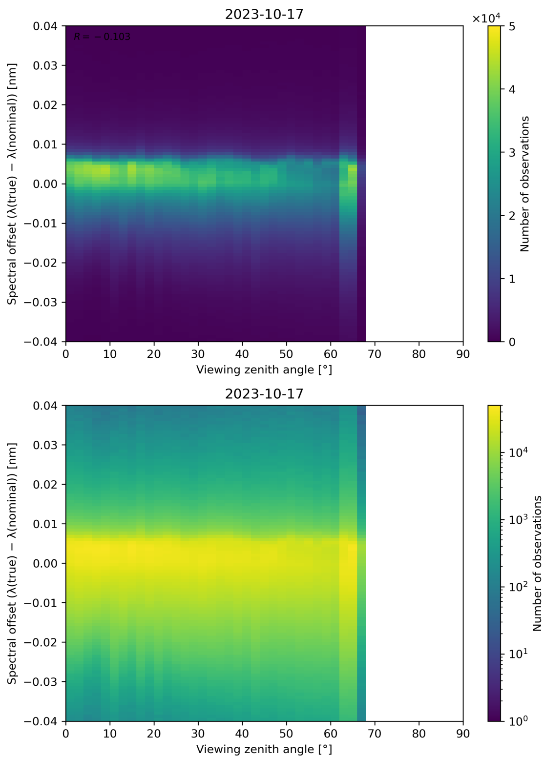
Figure 140: Scatter density plot of “Viewing zenith angle” against “Spectral offset ( \lambda(\text{true}) - \lambda(\text{nominal}) )” for 2023-10-17 to 2023-10-18.
