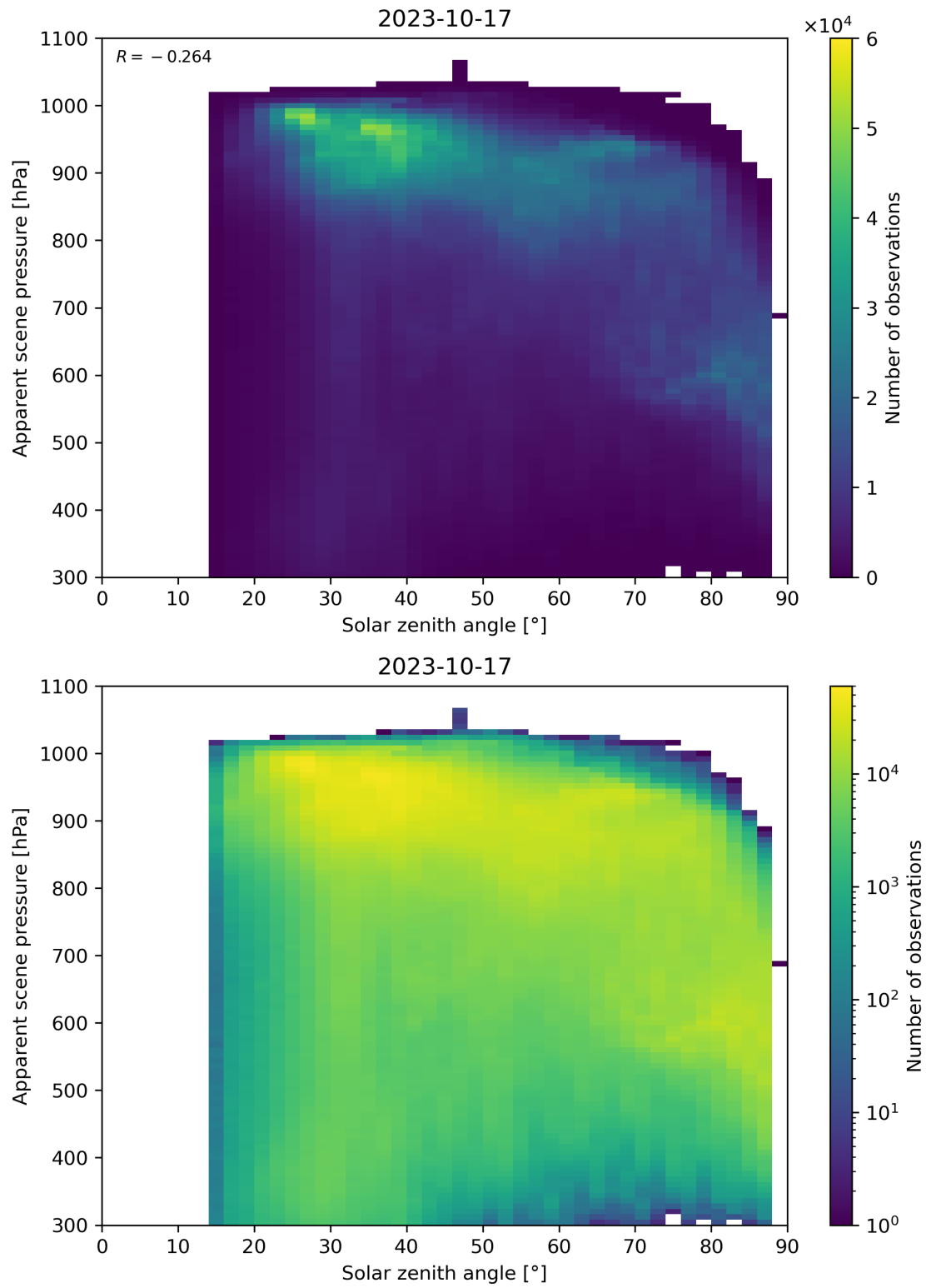
Figure 118: Scatter density plot of “Solar zenith angle” against “Apparent scene pressure” for 2023-10-17 to 2023-10-18.
