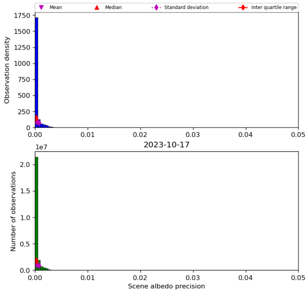
Figure 35: Histogram of “Scene albedo precision” for 2023-10-17 to 2023-10-18
