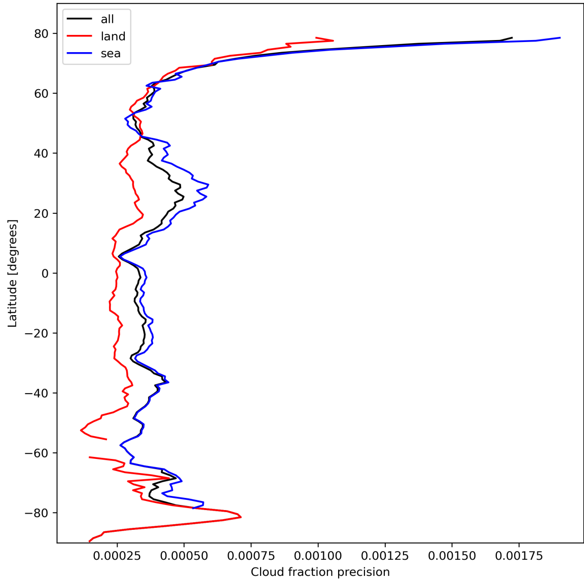
Figure 16: Zonal average of “Cloud fraction precision” for 2023-10-17 to 2023-10-18.
