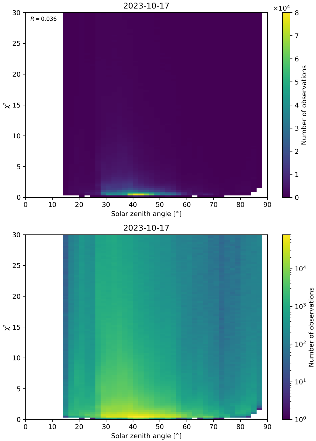
Figure 119: Scatter density plot of “Solar zenith angle” against “ \chi^2 ” for 2023-10-17 to 2023-10-18.
