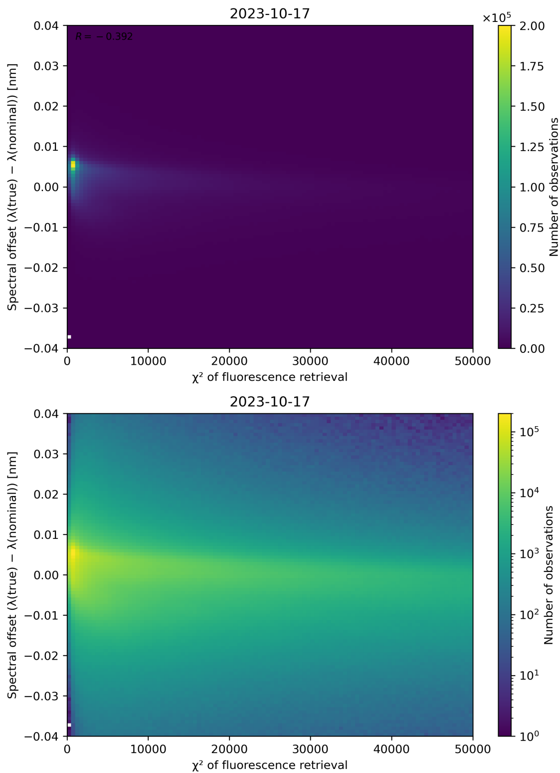
Figure 72: Scatter density plot of " \chi^2 of fluorescence retrieval" against "Spectral offset ( \lambda(\text{true}) - \lambda(\text{nominal}) )" for 2023-10-17 to 2023-10-18.
