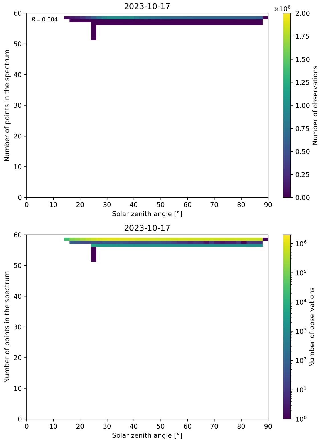
Figure 126: Scatter density plot of “Solar zenith angle” against “Number of points in the spectrum” for 2023-10-17 to 2023-10-18.
