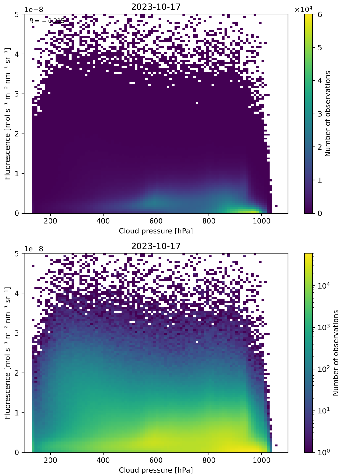
Figure 88: Scatter density plot of “Cloud pressure” against “Fluorescence” for 2023-10-17 to 2023-10-18.
