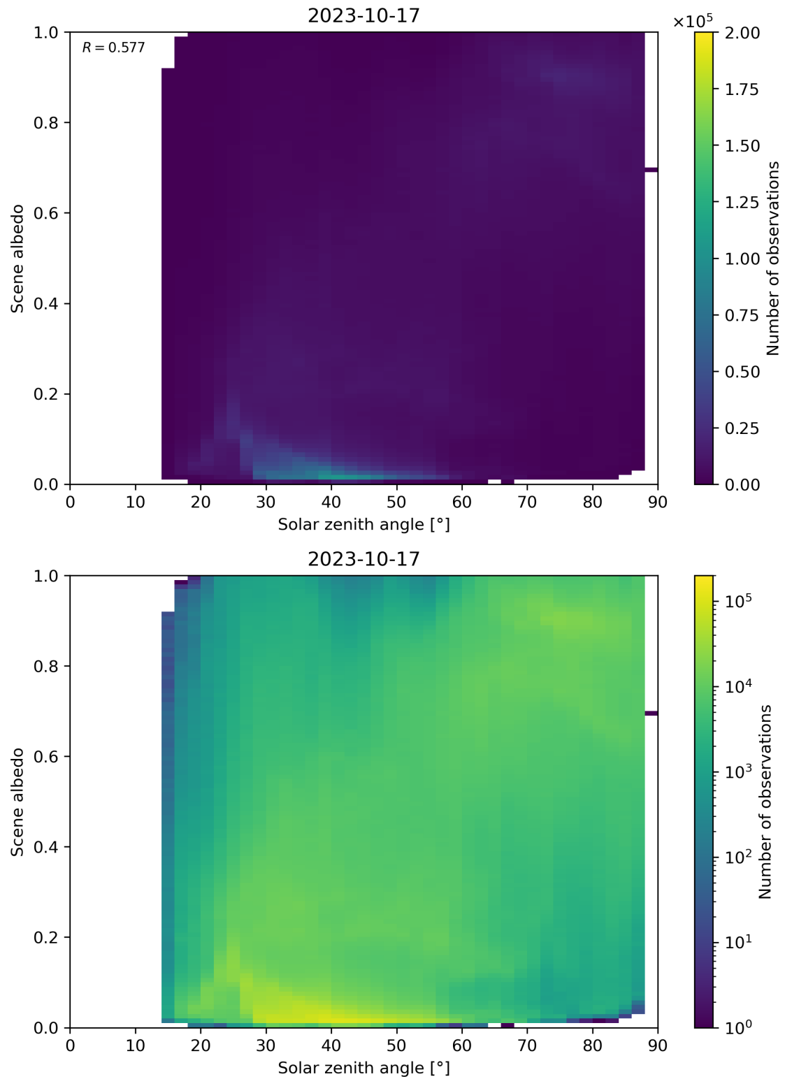
Figure 127: Scatter density plot of “Solar zenith angle” against “Scene albedo” for 2023-10-17 to 2023-10-18.
