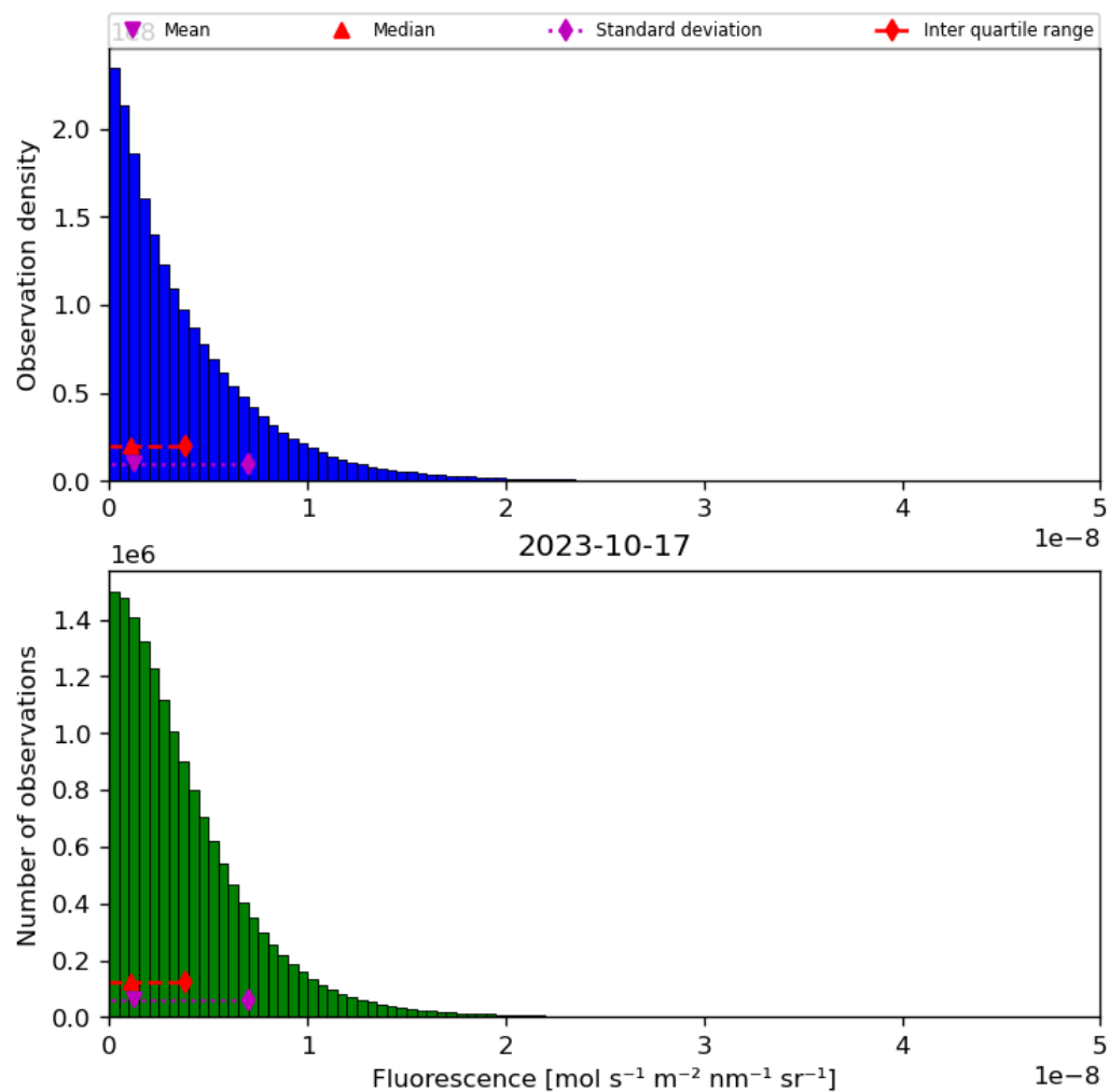
Figure 40: Histogram of “Fluorescence” for 2023-10-17 to 2023-10-18
