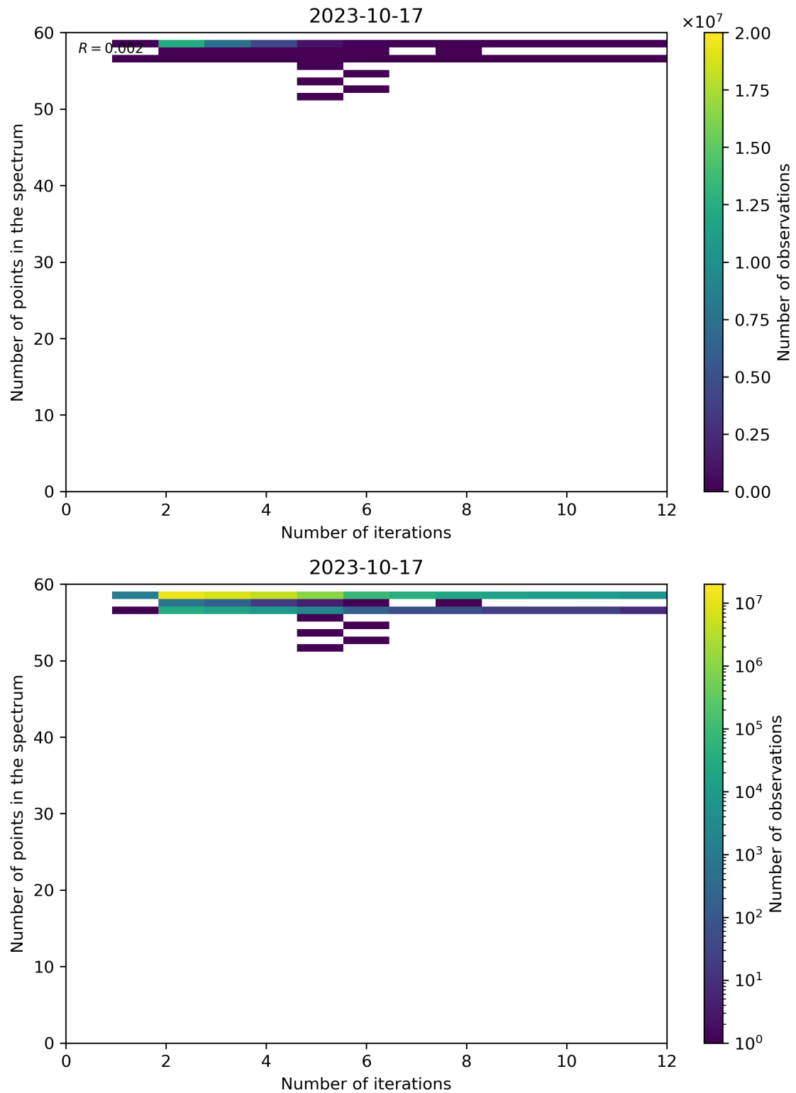
Figure 108: Scatter density plot of “Number of iterations” against “Number of points in the spectrum” for 2023-10-17 to 2023-10-18.
