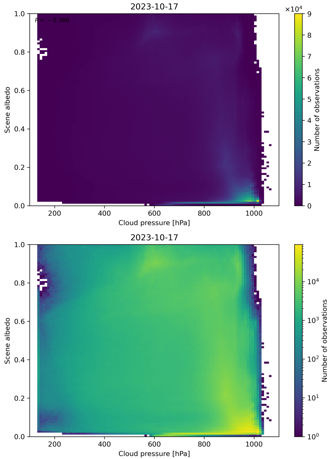
Figure 91: Scatter density plot of “Cloud pressure” against “Scene albedo” for 2023-10-17 to 2023-10-18.
