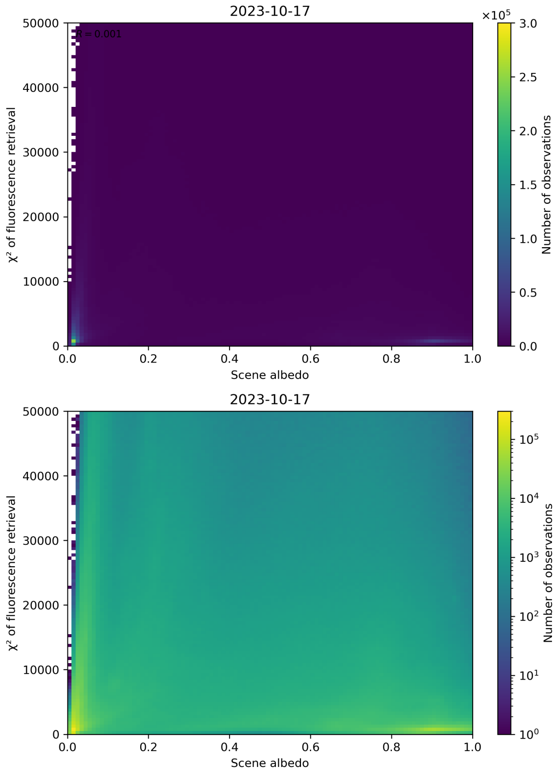
Figure 113: Scatter density plot of “Scene albedo” against “ \chi^2 of fluorescence retrieval” for 2023-10-17 to 2023-10-18.
