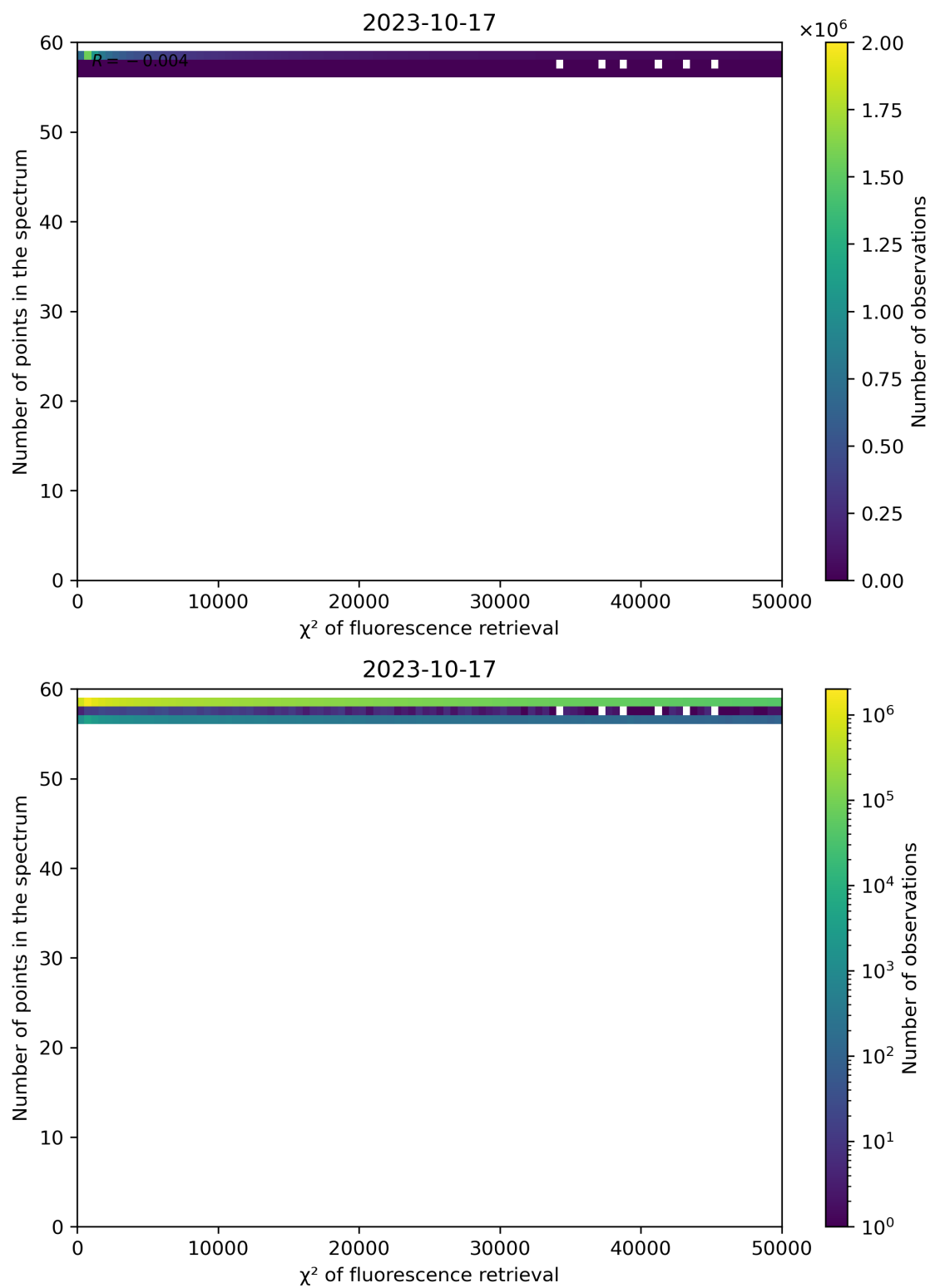
Figure 71: Scatter density plot of “ \chi^2 of fluorescence retrieval” against “Number of points in the spectrum” for 2023-10-17 to 2023-10-18.
