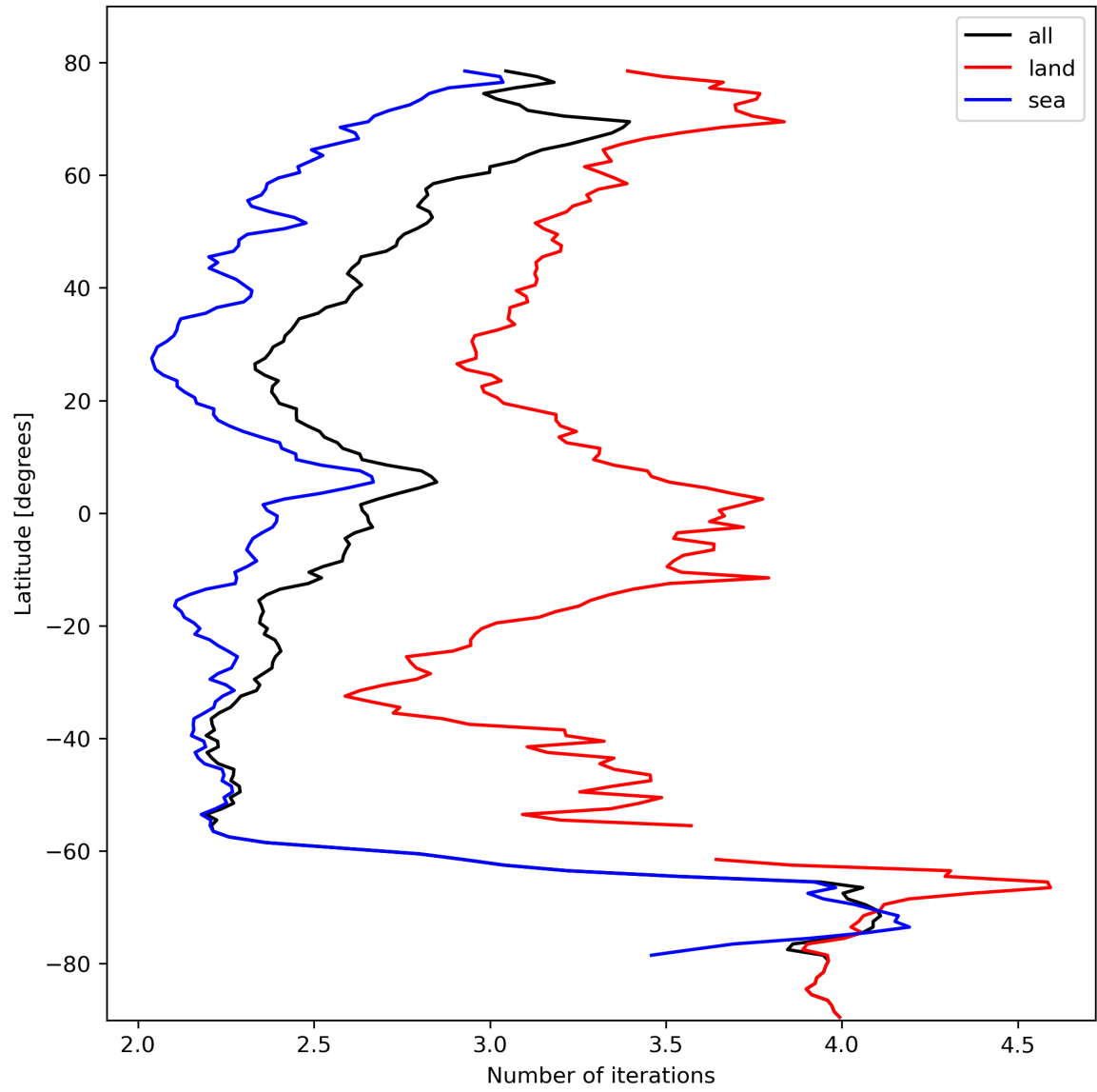
Figure 22: Zonal average of “Number of iterations” for 2023-10-17 to 2023-10-18.
