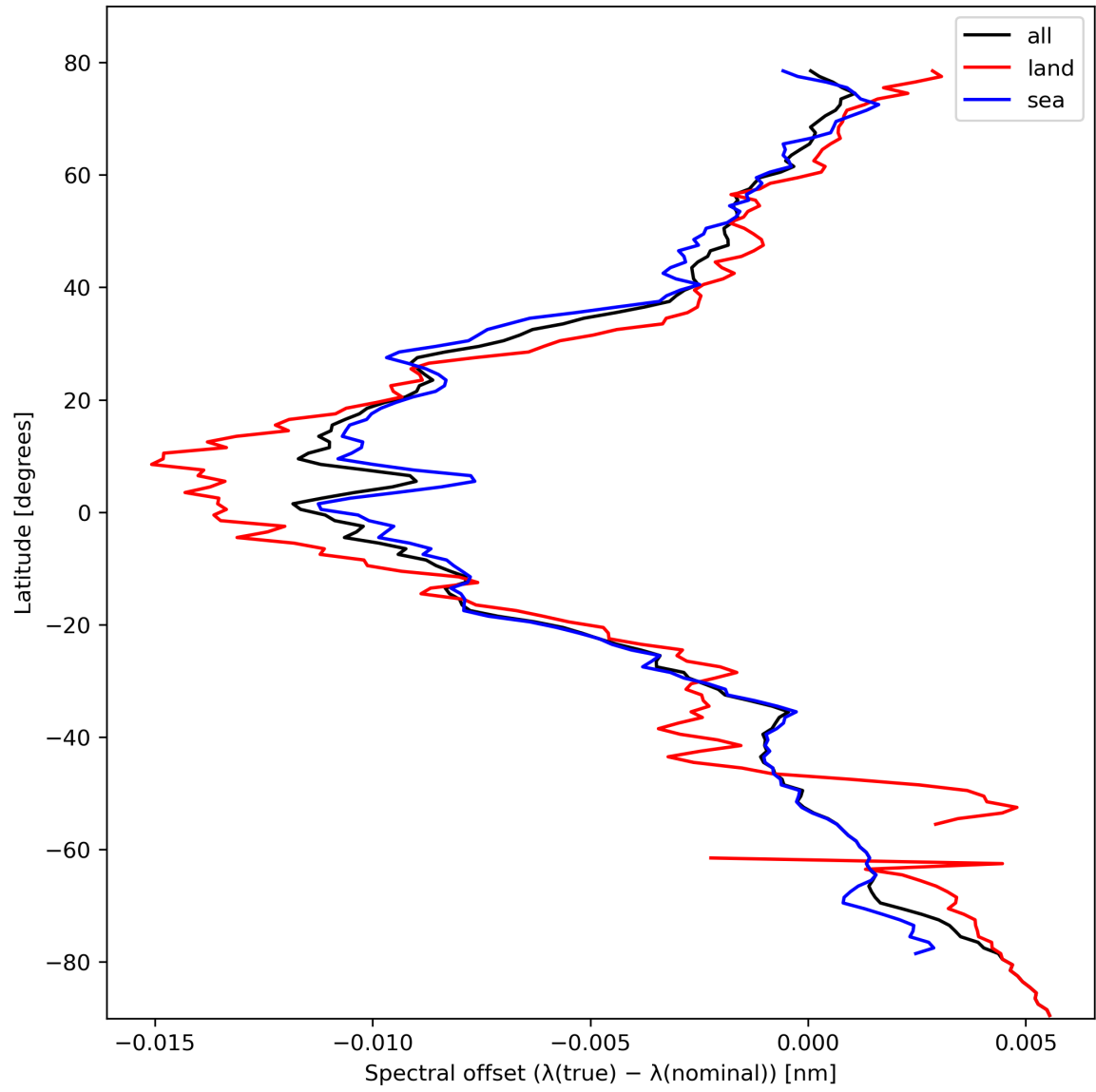
Figure 28: Zonal average of “Spectral offset ( \lambda(\text{true}) - \lambda(\text{nominal}) )” for 2023-10-17 to 2023-10-18.
