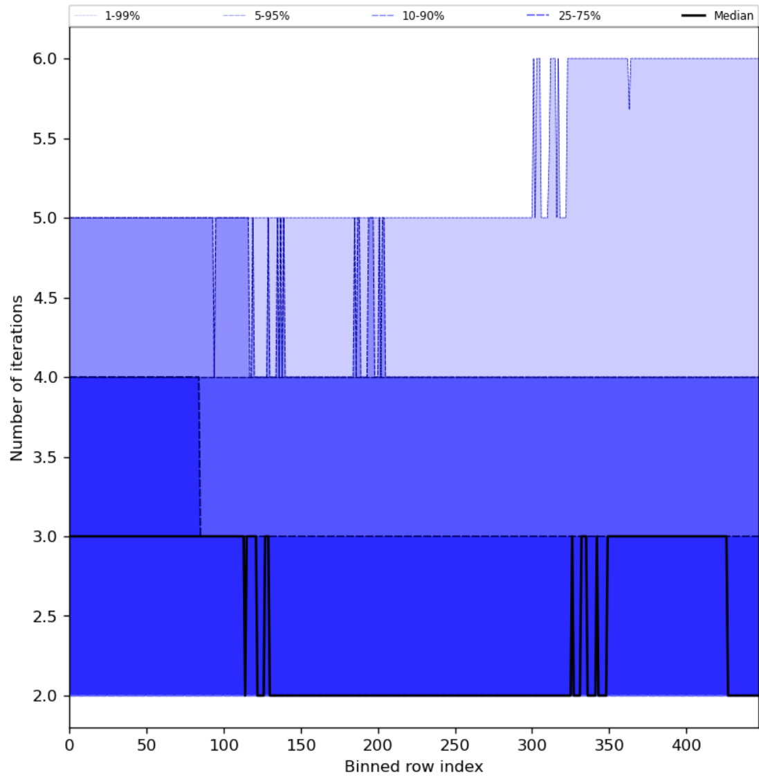
Figure 56: Along track statistics of "Number of iterations" for 2023-10-17 to 2023-10-18
