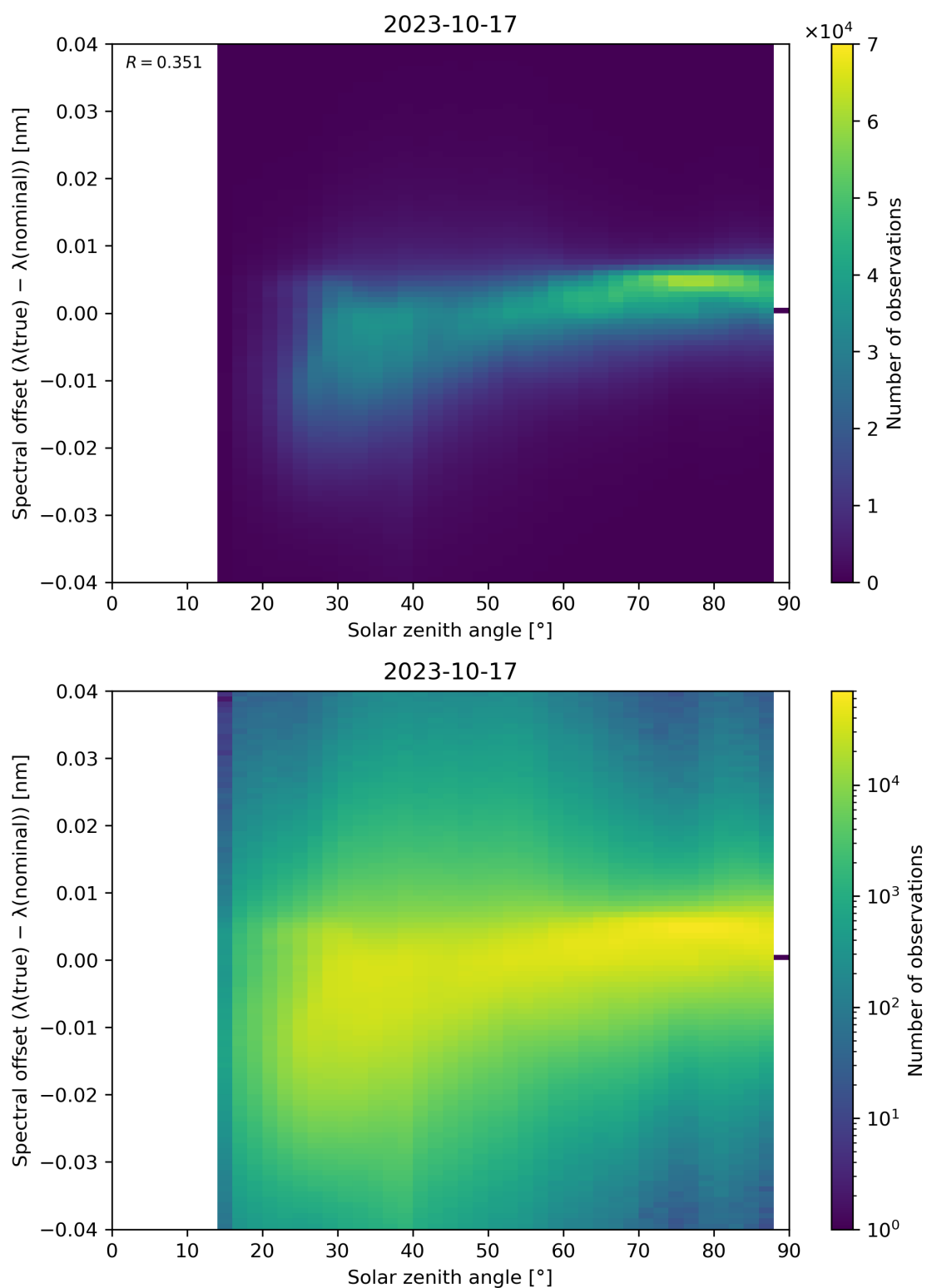
Figure 128: Scatter density plot of “Solar zenith angle” against “Spectral offset ( \lambda(\text{true}) - \lambda(\text{nominal}) )” for 2023-10-17 to 2023-10-18.
