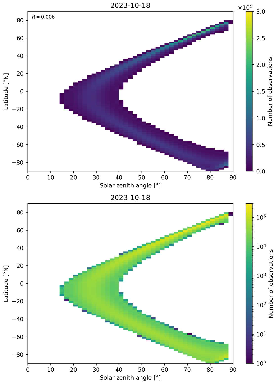
Figure 124: Scatter density plot of “Solar zenith angle” against “Latitude” for 2023-10-17 to 2023-10-19.
