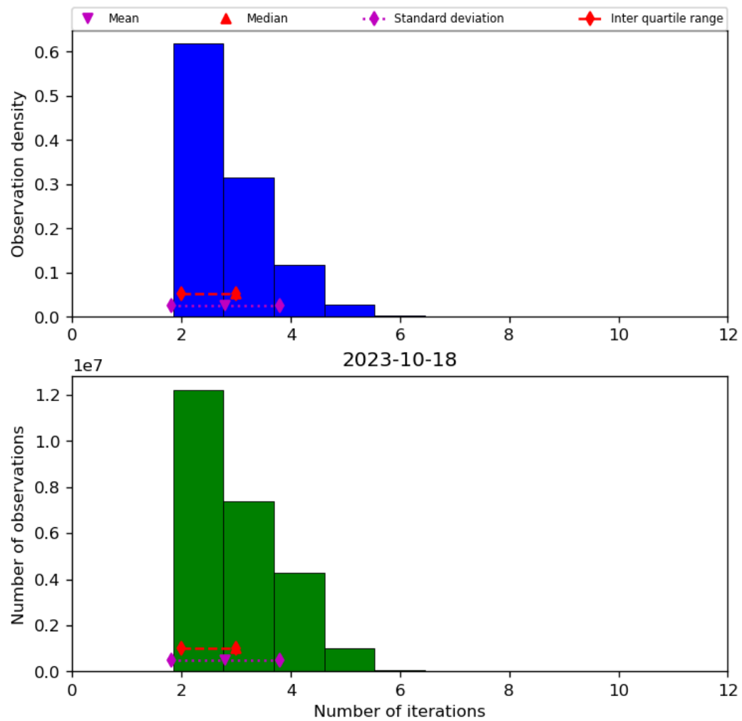
Figure 39: Histogram of “Number of iterations” for 2023-10-17 to 2023-10-19
