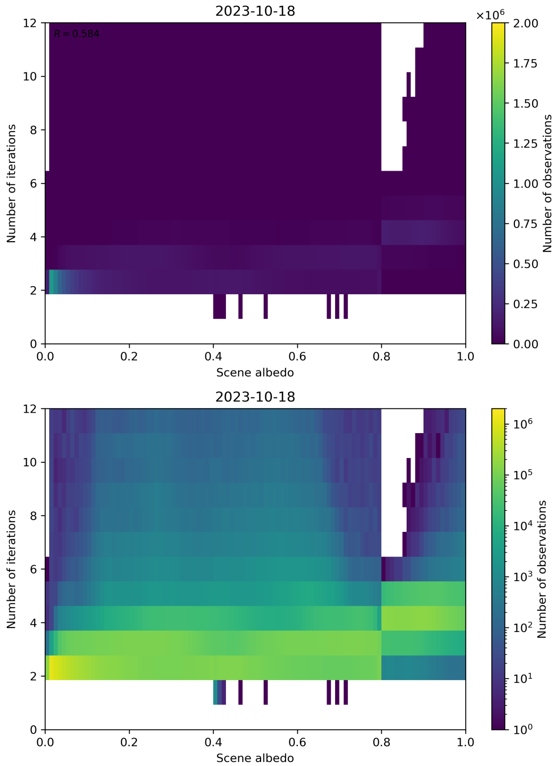
Figure 115: Scatter density plot of “Scene albedo” against “Number of iterations” for 2023-10-17 to 2023-10-19.
