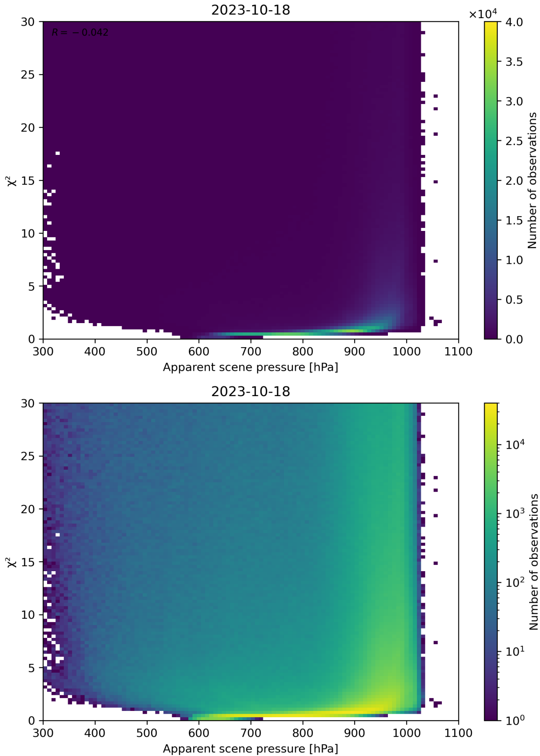
Figure 63: Scatter density plot of “Apparent scene pressure” against “ \chi^2 ” for 2023-10-17 to 2023-10-19.
