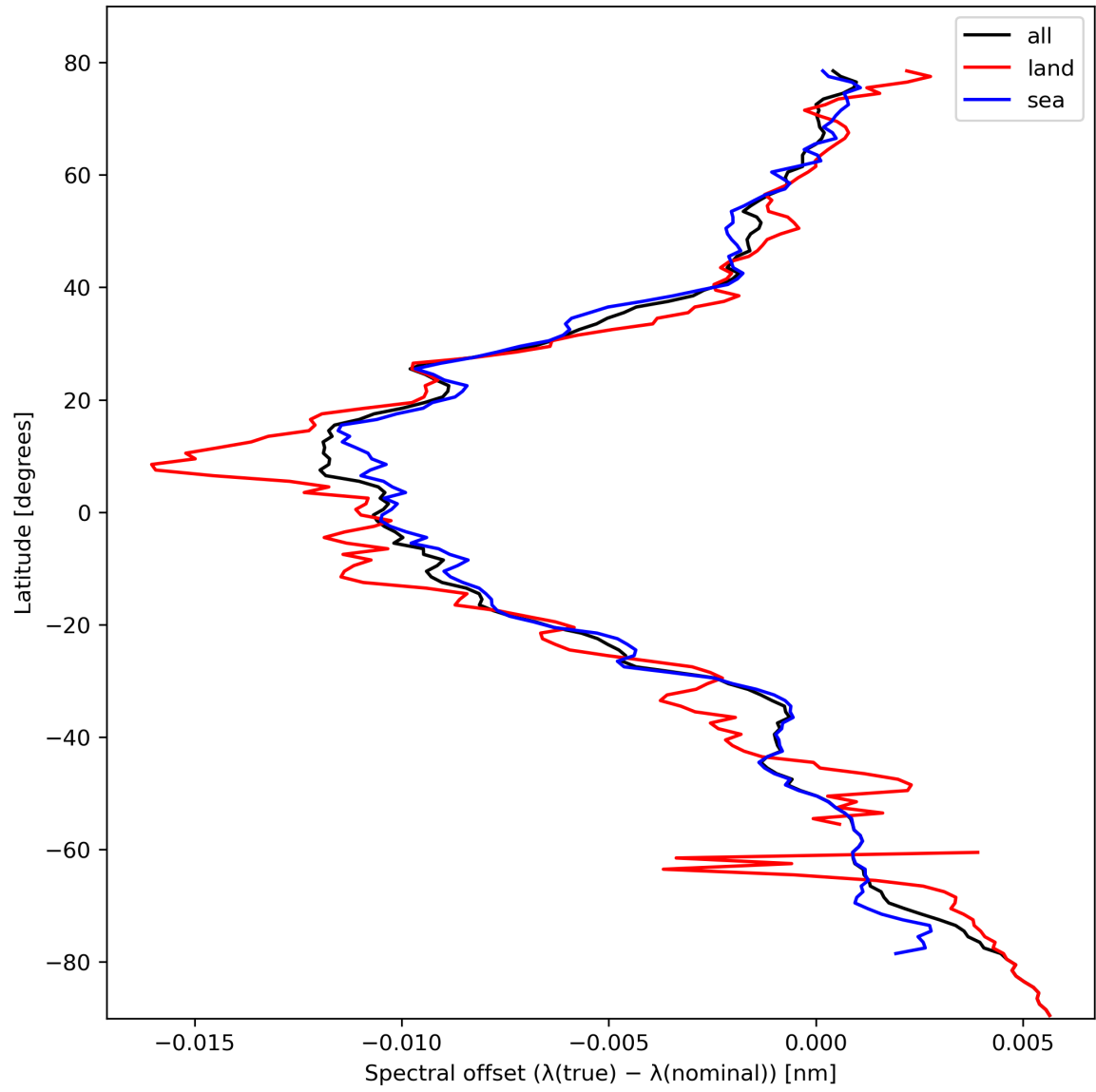
Figure 28: Zonal average of “Spectral offset ( \lambda(\text{true}) - \lambda(\text{nominal}) )” for 2023-10-17 to 2023-10-19.
