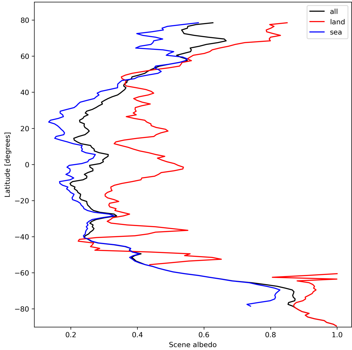
Figure 17: Zonal average of “Scene albedo” for 2023-10-17 to 2023-10-19.
