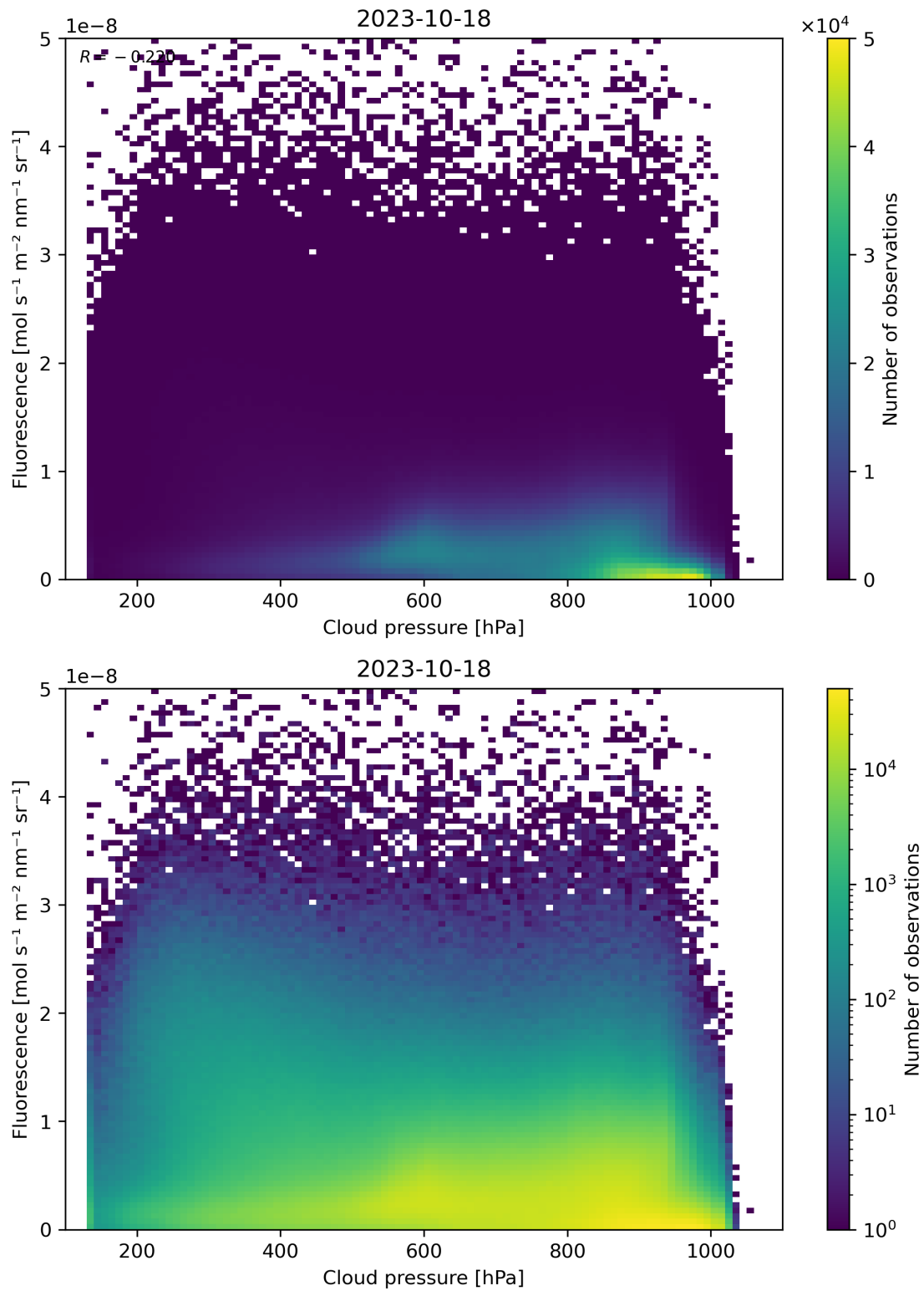
Figure 88: Scatter density plot of “Cloud pressure” against “Fluorescence” for 2023-10-17 to 2023-10-19.
