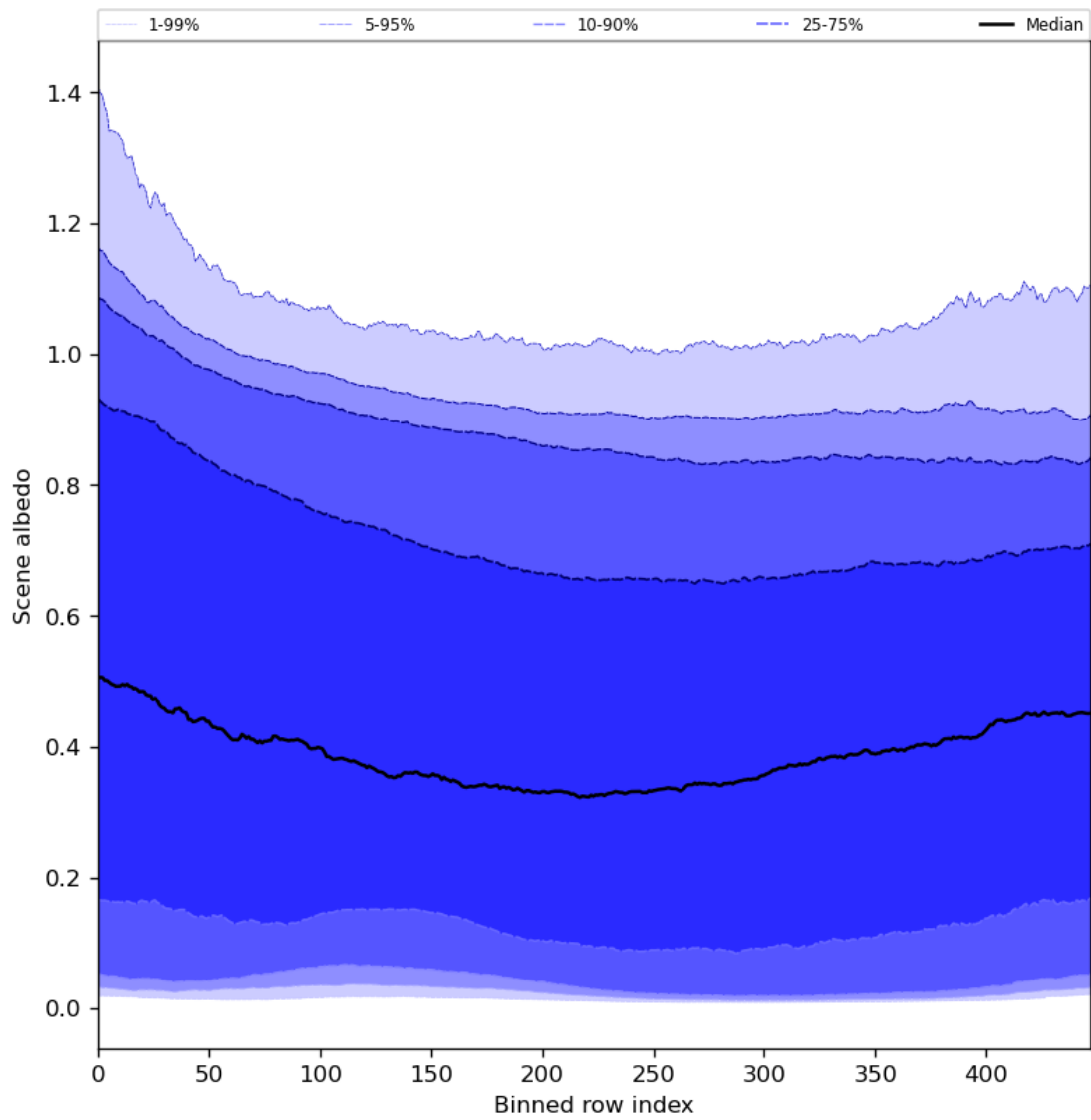
Figure 51: Along track statistics of “Scene albedo” for 2023-10-17 to 2023-10-19
