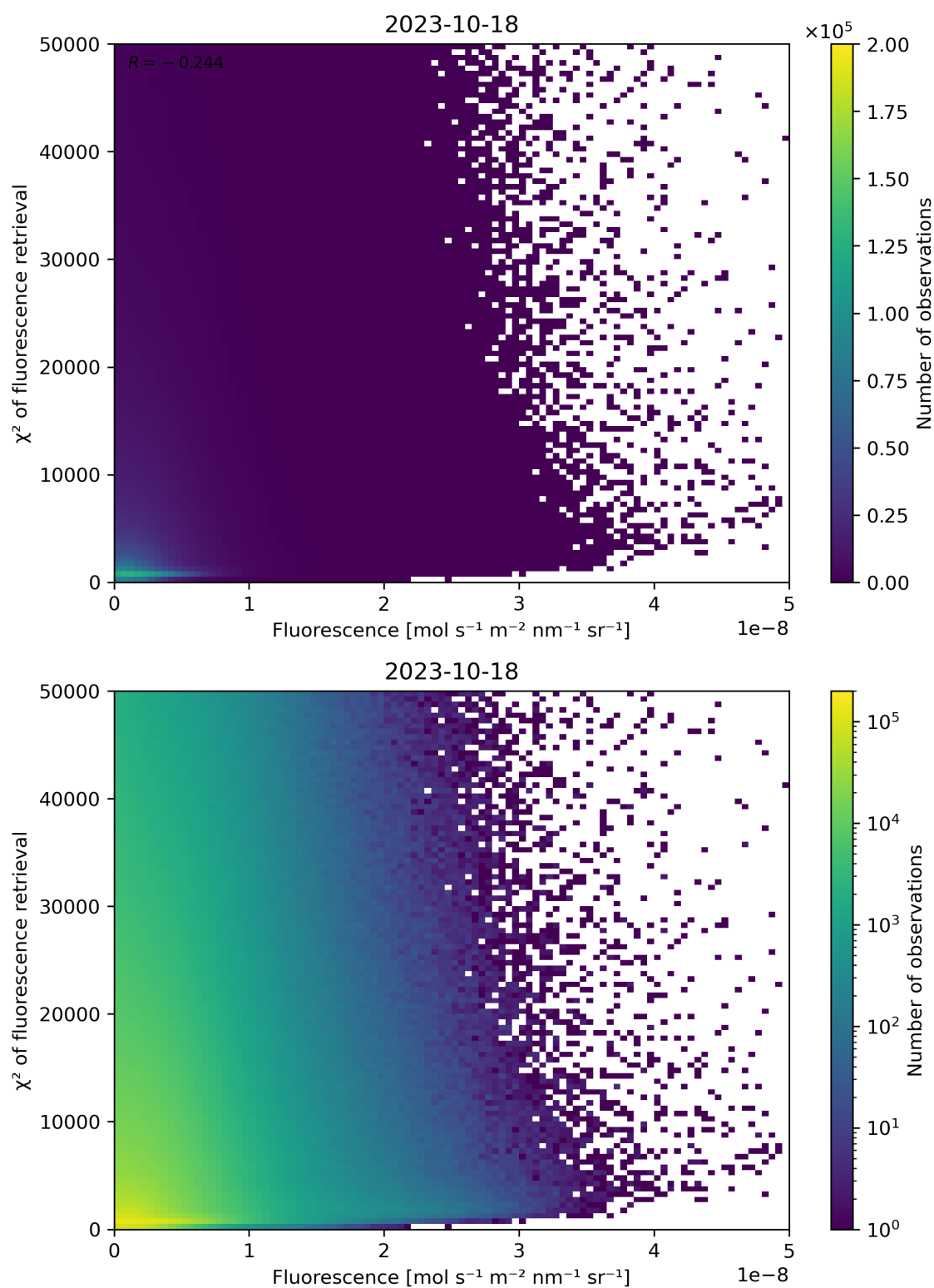
Figure 93: Scatter density plot of “Fluorescence” against “ \chi^2 of fluorescence retrieval” for 2023-10-17 to 2023-10-19.
