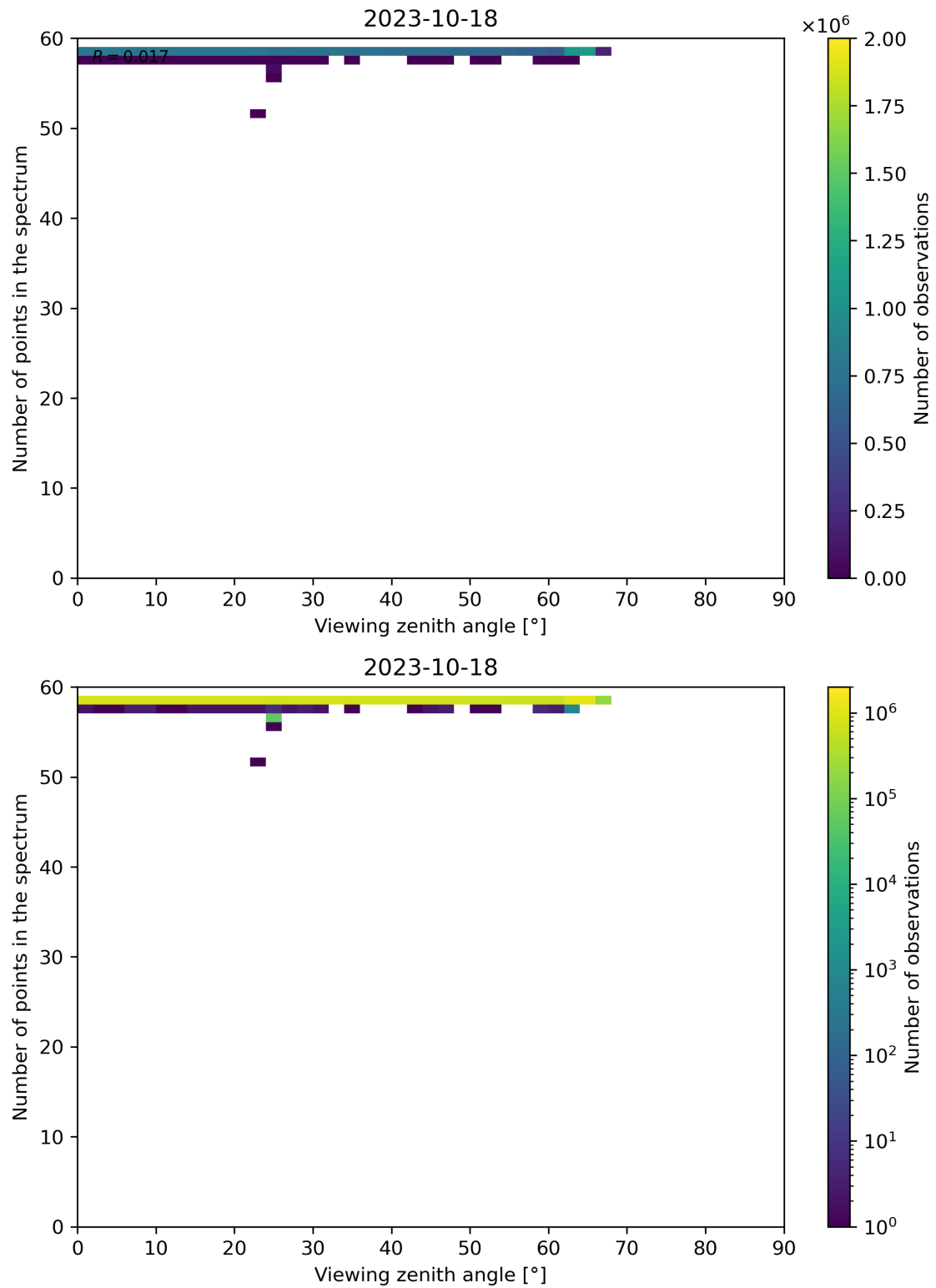
Figure 137: Scatter density plot of “Viewing zenith angle” against “Number of points in the spectrum” for 2023-10-17 to 2023-10-19.
