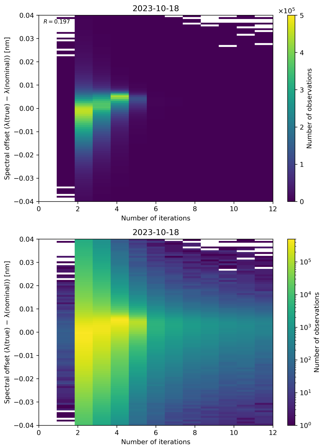
Figure 109: Scatter density plot of “Number of iterations” against “Spectral offset ( \lambda(\text{true}) - \lambda(\text{nominal}) )” for 2023-10-17 to 2023-10-19.
