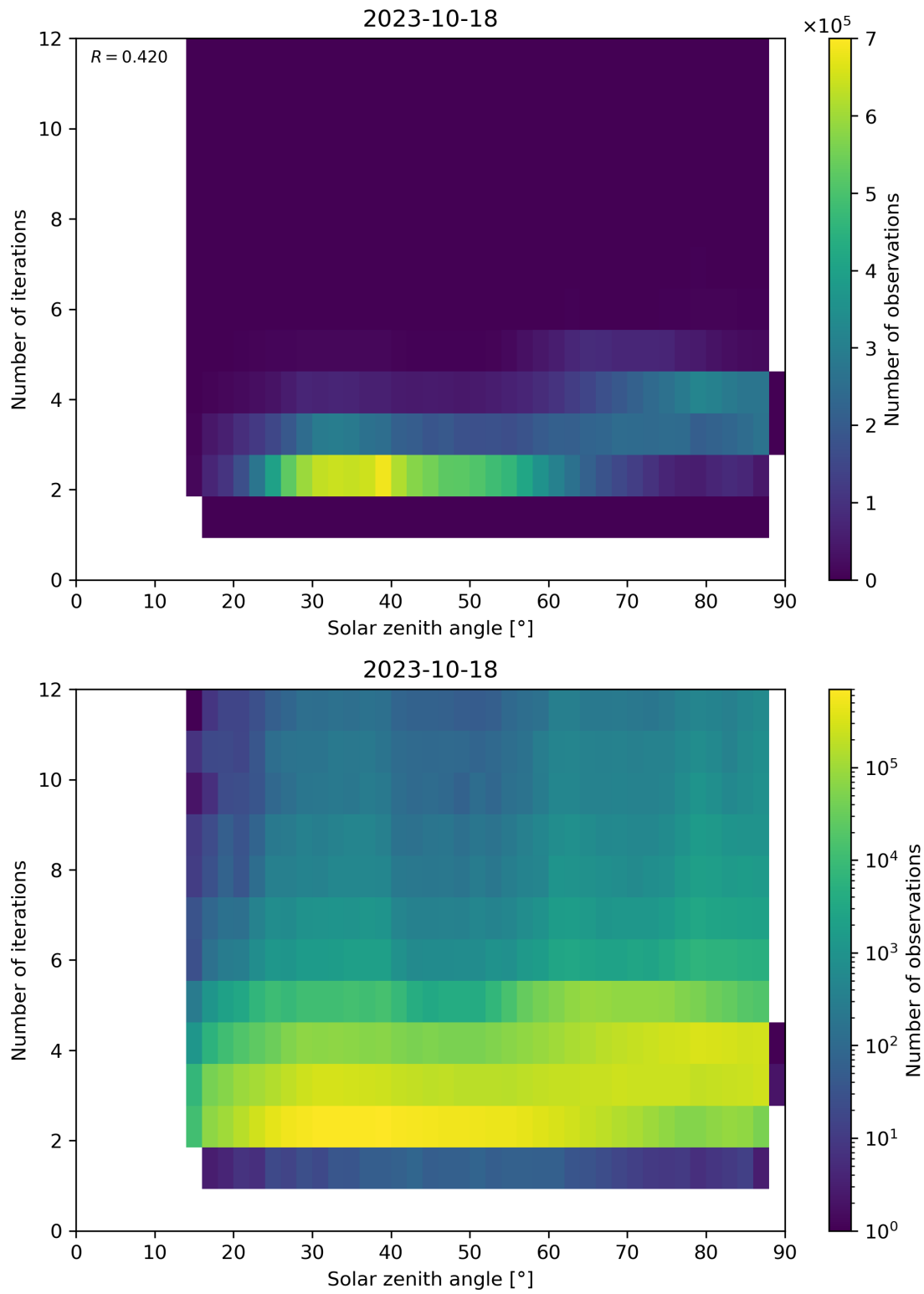
Figure 125: Scatter density plot of “Solar zenith angle” against “Number of iterations” for 2023-10-17 to 2023-10-19.
