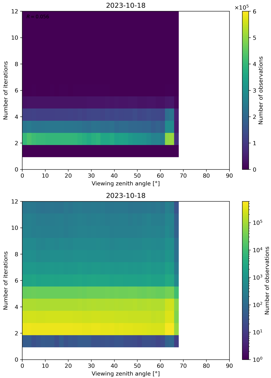
Figure 136: Scatter density plot of “Viewing zenith angle” against “Number of iterations” for 2023-10-17 to 2023-10-19.
