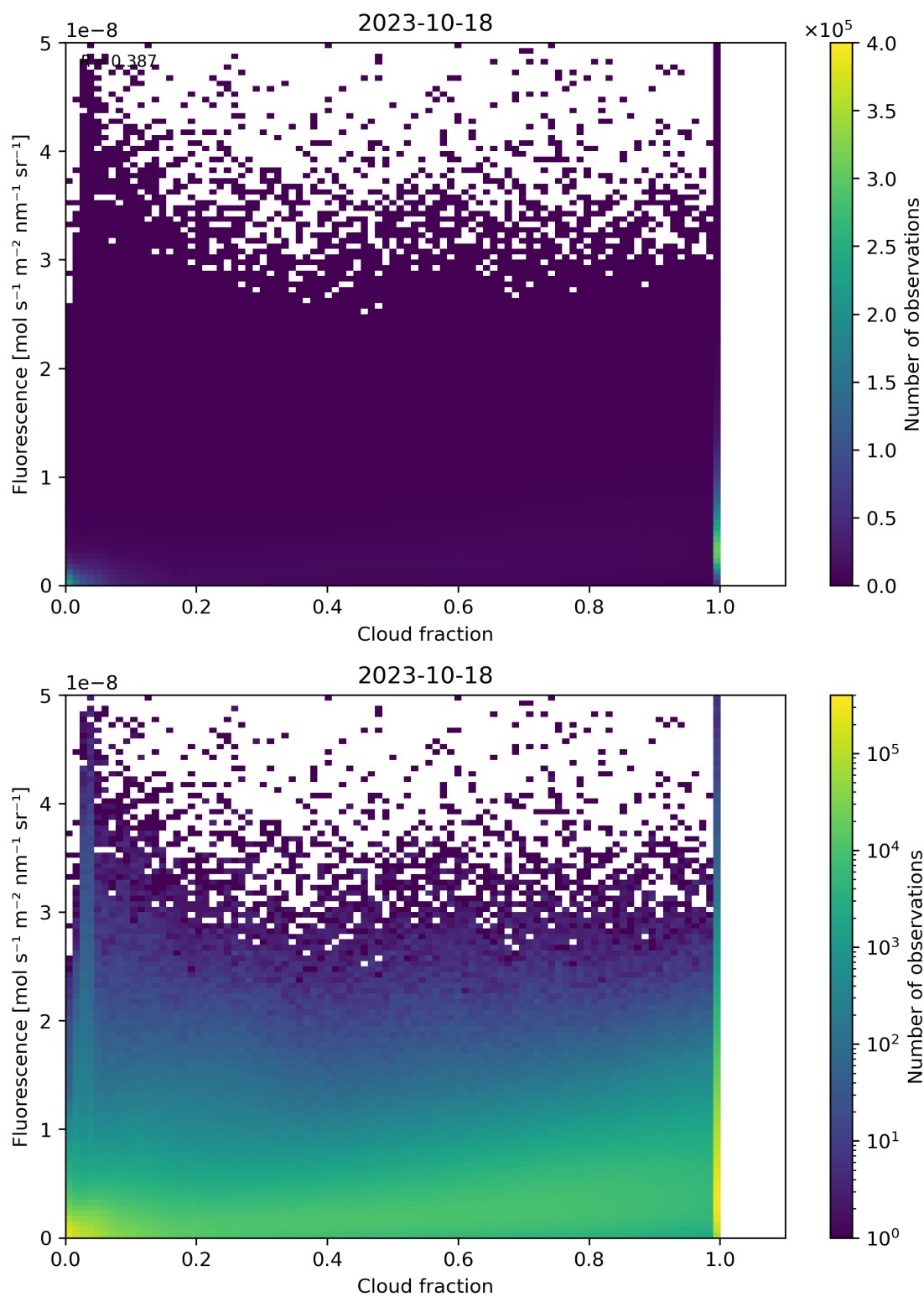
Figure 79: Scatter density plot of “Cloud fraction” against “Fluorescence” for 2023-10-17 to 2023-10-19.
