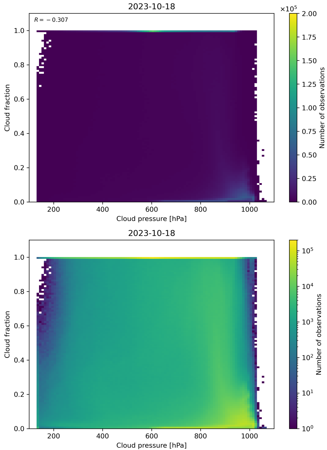
Figure 87: Scatter density plot of “Cloud pressure” against “Cloud fraction” for 2023-10-17 to 2023-10-19.
