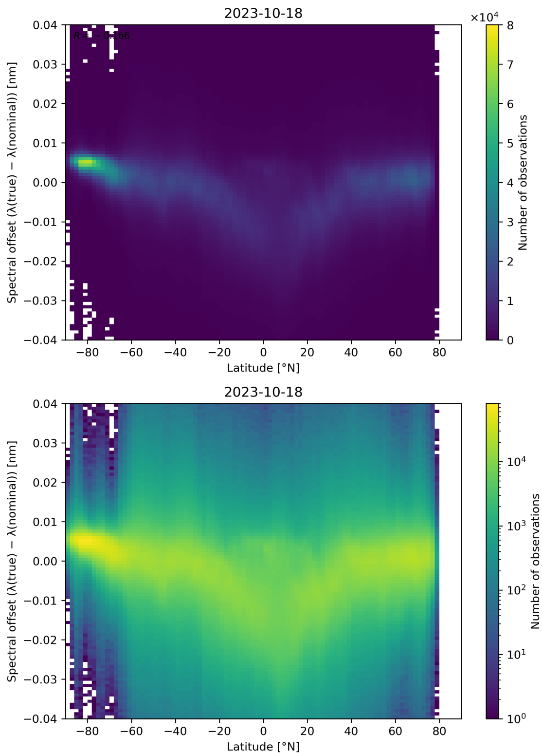
Figure 105: Scatter density plot of “Latitude” against “Spectral offset ( \lambda(\text{true}) - \lambda(\text{nominal}) )” for 2023-10-17 to 2023-10-19.
