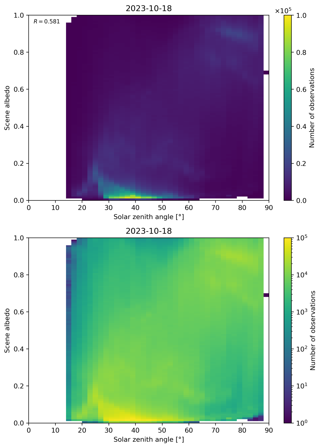
Figure 127: Scatter density plot of “Solar zenith angle” against “Scene albedo” for 2023-10-17 to 2023-10-19.
