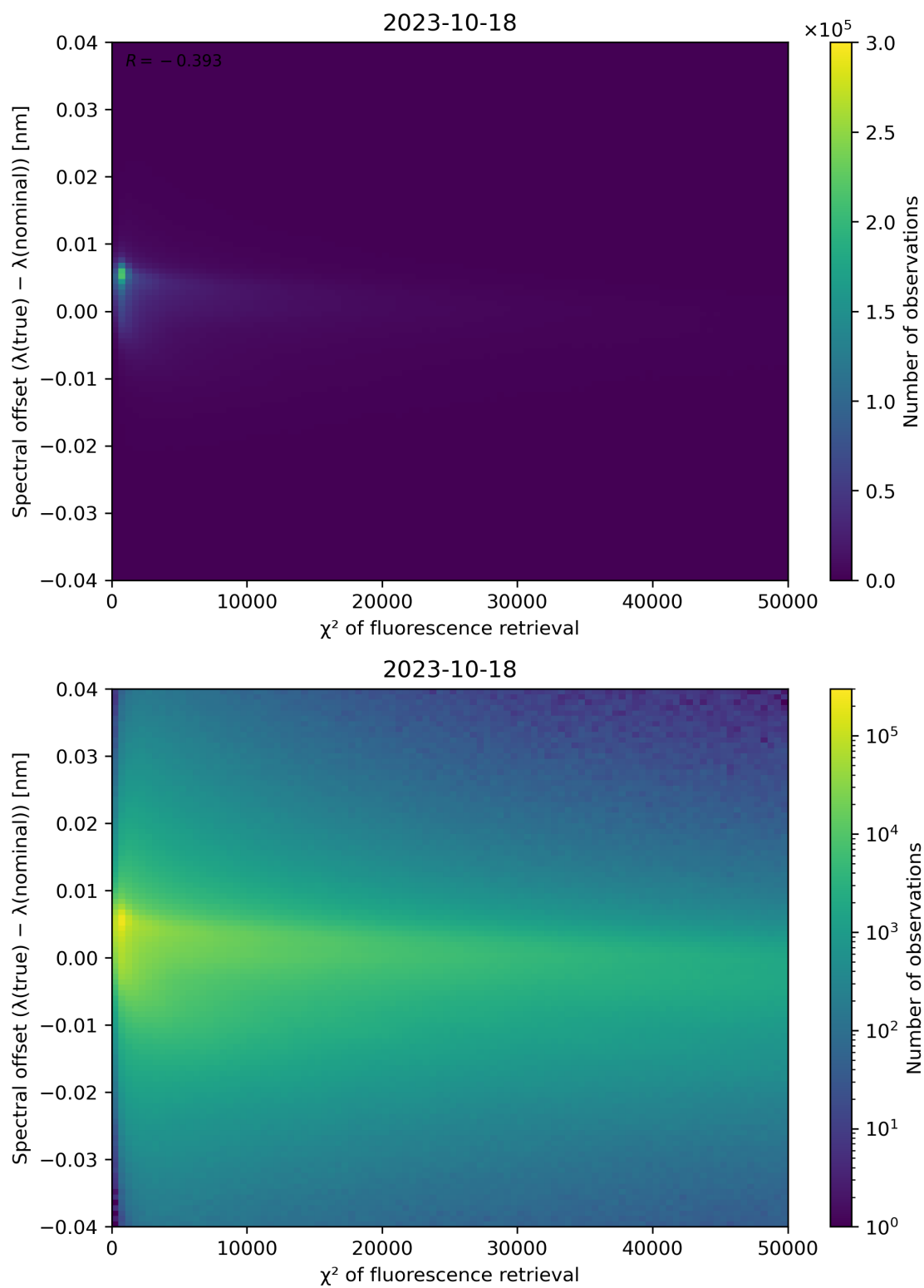
Figure 72: Scatter density plot of " \chi^2 of fluorescence retrieval" against "Spectral offset ( \lambda(\text{true}) - \lambda(\text{nominal}) )" for 2023-10-17 to 2023-10-19.
