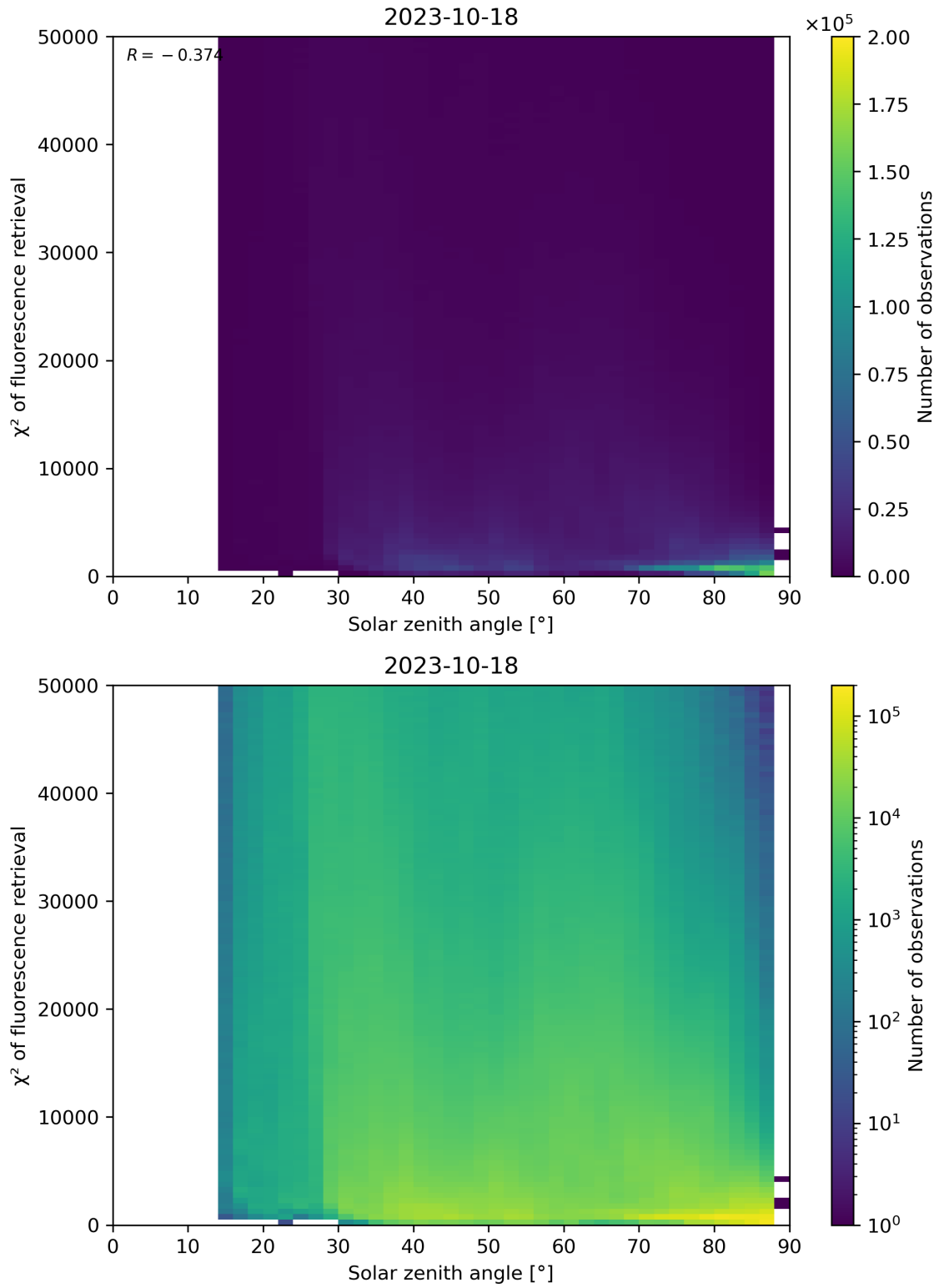
Figure 120: Scatter density plot of “Solar zenith angle” against “ \chi^2 of fluorescence retrieval” for 2023-10-17 to 2023-10-19.
