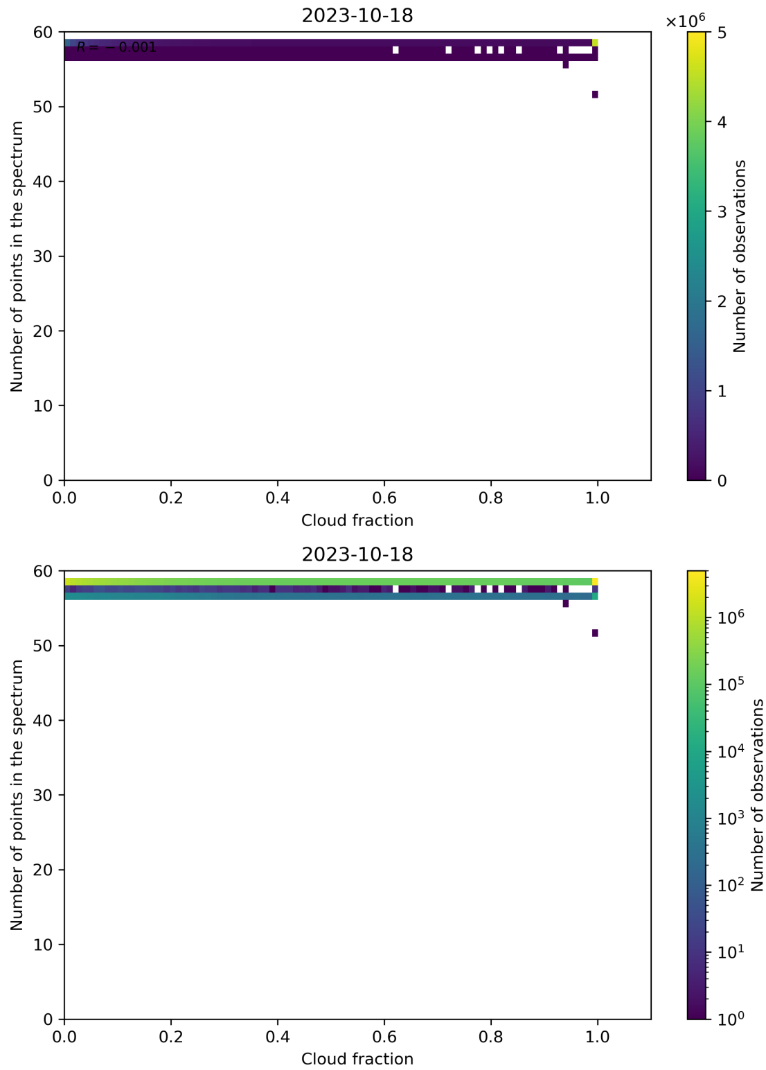
Figure 81: Scatter density plot of “Cloud fraction” against “Number of points in the spectrum” for 2023-10-17 to 2023-10-19.
