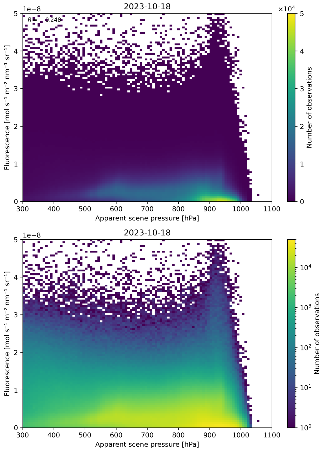
Figure 65: Scatter density plot of “Apparent scene pressure” against “Fluorescence” for 2023-10-17 to 2023-10-19.
