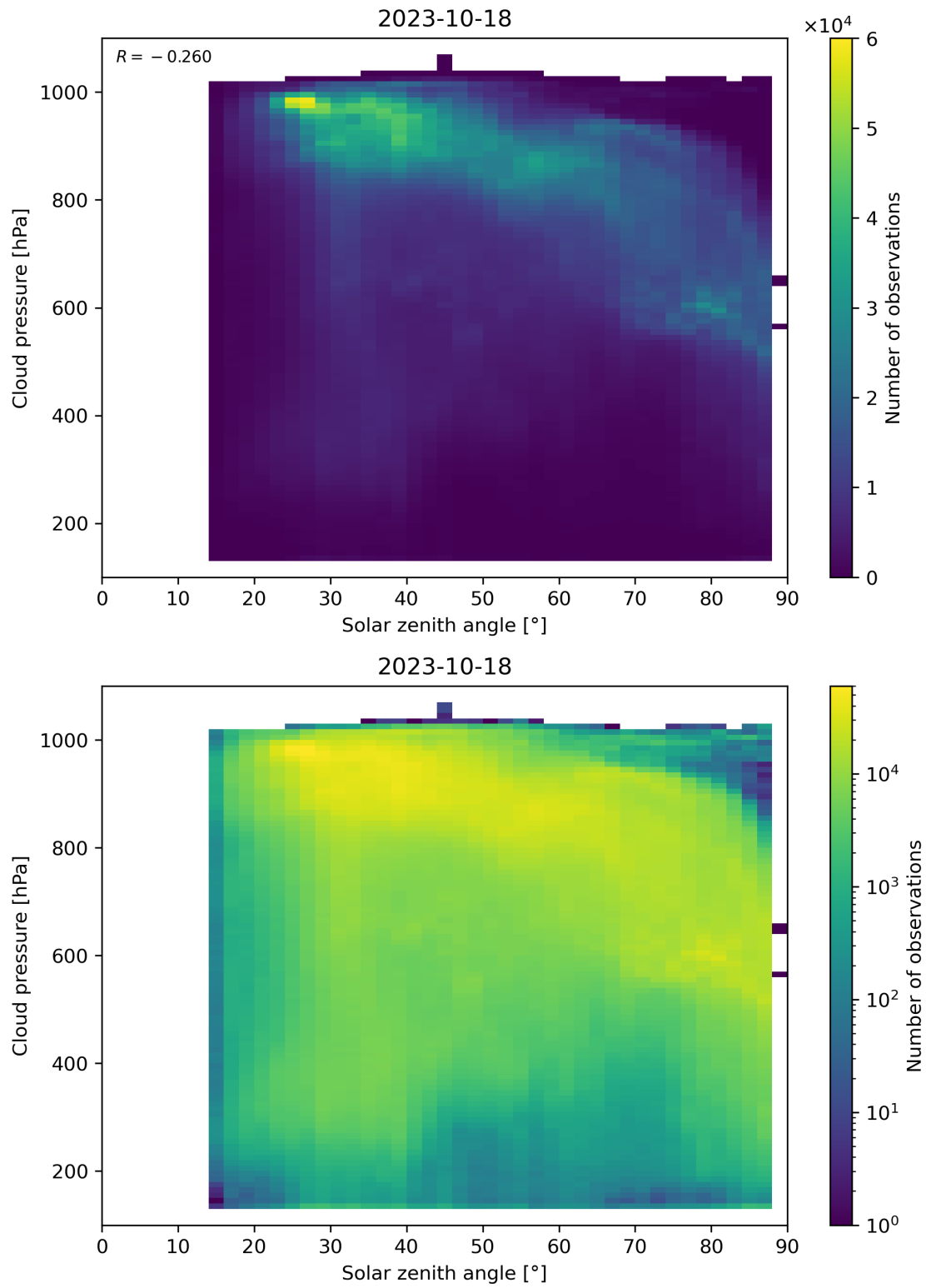
Figure 122: Scatter density plot of “Solar zenith angle” against “Cloud pressure” for 2023-10-17 to 2023-10-19.
