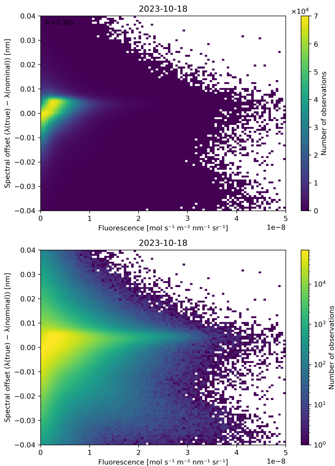
Figure 95: Scatter density plot of “Fluorescence” against “Spectral offset ( \lambda(\text{true}) - \lambda(\text{nominal}) )” for 2023-10-17 to 2023-10-19.
