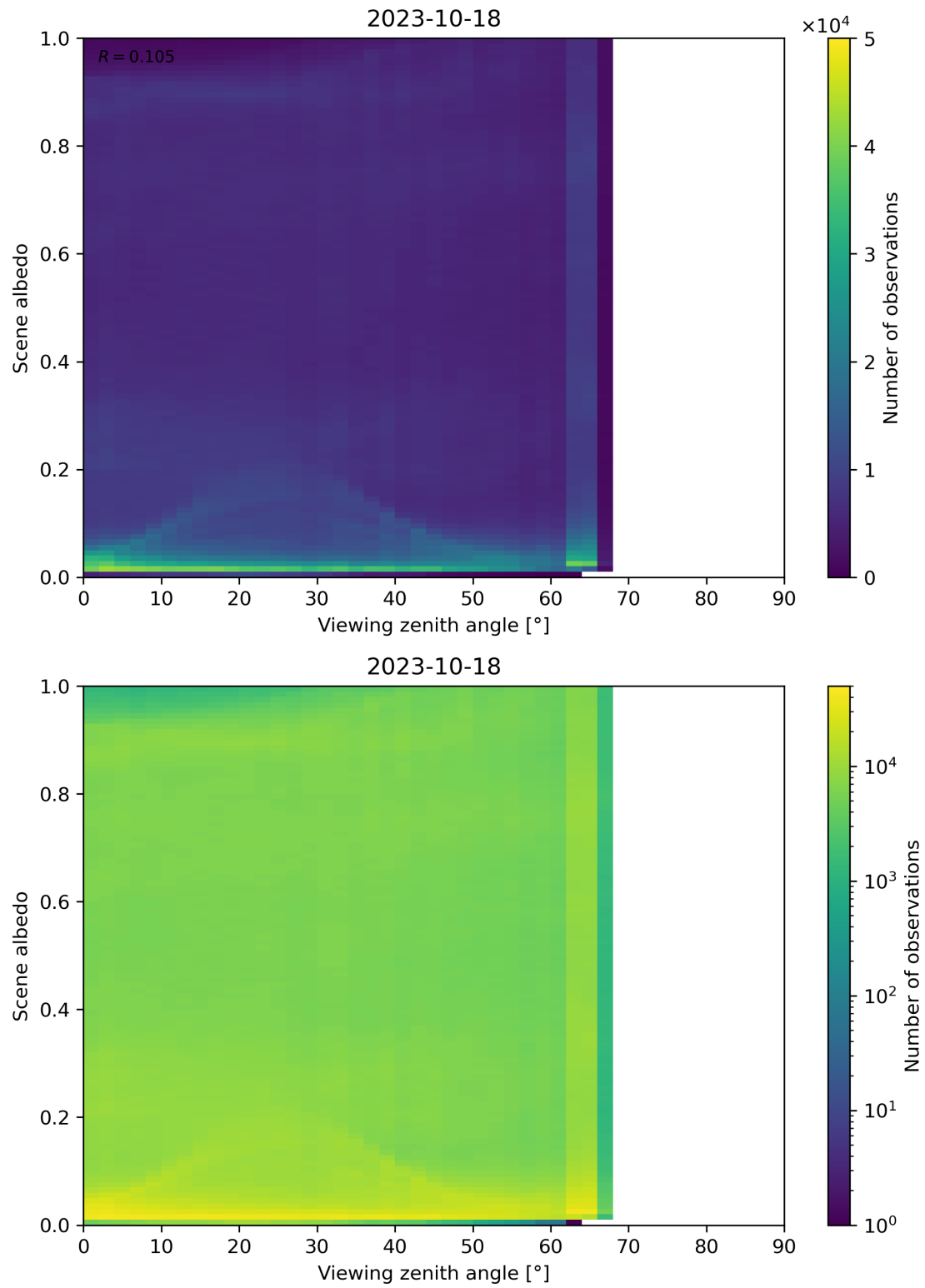
Figure 138: Scatter density plot of “Viewing zenith angle” against “Scene albedo” for 2023-10-17 to 2023-10-19.
