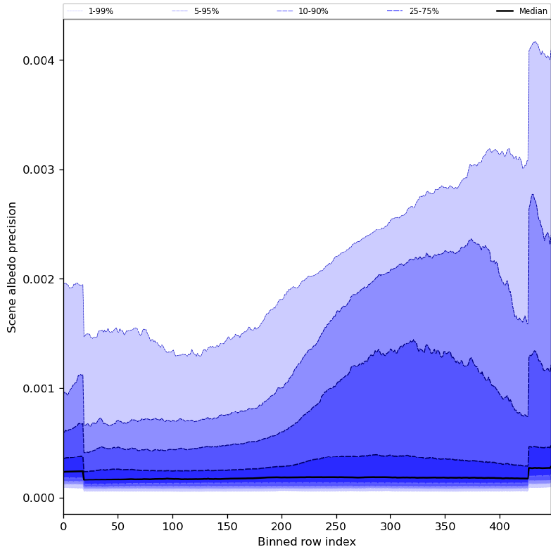
Figure 52: Along track statistics of “Scene albedo precision” for 2023-10-17 to 2023-10-19
