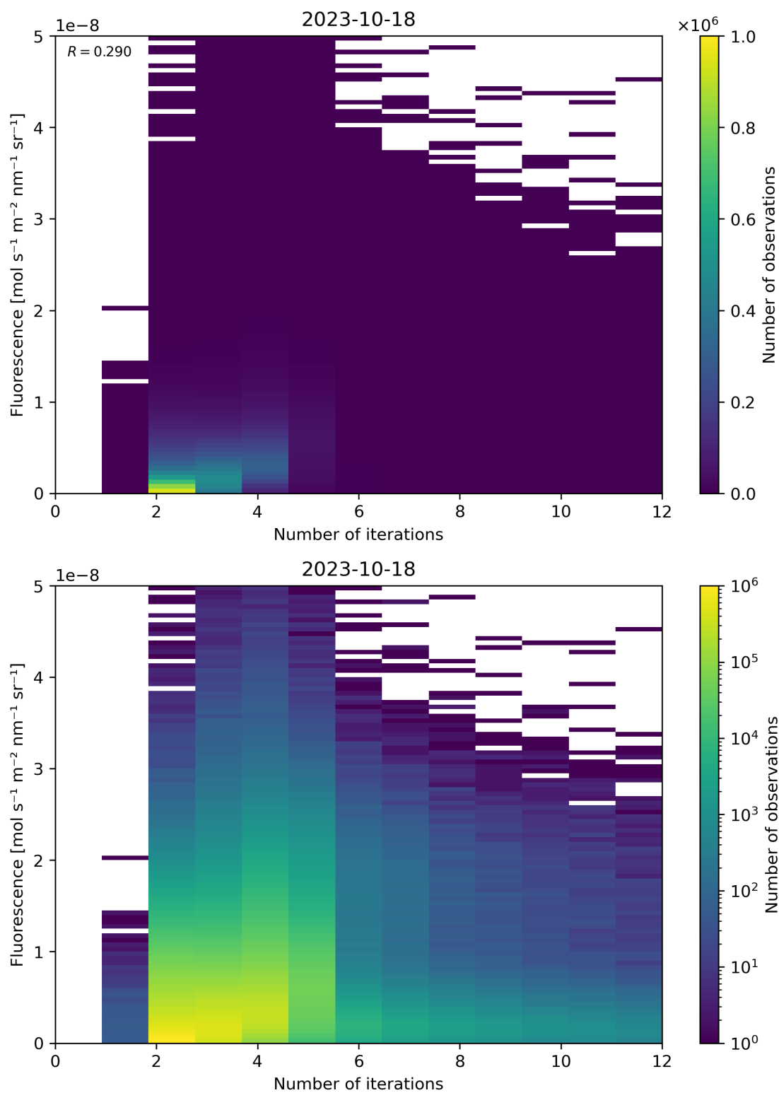
Figure 107: Scatter density plot of “Number of iterations” against “Fluorescence” for 2023-10-17 to 2023-10-19.
