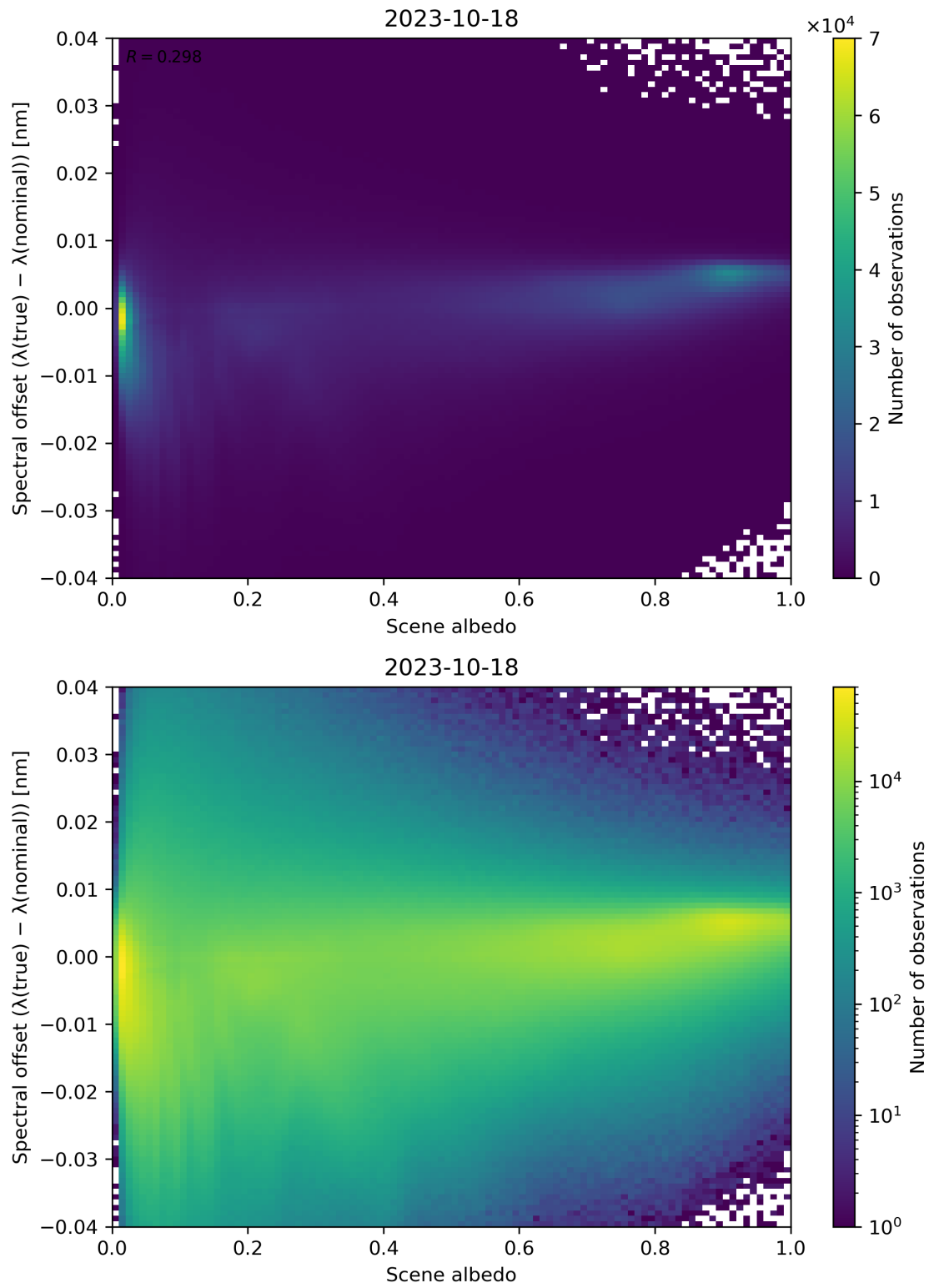
Figure 117: Scatter density plot of “Scene albedo” against “Spectral offset ( \lambda(\text{true}) - \lambda(\text{nominal}) )” for 2023-10-17 to 2023-10-19.
