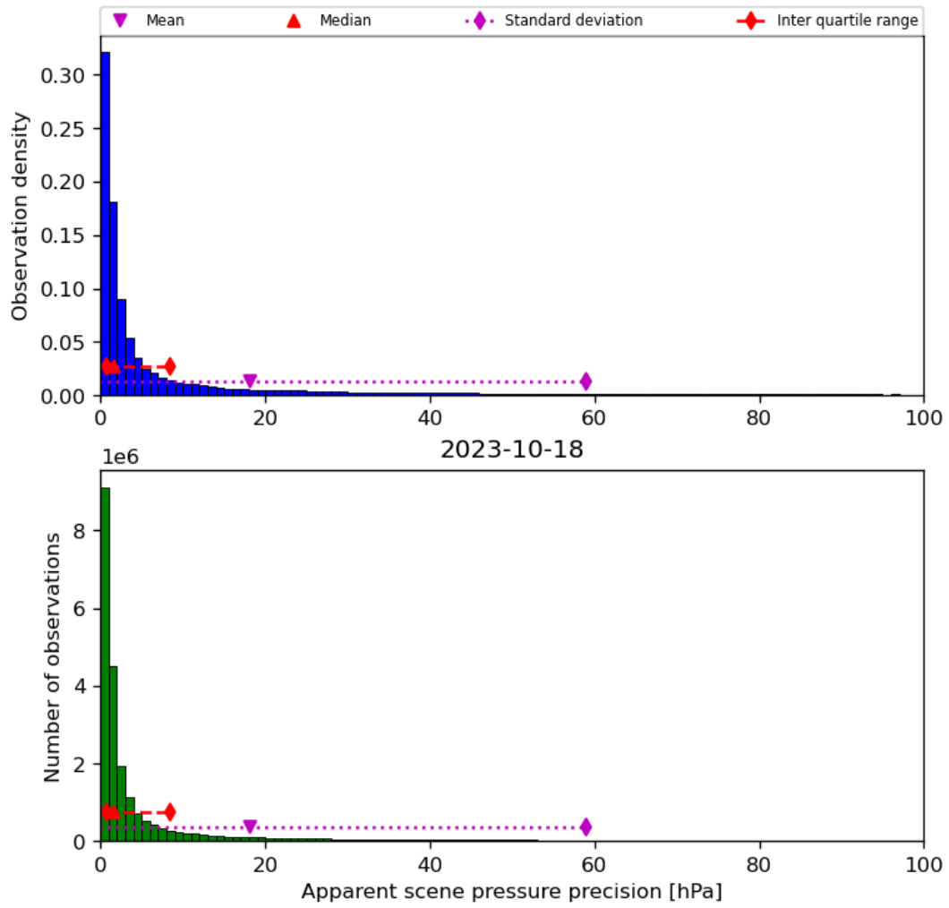
Figure 37: Histogram of “Apparent scene pressure precision” for 2023-10-17 to 2023-10-19
