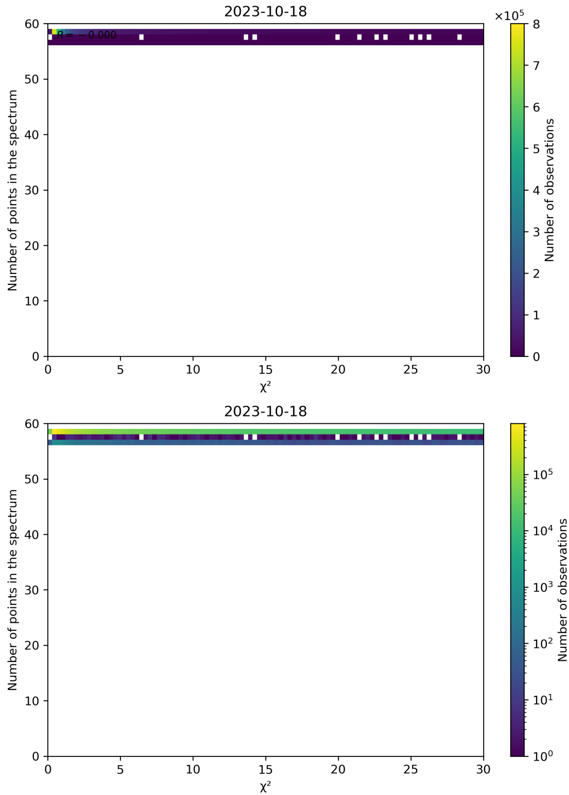
Figure 74: Scatter density plot of " \chi^2 " against "Number of points in the spectrum" for 2023-10-17 to 2023-10-19.
