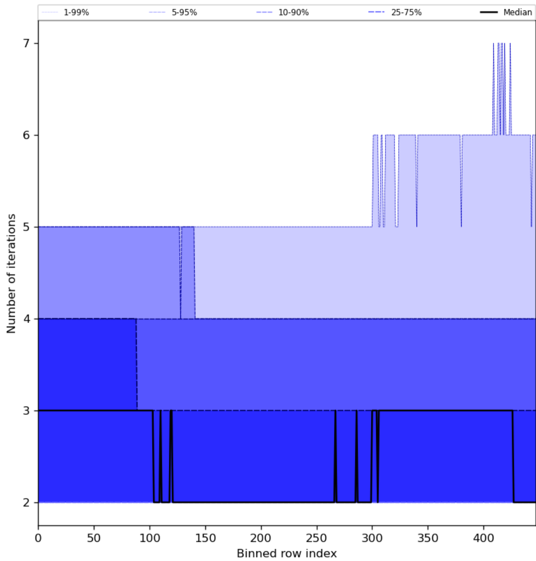
Figure 56: Along track statistics of “Number of iterations” for 2023-10-17 to 2023-10-19
