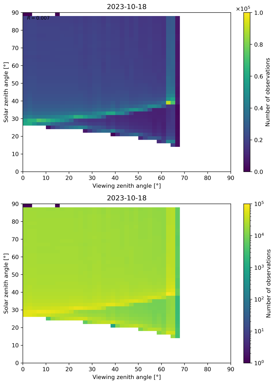
Figure 139: Scatter density plot of “Viewing zenith angle” against “Solar zenith angle” for 2023-10-17 to 2023-10-19.
