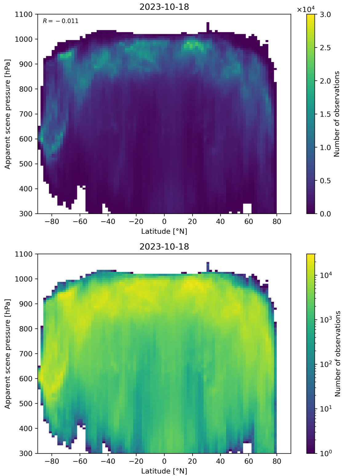
Figure 96: Scatter density plot of “Latitude” against “Apparent scene pressure” for 2023-10-17 to 2023-10-19.
