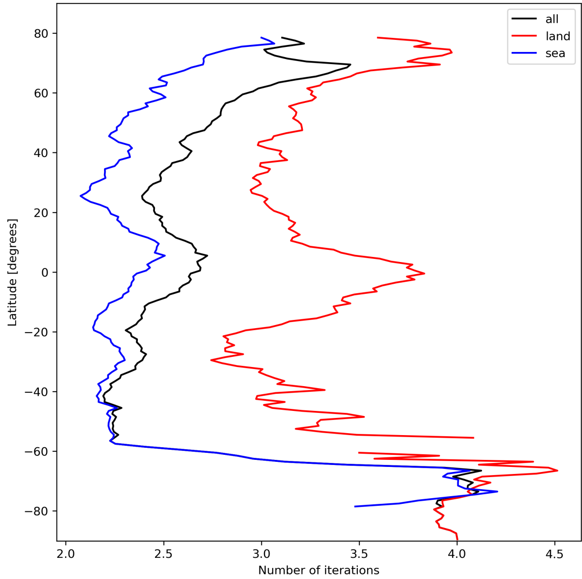
Figure 22: Zonal average of “Number of iterations” for 2023-10-17 to 2023-10-19.
