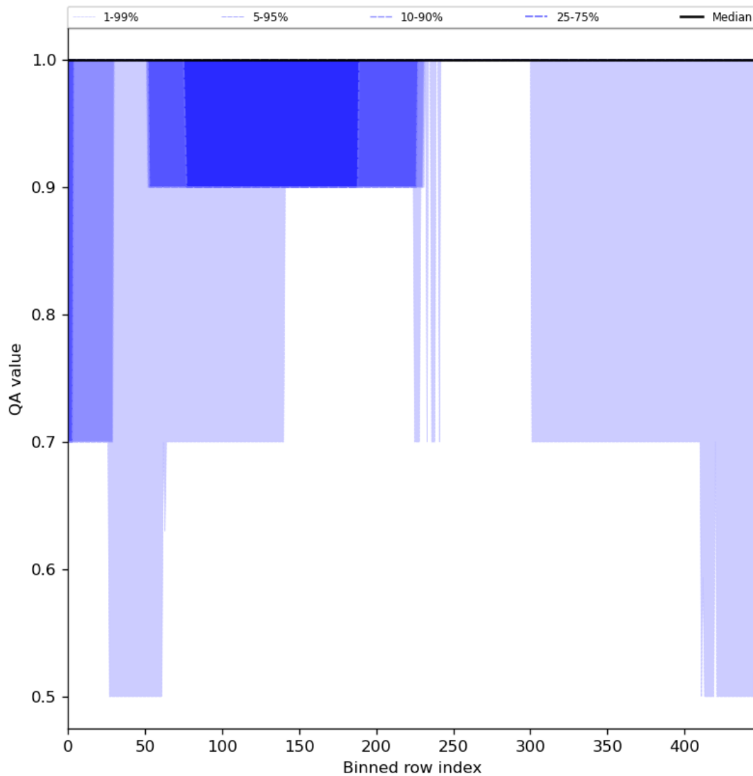
Figure 46: Along track statistics of “QA value” for 2023-10-17 to 2023-10-19
