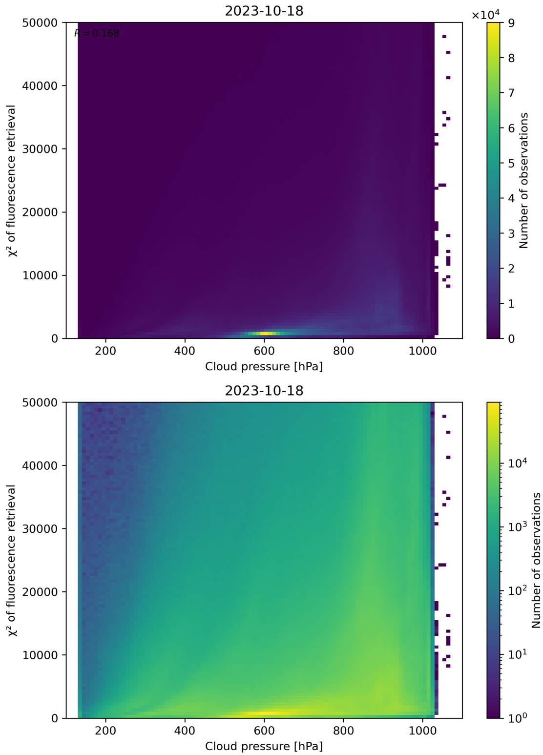
Figure 86: Scatter density plot of “Cloud pressure” against “ \chi^2 of fluorescence retrieval” for 2023-10-17 to 2023-10-19.
