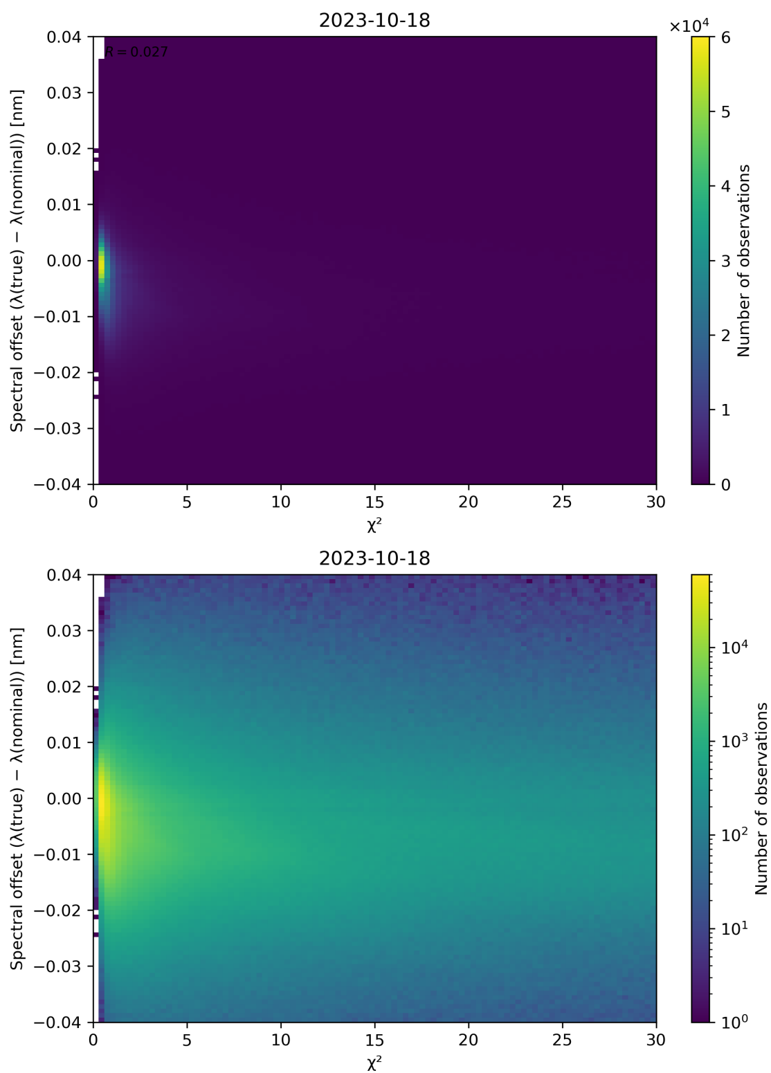
Figure 75: Scatter density plot of “ \chi^2 ” against “Spectral offset ( \lambda(\text{true}) - \lambda(\text{nominal}) )” for 2023-10-17 to 2023-10-19.
