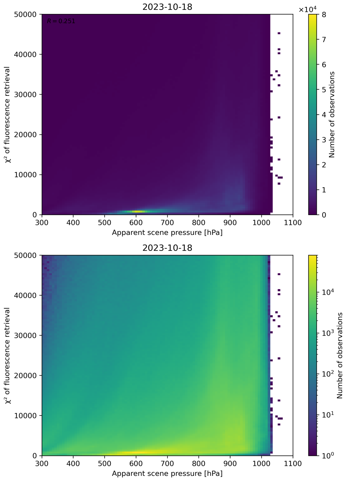
Figure 64: Scatter density plot of “Apparent scene pressure” against “ \chi^2 of fluorescence retrieval” for 2023-10-17 to 2023-10-19.
