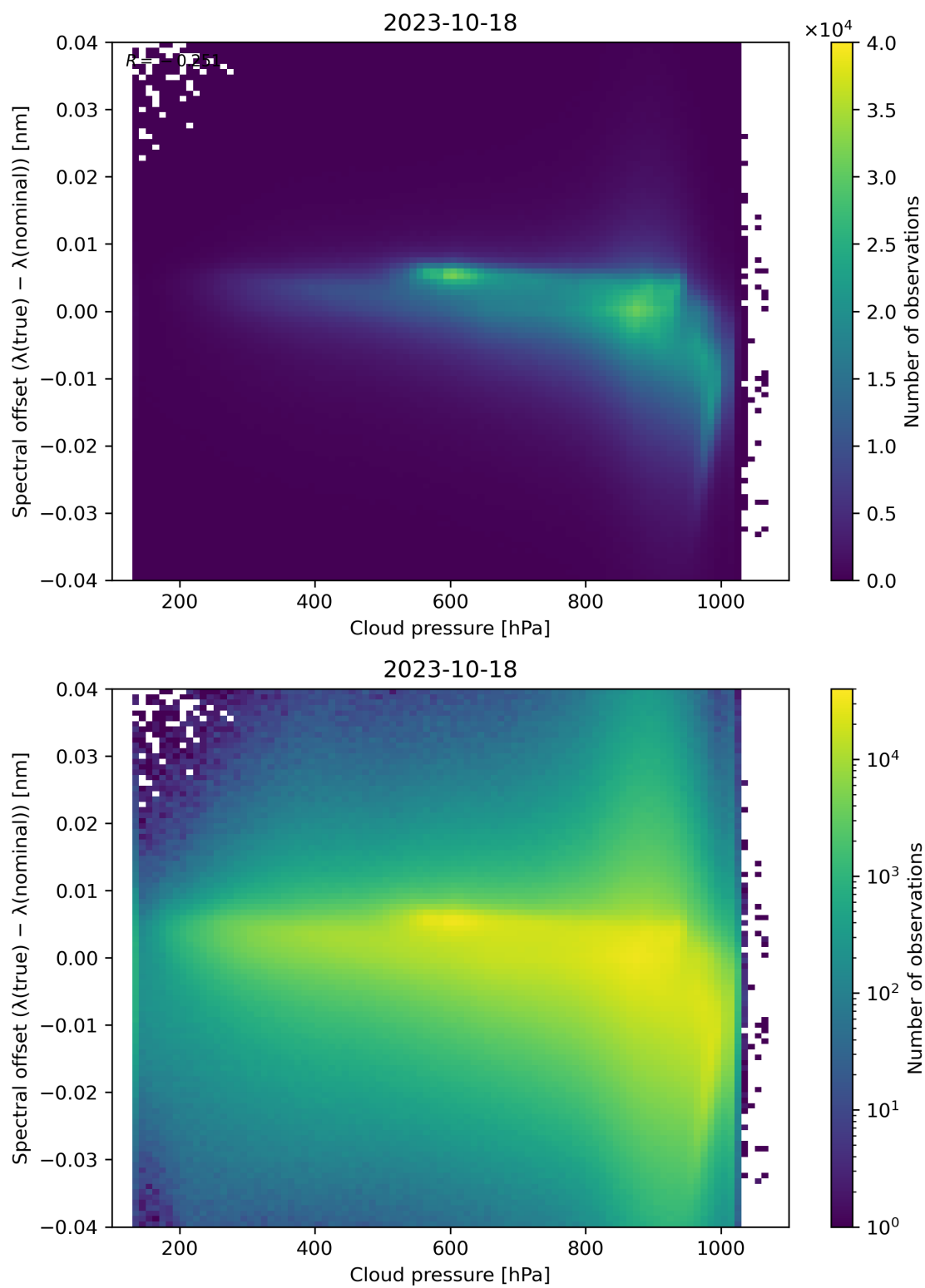
Figure 92: Scatter density plot of “Cloud pressure” against “Spectral offset ( \lambda(\text{true}) - \lambda(\text{nominal}) )” for 2023-10-17 to 2023-10-19.
