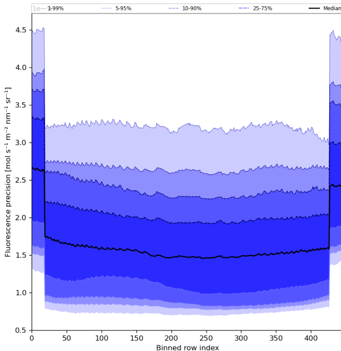
Figure 58: Along track statistics of “Fluorescence precision” for 2023-10-17 to 2023-10-19
