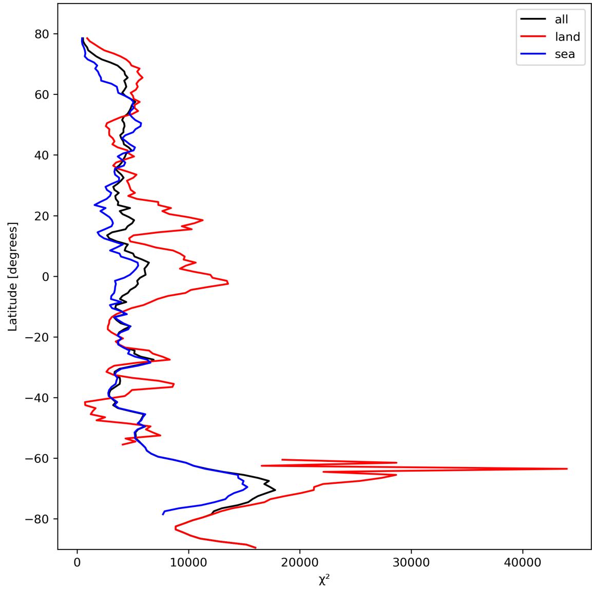
Figure 21: Zonal average of “ \chi^2 ” for 2023-10-17 to 2023-10-19.
