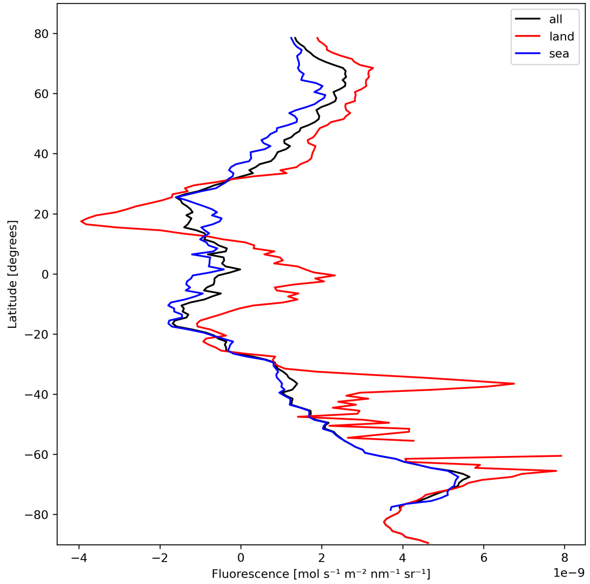
Figure 23: Zonal average of “Fluorescence” for 2023-10-17 to 2023-10-19.
