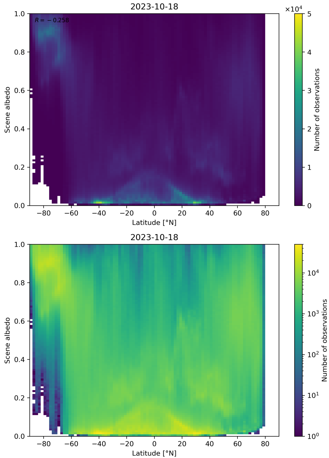
Figure 104: Scatter density plot of “Latitude” against “Scene albedo” for 2023-10-17 to 2023-10-19.
