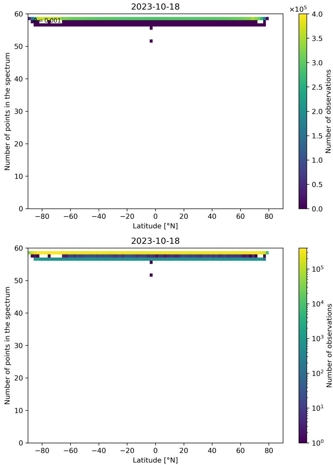
Figure 103: Scatter density plot of “Latitude” against “Number of points in the spectrum” for 2023-10-17 to 2023-10-19.
