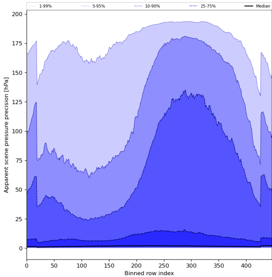
Figure 54: Along track statistics of “Apparent scene pressure precision” for 2023-10-17 to 2023-10-19
