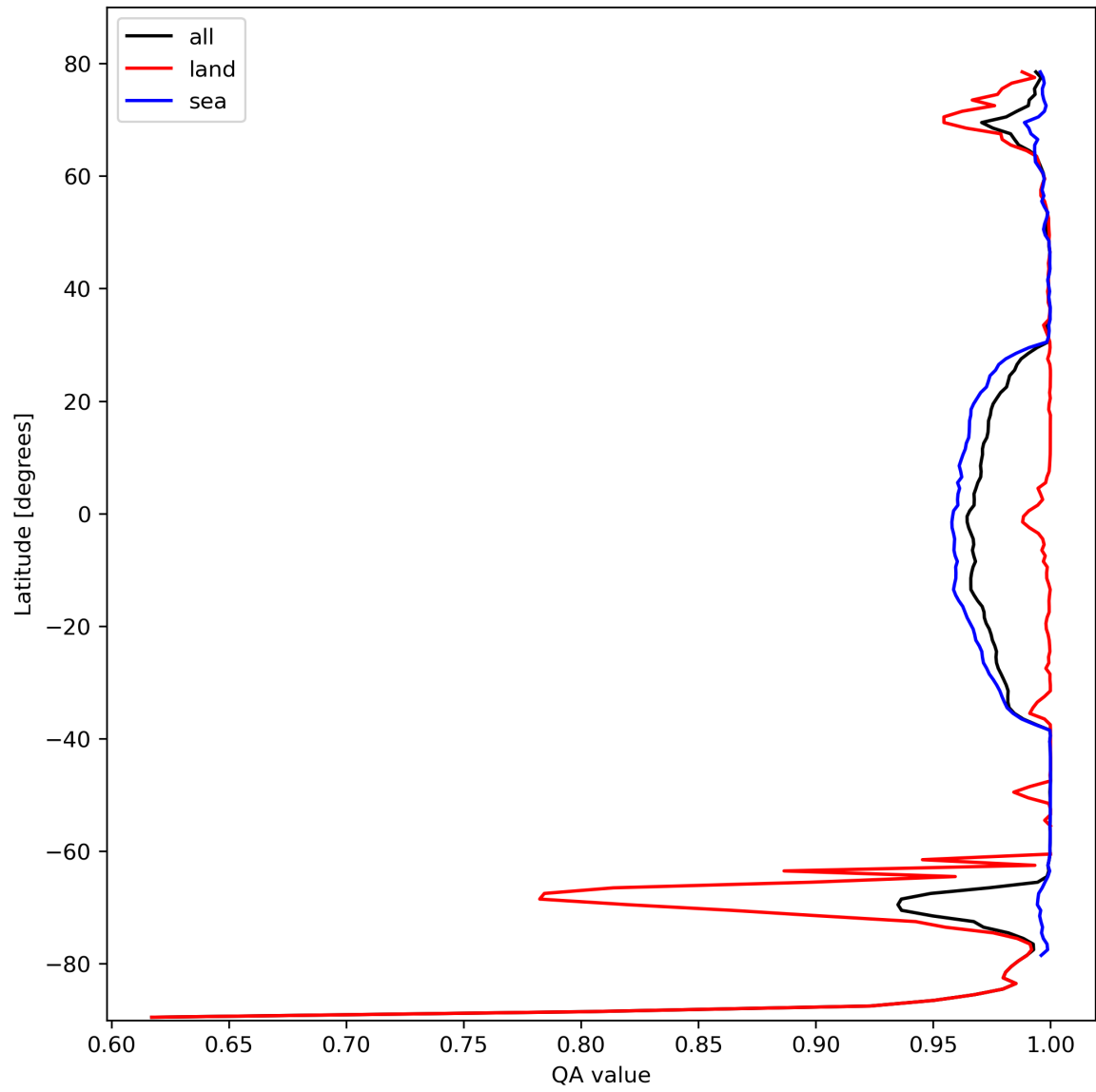
Figure 12: Zonal average of “QA value” for 2023-10-17 to 2023-10-19.
