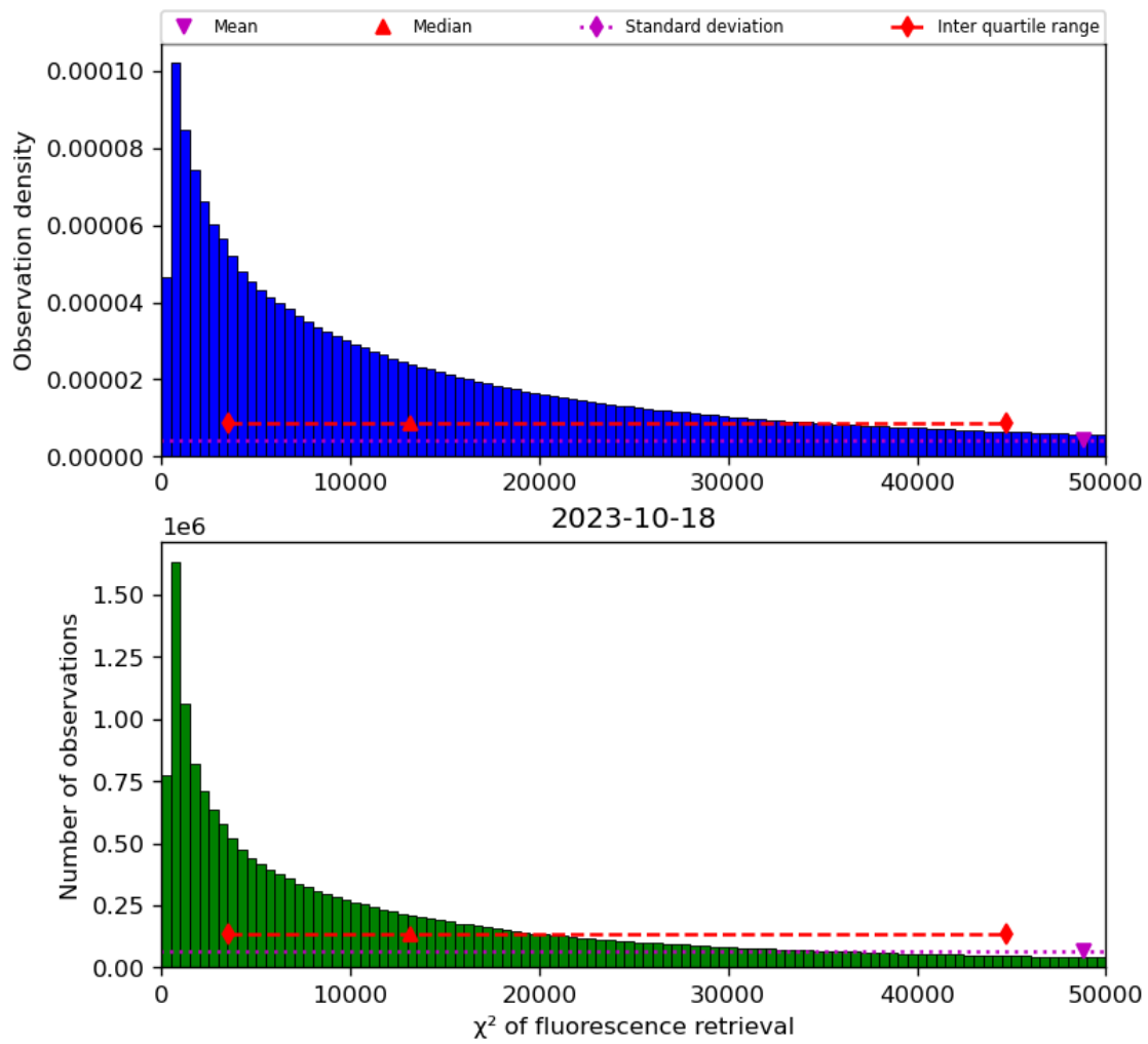
Figure 42: Histogram of “ \chi^2 of fluorescence retrieval” for 2023-10-17 to 2023-10-19
