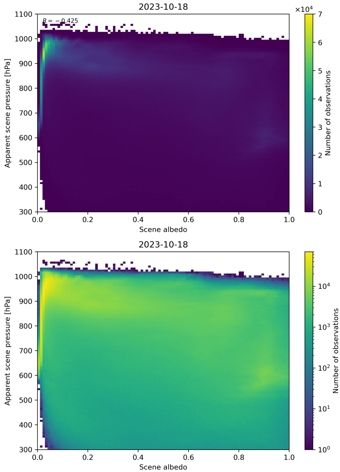
Figure 111: Scatter density plot of “Scene albedo” against “Apparent scene pressure” for 2023-10-17 to 2023-10-19.
