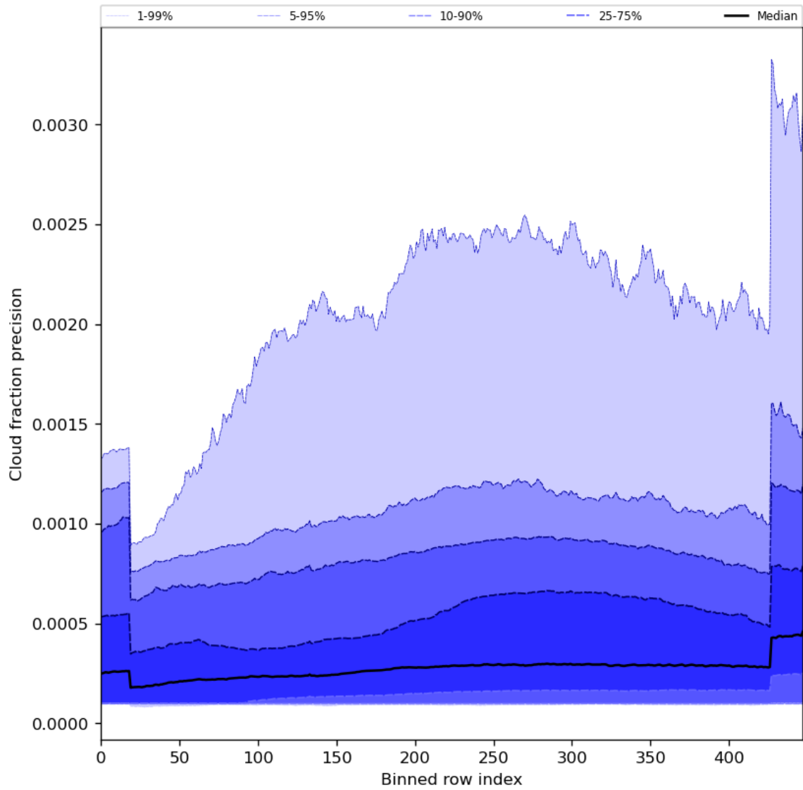
Figure 50: Along track statistics of “Cloud fraction precision” for 2023-10-17 to 2023-10-19
