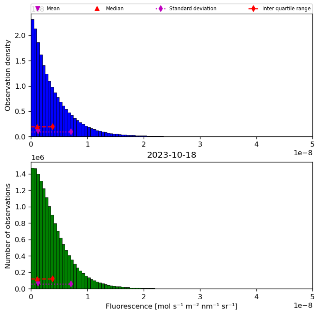
Figure 40: Histogram of “Fluorescence” for 2023-10-17 to 2023-10-19
