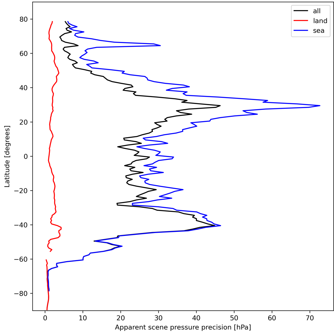
Figure 20: Zonal average of “Apparent scene pressure precision” for 2023-10-17 to 2023-10-19.
