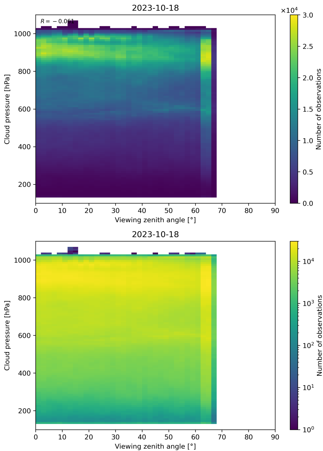
Figure 133: Scatter density plot of “Viewing zenith angle” against “Cloud pressure” for 2023-10-17 to 2023-10-19.
