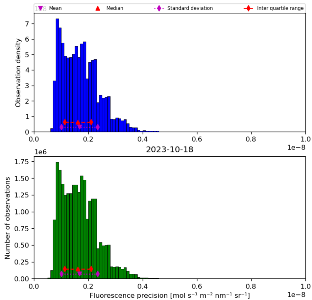
Figure 41: Histogram of “Fluorescence precision” for 2023-10-17 to 2023-10-19
