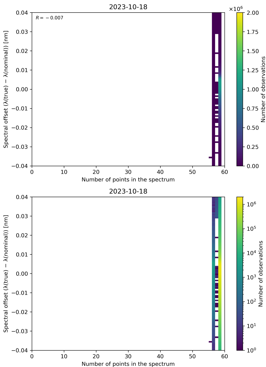
Figure 110: Scatter density plot of “Number of points in the spectrum” against “Spectral offset ( \lambda(\text{true}) - \lambda(\text{nominal}) )” for 2023-10-17 to 2023-10-19.
