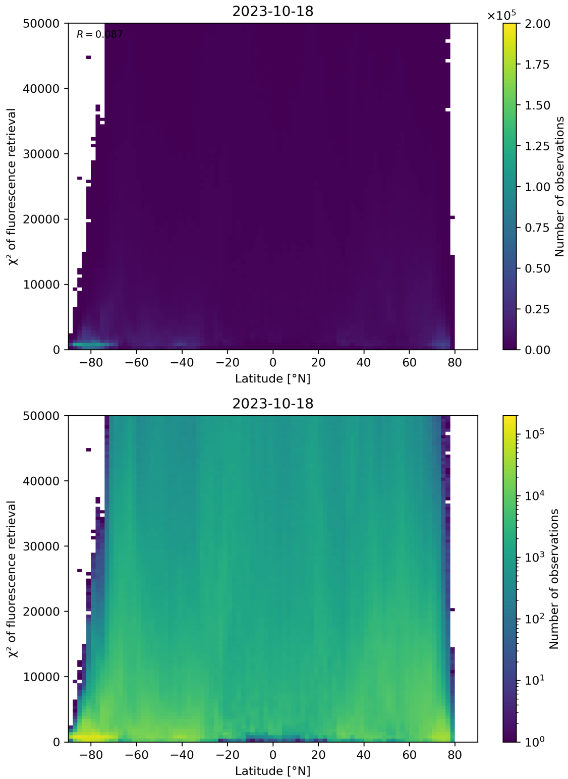
Figure 98: Scatter density plot of “Latitude” against “ \chi^2 of fluorescence retrieval” for 2023-10-17 to 2023-10-19.
