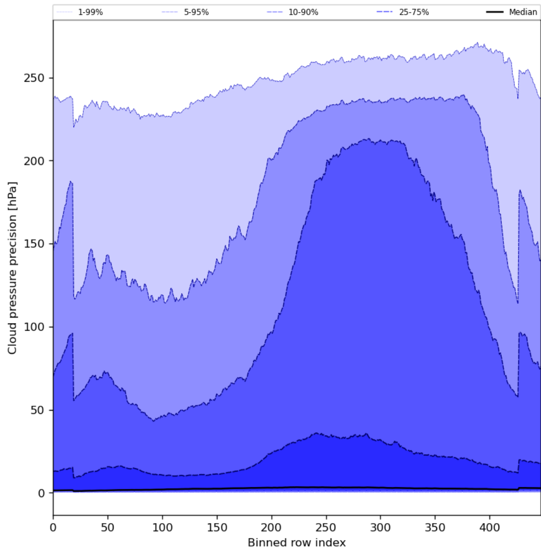
Figure 48: Along track statistics of “Cloud pressure precision” for 2023-10-17 to 2023-10-19
