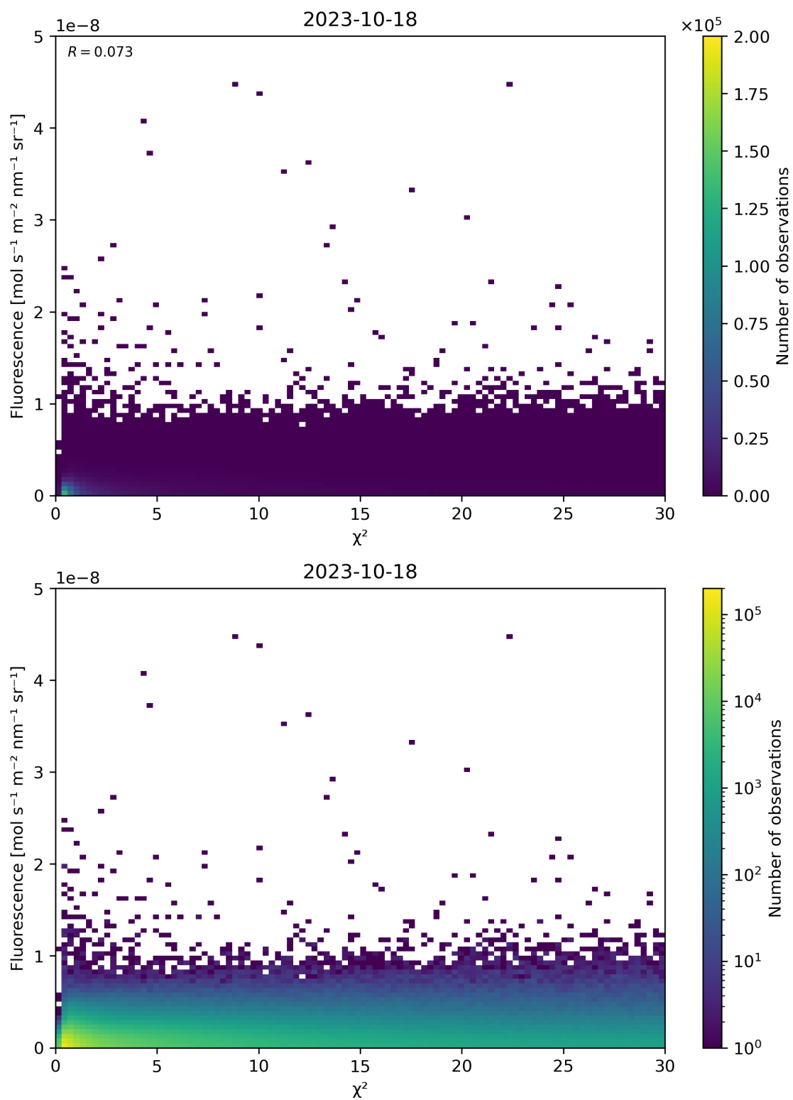
Figure 70: Scatter density plot of “ \chi^2 ” against “Fluorescence” for 2023-10-17 to 2023-10-19.
