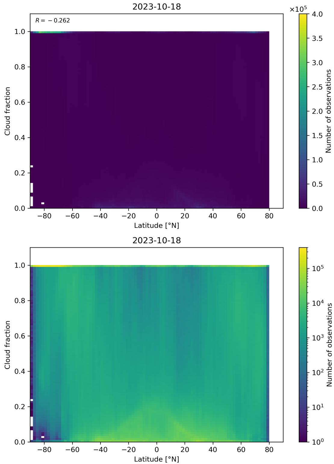
Figure 99: Scatter density plot of “Latitude” against “Cloud fraction” for 2023-10-17 to 2023-10-19.
