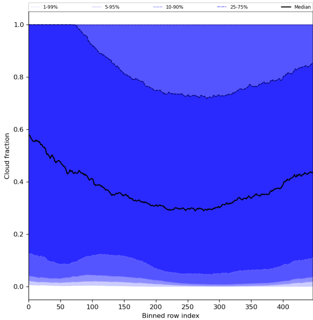
Figure 49: Along track statistics of “Cloud fraction” for 2023-10-17 to 2023-10-19
