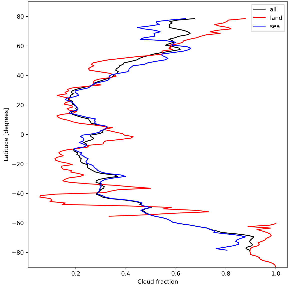
Figure 15: Zonal average of “Cloud fraction” for 2023-10-17 to 2023-10-19.
