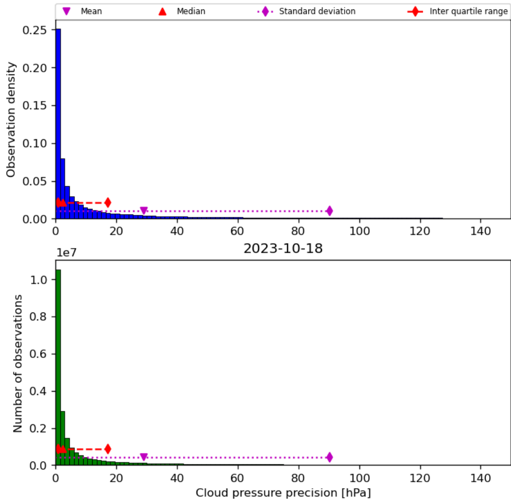
Figure 31: Histogram of “Cloud pressure precision” for 2023-10-17 to 2023-10-19
