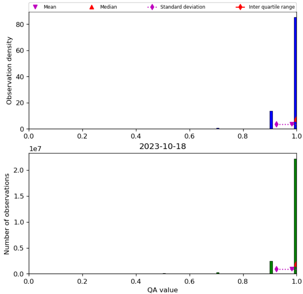
Figure 29: Histogram of “QA value” for 2023-10-17 to 2023-10-19
