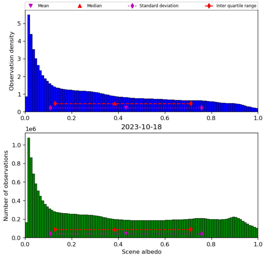
Figure 34: Histogram of “Scene albedo” for 2023-10-17 to 2023-10-19
