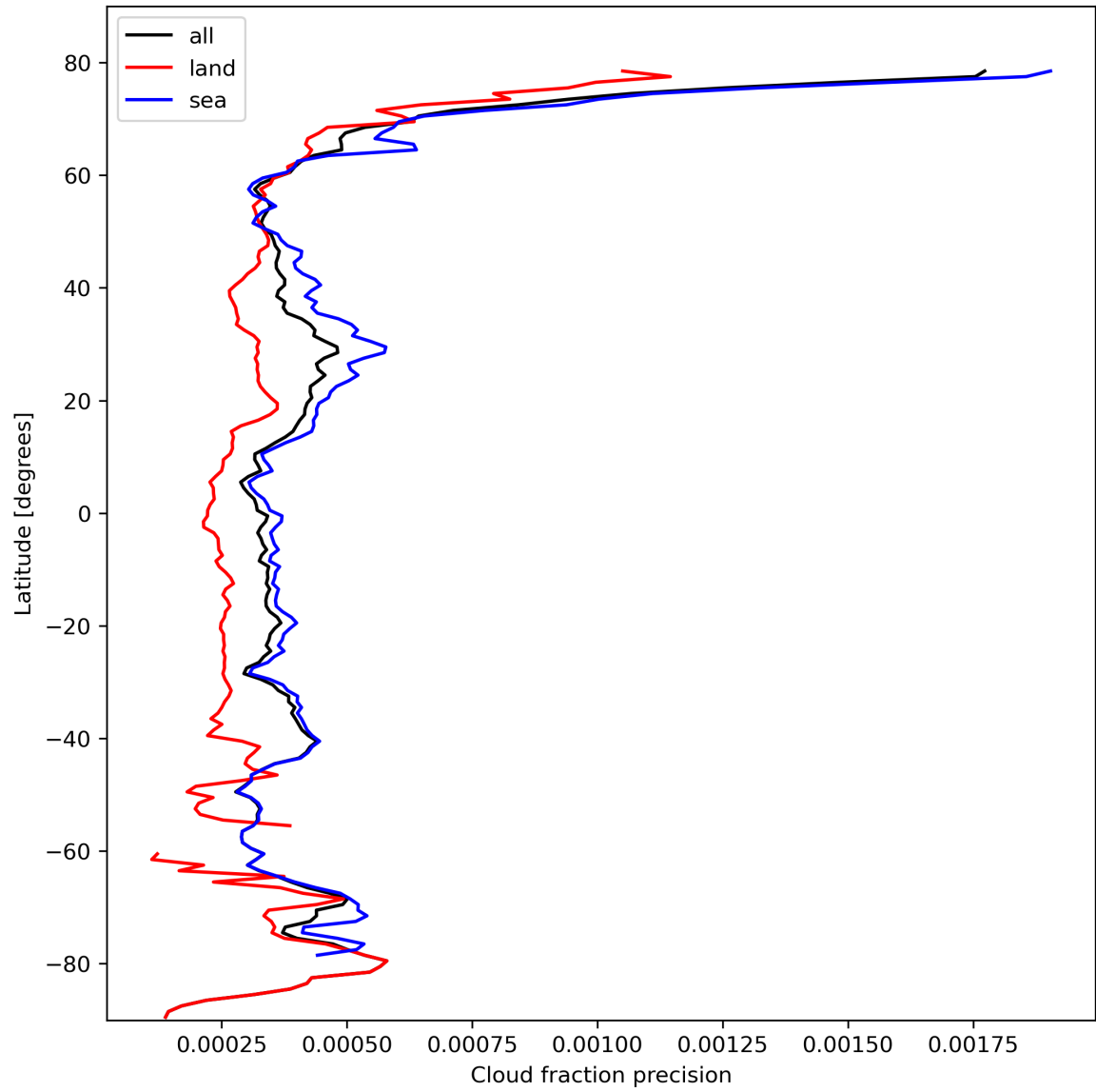
Figure 16: Zonal average of “Cloud fraction precision” for 2023-10-17 to 2023-10-19.
