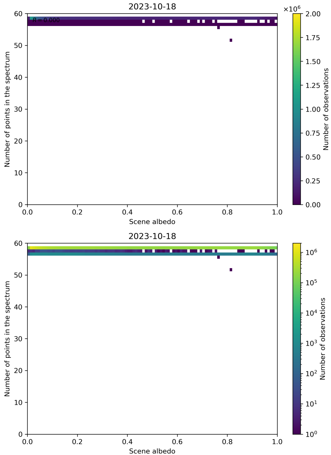
Figure 116: Scatter density plot of “Scene albedo” against “Number of points in the spectrum” for 2023-10-17 to 2023-10-19.
