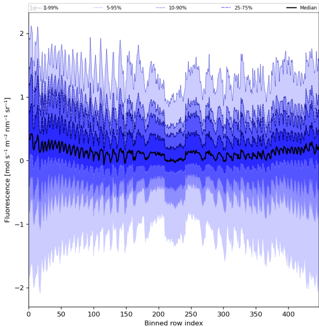
Figure 57: Along track statistics of “Fluorescence” for 2023-10-17 to 2023-10-19
