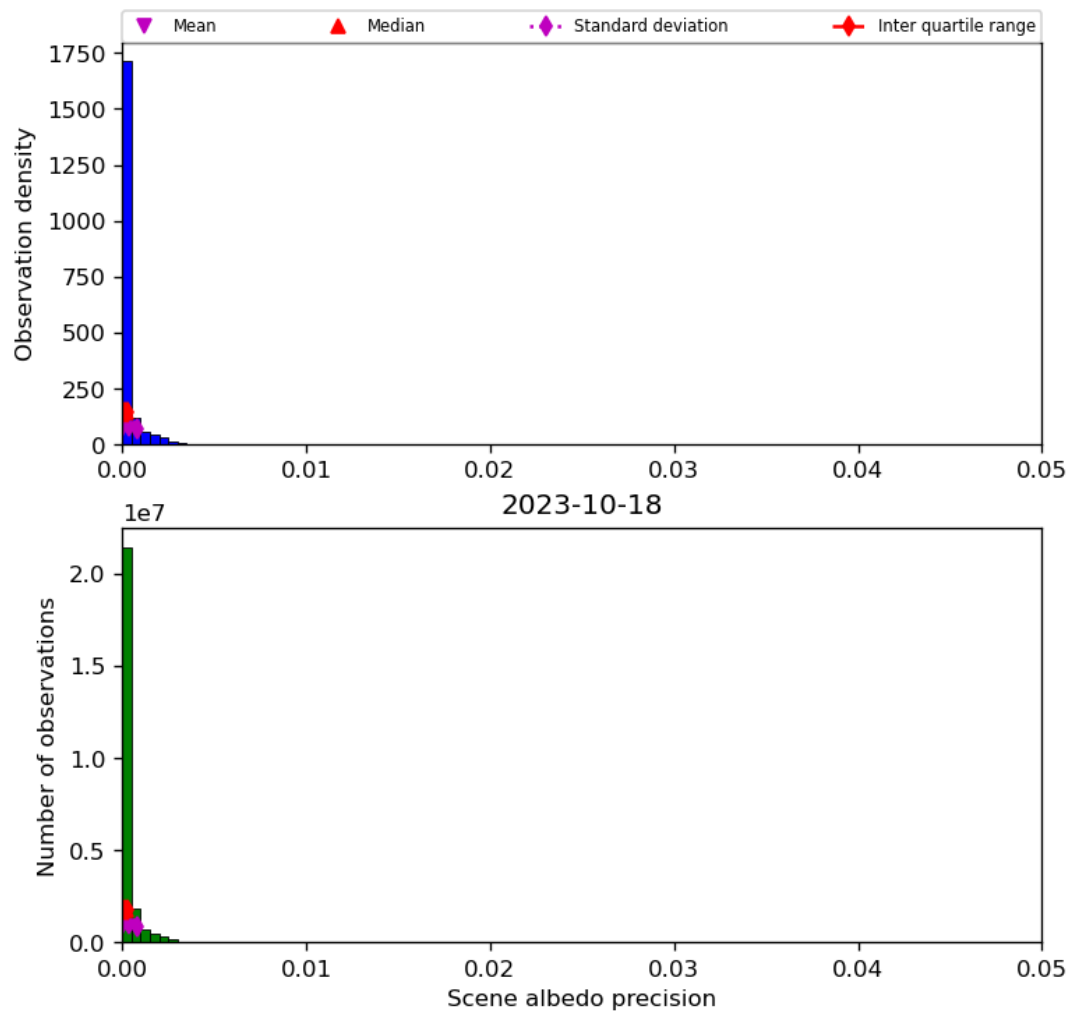
Figure 35: Histogram of “Scene albedo precision” for 2023-10-17 to 2023-10-19
