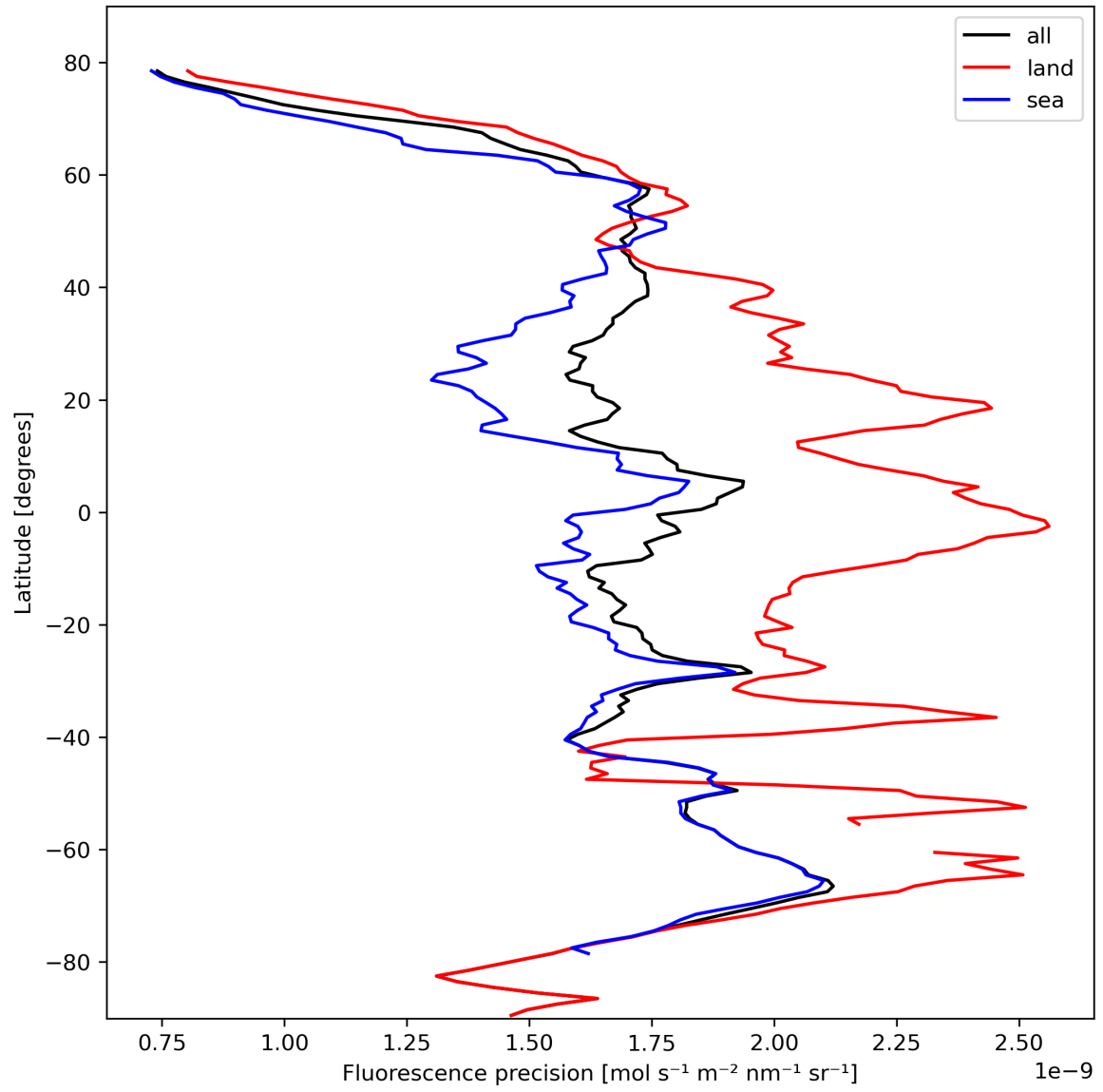
Figure 24: Zonal average of “Fluorescence precision” for 2023-10-17 to 2023-10-19.
