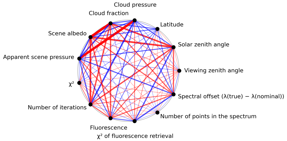
Figure 1: Map of correlation graph for 2023-10-17 to 2023-10-19.
