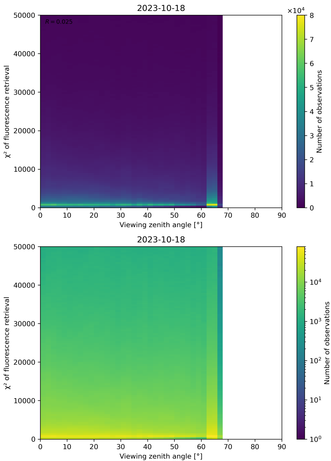
Figure 131: Scatter density plot of “Viewing zenith angle” against “ \chi^2 of fluorescence retrieval” for 2023-10-17 to 2023-10-19.
