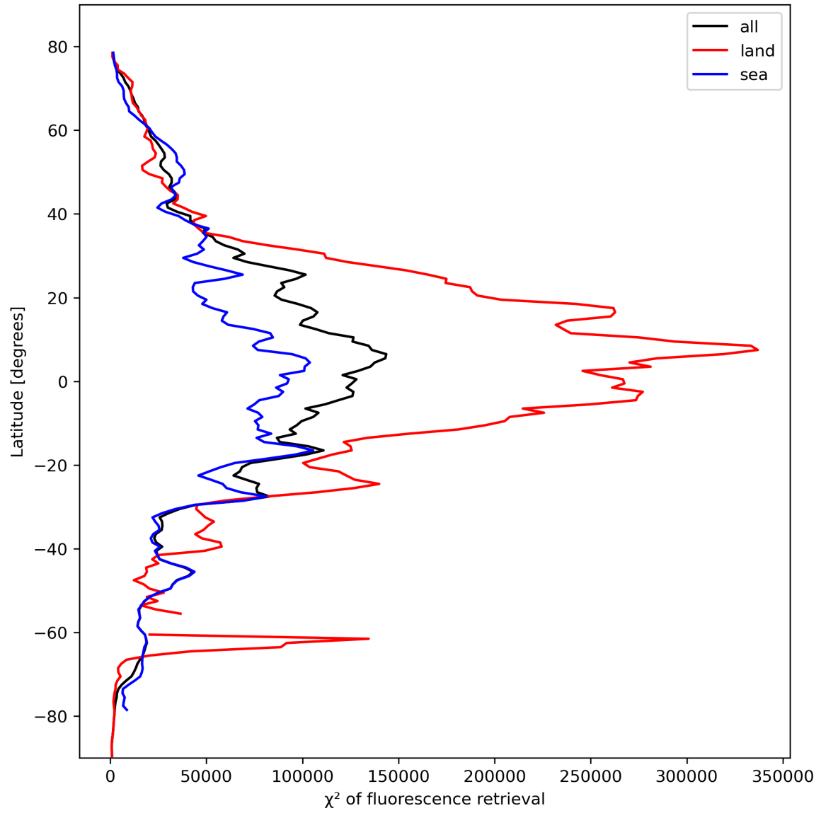
Figure 25: Zonal average of “ \chi^2 of fluorescence retrieval” for 2023-10-17 to 2023-10-19.
