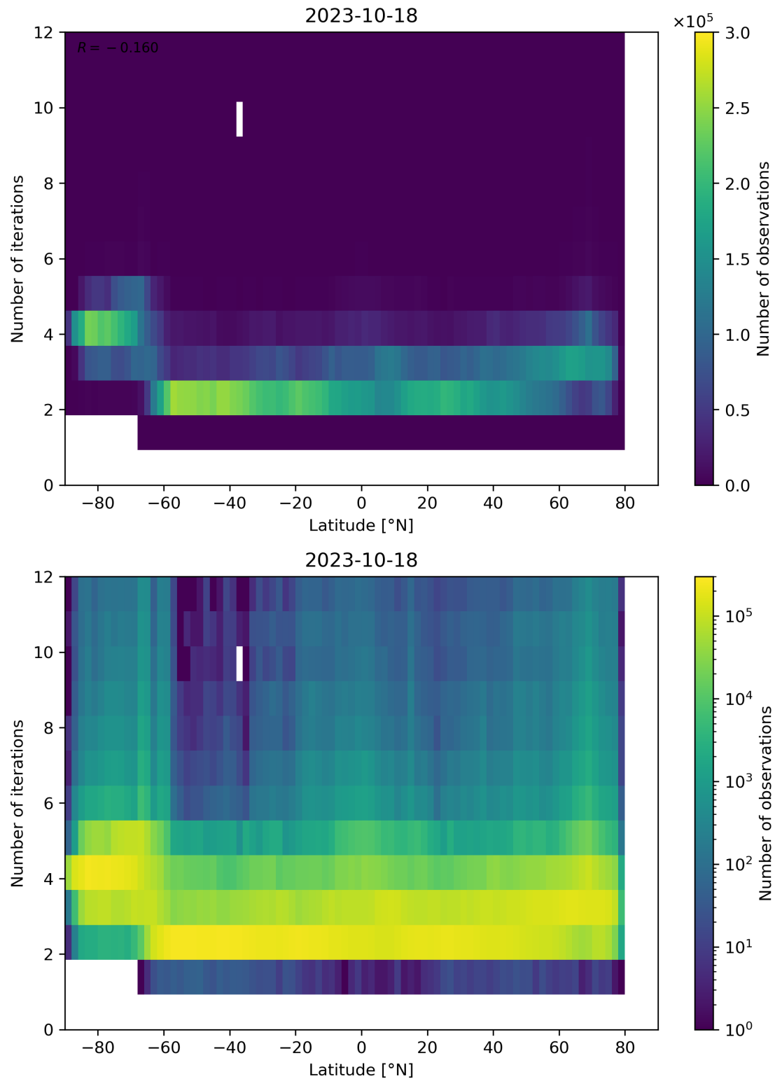
Figure 102: Scatter density plot of “Latitude” against “Number of iterations” for 2023-10-17 to 2023-10-19.
