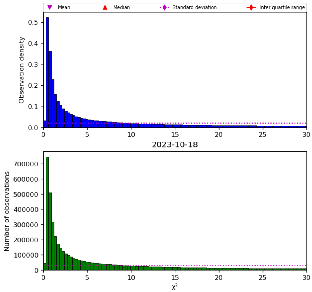
Figure 38: Histogram of “ \chi^2 ” for 2023-10-17 to 2023-10-19
