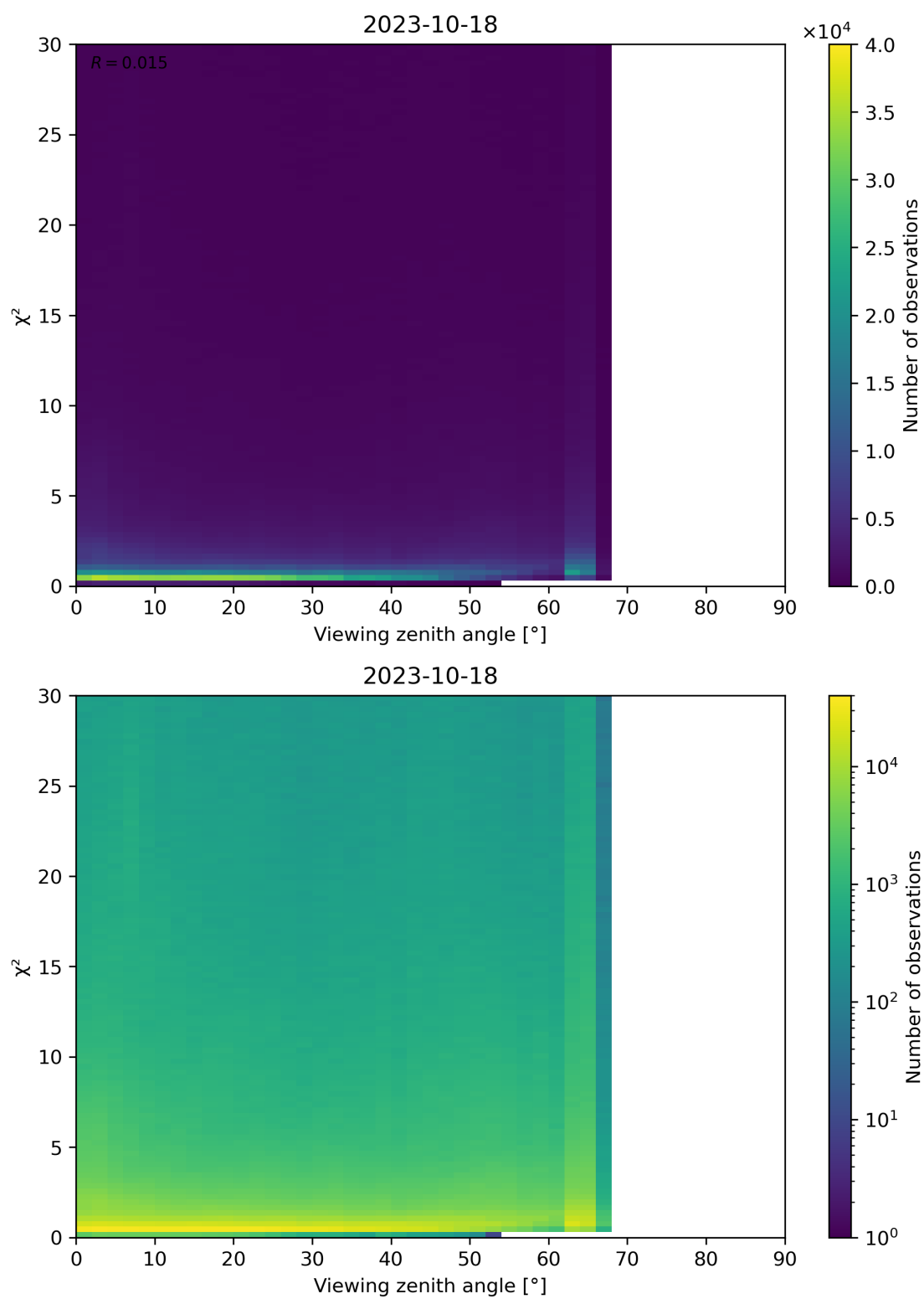
Figure 130: Scatter density plot of “Viewing zenith angle” against “ \chi^2 ” for 2023-10-17 to 2023-10-19.
