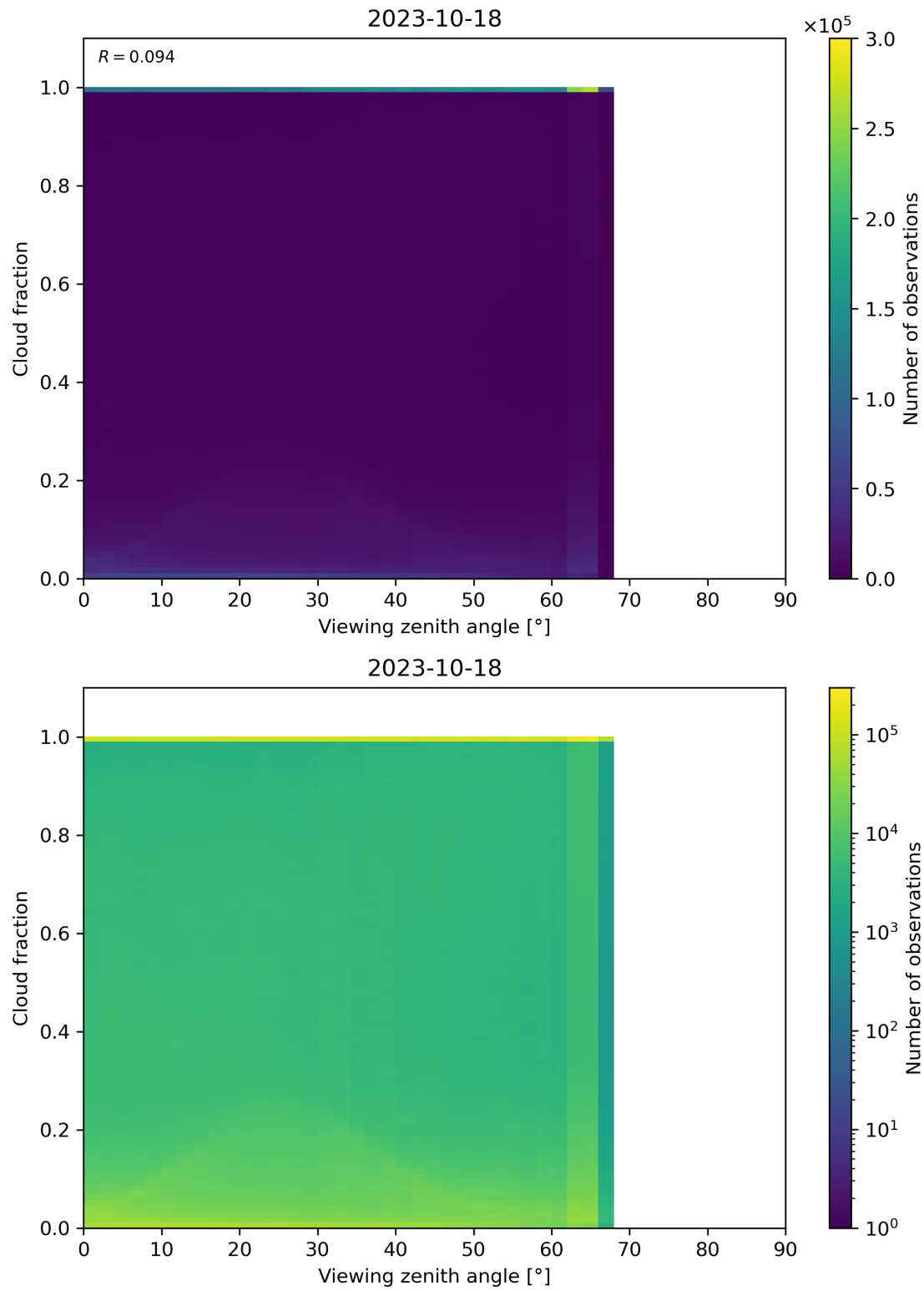
Figure 132: Scatter density plot of “Viewing zenith angle” against “Cloud fraction” for 2023-10-17 to 2023-10-19.
