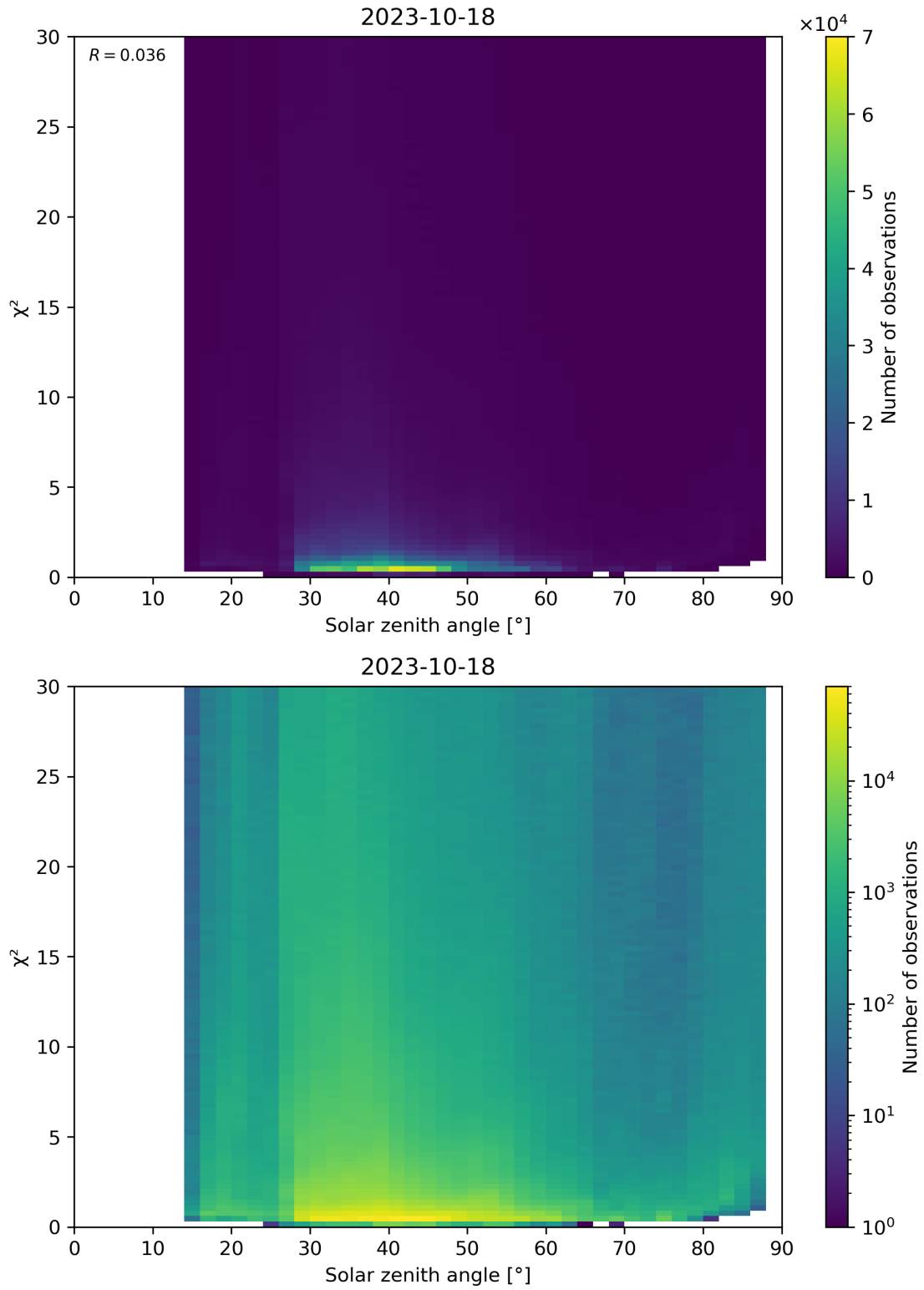
Figure 119: Scatter density plot of “Solar zenith angle” against “ \chi^2 ” for 2023-10-17 to 2023-10-19.
