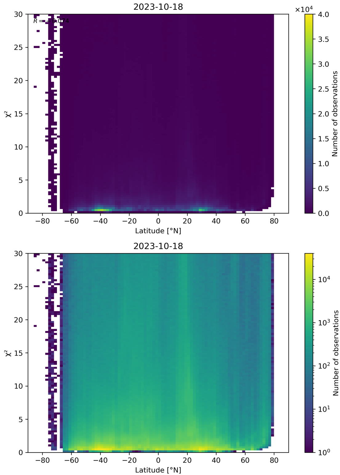
Figure 97: Scatter density plot of “Latitude” against “ \chi^2 ” for 2023-10-17 to 2023-10-19.
