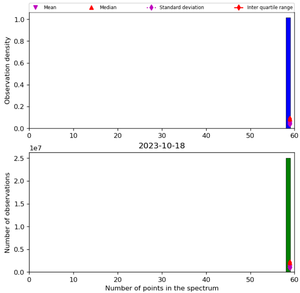
Figure 44: Histogram of “Number of points in the spectrum” for 2023-10-17 to 2023-10-19
