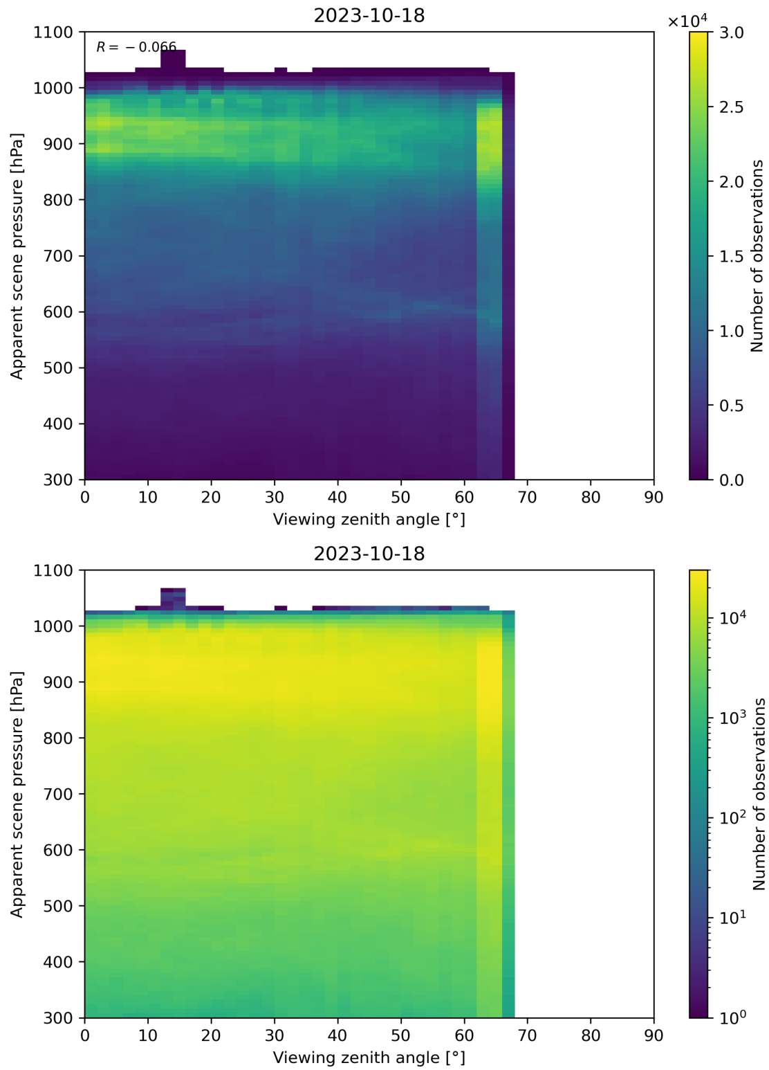
Figure 129: Scatter density plot of “Viewing zenith angle” against “Apparent scene pressure” for 2023-10-17 to 2023-10-19.
