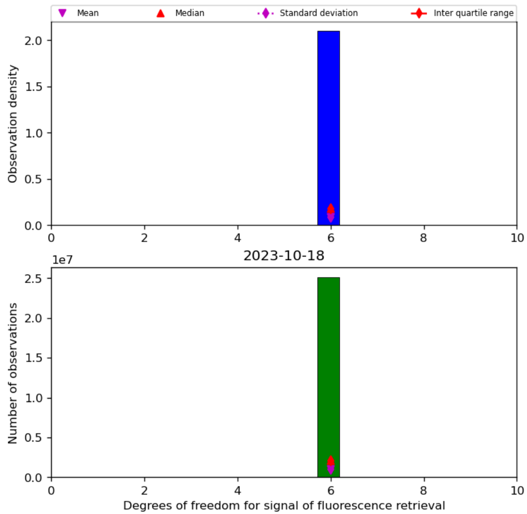
Figure 43: Histogram of “Degrees of freedom for signal of fluorescence retrieval” for 2023-10-17 to 2023-10-19
