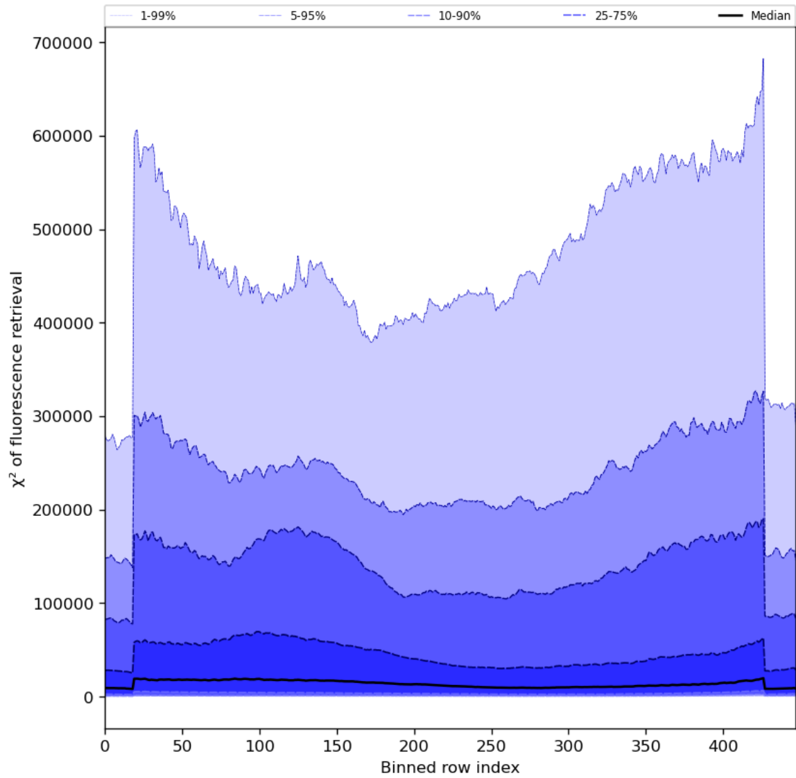
Figure 59: Along track statistics of “ \chi^2 of fluorescence retrieval” for 2023-10-17 to 2023-10-19
