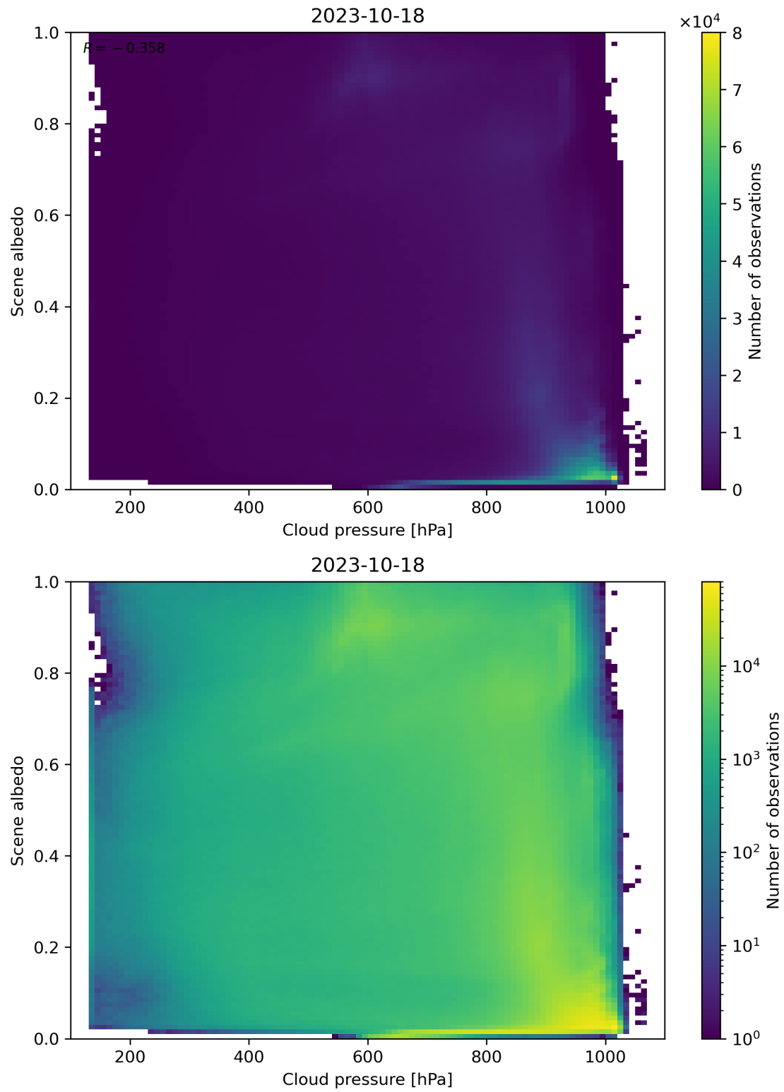
Figure 91: Scatter density plot of “Cloud pressure” against “Scene albedo” for 2023-10-17 to 2023-10-19.
