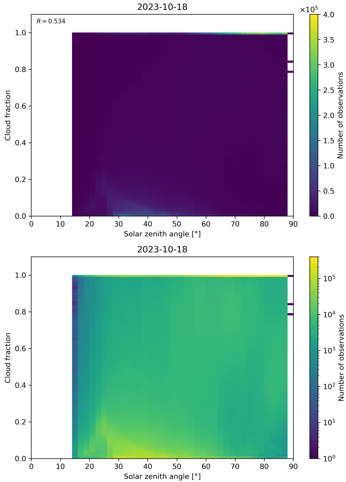
Figure 121: Scatter density plot of “Solar zenith angle” against “Cloud fraction” for 2023-10-17 to 2023-10-19.
