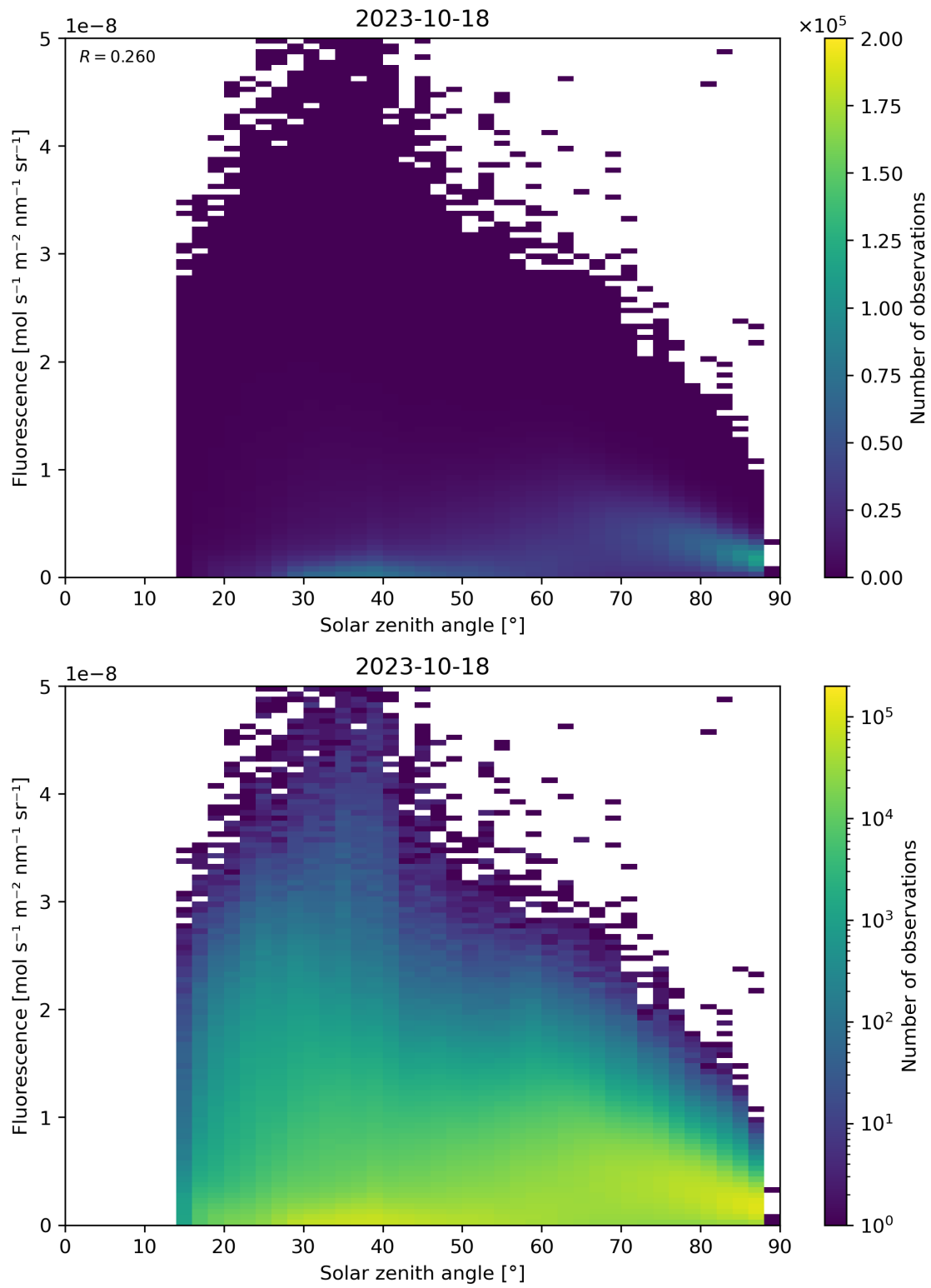
Figure 123: Scatter density plot of “Solar zenith angle” against “Fluorescence” for 2023-10-17 to 2023-10-19.
