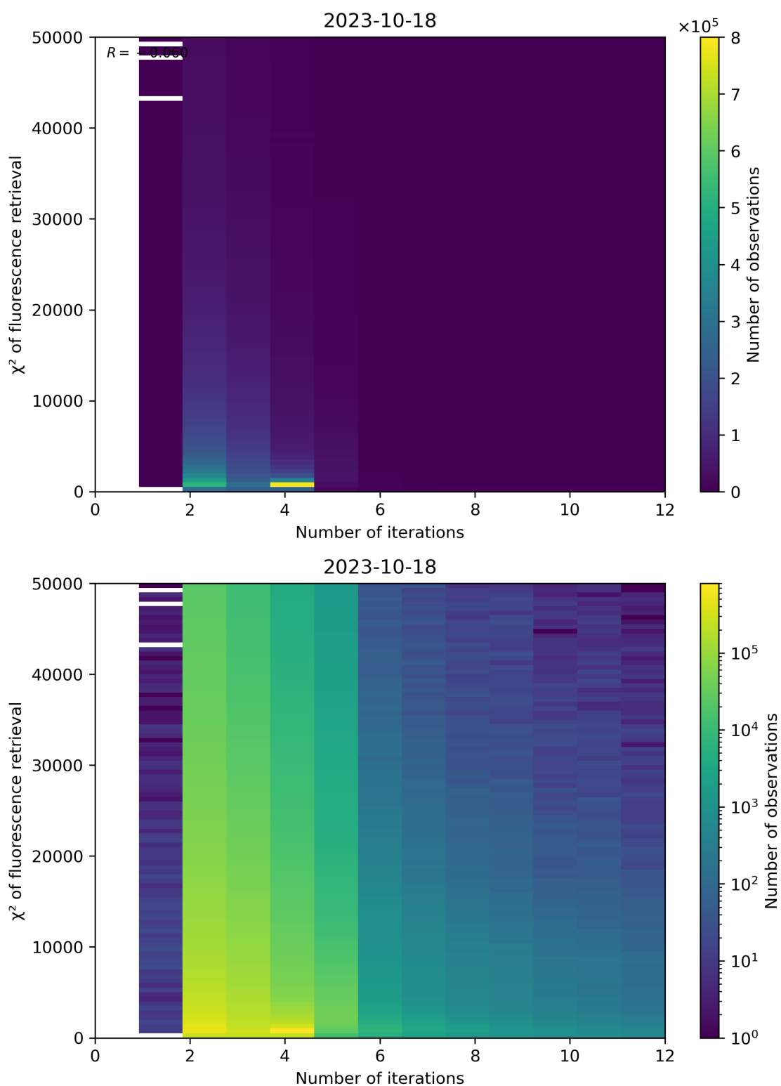
Figure 106: Scatter density plot of “Number of iterations” against “ \chi^2 of fluorescence retrieval” for 2023-10-17 to 2023-10-19.
