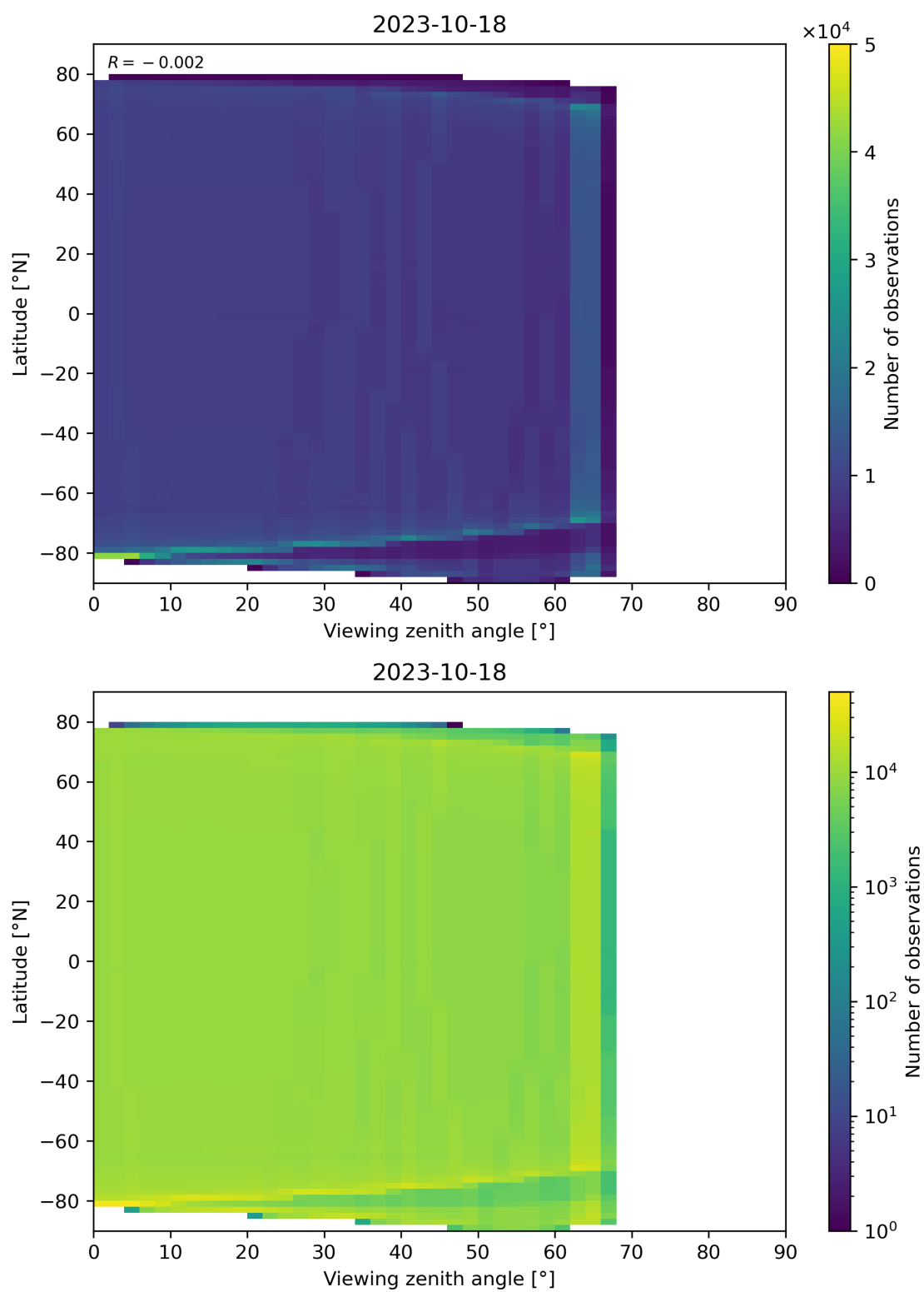
Figure 135: Scatter density plot of “Viewing zenith angle” against “Latitude” for 2023-10-17 to 2023-10-19.
