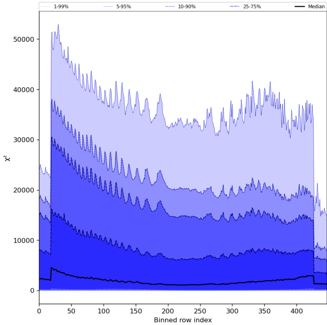
Figure 55: Along track statistics of " \chi^2 " for 2023-10-17 to 2023-10-19
