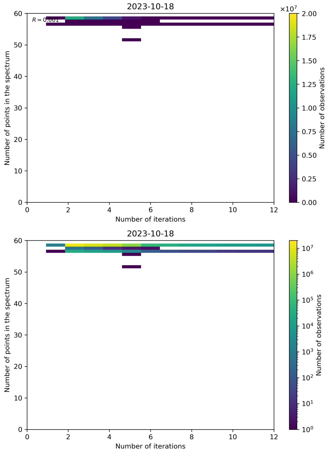
Figure 108: Scatter density plot of “Number of iterations” against “Number of points in the spectrum” for 2023-10-17 to 2023-10-19.
