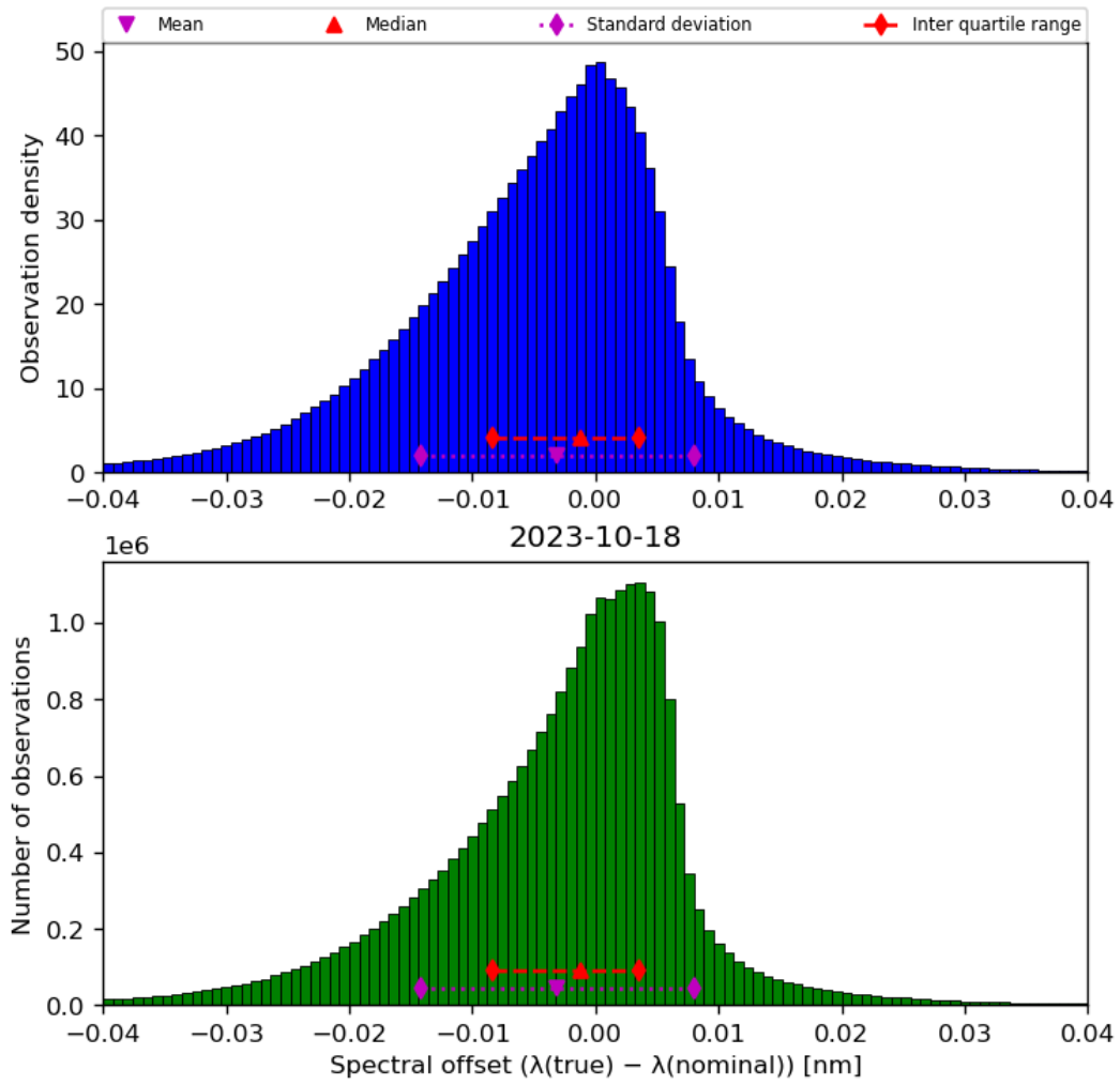
Figure 45: Histogram of “Spectral offset ( \lambda(\text{true}) - \lambda(\text{nominal}) )” for 2023-10-17 to 2023-10-19
