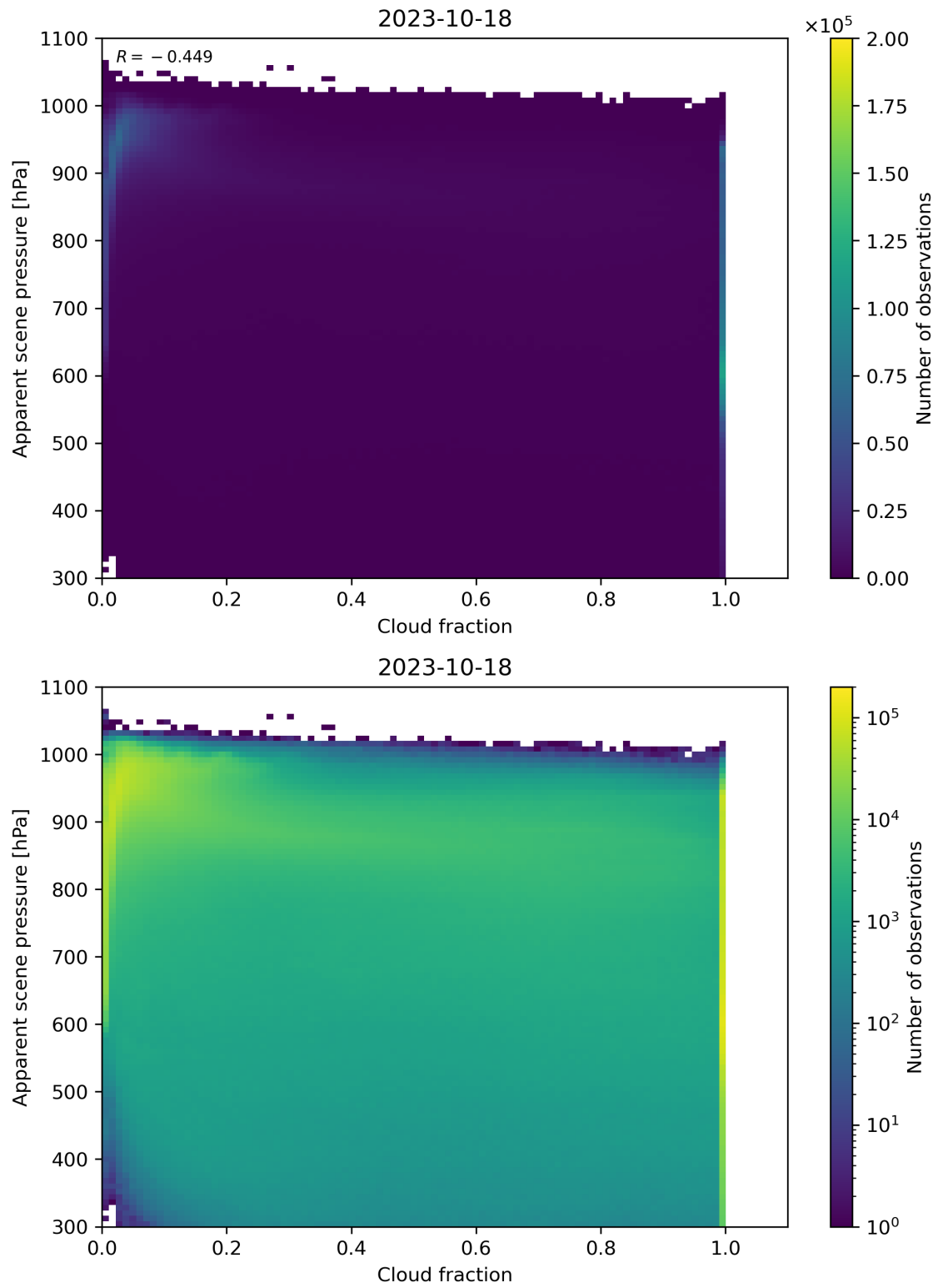
Figure 76: Scatter density plot of “Cloud fraction” against “Apparent scene pressure” for 2023-10-17 to 2023-10-19.
