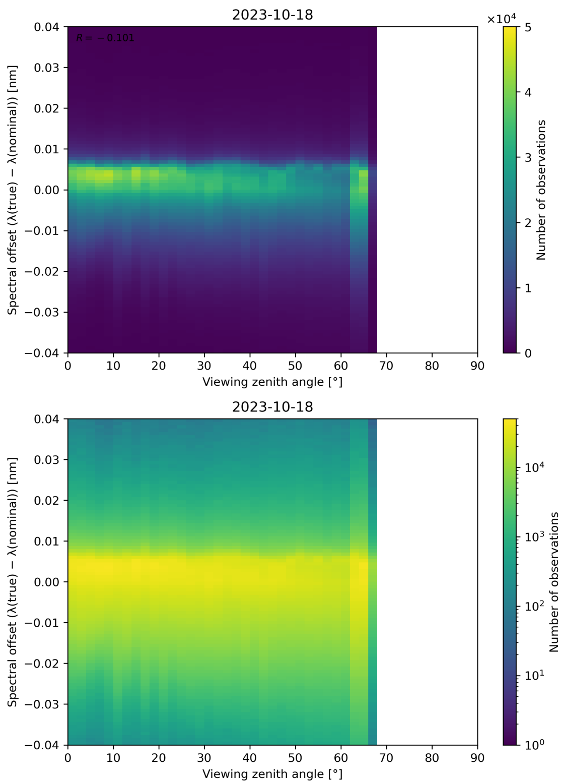
Figure 140: Scatter density plot of “Viewing zenith angle” against “Spectral offset ( \lambda(\text{true}) - \lambda(\text{nominal}) )” for 2023-10-17 to 2023-10-19.
