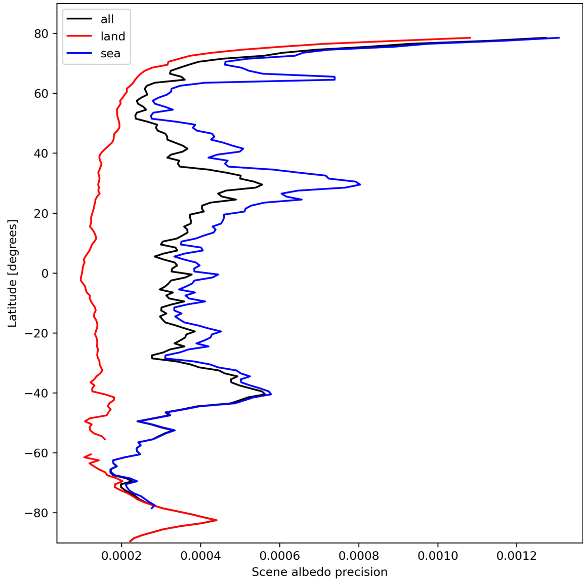
Figure 18: Zonal average of “Scene albedo precision” for 2023-10-17 to 2023-10-19.
