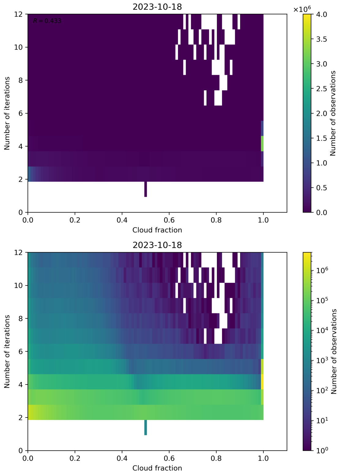
Figure 80: Scatter density plot of “Cloud fraction” against “Number of iterations” for 2023-10-17 to 2023-10-19.
