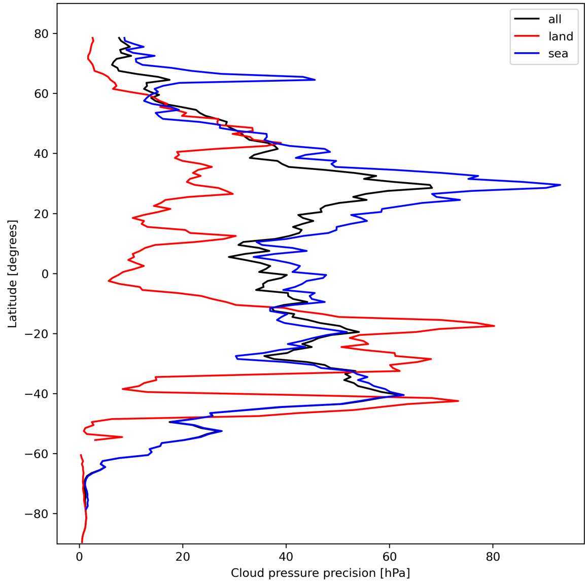
Figure 14: Zonal average of “Cloud pressure precision” for 2023-10-17 to 2023-10-19.
