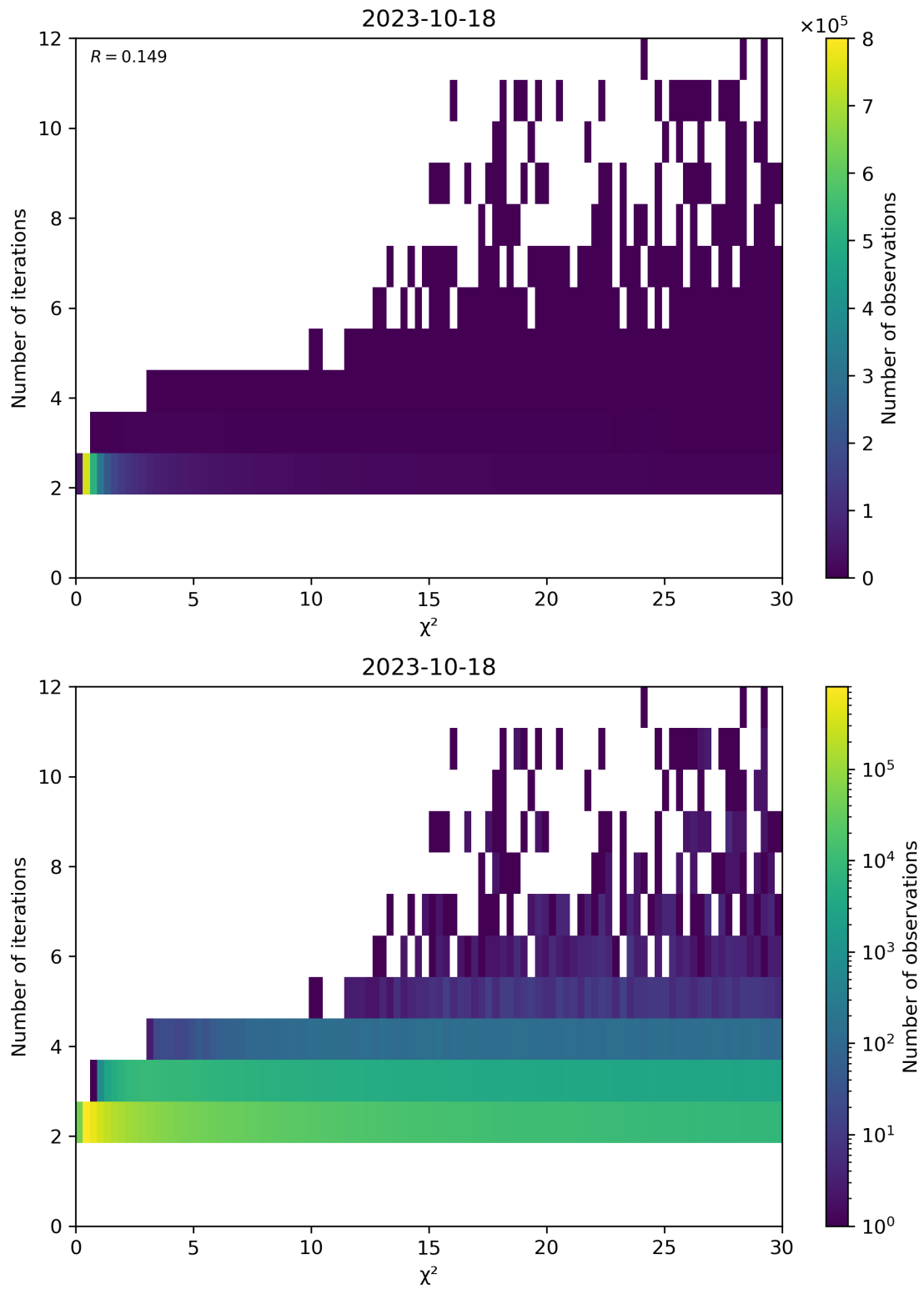
Figure 73: Scatter density plot of “ \chi^2 ” against “Number of iterations” for 2023-10-17 to 2023-10-19.
