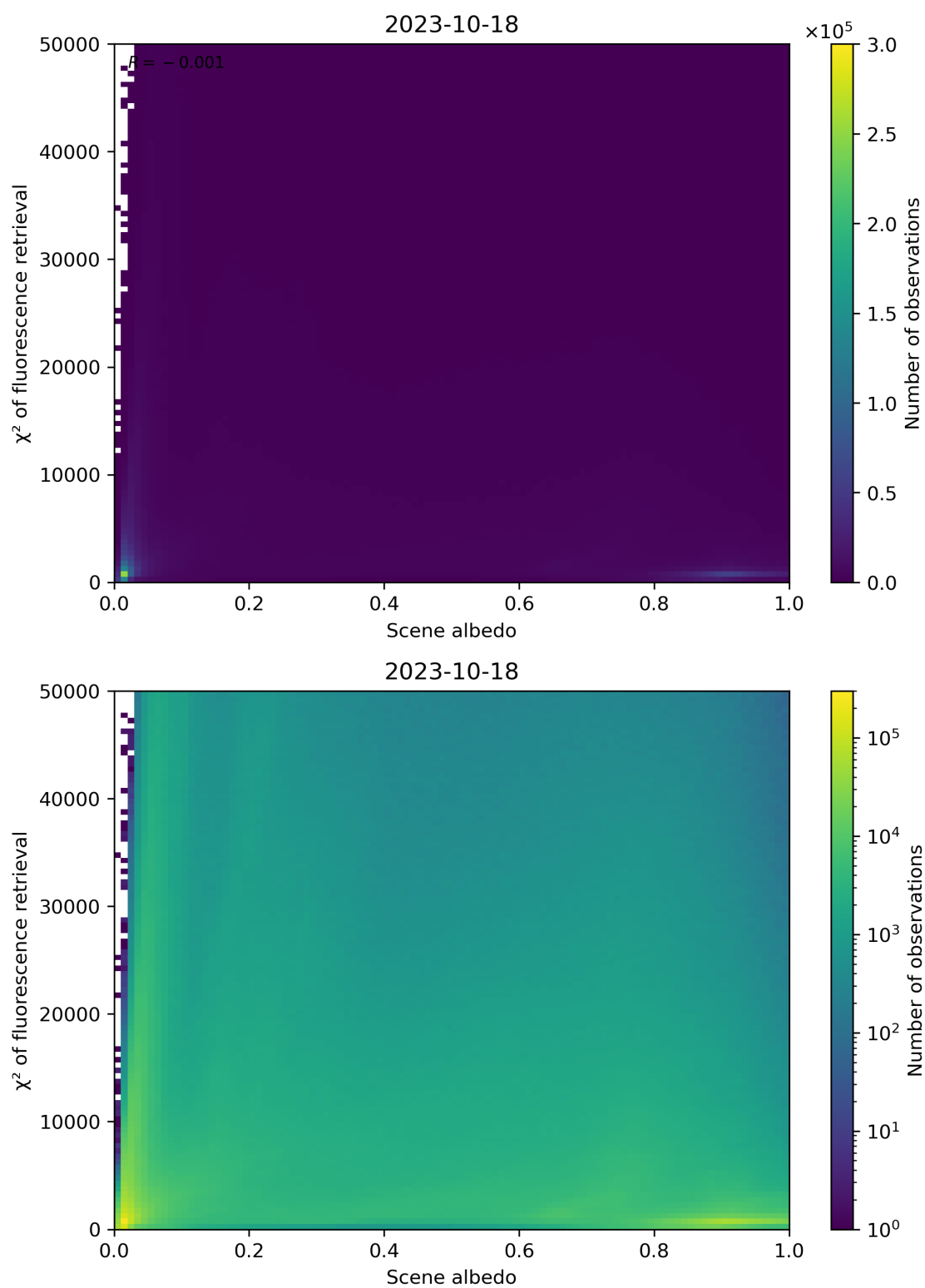
Figure 113: Scatter density plot of “Scene albedo” against “ \chi^2 of fluorescence retrieval” for 2023-10-17 to 2023-10-19.
