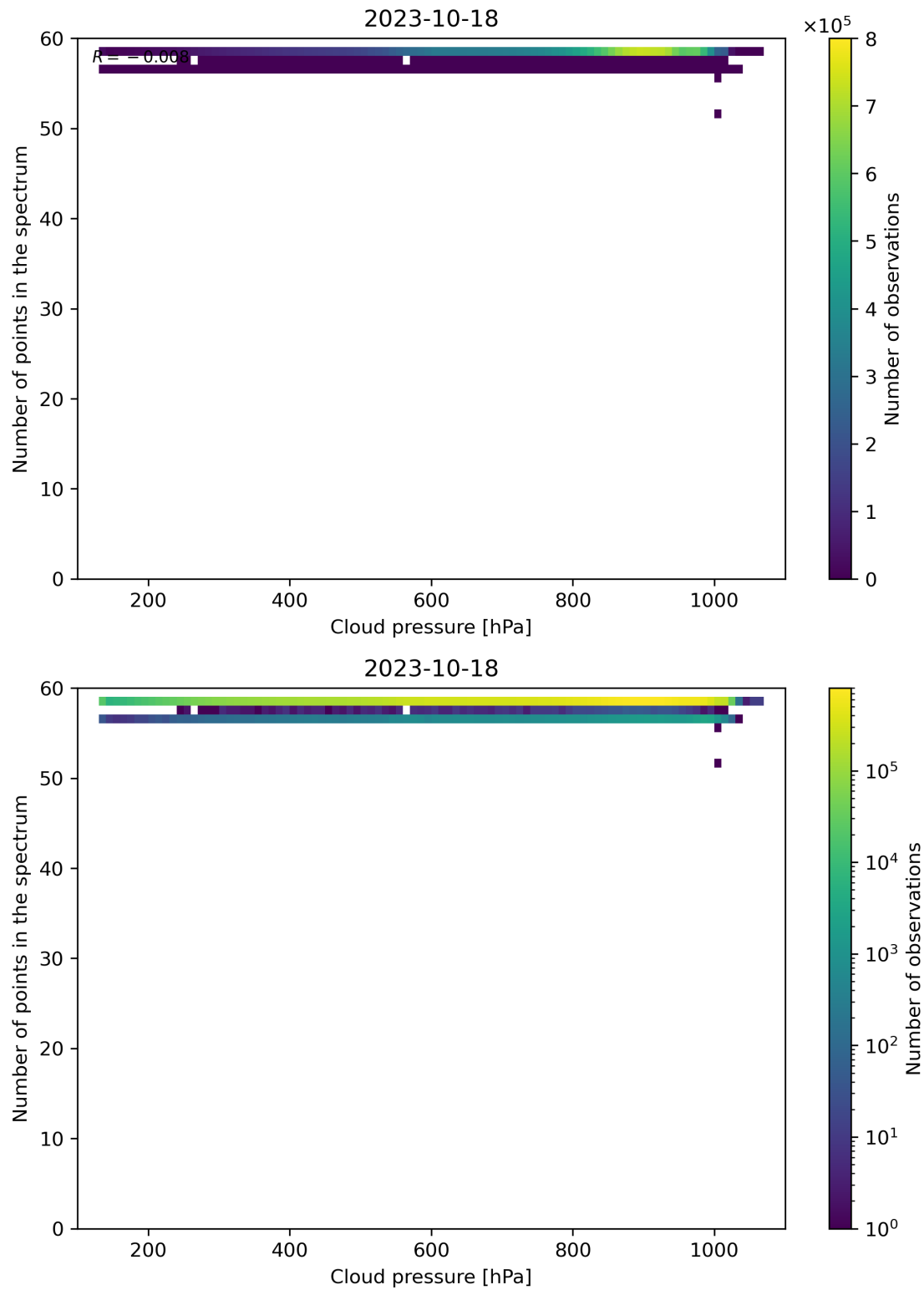
Figure 90: Scatter density plot of “Cloud pressure” against “Number of points in the spectrum” for 2023-10-17 to 2023-10-19.
