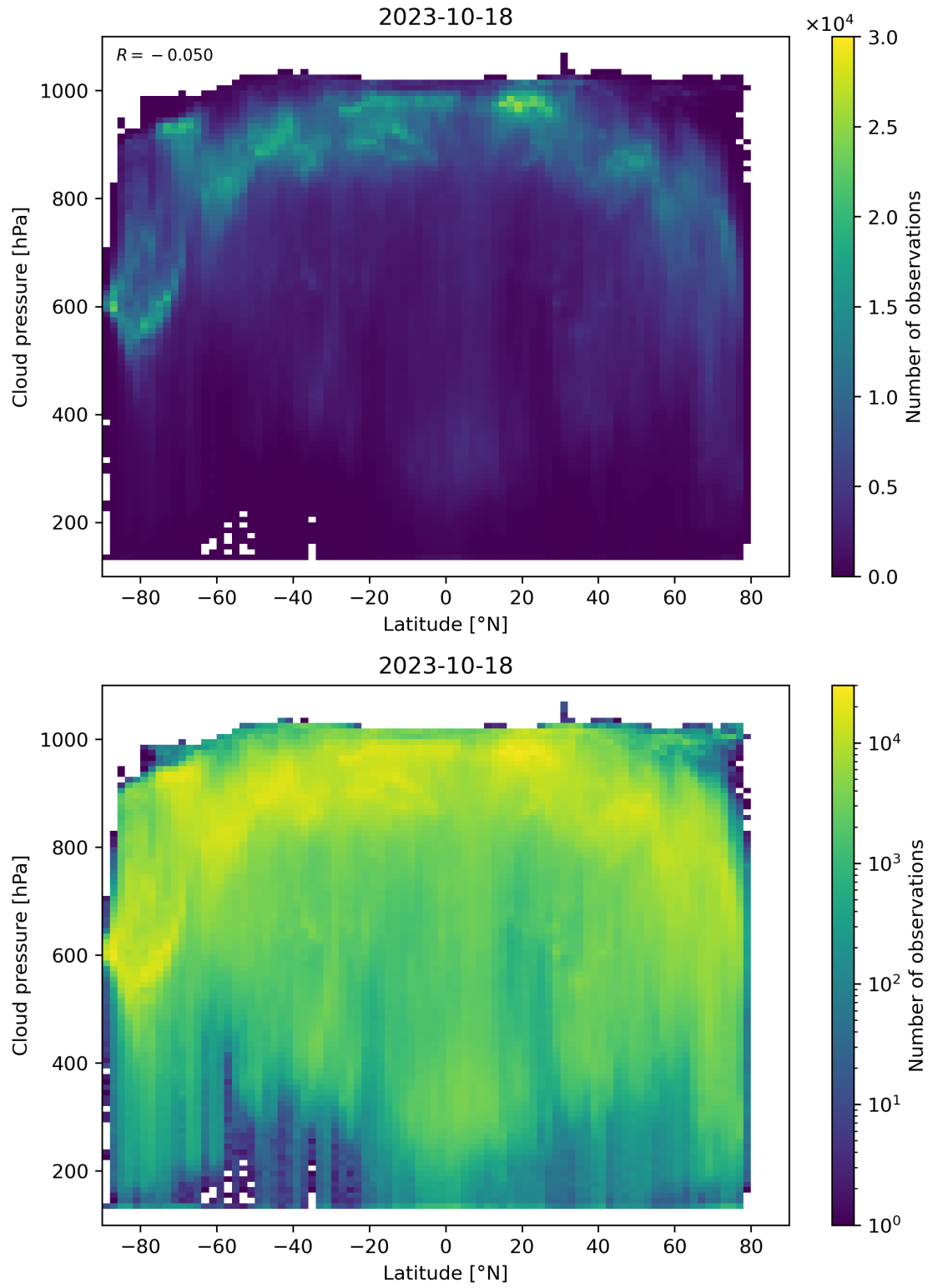
Figure 100: Scatter density plot of “Latitude” against “Cloud pressure” for 2023-10-17 to 2023-10-19.
