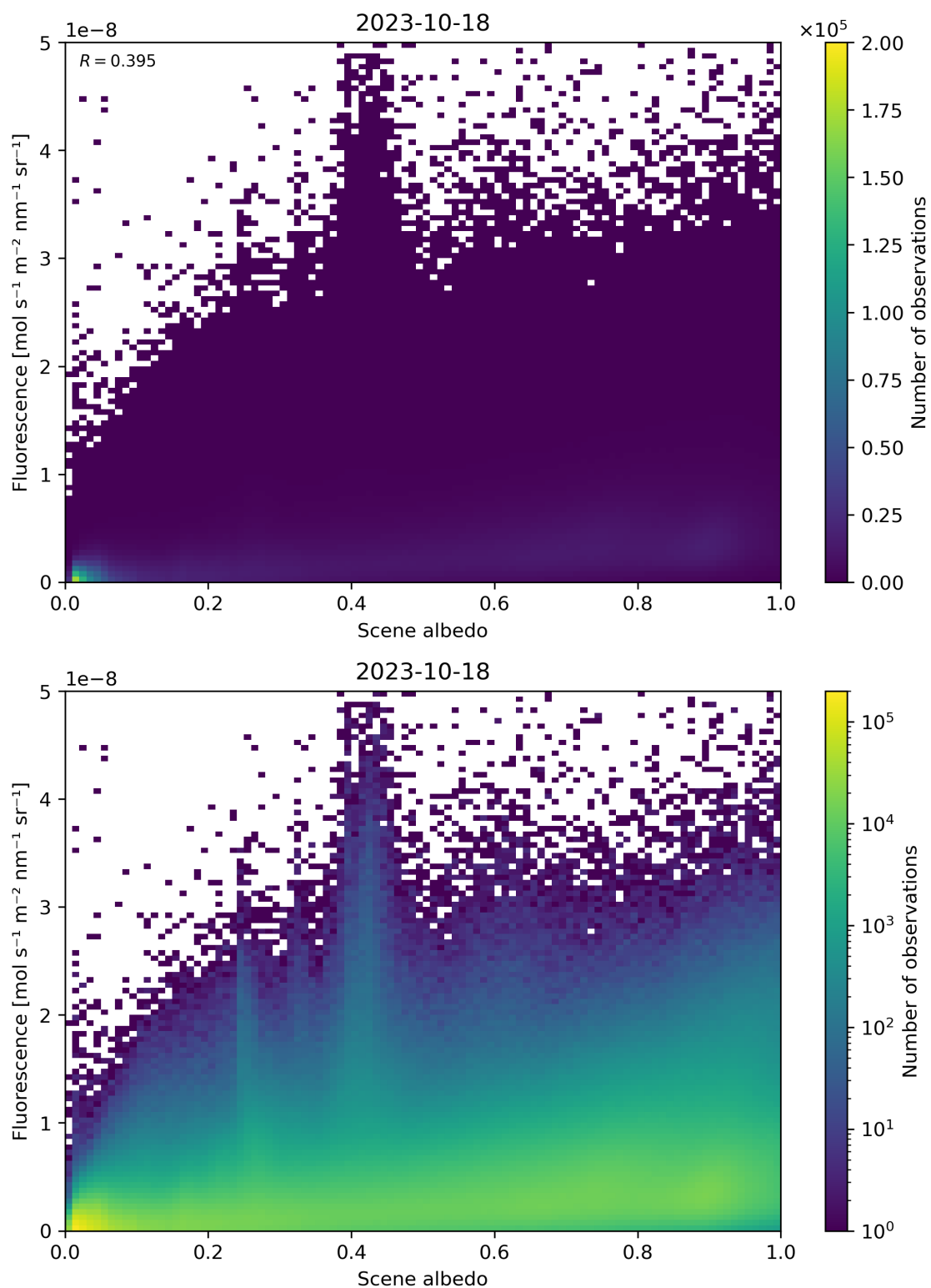
Figure 114: Scatter density plot of “Scene albedo” against “Fluorescence” for 2023-10-17 to 2023-10-19.
