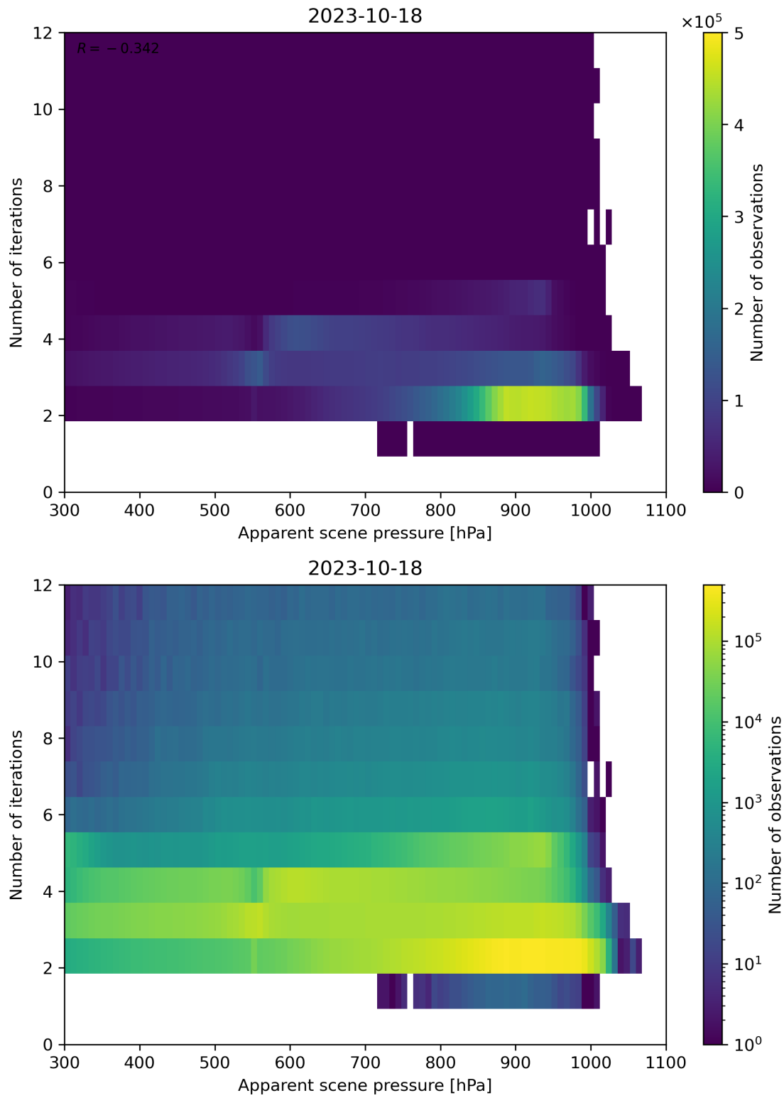
Figure 66: Scatter density plot of “Apparent scene pressure” against “Number of iterations” for 2023-10-17 to 2023-10-19.
