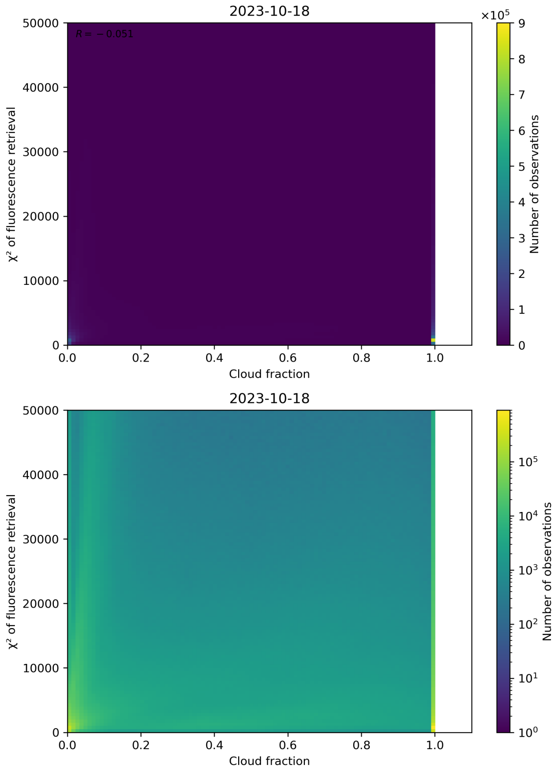
Figure 78: Scatter density plot of “Cloud fraction” against “ \chi^2 of fluorescence retrieval” for 2023-10-17 to 2023-10-19.
