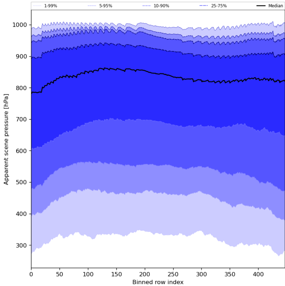
Figure 53: Along track statistics of “Apparent scene pressure” for 2023-10-17 to 2023-10-19
