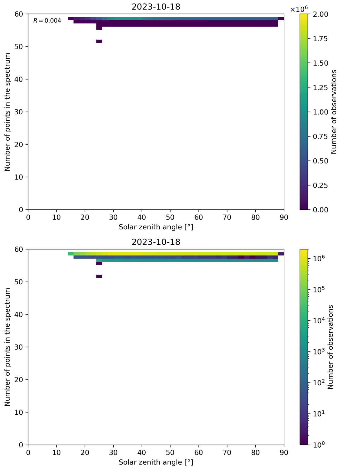
Figure 126: Scatter density plot of “Solar zenith angle” against “Number of points in the spectrum” for 2023-10-17 to 2023-10-19.
