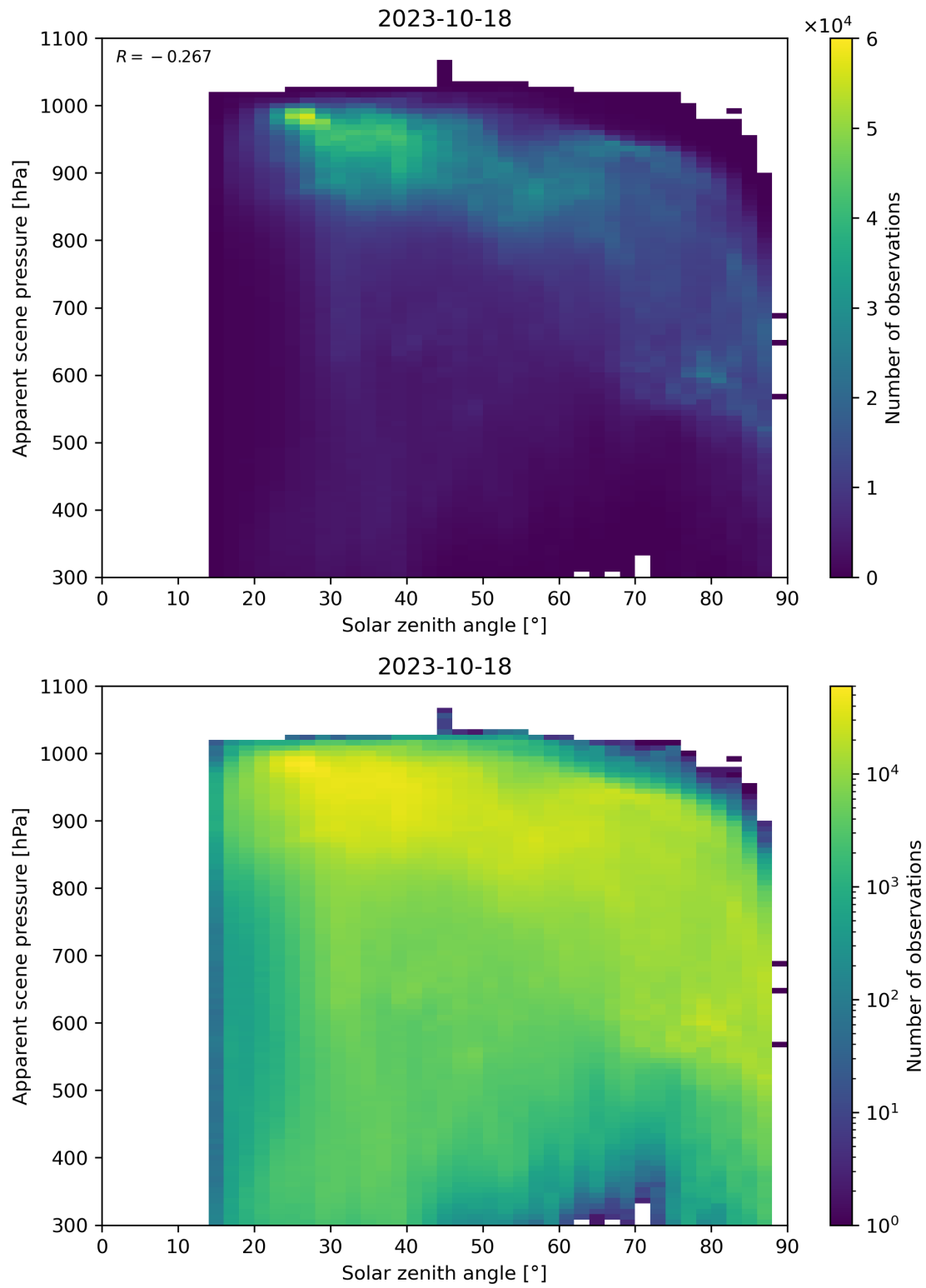
Figure 118: Scatter density plot of “Solar zenith angle” against “Apparent scene pressure” for 2023-10-17 to 2023-10-19.
