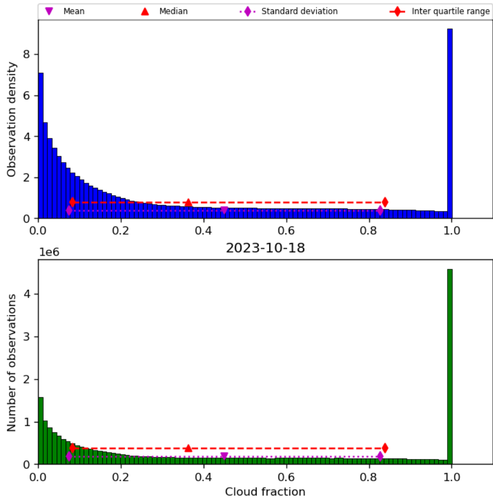
Figure 32: Histogram of “Cloud fraction” for 2023-10-17 to 2023-10-19
