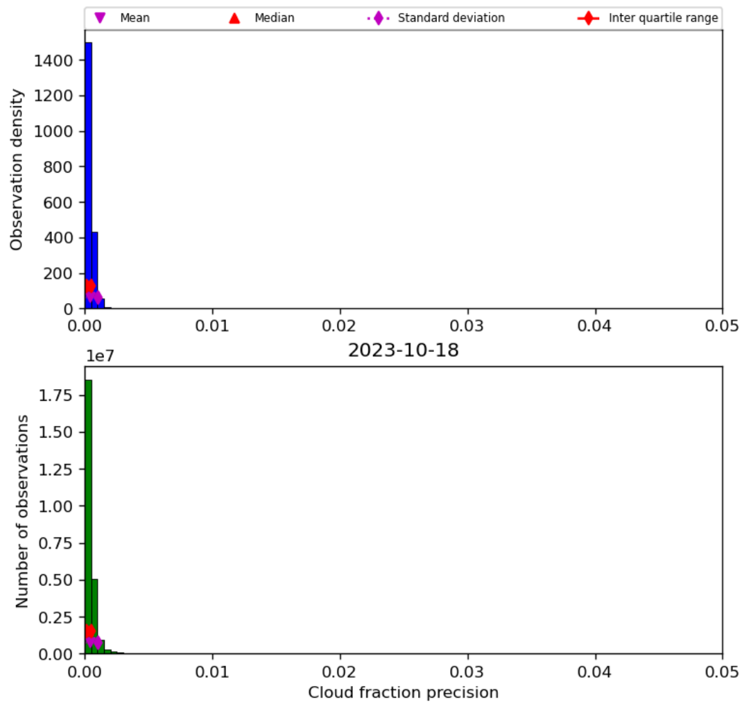
Figure 33: Histogram of “Cloud fraction precision” for 2023-10-17 to 2023-10-19
