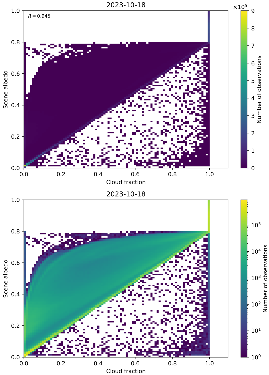
Figure 82: Scatter density plot of “Cloud fraction” against “Scene albedo” for 2023-10-17 to 2023-10-19.
