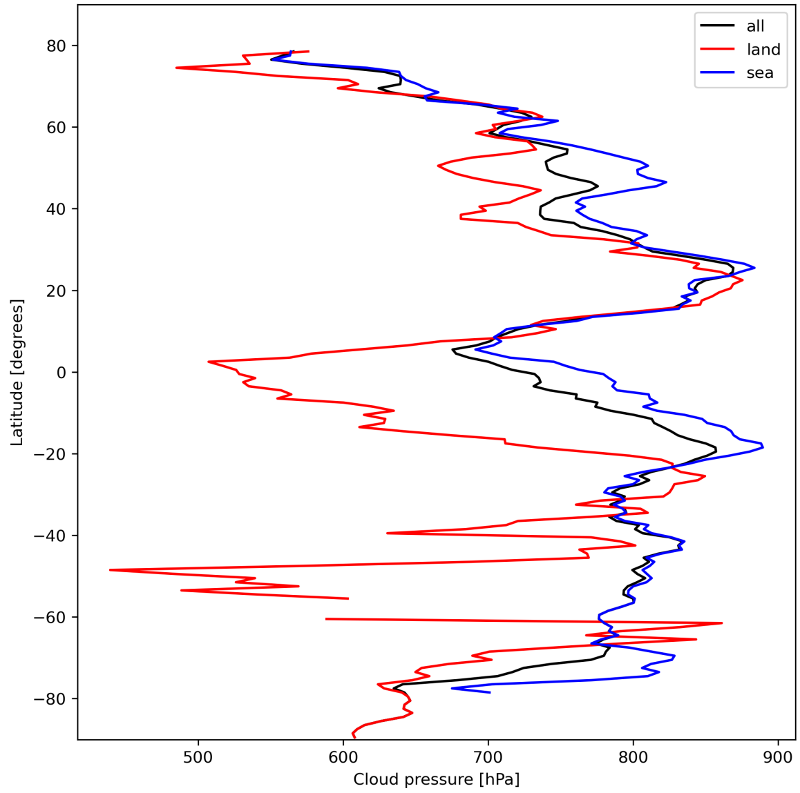
Figure 13: Zonal average of “Cloud pressure” for 2023-10-17 to 2023-10-19.
