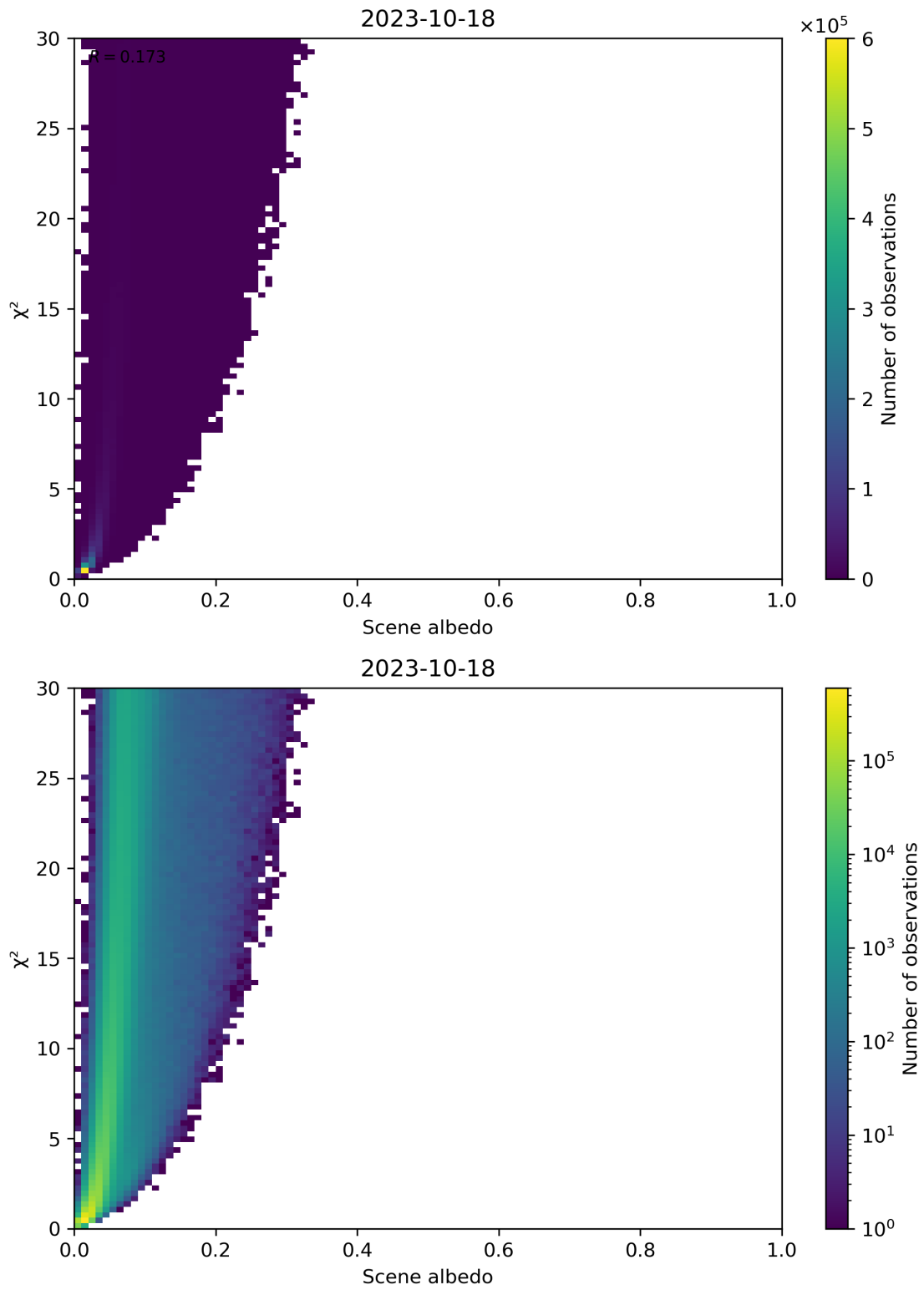
Figure 112: Scatter density plot of “Scene albedo” against “ \chi^2 ” for 2023-10-17 to 2023-10-19.
