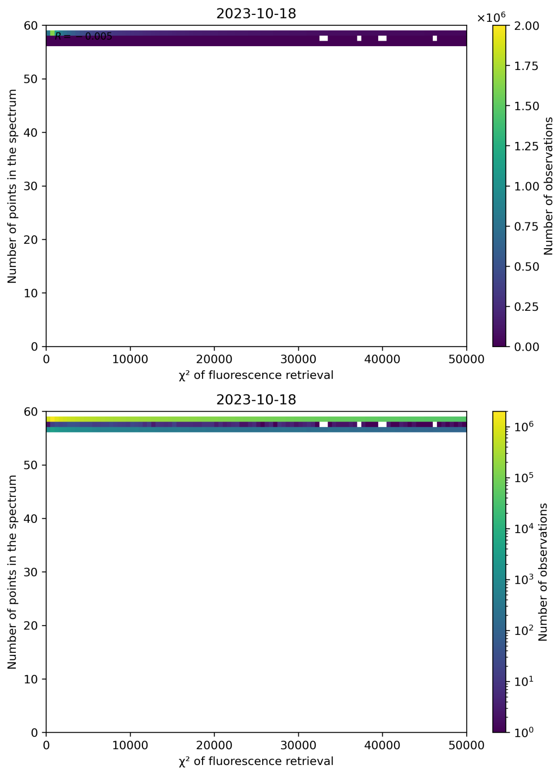
Figure 71: Scatter density plot of " \chi^2 of fluorescence retrieval" against "Number of points in the spectrum" for 2023-10-17 to 2023-10-19.
