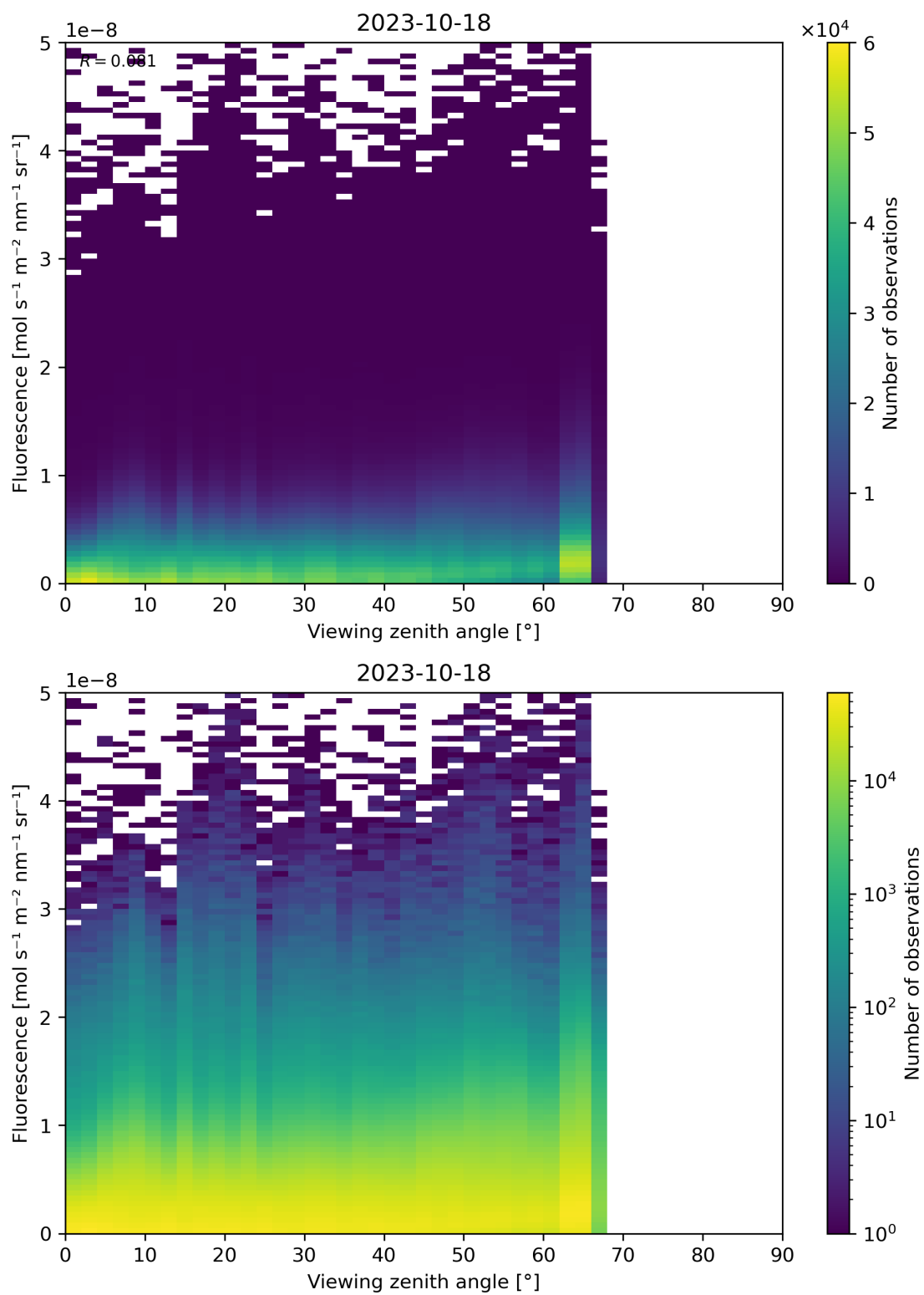
Figure 134: Scatter density plot of “Viewing zenith angle” against “Fluorescence” for 2023-10-17 to 2023-10-19.
