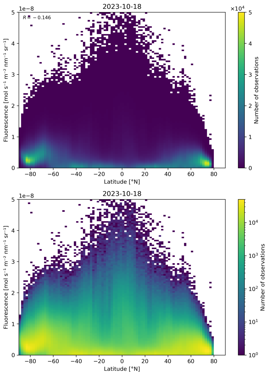
Figure 101: Scatter density plot of “Latitude” against “Fluorescence” for 2023-10-17 to 2023-10-19.
