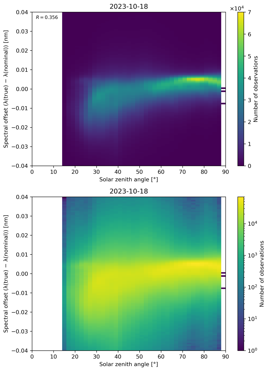
Figure 128: Scatter density plot of “Solar zenith angle” against “Spectral offset ( \lambda(\text{true}) - \lambda(\text{nominal}) )” for 2023-10-17 to 2023-10-19.
