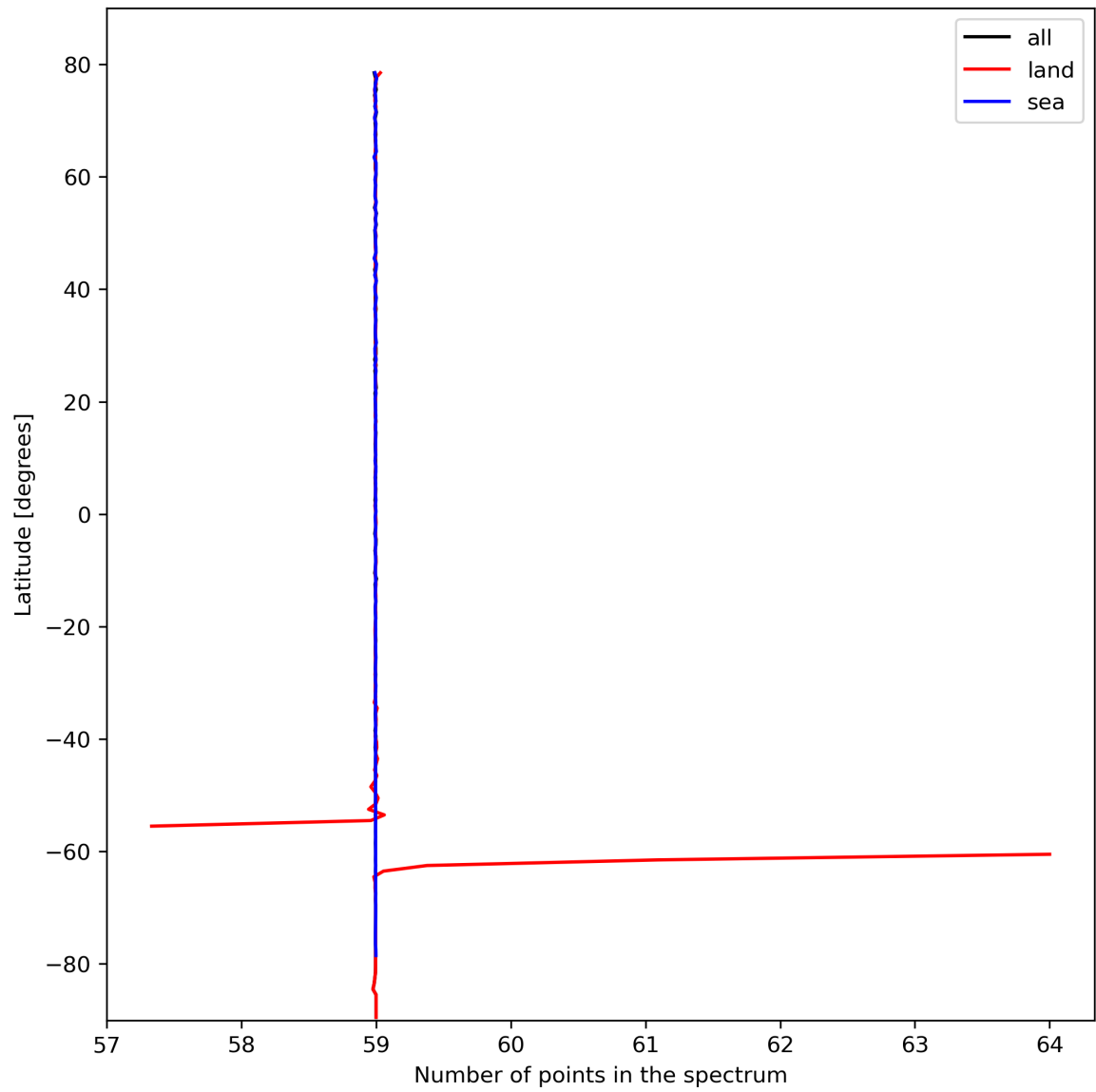
Figure 27: Zonal average of “Number of points in the spectrum” for 2023-10-17 to 2023-10-19.
