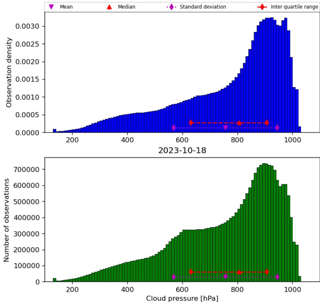
Figure 30: Histogram of “Cloud pressure” for 2023-10-17 to 2023-10-19
