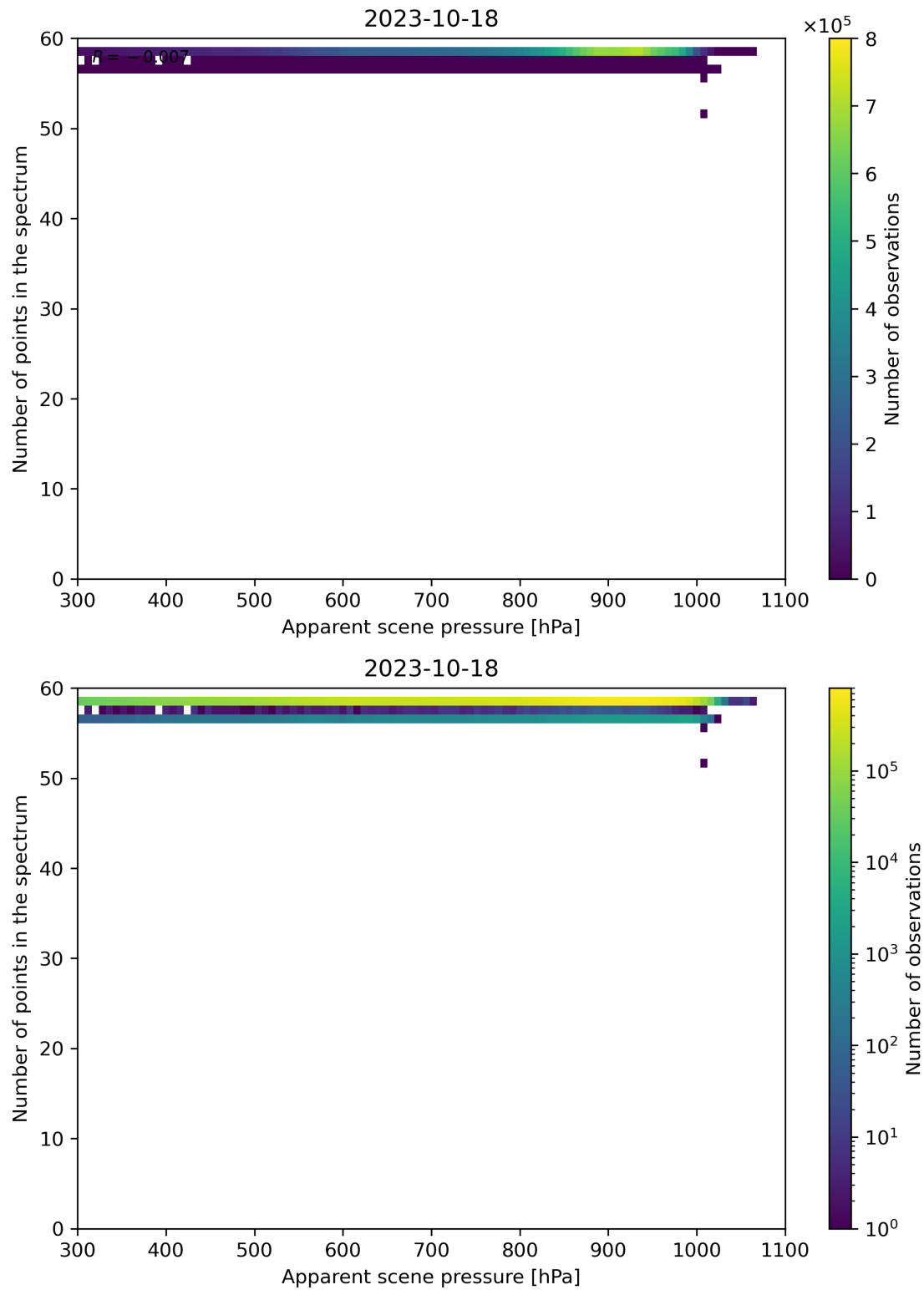
Figure 67: Scatter density plot of “Apparent scene pressure” against “Number of points in the spectrum” for 2023-10-17 to 2023-10-19.
