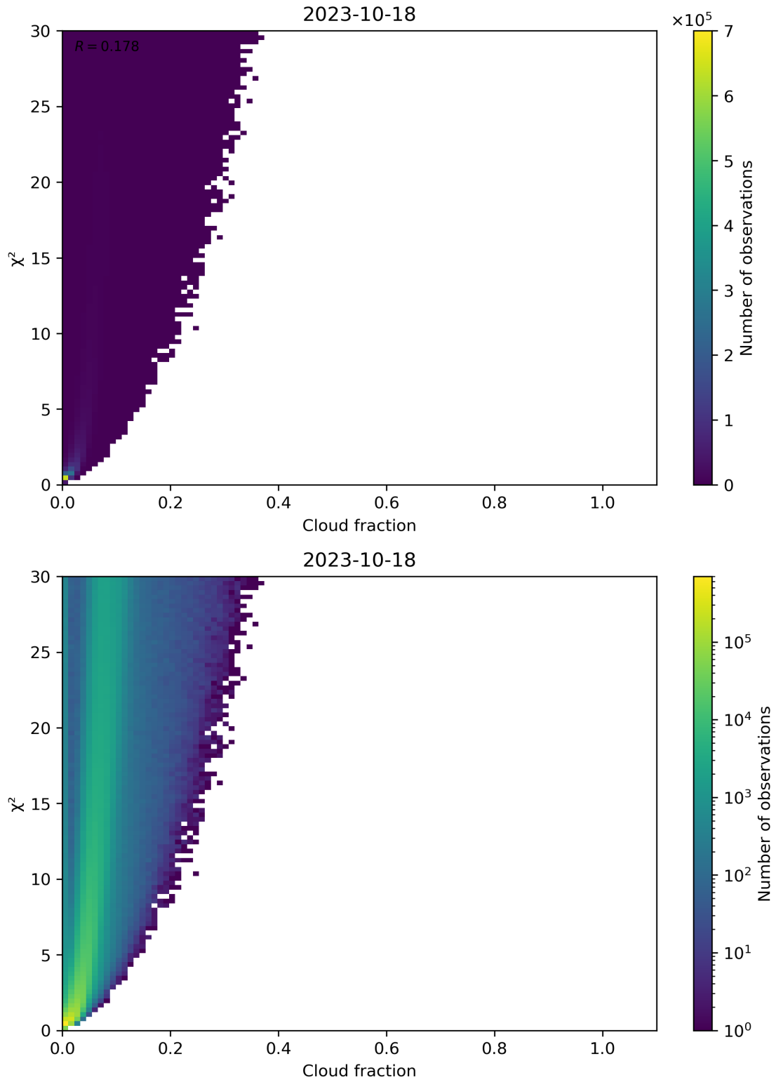
Figure 77: Scatter density plot of “Cloud fraction” against “ \chi^2 ” for 2023-10-17 to 2023-10-19.
