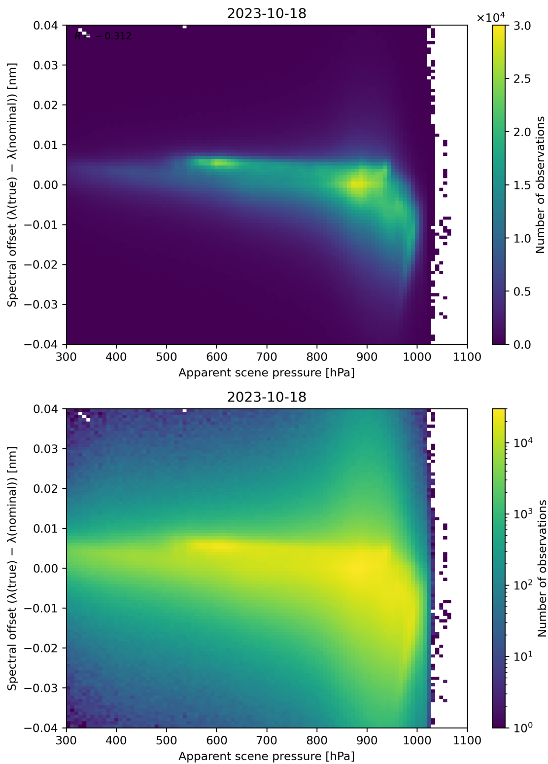
Figure 68: Scatter density plot of “Apparent scene pressure” against “Spectral offset ( \lambda(\text{true}) - \lambda(\text{nominal}) )” for 2023-10-17 to 2023-10-19.
