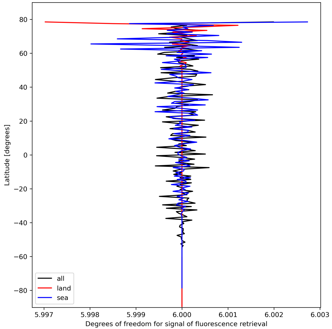
Figure 26: Zonal average of “Degrees of freedom for signal of fluorescence retrieval” for 2023-10-17 to 2023-10-19.
