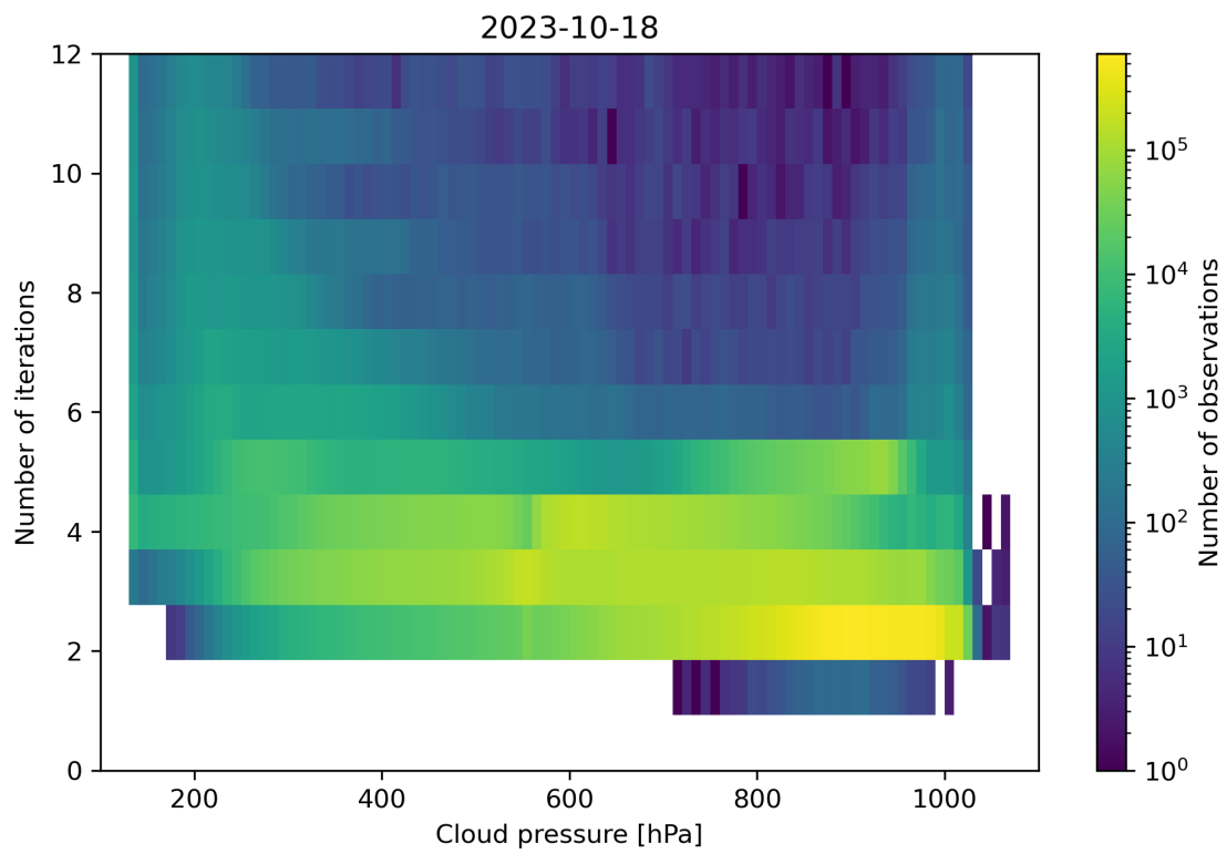
Figure 89: Scatter density plot of “Cloud pressure” against “Number of iterations” for 2023-10-17 to 2023-10-19.
