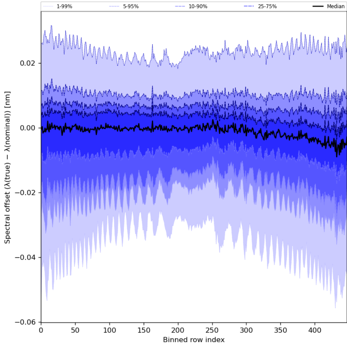
Figure 62: Along track statistics of “Spectral offset ( \lambda(\text{true}) - \lambda(\text{nominal}) )” for 2023-10-17 to 2023-10-19
