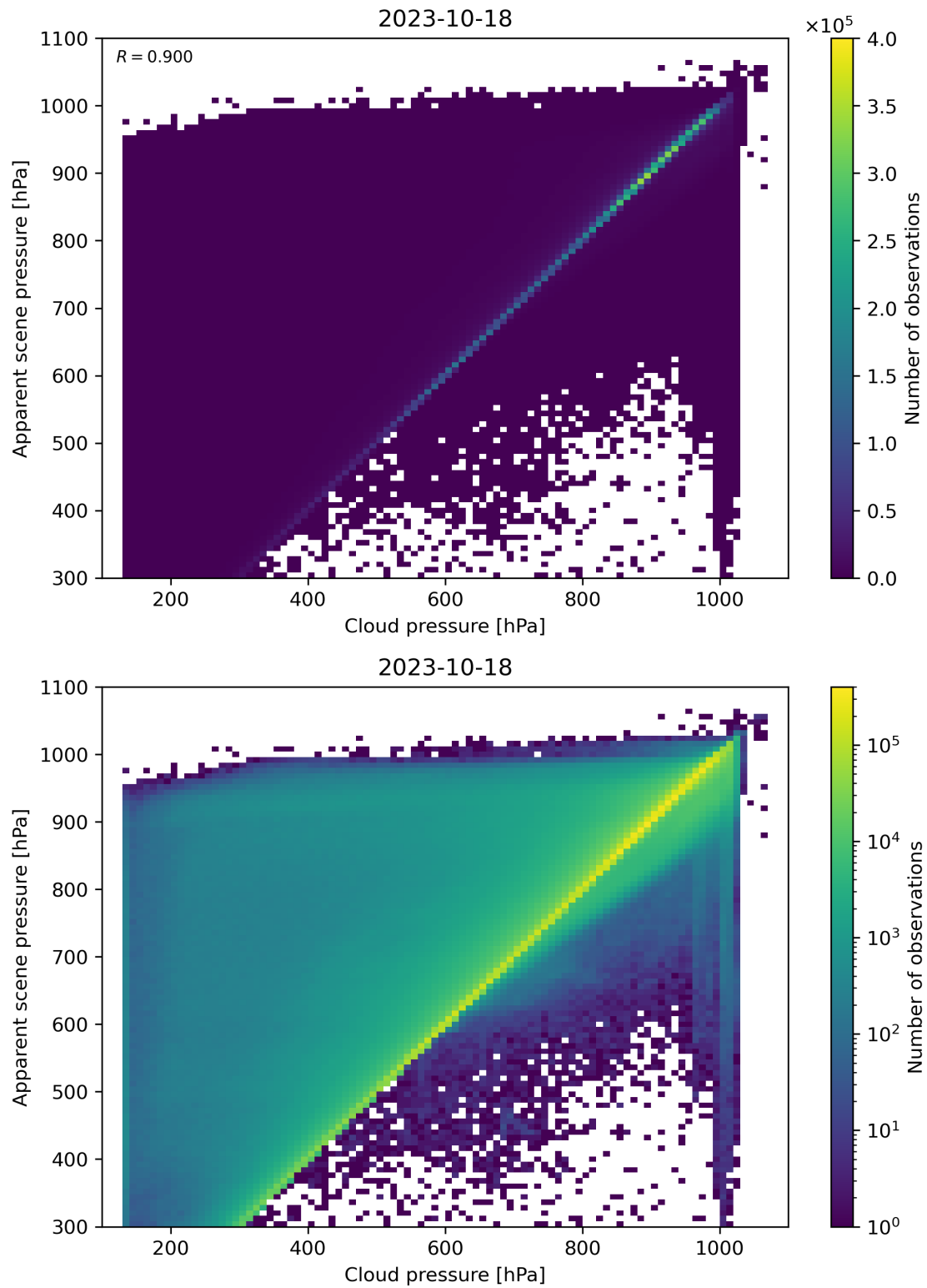
Figure 84: Scatter density plot of “Cloud pressure” against “Apparent scene pressure” for 2023-10-17 to 2023-10-19.
