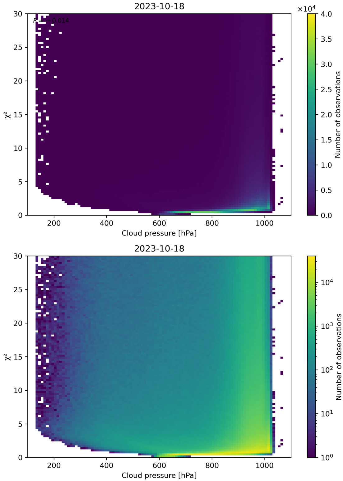
Figure 85: Scatter density plot of “Cloud pressure” against “ \chi^2 ” for 2023-10-17 to 2023-10-19.
