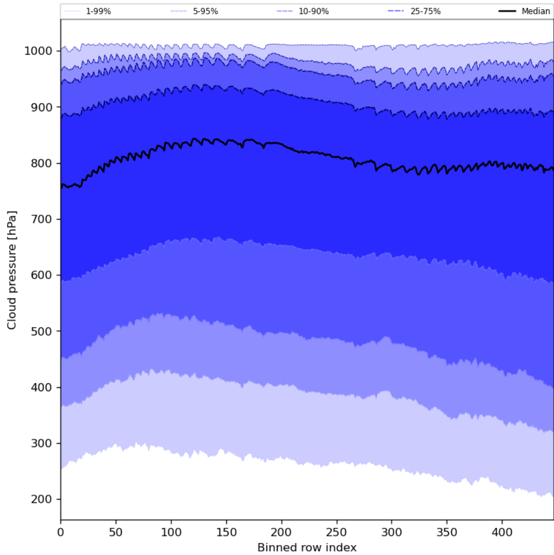
Figure 47: Along track statistics of “Cloud pressure” for 2023-10-17 to 2023-10-19
