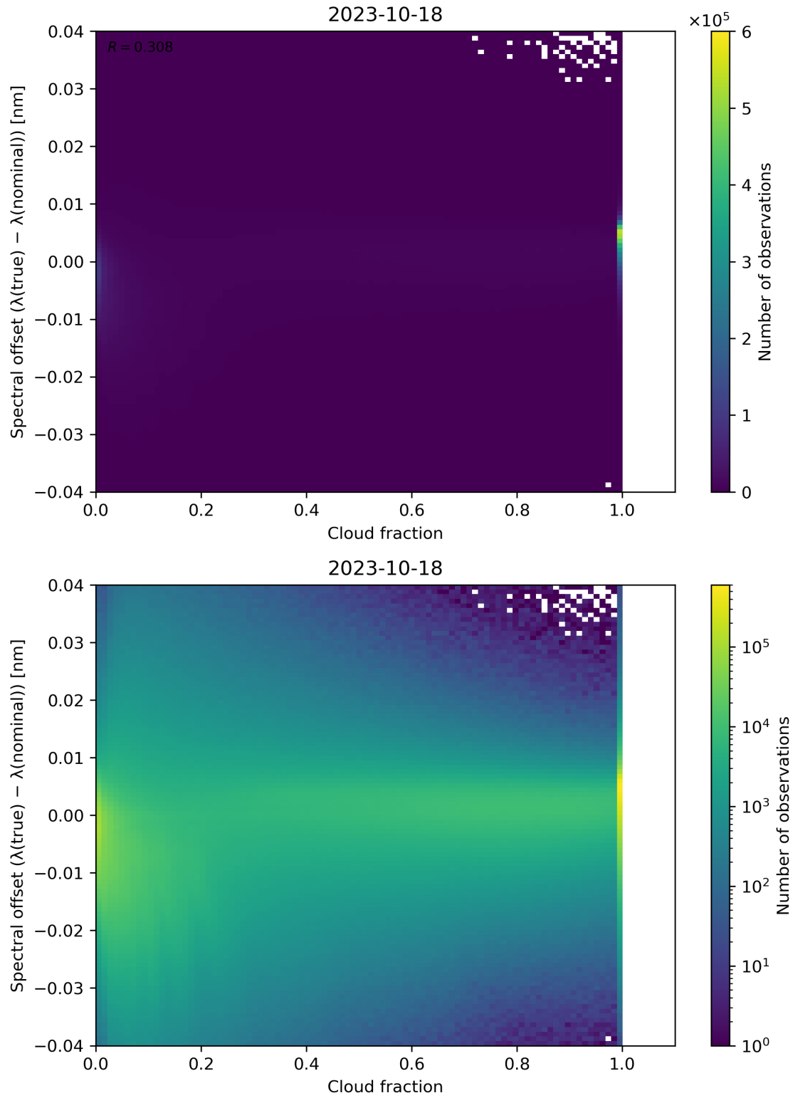
Figure 83: Scatter density plot of “Cloud fraction” against “Spectral offset ( \lambda(\text{true}) - \lambda(\text{nominal}) )” for 2023-10-17 to 2023-10-19.
