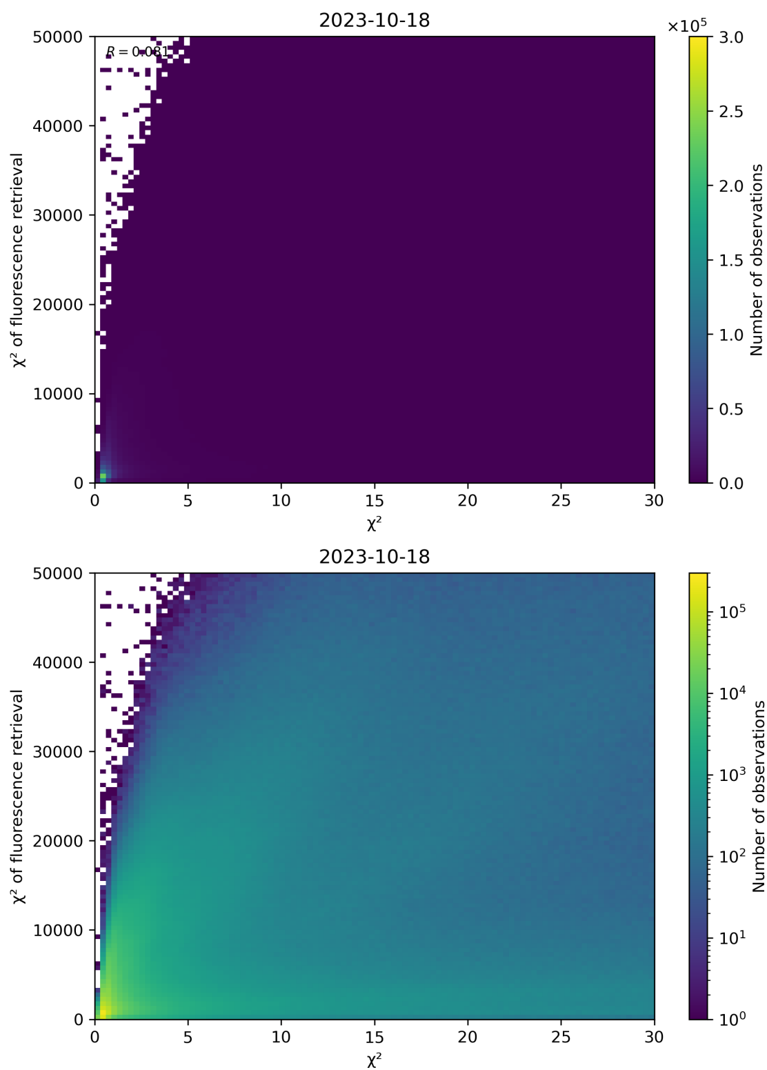
Figure 69: Scatter density plot of “ \chi^2 ” against “ \chi^2 of fluorescence retrieval” for 2023-10-17 to 2023-10-19.
