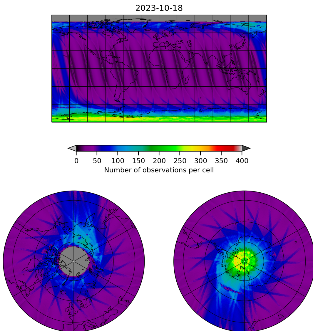
Figure 11: Map of the number of observations for 2023-10-17 to 2023-10-19
