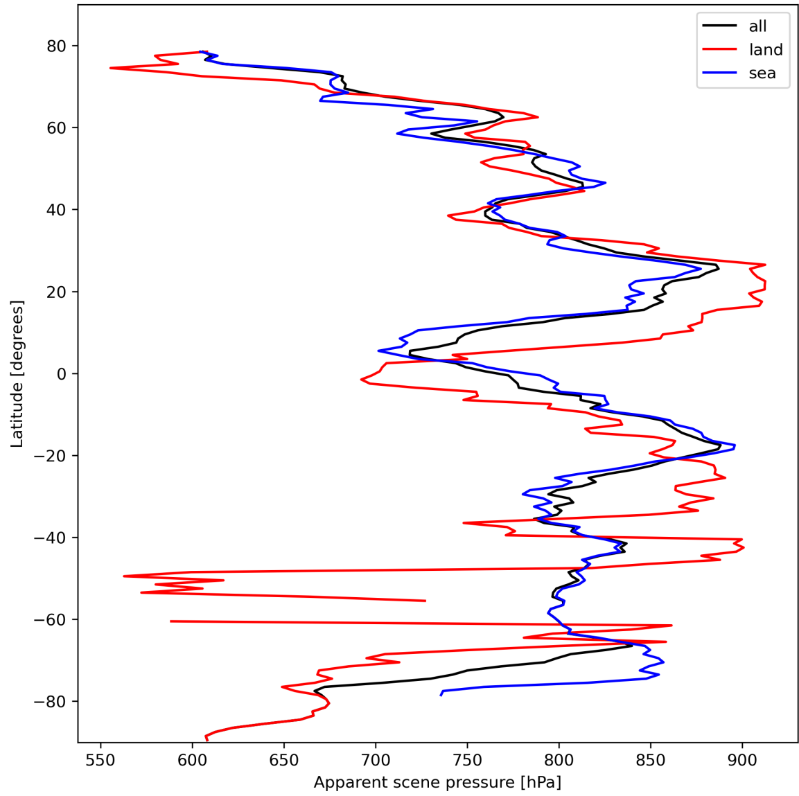
Figure 19: Zonal average of “Apparent scene pressure” for 2023-10-17 to 2023-10-19.
