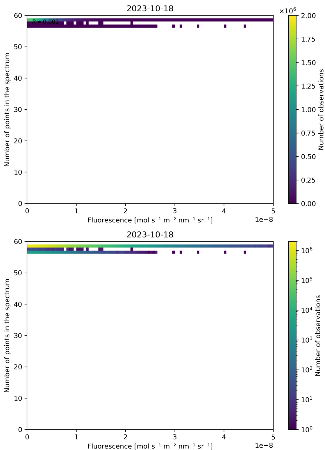
Figure 94: Scatter density plot of “Fluorescence” against “Number of points in the spectrum” for 2023-10-17 to 2023-10-19.
