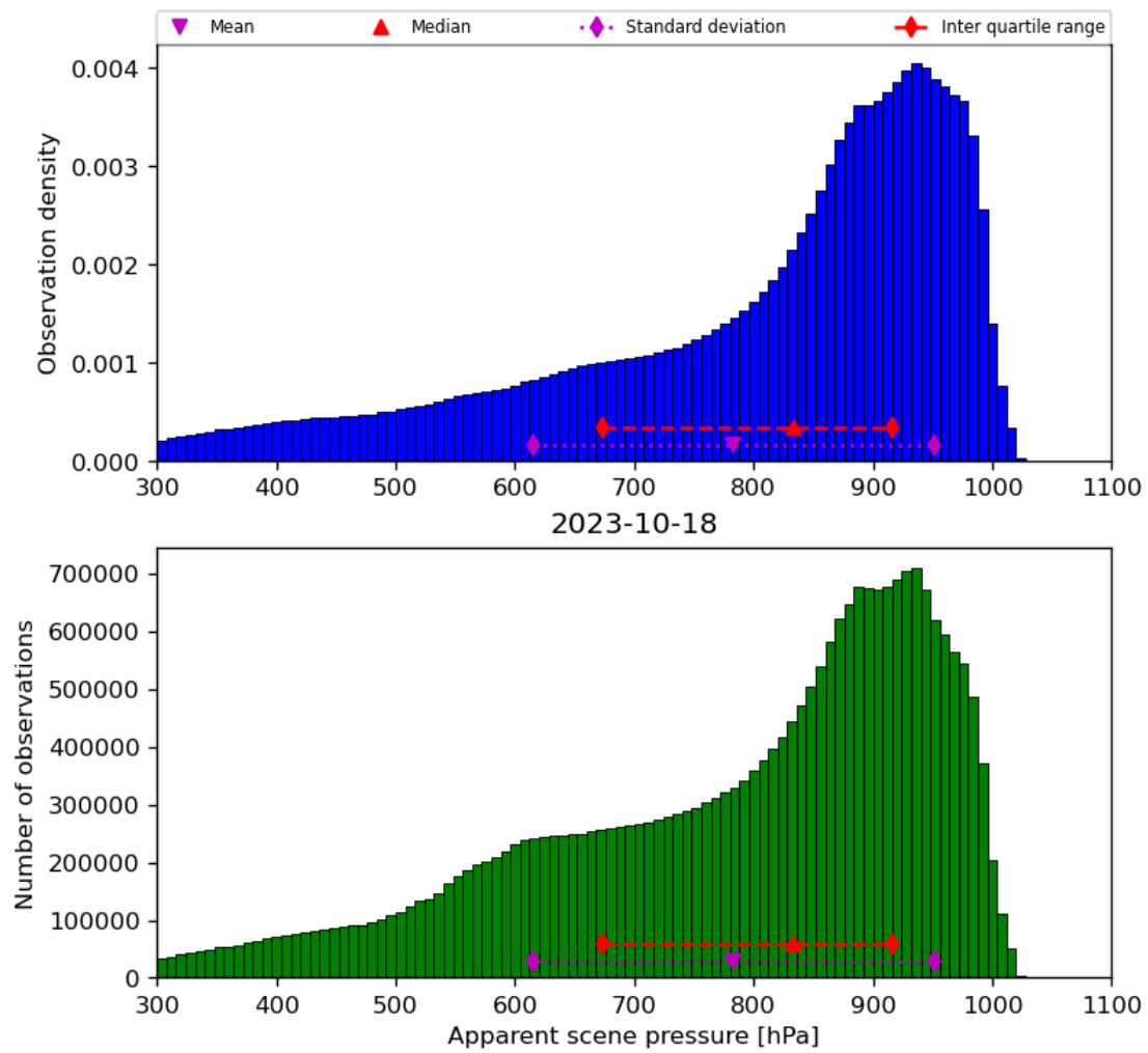
Figure 36: Histogram of “Apparent scene pressure” for 2023-10-17 to 2023-10-19
