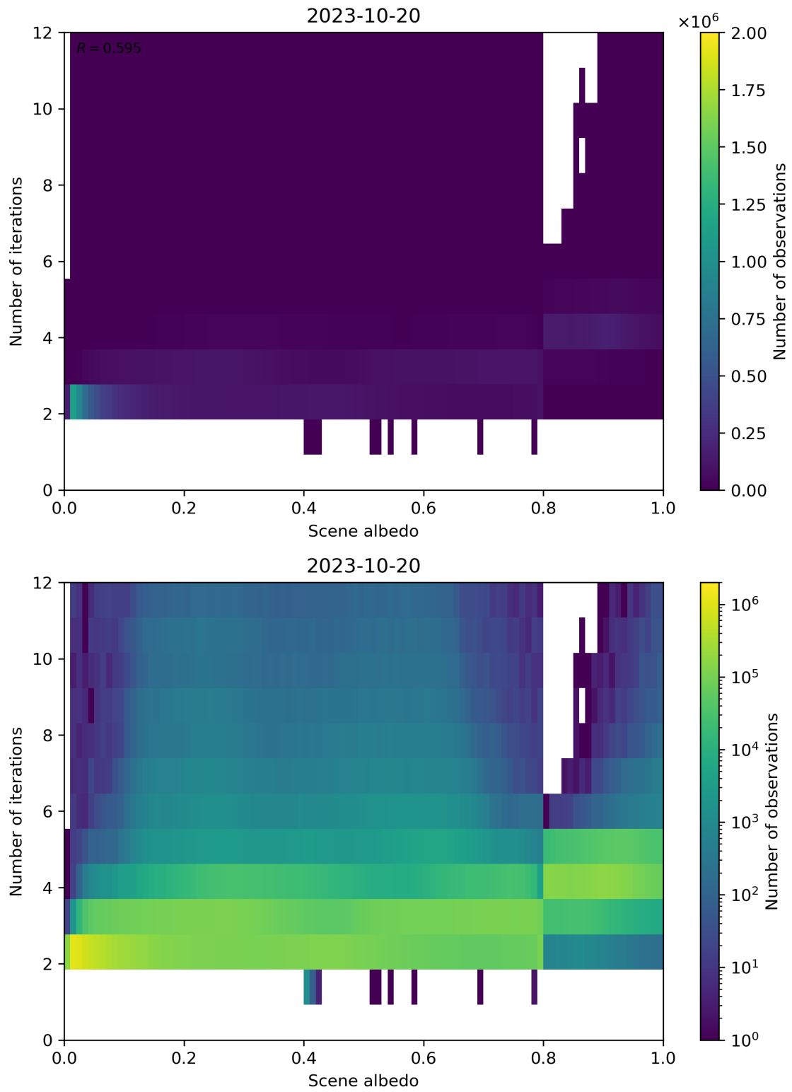
Figure 115: Scatter density plot of “Scene albedo” against “Number of iterations” for 2023-10-19 to 2023-10-21.
