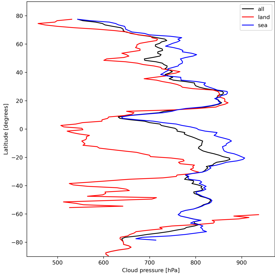
Figure 13: Zonal average of “Cloud pressure” for 2023-10-19 to 2023-10-21.
