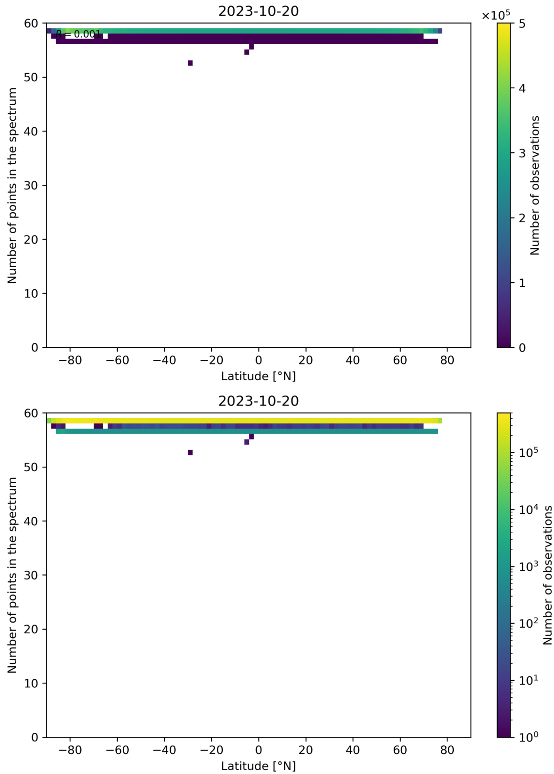
Figure 103: Scatter density plot of “Latitude” against “Number of points in the spectrum” for 2023-10-19 to 2023-10-21.
