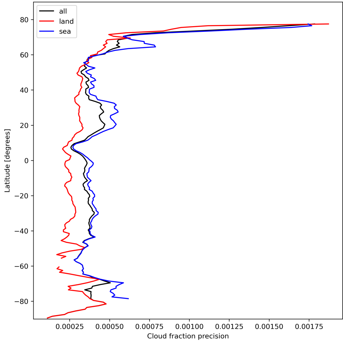
Figure 16: Zonal average of “Cloud fraction precision” for 2023-10-19 to 2023-10-21.
