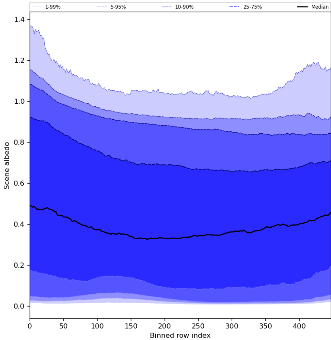
Figure 51: Along track statistics of “Scene albedo” for 2023-10-19 to 2023-10-21
