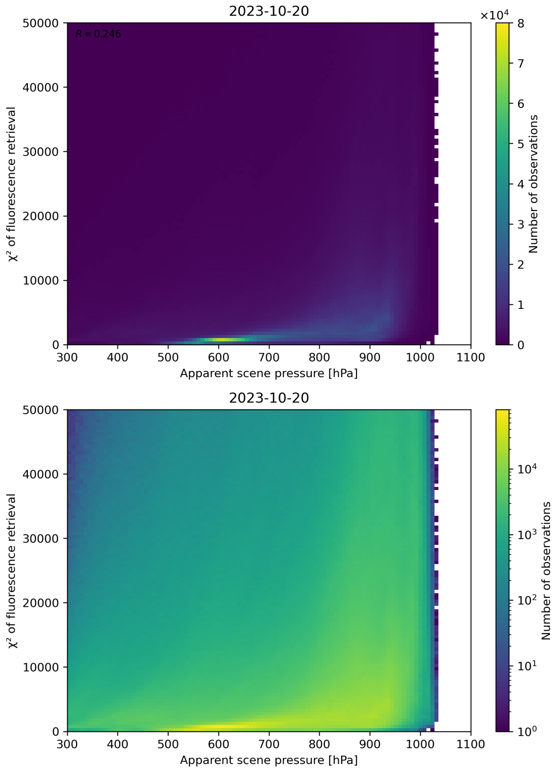
Figure 64: Scatter density plot of “Apparent scene pressure” against “ \chi^2 of fluorescence retrieval” for 2023-10-19 to 2023-10-21.
