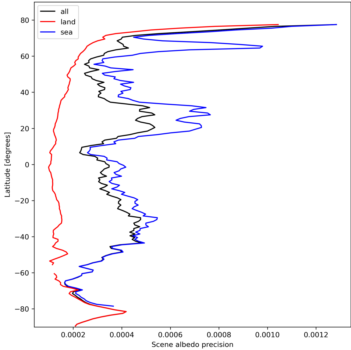
Figure 18: Zonal average of “Scene albedo precision” for 2023-10-19 to 2023-10-21.
