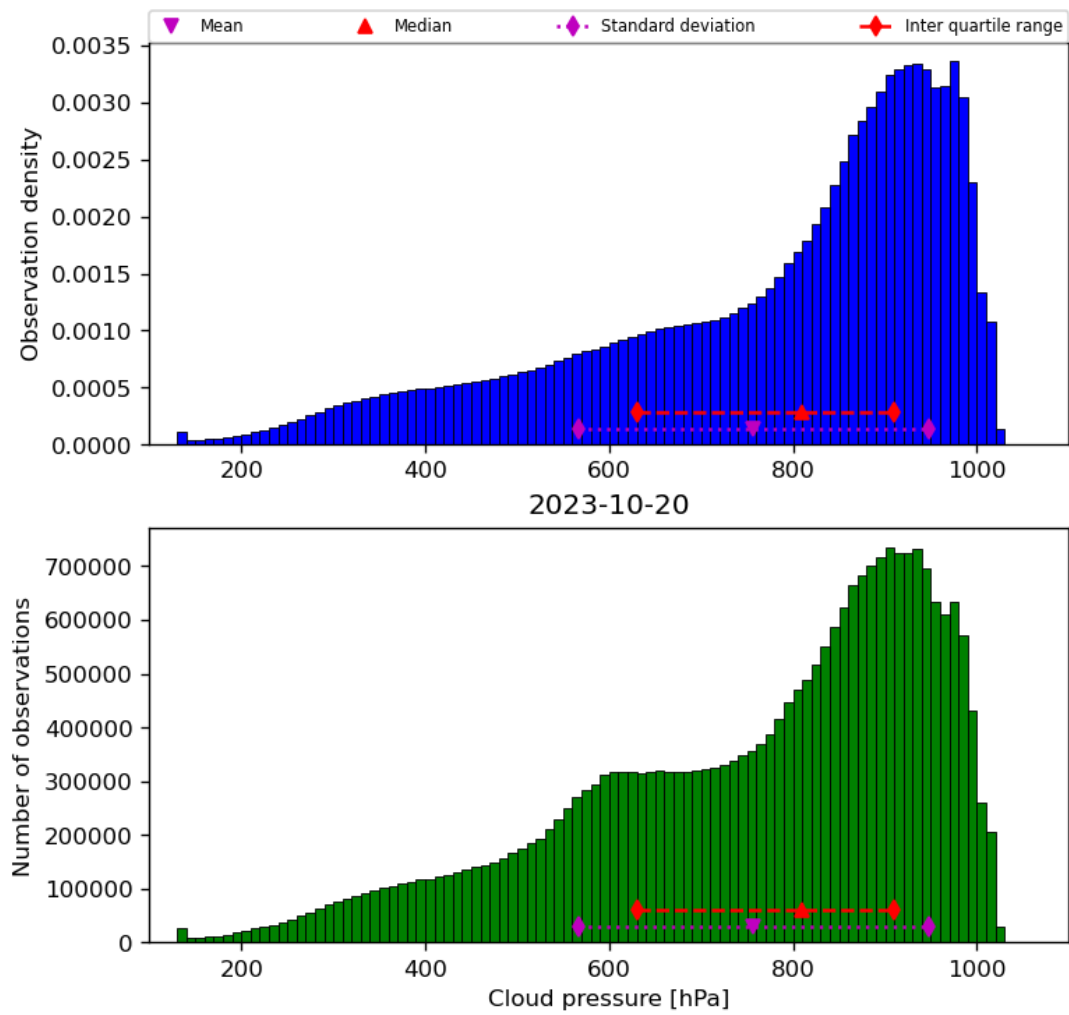
Figure 30: Histogram of “Cloud pressure” for 2023-10-19 to 2023-10-21
