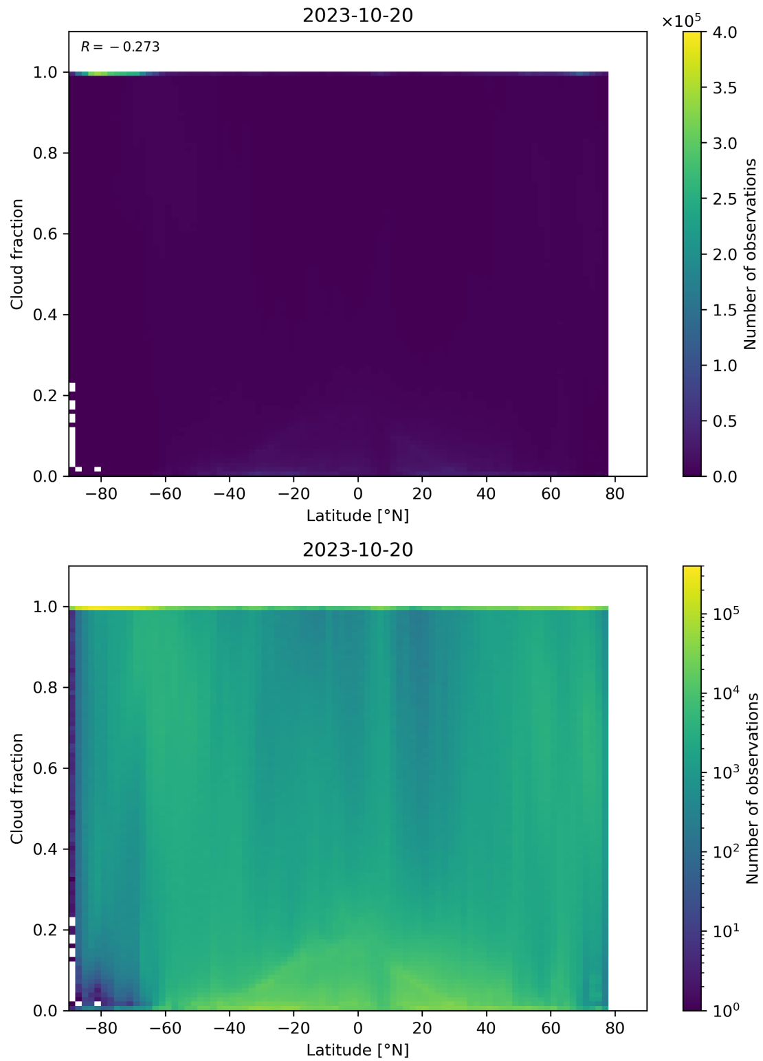
Figure 99: Scatter density plot of “Latitude” against “Cloud fraction” for 2023-10-19 to 2023-10-21.
