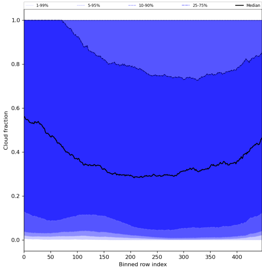
Figure 49: Along track statistics of “Cloud fraction” for 2023-10-19 to 2023-10-21
