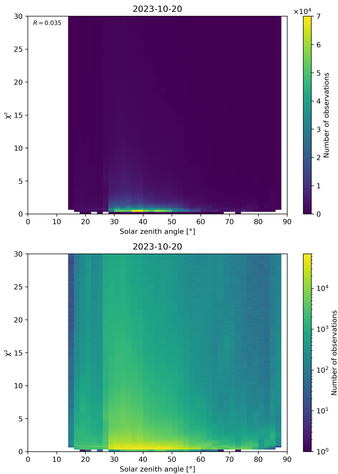
Figure 119: Scatter density plot of “Solar zenith angle” against “ \chi^2 ” for 2023-10-19 to 2023-10-21.
