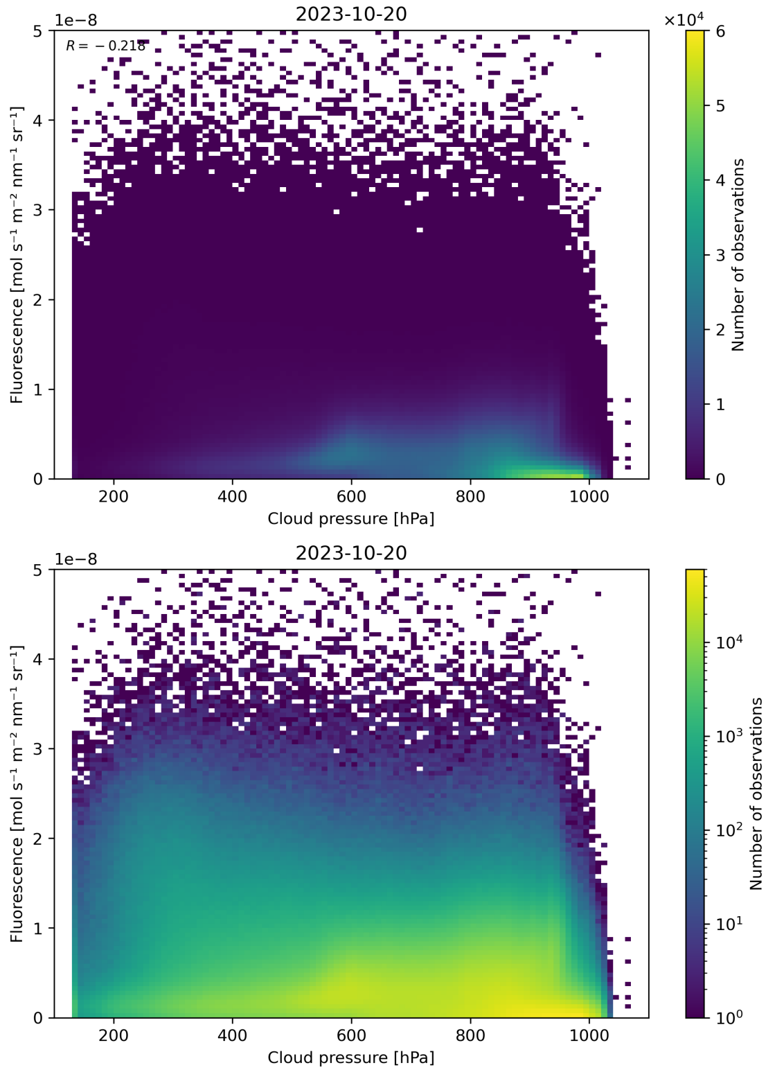
Figure 88: Scatter density plot of “Cloud pressure” against “Fluorescence” for 2023-10-19 to 2023-10-21.
