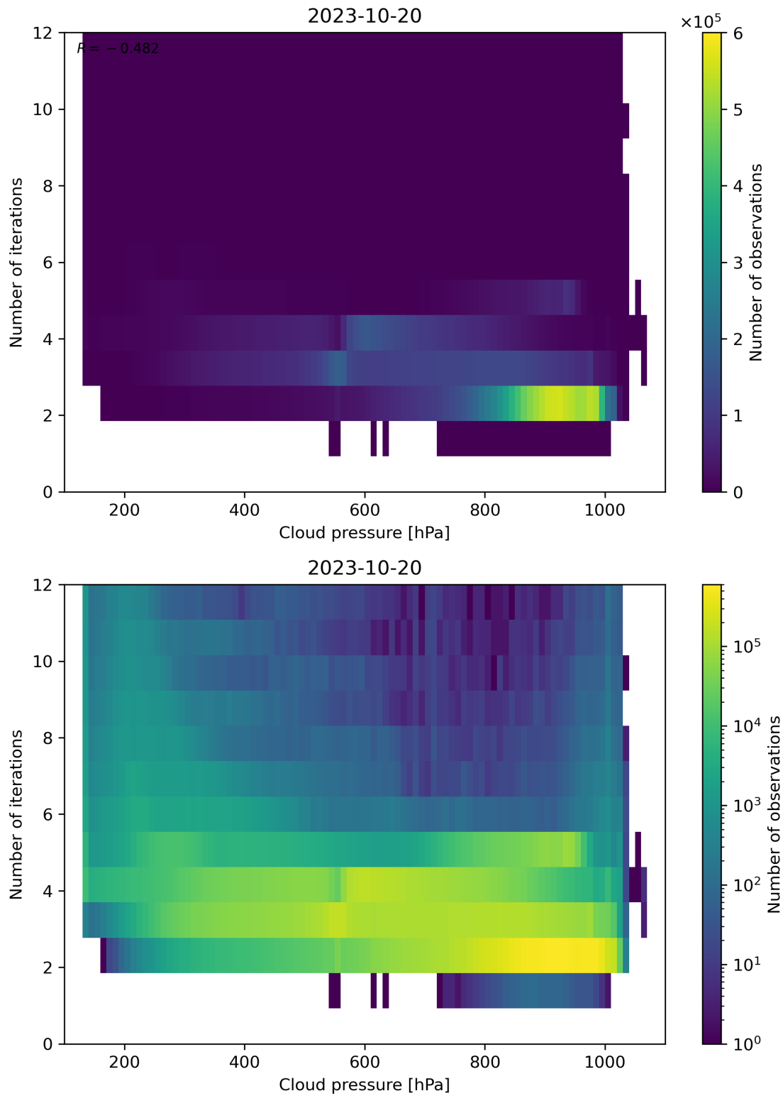
Figure 89: Scatter density plot of “Cloud pressure” against “Number of iterations” for 2023-10-19 to 2023-10-21.
