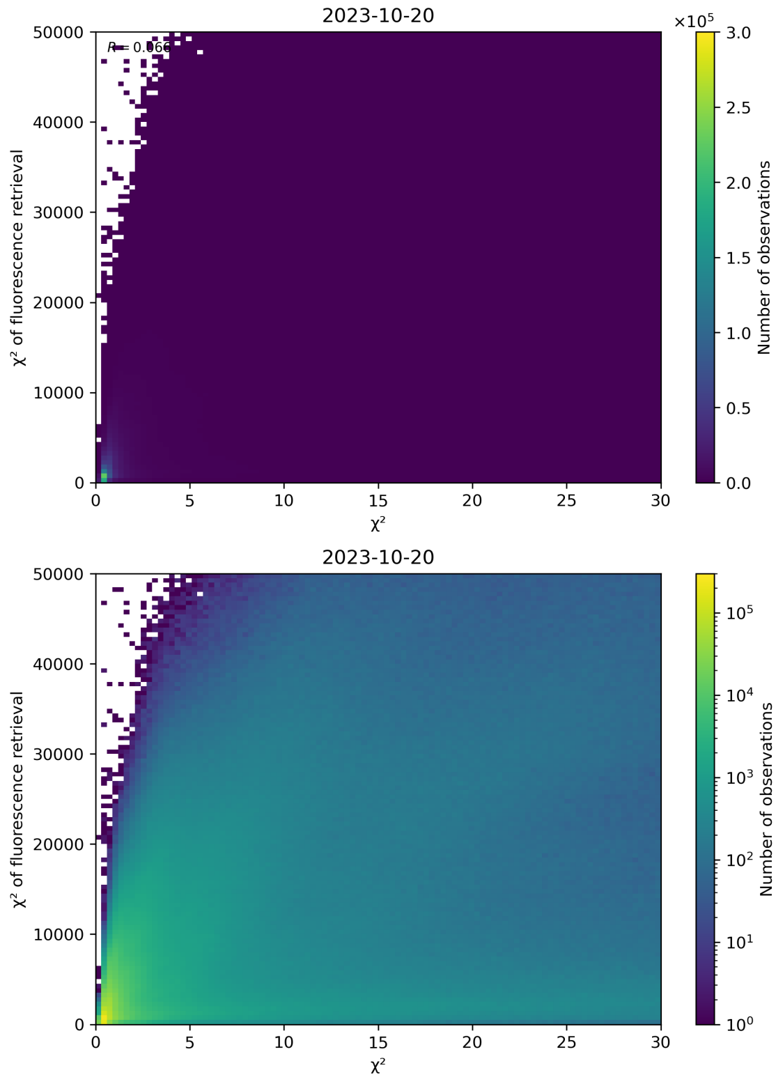
Figure 69: Scatter density plot of “ \chi^2 ” against “ \chi^2 of fluorescence retrieval” for 2023-10-19 to 2023-10-21.
