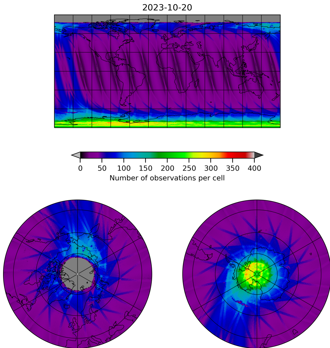
Figure 11: Map of the number of observations for 2023-10-19 to 2023-10-21
