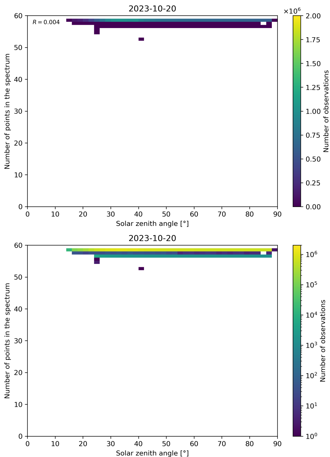
Figure 126: Scatter density plot of “Solar zenith angle” against “Number of points in the spectrum” for 2023-10-19 to 2023-10-21.
