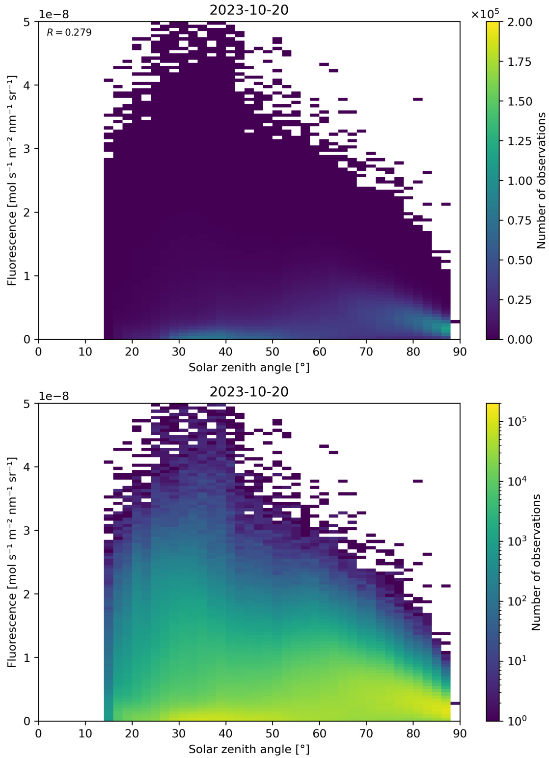
Figure 123: Scatter density plot of “Solar zenith angle” against “Fluorescence” for 2023-10-19 to 2023-10-21.
