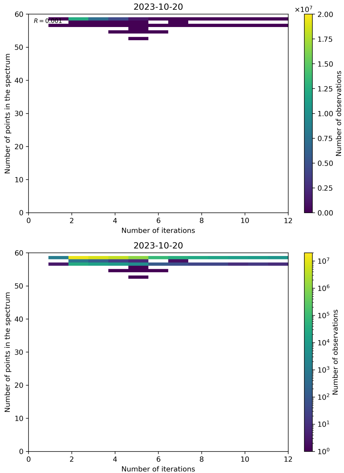
Figure 108: Scatter density plot of “Number of iterations” against “Number of points in the spectrum” for 2023-10-19 to 2023-10-21.
