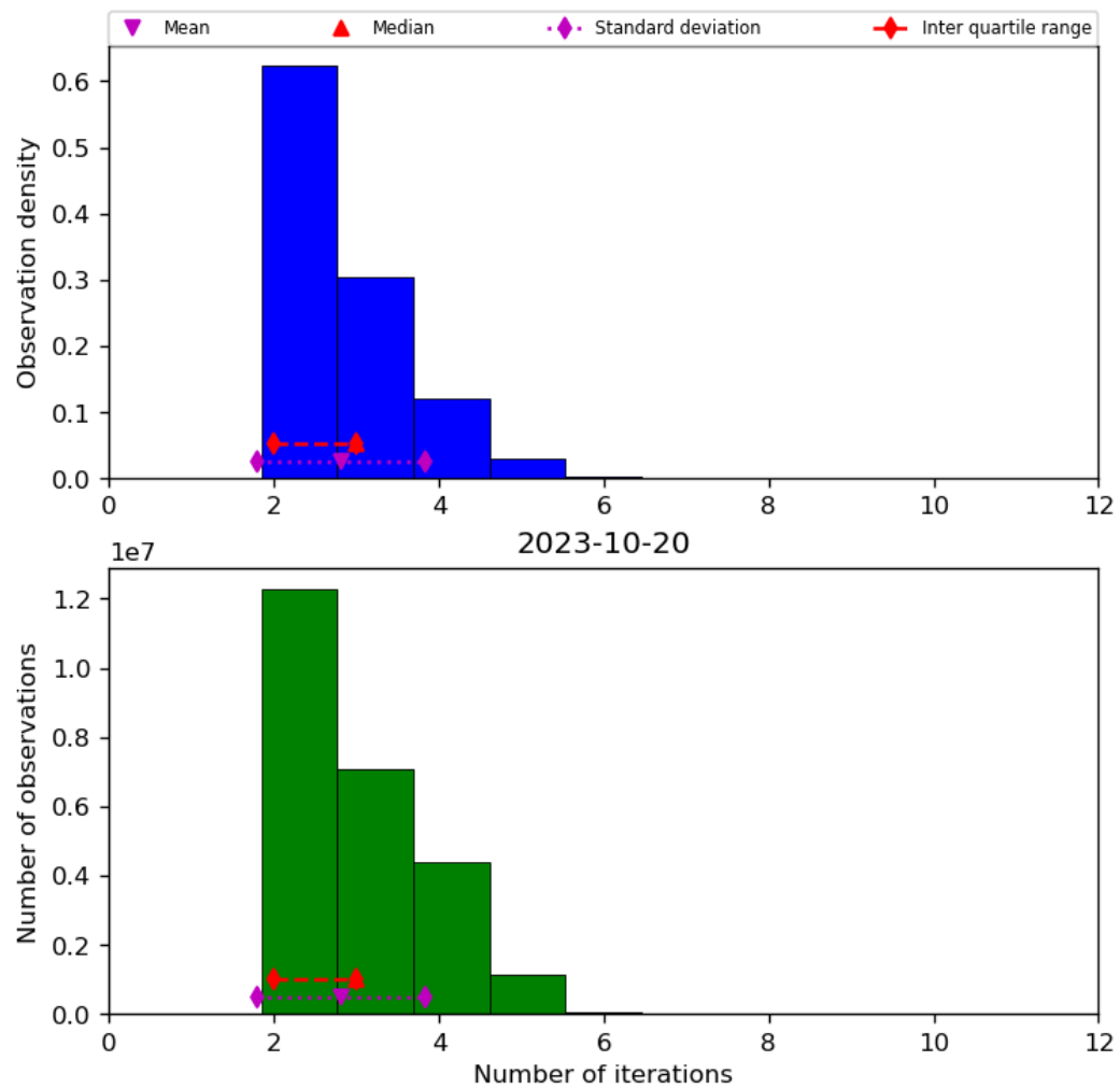
Figure 39: Histogram of “Number of iterations” for 2023-10-19 to 2023-10-21
