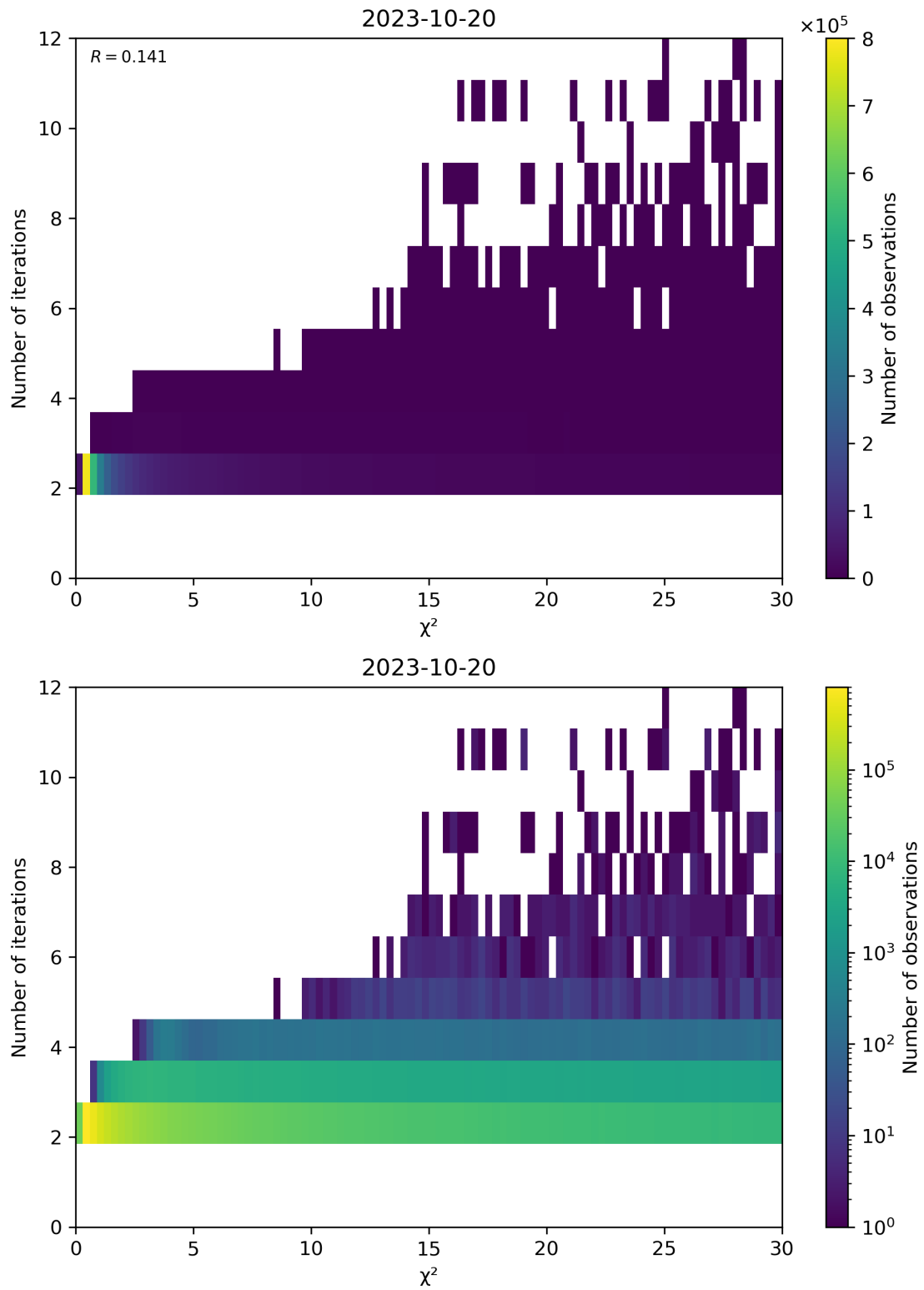
Figure 73: Scatter density plot of " \chi^2 " against "Number of iterations" for 2023-10-19 to 2023-10-21.
