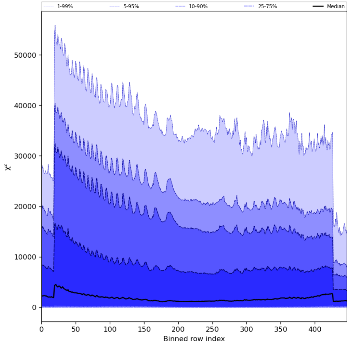
Figure 55: Along track statistics of “ \chi^2 ” for 2023-10-19 to 2023-10-21
