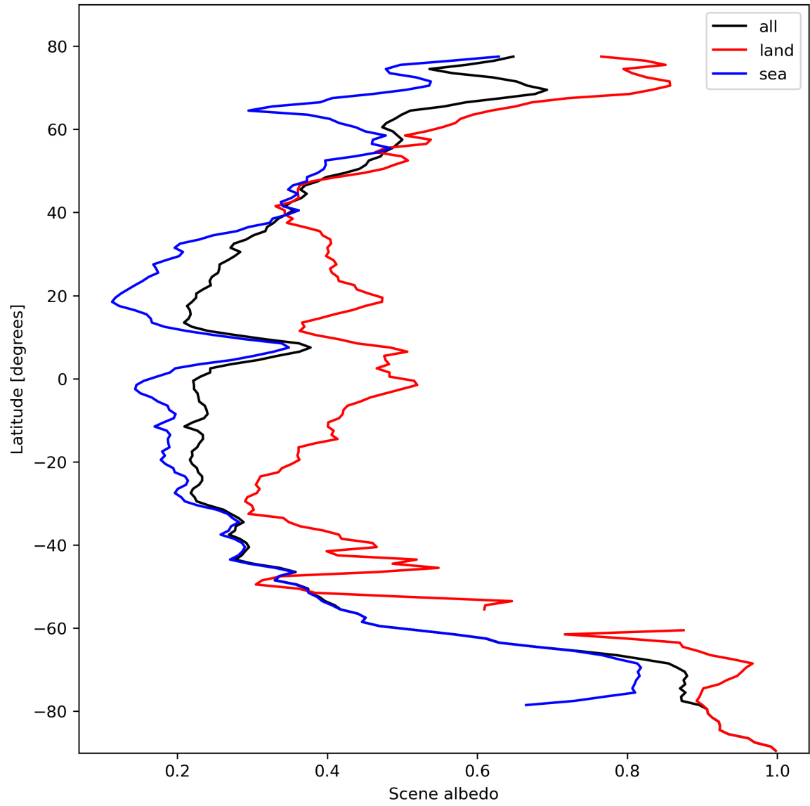
Figure 17: Zonal average of “Scene albedo” for 2023-10-19 to 2023-10-21.
