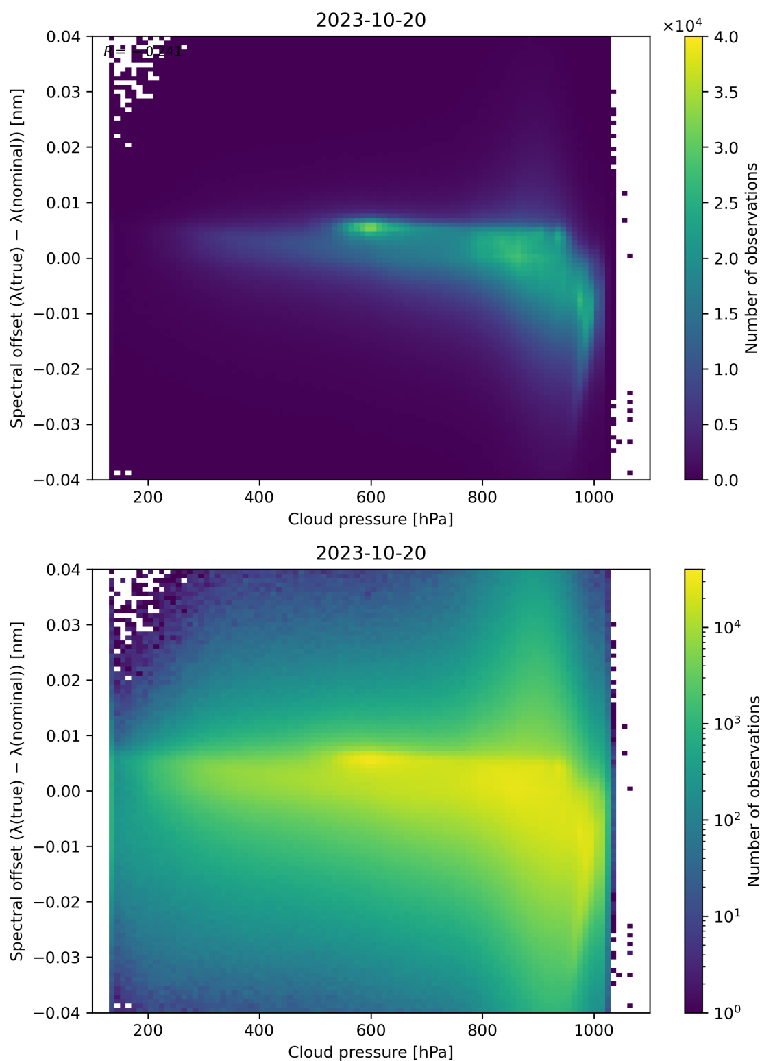
Figure 92: Scatter density plot of “Cloud pressure” against “Spectral offset ( \lambda(\text{true}) - \lambda(\text{nominal}) )” for 2023-10-19 to 2023-10-21.
