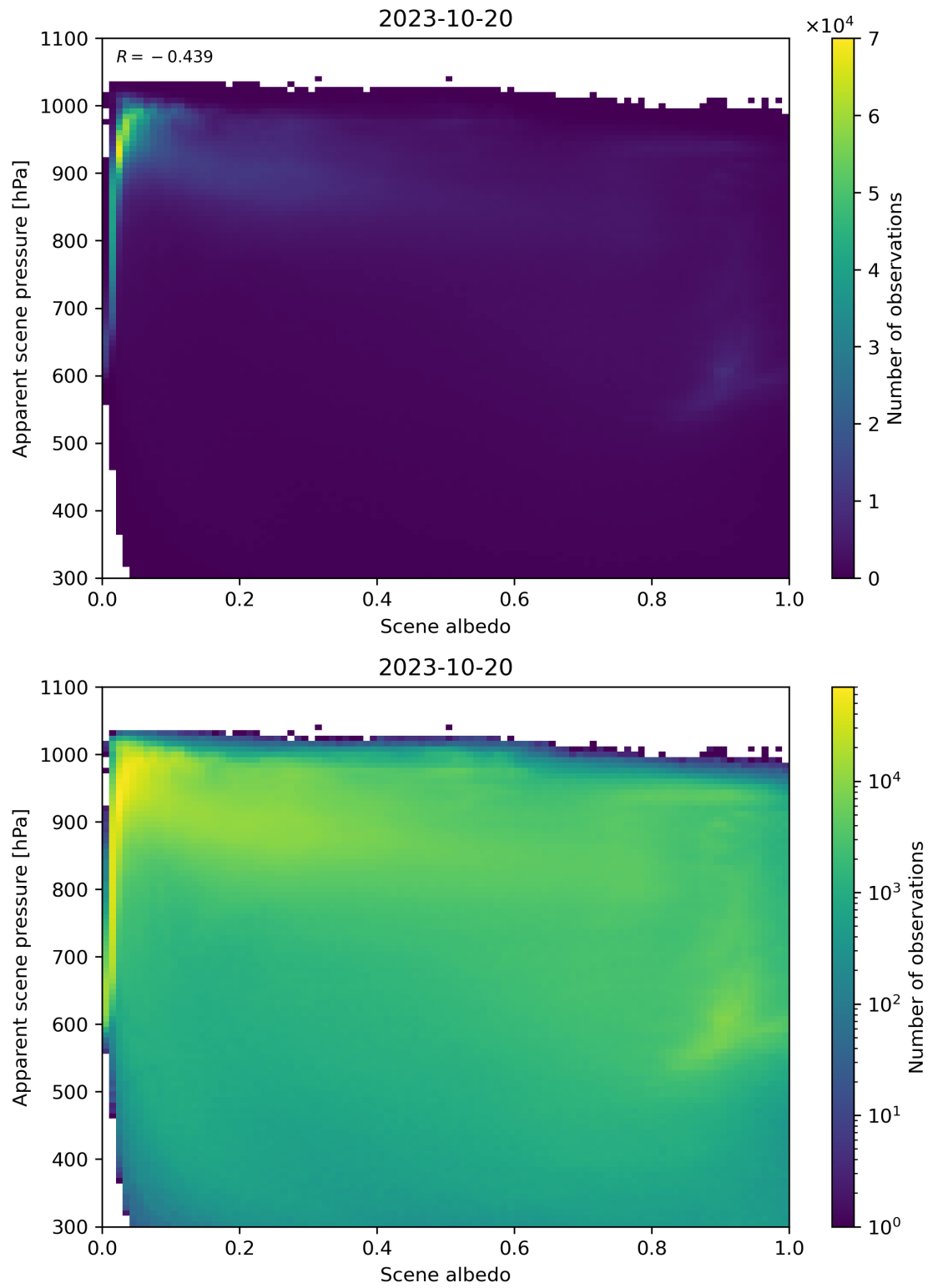
Figure 111: Scatter density plot of “Scene albedo” against “Apparent scene pressure” for 2023-10-19 to 2023-10-21.
