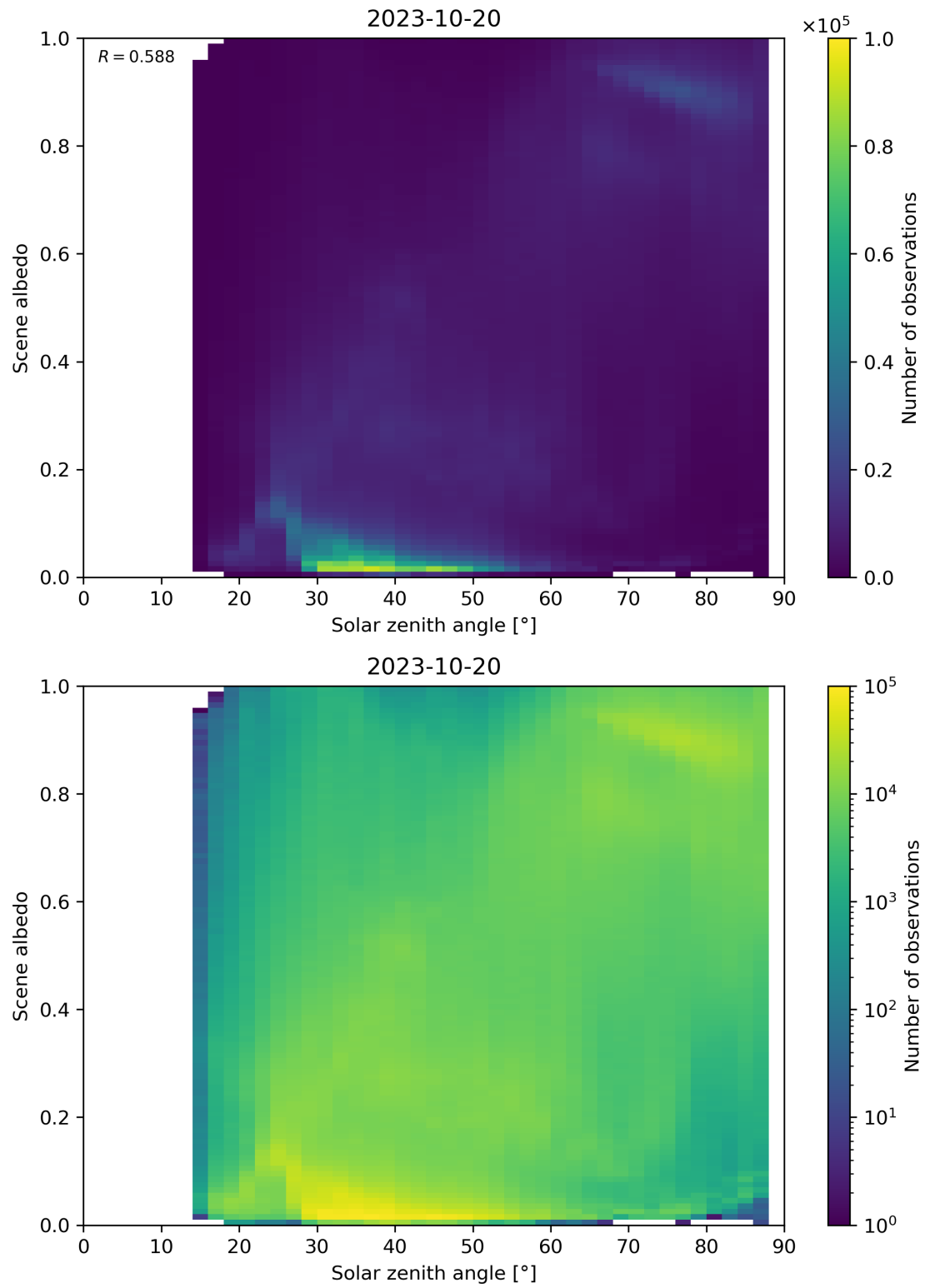
Figure 127: Scatter density plot of “Solar zenith angle” against “Scene albedo” for 2023-10-19 to 2023-10-21.
