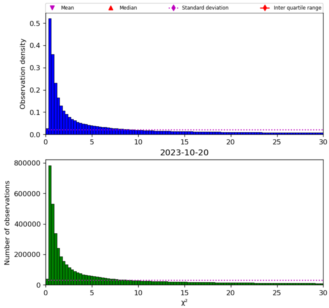
Figure 38: Histogram of “ \chi^2 ” for 2023-10-19 to 2023-10-21
