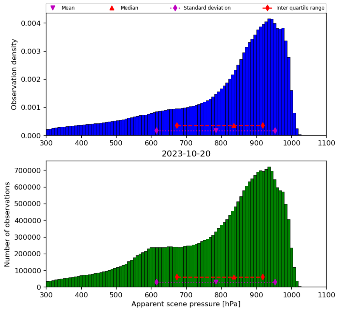
Figure 36: Histogram of “Apparent scene pressure” for 2023-10-19 to 2023-10-21
