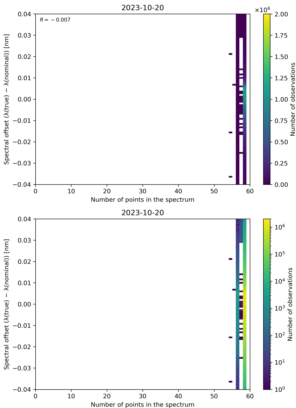
Figure 110: Scatter density plot of “Number of points in the spectrum” against “Spectral offset ( \lambda(\text{true}) - \lambda(\text{nominal}) )” for 2023-10-19 to 2023-10-21.
