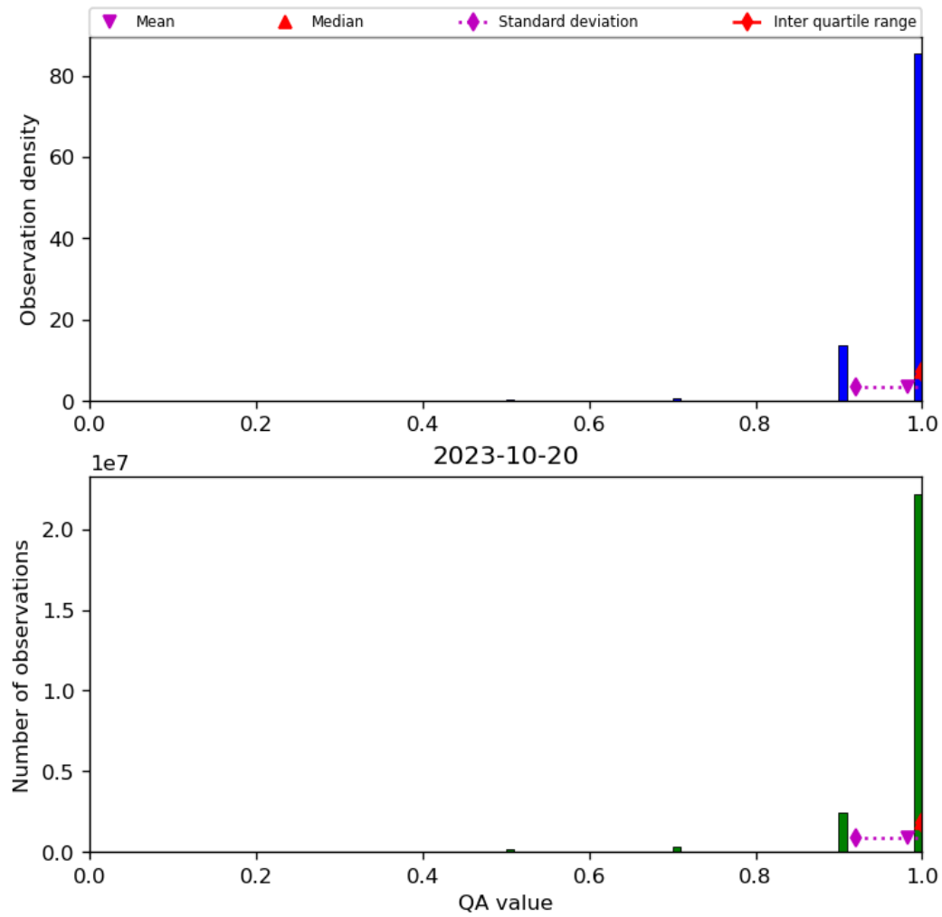
Figure 29: Histogram of “QA value” for 2023-10-19 to 2023-10-21
