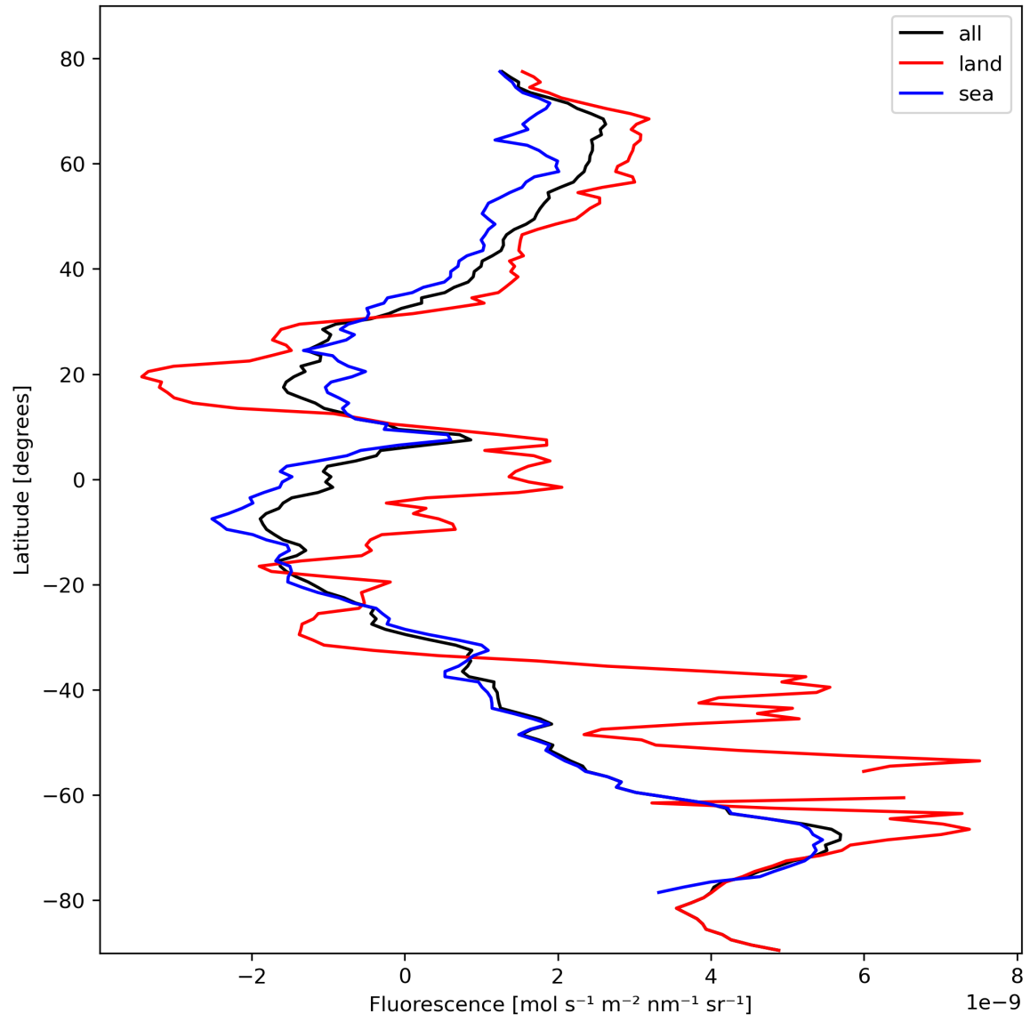
Figure 23: Zonal average of “Fluorescence” for 2023-10-19 to 2023-10-21.
