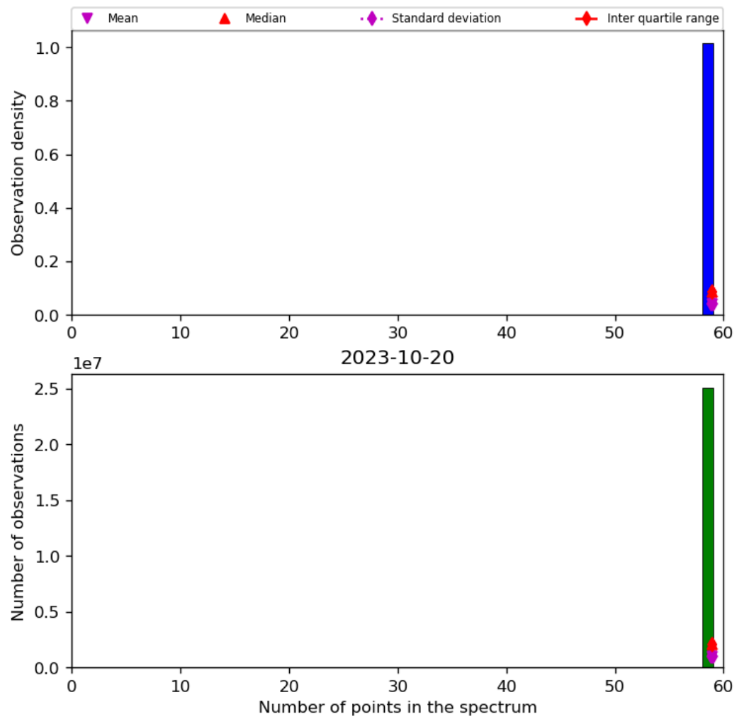
Figure 44: Histogram of “Number of points in the spectrum” for 2023-10-19 to 2023-10-21
