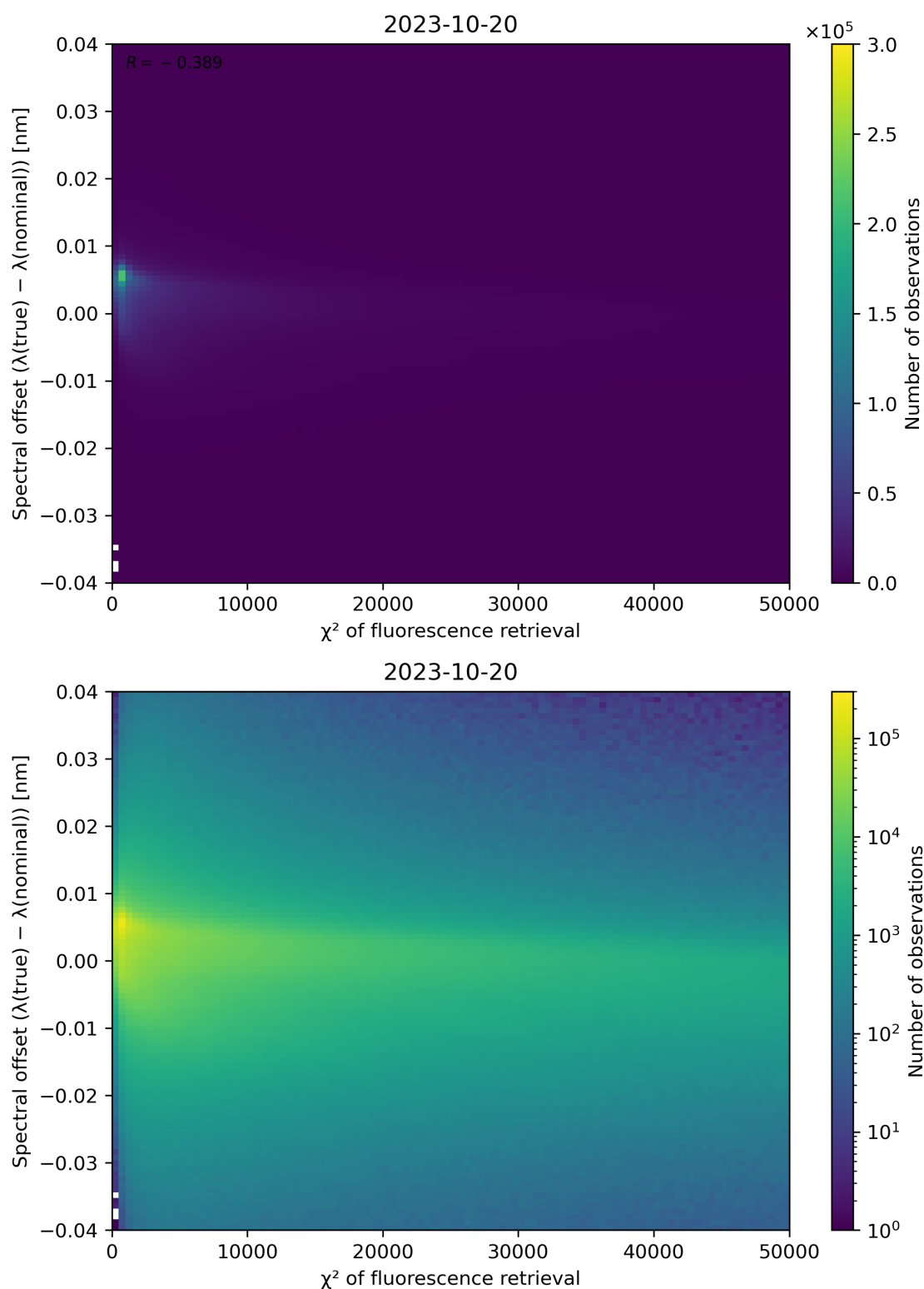
Figure 72: Scatter density plot of " \chi^2 of fluorescence retrieval" against "Spectral offset ( \lambda(\text{true}) - \lambda(\text{nominal}) )" for 2023-10-19 to 2023-10-21.
