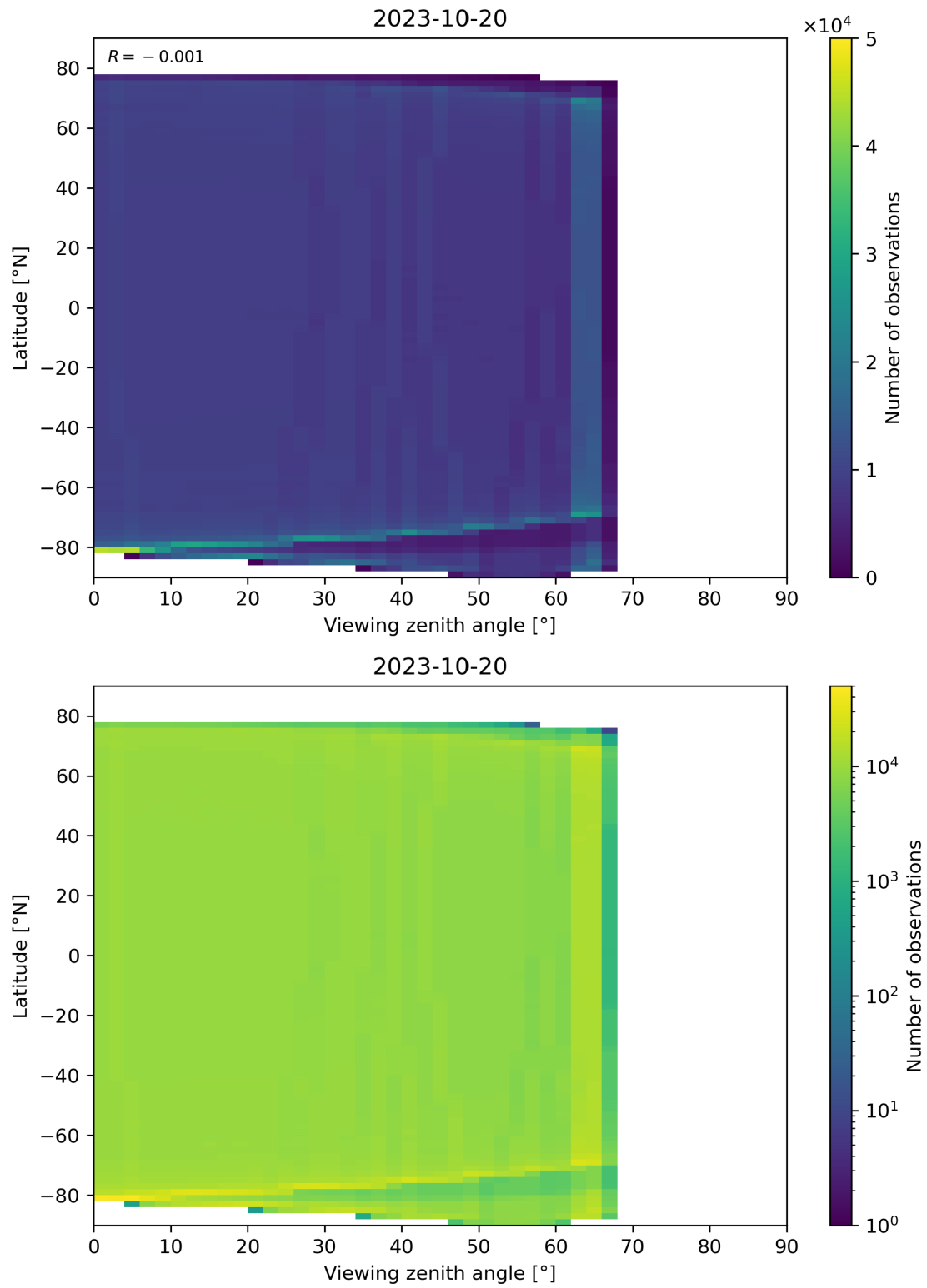
Figure 135: Scatter density plot of “Viewing zenith angle” against “Latitude” for 2023-10-19 to 2023-10-21.
