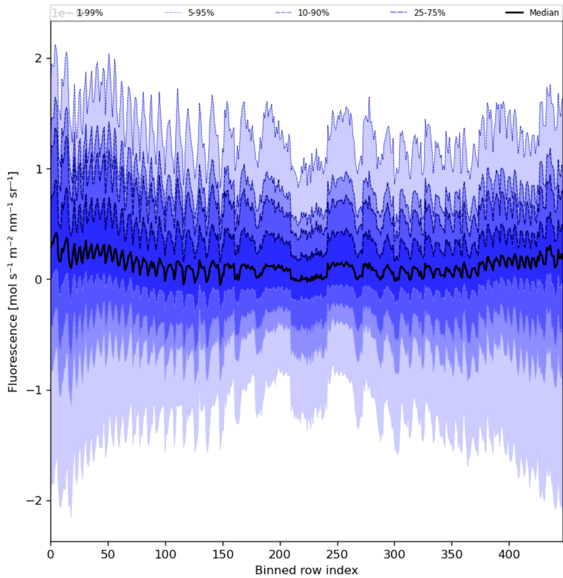
Figure 57: Along track statistics of "Fluorescence" for 2023-10-19 to 2023-10-21
