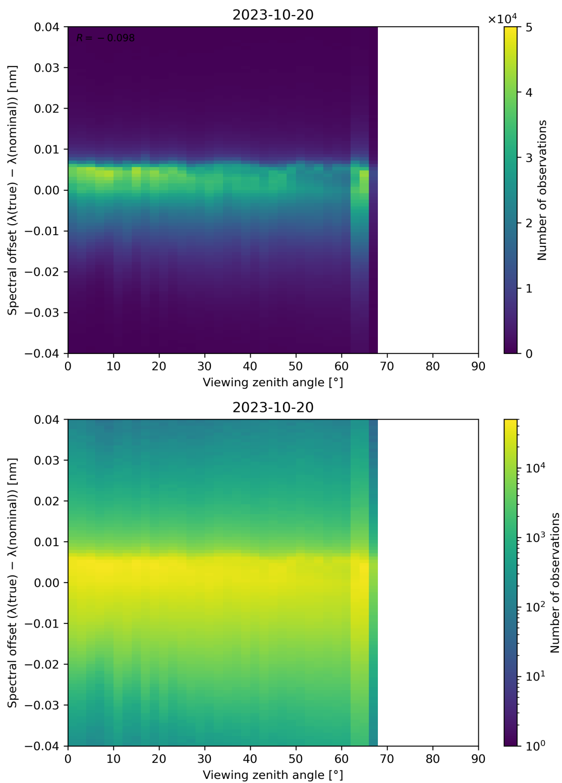
Figure 140: Scatter density plot of “Viewing zenith angle” against “Spectral offset ( \lambda(\text{true}) - \lambda(\text{nominal}) )” for 2023-10-19 to 2023-10-21.
