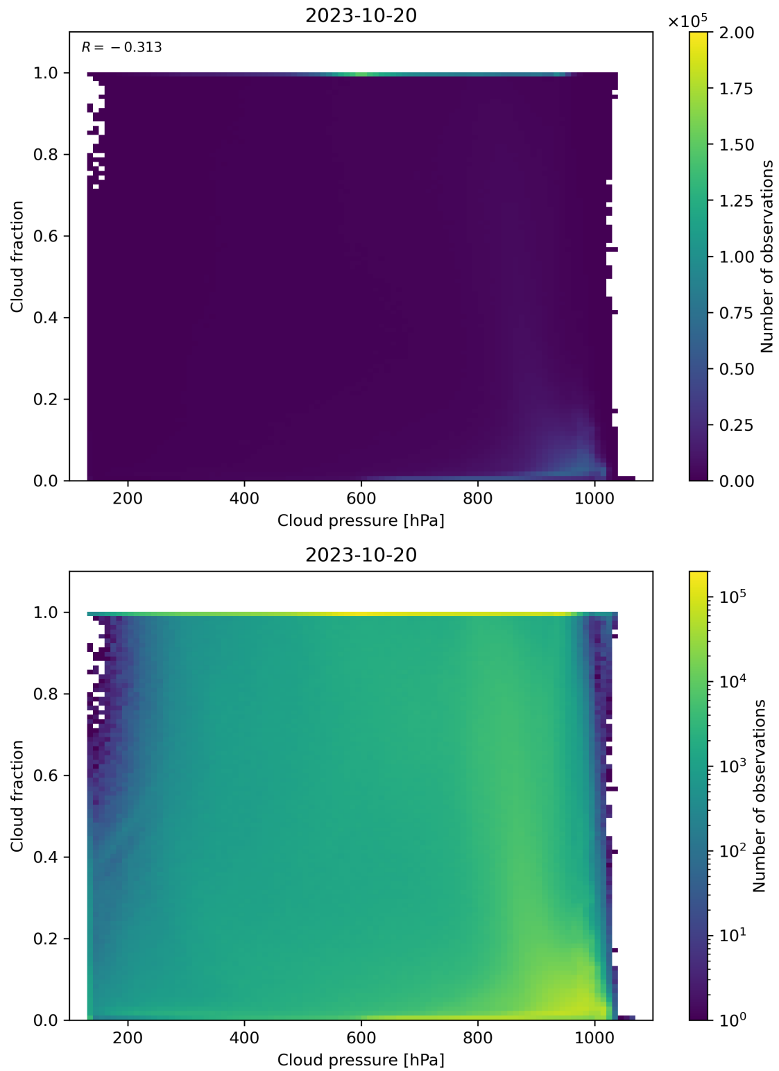
Figure 87: Scatter density plot of “Cloud pressure” against “Cloud fraction” for 2023-10-19 to 2023-10-21.
