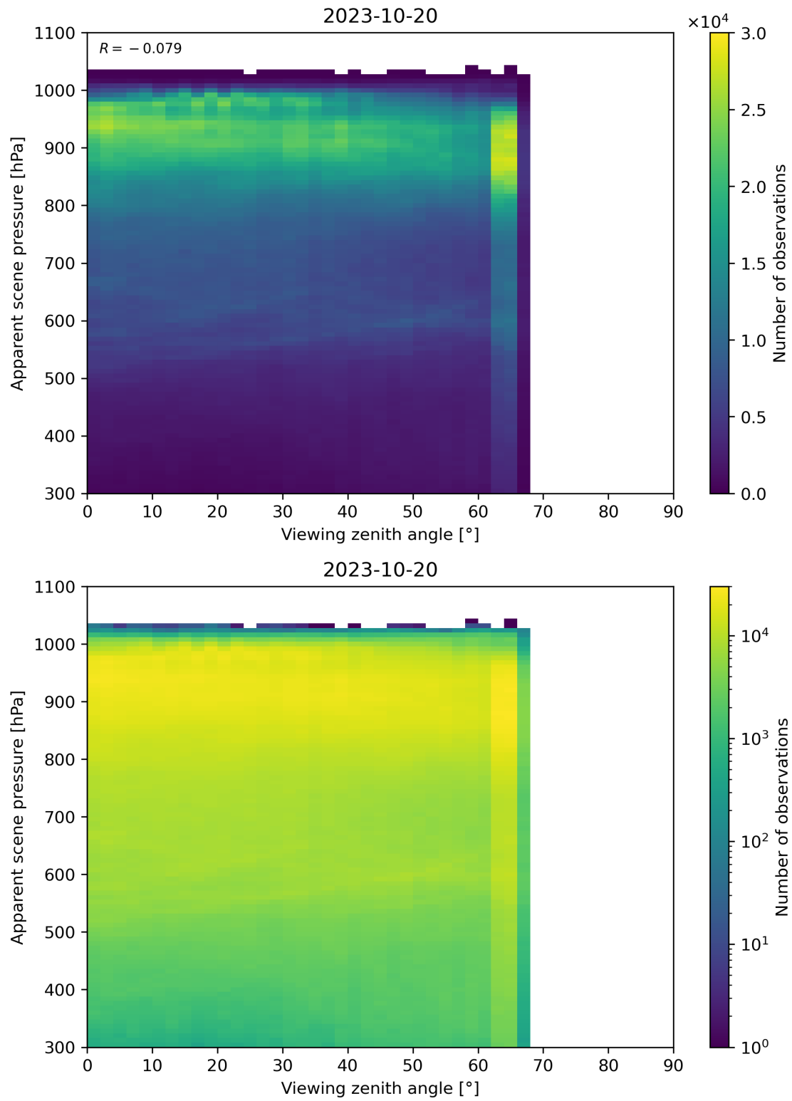
Figure 129: Scatter density plot of “Viewing zenith angle” against “Apparent scene pressure” for 2023-10-19 to 2023-10-21.
