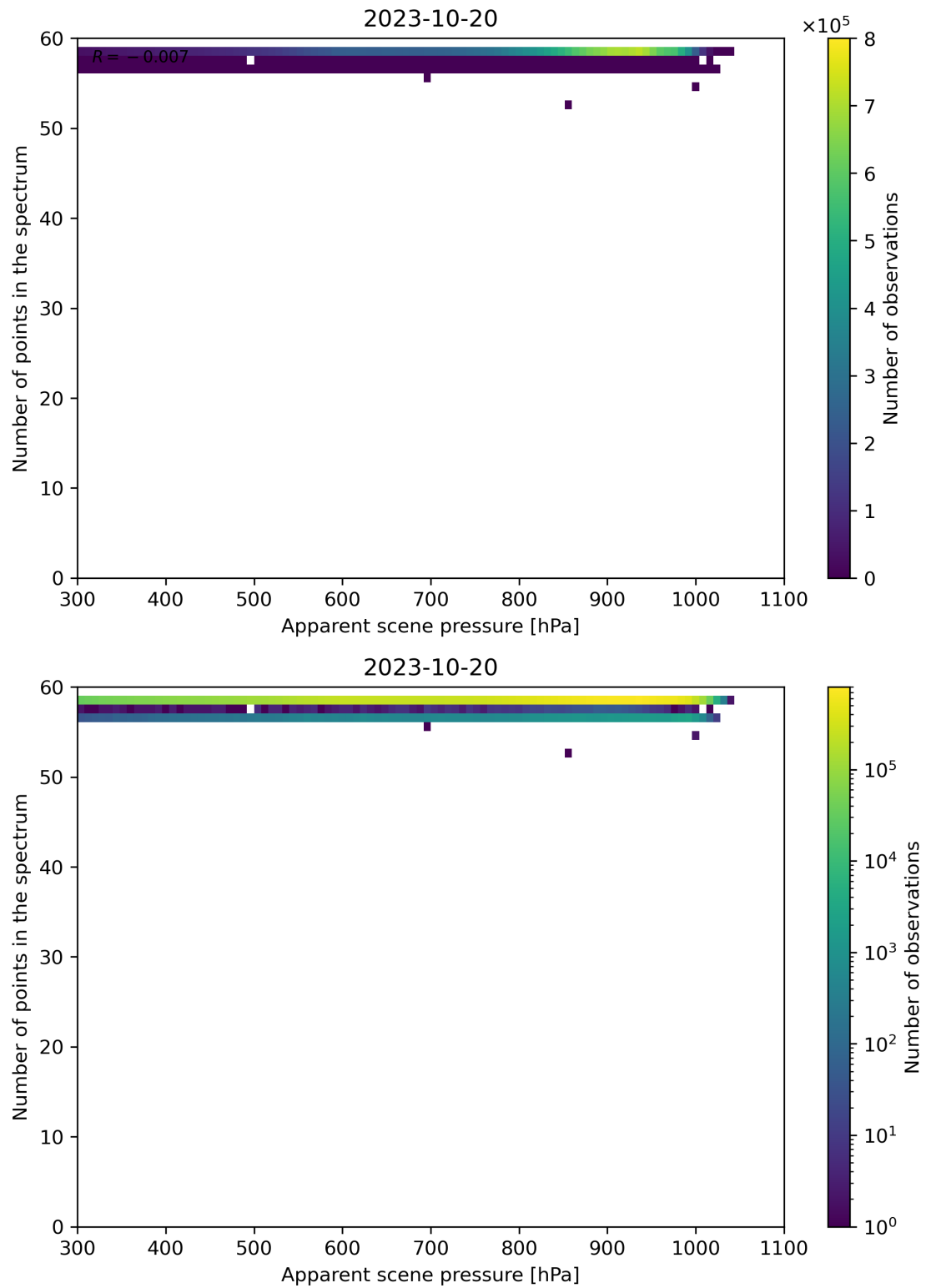
Figure 67: Scatter density plot of “Apparent scene pressure” against “Number of points in the spectrum” for 2023-10-19 to 2023-10-21.
