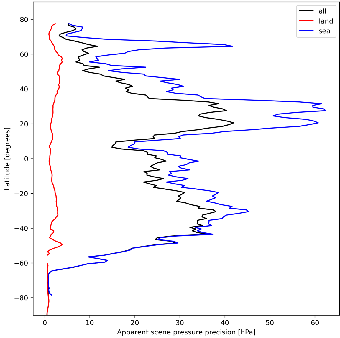
Figure 20: Zonal average of “Apparent scene pressure precision” for 2023-10-19 to 2023-10-21.
