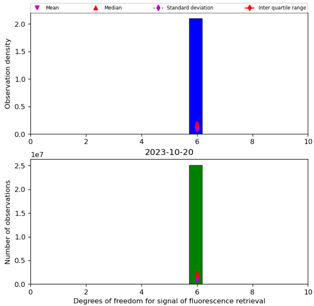
Figure 43: Histogram of “Degrees of freedom for signal of fluorescence retrieval” for 2023-10-19 to 2023-10-21
