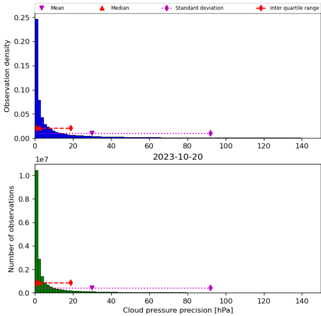
Figure 31: Histogram of “Cloud pressure precision” for 2023-10-19 to 2023-10-21
