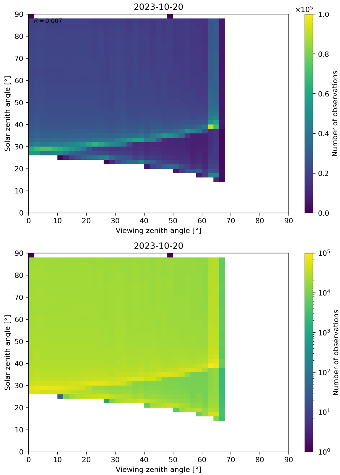
Figure 139: Scatter density plot of “Viewing zenith angle” against “Solar zenith angle” for 2023-10-19 to 2023-10-21.
