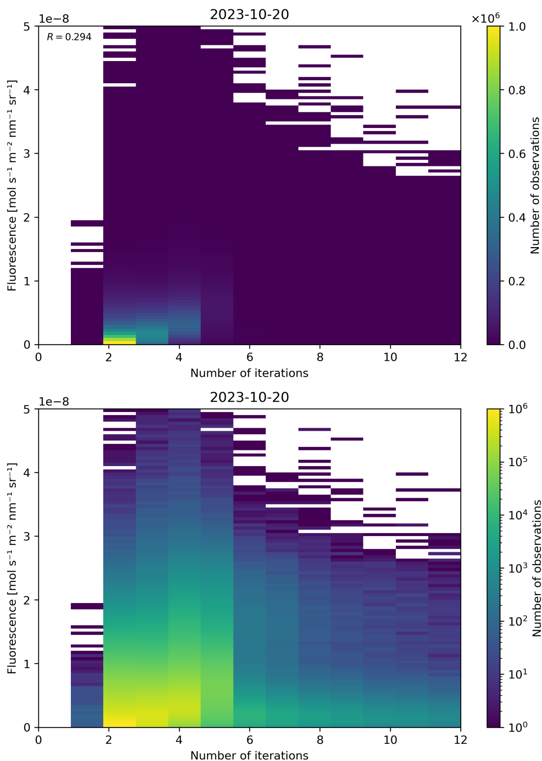
Figure 107: Scatter density plot of “Number of iterations” against “Fluorescence” for 2023-10-19 to 2023-10-21.
