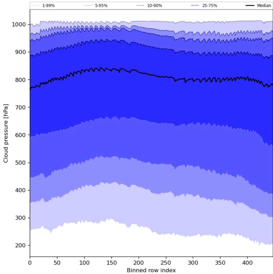
Figure 47: Along track statistics of “Cloud pressure” for 2023-10-19 to 2023-10-21
