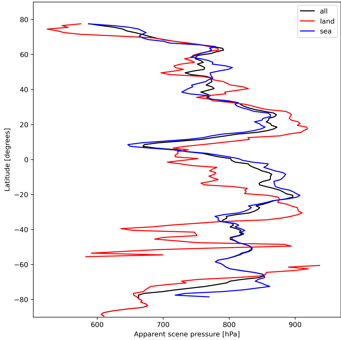
Figure 19: Zonal average of “Apparent scene pressure” for 2023-10-19 to 2023-10-21.
