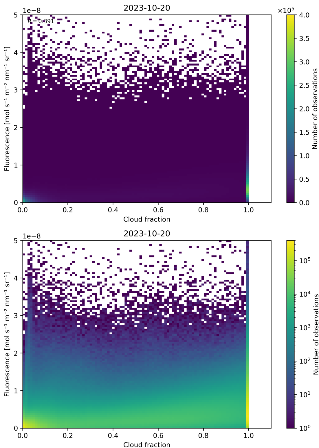
Figure 79: Scatter density plot of “Cloud fraction” against “Fluorescence” for 2023-10-19 to 2023-10-21.
