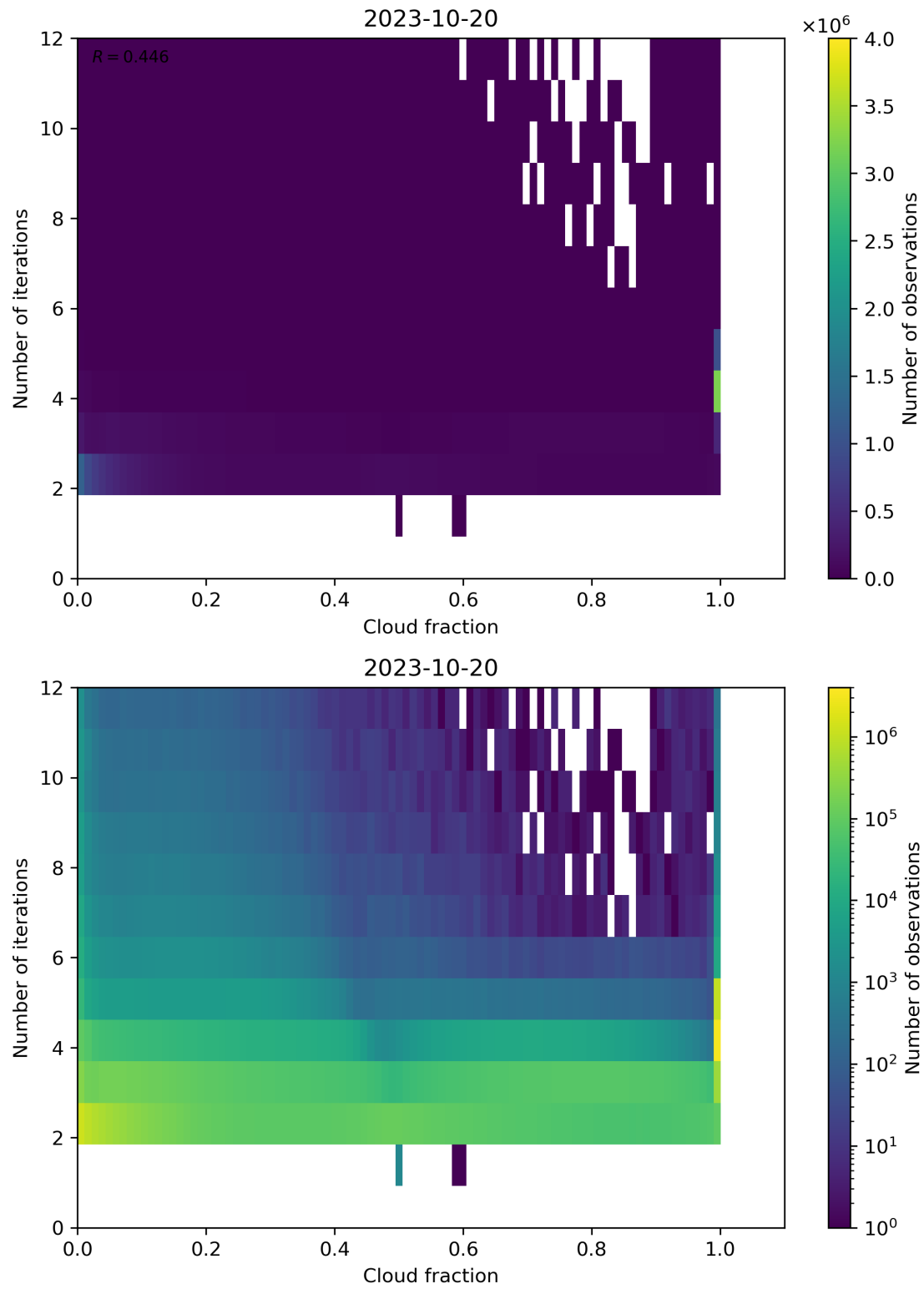
Figure 80: Scatter density plot of “Cloud fraction” against “Number of iterations” for 2023-10-19 to 2023-10-21.
