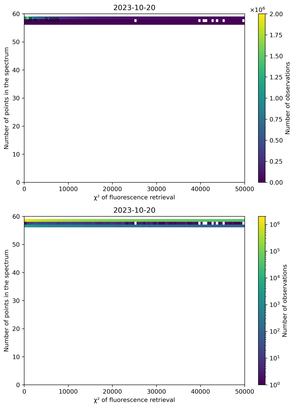
Figure 71: Scatter density plot of " \chi^2 of fluorescence retrieval" against "Number of points in the spectrum" for 2023-10-19 to 2023-10-21.
