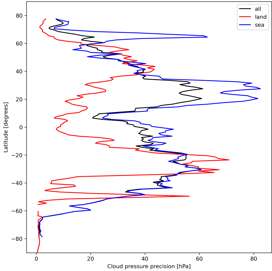
Figure 14: Zonal average of "Cloud pressure precision" for 2023-10-19 to 2023-10-21.
