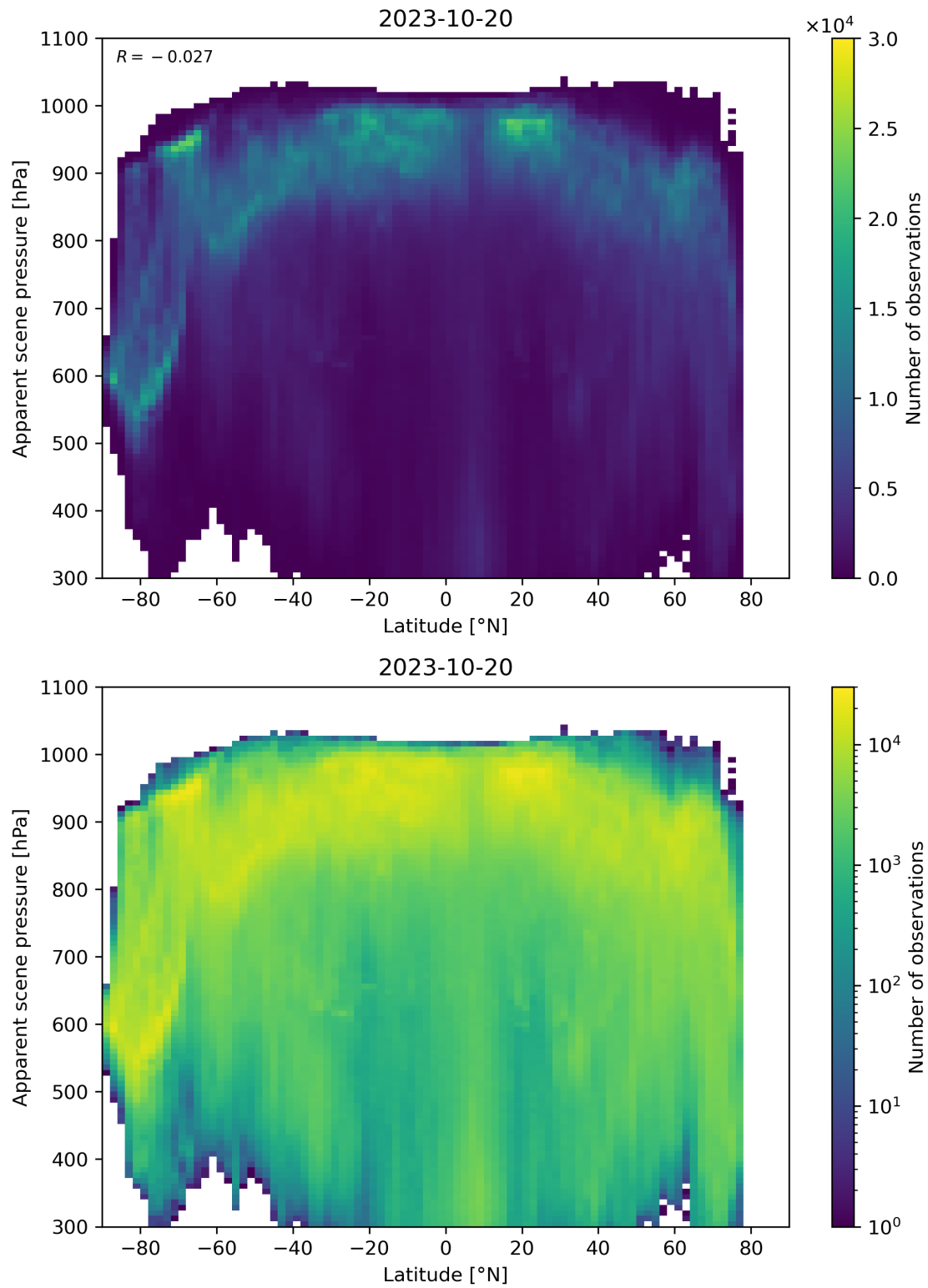
Figure 96: Scatter density plot of “Latitude” against “Apparent scene pressure” for 2023-10-19 to 2023-10-21.
