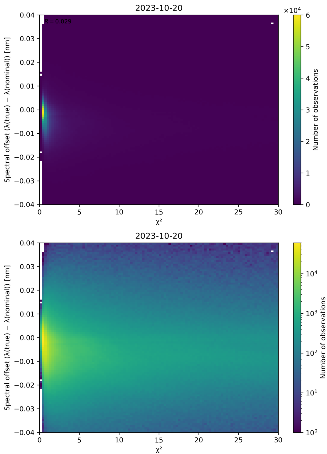
Figure 75: Scatter density plot of “ \chi^2 ” against “Spectral offset ( \lambda(\text{true}) - \lambda(\text{nominal}) )” for 2023-10-19 to 2023-10-21.
