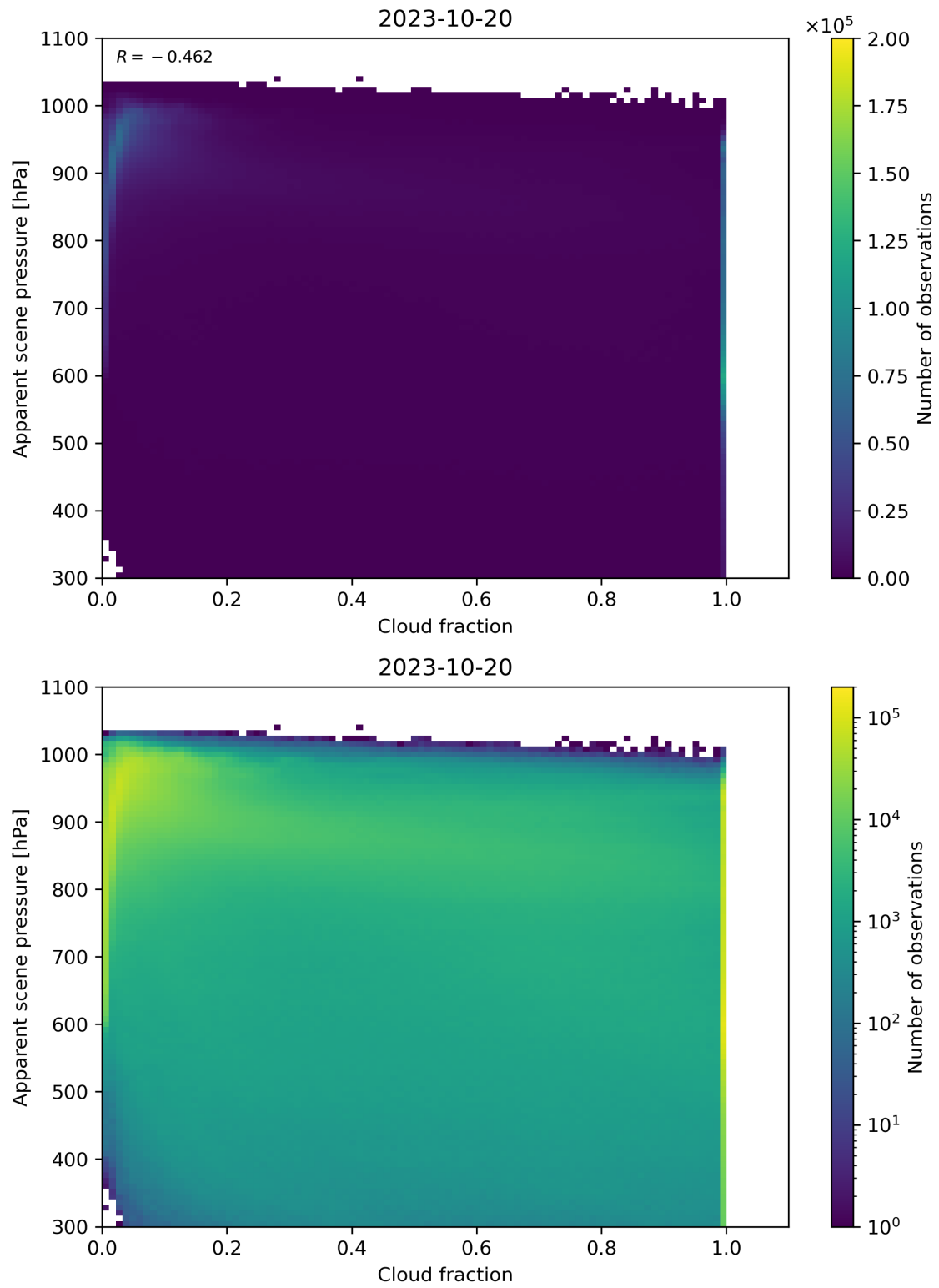
Figure 76: Scatter density plot of “Cloud fraction” against “Apparent scene pressure” for 2023-10-19 to 2023-10-21.
