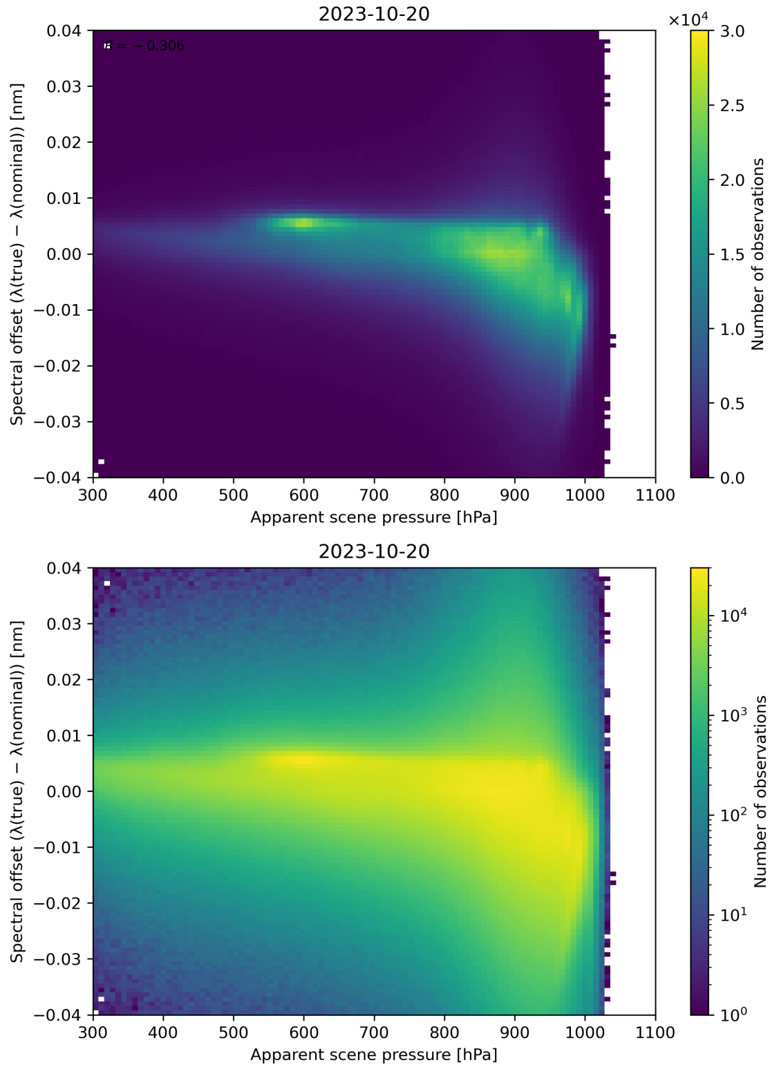
Figure 68: Scatter density plot of “Apparent scene pressure” against “Spectral offset ( \lambda(\text{true}) - \lambda(\text{nominal}) )” for 2023-10-19 to 2023-10-21.
