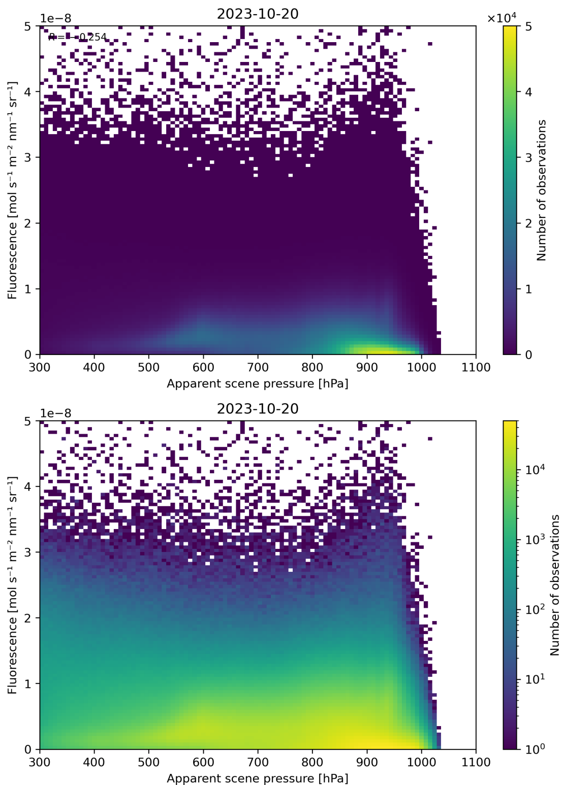
Figure 65: Scatter density plot of “Apparent scene pressure” against “Fluorescence” for 2023-10-19 to 2023-10-21.
