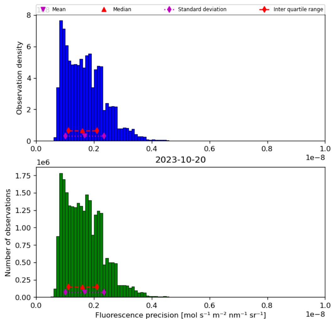
Figure 41: Histogram of “Fluorescence precision” for 2023-10-19 to 2023-10-21
