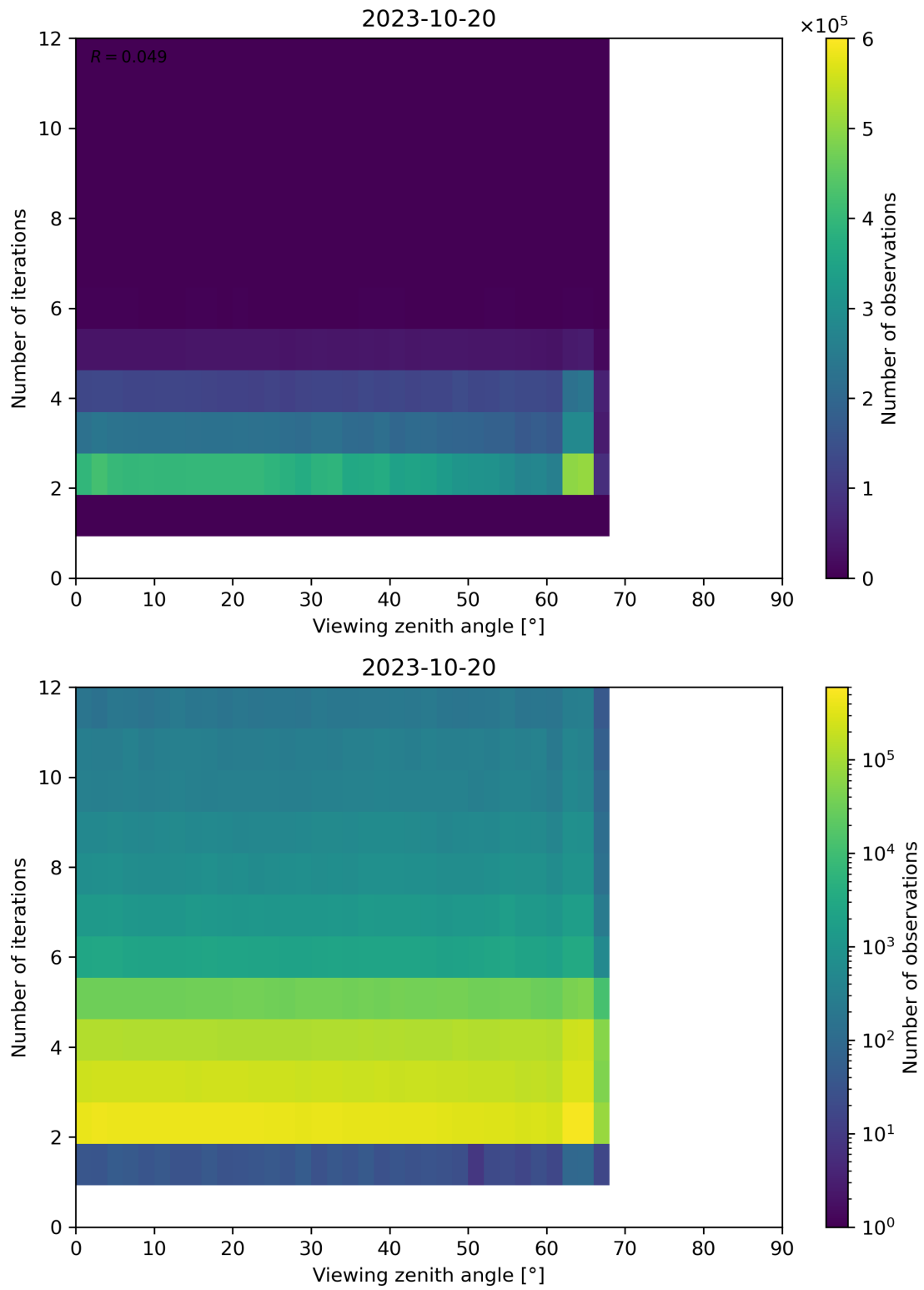
Figure 136: Scatter density plot of “Viewing zenith angle” against “Number of iterations” for 2023-10-19 to 2023-10-21.
