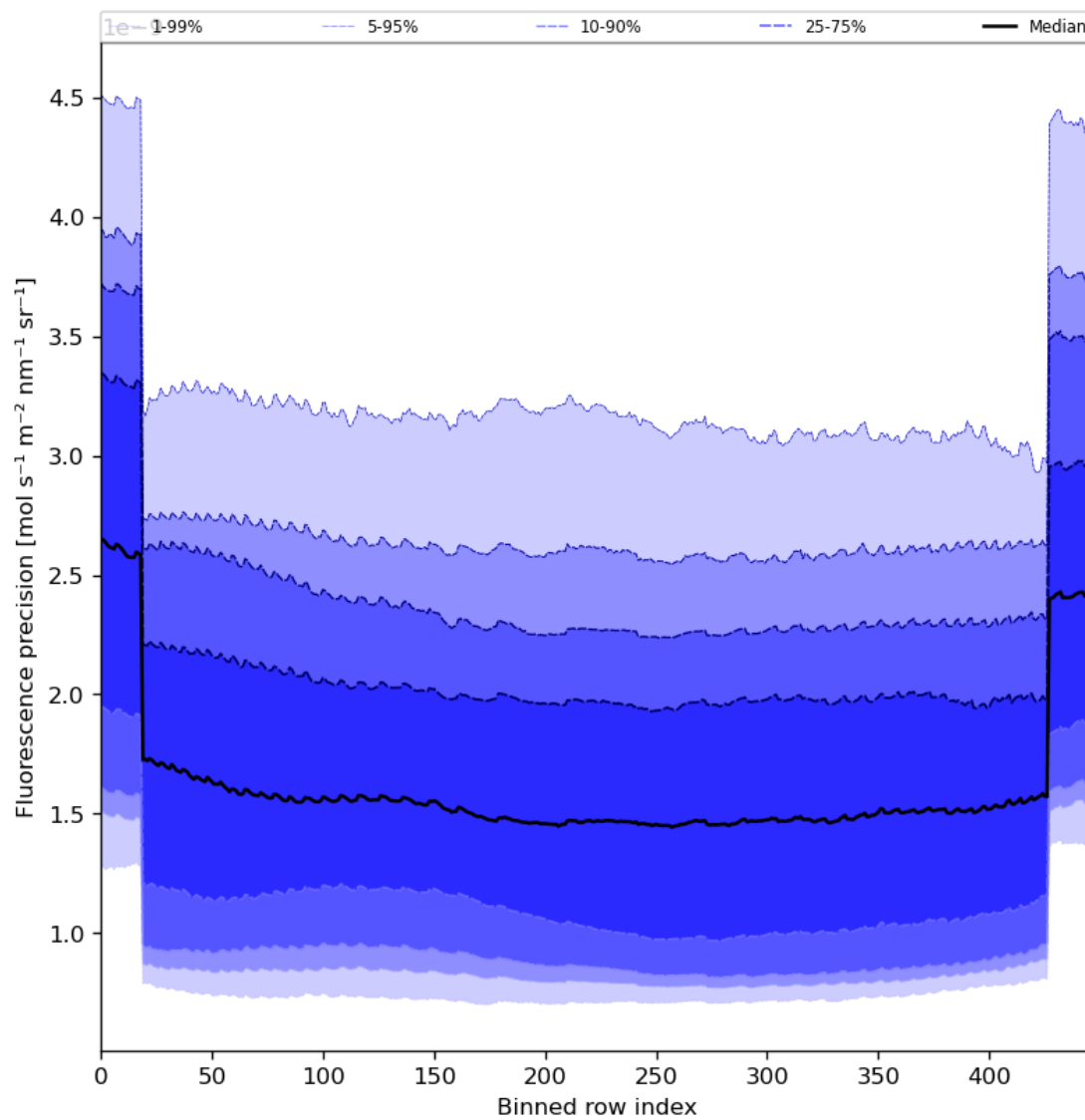
Figure 58: Along track statistics of “Fluorescence precision” for 2023-10-19 to 2023-10-21
