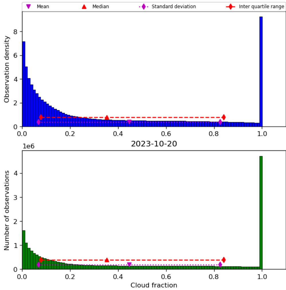
Figure 32: Histogram of “Cloud fraction” for 2023-10-19 to 2023-10-21
