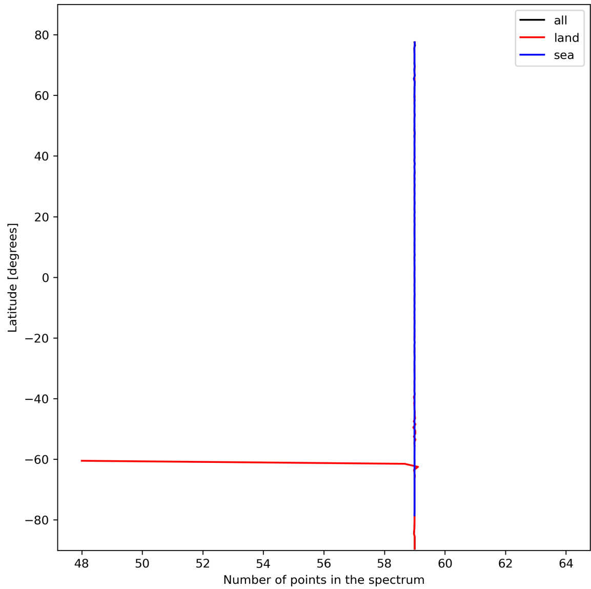
Figure 27: Zonal average of “Number of points in the spectrum” for 2023-10-19 to 2023-10-21.
