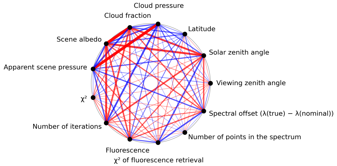
Figure 1: Map of correlation graph for 2023-10-19 to 2023-10-21.
