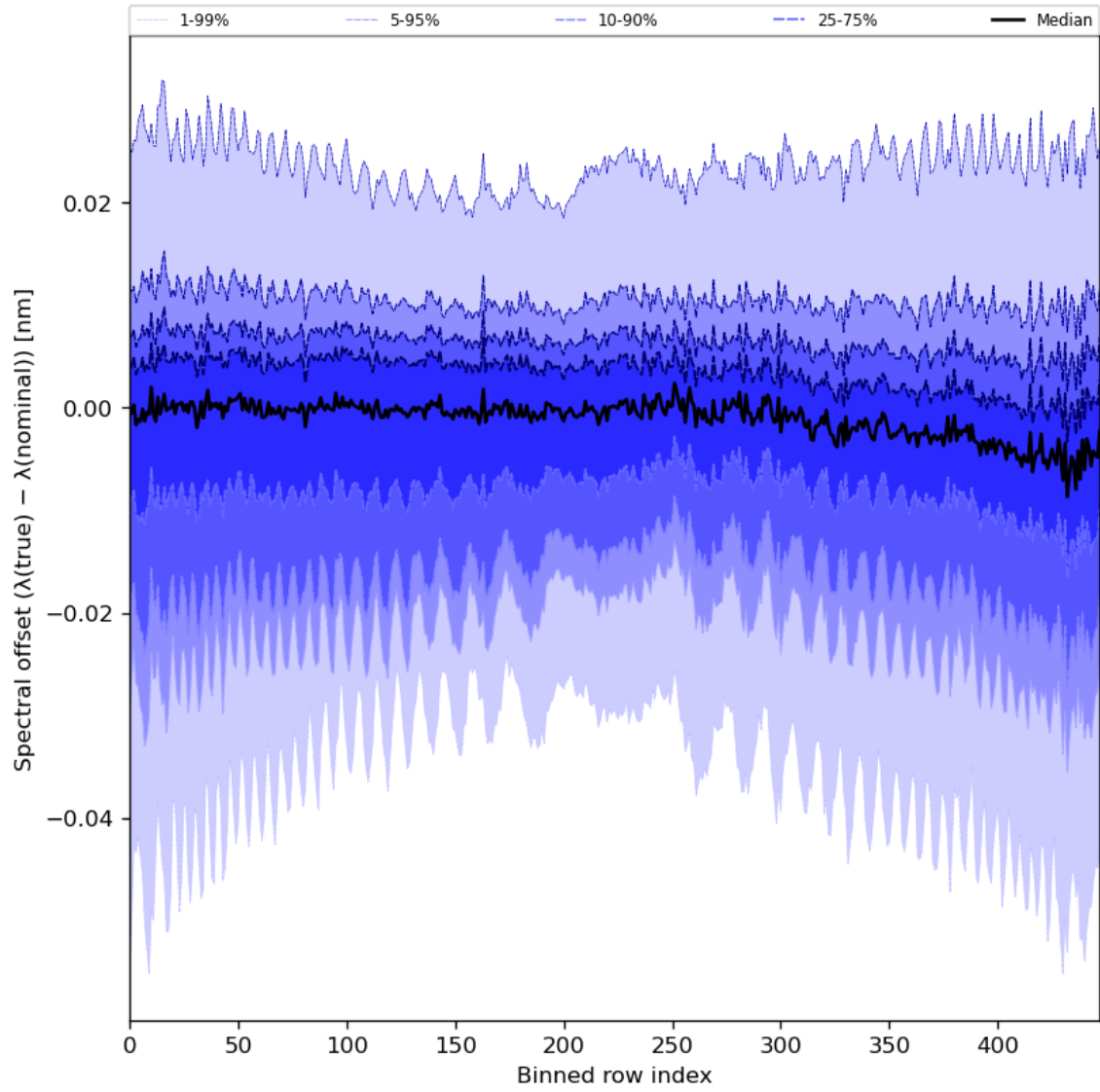
Figure 62: Along track statistics of “Spectral offset ( \lambda(\text{true}) - \lambda(\text{nominal}) )” for 2023-10-19 to 2023-10-21
