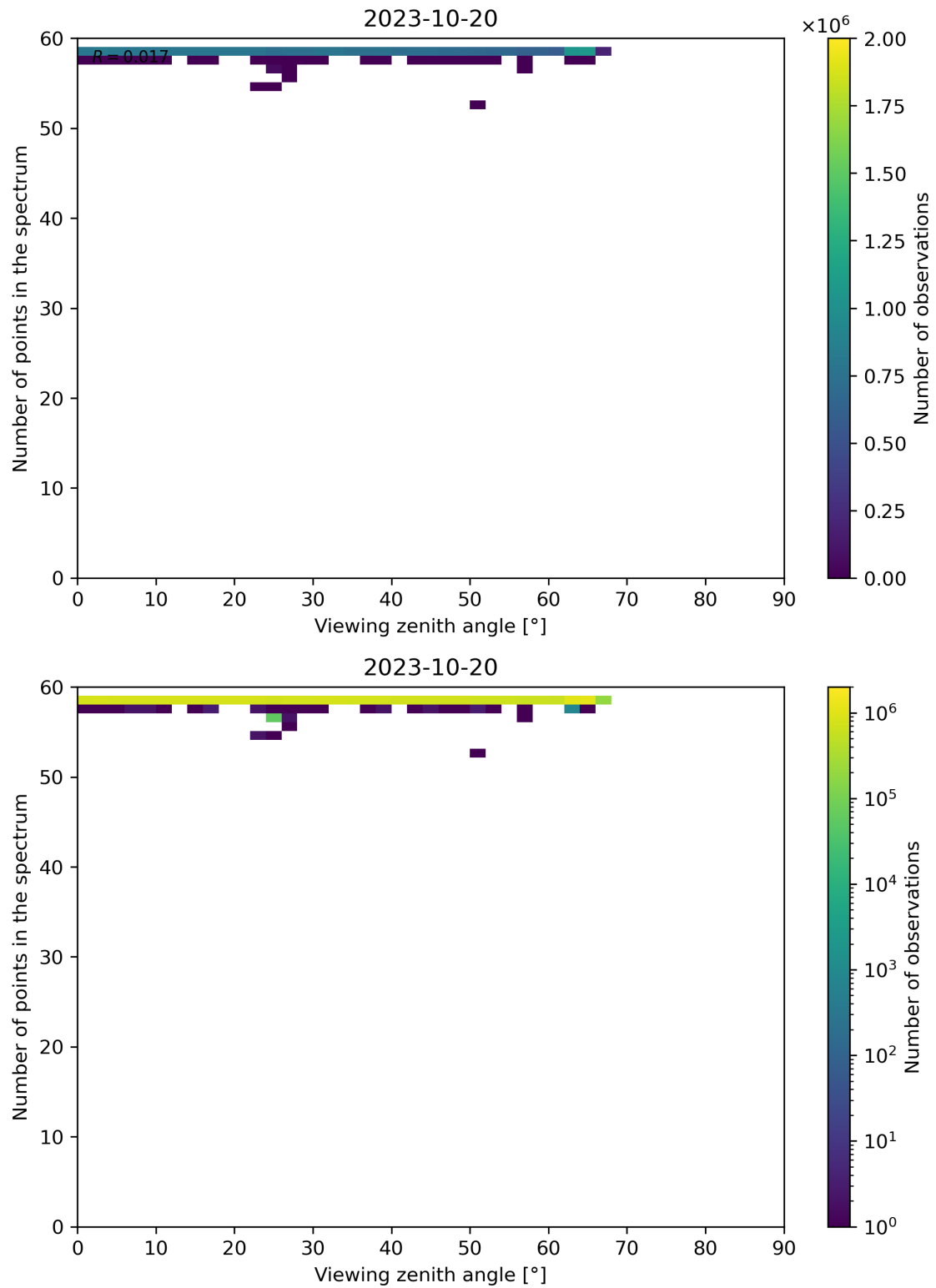
Figure 137: Scatter density plot of “Viewing zenith angle” against “Number of points in the spectrum” for 2023-10-19 to 2023-10-21.
