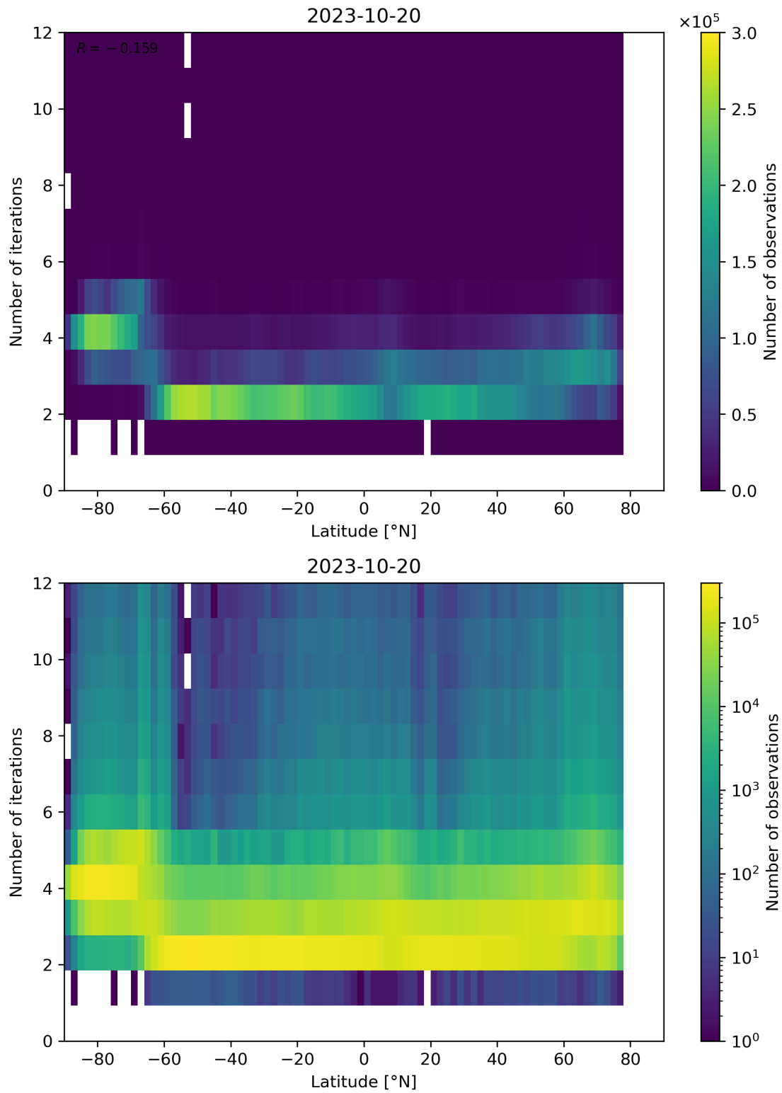
Figure 102: Scatter density plot of “Latitude” against “Number of iterations” for 2023-10-19 to 2023-10-21.
