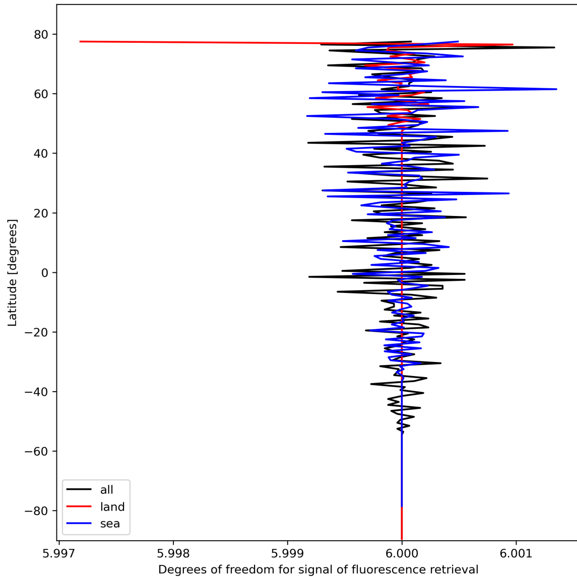
Figure 26: Zonal average of “Degrees of freedom for signal of fluorescence retrieval” for 2023-10-19 to 2023-10-21.
