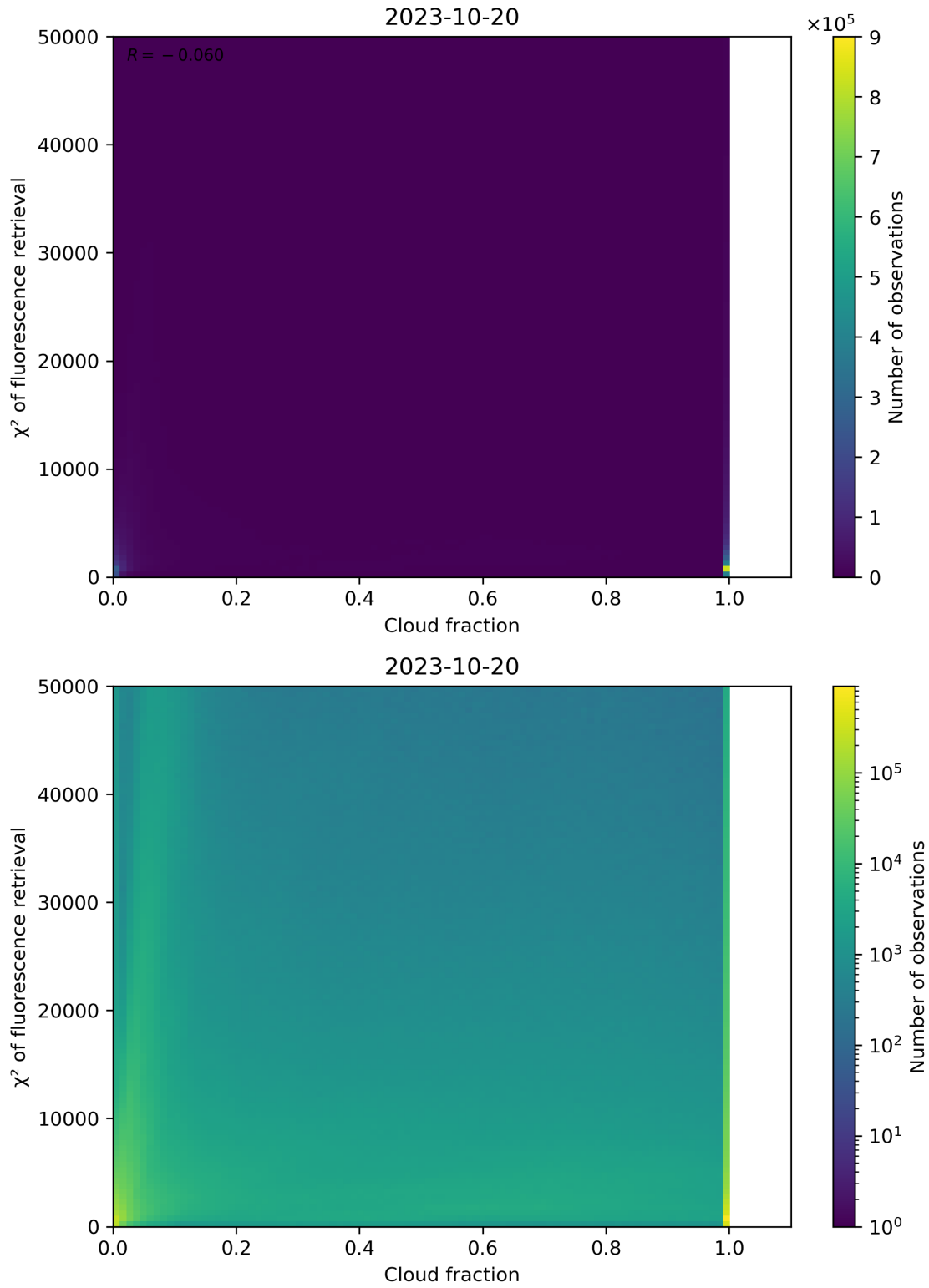
Figure 78: Scatter density plot of “Cloud fraction” against “ \chi^2 of fluorescence retrieval” for 2023-10-19 to 2023-10-21.
