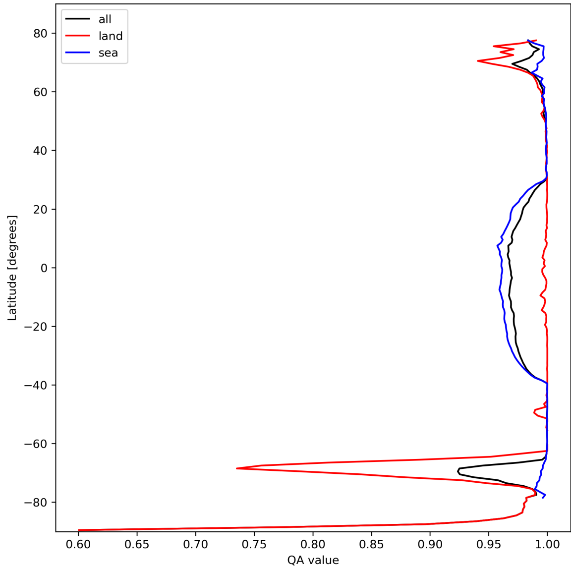
Figure 12: Zonal average of "QA value" for 2023-10-19 to 2023-10-21.
