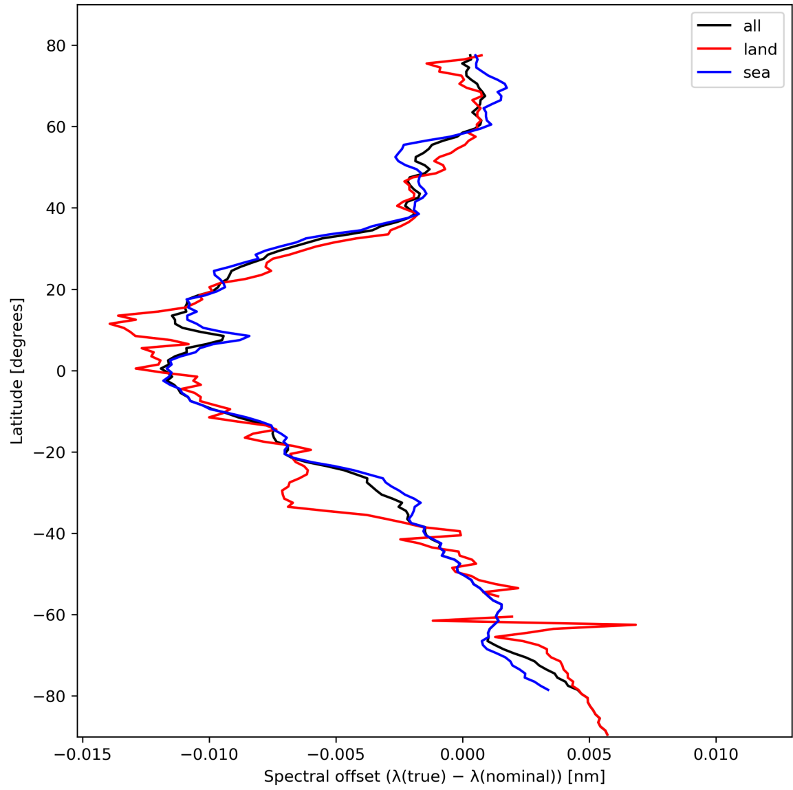
Figure 28: Zonal average of “Spectral offset ( \lambda(\text{true}) - \lambda(\text{nominal}) )” for 2023-10-19 to 2023-10-21.
