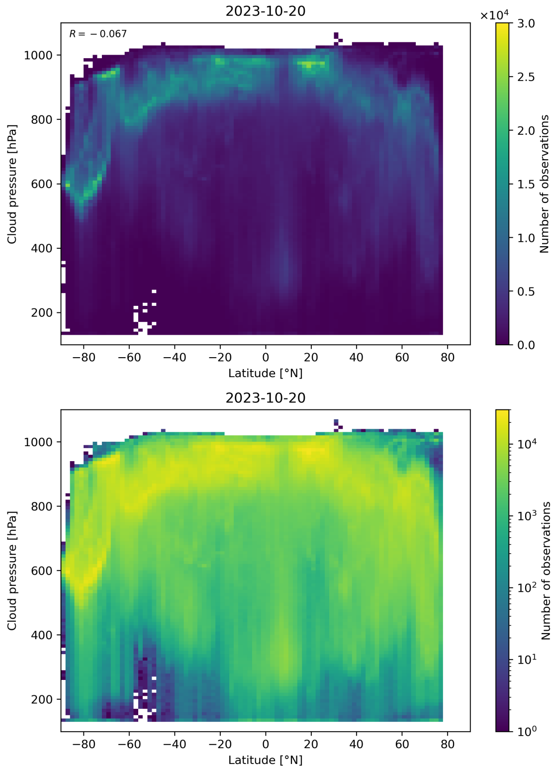
Figure 100: Scatter density plot of “Latitude” against “Cloud pressure” for 2023-10-19 to 2023-10-21.
