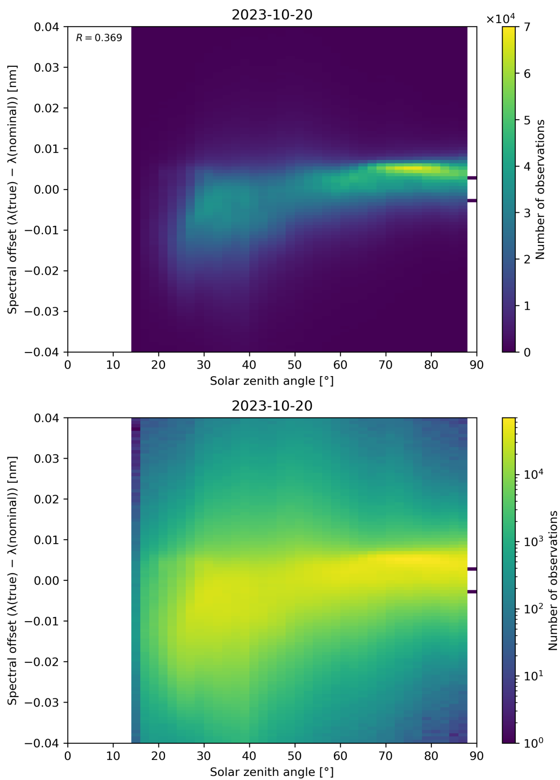
Figure 128: Scatter density plot of “Solar zenith angle” against “Spectral offset ( \lambda(\text{true}) - \lambda(\text{nominal}) )” for 2023-10-19 to 2023-10-21.
