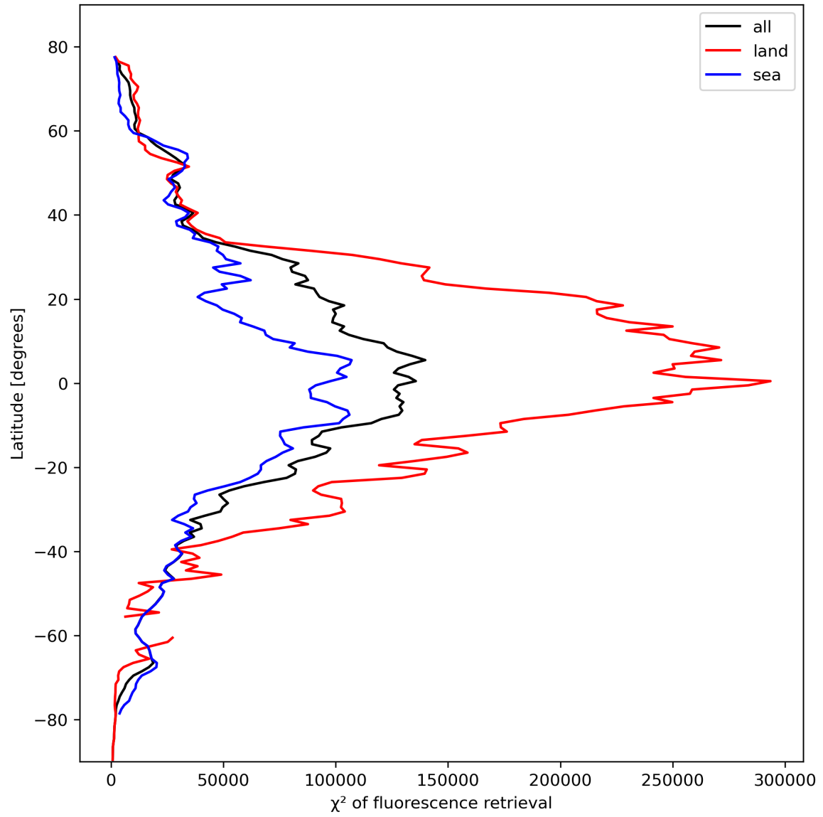
Figure 25: Zonal average of “ \chi^2 of fluorescence retrieval” for 2023-10-19 to 2023-10-21.
