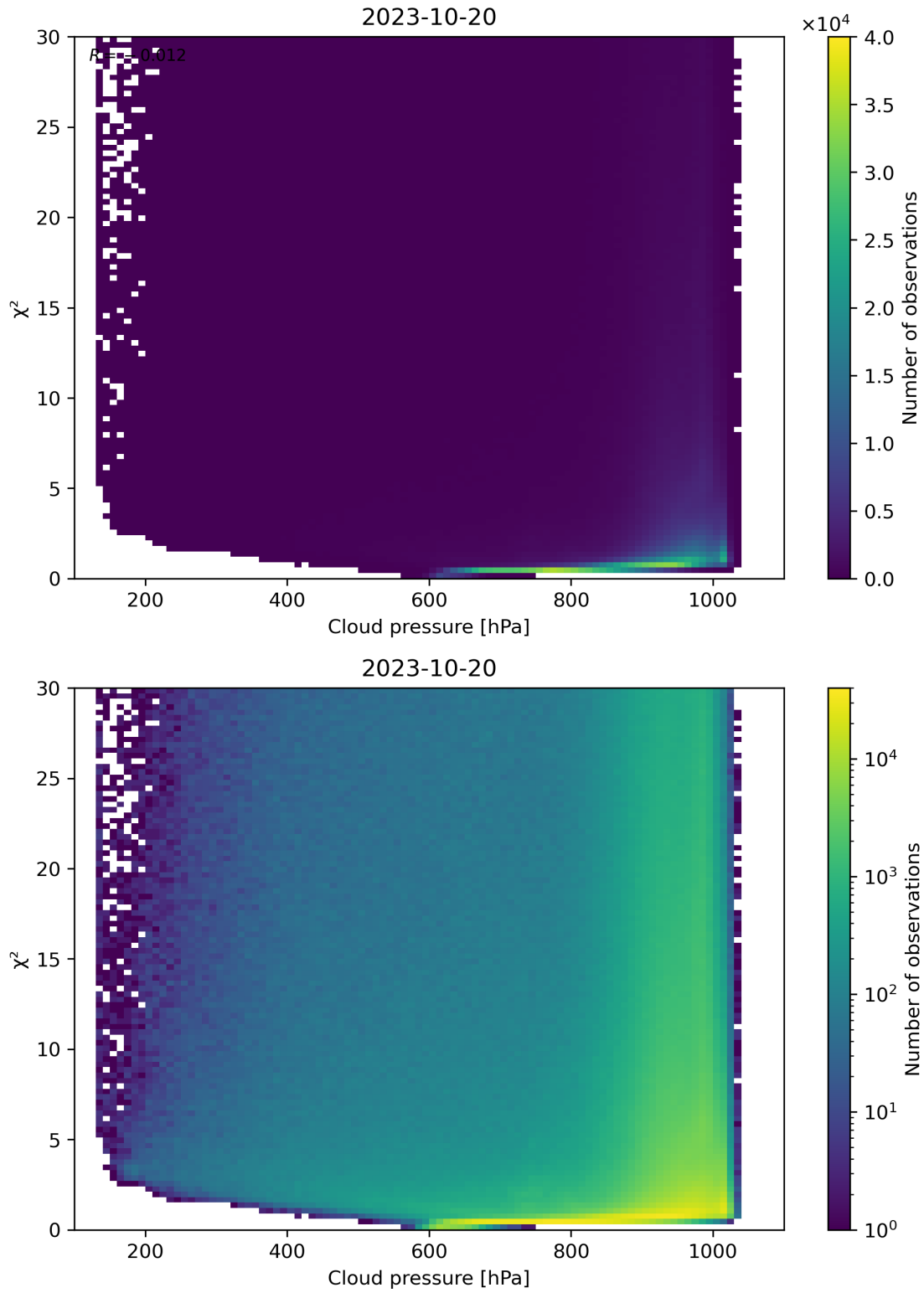
Figure 85: Scatter density plot of “Cloud pressure” against “ \chi^2 ” for 2023-10-19 to 2023-10-21.
