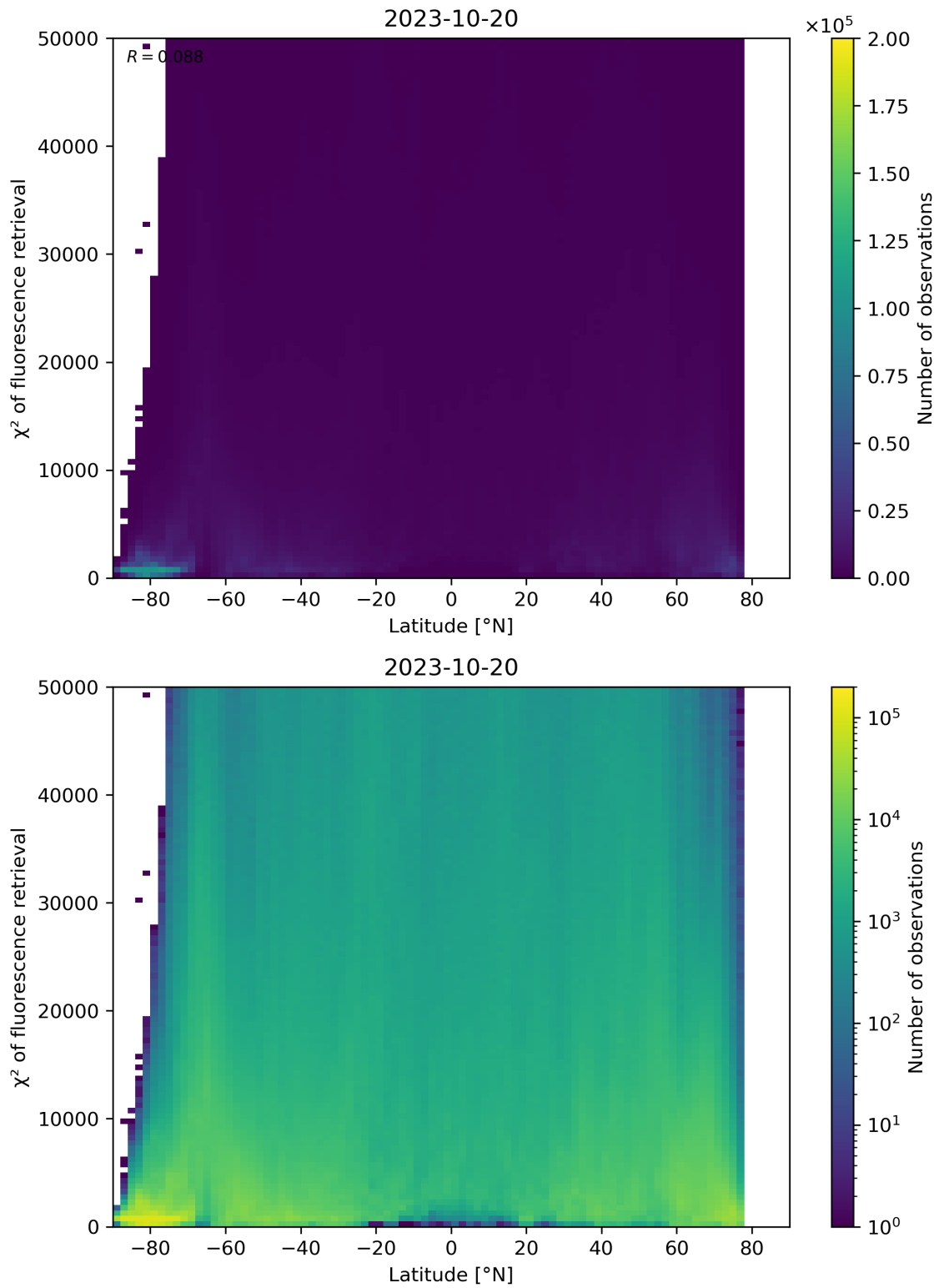
Figure 98: Scatter density plot of “Latitude” against “ \chi^2 of fluorescence retrieval” for 2023-10-19 to 2023-10-21.
