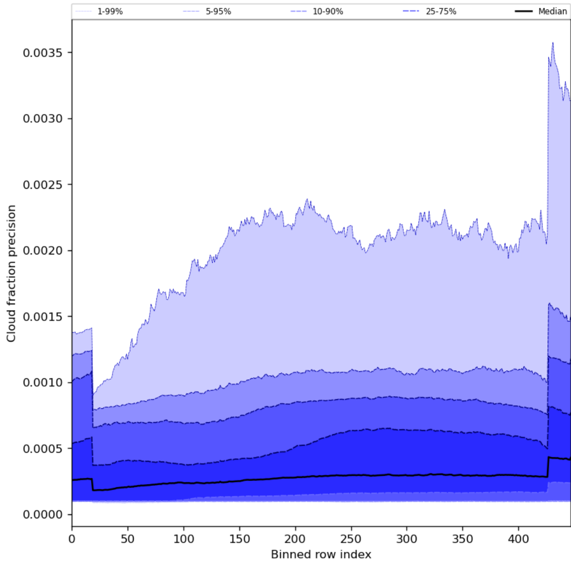
Figure 50: Along track statistics of “Cloud fraction precision” for 2023-10-19 to 2023-10-21
