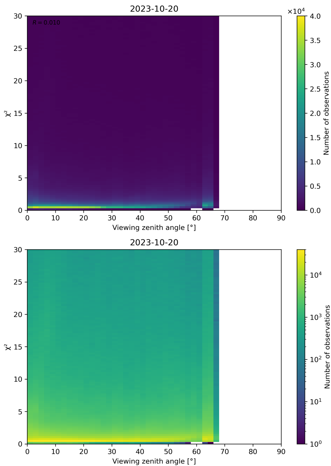
Figure 130: Scatter density plot of “Viewing zenith angle” against “ \chi^2 ” for 2023-10-19 to 2023-10-21.
