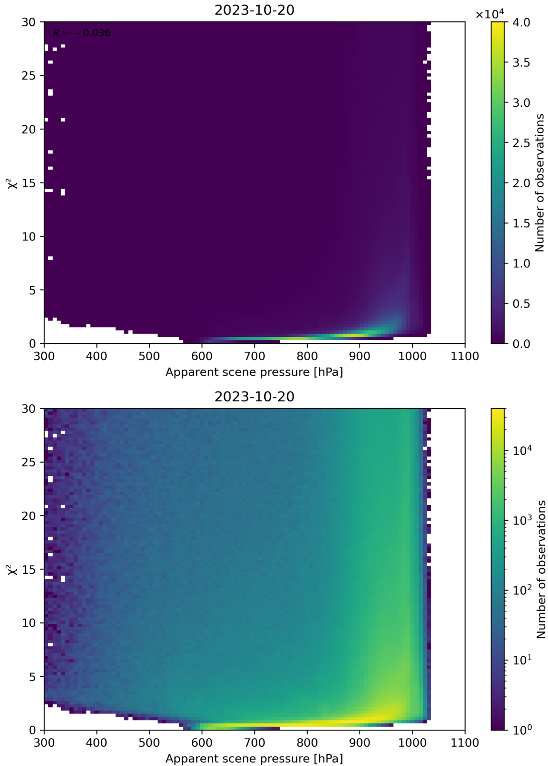
Figure 63: Scatter density plot of “Apparent scene pressure” against “ \chi^2 ” for 2023-10-19 to 2023-10-21.
