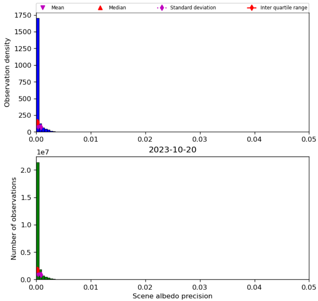
Figure 35: Histogram of “Scene albedo precision” for 2023-10-19 to 2023-10-21
