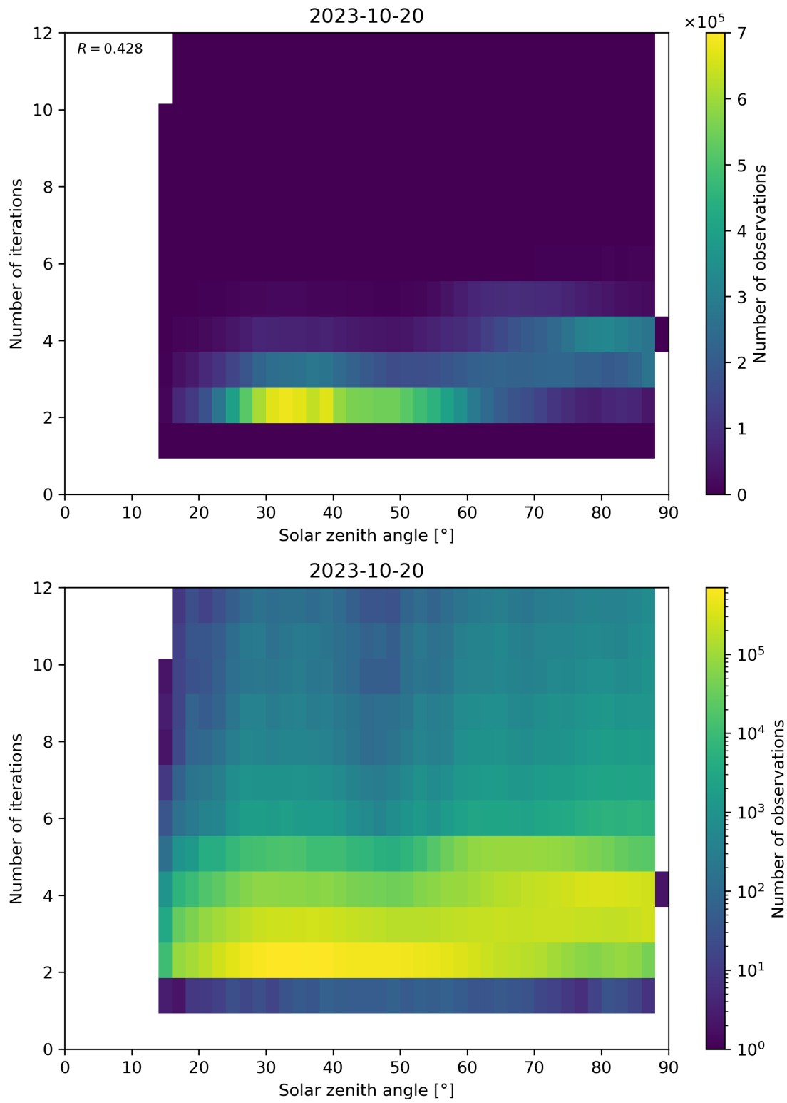
Figure 125: Scatter density plot of “Solar zenith angle” against “Number of iterations” for 2023-10-19 to 2023-10-21.
