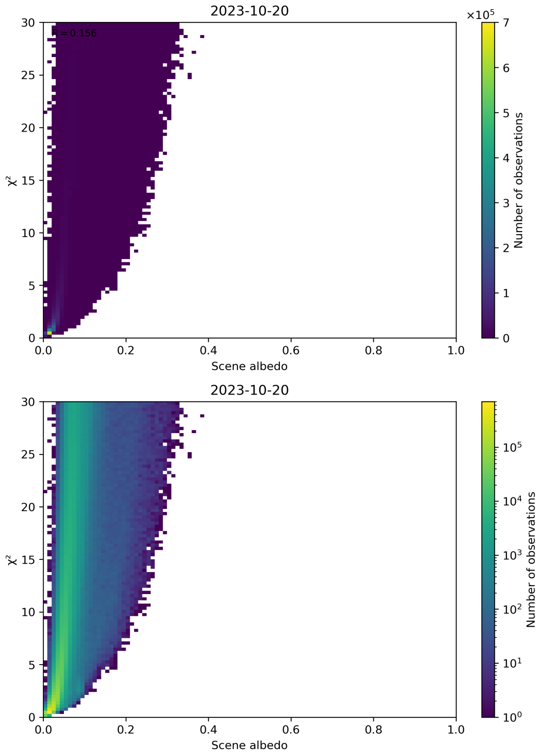
Figure 112: Scatter density plot of “Scene albedo” against “ \chi^2 ” for 2023-10-19 to 2023-10-21.
