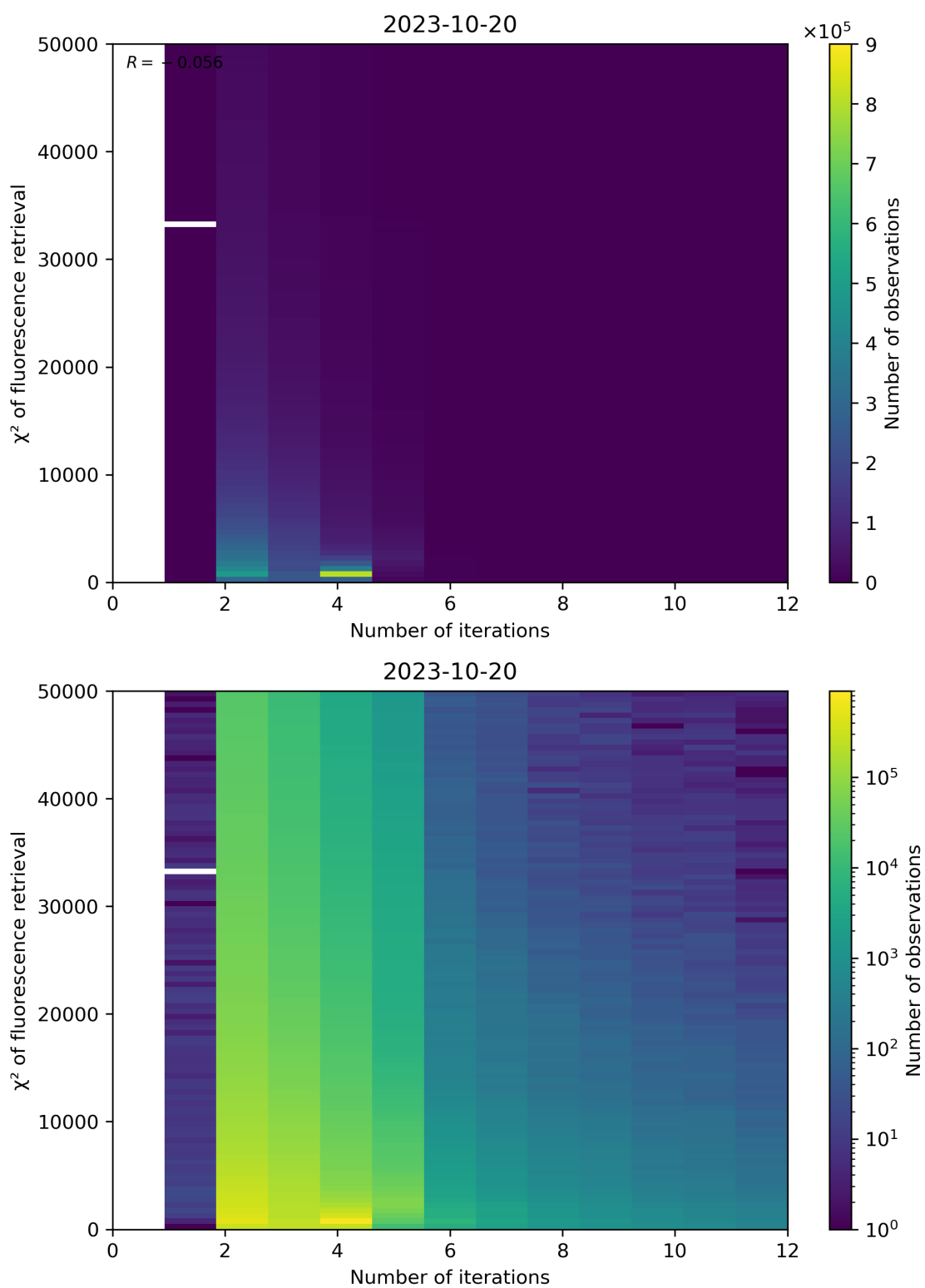
Figure 106: Scatter density plot of “Number of iterations” against “ \chi^2 of fluorescence retrieval” for 2023-10-19 to 2023-10-21.
