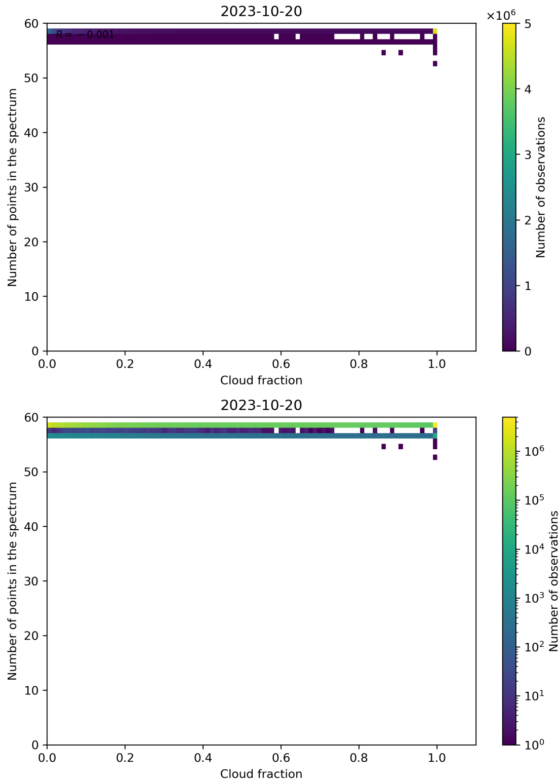
Figure 81: Scatter density plot of “Cloud fraction” against “Number of points in the spectrum” for 2023-10-19 to 2023-10-21.
