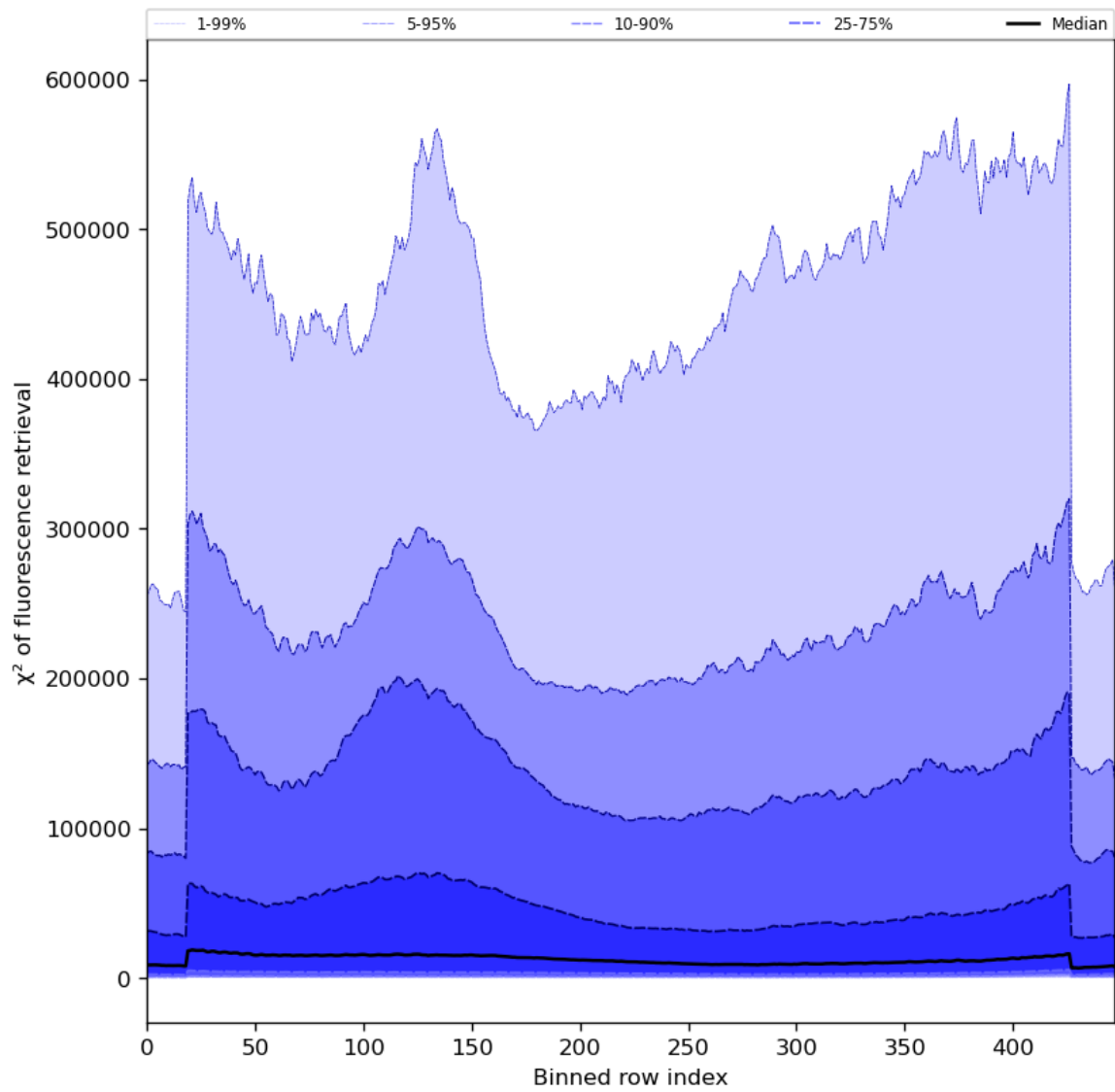
Figure 59: Along track statistics of “ \chi^2 of fluorescence retrieval” for 2023-10-19 to 2023-10-21
