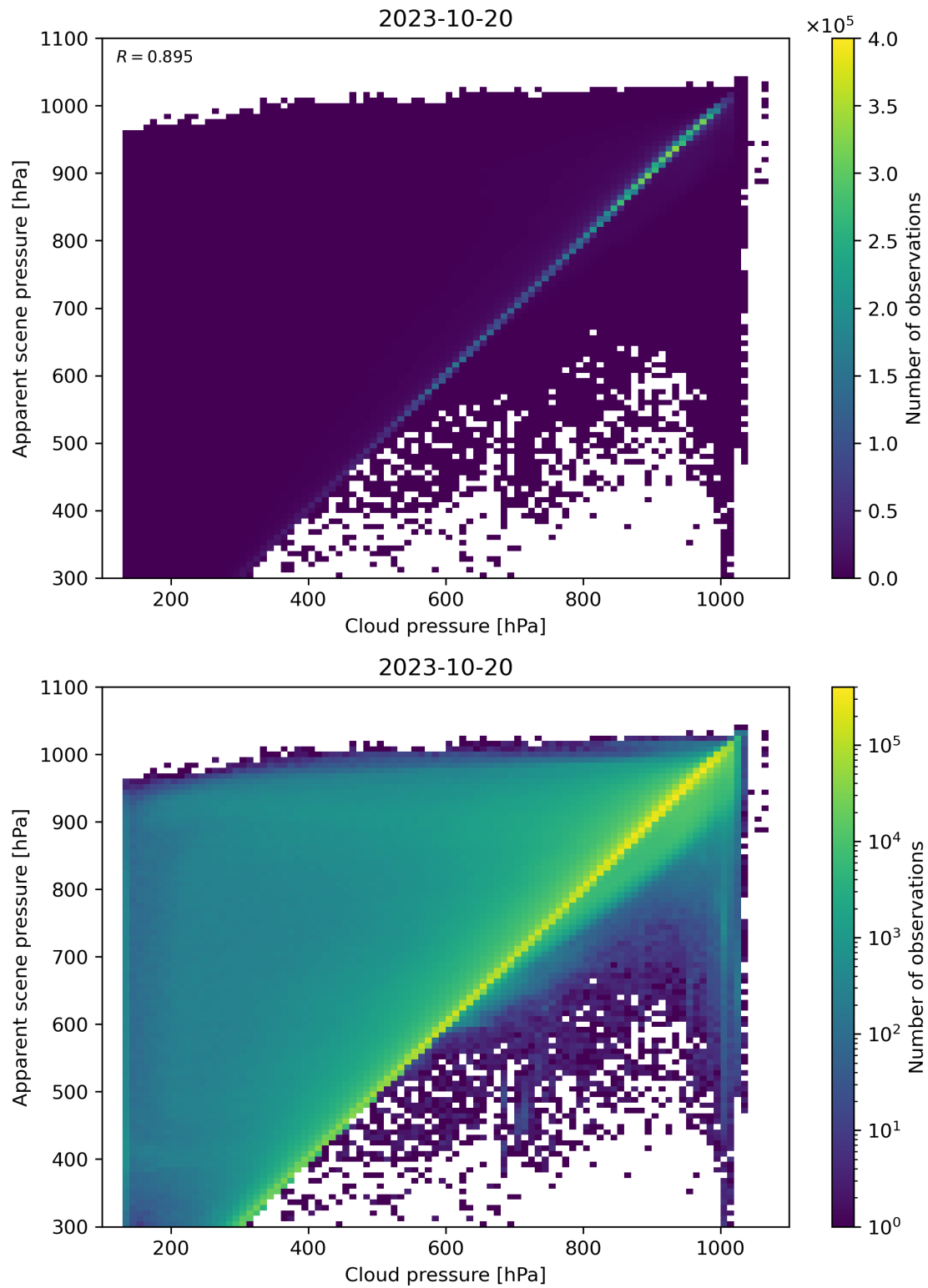
Figure 84: Scatter density plot of “Cloud pressure” against “Apparent scene pressure” for 2023-10-19 to 2023-10-21.
