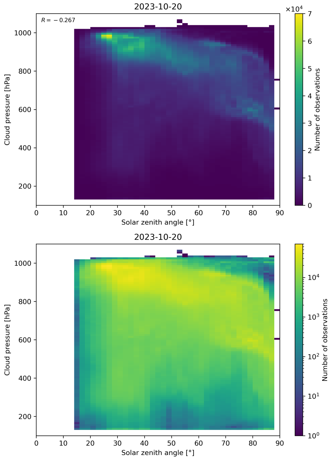
Figure 122: Scatter density plot of “Solar zenith angle” against “Cloud pressure” for 2023-10-19 to 2023-10-21.
