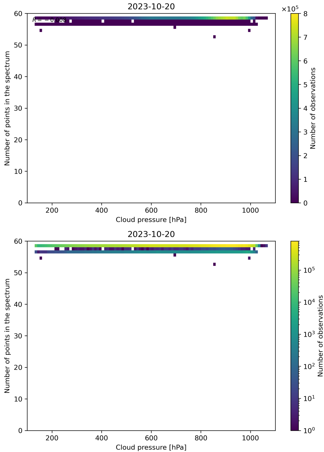
Figure 90: Scatter density plot of “Cloud pressure” against “Number of points in the spectrum” for 2023-10-19 to 2023-10-21.
