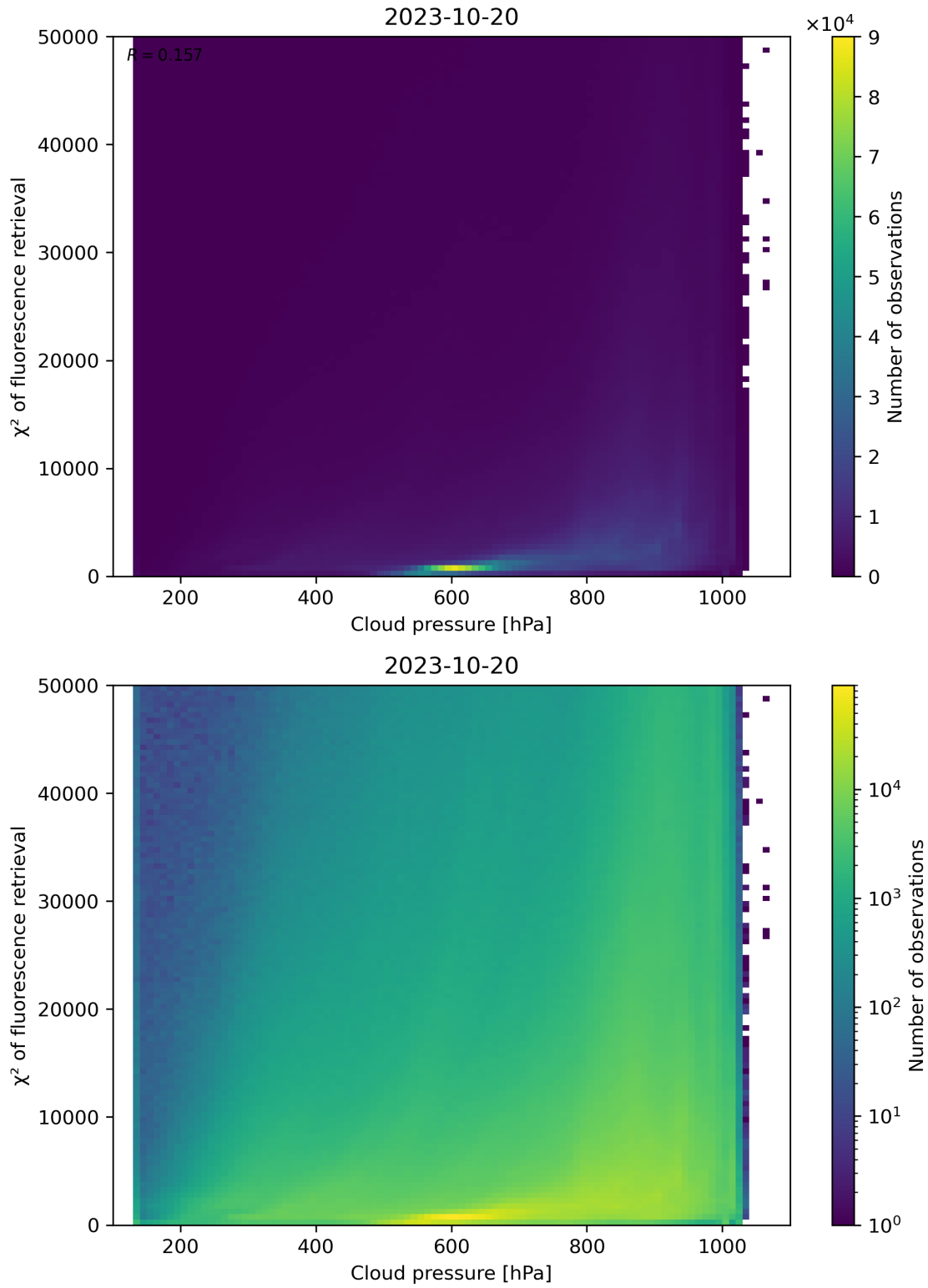
Figure 86: Scatter density plot of “Cloud pressure” against “ \chi^2 of fluorescence retrieval” for 2023-10-19 to 2023-10-21.
