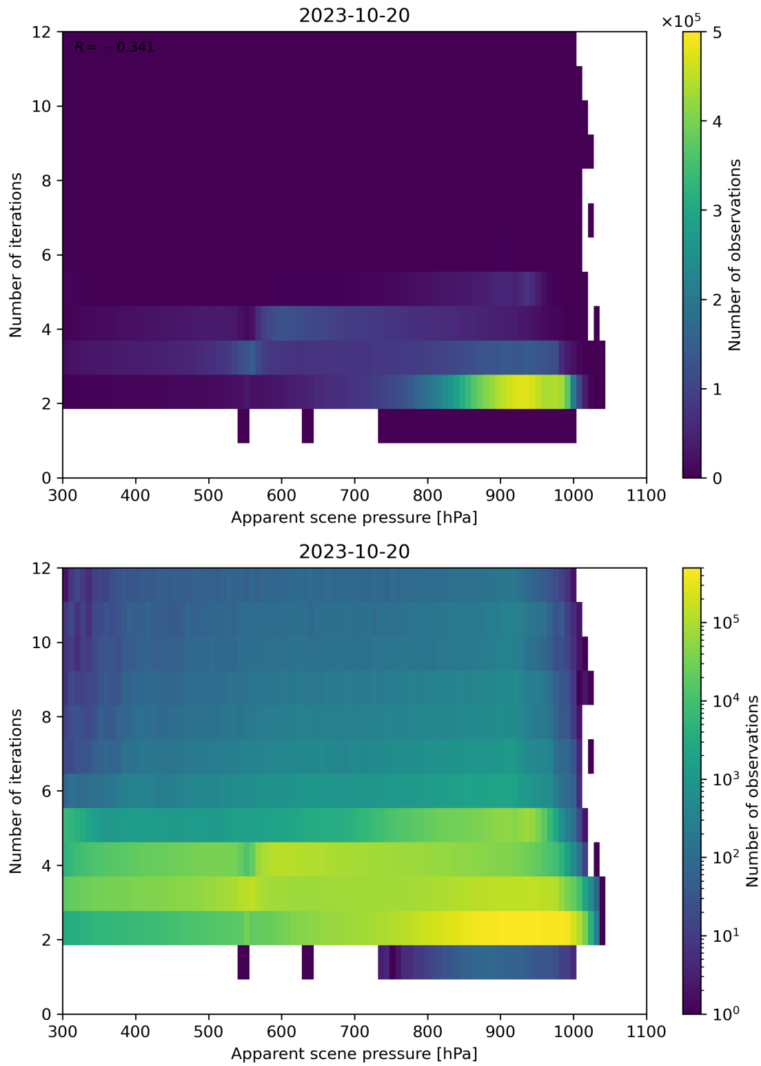
Figure 66: Scatter density plot of “Apparent scene pressure” against “Number of iterations” for 2023-10-19 to 2023-10-21.
