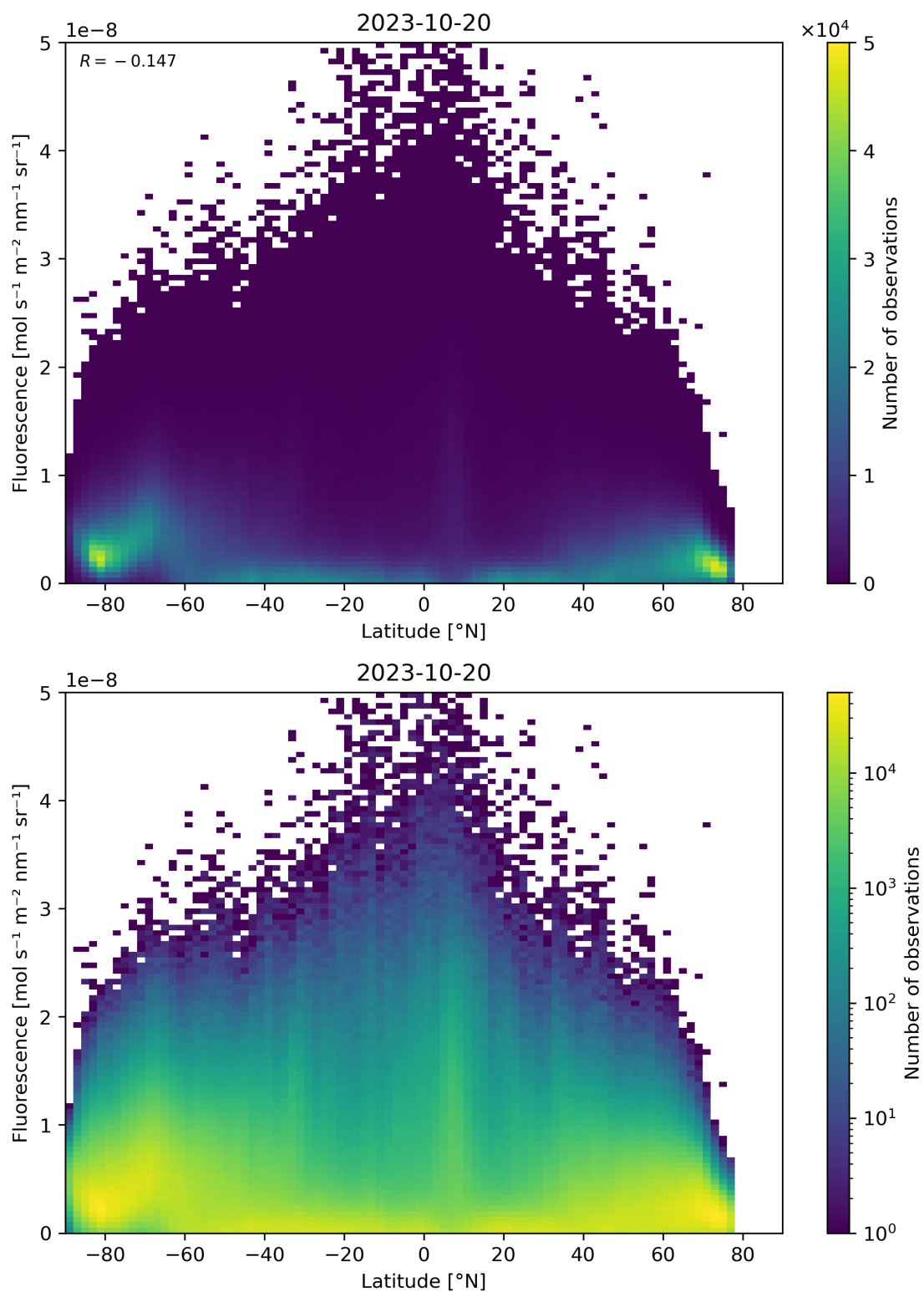
Figure 101: Scatter density plot of “Latitude” against “Fluorescence” for 2023-10-19 to 2023-10-21.
