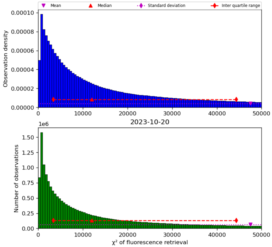
Figure 42: Histogram of “ \chi^2 of fluorescence retrieval” for 2023-10-19 to 2023-10-21
