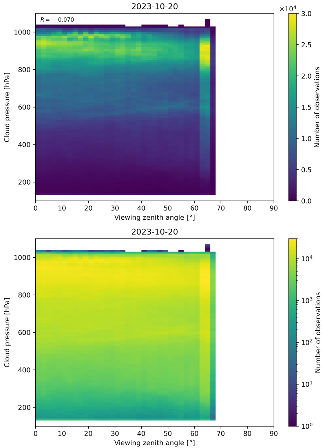
Figure 133: Scatter density plot of “Viewing zenith angle” against “Cloud pressure” for 2023-10-19 to 2023-10-21.
