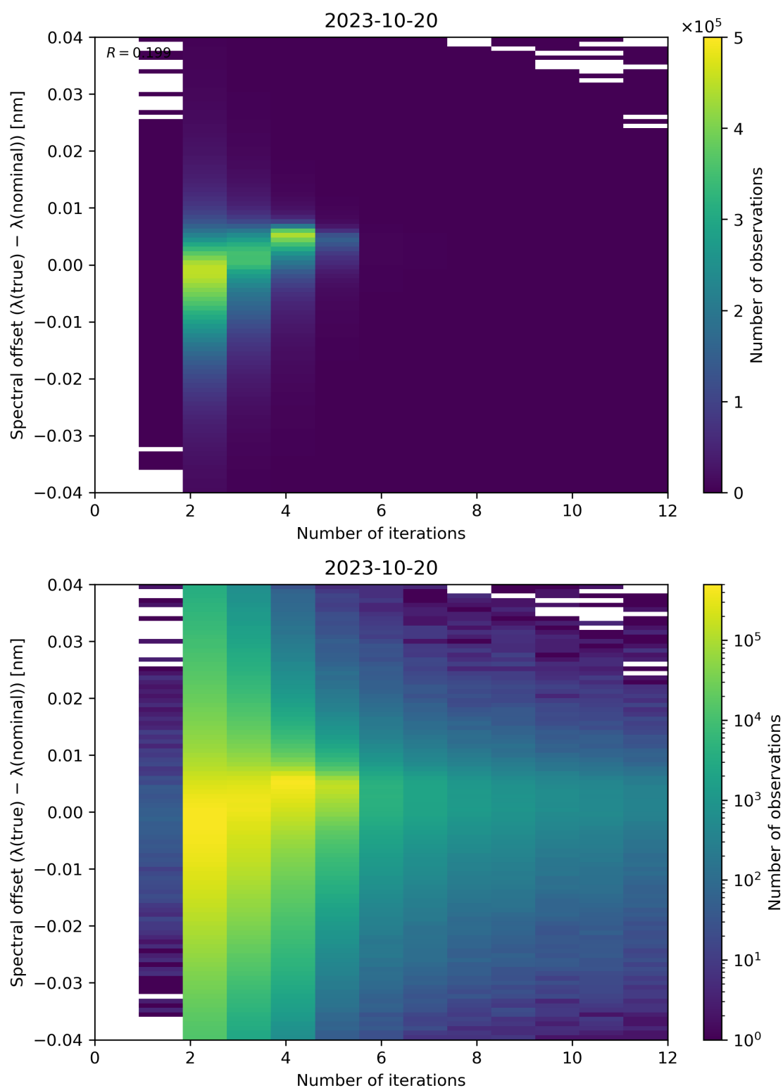
Figure 109: Scatter density plot of “Number of iterations” against “Spectral offset ( \lambda(\text{true}) - \lambda(\text{nominal}) )” for 2023-10-19 to 2023-10-21.
