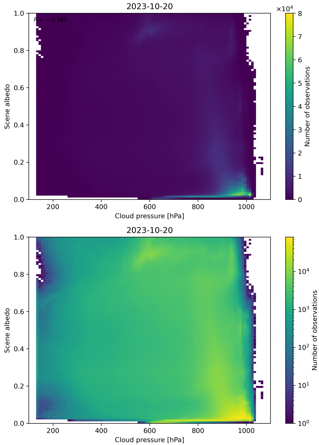
Figure 91: Scatter density plot of “Cloud pressure” against “Scene albedo” for 2023-10-19 to 2023-10-21.
