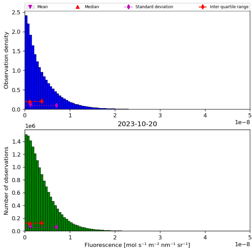
Figure 40: Histogram of “Fluorescence” for 2023-10-19 to 2023-10-21
