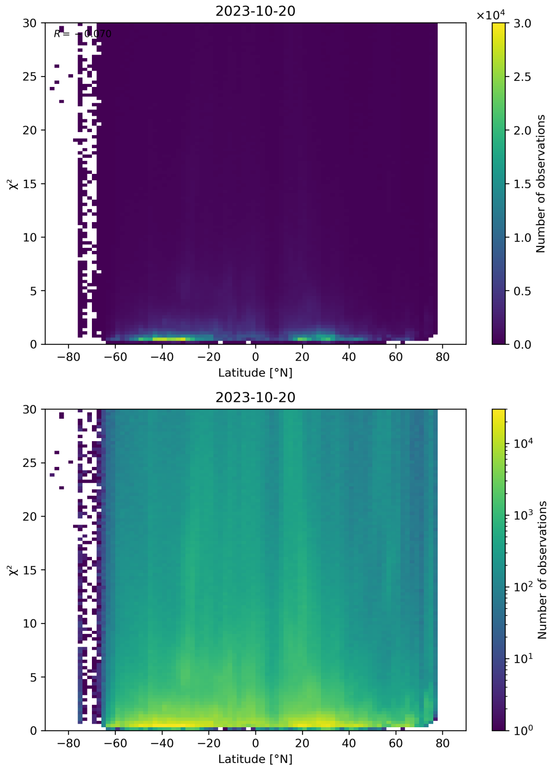
Figure 97: Scatter density plot of “Latitude” against “ \chi^2 ” for 2023-10-19 to 2023-10-21.
