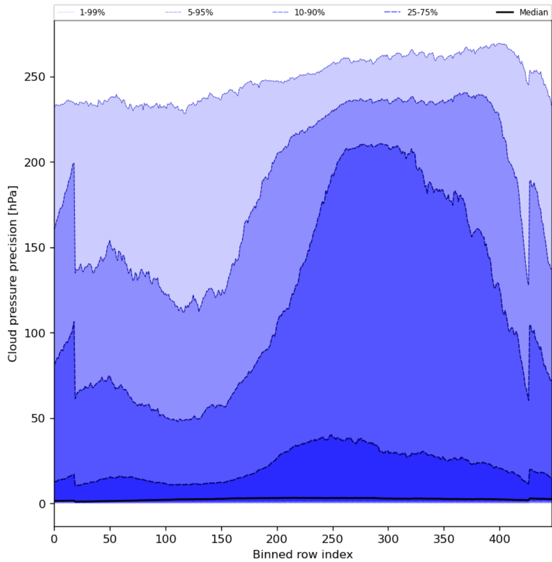
Figure 48: Along track statistics of “Cloud pressure precision” for 2023-10-19 to 2023-10-21
