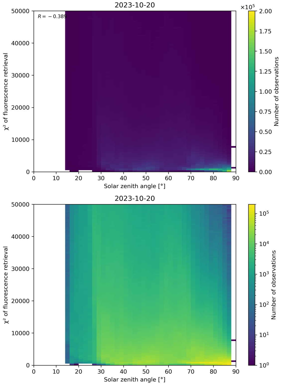
Figure 120: Scatter density plot of “Solar zenith angle” against “ \chi^2 of fluorescence retrieval” for 2023-10-19 to 2023-10-21.
