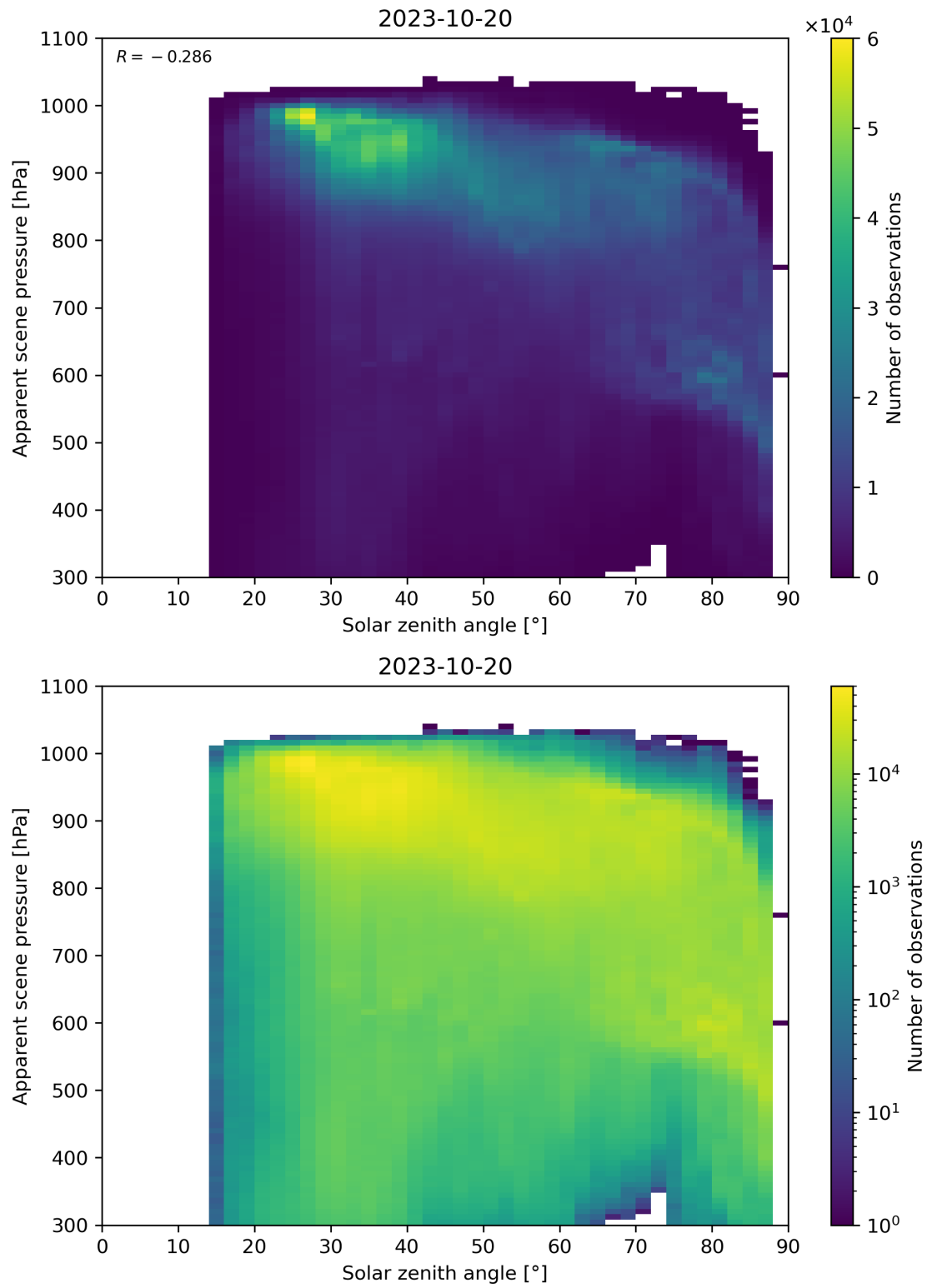
Figure 118: Scatter density plot of “Solar zenith angle” against “Apparent scene pressure” for 2023-10-19 to 2023-10-21.
