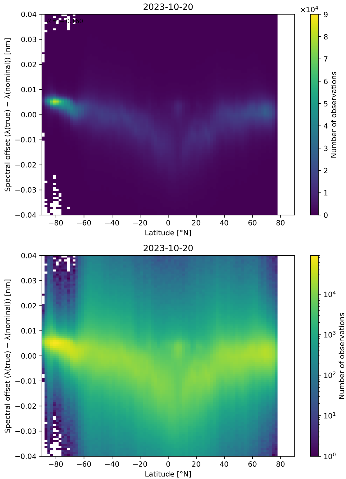
Figure 105: Scatter density plot of “Latitude” against “Spectral offset ( \lambda(\text{true}) - \lambda(\text{nominal}) )” for 2023-10-19 to 2023-10-21.
