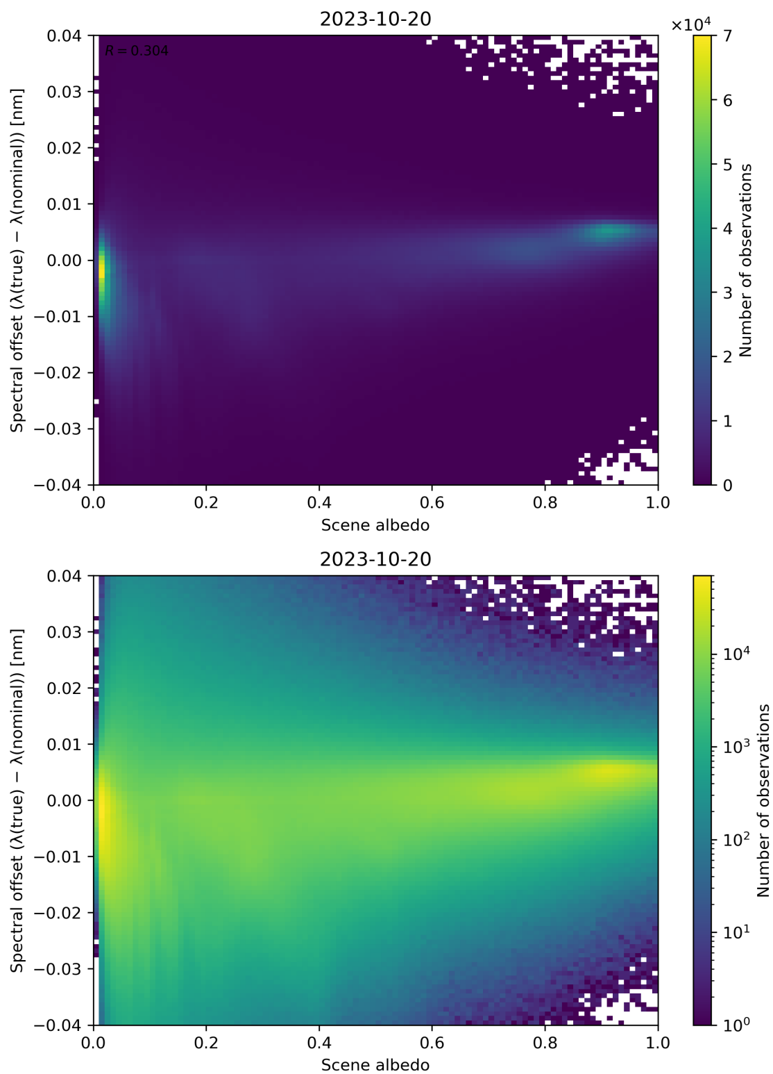
Figure 117: Scatter density plot of “Scene albedo” against “Spectral offset ( \lambda(\text{true}) - \lambda(\text{nominal}) )” for 2023-10-19 to 2023-10-21.
