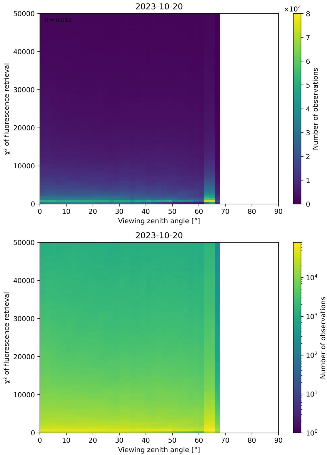
Figure 131: Scatter density plot of “Viewing zenith angle” against “ \chi^2 of fluorescence retrieval” for 2023-10-19 to 2023-10-21.
