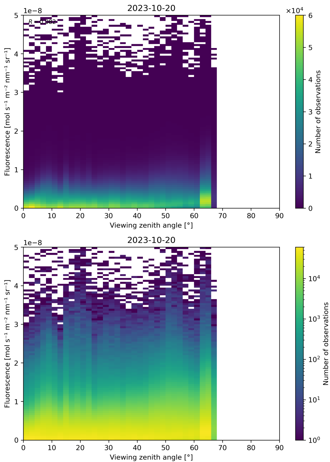
Figure 134: Scatter density plot of “Viewing zenith angle” against “Fluorescence” for 2023-10-19 to 2023-10-21.
