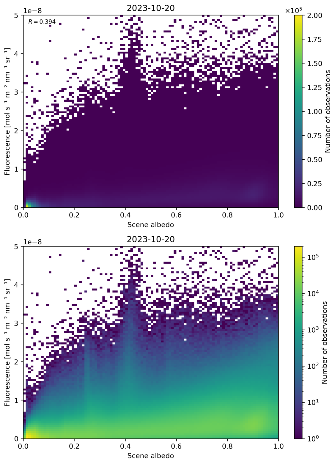
Figure 114: Scatter density plot of “Scene albedo” against “Fluorescence” for 2023-10-19 to 2023-10-21.
