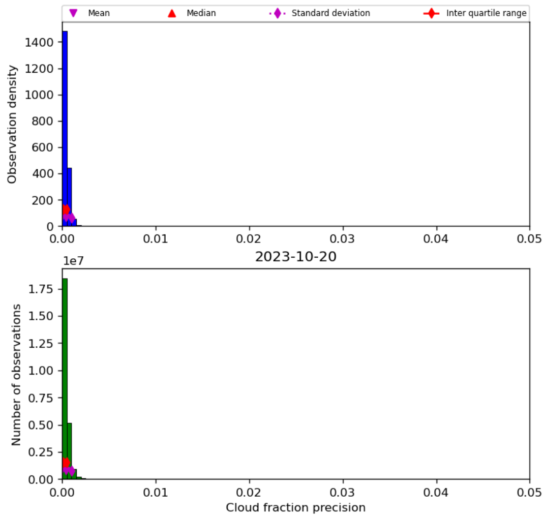
Figure 33: Histogram of “Cloud fraction precision” for 2023-10-19 to 2023-10-21
