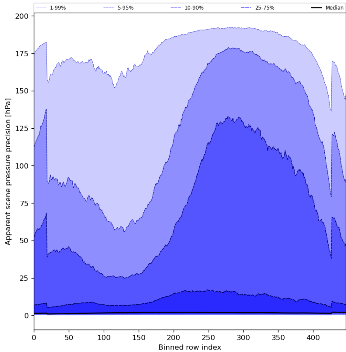
Figure 54: Along track statistics of “Apparent scene pressure precision” for 2023-10-19 to 2023-10-21
