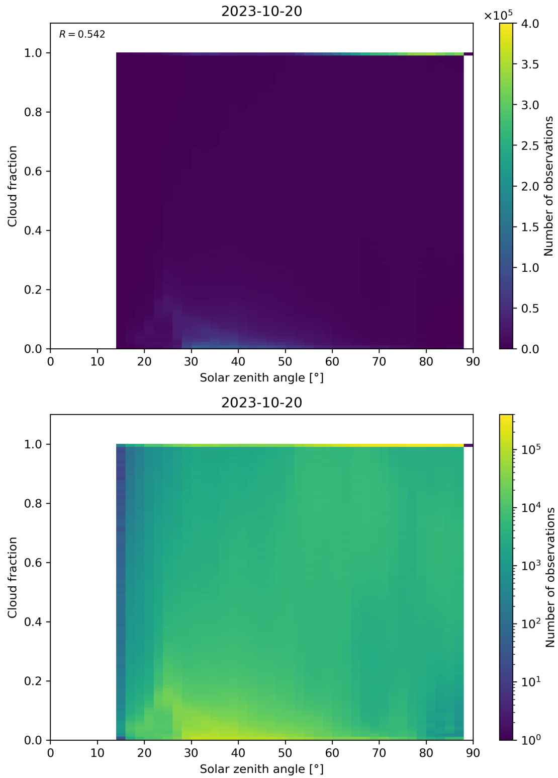
Figure 121: Scatter density plot of “Solar zenith angle” against “Cloud fraction” for 2023-10-19 to 2023-10-21.
