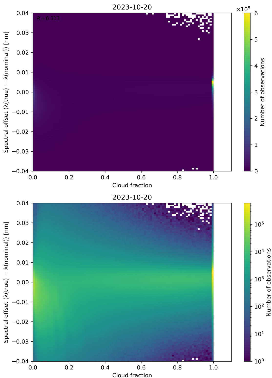
Figure 83: Scatter density plot of “Cloud fraction” against “Spectral offset ( \lambda(\text{true}) - \lambda(\text{nominal}) )” for 2023-10-19 to 2023-10-21.
