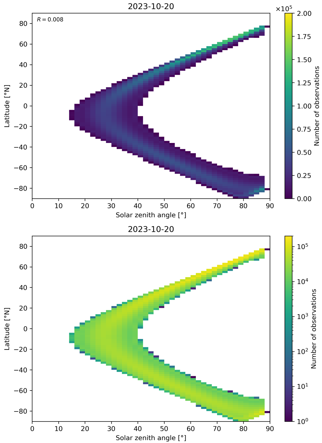
Figure 124: Scatter density plot of “Solar zenith angle” against “Latitude” for 2023-10-19 to 2023-10-21.
