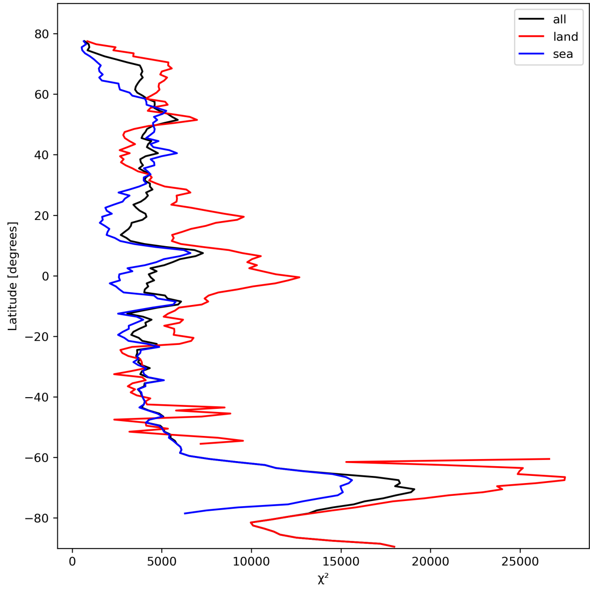
Figure 21: Zonal average of “ \chi^2 ” for 2023-10-19 to 2023-10-21.
