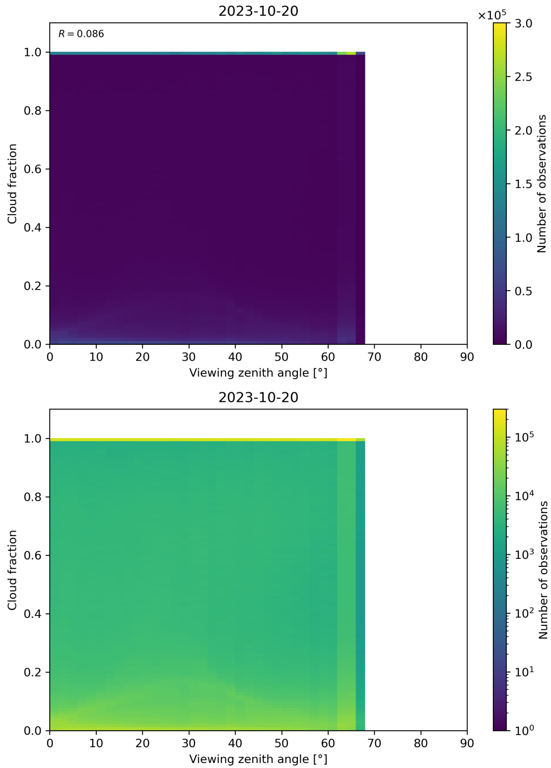
Figure 132: Scatter density plot of “Viewing zenith angle” against “Cloud fraction” for 2023-10-19 to 2023-10-21.
