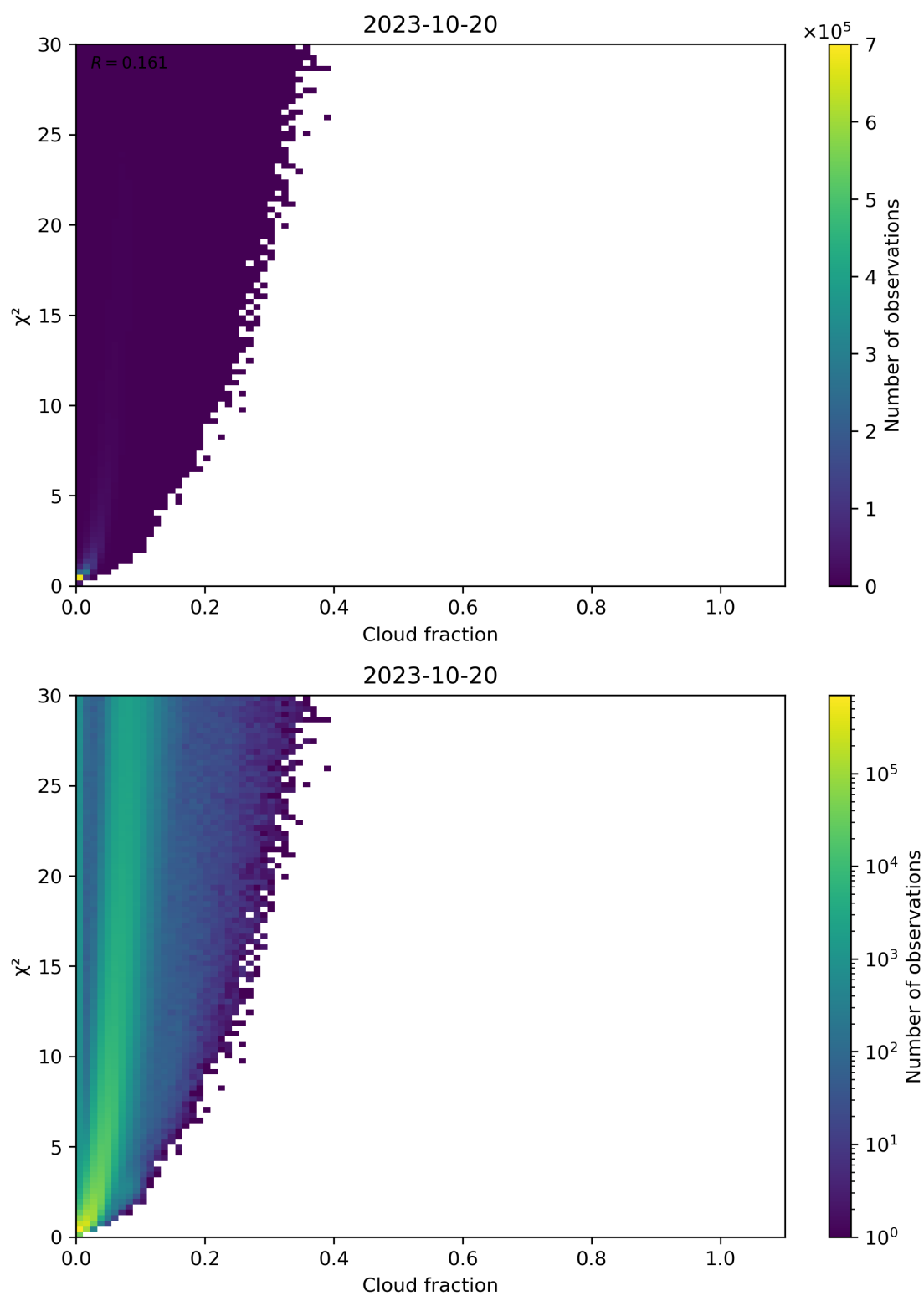
Figure 77: Scatter density plot of “Cloud fraction” against “ \chi^2 ” for 2023-10-19 to 2023-10-21.
