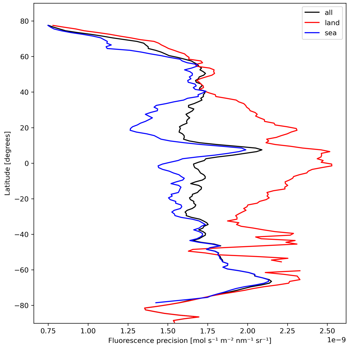
Figure 24: Zonal average of “Fluorescence precision” for 2023-10-19 to 2023-10-21.
