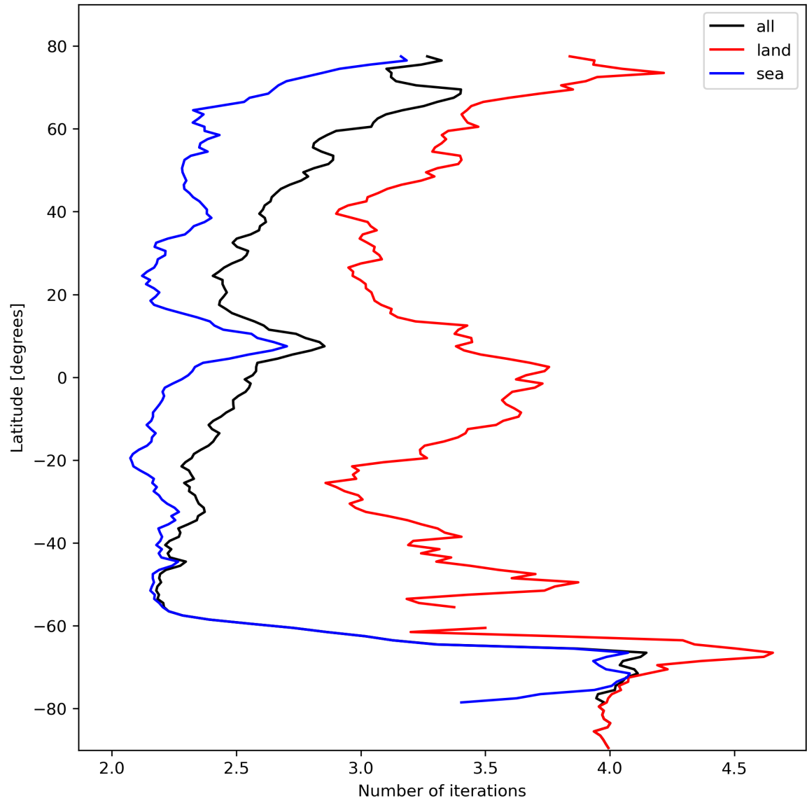
Figure 22: Zonal average of “Number of iterations” for 2023-10-19 to 2023-10-21.
