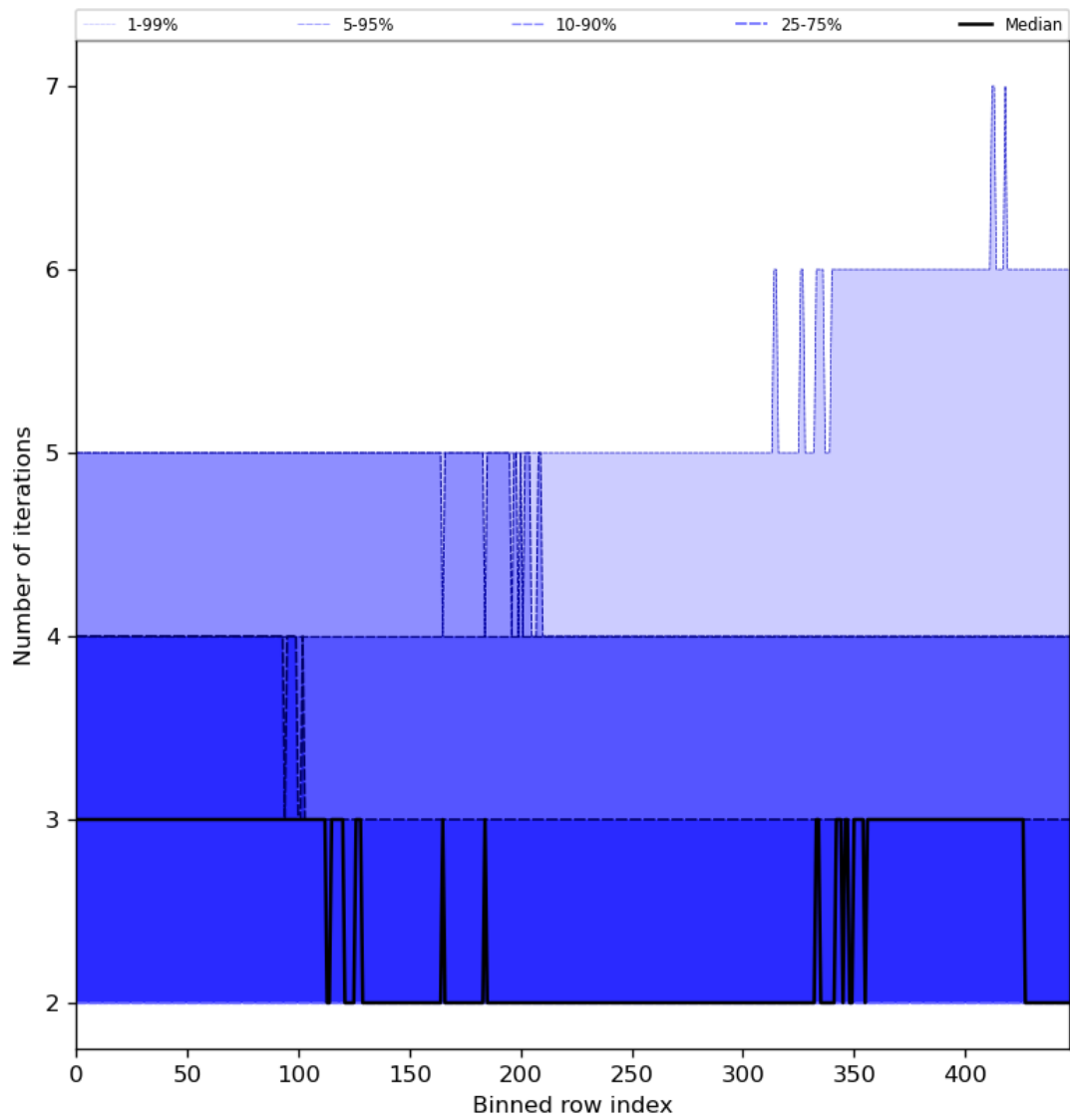
Figure 56: Along track statistics of “Number of iterations” for 2023-10-19 to 2023-10-21
