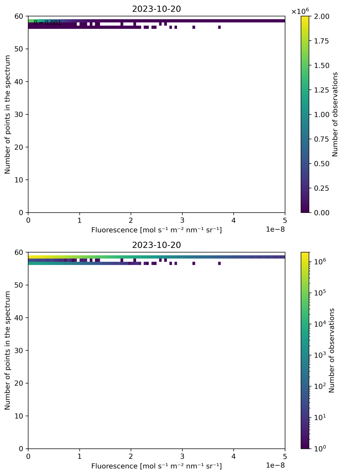
Figure 94: Scatter density plot of “Fluorescence” against “Number of points in the spectrum” for 2023-10-19 to 2023-10-21.
