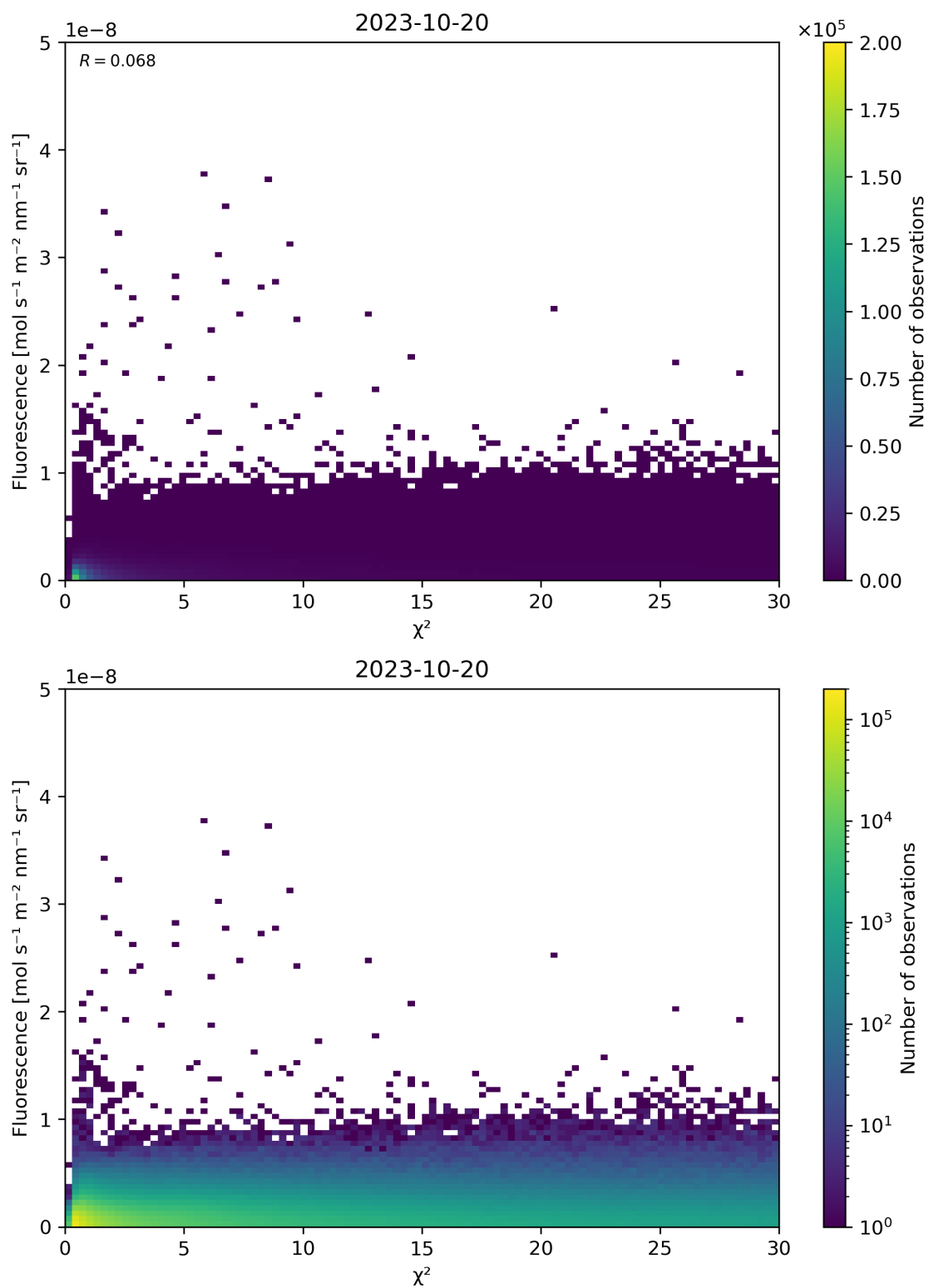
Figure 70: Scatter density plot of “ \chi^2 ” against “Fluorescence” for 2023-10-19 to 2023-10-21.
