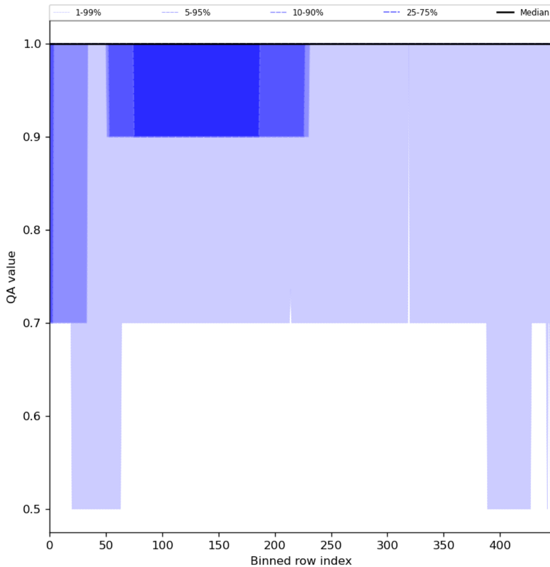
Figure 46: Along track statistics of “QA value” for 2023-10-19 to 2023-10-21
