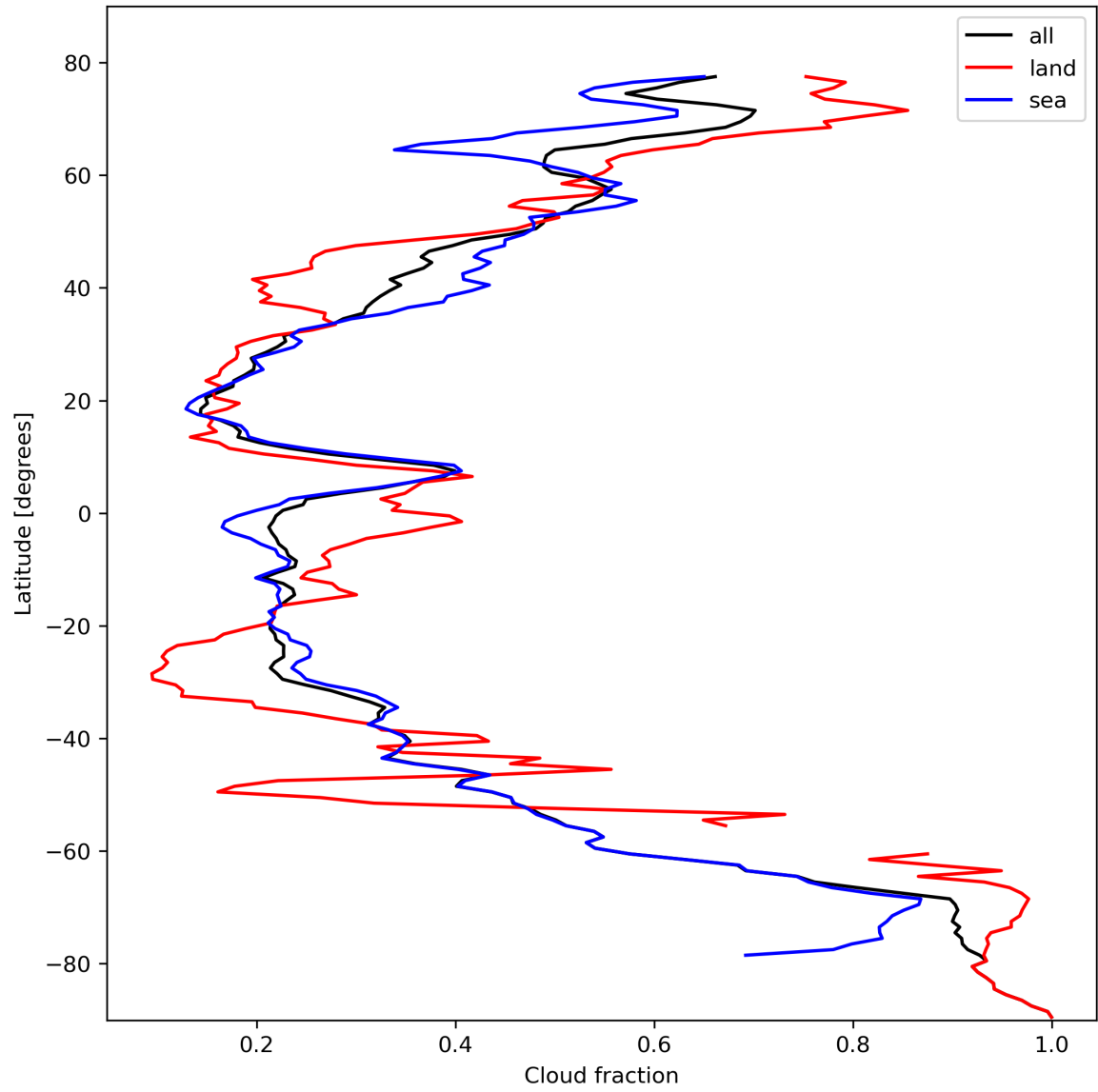
Figure 15: Zonal average of “Cloud fraction” for 2023-10-19 to 2023-10-21.
