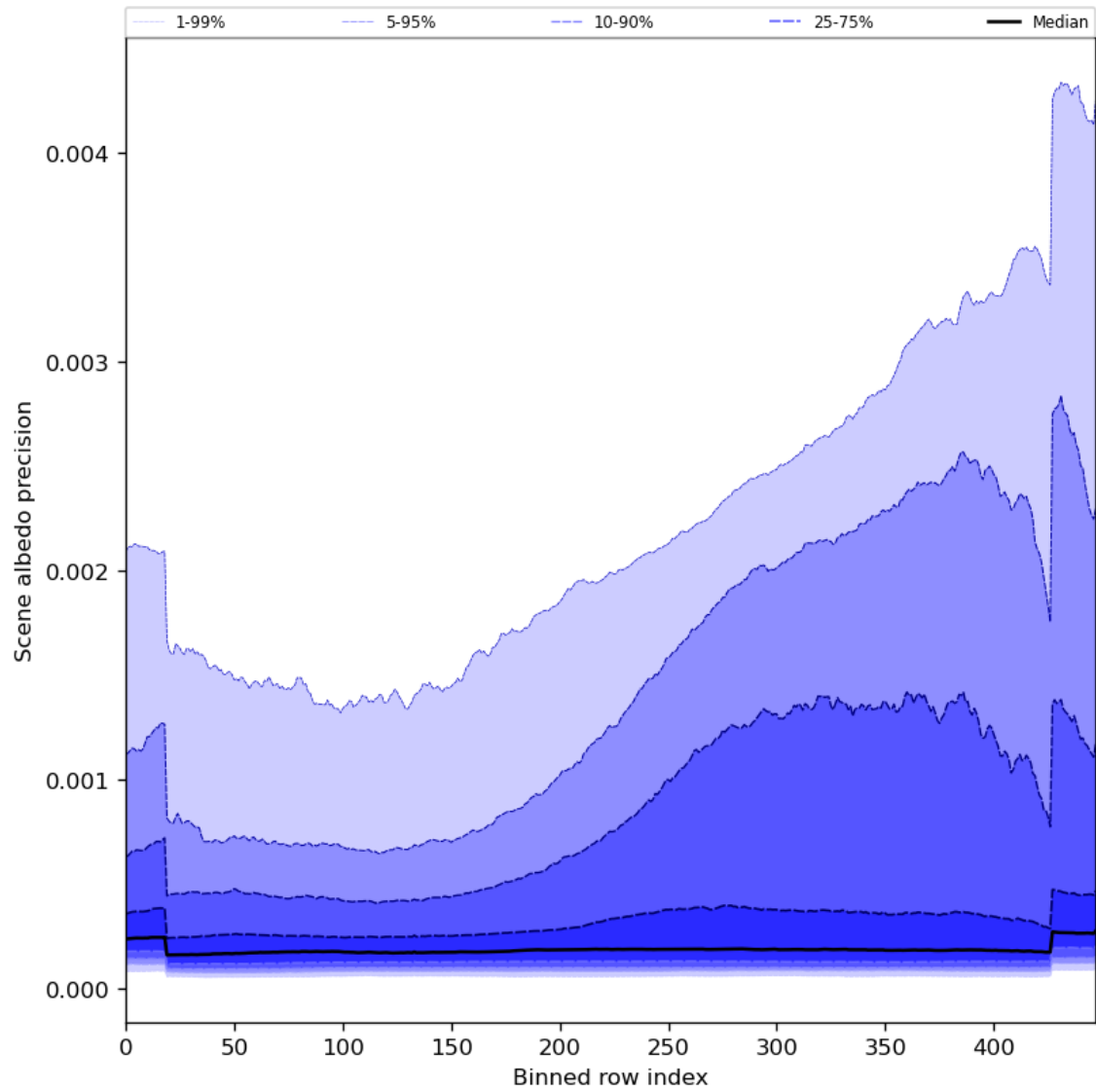
Figure 52: Along track statistics of “Scene albedo precision” for 2023-10-19 to 2023-10-21
