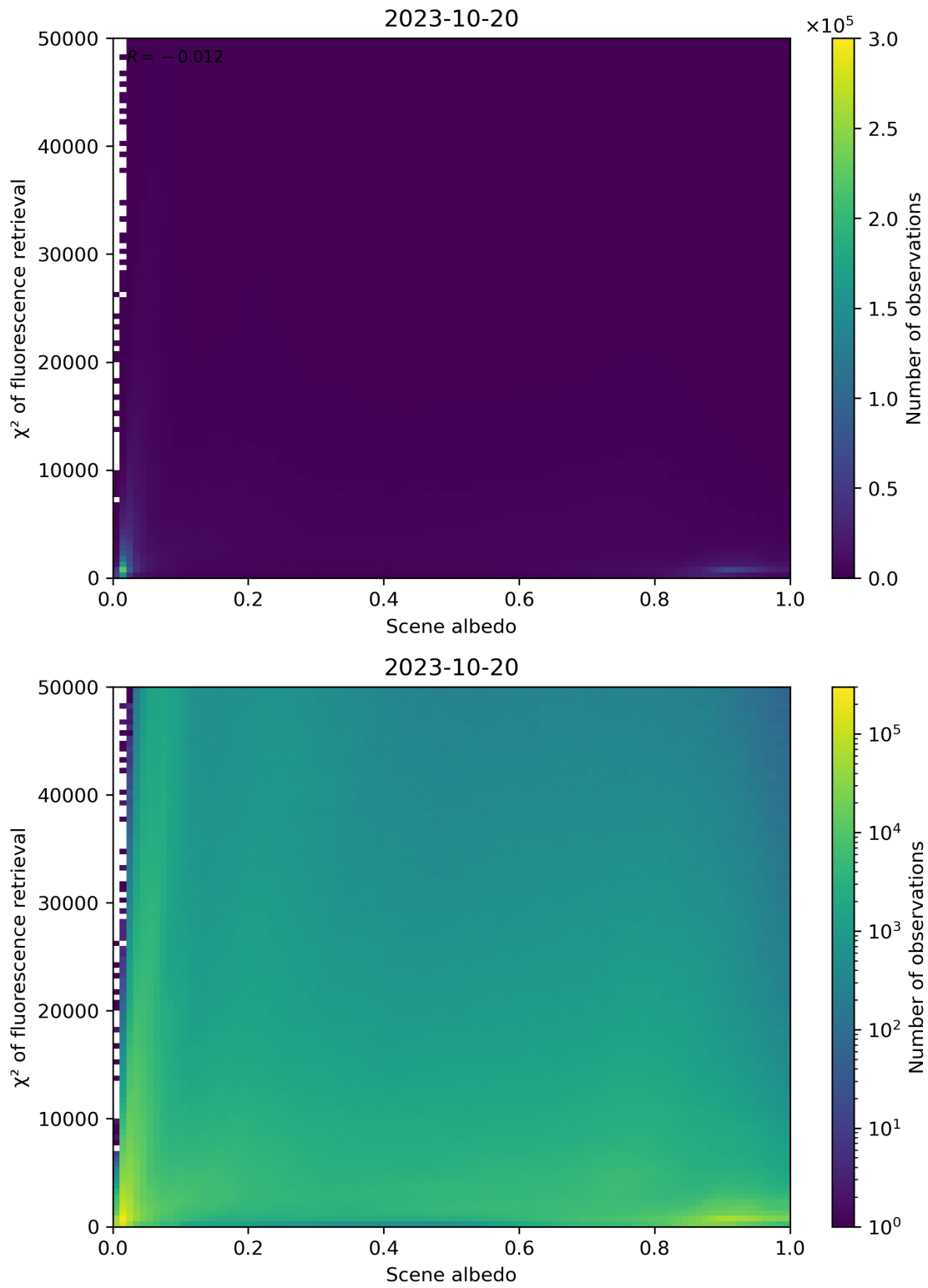
Figure 113: Scatter density plot of “Scene albedo” against “ \chi^2 of fluorescence retrieval” for 2023-10-19 to 2023-10-21.
