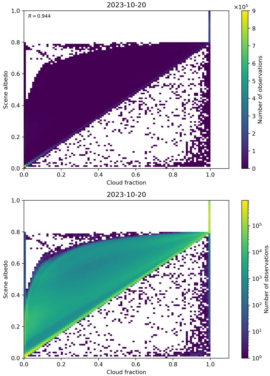
Figure 82: Scatter density plot of “Cloud fraction” against “Scene albedo” for 2023-10-19 to 2023-10-21.
