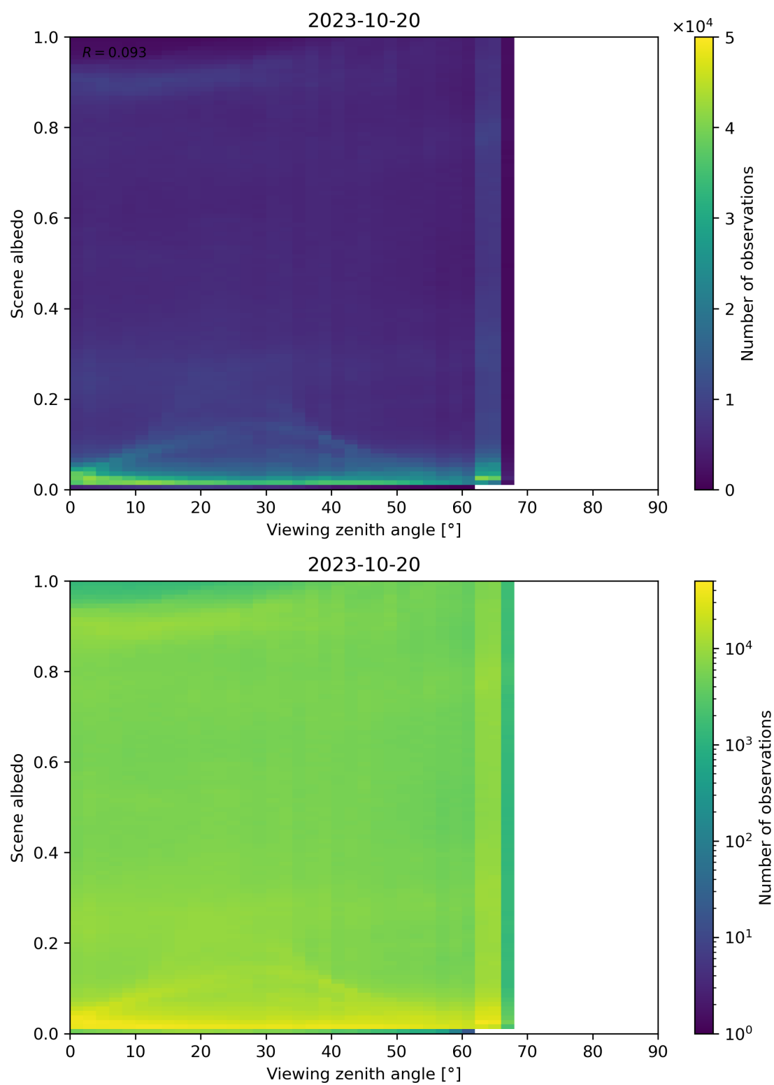
Figure 138: Scatter density plot of “Viewing zenith angle” against “Scene albedo” for 2023-10-19 to 2023-10-21.
