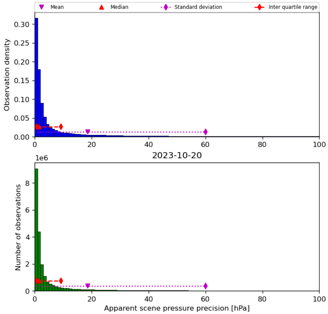
Figure 37: Histogram of “Apparent scene pressure precision” for 2023-10-19 to 2023-10-21
