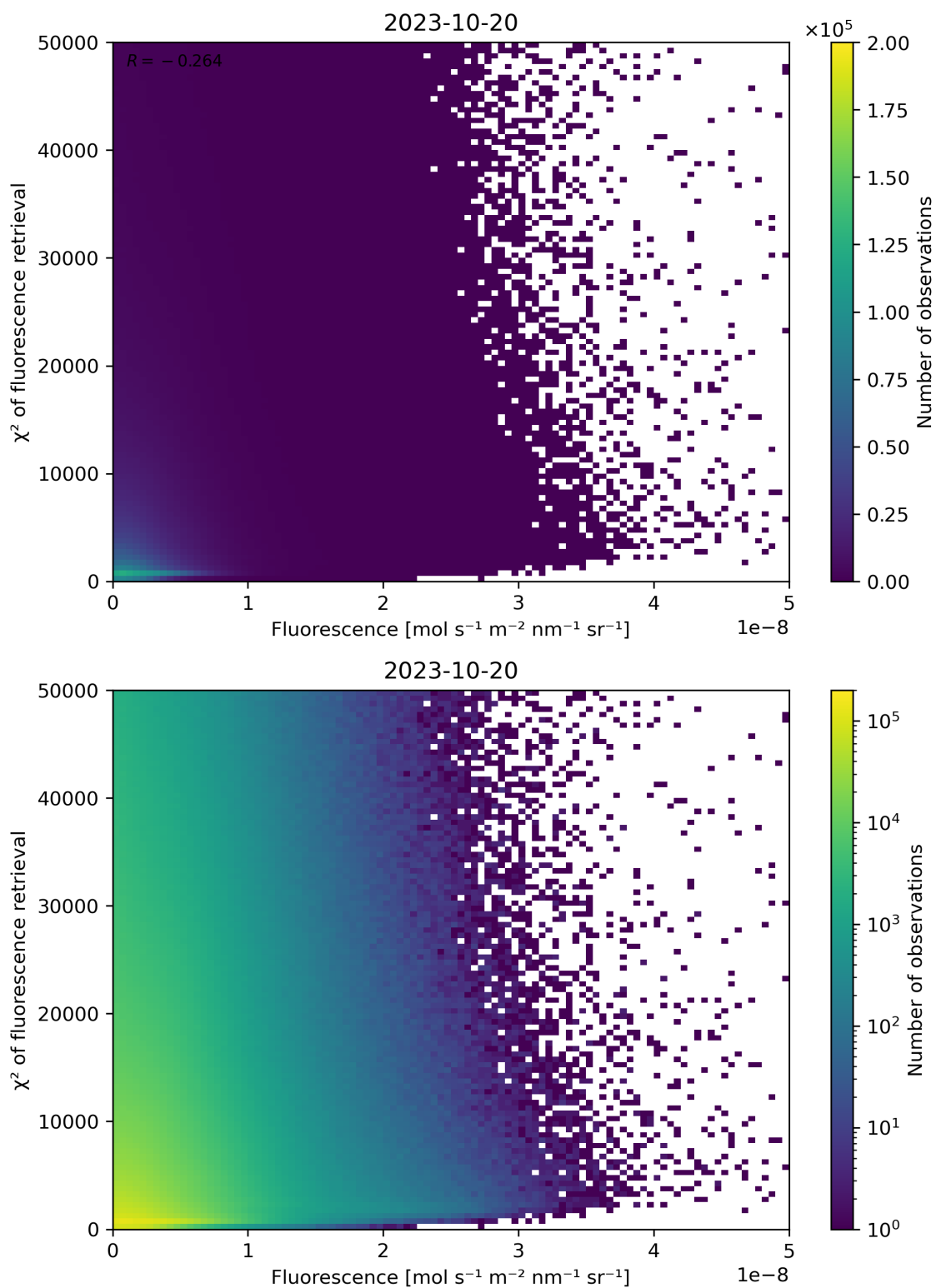
Figure 93: Scatter density plot of “Fluorescence” against “ \chi^2 of fluorescence retrieval” for 2023-10-19 to 2023-10-21.
