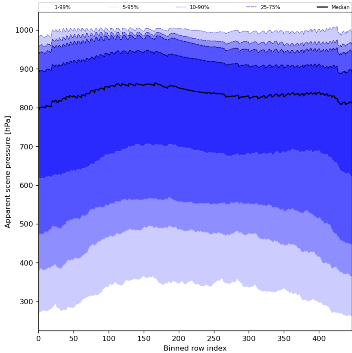
Figure 53: Along track statistics of “Apparent scene pressure” for 2023-10-19 to 2023-10-21
