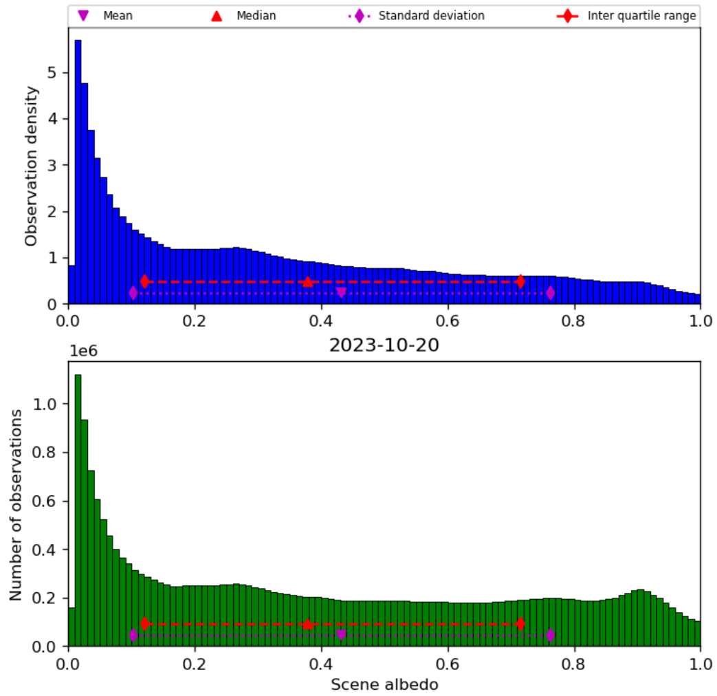
Figure 34: Histogram of “Scene albedo” for 2023-10-19 to 2023-10-21
