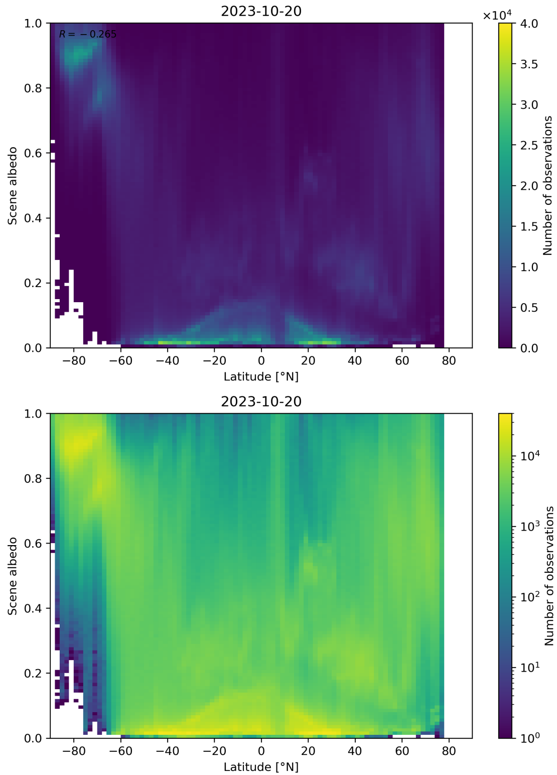
Figure 104: Scatter density plot of “Latitude” against “Scene albedo” for 2023-10-19 to 2023-10-21.
