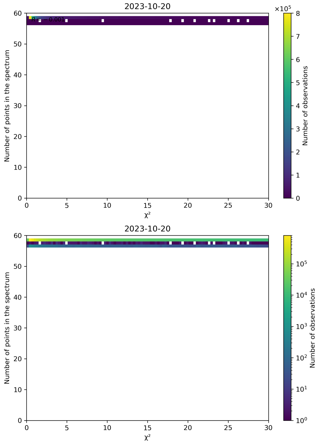
Figure 74: Scatter density plot of “ \chi^2 ” against “Number of points in the spectrum” for 2023-10-19 to 2023-10-21.
