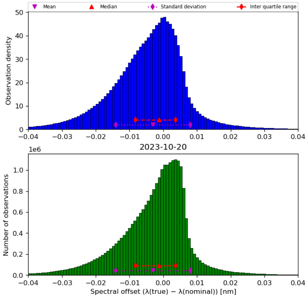
Figure 45: Histogram of “Spectral offset ( \lambda(\text{true}) - \lambda(\text{nominal}) )” for 2023-10-19 to 2023-10-21
