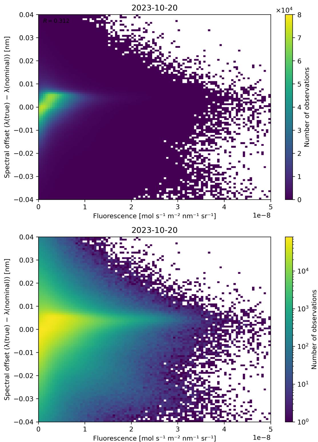
Figure 95: Scatter density plot of “Fluorescence” against “Spectral offset ( \lambda(\text{true}) - \lambda(\text{nominal}) )” for 2023-10-19 to 2023-10-21.
