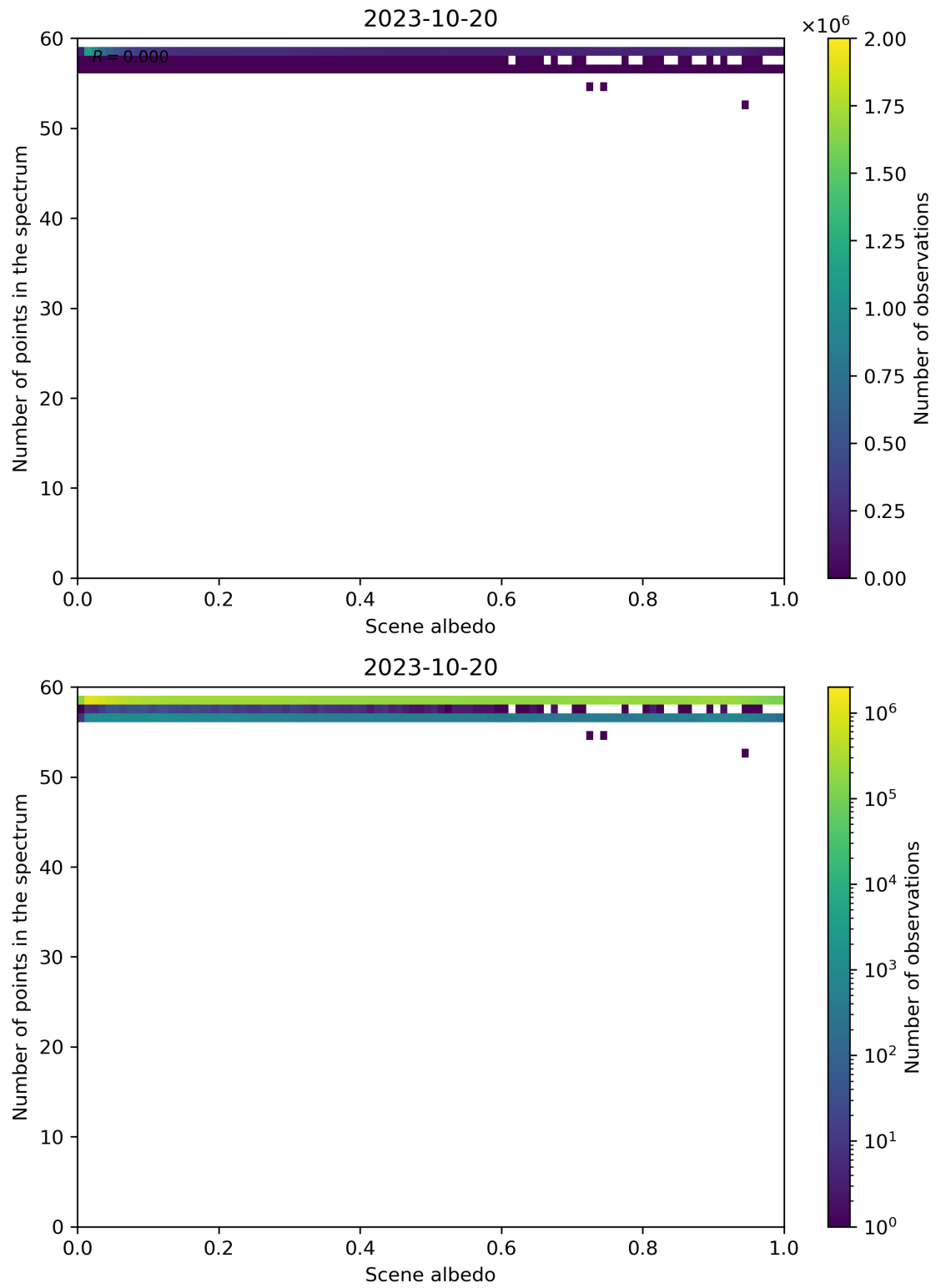
Figure 116: Scatter density plot of “Scene albedo” against “Number of points in the spectrum” for 2023-10-19 to 2023-10-21.
