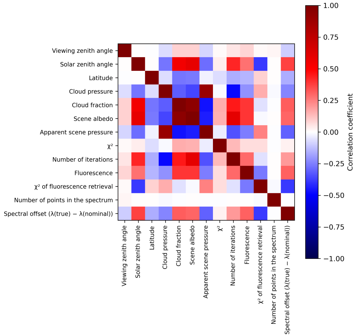
Figure 2: Map of correlation matrix for 2023-10-19 to 2023-10-21.
