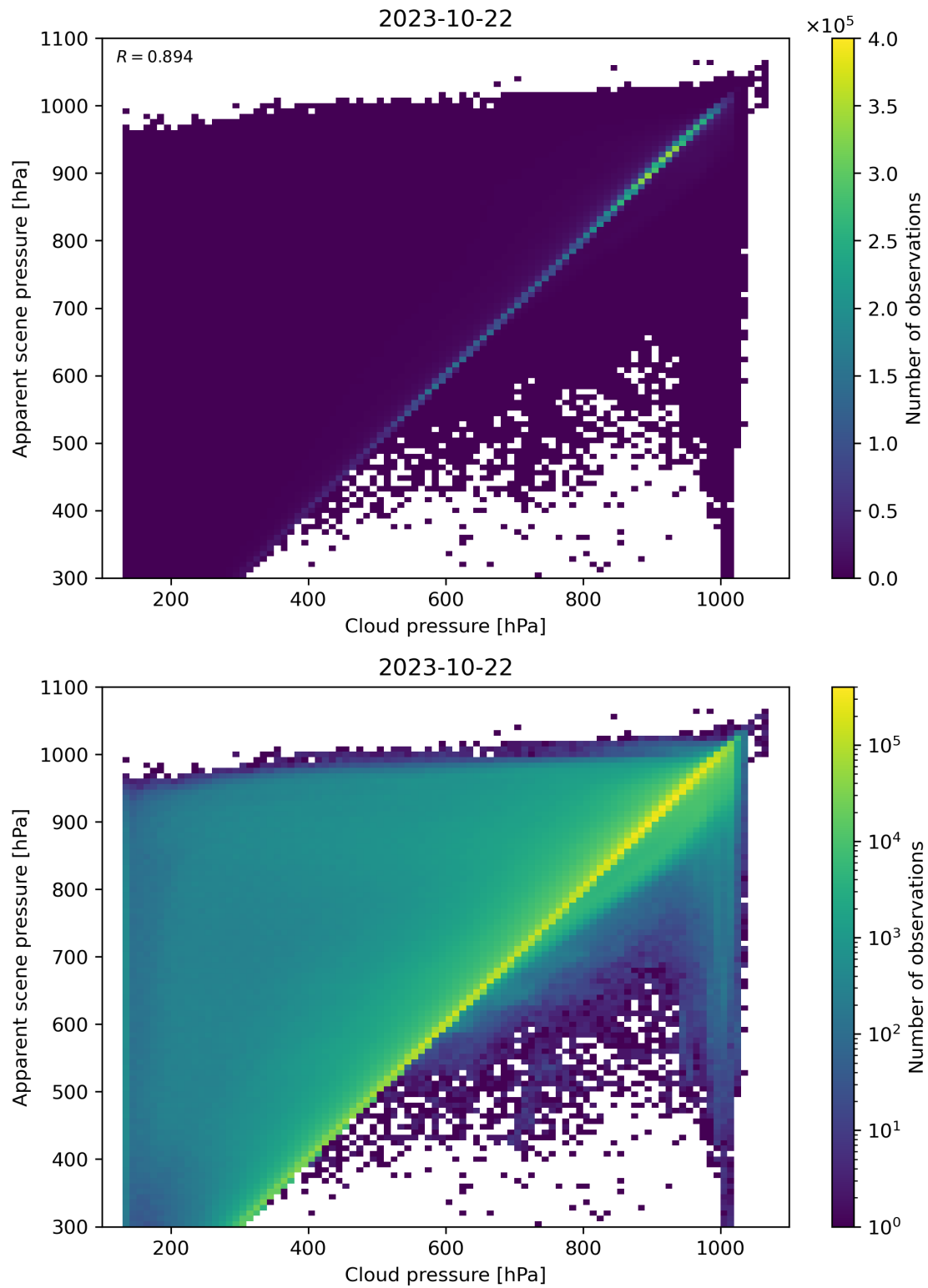
Figure 84: Scatter density plot of “Cloud pressure” against “Apparent scene pressure” for 2023-10-22 to 2023-10-23.
