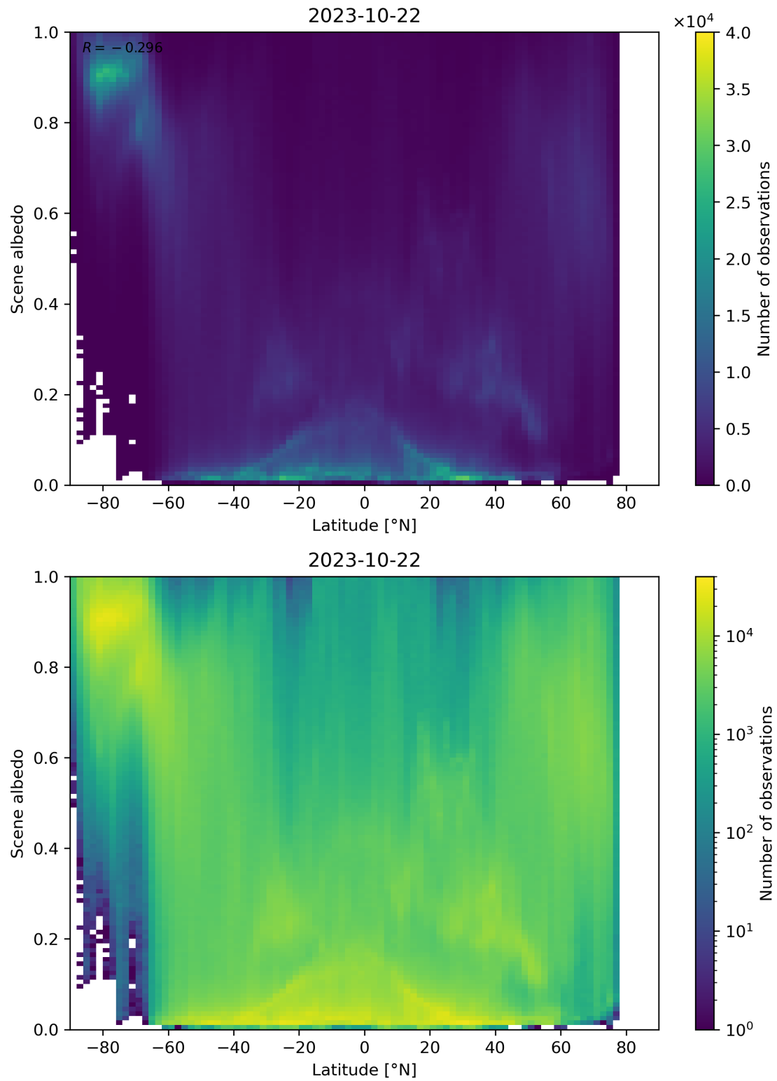
Figure 104: Scatter density plot of “Latitude” against “Scene albedo” for 2023-10-22 to 2023-10-23.
