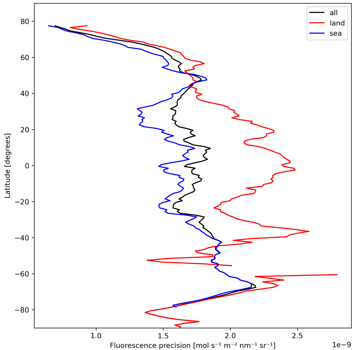
Figure 24: Zonal average of “Fluorescence precision” for 2023-10-22 to 2023-10-23.
