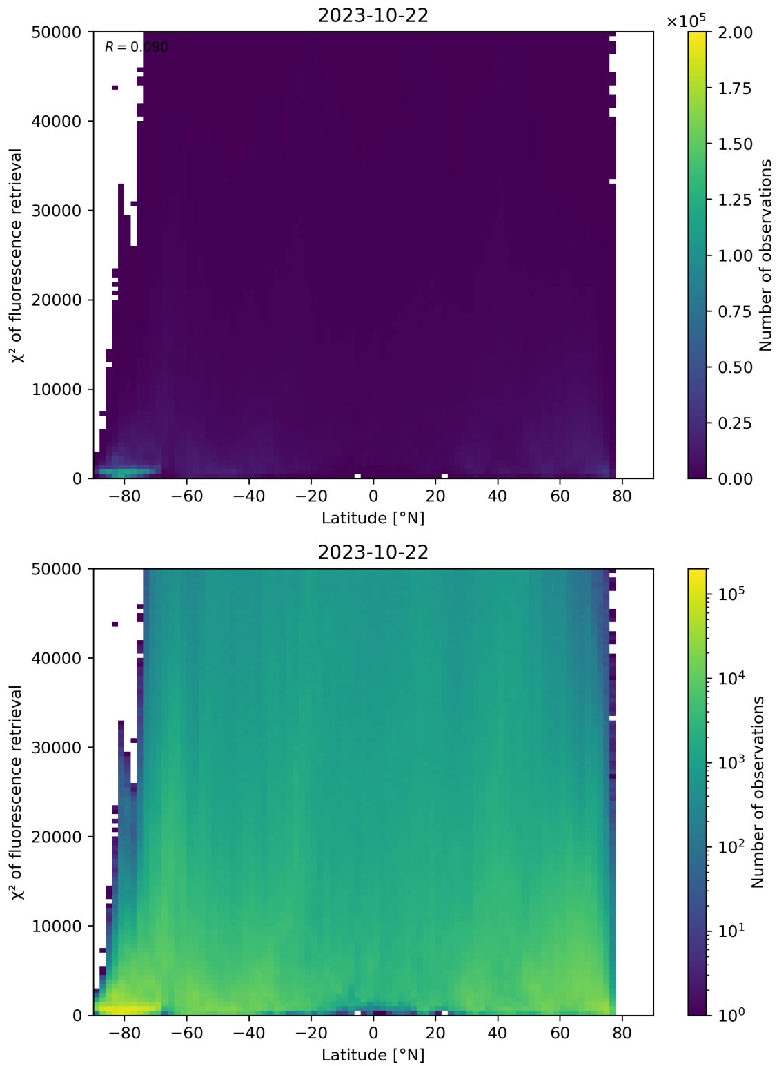
Figure 98: Scatter density plot of “Latitude” against “ \chi^2 of fluorescence retrieval” for 2023-10-22 to 2023-10-23.
