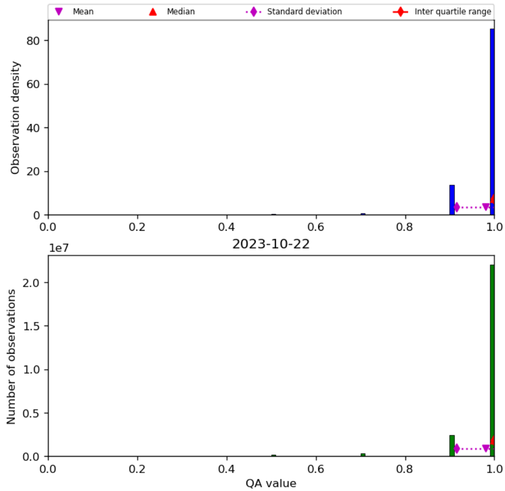
Figure 29: Histogram of “QA value” for 2023-10-22 to 2023-10-23
