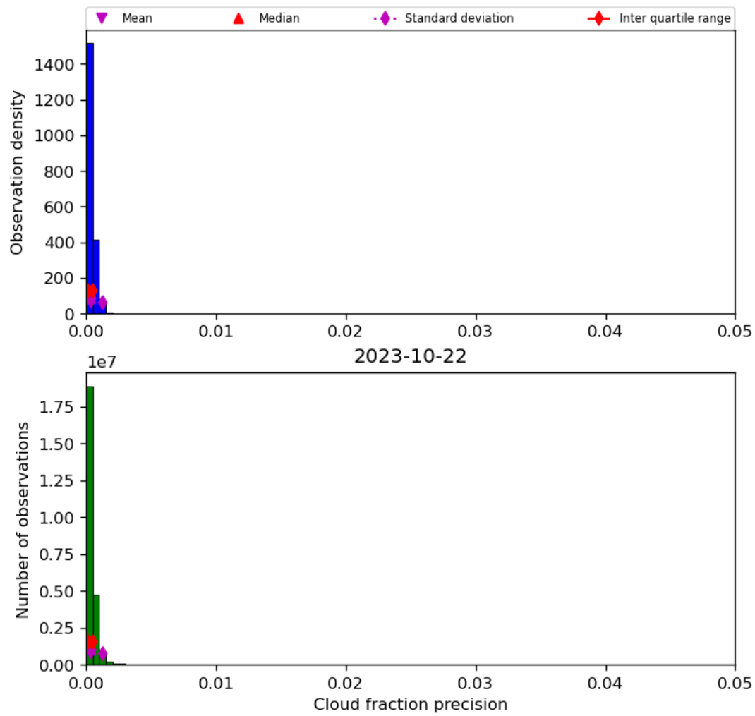
Figure 33: Histogram of “Cloud fraction precision” for 2023-10-22 to 2023-10-23
