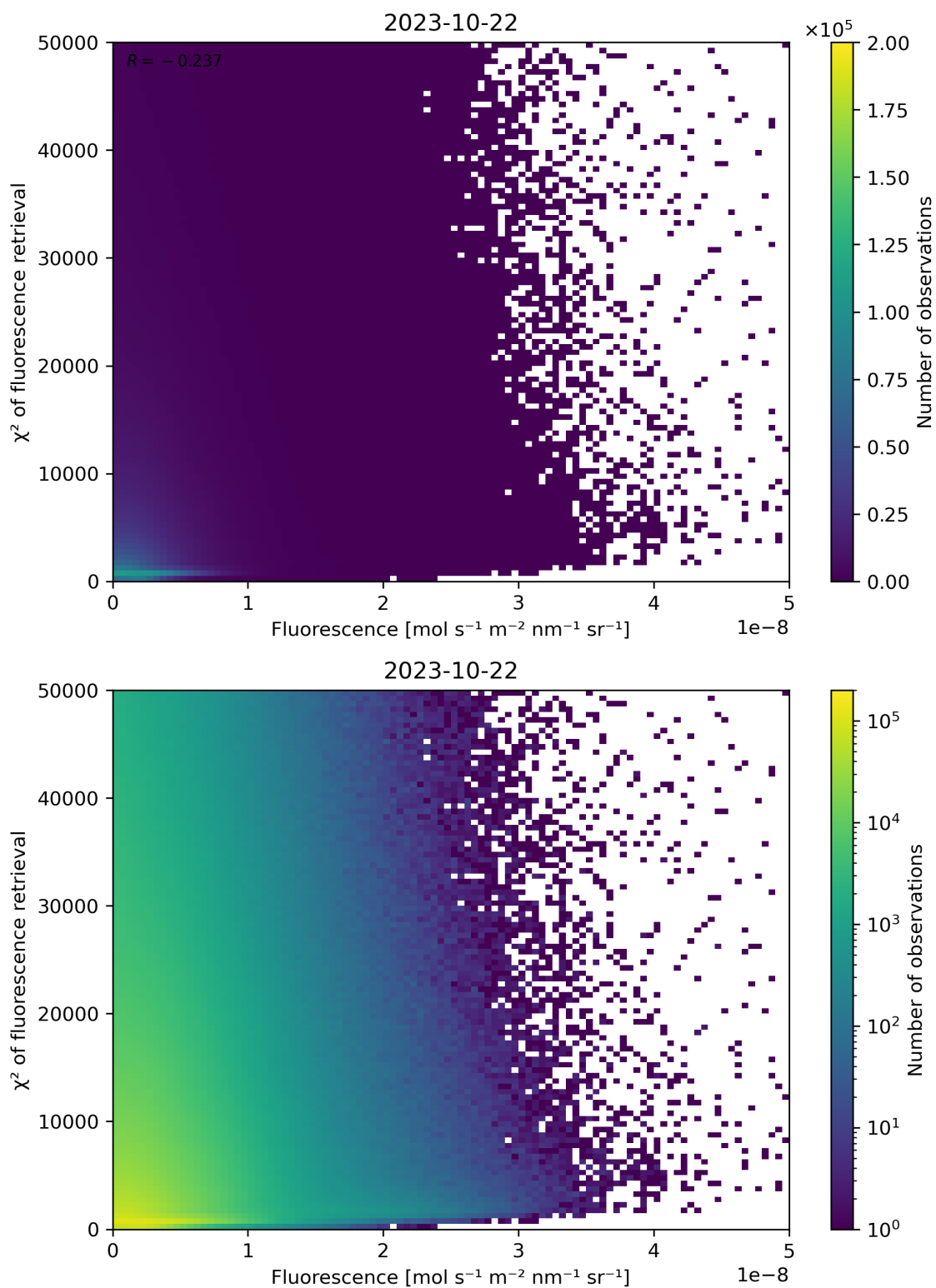
Figure 93: Scatter density plot of “Fluorescence” against “ \chi^2 of fluorescence retrieval” for 2023-10-22 to 2023-10-23.
