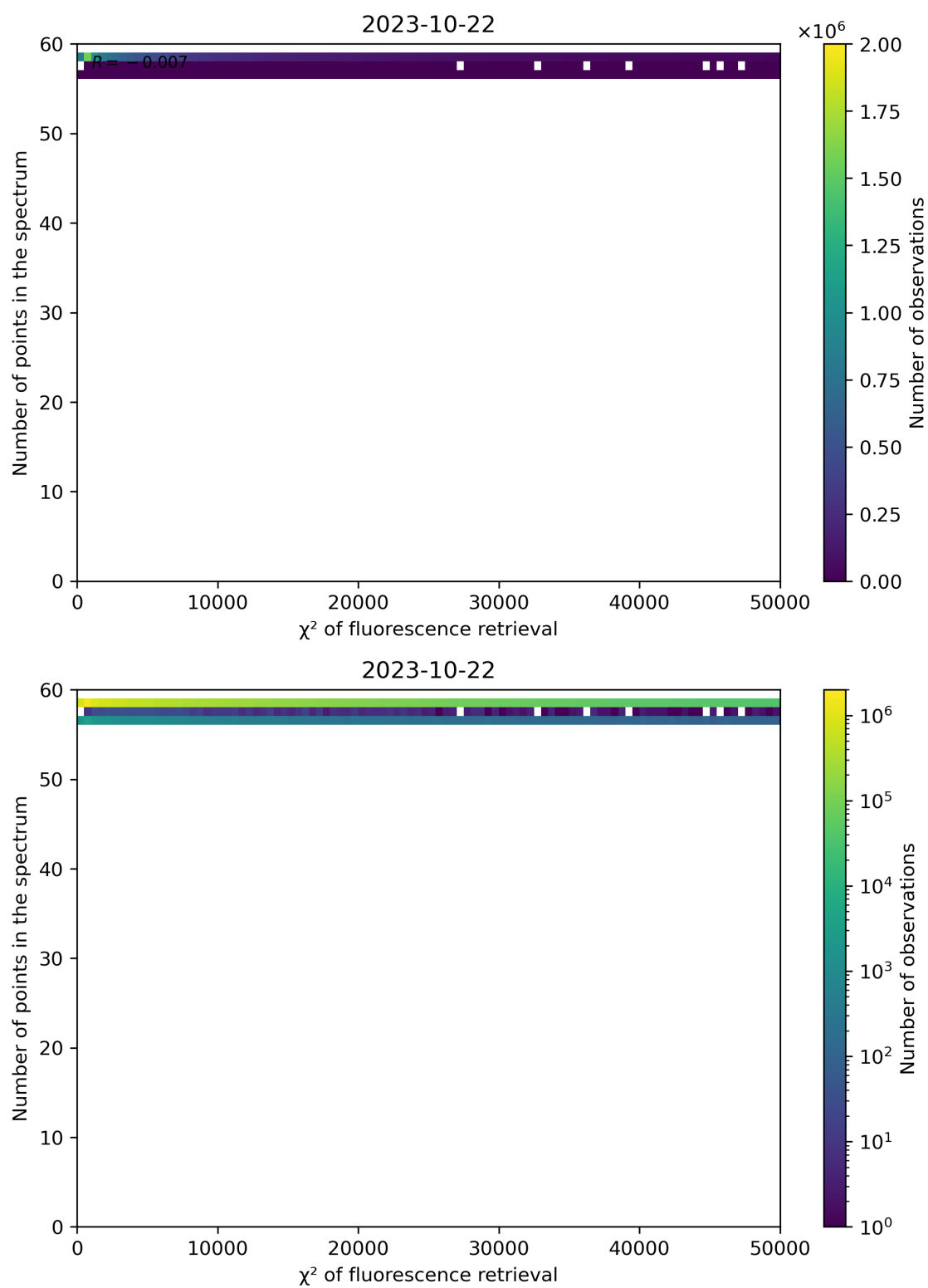
Figure 71: Scatter density plot of " \chi^2 of fluorescence retrieval" against "Number of points in the spectrum" for 2023-10-22 to 2023-10-23.
