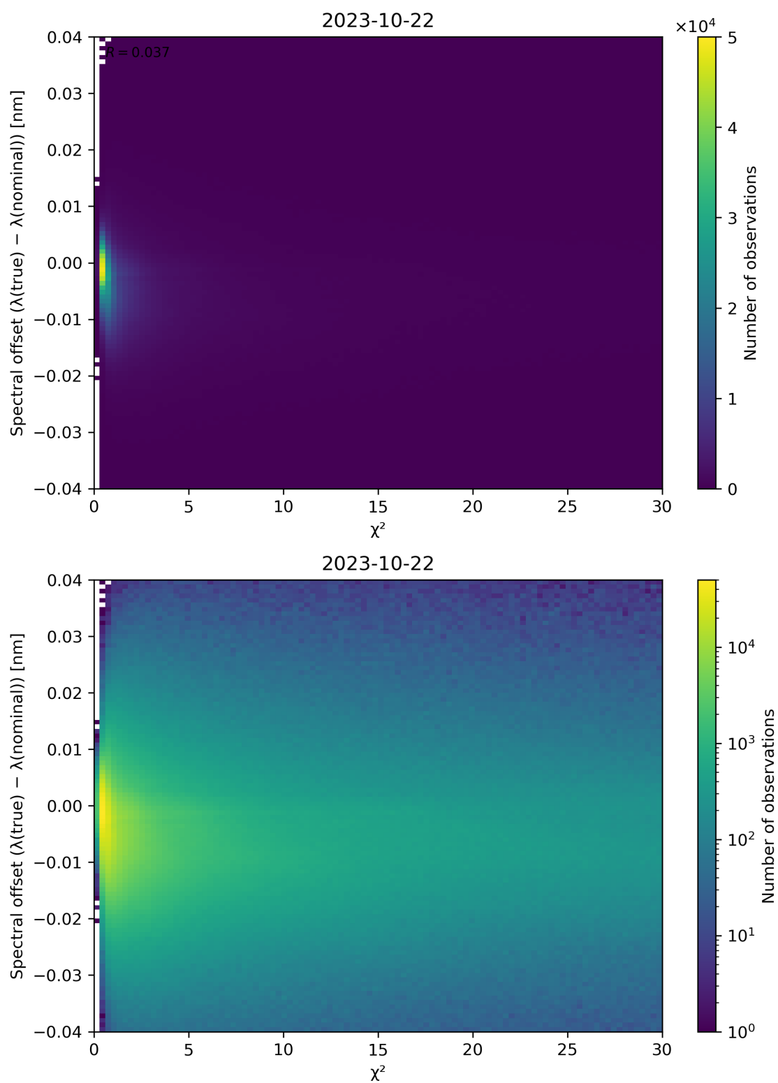
Figure 75: Scatter density plot of “ \chi^2 ” against “Spectral offset ( \lambda(\text{true}) - \lambda(\text{nominal}) )” for 2023-10-22 to 2023-10-23.
