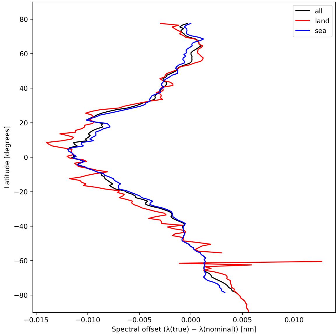
Figure 28: Zonal average of “Spectral offset ( \lambda(\text{true}) - \lambda(\text{nominal}) )” for 2023-10-22 to 2023-10-23.
