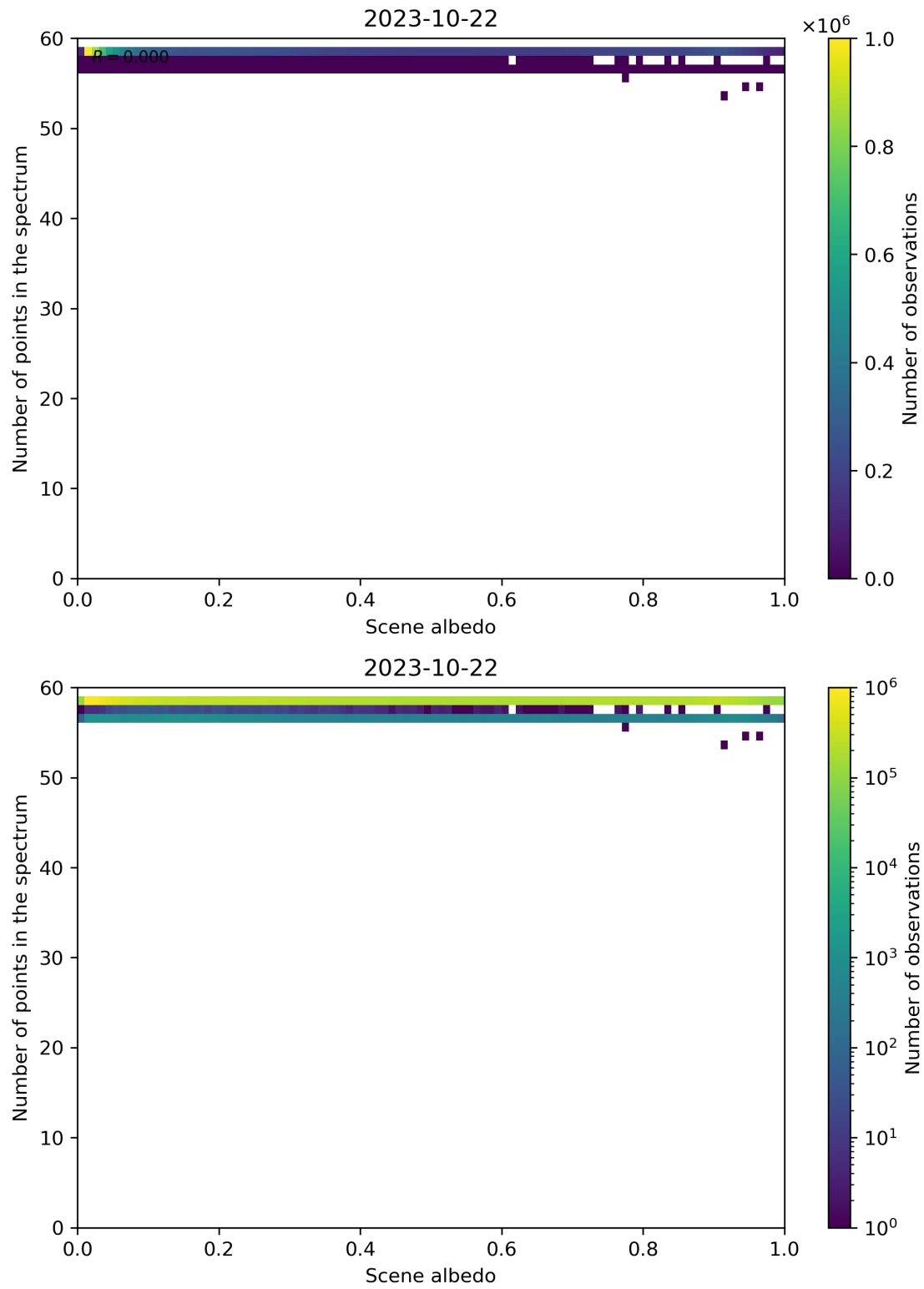
Figure 116: Scatter density plot of “Scene albedo” against “Number of points in the spectrum” for 2023-10-22 to 2023-10-23.
