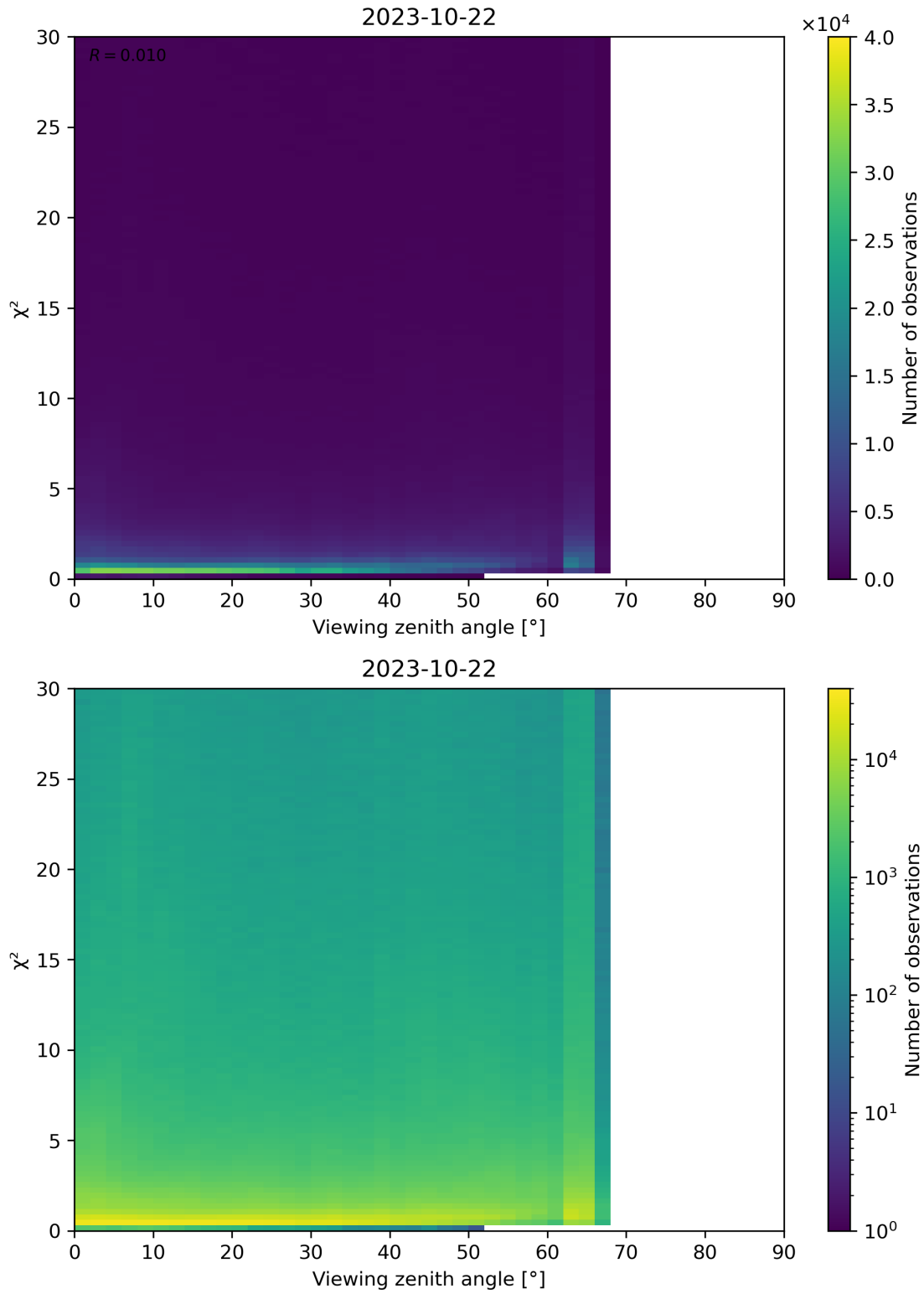
Figure 130: Scatter density plot of “Viewing zenith angle” against “ \chi^2 ” for 2023-10-22 to 2023-10-23.
