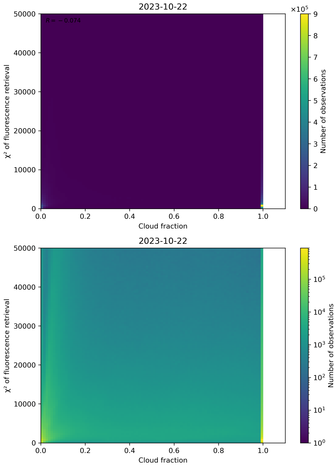
Figure 78: Scatter density plot of “Cloud fraction” against “ \chi^2 of fluorescence retrieval” for 2023-10-22 to 2023-10-23.
