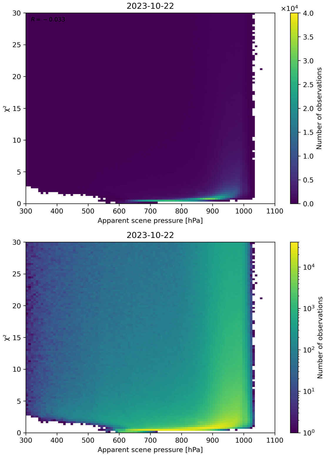
Figure 63: Scatter density plot of “Apparent scene pressure” against “ \chi^2 ” for 2023-10-22 to 2023-10-23.
