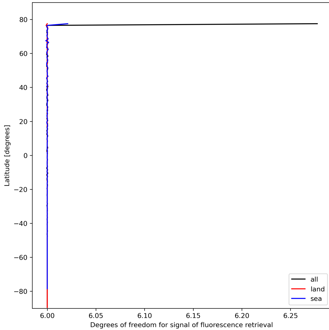
Figure 26: Zonal average of “Degrees of freedom for signal of fluorescence retrieval” for 2023-10-22 to 2023-10-23.
