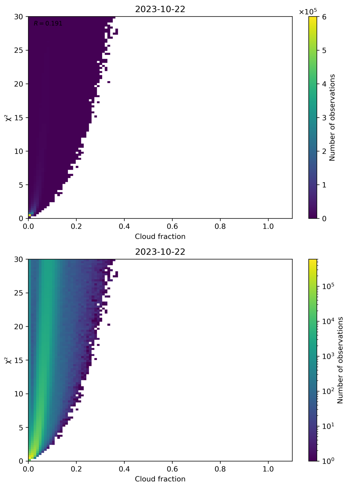
Figure 77: Scatter density plot of “Cloud fraction” against “ \chi^2 ” for 2023-10-22 to 2023-10-23.
