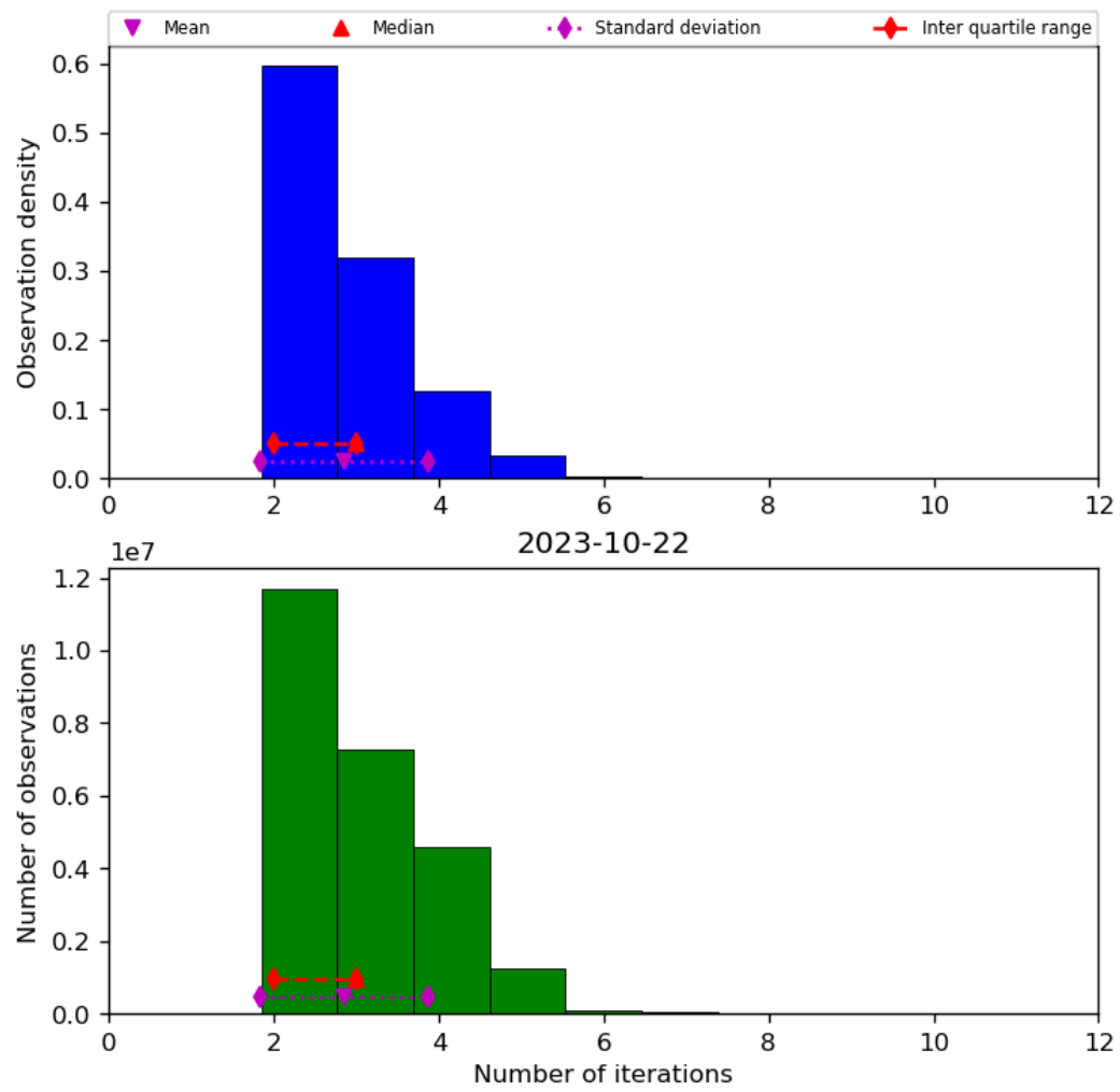
Figure 39: Histogram of “Number of iterations” for 2023-10-22 to 2023-10-23
