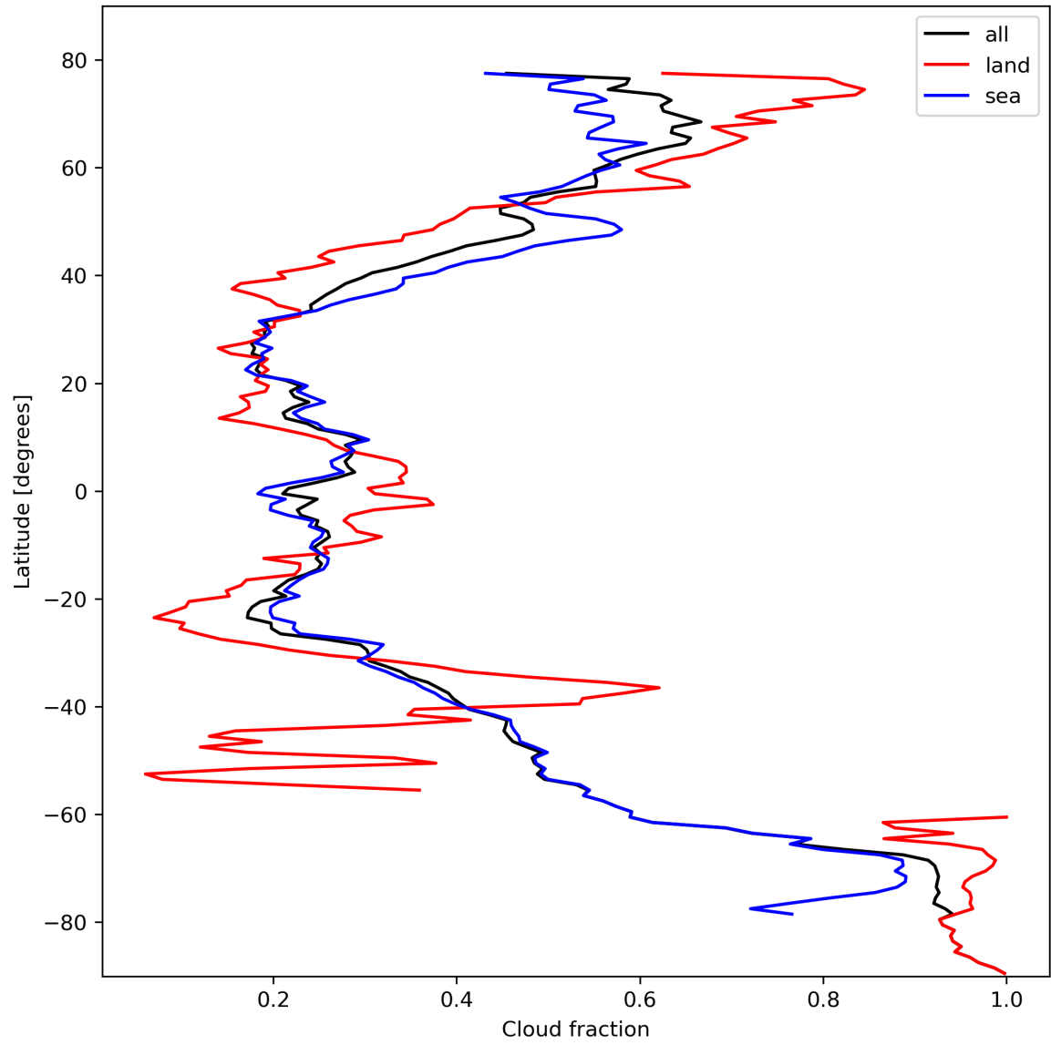
Figure 15: Zonal average of “Cloud fraction” for 2023-10-22 to 2023-10-23.
