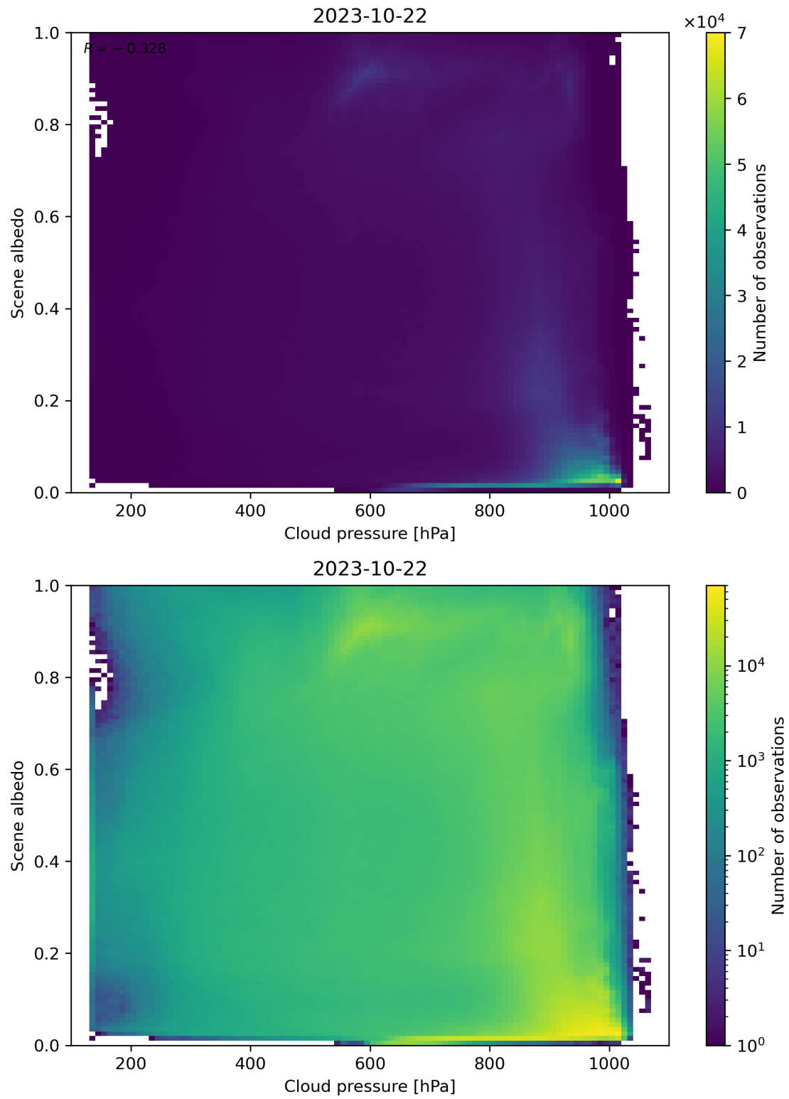
Figure 91: Scatter density plot of “Cloud pressure” against “Scene albedo” for 2023-10-22 to 2023-10-23.
