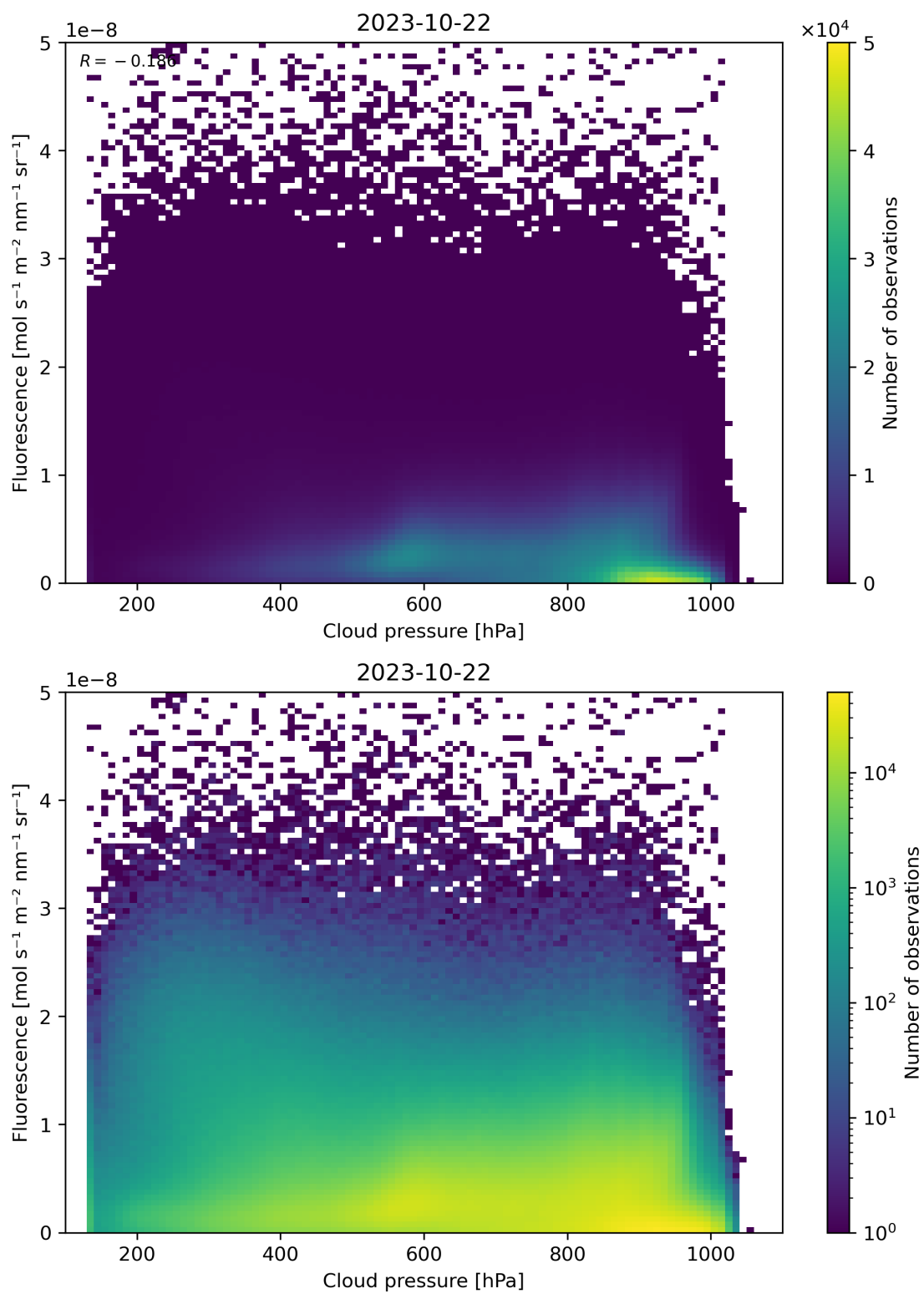
Figure 88: Scatter density plot of “Cloud pressure” against “Fluorescence” for 2023-10-22 to 2023-10-23.
