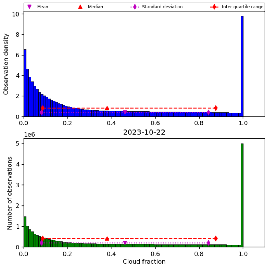
Figure 32: Histogram of “Cloud fraction” for 2023-10-22 to 2023-10-23
