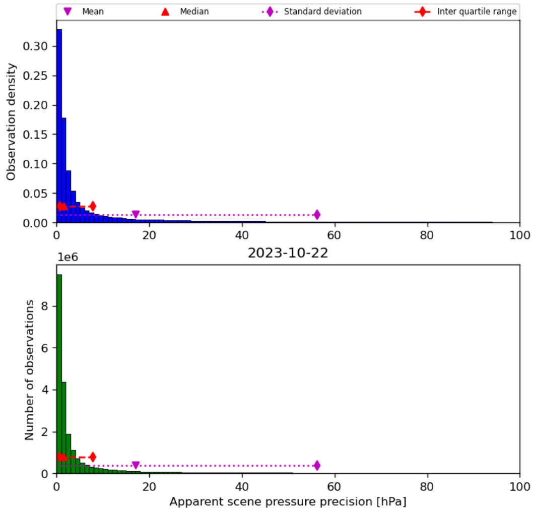
Figure 37: Histogram of “Apparent scene pressure precision” for 2023-10-22 to 2023-10-23
