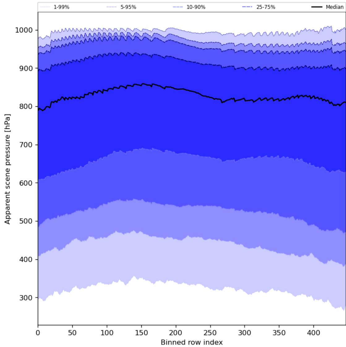
Figure 53: Along track statistics of “Apparent scene pressure” for 2023-10-22 to 2023-10-23
