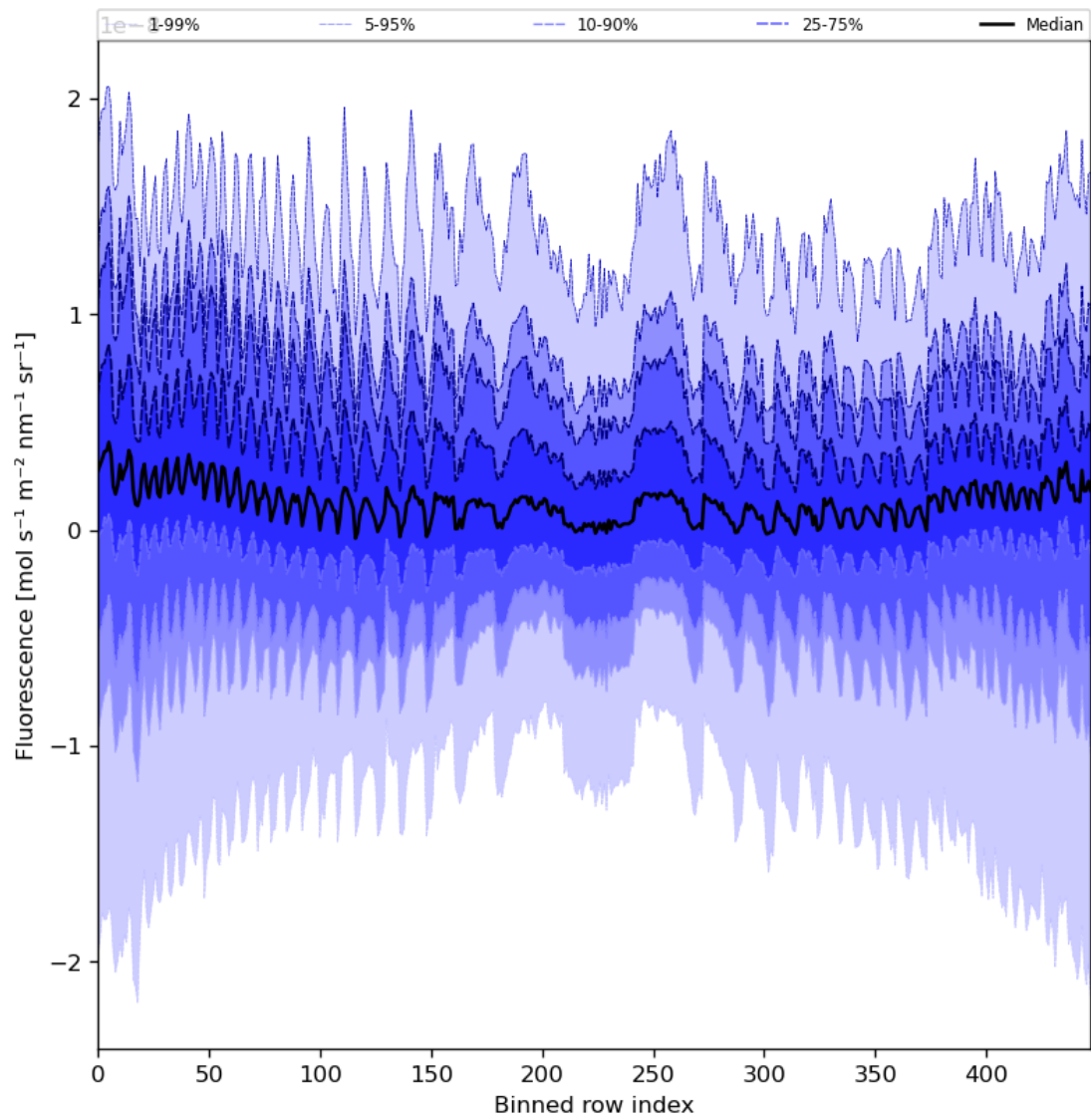
Figure 57: Along track statistics of “Fluorescence” for 2023-10-22 to 2023-10-23
