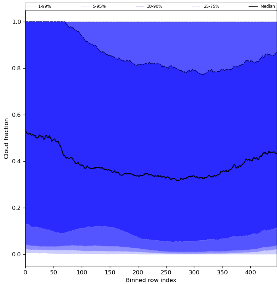
Figure 49: Along track statistics of “Cloud fraction” for 2023-10-22 to 2023-10-23
