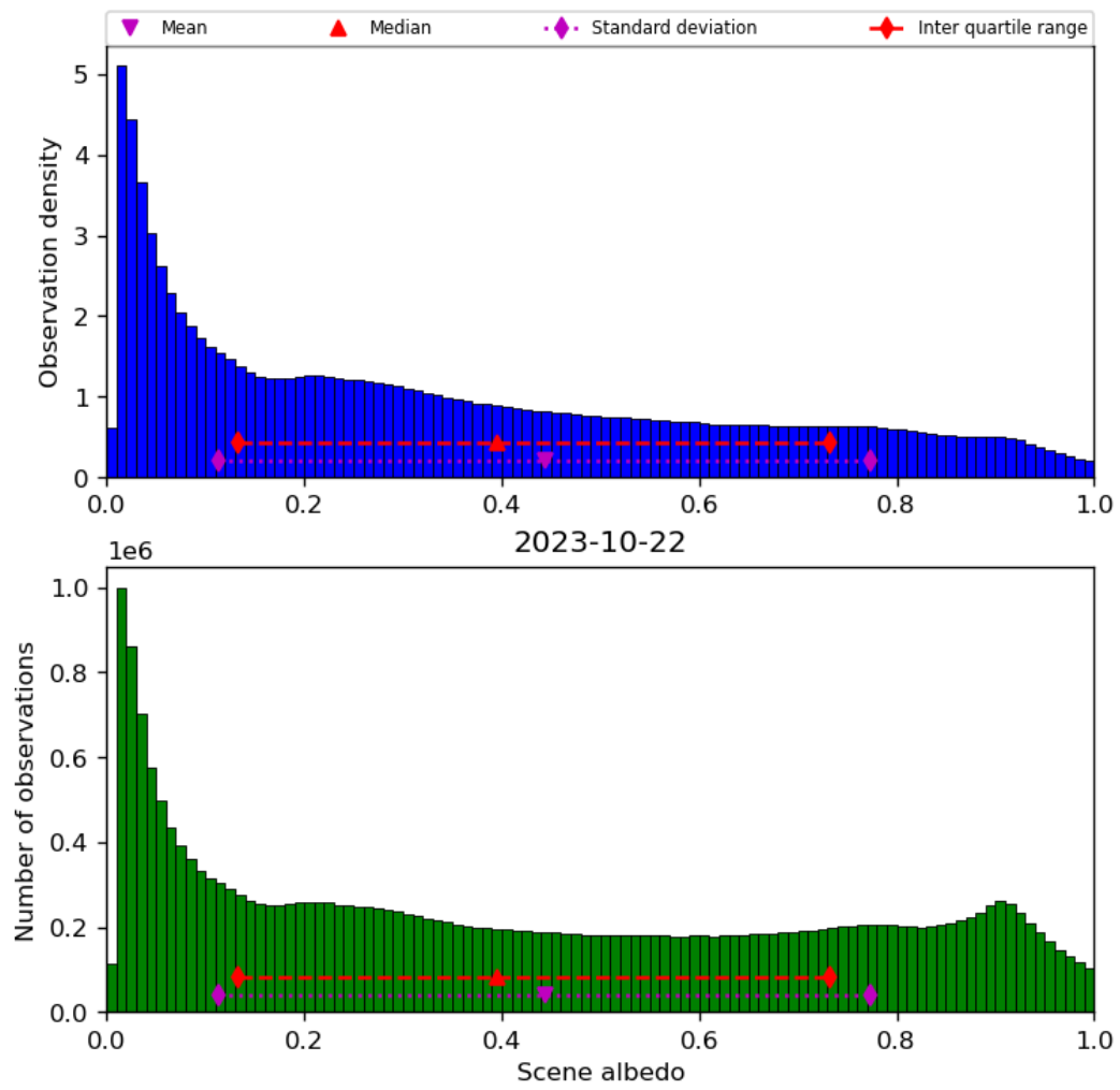
Figure 34: Histogram of “Scene albedo” for 2023-10-22 to 2023-10-23
