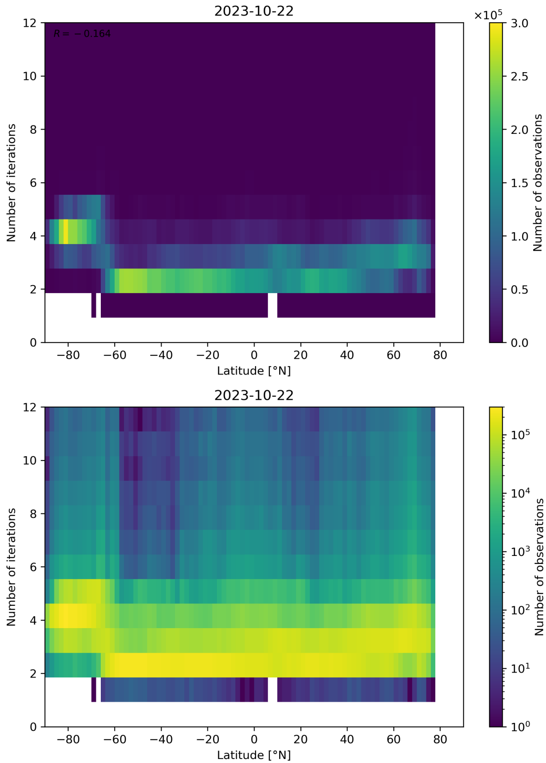
Figure 102: Scatter density plot of “Latitude” against “Number of iterations” for 2023-10-22 to 2023-10-23.
