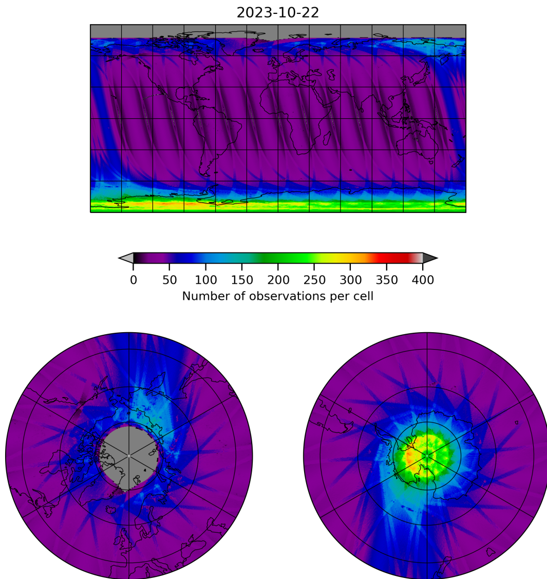
Figure 11: Map of the number of observations for 2023-10-22 to 2023-10-23
