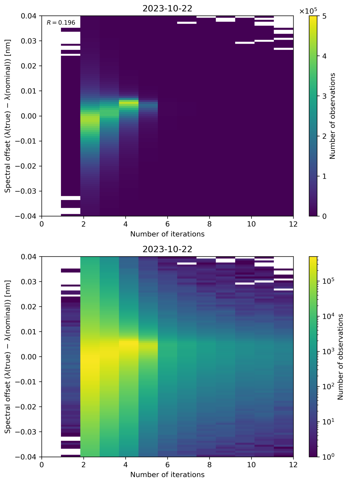
Figure 109: Scatter density plot of “Number of iterations” against “Spectral offset ( \lambda(\text{true}) - \lambda(\text{nominal}) )” for 2023-10-22 to 2023-10-23.
