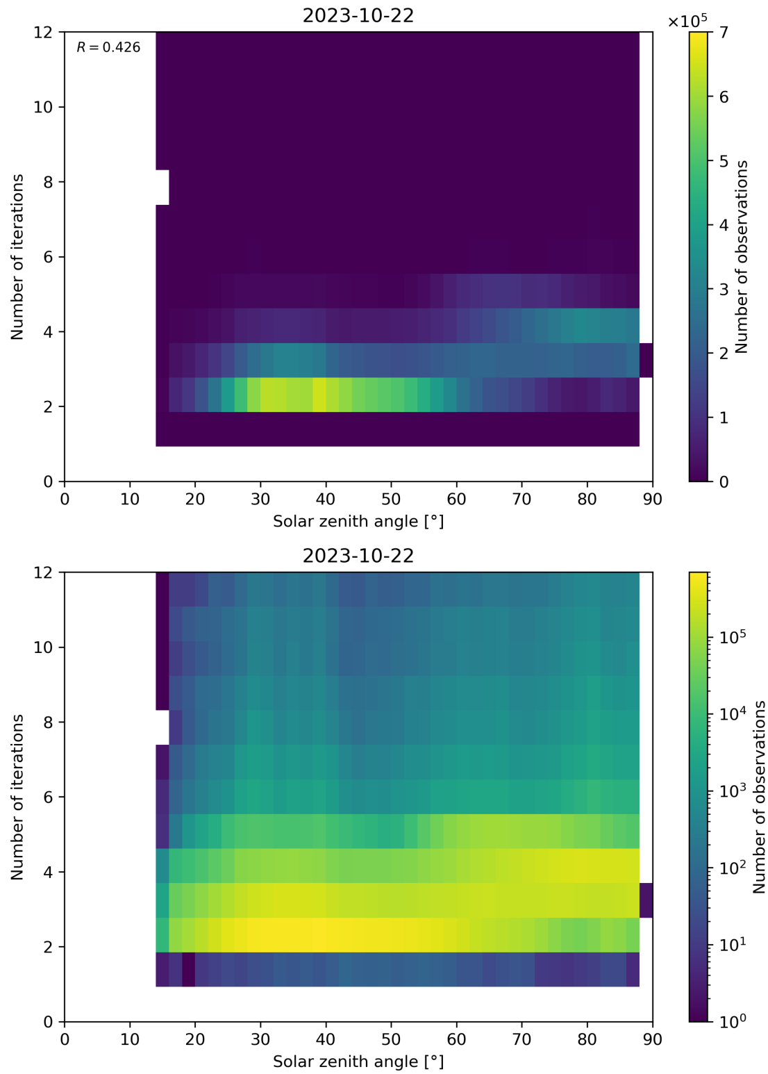
Figure 125: Scatter density plot of “Solar zenith angle” against “Number of iterations” for 2023-10-22 to 2023-10-23.
