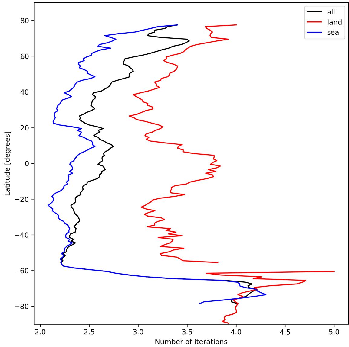
Figure 22: Zonal average of “Number of iterations” for 2023-10-22 to 2023-10-23.
