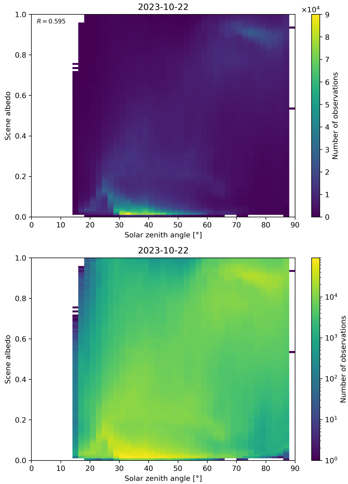
Figure 127: Scatter density plot of “Solar zenith angle” against “Scene albedo” for 2023-10-22 to 2023-10-23.
