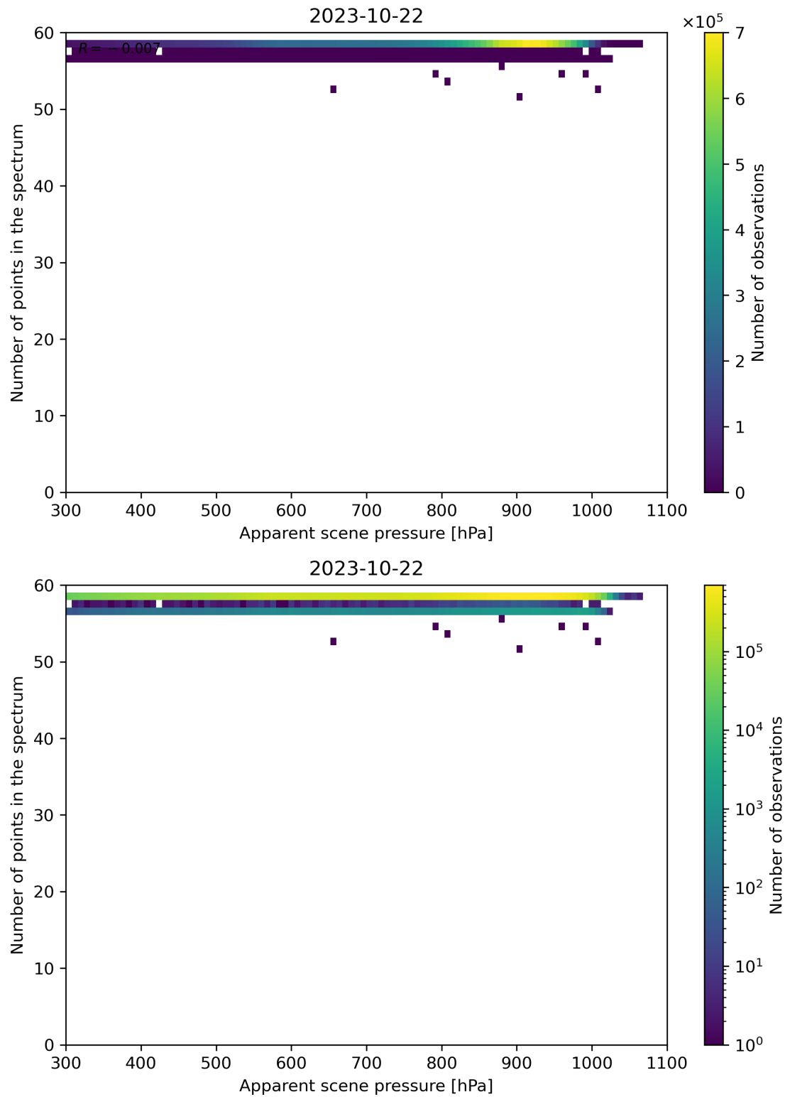
Figure 67: Scatter density plot of “Apparent scene pressure” against “Number of points in the spectrum” for 2023-10-22 to 2023-10-23.
