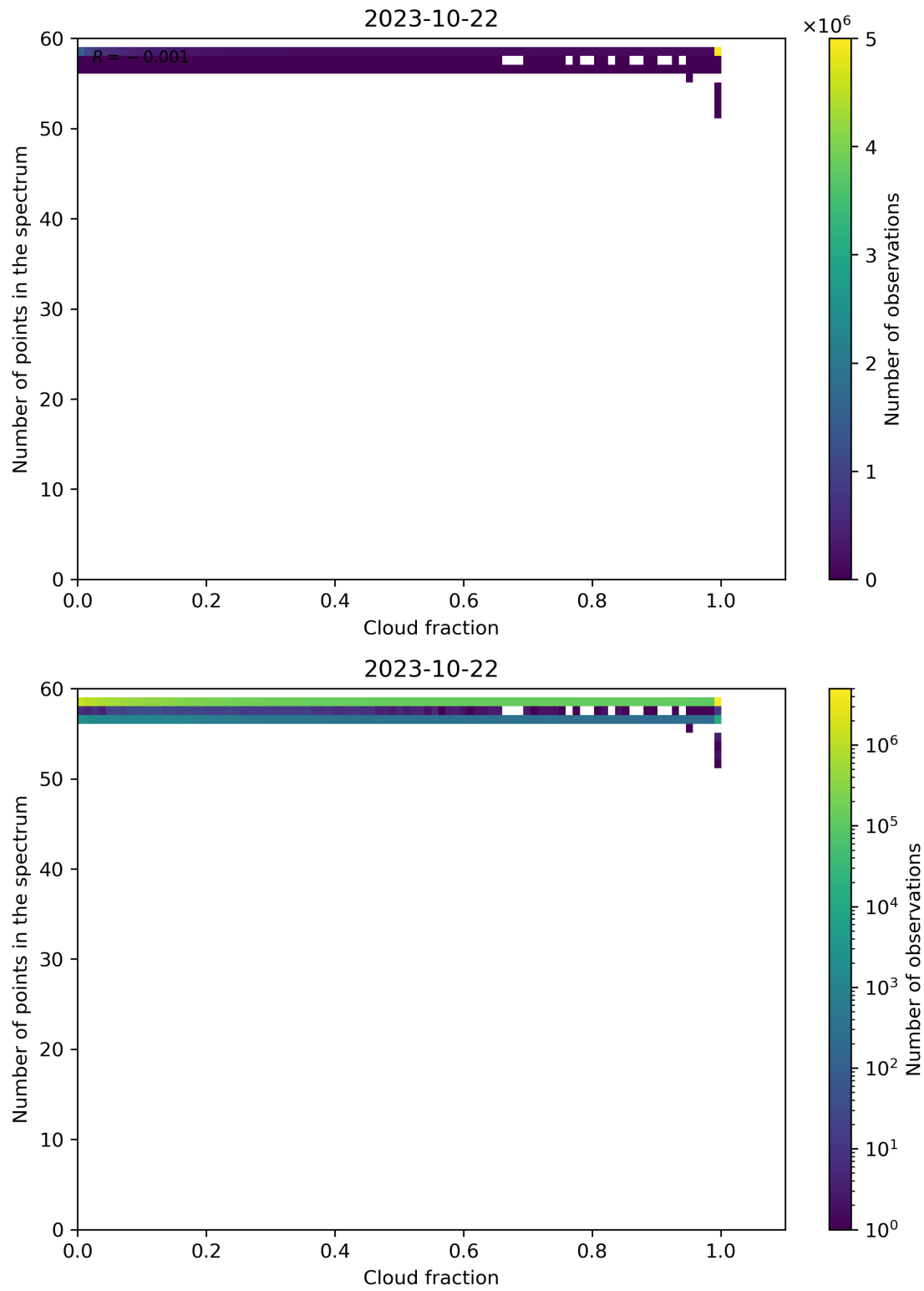
Figure 81: Scatter density plot of “Cloud fraction” against “Number of points in the spectrum” for 2023-10-22 to 2023-10-23.
