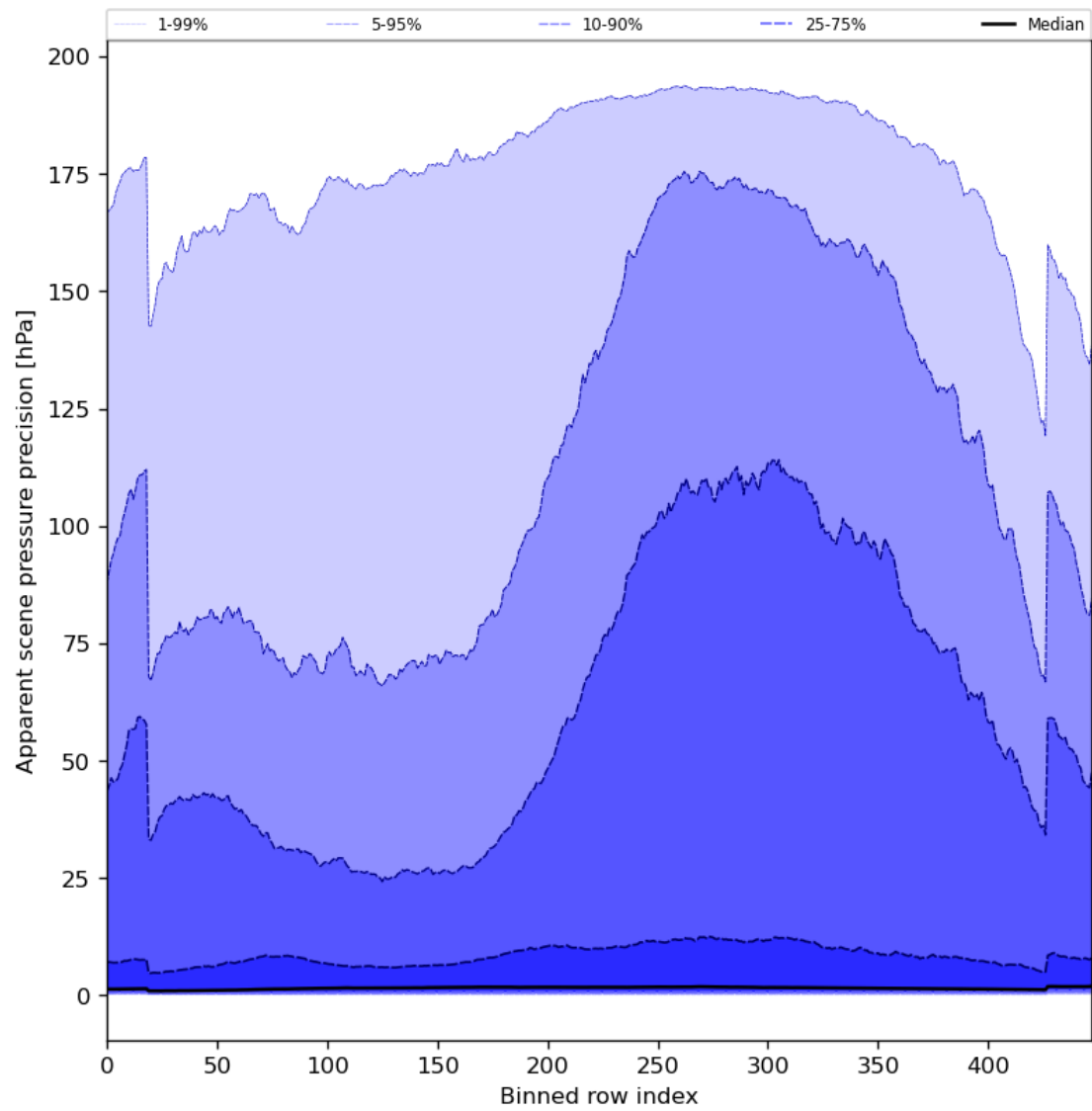
Figure 54: Along track statistics of “Apparent scene pressure precision” for 2023-10-22 to 2023-10-23
