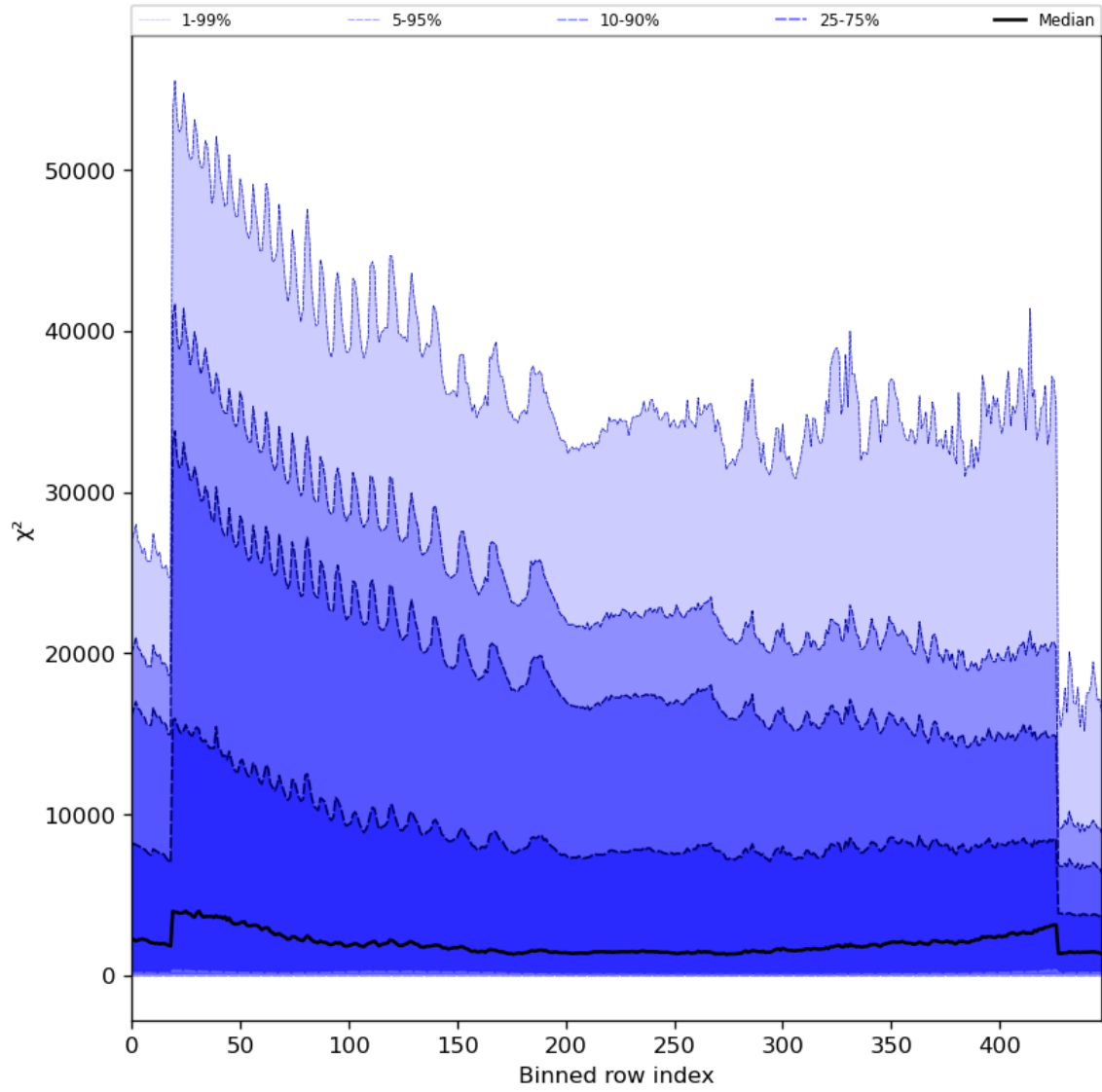
Figure 55: Along track statistics of “ \chi^2 ” for 2023-10-22 to 2023-10-23
