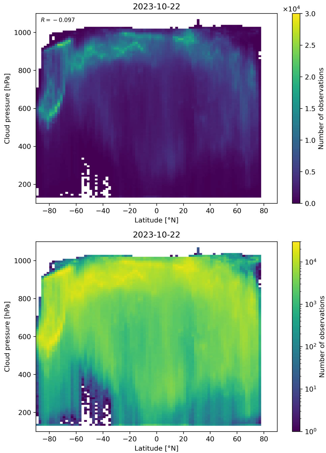
Figure 100: Scatter density plot of “Latitude” against “Cloud pressure” for 2023-10-22 to 2023-10-23.
