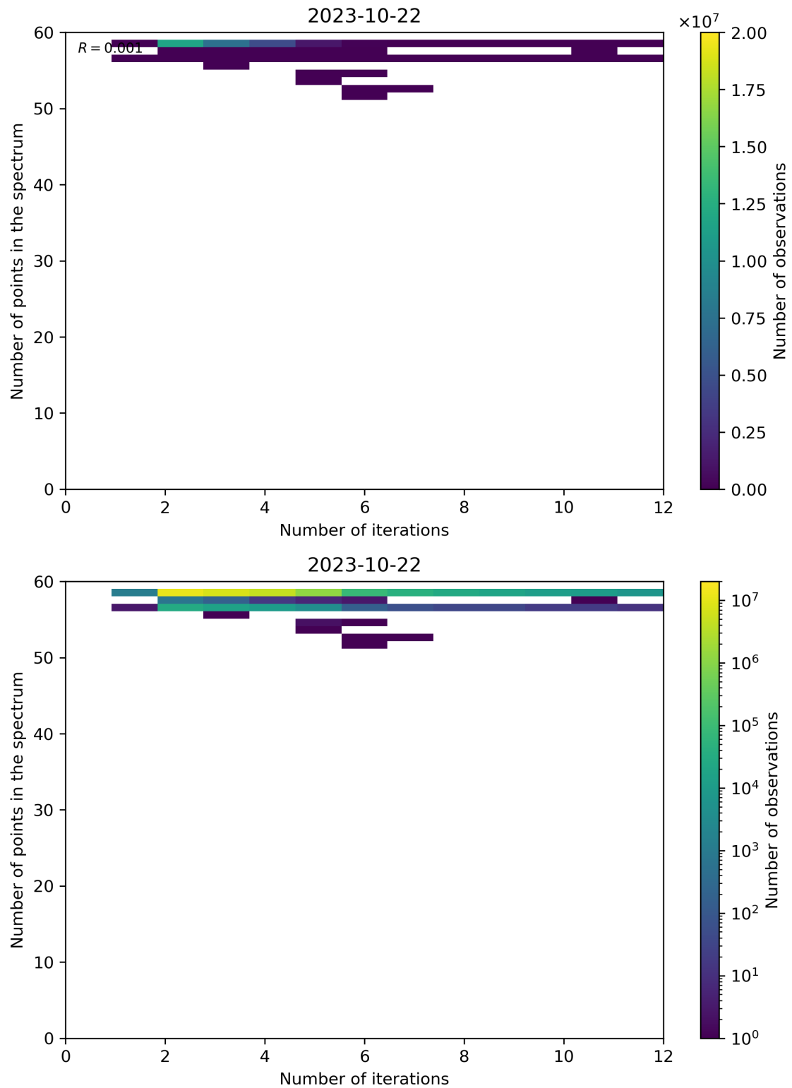
Figure 108: Scatter density plot of “Number of iterations” against “Number of points in the spectrum” for 2023-10-22 to 2023-10-23.
