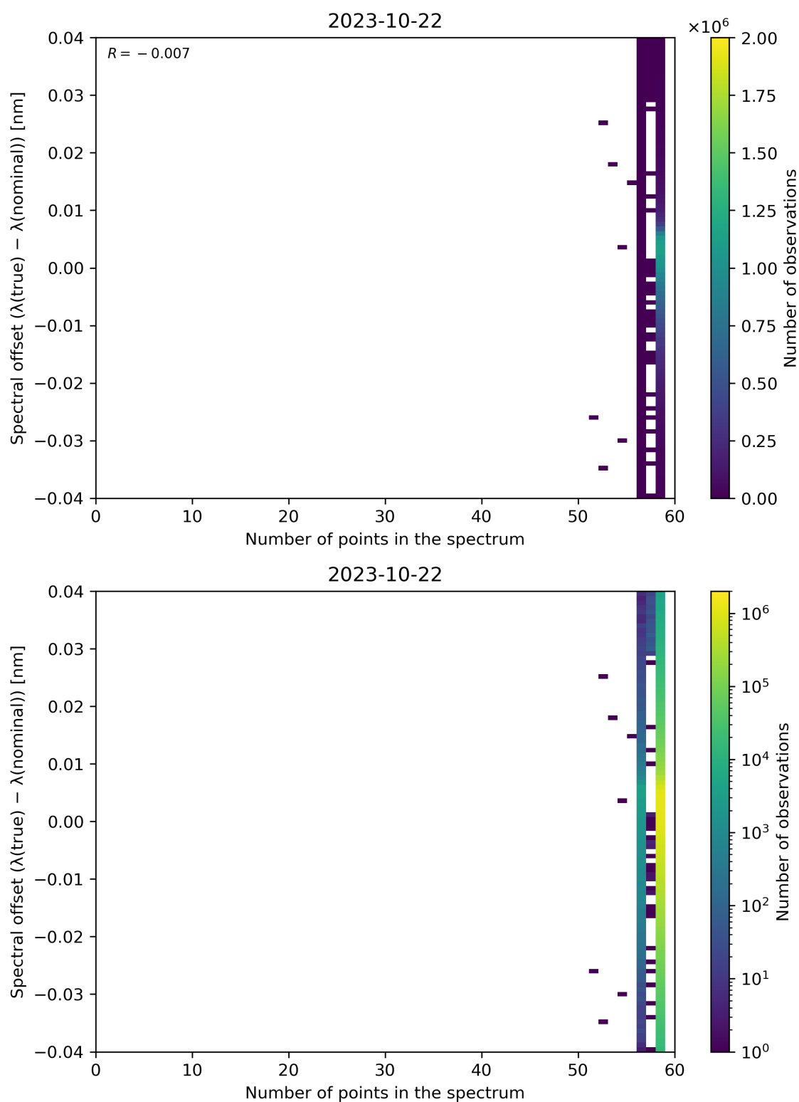
Figure 110: Scatter density plot of “Number of points in the spectrum” against “Spectral offset ( \lambda(\text{true}) - \lambda(\text{nominal}) )” for 2023-10-22 to 2023-10-23.
