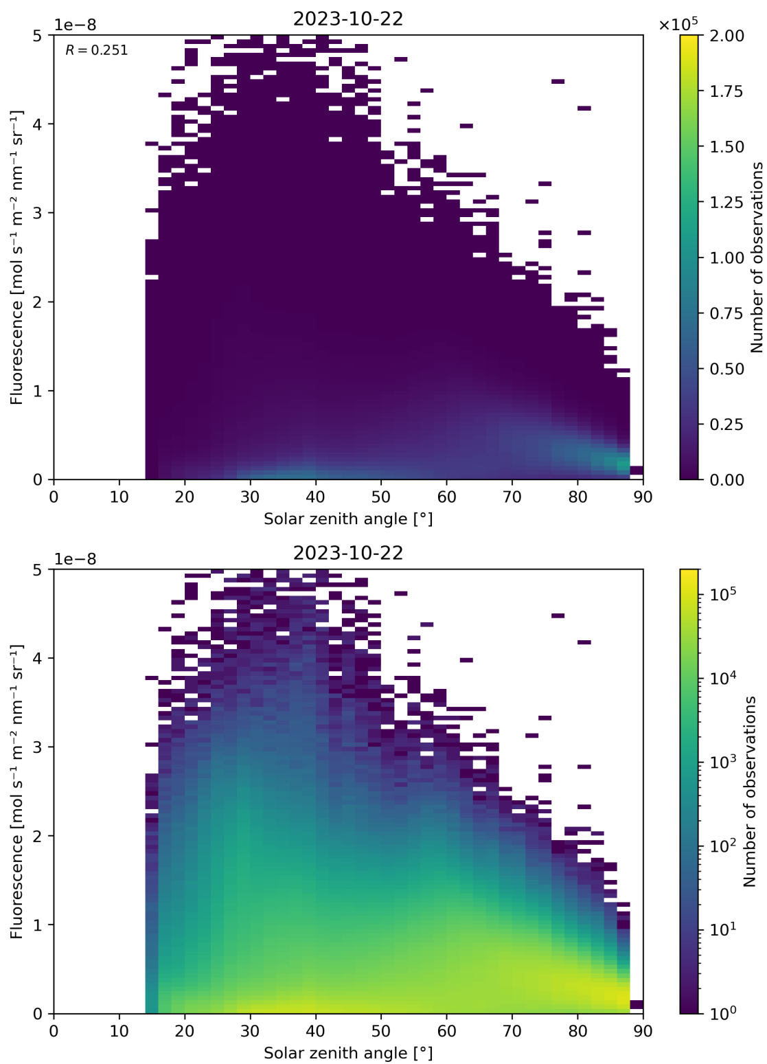
Figure 123: Scatter density plot of “Solar zenith angle” against “Fluorescence” for 2023-10-22 to 2023-10-23.
