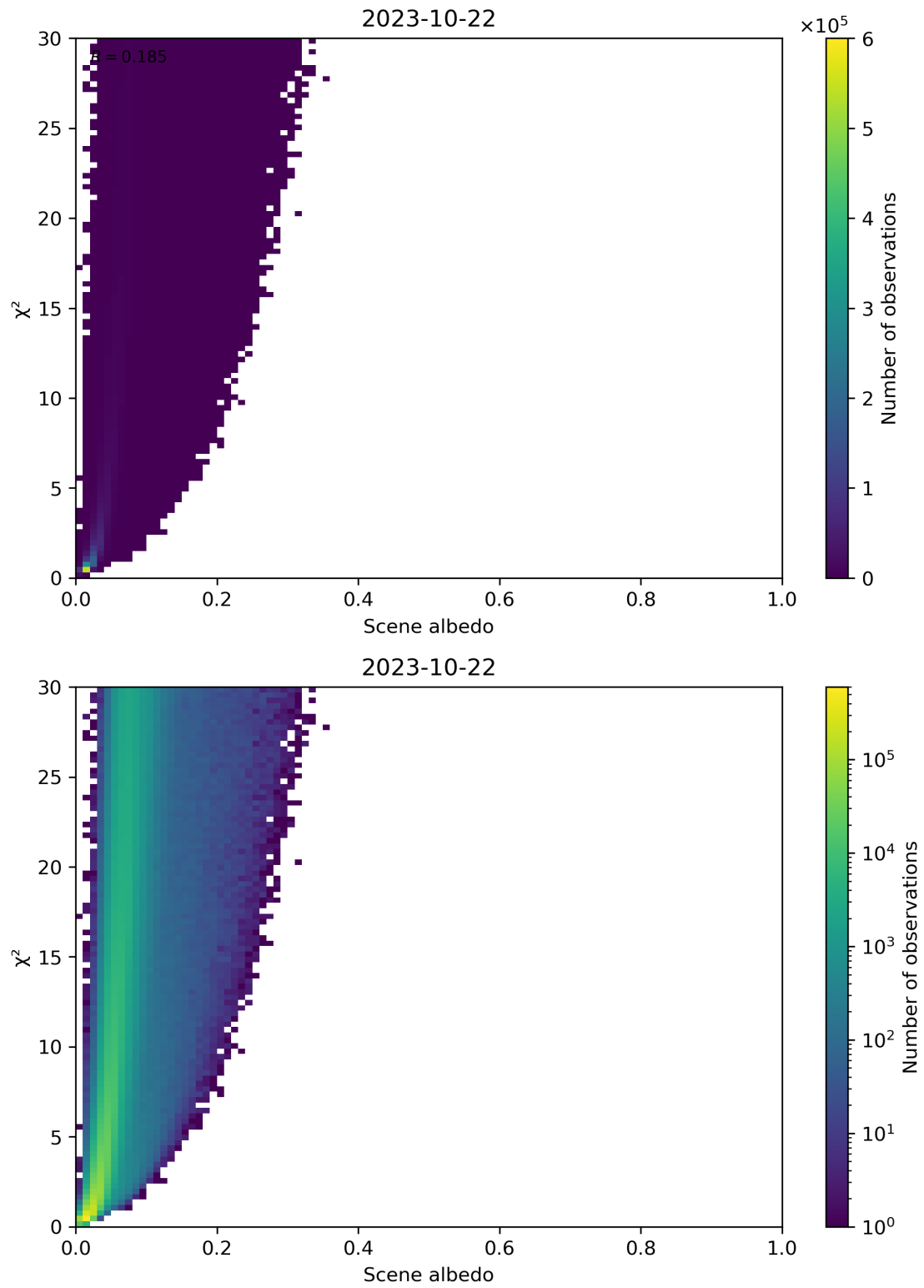
Figure 112: Scatter density plot of “Scene albedo” against “ \chi^2 ” for 2023-10-22 to 2023-10-23.
