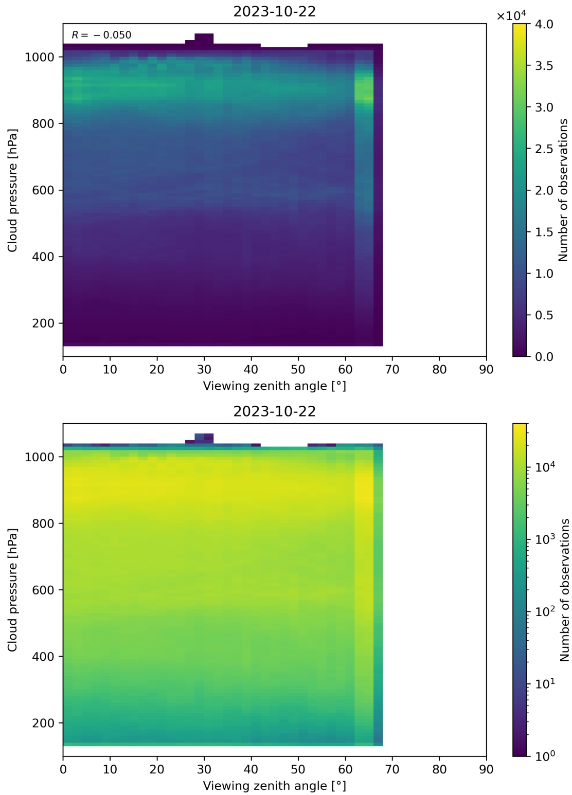
Figure 133: Scatter density plot of “Viewing zenith angle” against “Cloud pressure” for 2023-10-22 to 2023-10-23.
