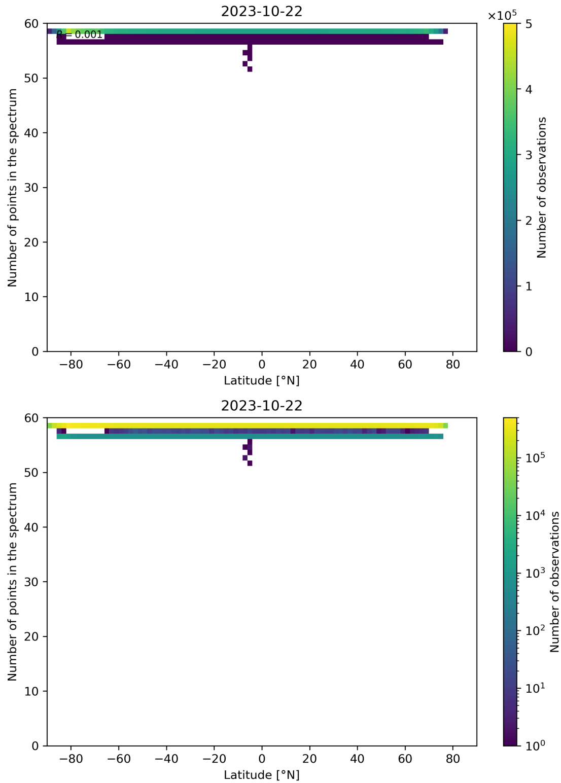
Figure 103: Scatter density plot of “Latitude” against “Number of points in the spectrum” for 2023-10-22 to 2023-10-23.
