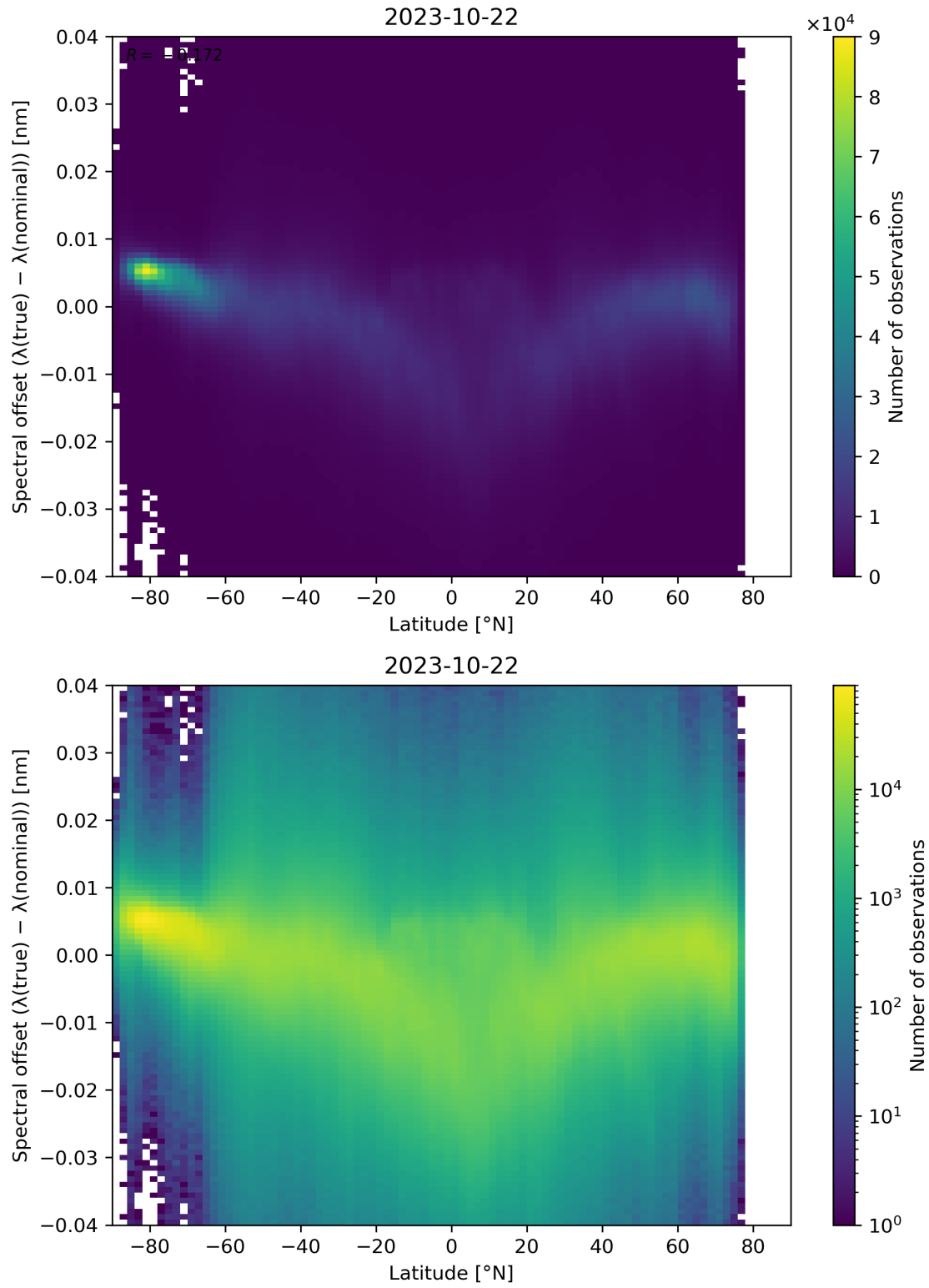
Figure 105: Scatter density plot of “Latitude” against “Spectral offset ( \lambda(\text{true}) - \lambda(\text{nominal}) )” for 2023-10-22 to 2023-10-23.
