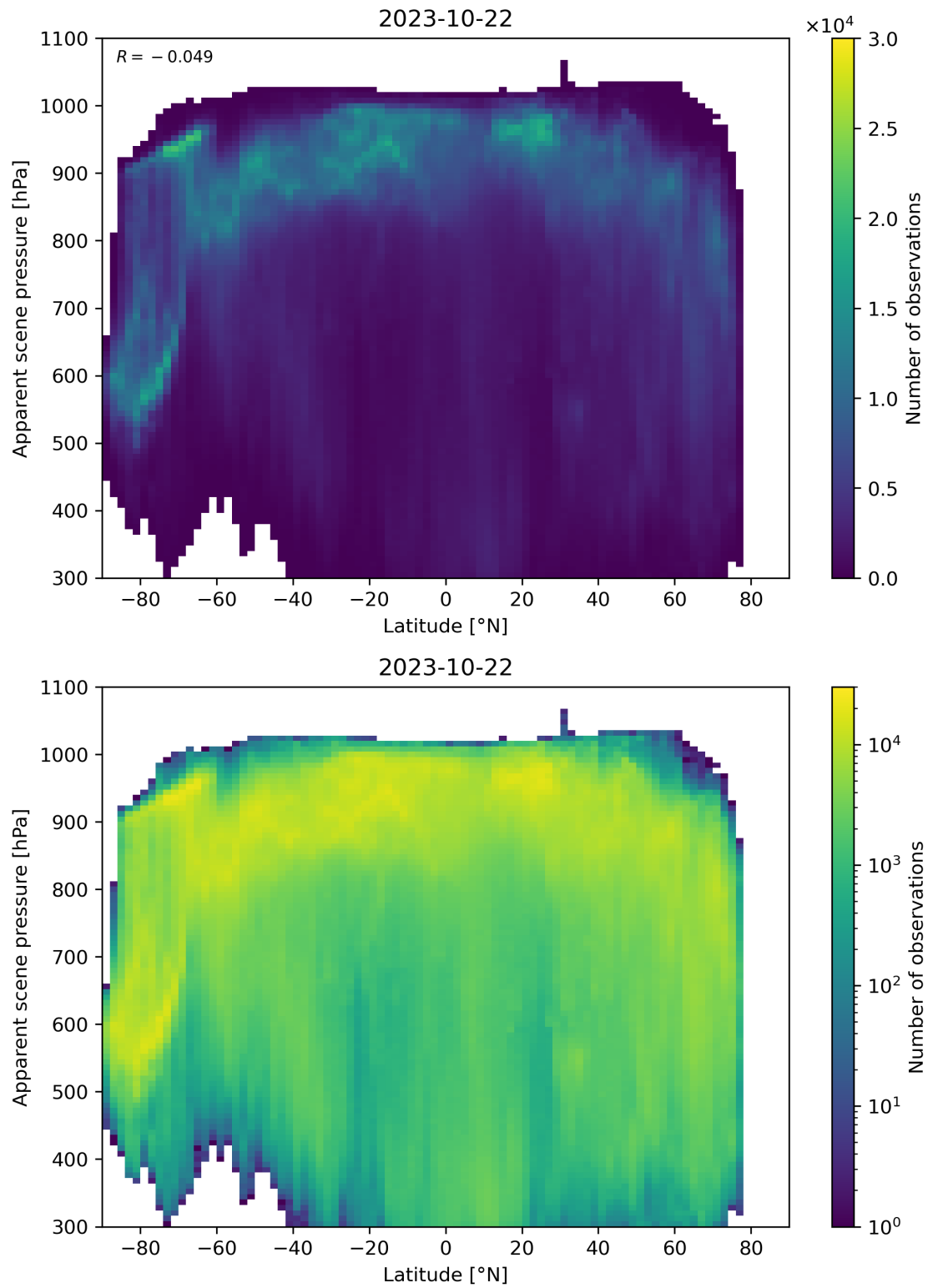
Figure 96: Scatter density plot of “Latitude” against “Apparent scene pressure” for 2023-10-22 to 2023-10-23.
