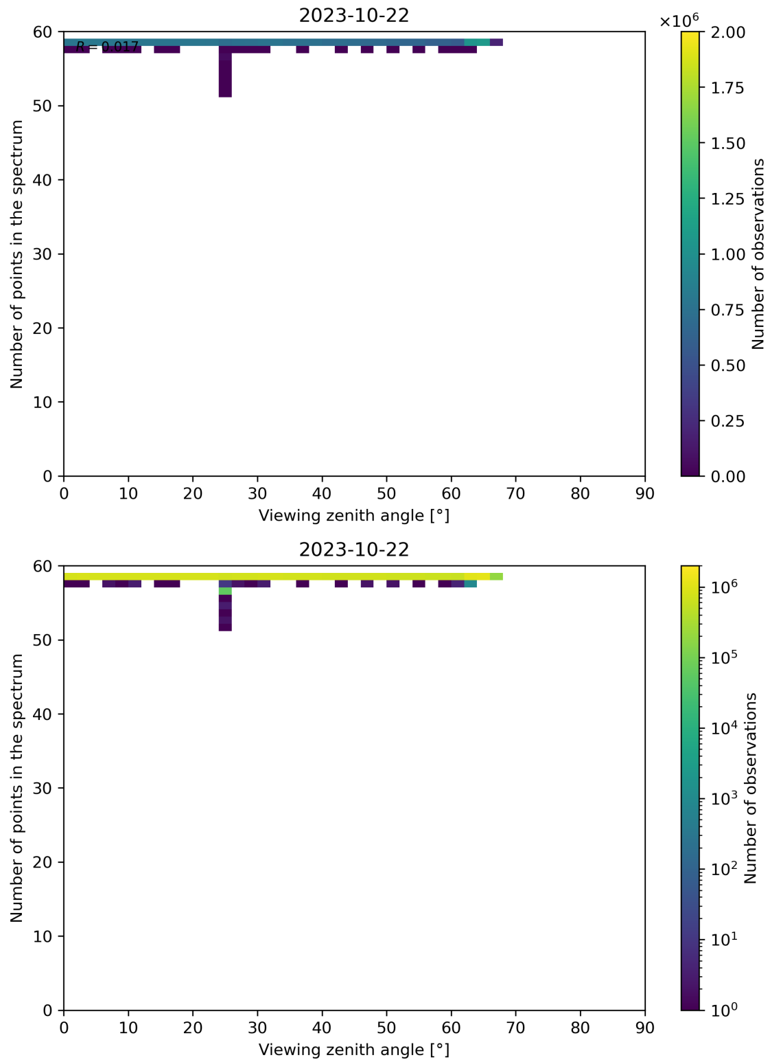
Figure 137: Scatter density plot of “Viewing zenith angle” against “Number of points in the spectrum” for 2023-10-22 to 2023-10-23.
