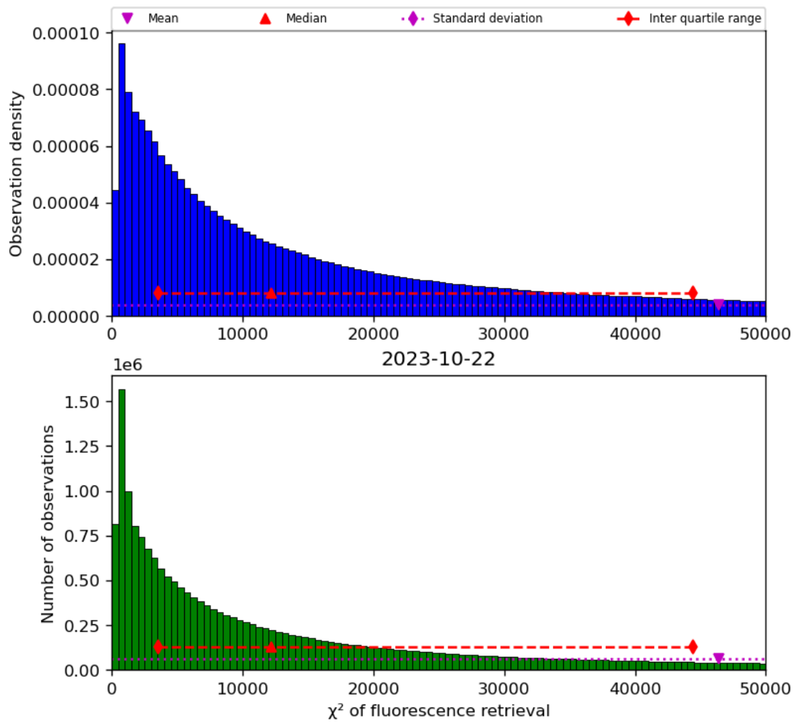
Figure 42: Histogram of “ \chi^2 of fluorescence retrieval” for 2023-10-22 to 2023-10-23
