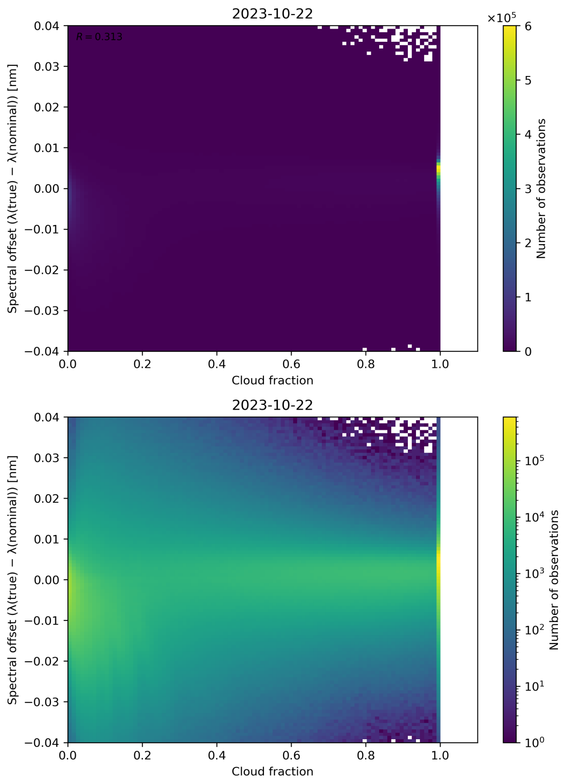
Figure 83: Scatter density plot of “Cloud fraction” against “Spectral offset ( \lambda(\text{true}) - \lambda(\text{nominal}) )” for 2023-10-22 to 2023-10-23.
