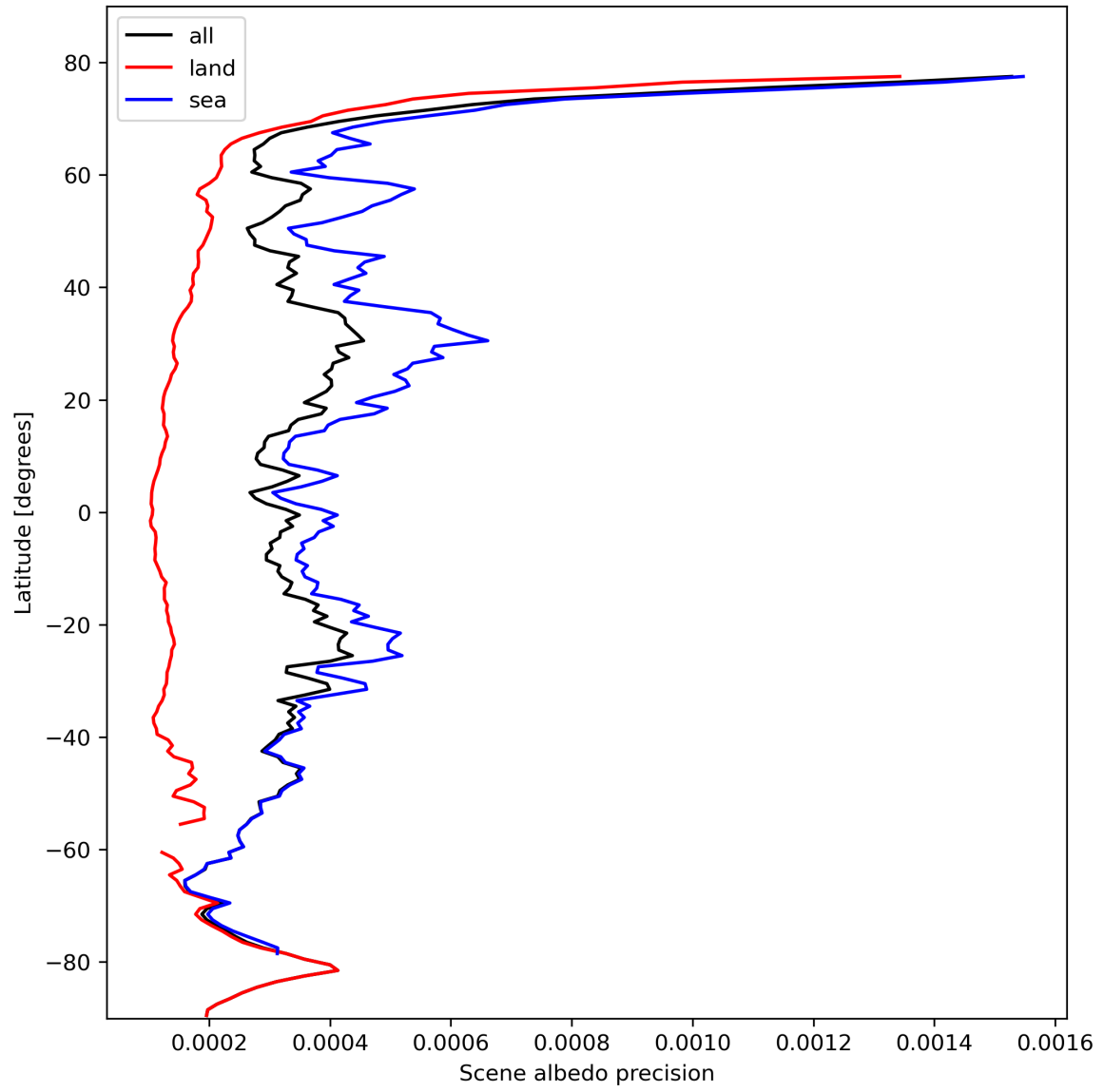
Figure 18: Zonal average of "Scene albedo precision" for 2023-10-22 to 2023-10-23.
