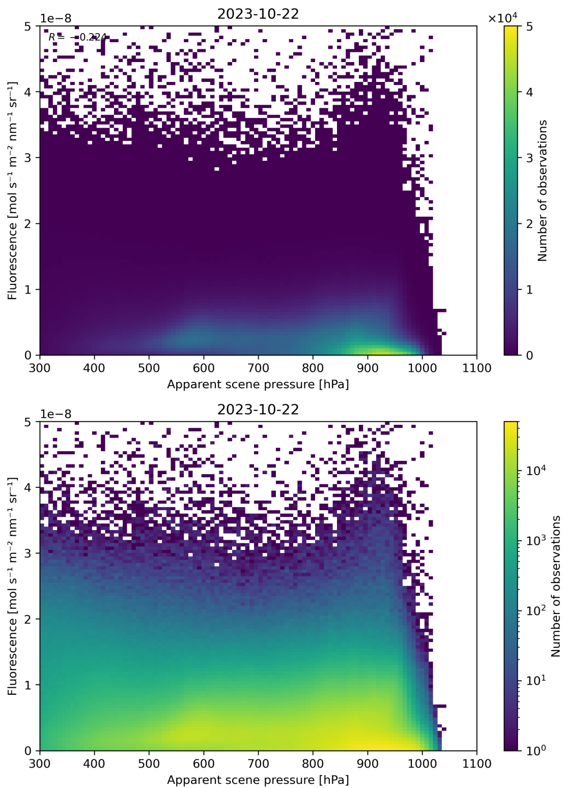
Figure 65: Scatter density plot of “Apparent scene pressure” against “Fluorescence” for 2023-10-22 to 2023-10-23.
