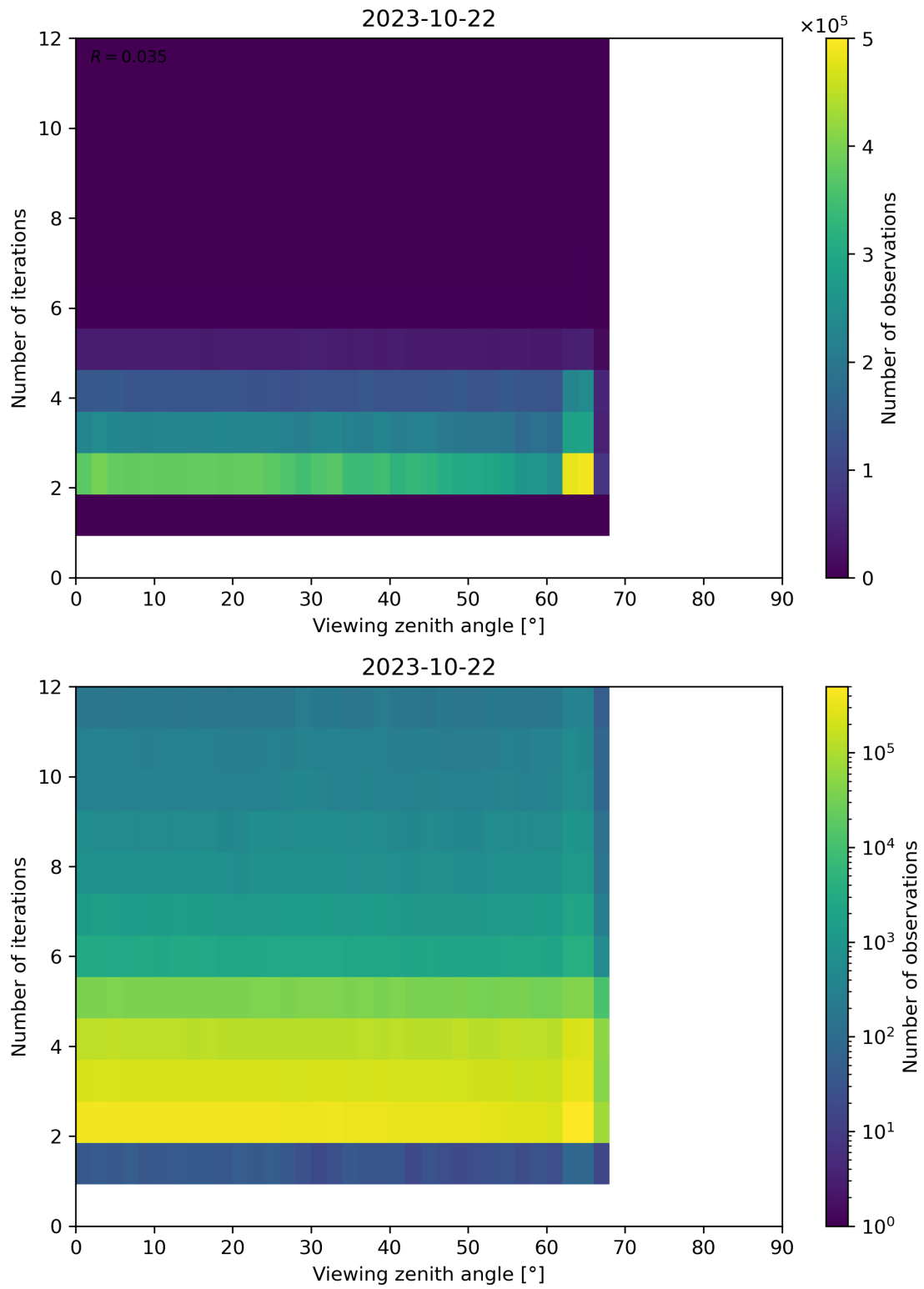
Figure 136: Scatter density plot of “Viewing zenith angle” against “Number of iterations” for 2023-10-22 to 2023-10-23.
