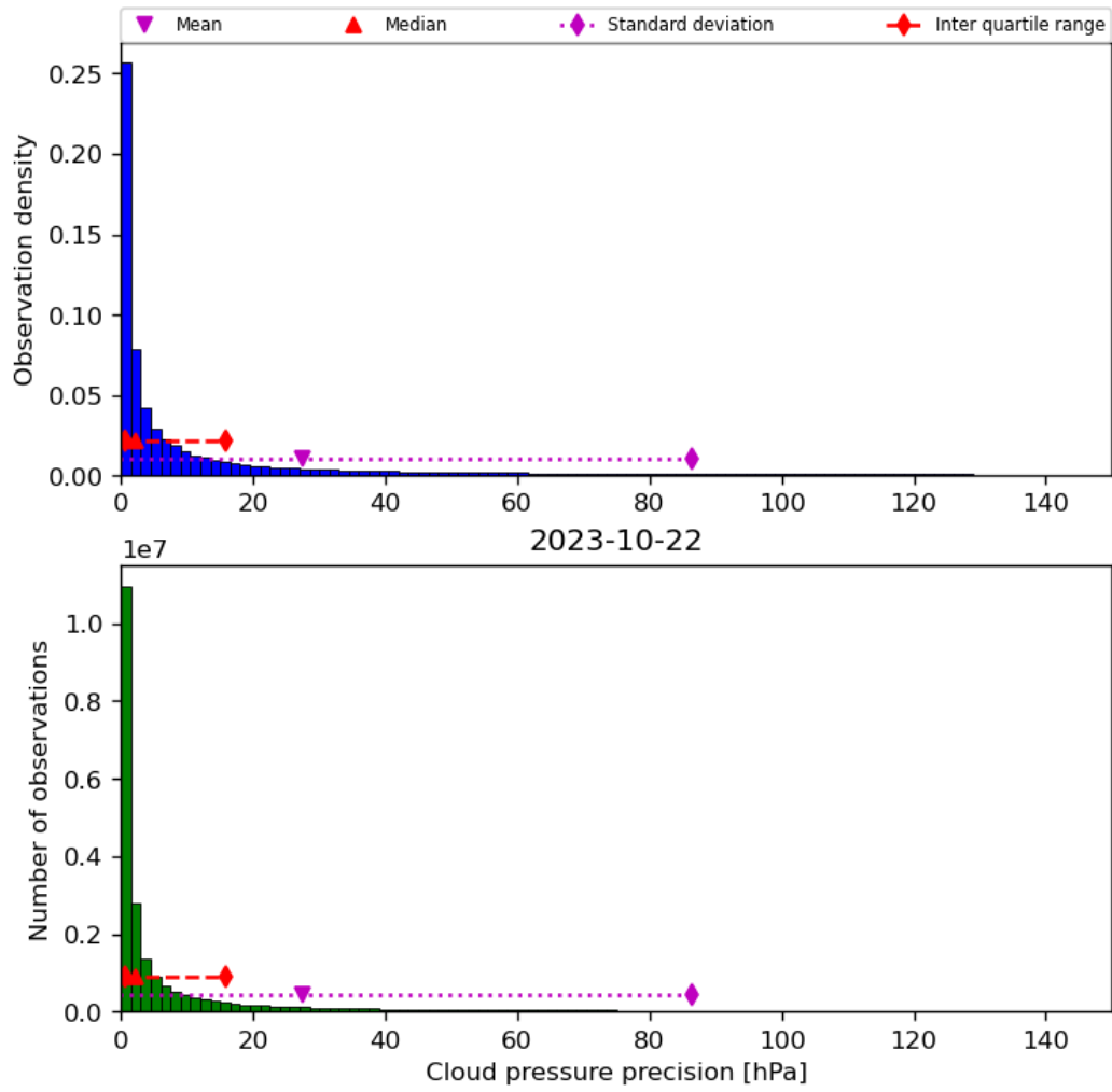
Figure 31: Histogram of “Cloud pressure precision” for 2023-10-22 to 2023-10-23
