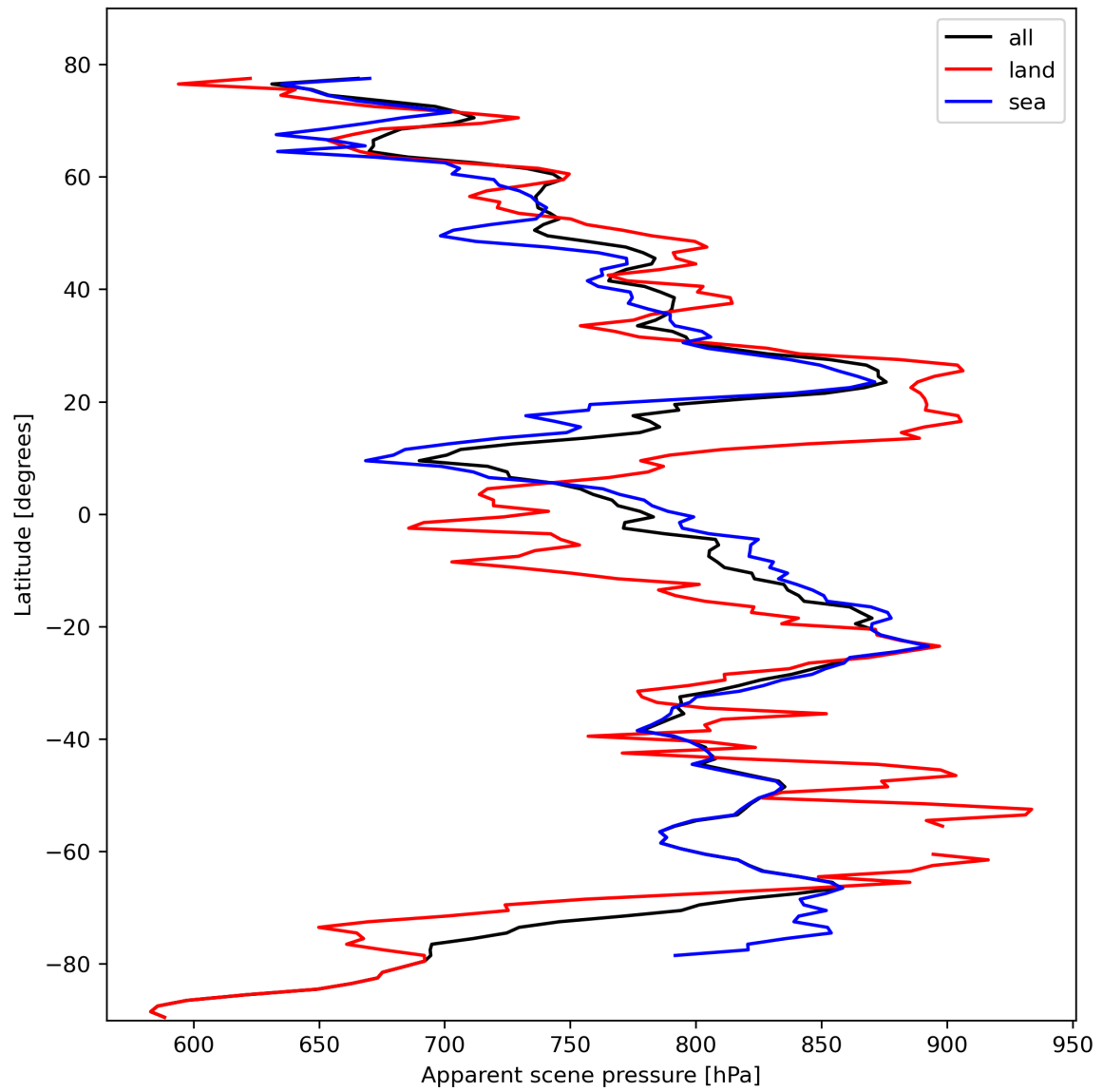
Figure 19: Zonal average of “Apparent scene pressure” for 2023-10-22 to 2023-10-23.
