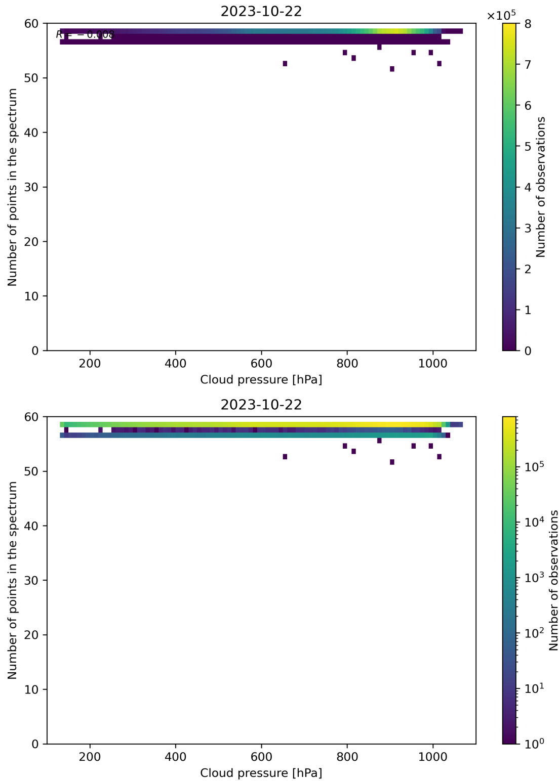
Figure 90: Scatter density plot of “Cloud pressure” against “Number of points in the spectrum” for 2023-10-22 to 2023-10-23.
