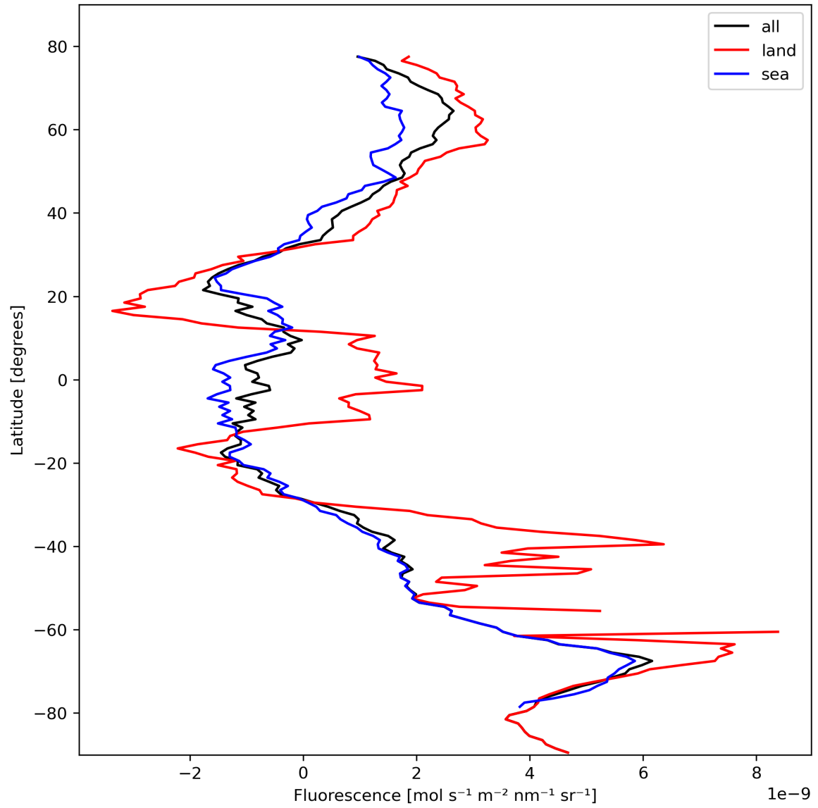
Figure 23: Zonal average of “Fluorescence” for 2023-10-22 to 2023-10-23.
