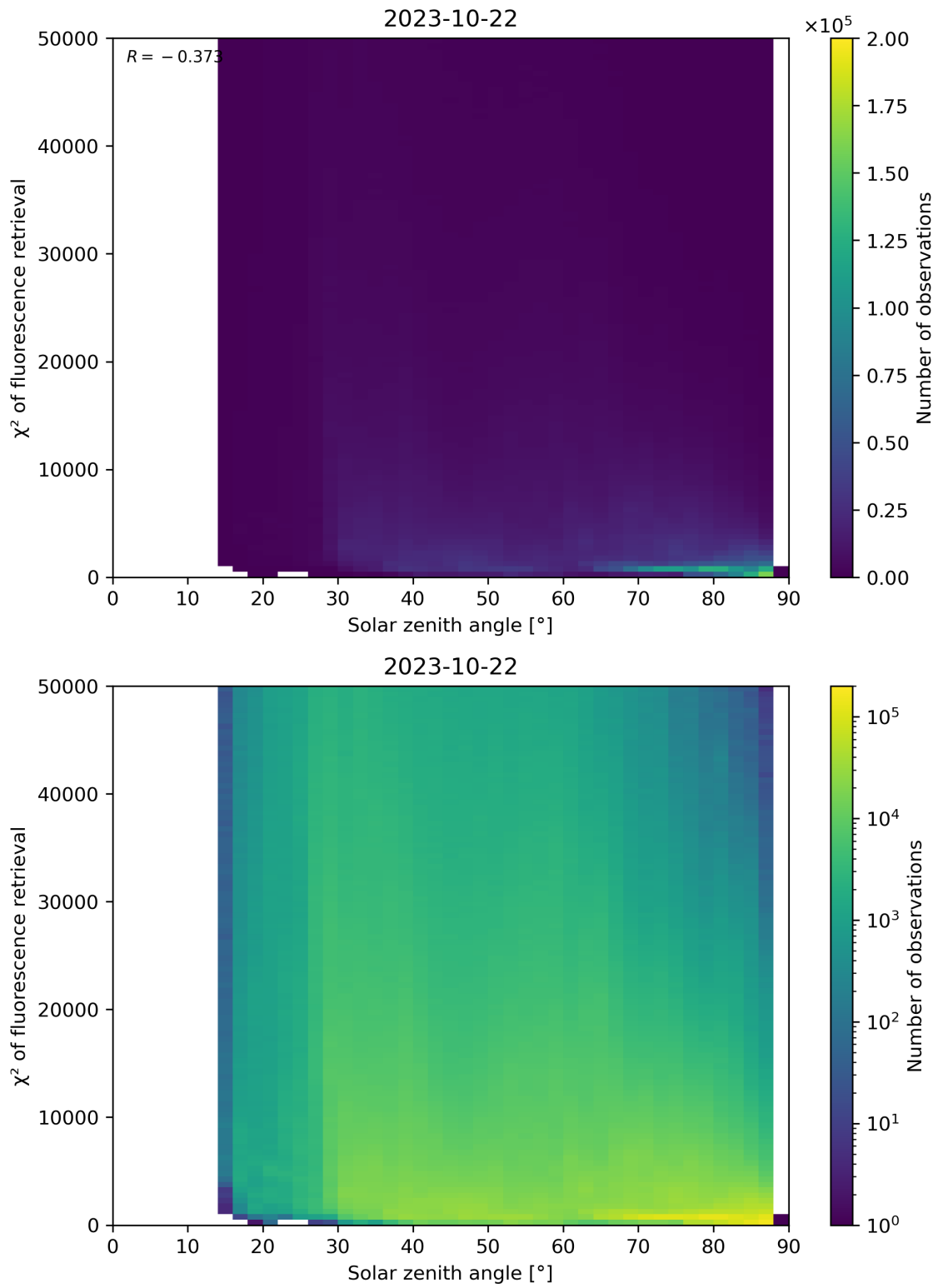
Figure 120: Scatter density plot of “Solar zenith angle” against “ \chi^2 of fluorescence retrieval” for 2023-10-22 to 2023-10-23.
