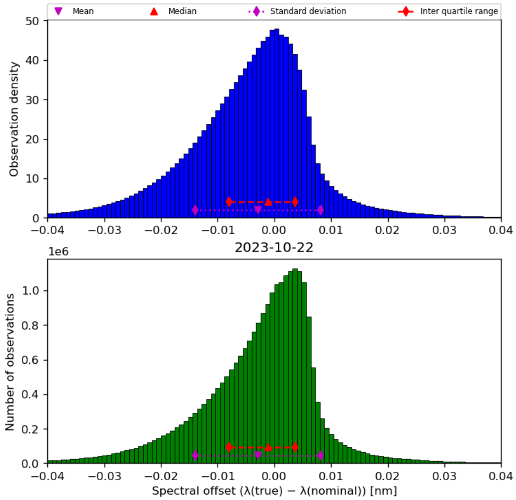
Figure 45: Histogram of “Spectral offset ( \lambda(\text{true}) - \lambda(\text{nominal}) )” for 2023-10-22 to 2023-10-23
