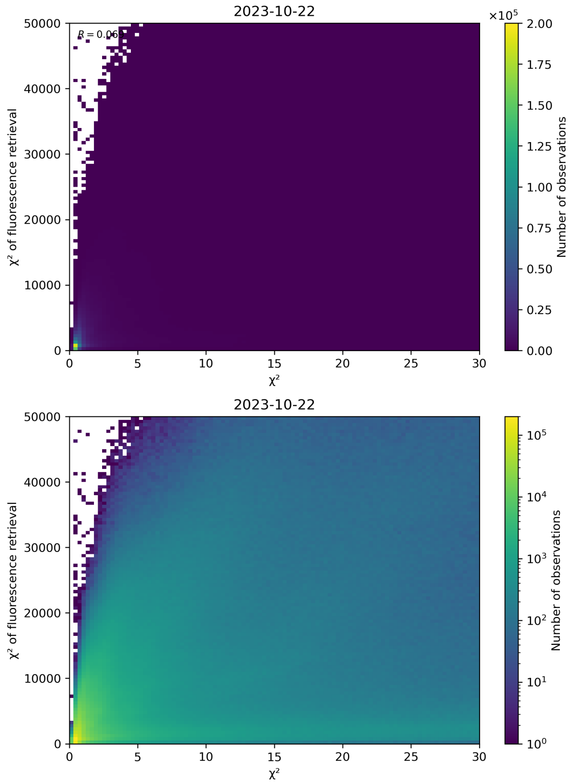
Figure 69: Scatter density plot of “ \chi^2 ” against “ \chi^2 of fluorescence retrieval” for 2023-10-22 to 2023-10-23.
