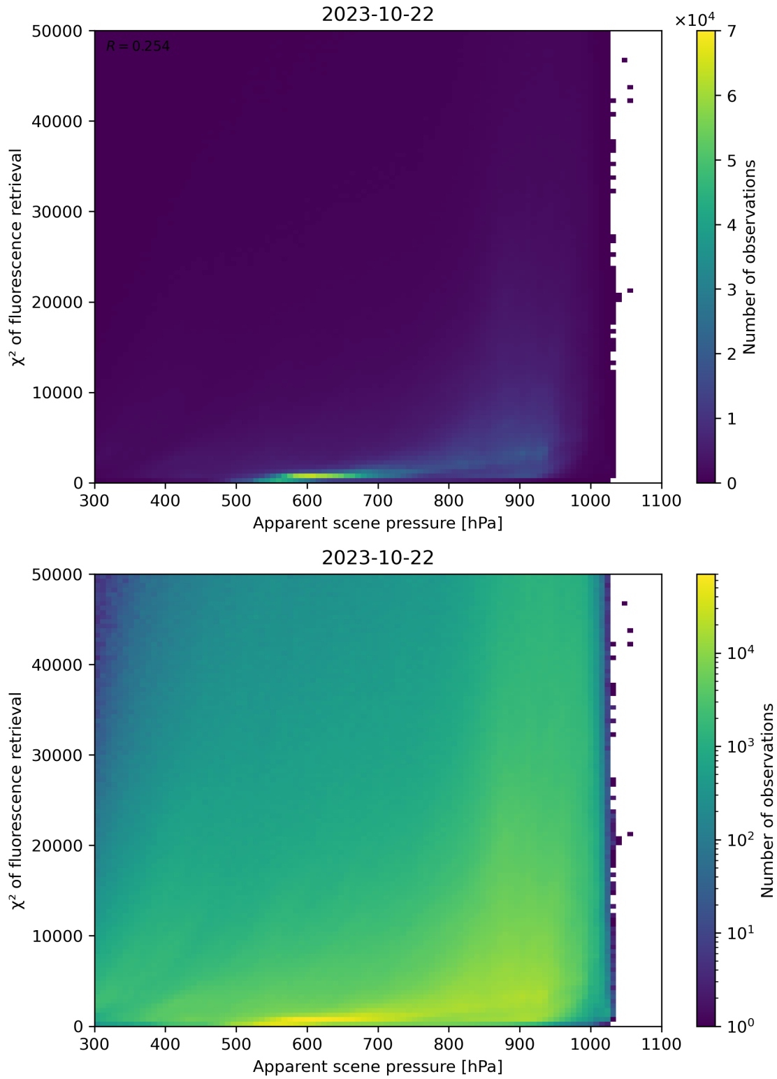
Figure 64: Scatter density plot of “Apparent scene pressure” against “ \chi^2 of fluorescence retrieval” for 2023-10-22 to 2023-10-23.
