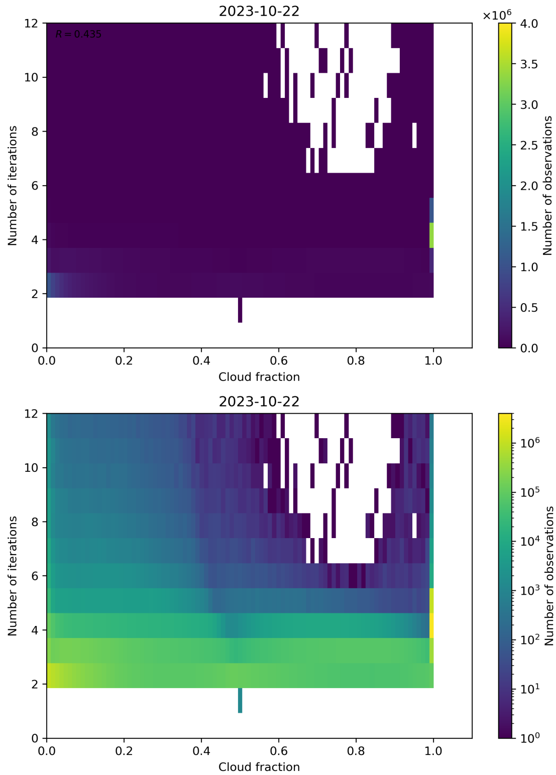
Figure 80: Scatter density plot of “Cloud fraction” against “Number of iterations” for 2023-10-22 to 2023-10-23.
