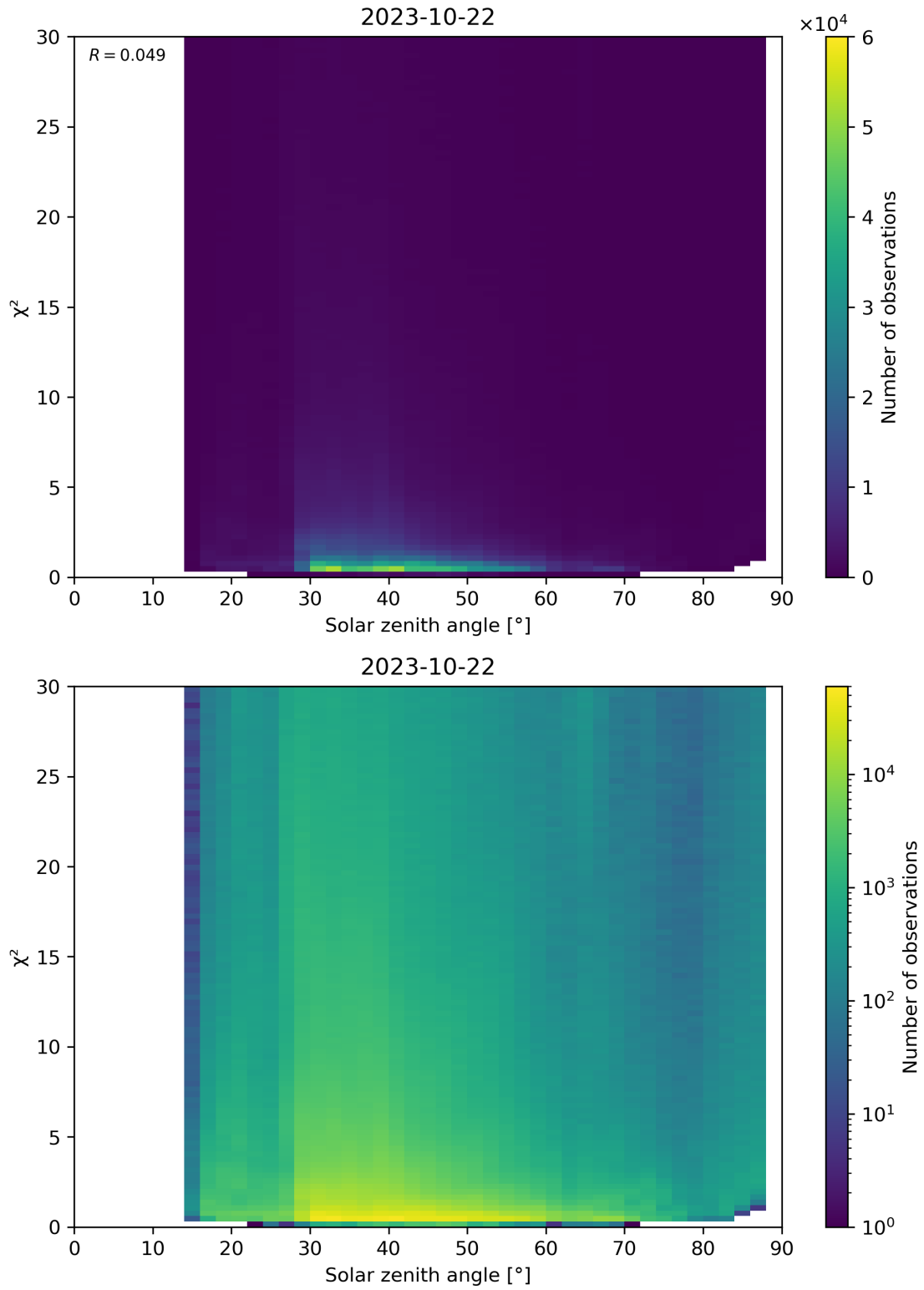
Figure 119: Scatter density plot of “Solar zenith angle” against “ \chi^2 ” for 2023-10-22 to 2023-10-23.
