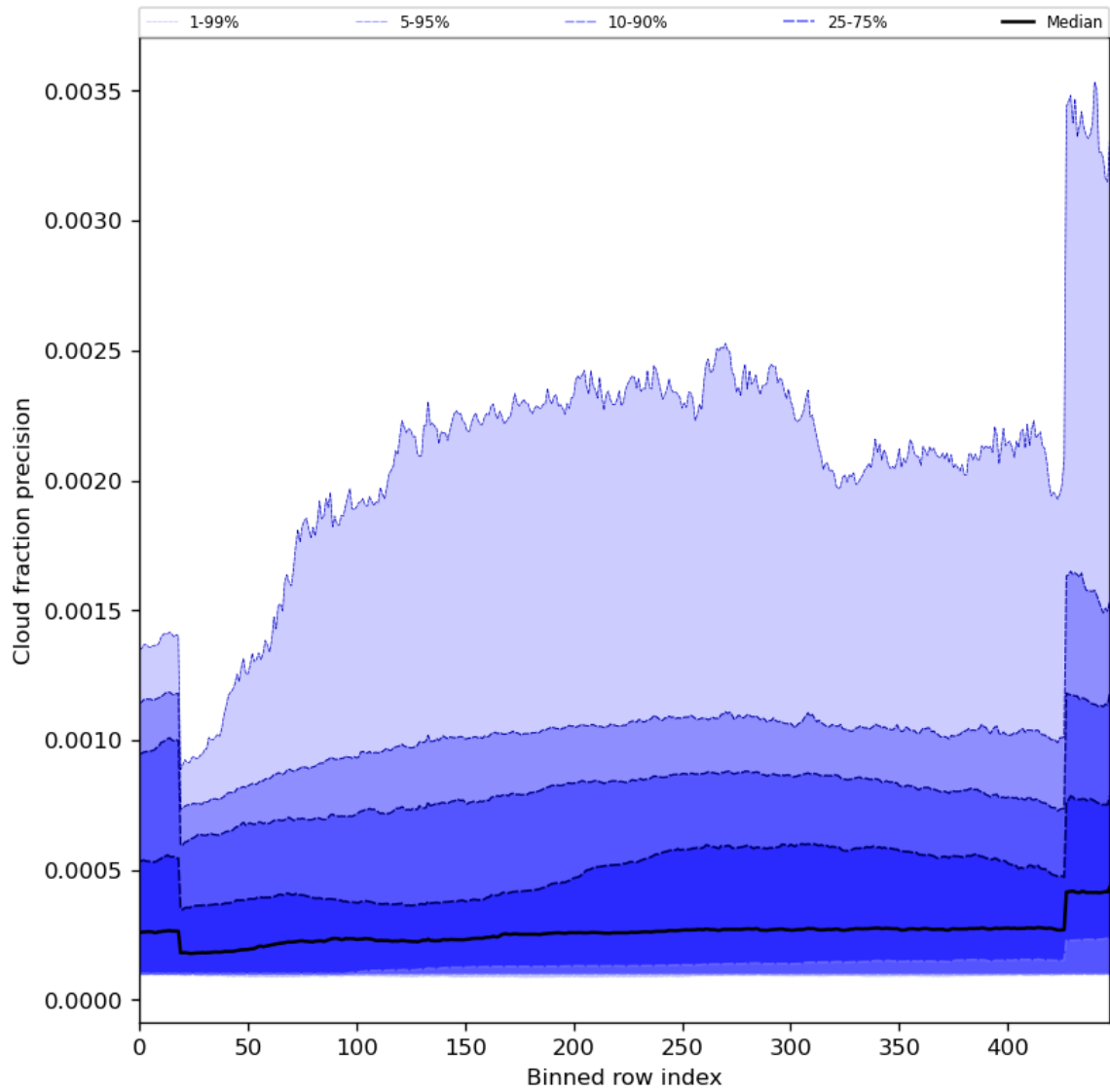
Figure 50: Along track statistics of “Cloud fraction precision” for 2023-10-22 to 2023-10-23
