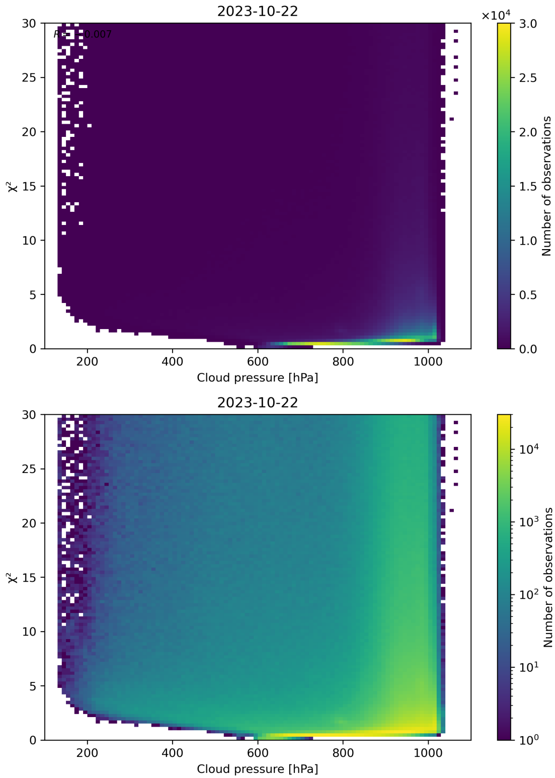
Figure 85: Scatter density plot of “Cloud pressure” against “ \chi^2 ” for 2023-10-22 to 2023-10-23.
