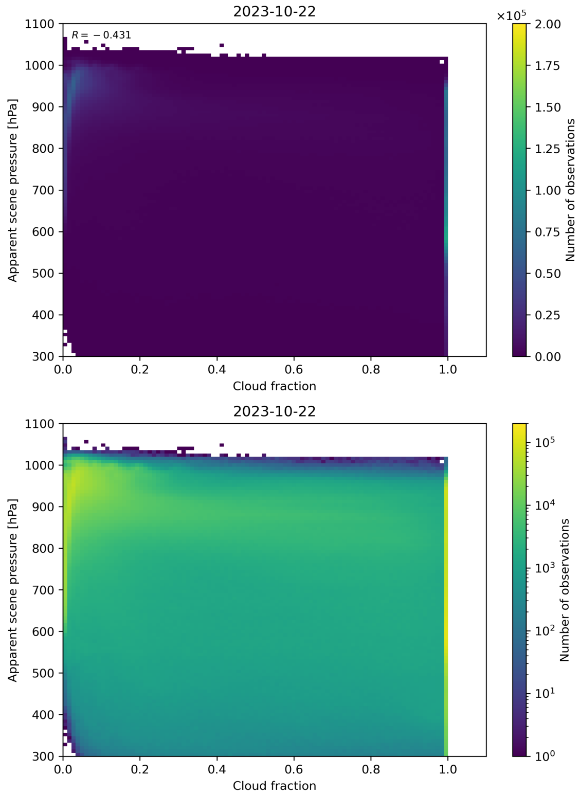
Figure 76: Scatter density plot of “Cloud fraction” against “Apparent scene pressure” for 2023-10-22 to 2023-10-23.
