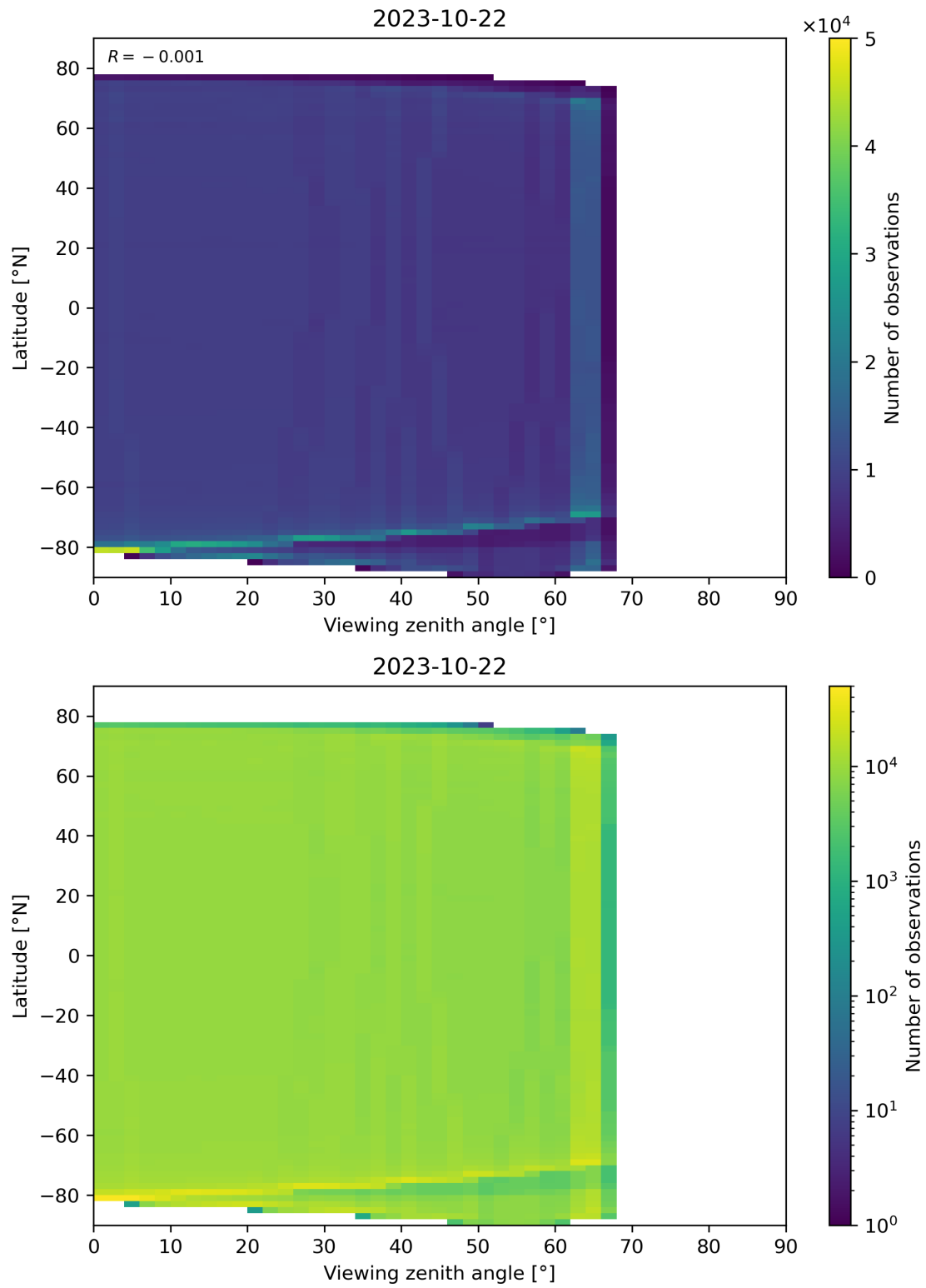
Figure 135: Scatter density plot of “Viewing zenith angle” against “Latitude” for 2023-10-22 to 2023-10-23.
