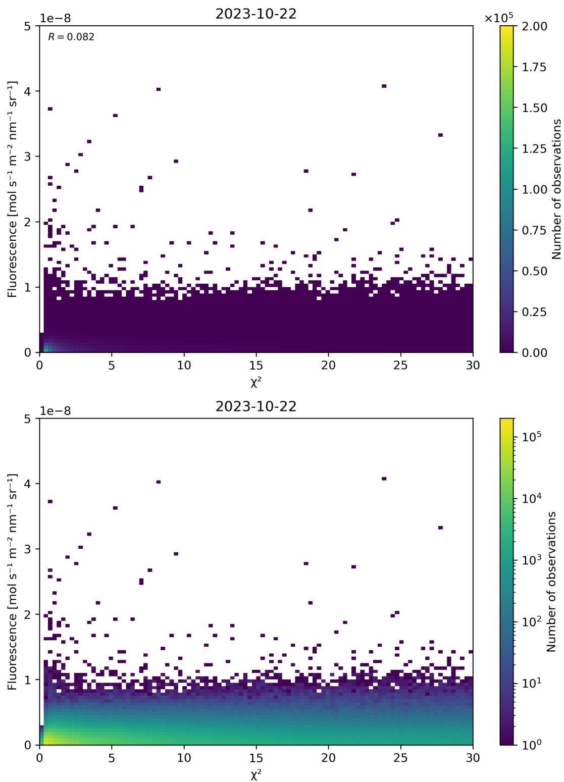
Figure 70: Scatter density plot of “ \chi^2 ” against “Fluorescence” for 2023-10-22 to 2023-10-23.
