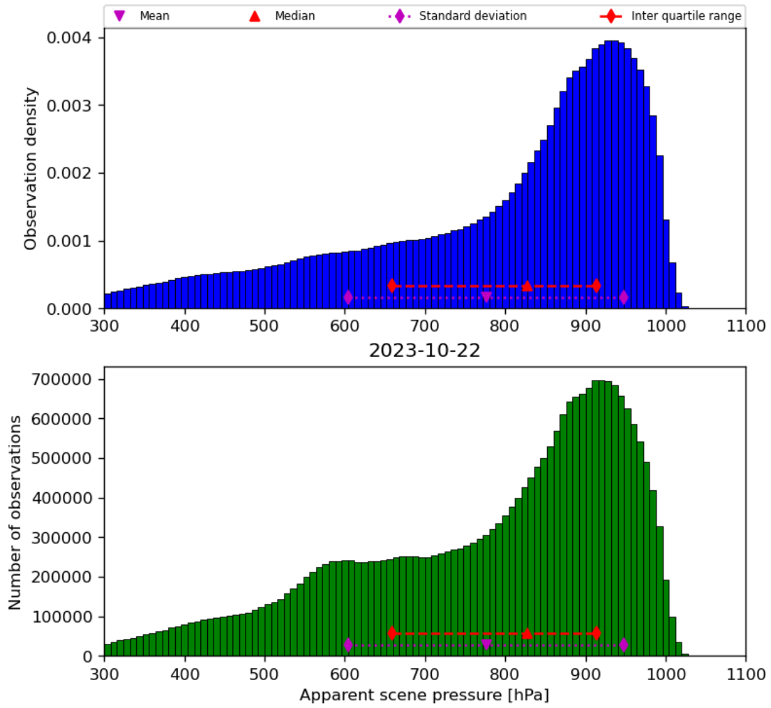
Figure 36: Histogram of “Apparent scene pressure” for 2023-10-22 to 2023-10-23
