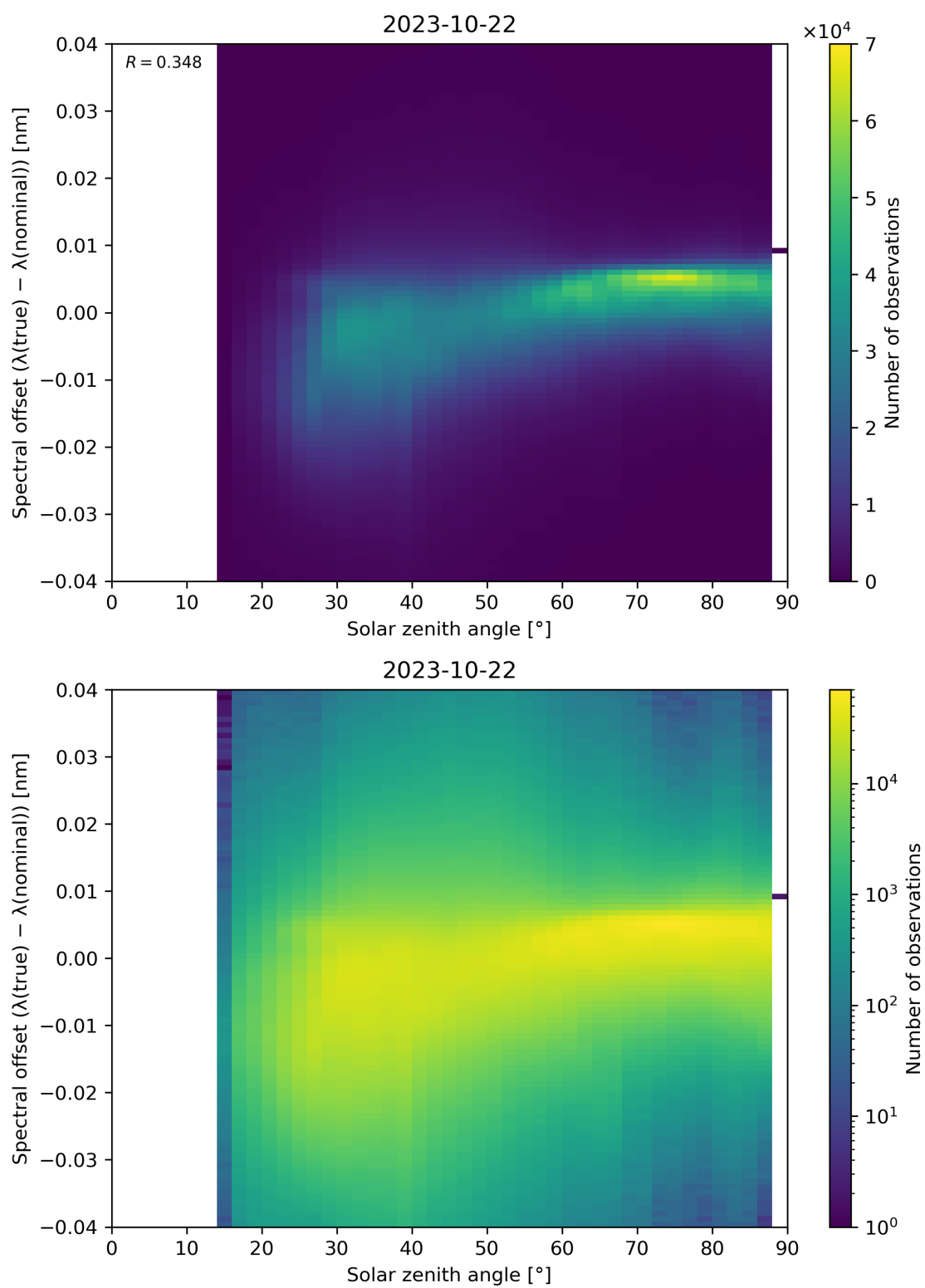
Figure 128: Scatter density plot of “Solar zenith angle” against “Spectral offset ( \lambda(\text{true}) - \lambda(\text{nominal}) )” for 2023-10-22 to 2023-10-23.
