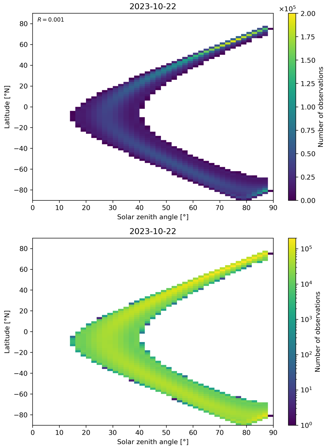
Figure 124: Scatter density plot of “Solar zenith angle” against “Latitude” for 2023-10-22 to 2023-10-23.
