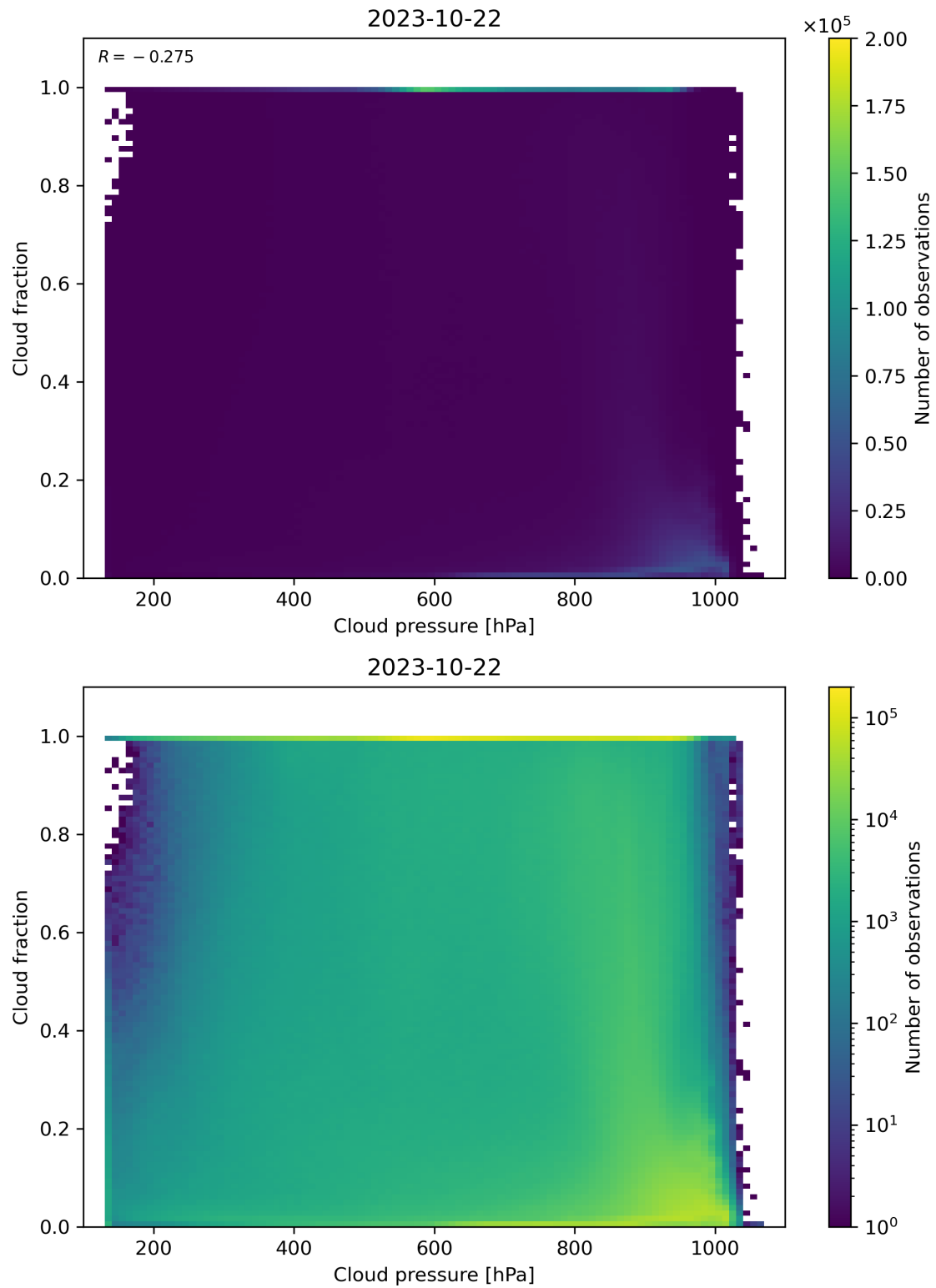
Figure 87: Scatter density plot of “Cloud pressure” against “Cloud fraction” for 2023-10-22 to 2023-10-23.
