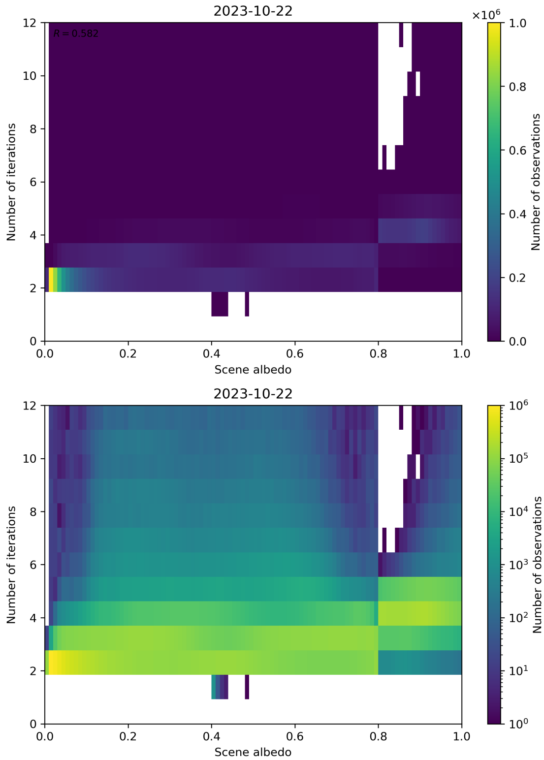
Figure 115: Scatter density plot of “Scene albedo” against “Number of iterations” for 2023-10-22 to 2023-10-23.
