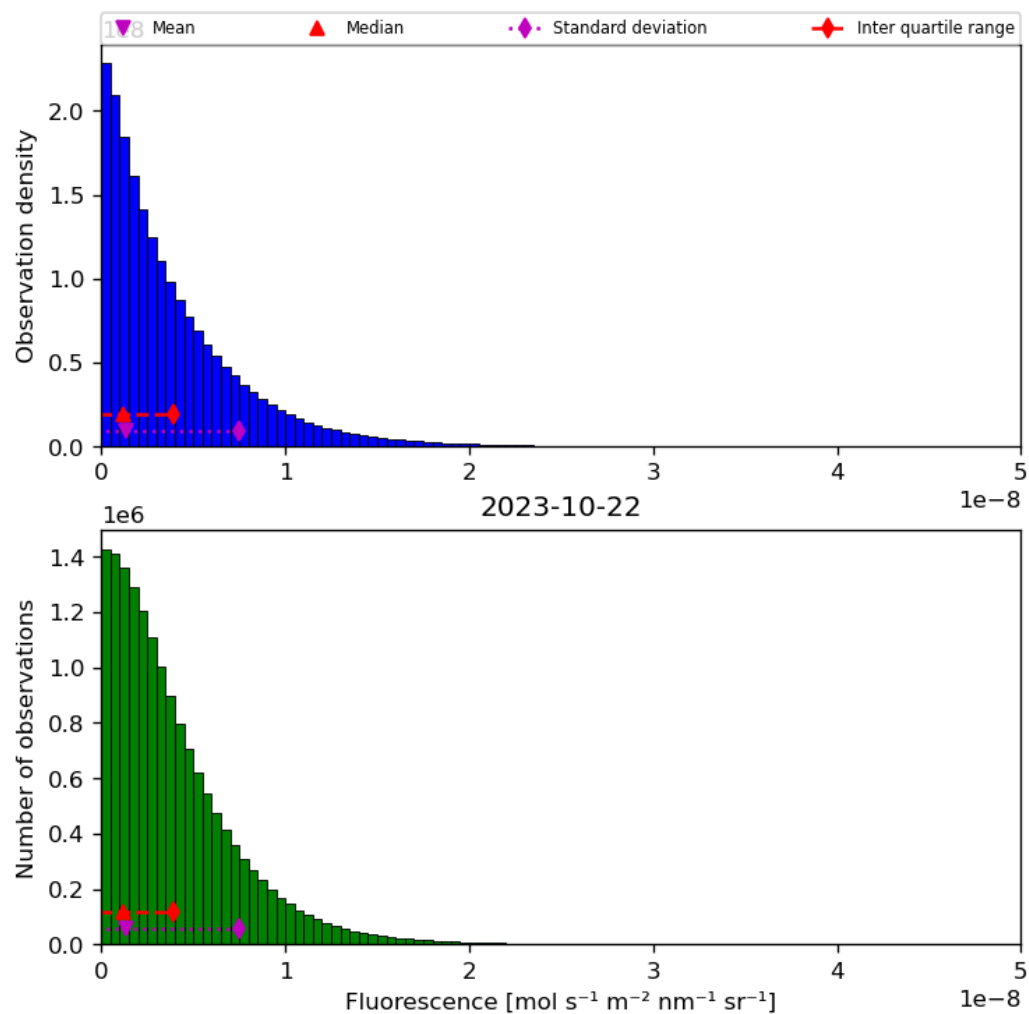
Figure 40: Histogram of “Fluorescence” for 2023-10-22 to 2023-10-23
