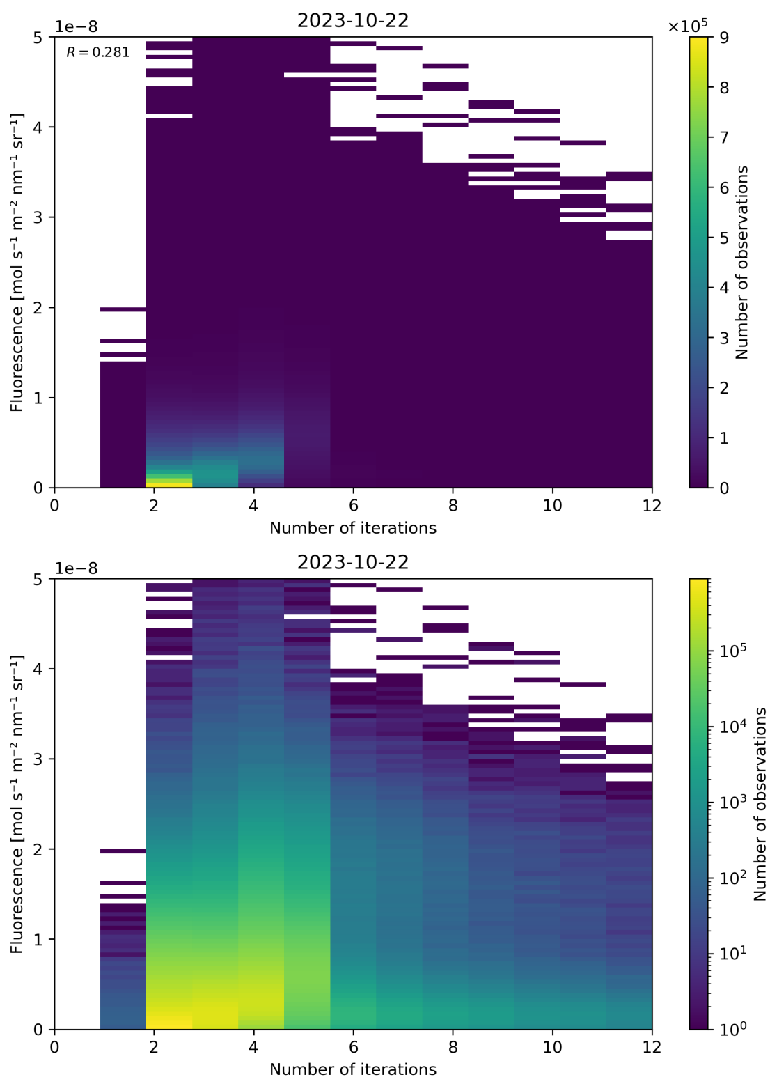
Figure 107: Scatter density plot of “Number of iterations” against “Fluorescence” for 2023-10-22 to 2023-10-23.
