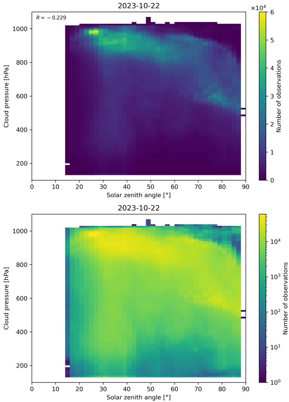
Figure 122: Scatter density plot of “Solar zenith angle” against “Cloud pressure” for 2023-10-22 to 2023-10-23.
