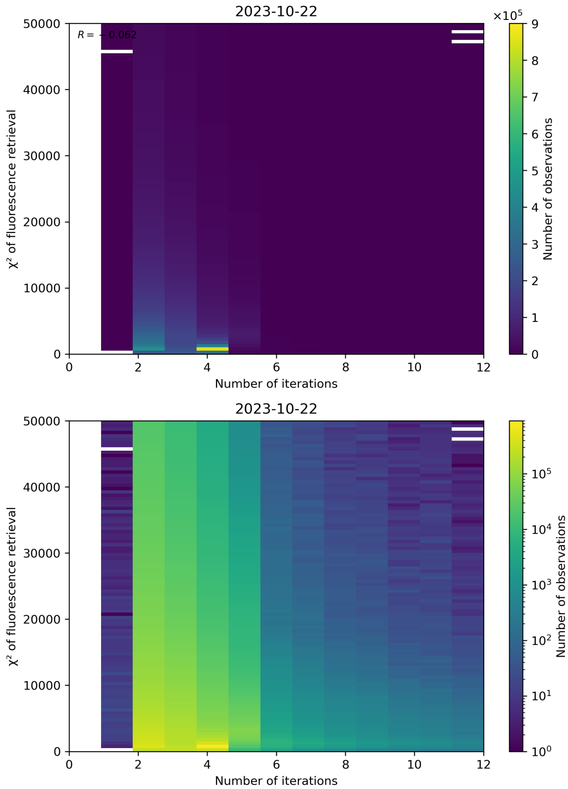
Figure 106: Scatter density plot of “Number of iterations” against “ \chi^2 of fluorescence retrieval” for 2023-10-22 to 2023-10-23.
