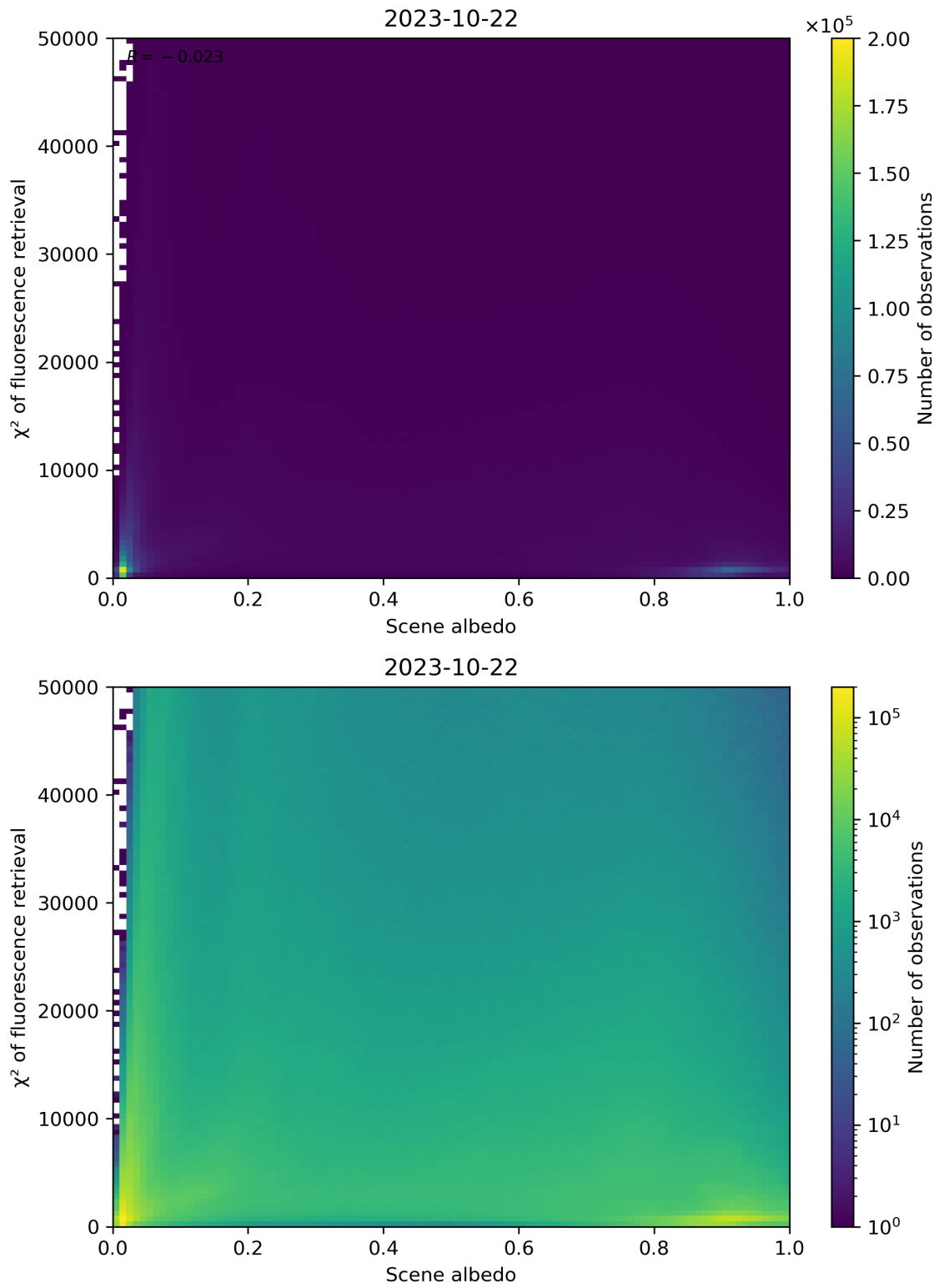
Figure 113: Scatter density plot of “Scene albedo” against “ \chi^2 of fluorescence retrieval” for 2023-10-22 to 2023-10-23.
