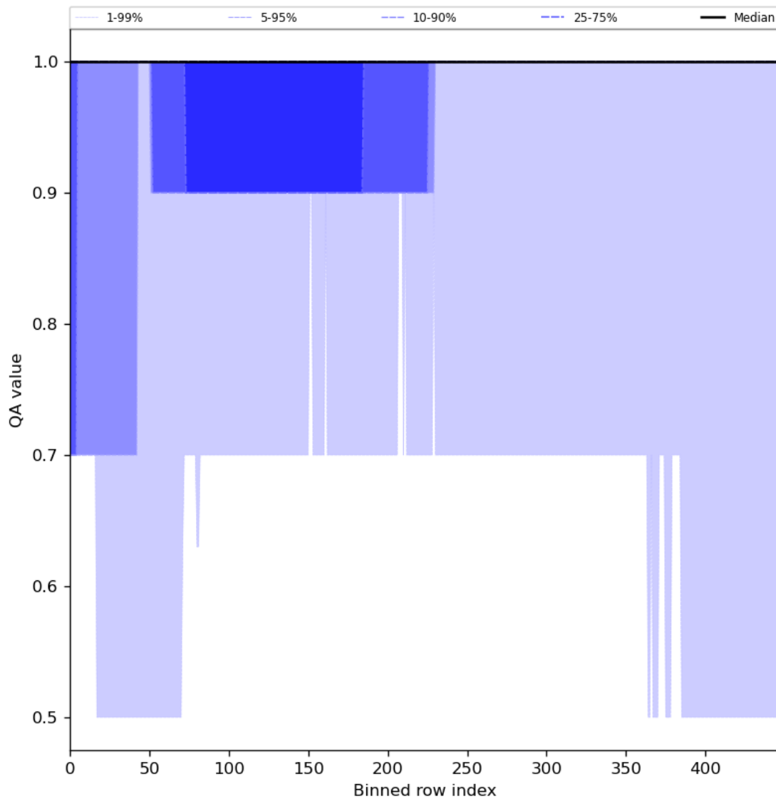
Figure 46: Along track statistics of “QA value” for 2023-10-22 to 2023-10-23
