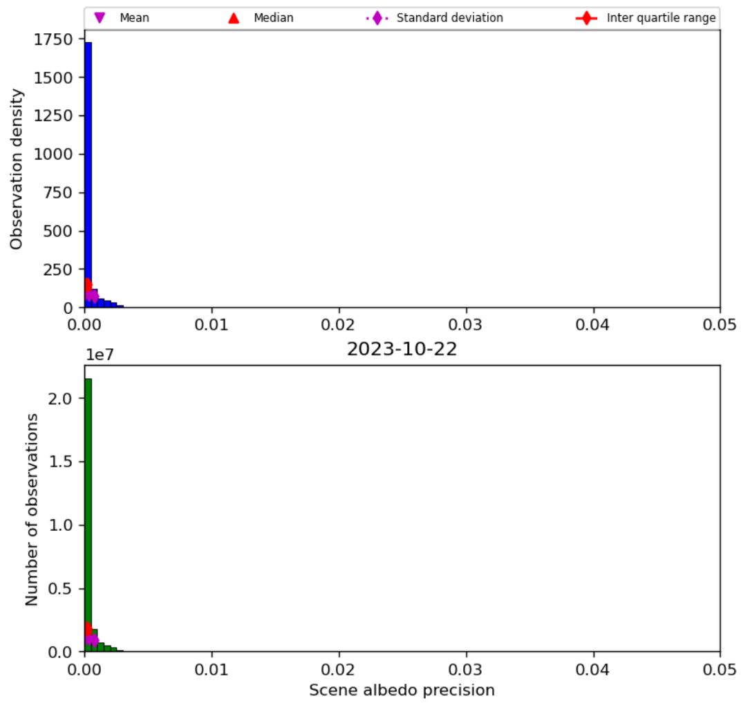
Figure 35: Histogram of “Scene albedo precision” for 2023-10-22 to 2023-10-23
