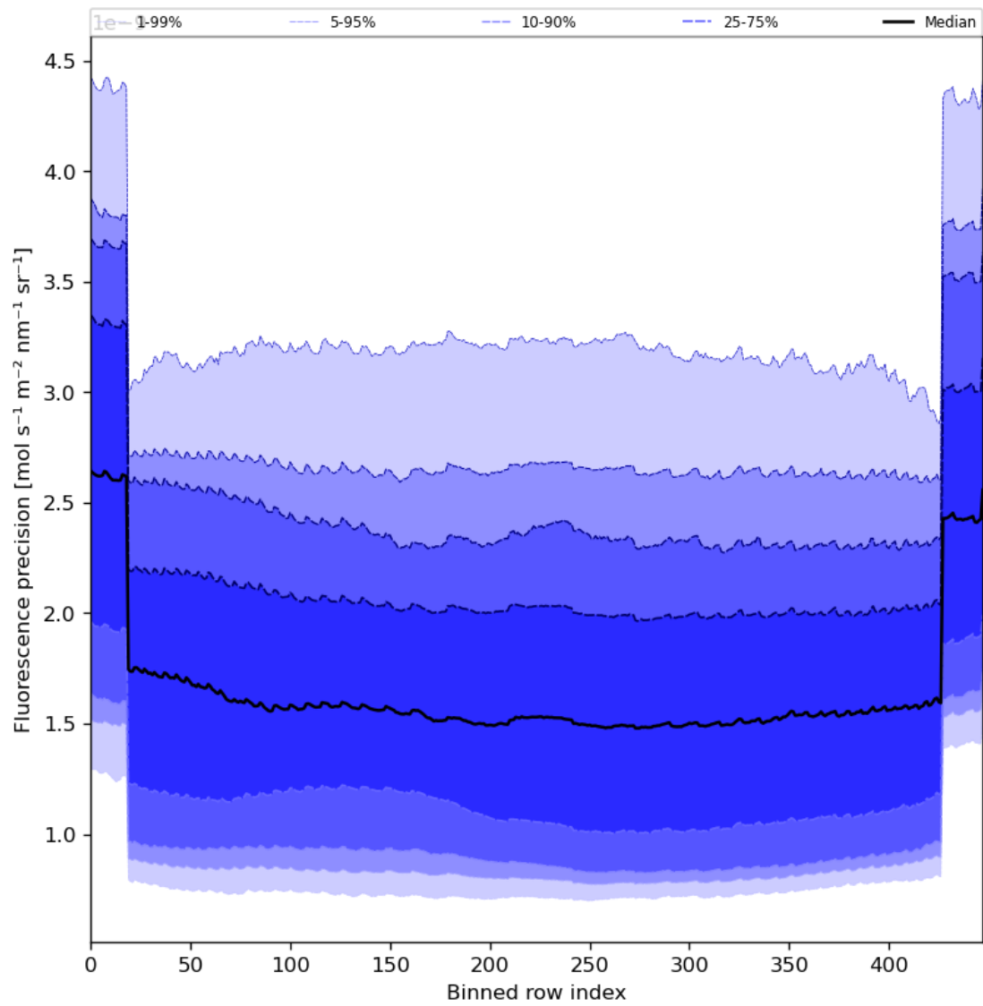
Figure 58: Along track statistics of “Fluorescence precision” for 2023-10-22 to 2023-10-23
