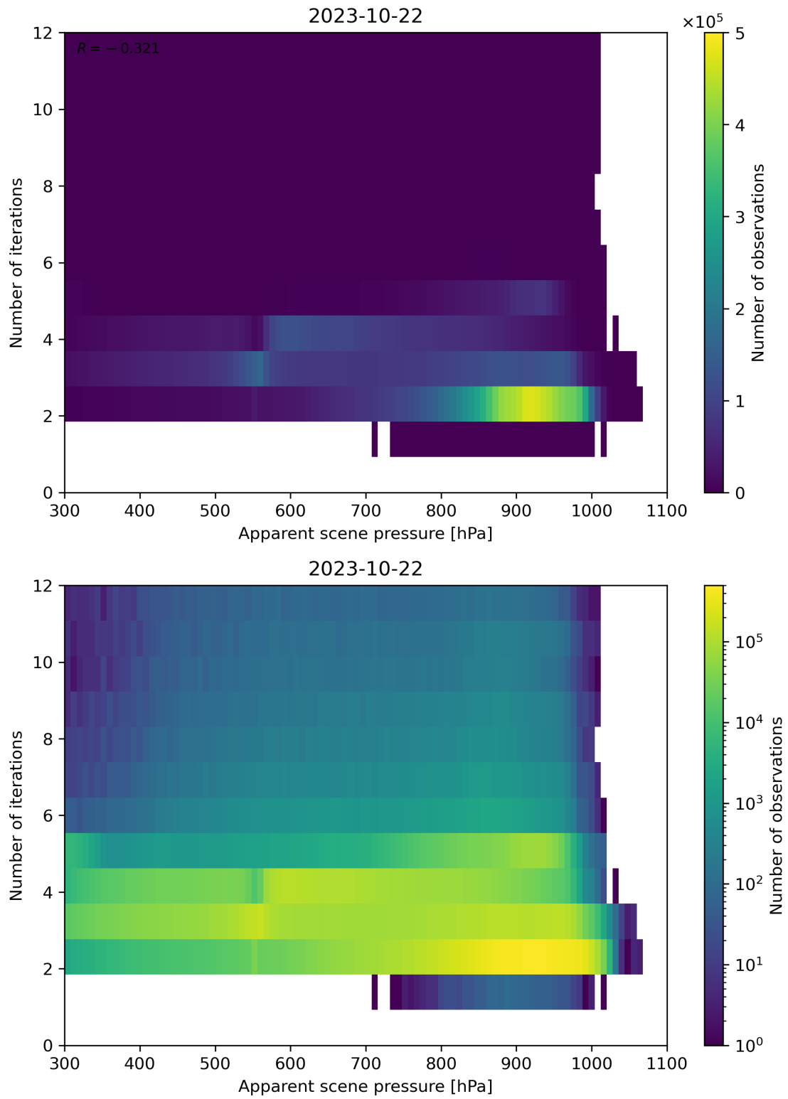
Figure 66: Scatter density plot of “Apparent scene pressure” against “Number of iterations” for 2023-10-22 to 2023-10-23.
