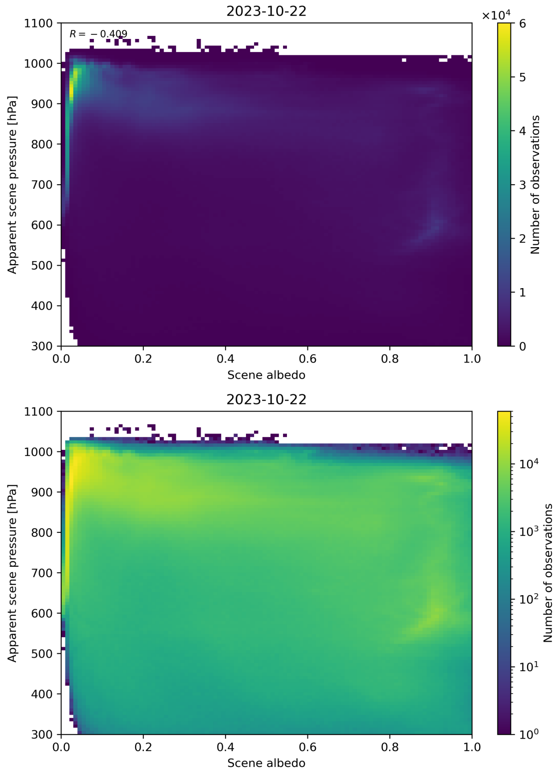
Figure 111: Scatter density plot of “Scene albedo” against “Apparent scene pressure” for 2023-10-22 to 2023-10-23.
