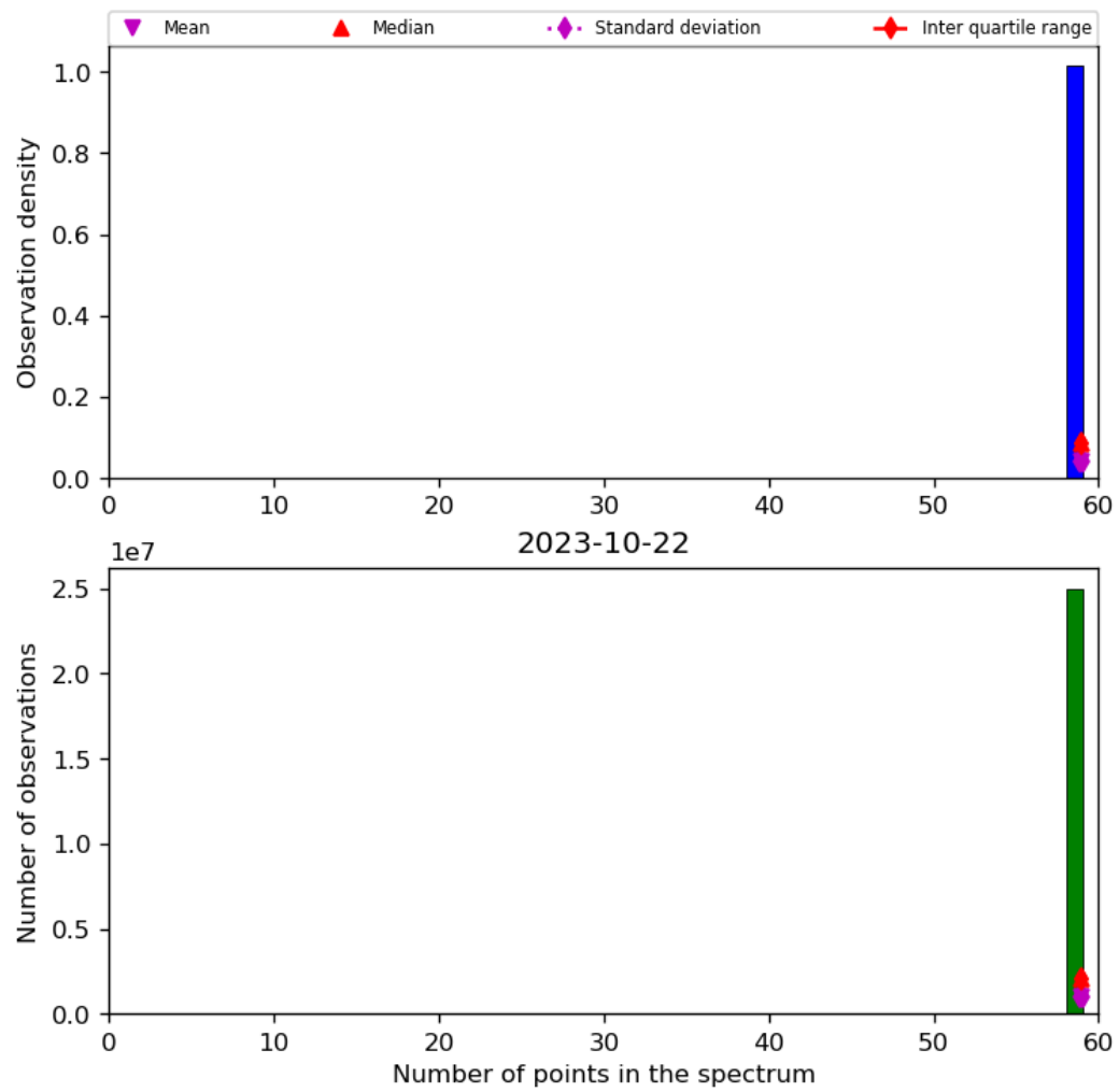
Figure 44: Histogram of “Number of points in the spectrum” for 2023-10-22 to 2023-10-23
