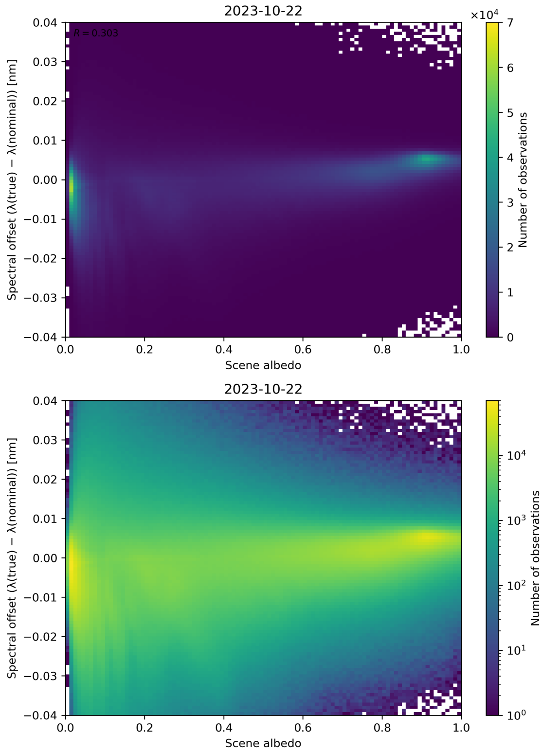
Figure 117: Scatter density plot of “Scene albedo” against “Spectral offset ( \lambda(\text{true}) - \lambda(\text{nominal}) )” for 2023-10-22 to 2023-10-23.
