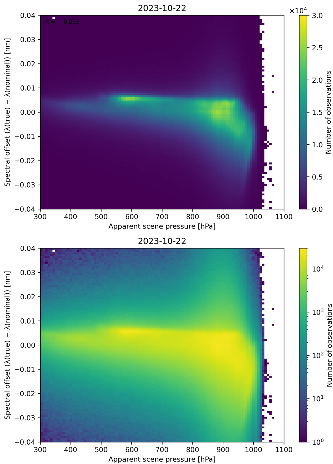
Figure 68: Scatter density plot of “Apparent scene pressure” against “Spectral offset ( \lambda(\text{true}) - \lambda(\text{nominal}) )” for 2023-10-22 to 2023-10-23.
