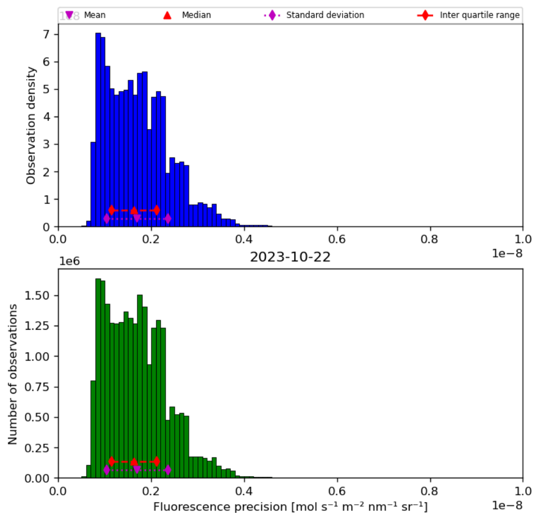
Figure 41: Histogram of “Fluorescence precision” for 2023-10-22 to 2023-10-23
