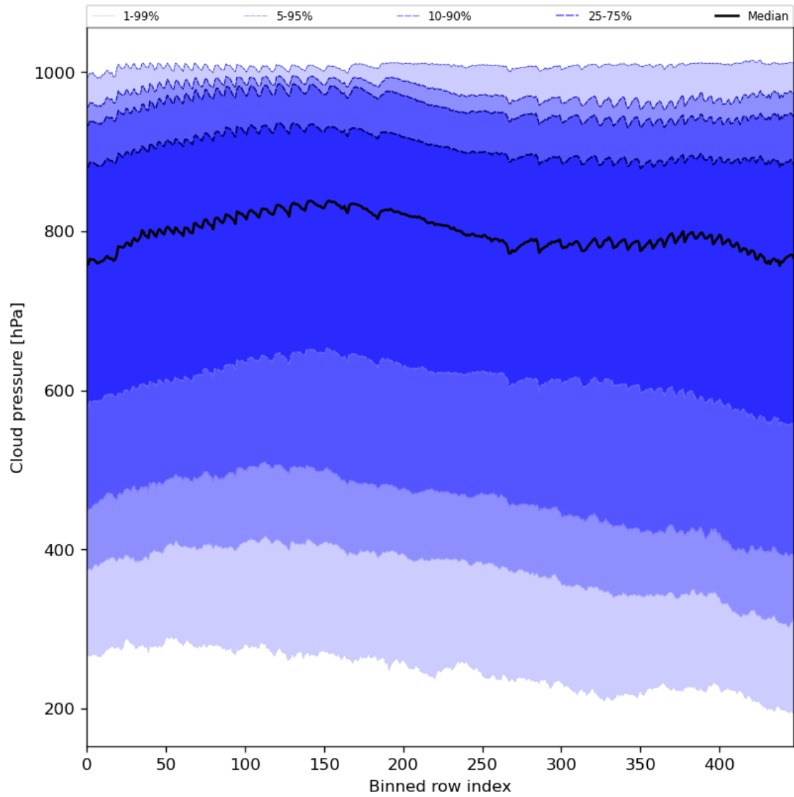
Figure 47: Along track statistics of “Cloud pressure” for 2023-10-22 to 2023-10-23
