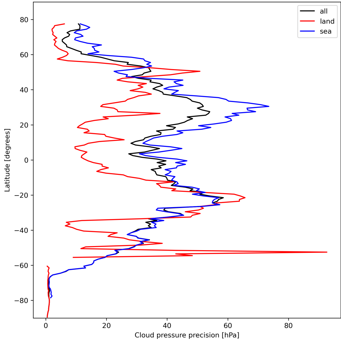
Figure 14: Zonal average of “Cloud pressure precision” for 2023-10-22 to 2023-10-23.
