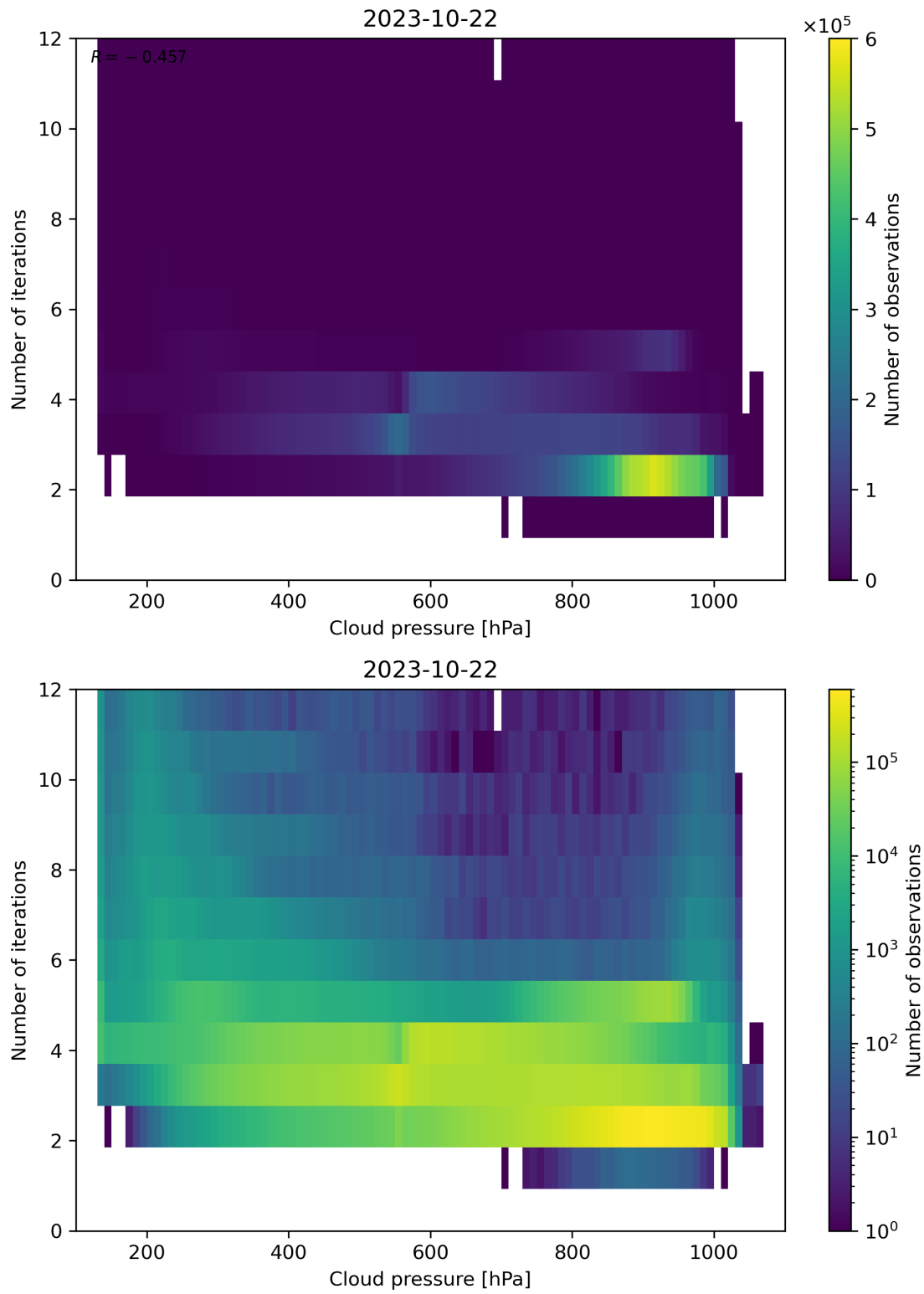
Figure 89: Scatter density plot of “Cloud pressure” against “Number of iterations” for 2023-10-22 to 2023-10-23.
