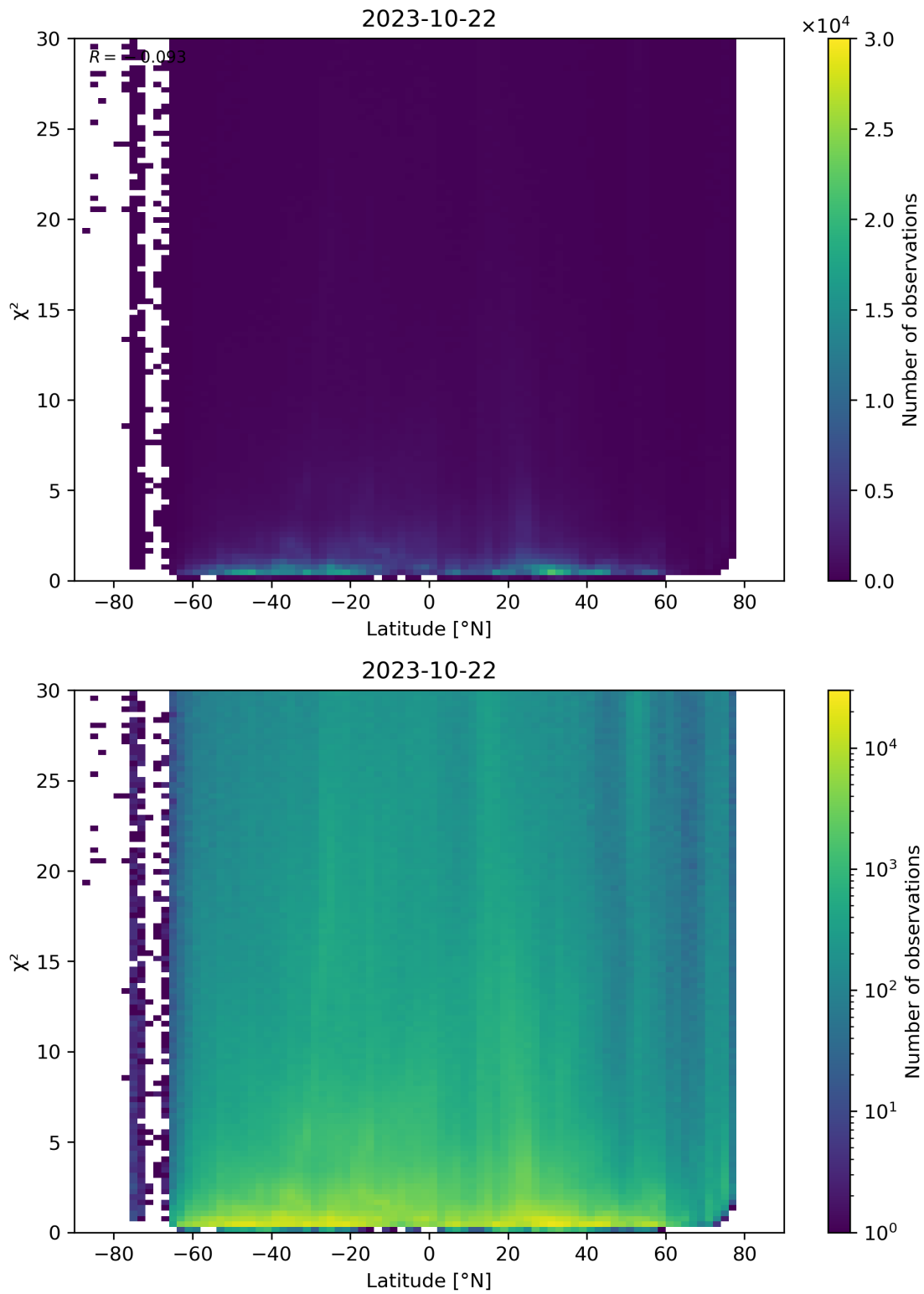
Figure 97: Scatter density plot of “Latitude” against “ \chi^2 ” for 2023-10-22 to 2023-10-23.
