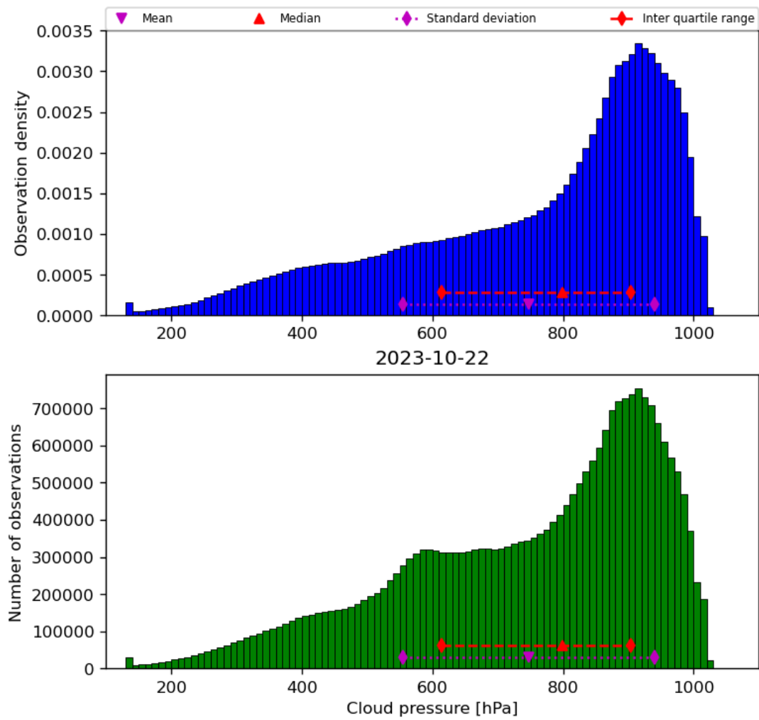
Figure 30: Histogram of “Cloud pressure” for 2023-10-22 to 2023-10-23
