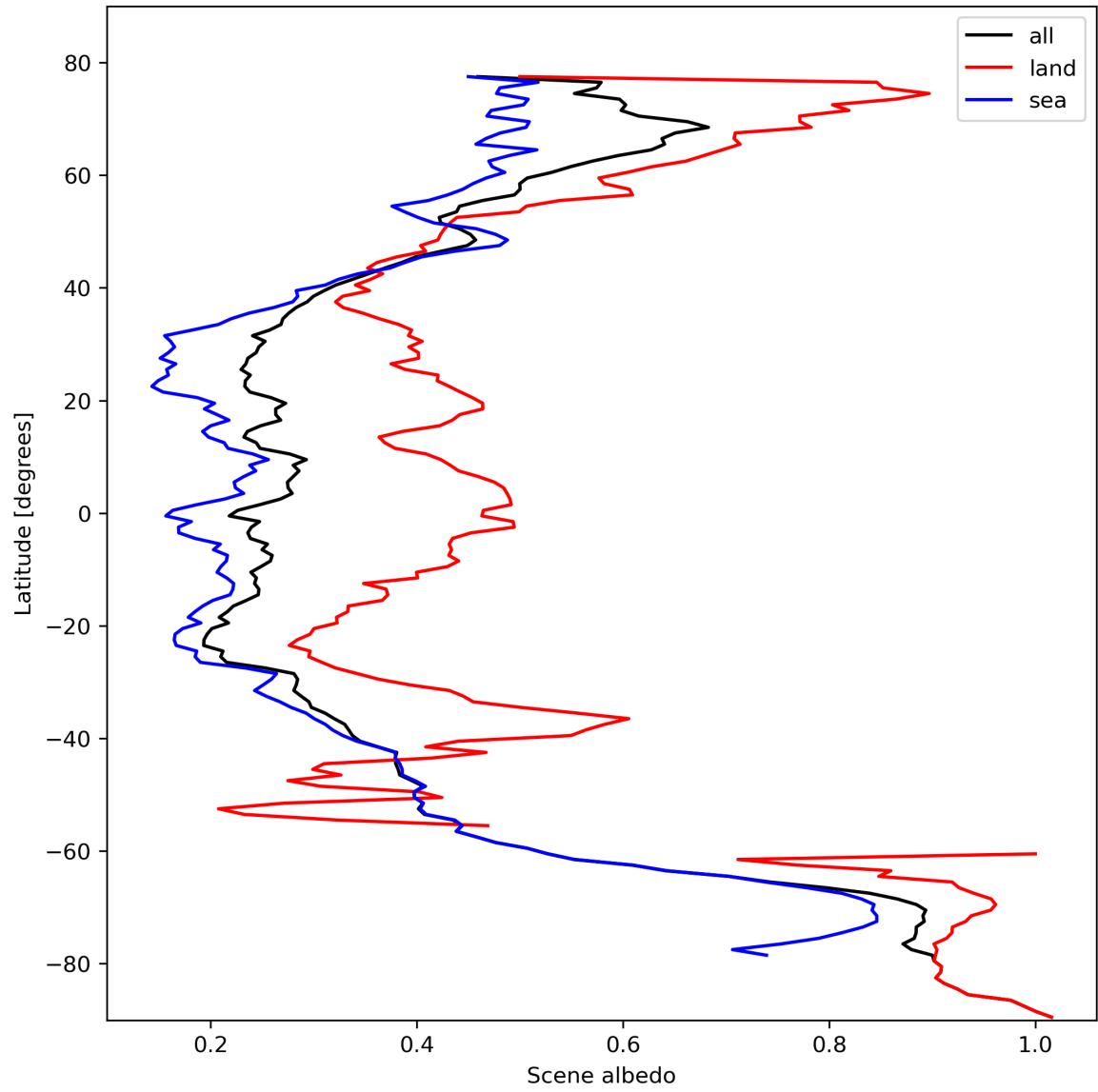
Figure 17: Zonal average of “Scene albedo” for 2023-10-22 to 2023-10-23.
