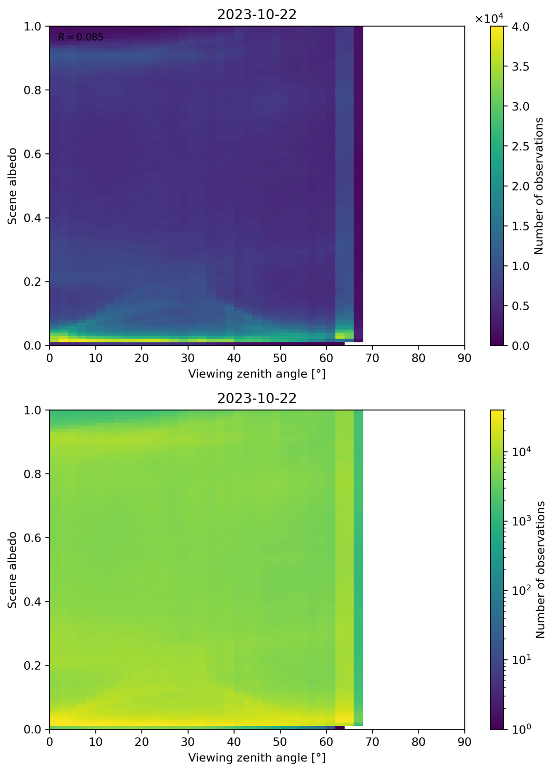
Figure 138: Scatter density plot of “Viewing zenith angle” against “Scene albedo” for 2023-10-22 to 2023-10-23.
