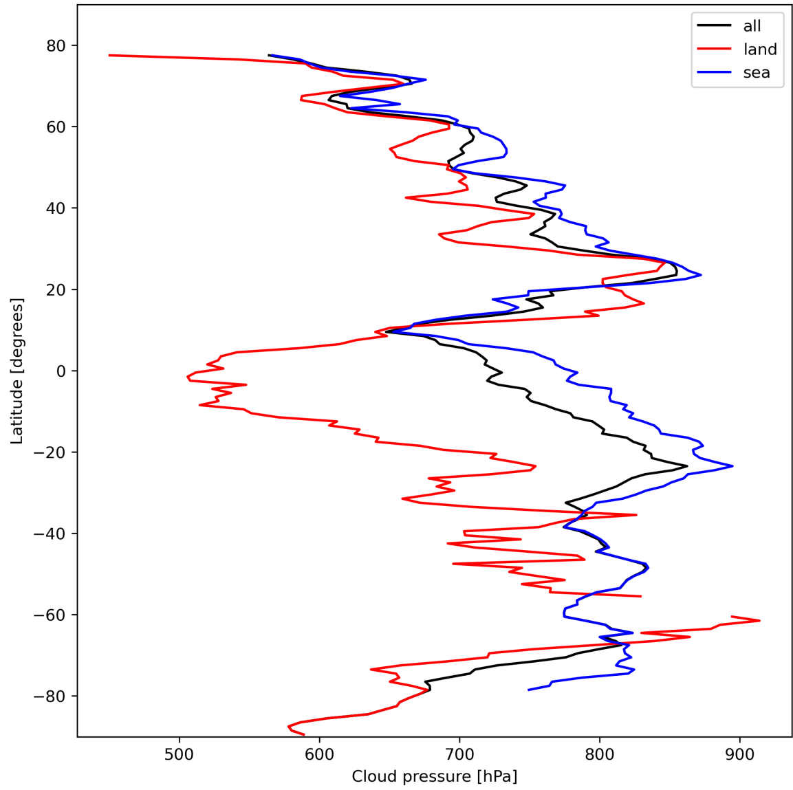
Figure 13: Zonal average of “Cloud pressure” for 2023-10-22 to 2023-10-23.
