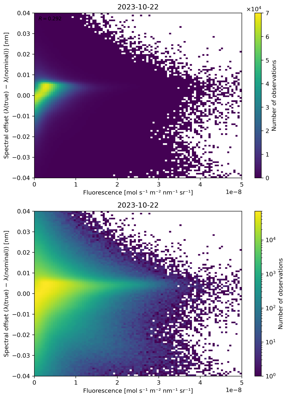
Figure 95: Scatter density plot of “Fluorescence” against “Spectral offset ( \lambda(\text{true}) - \lambda(\text{nominal}) )” for 2023-10-22 to 2023-10-23.
