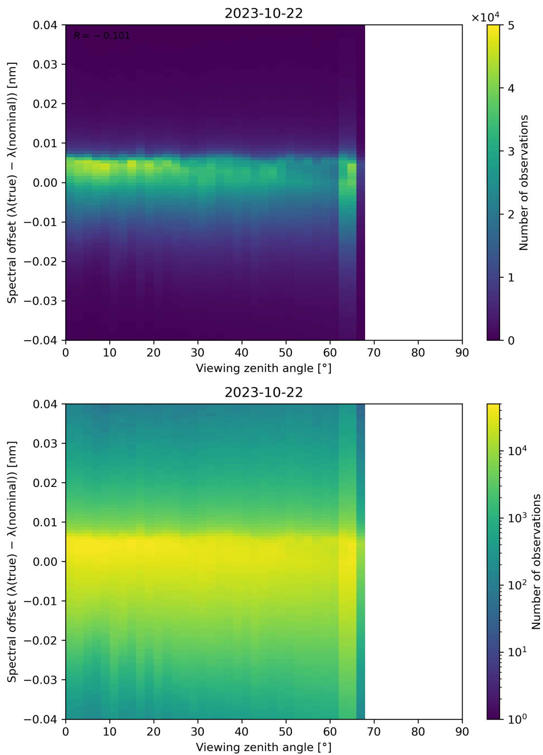
Figure 140: Scatter density plot of “Viewing zenith angle” against “Spectral offset ( \lambda(\text{true}) - \lambda(\text{nominal}) )” for 2023-10-22 to 2023-10-23.
