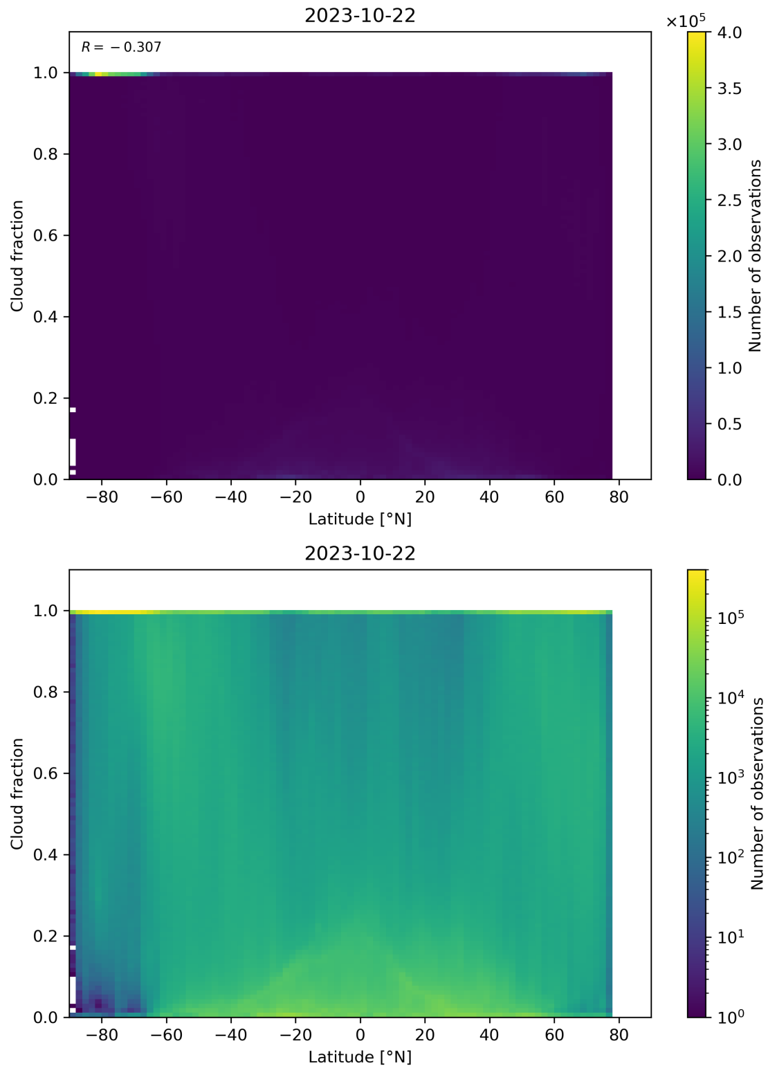
Figure 99: Scatter density plot of “Latitude” against “Cloud fraction” for 2023-10-22 to 2023-10-23.
