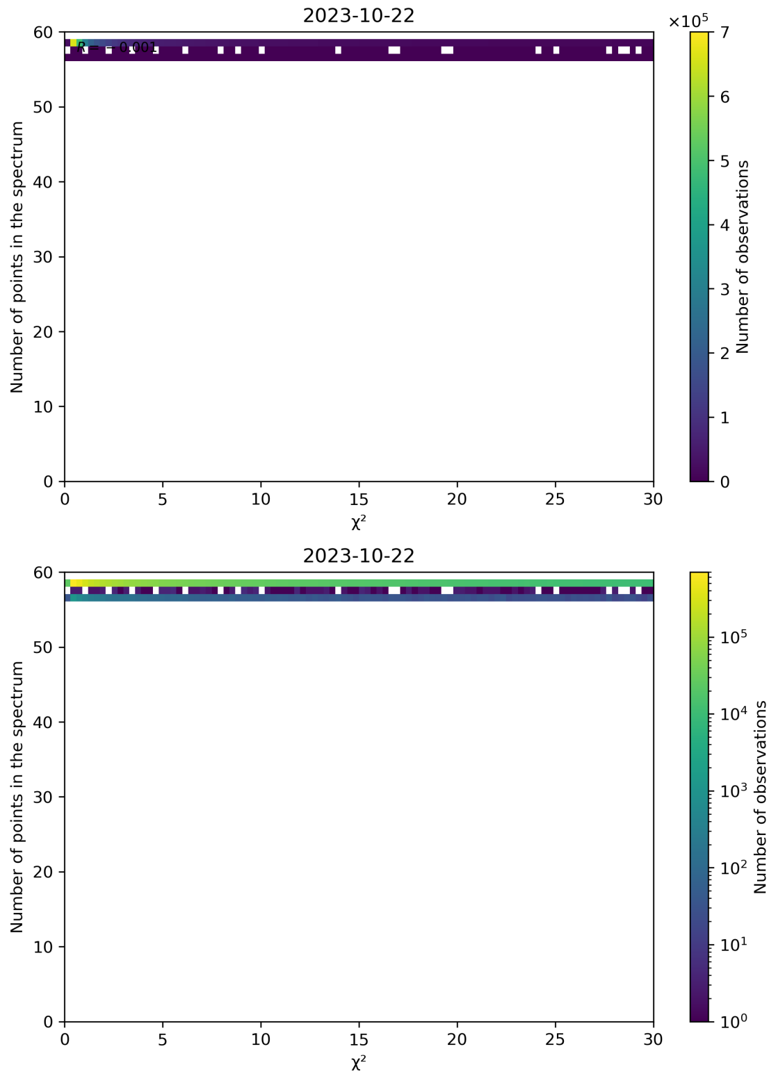
Figure 74: Scatter density plot of " \chi^2 " against "Number of points in the spectrum" for 2023-10-22 to 2023-10-23.
