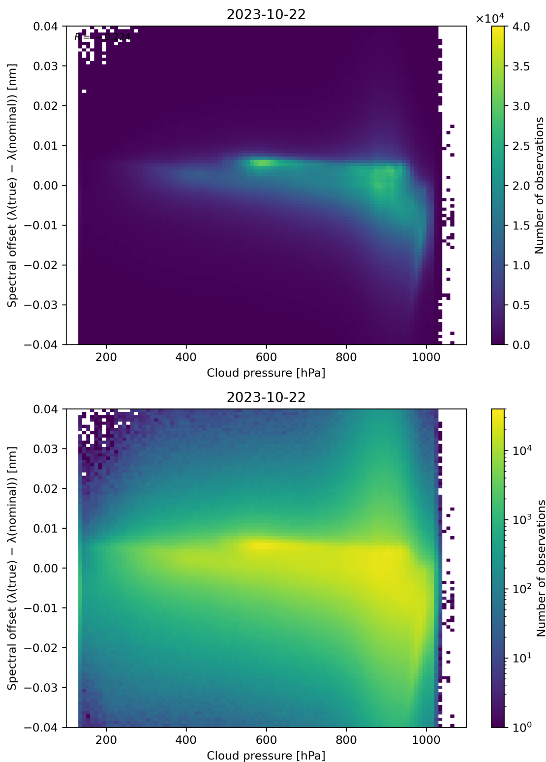
Figure 92: Scatter density plot of “Cloud pressure” against “Spectral offset ( \lambda(\text{true}) - \lambda(\text{nominal}) )” for 2023-10-22 to 2023-10-23.
