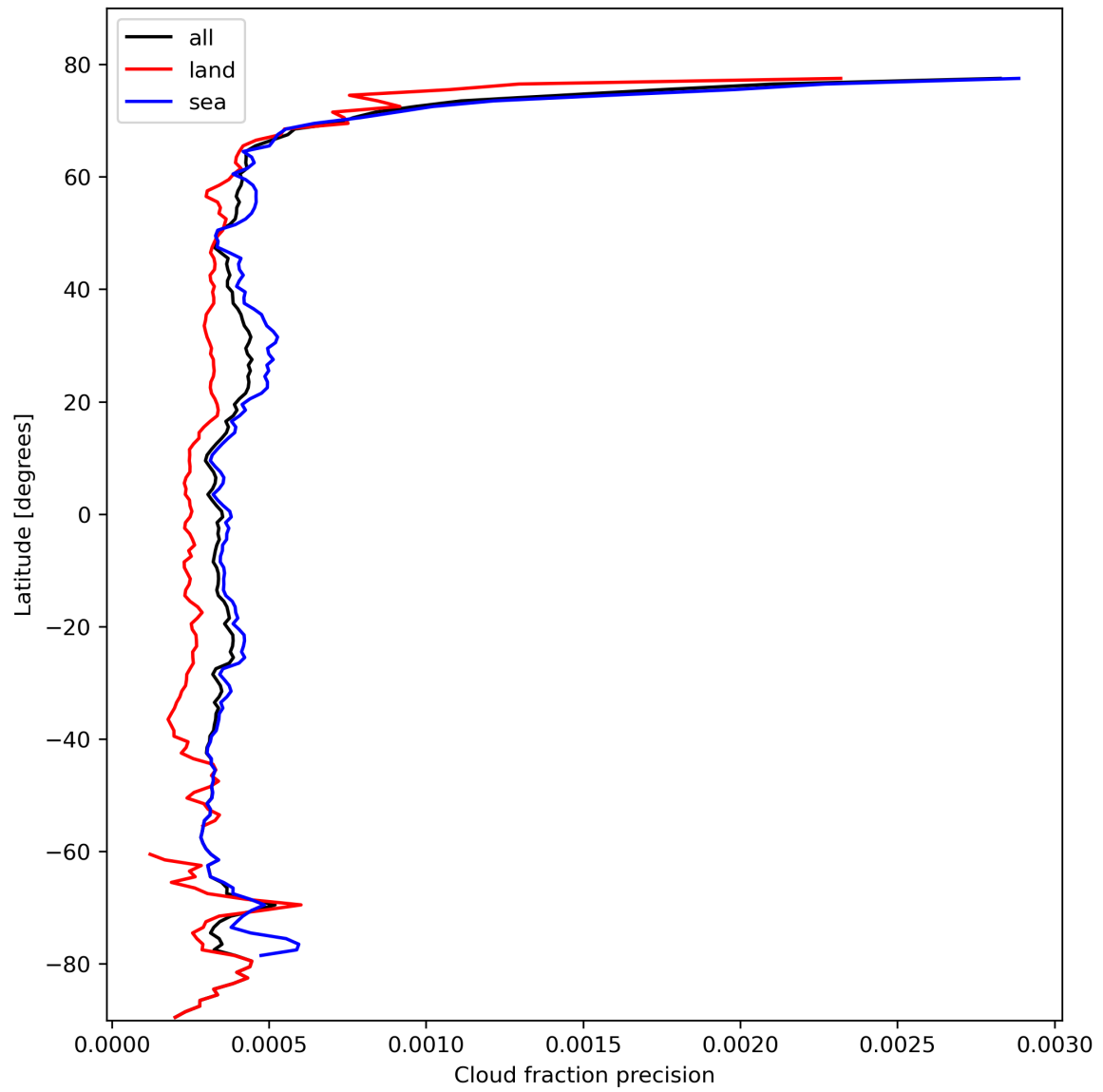
Figure 16: Zonal average of “Cloud fraction precision” for 2023-10-22 to 2023-10-23.
