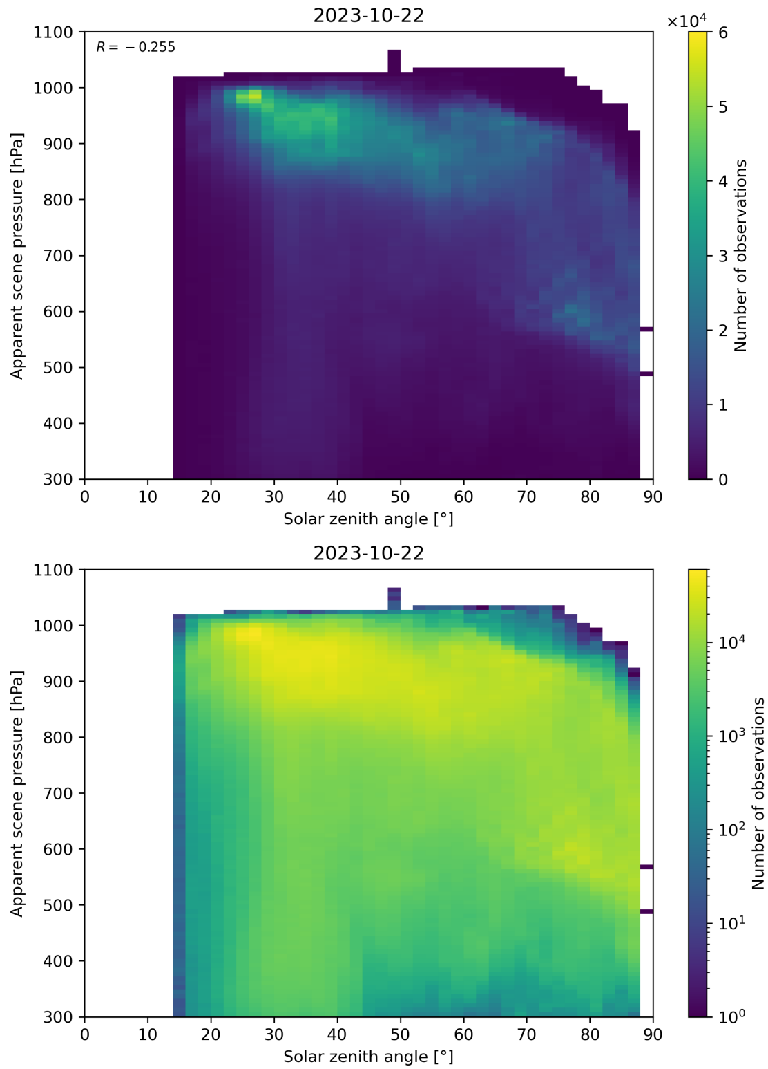
Figure 118: Scatter density plot of “Solar zenith angle” against “Apparent scene pressure” for 2023-10-22 to 2023-10-23.
