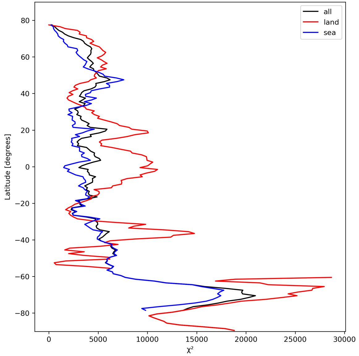
Figure 21: Zonal average of “ \chi^2 ” for 2023-10-22 to 2023-10-23.
