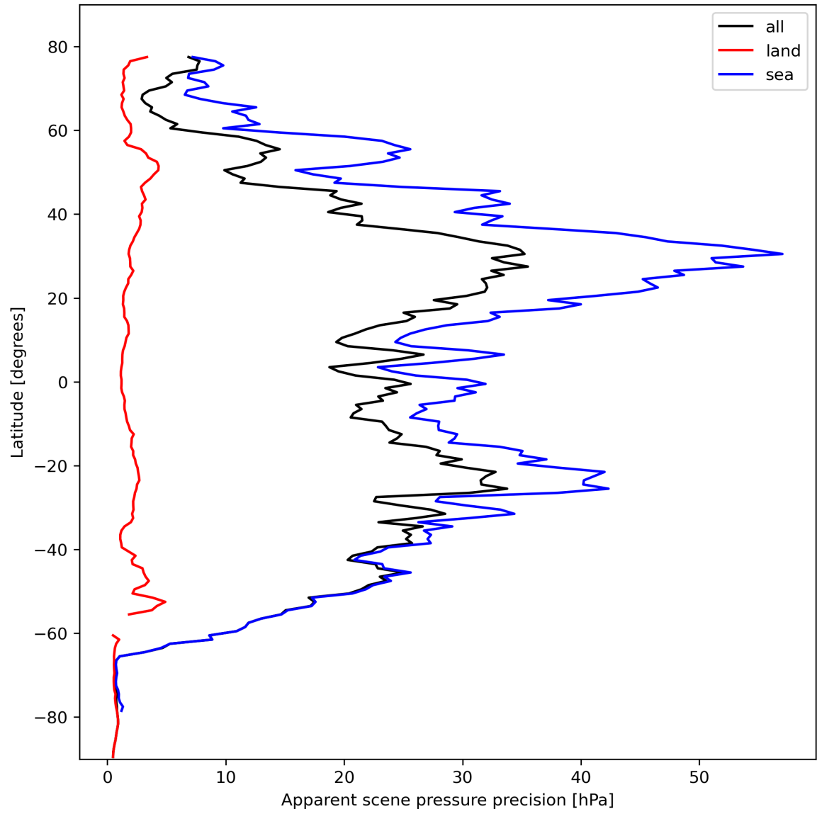
Figure 20: Zonal average of “Apparent scene pressure precision” for 2023-10-22 to 2023-10-23.
