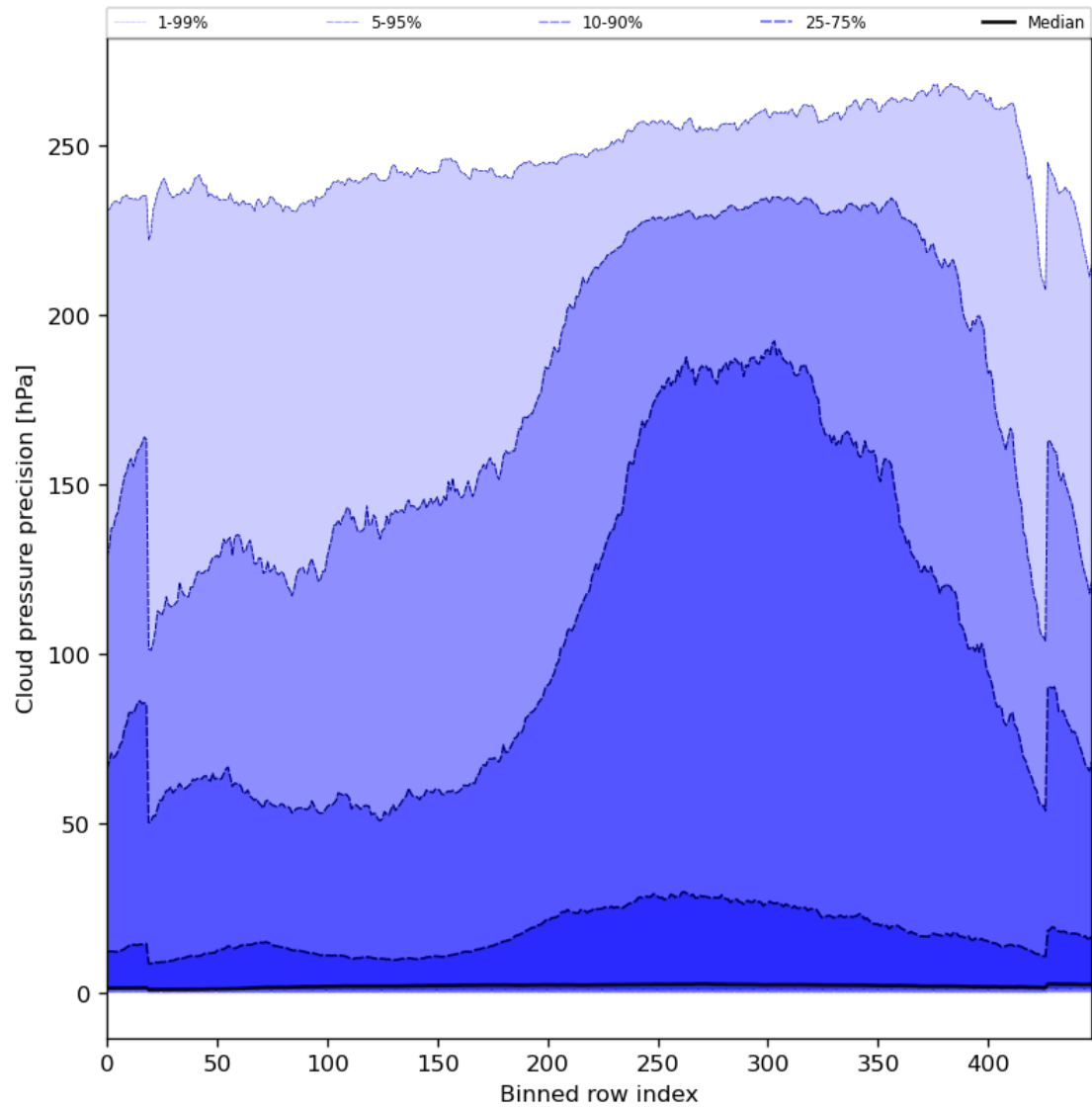
Figure 48: Along track statistics of “Cloud pressure precision” for 2023-10-22 to 2023-10-23
