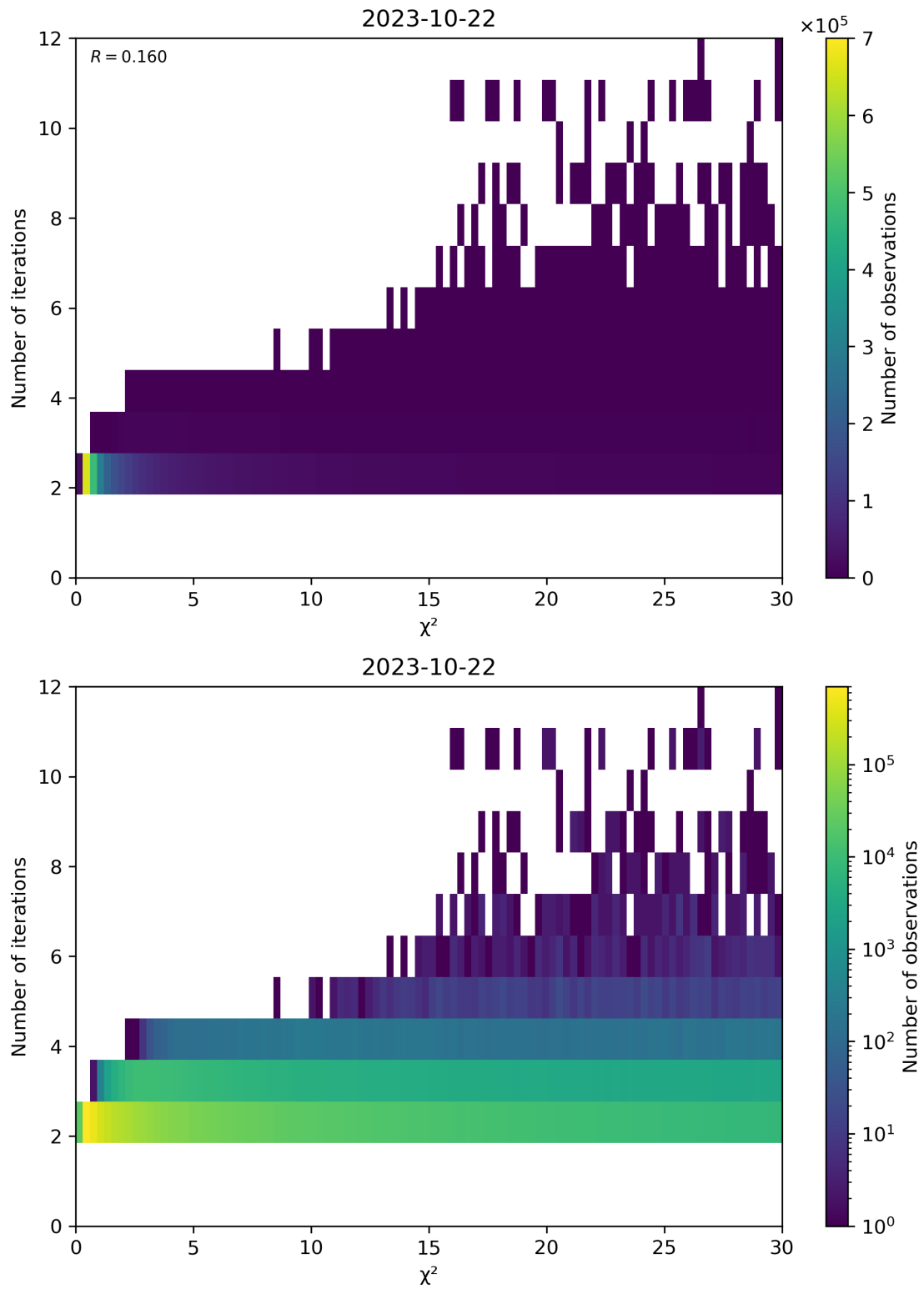
Figure 73: Scatter density plot of “ \chi^2 ” against “Number of iterations” for 2023-10-22 to 2023-10-23.
