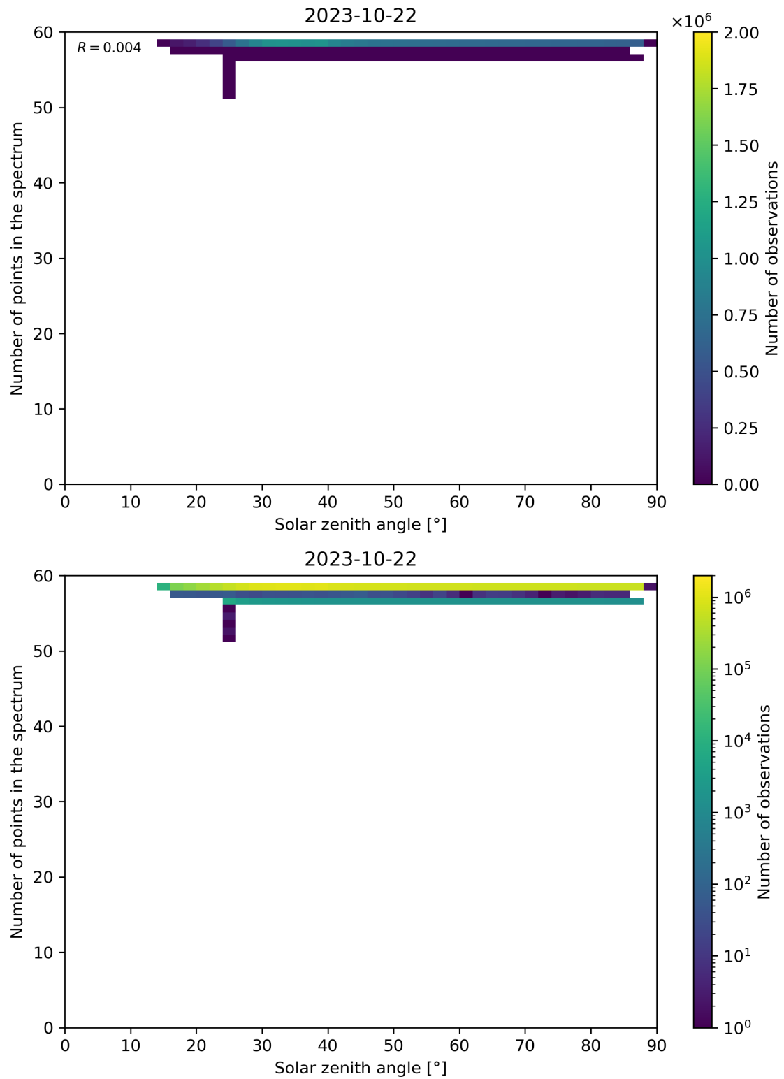
Figure 126: Scatter density plot of “Solar zenith angle” against “Number of points in the spectrum” for 2023-10-22 to 2023-10-23.
