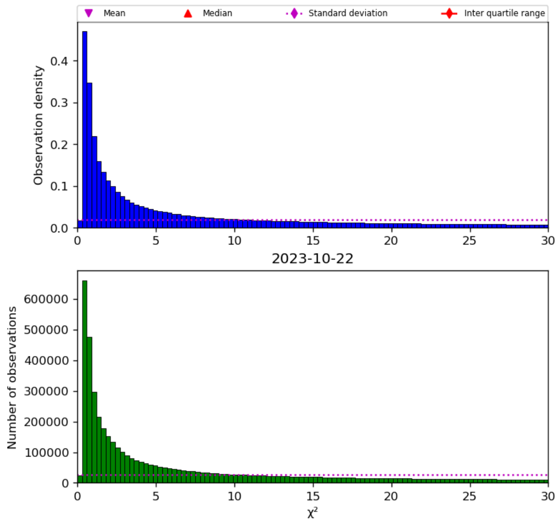
Figure 38: Histogram of “ \chi^2 ” for 2023-10-22 to 2023-10-23
