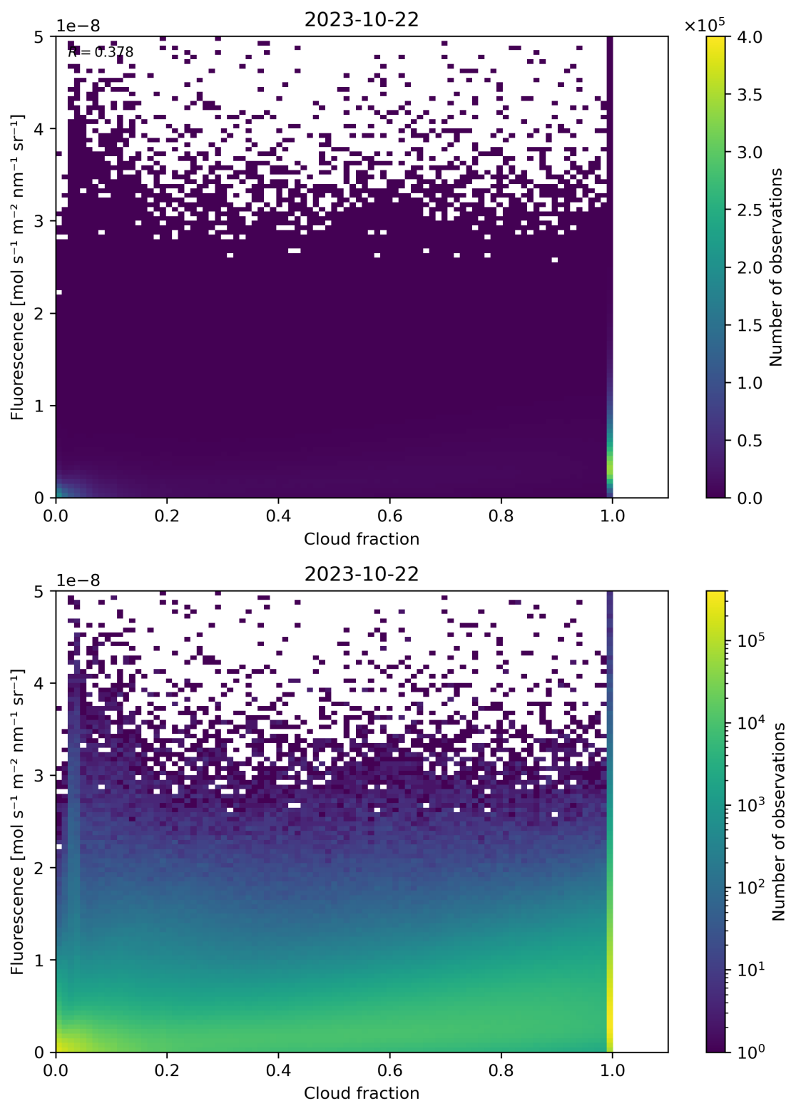
Figure 79: Scatter density plot of “Cloud fraction” against “Fluorescence” for 2023-10-22 to 2023-10-23.
