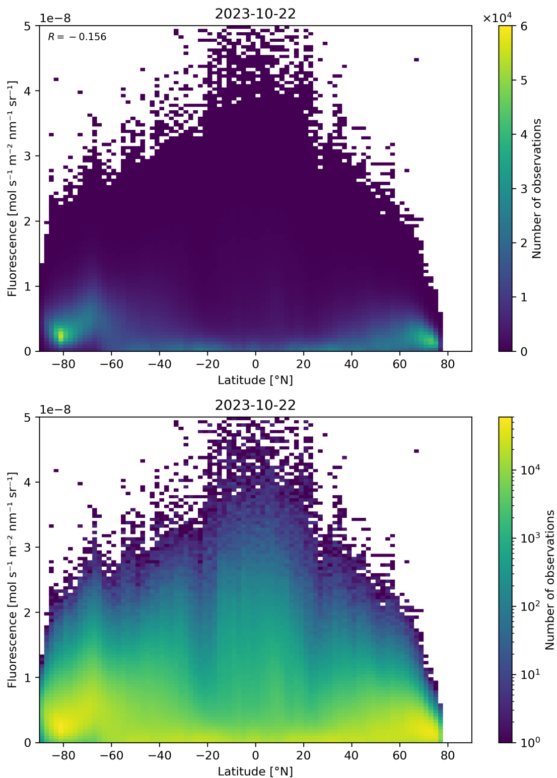
Figure 101: Scatter density plot of “Latitude” against “Fluorescence” for 2023-10-22 to 2023-10-23.
