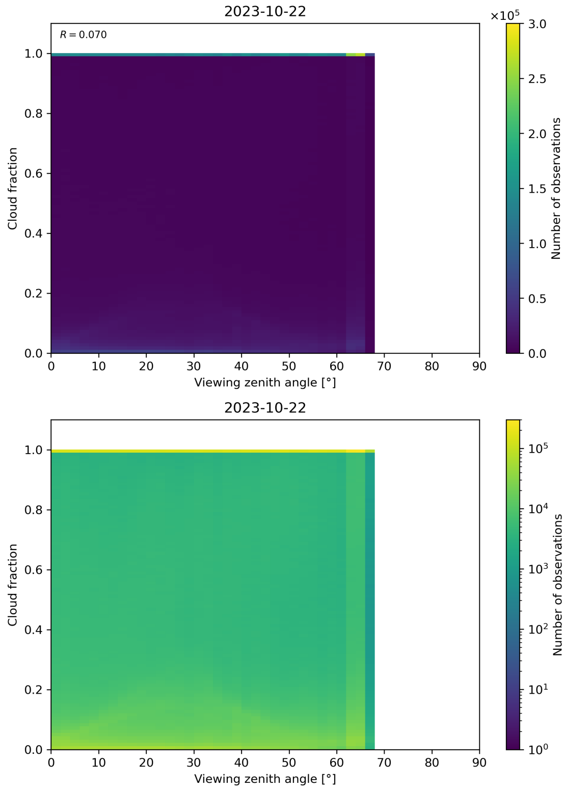
Figure 132: Scatter density plot of “Viewing zenith angle” against “Cloud fraction” for 2023-10-22 to 2023-10-23.
