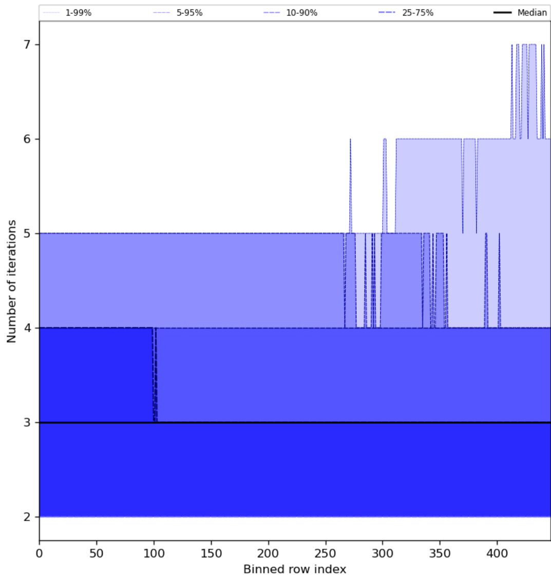
Figure 56: Along track statistics of “Number of iterations” for 2023-10-22 to 2023-10-23
