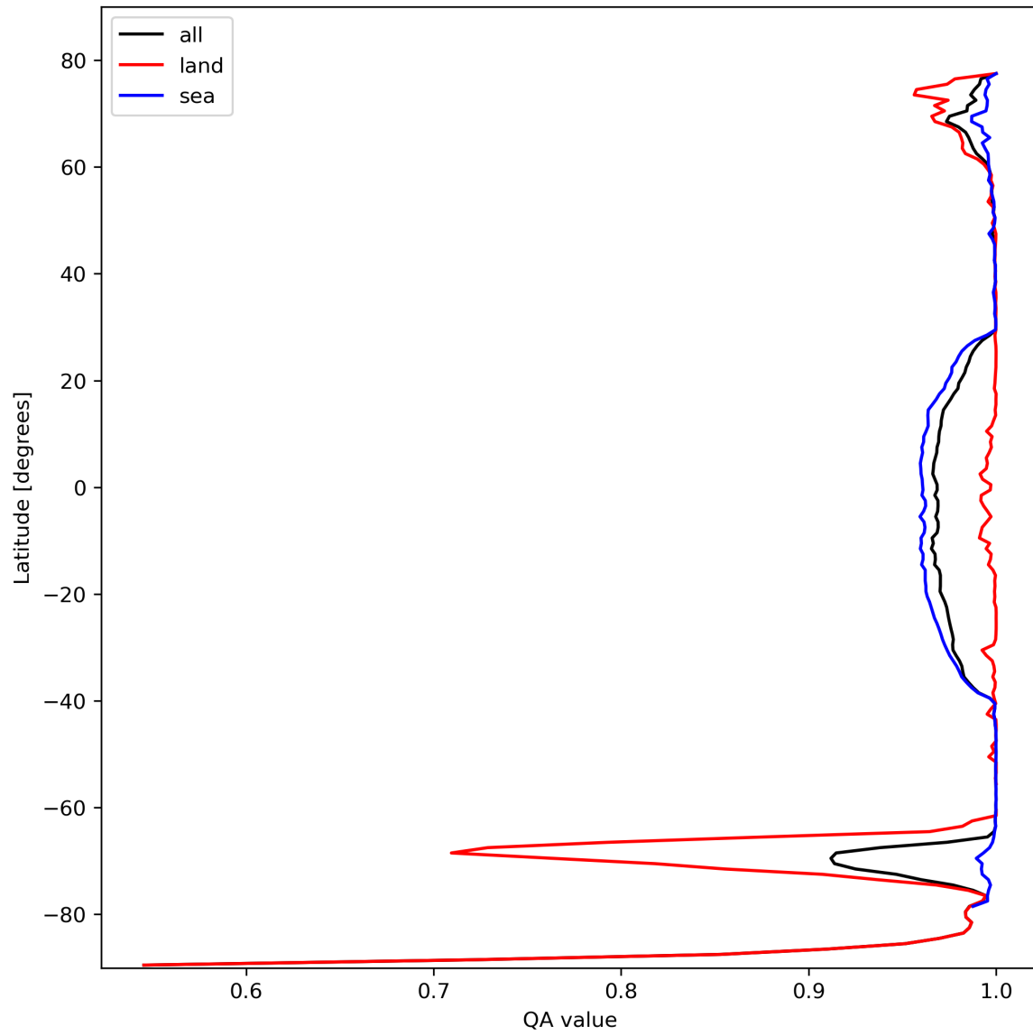
Figure 12: Zonal average of "QA value" for 2023-10-22 to 2023-10-23.
