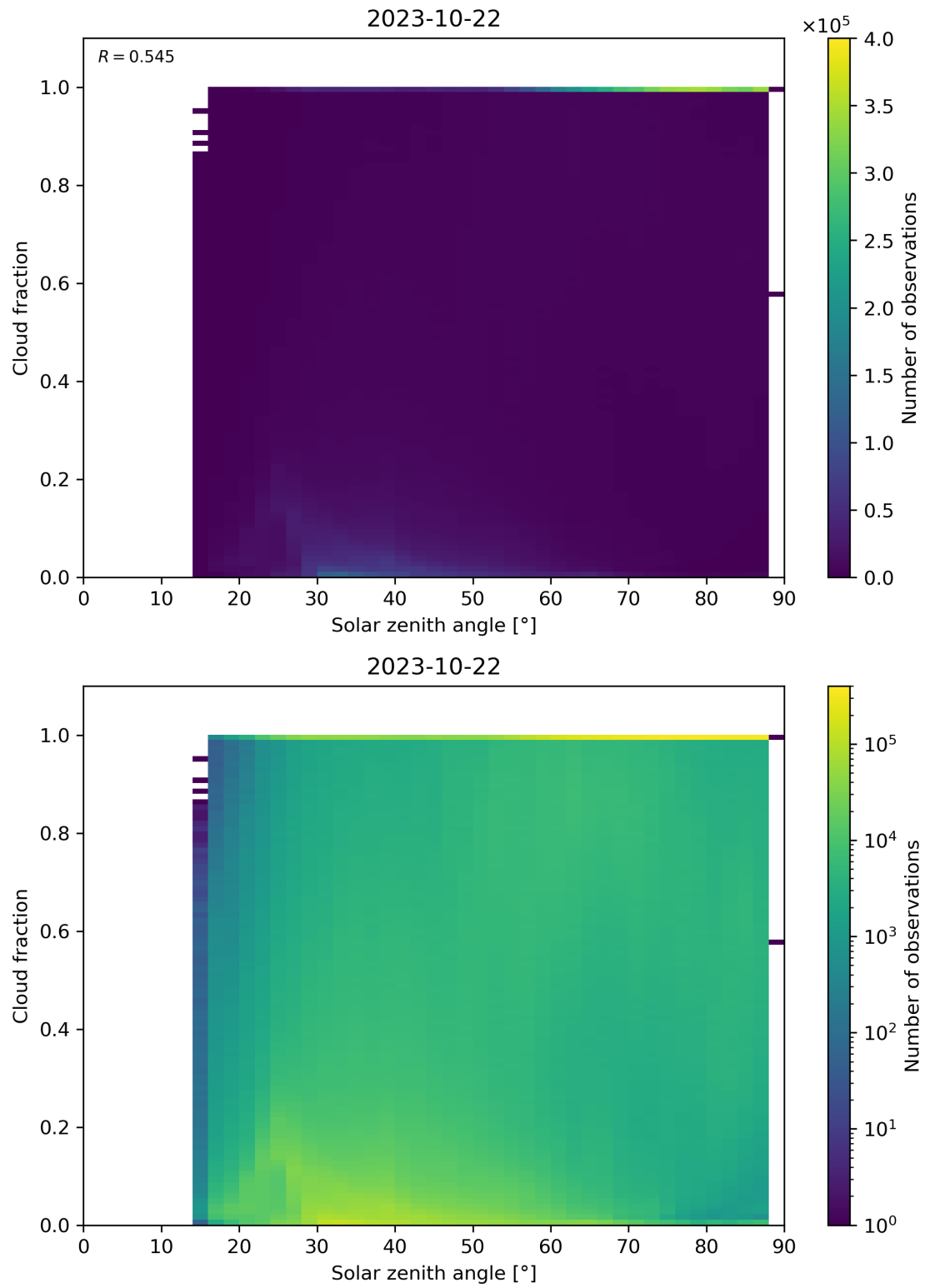
Figure 121: Scatter density plot of “Solar zenith angle” against “Cloud fraction” for 2023-10-22 to 2023-10-23.
