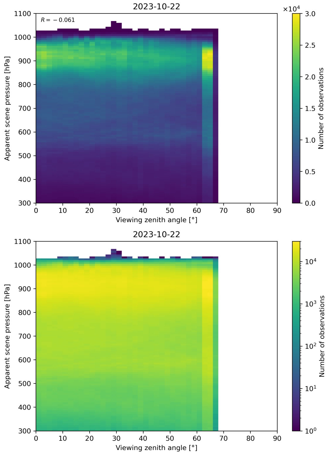
Figure 129: Scatter density plot of “Viewing zenith angle” against “Apparent scene pressure” for 2023-10-22 to 2023-10-23.
