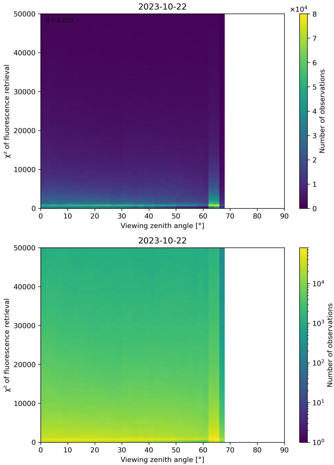
Figure 131: Scatter density plot of “Viewing zenith angle” against “ \chi^2 of fluorescence retrieval” for 2023-10-22 to 2023-10-23.
