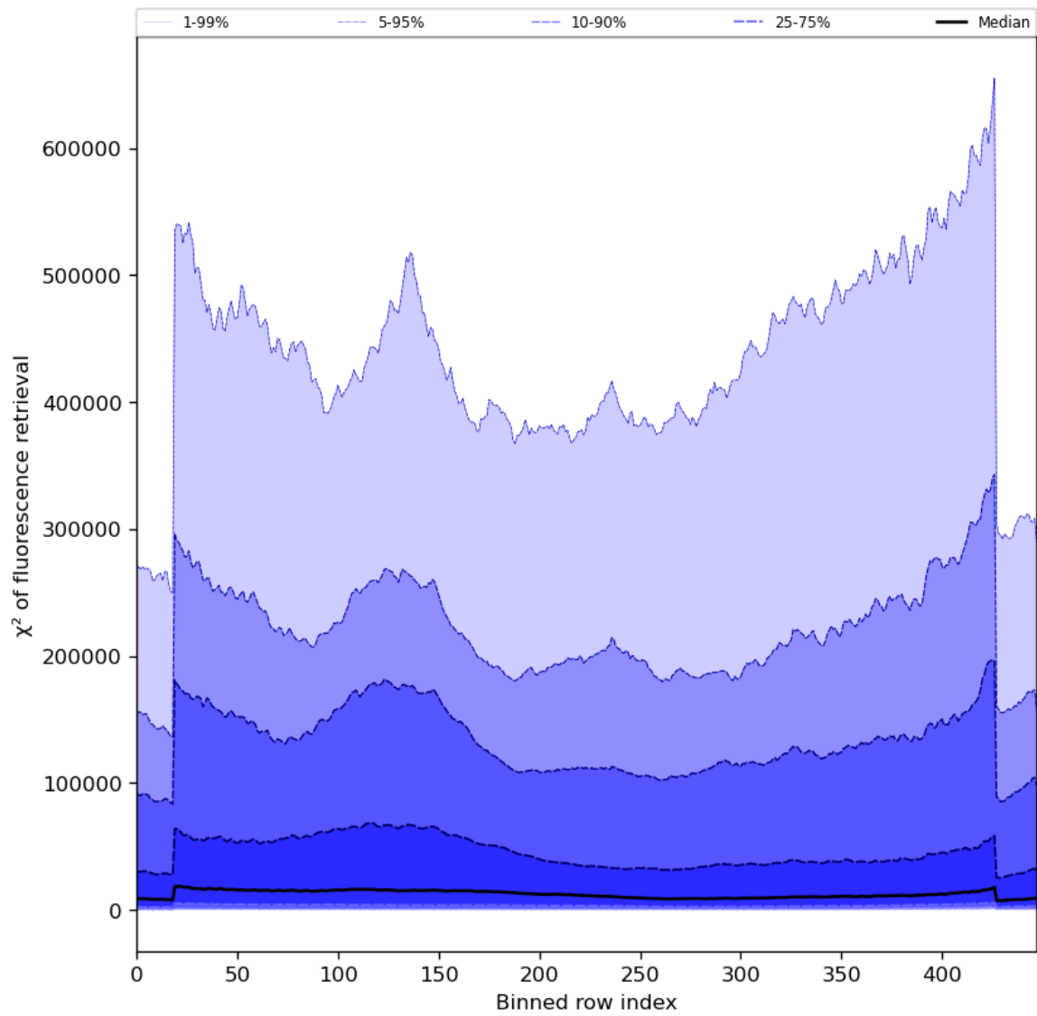
Figure 59: Along track statistics of “ \chi^2 of fluorescence retrieval” for 2023-10-22 to 2023-10-23
