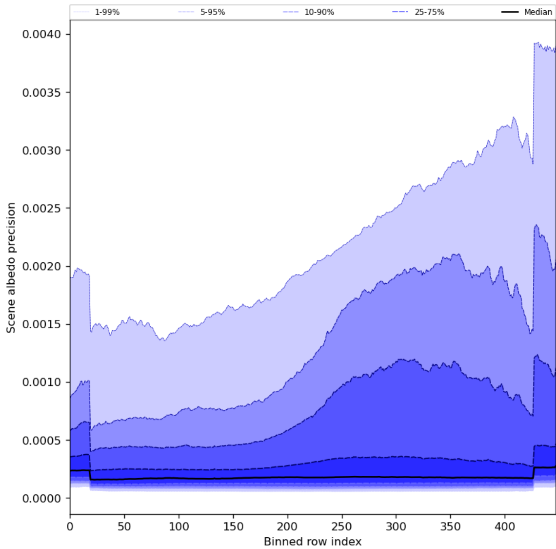
Figure 52: Along track statistics of “Scene albedo precision” for 2023-10-22 to 2023-10-23
