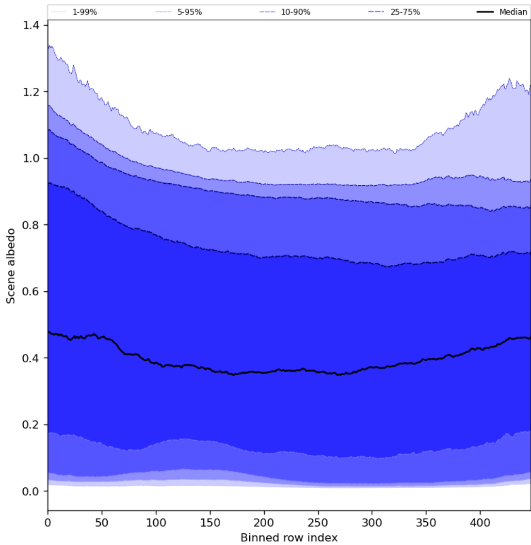
Figure 51: Along track statistics of “Scene albedo” for 2023-10-22 to 2023-10-23
