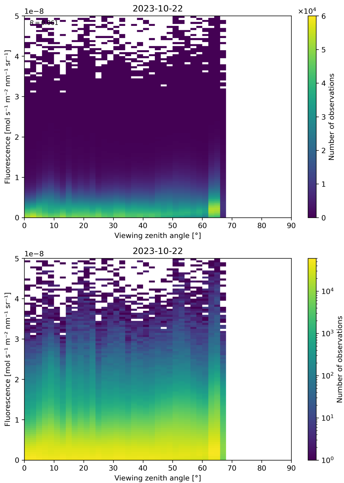
Figure 134: Scatter density plot of “Viewing zenith angle” against “Fluorescence” for 2023-10-22 to 2023-10-23.
