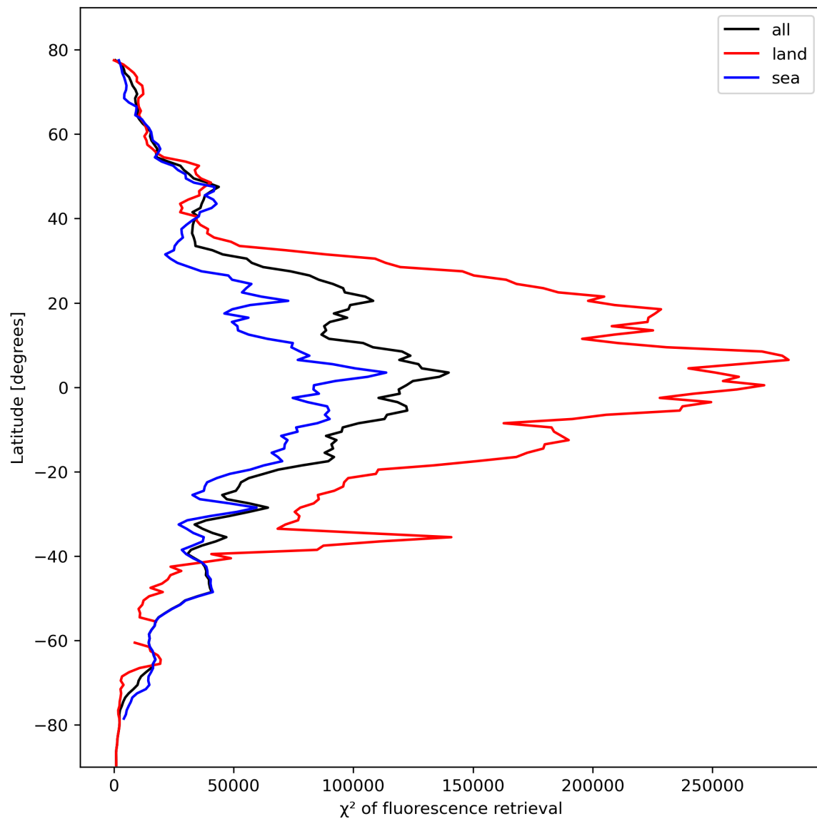
Figure 25: Zonal average of “ \chi^2 of fluorescence retrieval” for 2023-10-22 to 2023-10-23.
