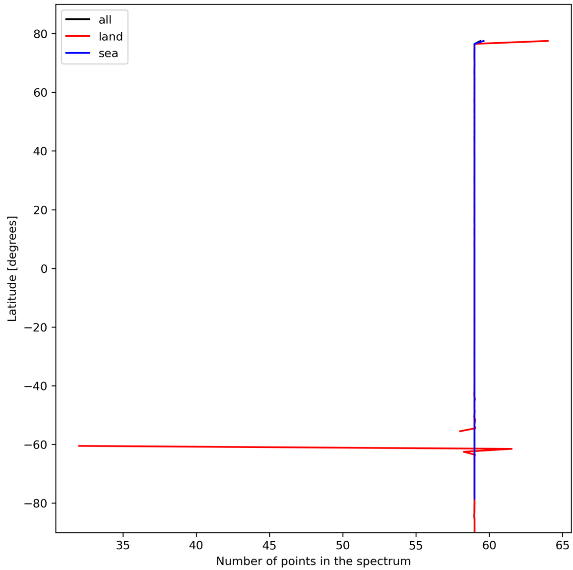
Figure 27: Zonal average of “Number of points in the spectrum” for 2023-10-22 to 2023-10-23.
