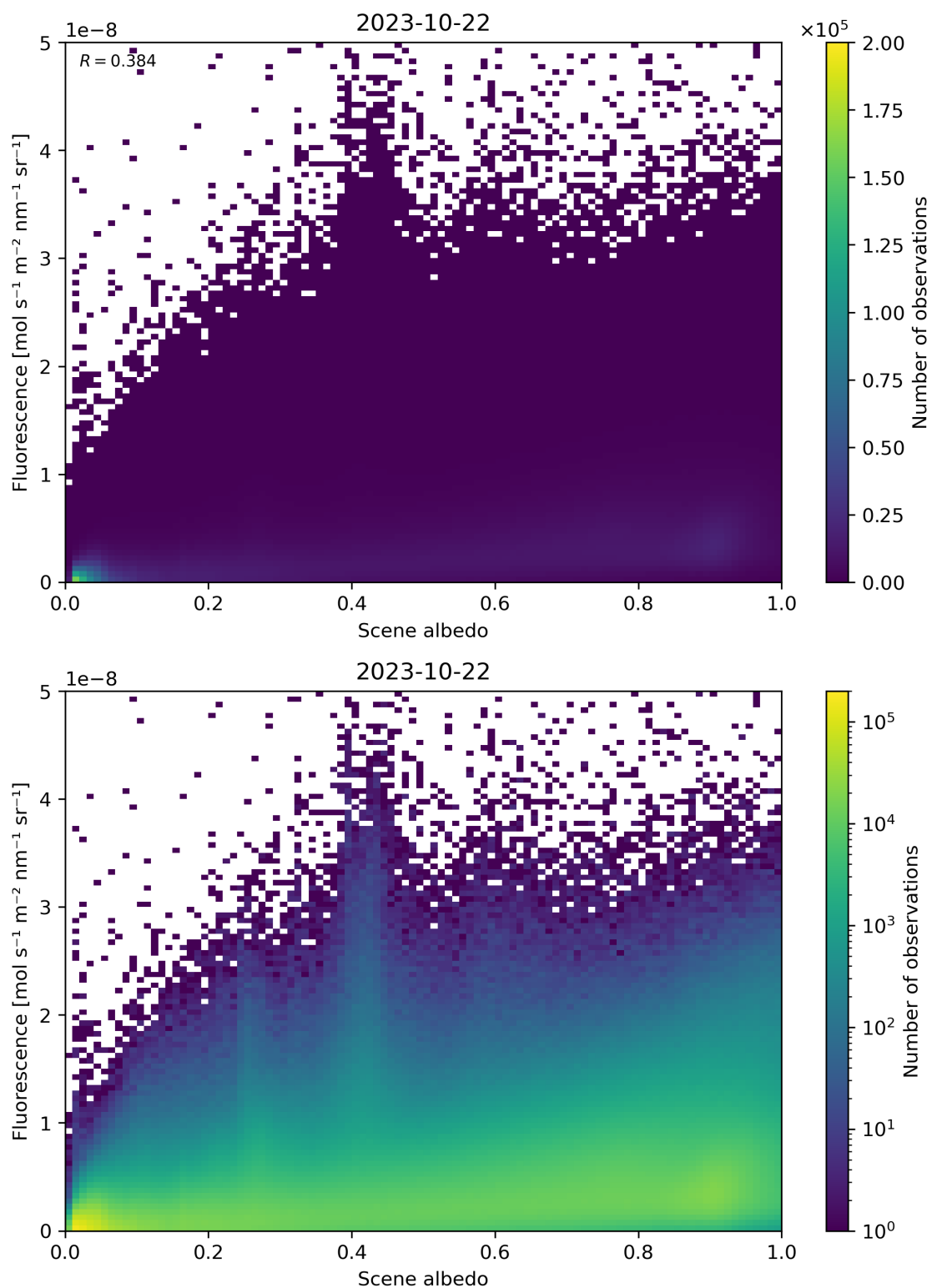
Figure 114: Scatter density plot of “Scene albedo” against “Fluorescence” for 2023-10-22 to 2023-10-23.
