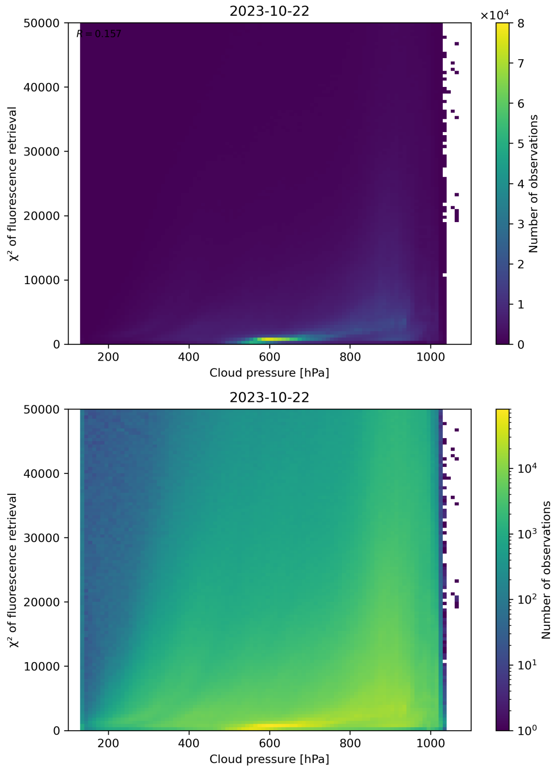
Figure 86: Scatter density plot of “Cloud pressure” against “ \chi^2 of fluorescence retrieval” for 2023-10-22 to 2023-10-23.
