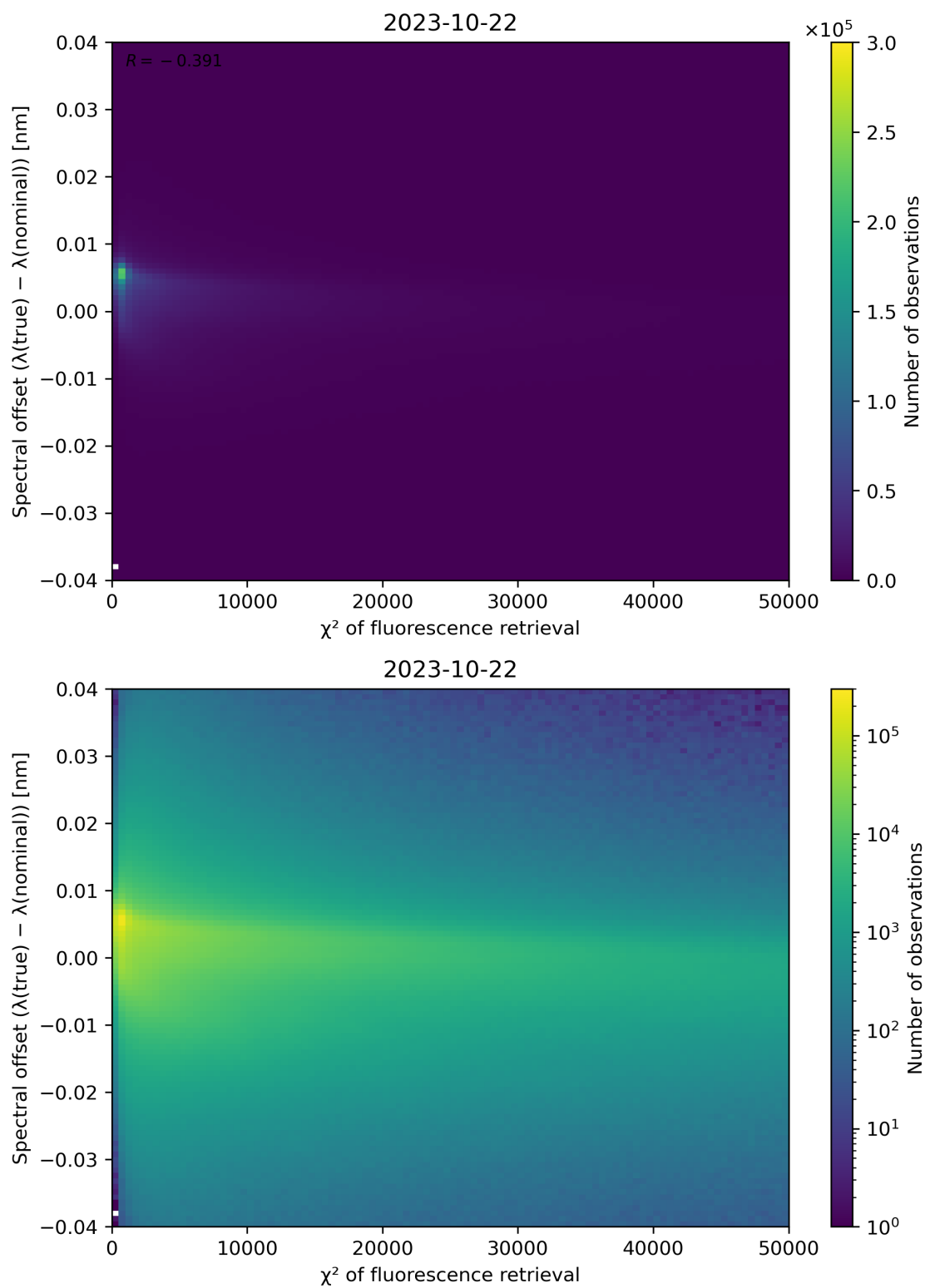
Figure 72: Scatter density plot of " \chi^2 of fluorescence retrieval" against "Spectral offset ( \lambda(\text{true}) - \lambda(\text{nominal}) )" for 2023-10-22 to 2023-10-23.
