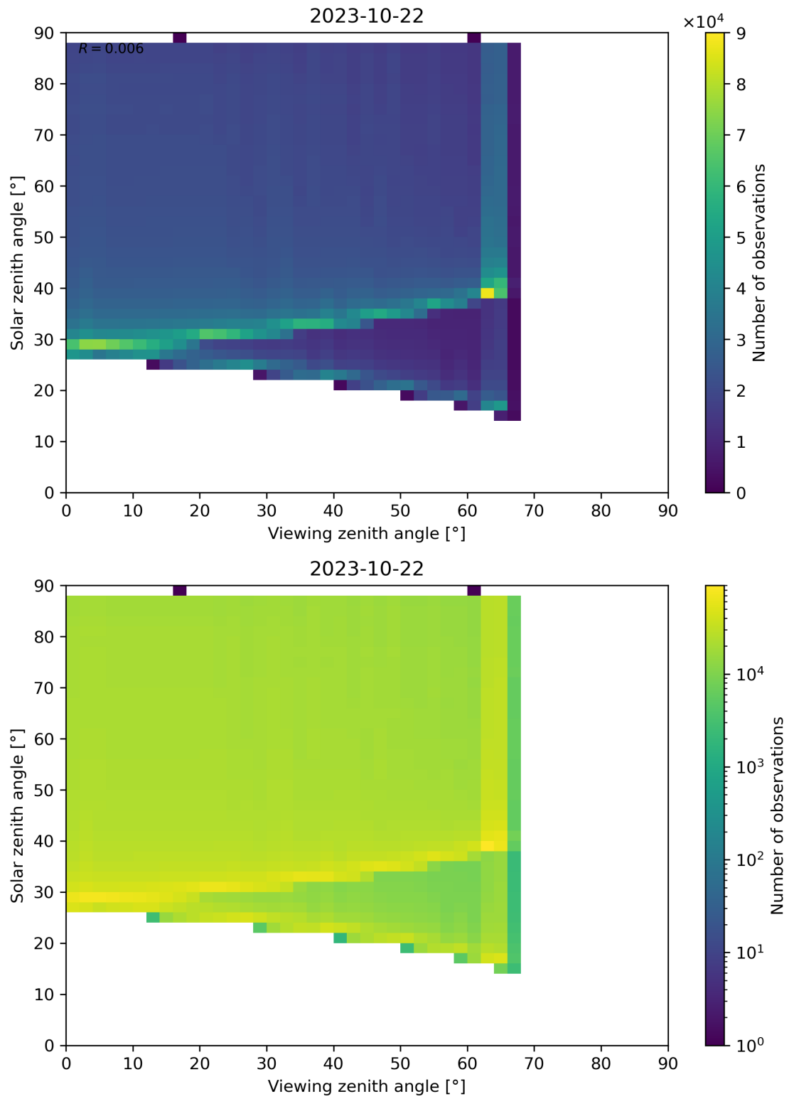
Figure 139: Scatter density plot of “Viewing zenith angle” against “Solar zenith angle” for 2023-10-22 to 2023-10-23.
