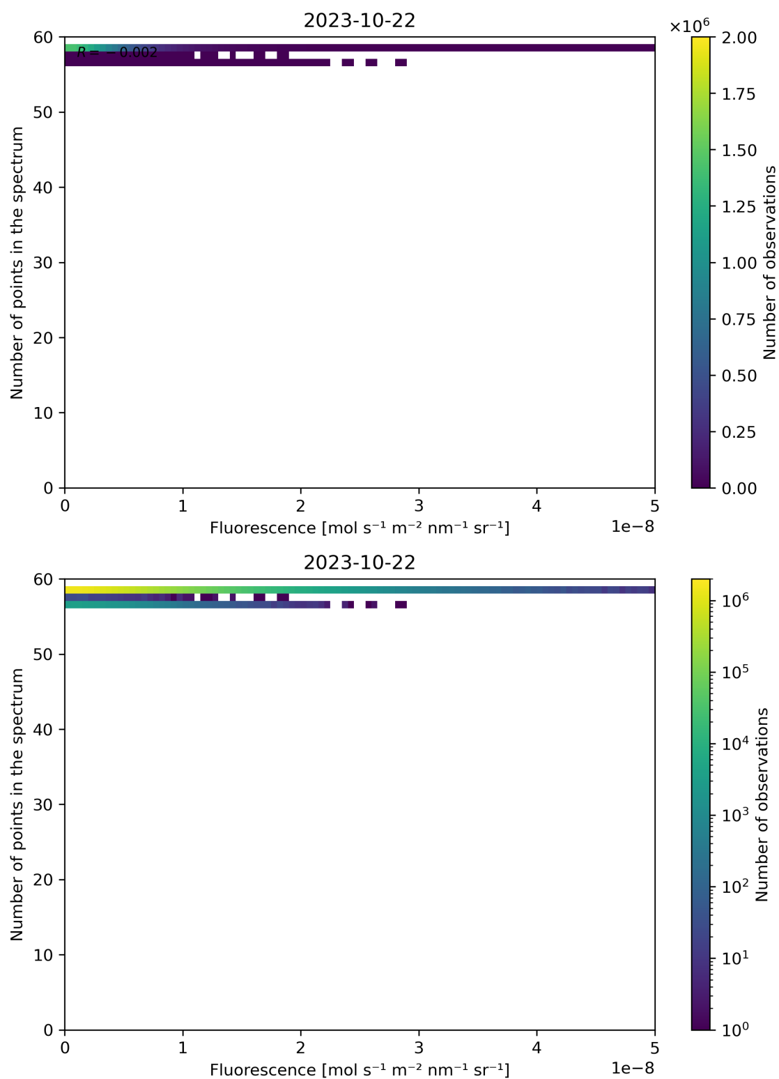
Figure 94: Scatter density plot of “Fluorescence” against “Number of points in the spectrum” for 2023-10-22 to 2023-10-23.
