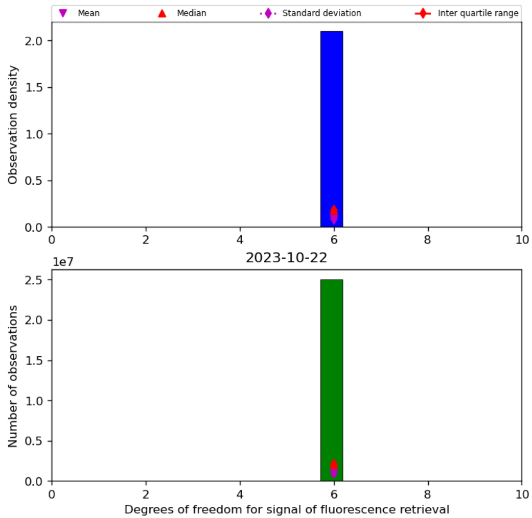
Figure 43: Histogram of “Degrees of freedom for signal of fluorescence retrieval” for 2023-10-22 to 2023-10-23
