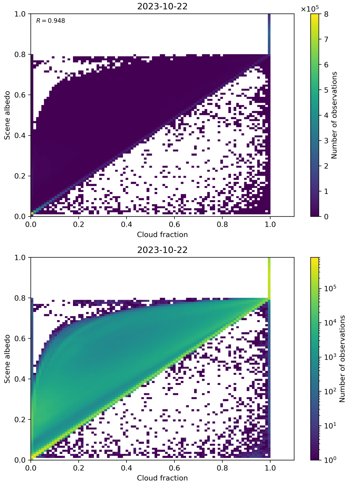
Figure 82: Scatter density plot of “Cloud fraction” against “Scene albedo” for 2023-10-22 to 2023-10-23.
