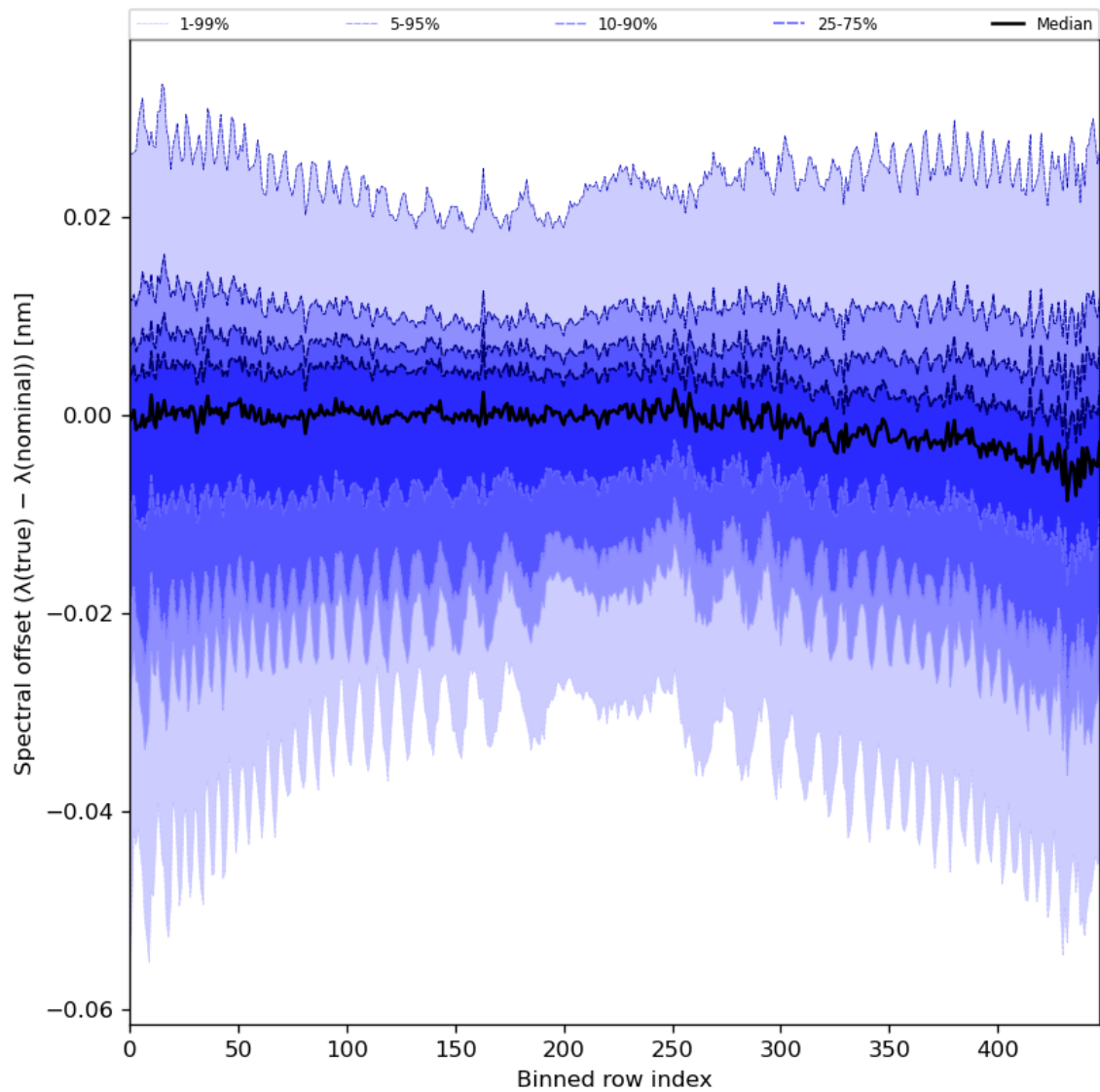
Figure 62: Along track statistics of “Spectral offset ( \lambda(\text{true}) - \lambda(\text{nominal}) )” for 2023-10-22 to 2023-10-23
