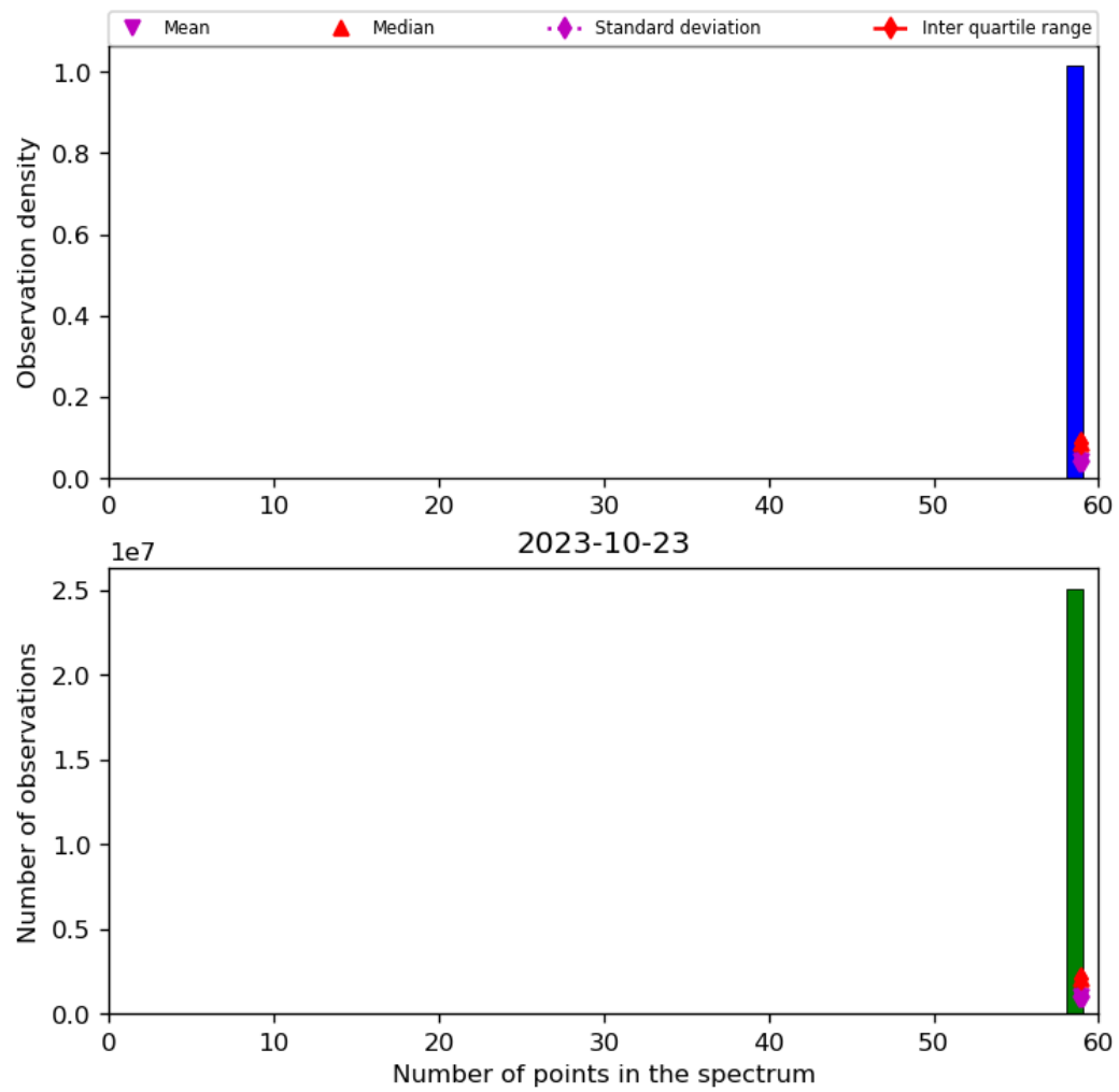
Figure 44: Histogram of "Number of points in the spectrum" for 2023-10-22 to 2023-10-24
