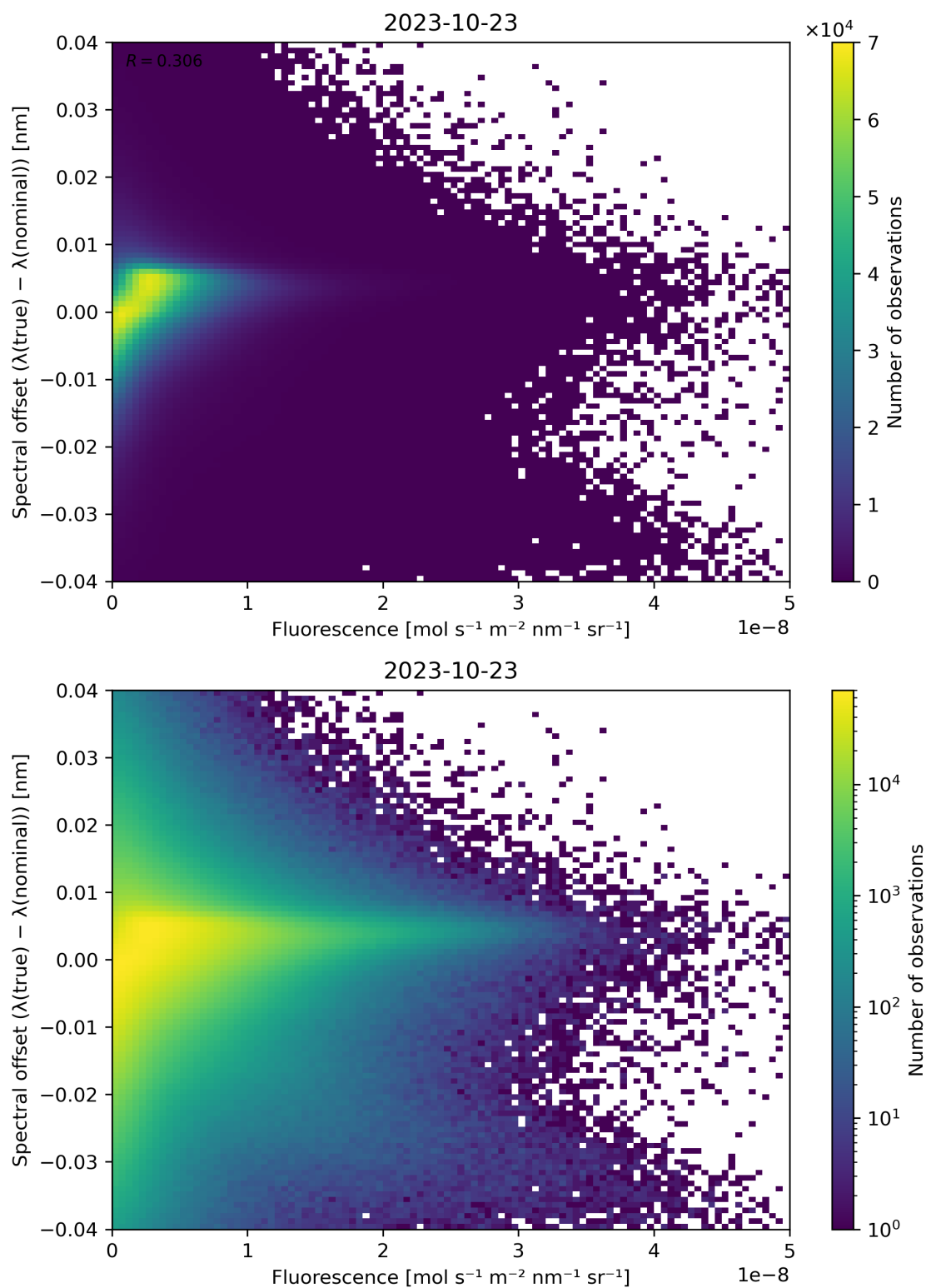
Figure 95: Scatter density plot of “Fluorescence” against “Spectral offset ( \lambda(\text{true}) - \lambda(\text{nominal}) )” for 2023-10-22 to 2023-10-24.
