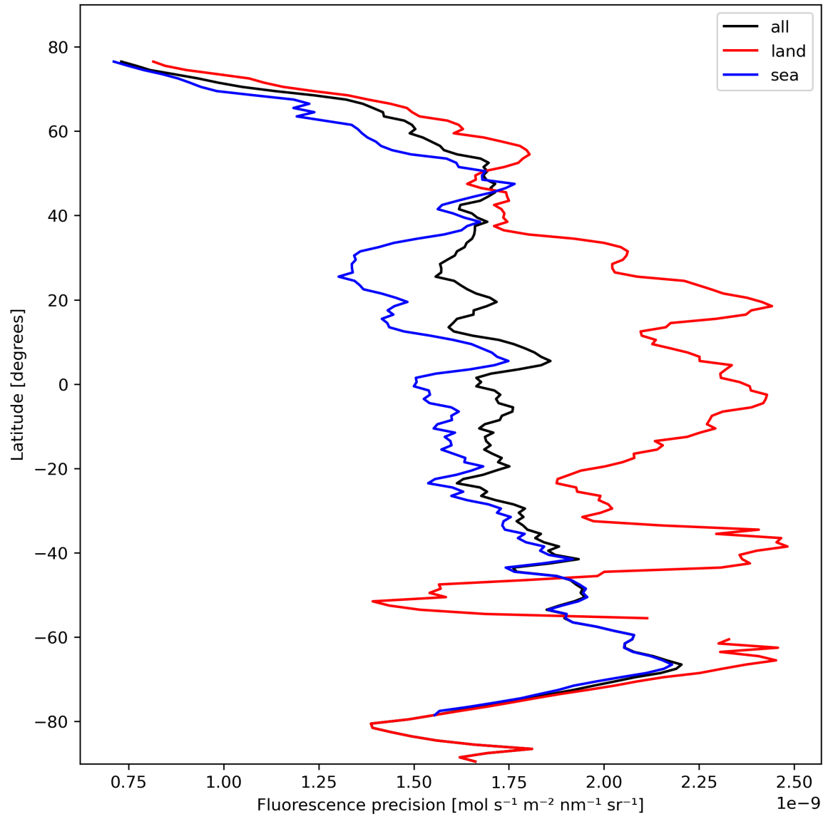
Figure 24: Zonal average of “Fluorescence precision” for 2023-10-22 to 2023-10-24.
