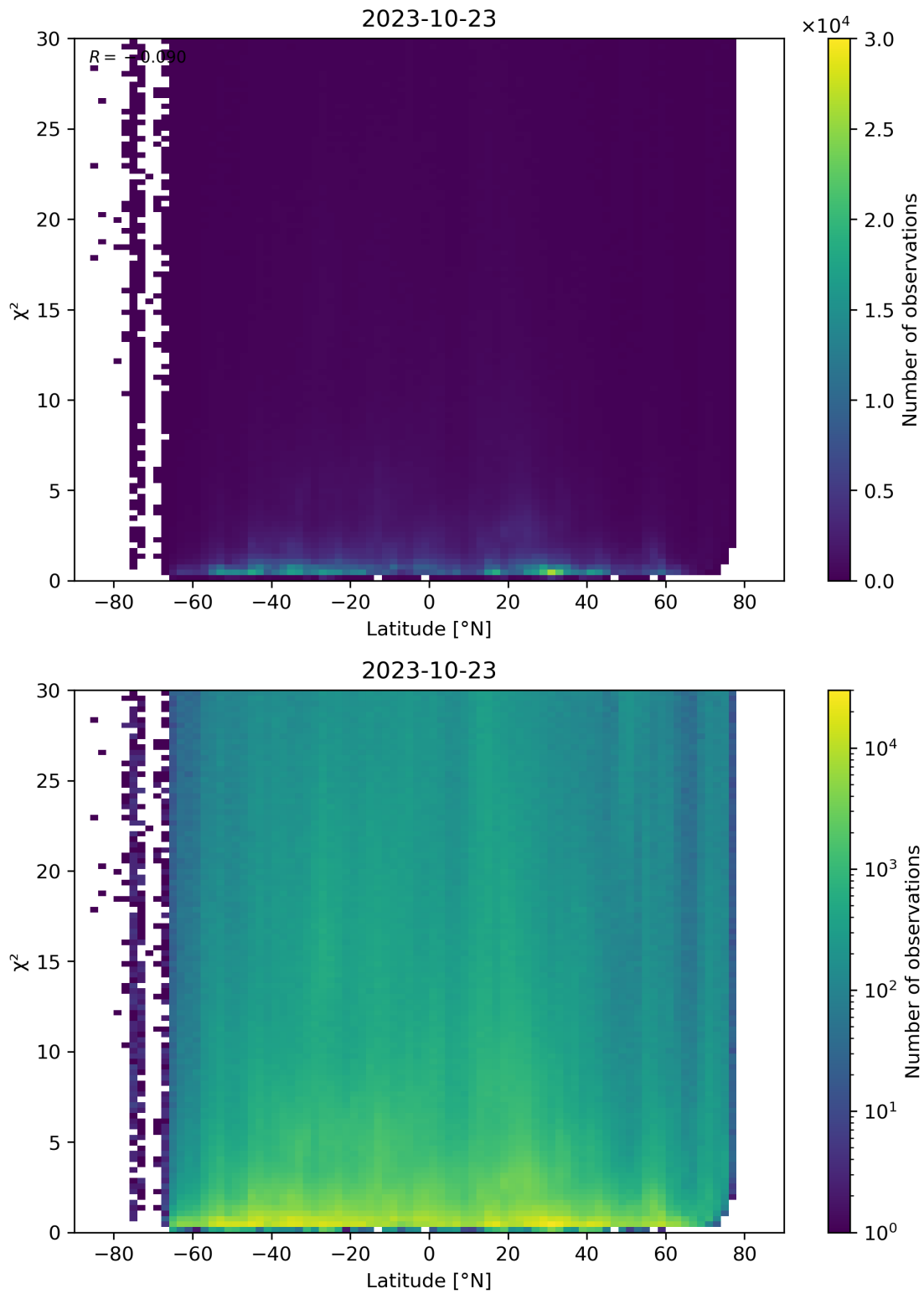
Figure 97: Scatter density plot of “Latitude” against “ \chi^2 ” for 2023-10-22 to 2023-10-24.
