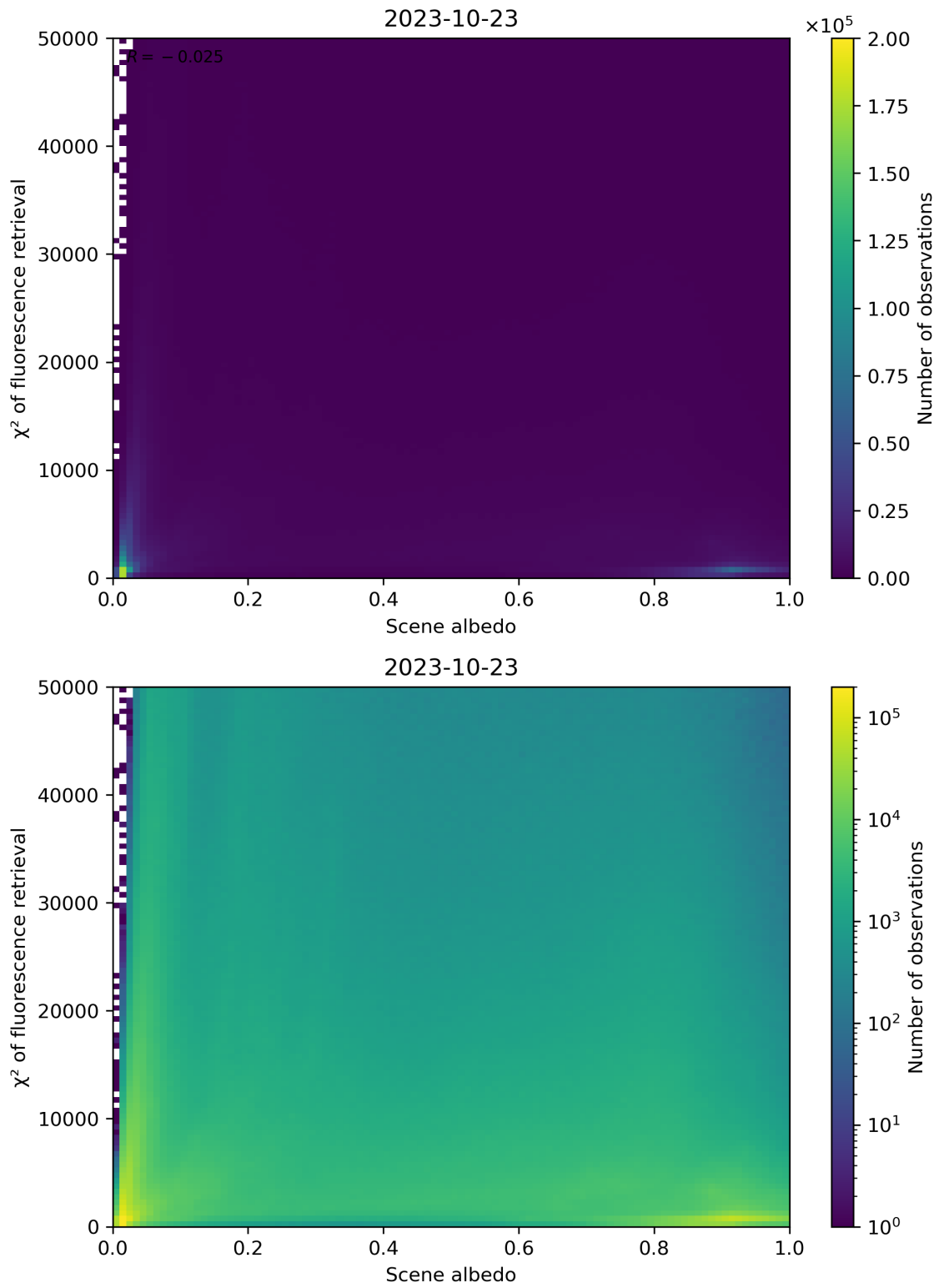
Figure 113: Scatter density plot of “Scene albedo” against “ \chi^2 of fluorescence retrieval” for 2023-10-22 to 2023-10-24.
