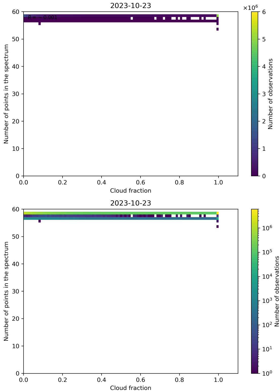
Figure 81: Scatter density plot of “Cloud fraction” against “Number of points in the spectrum” for 2023-10-22 to 2023-10-24.
