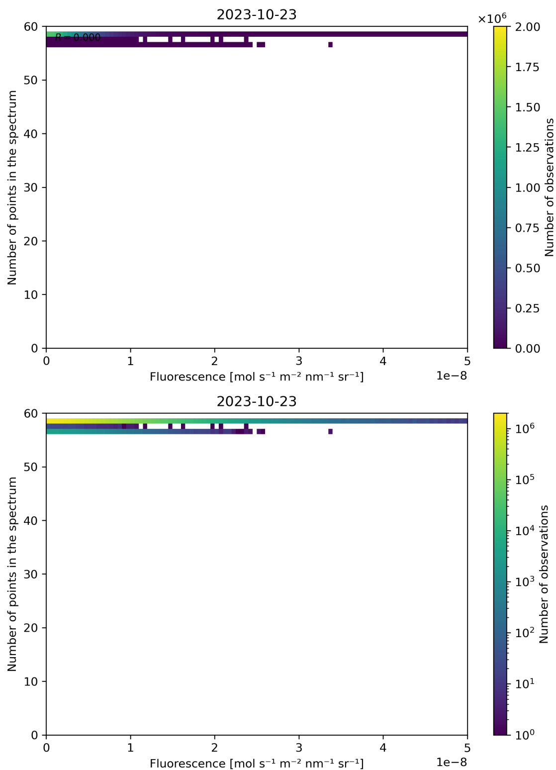
Figure 94: Scatter density plot of “Fluorescence” against “Number of points in the spectrum” for 2023-10-22 to 2023-10-24.
