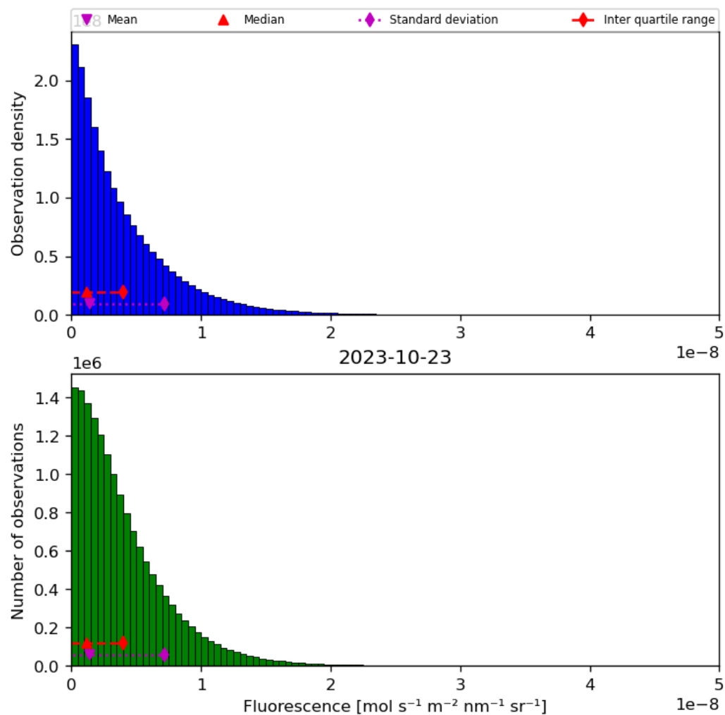
Figure 40: Histogram of “Fluorescence” for 2023-10-22 to 2023-10-24
