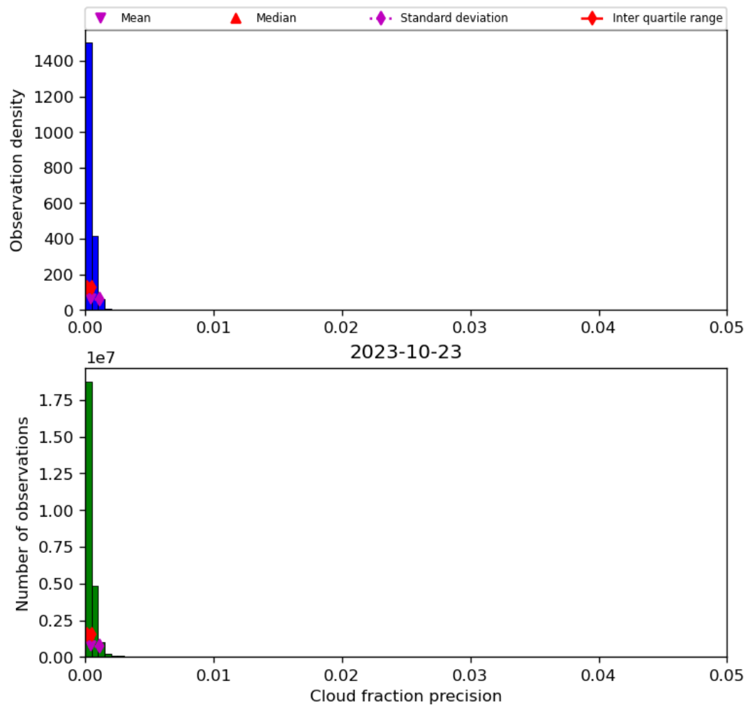
Figure 33: Histogram of “Cloud fraction precision” for 2023-10-22 to 2023-10-24
