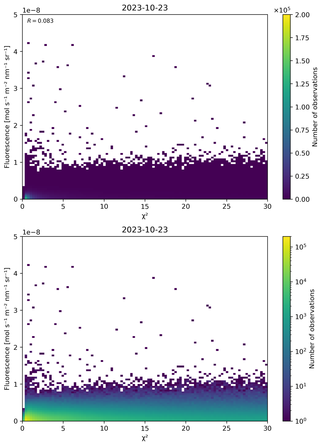
Figure 70: Scatter density plot of “ \chi^2 ” against “Fluorescence” for 2023-10-22 to 2023-10-24.
