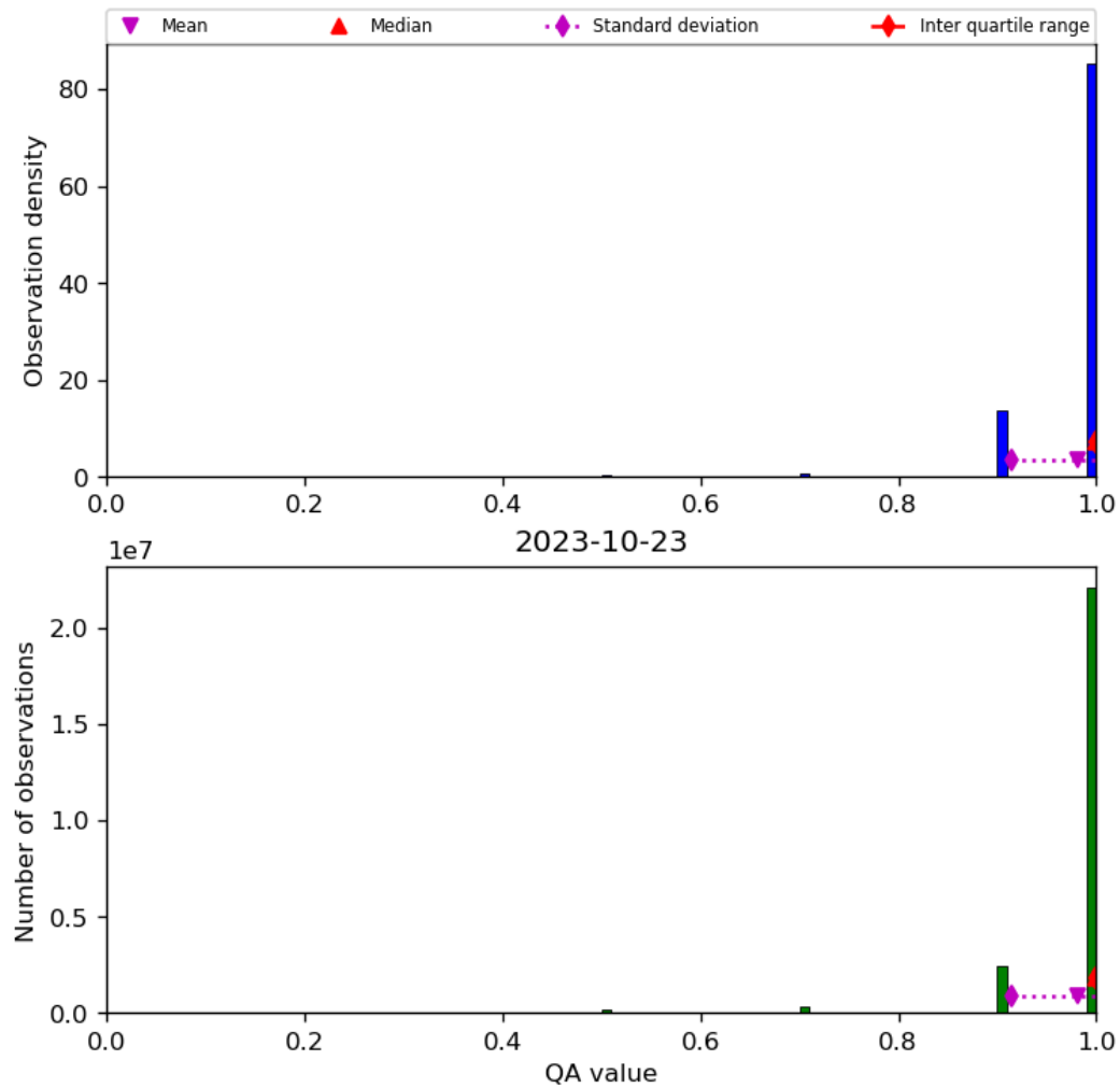
Figure 29: Histogram of “QA value” for 2023-10-22 to 2023-10-24
