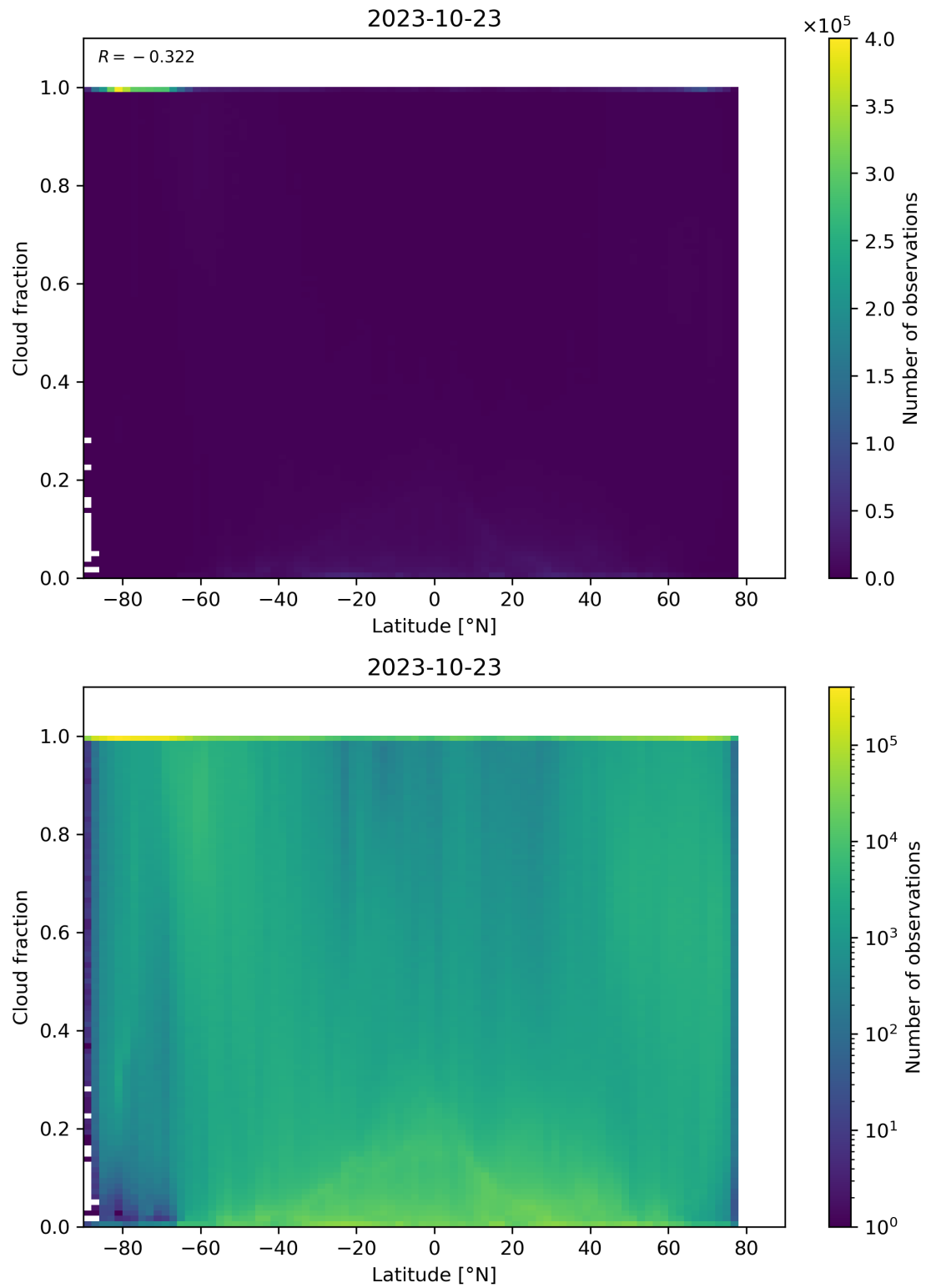
Figure 99: Scatter density plot of “Latitude” against “Cloud fraction” for 2023-10-22 to 2023-10-24.
