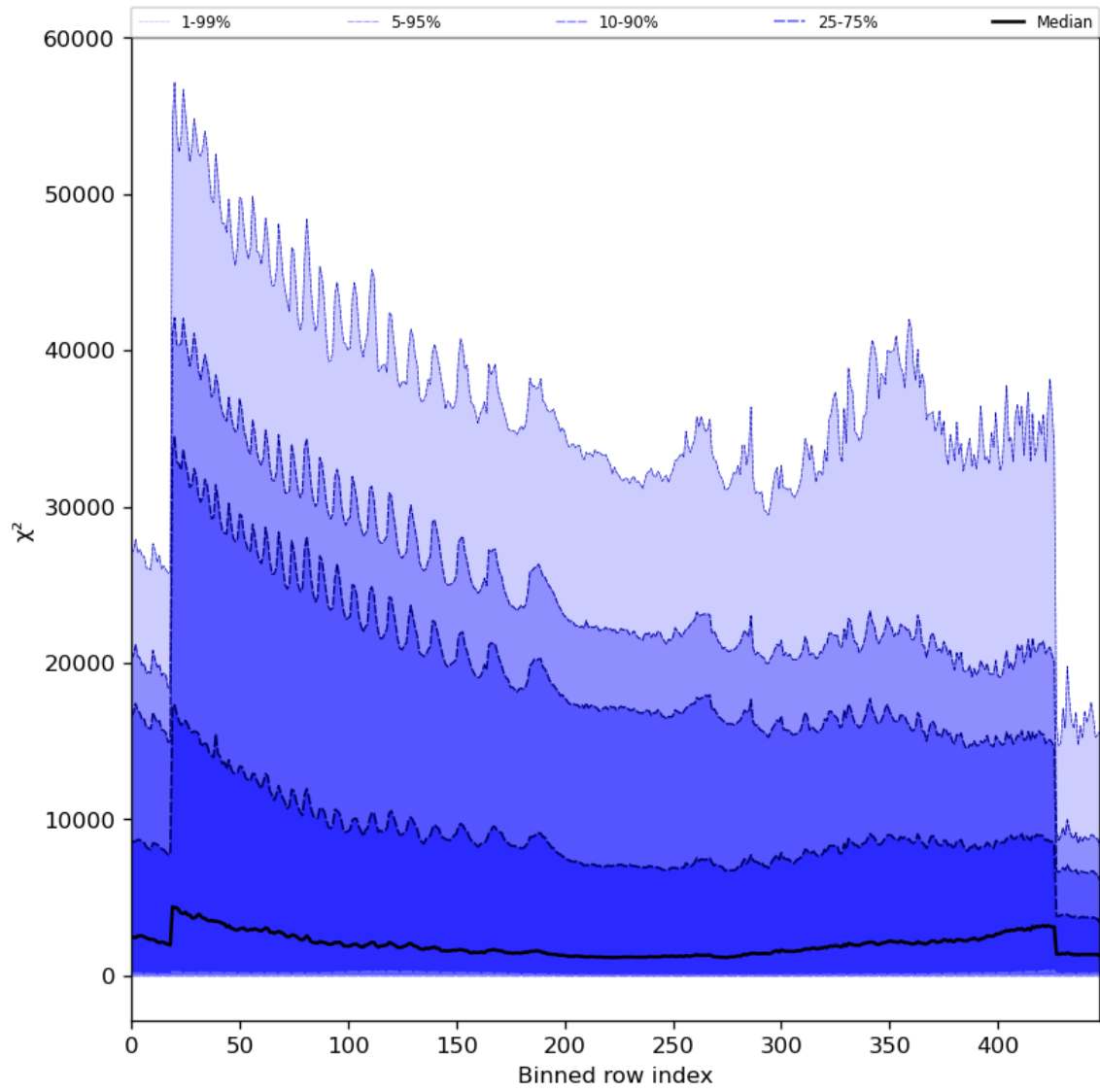
Figure 55: Along track statistics of “ \chi^2 ” for 2023-10-22 to 2023-10-24
