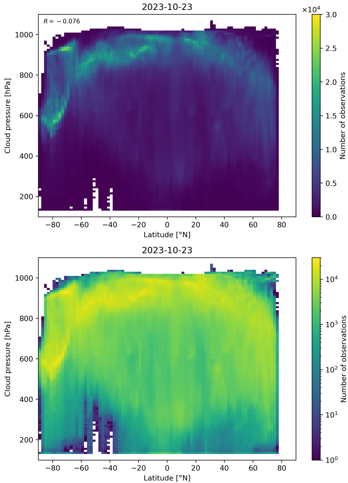
Figure 100: Scatter density plot of “Latitude” against “Cloud pressure” for 2023-10-22 to 2023-10-24.
