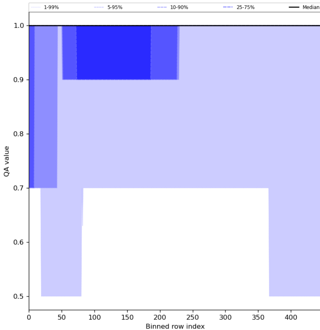
Figure 46: Along track statistics of “QA value” for 2023-10-22 to 2023-10-24
