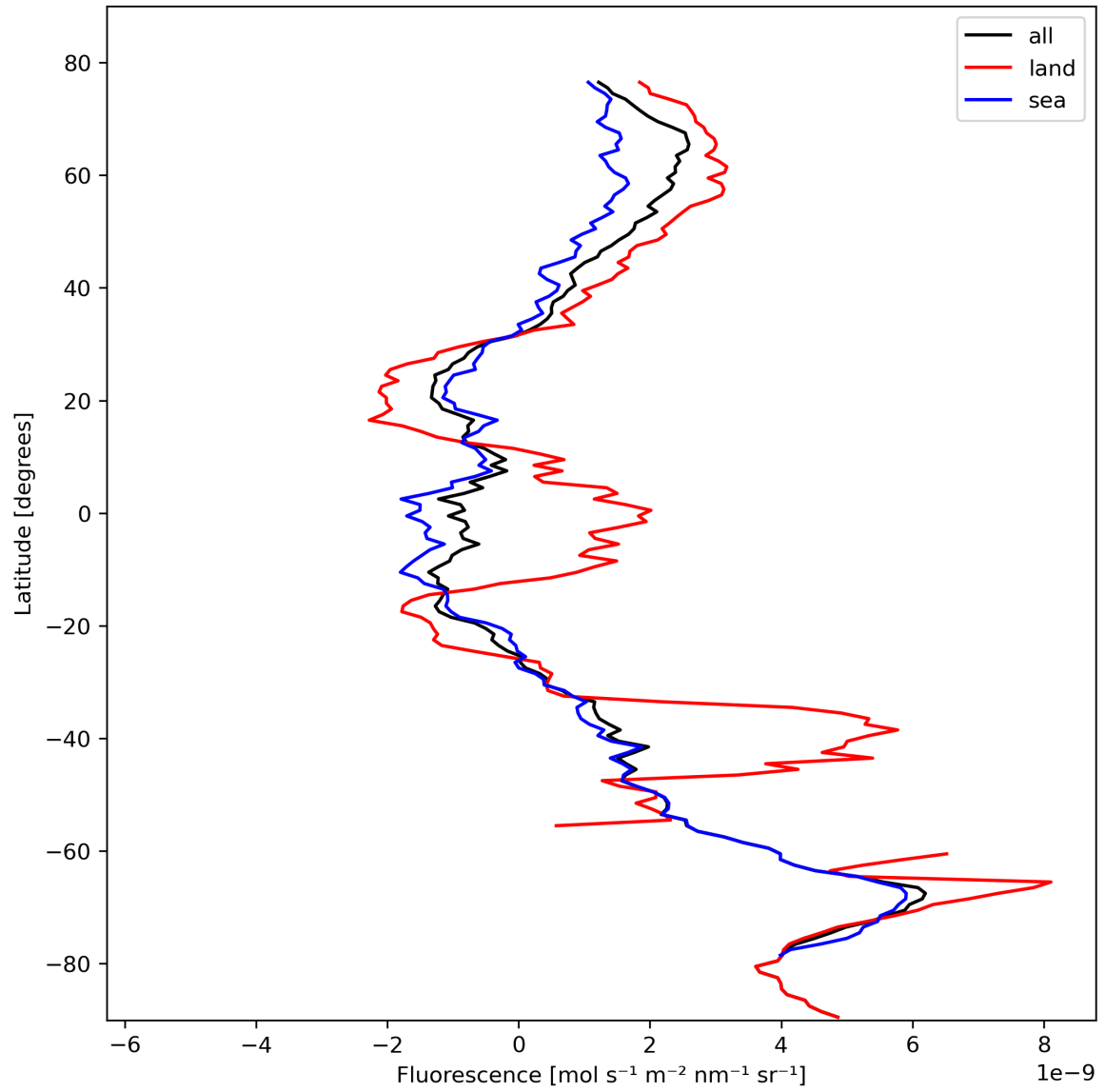
Figure 23: Zonal average of “Fluorescence” for 2023-10-22 to 2023-10-24.
