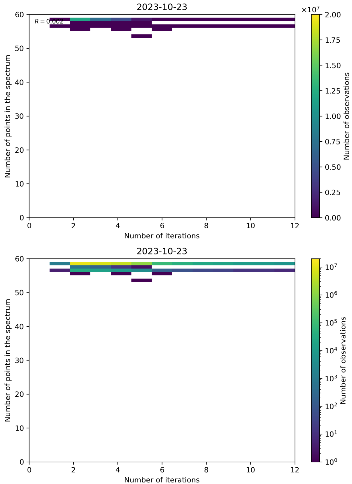
Figure 108: Scatter density plot of “Number of iterations” against “Number of points in the spectrum” for 2023-10-22 to 2023-10-24.
