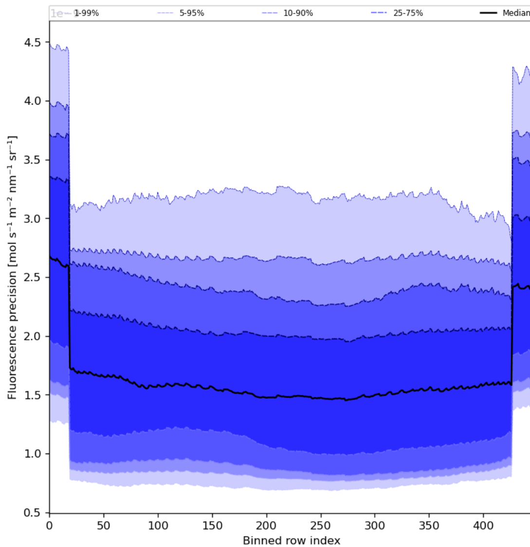
Figure 58: Along track statistics of “Fluorescence precision” for 2023-10-22 to 2023-10-24
