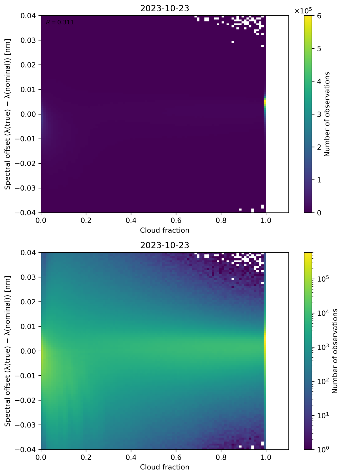
Figure 83: Scatter density plot of “Cloud fraction” against “Spectral offset ( \lambda(\text{true}) - \lambda(\text{nominal}) )” for 2023-10-22 to 2023-10-24.
