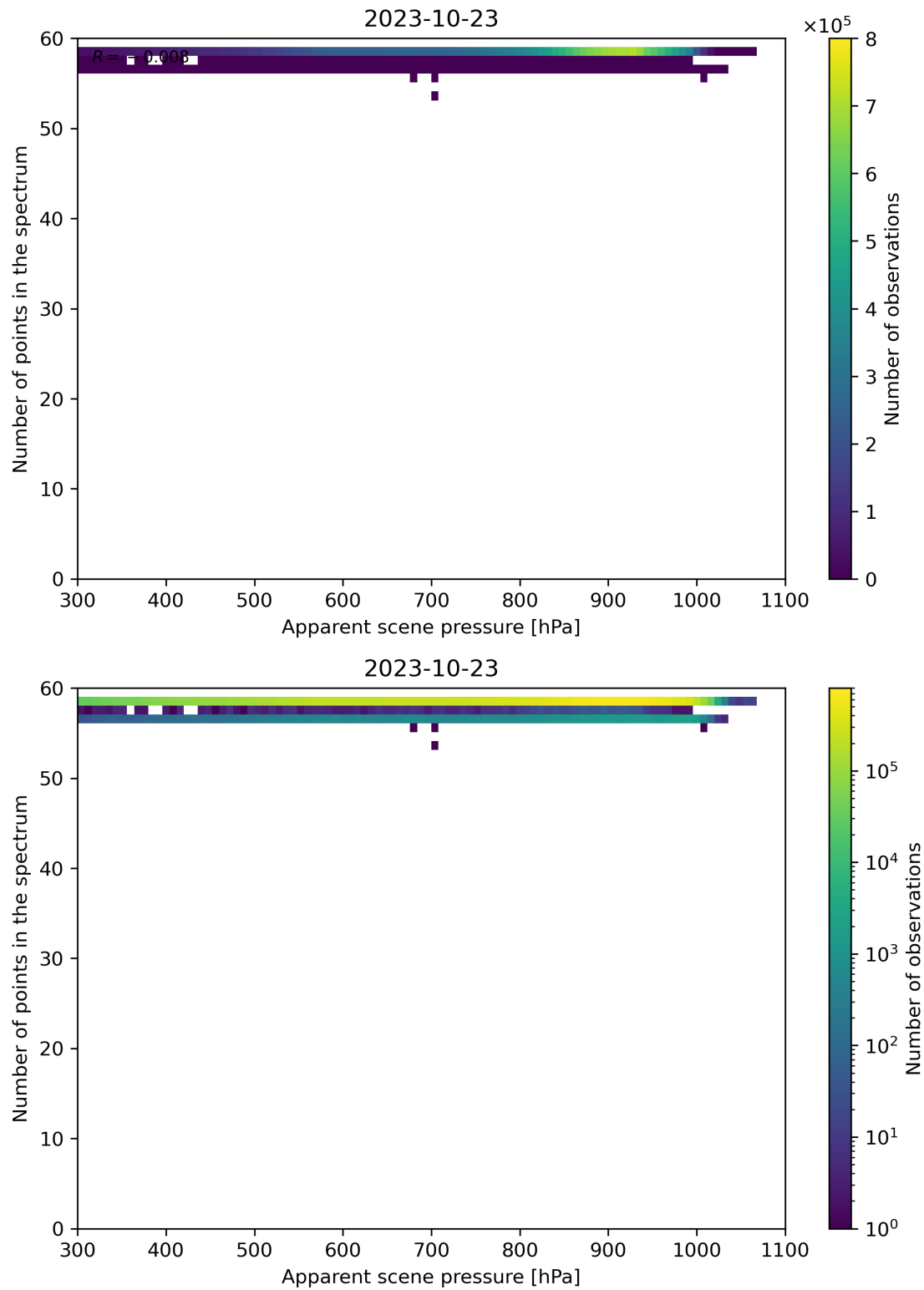
Figure 67: Scatter density plot of “Apparent scene pressure” against “Number of points in the spectrum” for 2023-10-22 to 2023-10-24.
