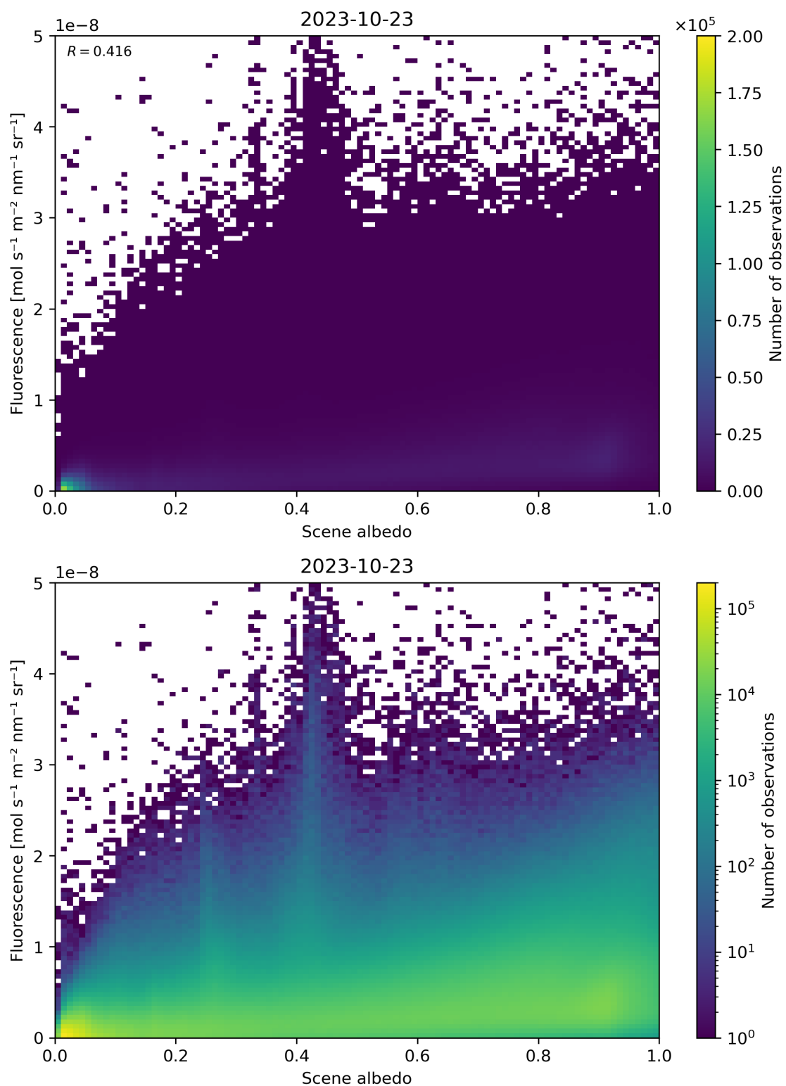
Figure 114: Scatter density plot of “Scene albedo” against “Fluorescence” for 2023-10-22 to 2023-10-24.
