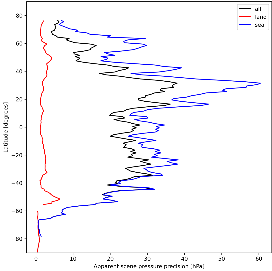
Figure 20: Zonal average of “Apparent scene pressure precision” for 2023-10-22 to 2023-10-24.
