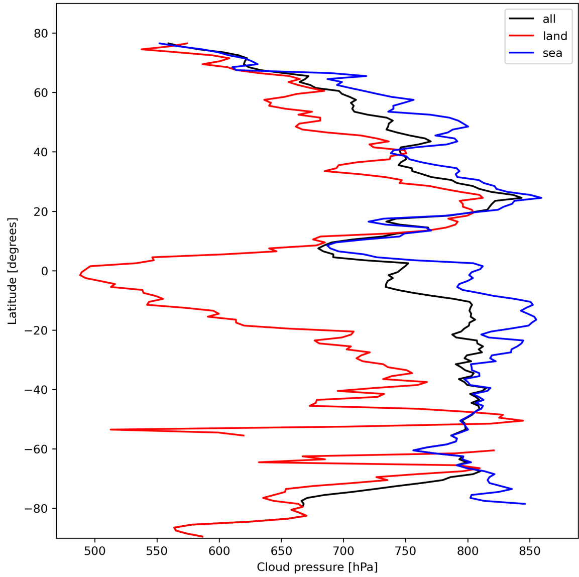
Figure 13: Zonal average of “Cloud pressure” for 2023-10-22 to 2023-10-24.
