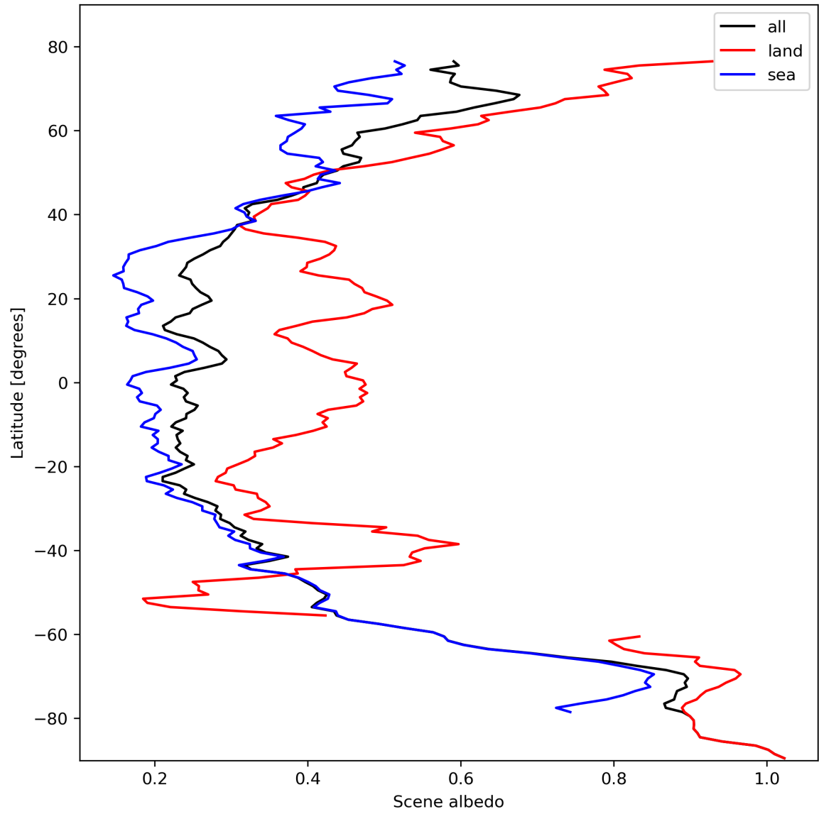
Figure 17: Zonal average of “Scene albedo” for 2023-10-22 to 2023-10-24.
