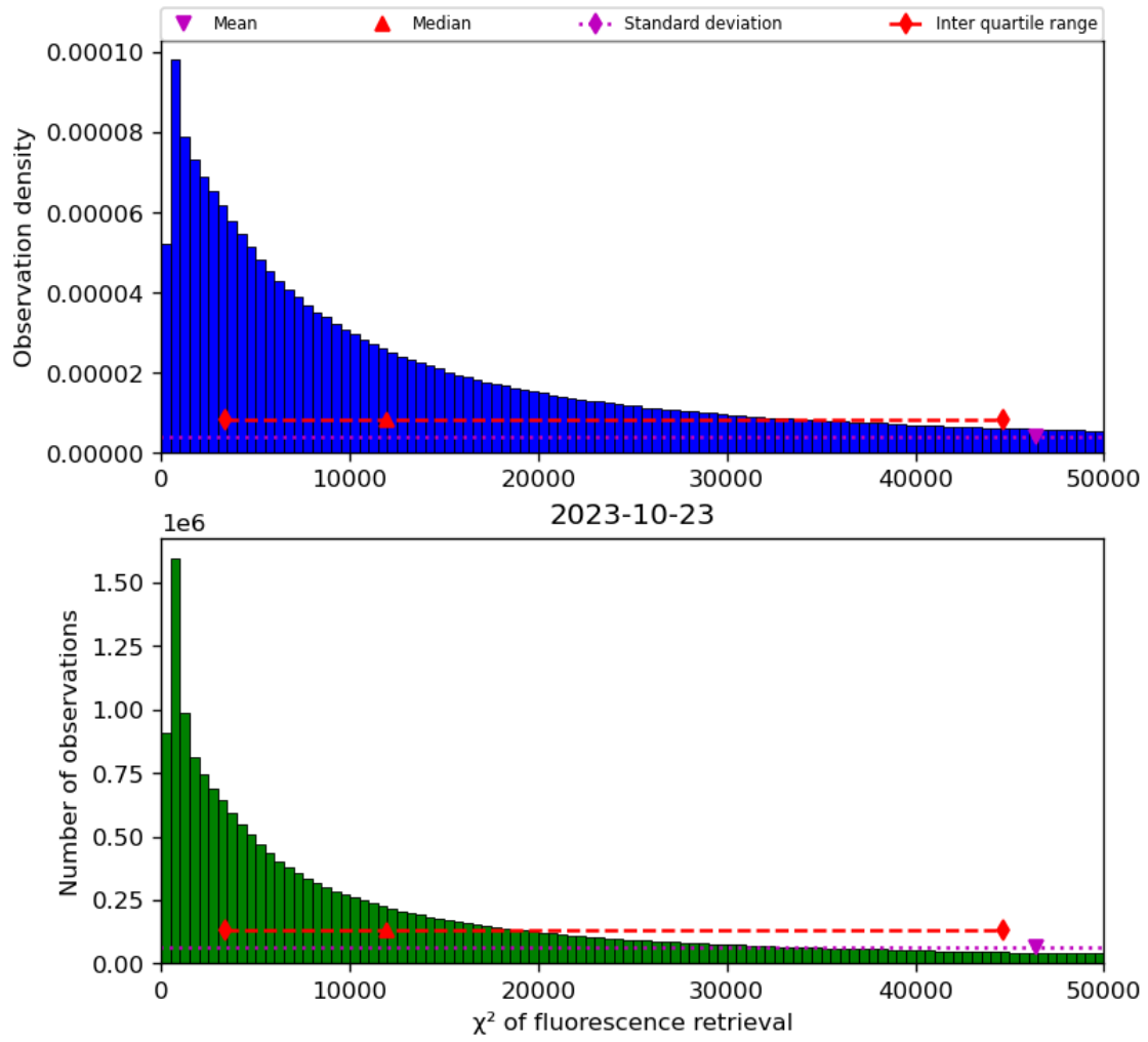
Figure 42: Histogram of “ \chi^2 of fluorescence retrieval” for 2023-10-22 to 2023-10-24
