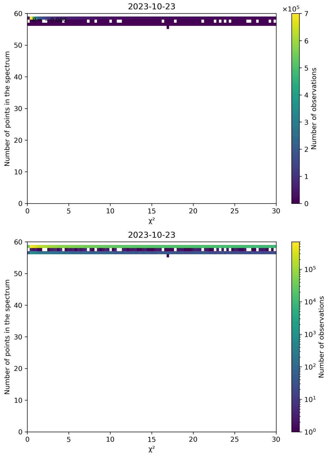
Figure 74: Scatter density plot of " \chi^2 " against "Number of points in the spectrum" for 2023-10-22 to 2023-10-24.
