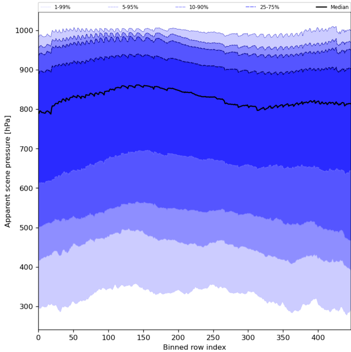
Figure 53: Along track statistics of “Apparent scene pressure” for 2023-10-22 to 2023-10-24
