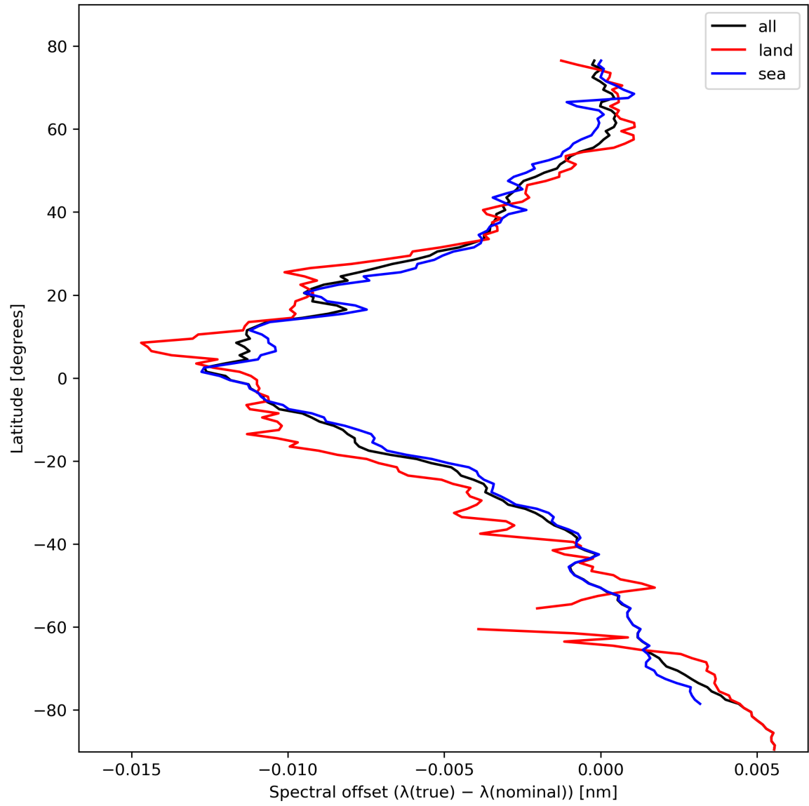
Figure 28: Zonal average of “Spectral offset ( \lambda(\text{true}) - \lambda(\text{nominal}) )” for 2023-10-22 to 2023-10-24.
