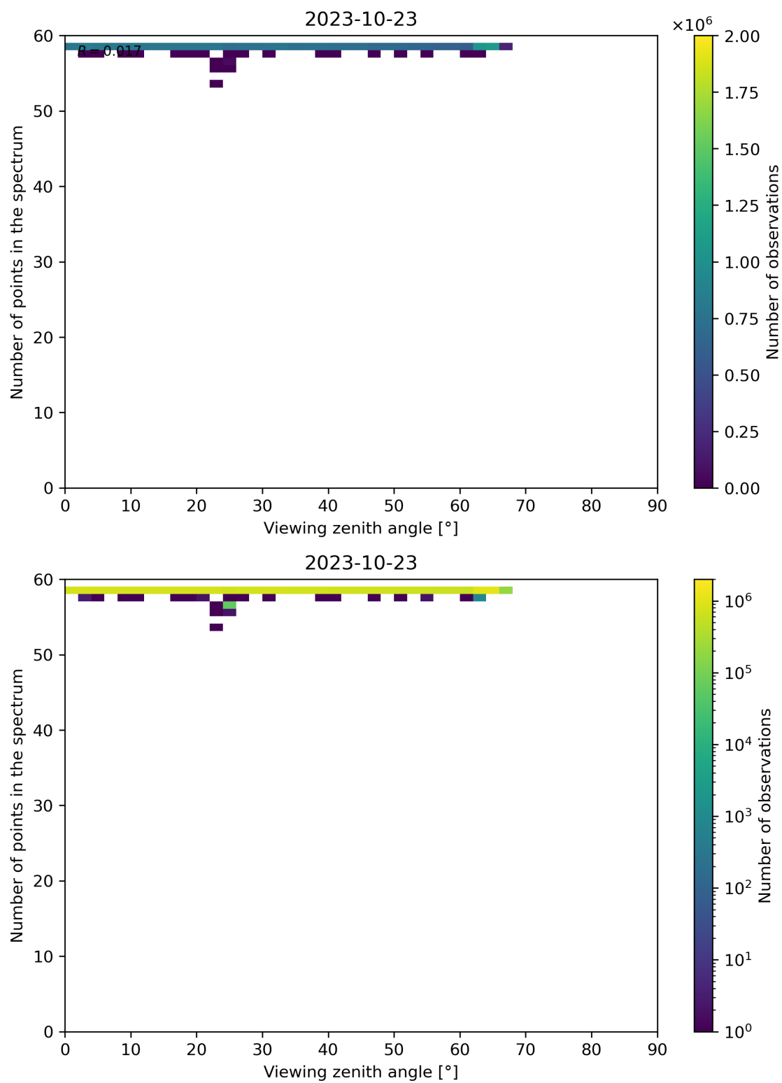
Figure 137: Scatter density plot of “Viewing zenith angle” against “Number of points in the spectrum” for 2023-10-22 to 2023-10-24.
