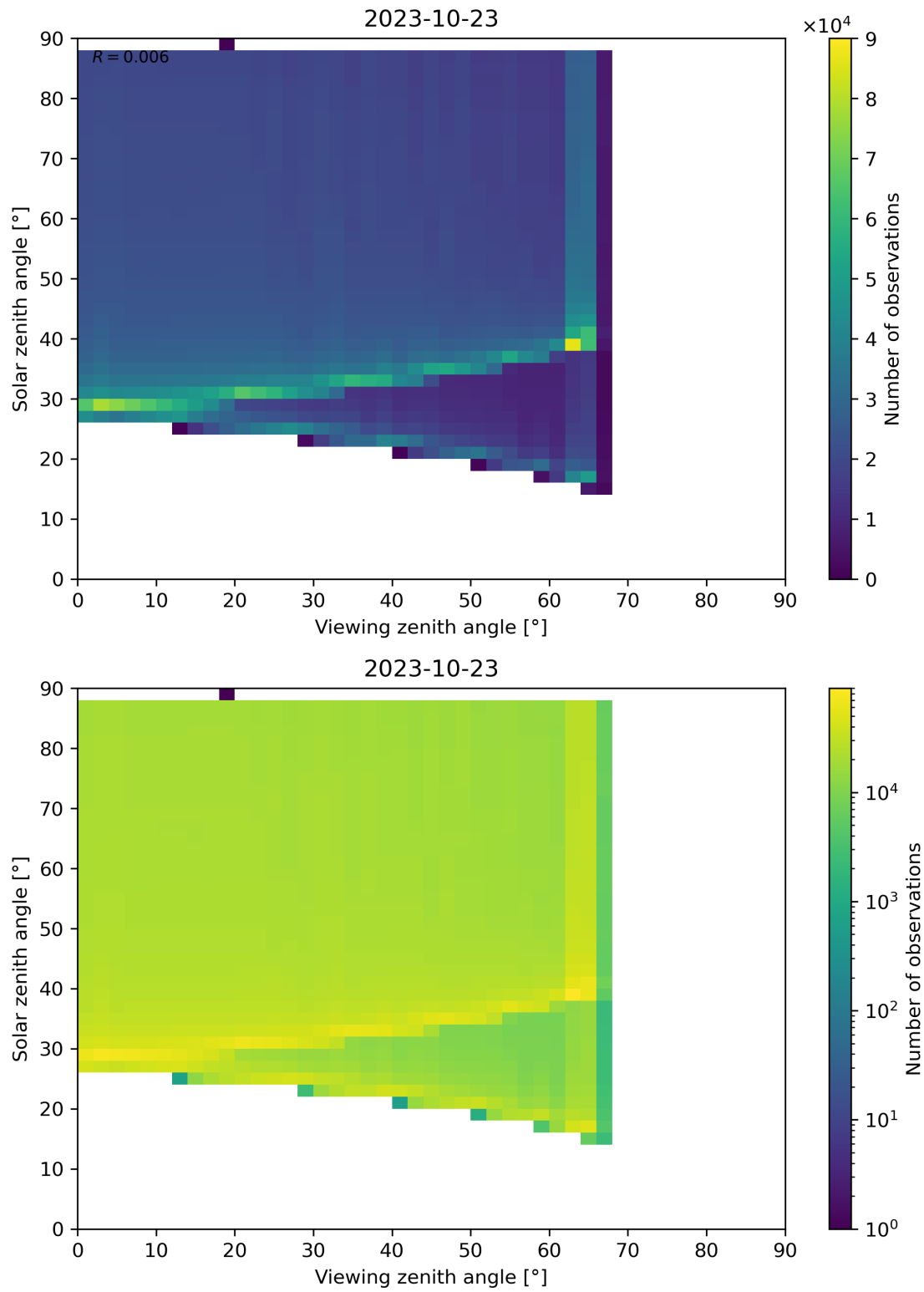
Figure 139: Scatter density plot of “Viewing zenith angle” against “Solar zenith angle” for 2023-10-22 to 2023-10-24.
