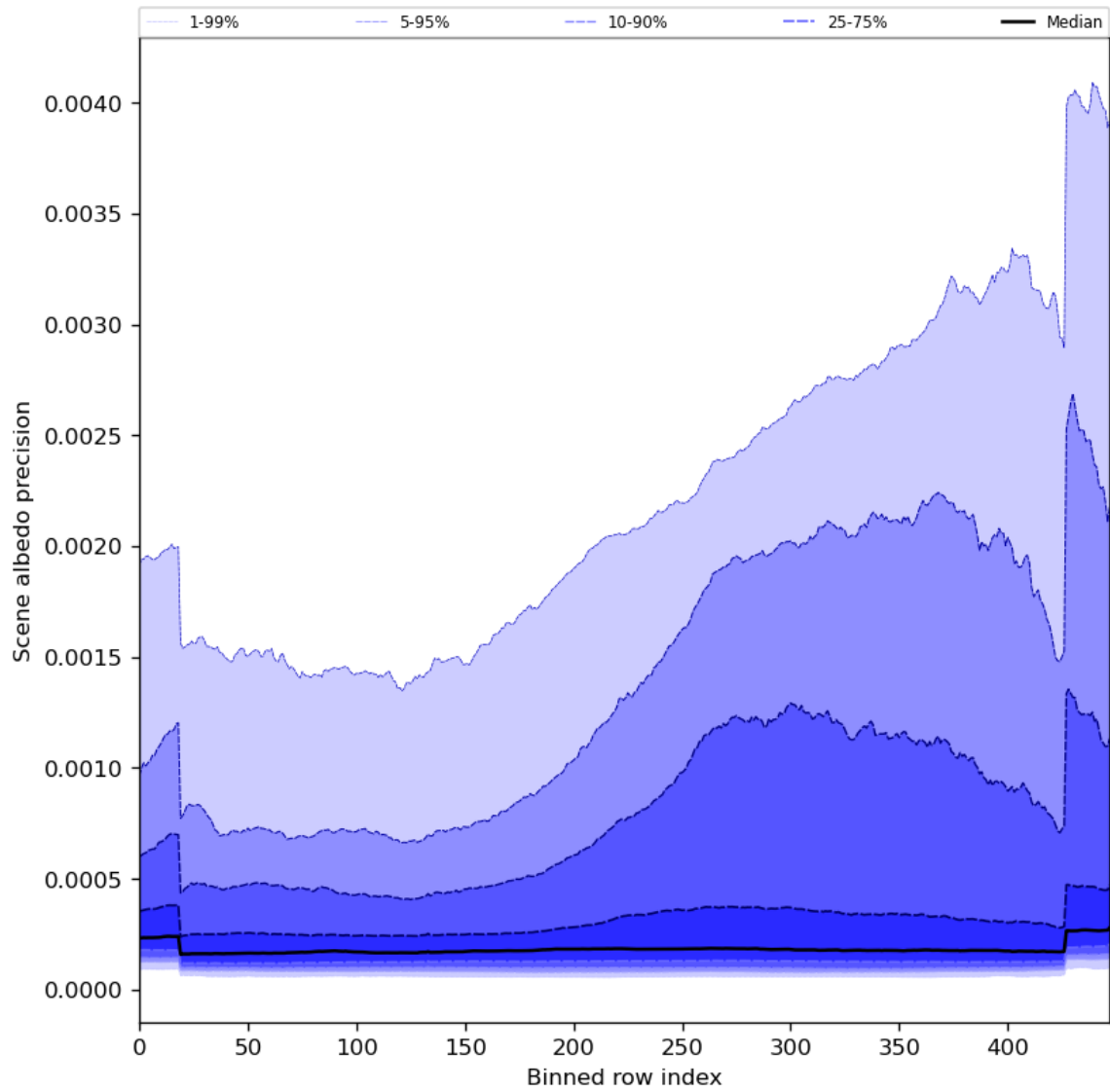
Figure 52: Along track statistics of “Scene albedo precision” for 2023-10-22 to 2023-10-24
