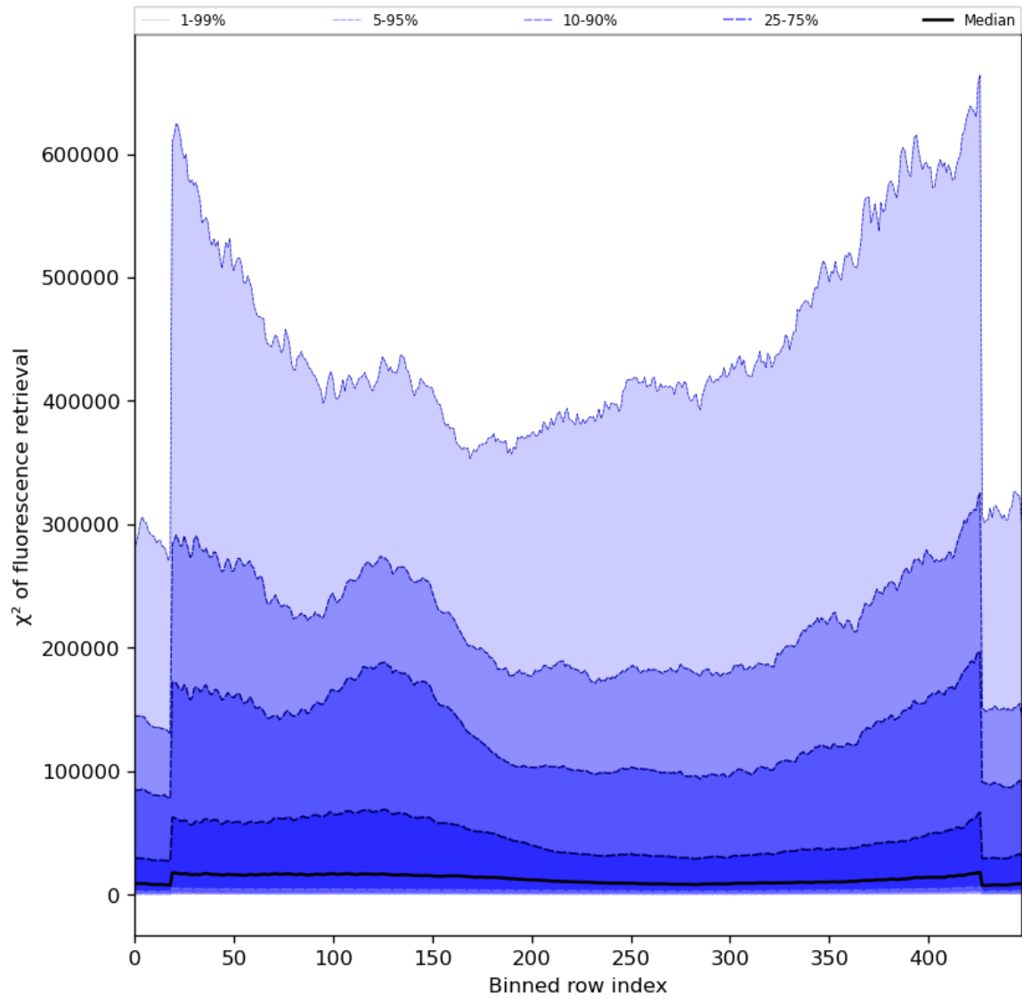
Figure 59: Along track statistics of “ \chi^2 of fluorescence retrieval” for 2023-10-22 to 2023-10-24
