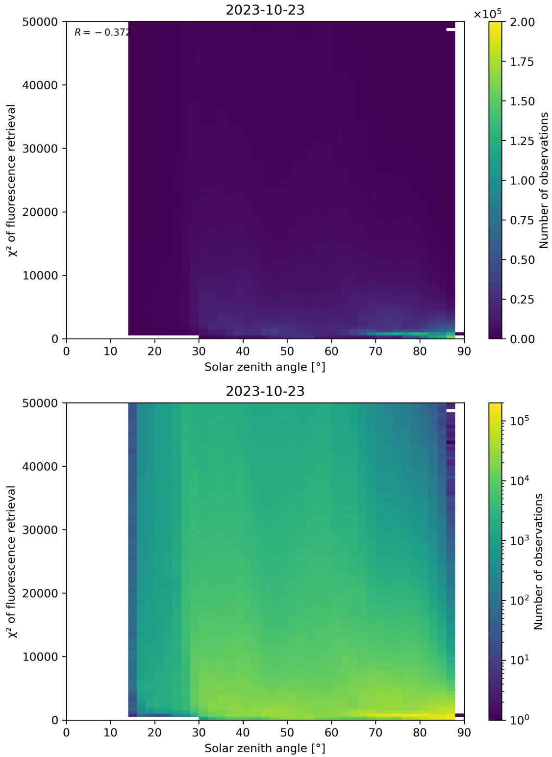
Figure 120: Scatter density plot of “Solar zenith angle” against “ \chi^2 of fluorescence retrieval” for 2023-10-22 to 2023-10-24.
