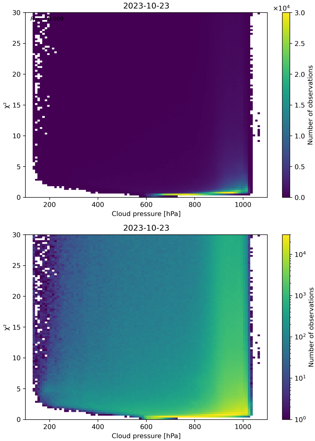
Figure 85: Scatter density plot of “Cloud pressure” against “ \chi^2 ” for 2023-10-22 to 2023-10-24.
