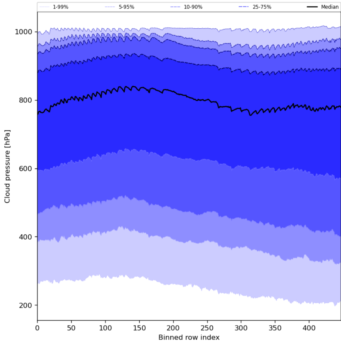
Figure 47: Along track statistics of “Cloud pressure” for 2023-10-22 to 2023-10-24
