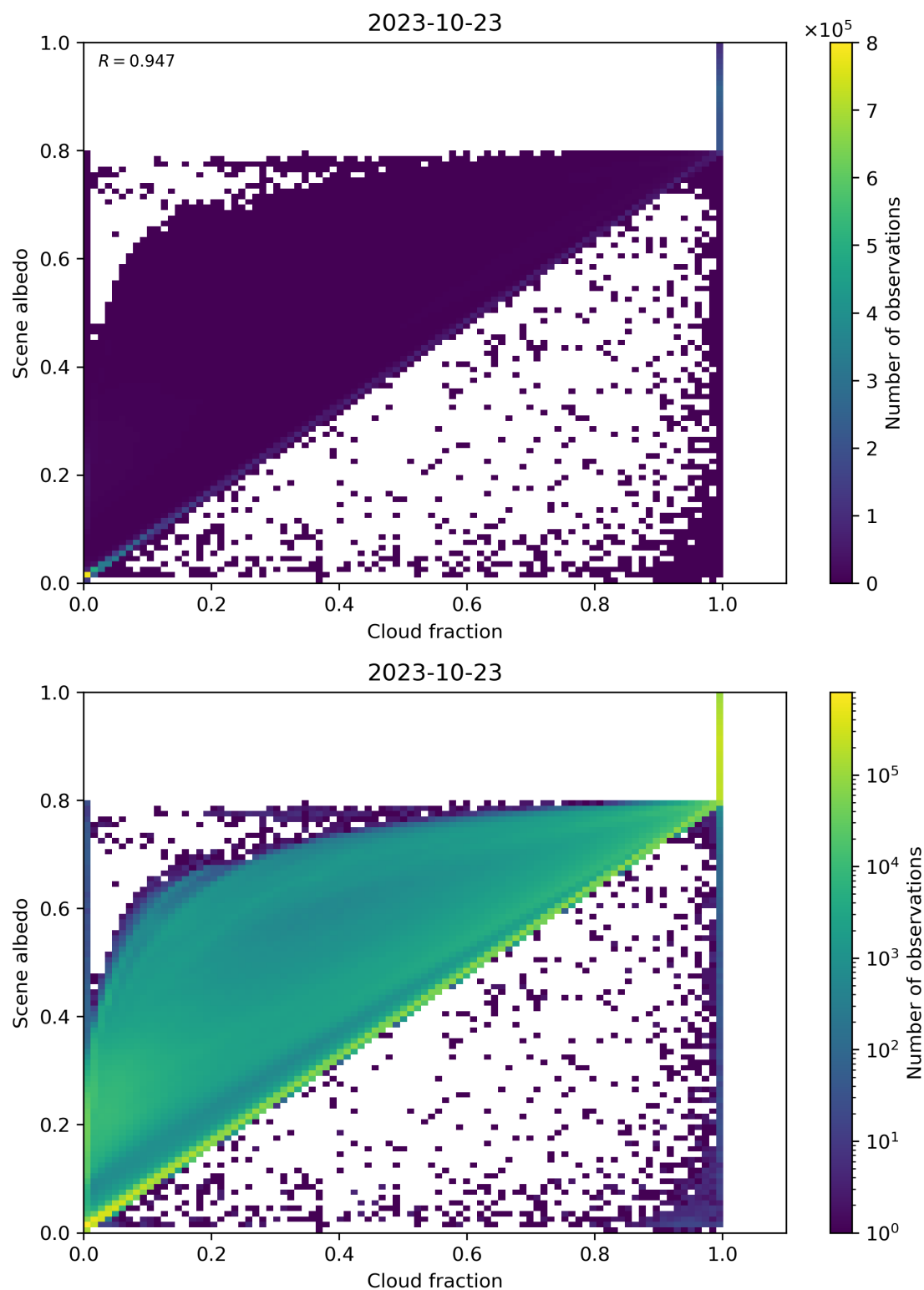
Figure 82: Scatter density plot of “Cloud fraction” against “Scene albedo” for 2023-10-22 to 2023-10-24.
