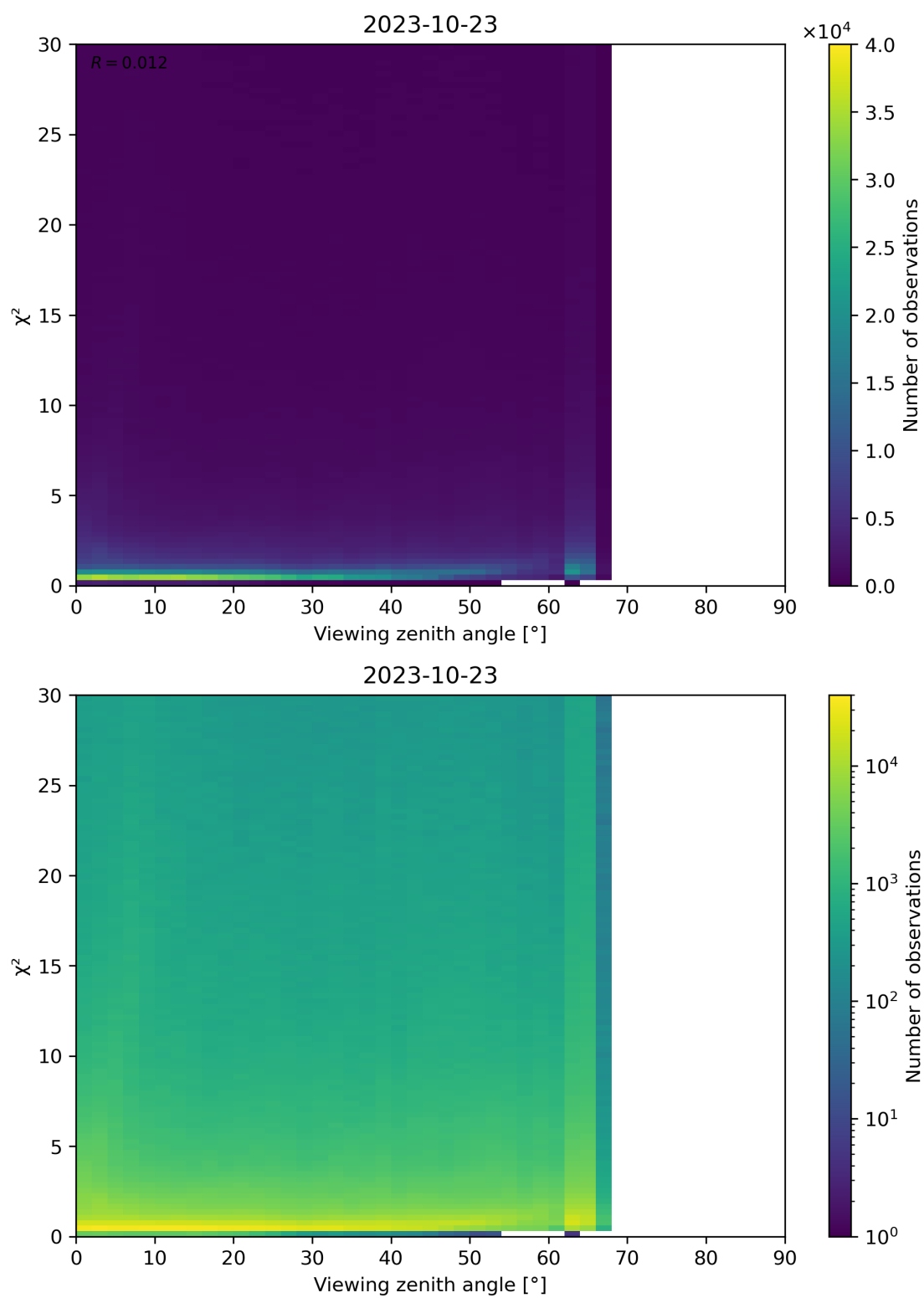
Figure 130: Scatter density plot of “Viewing zenith angle” against “ \chi^2 ” for 2023-10-22 to 2023-10-24.
