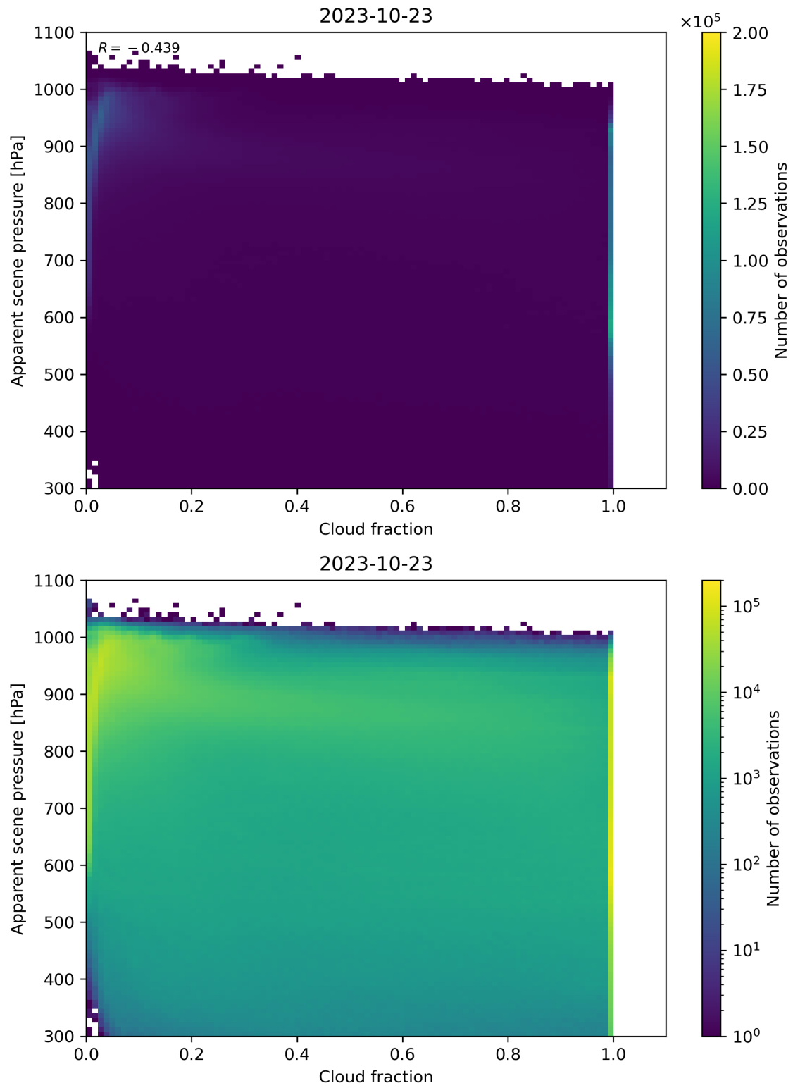
Figure 76: Scatter density plot of “Cloud fraction” against “Apparent scene pressure” for 2023-10-22 to 2023-10-24.
