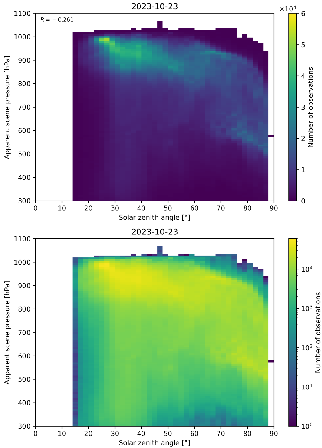
Figure 118: Scatter density plot of “Solar zenith angle” against “Apparent scene pressure” for 2023-10-22 to 2023-10-24.
