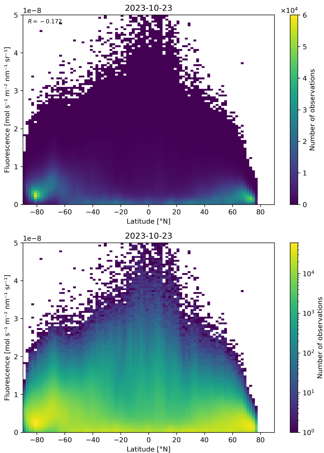
Figure 101: Scatter density plot of “Latitude” against “Fluorescence” for 2023-10-22 to 2023-10-24.
