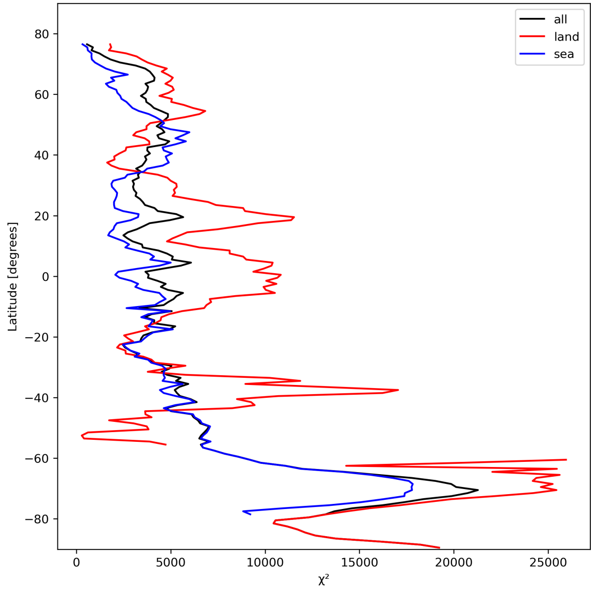
Figure 21: Zonal average of “ \chi^2 ” for 2023-10-22 to 2023-10-24.
