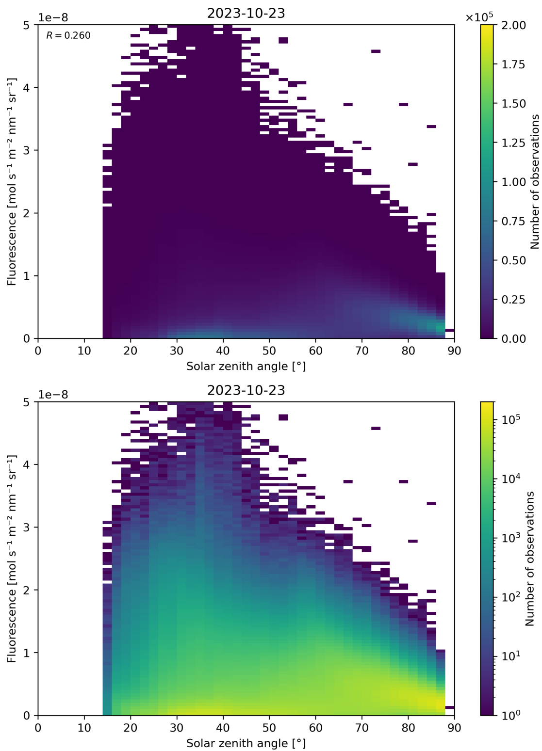
Figure 123: Scatter density plot of “Solar zenith angle” against “Fluorescence” for 2023-10-22 to 2023-10-24.
