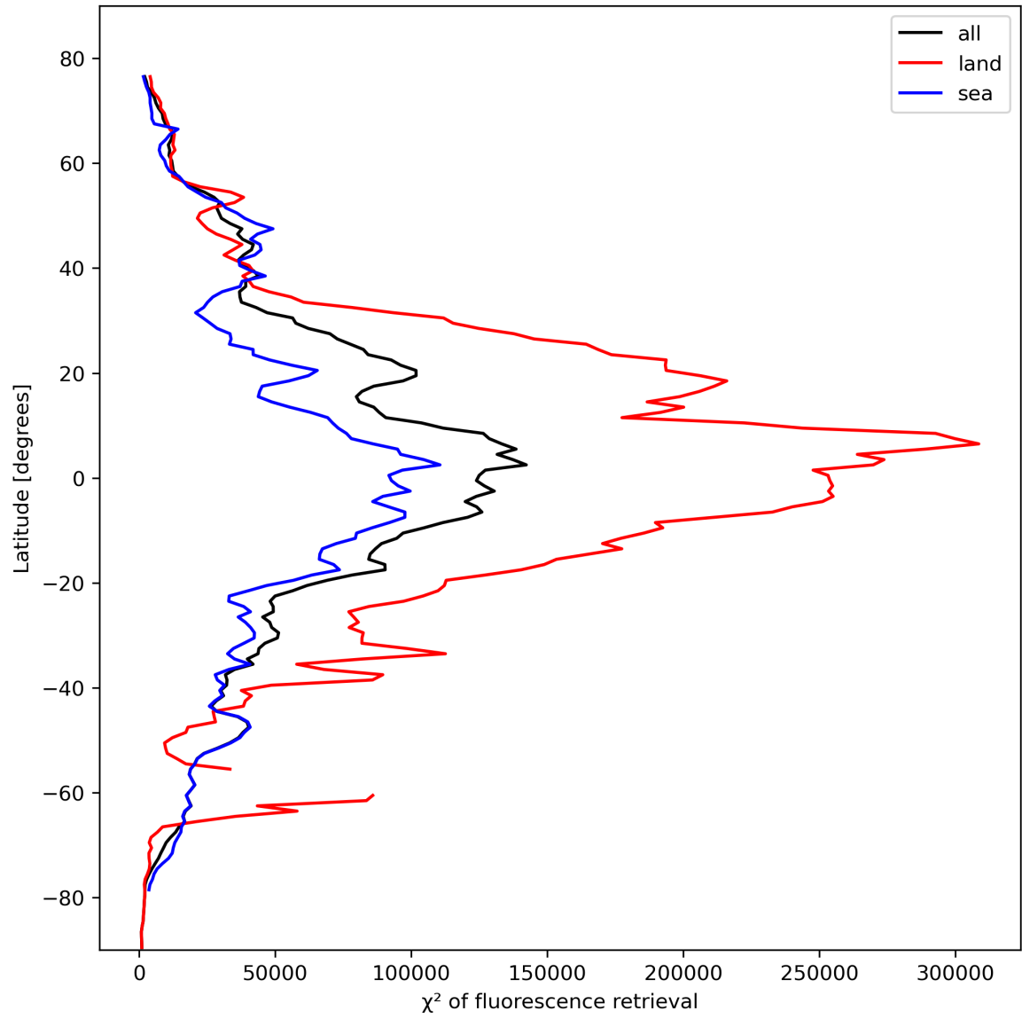
Figure 25: Zonal average of “ \chi^2 of fluorescence retrieval” for 2023-10-22 to 2023-10-24.
