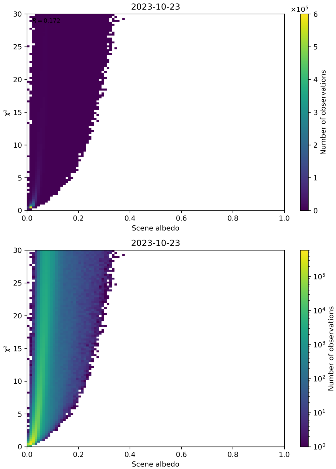
Figure 112: Scatter density plot of “Scene albedo” against “ \chi^2 ” for 2023-10-22 to 2023-10-24.
