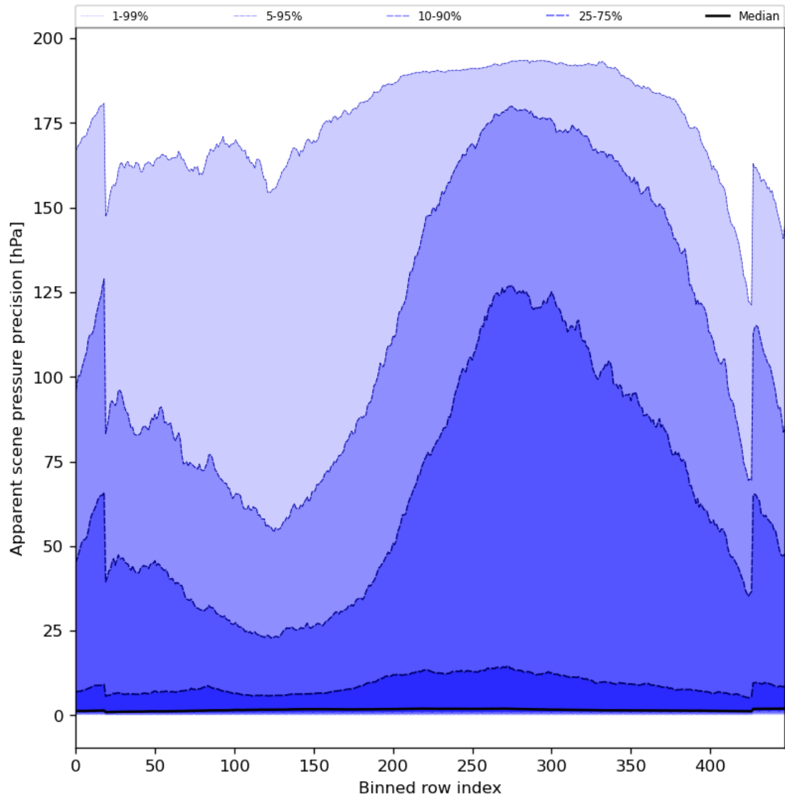
Figure 54: Along track statistics of “Apparent scene pressure precision” for 2023-10-22 to 2023-10-24
