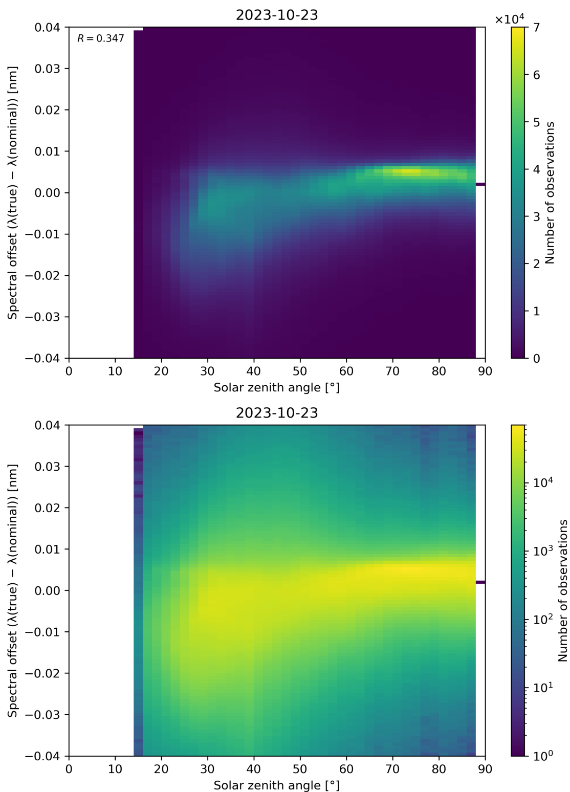
Figure 128: Scatter density plot of “Solar zenith angle” against “Spectral offset ( \lambda(\text{true}) - \lambda(\text{nominal}) )” for 2023-10-22 to 2023-10-24.
