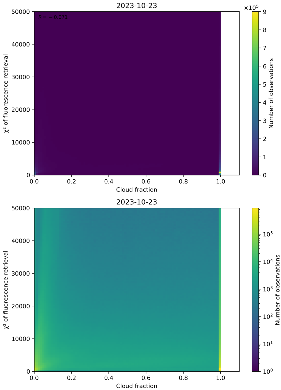
Figure 78: Scatter density plot of “Cloud fraction” against “ \chi^2 of fluorescence retrieval” for 2023-10-22 to 2023-10-24.
