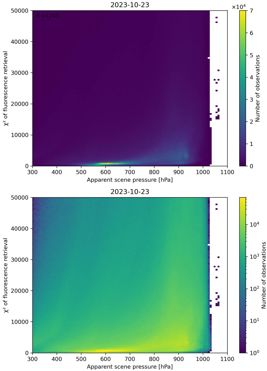
Figure 64: Scatter density plot of “Apparent scene pressure” against “ \chi^2 of fluorescence retrieval” for 2023-10-22 to 2023-10-24.
