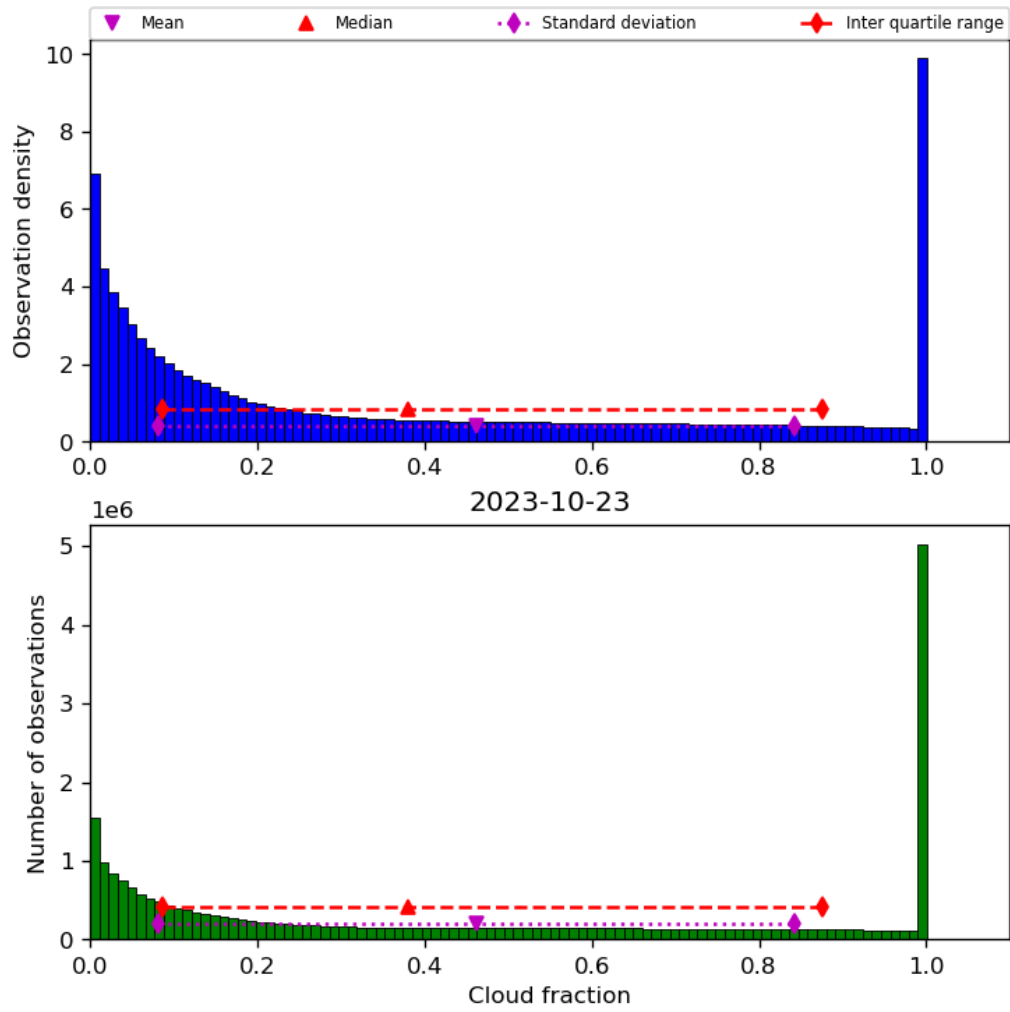
Figure 32: Histogram of “Cloud fraction” for 2023-10-22 to 2023-10-24
