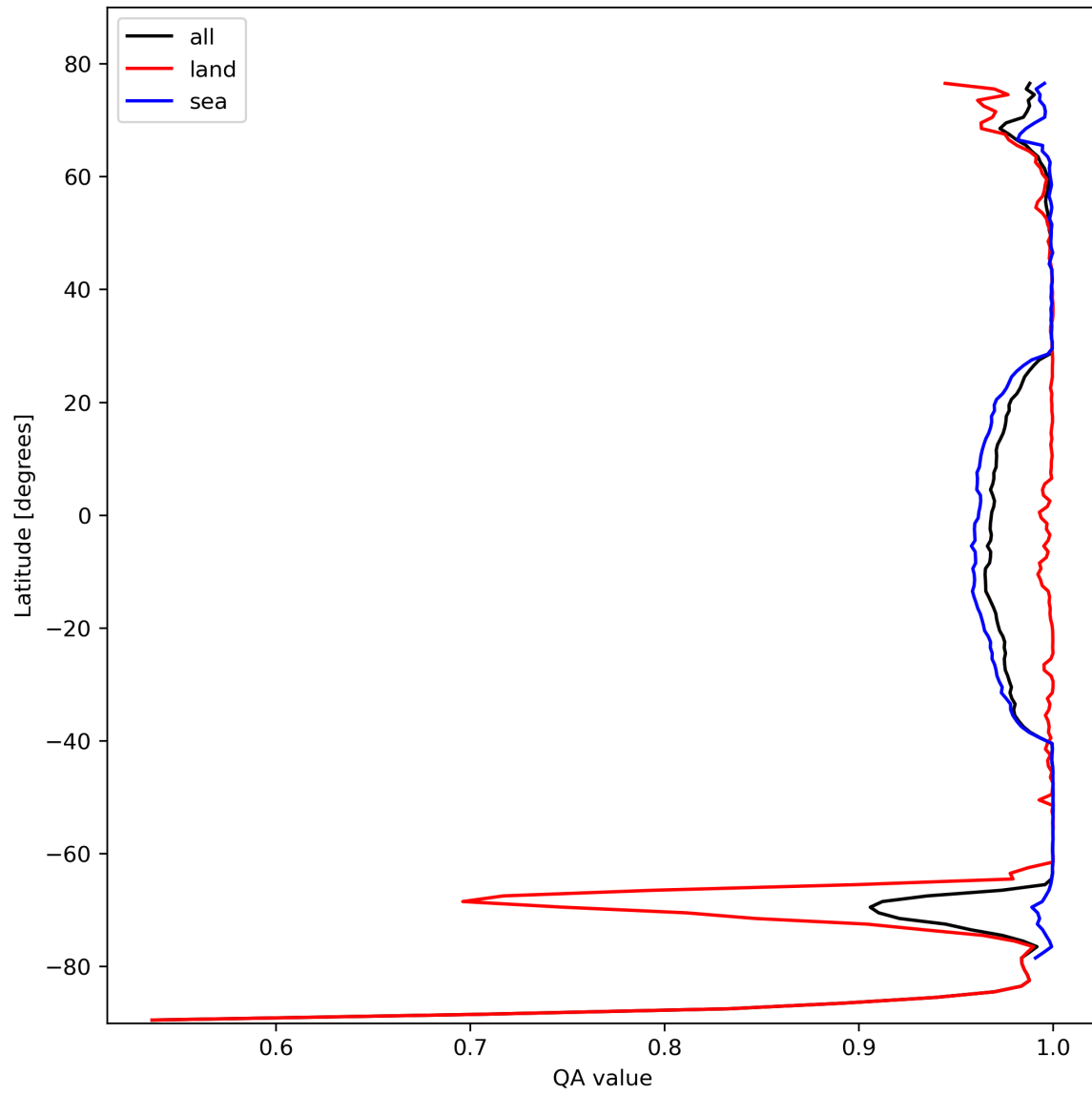
Figure 12: Zonal average of “QA value” for 2023-10-22 to 2023-10-24.
