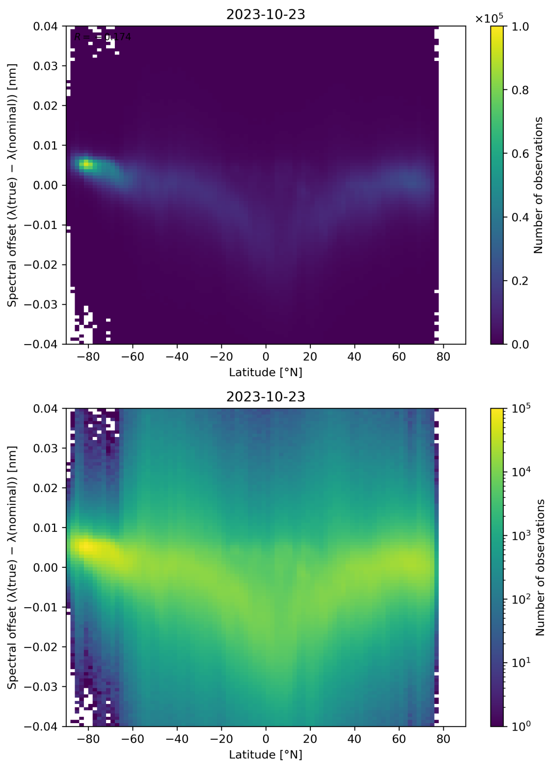
Figure 105: Scatter density plot of “Latitude” against “Spectral offset ( \lambda(\text{true}) - \lambda(\text{nominal}) )” for 2023-10-22 to 2023-10-24.
