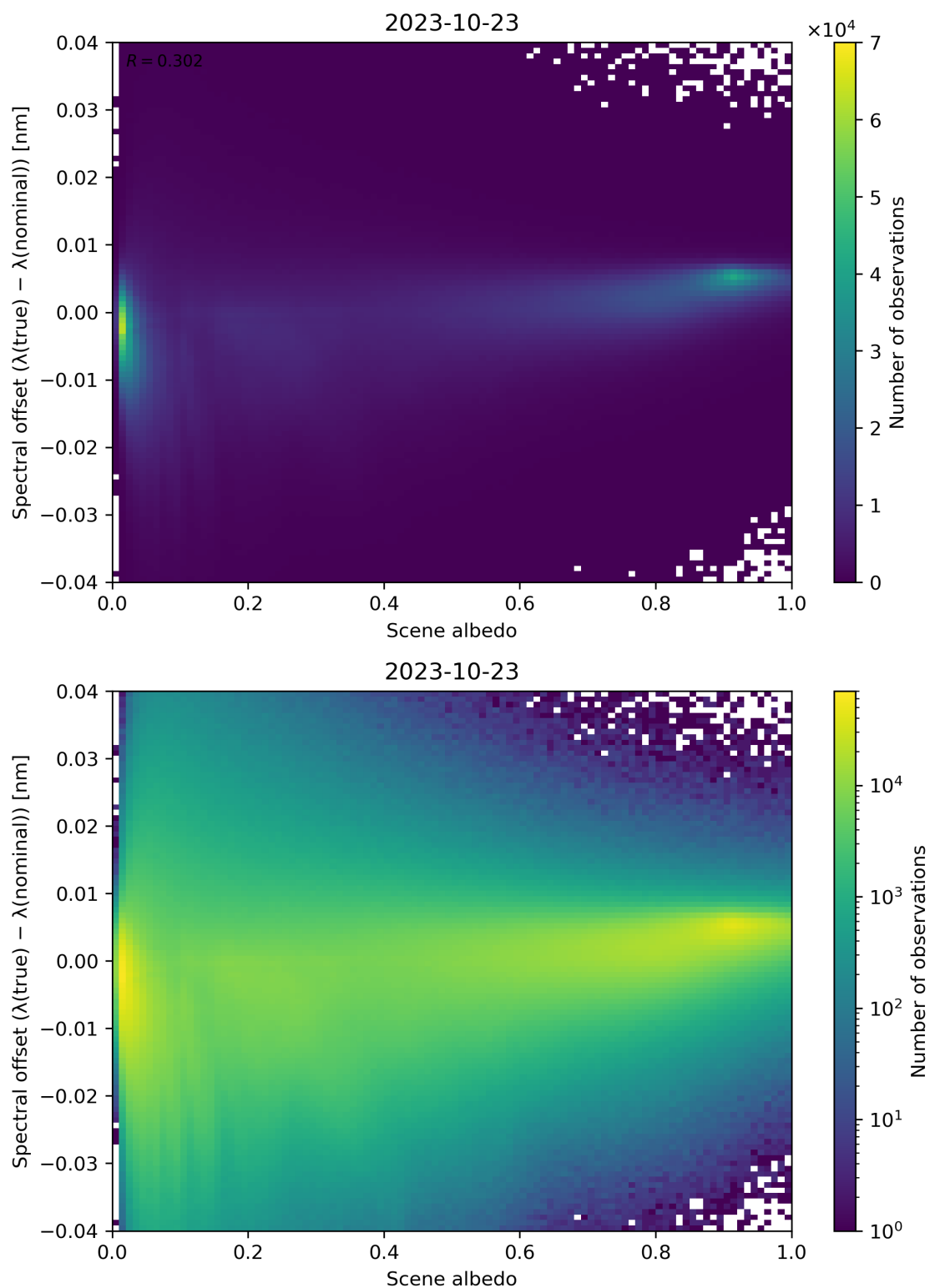
Figure 117: Scatter density plot of “Scene albedo” against “Spectral offset ( \lambda(\text{true}) - \lambda(\text{nominal}) )” for 2023-10-22 to 2023-10-24.
