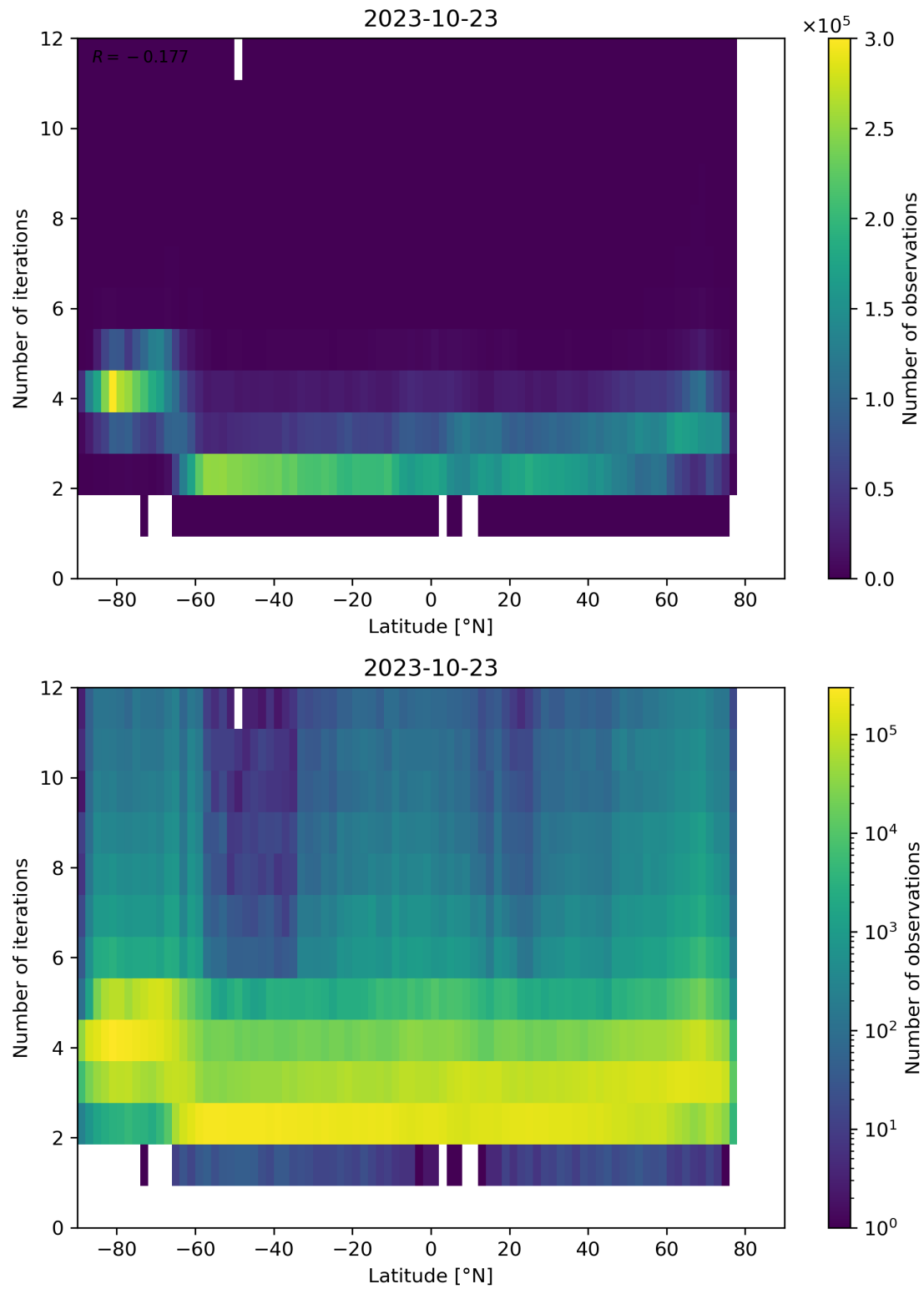
Figure 102: Scatter density plot of “Latitude” against “Number of iterations” for 2023-10-22 to 2023-10-24.
