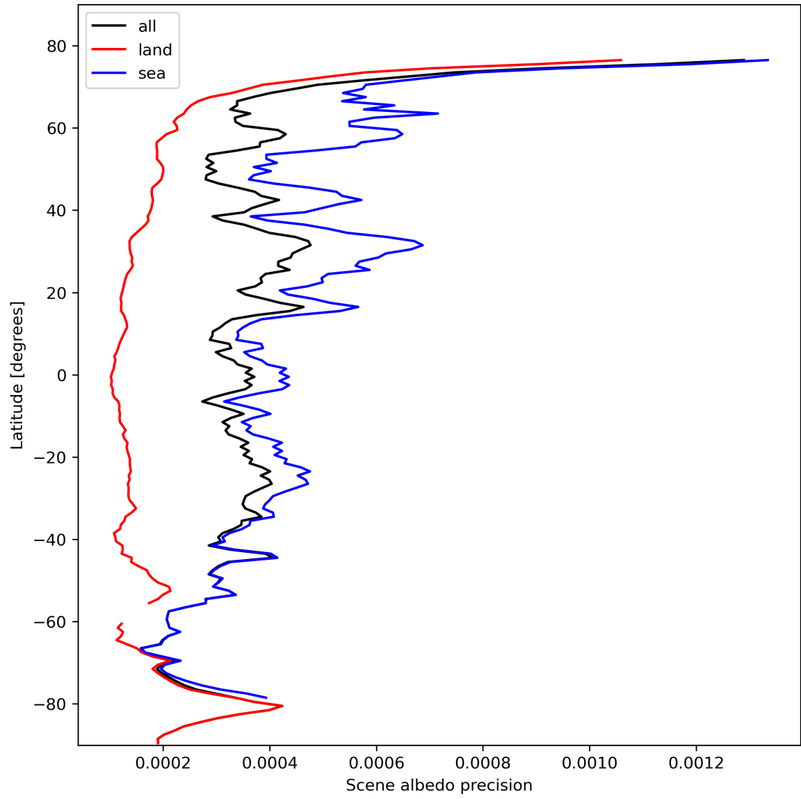
Figure 18: Zonal average of “Scene albedo precision” for 2023-10-22 to 2023-10-24.
