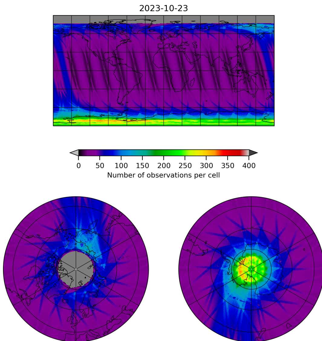
Figure 11: Map of the number of observations for 2023-10-22 to 2023-10-24
