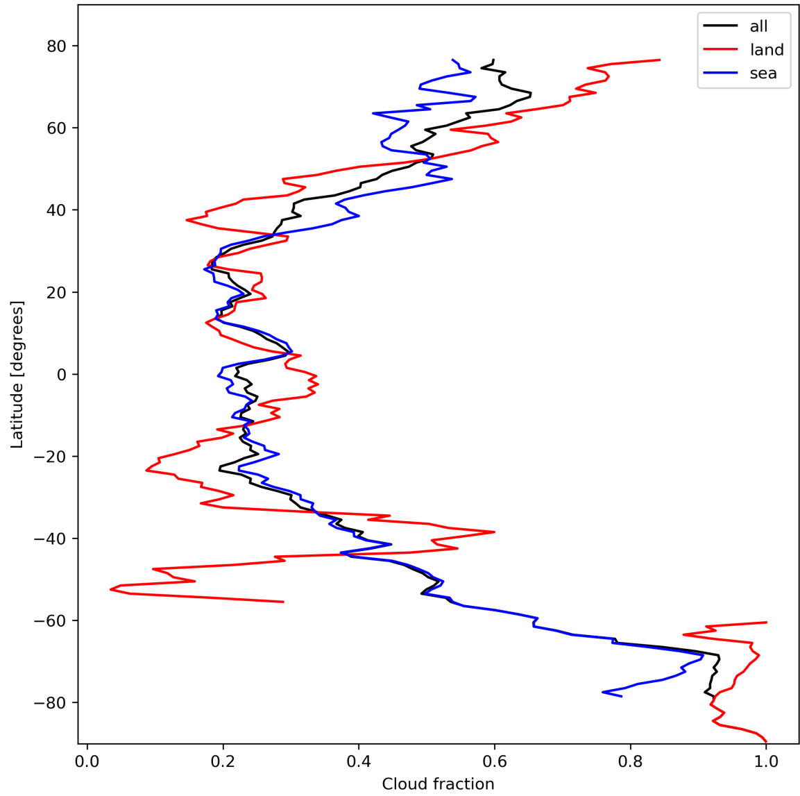
Figure 15: Zonal average of “Cloud fraction” for 2023-10-22 to 2023-10-24.
