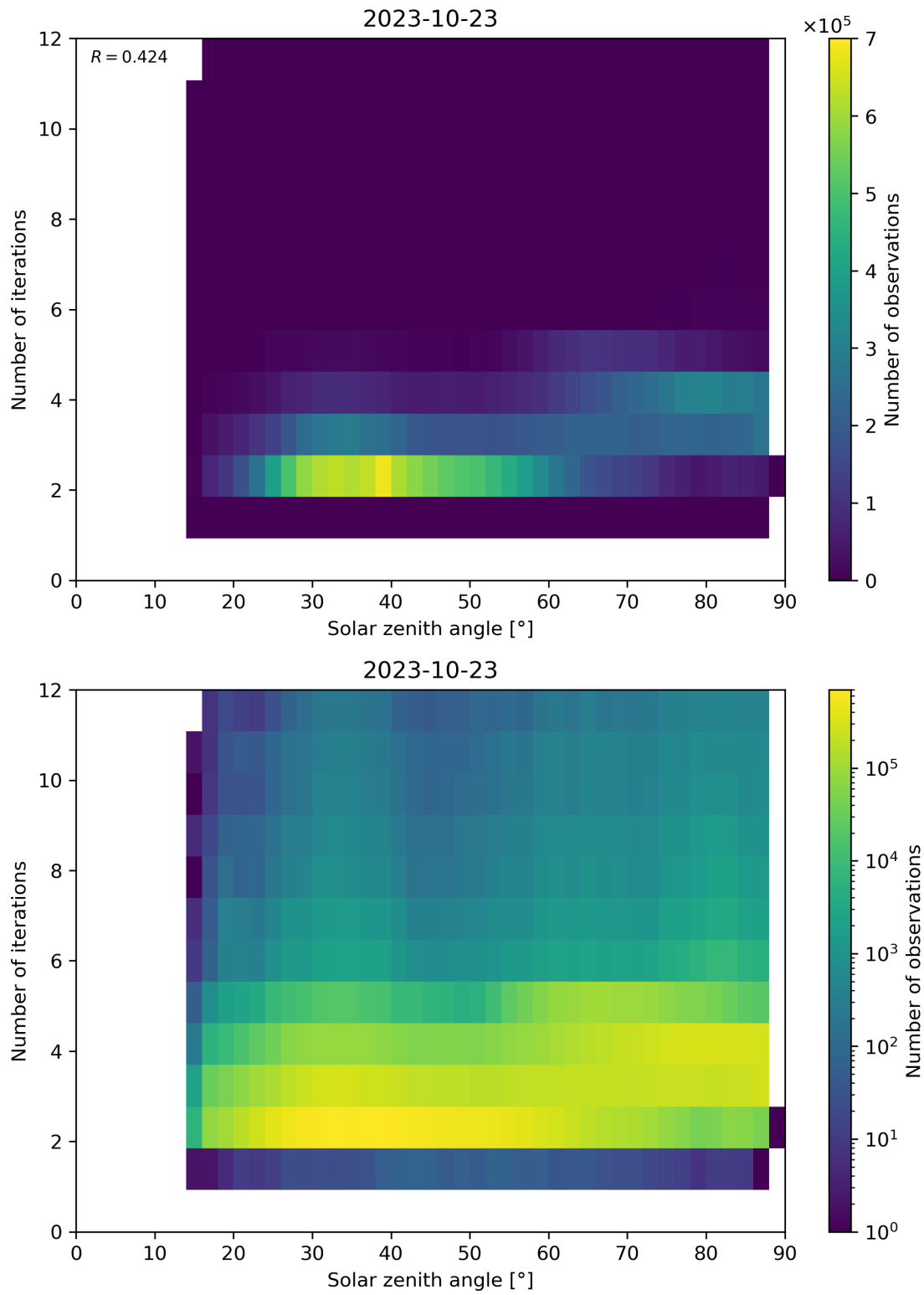
Figure 125: Scatter density plot of “Solar zenith angle” against “Number of iterations” for 2023-10-22 to 2023-10-24.
