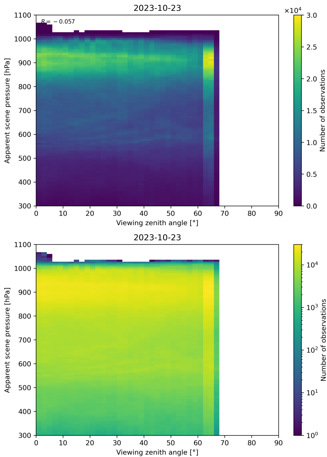
Figure 129: Scatter density plot of “Viewing zenith angle” against “Apparent scene pressure” for 2023-10-22 to 2023-10-24.
