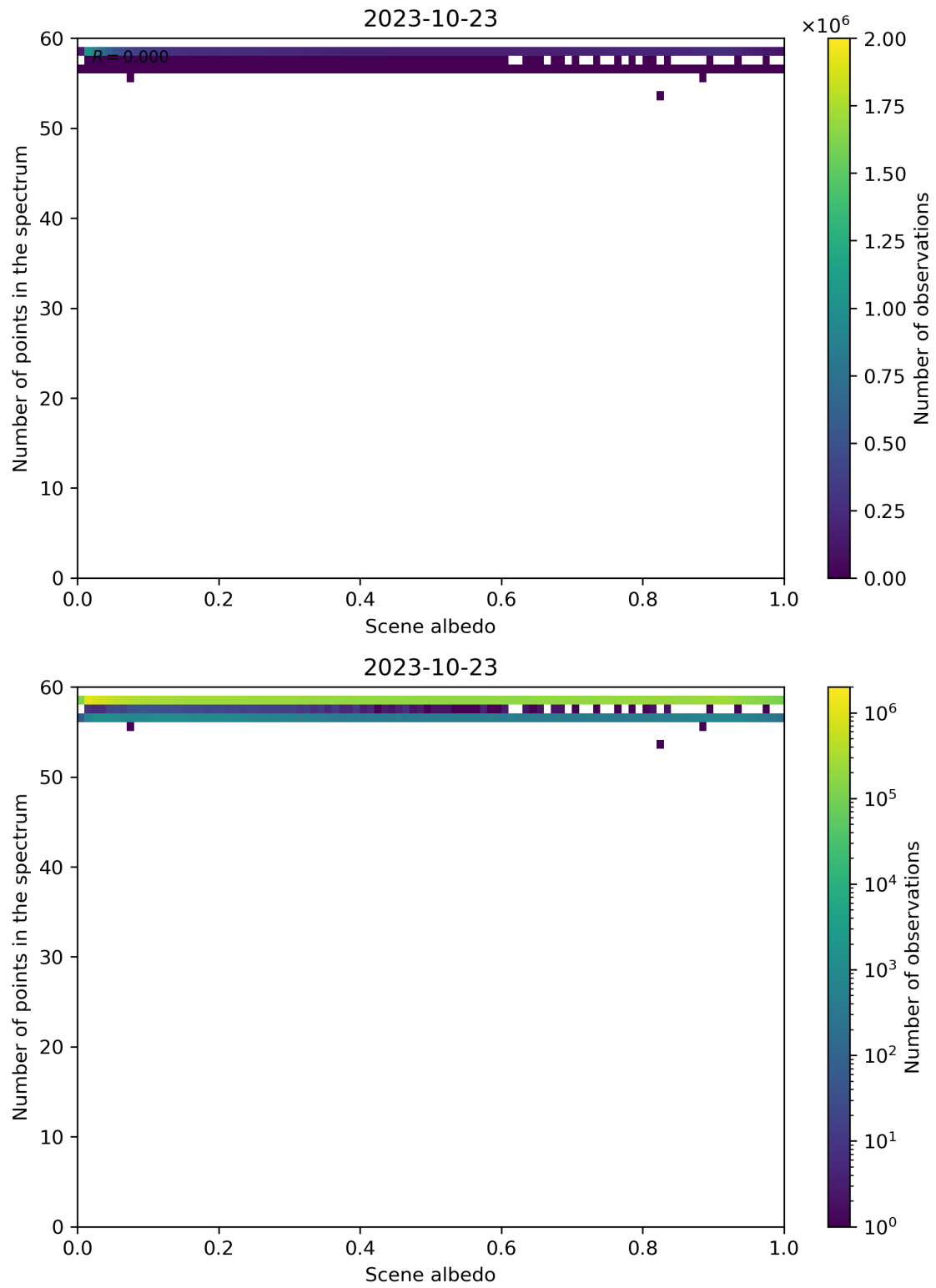
Figure 116: Scatter density plot of “Scene albedo” against “Number of points in the spectrum” for 2023-10-22 to 2023-10-24.
