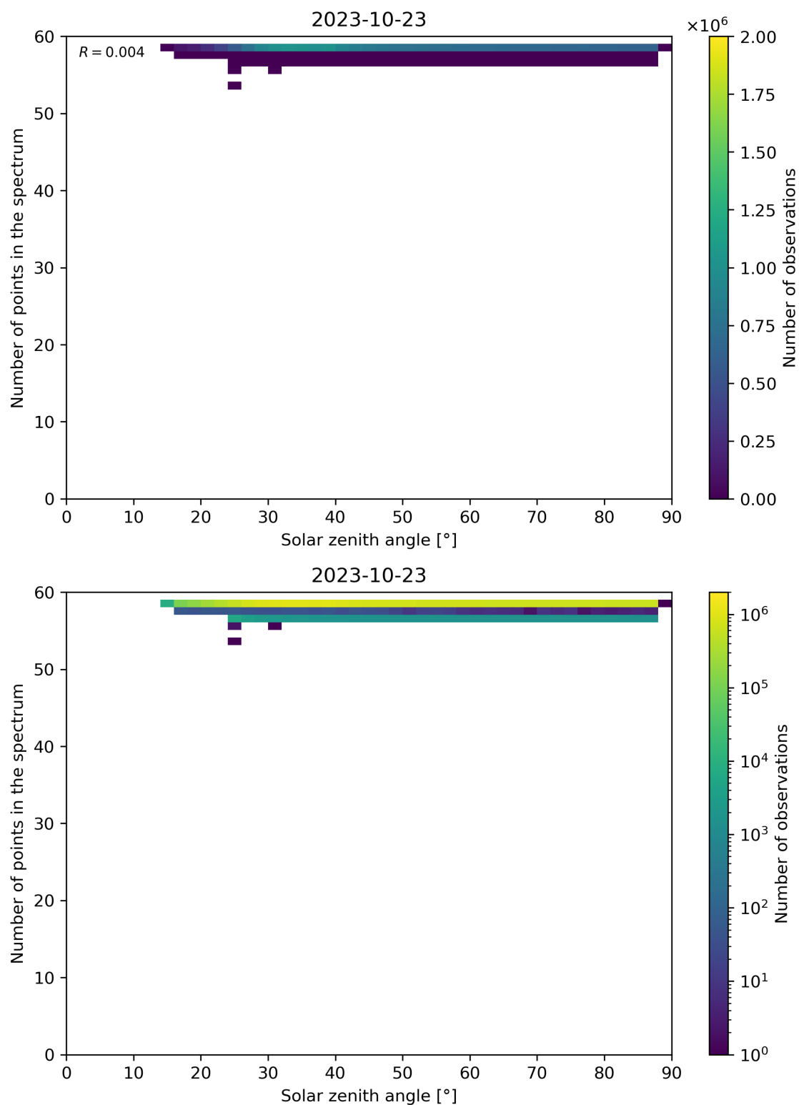
Figure 126: Scatter density plot of “Solar zenith angle” against “Number of points in the spectrum” for 2023-10-22 to 2023-10-24.
