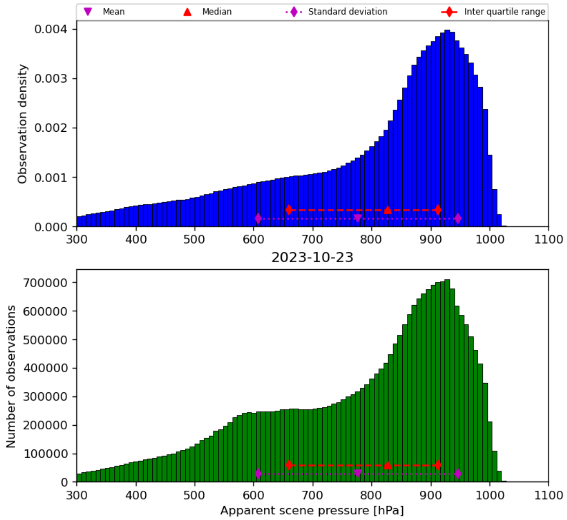
Figure 36: Histogram of “Apparent scene pressure” for 2023-10-22 to 2023-10-24
