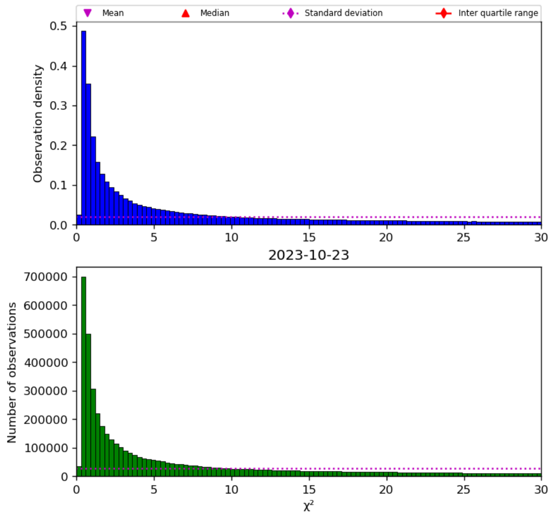
Figure 38: Histogram of “ \chi^2 ” for 2023-10-22 to 2023-10-24
