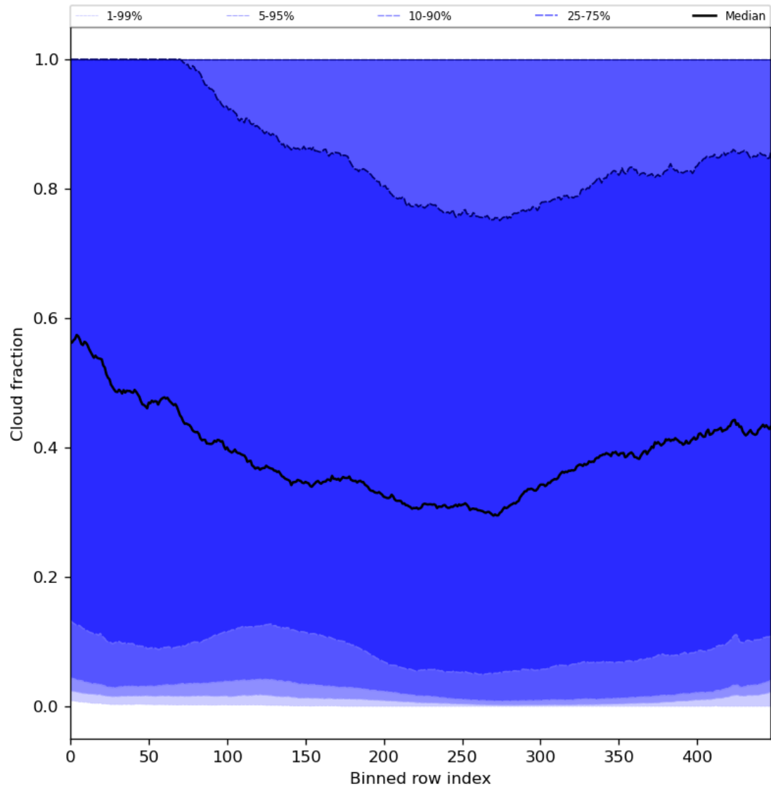
Figure 49: Along track statistics of “Cloud fraction” for 2023-10-22 to 2023-10-24
