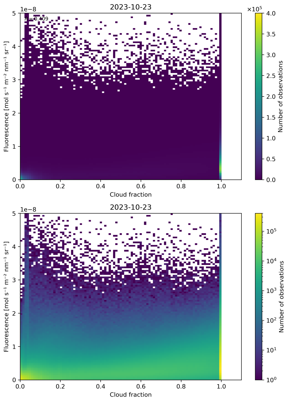
Figure 79: Scatter density plot of “Cloud fraction” against “Fluorescence” for 2023-10-22 to 2023-10-24.
