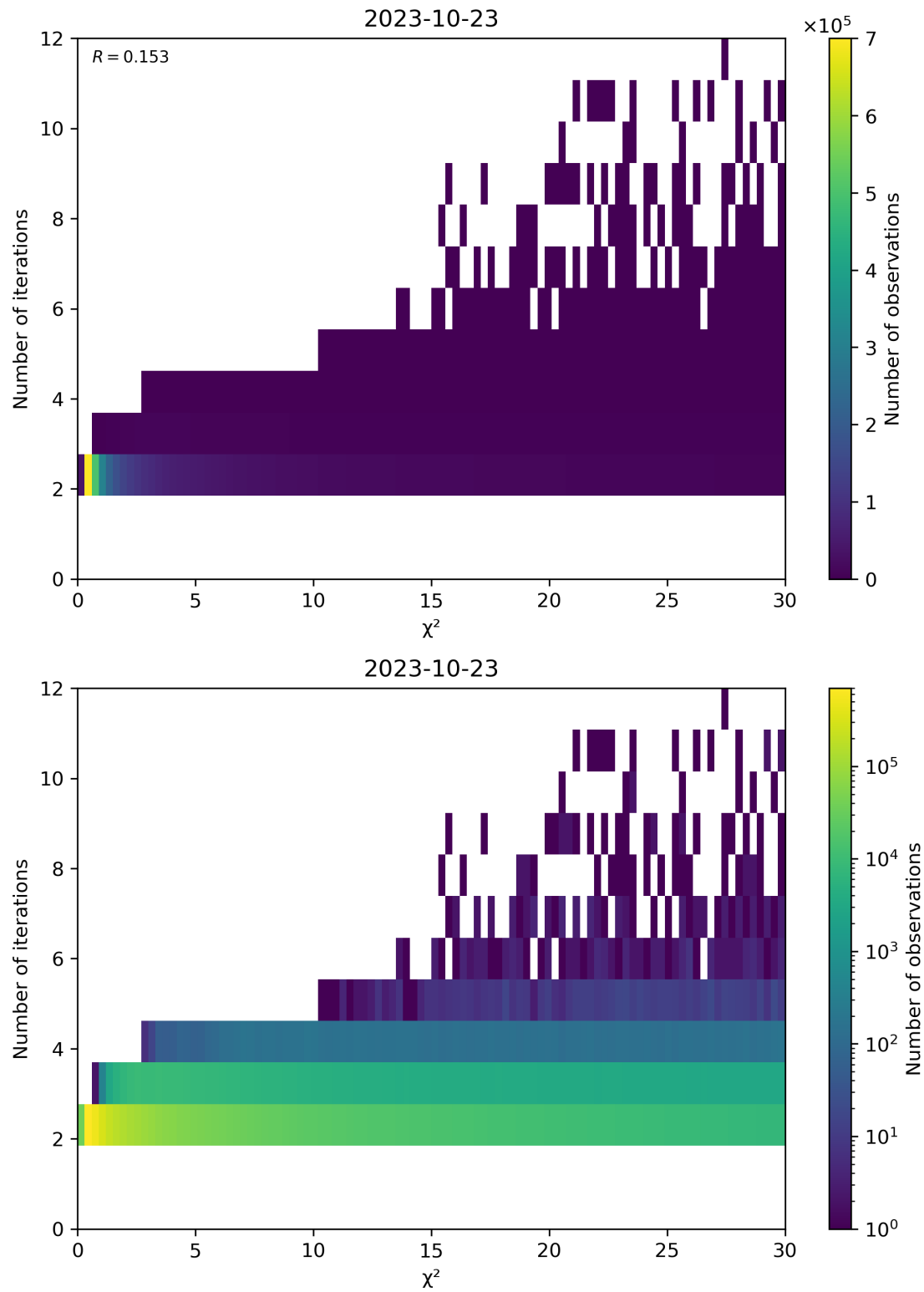
Figure 73: Scatter density plot of “ \chi^2 ” against “Number of iterations” for 2023-10-22 to 2023-10-24.
