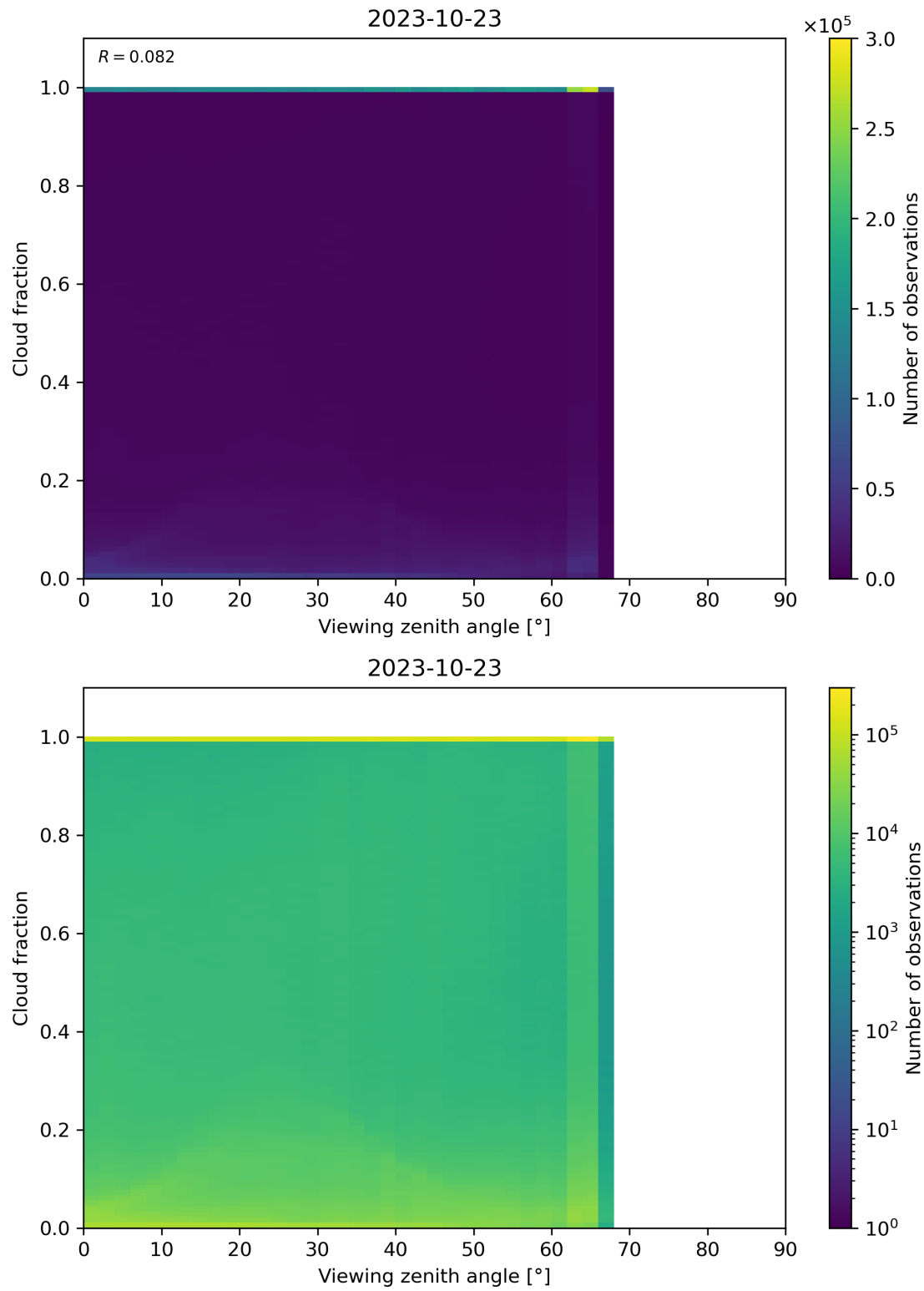
Figure 132: Scatter density plot of “Viewing zenith angle” against “Cloud fraction” for 2023-10-22 to 2023-10-24.
