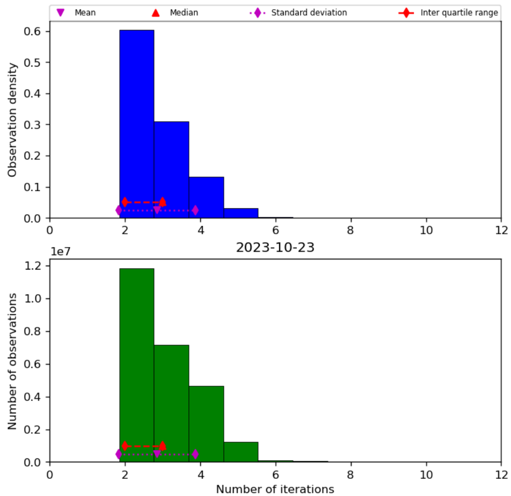
Figure 39: Histogram of “Number of iterations” for 2023-10-22 to 2023-10-24
