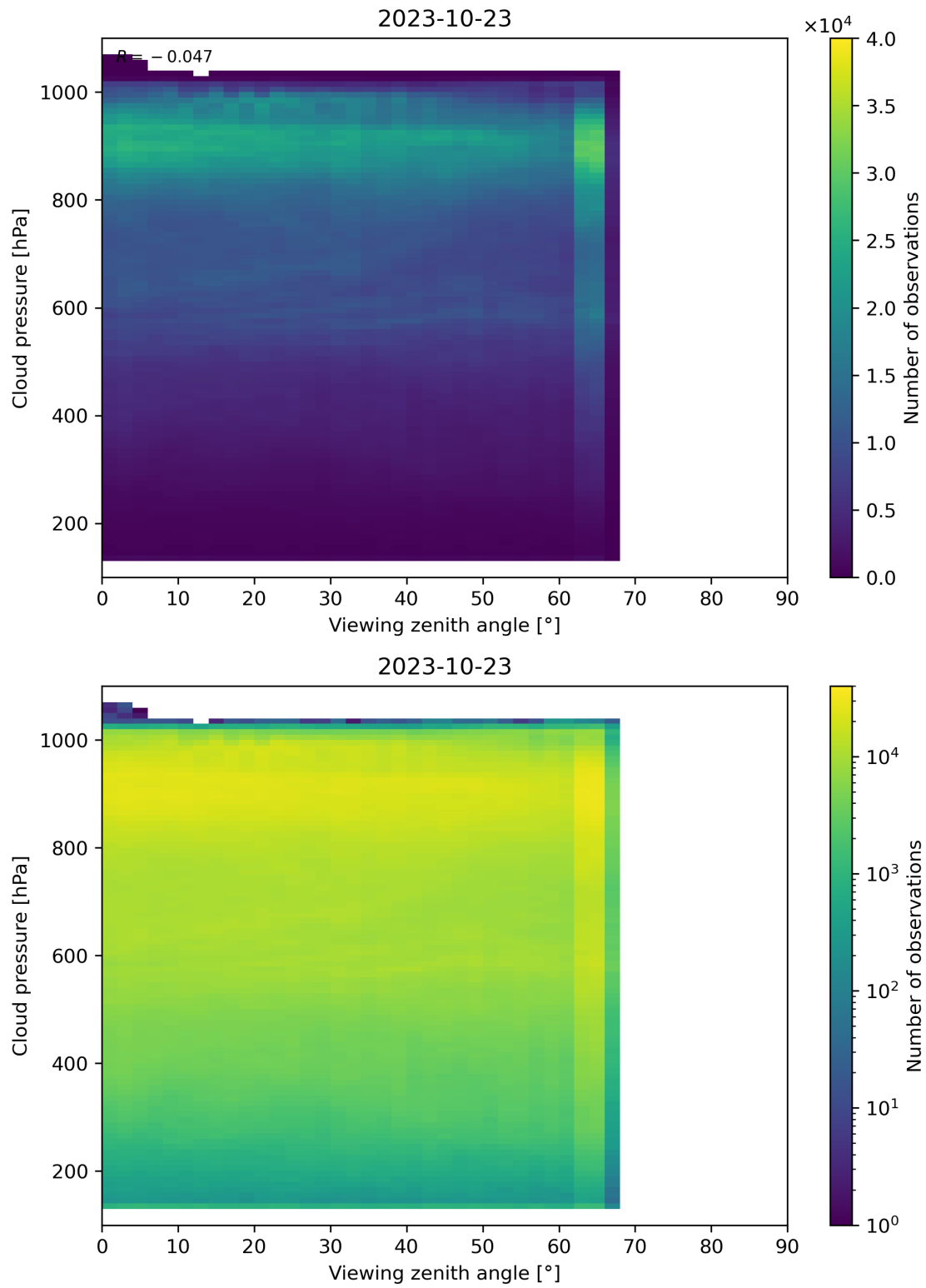
Figure 133: Scatter density plot of “Viewing zenith angle” against “Cloud pressure” for 2023-10-22 to 2023-10-24.
