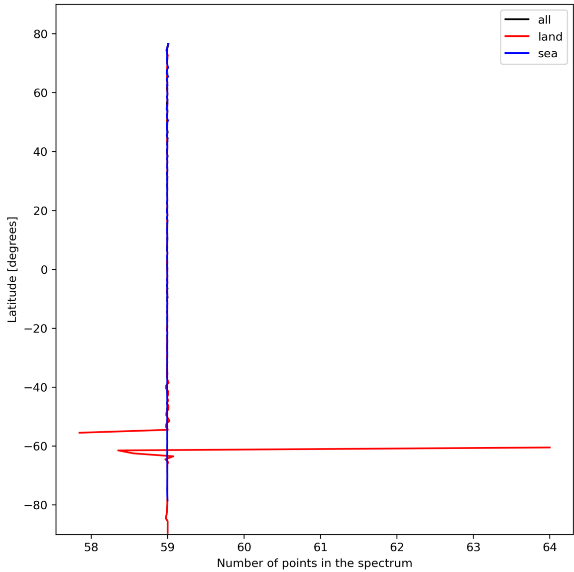
Figure 27: Zonal average of “Number of points in the spectrum” for 2023-10-22 to 2023-10-24.
