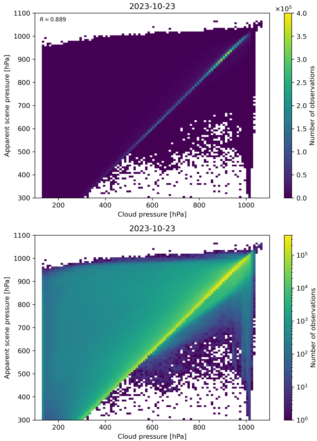
Figure 84: Scatter density plot of “Cloud pressure” against “Apparent scene pressure” for 2023-10-22 to 2023-10-24.
