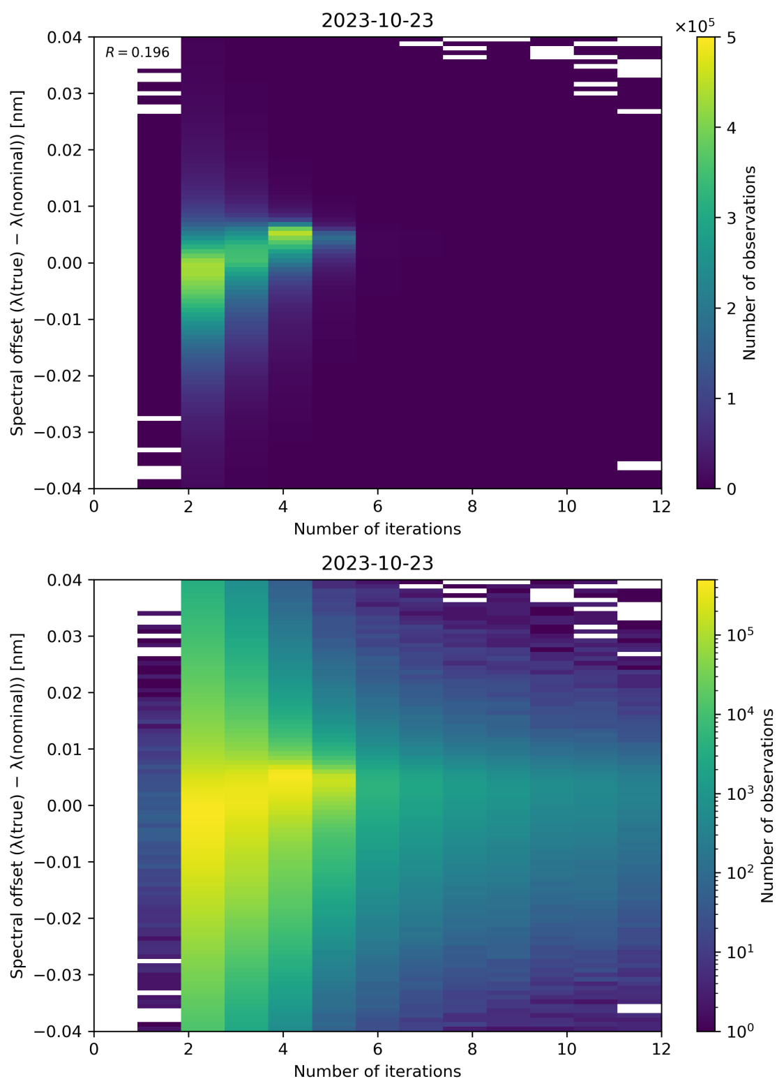
Figure 109: Scatter density plot of “Number of iterations” against “Spectral offset ( \lambda(\text{true}) - \lambda(\text{nominal}) )” for 2023-10-22 to 2023-10-24.
