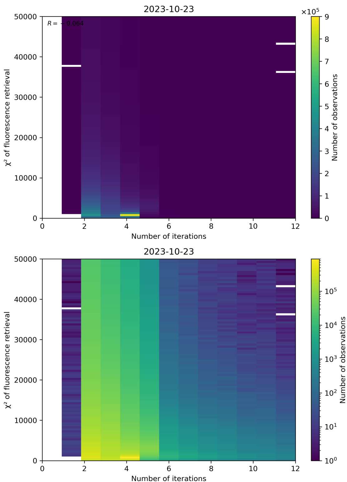
Figure 106: Scatter density plot of “Number of iterations” against “ \chi^2 of fluorescence retrieval” for 2023-10-22 to 2023-10-24.
