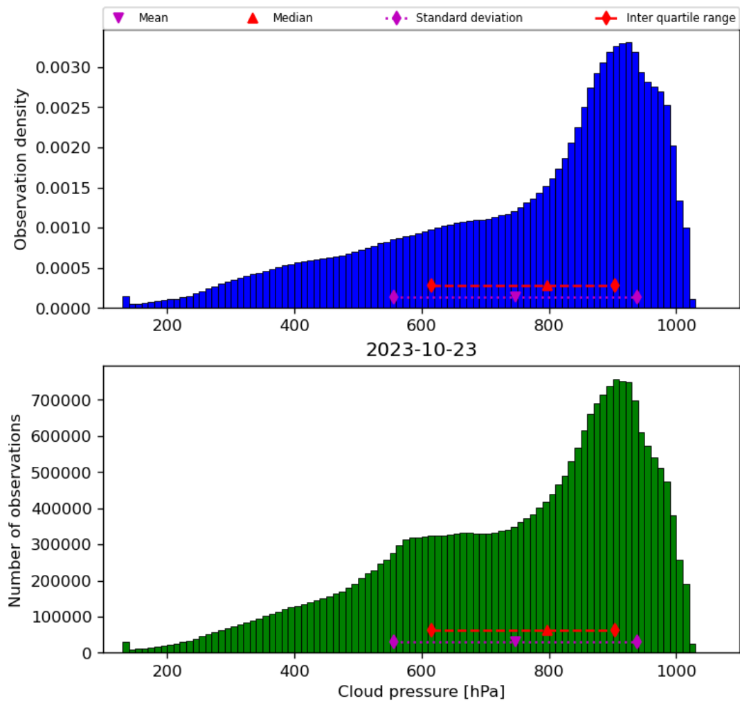
Figure 30: Histogram of “Cloud pressure” for 2023-10-22 to 2023-10-24
