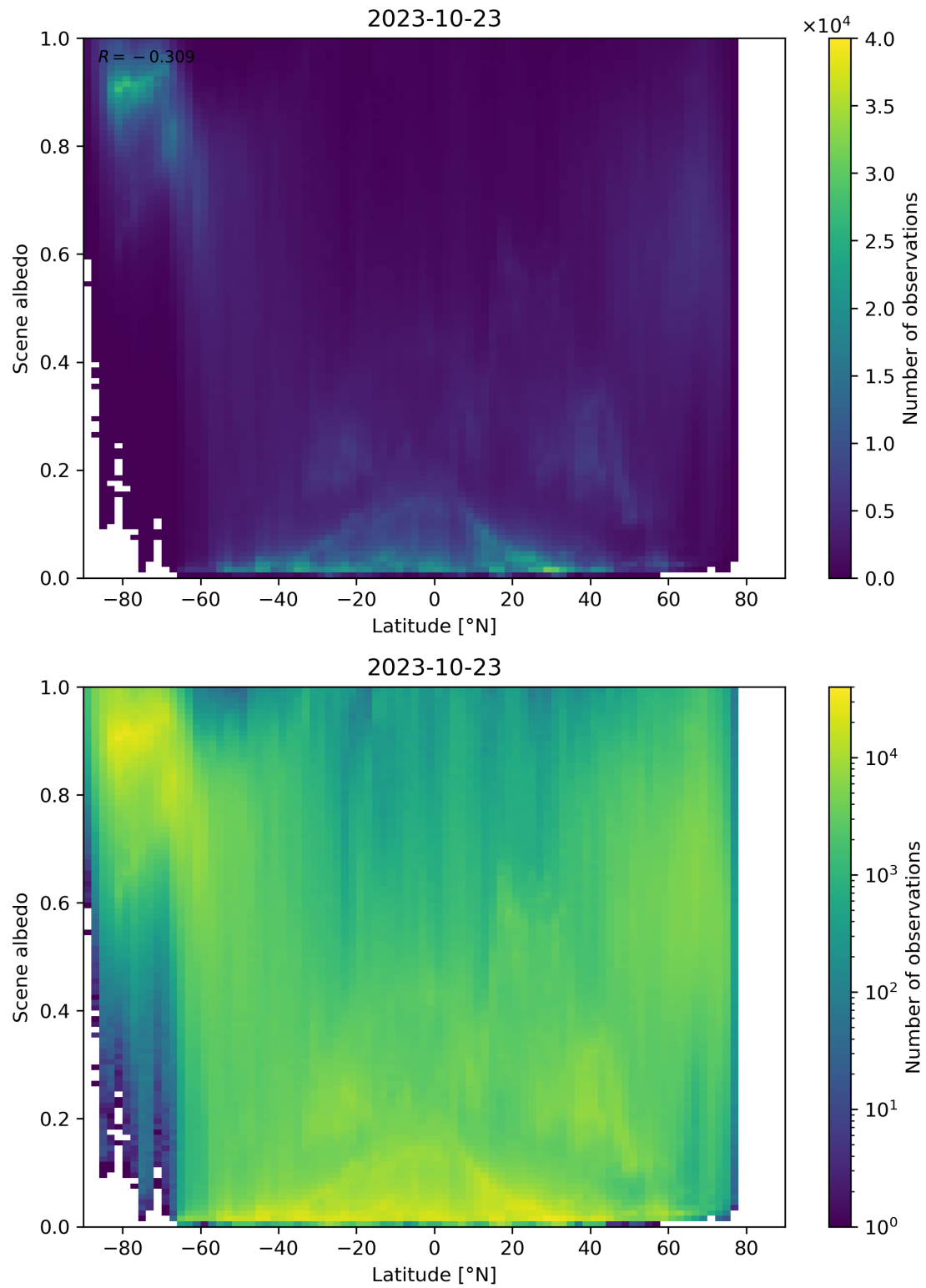
Figure 104: Scatter density plot of “Latitude” against “Scene albedo” for 2023-10-22 to 2023-10-24.
