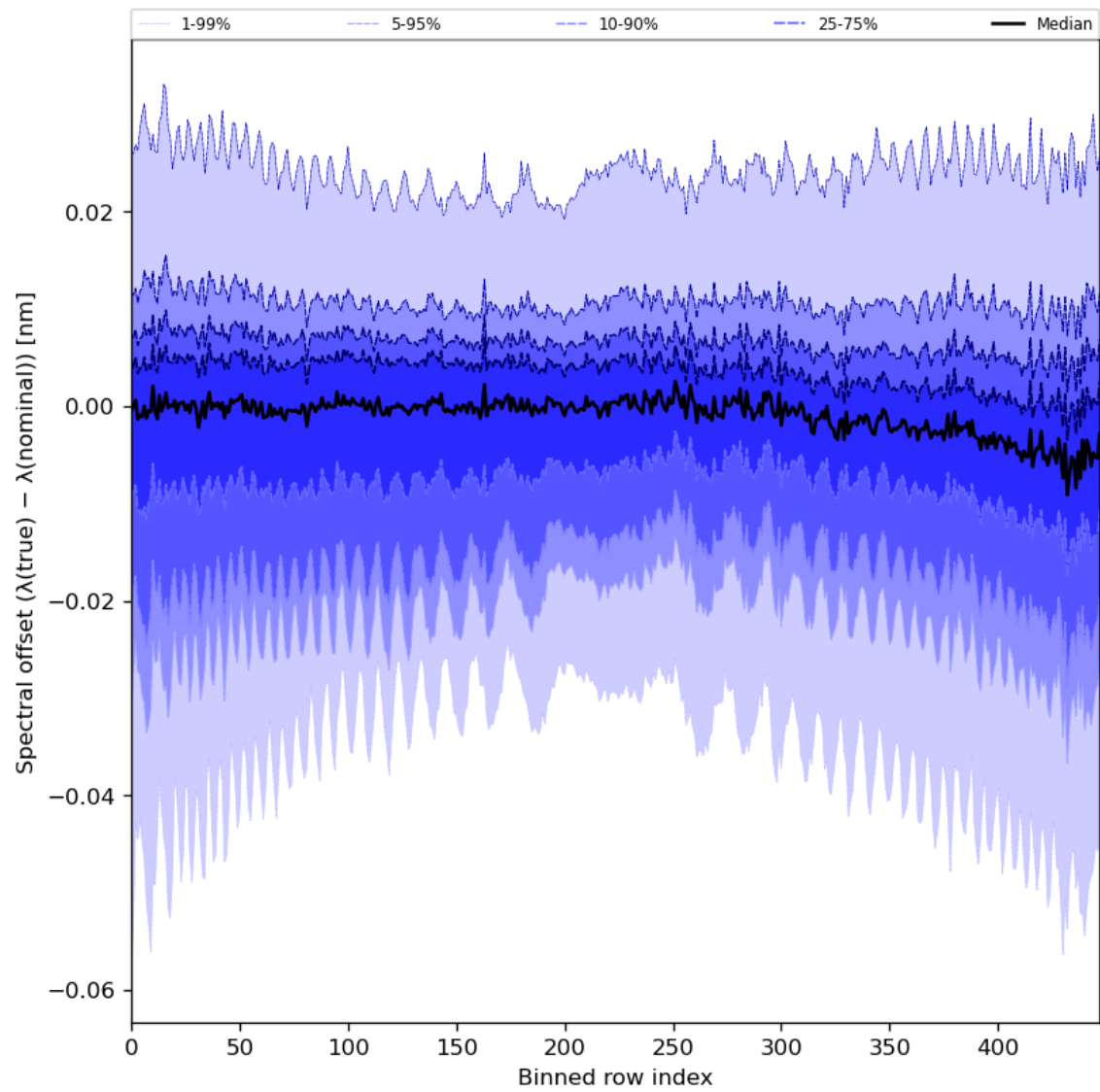
Figure 62: Along track statistics of “Spectral offset ( \lambda(\text{true}) - \lambda(\text{nominal}) )” for 2023-10-22 to 2023-10-24
