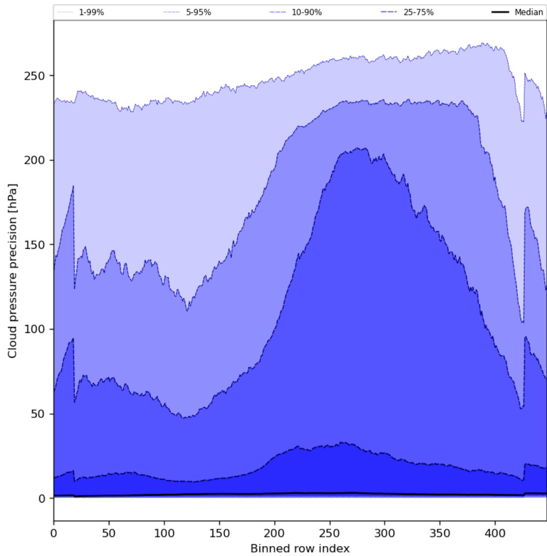
Figure 48: Along track statistics of “Cloud pressure precision” for 2023-10-22 to 2023-10-24
