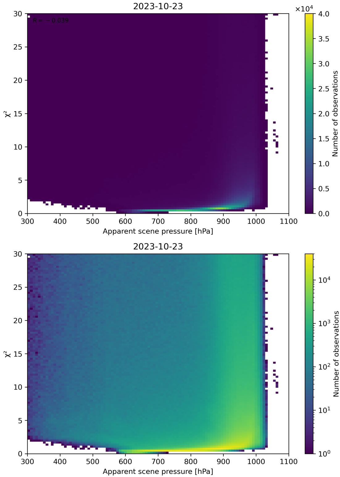
Figure 63: Scatter density plot of “Apparent scene pressure” against “ \chi^2 ” for 2023-10-22 to 2023-10-24.
