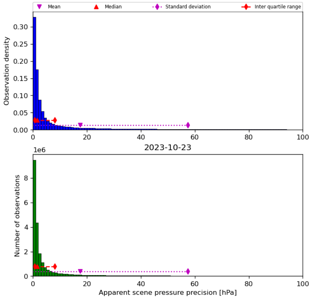
Figure 37: Histogram of “Apparent scene pressure precision” for 2023-10-22 to 2023-10-24
