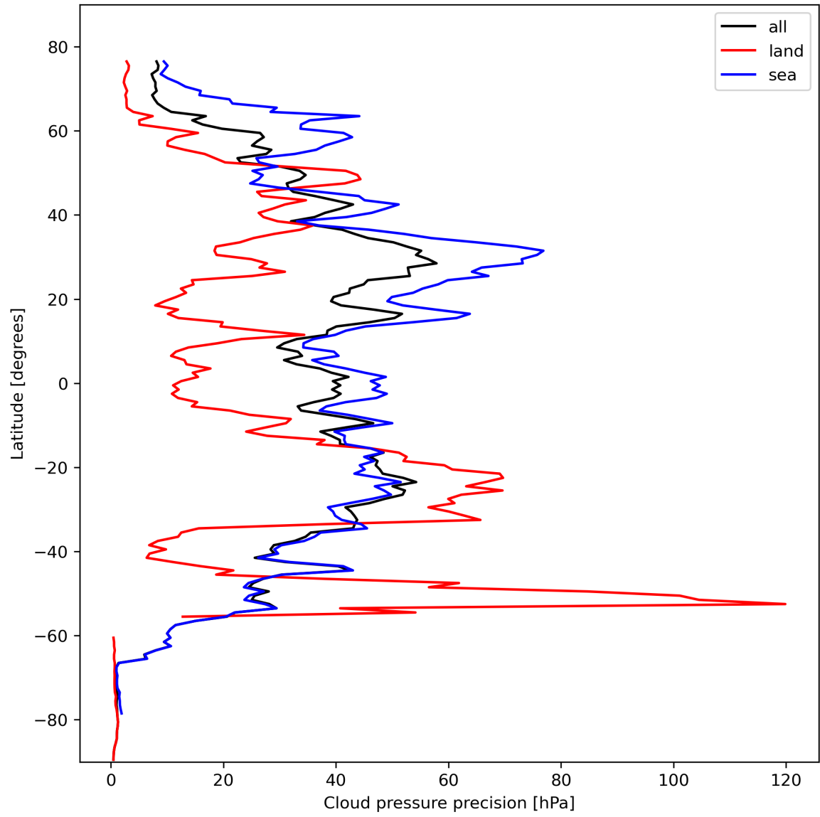
Figure 14: Zonal average of “Cloud pressure precision” for 2023-10-22 to 2023-10-24.
