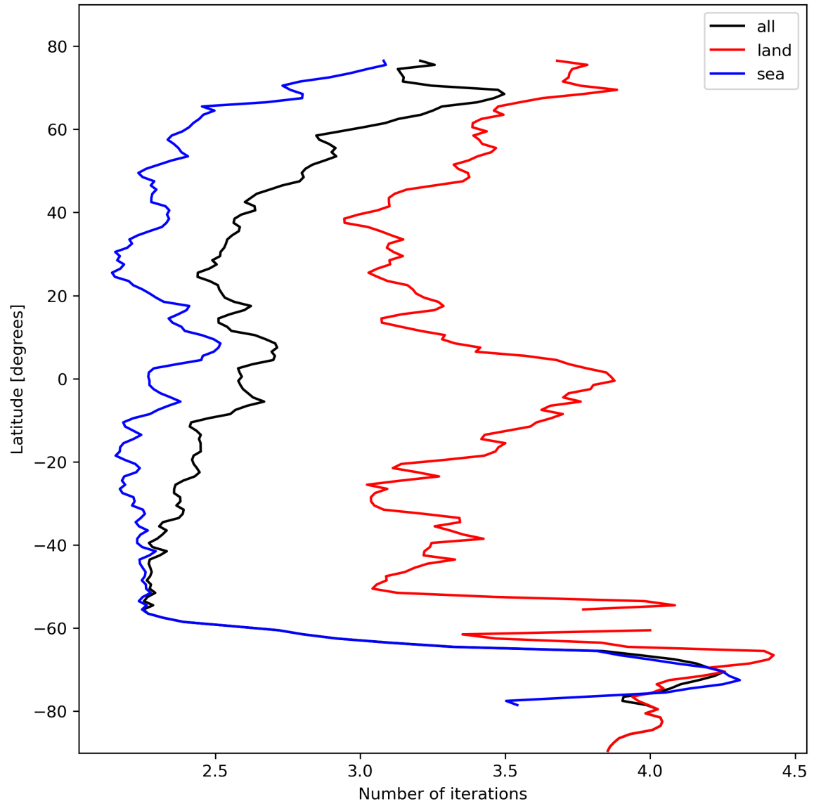
Figure 22: Zonal average of “Number of iterations” for 2023-10-22 to 2023-10-24.
