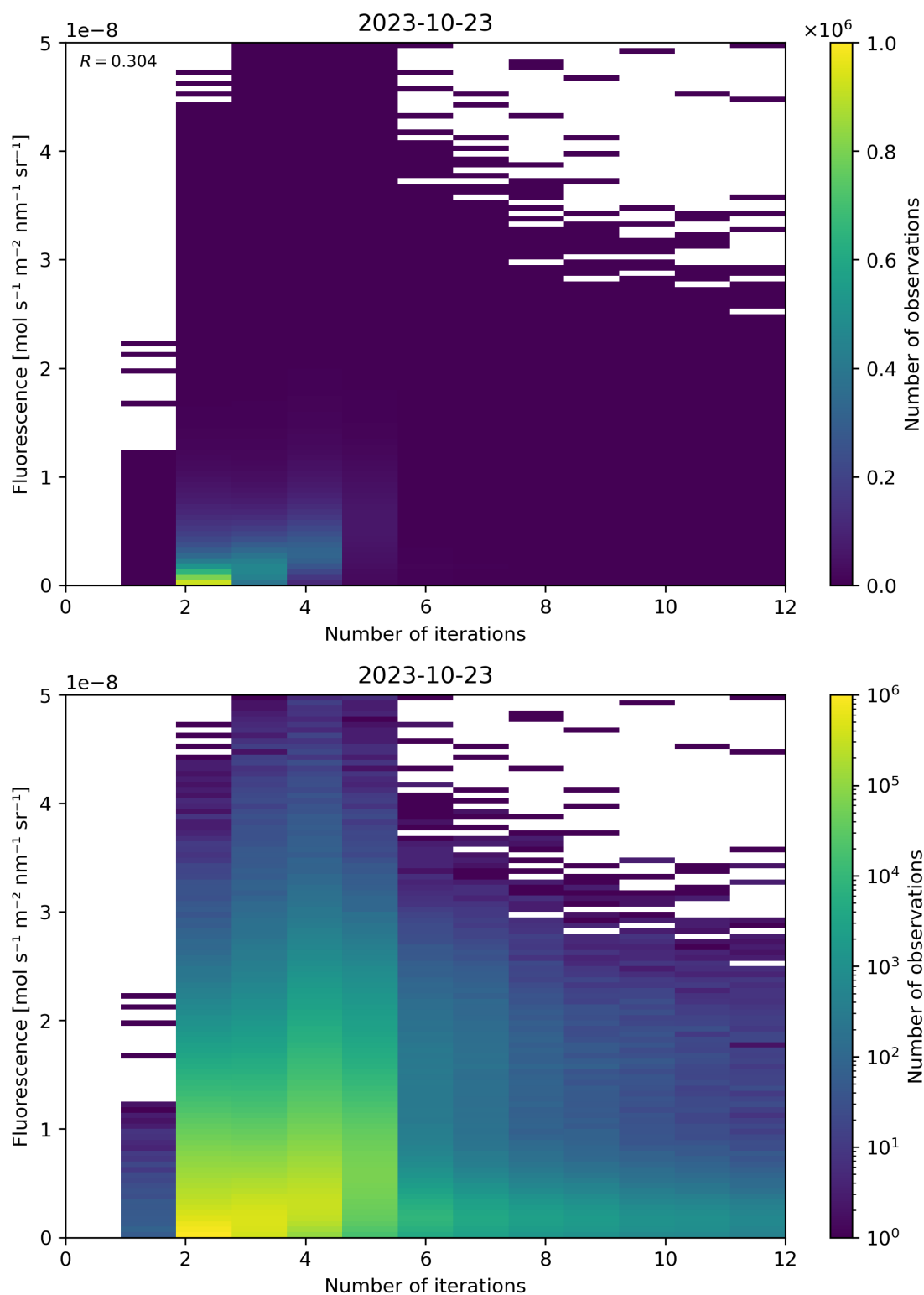
Figure 107: Scatter density plot of “Number of iterations” against “Fluorescence” for 2023-10-22 to 2023-10-24.
