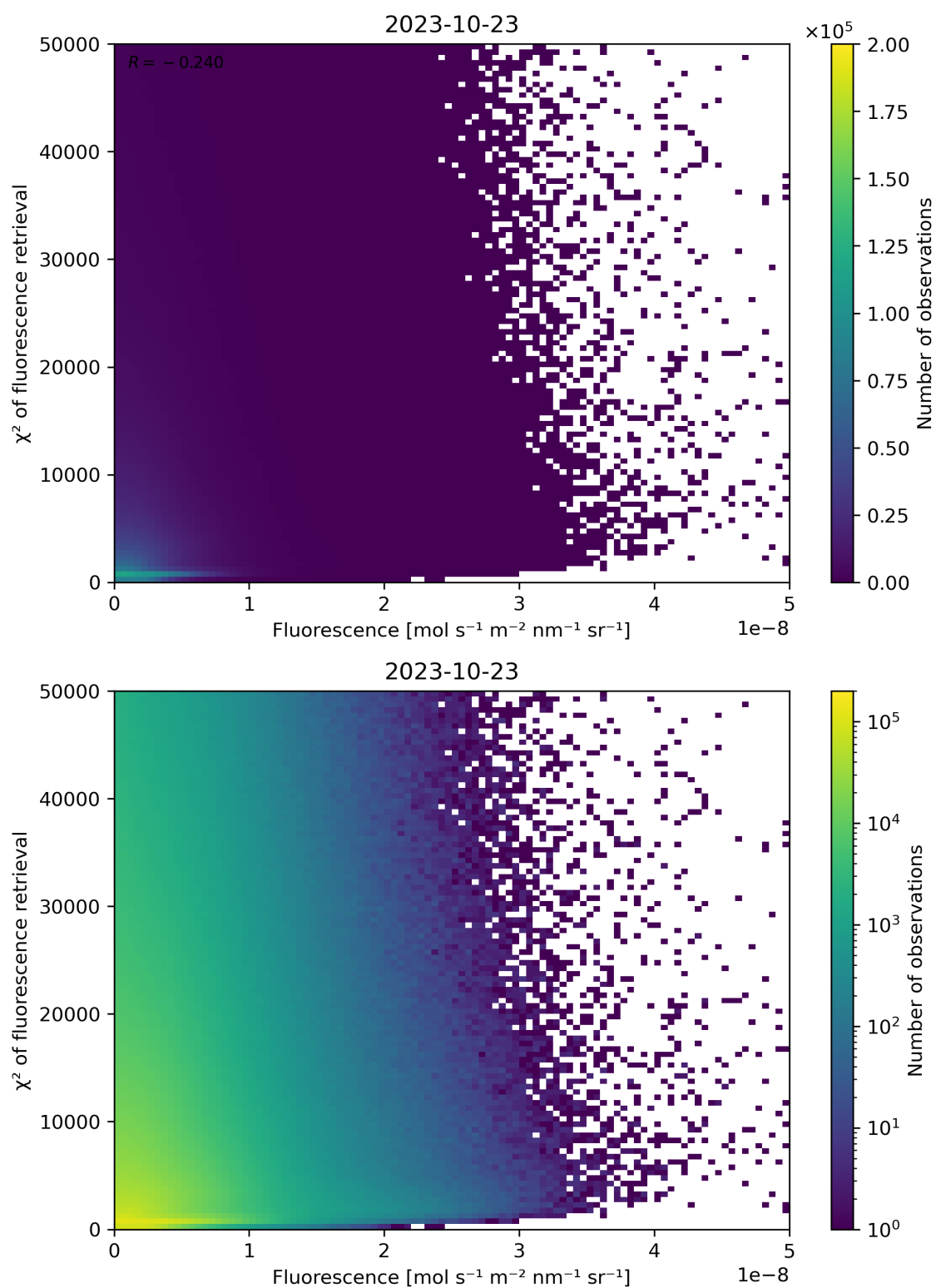
Figure 93: Scatter density plot of “Fluorescence” against “ \chi^2 of fluorescence retrieval” for 2023-10-22 to 2023-10-24.
