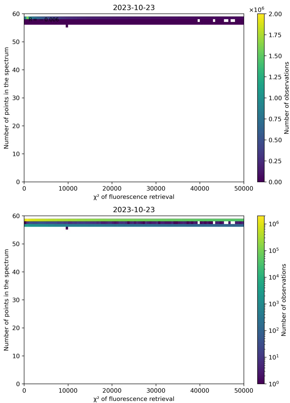
Figure 71: Scatter density plot of " \chi^2 of fluorescence retrieval" against "Number of points in the spectrum" for 2023-10-22 to 2023-10-24.
