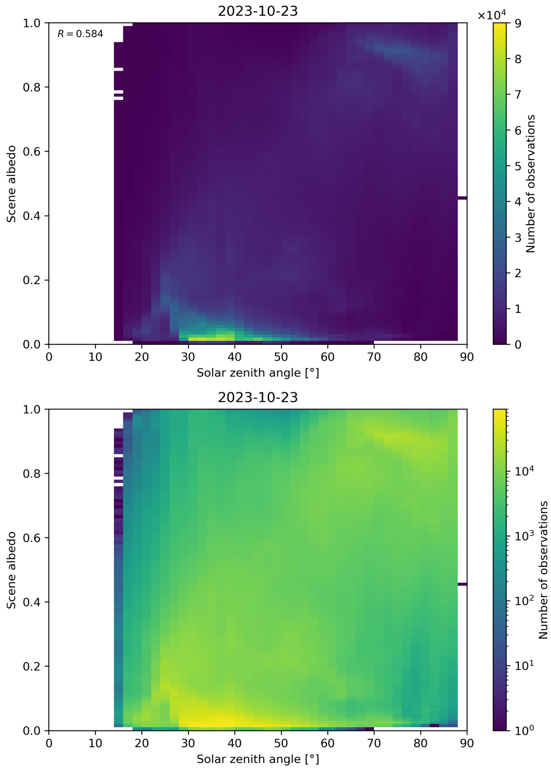
Figure 127: Scatter density plot of “Solar zenith angle” against “Scene albedo” for 2023-10-22 to 2023-10-24.
