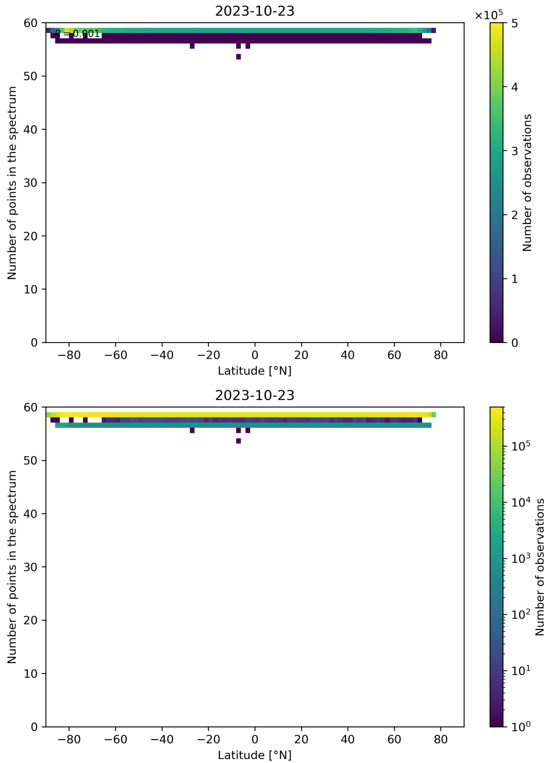
Figure 103: Scatter density plot of “Latitude” against “Number of points in the spectrum” for 2023-10-22 to 2023-10-24.
