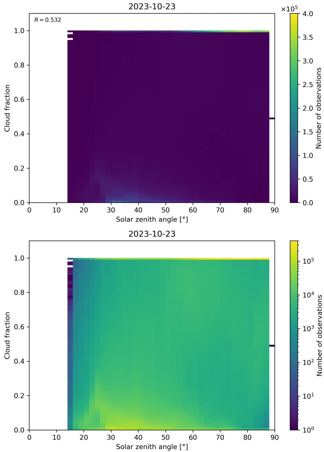
Figure 121: Scatter density plot of “Solar zenith angle” against “Cloud fraction” for 2023-10-22 to 2023-10-24.
