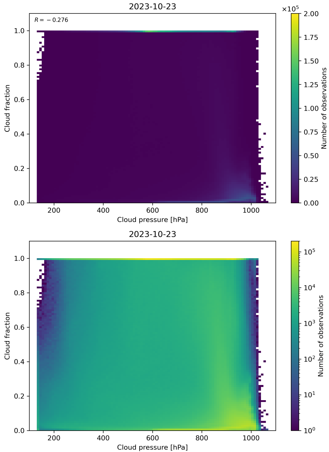
Figure 87: Scatter density plot of “Cloud pressure” against “Cloud fraction” for 2023-10-22 to 2023-10-24.
