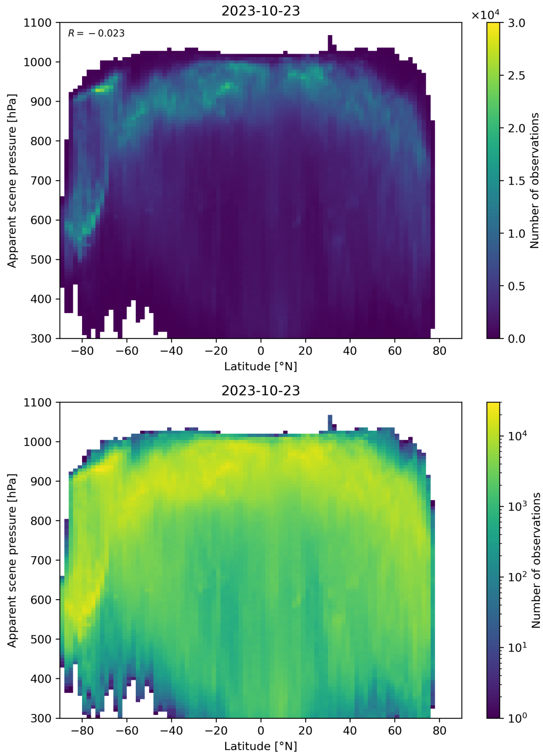
Figure 96: Scatter density plot of “Latitude” against “Apparent scene pressure” for 2023-10-22 to 2023-10-24.
