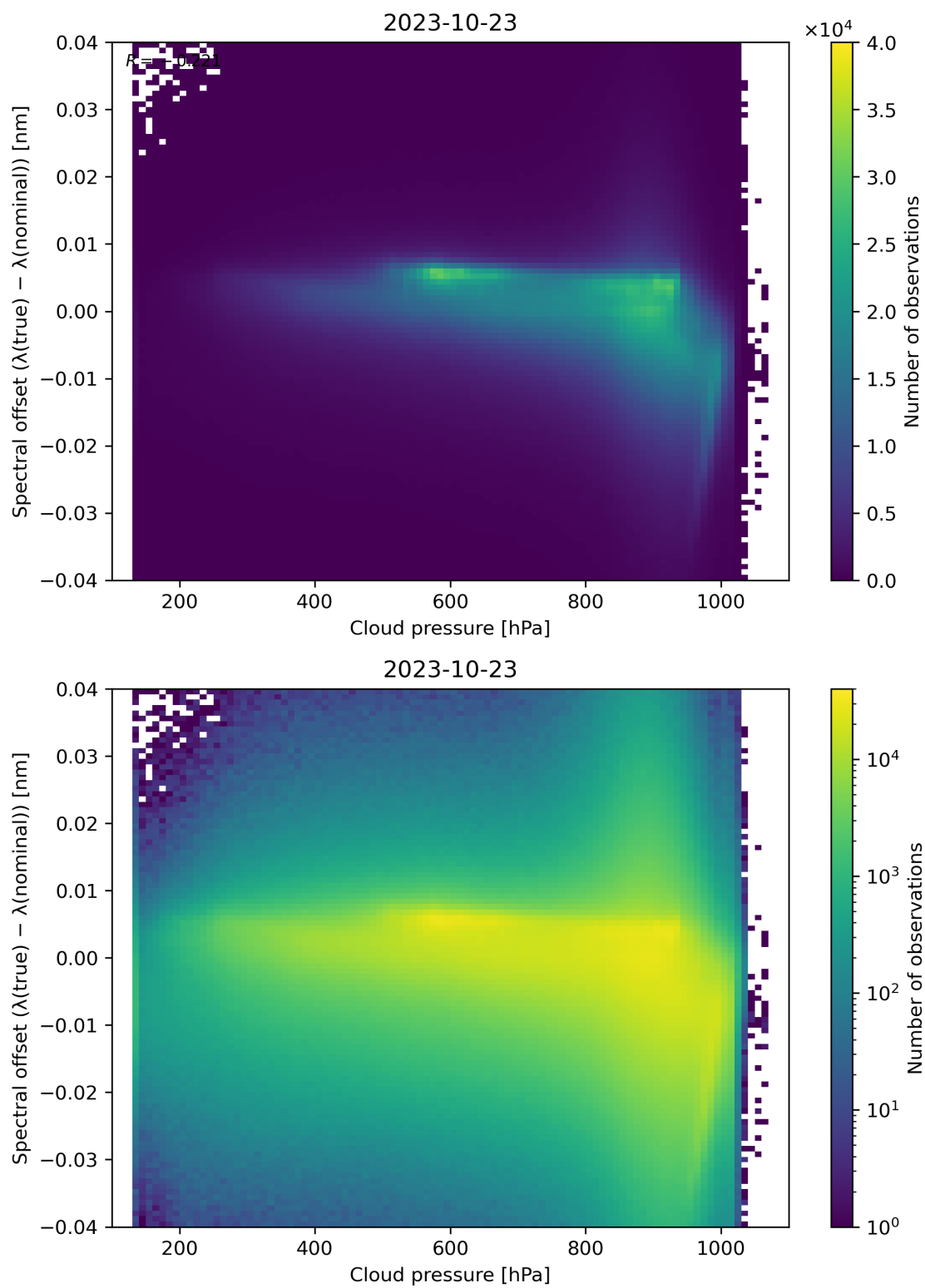
Figure 92: Scatter density plot of “Cloud pressure” against “Spectral offset ( \lambda(\text{true}) - \lambda(\text{nominal}) )” for 2023-10-22 to 2023-10-24.
