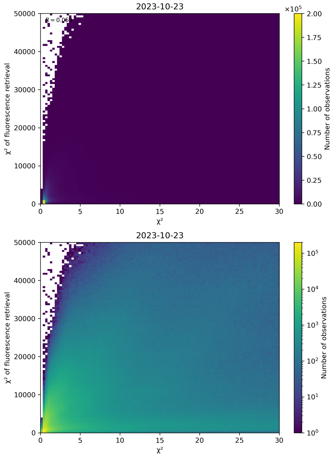
Figure 69: Scatter density plot of “ \chi^2 ” against “ \chi^2 of fluorescence retrieval” for 2023-10-22 to 2023-10-24.
