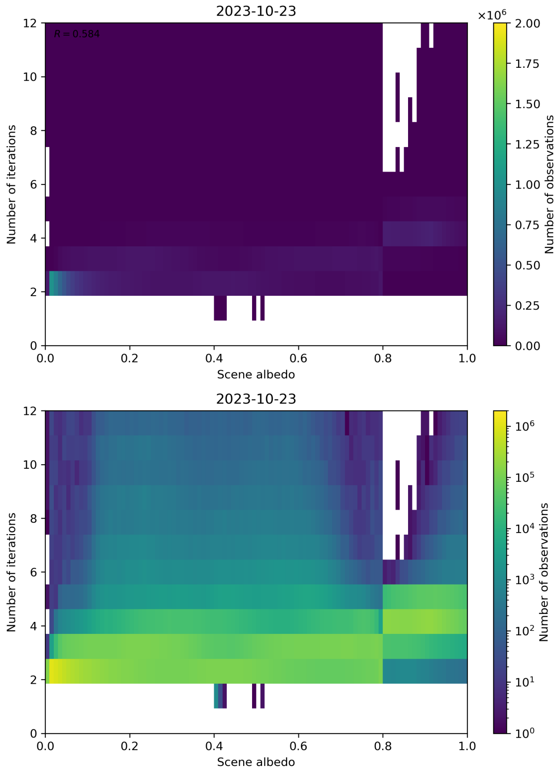
Figure 115: Scatter density plot of “Scene albedo” against “Number of iterations” for 2023-10-22 to 2023-10-24.
