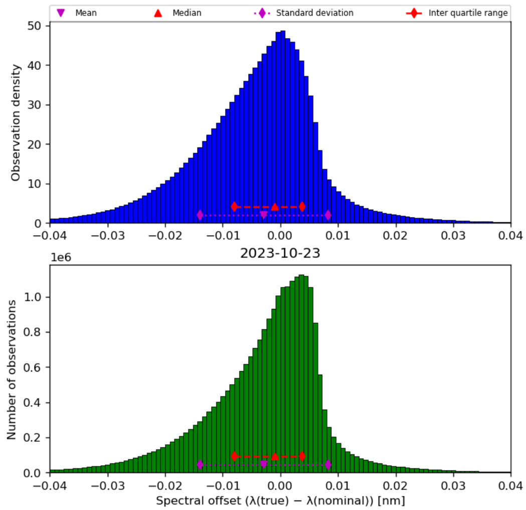
Figure 45: Histogram of “Spectral offset ( \lambda(\text{true}) - \lambda(\text{nominal}) )” for 2023-10-22 to 2023-10-24
