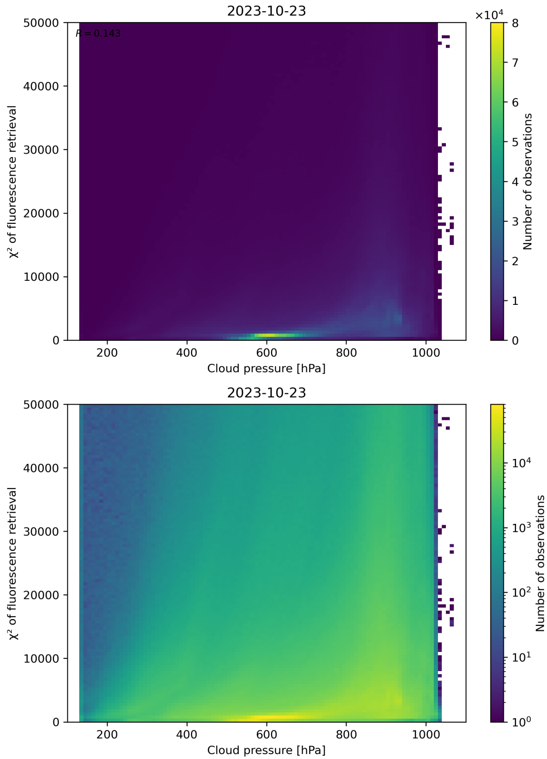
Figure 86: Scatter density plot of “Cloud pressure” against “ \chi^2 of fluorescence retrieval” for 2023-10-22 to 2023-10-24.
