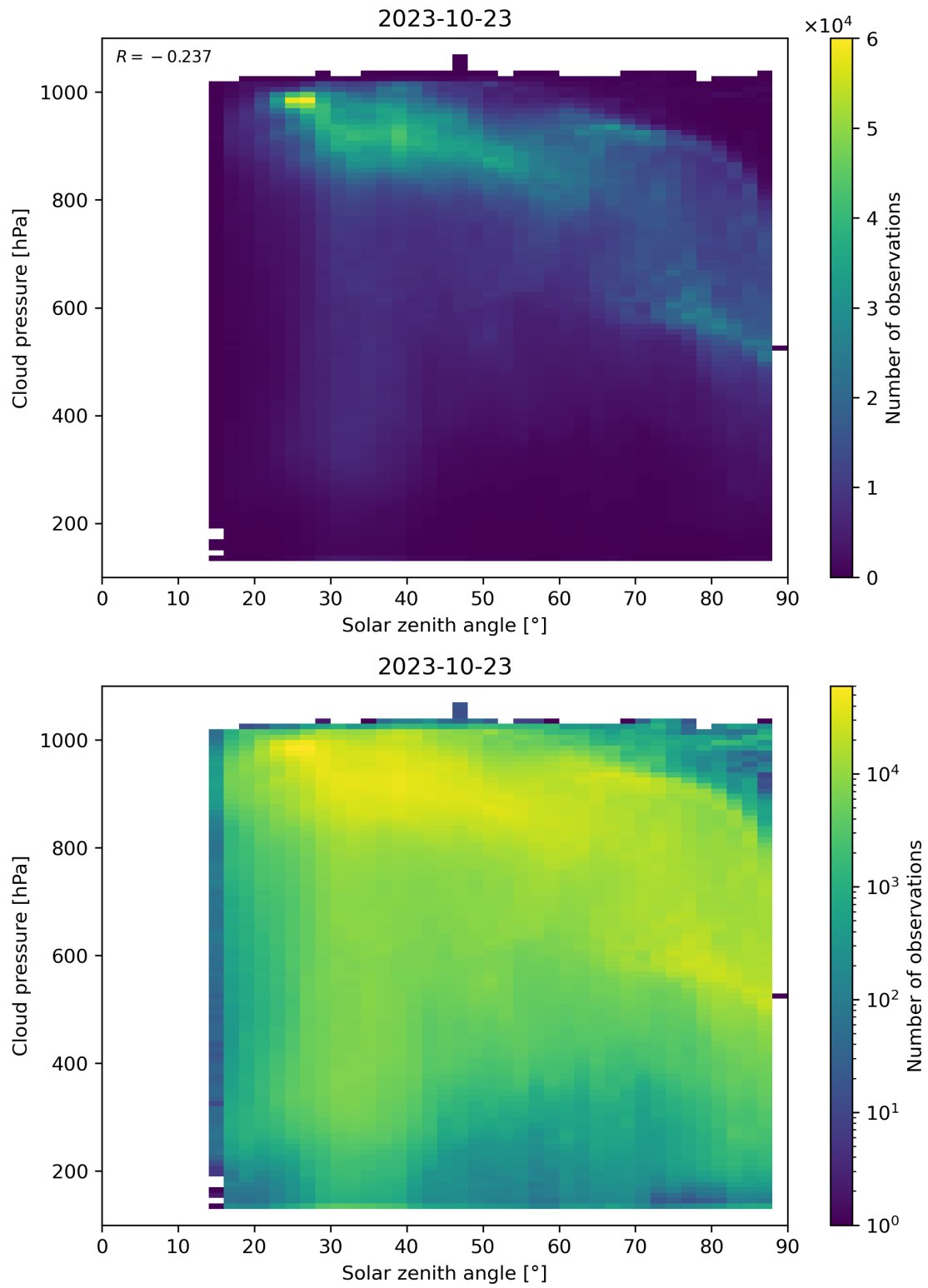
Figure 122: Scatter density plot of “Solar zenith angle” against “Cloud pressure” for 2023-10-22 to 2023-10-24.
