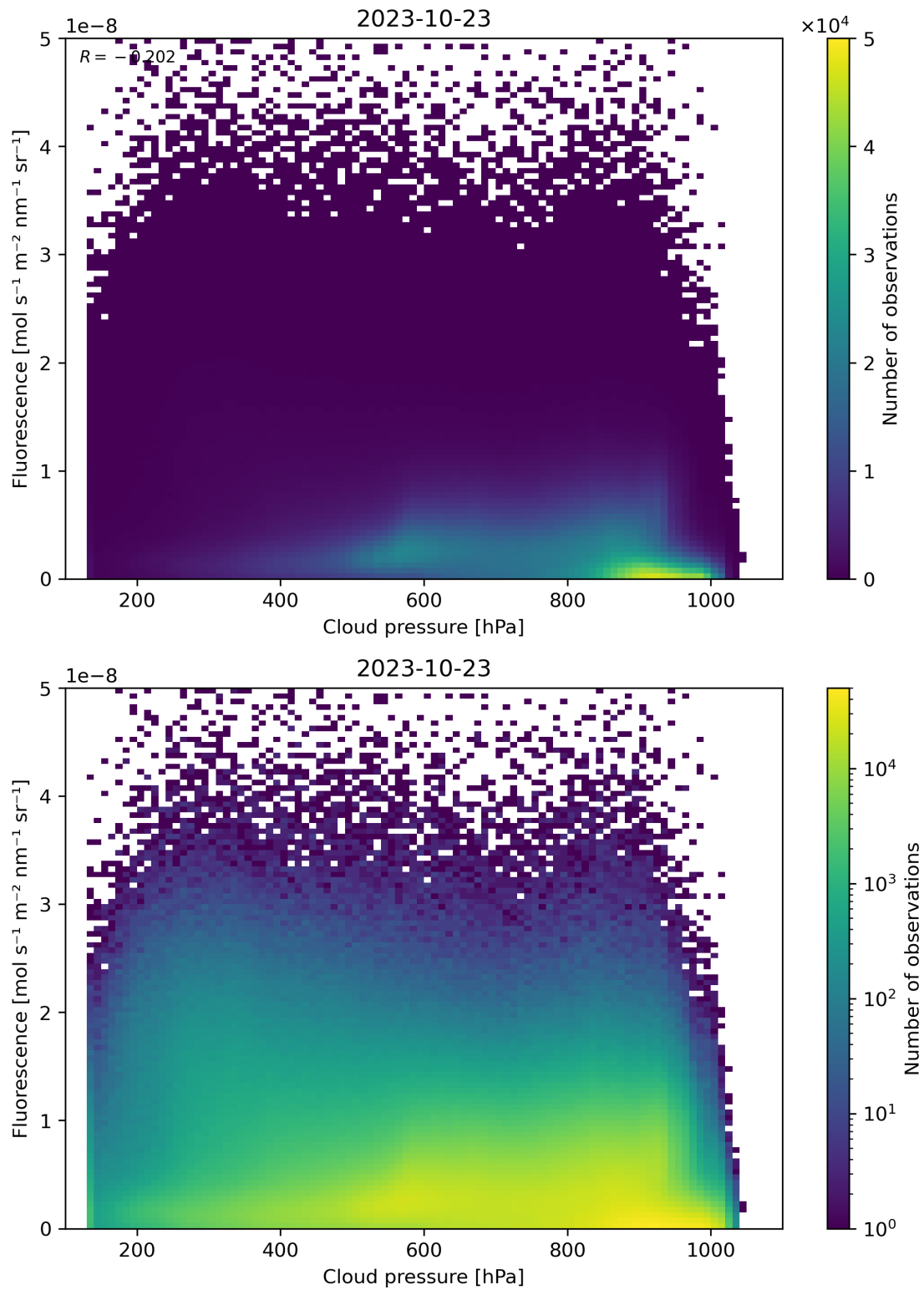
Figure 88: Scatter density plot of “Cloud pressure” against “Fluorescence” for 2023-10-22 to 2023-10-24.
