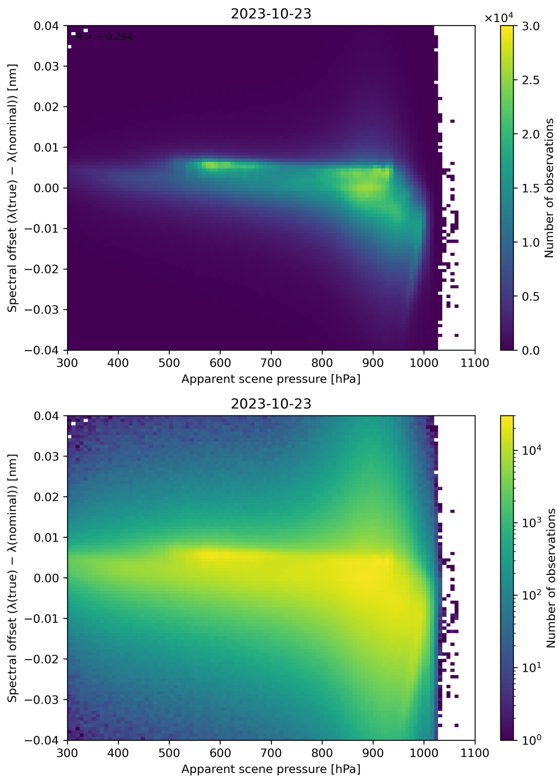
Figure 68: Scatter density plot of “Apparent scene pressure” against “Spectral offset ( \lambda(\text{true}) - \lambda(\text{nominal}) )” for 2023-10-22 to 2023-10-24.
