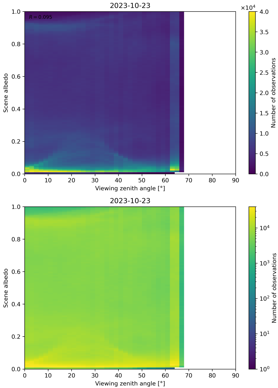
Figure 138: Scatter density plot of “Viewing zenith angle” against “Scene albedo” for 2023-10-22 to 2023-10-24.
