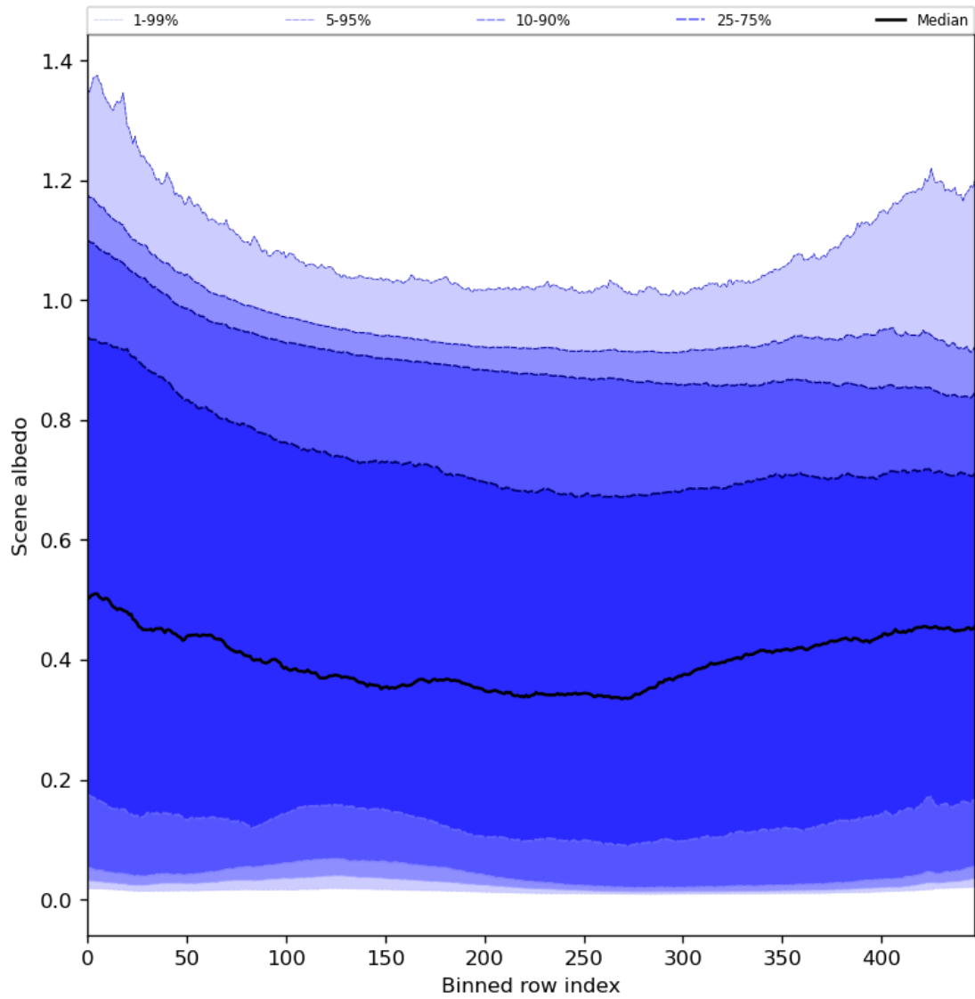
Figure 51: Along track statistics of “Scene albedo” for 2023-10-22 to 2023-10-24
