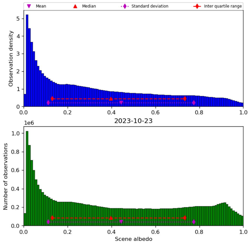
Figure 34: Histogram of “Scene albedo” for 2023-10-22 to 2023-10-24
