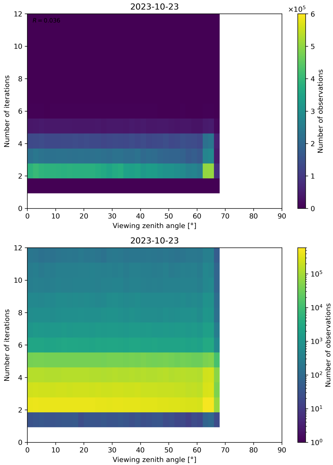
Figure 136: Scatter density plot of “Viewing zenith angle” against “Number of iterations” for 2023-10-22 to 2023-10-24.
