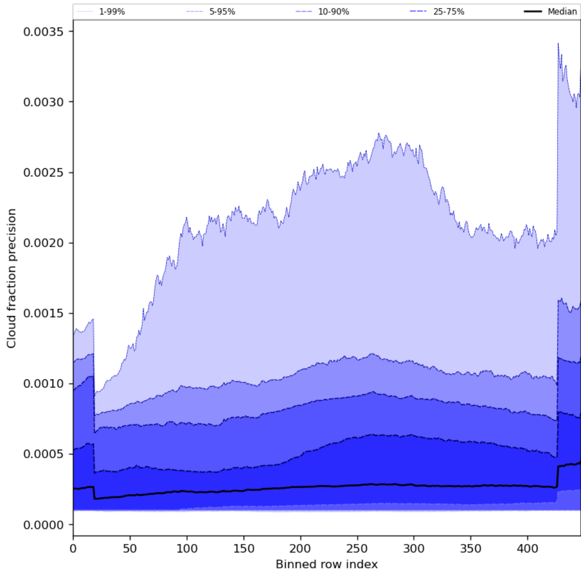
Figure 50: Along track statistics of “Cloud fraction precision” for 2023-10-22 to 2023-10-24
