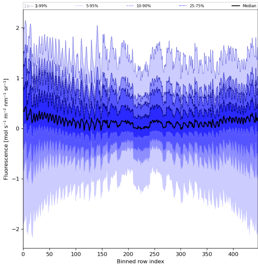
Figure 57: Along track statistics of “Fluorescence” for 2023-10-22 to 2023-10-24
