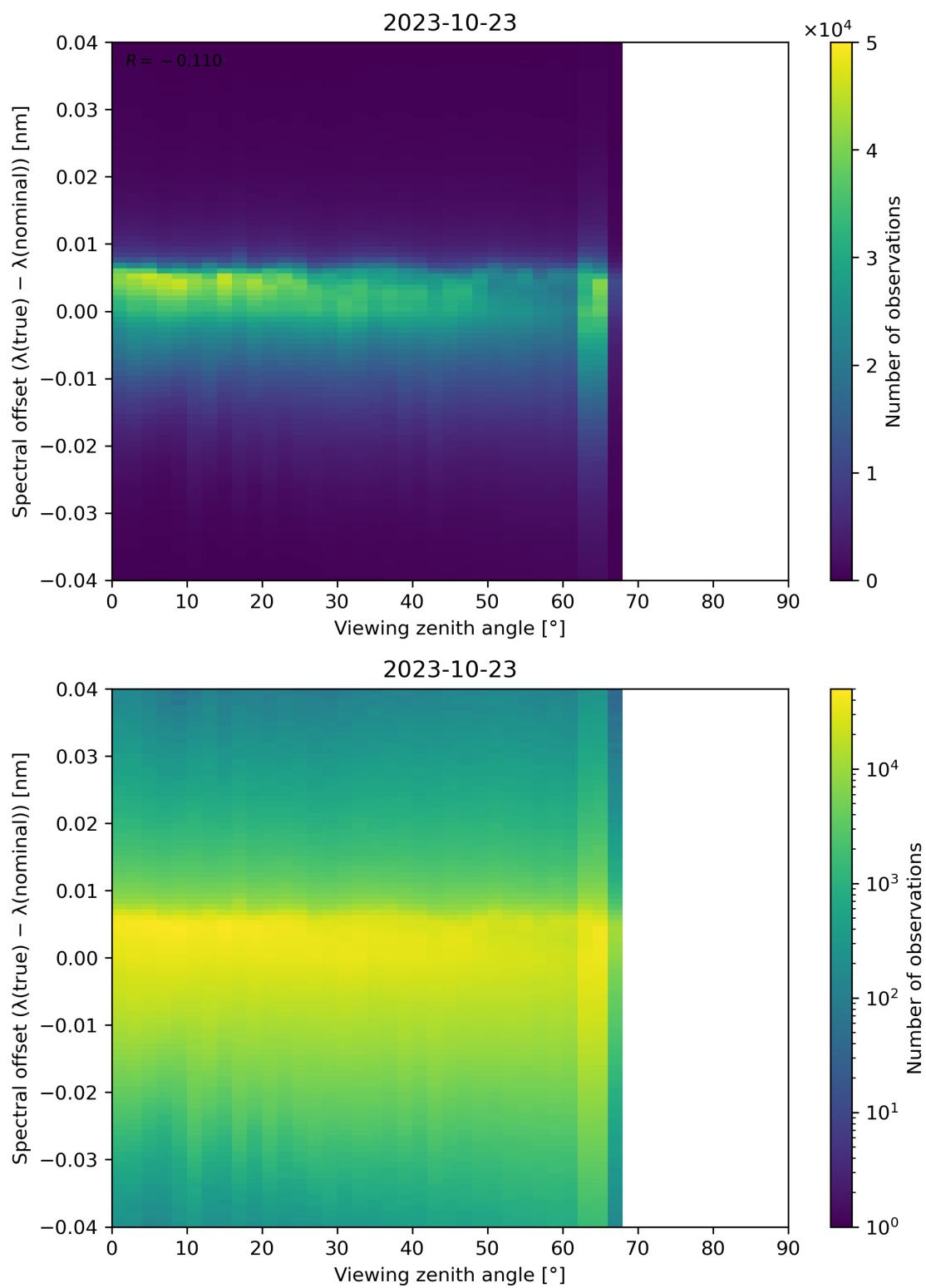
Figure 140: Scatter density plot of “Viewing zenith angle” against “Spectral offset ( \lambda(\text{true}) - \lambda(\text{nominal}) )” for 2023-10-22 to 2023-10-24.
