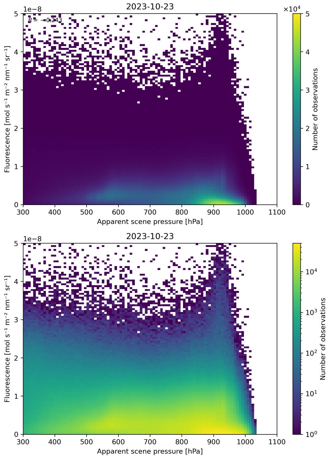
Figure 65: Scatter density plot of “Apparent scene pressure” against “Fluorescence” for 2023-10-22 to 2023-10-24.
