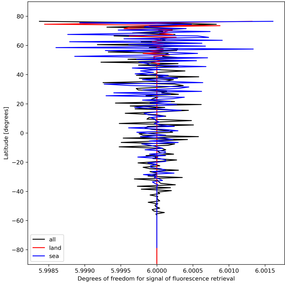
Figure 26: Zonal average of “Degrees of freedom for signal of fluorescence retrieval” for 2023-10-22 to 2023-10-24.
