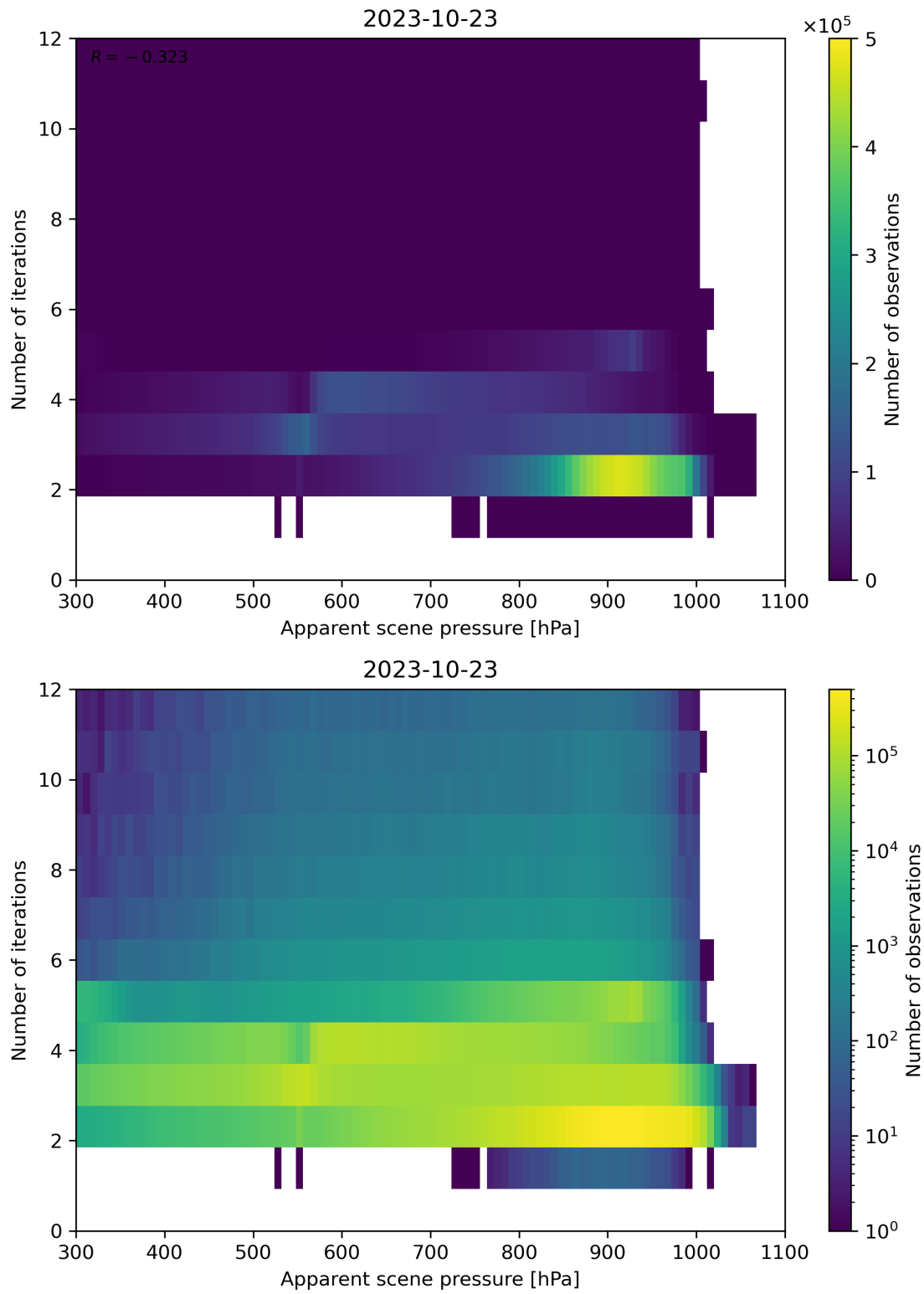
Figure 66: Scatter density plot of “Apparent scene pressure” against “Number of iterations” for 2023-10-22 to 2023-10-24.
