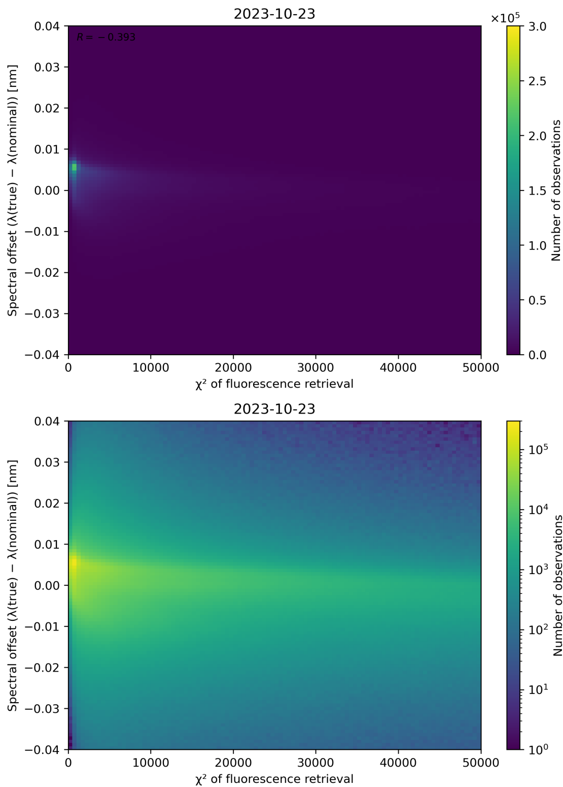
Figure 72: Scatter density plot of " \chi^2 of fluorescence retrieval" against "Spectral offset ( \lambda(\text{true}) - \lambda(\text{nominal}) )" for 2023-10-22 to 2023-10-24.
