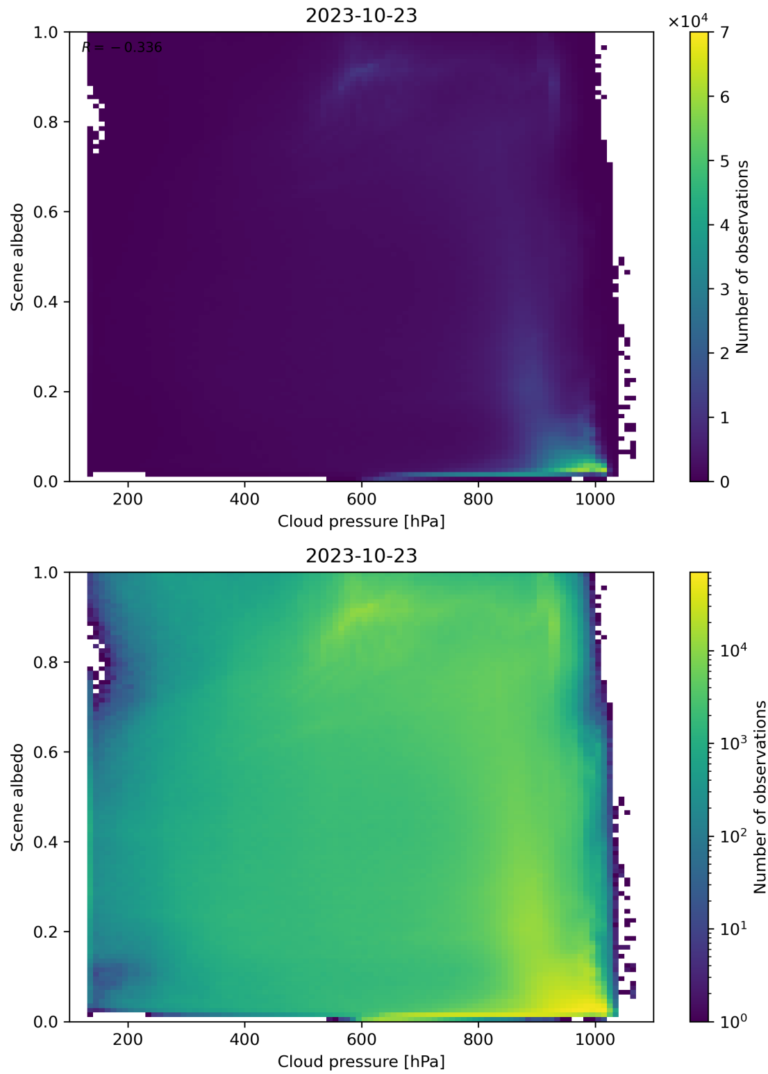
Figure 91: Scatter density plot of “Cloud pressure” against “Scene albedo” for 2023-10-22 to 2023-10-24.
