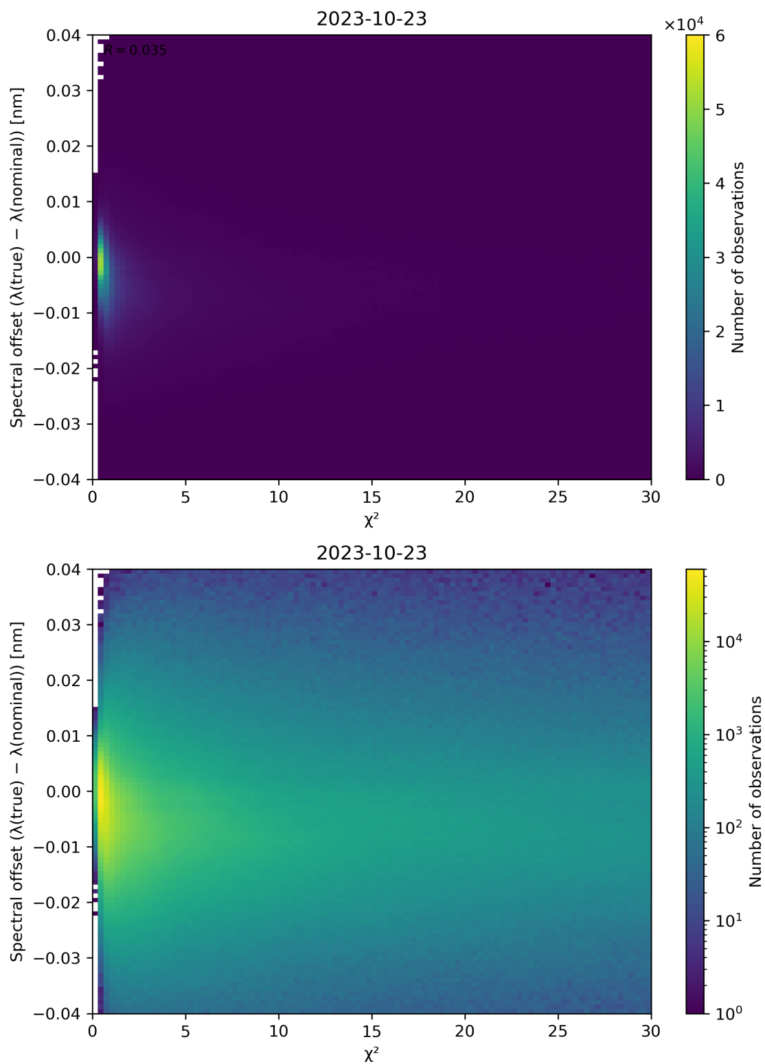
Figure 75: Scatter density plot of “ \chi^2 ” against “Spectral offset ( \lambda(\text{true}) - \lambda(\text{nominal}) )” for 2023-10-22 to 2023-10-24.
