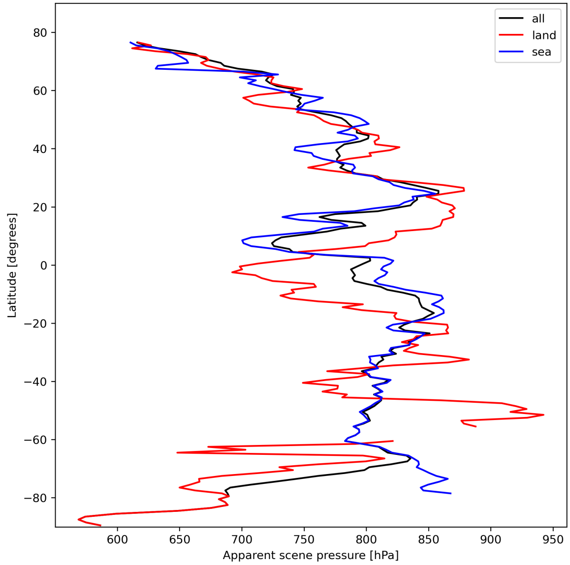
Figure 19: Zonal average of “Apparent scene pressure” for 2023-10-22 to 2023-10-24.
