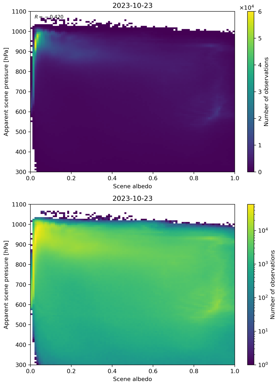
Figure 111: Scatter density plot of “Scene albedo” against “Apparent scene pressure” for 2023-10-22 to 2023-10-24.
