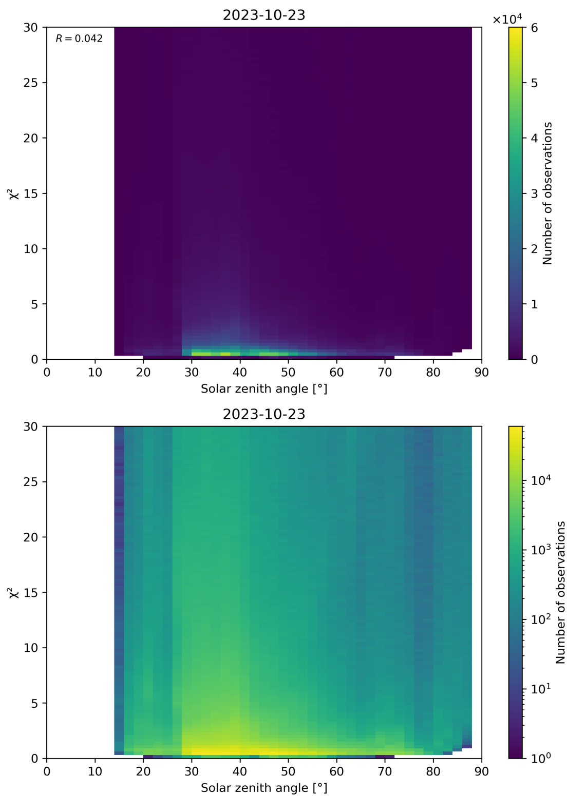
Figure 119: Scatter density plot of “Solar zenith angle” against “ \chi^2 ” for 2023-10-22 to 2023-10-24.
