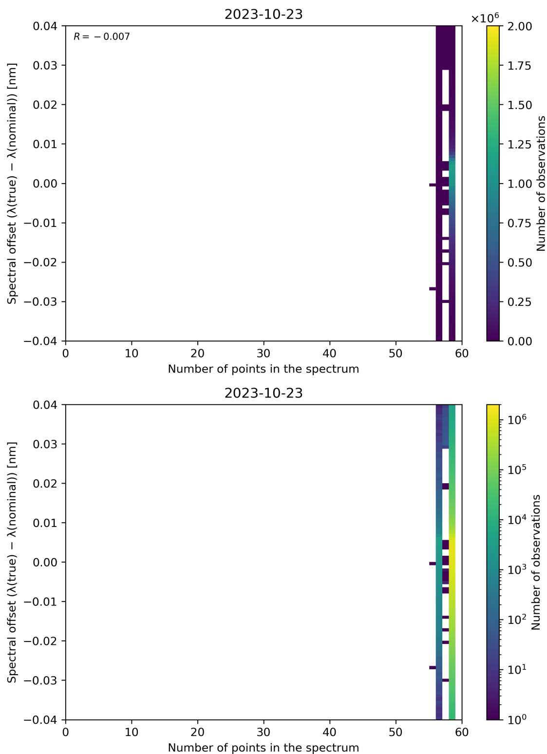
Figure 110: Scatter density plot of “Number of points in the spectrum” against “Spectral offset ( \lambda(\text{true}) - \lambda(\text{nominal}) )” for 2023-10-22 to 2023-10-24.
