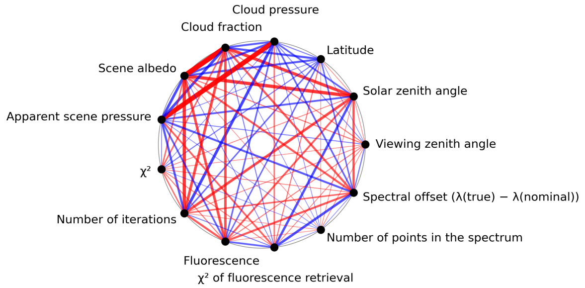
Figure 1: Map of correlation graph for 2023-10-22 to 2023-10-24.
