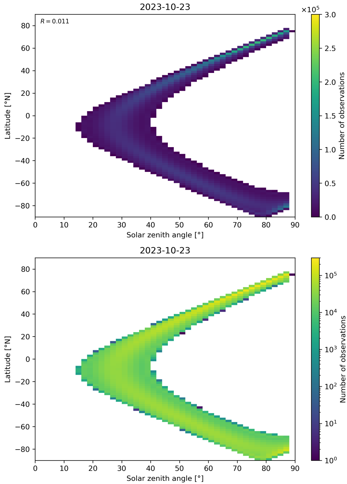
Figure 124: Scatter density plot of “Solar zenith angle” against “Latitude” for 2023-10-22 to 2023-10-24.
