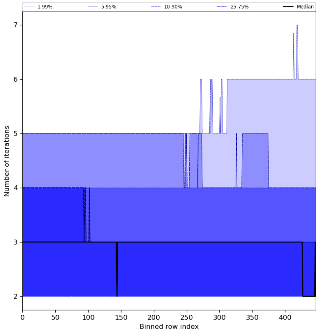
Figure 56: Along track statistics of “Number of iterations” for 2023-10-22 to 2023-10-24
