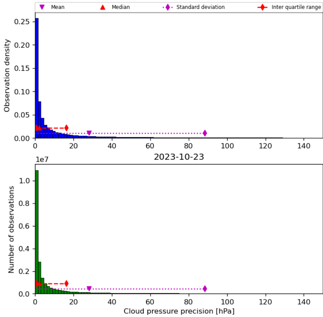
Figure 31: Histogram of “Cloud pressure precision” for 2023-10-22 to 2023-10-24
