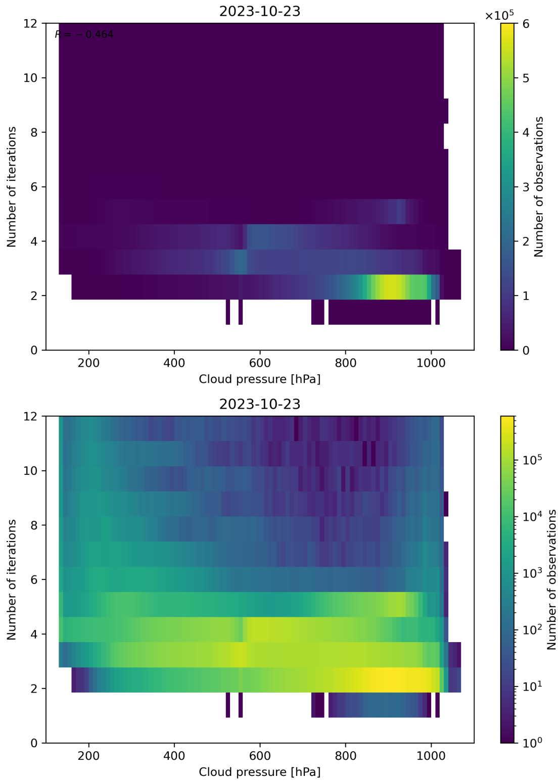
Figure 89: Scatter density plot of “Cloud pressure” against “Number of iterations” for 2023-10-22 to 2023-10-24.
