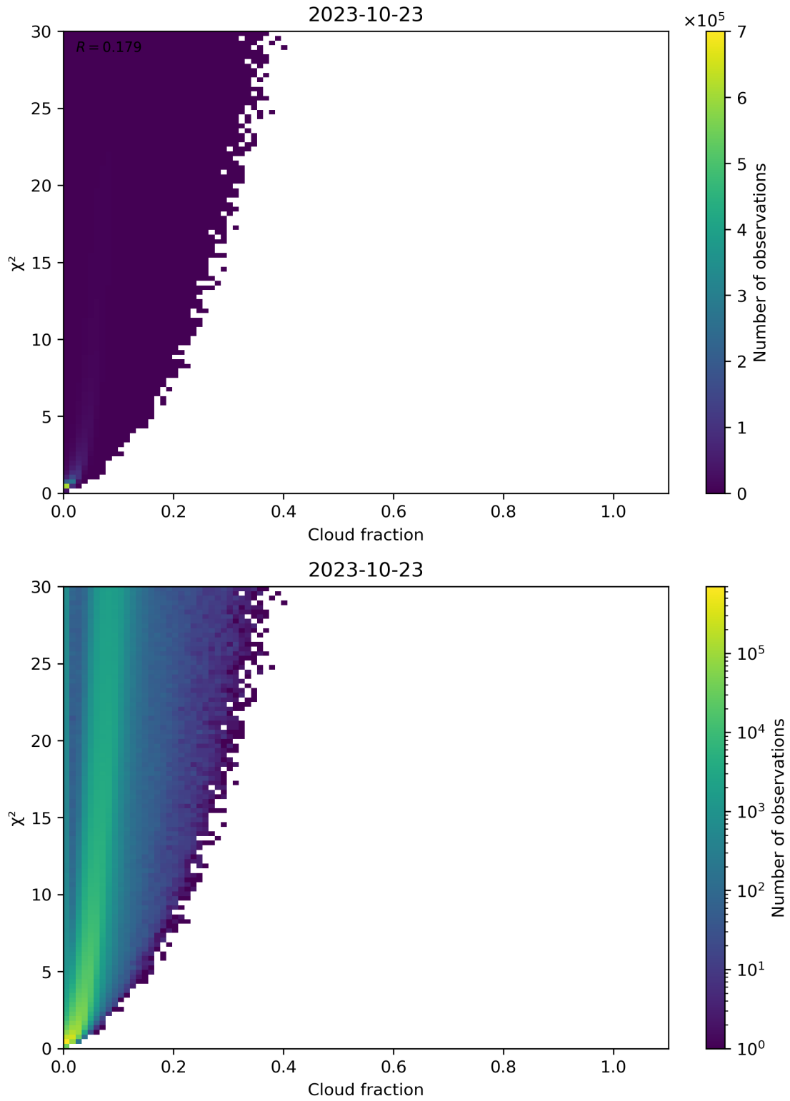
Figure 77: Scatter density plot of “Cloud fraction” against “ \chi^2 ” for 2023-10-22 to 2023-10-24.
