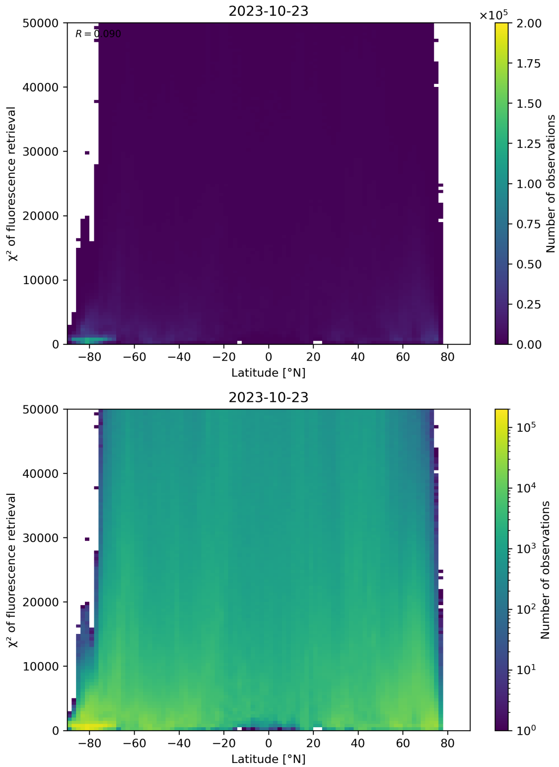
Figure 98: Scatter density plot of “Latitude” against “ \chi^2 of fluorescence retrieval” for 2023-10-22 to 2023-10-24.
