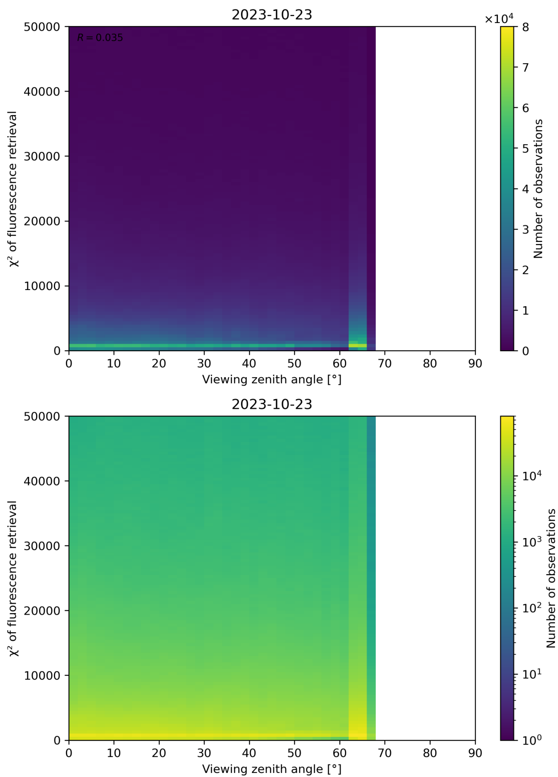
Figure 131: Scatter density plot of “Viewing zenith angle” against “ \chi^2 of fluorescence retrieval” for 2023-10-22 to 2023-10-24.
