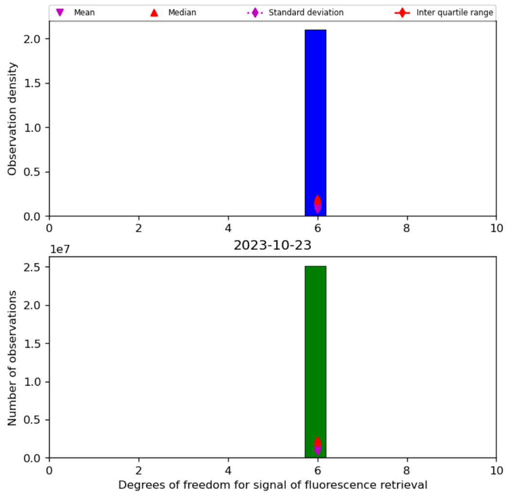
Figure 43: Histogram of “Degrees of freedom for signal of fluorescence retrieval” for 2023-10-22 to 2023-10-24
