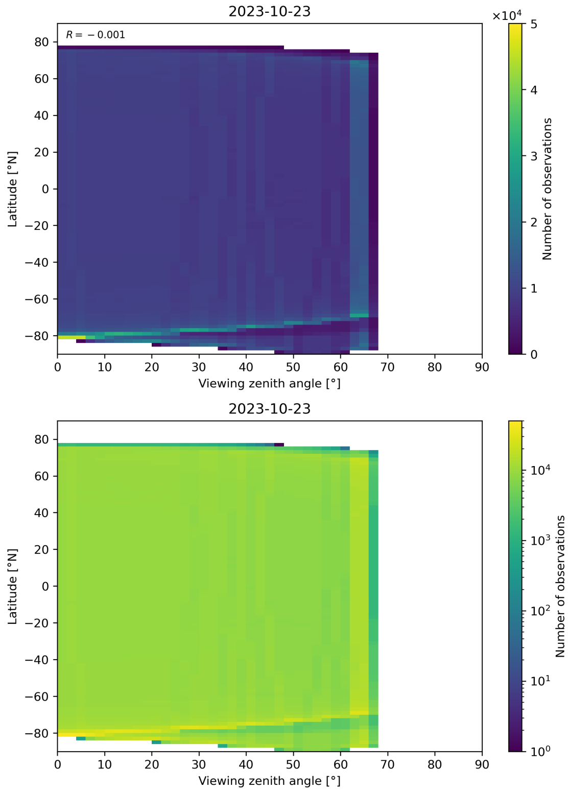
Figure 135: Scatter density plot of “Viewing zenith angle” against “Latitude” for 2023-10-22 to 2023-10-24.
