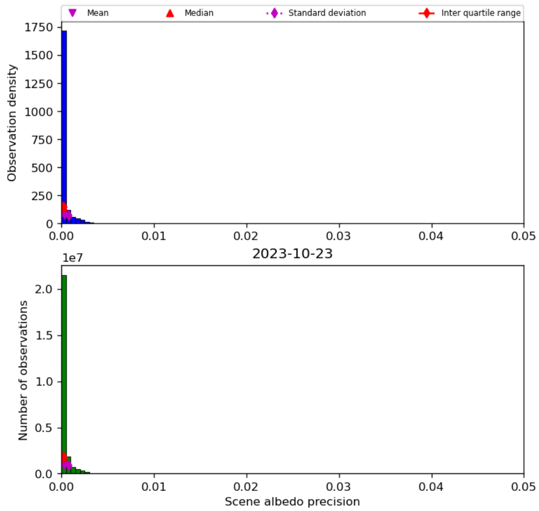
Figure 35: Histogram of “Scene albedo precision” for 2023-10-22 to 2023-10-24
