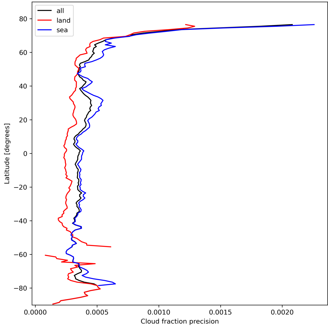
Figure 16: Zonal average of “Cloud fraction precision” for 2023-10-22 to 2023-10-24.
