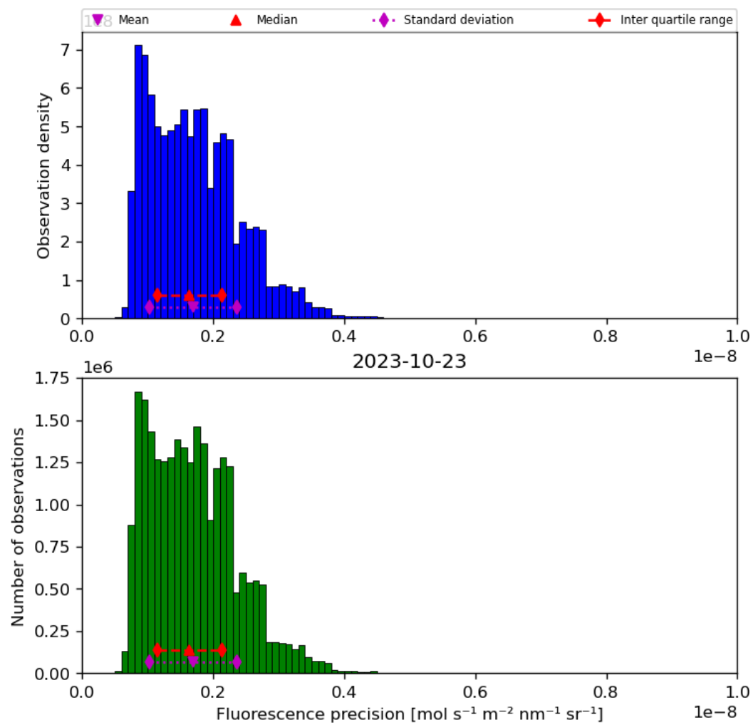
Figure 41: Histogram of “Fluorescence precision” for 2023-10-22 to 2023-10-24
