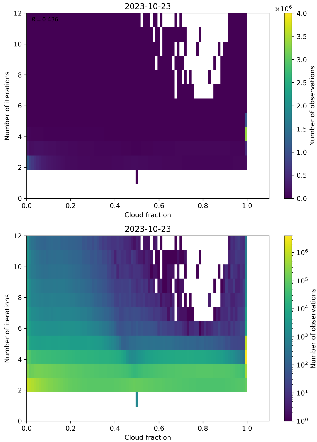
Figure 80: Scatter density plot of “Cloud fraction” against “Number of iterations” for 2023-10-22 to 2023-10-24.
