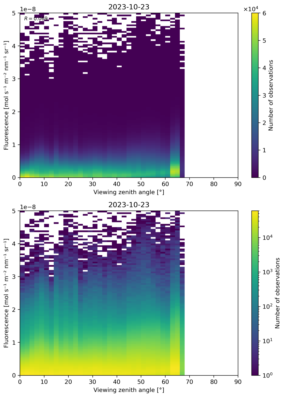
Figure 134: Scatter density plot of “Viewing zenith angle” against “Fluorescence” for 2023-10-22 to 2023-10-24.
