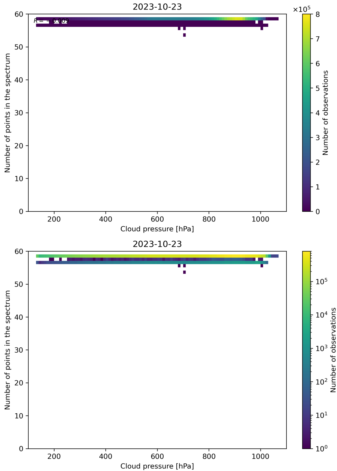
Figure 90: Scatter density plot of “Cloud pressure” against “Number of points in the spectrum” for 2023-10-22 to 2023-10-24.
