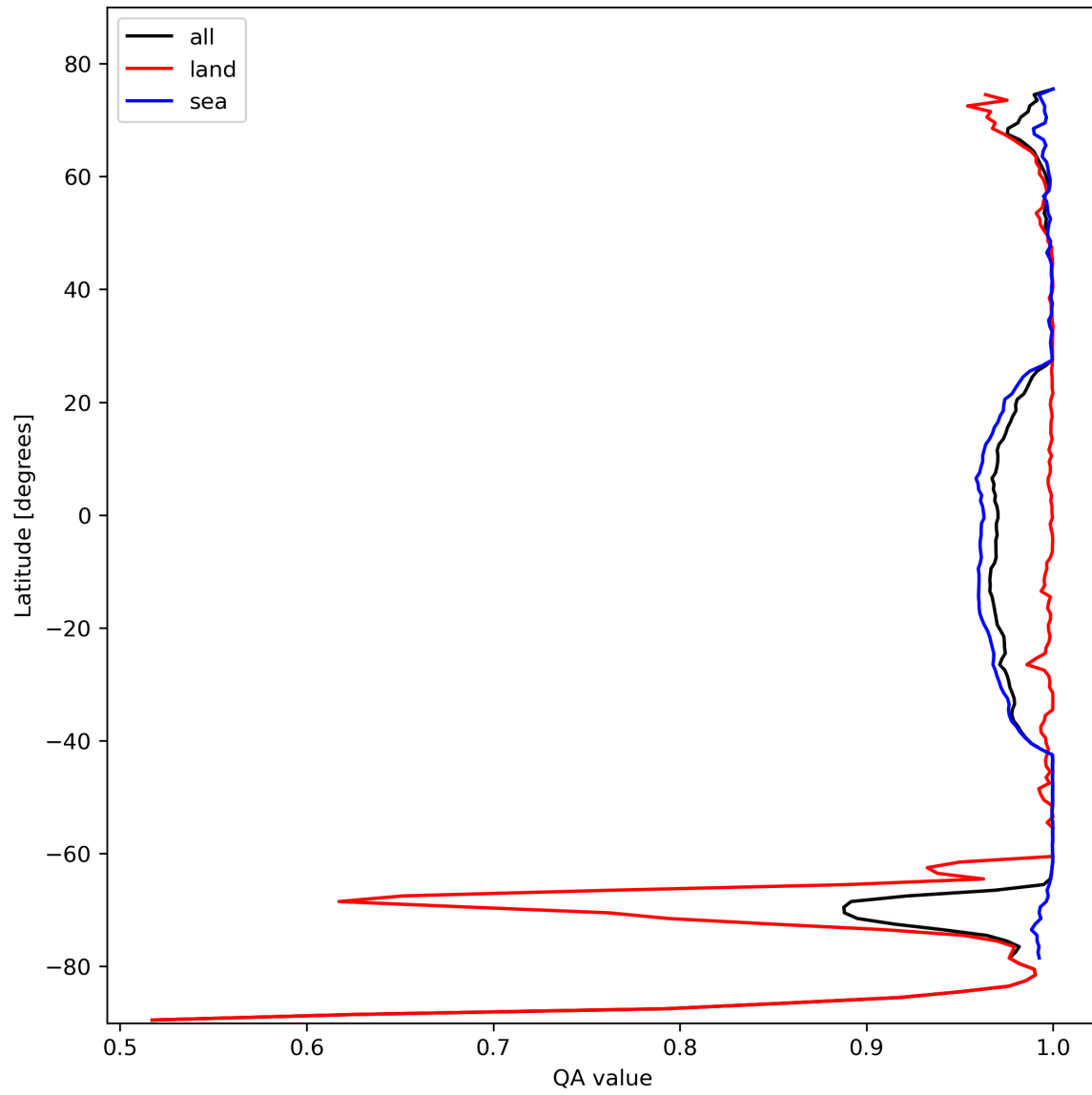
Figure 12: Zonal average of “QA value” for 2023-10-28 to 2023-10-29.
