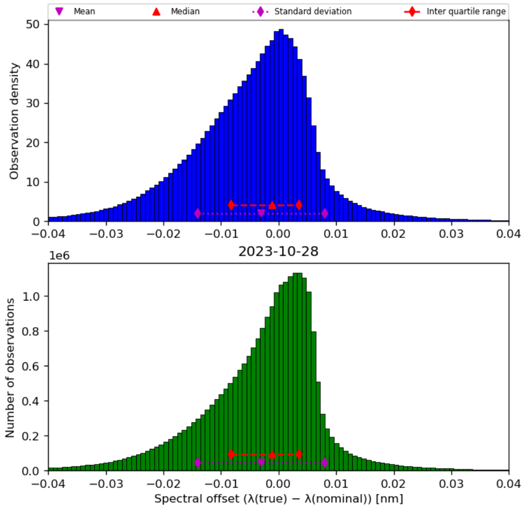
Figure 45: Histogram of “Spectral offset ( \lambda(\text{true}) - \lambda(\text{nominal}) )” for 2023-10-28 to 2023-10-29
