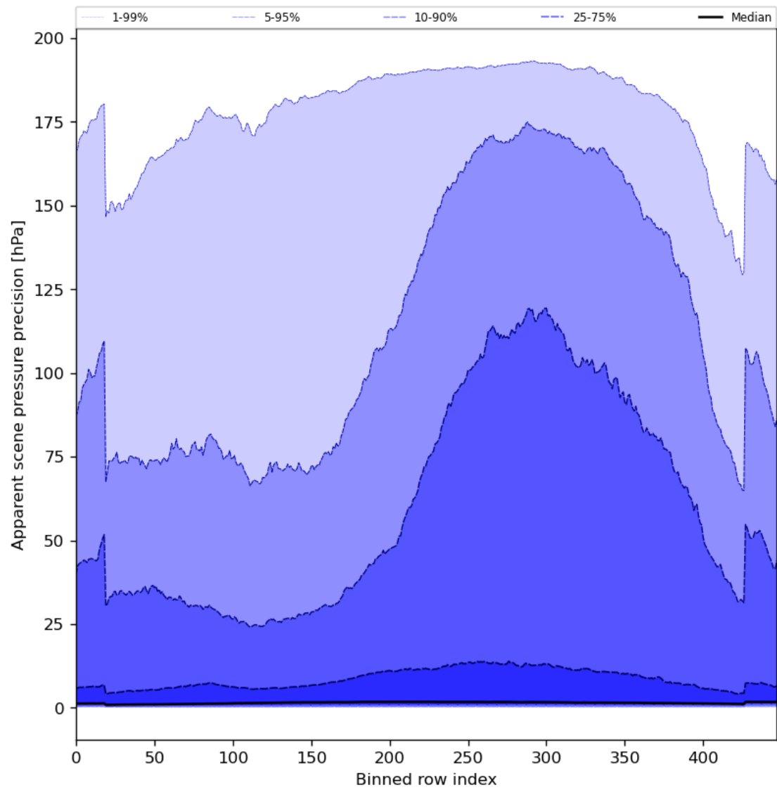
Figure 54: Along track statistics of “Apparent scene pressure precision” for 2023-10-28 to 2023-10-29
