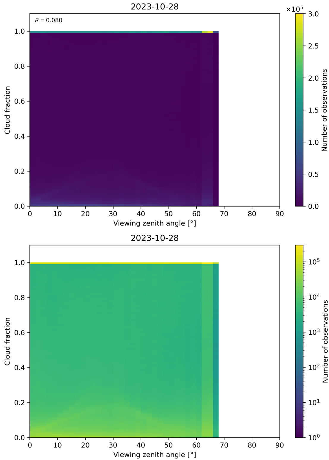
Figure 132: Scatter density plot of “Viewing zenith angle” against “Cloud fraction” for 2023-10-28 to 2023-10-29.
