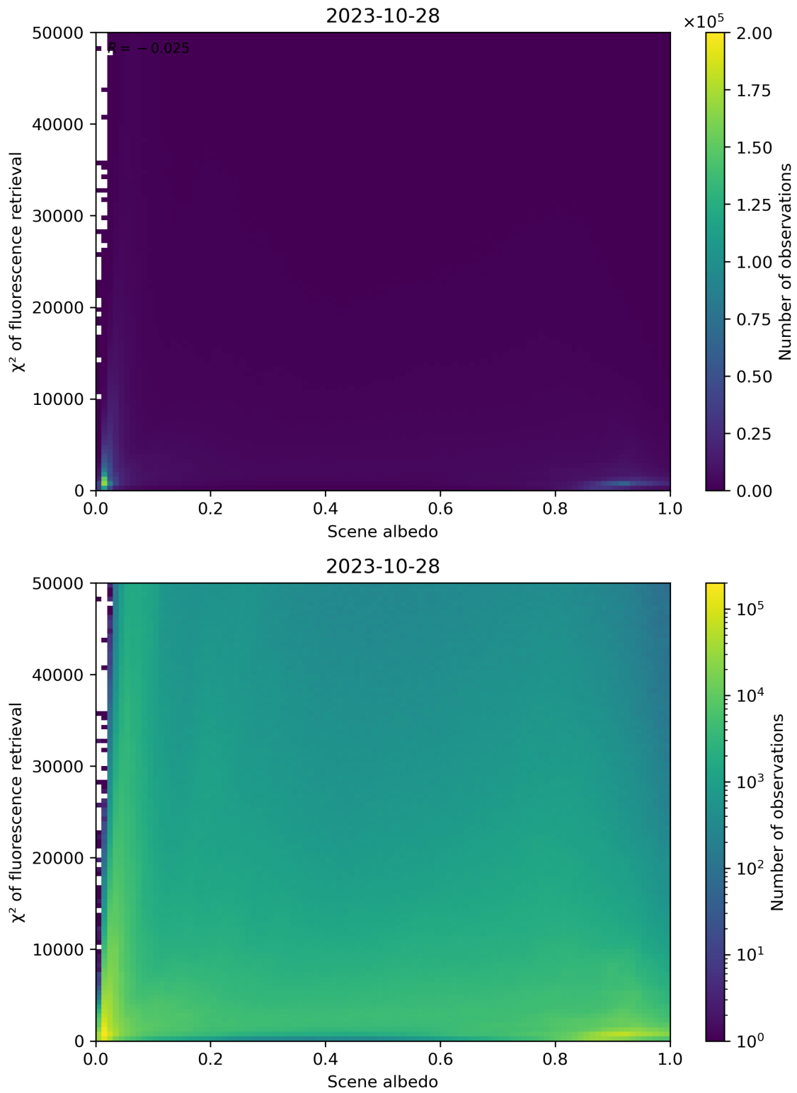
Figure 113: Scatter density plot of “Scene albedo” against “ \chi^2 of fluorescence retrieval” for 2023-10-28 to 2023-10-29.
