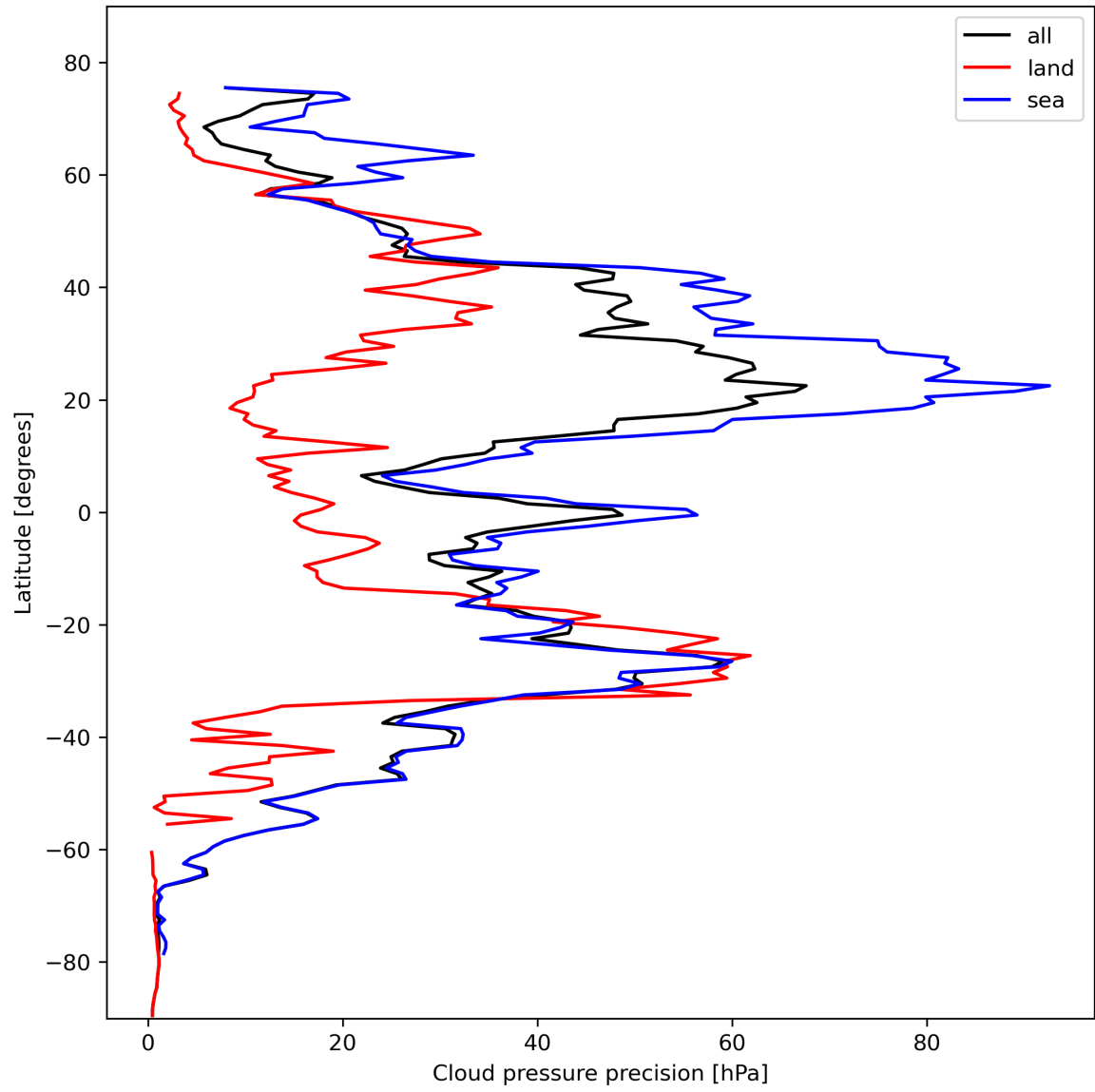
Figure 14: Zonal average of “Cloud pressure precision” for 2023-10-28 to 2023-10-29.
