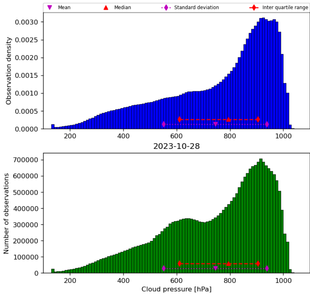
Figure 30: Histogram of “Cloud pressure” for 2023-10-28 to 2023-10-29
