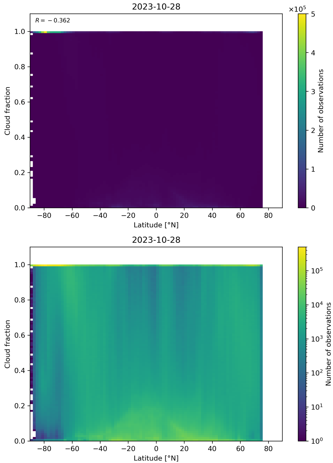
Figure 99: Scatter density plot of “Latitude” against “Cloud fraction” for 2023-10-28 to 2023-10-29.
