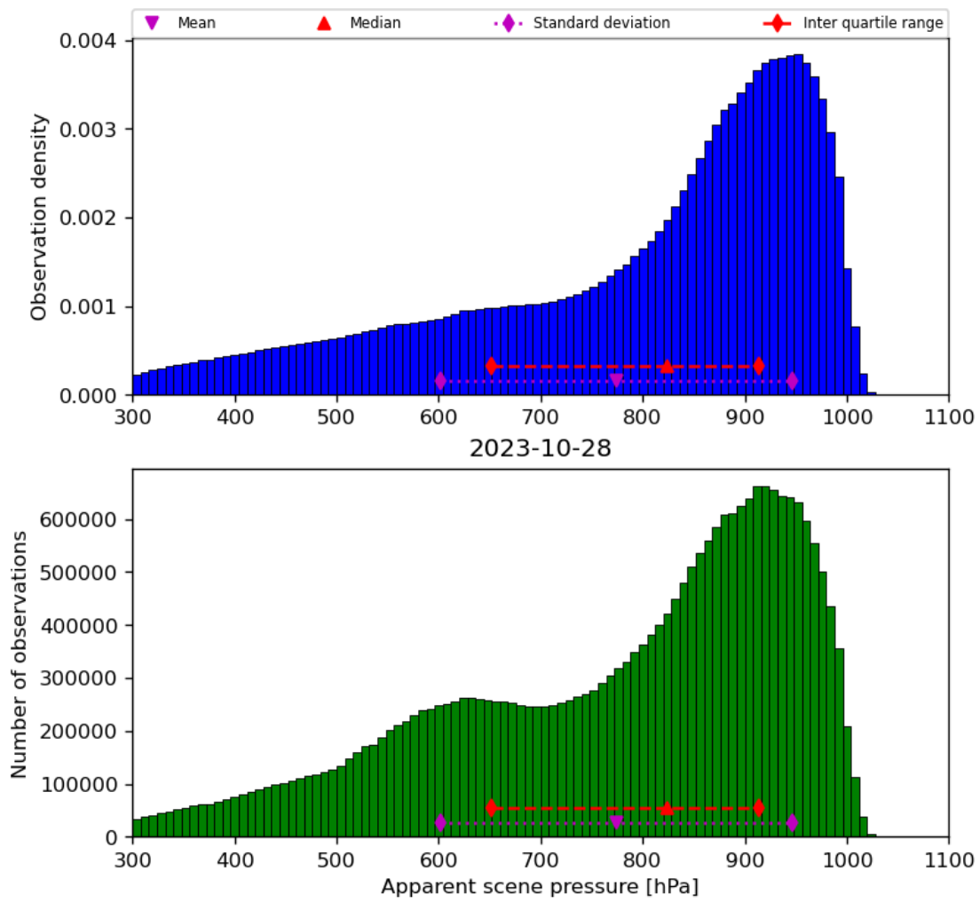
Figure 36: Histogram of “Apparent scene pressure” for 2023-10-28 to 2023-10-29
