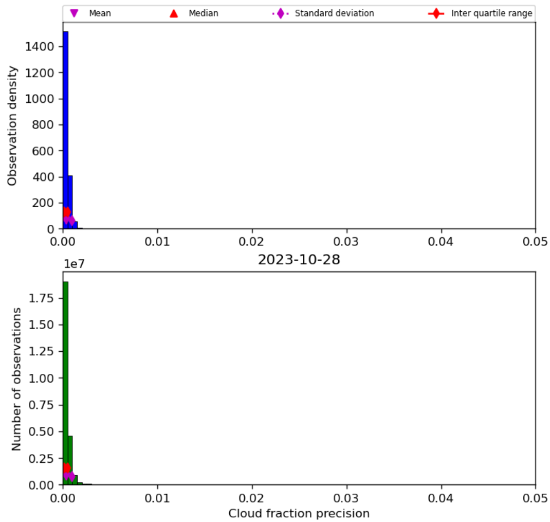
Figure 33: Histogram of “Cloud fraction precision” for 2023-10-28 to 2023-10-29
