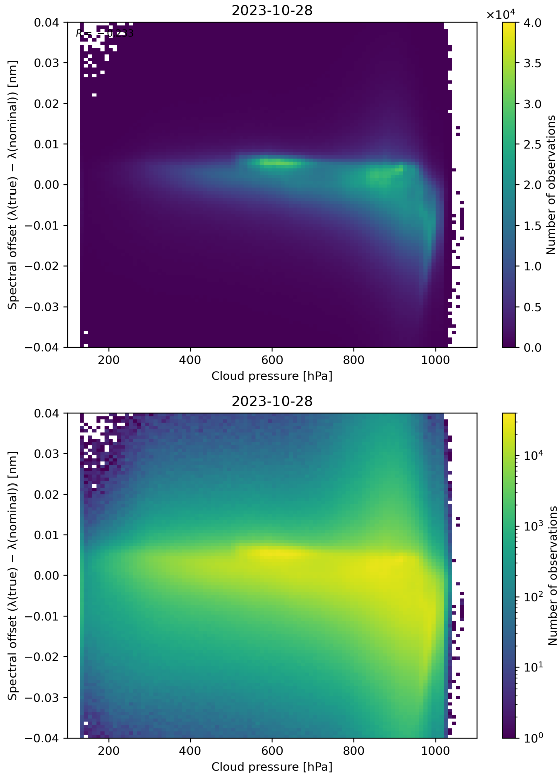
Figure 92: Scatter density plot of “Cloud pressure” against “Spectral offset ( \lambda(\text{true}) - \lambda(\text{nominal}) )” for 2023-10-28 to 2023-10-29.
