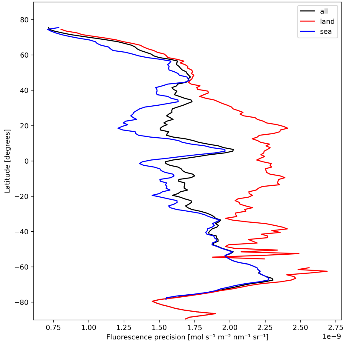
Figure 24: Zonal average of “Fluorescence precision” for 2023-10-28 to 2023-10-29.
