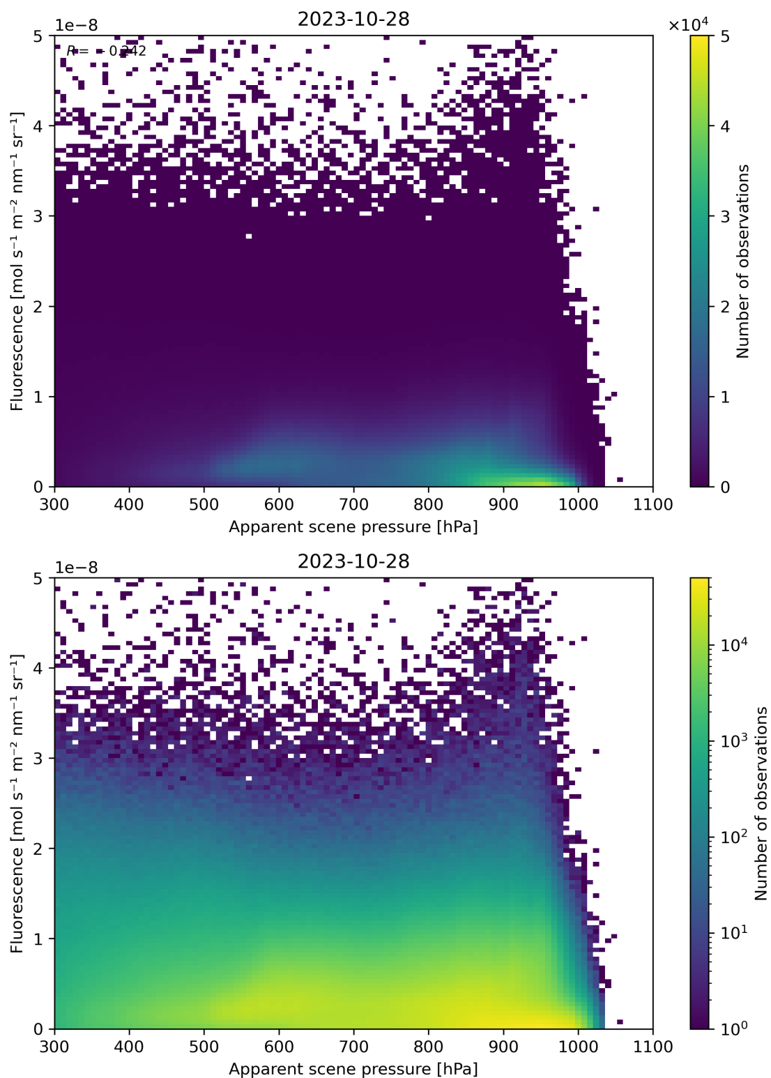
Figure 65: Scatter density plot of “Apparent scene pressure” against “Fluorescence” for 2023-10-28 to 2023-10-29.
