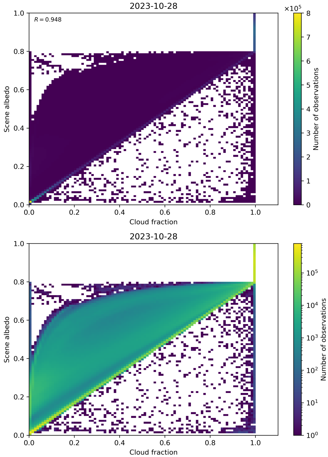
Figure 82: Scatter density plot of “Cloud fraction” against “Scene albedo” for 2023-10-28 to 2023-10-29.
