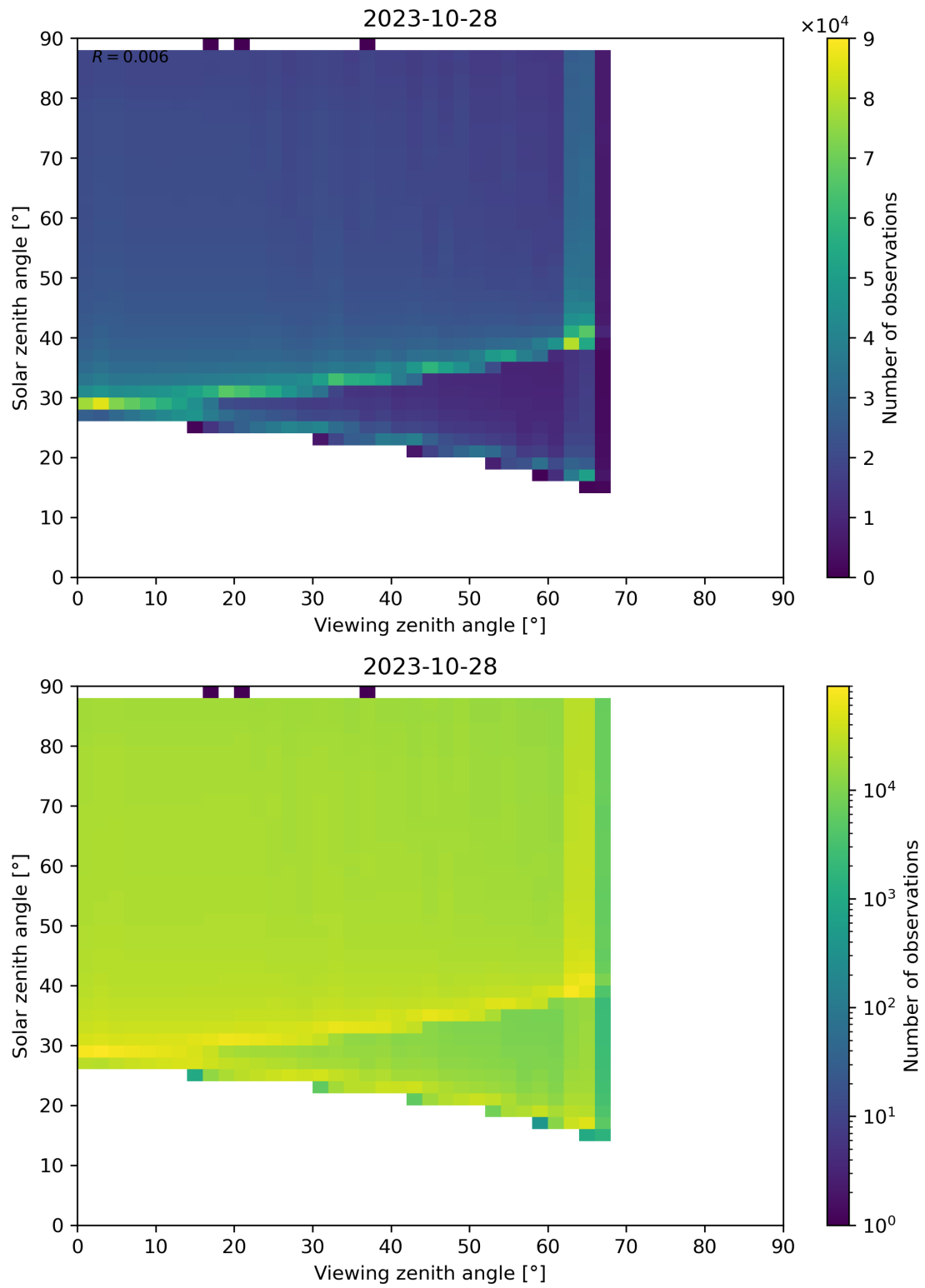
Figure 139: Scatter density plot of “Viewing zenith angle” against “Solar zenith angle” for 2023-10-28 to 2023-10-29.
