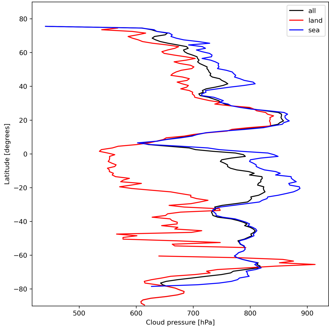
Figure 13: Zonal average of “Cloud pressure” for 2023-10-28 to 2023-10-29.
