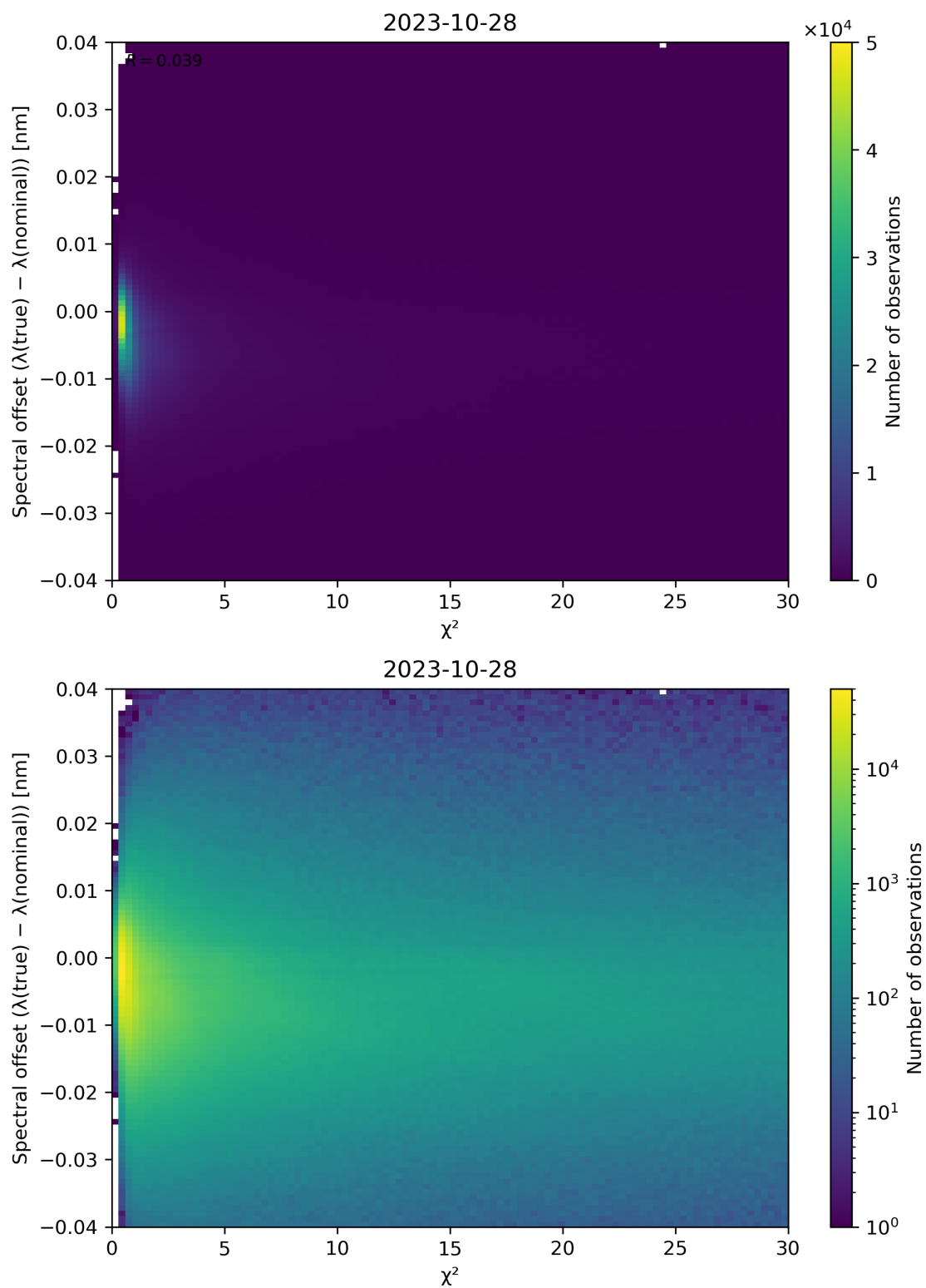
Figure 75: Scatter density plot of “ \chi^2 ” against “Spectral offset ( \lambda(\text{true}) - \lambda(\text{nominal}) )” for 2023-10-28 to 2023-10-29.
