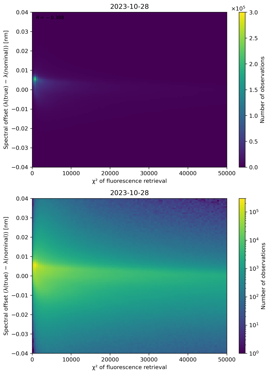
Figure 72: Scatter density plot of " \chi^2 of fluorescence retrieval" against "Spectral offset ( \lambda(\text{true}) - \lambda(\text{nominal})) " for 2023-10-28 to 2023-10-29.
