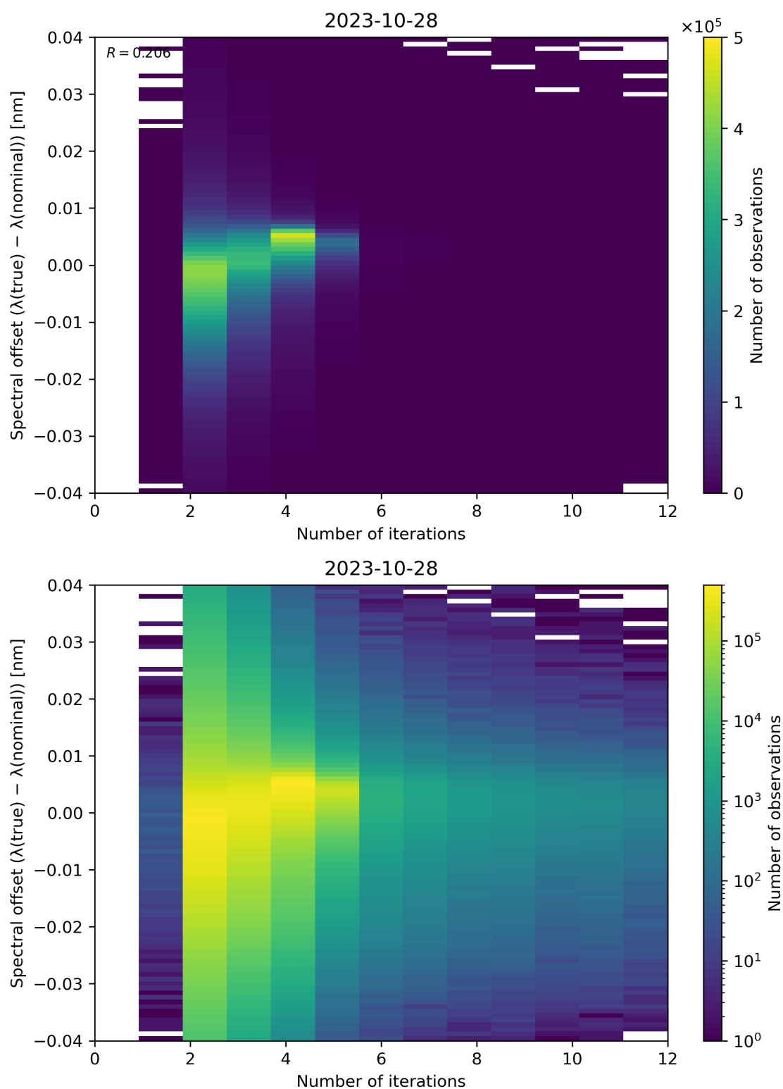
Figure 109: Scatter density plot of “Number of iterations” against “Spectral offset ( \lambda(\text{true}) - \lambda(\text{nominal}) )” for 2023-10-28 to 2023-10-29.
