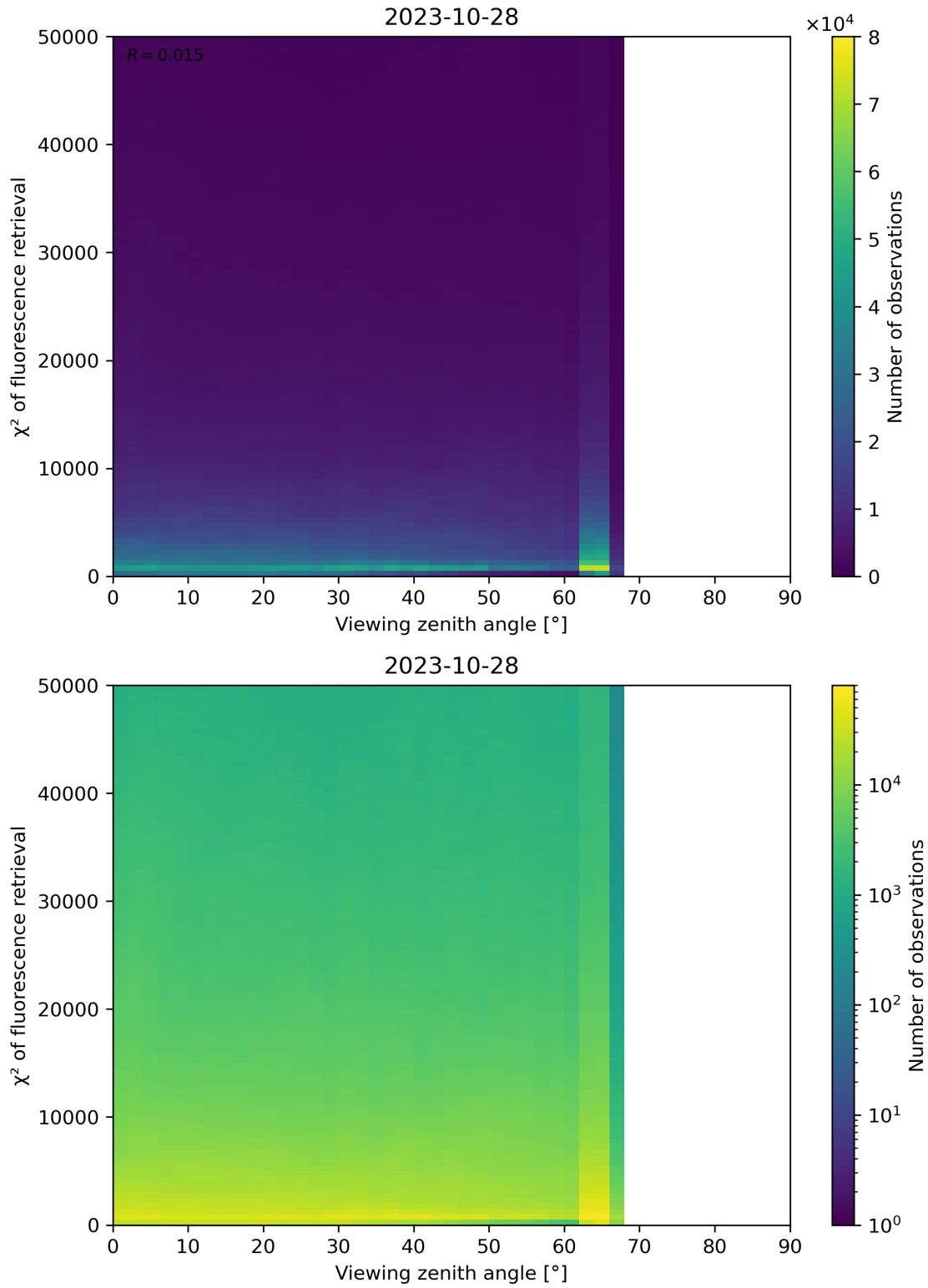
Figure 131: Scatter density plot of “Viewing zenith angle” against “ \chi^2 of fluorescence retrieval” for 2023-10-28 to 2023-10-29.
