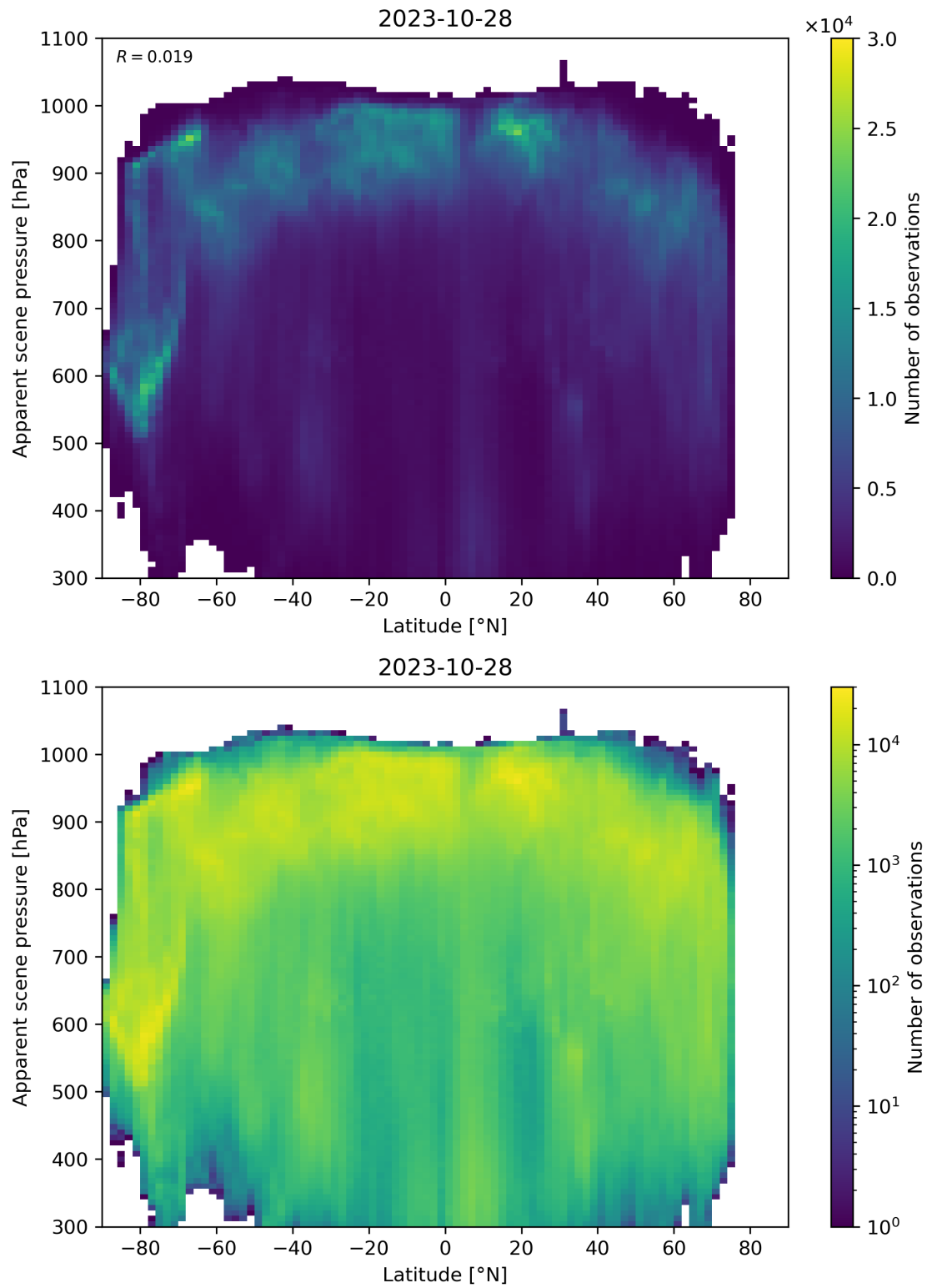
Figure 96: Scatter density plot of “Latitude” against “Apparent scene pressure” for 2023-10-28 to 2023-10-29.
