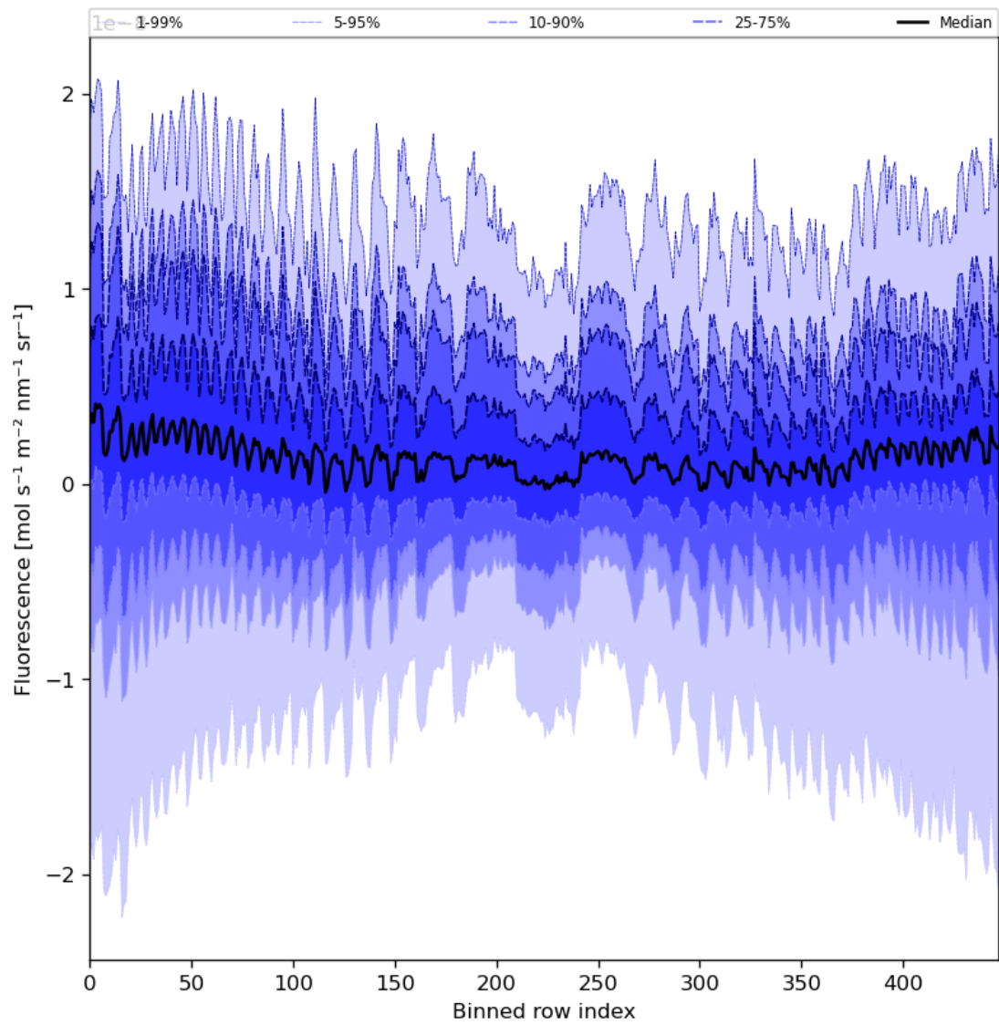
Figure 57: Along track statistics of “Fluorescence” for 2023-10-28 to 2023-10-29
