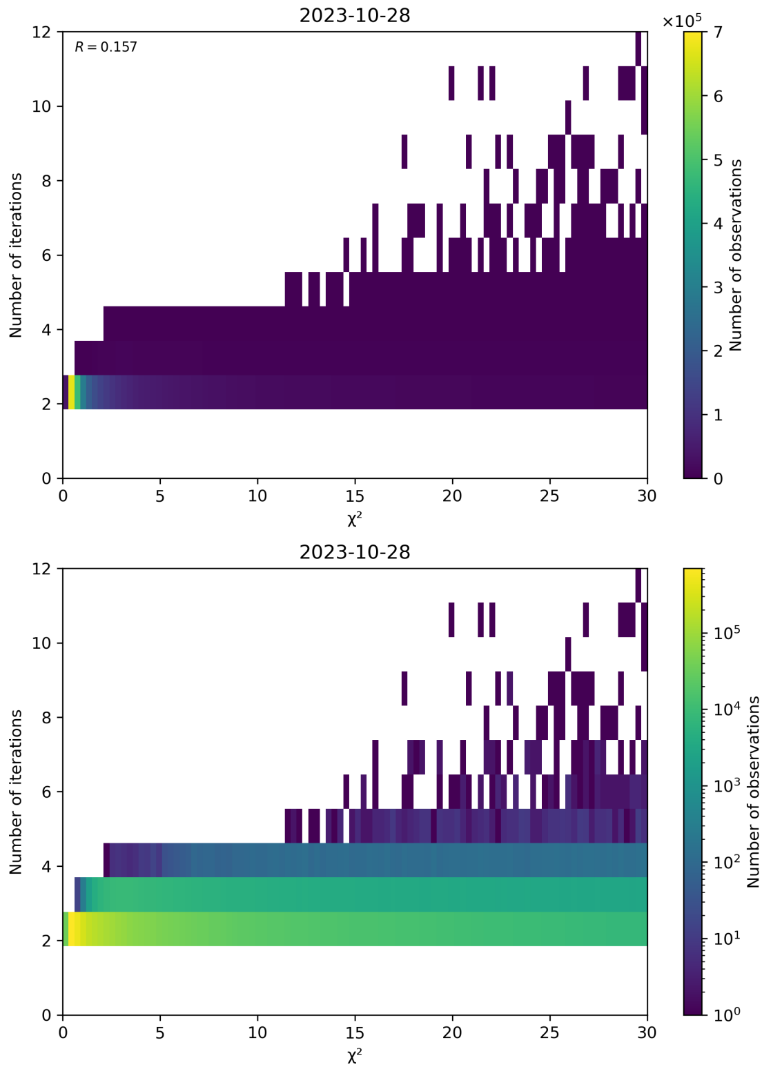
Figure 73: Scatter density plot of “ \chi^2 ” against “Number of iterations” for 2023-10-28 to 2023-10-29.
