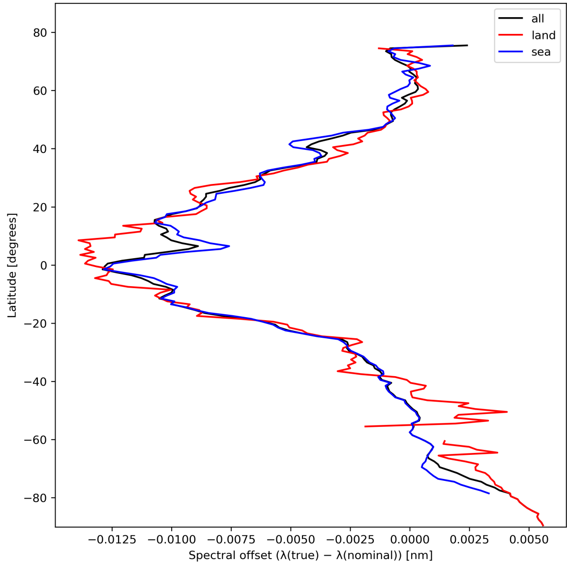
Figure 28: Zonal average of “Spectral offset ( \lambda(\text{true}) - \lambda(\text{nominal}) )” for 2023-10-28 to 2023-10-29.
