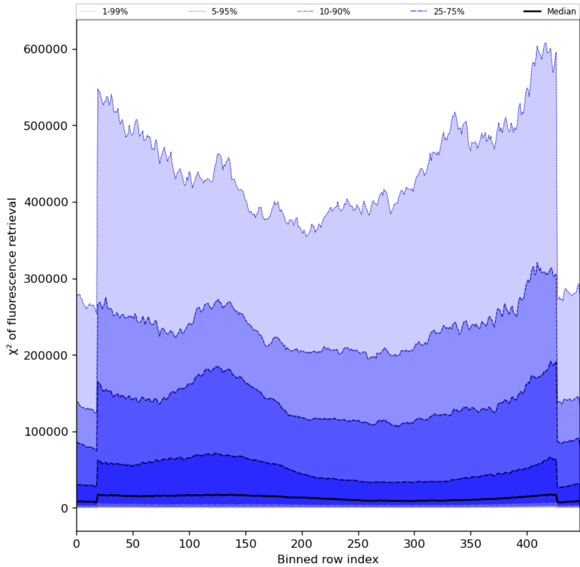
Figure 59: Along track statistics of “ \chi^2 of fluorescence retrieval” for 2023-10-28 to 2023-10-29
