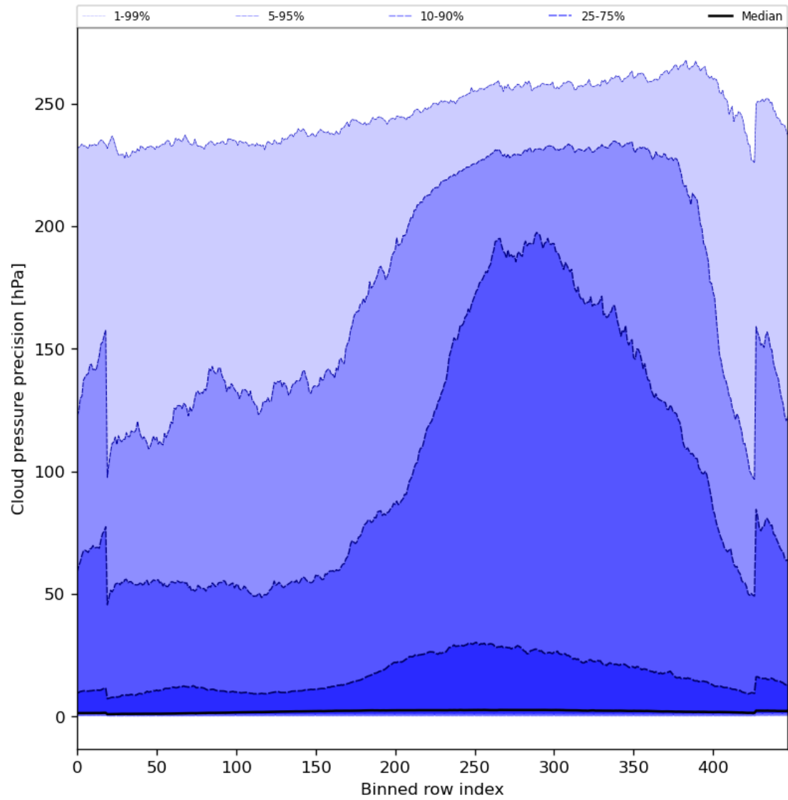
Figure 48: Along track statistics of “Cloud pressure precision” for 2023-10-28 to 2023-10-29
