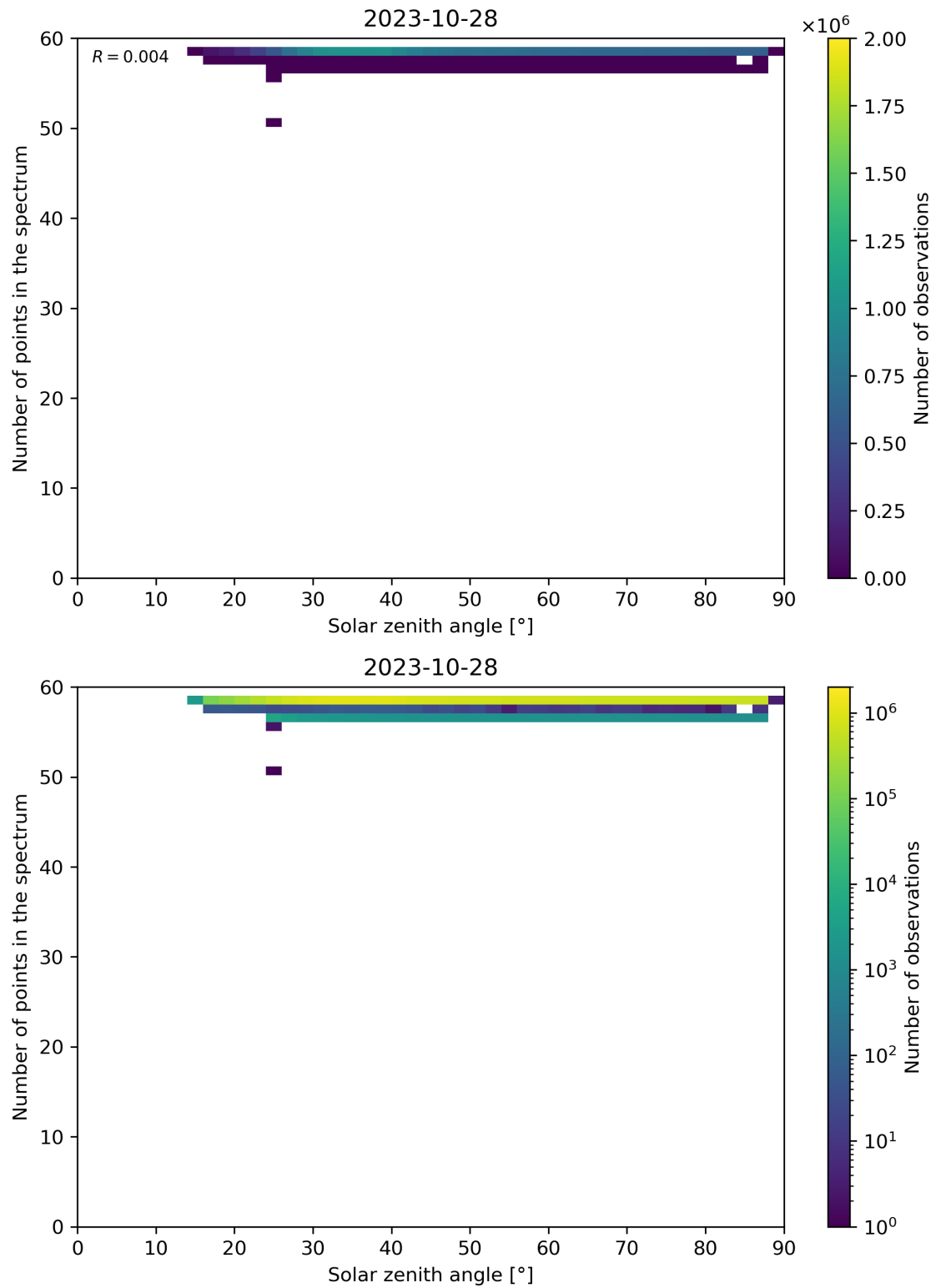
Figure 126: Scatter density plot of “Solar zenith angle” against “Number of points in the spectrum” for 2023-10-28 to 2023-10-29.
