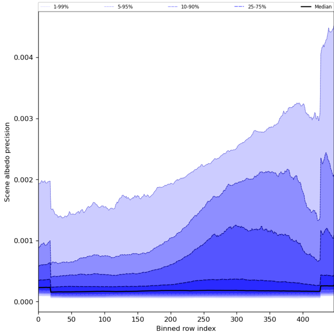
Figure 52: Along track statistics of “Scene albedo precision” for 2023-10-28 to 2023-10-29
