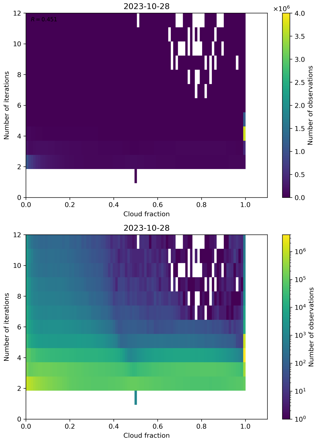
Figure 80: Scatter density plot of “Cloud fraction” against “Number of iterations” for 2023-10-28 to 2023-10-29.
