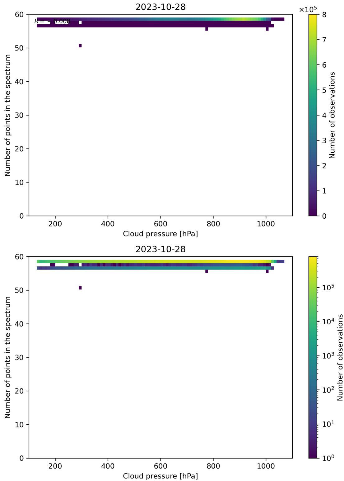
Figure 90: Scatter density plot of “Cloud pressure” against “Number of points in the spectrum” for 2023-10-28 to 2023-10-29.
