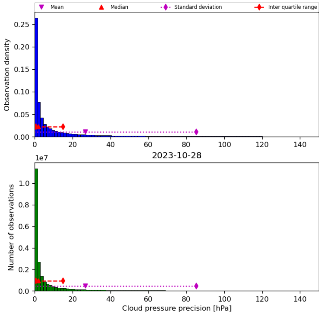
Figure 31: Histogram of “Cloud pressure precision” for 2023-10-28 to 2023-10-29
