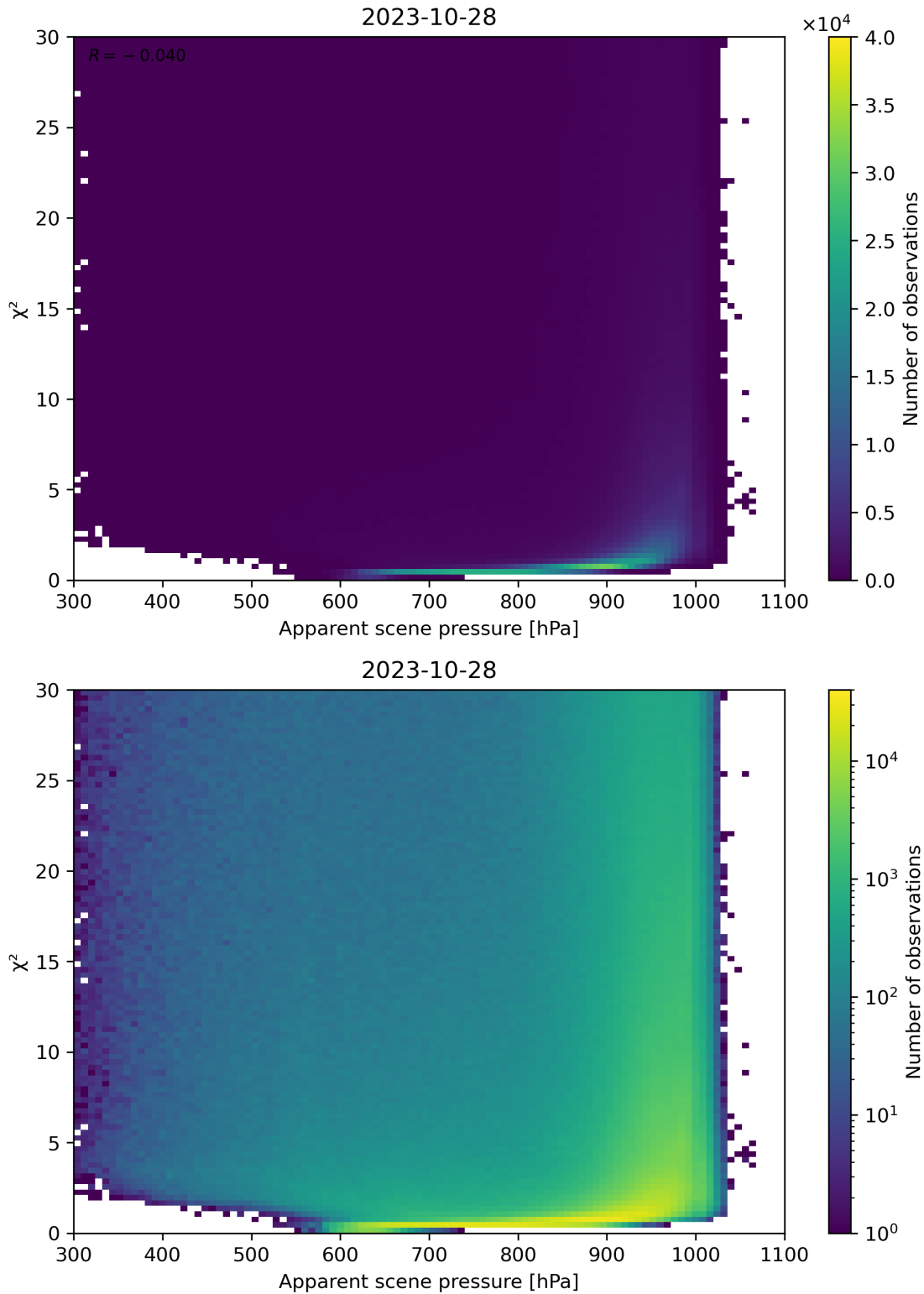
Figure 63: Scatter density plot of “Apparent scene pressure” against “ \chi^2 ” for 2023-10-28 to 2023-10-29.
