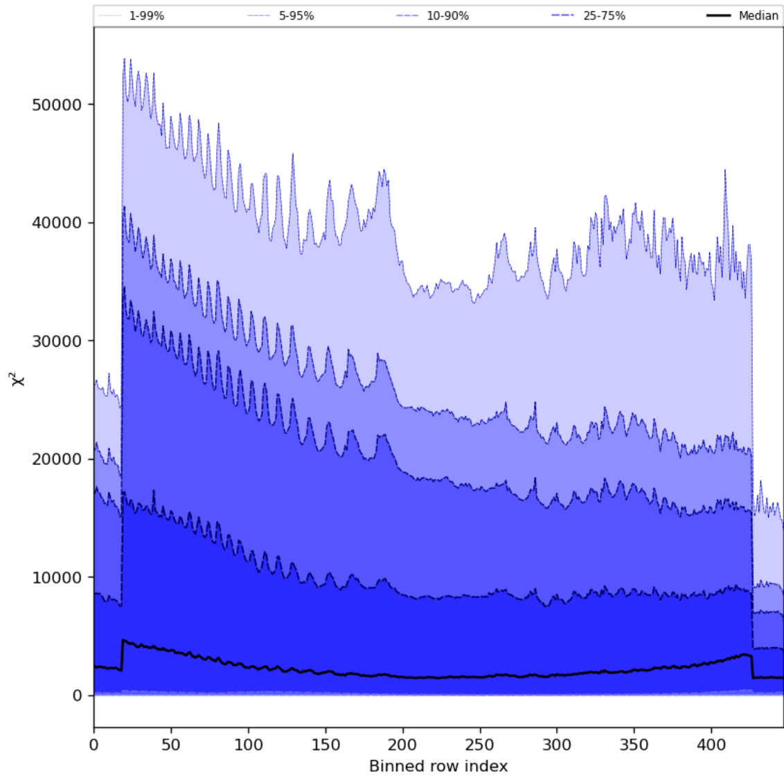
Figure 55: Along track statistics of " \chi^2 " for 2023-10-28 to 2023-10-29
