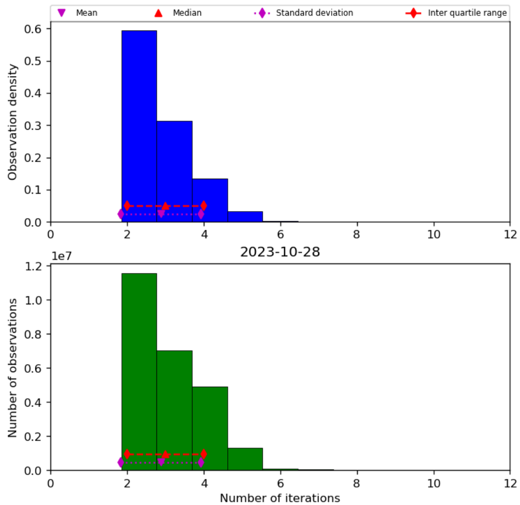
Figure 39: Histogram of “Number of iterations” for 2023-10-28 to 2023-10-29
