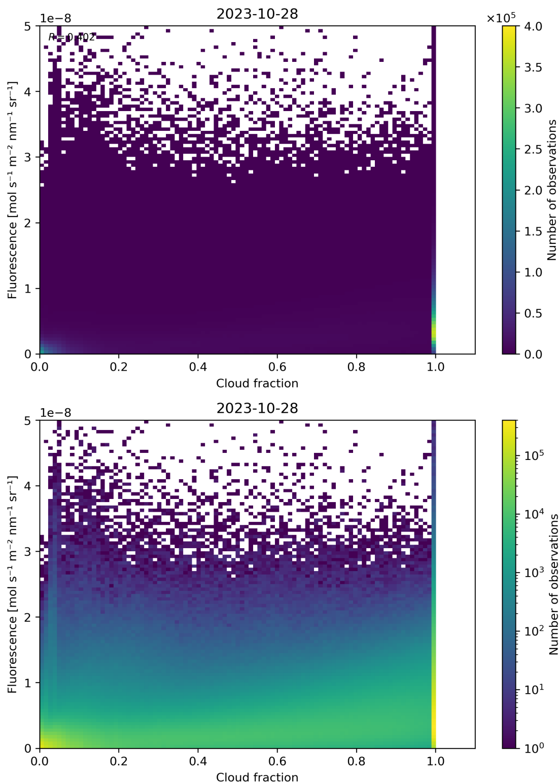
Figure 79: Scatter density plot of “Cloud fraction” against “Fluorescence” for 2023-10-28 to 2023-10-29.
