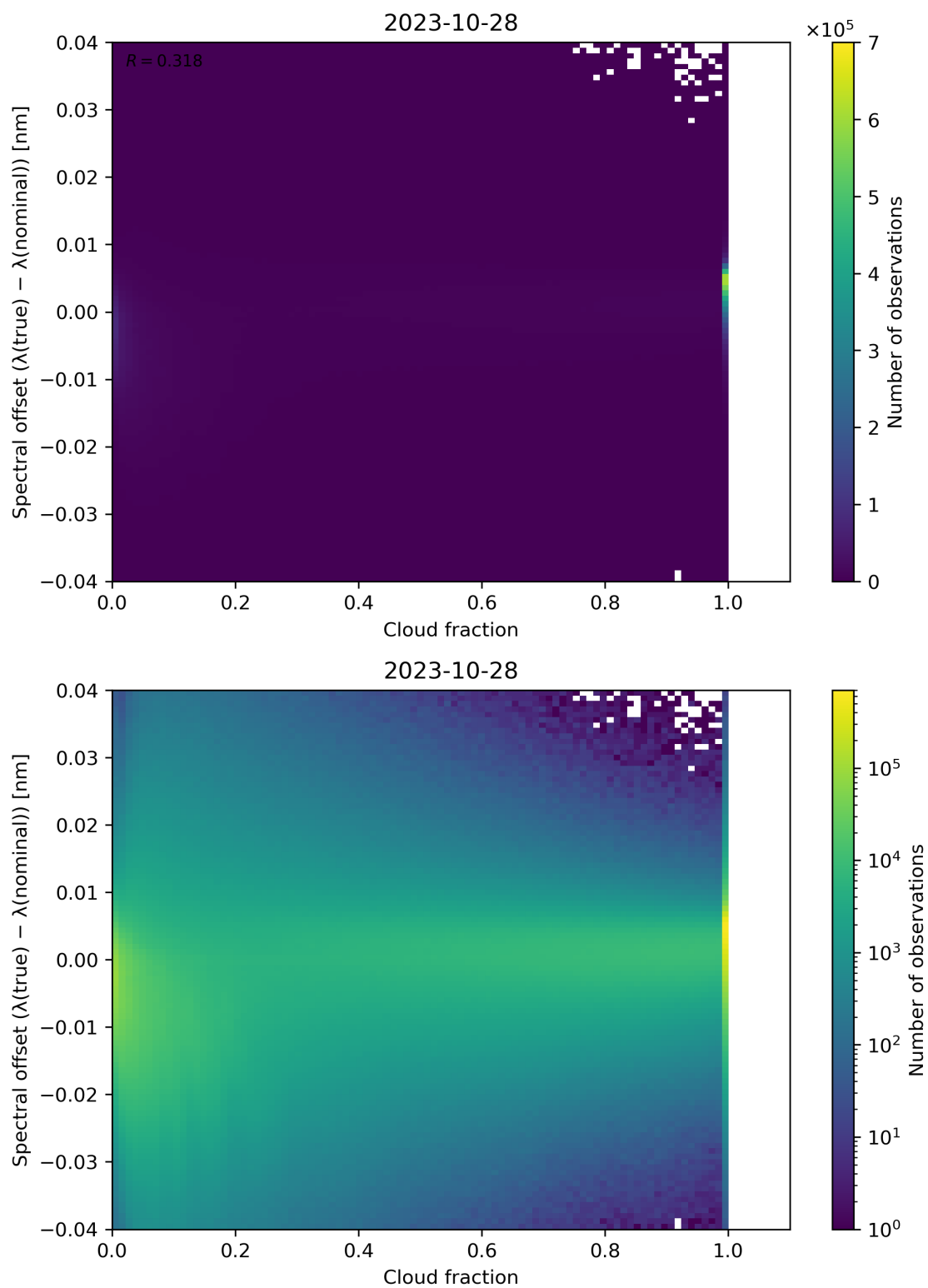
Figure 83: Scatter density plot of “Cloud fraction” against “Spectral offset ( \lambda(\text{true}) - \lambda(\text{nominal}) )” for 2023-10-28 to 2023-10-29.
