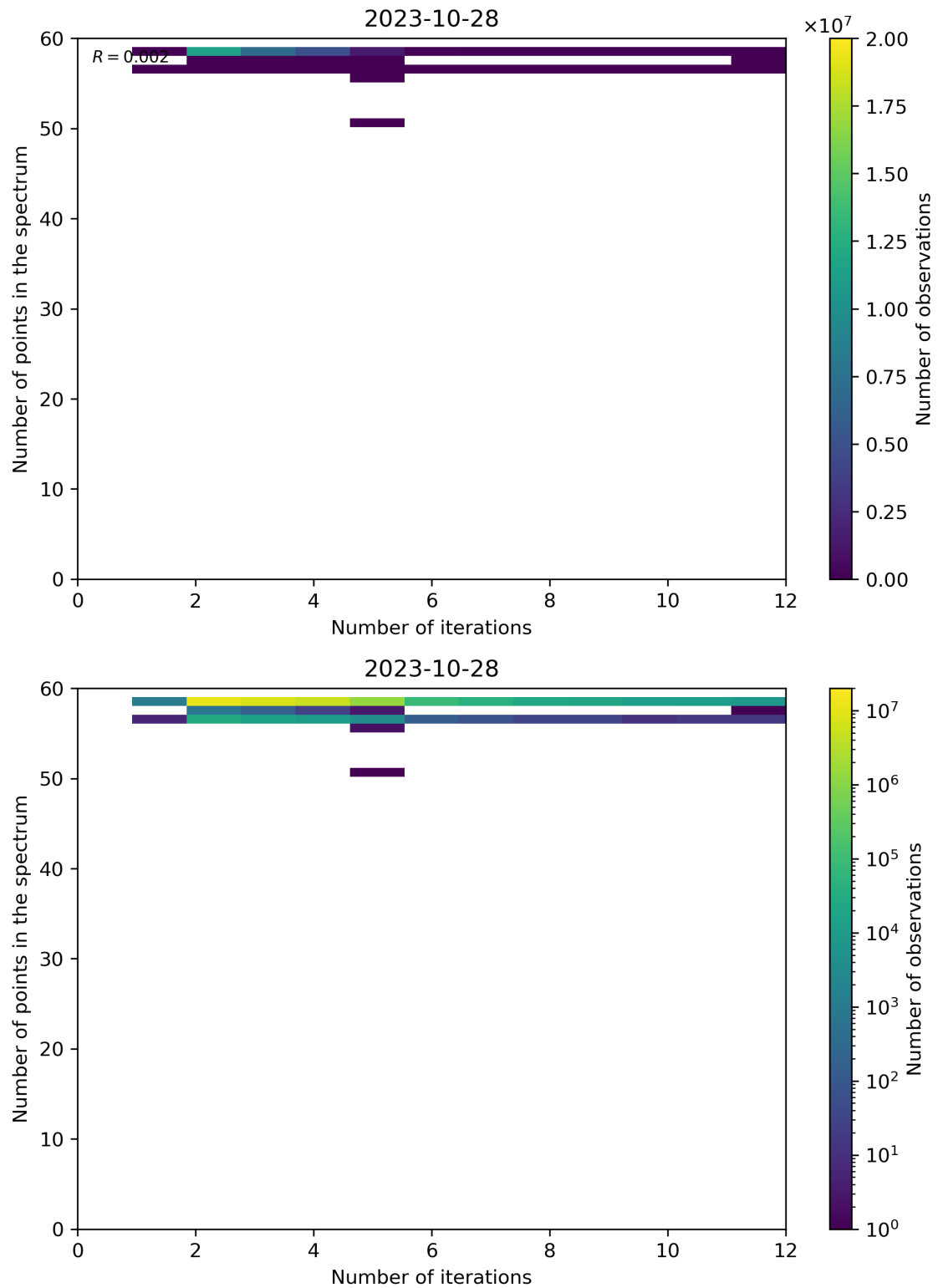
Figure 108: Scatter density plot of “Number of iterations” against “Number of points in the spectrum” for 2023-10-28 to 2023-10-29.
