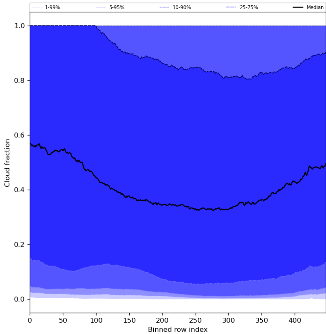
Figure 49: Along track statistics of “Cloud fraction” for 2023-10-28 to 2023-10-29
