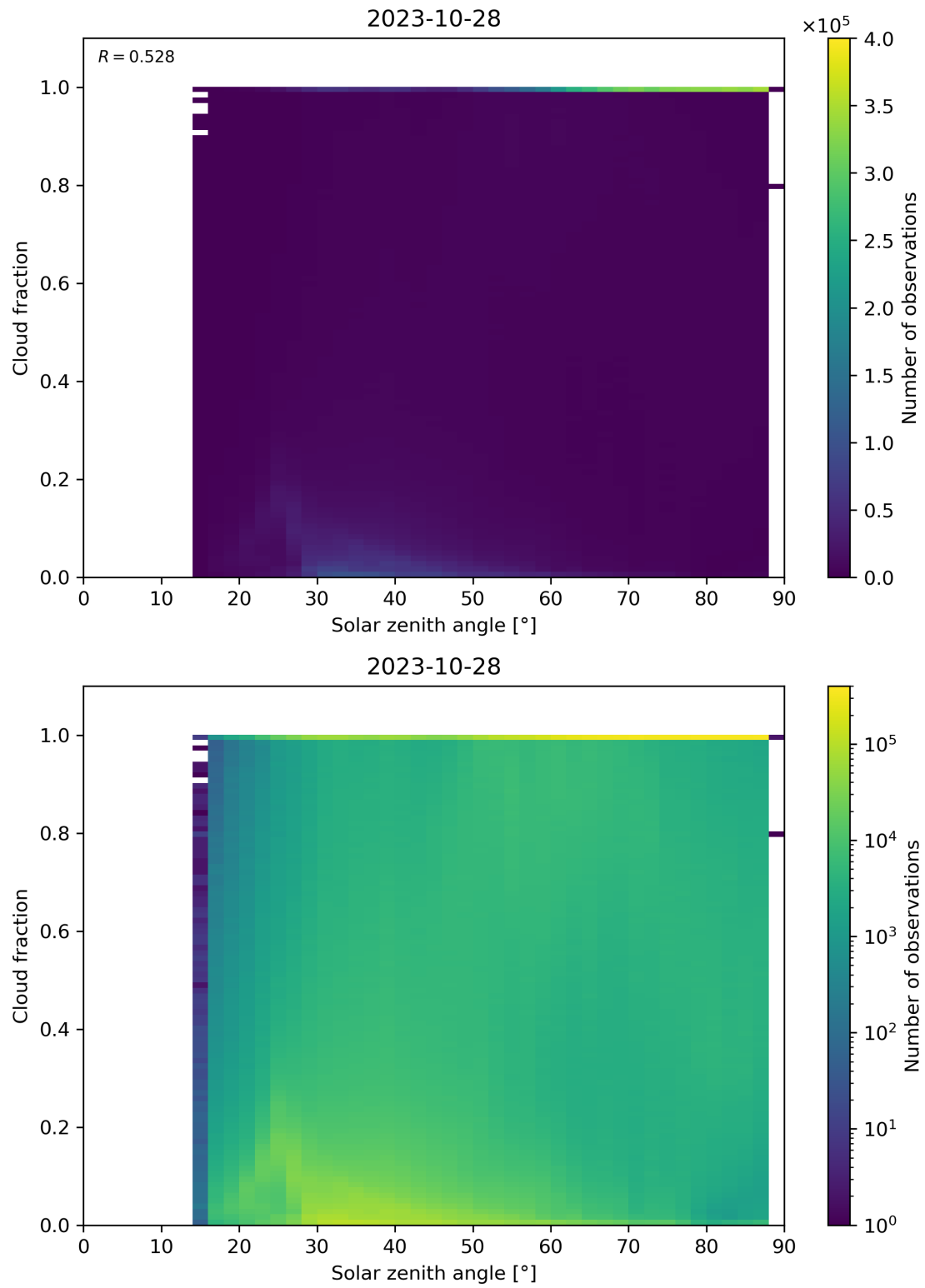
Figure 121: Scatter density plot of “Solar zenith angle” against “Cloud fraction” for 2023-10-28 to 2023-10-29.
