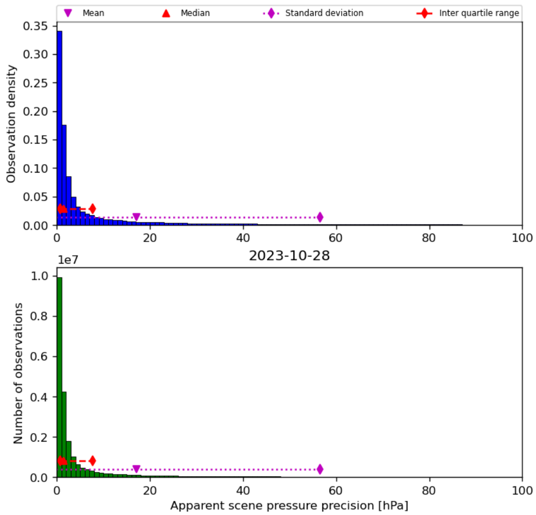
Figure 37: Histogram of “Apparent scene pressure precision” for 2023-10-28 to 2023-10-29
