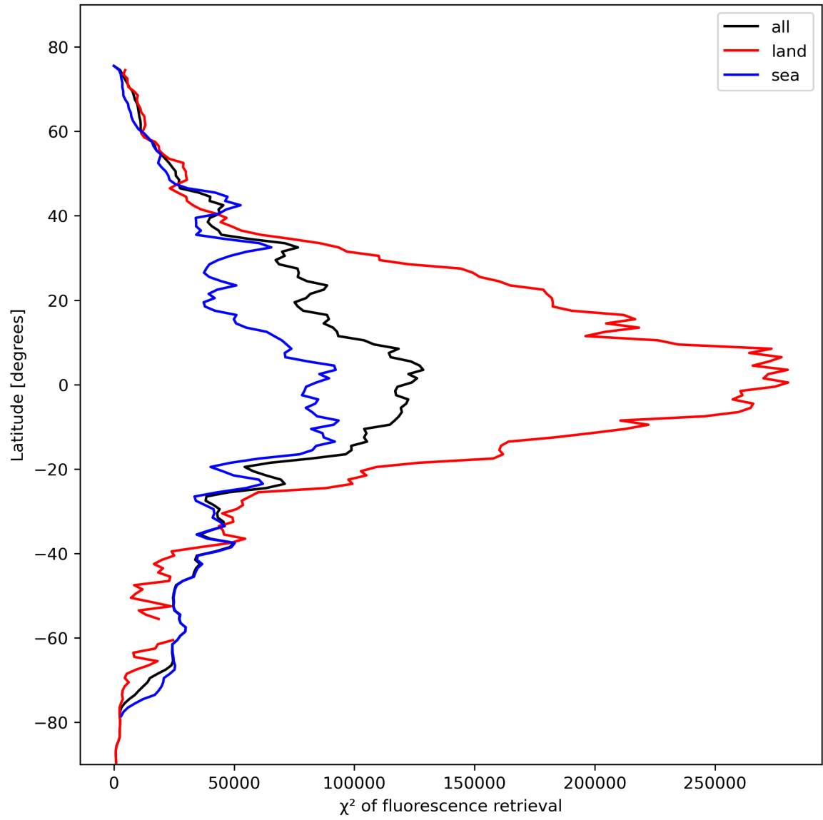
Figure 25: Zonal average of “ \chi^2 of fluorescence retrieval” for 2023-10-28 to 2023-10-29.
