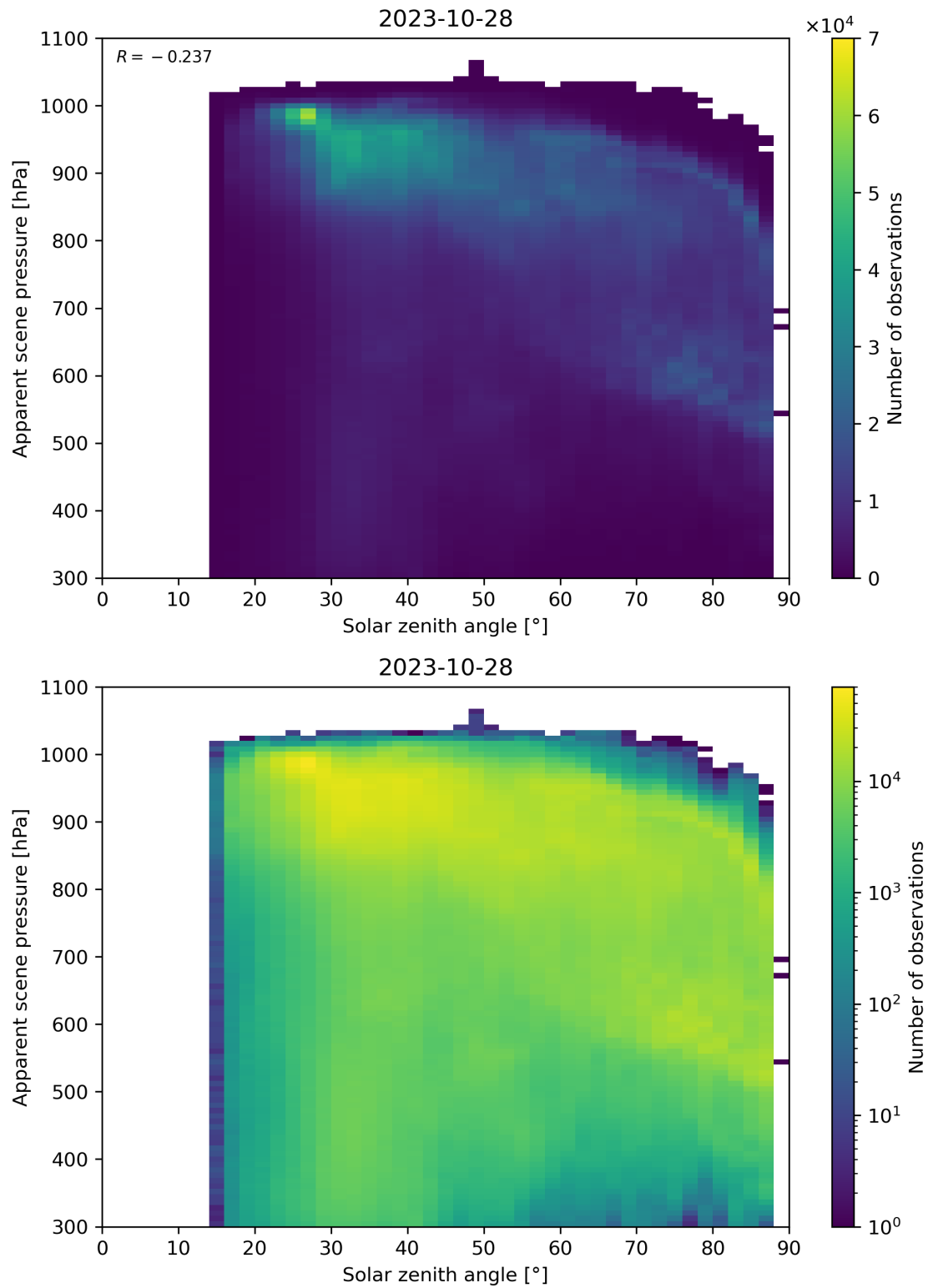
Figure 118: Scatter density plot of “Solar zenith angle” against “Apparent scene pressure” for 2023-10-28 to 2023-10-29.
