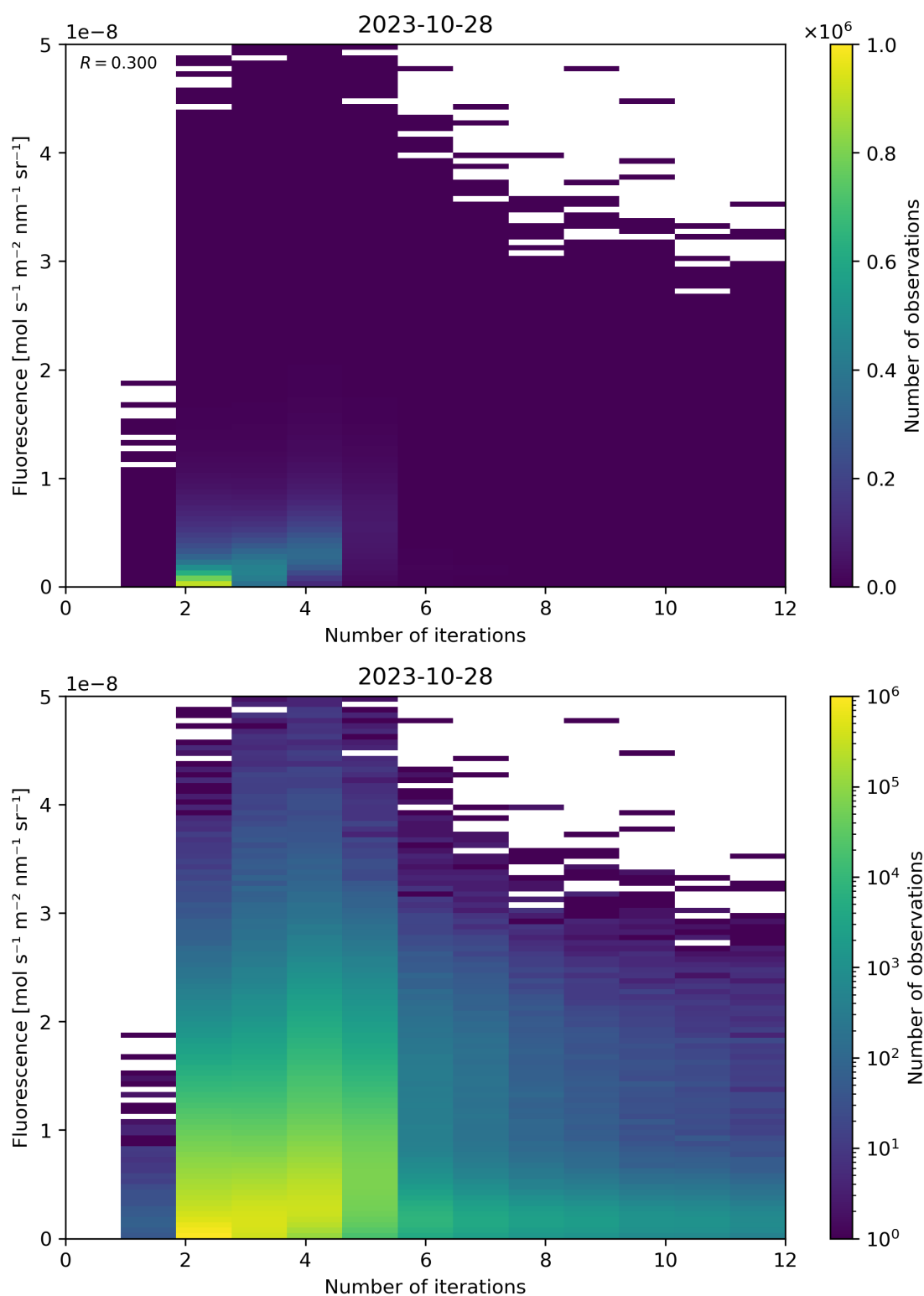
Figure 107: Scatter density plot of “Number of iterations” against “Fluorescence” for 2023-10-28 to 2023-10-29.
