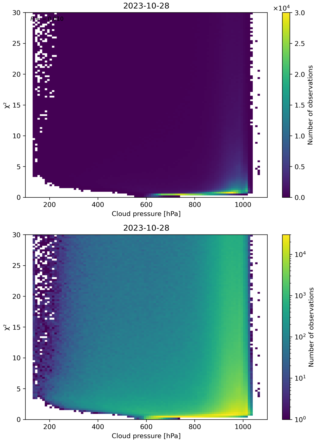
Figure 85: Scatter density plot of “Cloud pressure” against “ \chi^2 ” for 2023-10-28 to 2023-10-29.
