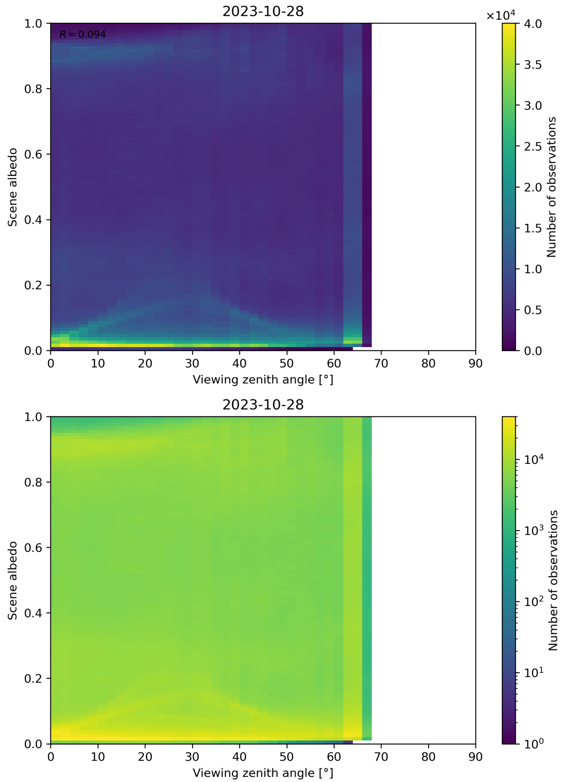
Figure 138: Scatter density plot of “Viewing zenith angle” against “Scene albedo” for 2023-10-28 to 2023-10-29.
