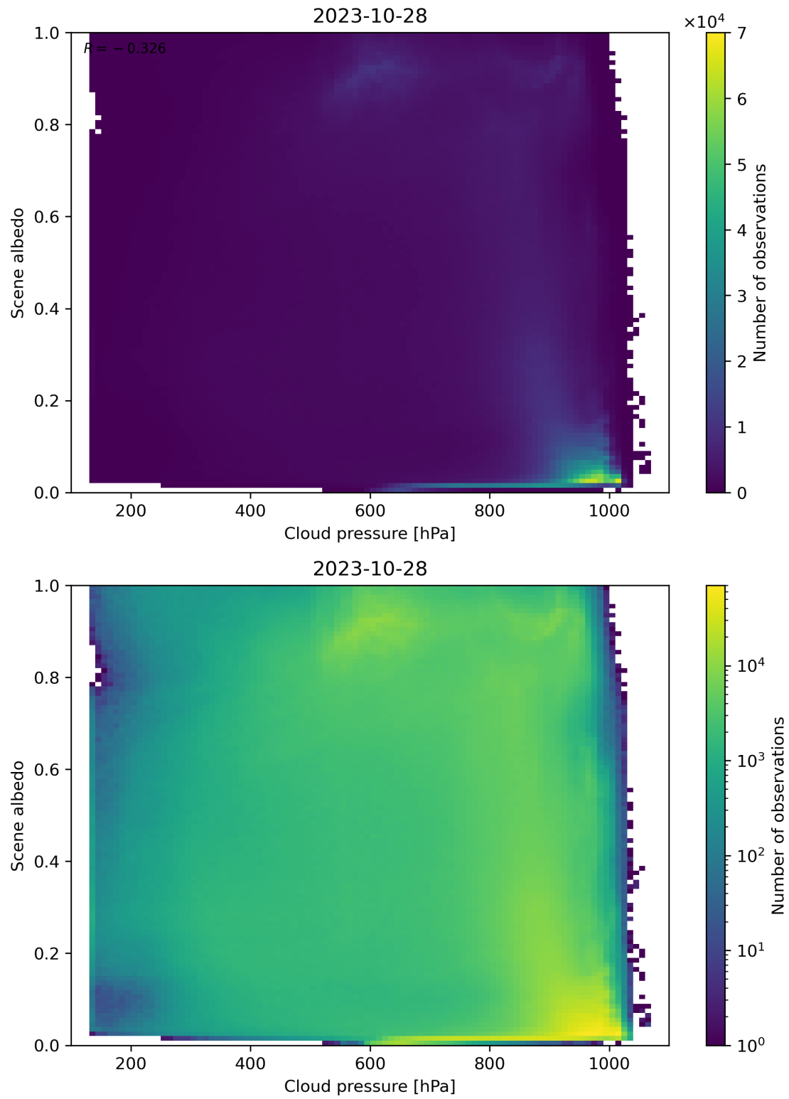
Figure 91: Scatter density plot of “Cloud pressure” against “Scene albedo” for 2023-10-28 to 2023-10-29.
