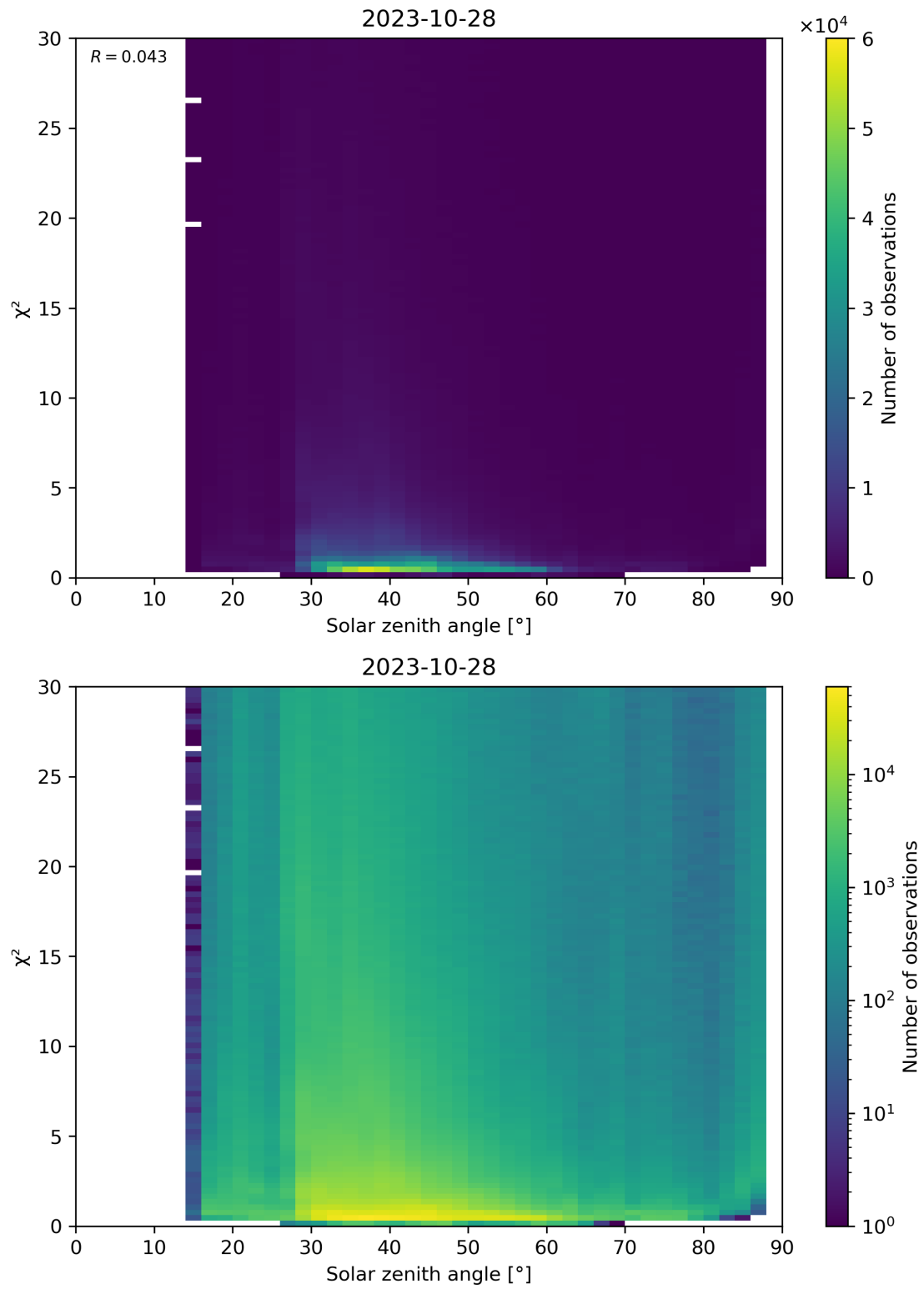
Figure 119: Scatter density plot of “Solar zenith angle” against “ \chi^2 ” for 2023-10-28 to 2023-10-29.
