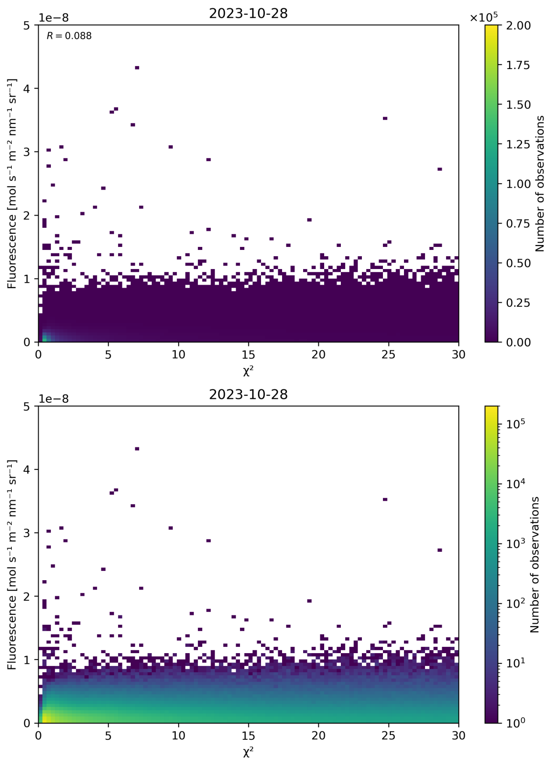
Figure 70: Scatter density plot of “ \chi^2 ” against “Fluorescence” for 2023-10-28 to 2023-10-29.
