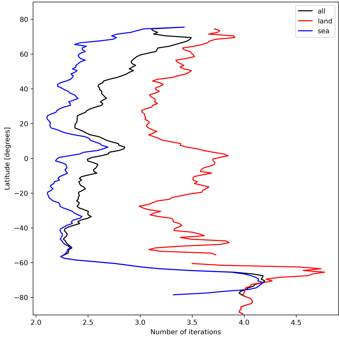
Figure 22: Zonal average of “Number of iterations” for 2023-10-28 to 2023-10-29.
