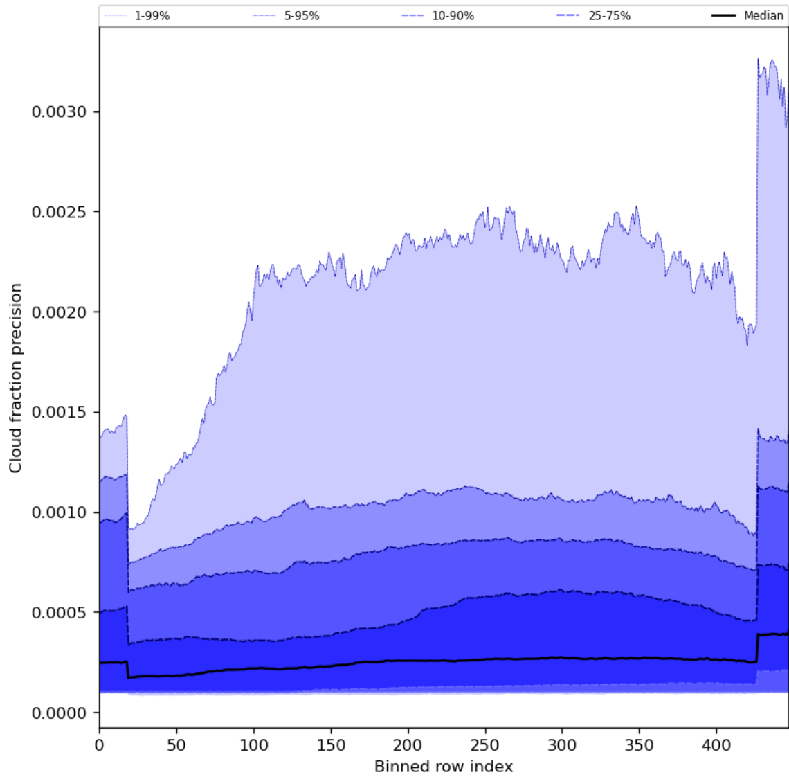
Figure 50: Along track statistics of “Cloud fraction precision” for 2023-10-28 to 2023-10-29
