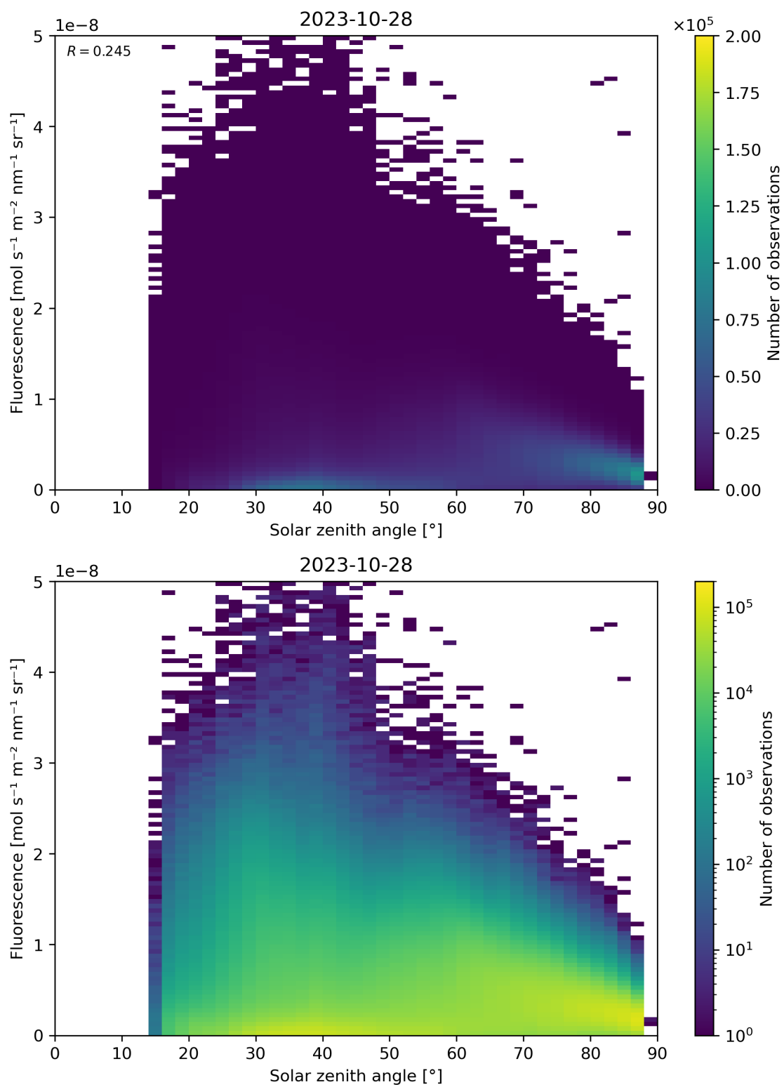
Figure 123: Scatter density plot of “Solar zenith angle” against “Fluorescence” for 2023-10-28 to 2023-10-29.
