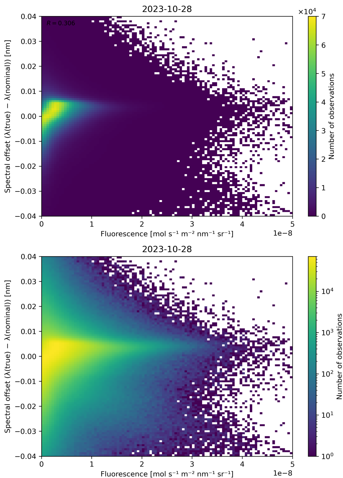
Figure 95: Scatter density plot of “Fluorescence” against “Spectral offset ( \lambda(\text{true}) - \lambda(\text{nominal}) )” for 2023-10-28 to 2023-10-29.
