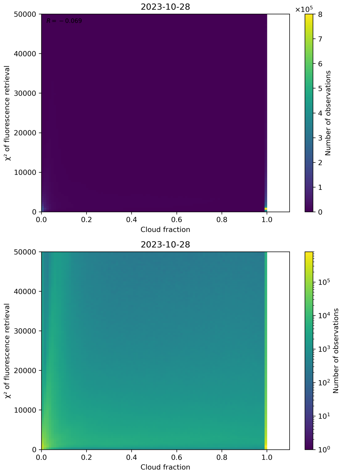
Figure 78: Scatter density plot of “Cloud fraction” against “ \chi^2 of fluorescence retrieval” for 2023-10-28 to 2023-10-29.
