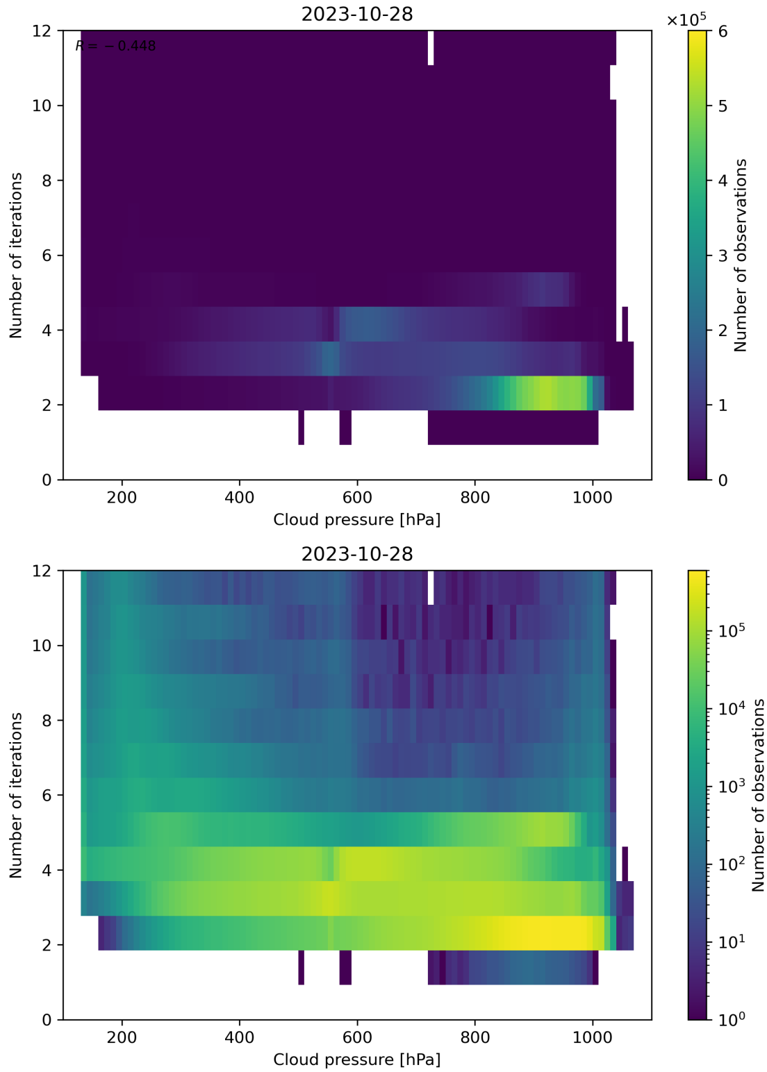
Figure 89: Scatter density plot of “Cloud pressure” against “Number of iterations” for 2023-10-28 to 2023-10-29.
