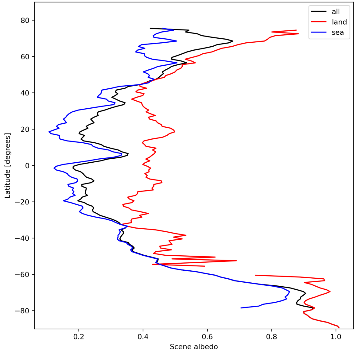
Figure 17: Zonal average of “Scene albedo” for 2023-10-28 to 2023-10-29.
