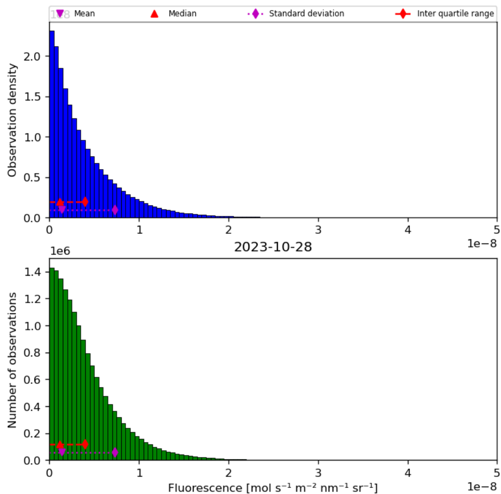
Figure 40: Histogram of “Fluorescence” for 2023-10-28 to 2023-10-29
