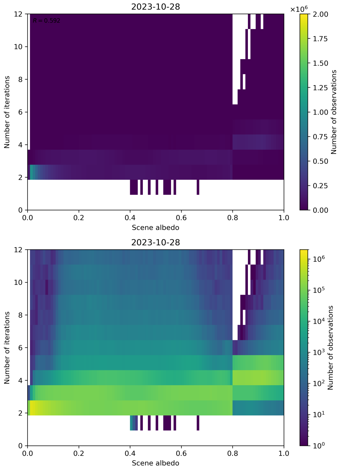
Figure 115: Scatter density plot of “Scene albedo” against “Number of iterations” for 2023-10-28 to 2023-10-29.
