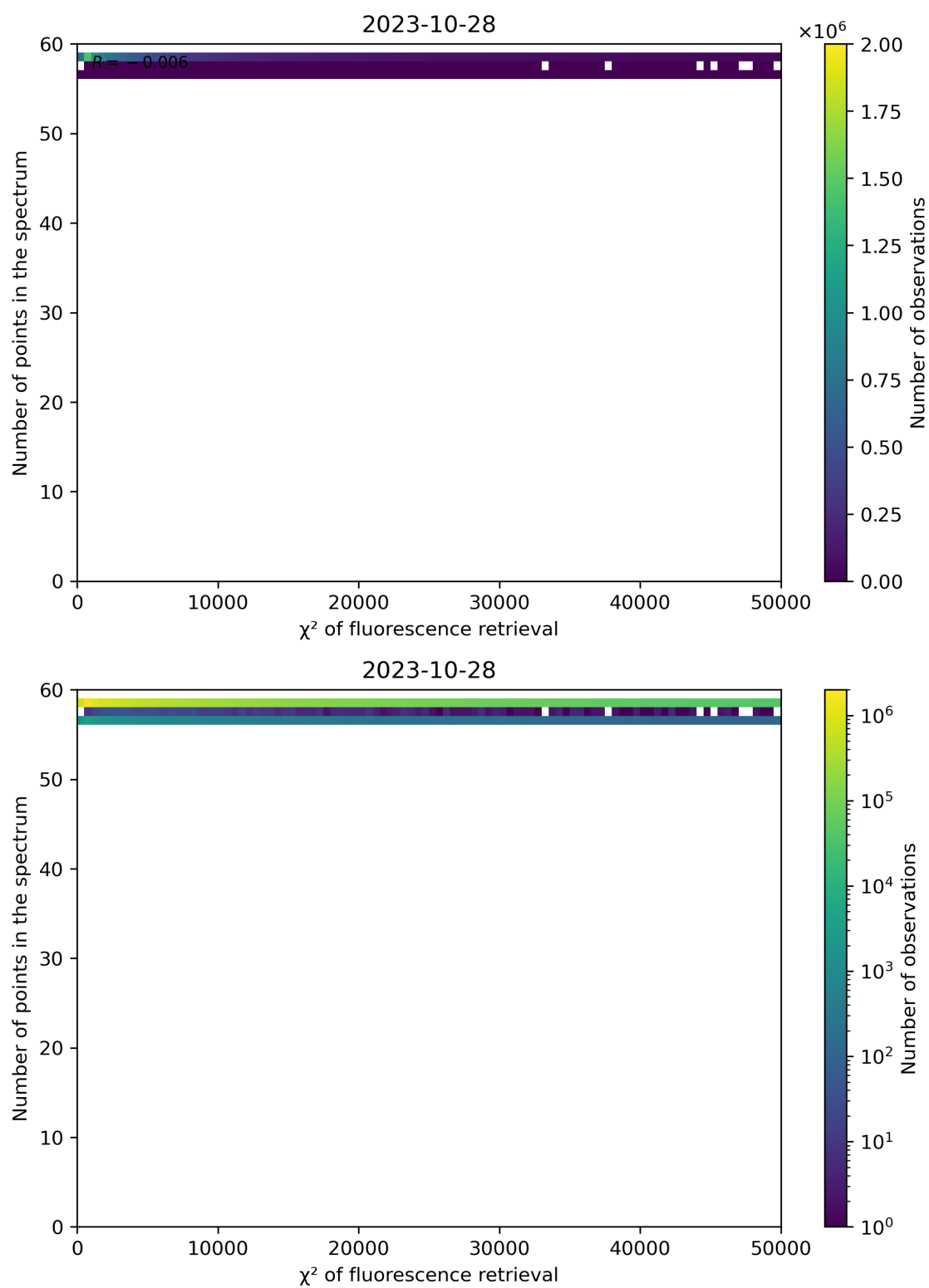
Figure 71: Scatter density plot of " \chi^2 of fluorescence retrieval" against "Number of points in the spectrum" for 2023-10-28 to 2023-10-29.
