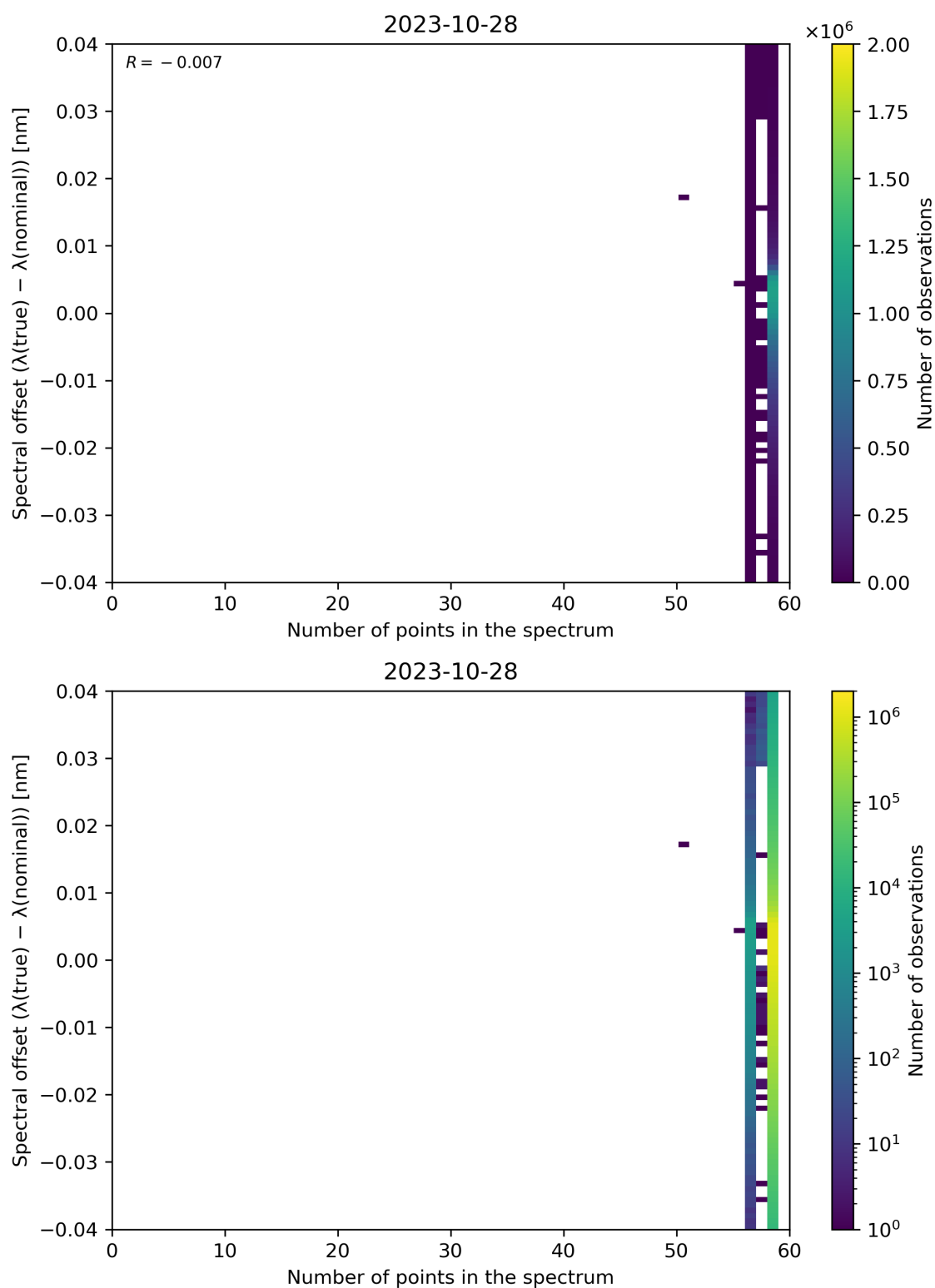
Figure 110: Scatter density plot of “Number of points in the spectrum” against “Spectral offset ( \lambda(\text{true}) - \lambda(\text{nominal}) )” for 2023-10-28 to 2023-10-29.
