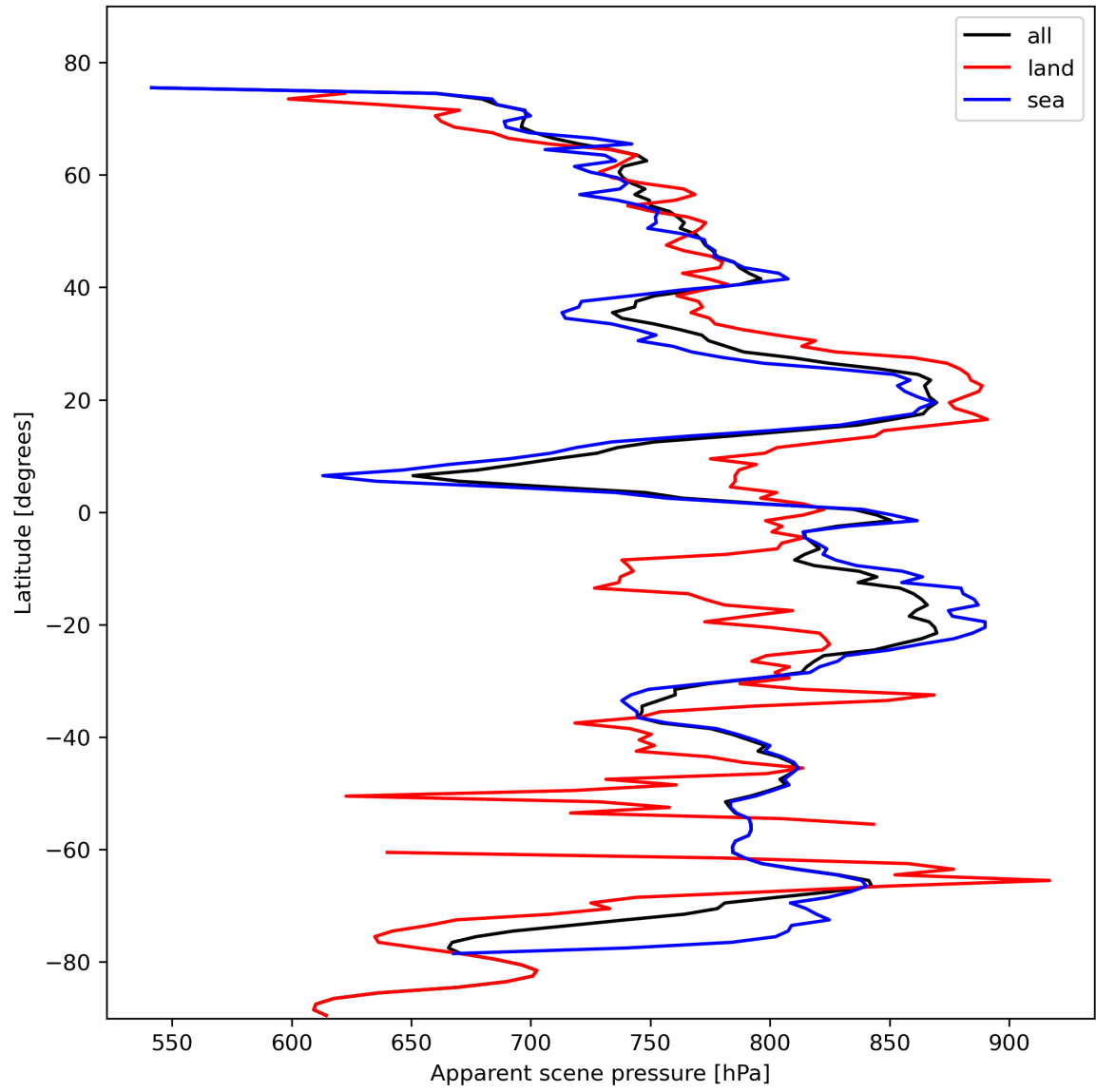
Figure 19: Zonal average of “Apparent scene pressure” for 2023-10-28 to 2023-10-29.
