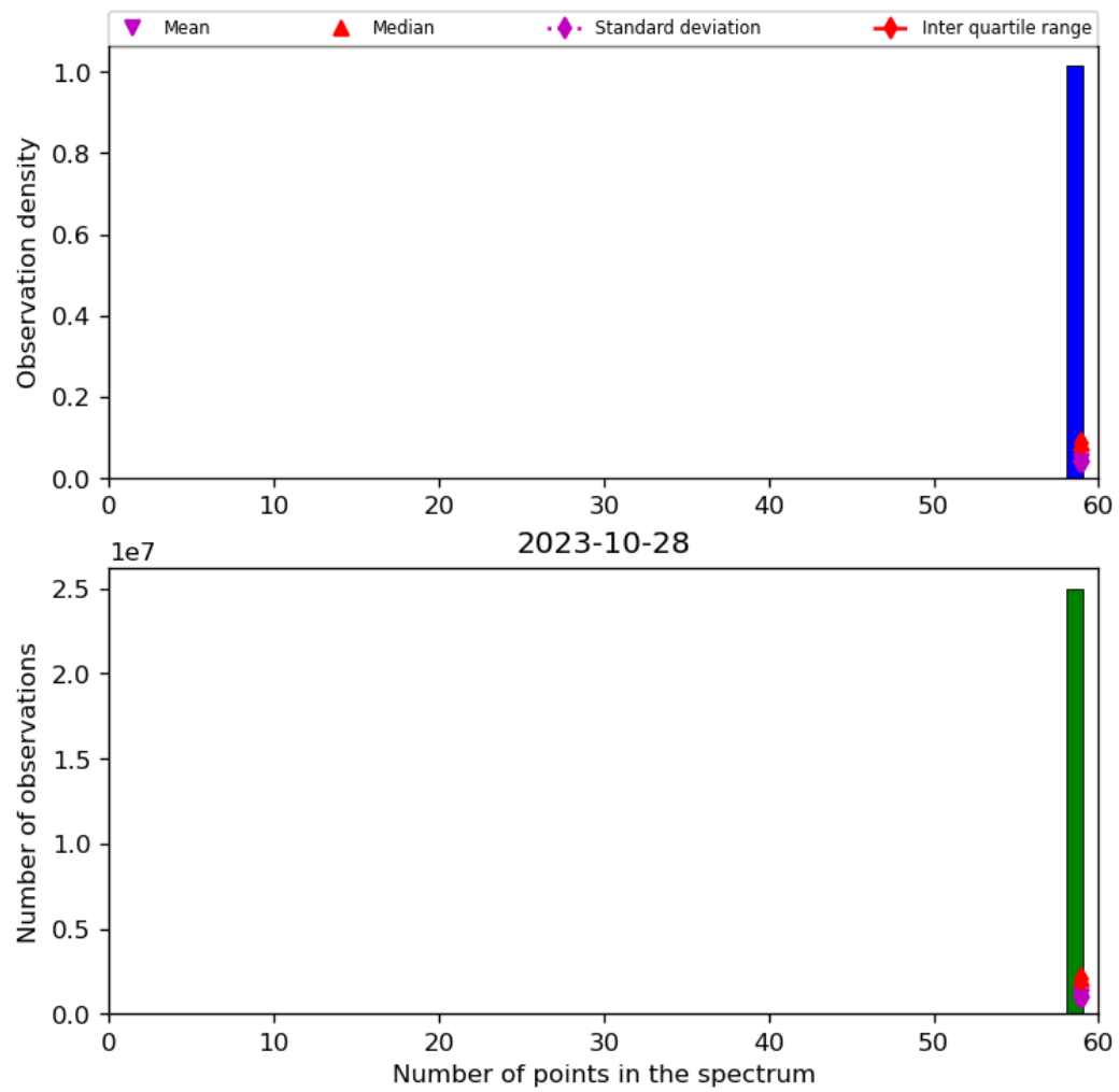
Figure 44: Histogram of “Number of points in the spectrum” for 2023-10-28 to 2023-10-29
