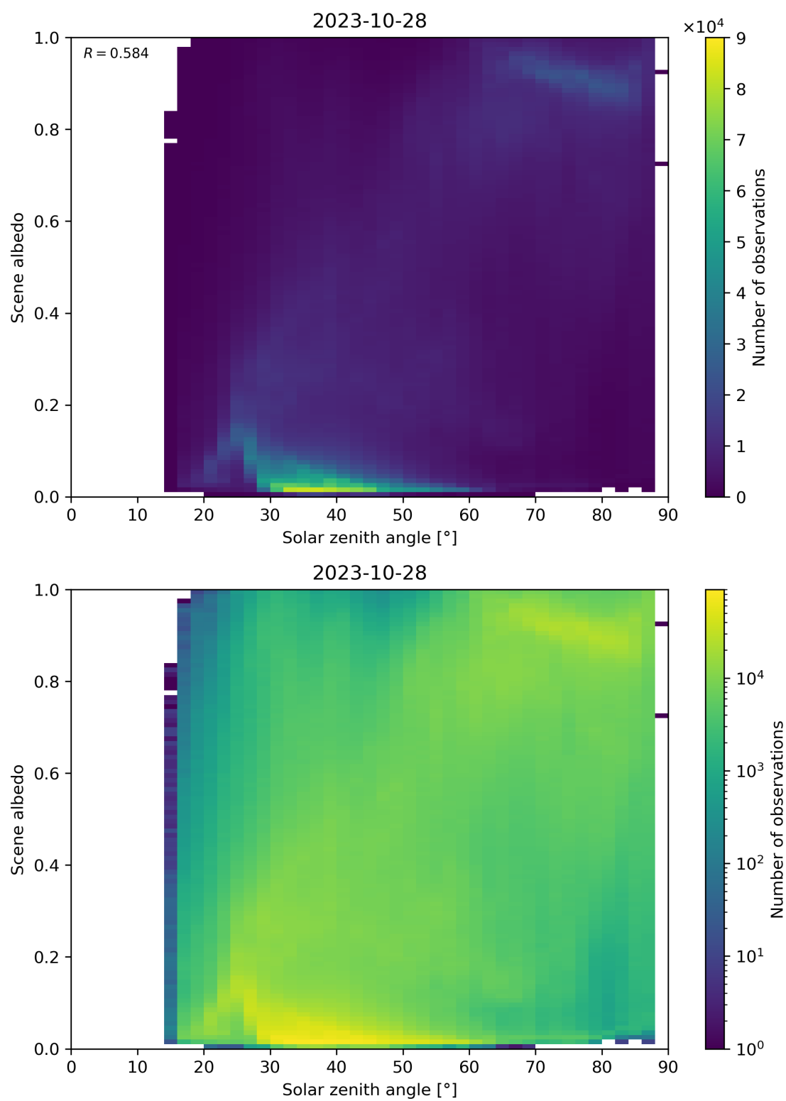
Figure 127: Scatter density plot of “Solar zenith angle” against “Scene albedo” for 2023-10-28 to 2023-10-29.
