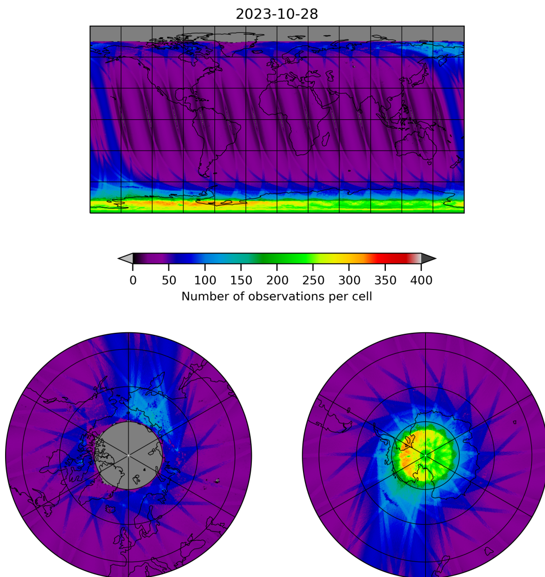
Figure 11: Map of the number of observations for 2023-10-28 to 2023-10-29
