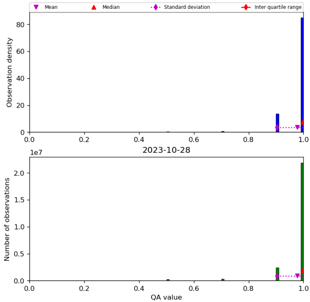
Figure 29: Histogram of “QA value” for 2023-10-28 to 2023-10-29
