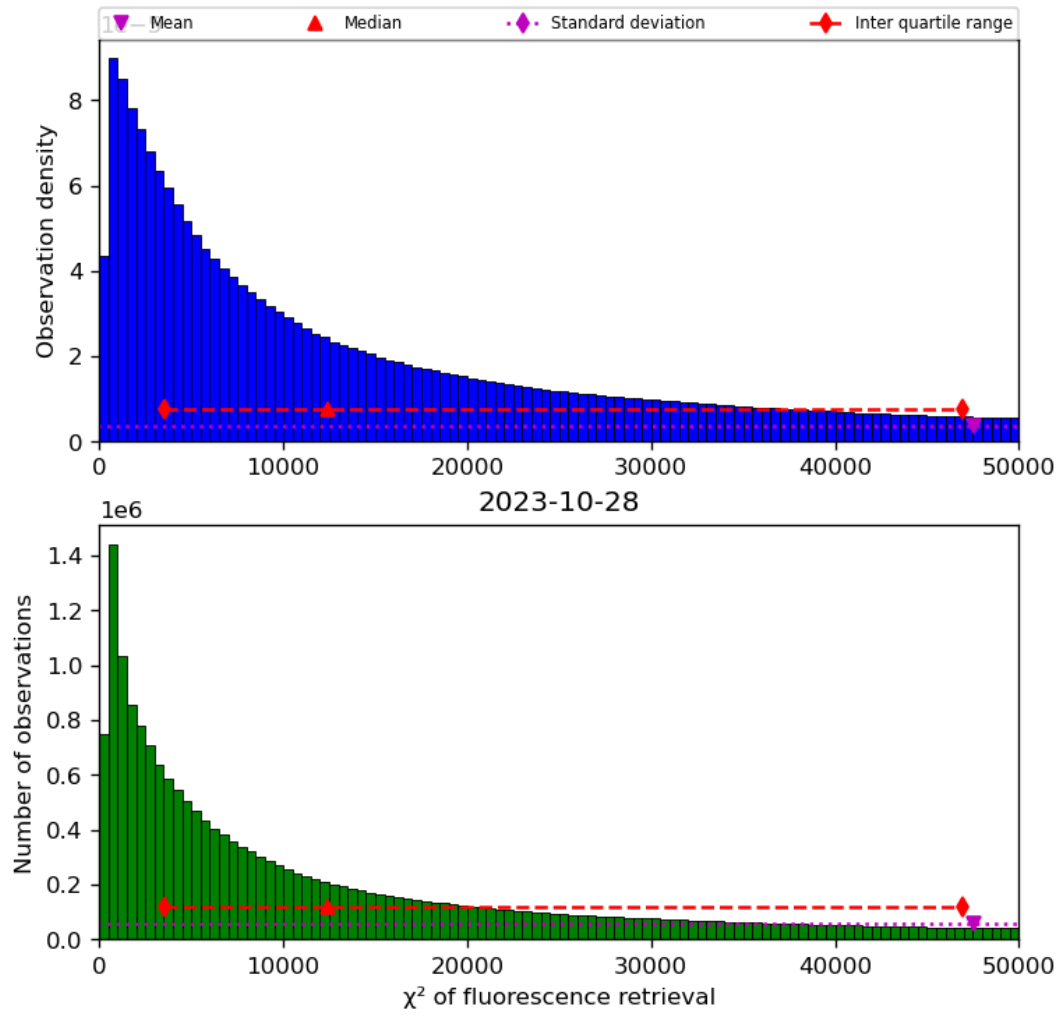
Figure 42: Histogram of “ \chi^2 of fluorescence retrieval” for 2023-10-28 to 2023-10-29
