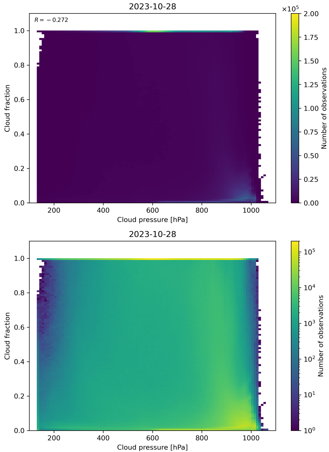
Figure 87: Scatter density plot of “Cloud pressure” against “Cloud fraction” for 2023-10-28 to 2023-10-29.
