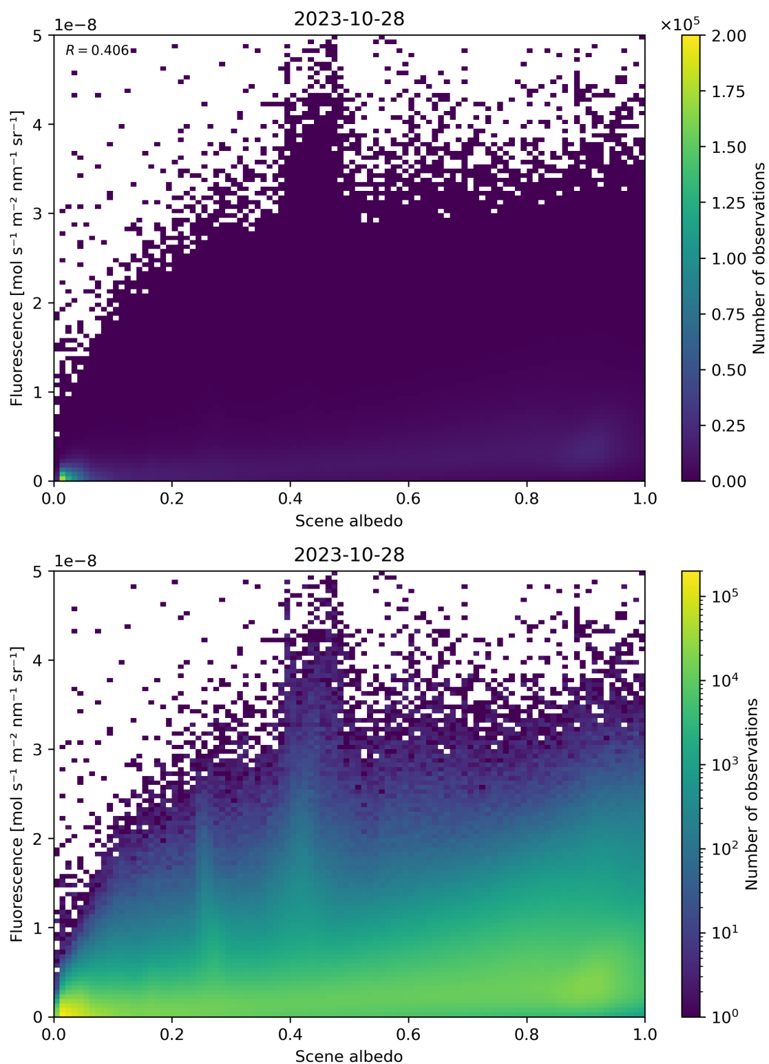
Figure 114: Scatter density plot of “Scene albedo” against “Fluorescence” for 2023-10-28 to 2023-10-29.
