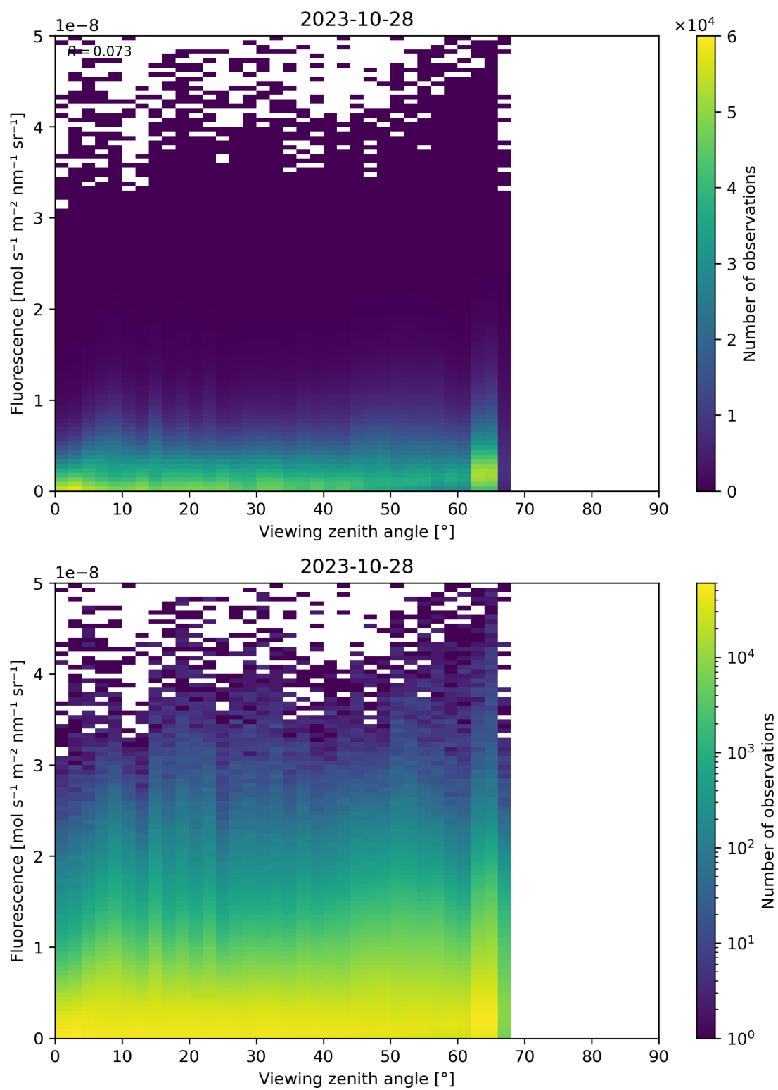
Figure 134: Scatter density plot of “Viewing zenith angle” against “Fluorescence” for 2023-10-28 to 2023-10-29.
