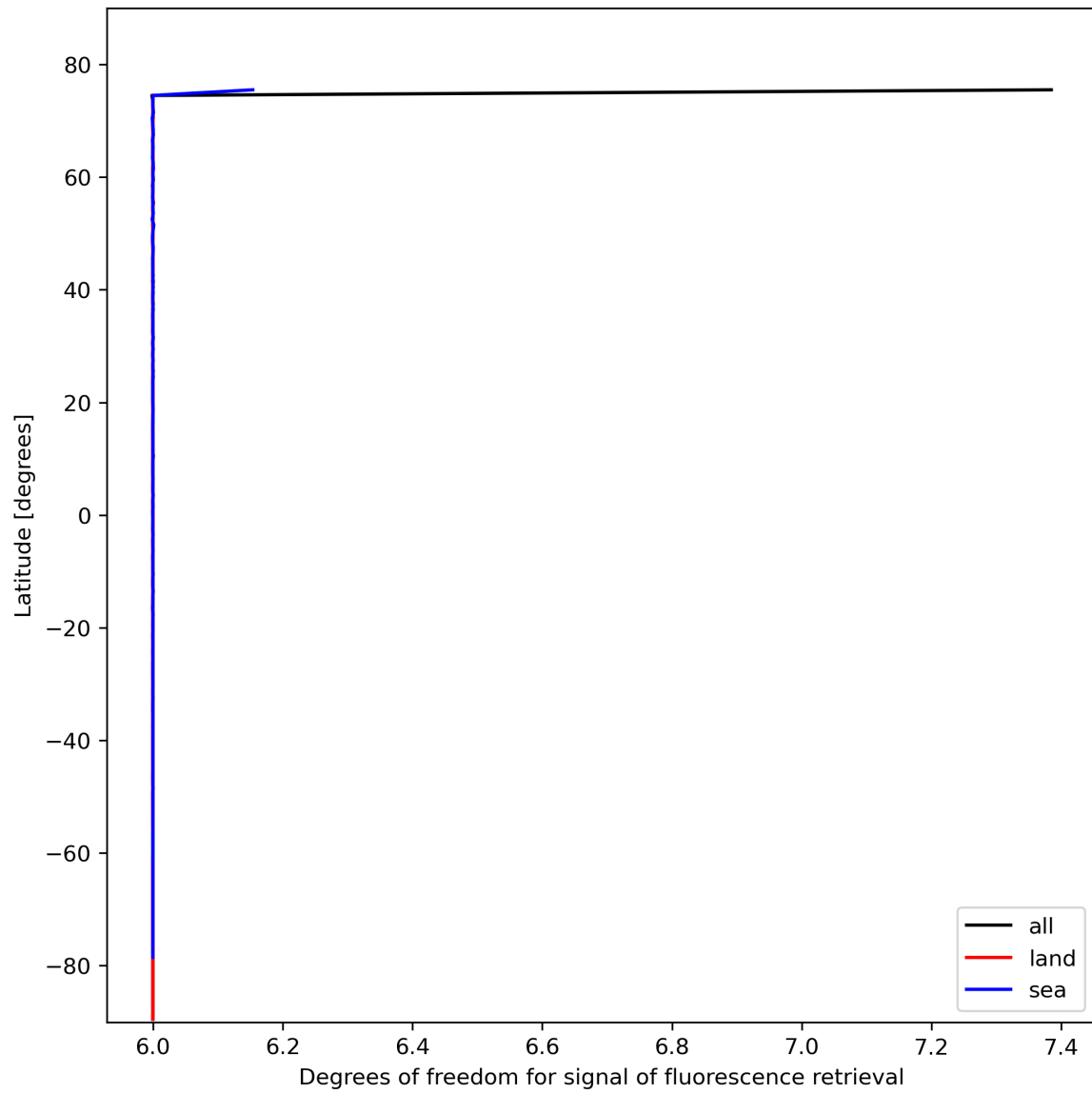
Figure 26: Zonal average of “Degrees of freedom for signal of fluorescence retrieval” for 2023-10-28 to 2023-10-29.
