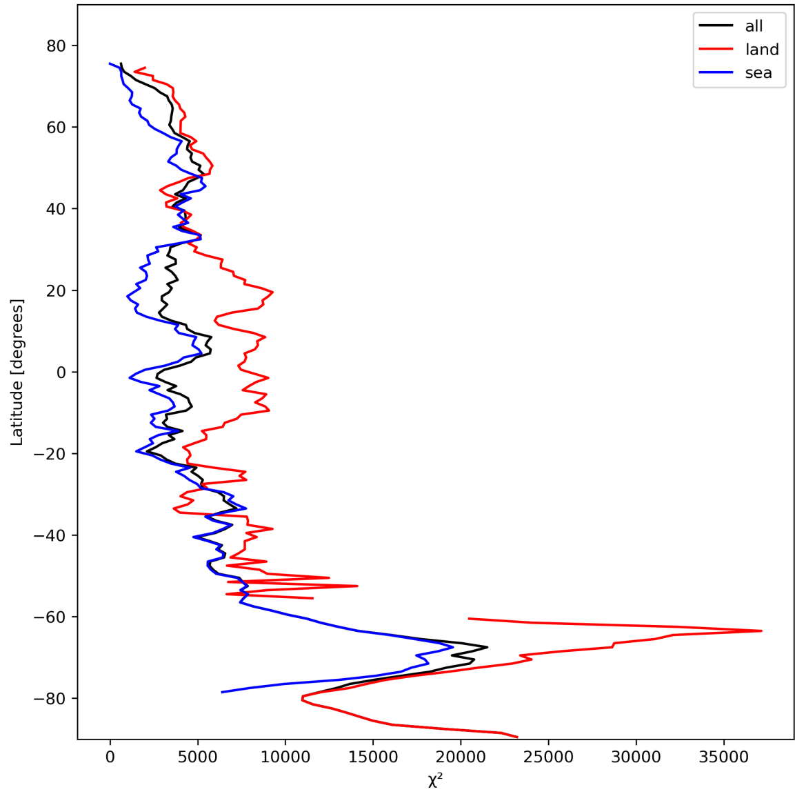
Figure 21: Zonal average of “ \chi^2 ” for 2023-10-28 to 2023-10-29.
