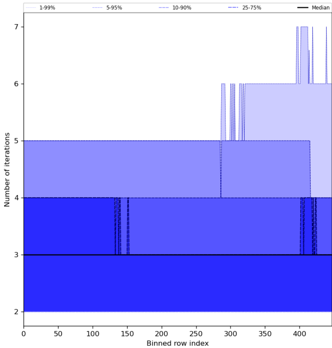
Figure 56: Along track statistics of “Number of iterations” for 2023-10-28 to 2023-10-29
