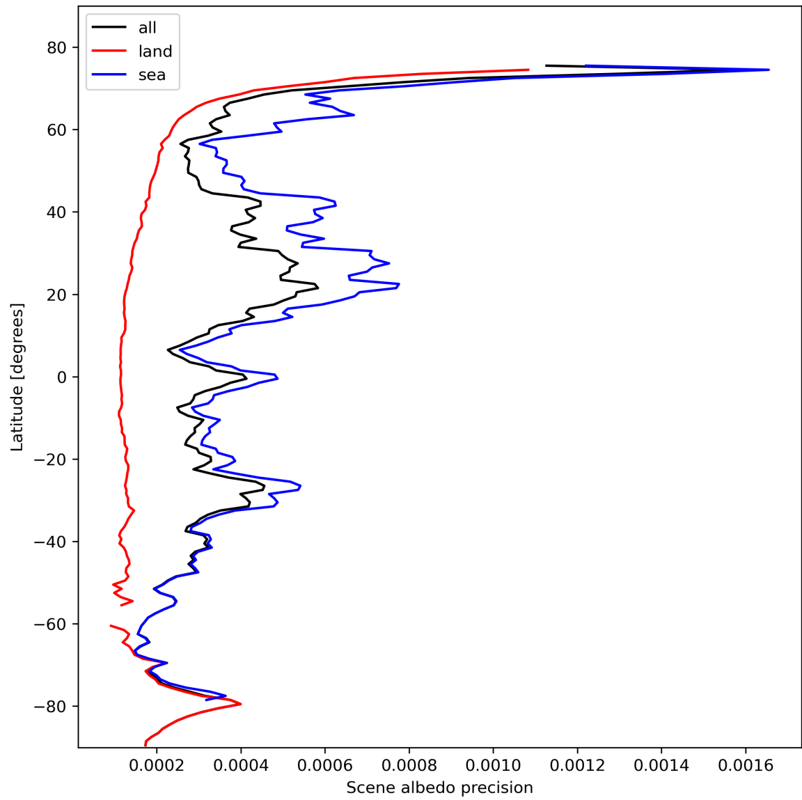
Figure 18: Zonal average of “Scene albedo precision” for 2023-10-28 to 2023-10-29.
