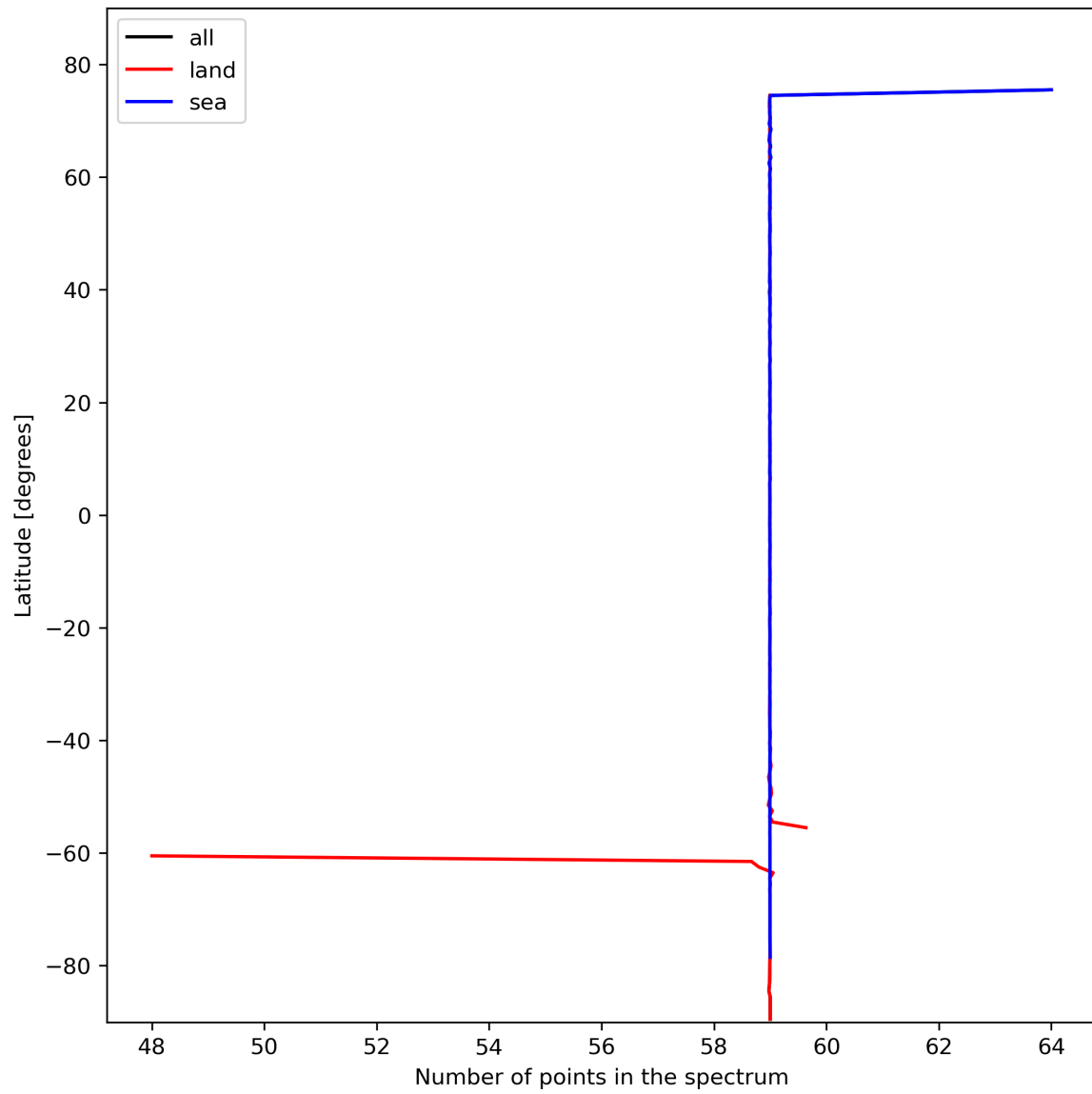
Figure 27: Zonal average of “Number of points in the spectrum” for 2023-10-28 to 2023-10-29.
