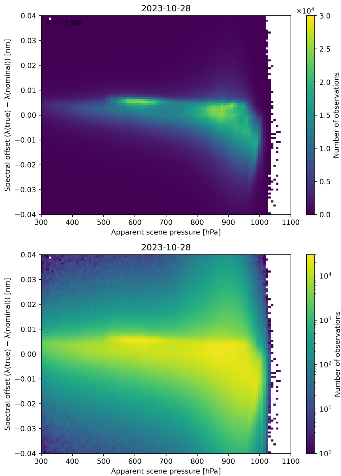
Figure 68: Scatter density plot of “Apparent scene pressure” against “Spectral offset ( \lambda(\text{true}) - \lambda(\text{nominal}) )” for 2023-10-28 to 2023-10-29.
