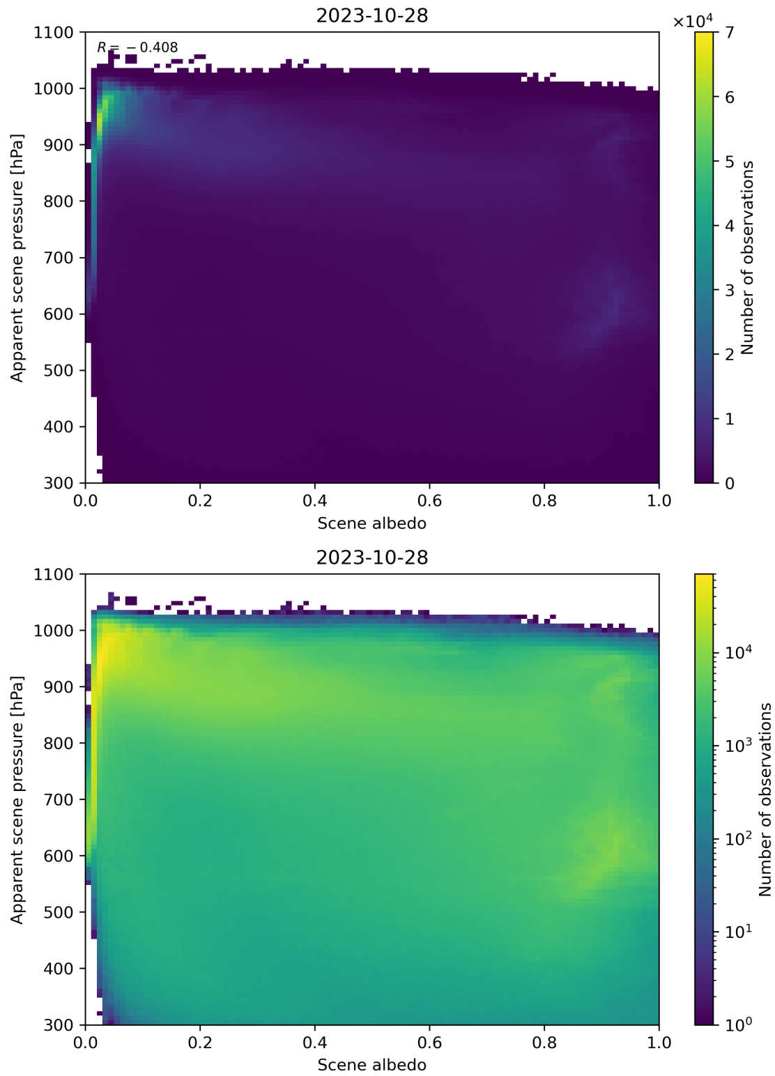
Figure 111: Scatter density plot of “Scene albedo” against “Apparent scene pressure” for 2023-10-28 to 2023-10-29.
