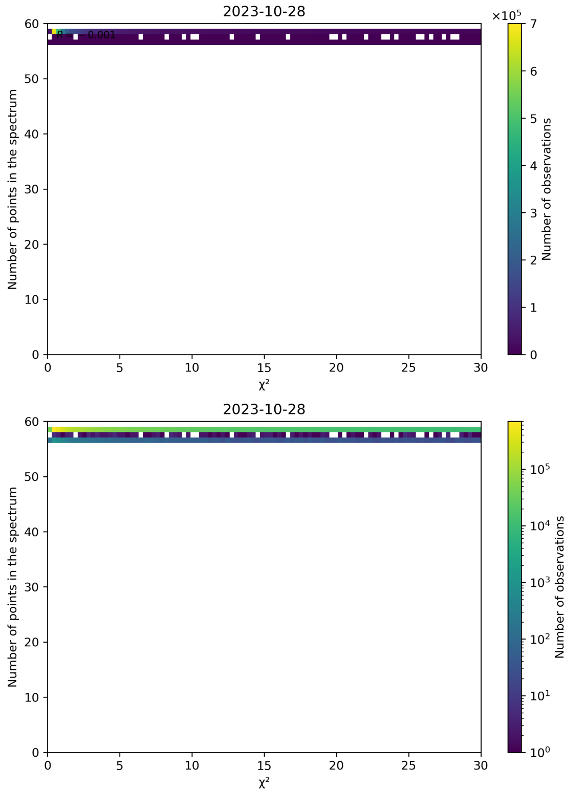
Figure 74: Scatter density plot of " \chi^2 " against "Number of points in the spectrum" for 2023-10-28 to 2023-10-29.
