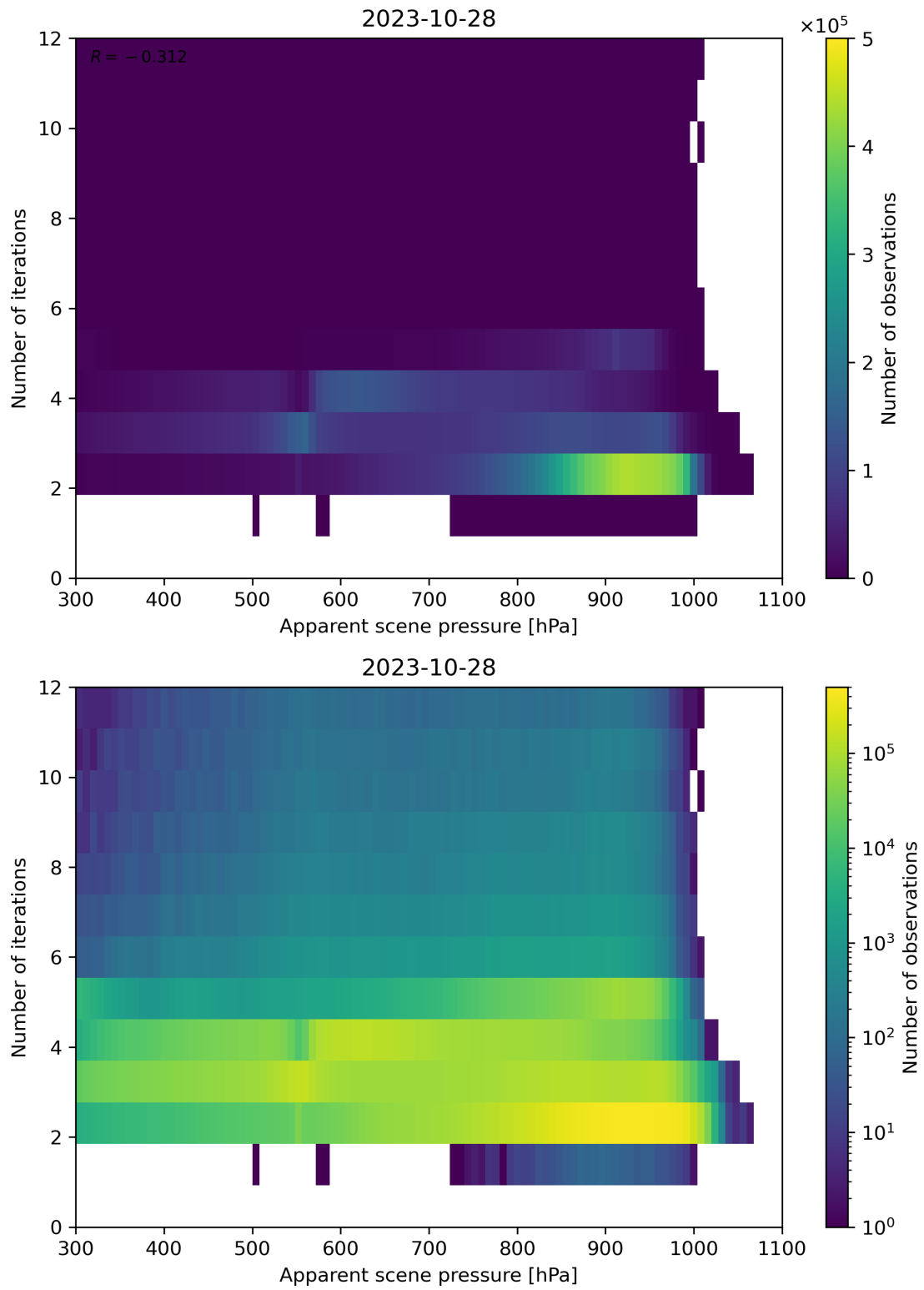
Figure 66: Scatter density plot of “Apparent scene pressure” against “Number of iterations” for 2023-10-28 to 2023-10-29.
