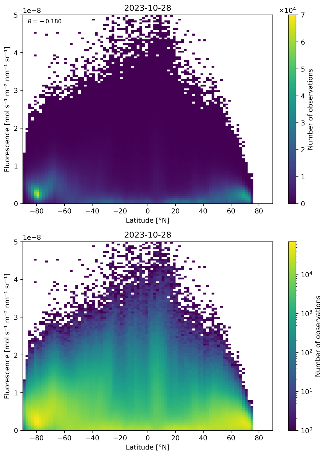
Figure 101: Scatter density plot of “Latitude” against “Fluorescence” for 2023-10-28 to 2023-10-29.
