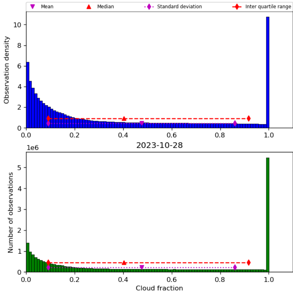
Figure 32: Histogram of “Cloud fraction” for 2023-10-28 to 2023-10-29
