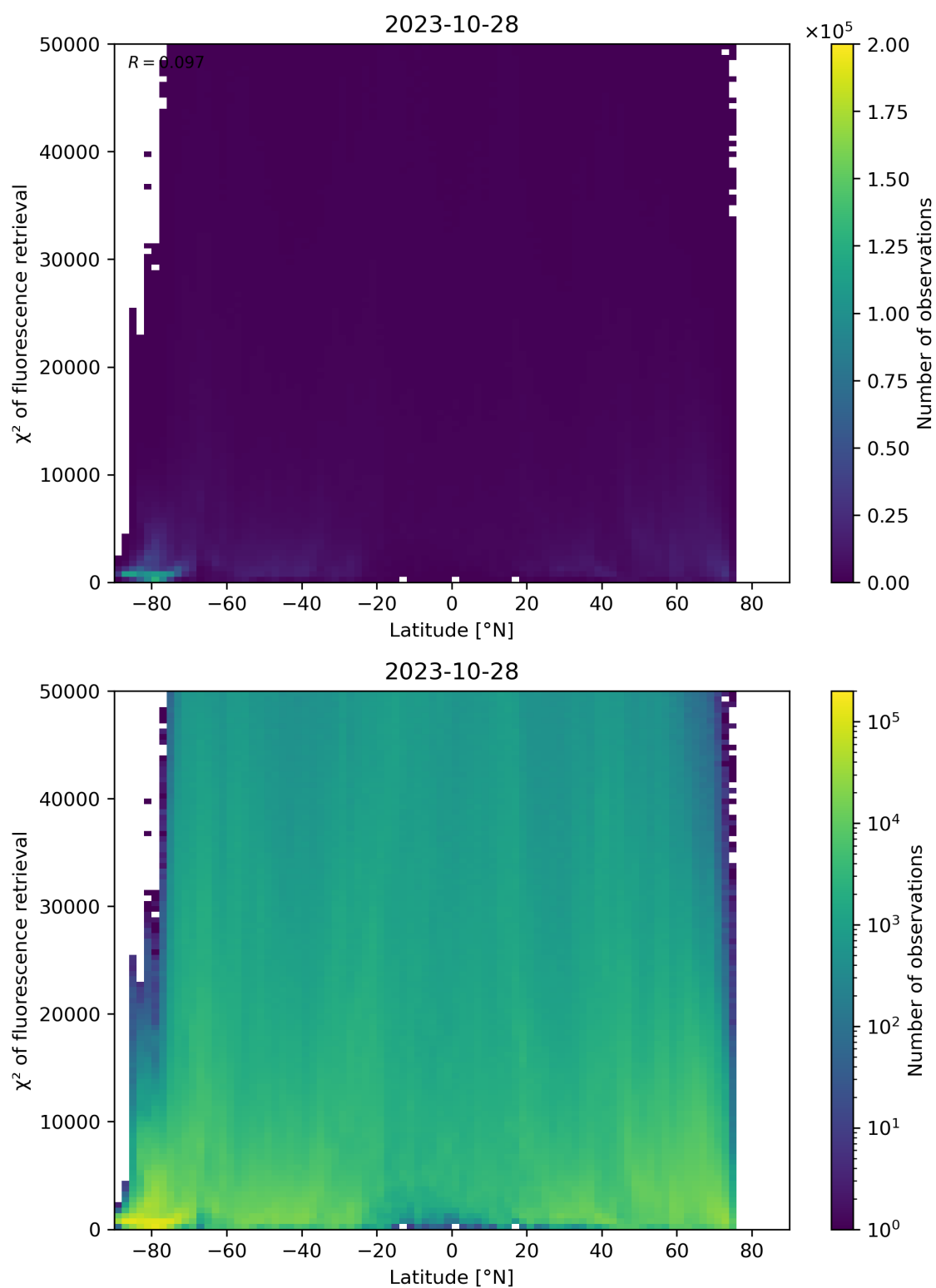
Figure 98: Scatter density plot of “Latitude” against “ \chi^2 of fluorescence retrieval” for 2023-10-28 to 2023-10-29.
