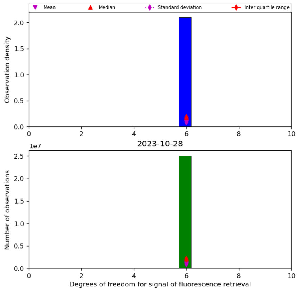
Figure 43: Histogram of “Degrees of freedom for signal of fluorescence retrieval” for 2023-10-28 to 2023-10-29
