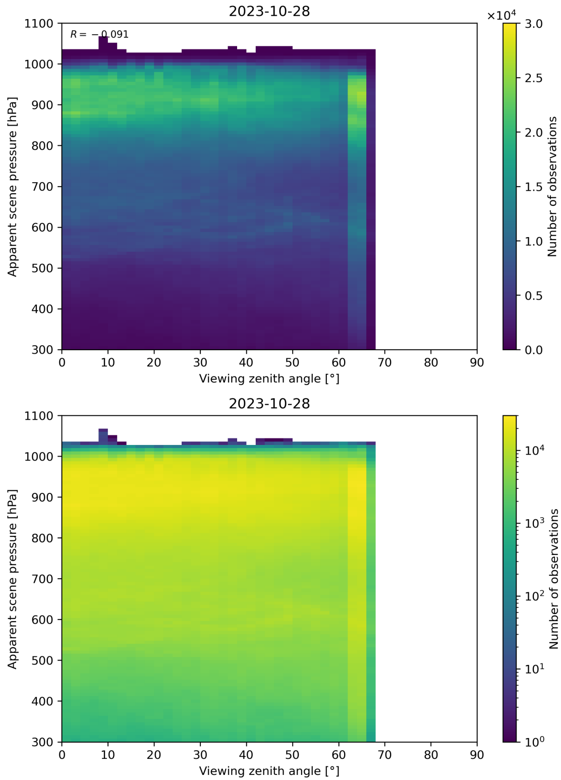
Figure 129: Scatter density plot of “Viewing zenith angle” against “Apparent scene pressure” for 2023-10-28 to 2023-10-29.
