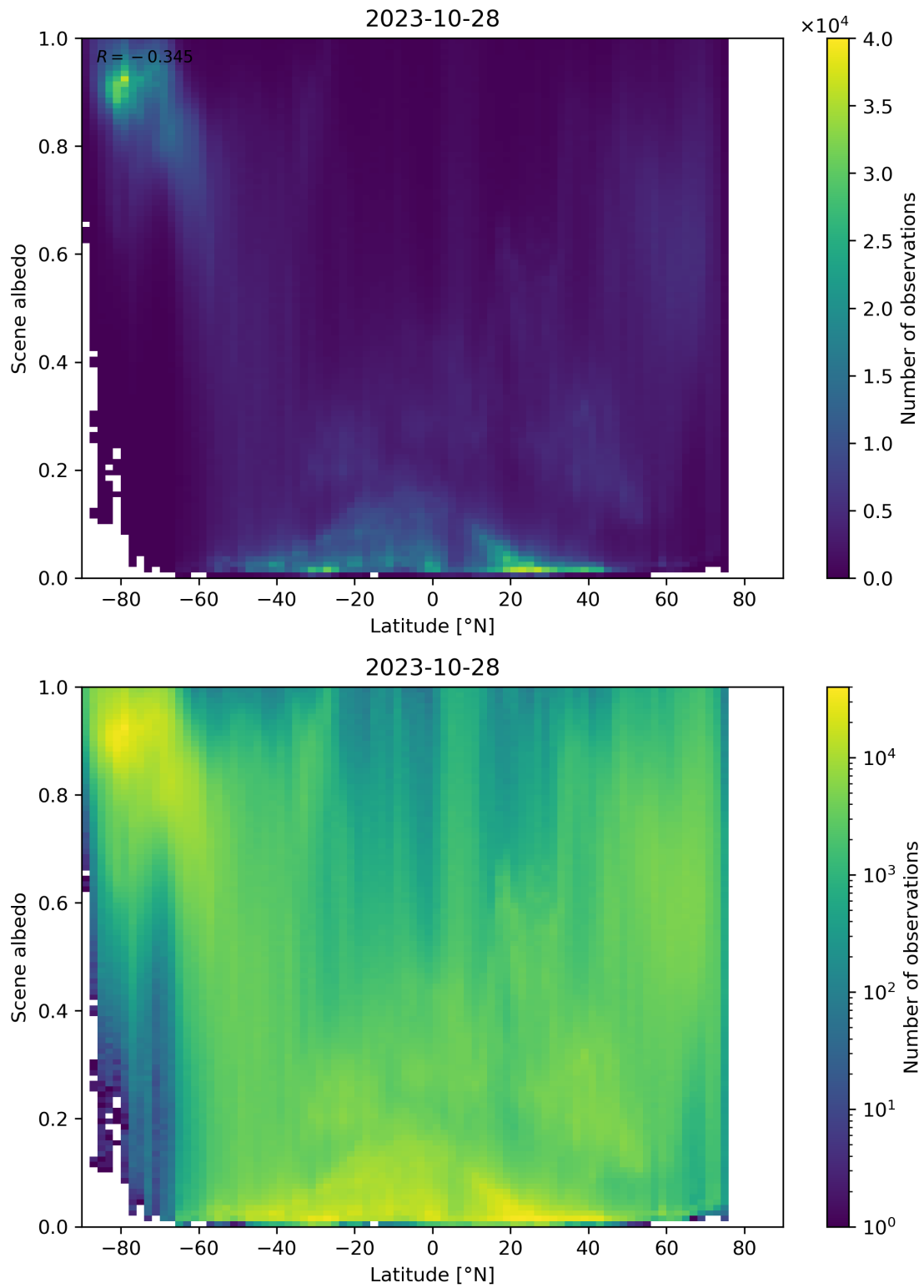
Figure 104: Scatter density plot of “Latitude” against “Scene albedo” for 2023-10-28 to 2023-10-29.
