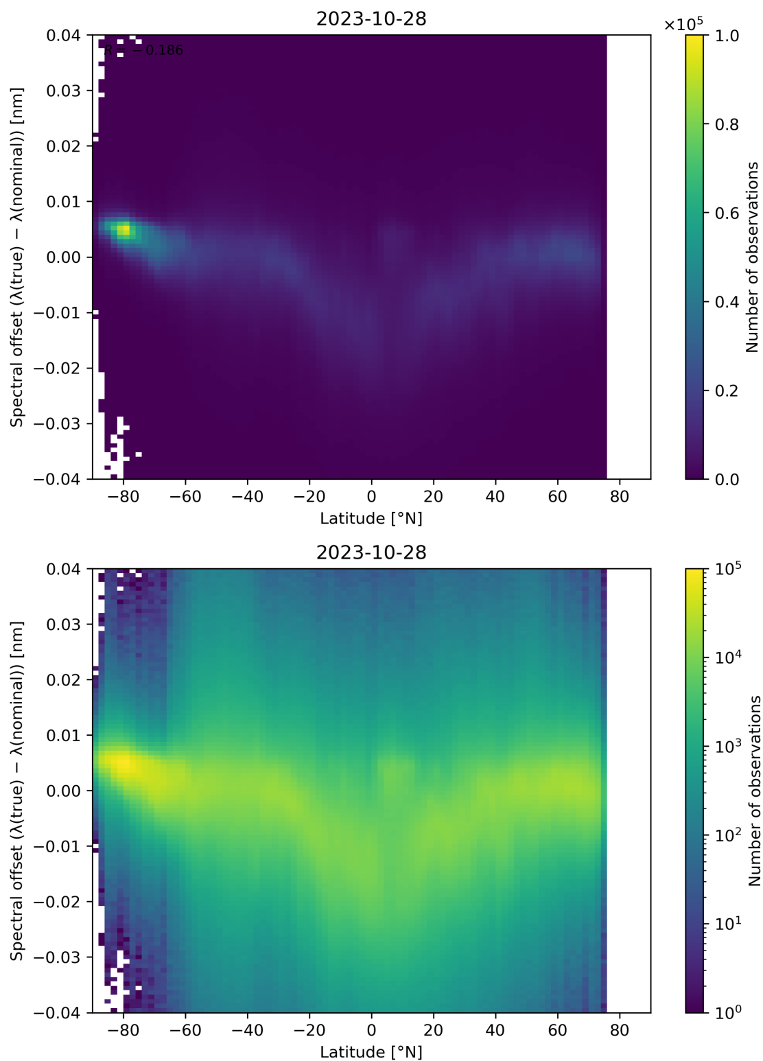
Figure 105: Scatter density plot of “Latitude” against “Spectral offset ( \lambda(\text{true}) - \lambda(\text{nominal}) )” for 2023-10-28 to 2023-10-29.
