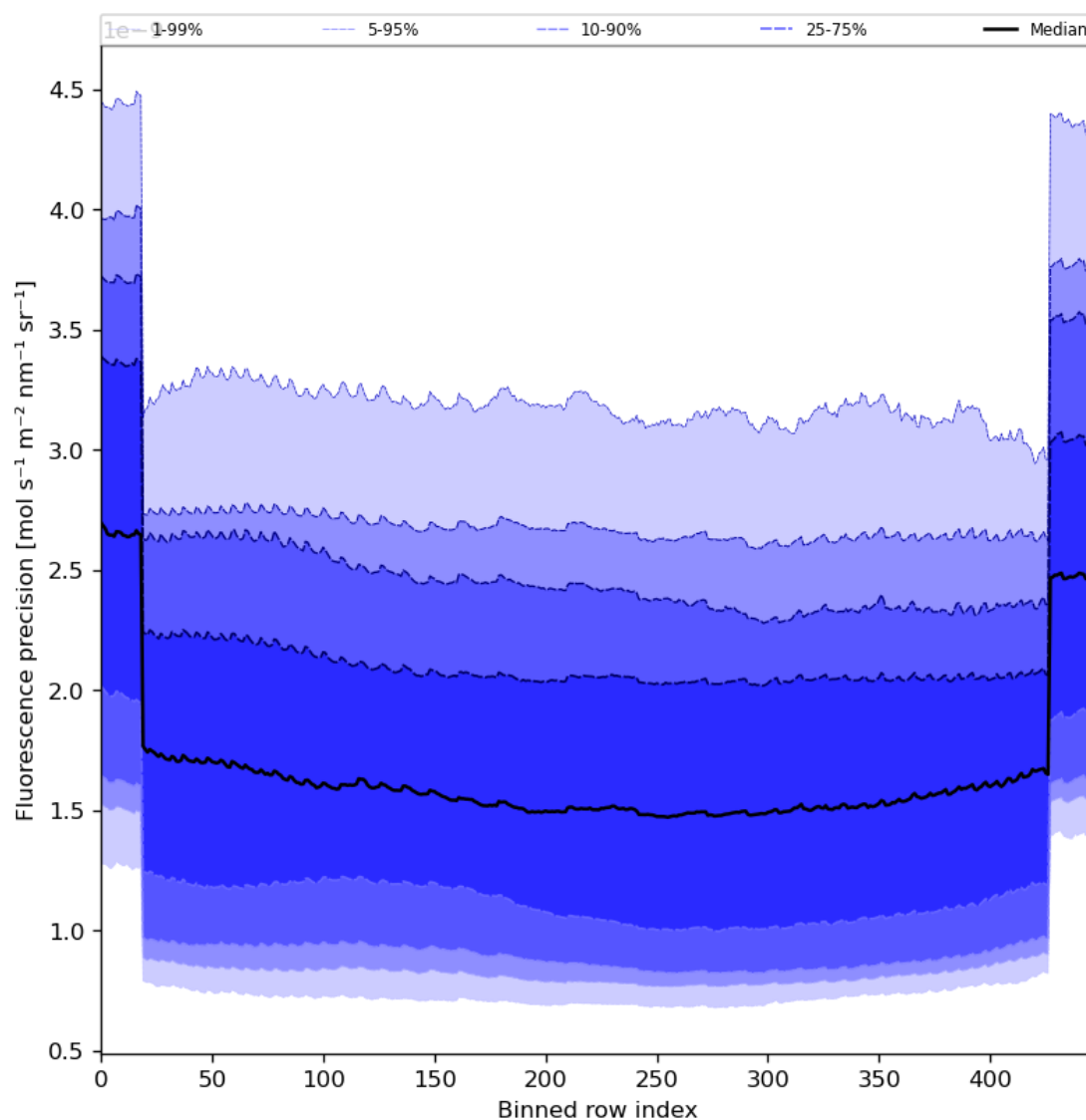
Figure 58: Along track statistics of “Fluorescence precision” for 2023-10-28 to 2023-10-29
