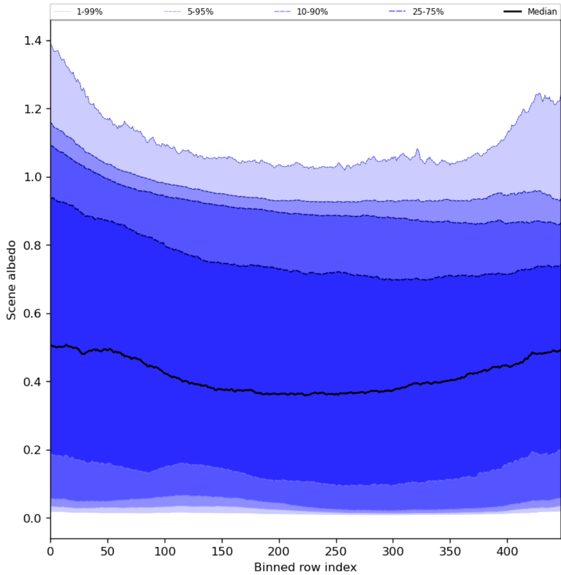
Figure 51: Along track statistics of “Scene albedo” for 2023-10-28 to 2023-10-29
