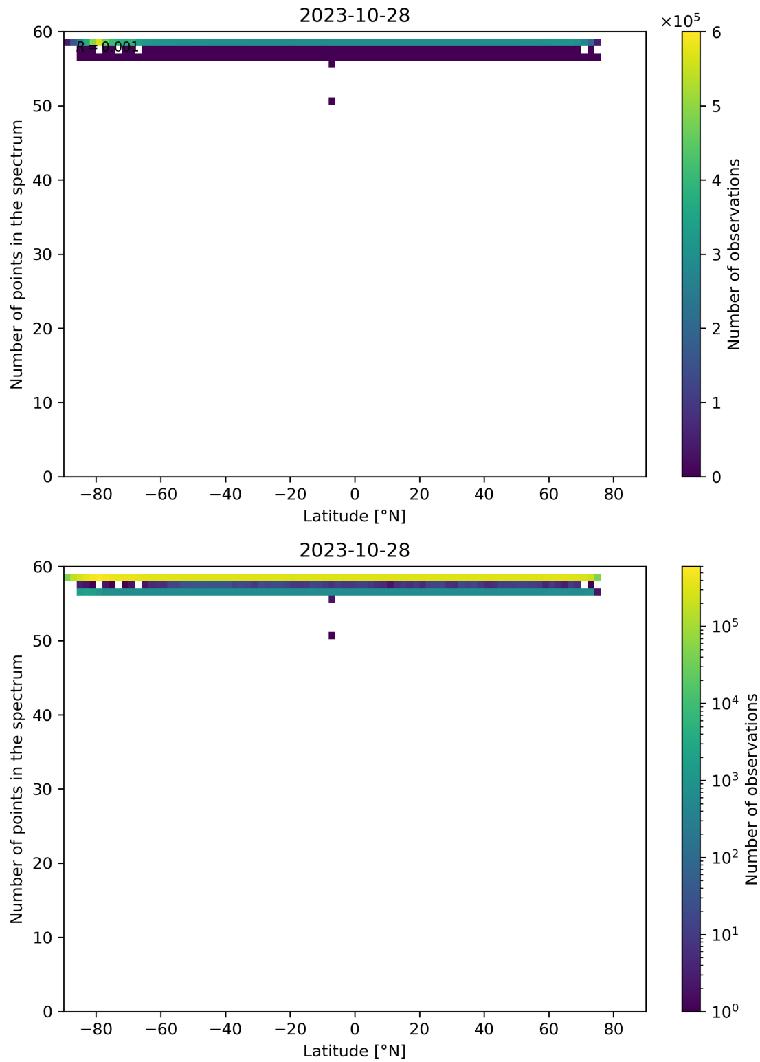
Figure 103: Scatter density plot of “Latitude” against “Number of points in the spectrum” for 2023-10-28 to 2023-10-29.
