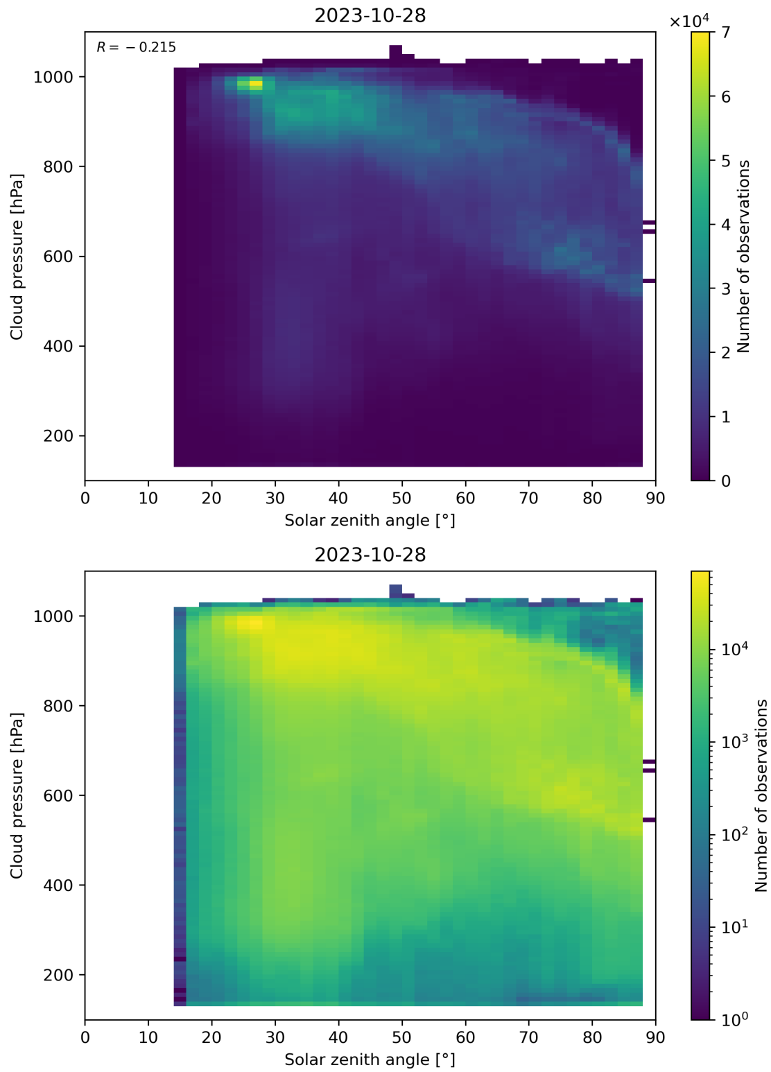
Figure 122: Scatter density plot of “Solar zenith angle” against “Cloud pressure” for 2023-10-28 to 2023-10-29.
