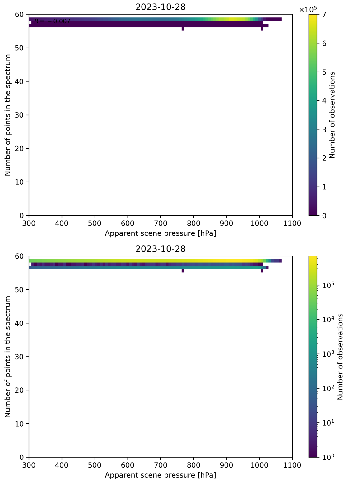
Figure 67: Scatter density plot of “Apparent scene pressure” against “Number of points in the spectrum” for 2023-10-28 to 2023-10-29.
