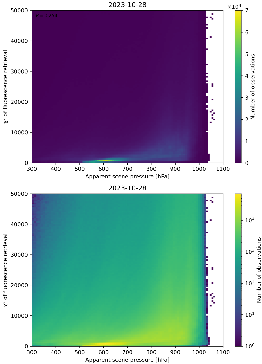
Figure 64: Scatter density plot of “Apparent scene pressure” against “ \chi^2 of fluorescence retrieval” for 2023-10-28 to 2023-10-29.
