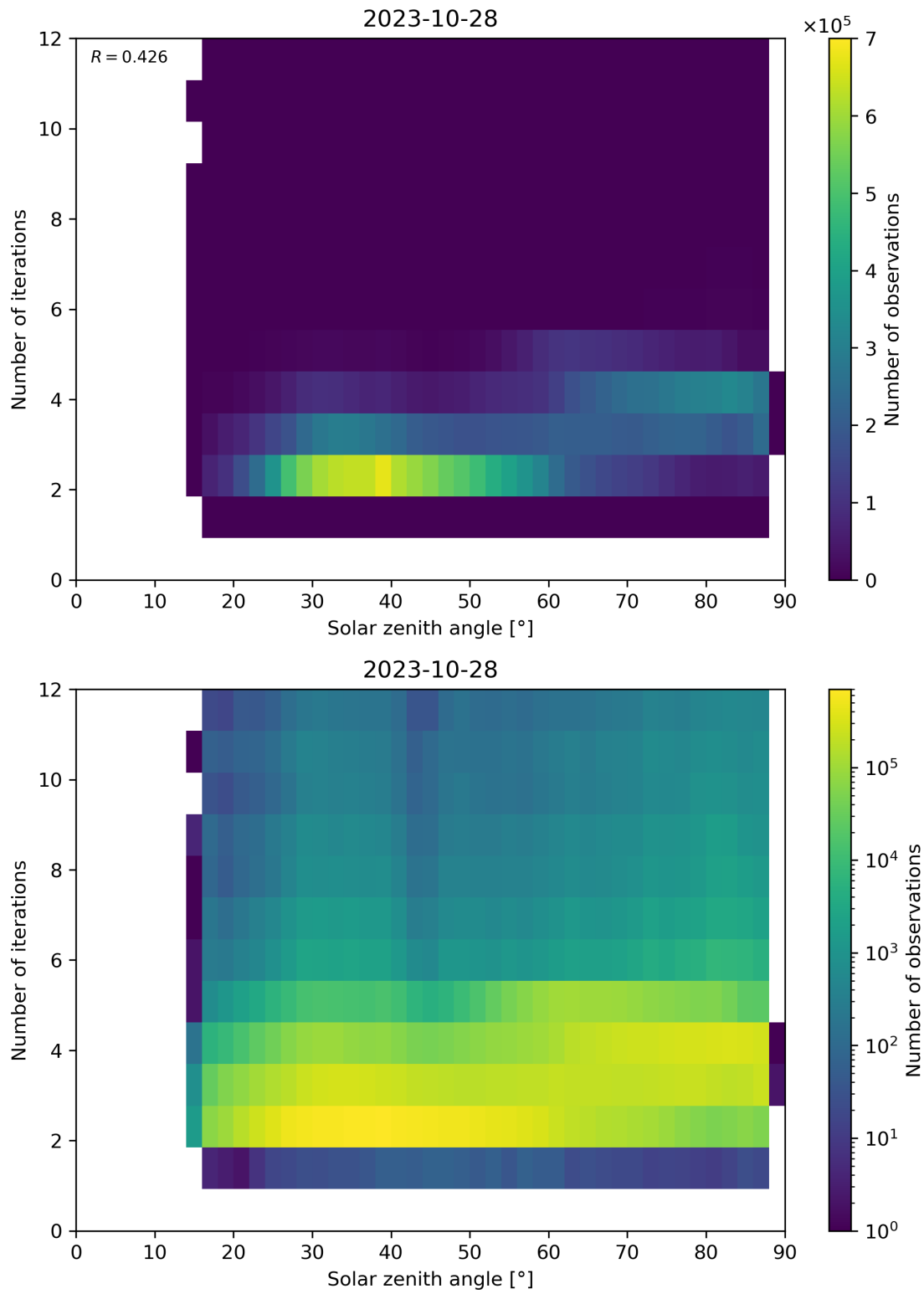
Figure 125: Scatter density plot of “Solar zenith angle” against “Number of iterations” for 2023-10-28 to 2023-10-29.
