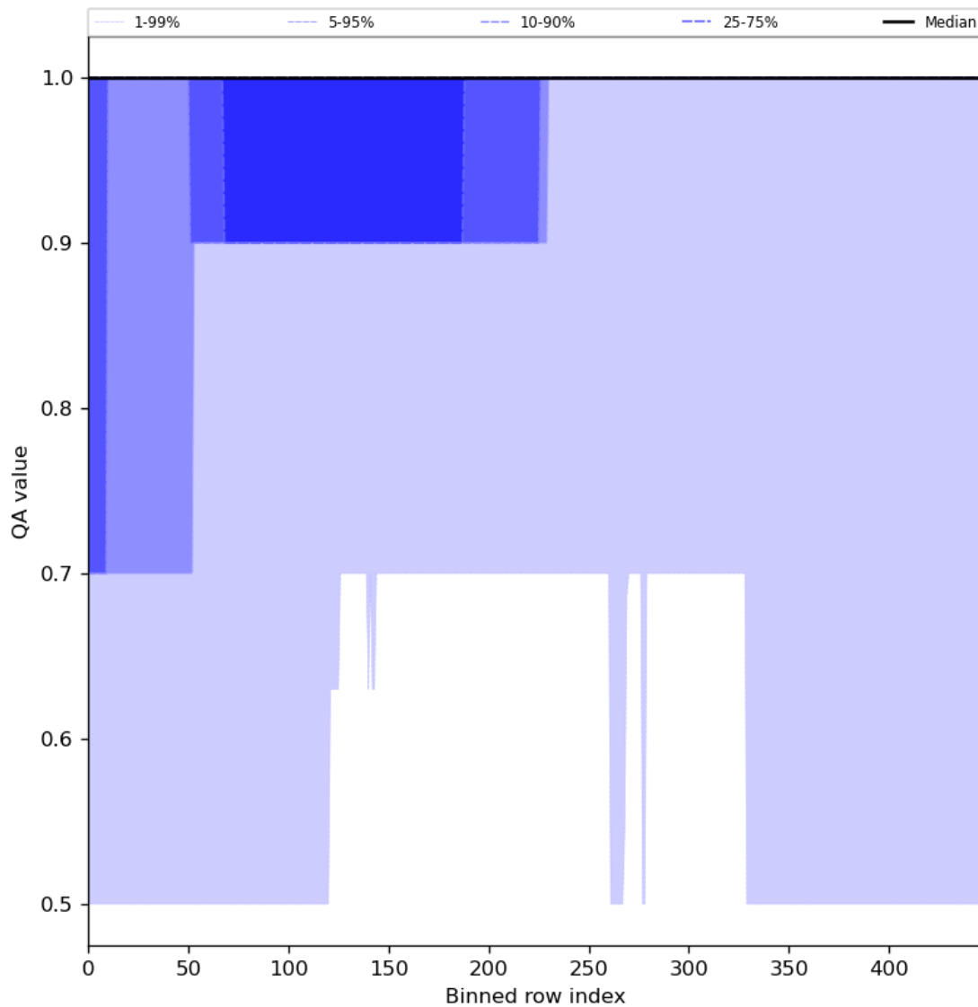
Figure 46: Along track statistics of “QA value” for 2023-10-28 to 2023-10-29
