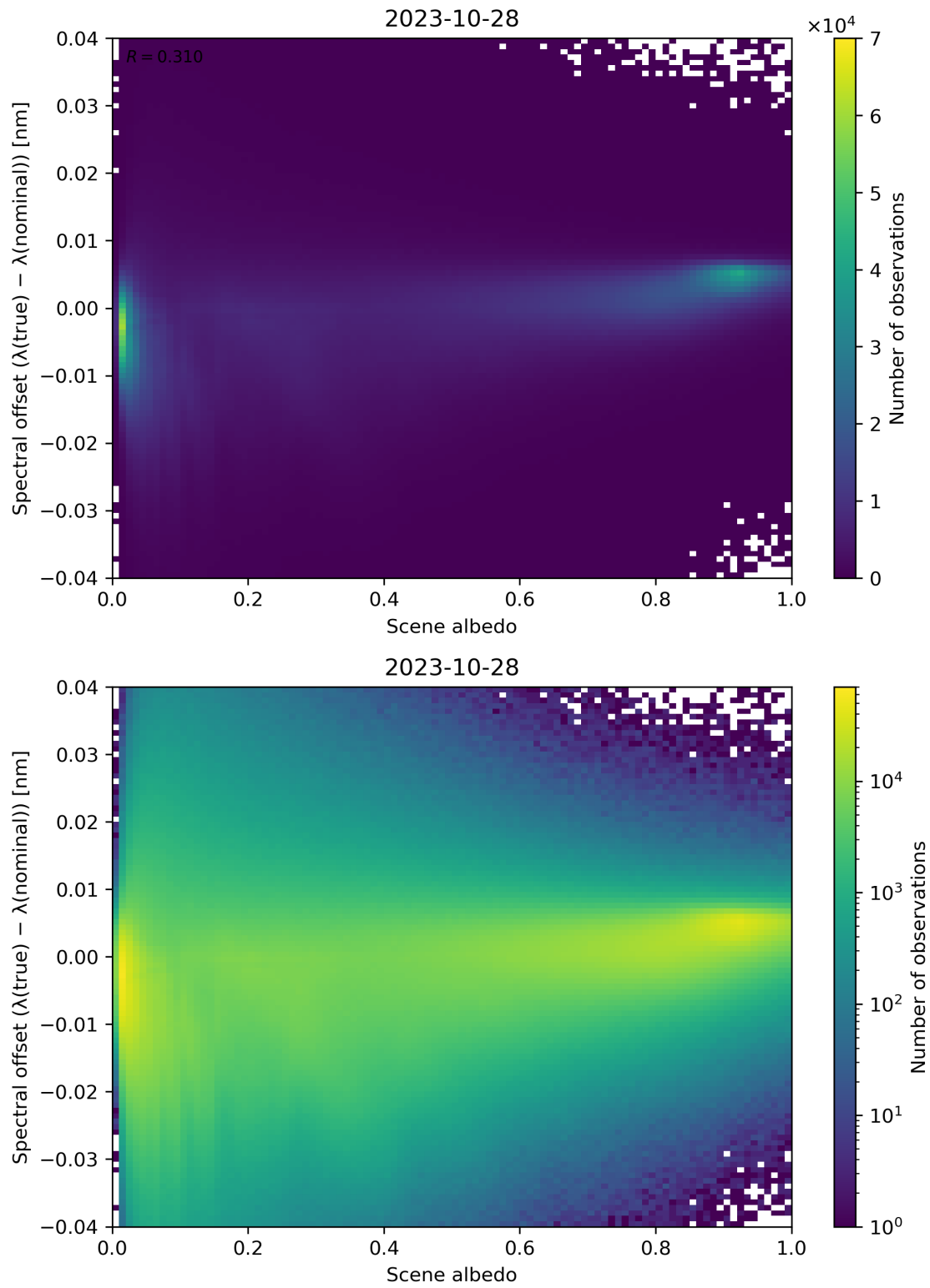
Figure 117: Scatter density plot of “Scene albedo” against “Spectral offset ( \lambda(\text{true}) - \lambda(\text{nominal}) )” for 2023-10-28 to 2023-10-29.
