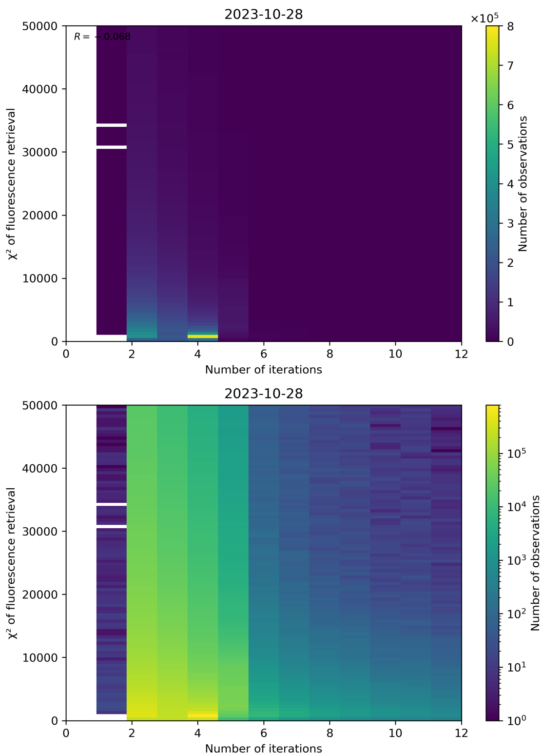
Figure 106: Scatter density plot of “Number of iterations” against “ \chi^2 of fluorescence retrieval” for 2023-10-28 to 2023-10-29.
