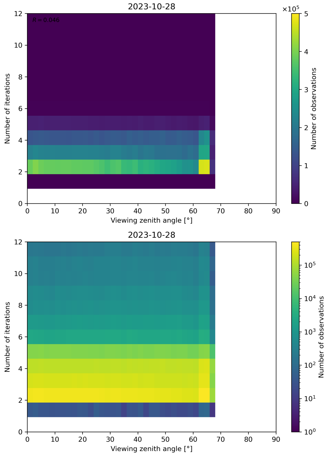
Figure 136: Scatter density plot of “Viewing zenith angle” against “Number of iterations” for 2023-10-28 to 2023-10-29.
