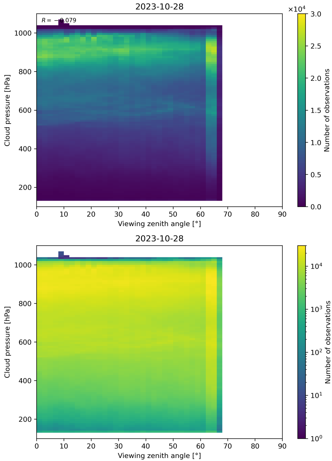
Figure 133: Scatter density plot of “Viewing zenith angle” against “Cloud pressure” for 2023-10-28 to 2023-10-29.
