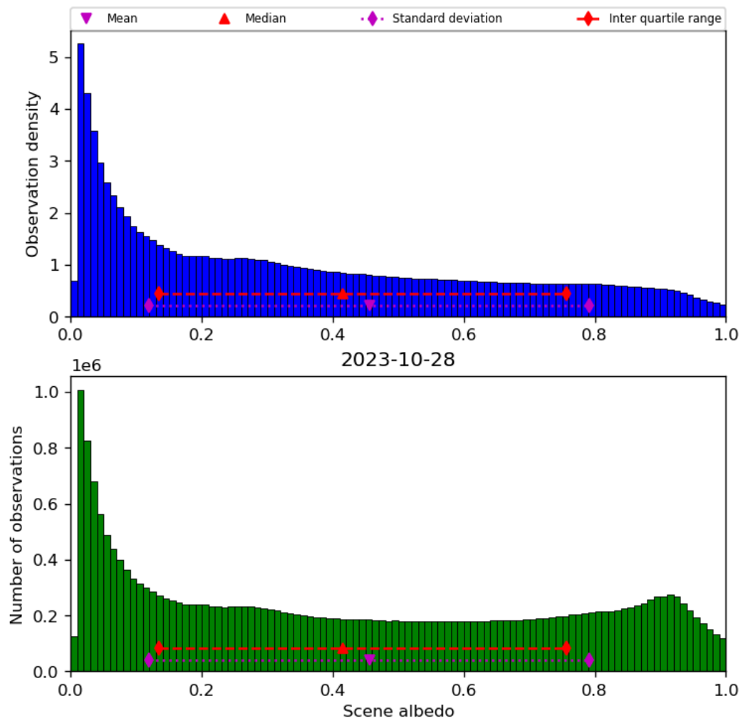
Figure 34: Histogram of “Scene albedo” for 2023-10-28 to 2023-10-29
