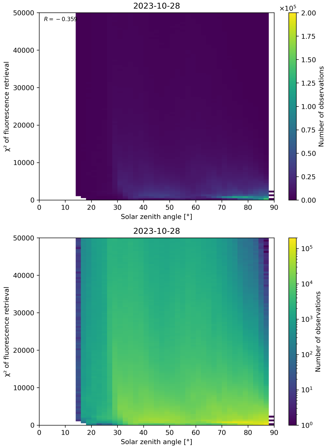
Figure 120: Scatter density plot of “Solar zenith angle” against “ \chi^2 of fluorescence retrieval” for 2023-10-28 to 2023-10-29.
