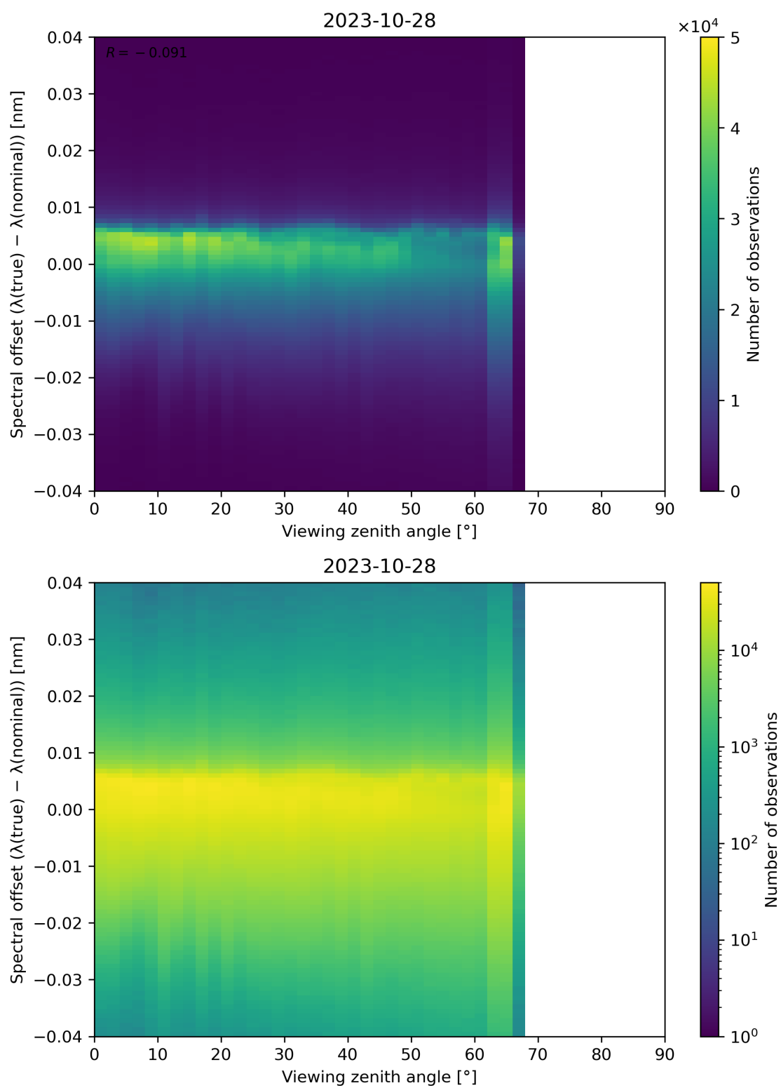
Figure 140: Scatter density plot of “Viewing zenith angle” against “Spectral offset ( \lambda(\text{true}) - \lambda(\text{nominal}) )” for 2023-10-28 to 2023-10-29.
