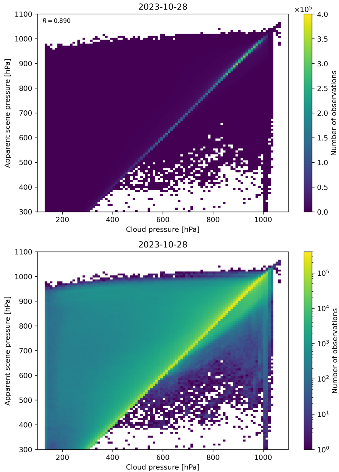
Figure 84: Scatter density plot of “Cloud pressure” against “Apparent scene pressure” for 2023-10-28 to 2023-10-29.
