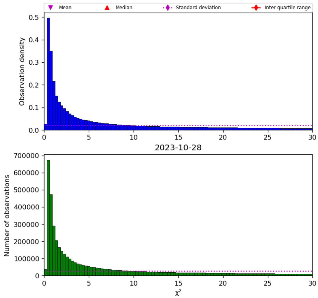
Figure 38: Histogram of “ \chi^2 ” for 2023-10-28 to 2023-10-29
