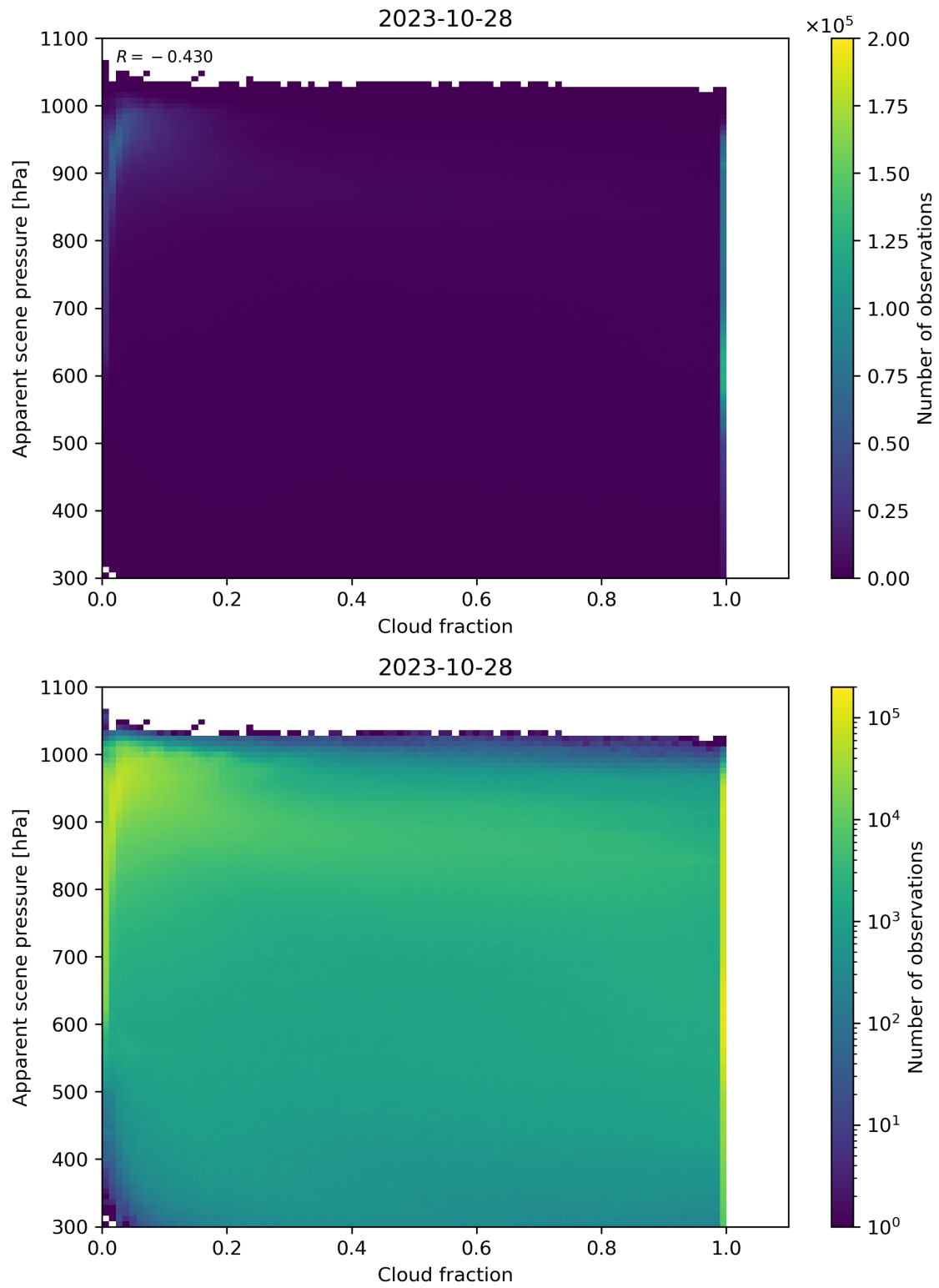
Figure 76: Scatter density plot of “Cloud fraction” against “Apparent scene pressure” for 2023-10-28 to 2023-10-29.
