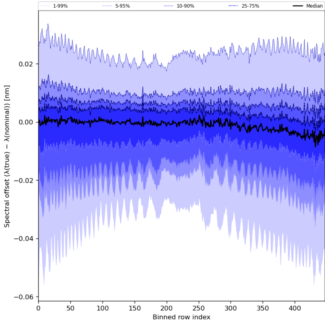
Figure 62: Along track statistics of “Spectral offset ( \lambda(\text{true}) - \lambda(\text{nominal}) )” for 2023-10-28 to 2023-10-29
