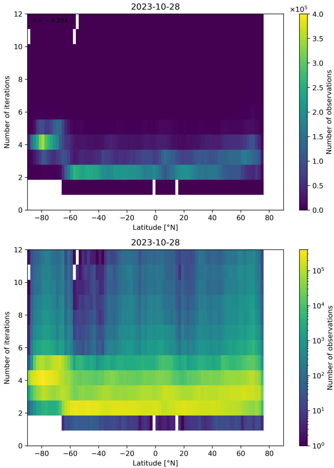
Figure 102: Scatter density plot of “Latitude” against “Number of iterations” for 2023-10-28 to 2023-10-29.
