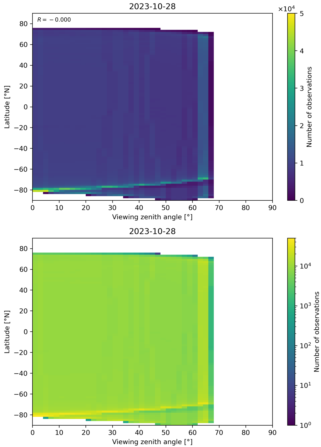
Figure 135: Scatter density plot of “Viewing zenith angle” against “Latitude” for 2023-10-28 to 2023-10-29.
