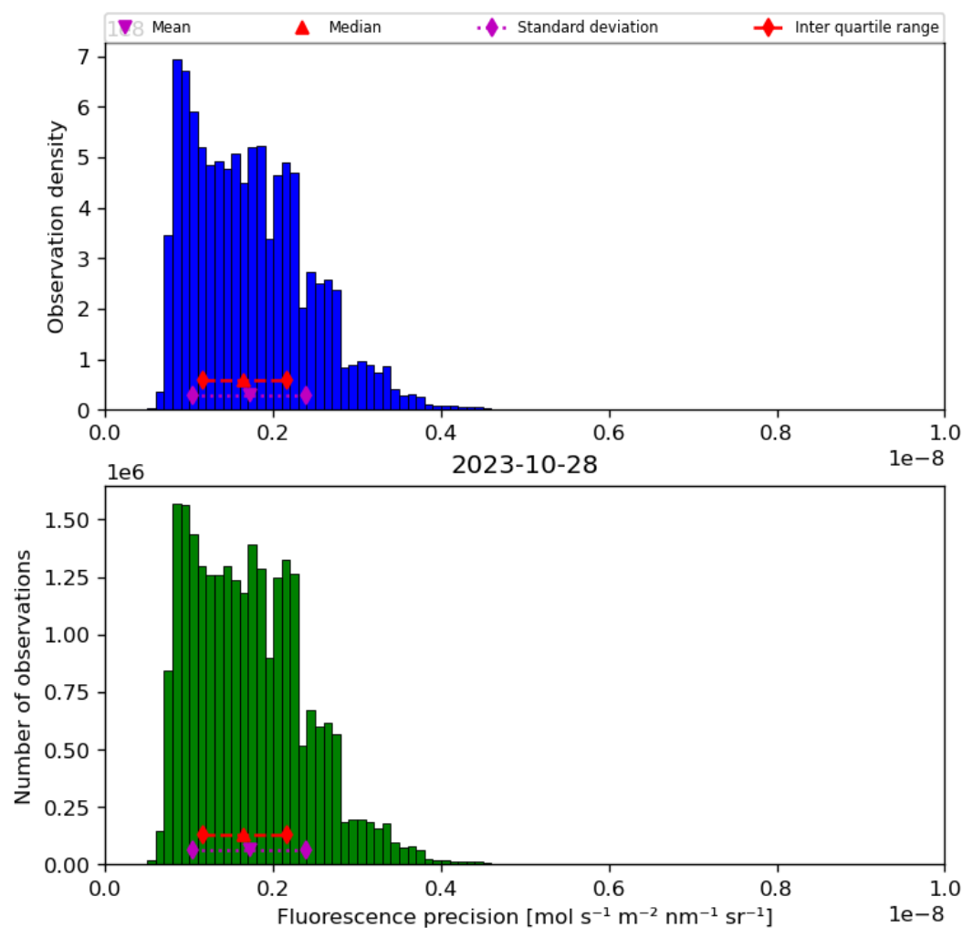
Figure 41: Histogram of “Fluorescence precision” for 2023-10-28 to 2023-10-29
