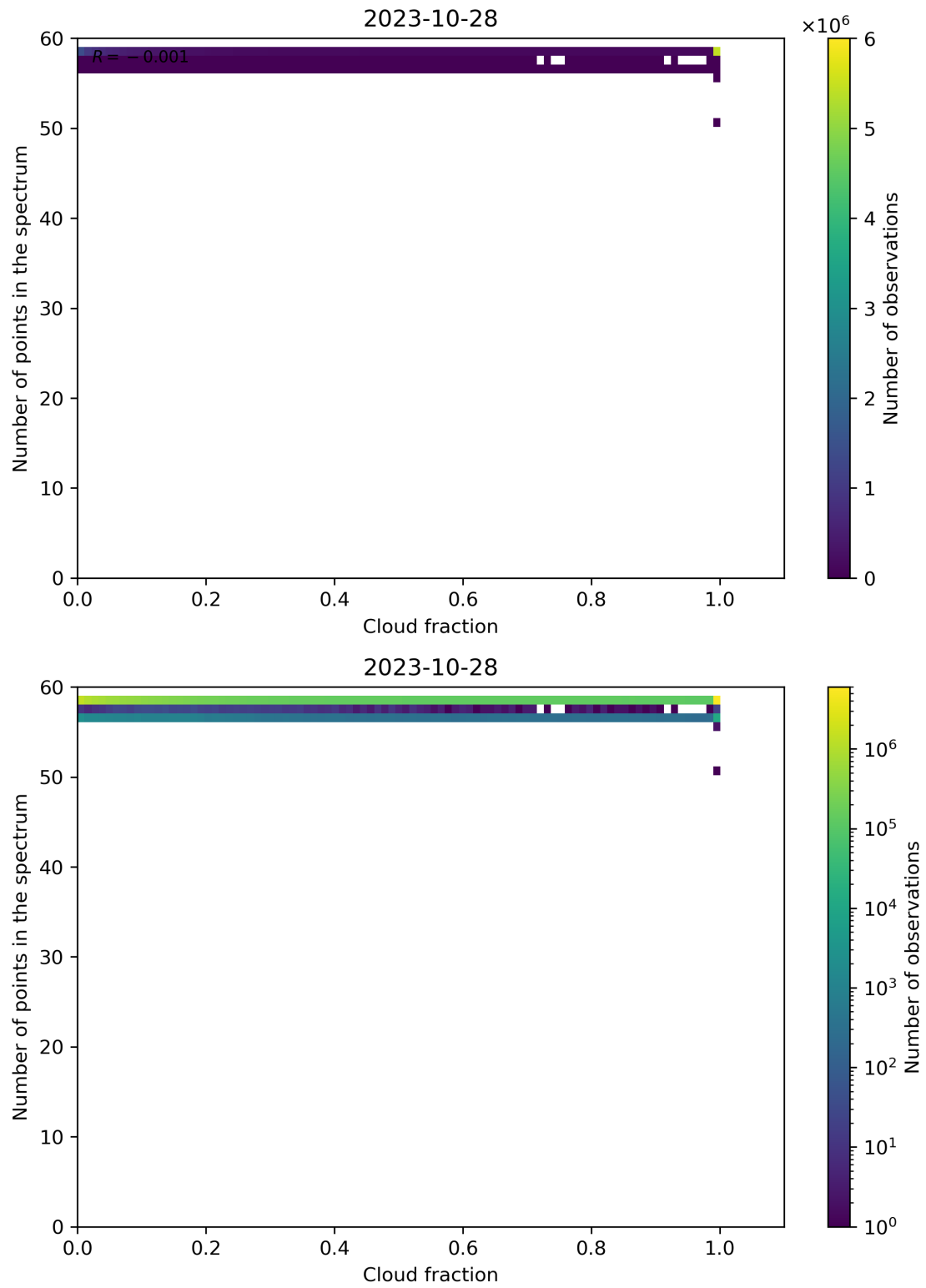
Figure 81: Scatter density plot of “Cloud fraction” against “Number of points in the spectrum” for 2023-10-28 to 2023-10-29.
