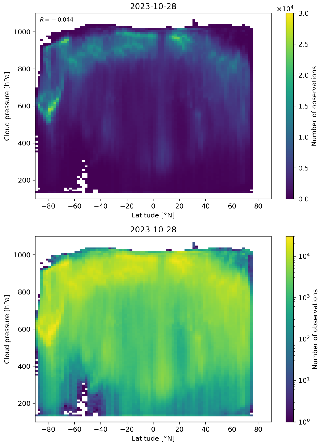
Figure 100: Scatter density plot of “Latitude” against “Cloud pressure” for 2023-10-28 to 2023-10-29.
