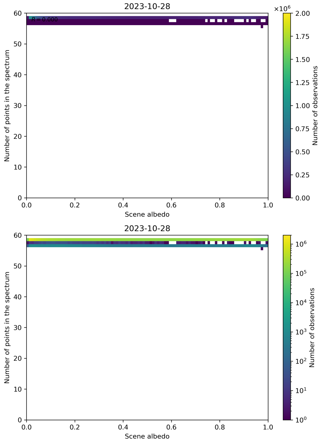
Figure 116: Scatter density plot of “Scene albedo” against “Number of points in the spectrum” for 2023-10-28 to 2023-10-29.
