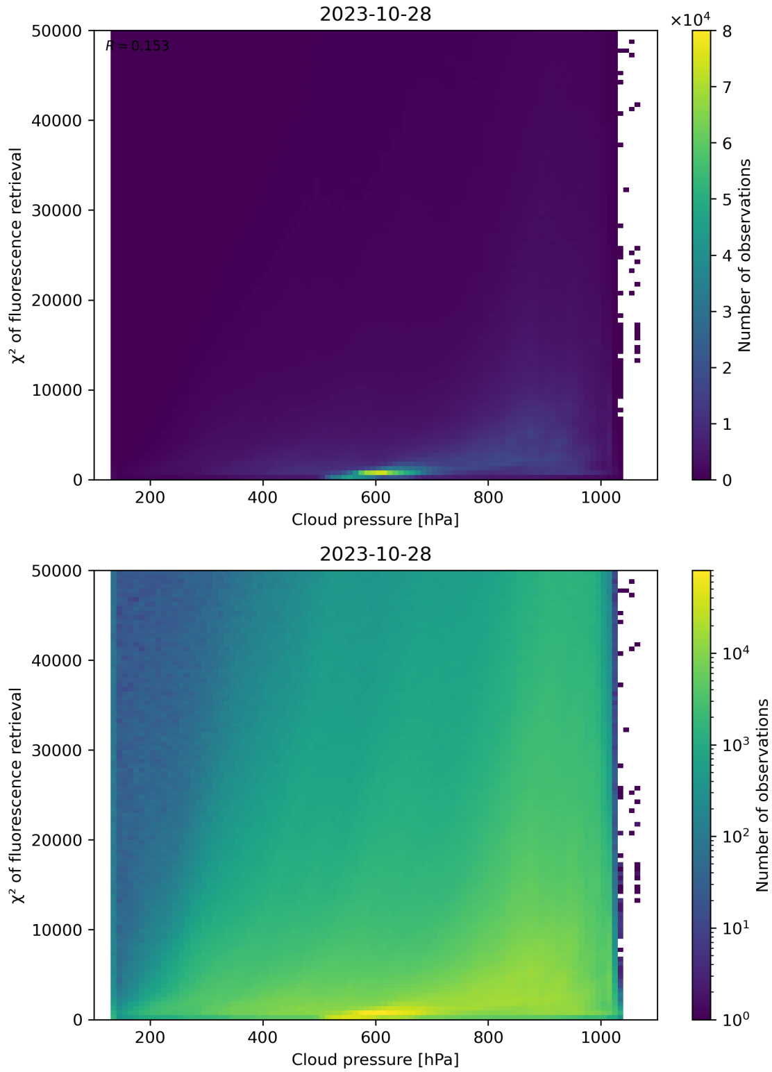
Figure 86: Scatter density plot of “Cloud pressure” against “ \chi^2 of fluorescence retrieval” for 2023-10-28 to 2023-10-29.
