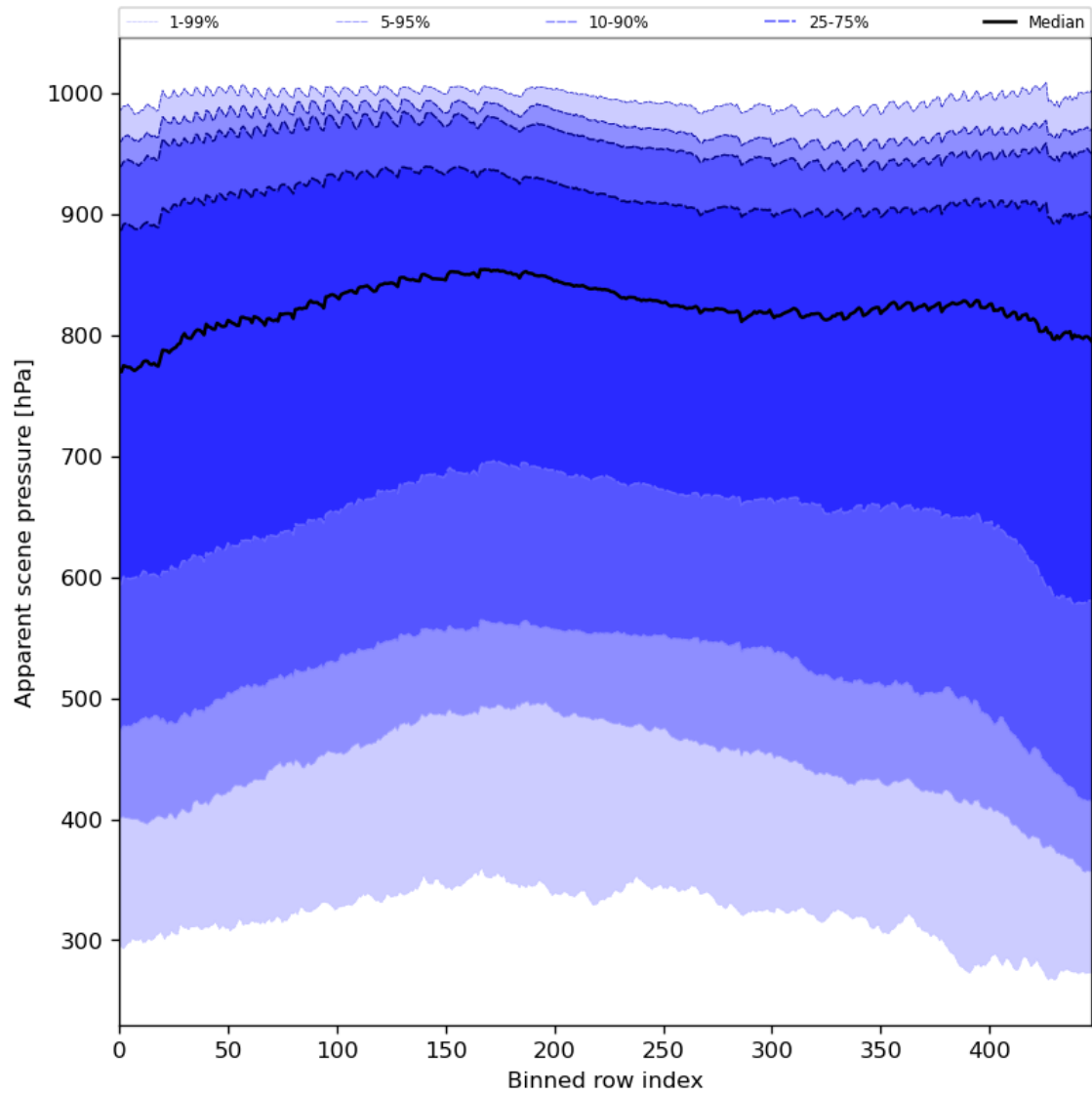
Figure 53: Along track statistics of “Apparent scene pressure” for 2023-10-28 to 2023-10-29
