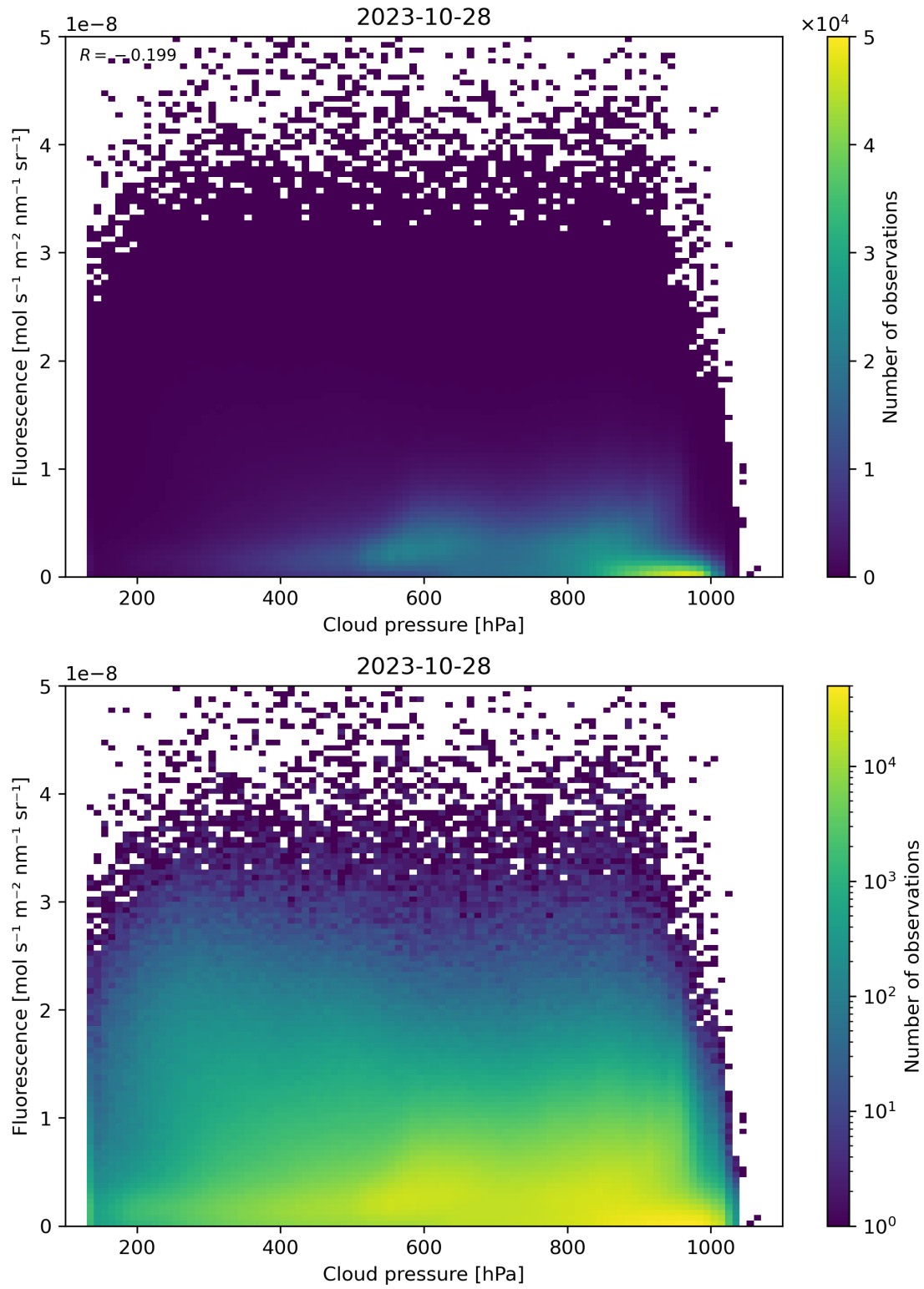
Figure 88: Scatter density plot of “Cloud pressure” against “Fluorescence” for 2023-10-28 to 2023-10-29.
