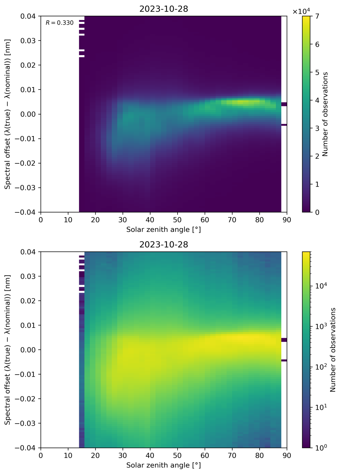
Figure 128: Scatter density plot of “Solar zenith angle” against “Spectral offset ( \lambda(\text{true}) - \lambda(\text{nominal}) )” for 2023-10-28 to 2023-10-29.
