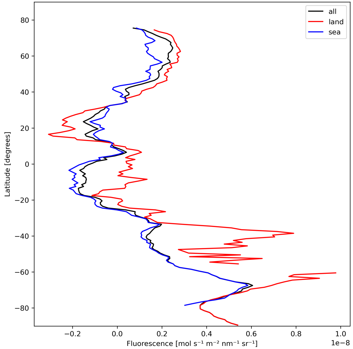
Figure 23: Zonal average of “Fluorescence” for 2023-10-28 to 2023-10-29.
