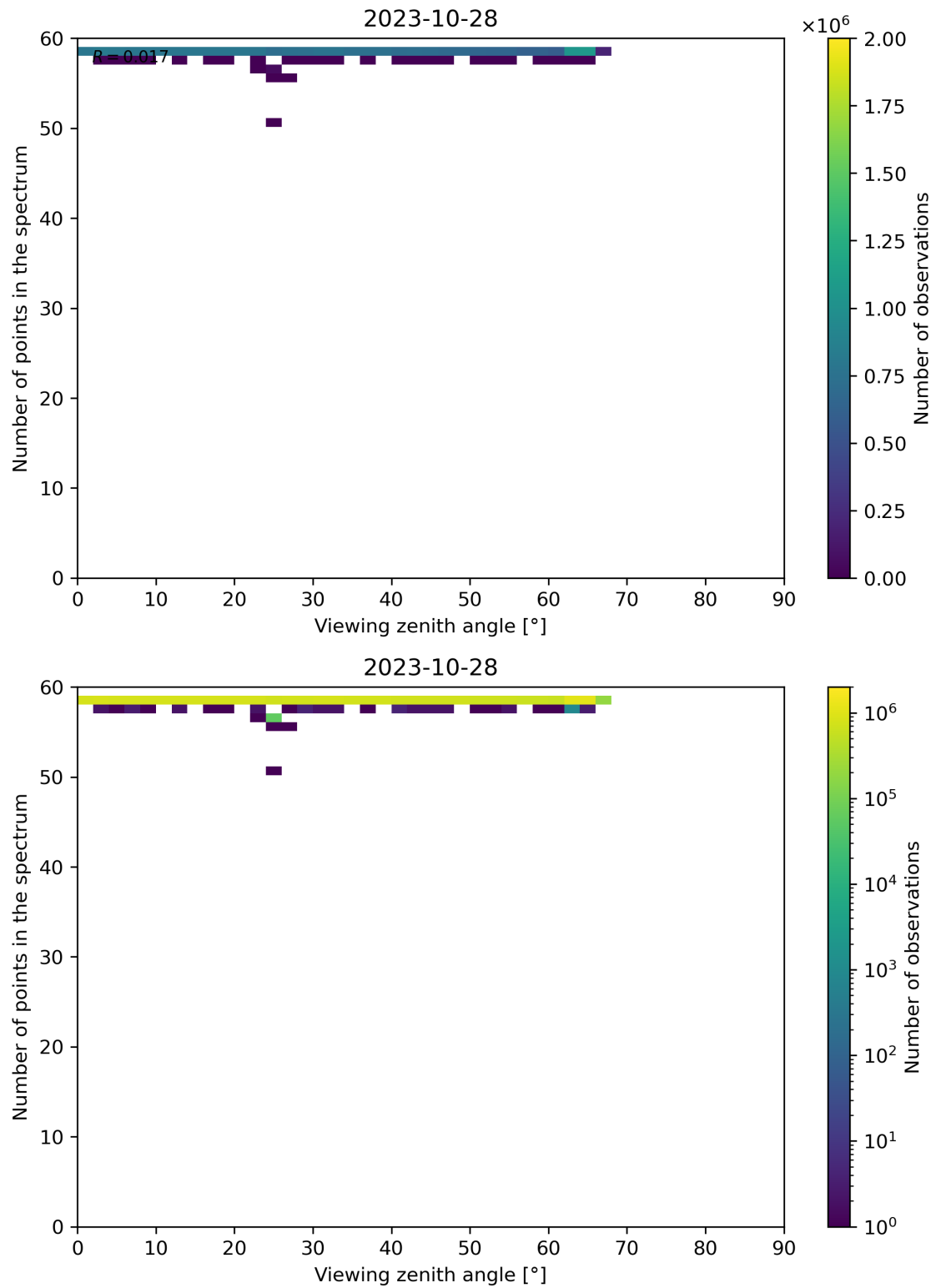
Figure 137: Scatter density plot of “Viewing zenith angle” against “Number of points in the spectrum” for 2023-10-28 to 2023-10-29.
