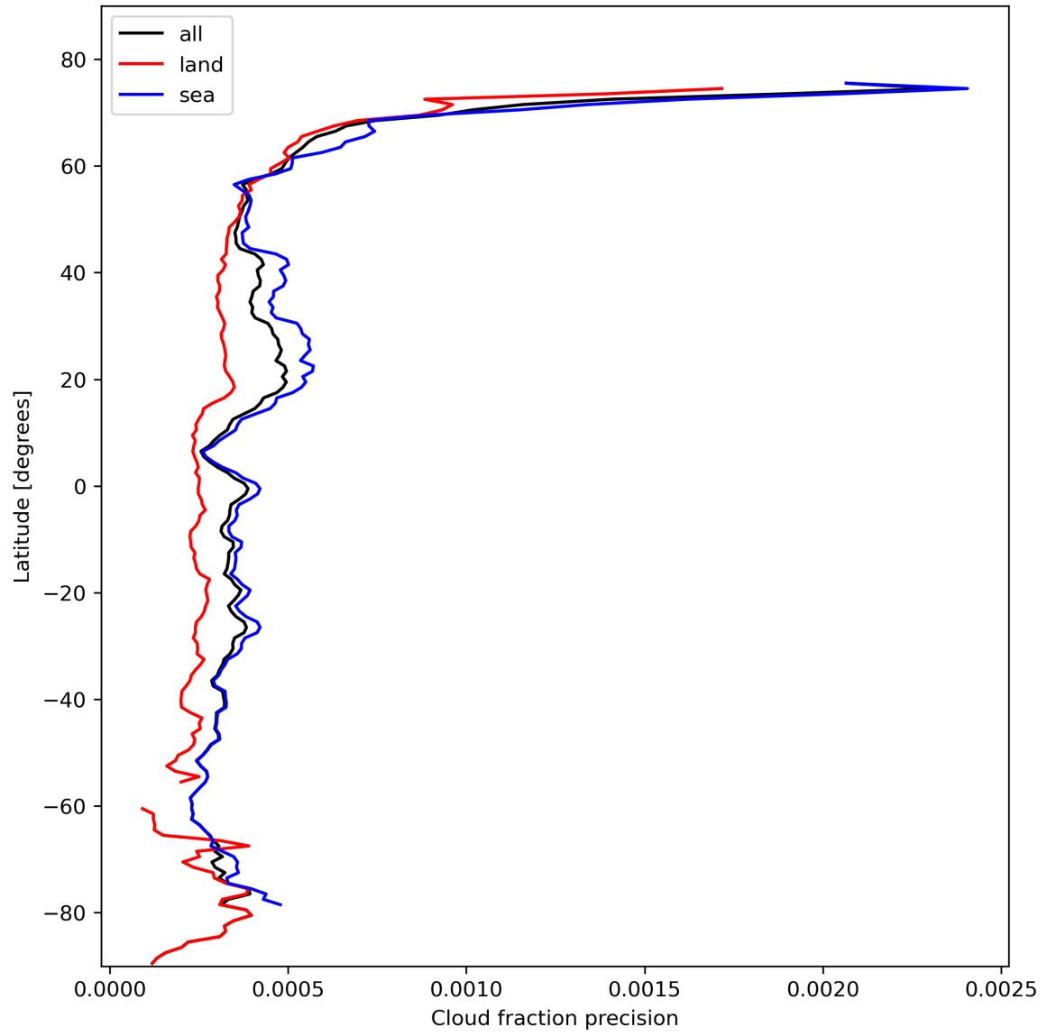
Figure 16: Zonal average of “Cloud fraction precision” for 2023-10-28 to 2023-10-29.
