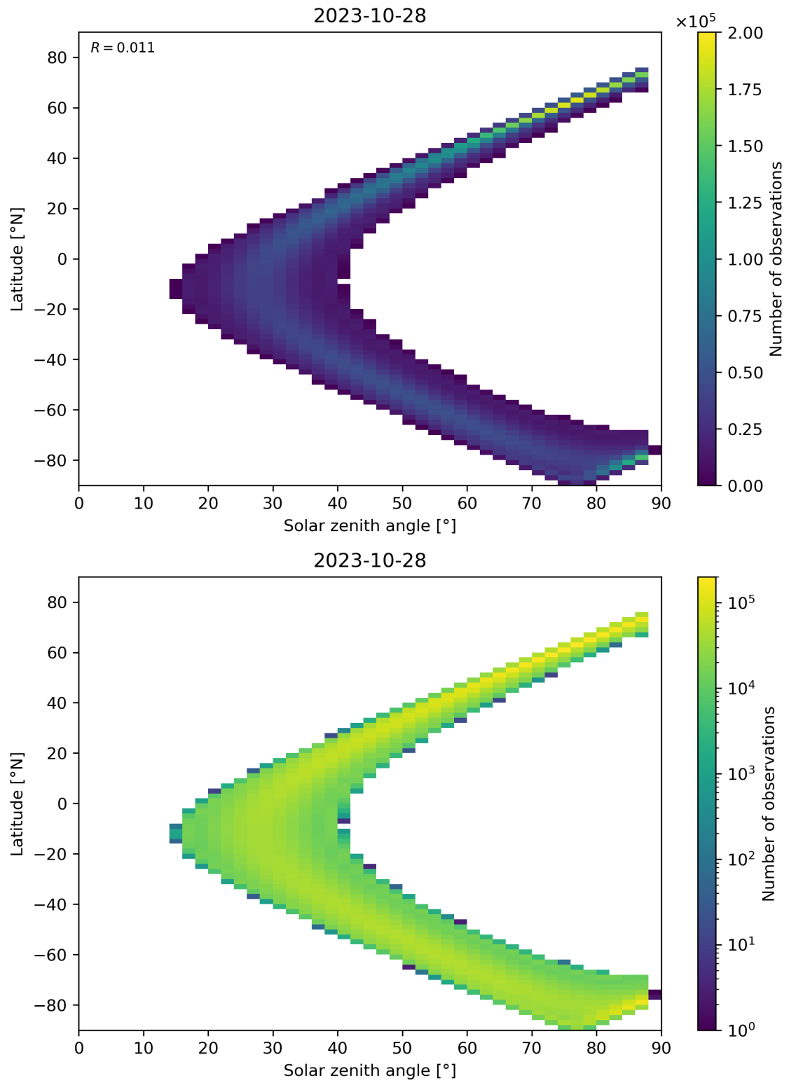
Figure 124: Scatter density plot of “Solar zenith angle” against “Latitude” for 2023-10-28 to 2023-10-29.
