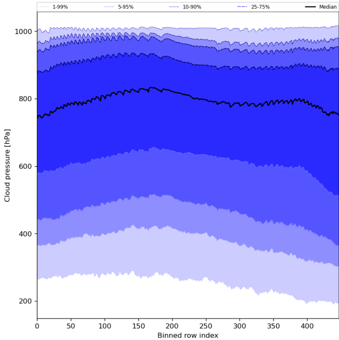
Figure 47: Along track statistics of “Cloud pressure” for 2023-10-28 to 2023-10-29
