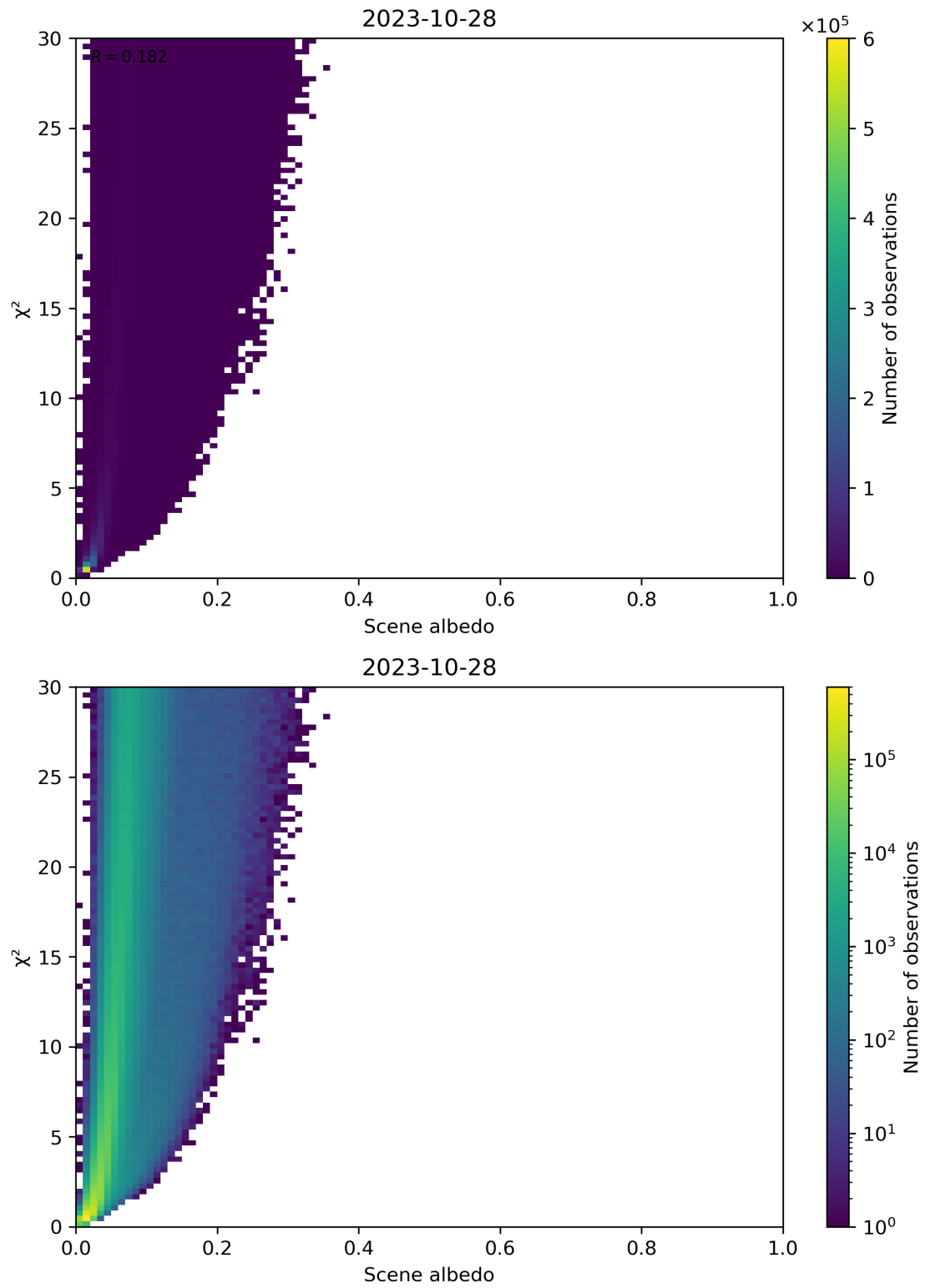
Figure 112: Scatter density plot of “Scene albedo” against “ \chi^2 ” for 2023-10-28 to 2023-10-29.
