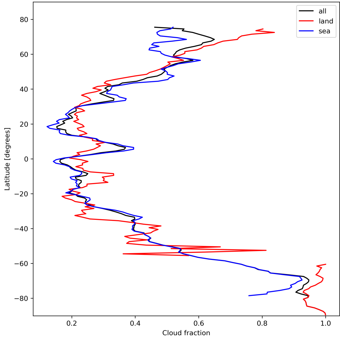
Figure 15: Zonal average of “Cloud fraction” for 2023-10-28 to 2023-10-29.
