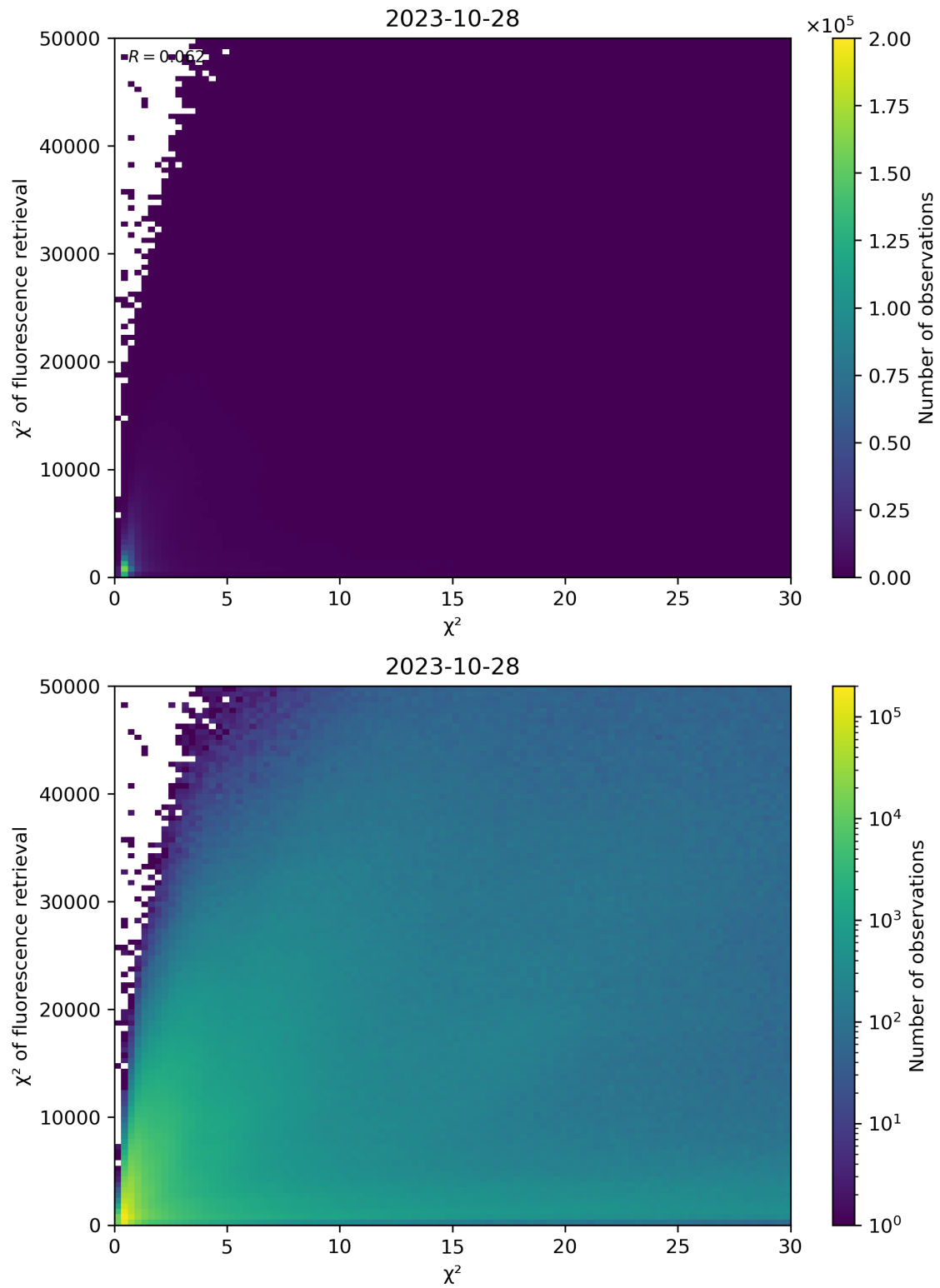
Figure 69: Scatter density plot of “ \chi^2 ” against “ \chi^2 of fluorescence retrieval” for 2023-10-28 to 2023-10-29.
