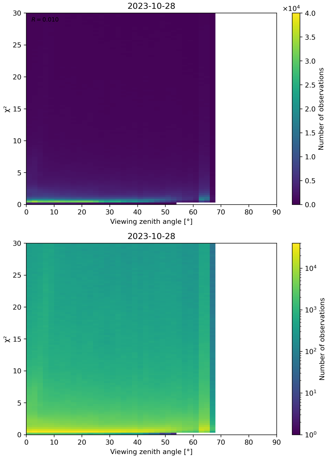
Figure 130: Scatter density plot of “Viewing zenith angle” against “ \chi^2 ” for 2023-10-28 to 2023-10-29.
