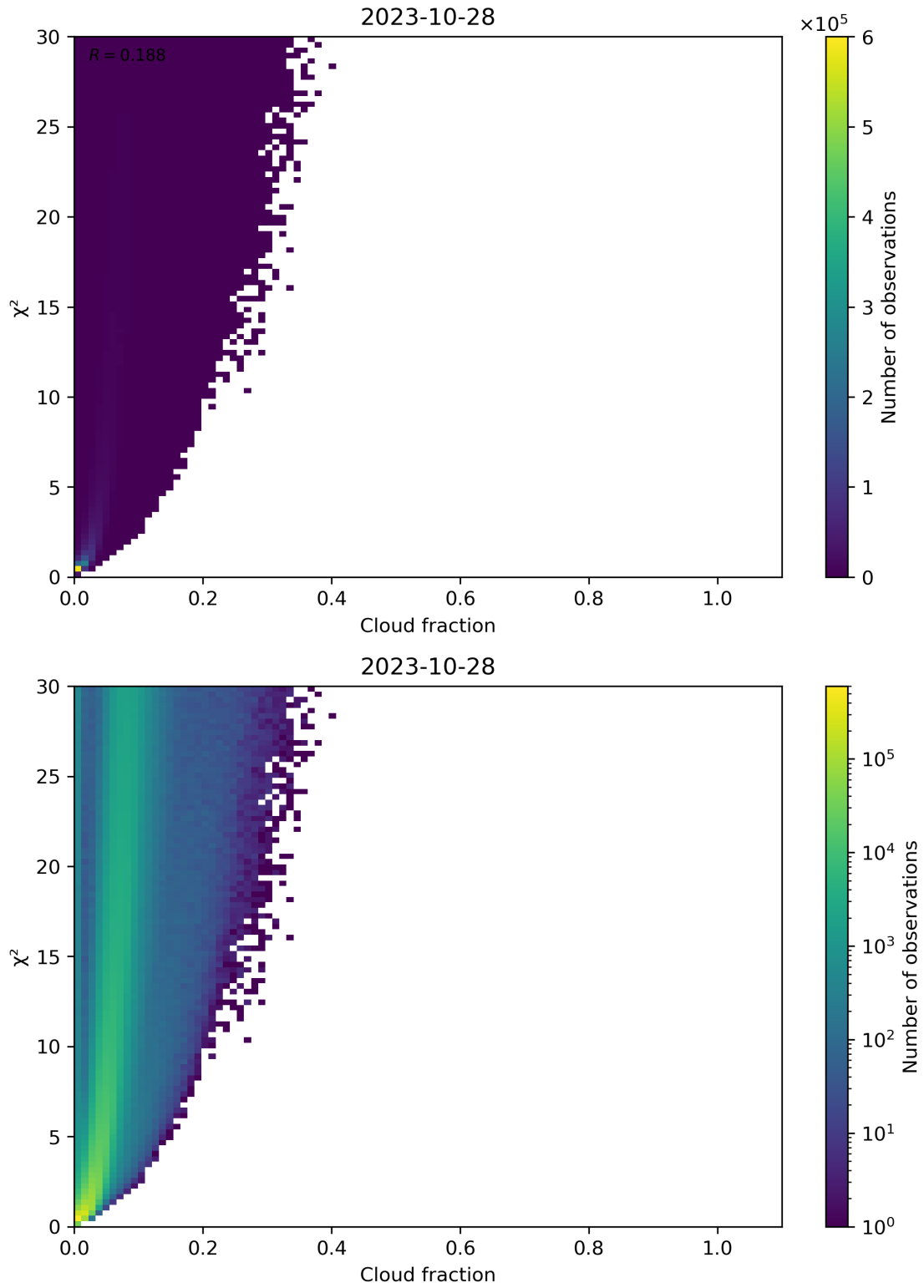
Figure 77: Scatter density plot of “Cloud fraction” against “ \chi^2 ” for 2023-10-28 to 2023-10-29.
