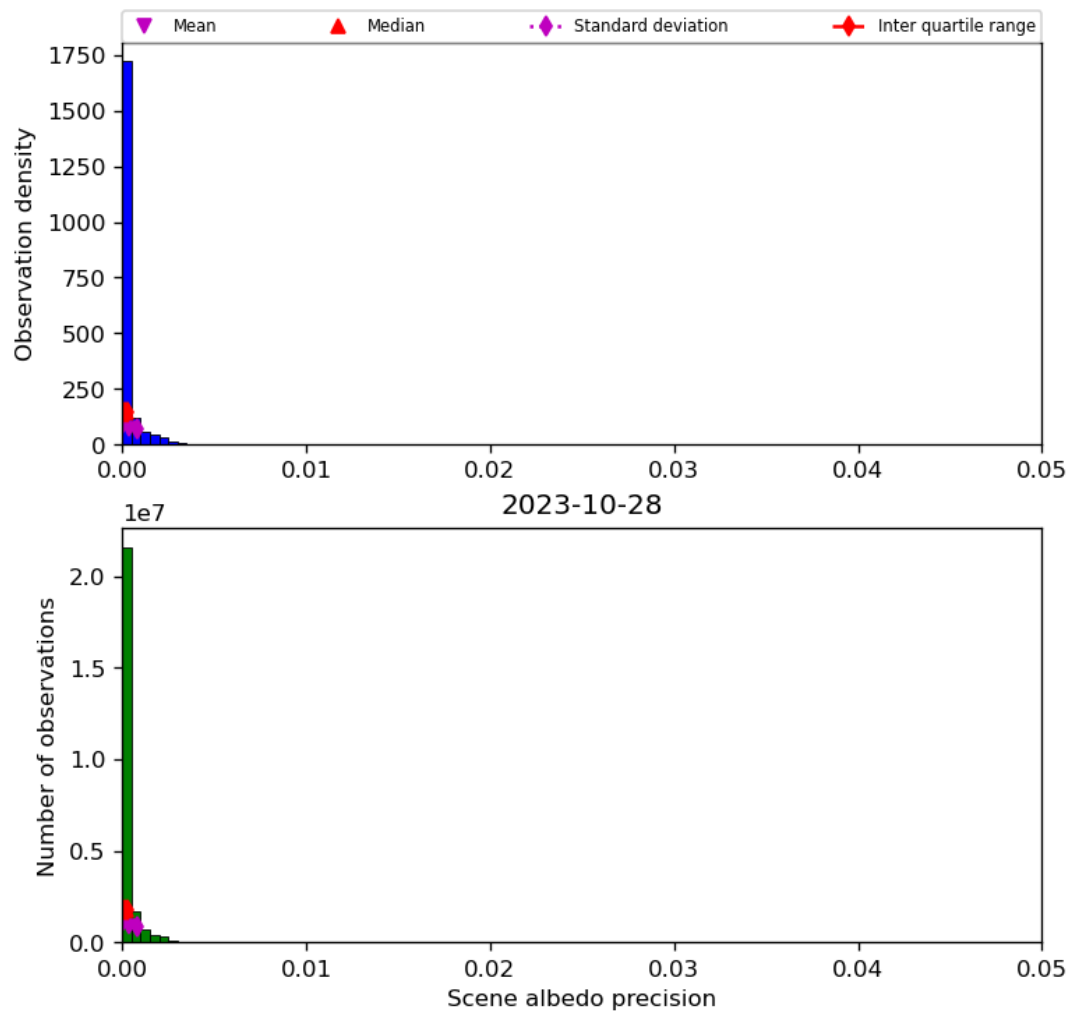
Figure 35: Histogram of “Scene albedo precision” for 2023-10-28 to 2023-10-29
