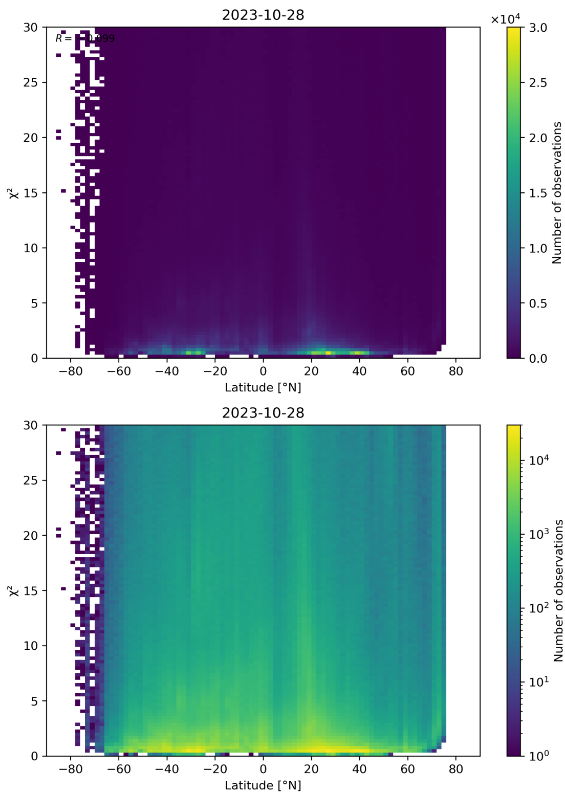
Figure 97: Scatter density plot of “Latitude” against “ \chi^2 ” for 2023-10-28 to 2023-10-29.
