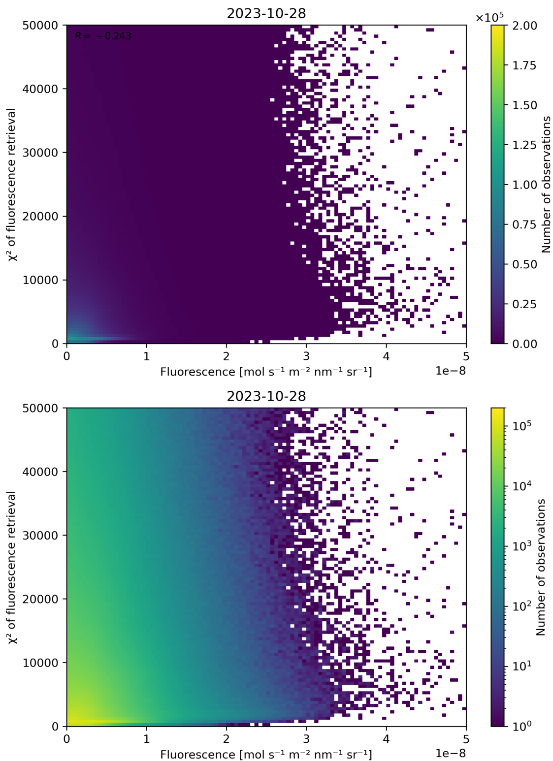
Figure 93: Scatter density plot of “Fluorescence” against “ \chi^2 of fluorescence retrieval” for 2023-10-28 to 2023-10-29.
