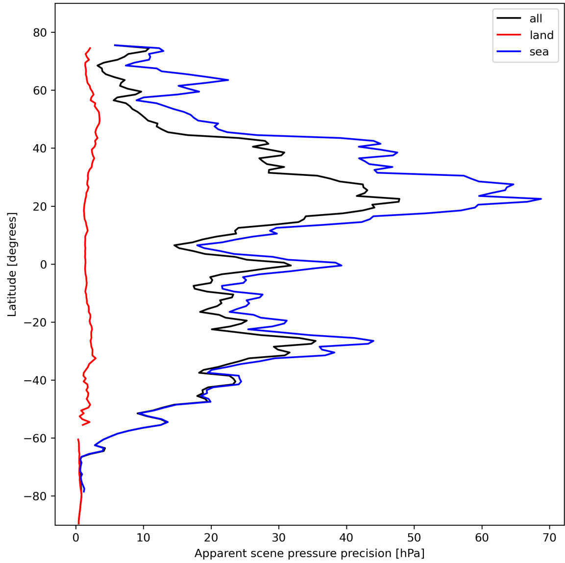
Figure 20: Zonal average of “Apparent scene pressure precision” for 2023-10-28 to 2023-10-29.
