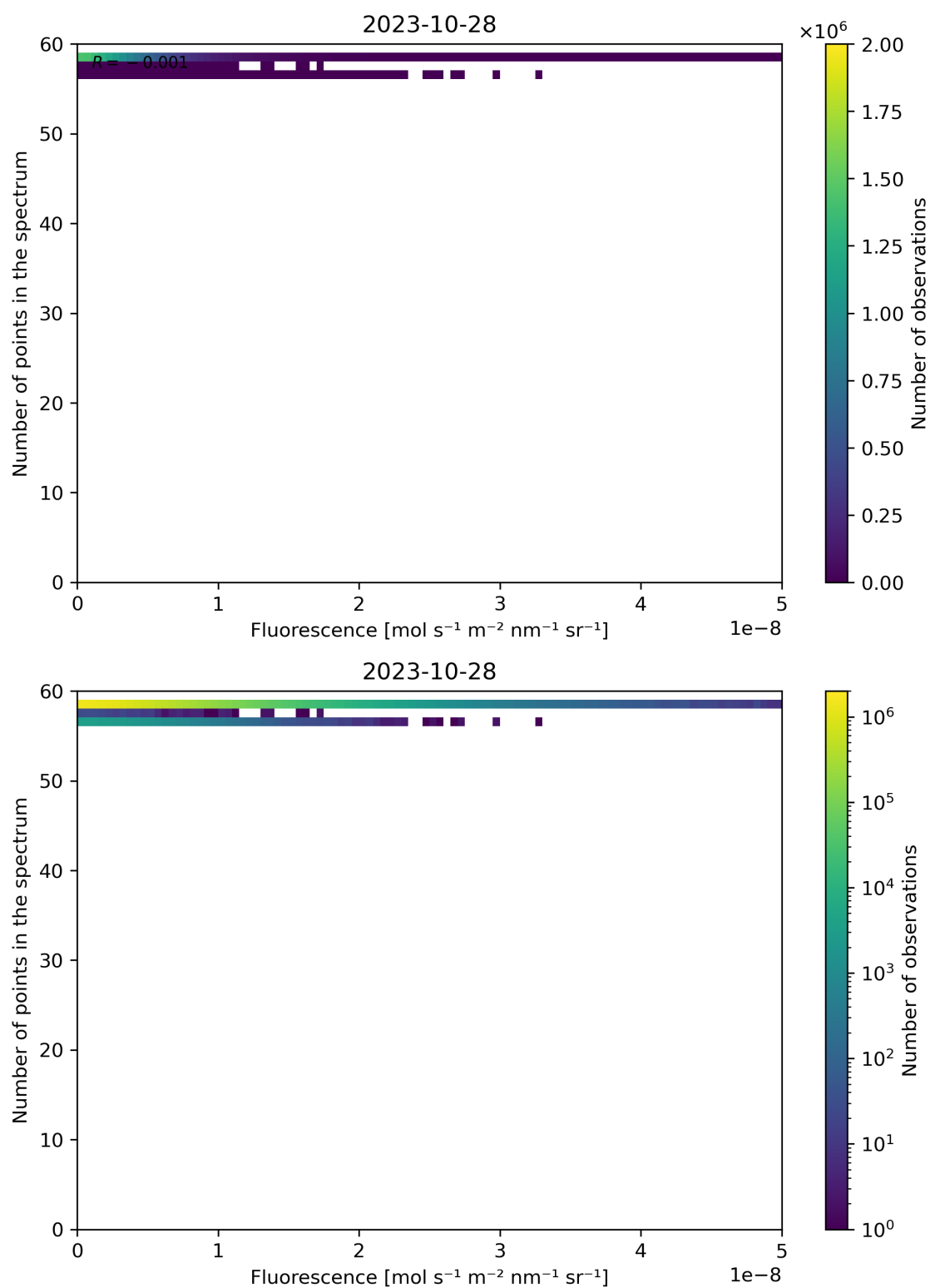
Figure 94: Scatter density plot of “Fluorescence” against “Number of points in the spectrum” for 2023-10-28 to 2023-10-29.
