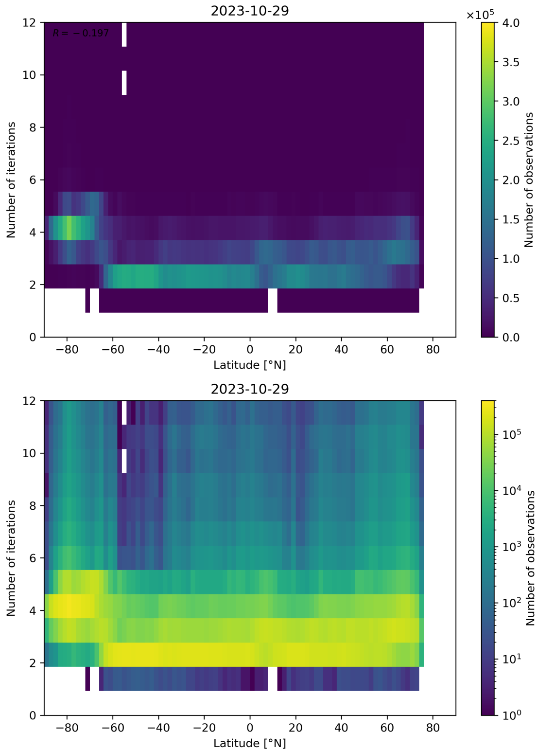
Figure 102: Scatter density plot of “Latitude” against “Number of iterations” for 2023-10-28 to 2023-10-30.
