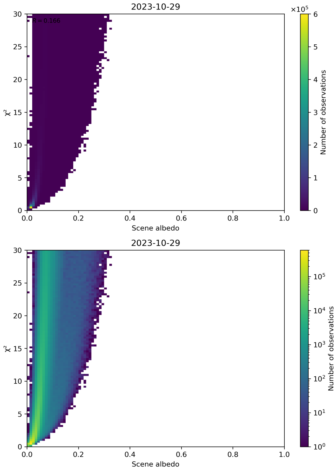
Figure 112: Scatter density plot of “Scene albedo” against “ \chi^2 ” for 2023-10-28 to 2023-10-30.
