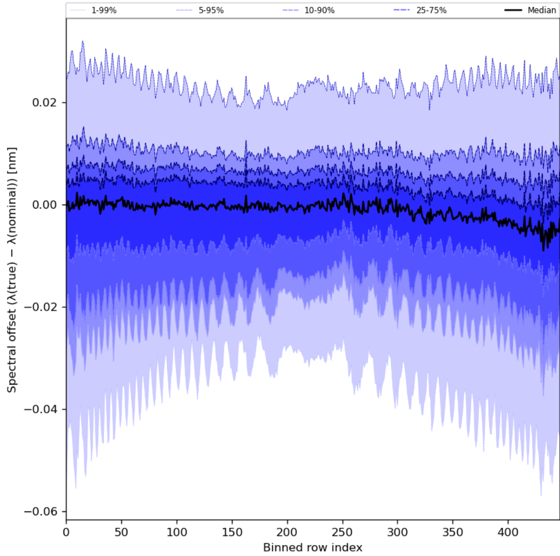
Figure 62: Along track statistics of “Spectral offset ( \lambda(\text{true}) - \lambda(\text{nominal}) )” for 2023-10-28 to 2023-10-30
