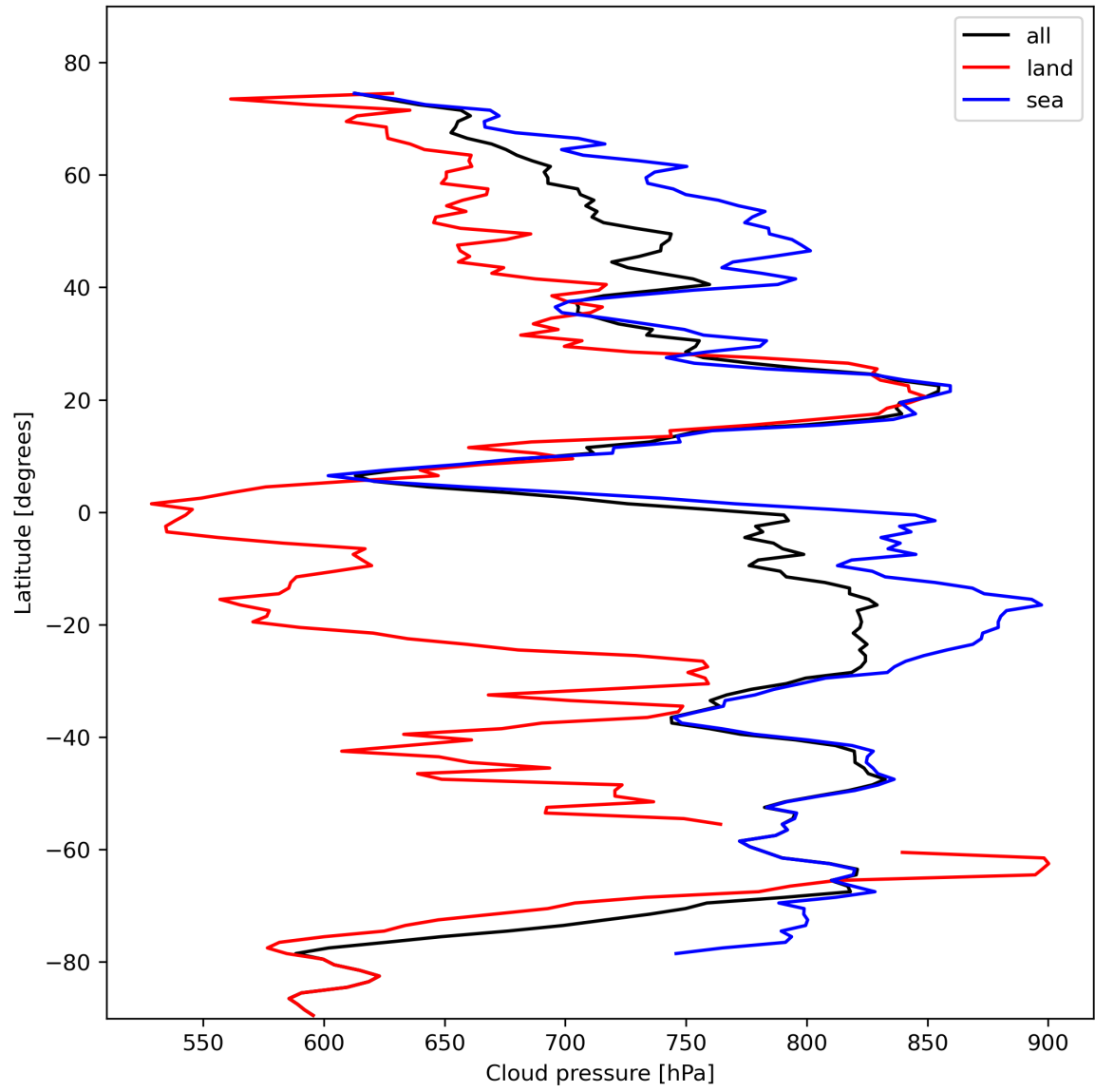
Figure 13: Zonal average of “Cloud pressure” for 2023-10-28 to 2023-10-30.
