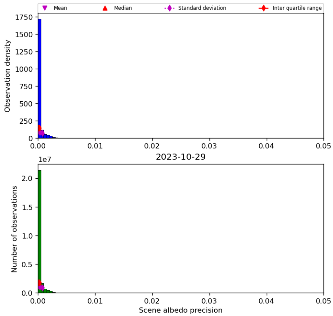
Figure 35: Histogram of “Scene albedo precision” for 2023-10-28 to 2023-10-30
