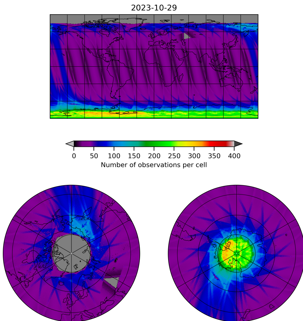
Figure 11: Map of the number of observations for 2023-10-28 to 2023-10-30
