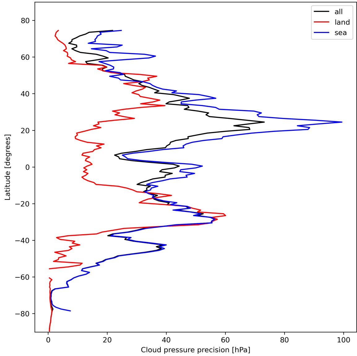
Figure 14: Zonal average of “Cloud pressure precision” for 2023-10-28 to 2023-10-30.
