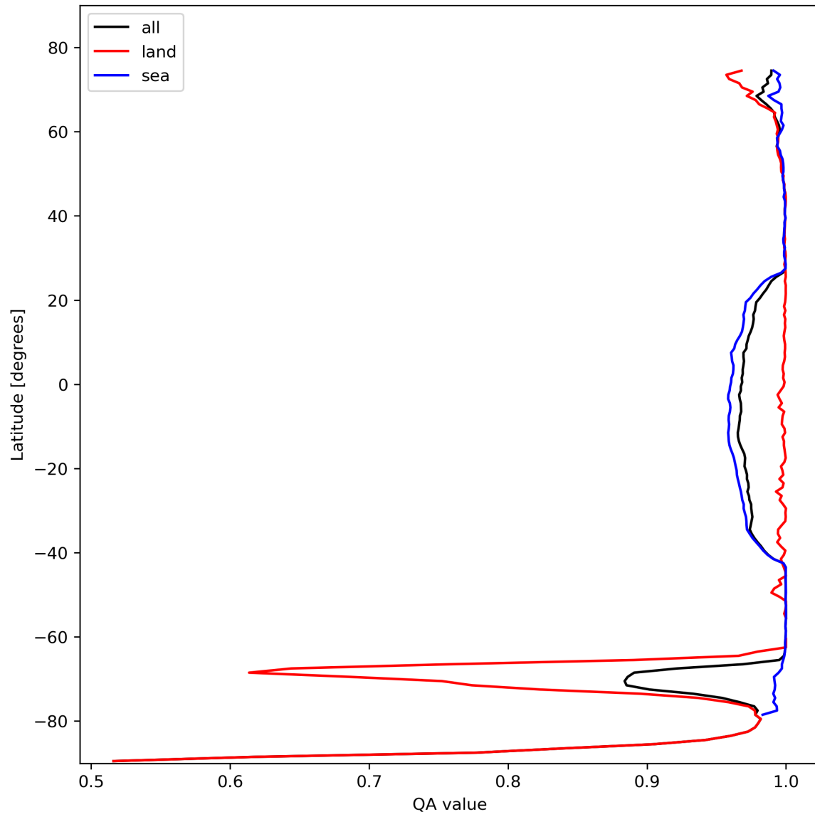
Figure 12: Zonal average of “QA value” for 2023-10-28 to 2023-10-30.
