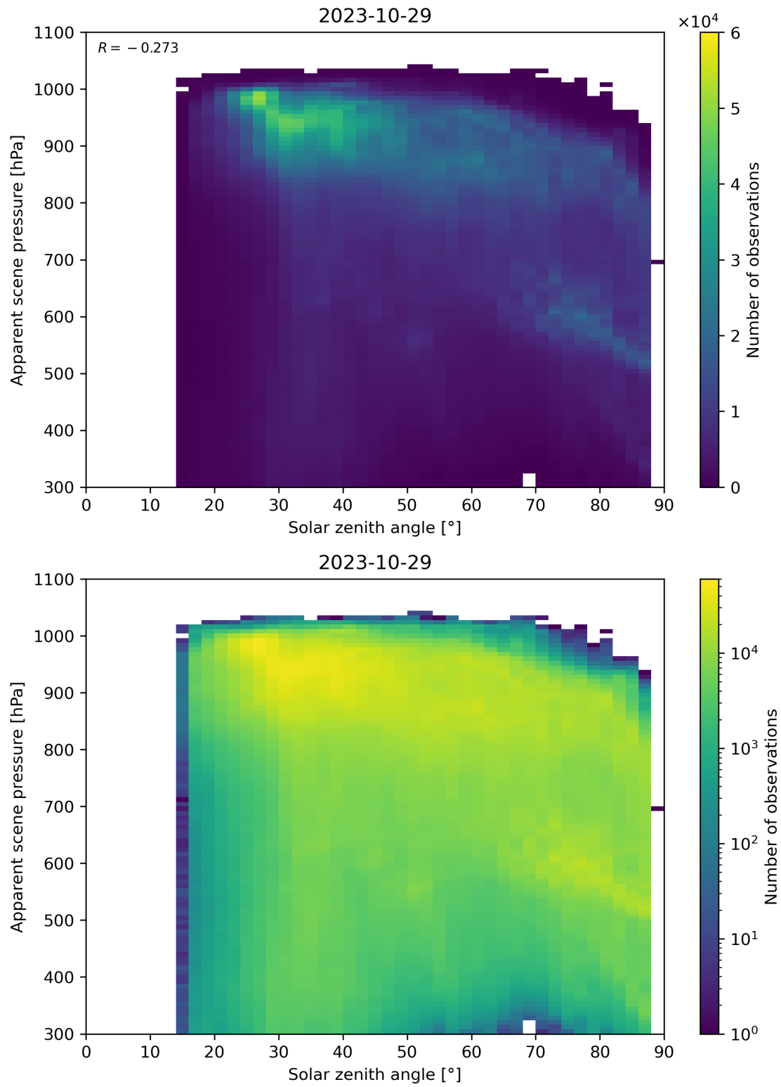
Figure 118: Scatter density plot of “Solar zenith angle” against “Apparent scene pressure” for 2023-10-28 to 2023-10-30.
