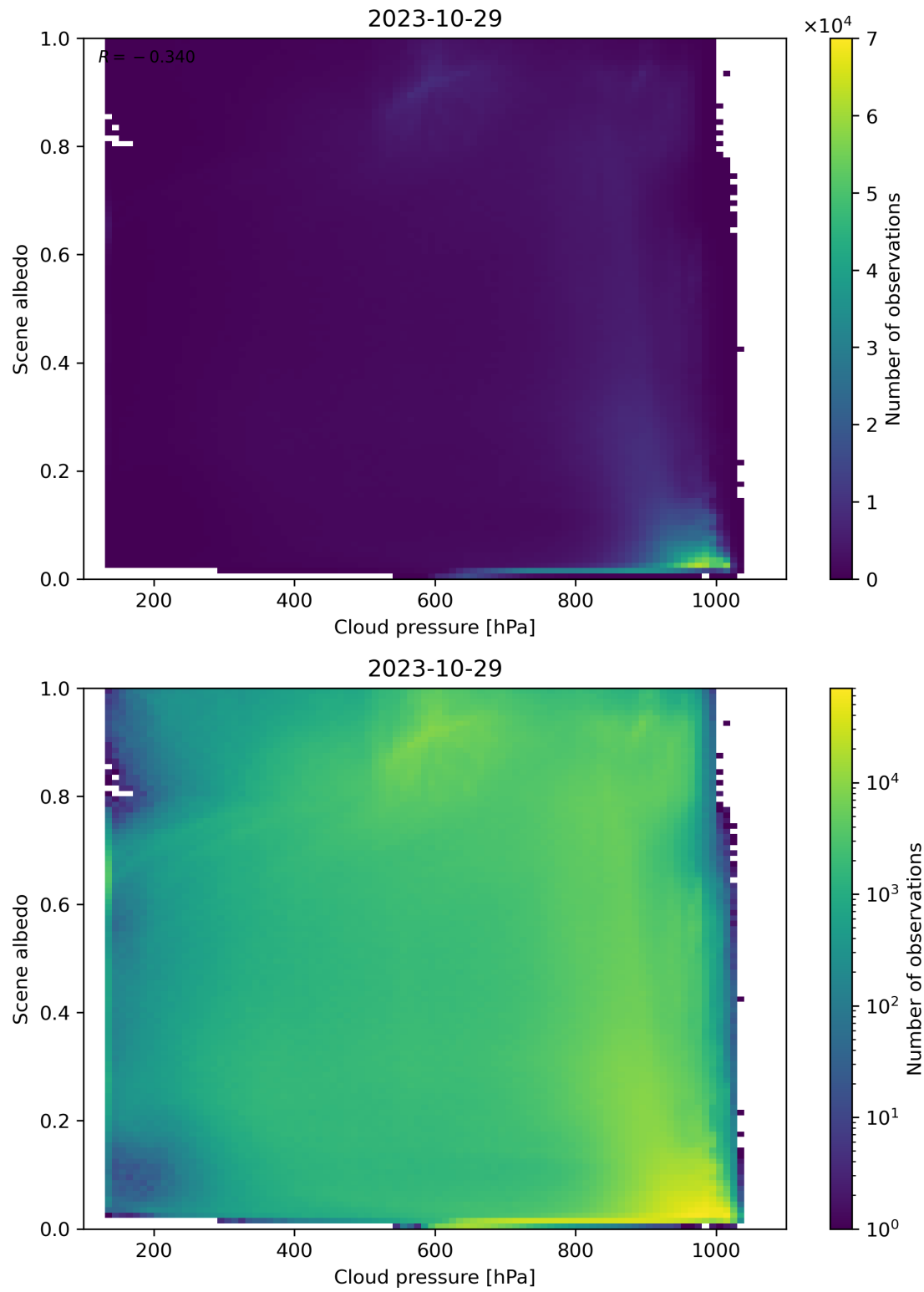
Figure 91: Scatter density plot of “Cloud pressure” against “Scene albedo” for 2023-10-28 to 2023-10-30.
