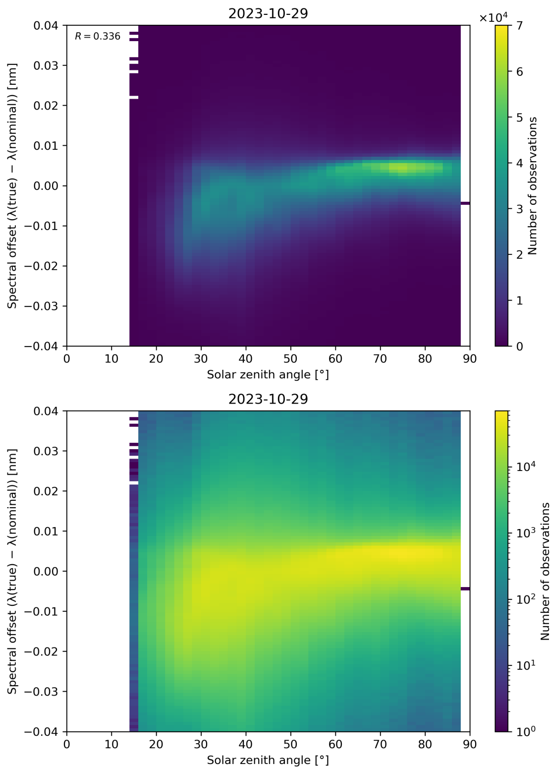
Figure 128: Scatter density plot of “Solar zenith angle” against “Spectral offset ( \lambda(\text{true}) - \lambda(\text{nominal}) )” for 2023-10-28 to 2023-10-30.
