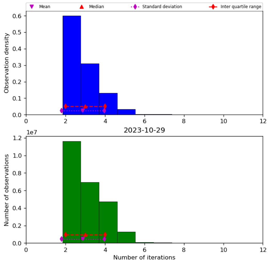
Figure 39: Histogram of “Number of iterations” for 2023-10-28 to 2023-10-30
