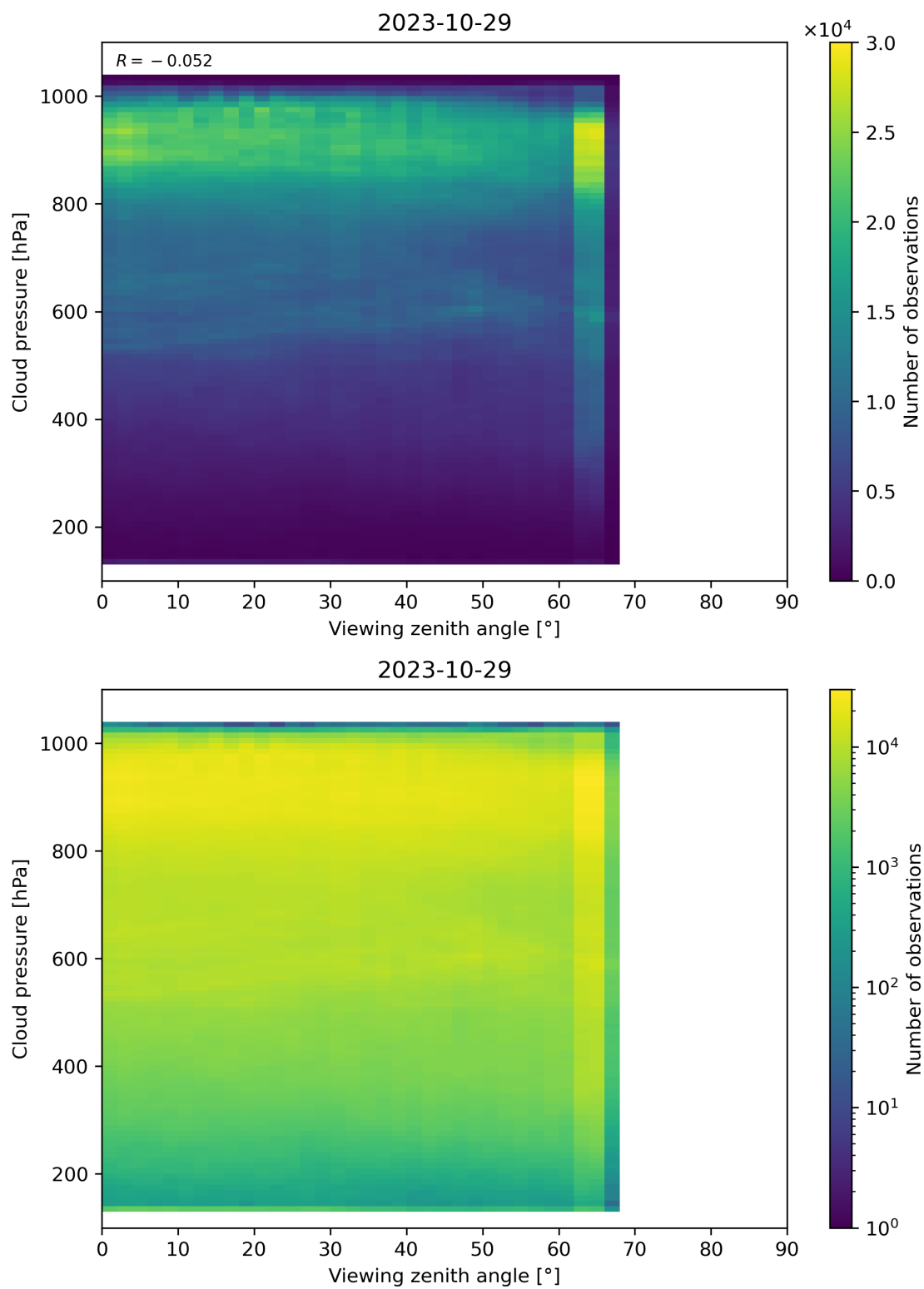
Figure 133: Scatter density plot of “Viewing zenith angle” against “Cloud pressure” for 2023-10-28 to 2023-10-30.
