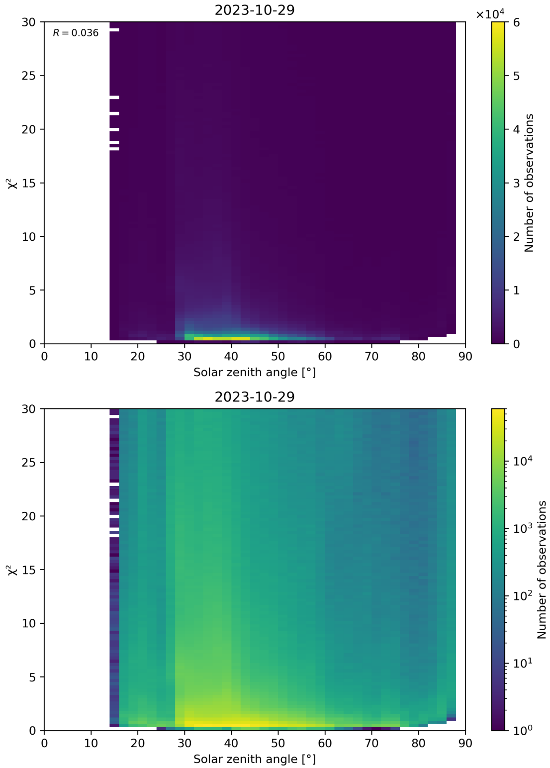
Figure 119: Scatter density plot of “Solar zenith angle” against “ \chi^2 ” for 2023-10-28 to 2023-10-30.
