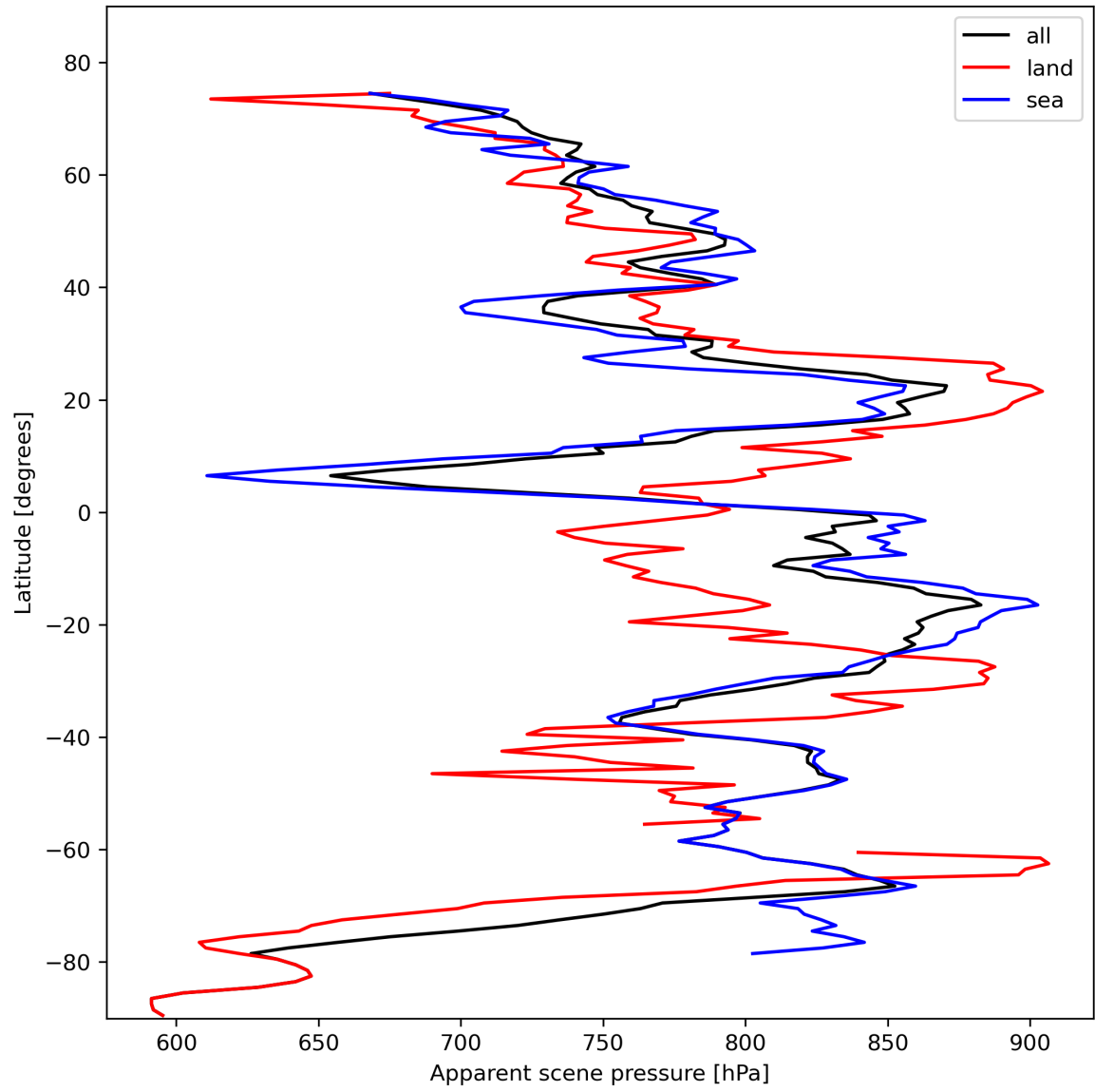
Figure 19: Zonal average of “Apparent scene pressure” for 2023-10-28 to 2023-10-30.
