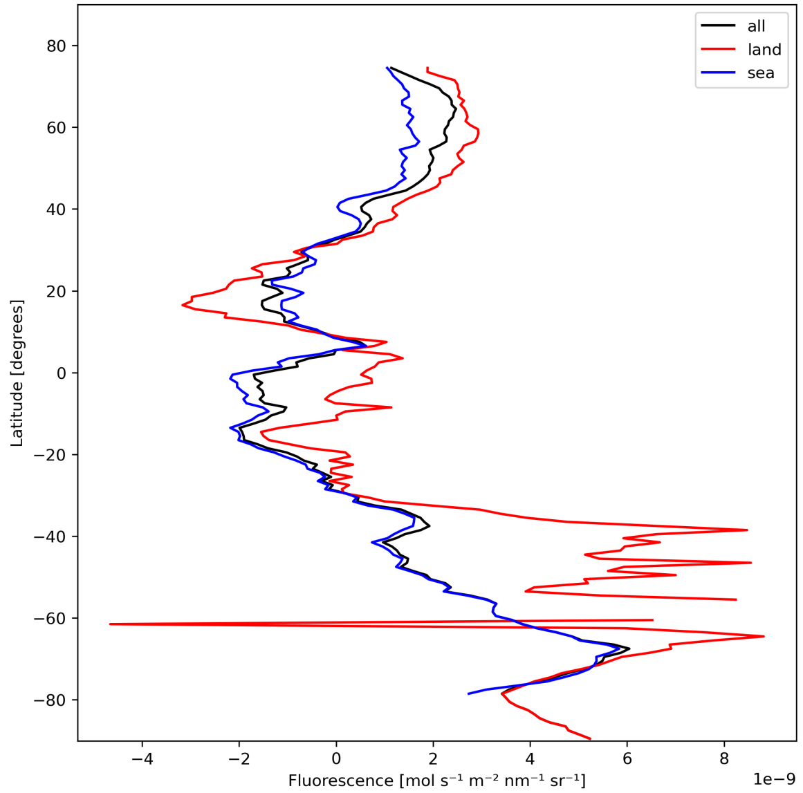
Figure 23: Zonal average of “Fluorescence” for 2023-10-28 to 2023-10-30.
