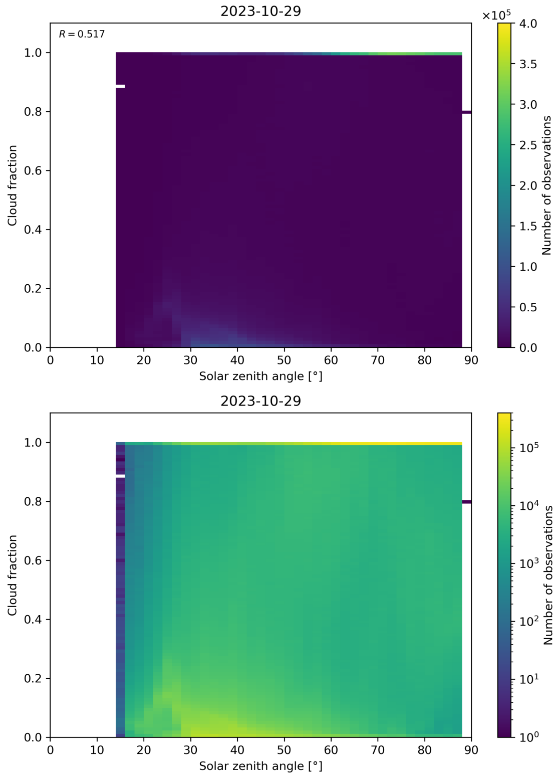
Figure 121: Scatter density plot of “Solar zenith angle” against “Cloud fraction” for 2023-10-28 to 2023-10-30.
