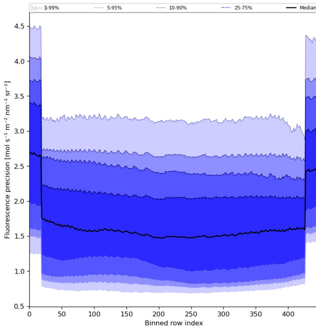
Figure 58: Along track statistics of “Fluorescence precision” for 2023-10-28 to 2023-10-30
