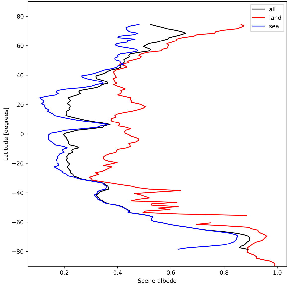
Figure 17: Zonal average of “Scene albedo” for 2023-10-28 to 2023-10-30.
