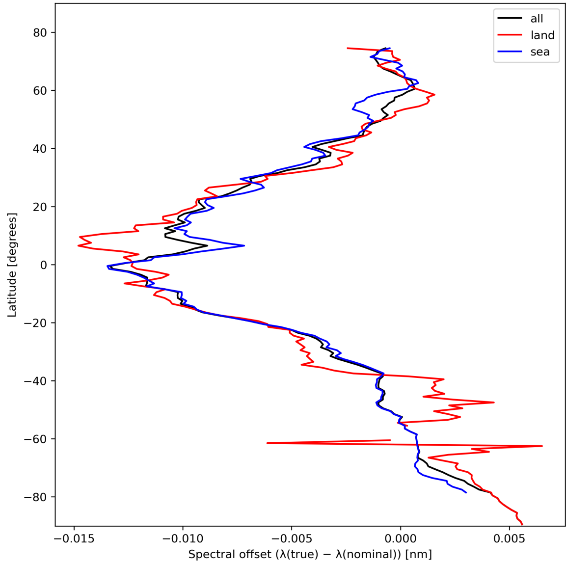
Figure 28: Zonal average of “Spectral offset ( \lambda(\text{true}) - \lambda(\text{nominal}) )” for 2023-10-28 to 2023-10-30.
