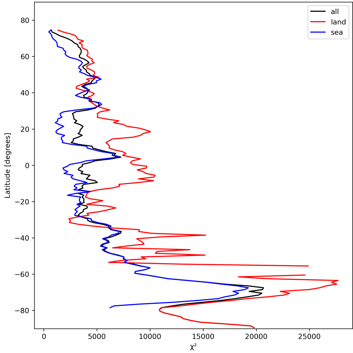
Figure 21: Zonal average of “ \chi^2 ” for 2023-10-28 to 2023-10-30.
