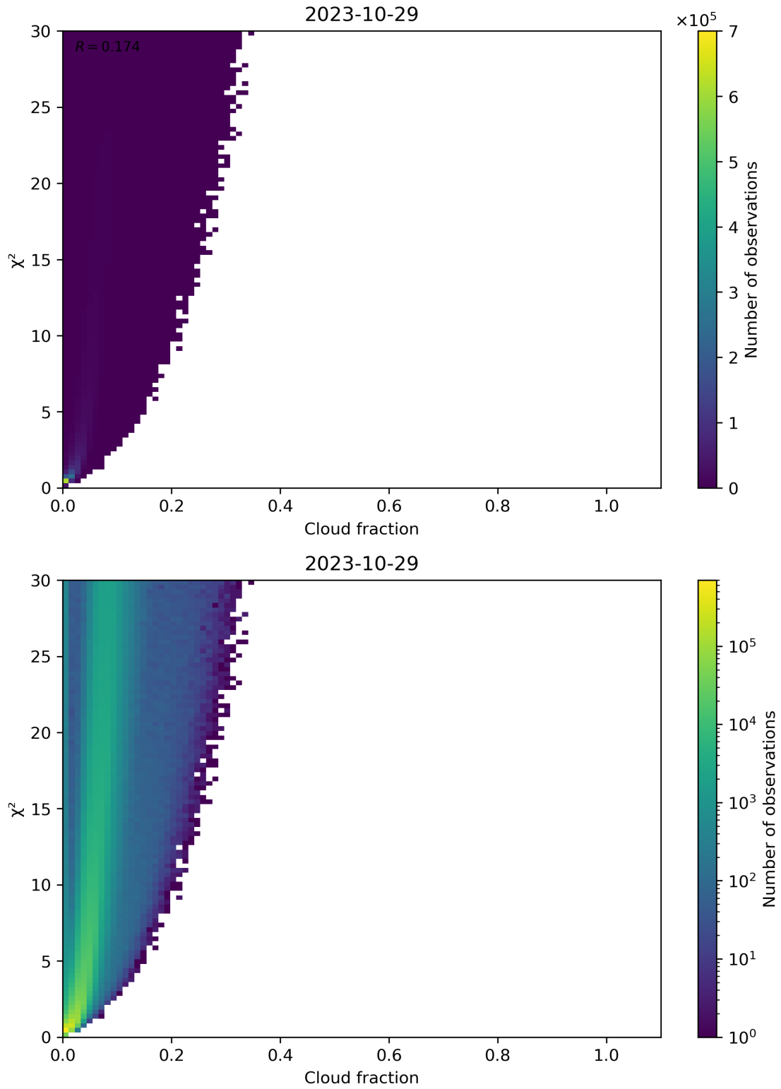
Figure 77: Scatter density plot of “Cloud fraction” against “ \chi^2 ” for 2023-10-28 to 2023-10-30.
