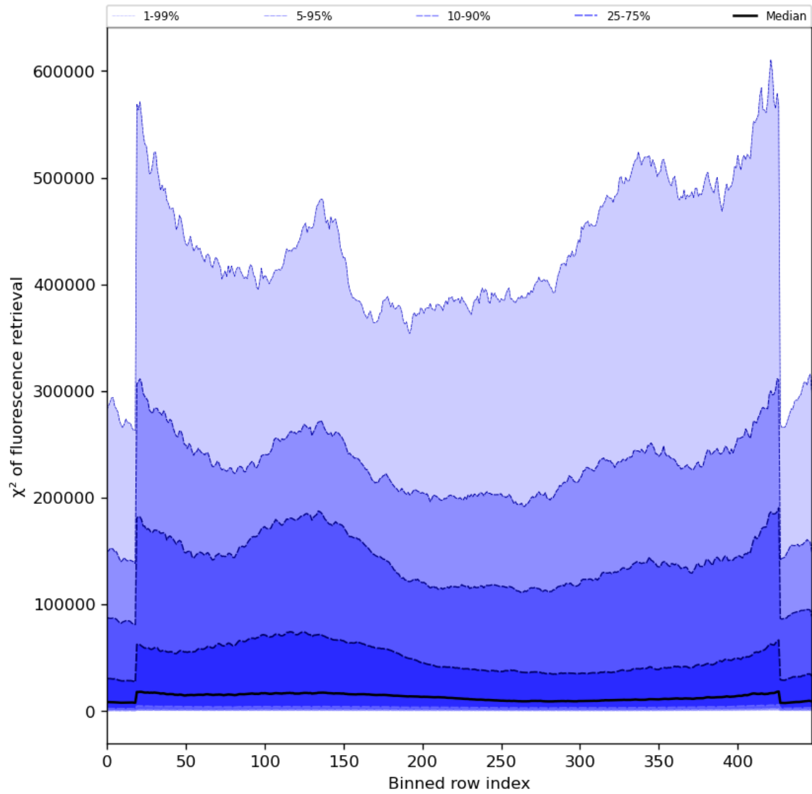
Figure 59: Along track statistics of “ \chi^2 of fluorescence retrieval” for 2023-10-28 to 2023-10-30
