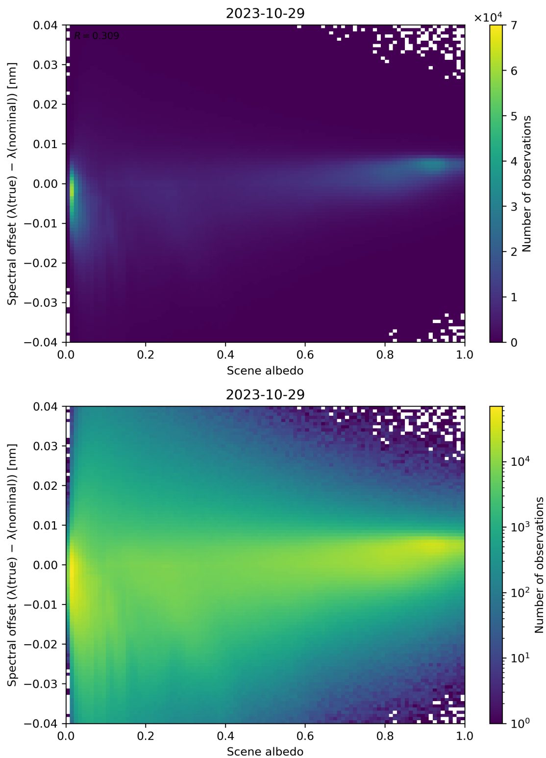
Figure 117: Scatter density plot of “Scene albedo” against “Spectral offset ( \lambda(\text{true}) - \lambda(\text{nominal}) )” for 2023-10-28 to 2023-10-30.
