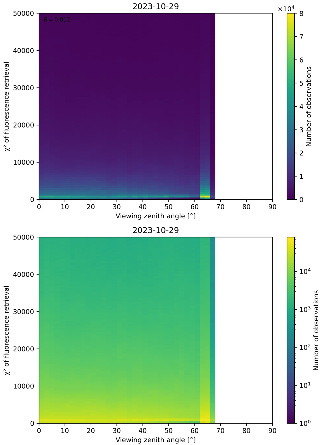
Figure 131: Scatter density plot of “Viewing zenith angle” against “ \chi^2 of fluorescence retrieval” for 2023-10-28 to 2023-10-30.
