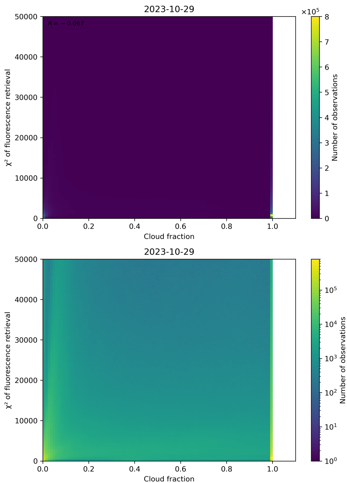
Figure 78: Scatter density plot of “Cloud fraction” against “ \chi^2 of fluorescence retrieval” for 2023-10-28 to 2023-10-30.
