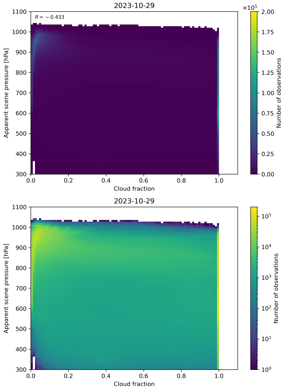
Figure 76: Scatter density plot of “Cloud fraction” against “Apparent scene pressure” for 2023-10-28 to 2023-10-30.
