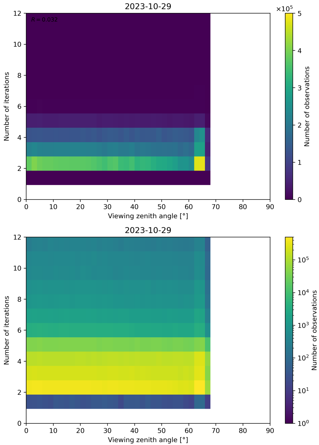
Figure 136: Scatter density plot of “Viewing zenith angle” against “Number of iterations” for 2023-10-28 to 2023-10-30.
