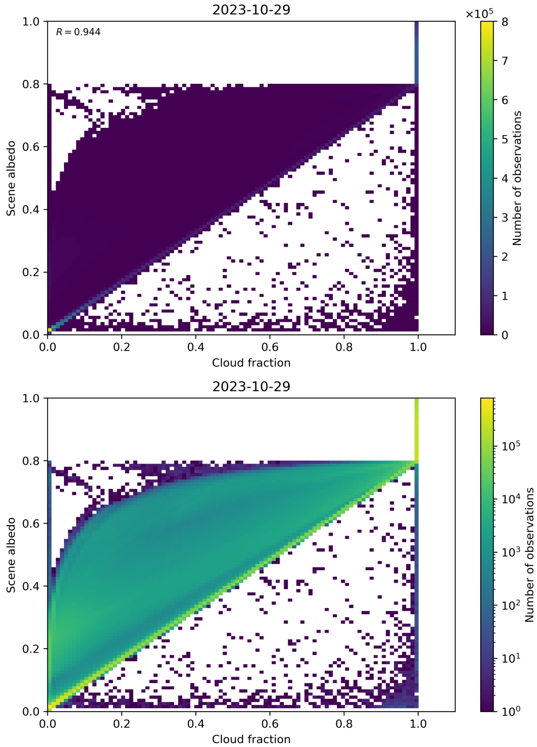
Figure 82: Scatter density plot of “Cloud fraction” against “Scene albedo” for 2023-10-28 to 2023-10-30.
