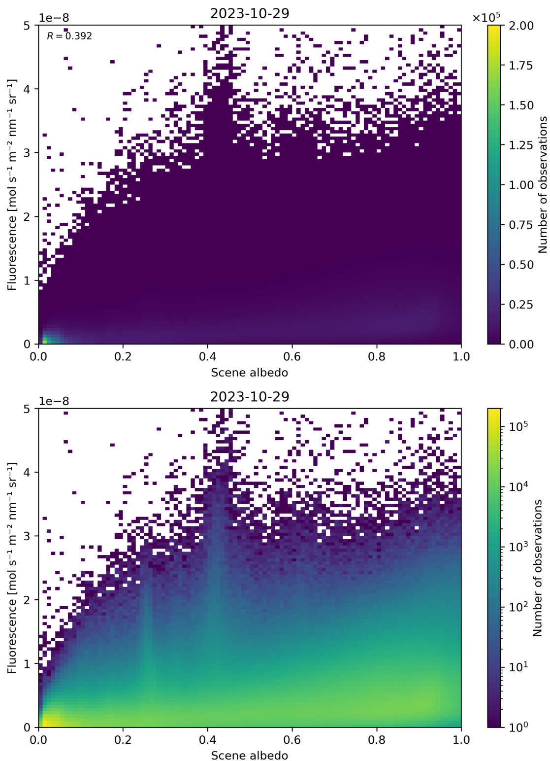
Figure 114: Scatter density plot of “Scene albedo” against “Fluorescence” for 2023-10-28 to 2023-10-30.
