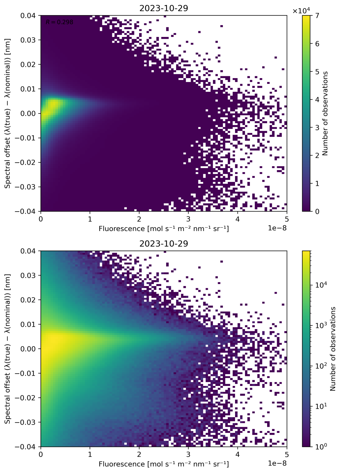
Figure 95: Scatter density plot of “Fluorescence” against “Spectral offset ( \lambda(\text{true}) - \lambda(\text{nominal}) )” for 2023-10-28 to 2023-10-30.
