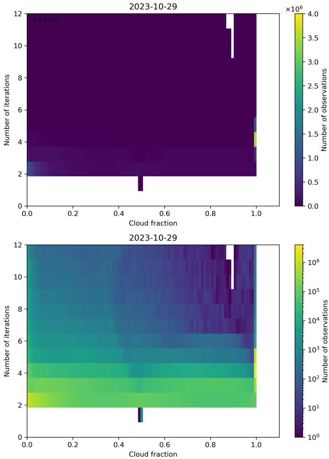
Figure 80: Scatter density plot of “Cloud fraction” against “Number of iterations” for 2023-10-28 to 2023-10-30.
