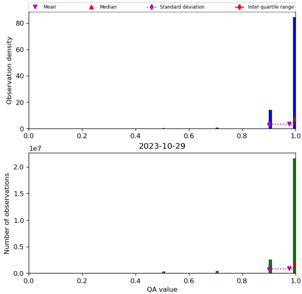
Figure 29: Histogram of “QA value” for 2023-10-28 to 2023-10-30
