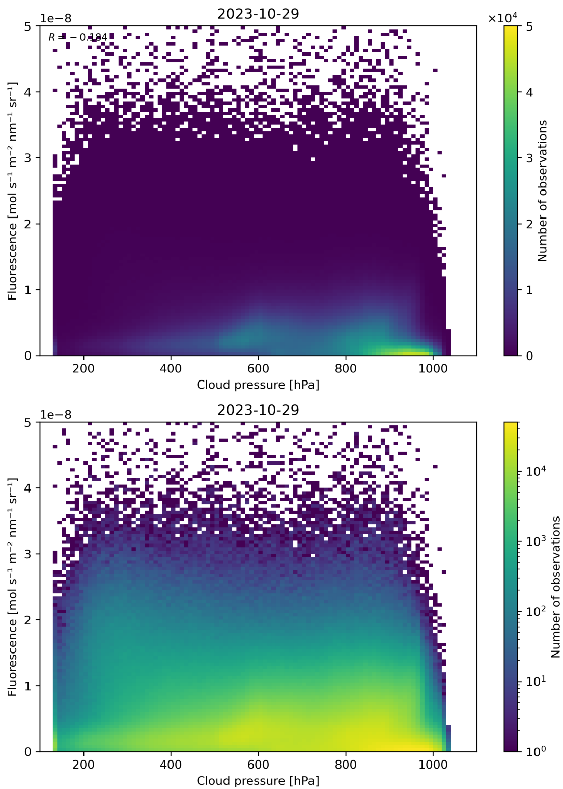
Figure 88: Scatter density plot of “Cloud pressure” against “Fluorescence” for 2023-10-28 to 2023-10-30.
