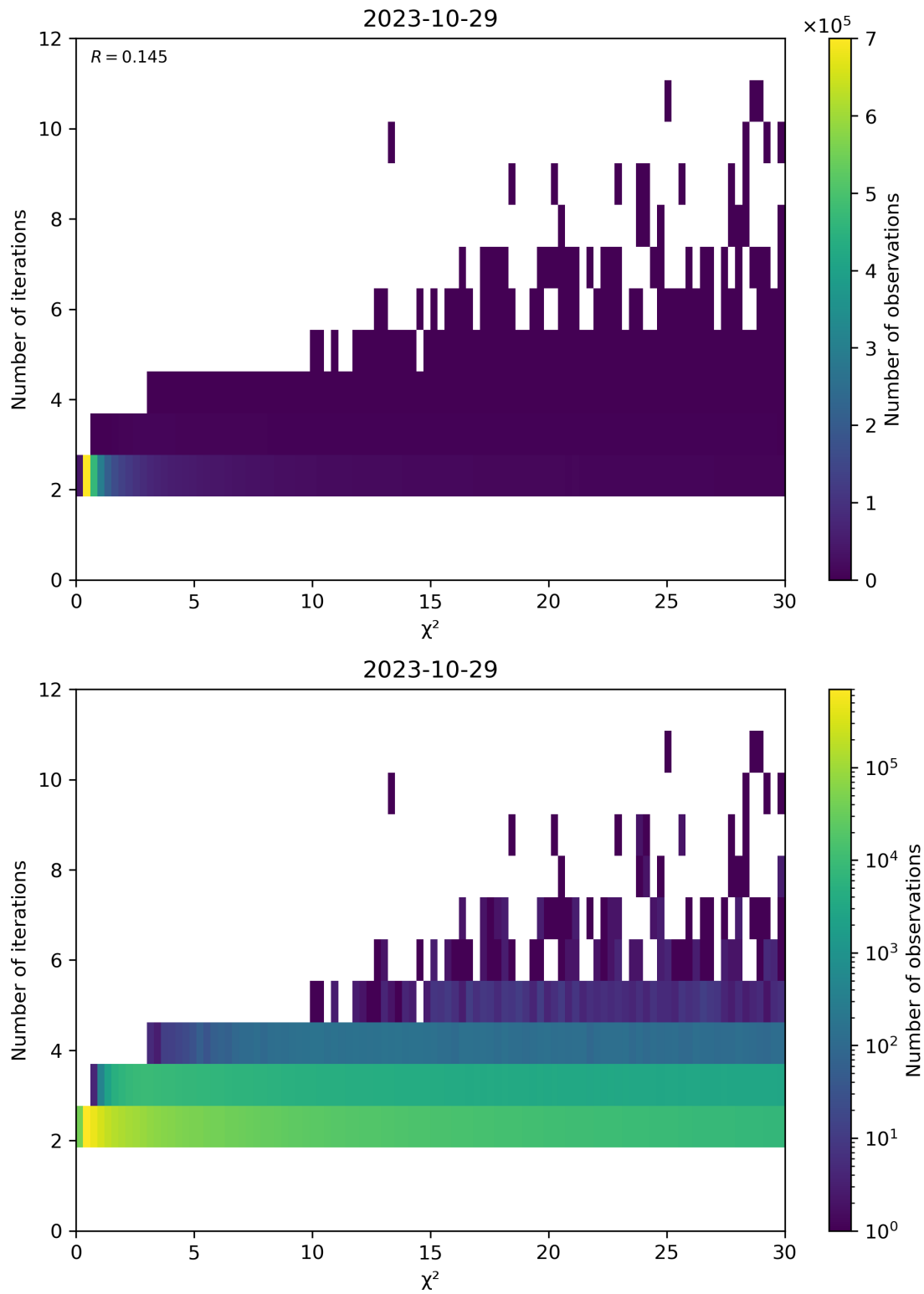
Figure 73: Scatter density plot of “ \chi^2 ” against “Number of iterations” for 2023-10-28 to 2023-10-30.
