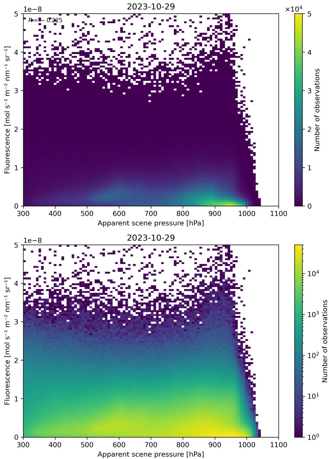
Figure 65: Scatter density plot of “Apparent scene pressure” against “Fluorescence” for 2023-10-28 to 2023-10-30.
