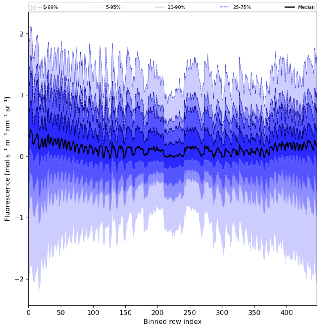
Figure 57: Along track statistics of “Fluorescence” for 2023-10-28 to 2023-10-30
