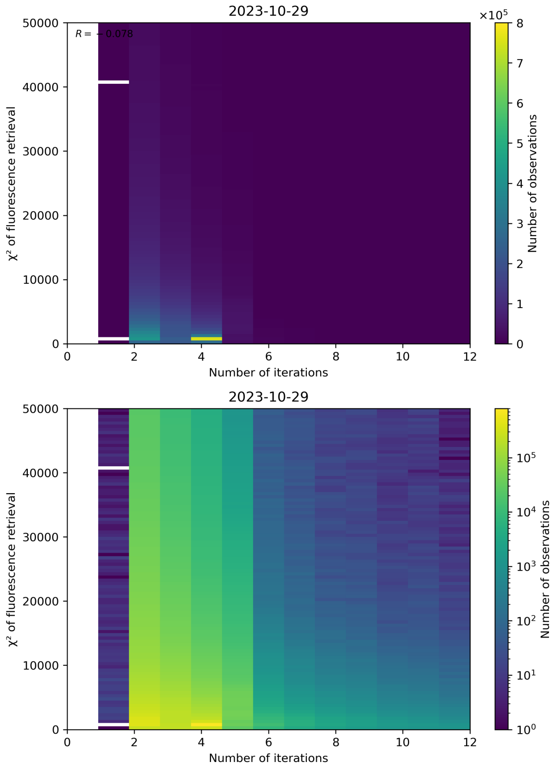
Figure 106: Scatter density plot of “Number of iterations” against “ \chi^2 of fluorescence retrieval” for 2023-10-28 to 2023-10-30.
