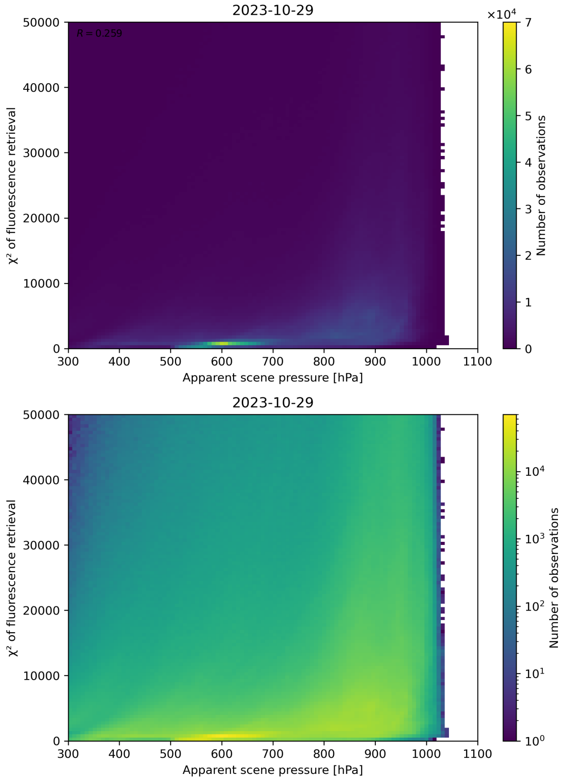
Figure 64: Scatter density plot of “Apparent scene pressure” against “ \chi^2 of fluorescence retrieval” for 2023-10-28 to 2023-10-30.
