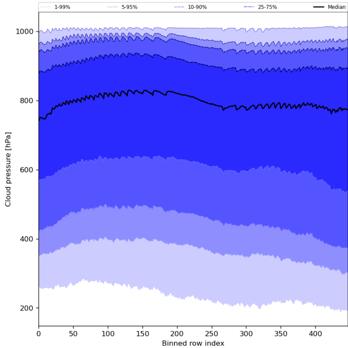
Figure 47: Along track statistics of “Cloud pressure” for 2023-10-28 to 2023-10-30
