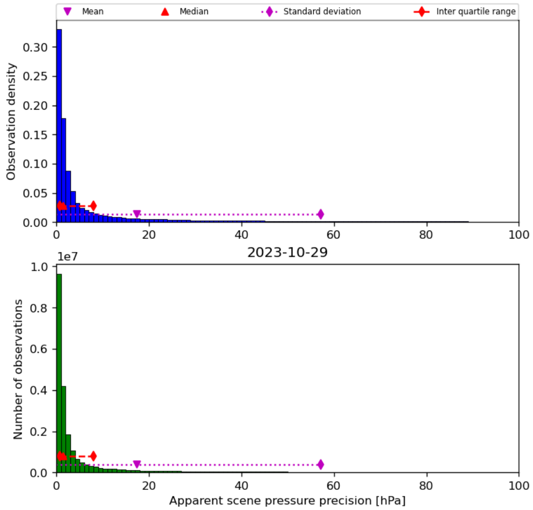
Figure 37: Histogram of “Apparent scene pressure precision” for 2023-10-28 to 2023-10-30
