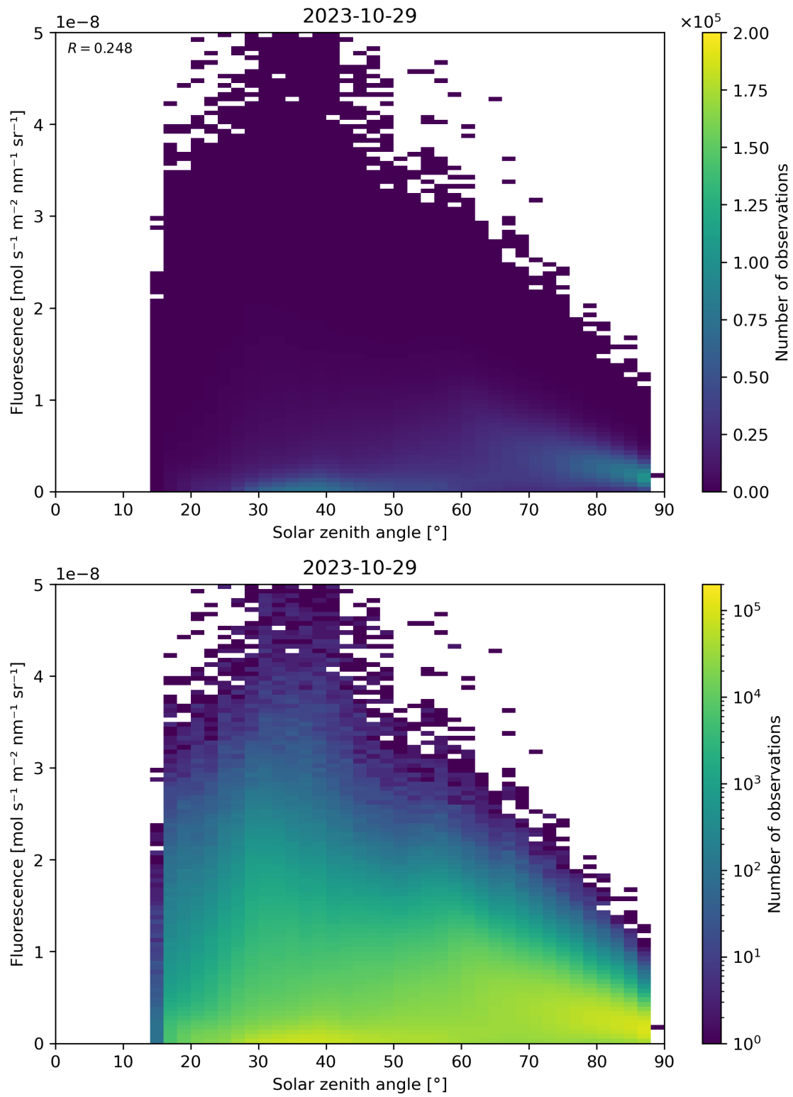
Figure 123: Scatter density plot of “Solar zenith angle” against “Fluorescence” for 2023-10-28 to 2023-10-30.
