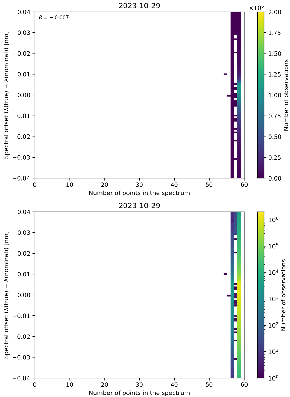
Figure 110: Scatter density plot of “Number of points in the spectrum” against “Spectral offset ( \lambda(\text{true}) - \lambda(\text{nominal}) )” for 2023-10-28 to 2023-10-30.
