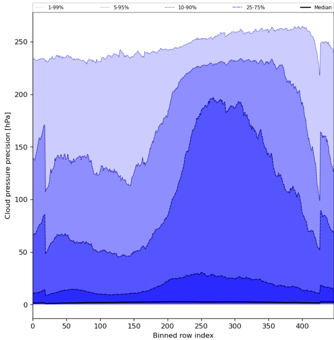
Figure 48: Along track statistics of “Cloud pressure precision” for 2023-10-28 to 2023-10-30
