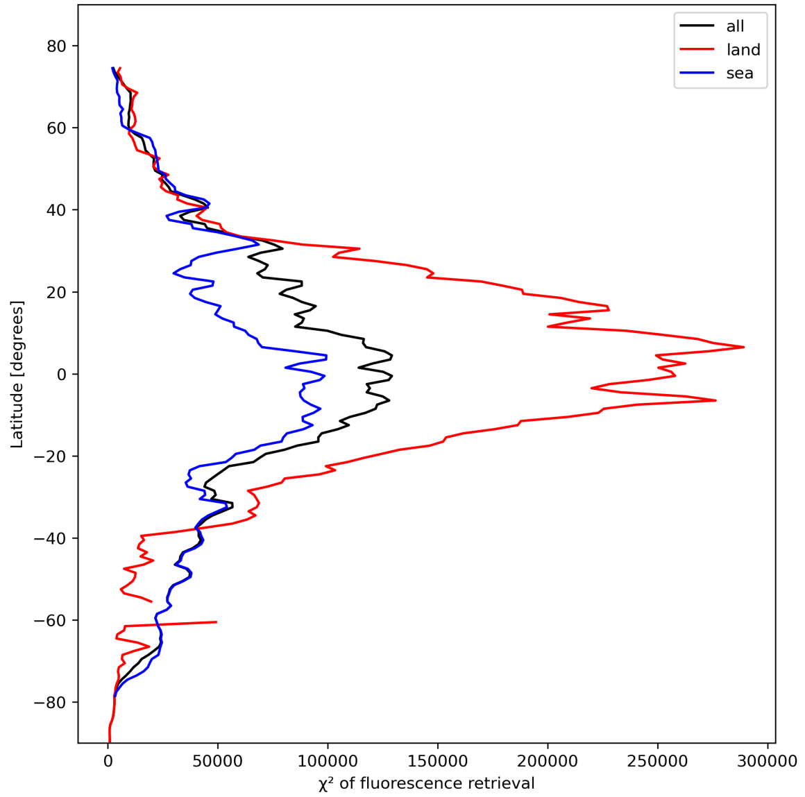
Figure 25: Zonal average of “ \chi^2 of fluorescence retrieval” for 2023-10-28 to 2023-10-30.
