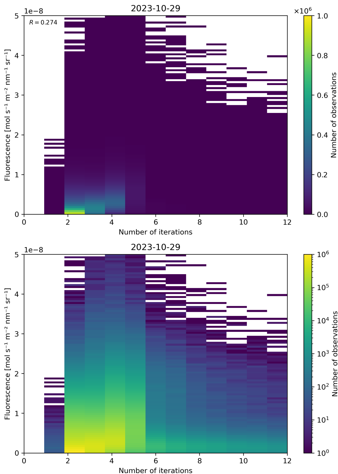
Figure 107: Scatter density plot of “Number of iterations” against “Fluorescence” for 2023-10-28 to 2023-10-30.
