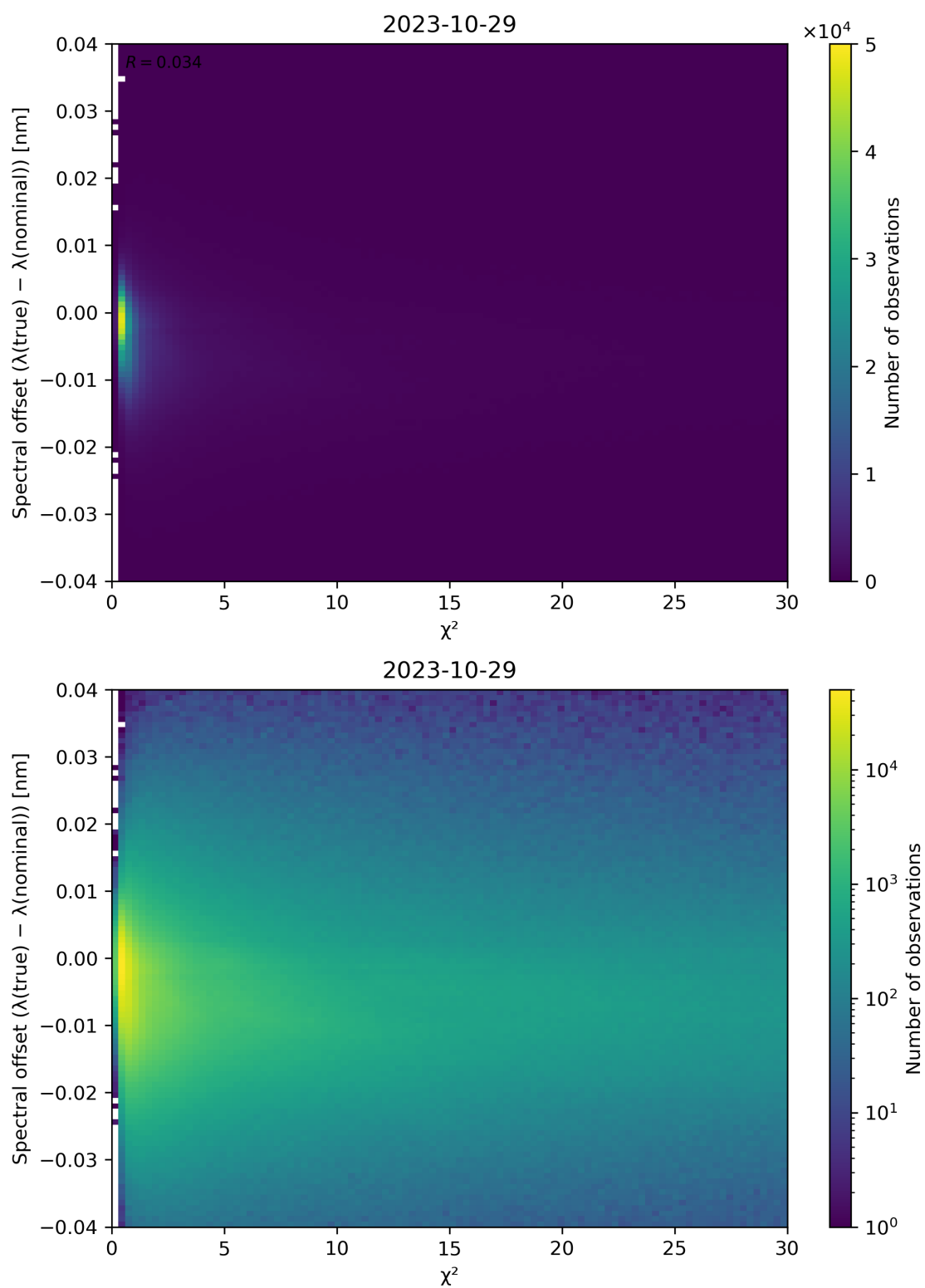
Figure 75: Scatter density plot of “ \chi^2 ” against “Spectral offset ( \lambda(\text{true}) - \lambda(\text{nominal}) )” for 2023-10-28 to 2023-10-30.
