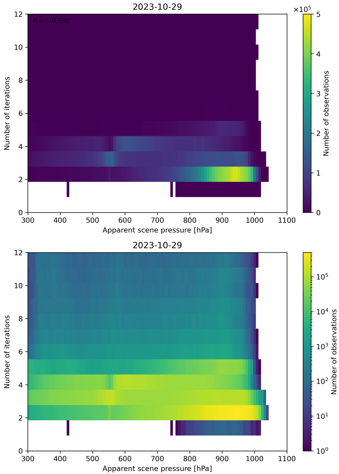
Figure 66: Scatter density plot of “Apparent scene pressure” against “Number of iterations” for 2023-10-28 to 2023-10-30.
