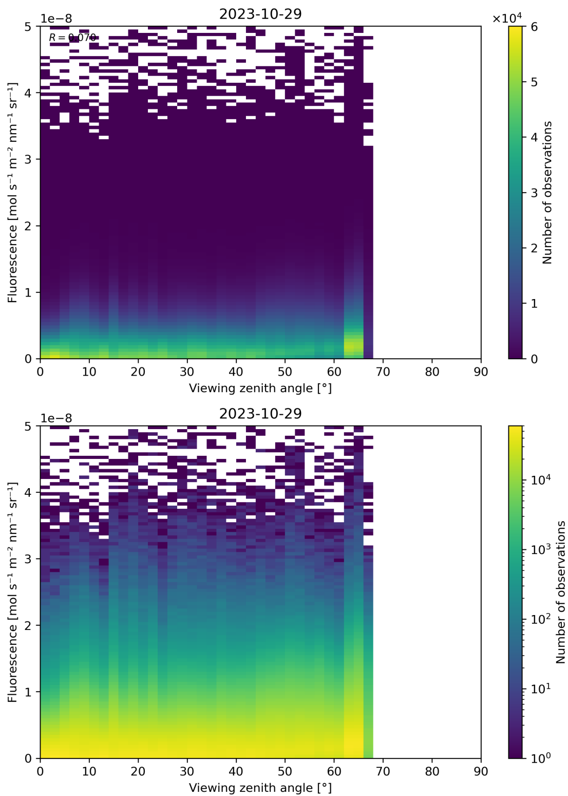
Figure 134: Scatter density plot of “Viewing zenith angle” against “Fluorescence” for 2023-10-28 to 2023-10-30.
