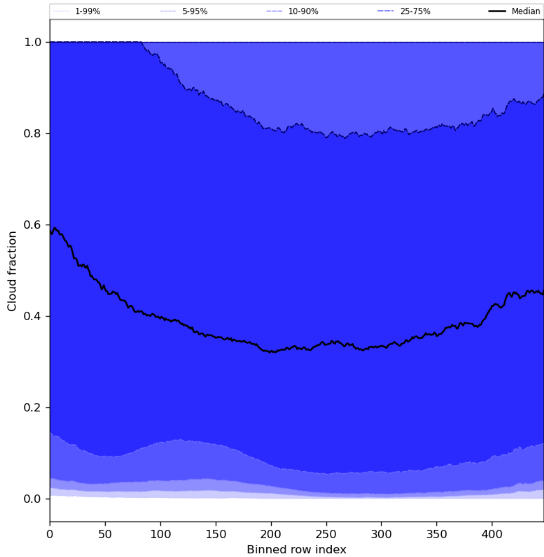
Figure 49: Along track statistics of “Cloud fraction” for 2023-10-28 to 2023-10-30
