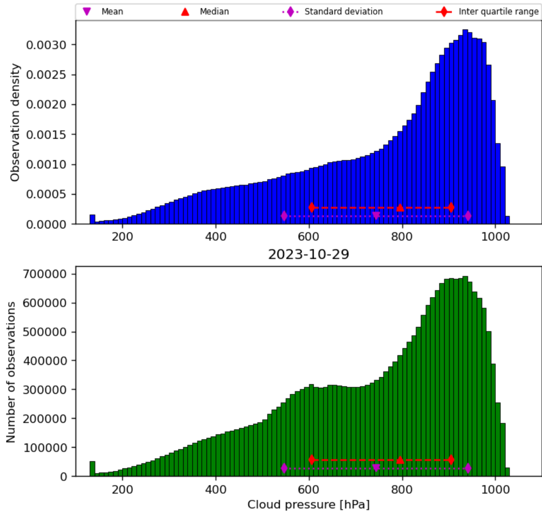
Figure 30: Histogram of “Cloud pressure” for 2023-10-28 to 2023-10-30
