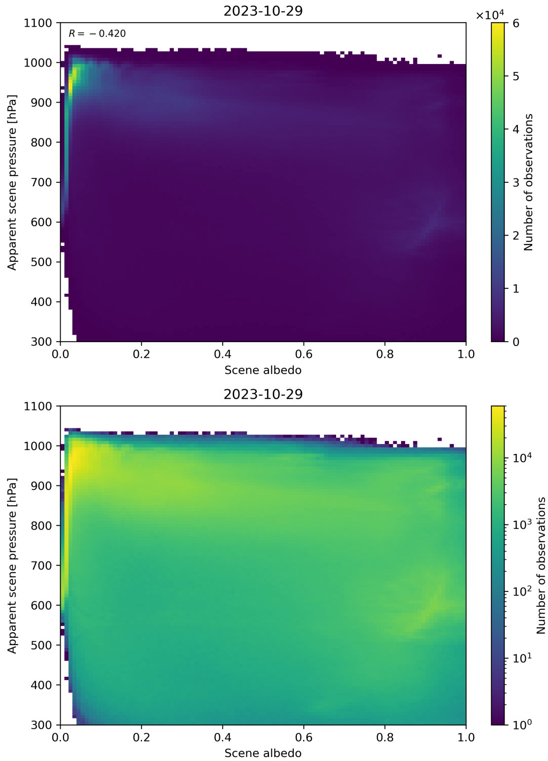
Figure 111: Scatter density plot of “Scene albedo” against “Apparent scene pressure” for 2023-10-28 to 2023-10-30.
