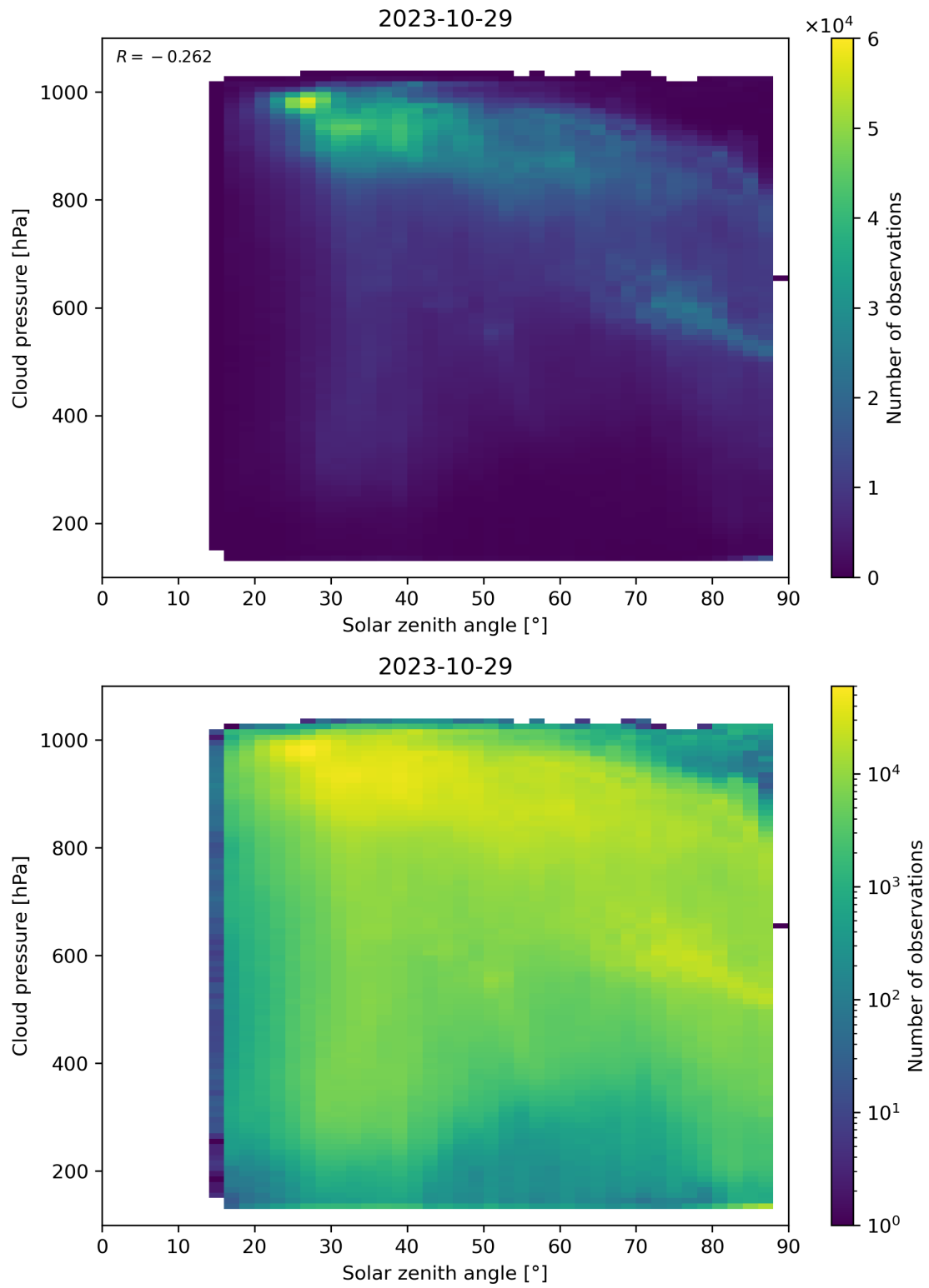
Figure 122: Scatter density plot of “Solar zenith angle” against “Cloud pressure” for 2023-10-28 to 2023-10-30.
