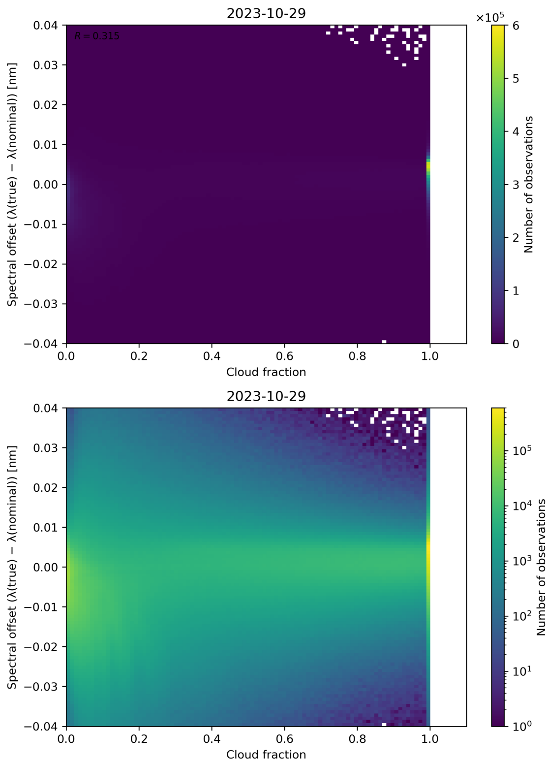
Figure 83: Scatter density plot of “Cloud fraction” against “Spectral offset ( \lambda(\text{true}) - \lambda(\text{nominal}) )” for 2023-10-28 to 2023-10-30.
