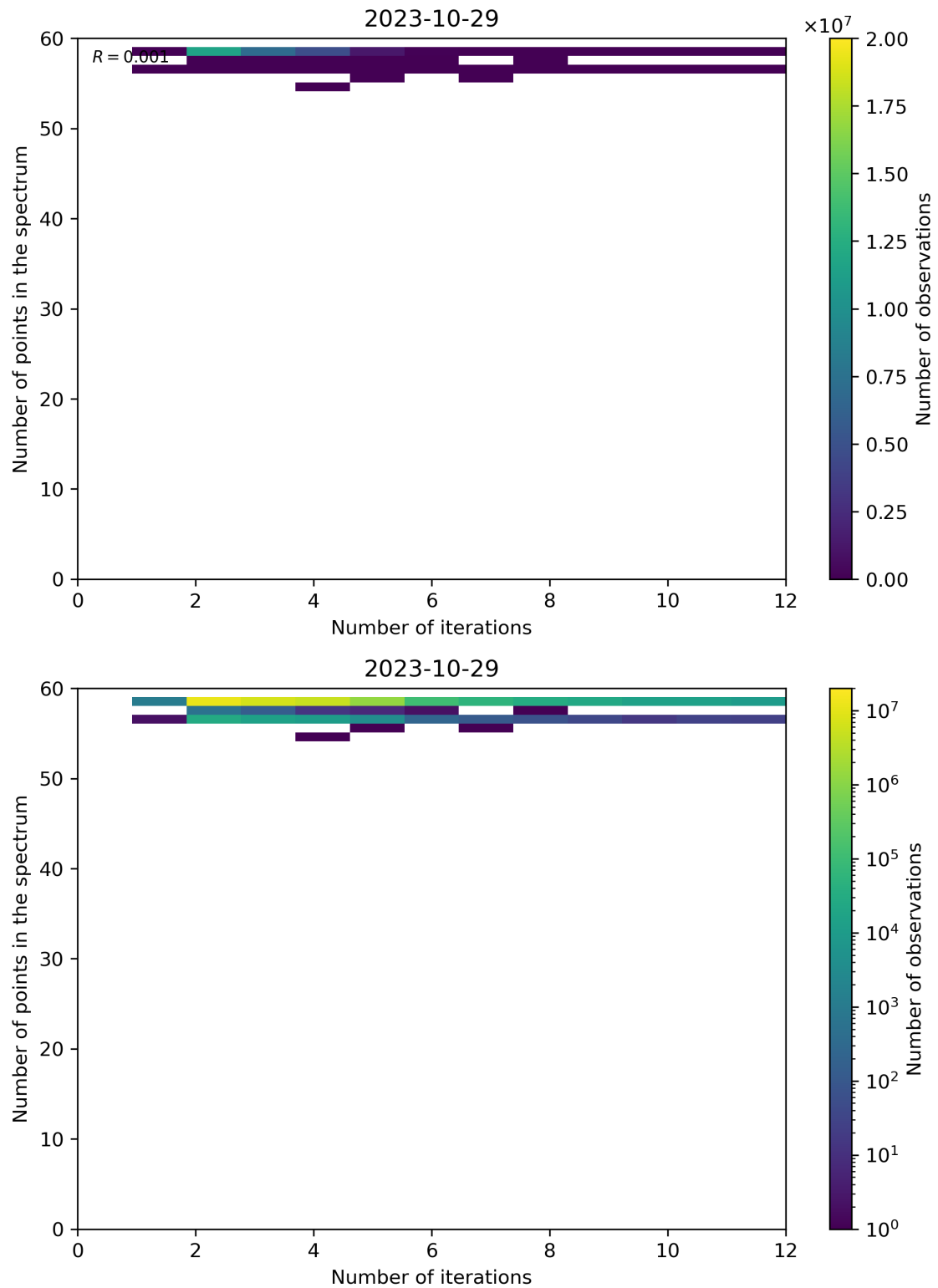
Figure 108: Scatter density plot of “Number of iterations” against “Number of points in the spectrum” for 2023-10-28 to 2023-10-30.
