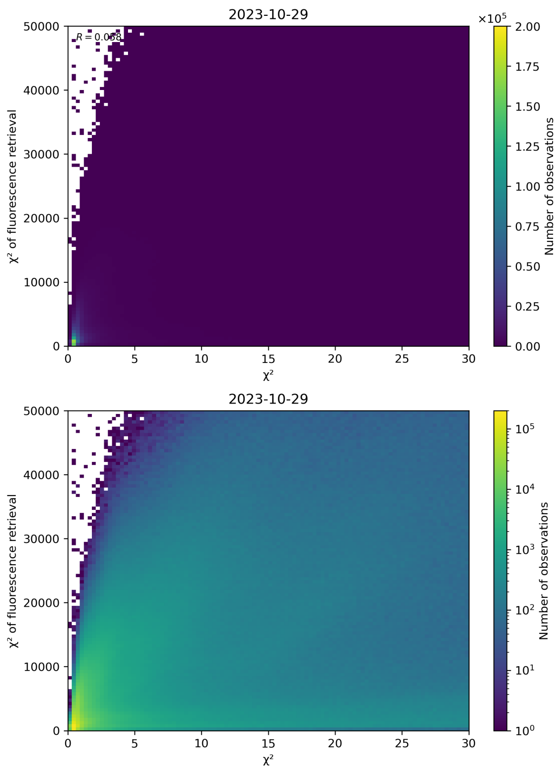
Figure 69: Scatter density plot of “ \chi^2 ” against “ \chi^2 of fluorescence retrieval” for 2023-10-28 to 2023-10-30.
