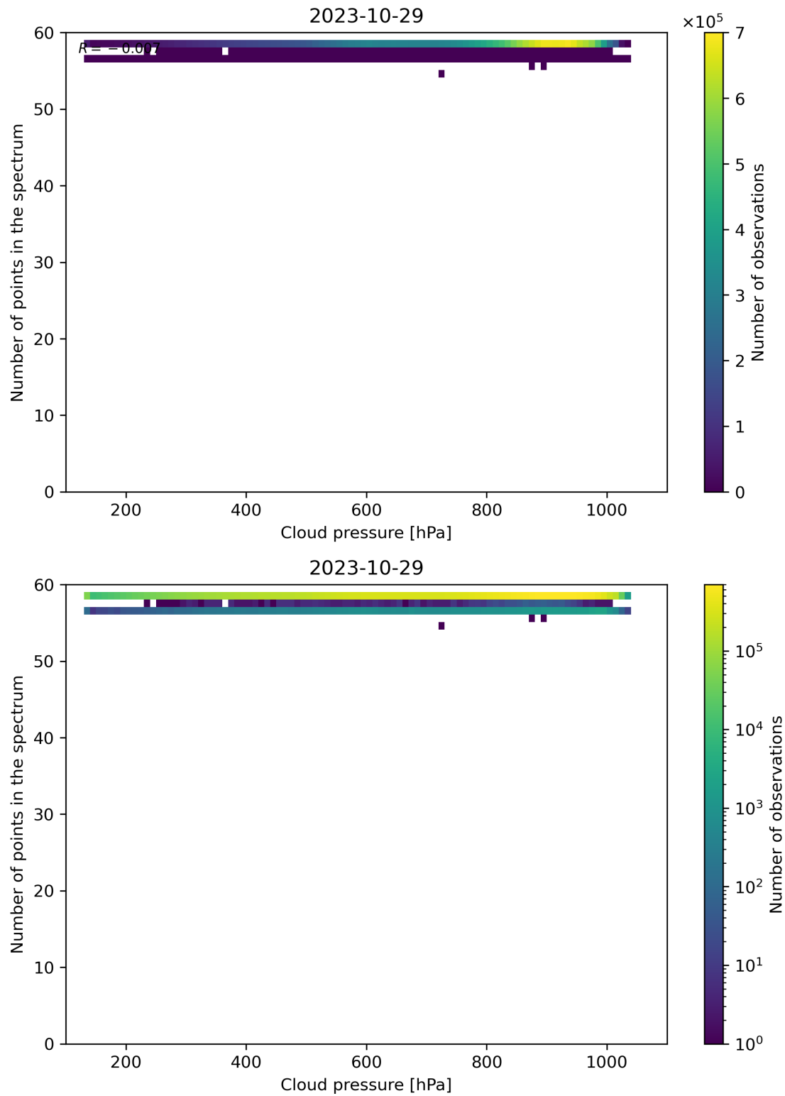
Figure 90: Scatter density plot of “Cloud pressure” against “Number of points in the spectrum” for 2023-10-28 to 2023-10-30.
