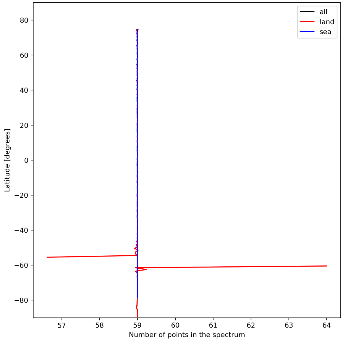
Figure 27: Zonal average of “Number of points in the spectrum” for 2023-10-28 to 2023-10-30.
