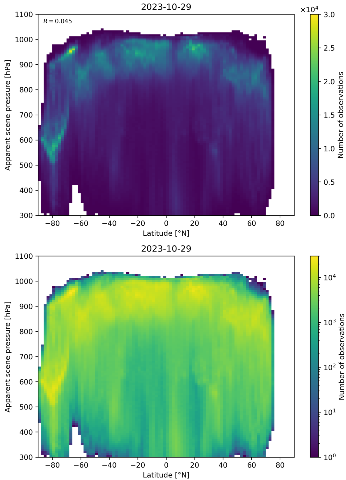
Figure 96: Scatter density plot of “Latitude” against “Apparent scene pressure” for 2023-10-28 to 2023-10-30.
