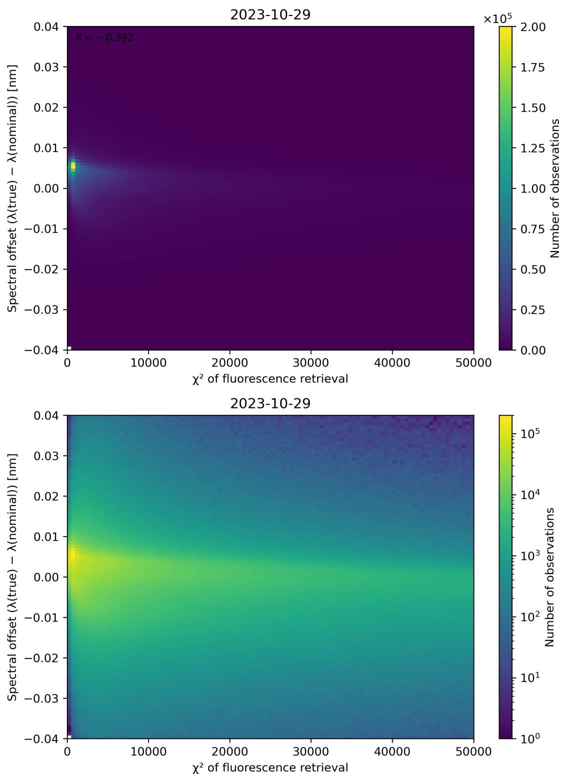
Figure 72: Scatter density plot of " \chi^2 of fluorescence retrieval" against "Spectral offset ( \lambda(\text{true}) - \lambda(\text{nominal}) )" for 2023-10-28 to 2023-10-30.
