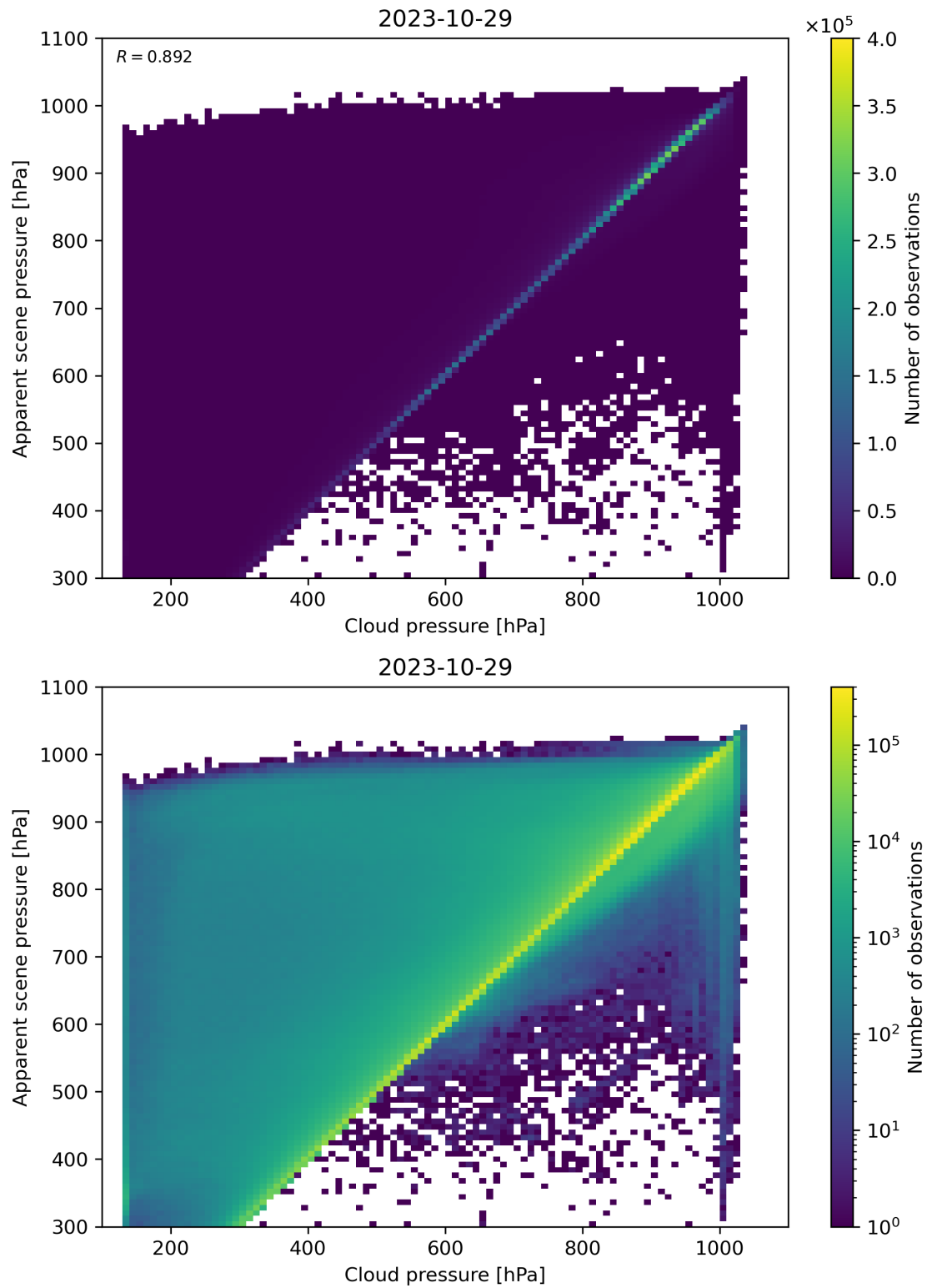
Figure 84: Scatter density plot of “Cloud pressure” against “Apparent scene pressure” for 2023-10-28 to 2023-10-30.
