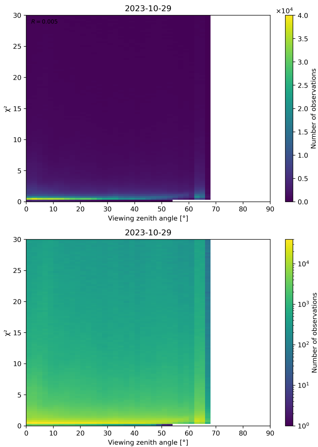
Figure 130: Scatter density plot of “Viewing zenith angle” against “ \chi^2 ” for 2023-10-28 to 2023-10-30.
