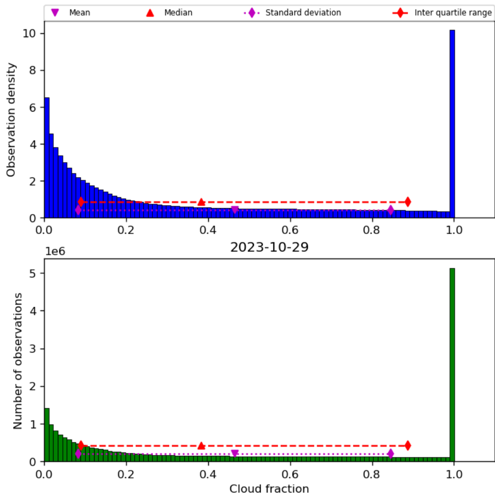
Figure 32: Histogram of “Cloud fraction” for 2023-10-28 to 2023-10-30
