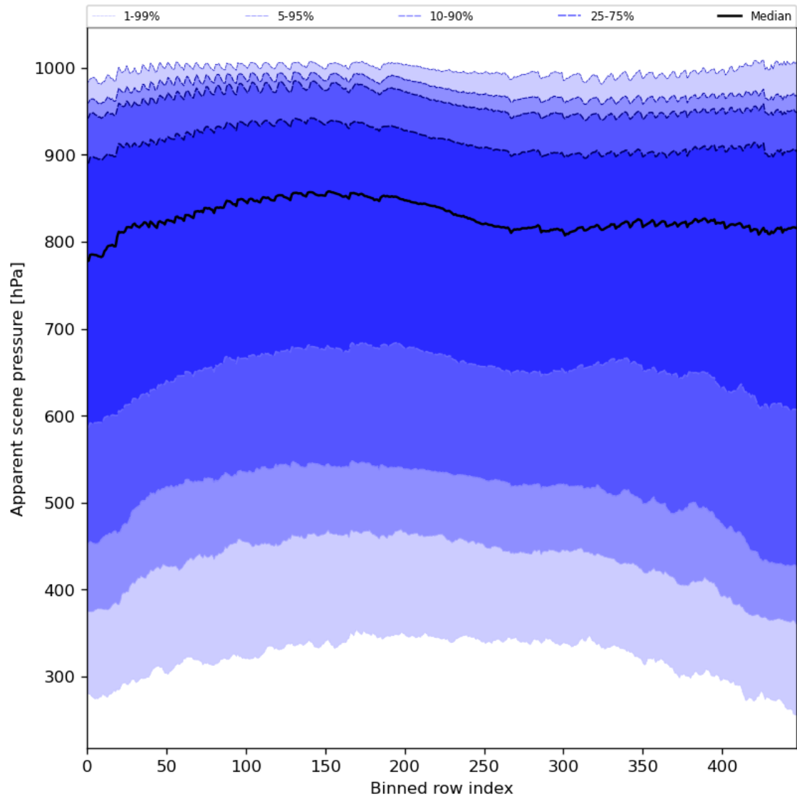
Figure 53: Along track statistics of “Apparent scene pressure” for 2023-10-28 to 2023-10-30
