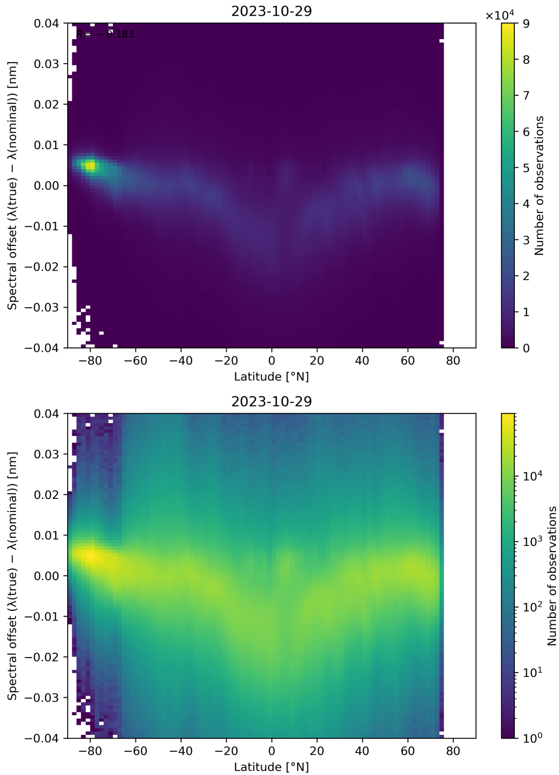
Figure 105: Scatter density plot of “Latitude” against “Spectral offset ( \lambda(\text{true}) - \lambda(\text{nominal}) )” for 2023-10-28 to 2023-10-30.
