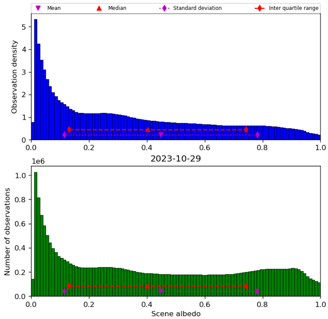
Figure 34: Histogram of “Scene albedo” for 2023-10-28 to 2023-10-30
