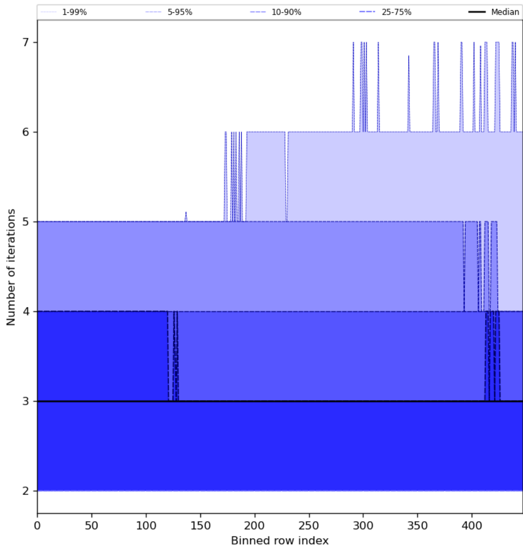
Figure 56: Along track statistics of “Number of iterations” for 2023-10-28 to 2023-10-30
