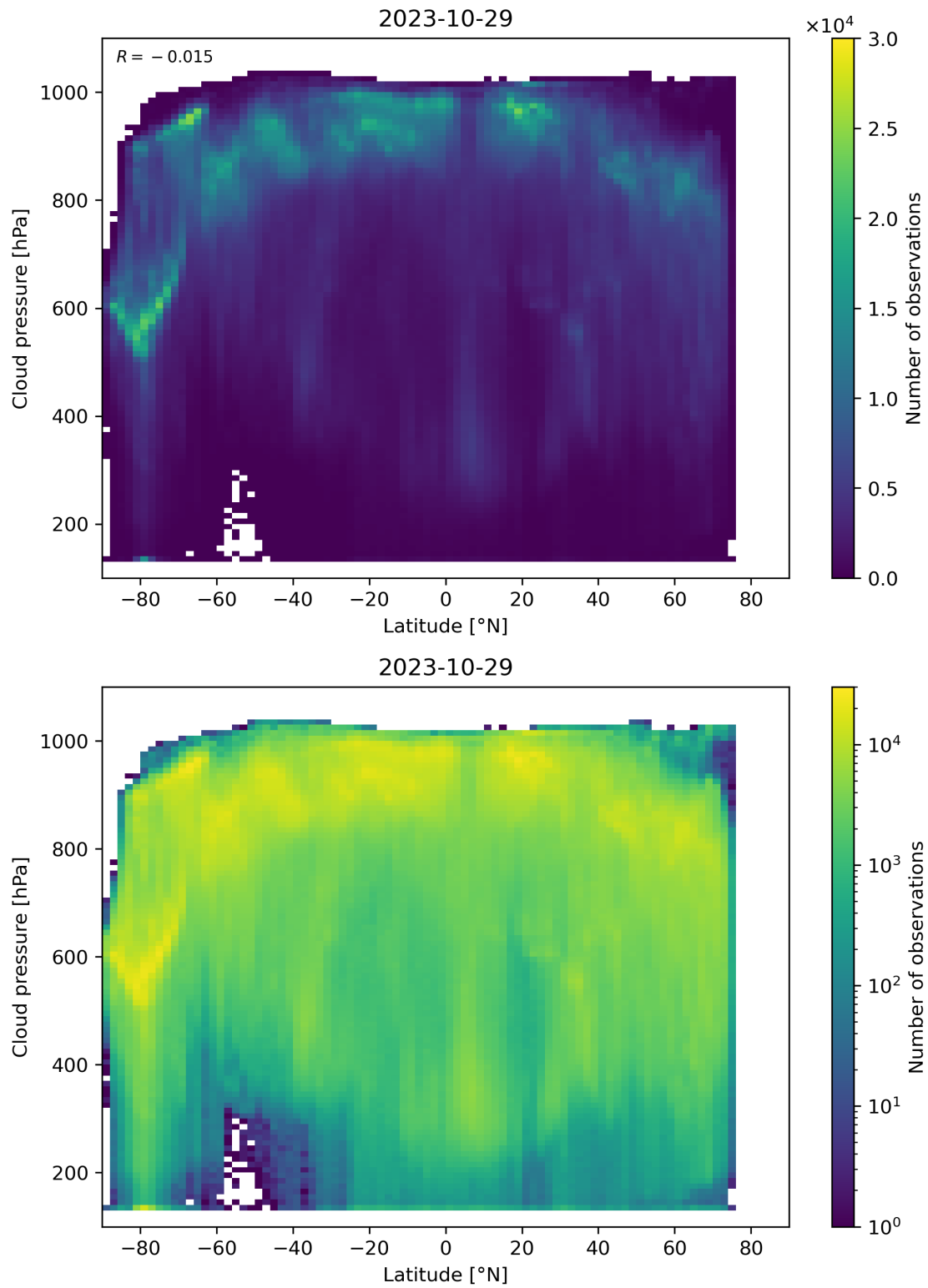
Figure 100: Scatter density plot of “Latitude” against “Cloud pressure” for 2023-10-28 to 2023-10-30.
