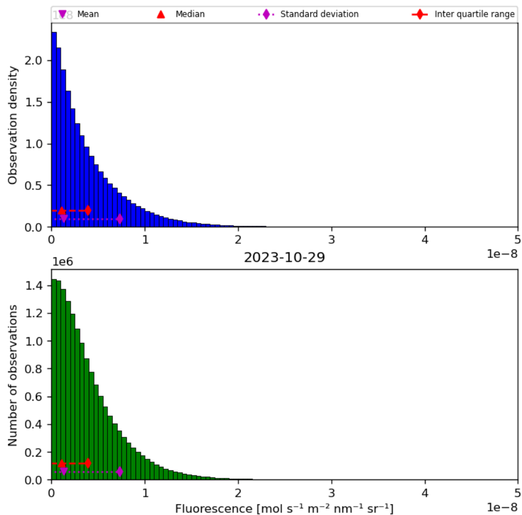
Figure 40: Histogram of “Fluorescence” for 2023-10-28 to 2023-10-30
