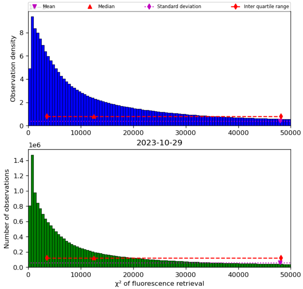
Figure 42: Histogram of “ \chi^2 of fluorescence retrieval” for 2023-10-28 to 2023-10-30
