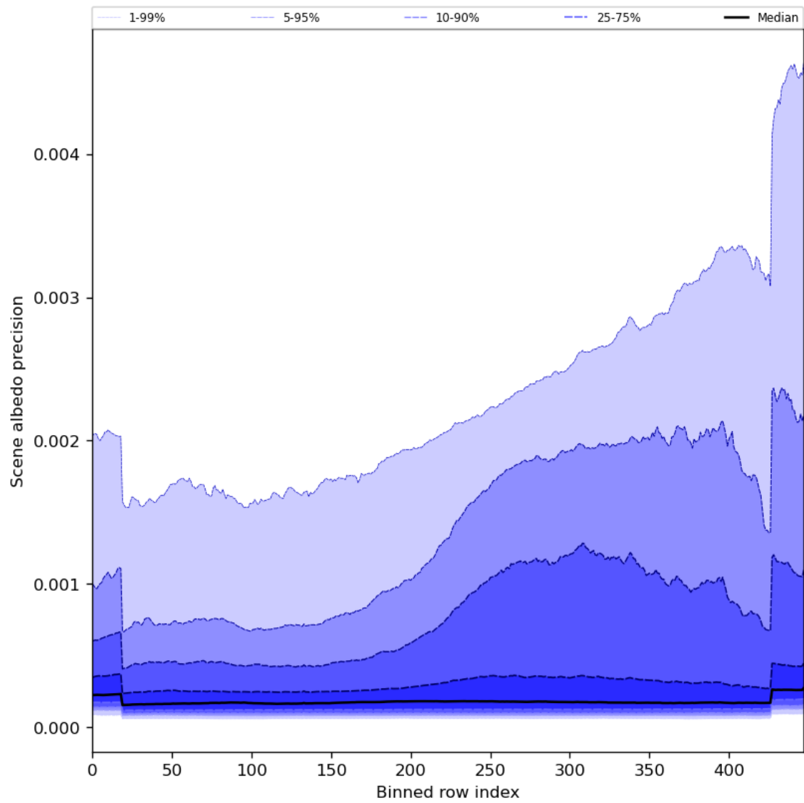
Figure 52: Along track statistics of “Scene albedo precision” for 2023-10-28 to 2023-10-30
