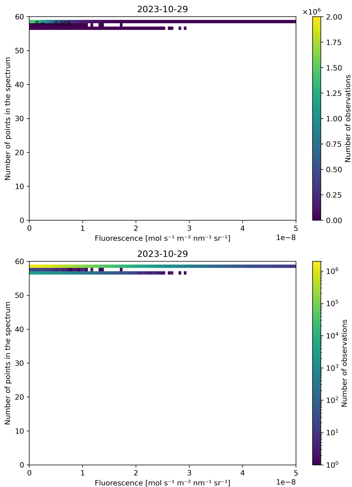
Figure 94: Scatter density plot of “Fluorescence” against “Number of points in the spectrum” for 2023-10-28 to 2023-10-30.
