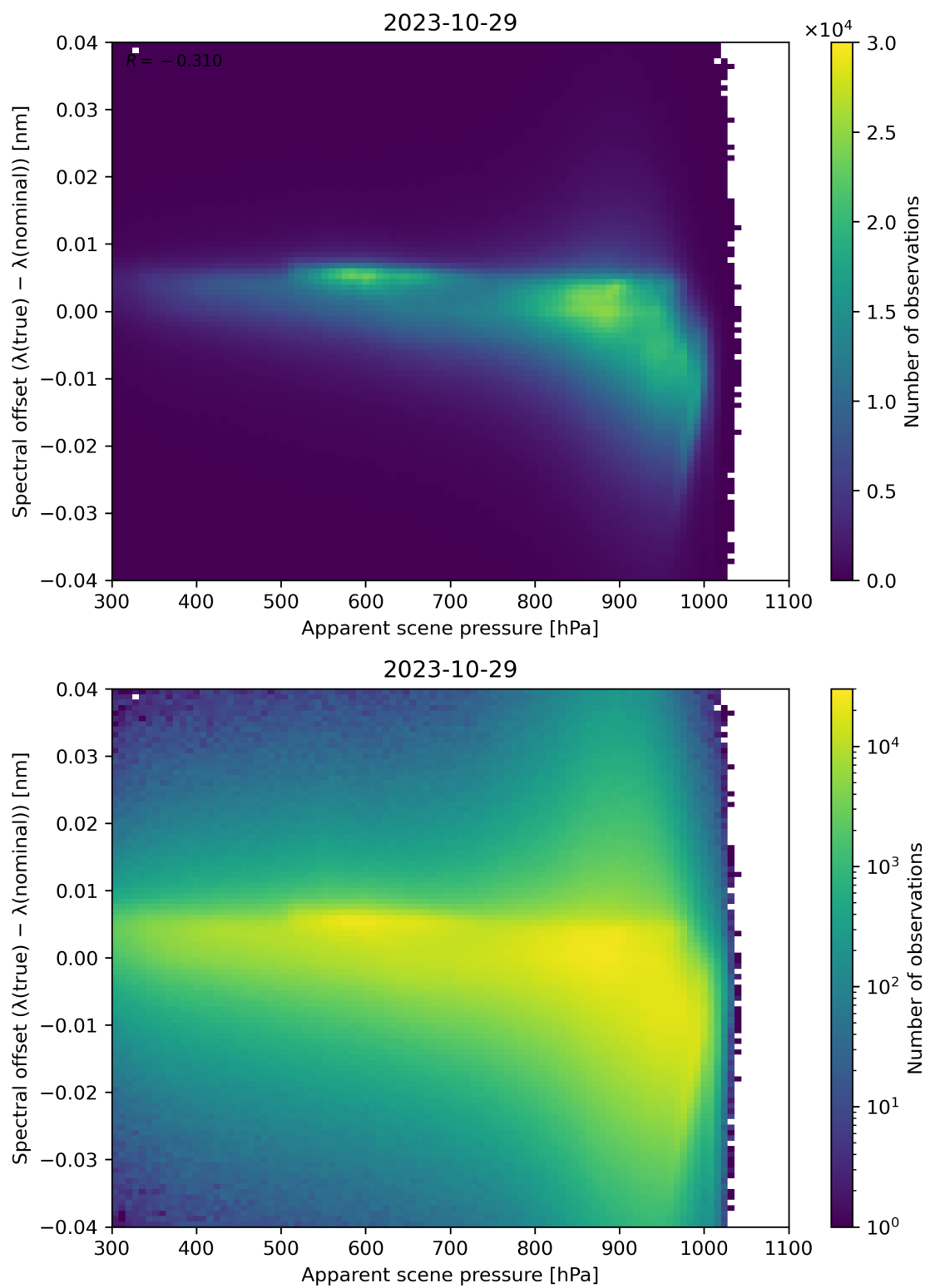
Figure 68: Scatter density plot of “Apparent scene pressure” against “Spectral offset ( \lambda(\text{true}) - \lambda(\text{nominal}) )” for 2023-10-28 to 2023-10-30.
