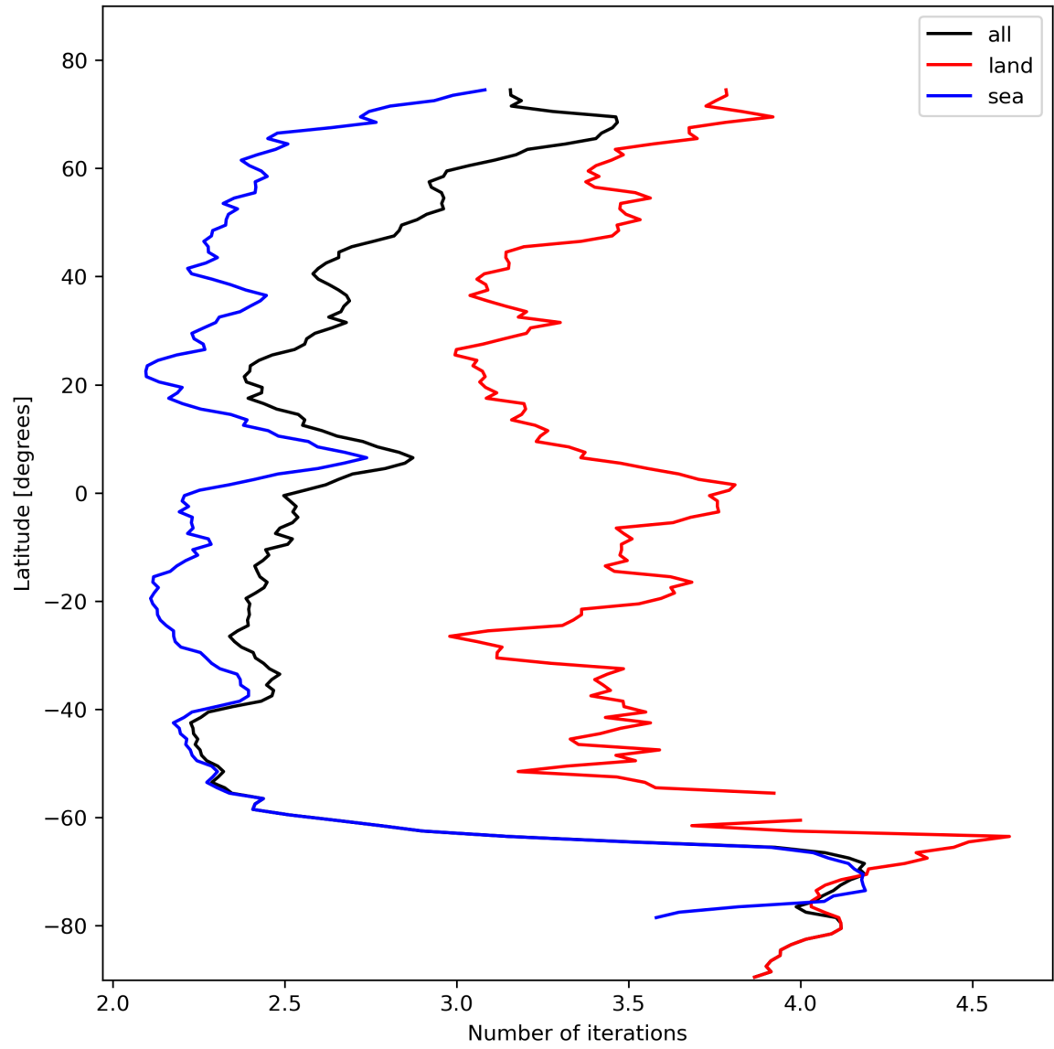
Figure 22: Zonal average of “Number of iterations” for 2023-10-28 to 2023-10-30.
