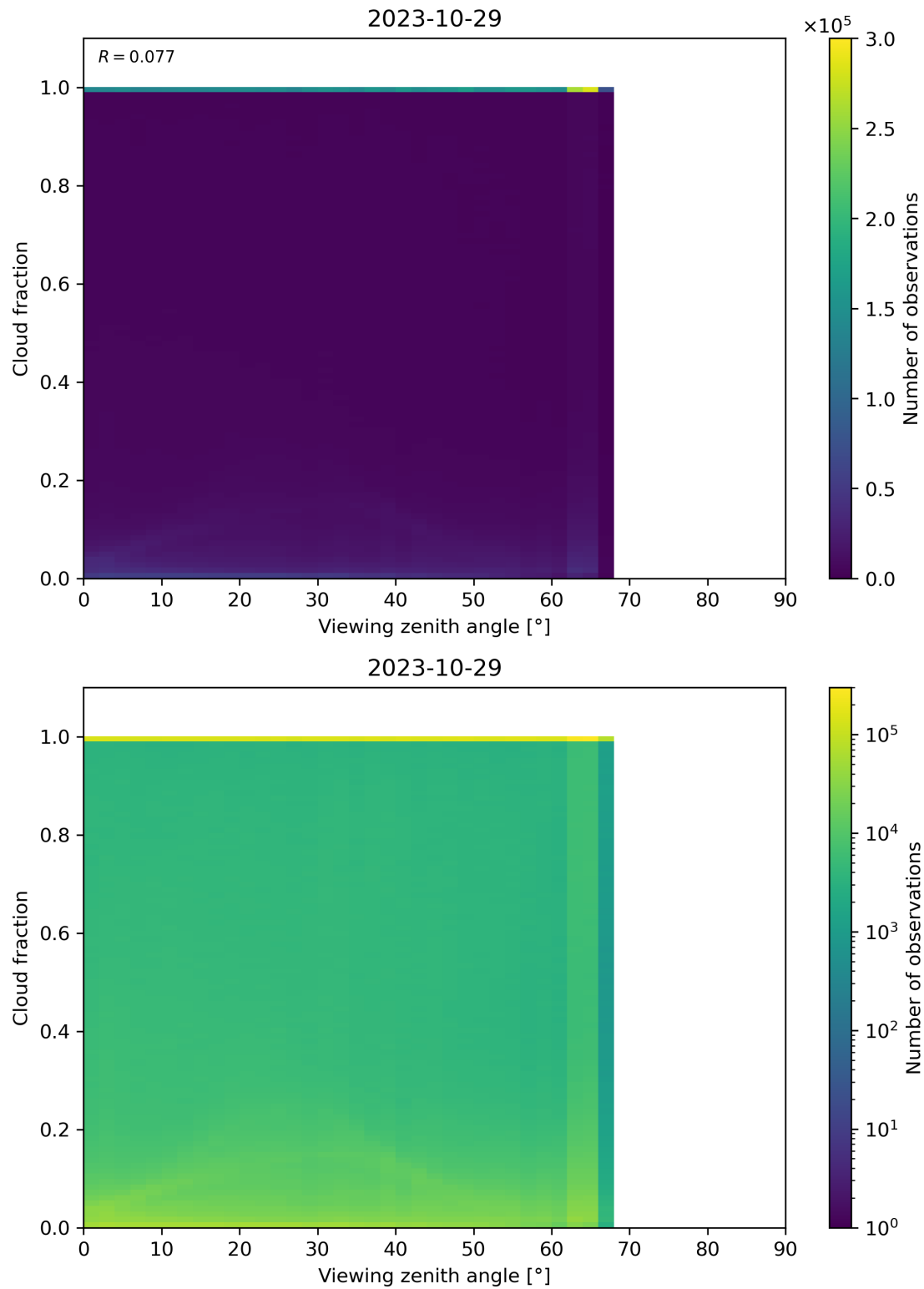
Figure 132: Scatter density plot of “Viewing zenith angle” against “Cloud fraction” for 2023-10-28 to 2023-10-30.
