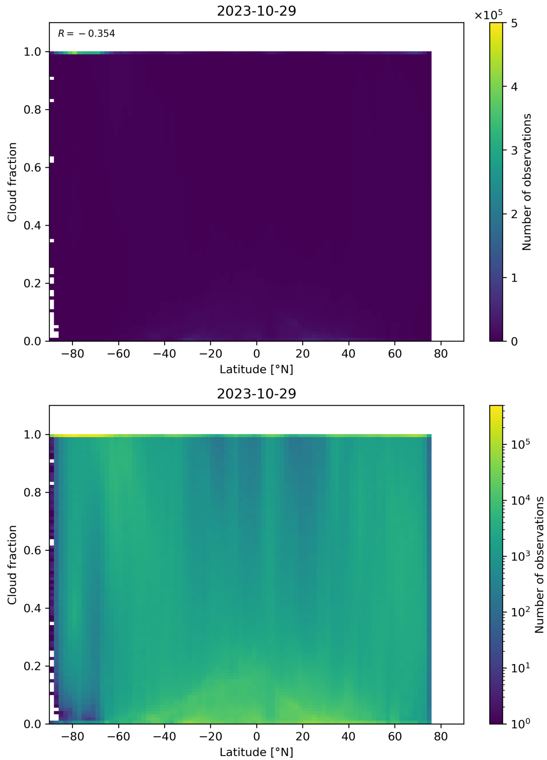
Figure 99: Scatter density plot of “Latitude” against “Cloud fraction” for 2023-10-28 to 2023-10-30.
