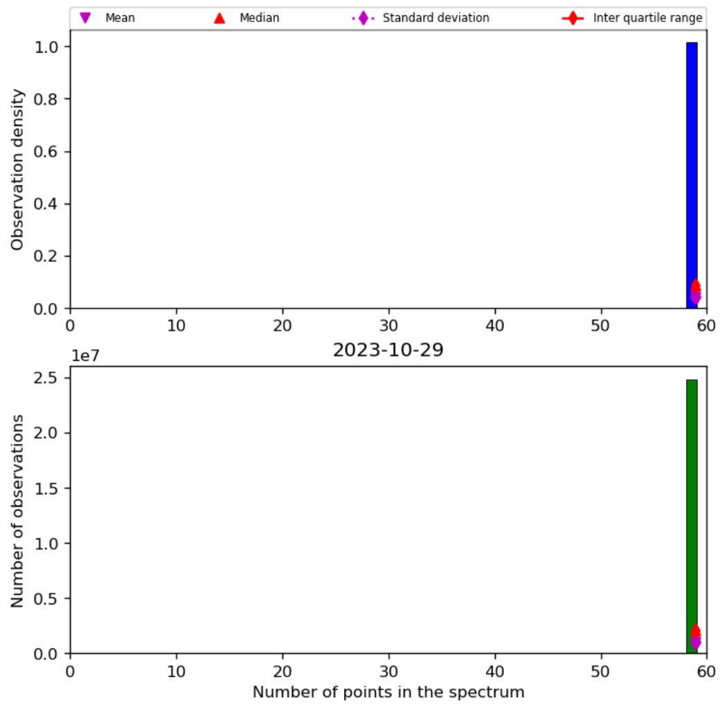
Figure 44: Histogram of “Number of points in the spectrum” for 2023-10-28 to 2023-10-30
