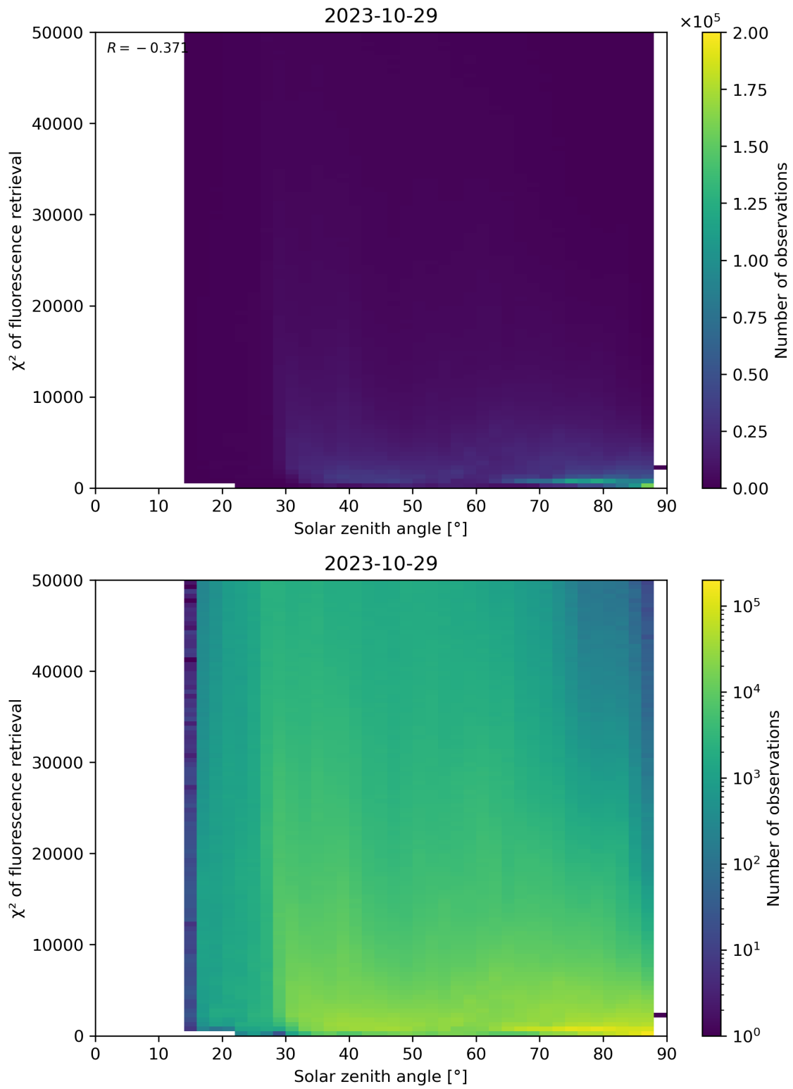
Figure 120: Scatter density plot of “Solar zenith angle” against “ \chi^2 of fluorescence retrieval” for 2023-10-28 to 2023-10-30.
