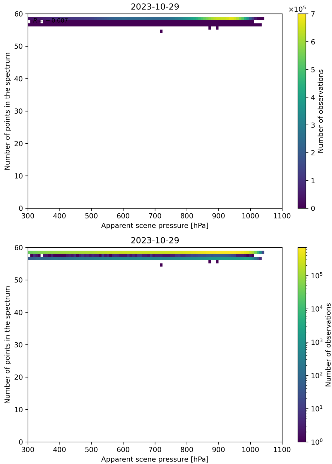
Figure 67: Scatter density plot of “Apparent scene pressure” against “Number of points in the spectrum” for 2023-10-28 to 2023-10-30.
