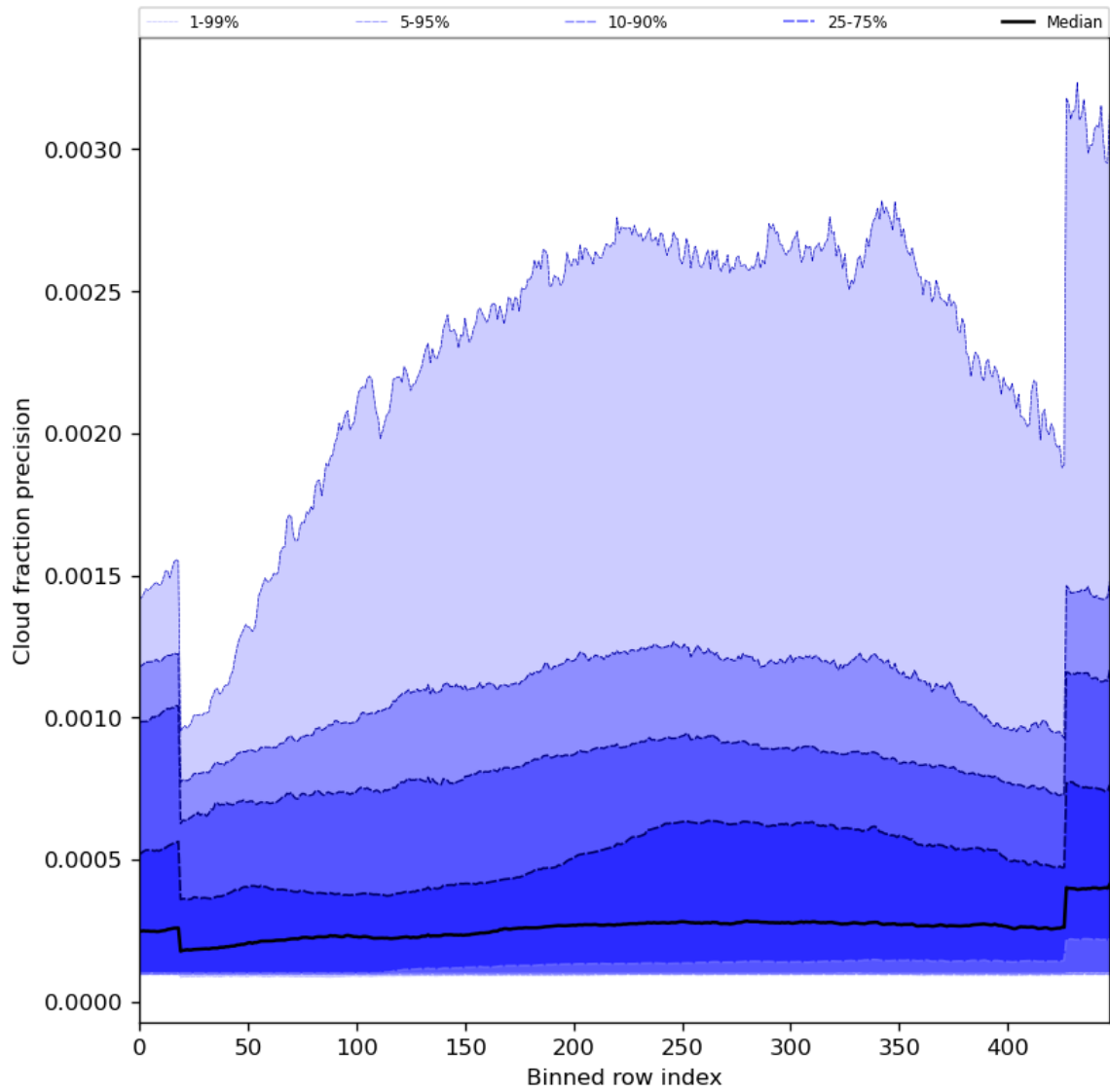
Figure 50: Along track statistics of “Cloud fraction precision” for 2023-10-28 to 2023-10-30
