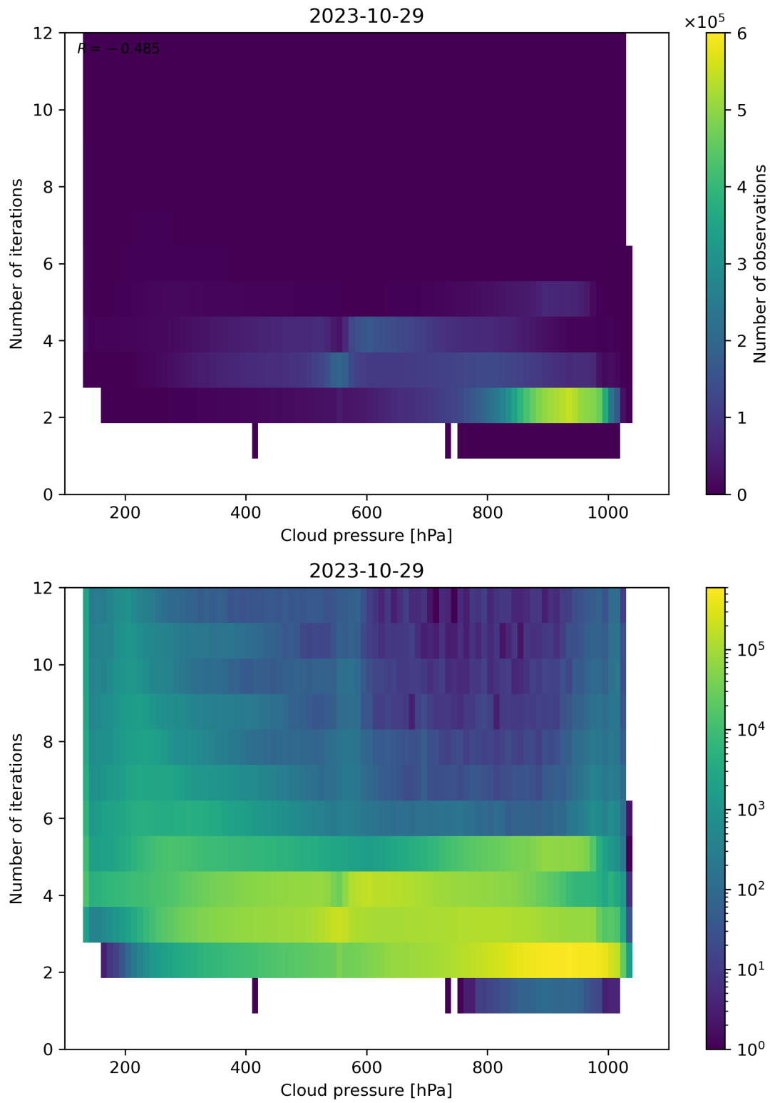
Figure 89: Scatter density plot of “Cloud pressure” against “Number of iterations” for 2023-10-28 to 2023-10-30.
