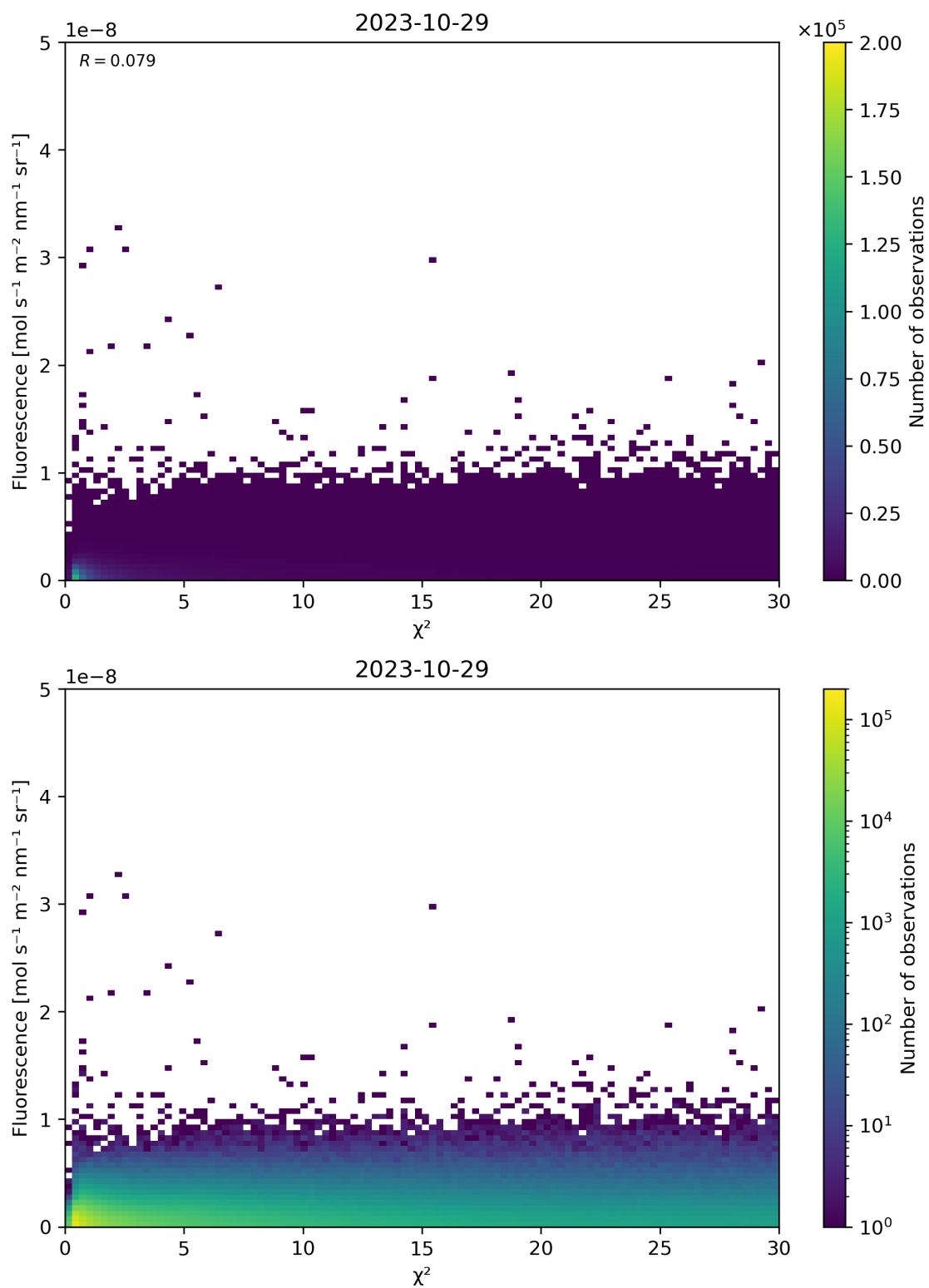
Figure 70: Scatter density plot of “ \chi^2 ” against “Fluorescence” for 2023-10-28 to 2023-10-30.
