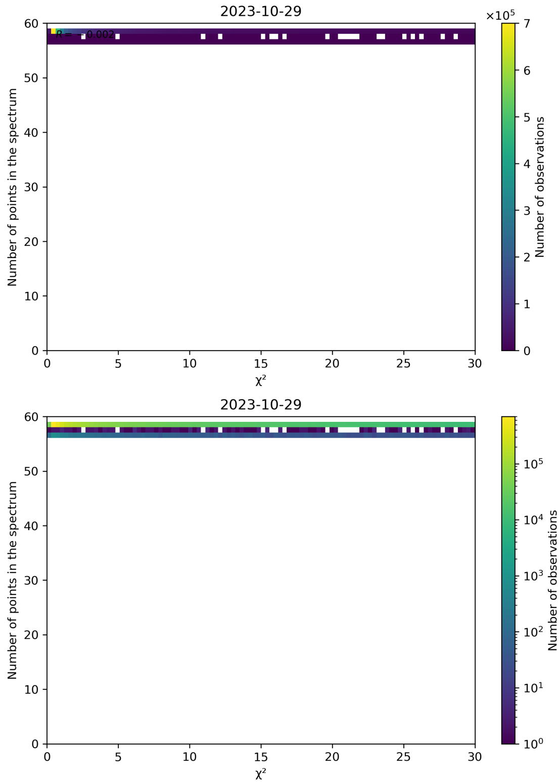
Figure 74: Scatter density plot of " \chi^2 " against "Number of points in the spectrum" for 2023-10-28 to 2023-10-30.
