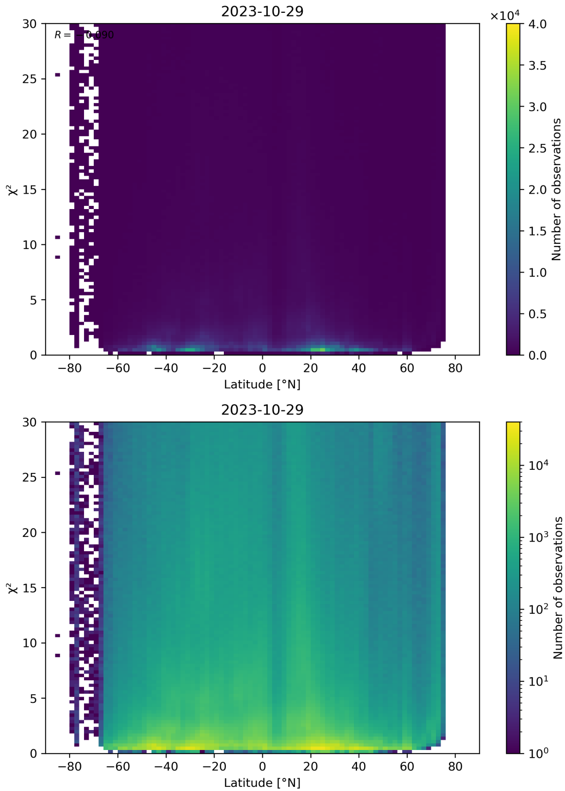
Figure 97: Scatter density plot of “Latitude” against “ \chi^2 ” for 2023-10-28 to 2023-10-30.
