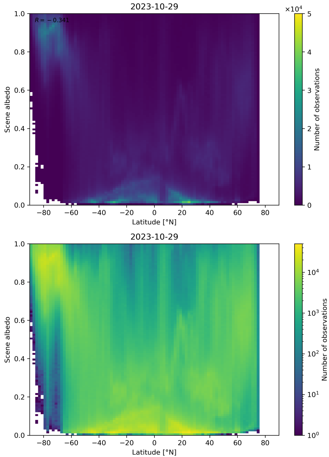
Figure 104: Scatter density plot of “Latitude” against “Scene albedo” for 2023-10-28 to 2023-10-30.
