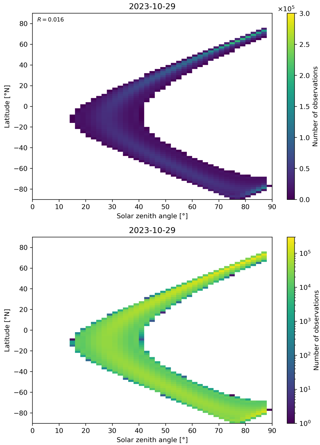
Figure 124: Scatter density plot of “Solar zenith angle” against “Latitude” for 2023-10-28 to 2023-10-30.
