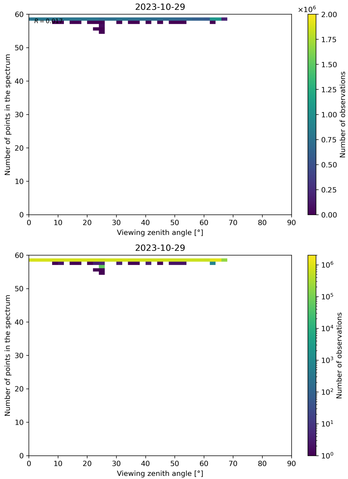
Figure 137: Scatter density plot of “Viewing zenith angle” against “Number of points in the spectrum” for 2023-10-28 to 2023-10-30.
