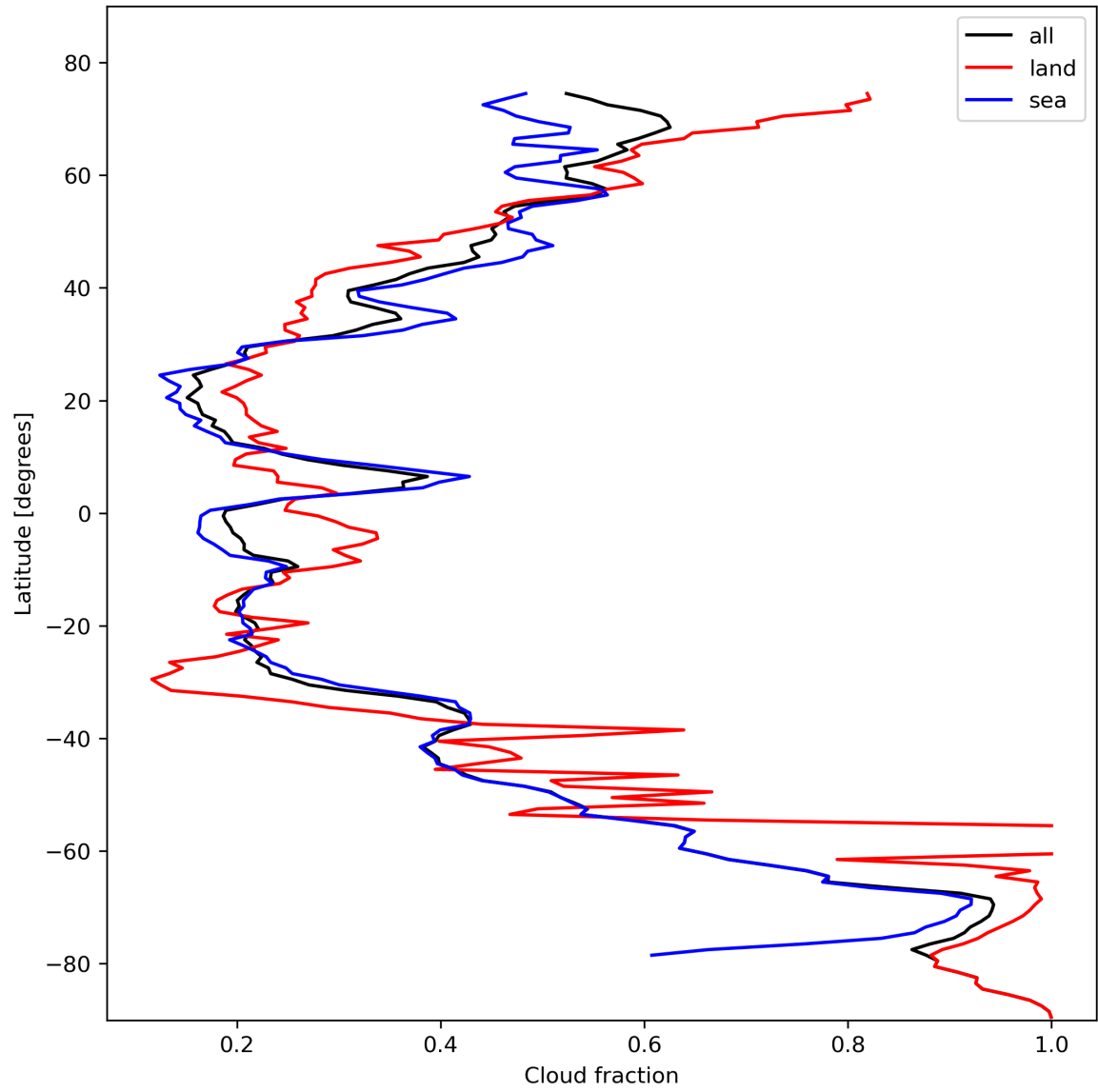
Figure 15: Zonal average of “Cloud fraction” for 2023-10-28 to 2023-10-30.
