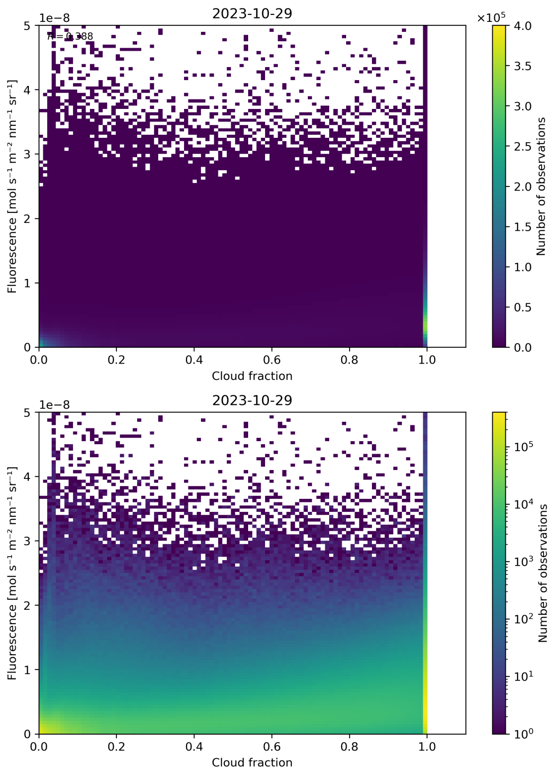
Figure 79: Scatter density plot of “Cloud fraction” against “Fluorescence” for 2023-10-28 to 2023-10-30.
