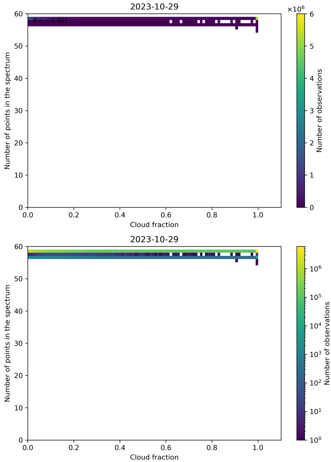
Figure 81: Scatter density plot of “Cloud fraction” against “Number of points in the spectrum” for 2023-10-28 to 2023-10-30.
