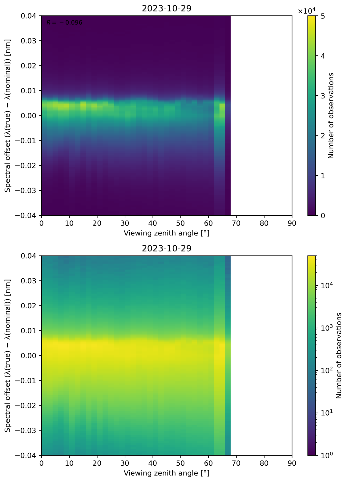
Figure 140: Scatter density plot of “Viewing zenith angle” against “Spectral offset ( \lambda(\text{true}) - \lambda(\text{nominal}) )” for 2023-10-28 to 2023-10-30.
