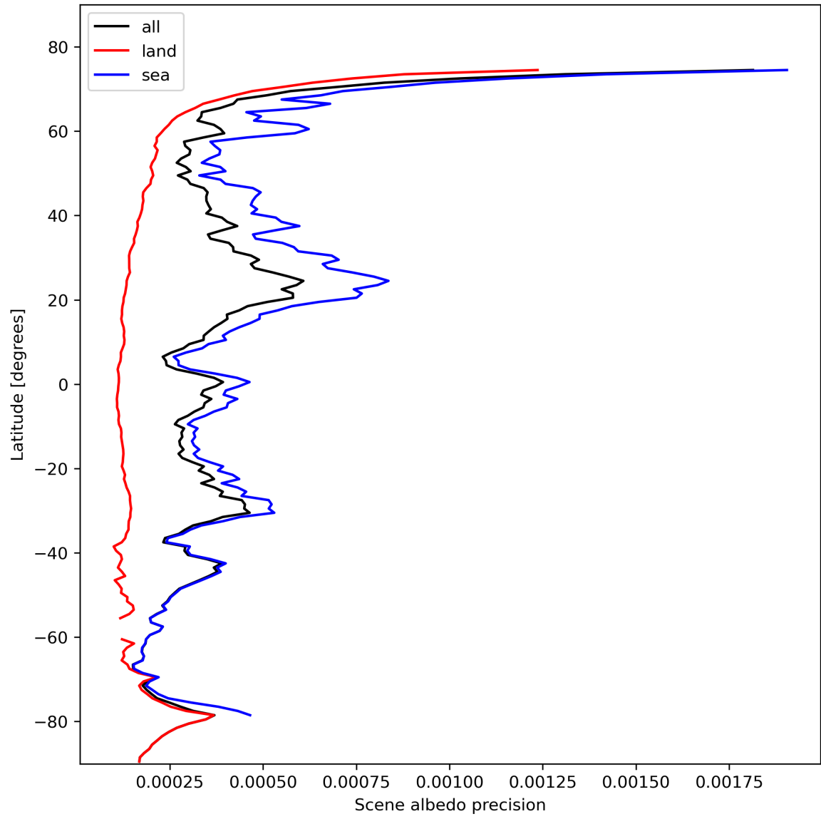
Figure 18: Zonal average of “Scene albedo precision” for 2023-10-28 to 2023-10-30.
