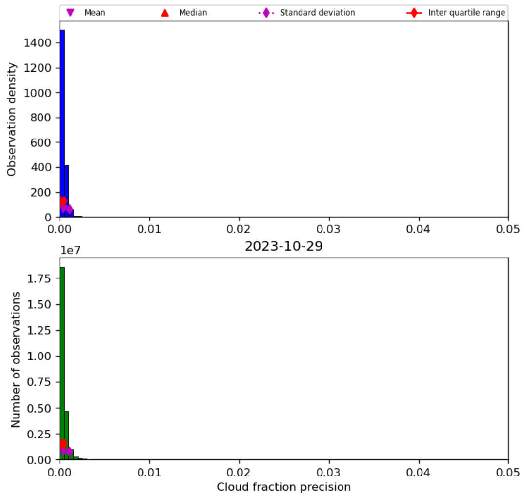
Figure 33: Histogram of “Cloud fraction precision” for 2023-10-28 to 2023-10-30
