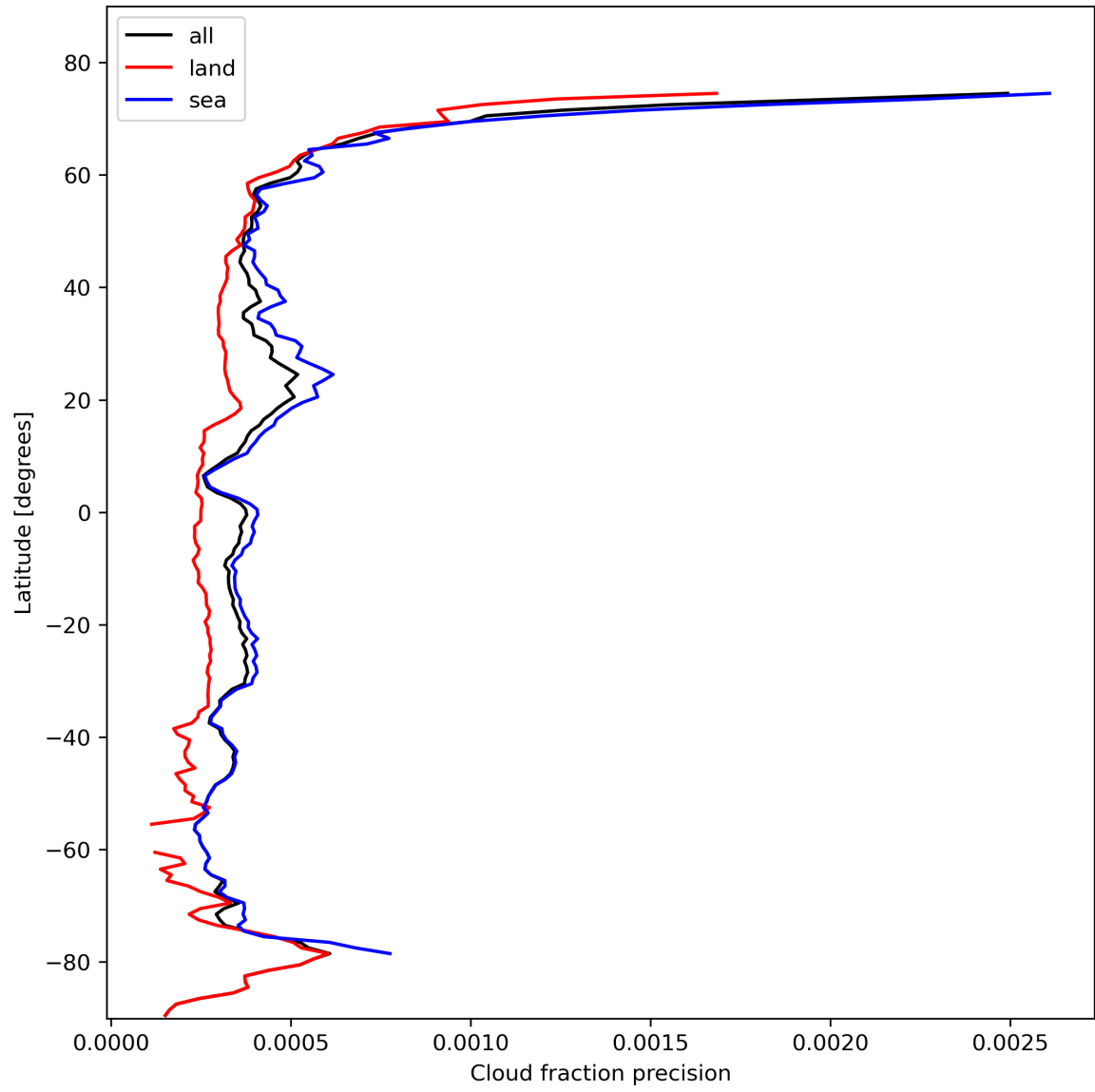
Figure 16: Zonal average of “Cloud fraction precision” for 2023-10-28 to 2023-10-30.
