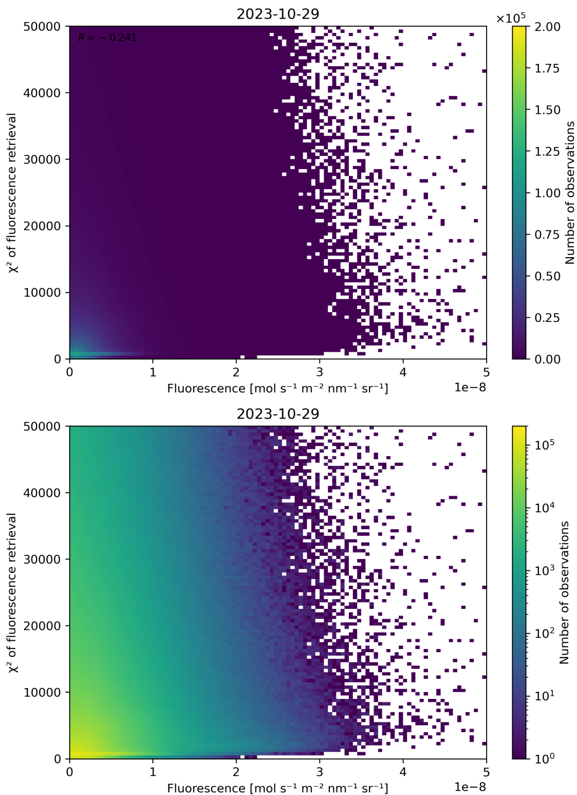
Figure 93: Scatter density plot of “Fluorescence” against “ \chi^2 of fluorescence retrieval” for 2023-10-28 to 2023-10-30.
