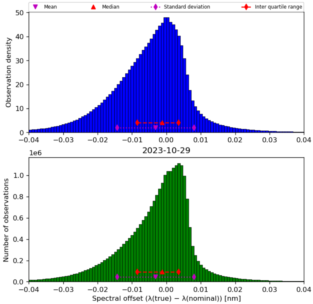
Figure 45: Histogram of “Spectral offset ( \lambda(\text{true}) - \lambda(\text{nominal}) )” for 2023-10-28 to 2023-10-30
