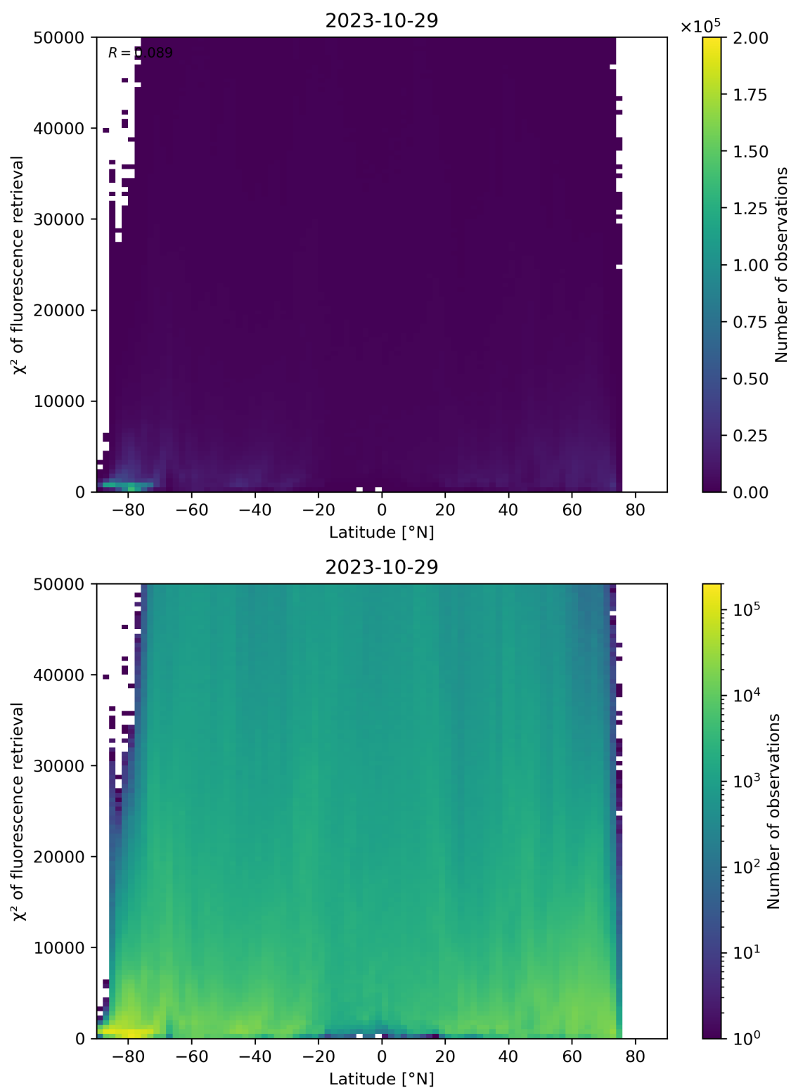
Figure 98: Scatter density plot of “Latitude” against “ \chi^2 of fluorescence retrieval” for 2023-10-28 to 2023-10-30.
