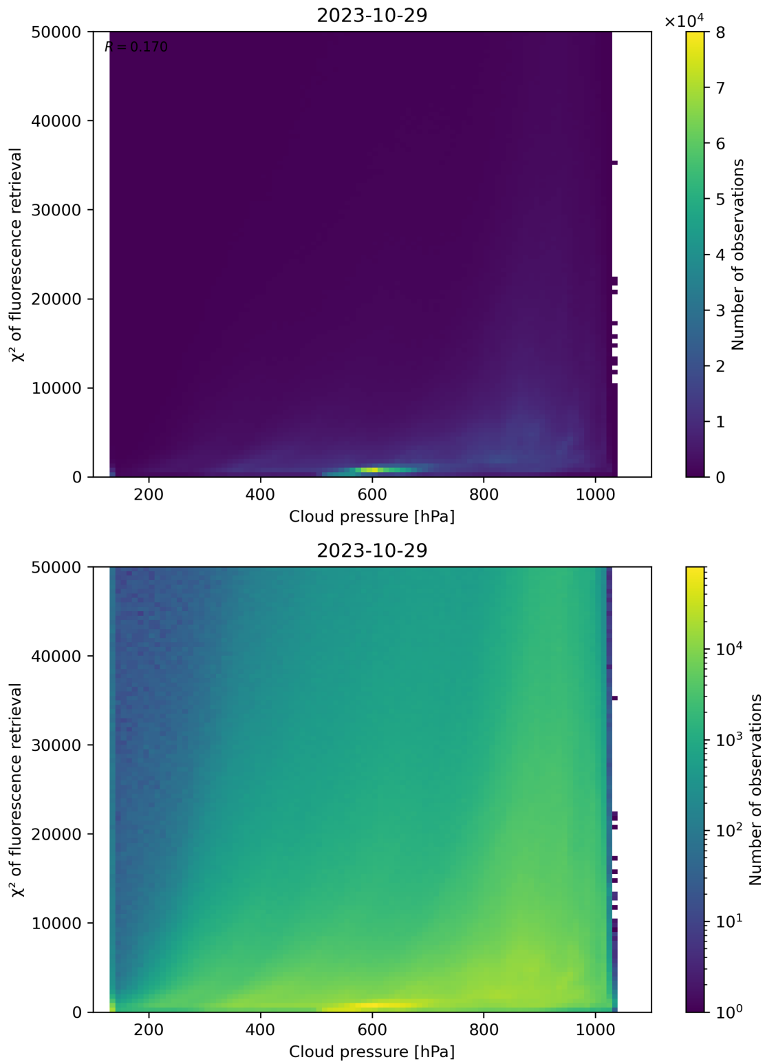
Figure 86: Scatter density plot of “Cloud pressure” against “ \chi^2 of fluorescence retrieval” for 2023-10-28 to 2023-10-30.
