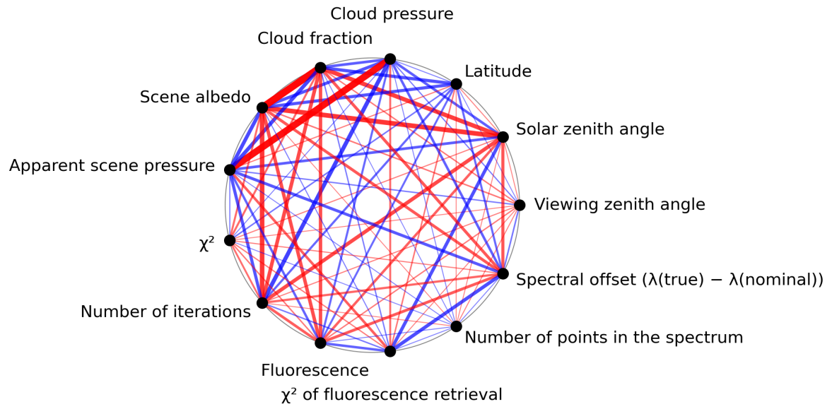
Figure 1: Map of correlation graph for 2023-10-28 to 2023-10-30.
