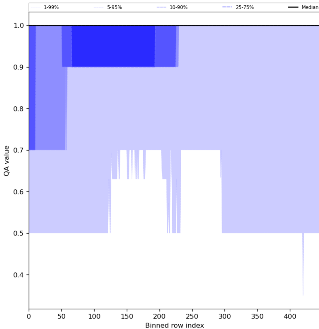
Figure 46: Along track statistics of “QA value” for 2023-10-28 to 2023-10-30
