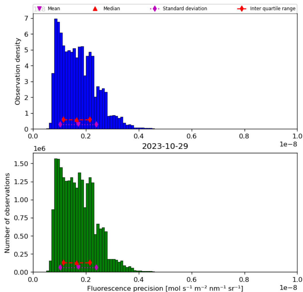
Figure 41: Histogram of “Fluorescence precision” for 2023-10-28 to 2023-10-30
