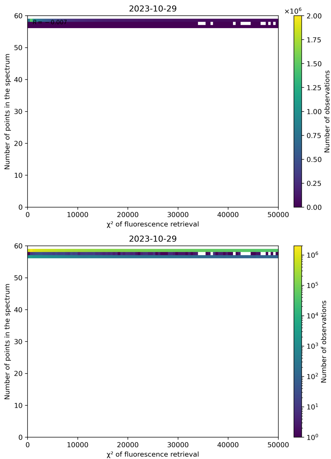
Figure 71: Scatter density plot of " \chi^2 of fluorescence retrieval" against "Number of points in the spectrum" for 2023-10-28 to 2023-10-30.
