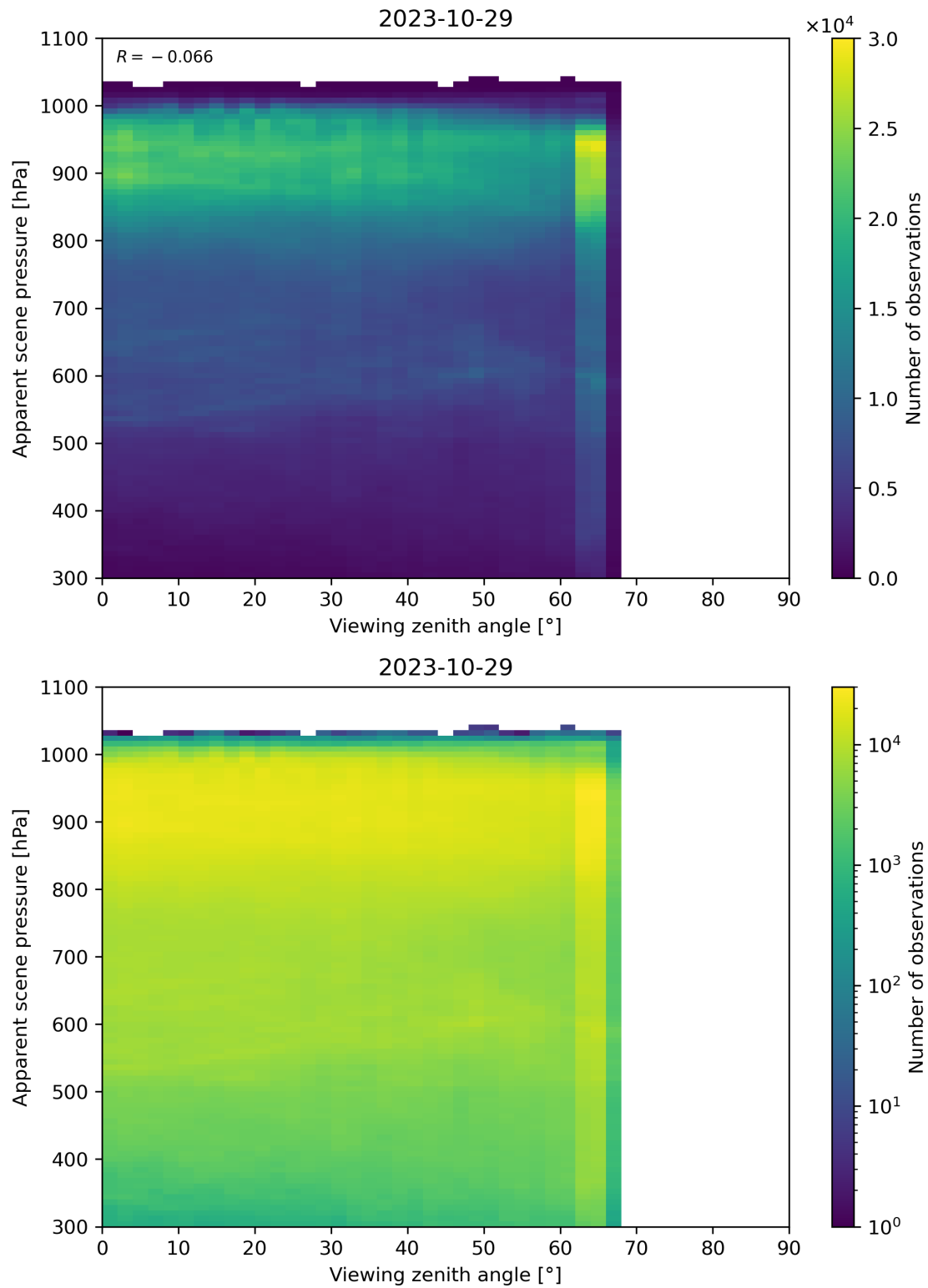
Figure 129: Scatter density plot of “Viewing zenith angle” against “Apparent scene pressure” for 2023-10-28 to 2023-10-30.
