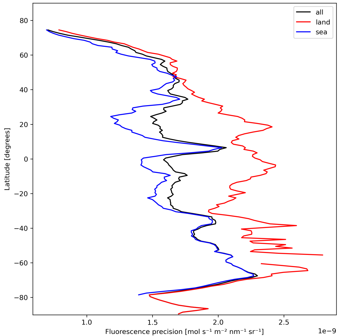
Figure 24: Zonal average of “Fluorescence precision” for 2023-10-28 to 2023-10-30.
