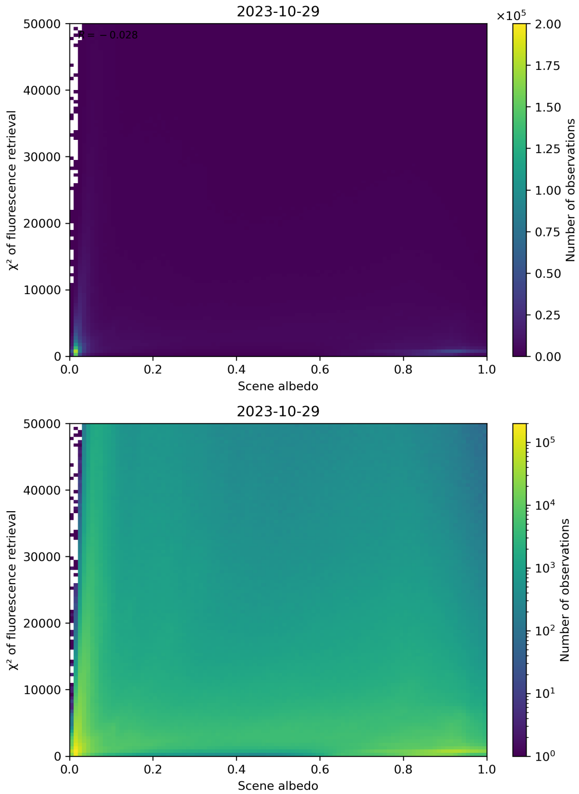
Figure 113: Scatter density plot of “Scene albedo” against “ \chi^2 of fluorescence retrieval” for 2023-10-28 to 2023-10-30.
