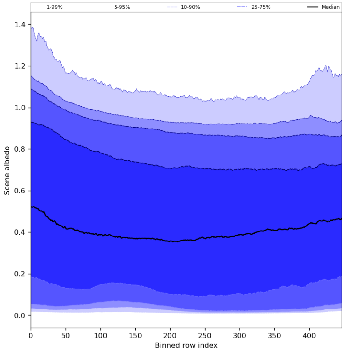
Figure 51: Along track statistics of “Scene albedo” for 2023-10-28 to 2023-10-30
