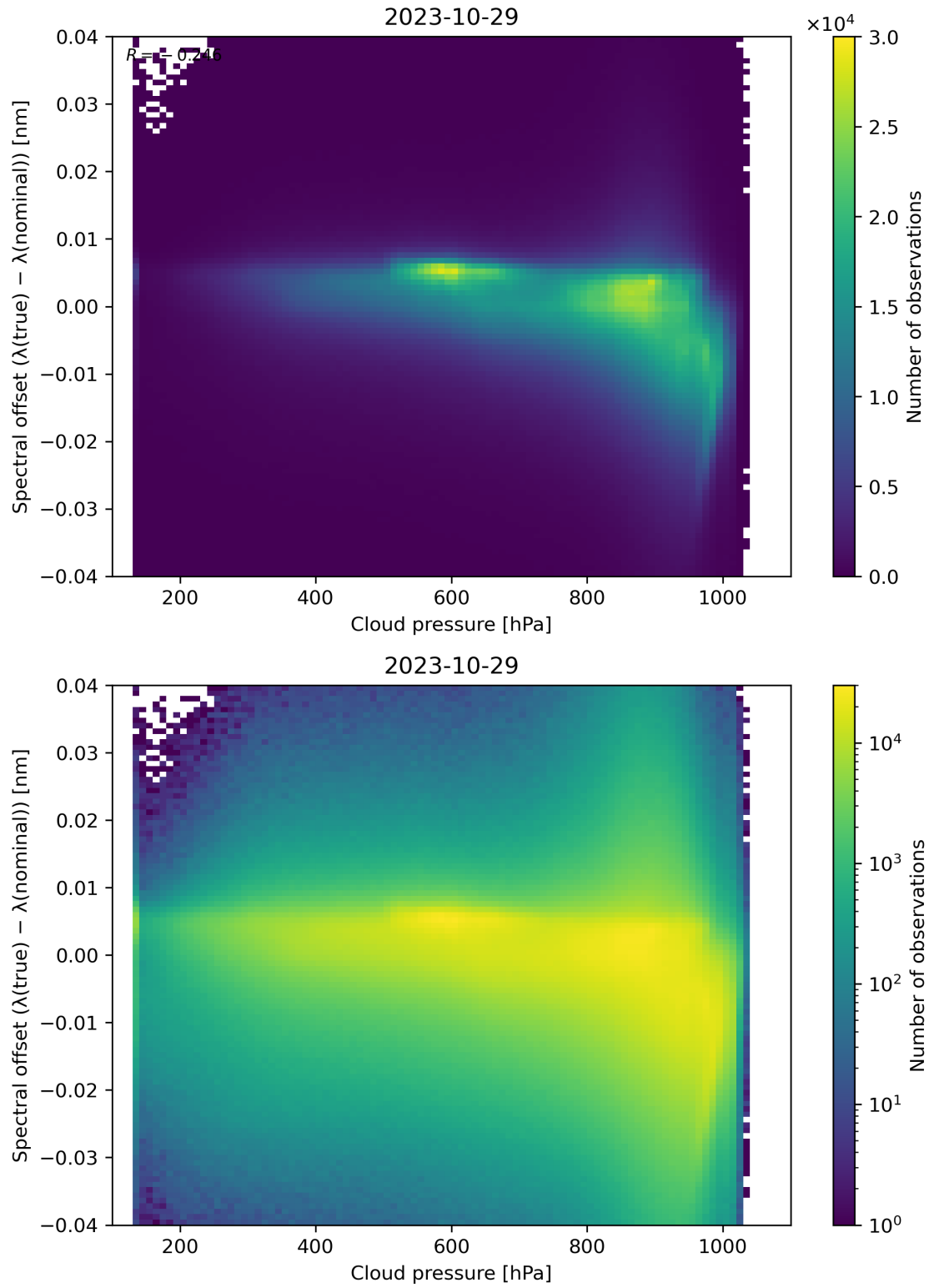
Figure 92: Scatter density plot of “Cloud pressure” against “Spectral offset ( \lambda(\text{true}) - \lambda(\text{nominal}) )” for 2023-10-28 to 2023-10-30.
