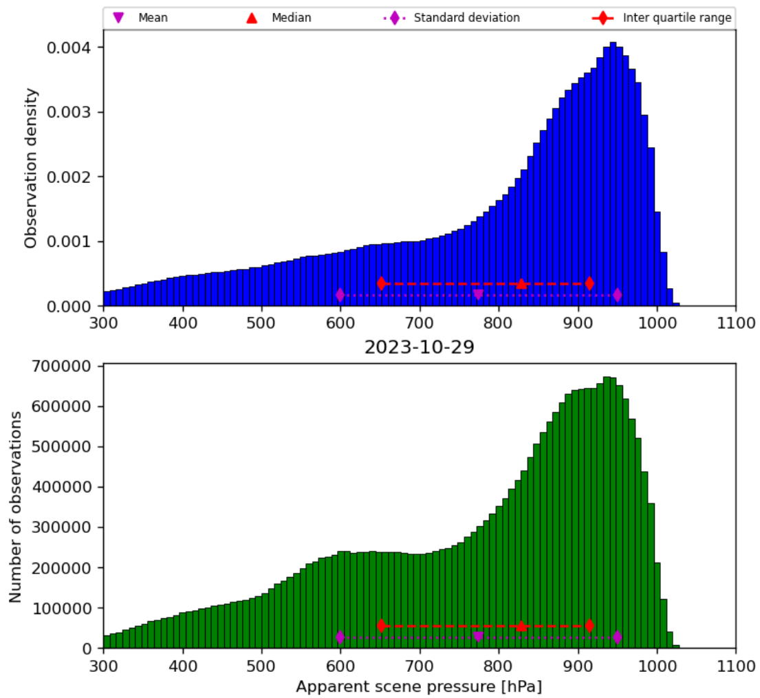
Figure 36: Histogram of “Apparent scene pressure” for 2023-10-28 to 2023-10-30
