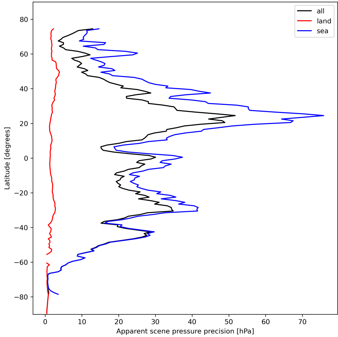
Figure 20: Zonal average of “Apparent scene pressure precision” for 2023-10-28 to 2023-10-30.
