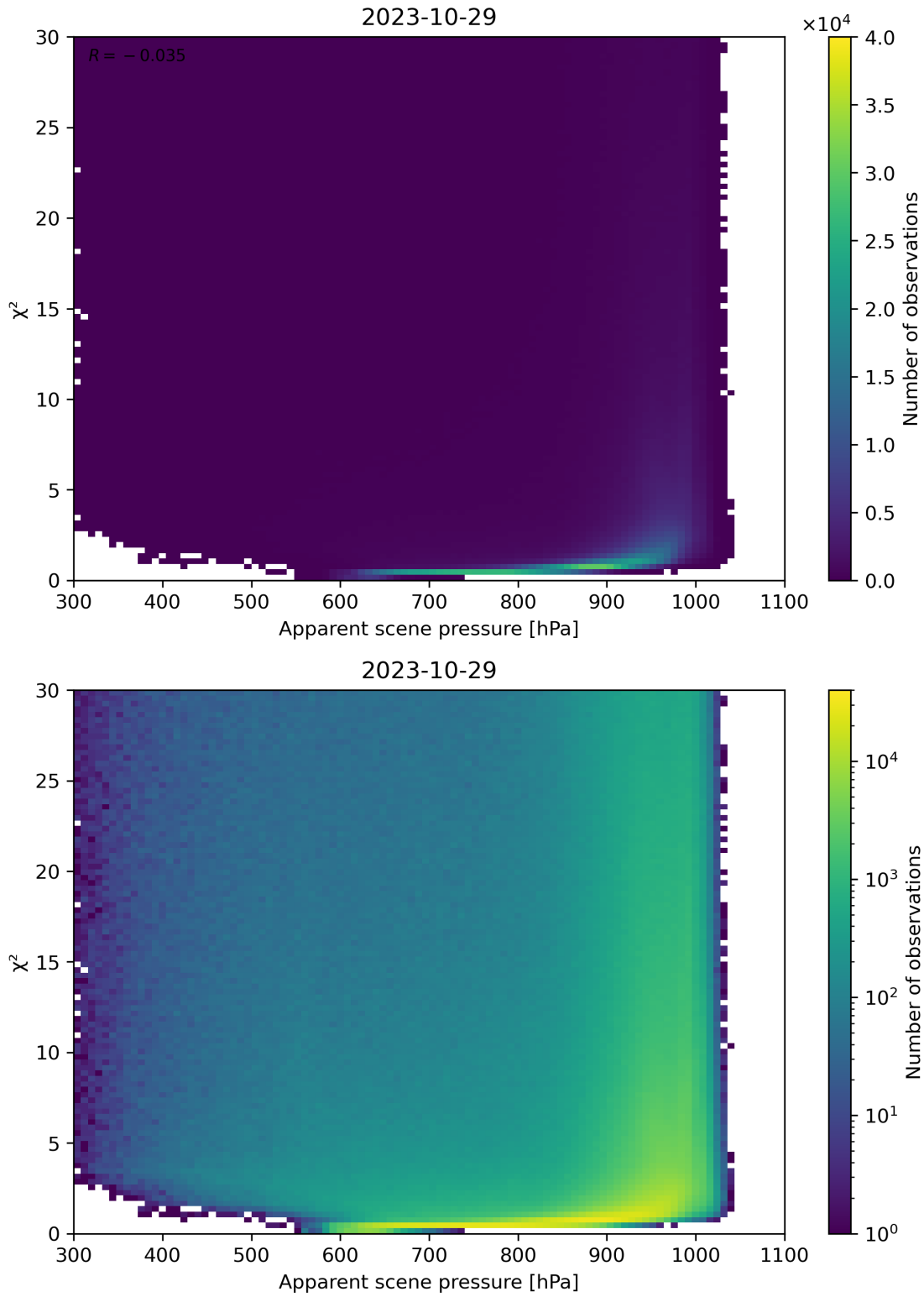
Figure 63: Scatter density plot of “Apparent scene pressure” against “ \chi^2 ” for 2023-10-28 to 2023-10-30.
