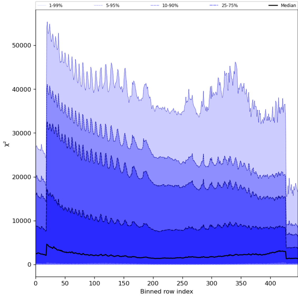
Figure 55: Along track statistics of “ \chi^2 ” for 2023-10-28 to 2023-10-30
