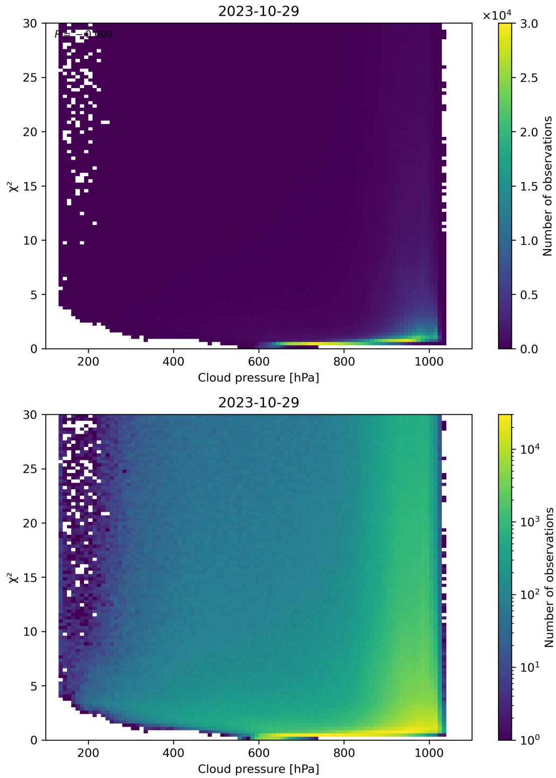
Figure 85: Scatter density plot of “Cloud pressure” against “ \chi^2 ” for 2023-10-28 to 2023-10-30.
