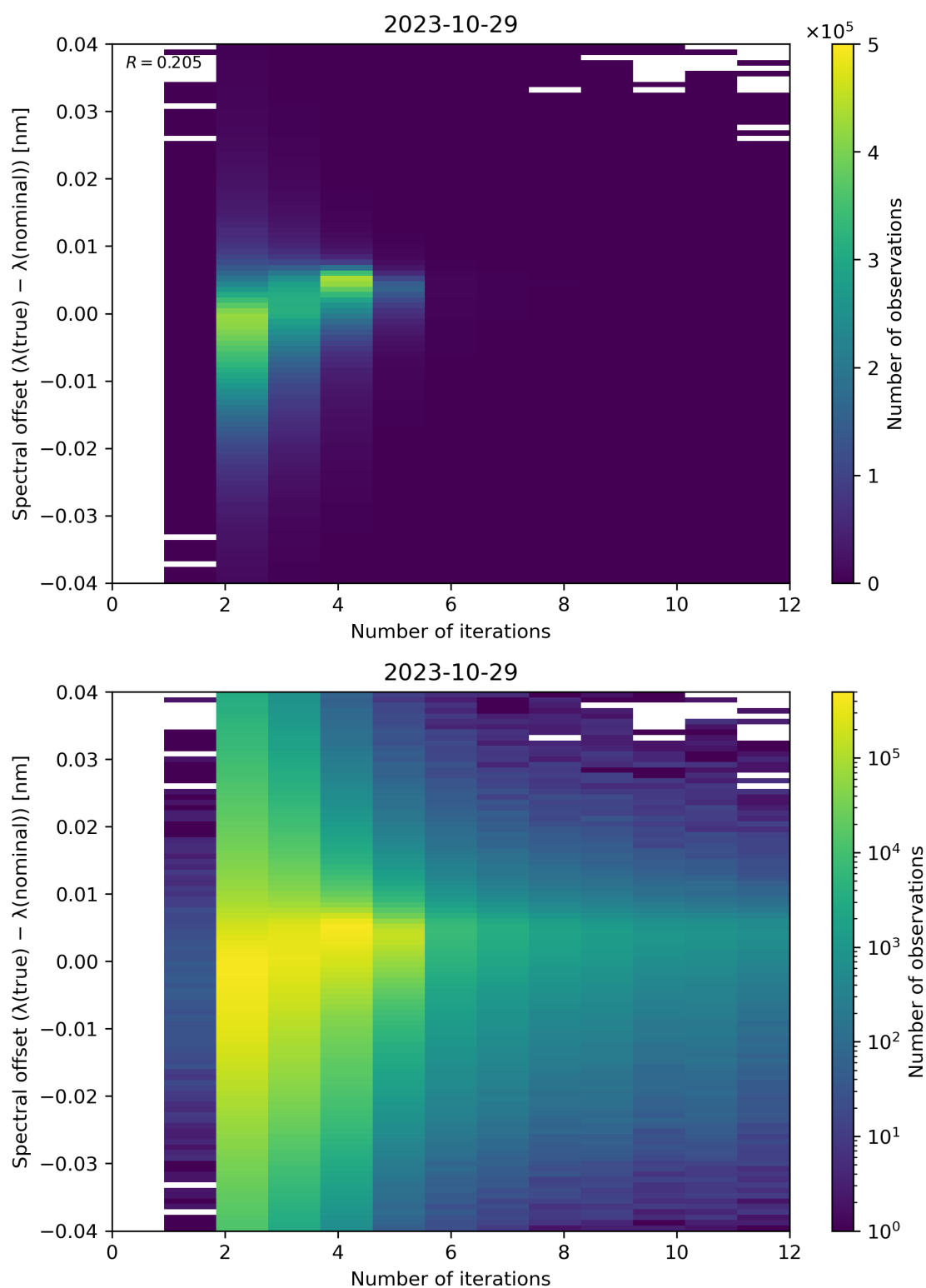
Figure 109: Scatter density plot of “Number of iterations” against “Spectral offset ( \lambda(\text{true}) - \lambda(\text{nominal}) )” for 2023-10-28 to 2023-10-30.
