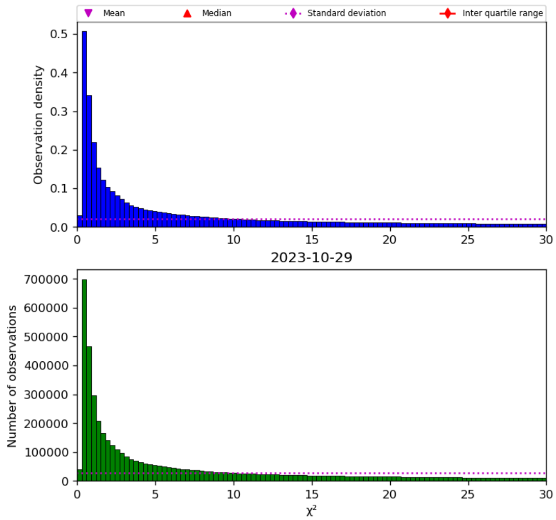
Figure 38: Histogram of " \chi^2 " for 2023-10-28 to 2023-10-30
