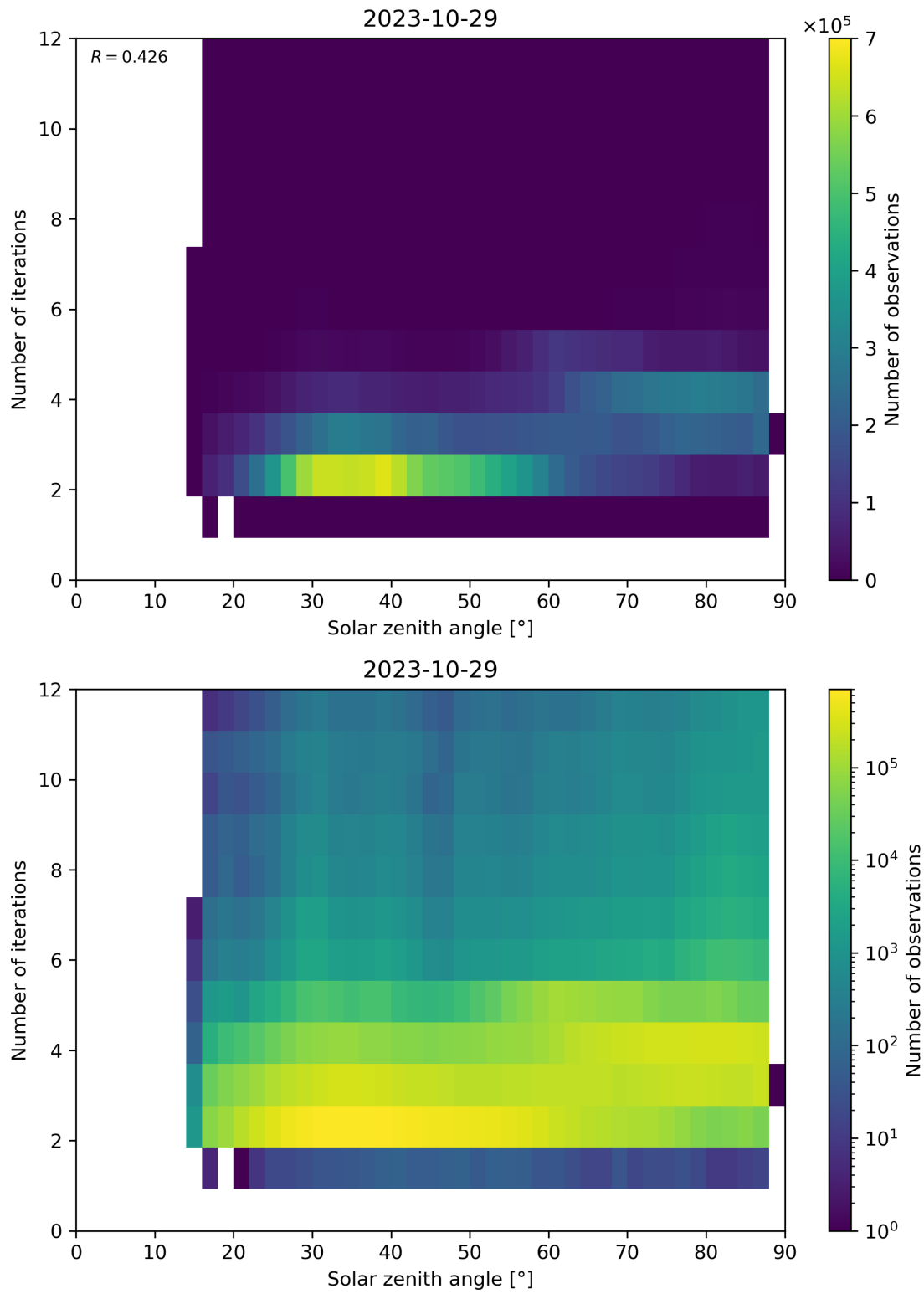
Figure 125: Scatter density plot of “Solar zenith angle” against “Number of iterations” for 2023-10-28 to 2023-10-30.
