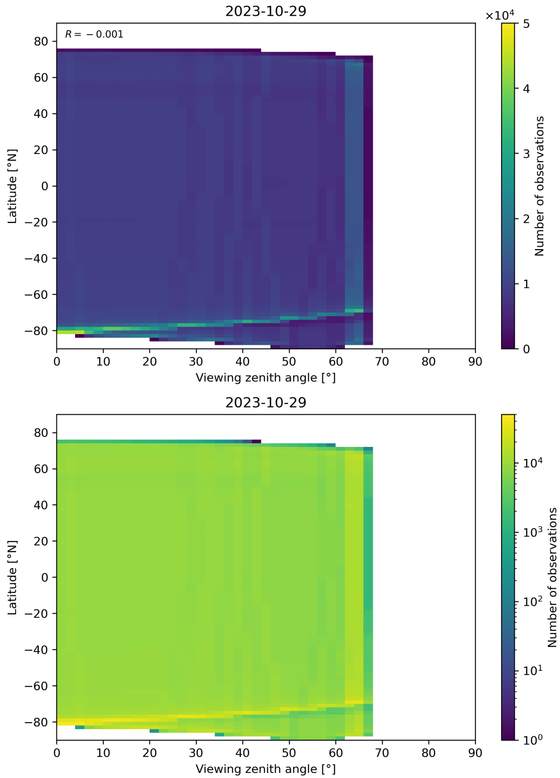
Figure 135: Scatter density plot of “Viewing zenith angle” against “Latitude” for 2023-10-28 to 2023-10-30.
