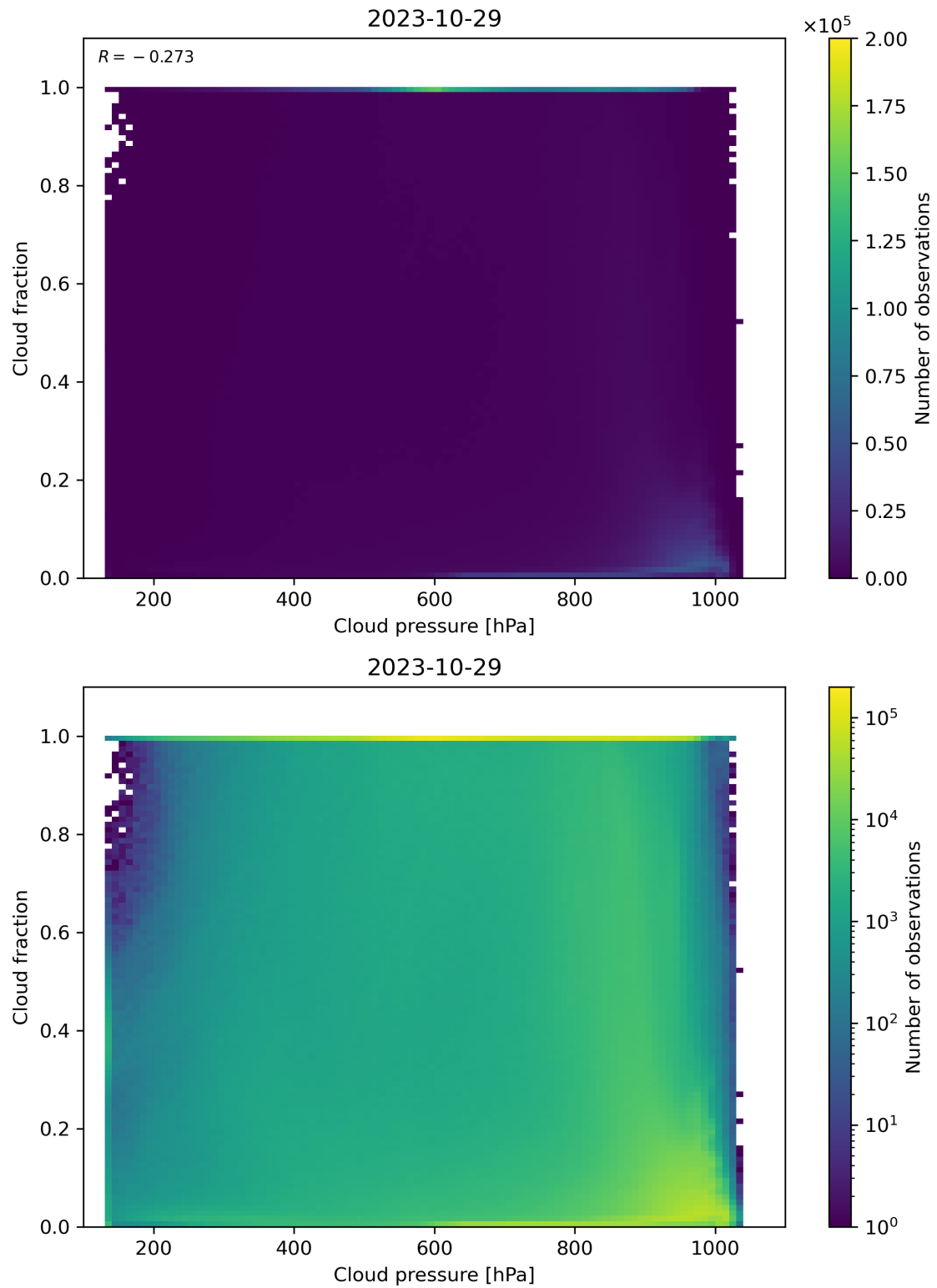
Figure 87: Scatter density plot of “Cloud pressure” against “Cloud fraction” for 2023-10-28 to 2023-10-30.
