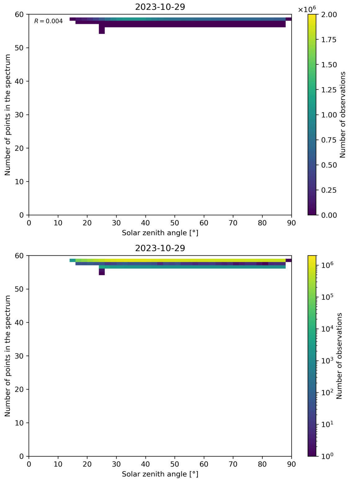
Figure 126: Scatter density plot of “Solar zenith angle” against “Number of points in the spectrum” for 2023-10-28 to 2023-10-30.
