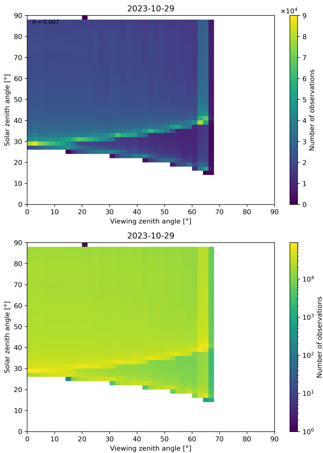
Figure 139: Scatter density plot of “Viewing zenith angle” against “Solar zenith angle” for 2023-10-28 to 2023-10-30.
