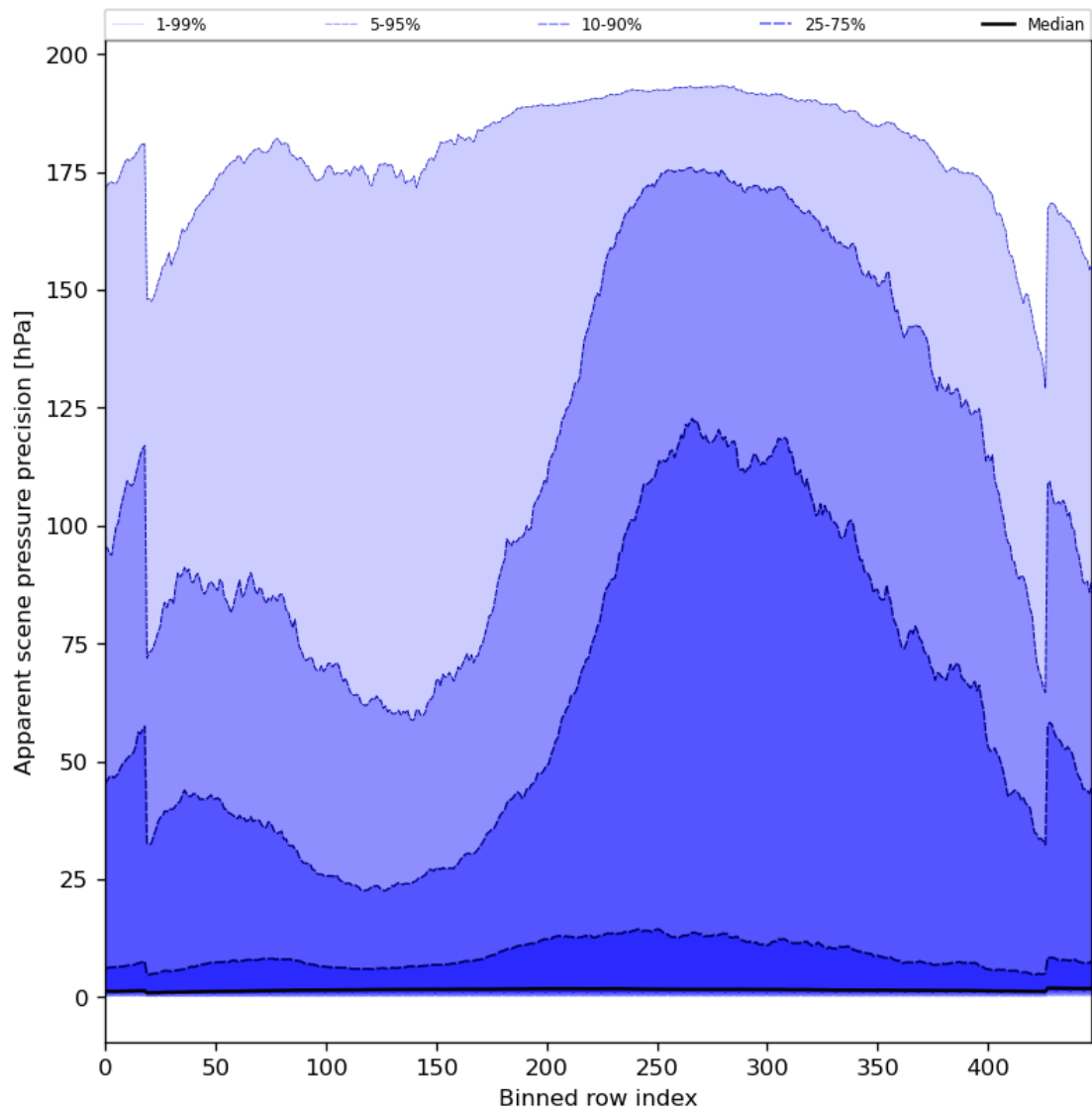
Figure 54: Along track statistics of “Apparent scene pressure precision” for 2023-10-28 to 2023-10-30
