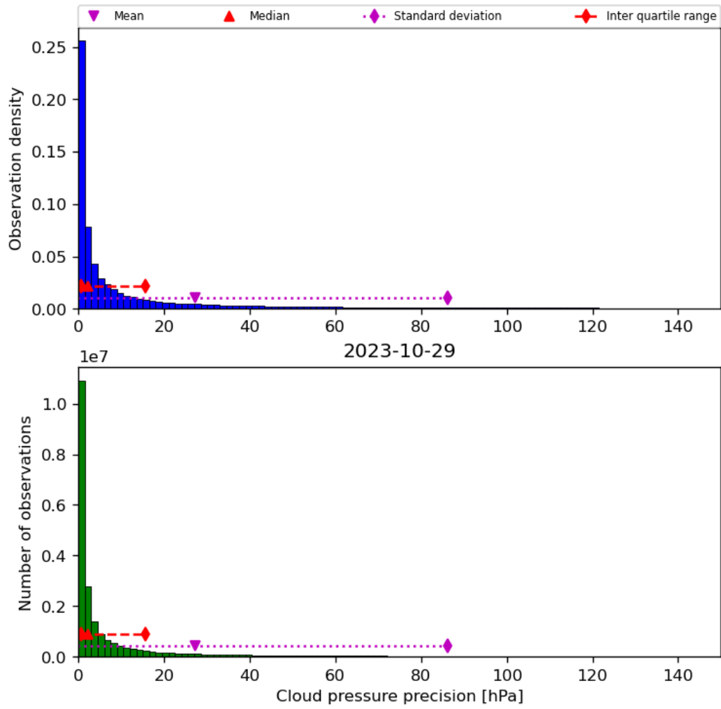
Figure 31: Histogram of “Cloud pressure precision” for 2023-10-28 to 2023-10-30
