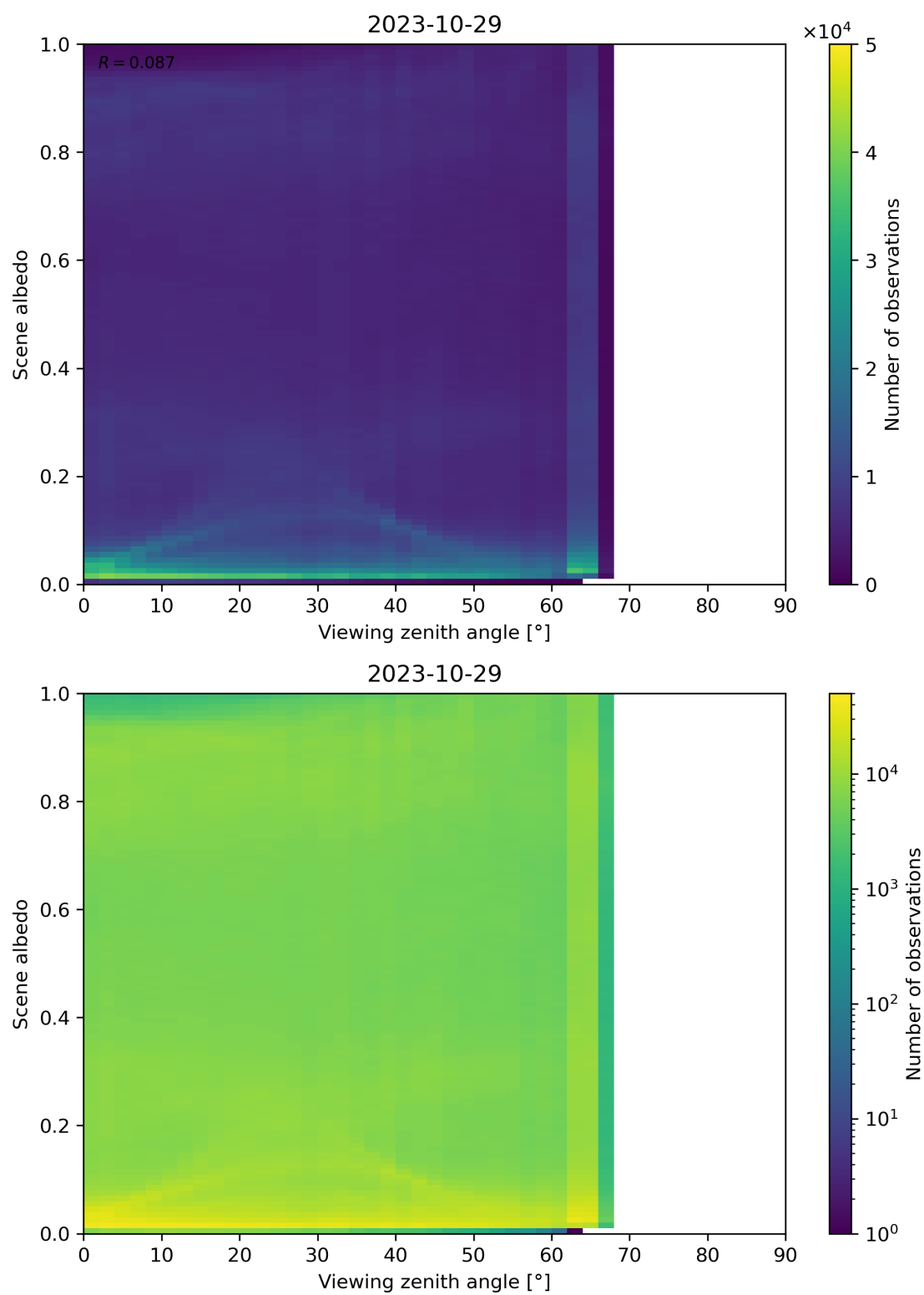
Figure 138: Scatter density plot of “Viewing zenith angle” against “Scene albedo” for 2023-10-28 to 2023-10-30.
