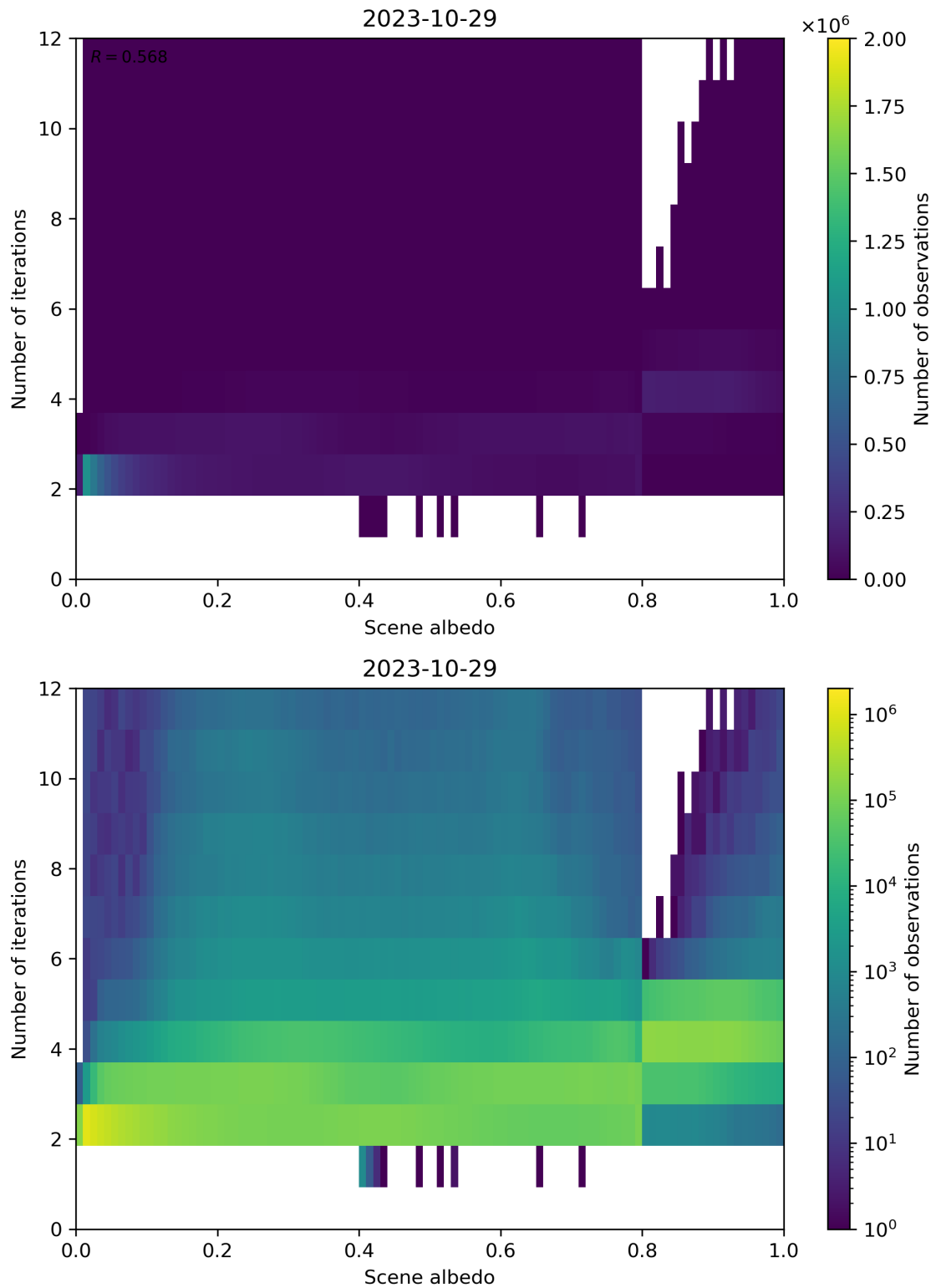
Figure 115: Scatter density plot of “Scene albedo” against “Number of iterations” for 2023-10-28 to 2023-10-30.
