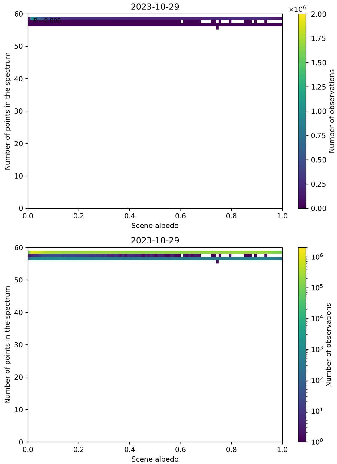
Figure 116: Scatter density plot of “Scene albedo” against “Number of points in the spectrum” for 2023-10-28 to 2023-10-30.
