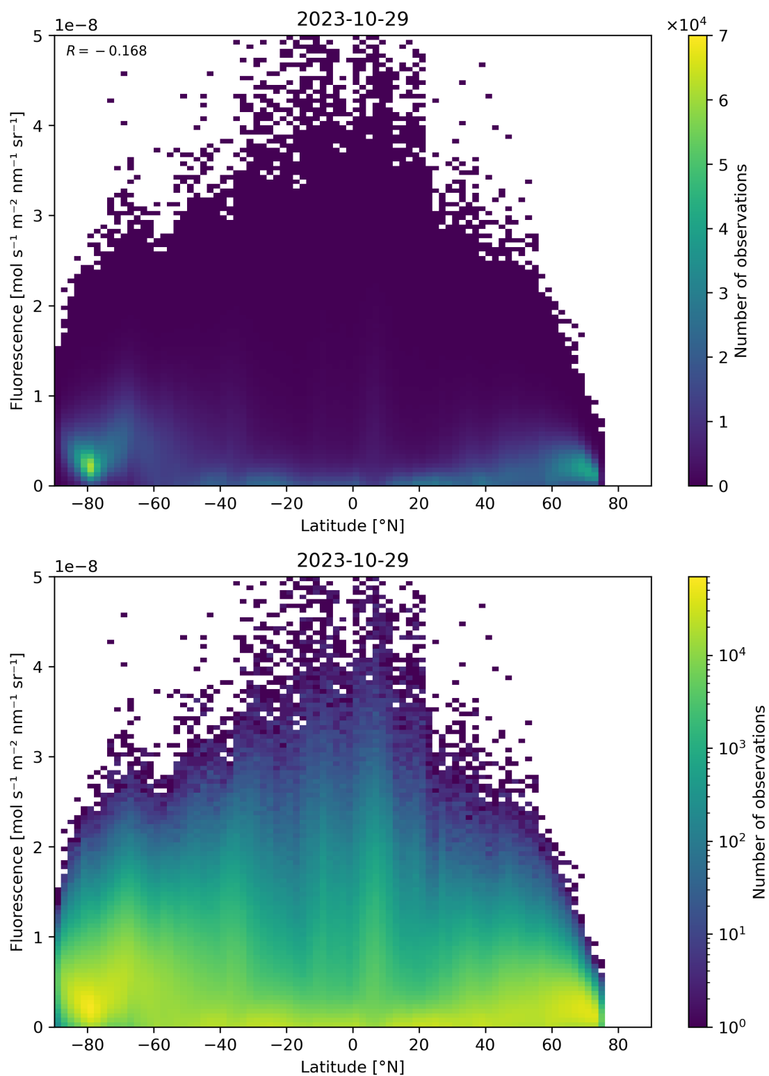
Figure 101: Scatter density plot of “Latitude” against “Fluorescence” for 2023-10-28 to 2023-10-30.
