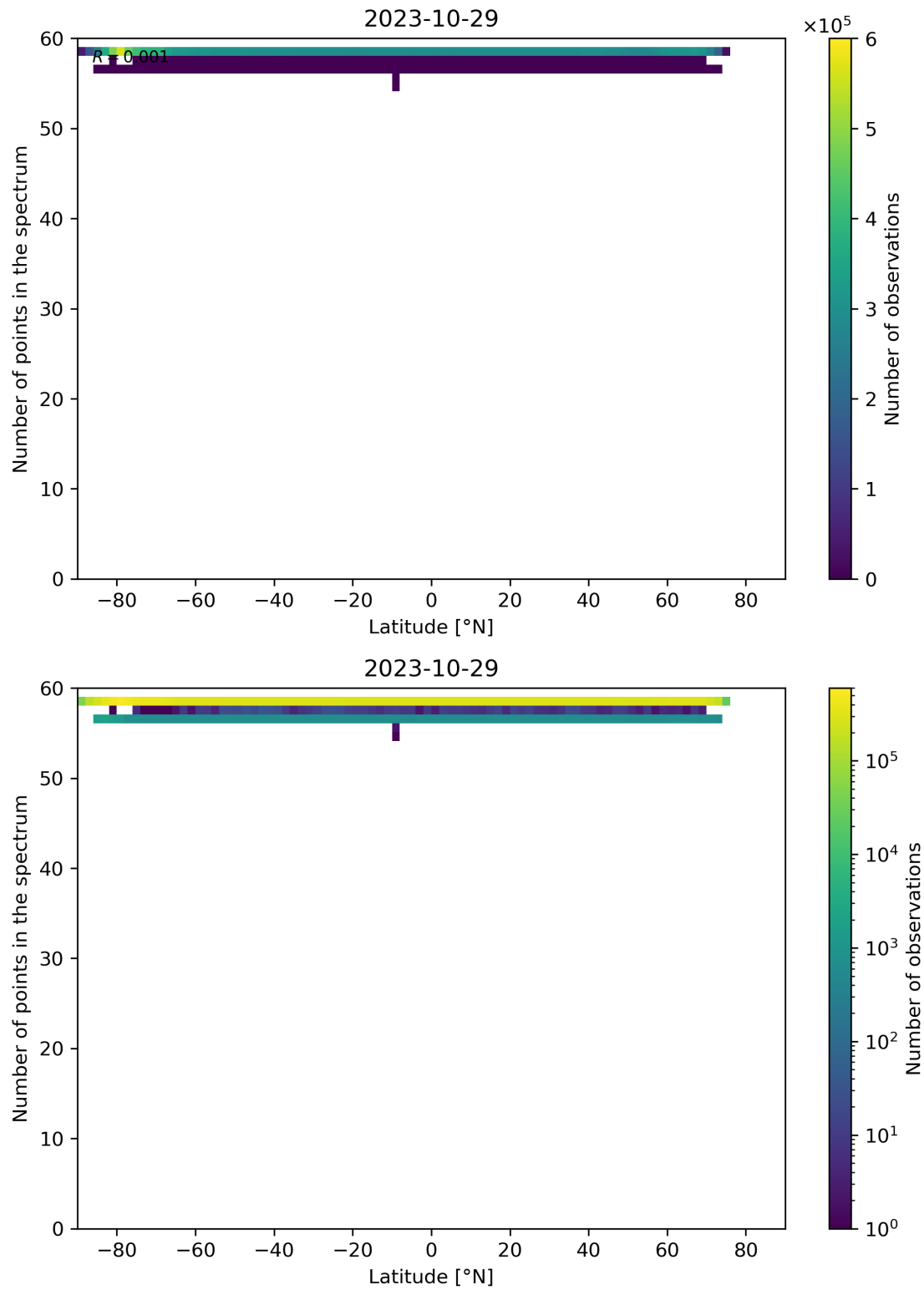
Figure 103: Scatter density plot of “Latitude” against “Number of points in the spectrum” for 2023-10-28 to 2023-10-30.
