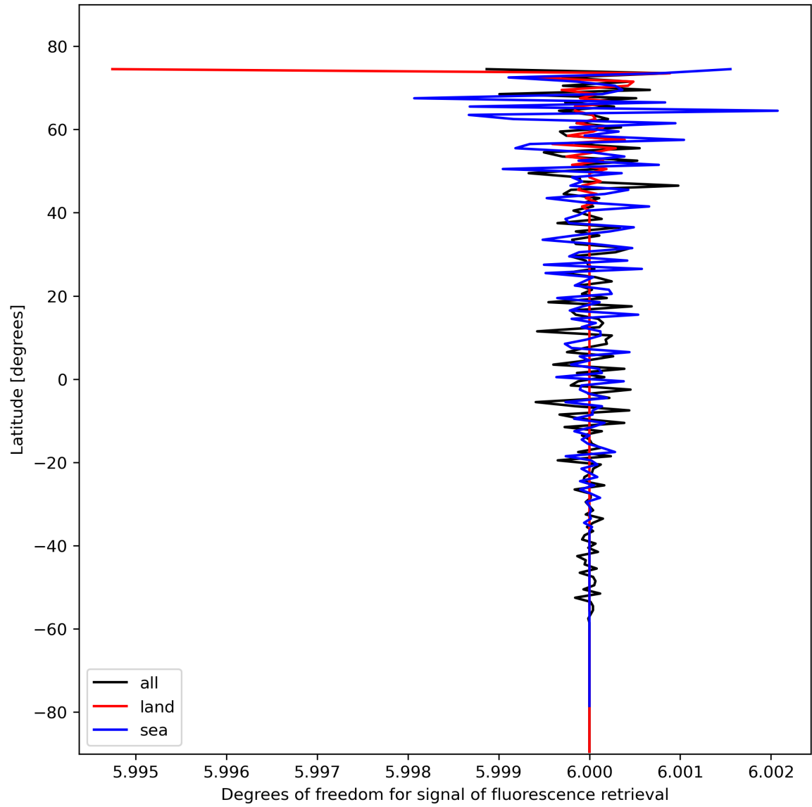
Figure 26: Zonal average of “Degrees of freedom for signal of fluorescence retrieval” for 2023-10-28 to 2023-10-30.
