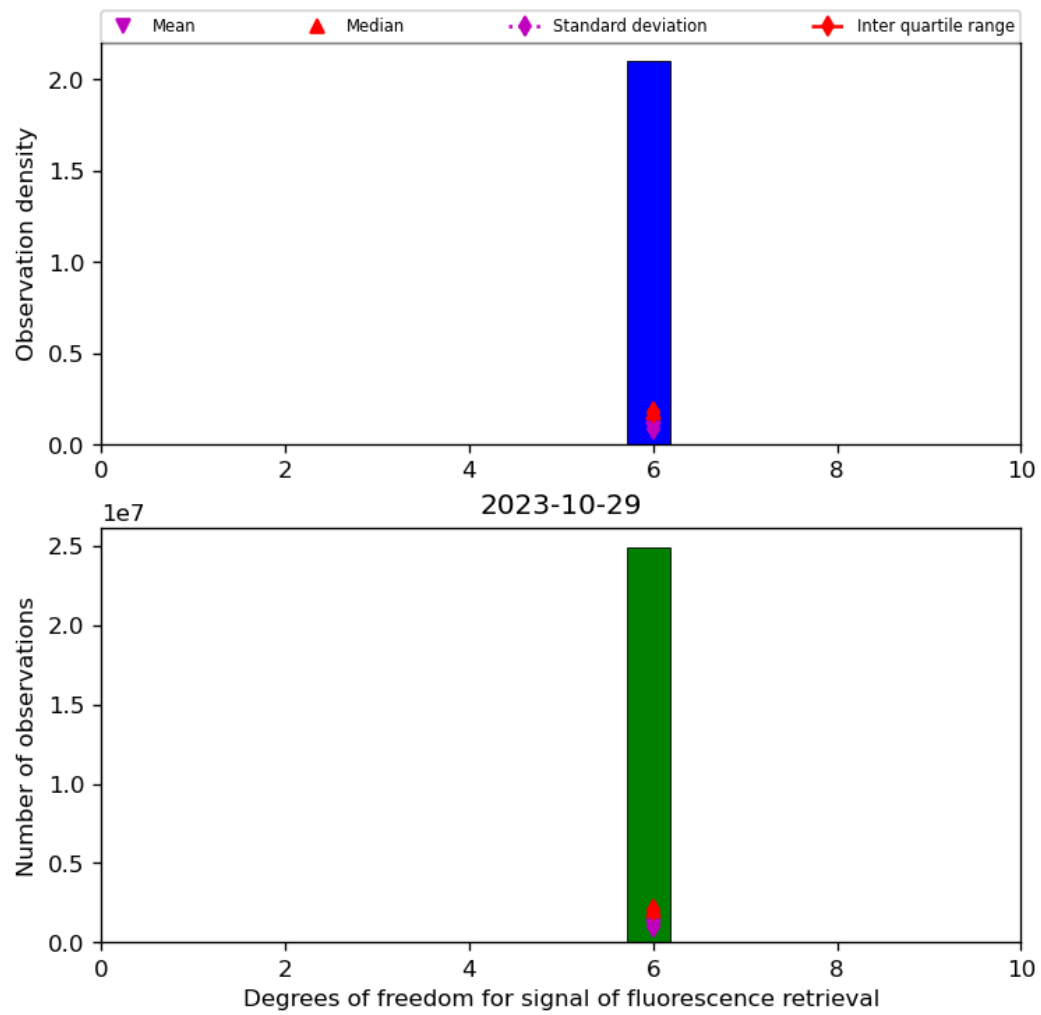
Figure 43: Histogram of “Degrees of freedom for signal of fluorescence retrieval” for 2023-10-28 to 2023-10-30
