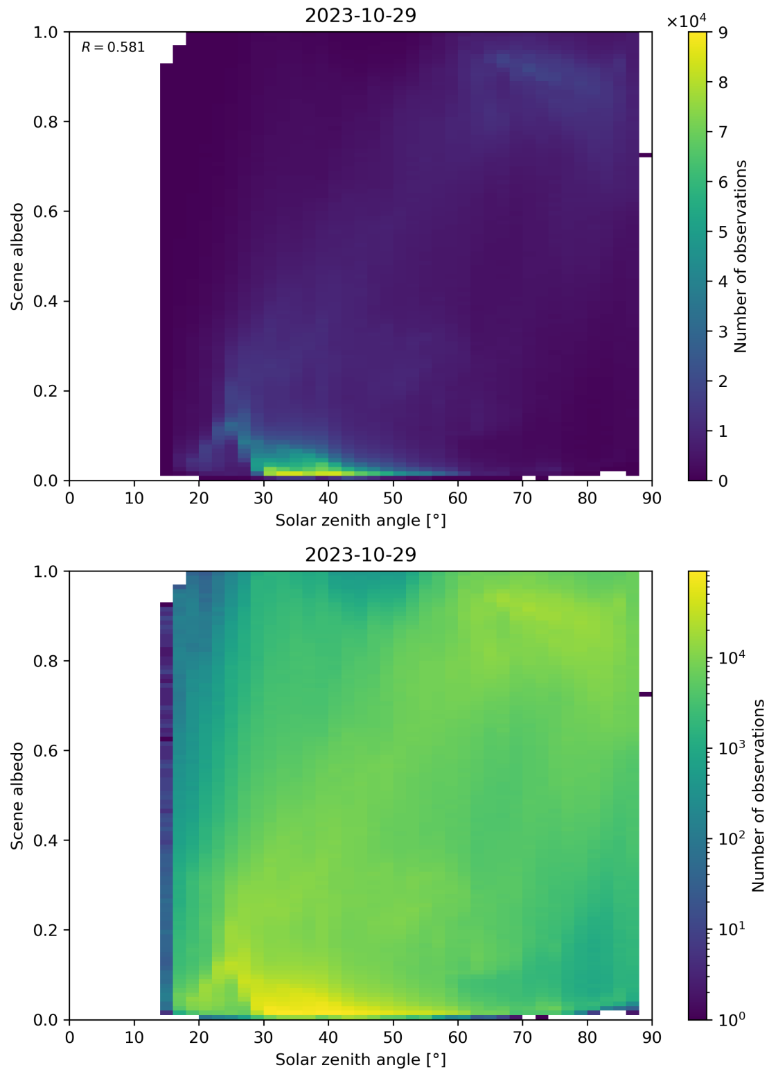
Figure 127: Scatter density plot of “Solar zenith angle” against “Scene albedo” for 2023-10-28 to 2023-10-30.
