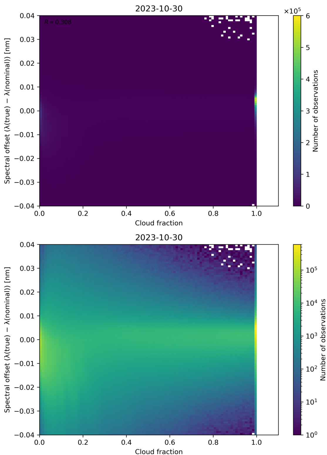
Figure 83: Scatter density plot of “Cloud fraction” against “Spectral offset ( \lambda(\text{true}) - \lambda(\text{nominal}) )” for 2023-10-29 to 2023-10-31.
