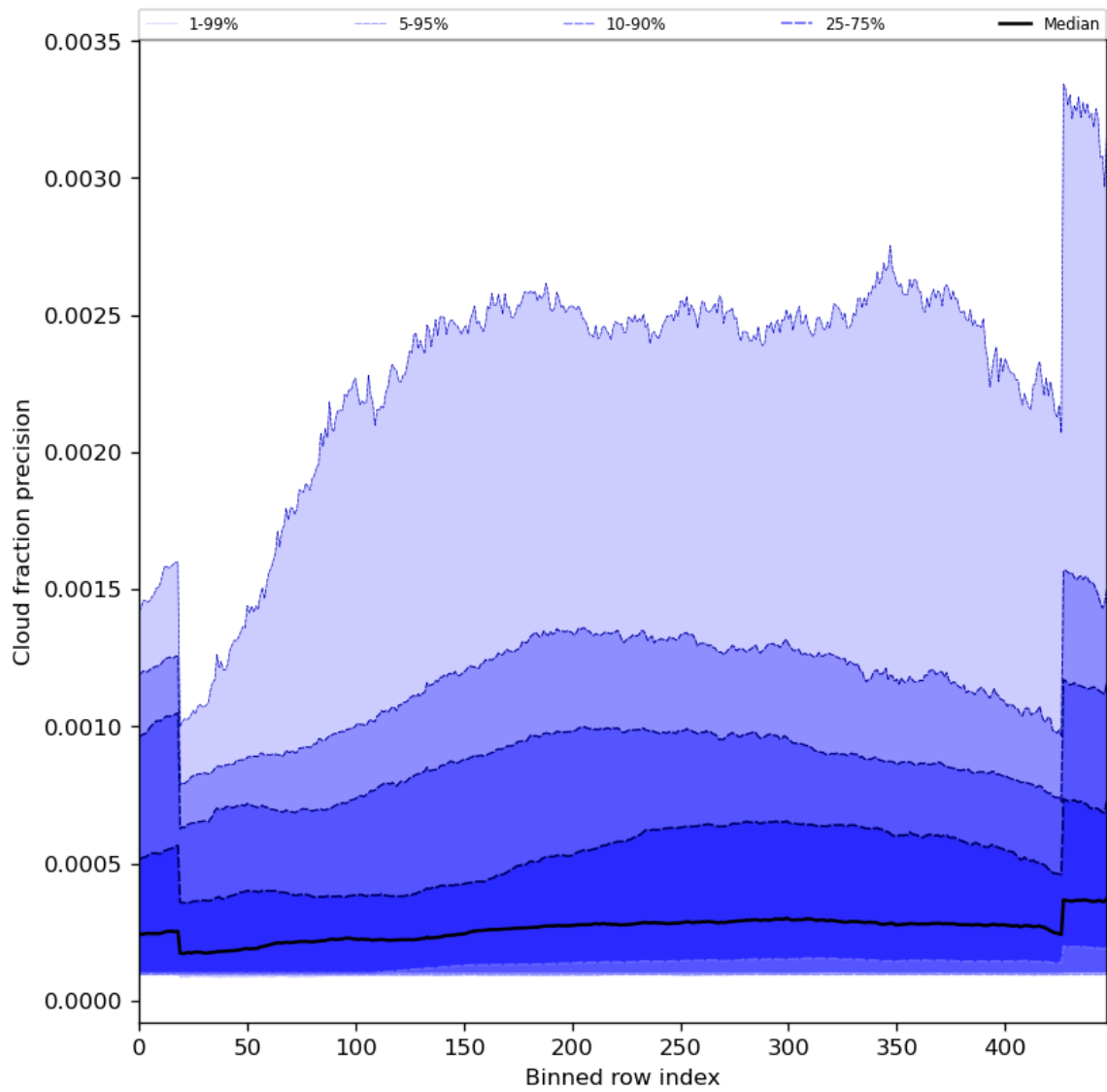
Figure 50: Along track statistics of “Cloud fraction precision” for 2023-10-29 to 2023-10-31
