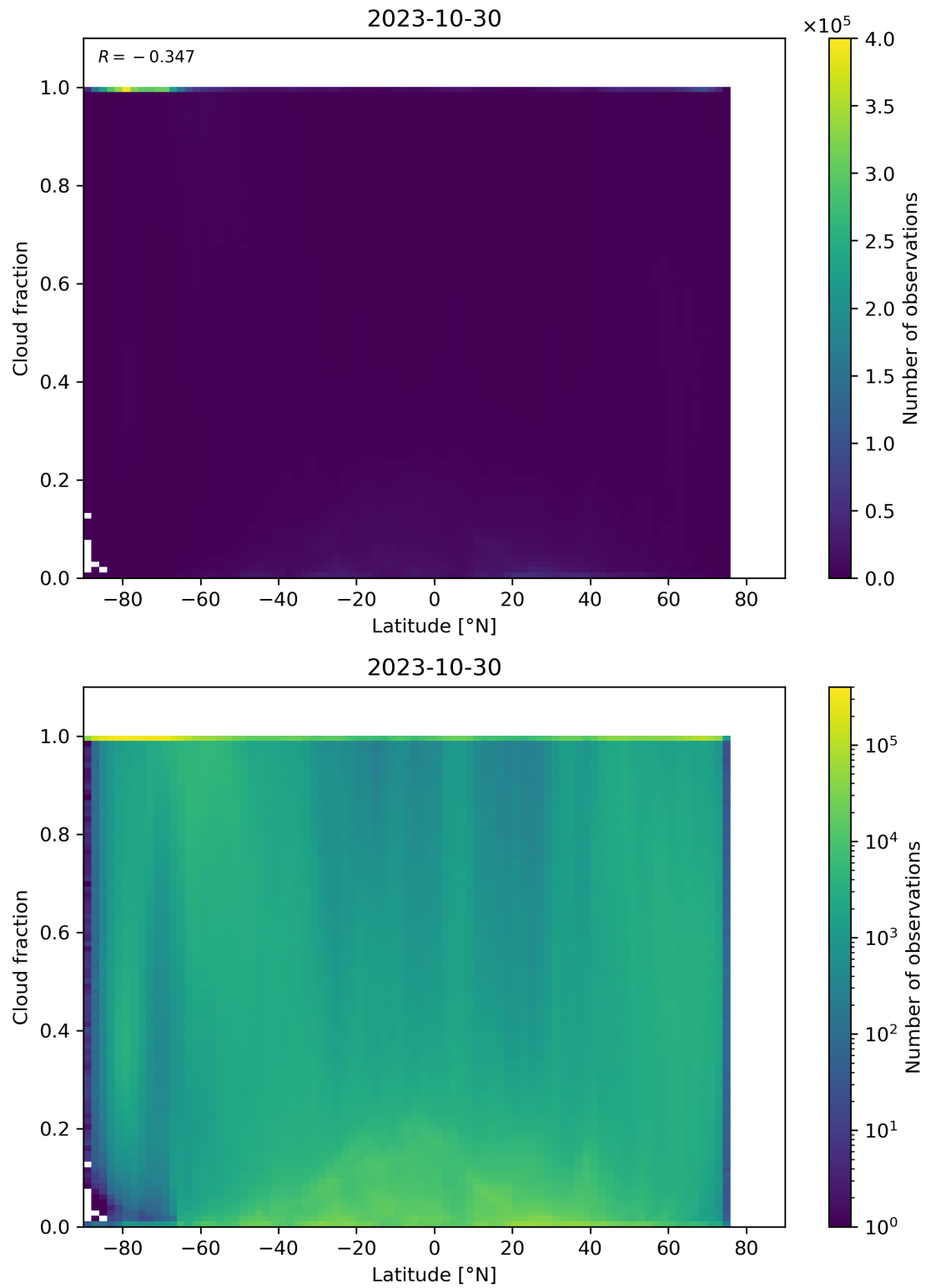
Figure 99: Scatter density plot of “Latitude” against “Cloud fraction” for 2023-10-29 to 2023-10-31.
