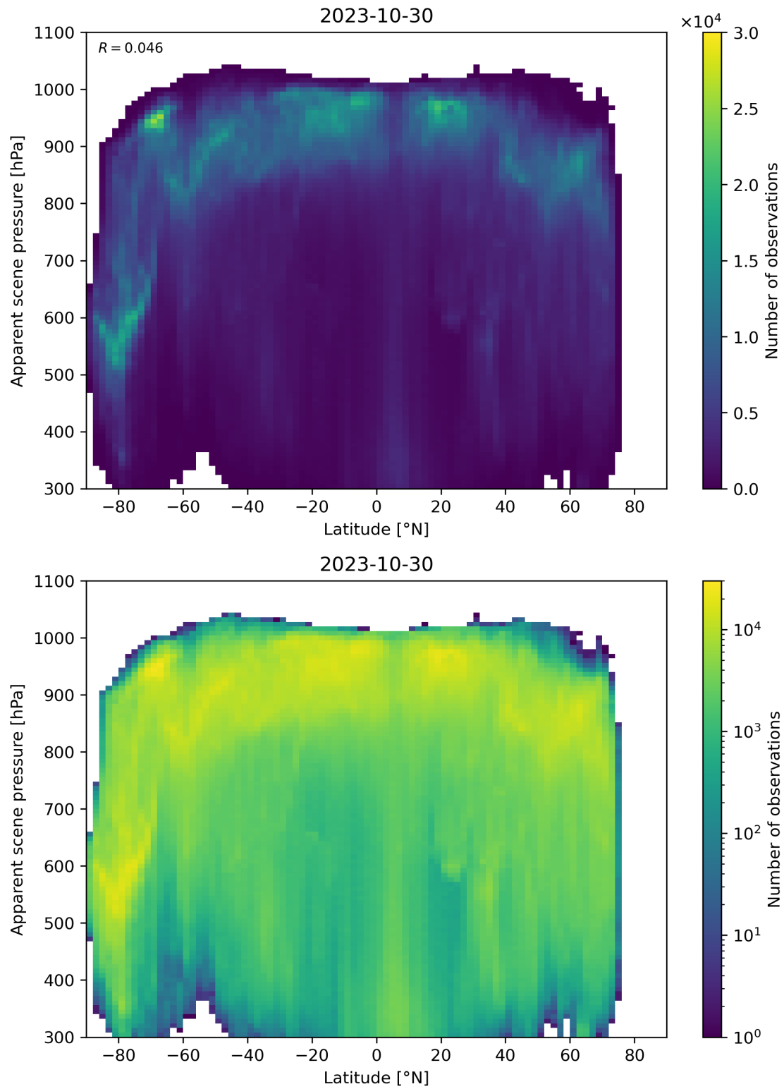
Figure 96: Scatter density plot of “Latitude” against “Apparent scene pressure” for 2023-10-29 to 2023-10-31.
