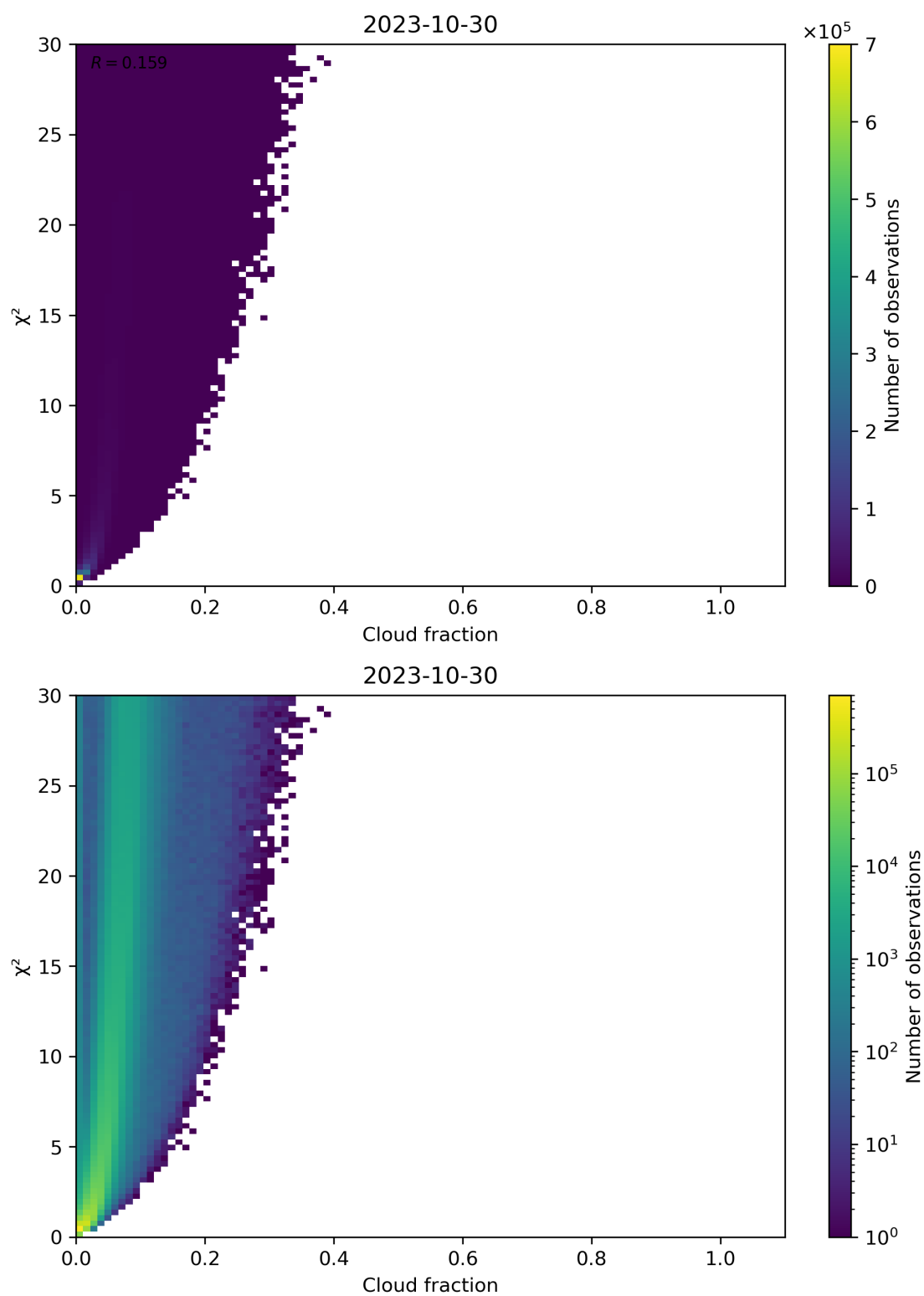
Figure 77: Scatter density plot of “Cloud fraction” against “ \chi^2 ” for 2023-10-29 to 2023-10-31.
