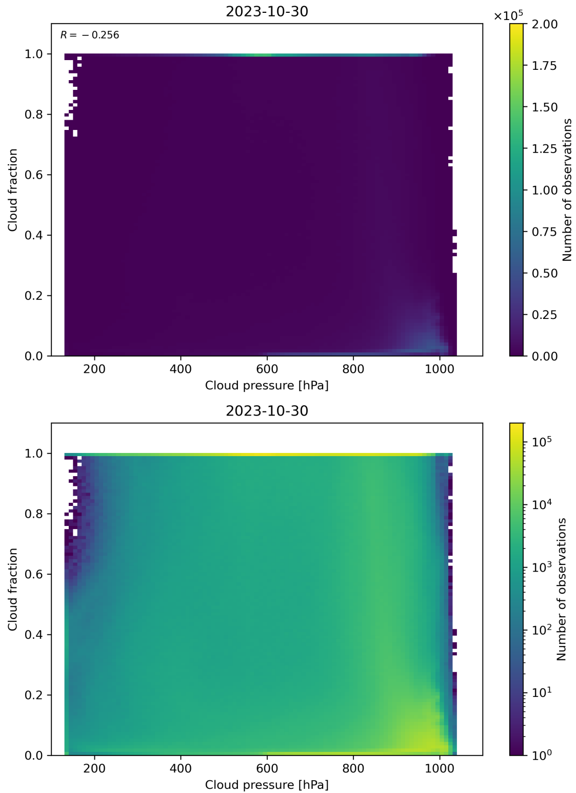
Figure 87: Scatter density plot of “Cloud pressure” against “Cloud fraction” for 2023-10-29 to 2023-10-31.
