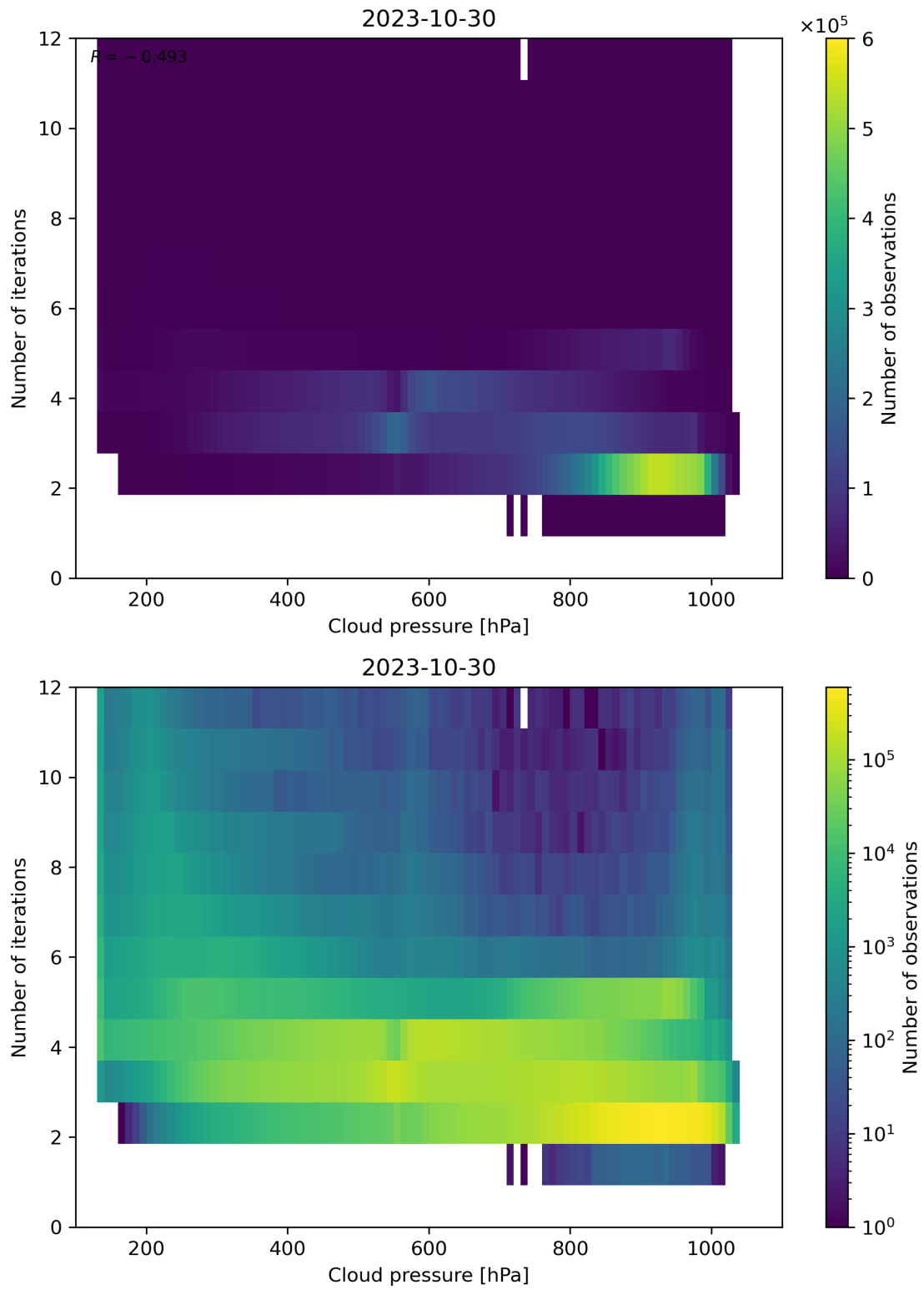
Figure 89: Scatter density plot of “Cloud pressure” against “Number of iterations” for 2023-10-29 to 2023-10-31.
