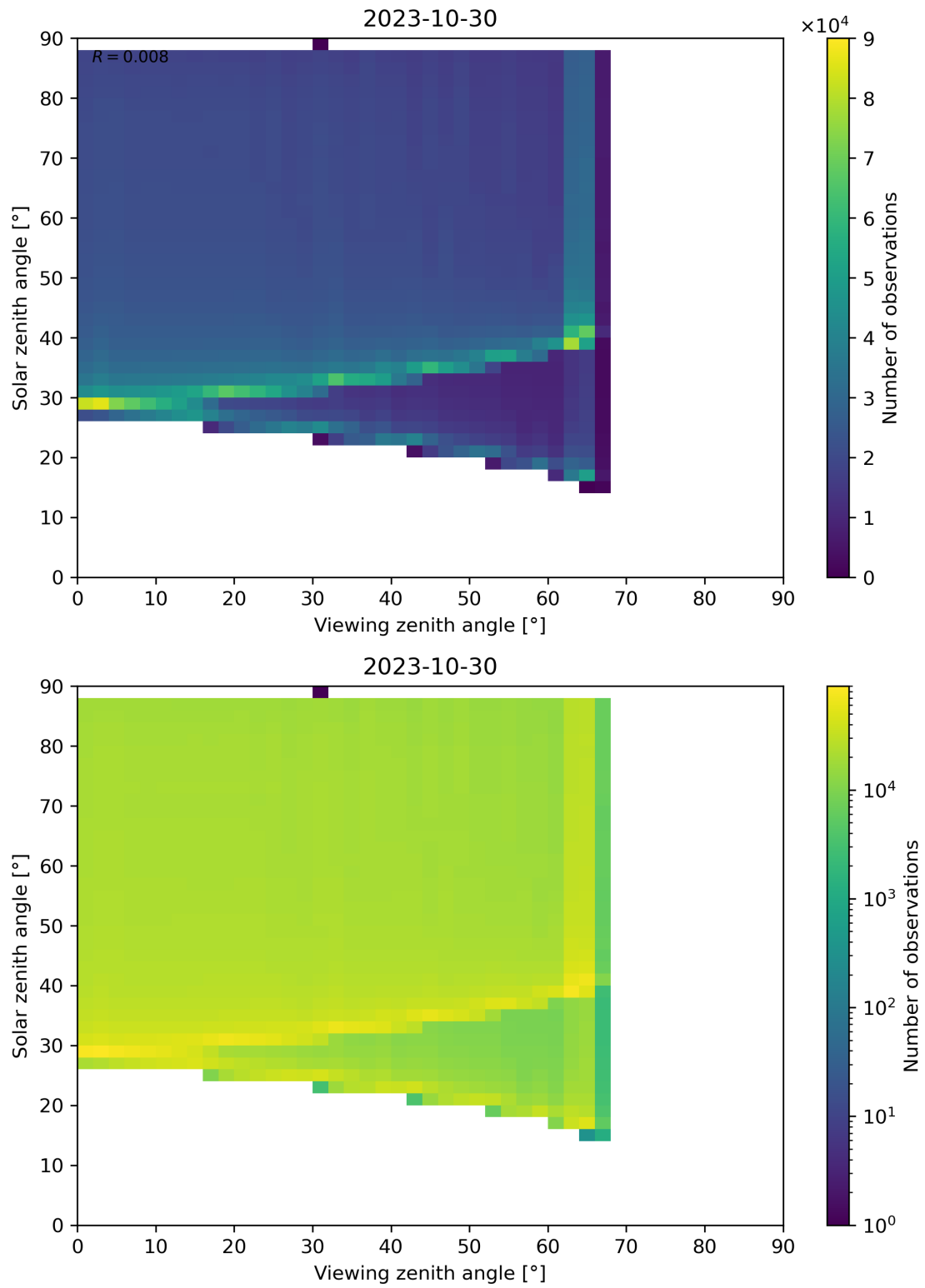
Figure 139: Scatter density plot of “Viewing zenith angle” against “Solar zenith angle” for 2023-10-29 to 2023-10-31.
