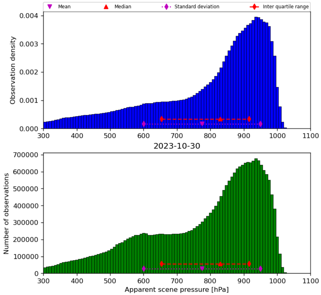
Figure 36: Histogram of “Apparent scene pressure” for 2023-10-29 to 2023-10-31
