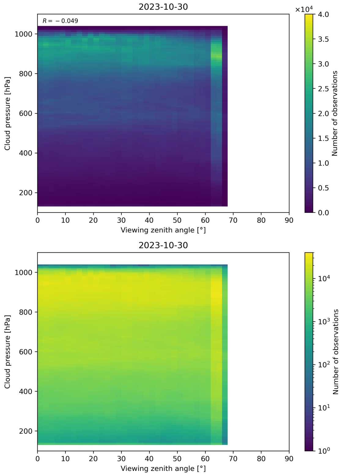
Figure 133: Scatter density plot of “Viewing zenith angle” against “Cloud pressure” for 2023-10-29 to 2023-10-31.
