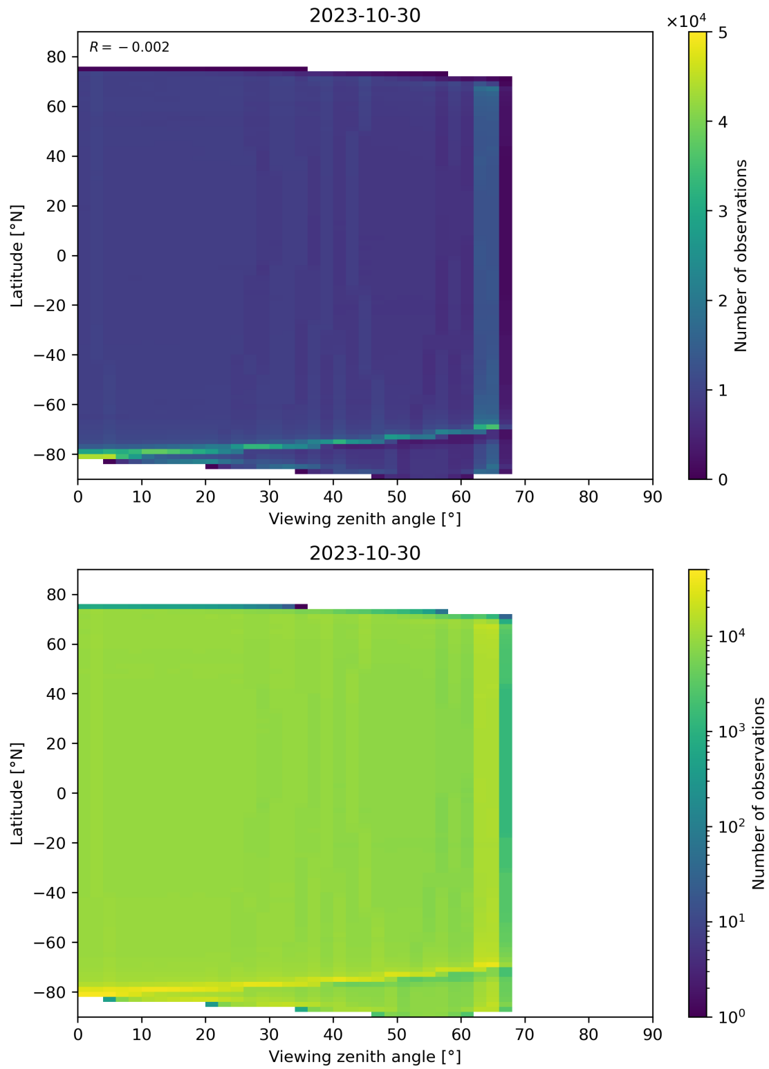
Figure 135: Scatter density plot of “Viewing zenith angle” against “Latitude” for 2023-10-29 to 2023-10-31.
