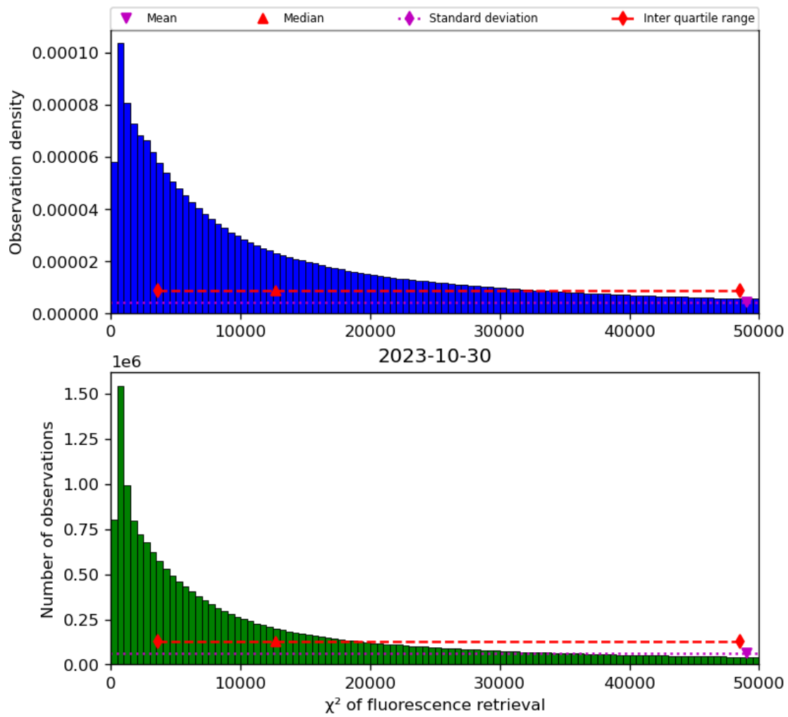
Figure 42: Histogram of “ \chi^2 of fluorescence retrieval” for 2023-10-29 to 2023-10-31
