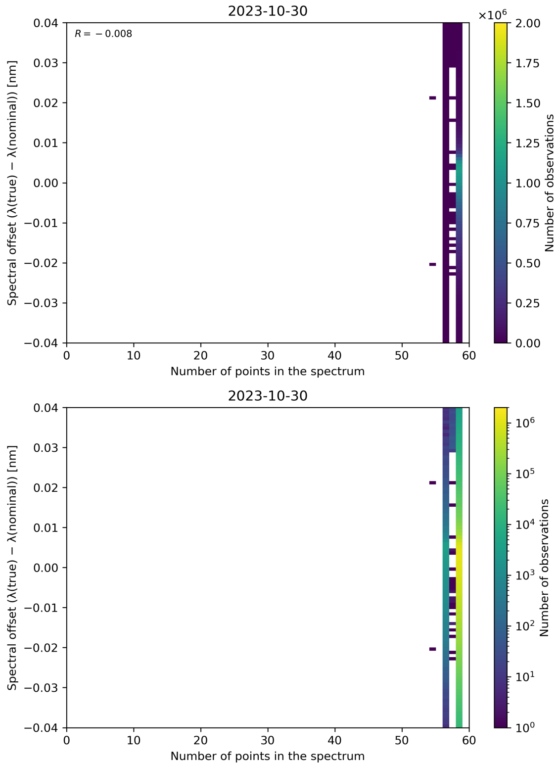
Figure 110: Scatter density plot of “Number of points in the spectrum” against “Spectral offset ( \lambda(\text{true}) - \lambda(\text{nominal}) )” for 2023-10-29 to 2023-10-31.
