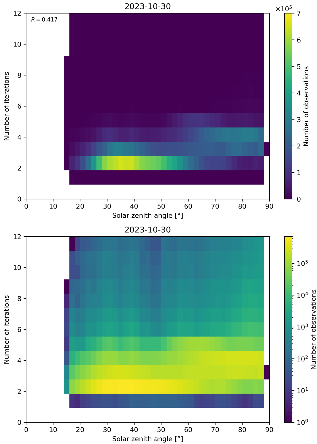
Figure 125: Scatter density plot of “Solar zenith angle” against “Number of iterations” for 2023-10-29 to 2023-10-31.
