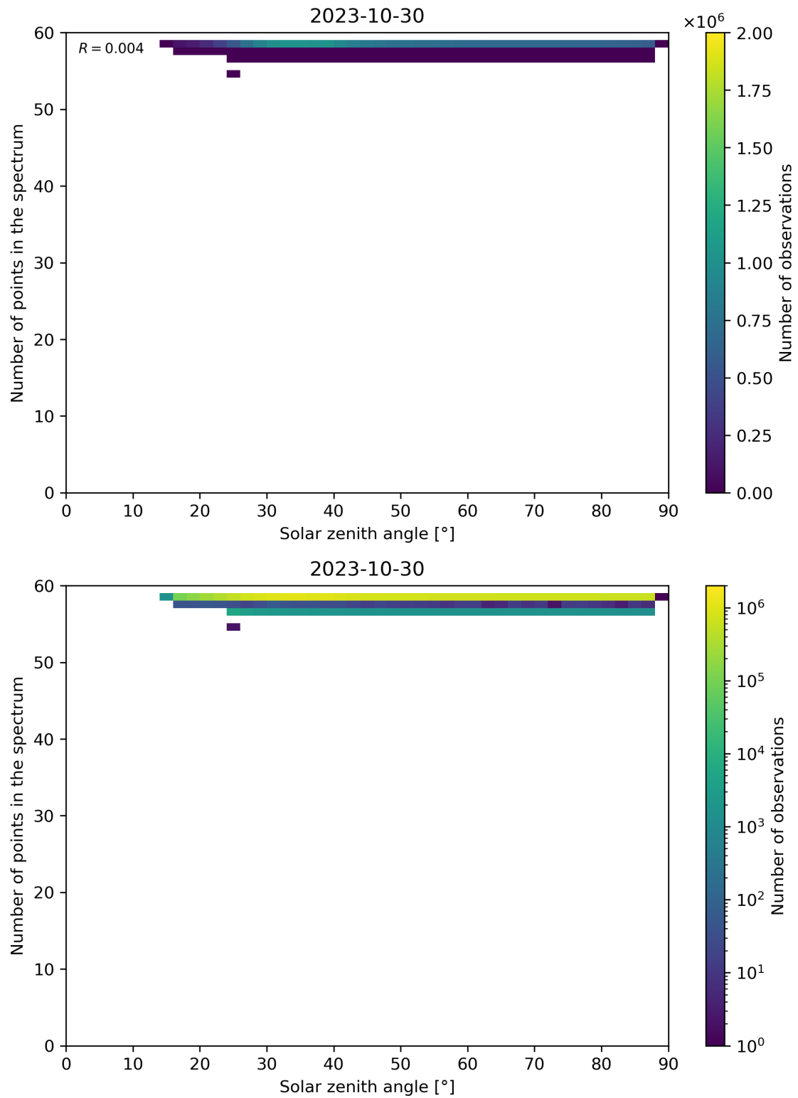
Figure 126: Scatter density plot of “Solar zenith angle” against “Number of points in the spectrum” for 2023-10-29 to 2023-10-31.
