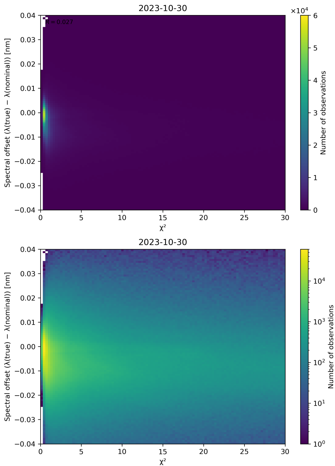
Figure 75: Scatter density plot of “ \chi^2 ” against “Spectral offset ( \lambda(\text{true}) - \lambda(\text{nominal}) )” for 2023-10-29 to 2023-10-31.
