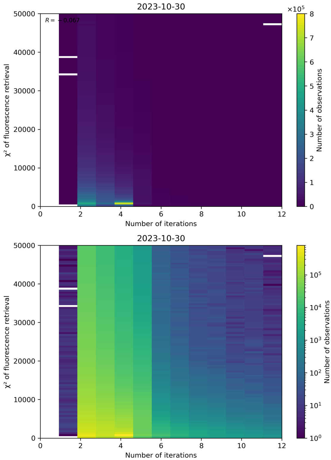
Figure 106: Scatter density plot of “Number of iterations” against “ \chi^2 of fluorescence retrieval” for 2023-10-29 to 2023-10-31.
