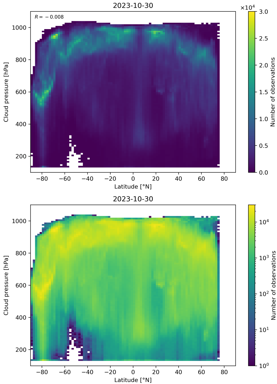
Figure 100: Scatter density plot of “Latitude” against “Cloud pressure” for 2023-10-29 to 2023-10-31.
