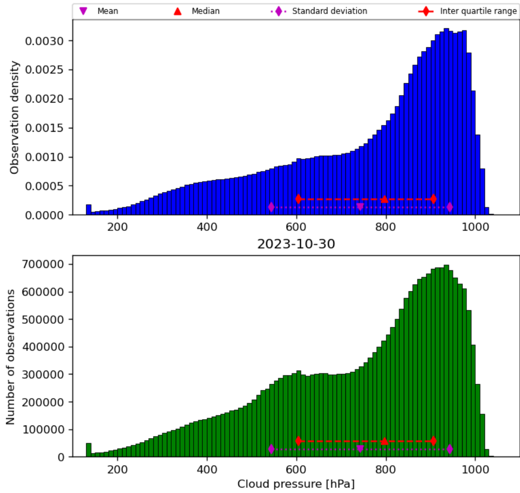
Figure 30: Histogram of “Cloud pressure” for 2023-10-29 to 2023-10-31
