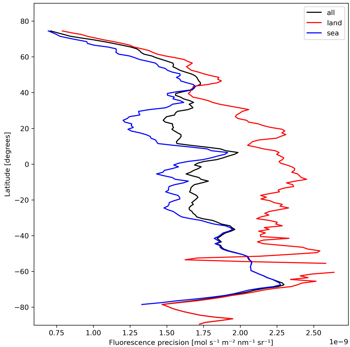
Figure 24: Zonal average of “Fluorescence precision” for 2023-10-29 to 2023-10-31.
