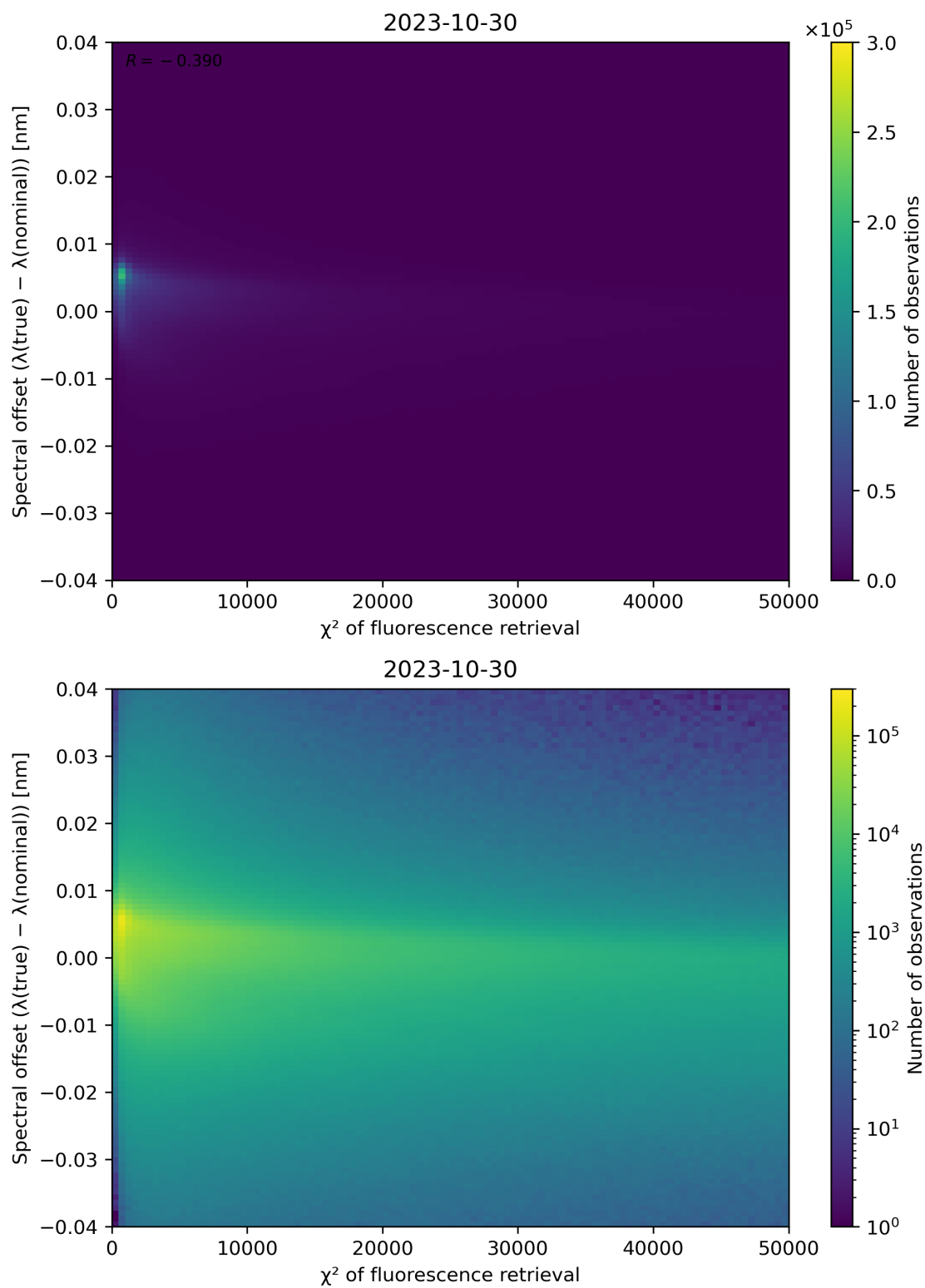
Figure 72: Scatter density plot of " \chi^2 of fluorescence retrieval" against "Spectral offset ( \lambda(\text{true}) - \lambda(\text{nominal}) )" for 2023-10-29 to 2023-10-31.
