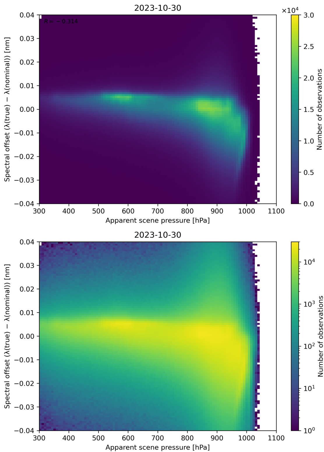
Figure 68: Scatter density plot of “Apparent scene pressure” against “Spectral offset ( \lambda(\text{true}) - \lambda(\text{nominal}) )” for 2023-10-29 to 2023-10-31.
