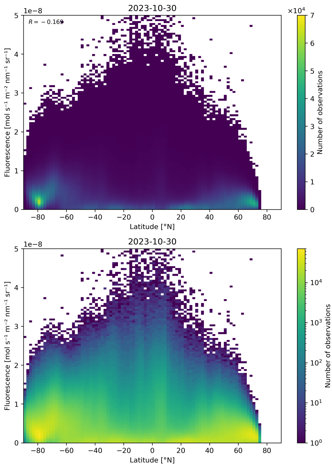
Figure 101: Scatter density plot of “Latitude” against “Fluorescence” for 2023-10-29 to 2023-10-31.
