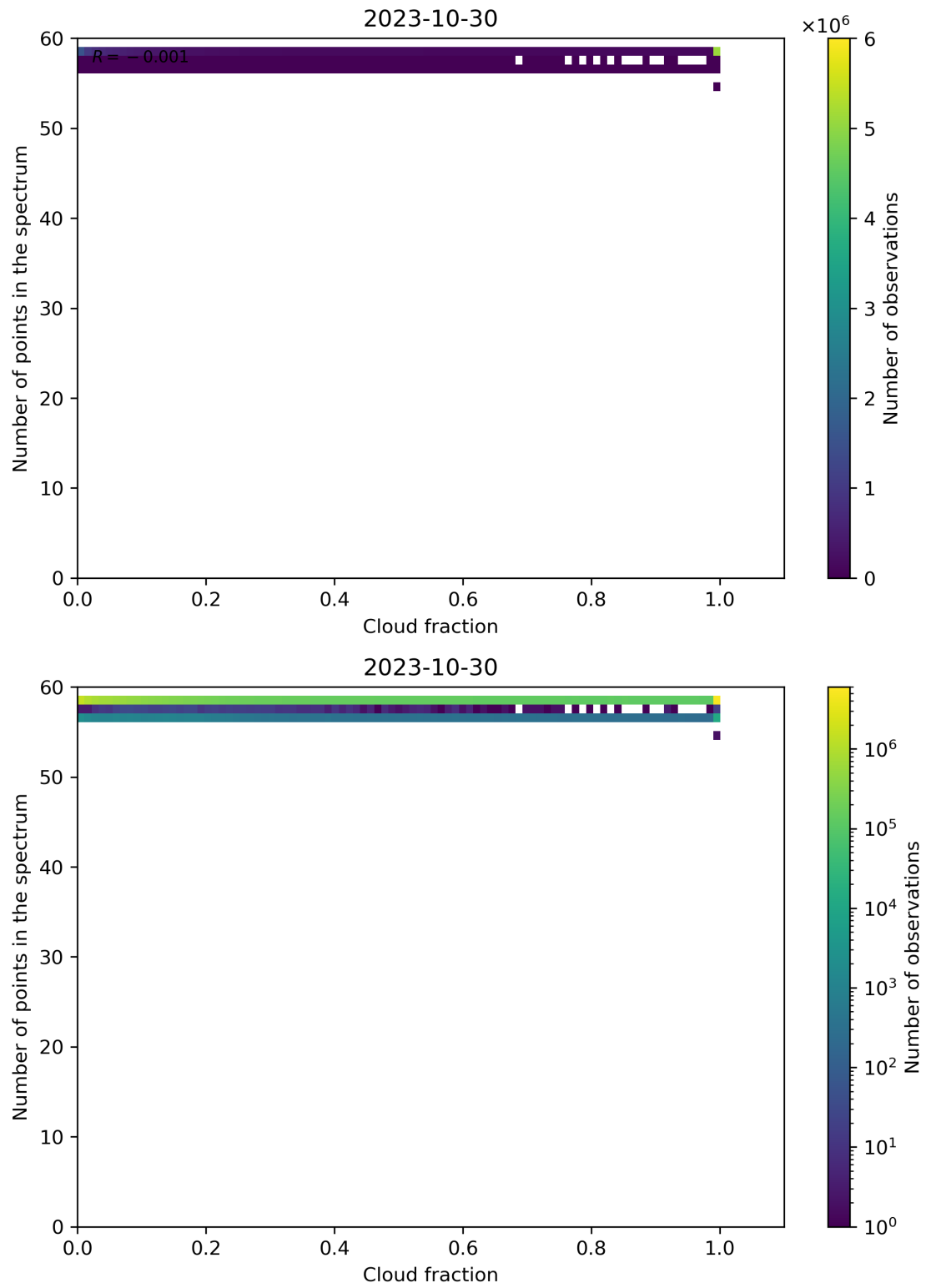
Figure 81: Scatter density plot of “Cloud fraction” against “Number of points in the spectrum” for 2023-10-29 to 2023-10-31.
