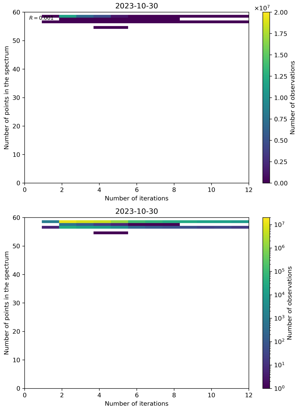
Figure 108: Scatter density plot of “Number of iterations” against “Number of points in the spectrum” for 2023-10-29 to 2023-10-31.
