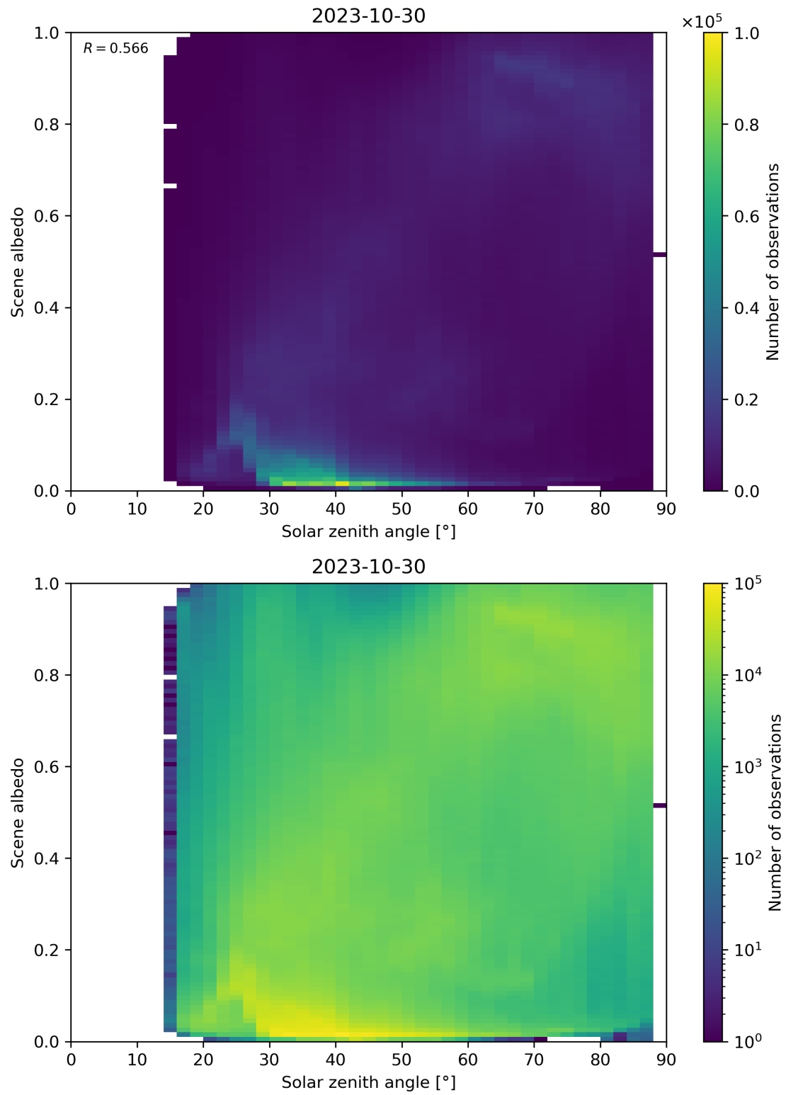
Figure 127: Scatter density plot of “Solar zenith angle” against “Scene albedo” for 2023-10-29 to 2023-10-31.
