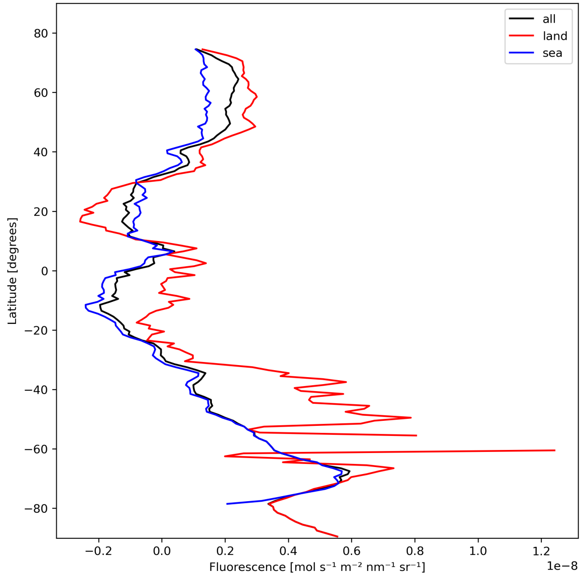
Figure 23: Zonal average of “Fluorescence” for 2023-10-29 to 2023-10-31.
