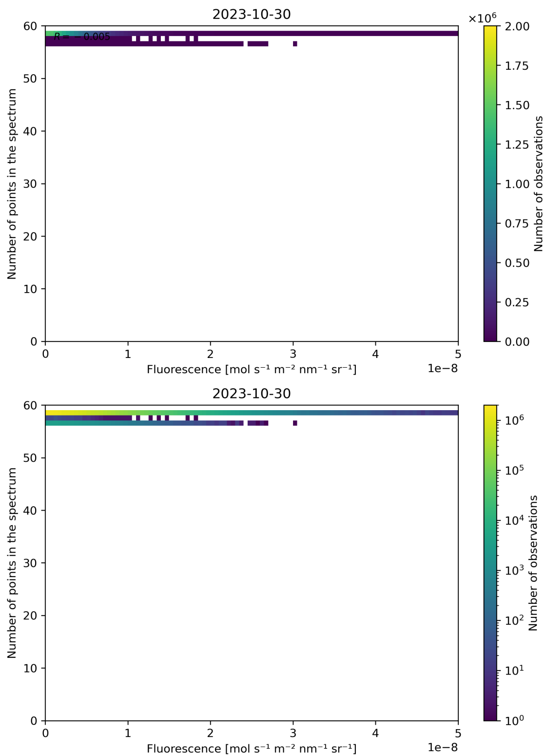
Figure 94: Scatter density plot of “Fluorescence” against “Number of points in the spectrum” for 2023-10-29 to 2023-10-31.
