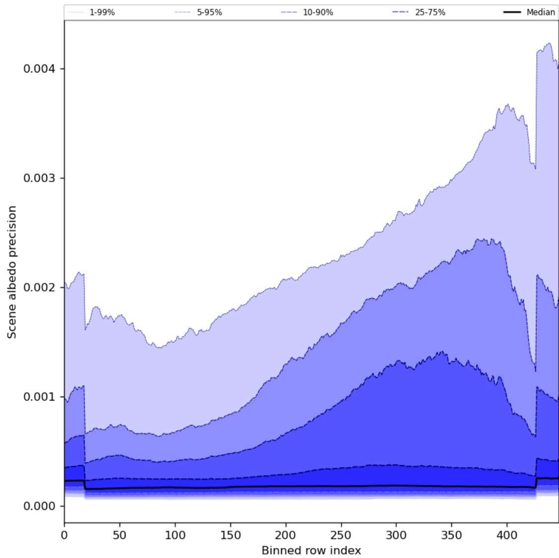
Figure 52: Along track statistics of “Scene albedo precision” for 2023-10-29 to 2023-10-31
