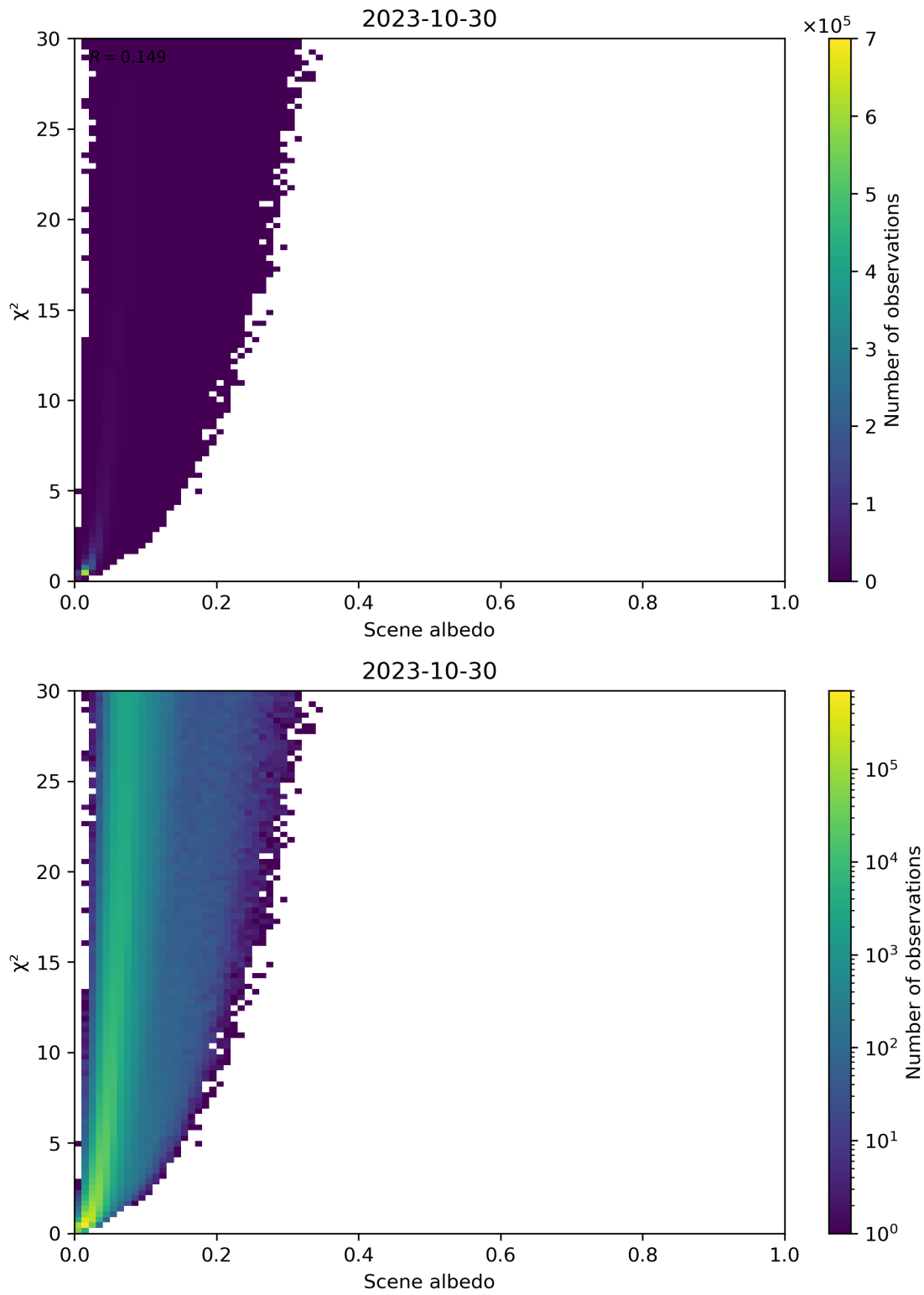
Figure 112: Scatter density plot of “Scene albedo” against “ \chi^2 ” for 2023-10-29 to 2023-10-31.
