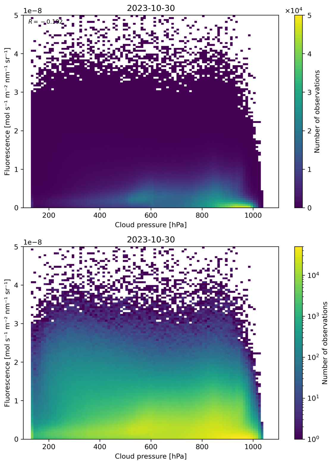
Figure 88: Scatter density plot of “Cloud pressure” against “Fluorescence” for 2023-10-29 to 2023-10-31.
