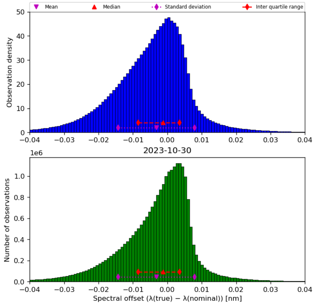
Figure 45: Histogram of “Spectral offset ( \lambda(\text{true}) - \lambda(\text{nominal}) )” for 2023-10-29 to 2023-10-31
