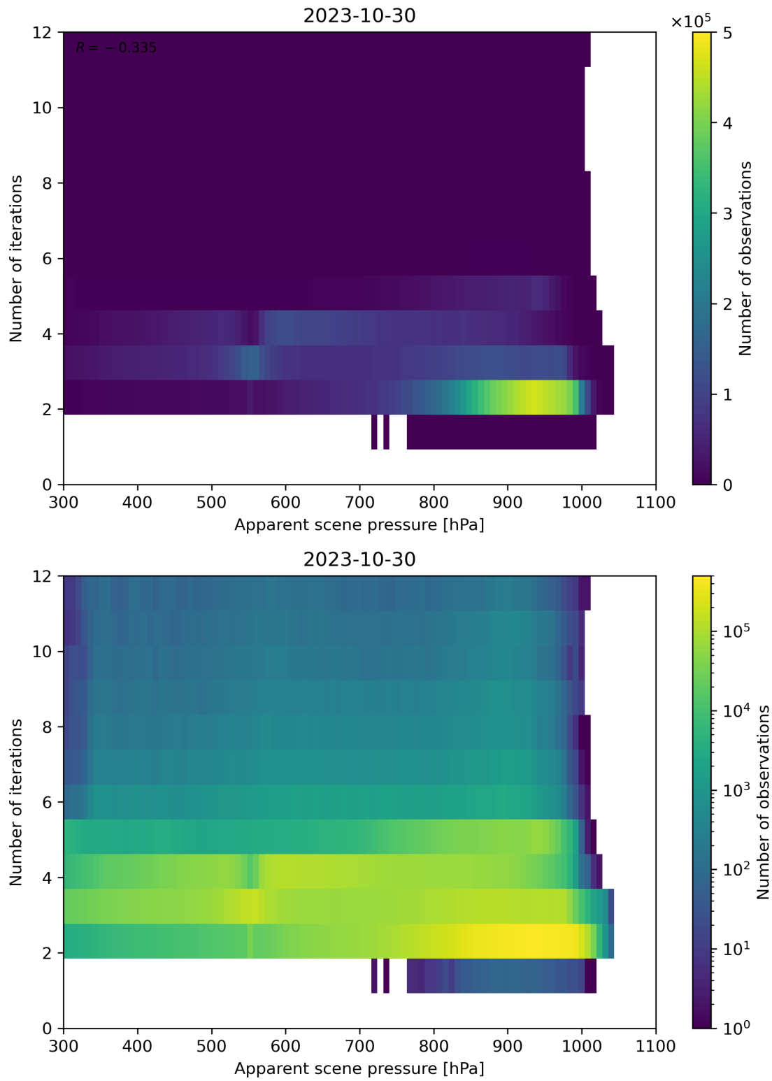
Figure 66: Scatter density plot of “Apparent scene pressure” against “Number of iterations” for 2023-10-29 to 2023-10-31.
