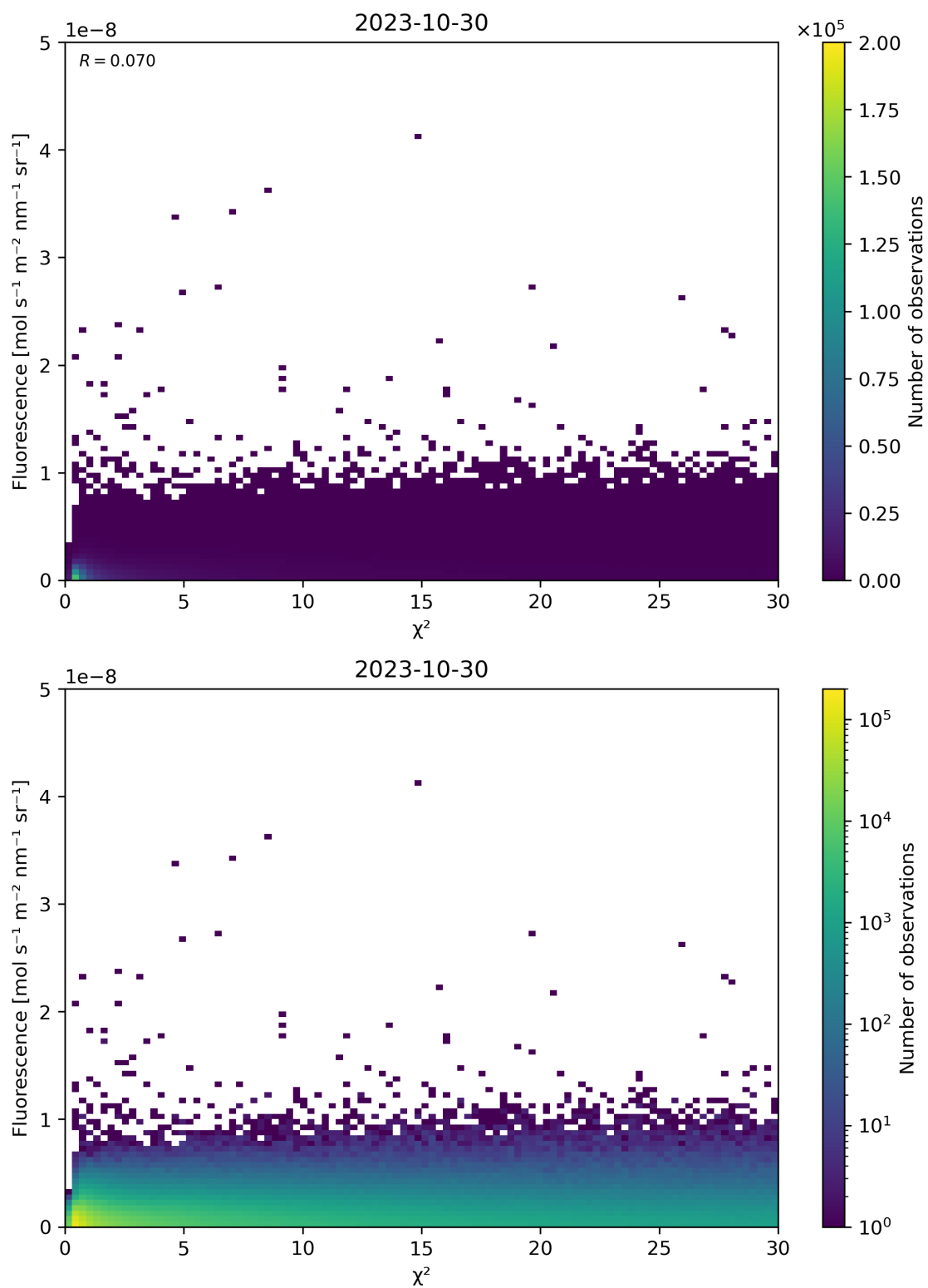
Figure 70: Scatter density plot of “ \chi^2 ” against “Fluorescence” for 2023-10-29 to 2023-10-31.
