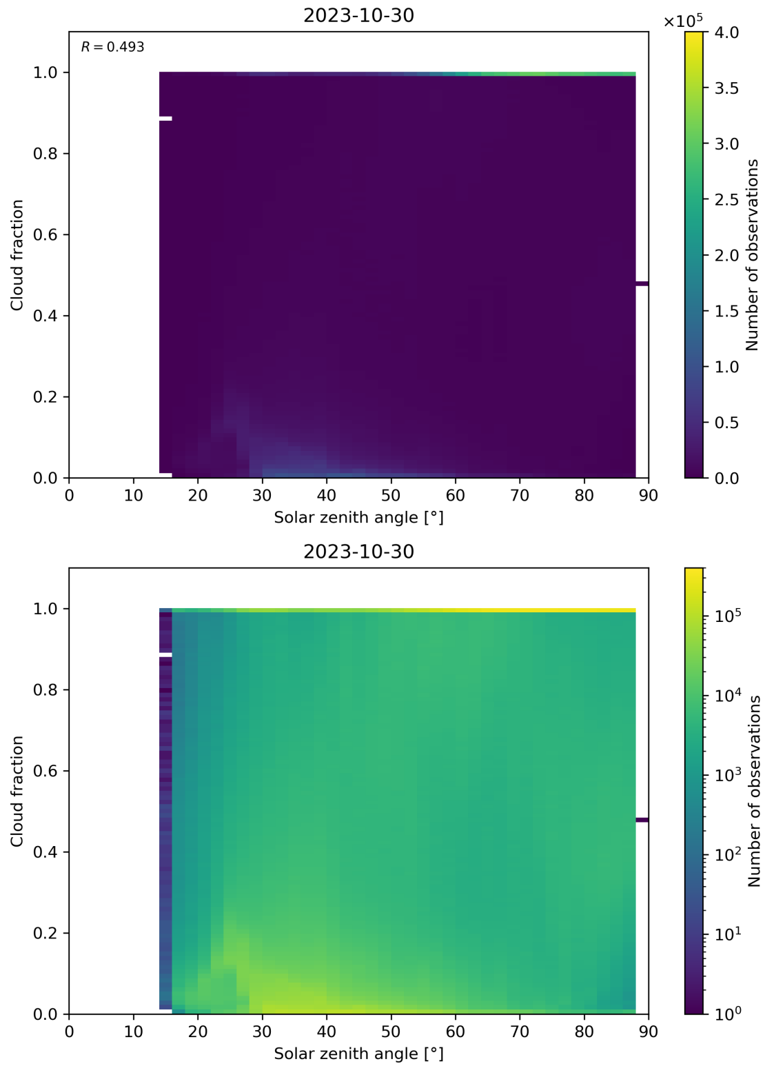
Figure 121: Scatter density plot of “Solar zenith angle” against “Cloud fraction” for 2023-10-29 to 2023-10-31.
