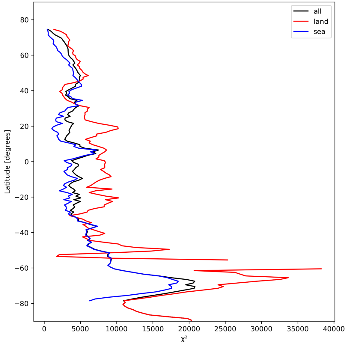
Figure 21: Zonal average of “ \chi^2 ” for 2023-10-29 to 2023-10-31.
