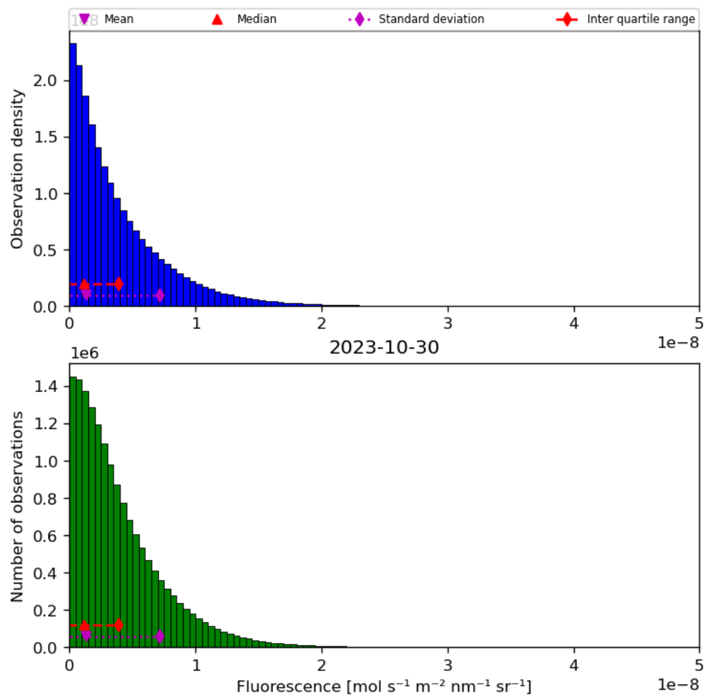
Figure 40: Histogram of “Fluorescence” for 2023-10-29 to 2023-10-31
