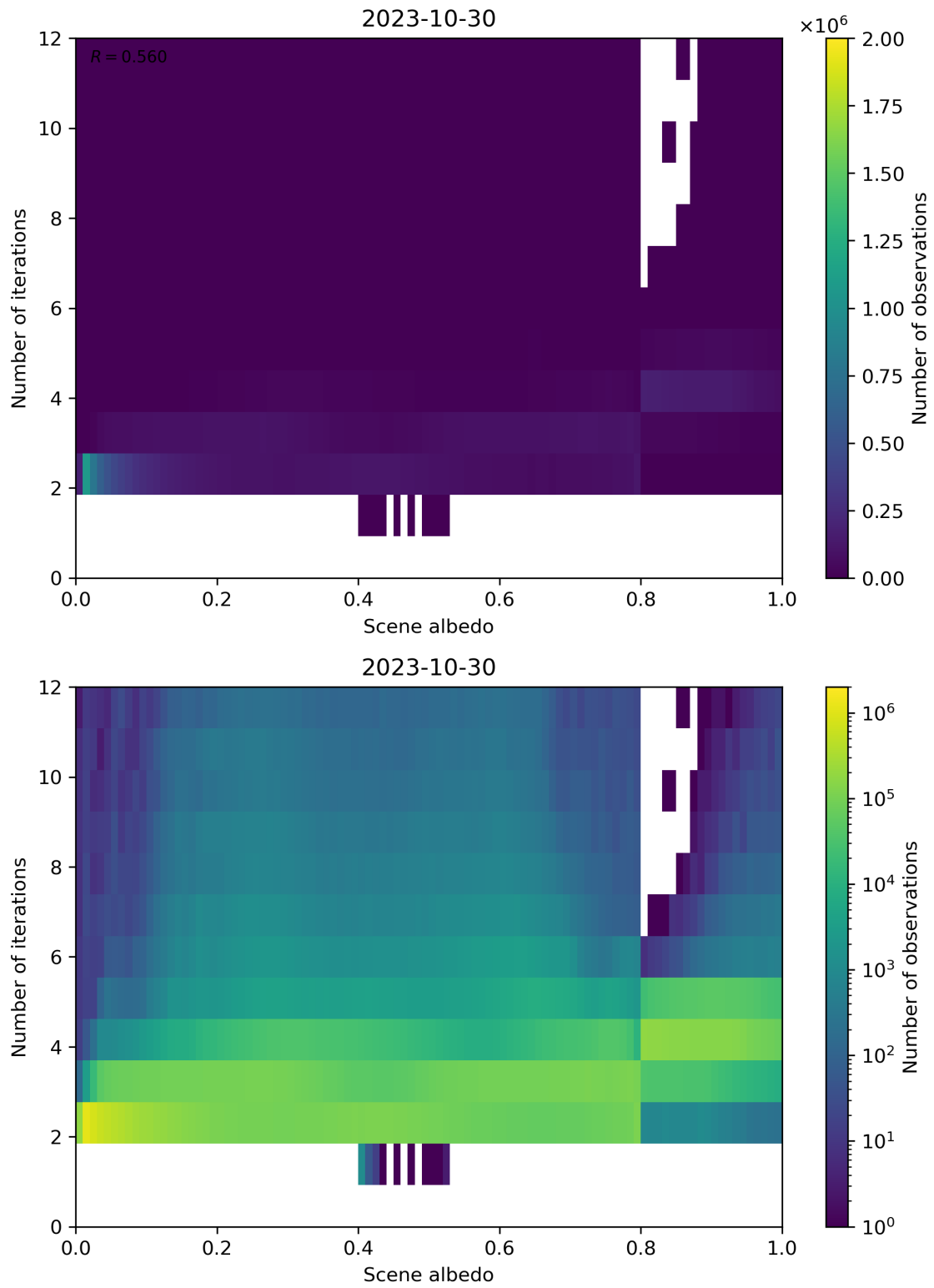
Figure 115: Scatter density plot of “Scene albedo” against “Number of iterations” for 2023-10-29 to 2023-10-31.
