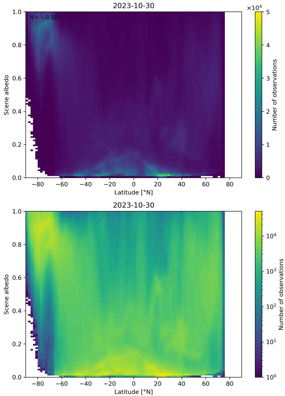
Figure 104: Scatter density plot of “Latitude” against “Scene albedo” for 2023-10-29 to 2023-10-31.
