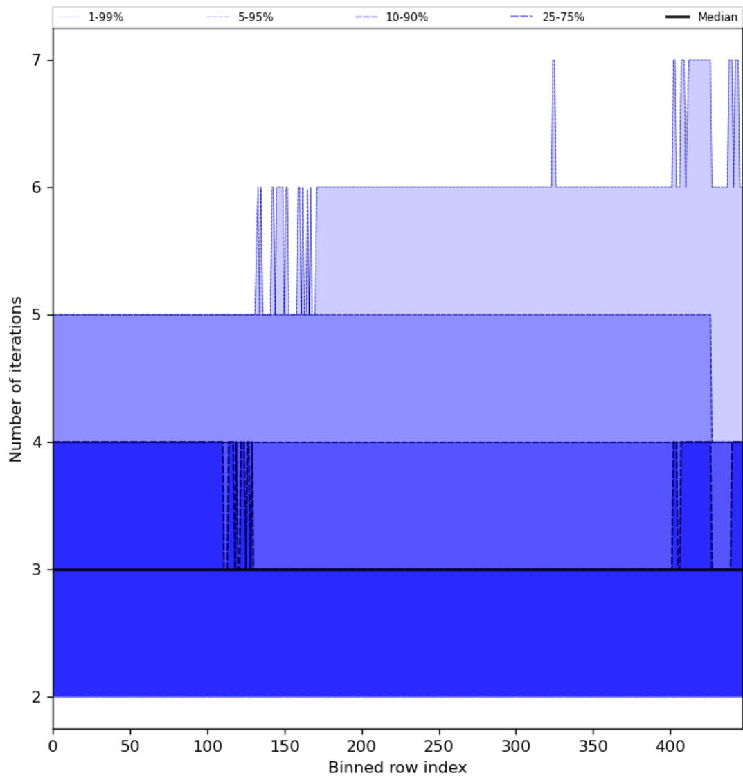
Figure 56: Along track statistics of “Number of iterations” for 2023-10-29 to 2023-10-31
