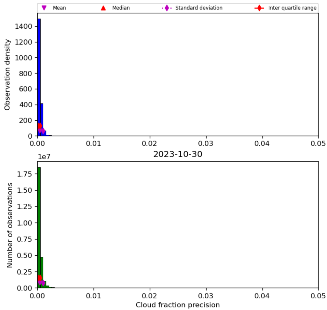
Figure 33: Histogram of “Cloud fraction precision” for 2023-10-29 to 2023-10-31
