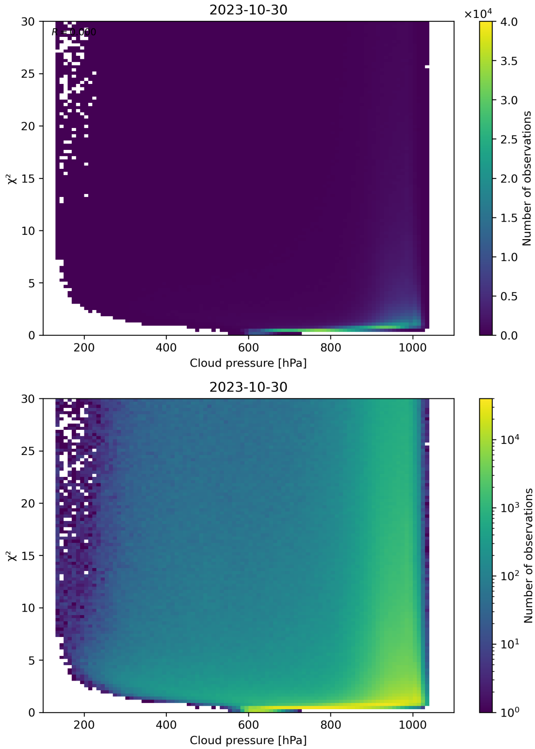
Figure 85: Scatter density plot of “Cloud pressure” against “ \chi^2 ” for 2023-10-29 to 2023-10-31.
