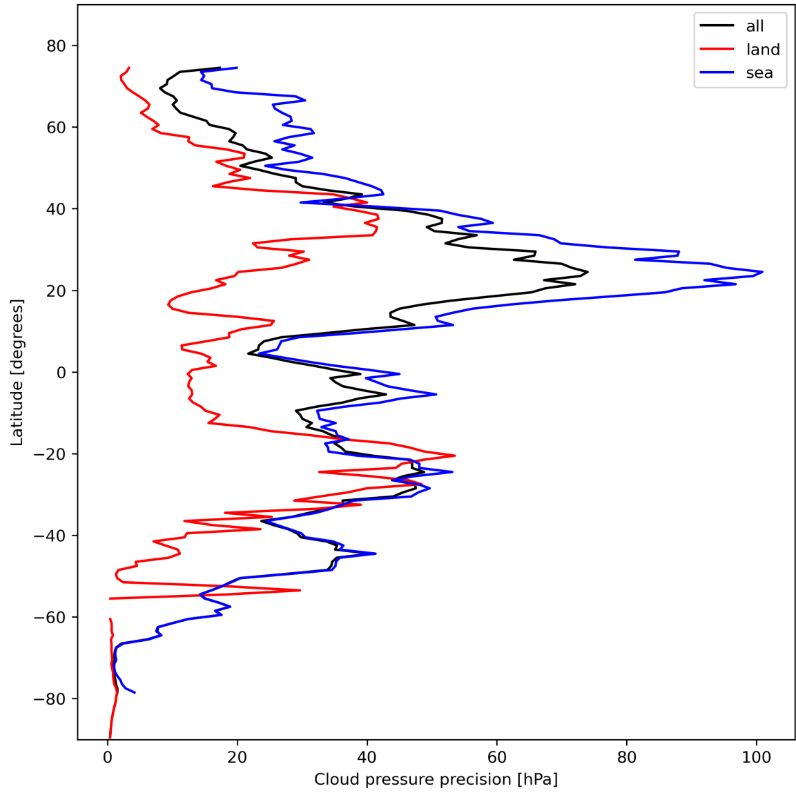
Figure 14: Zonal average of “Cloud pressure precision” for 2023-10-29 to 2023-10-31.
