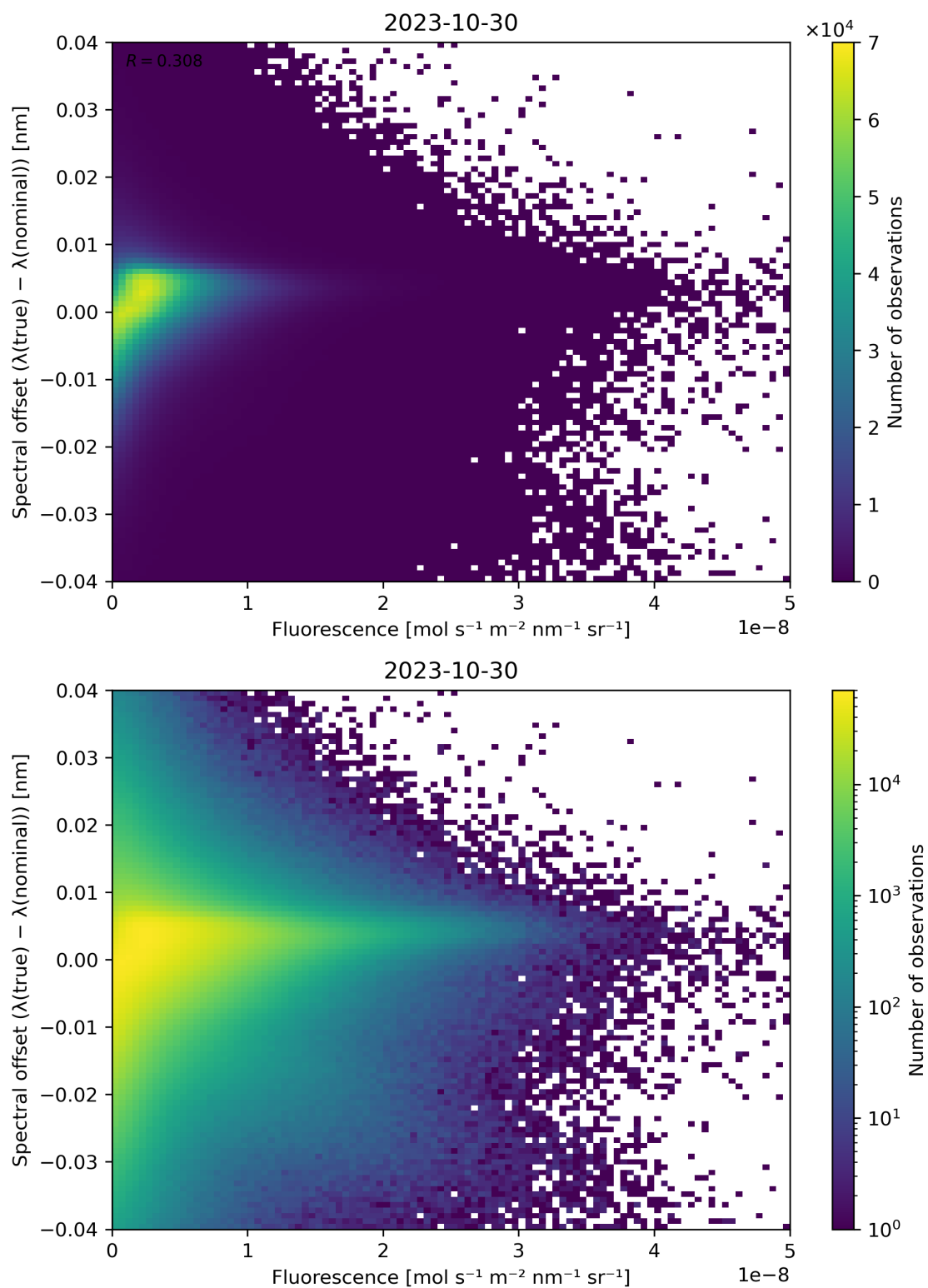
Figure 95: Scatter density plot of “Fluorescence” against “Spectral offset ( \lambda(\text{true}) - \lambda(\text{nominal}) )” for 2023-10-29 to 2023-10-31.
