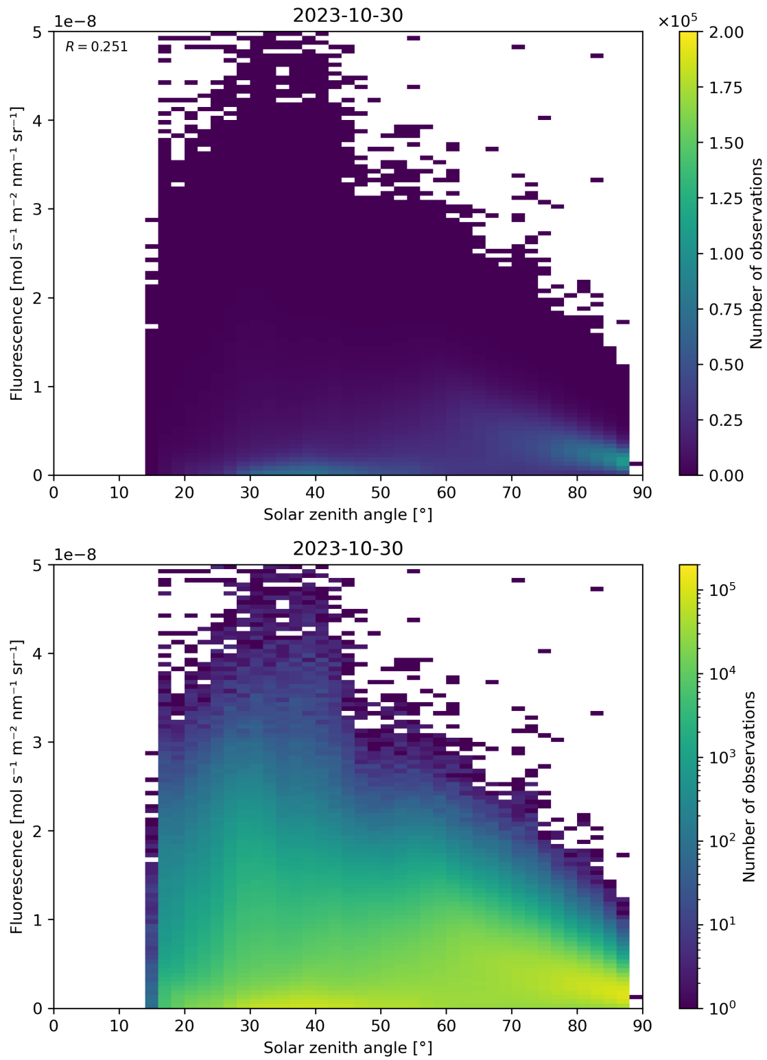
Figure 123: Scatter density plot of “Solar zenith angle” against “Fluorescence” for 2023-10-29 to 2023-10-31.
