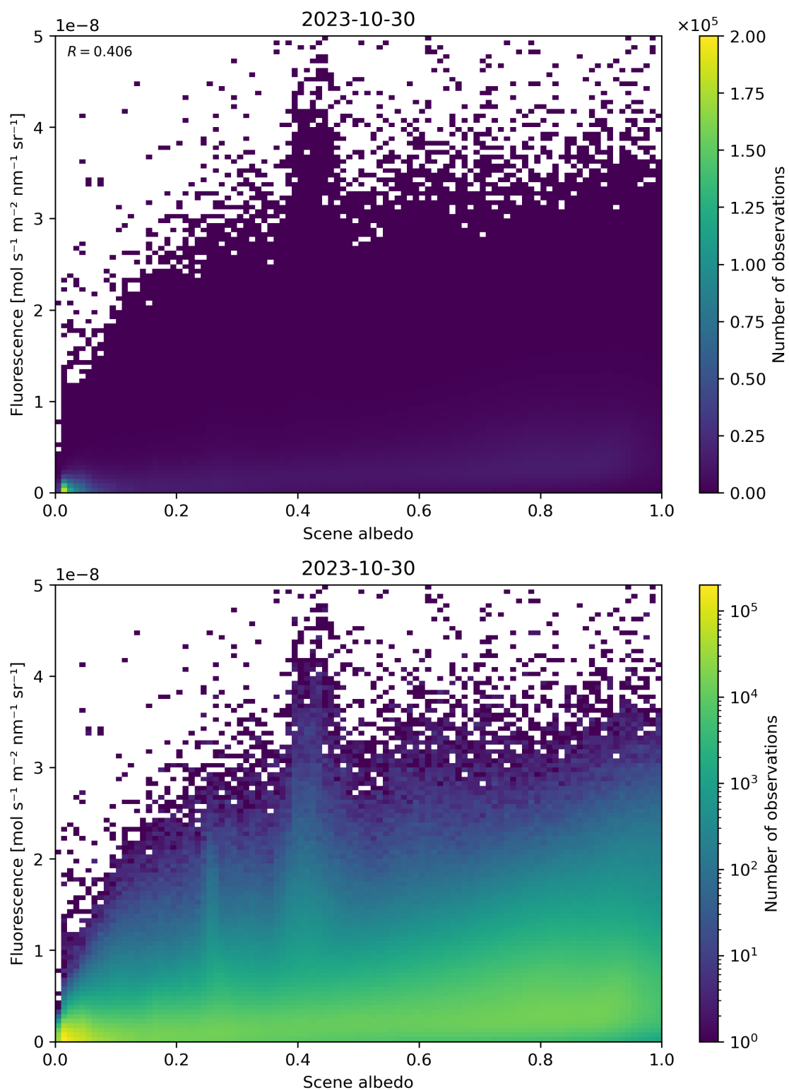
Figure 114: Scatter density plot of “Scene albedo” against “Fluorescence” for 2023-10-29 to 2023-10-31.
