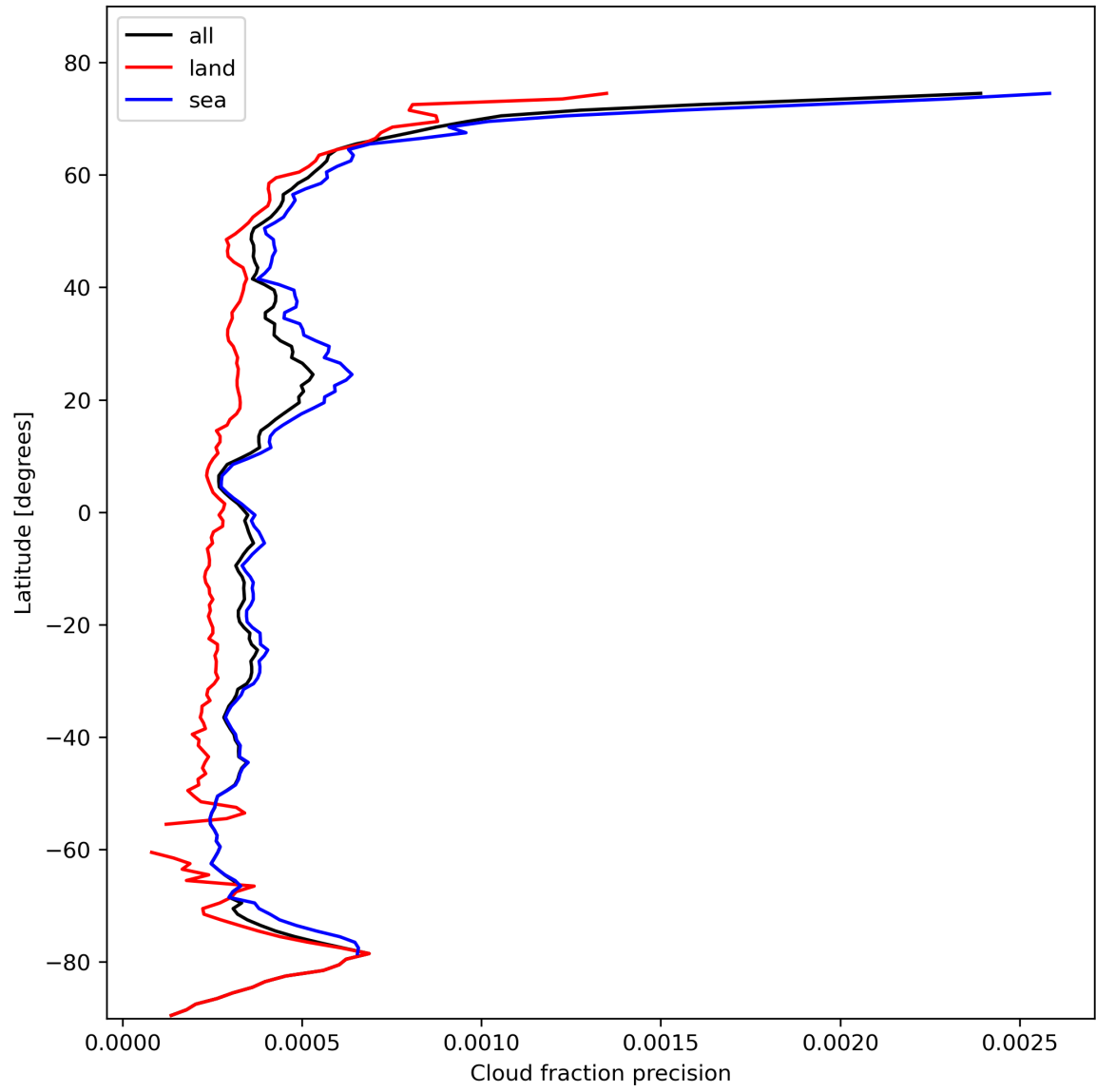
Figure 16: Zonal average of “Cloud fraction precision” for 2023-10-29 to 2023-10-31.
