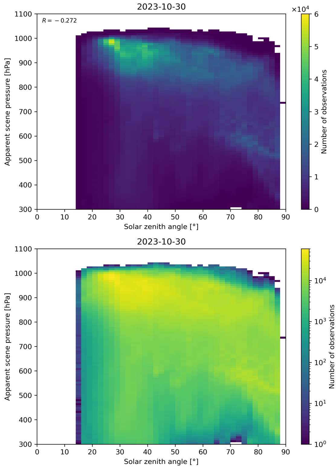
Figure 118: Scatter density plot of “Solar zenith angle” against “Apparent scene pressure” for 2023-10-29 to 2023-10-31.
