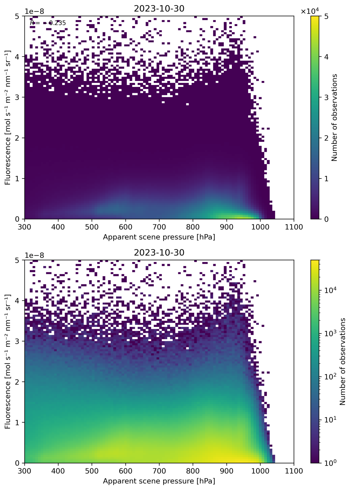
Figure 65: Scatter density plot of “Apparent scene pressure” against “Fluorescence” for 2023-10-29 to 2023-10-31.
