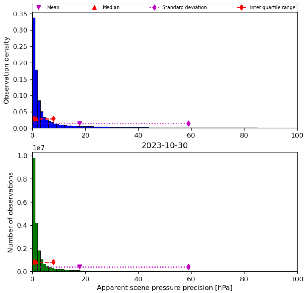
Figure 37: Histogram of “Apparent scene pressure precision” for 2023-10-29 to 2023-10-31
