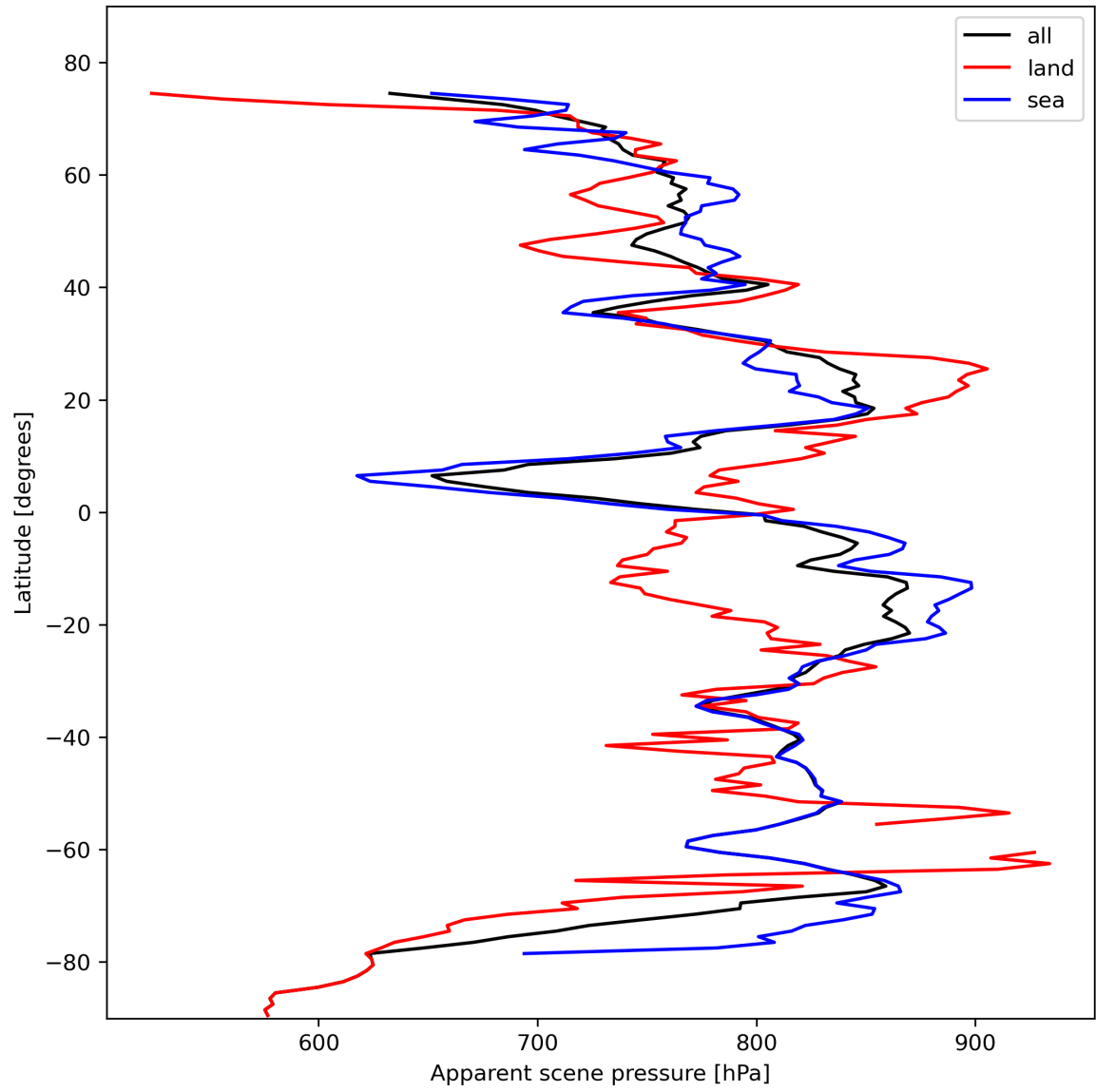
Figure 19: Zonal average of “Apparent scene pressure” for 2023-10-29 to 2023-10-31.
