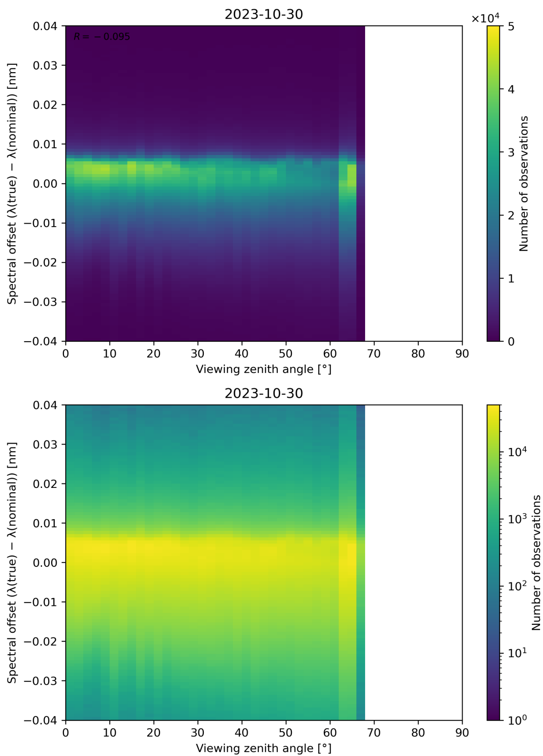
Figure 140: Scatter density plot of “Viewing zenith angle” against “Spectral offset ( \lambda(\text{true}) - \lambda(\text{nominal}) )” for 2023-10-29 to 2023-10-31.
