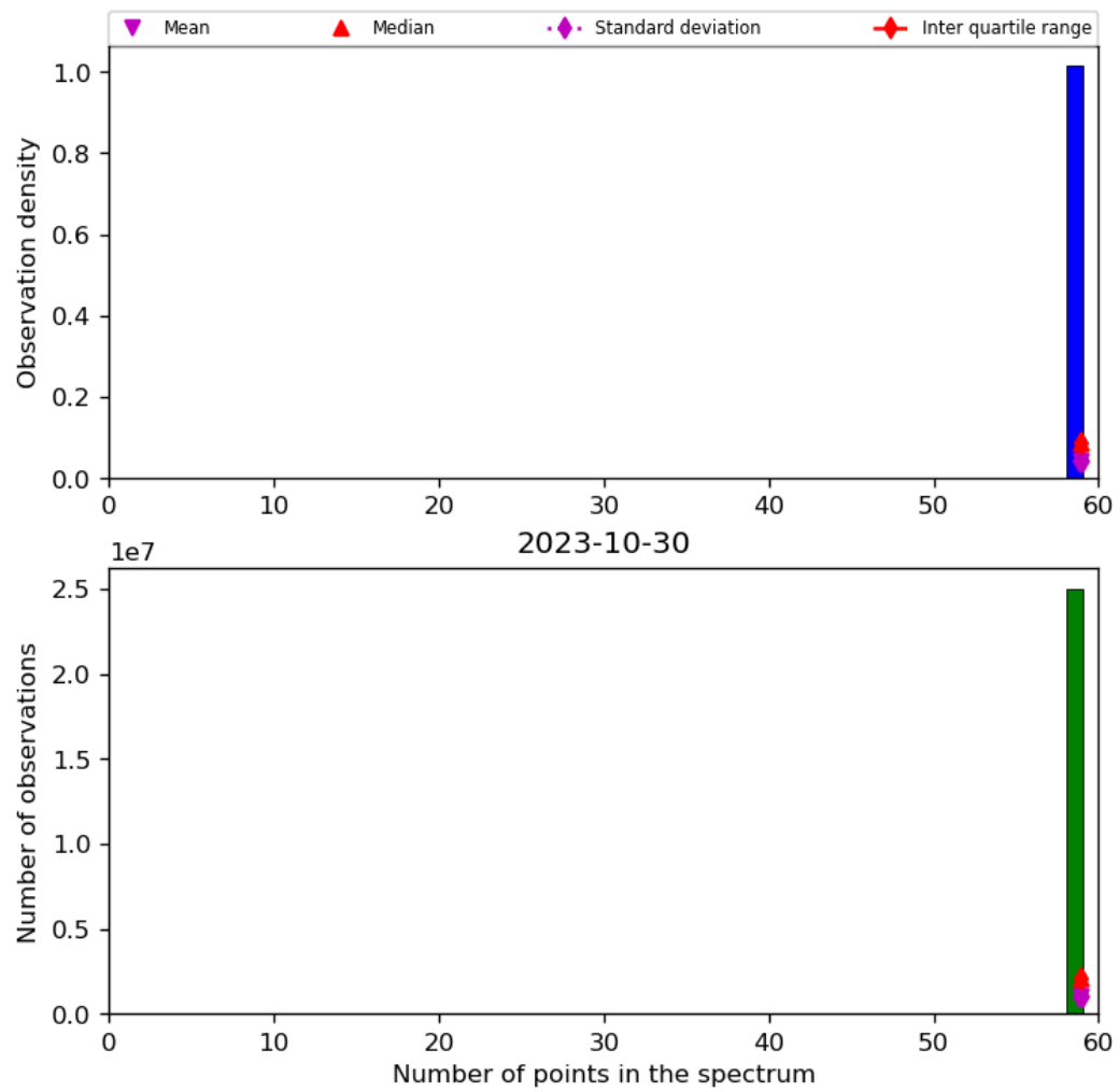
Figure 44: Histogram of “Number of points in the spectrum” for 2023-10-29 to 2023-10-31
