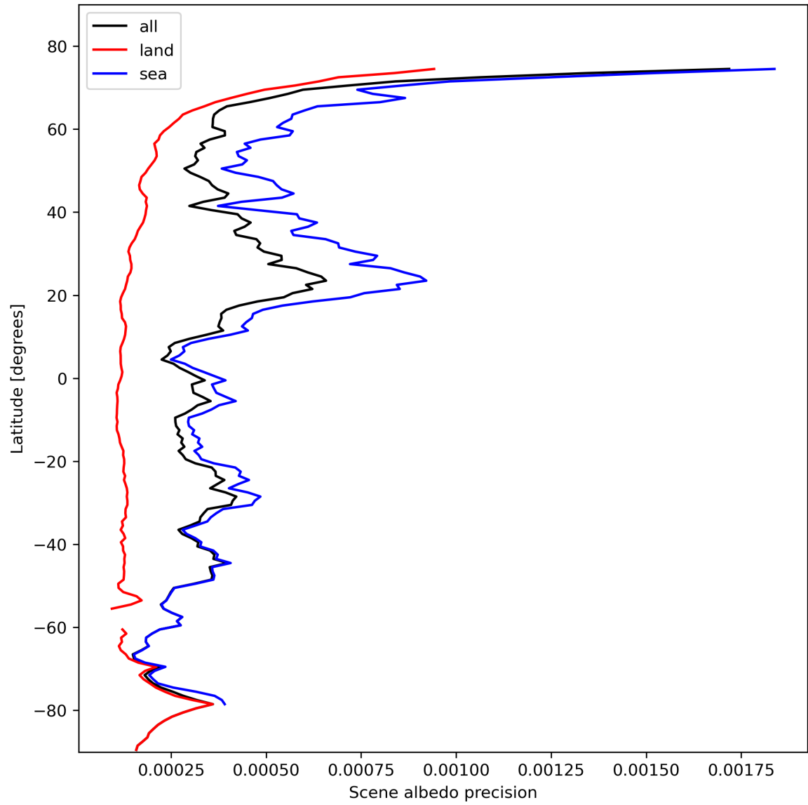
Figure 18: Zonal average of “Scene albedo precision” for 2023-10-29 to 2023-10-31.
