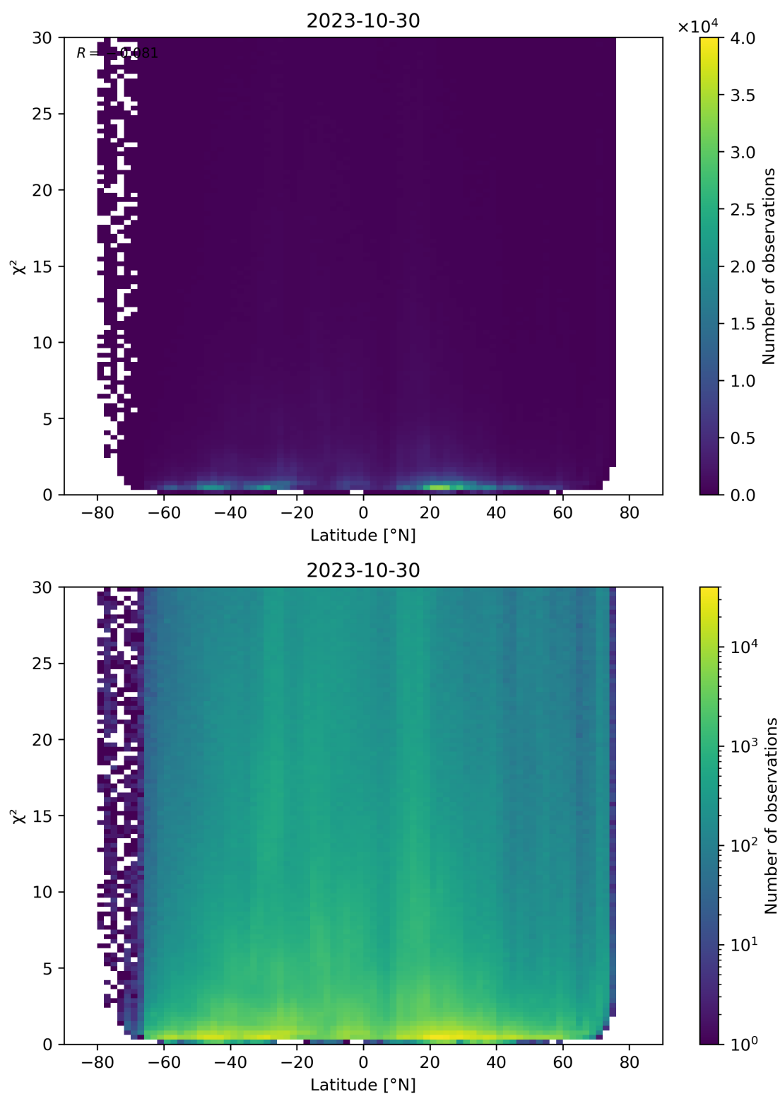
Figure 97: Scatter density plot of “Latitude” against “ \chi^2 ” for 2023-10-29 to 2023-10-31.
