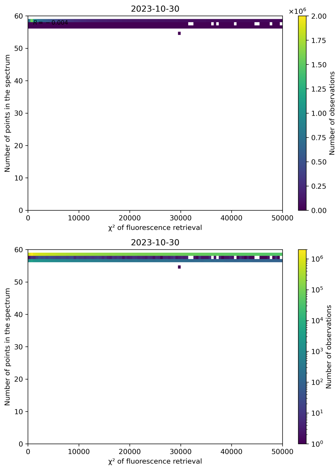
Figure 71: Scatter density plot of " \chi^2 of fluorescence retrieval" against "Number of points in the spectrum" for 2023-10-29 to 2023-10-31.
