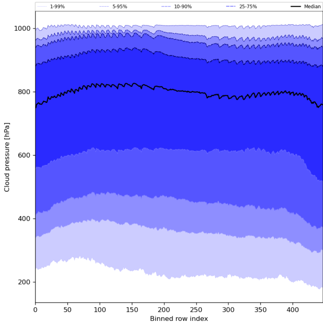
Figure 47: Along track statistics of “Cloud pressure” for 2023-10-29 to 2023-10-31
