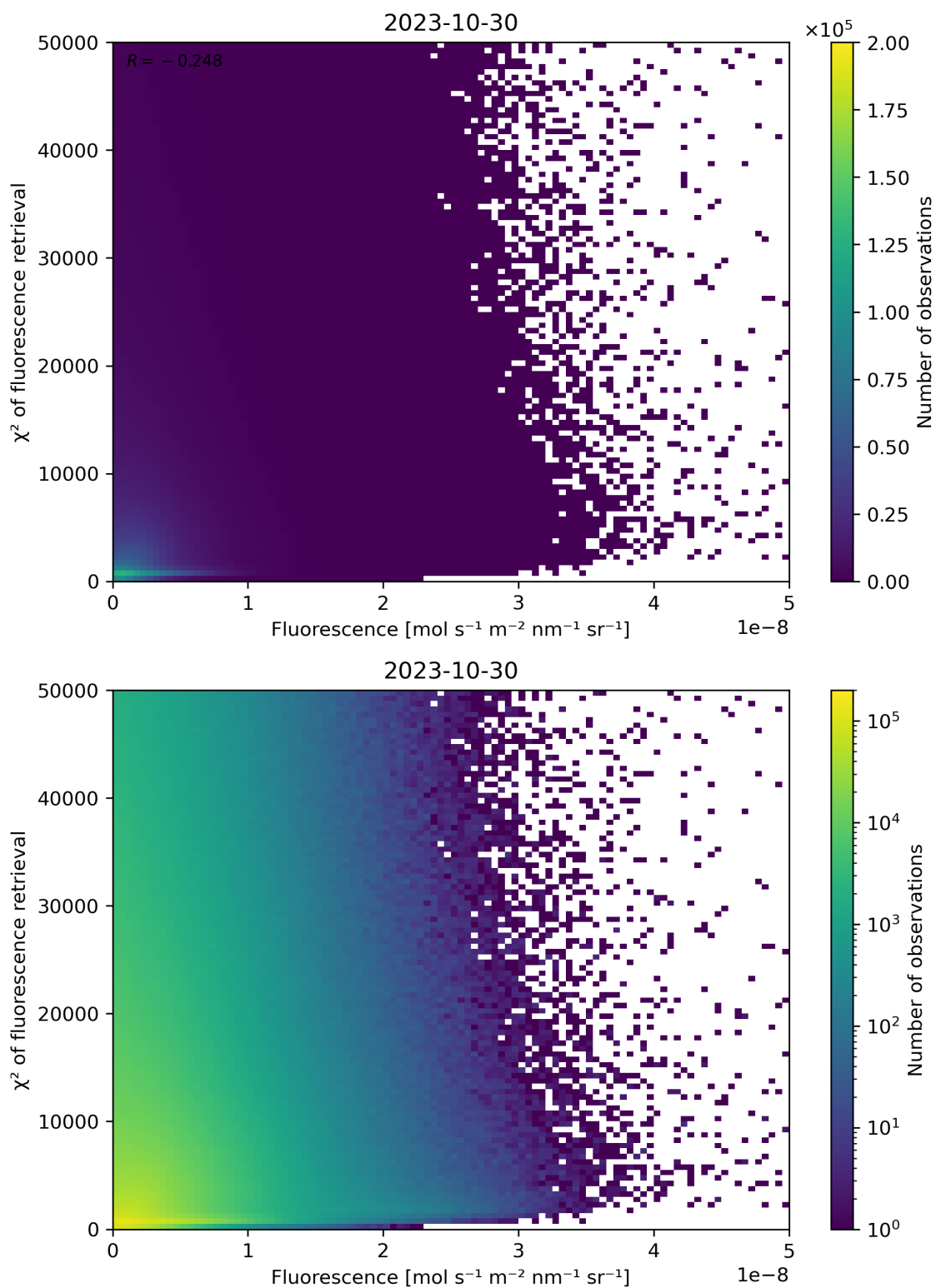
Figure 93: Scatter density plot of “Fluorescence” against “ \chi^2 of fluorescence retrieval” for 2023-10-29 to 2023-10-31.
