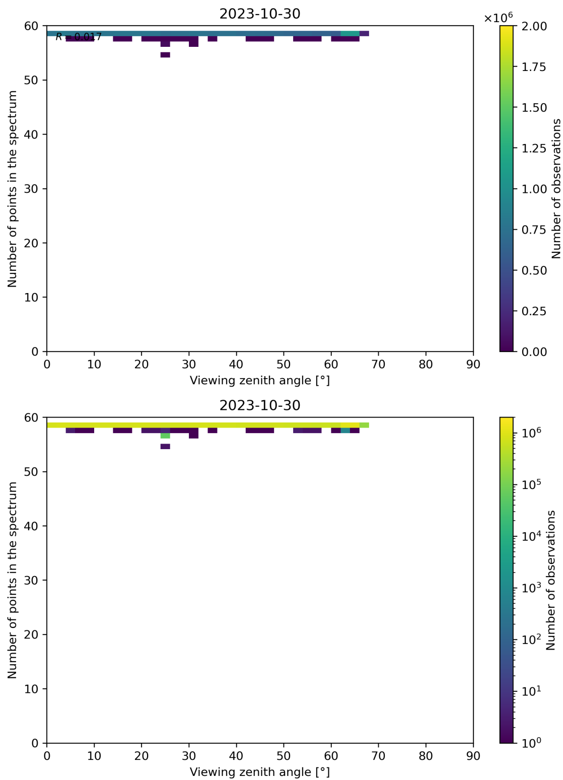
Figure 137: Scatter density plot of “Viewing zenith angle” against “Number of points in the spectrum” for 2023-10-29 to 2023-10-31.
