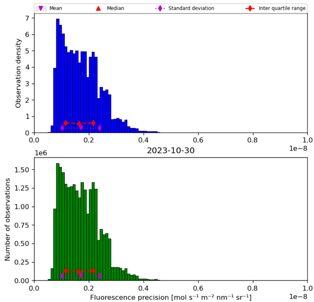
Figure 41: Histogram of “Fluorescence precision” for 2023-10-29 to 2023-10-31
