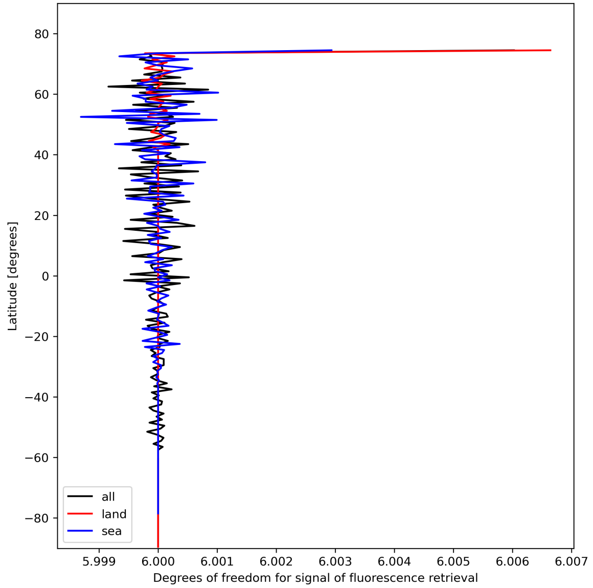
Figure 26: Zonal average of “Degrees of freedom for signal of fluorescence retrieval” for 2023-10-29 to 2023-10-31.
