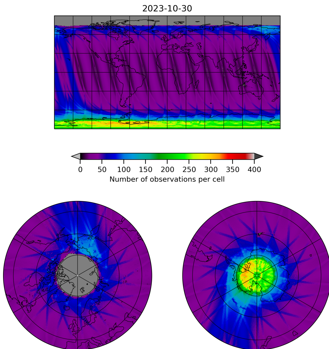
Figure 11: Map of the number of observations for 2023-10-29 to 2023-10-31
