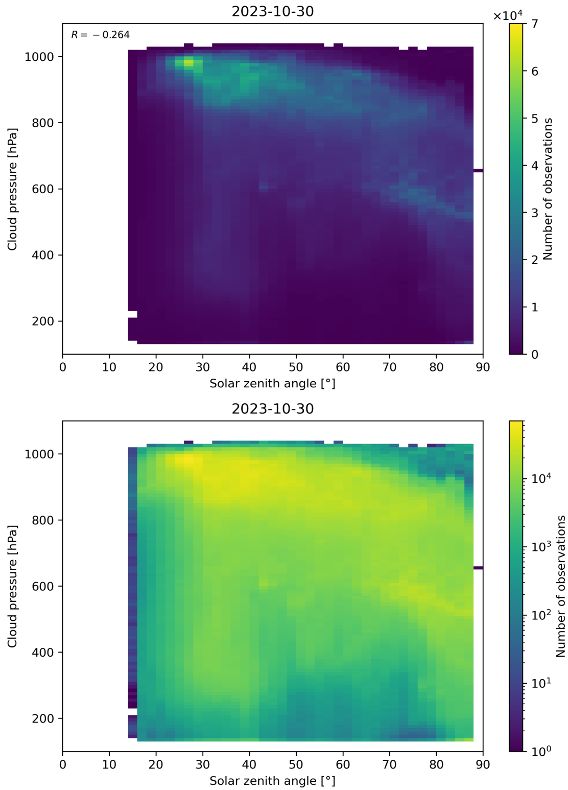
Figure 122: Scatter density plot of “Solar zenith angle” against “Cloud pressure” for 2023-10-29 to 2023-10-31.
