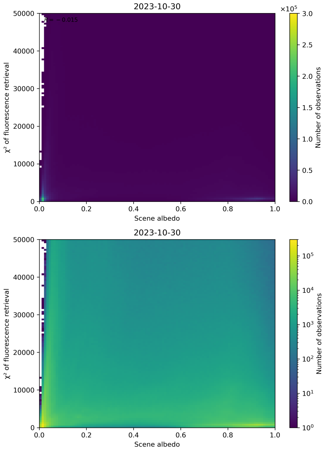
Figure 113: Scatter density plot of “Scene albedo” against “ \chi^2 of fluorescence retrieval” for 2023-10-29 to 2023-10-31.
