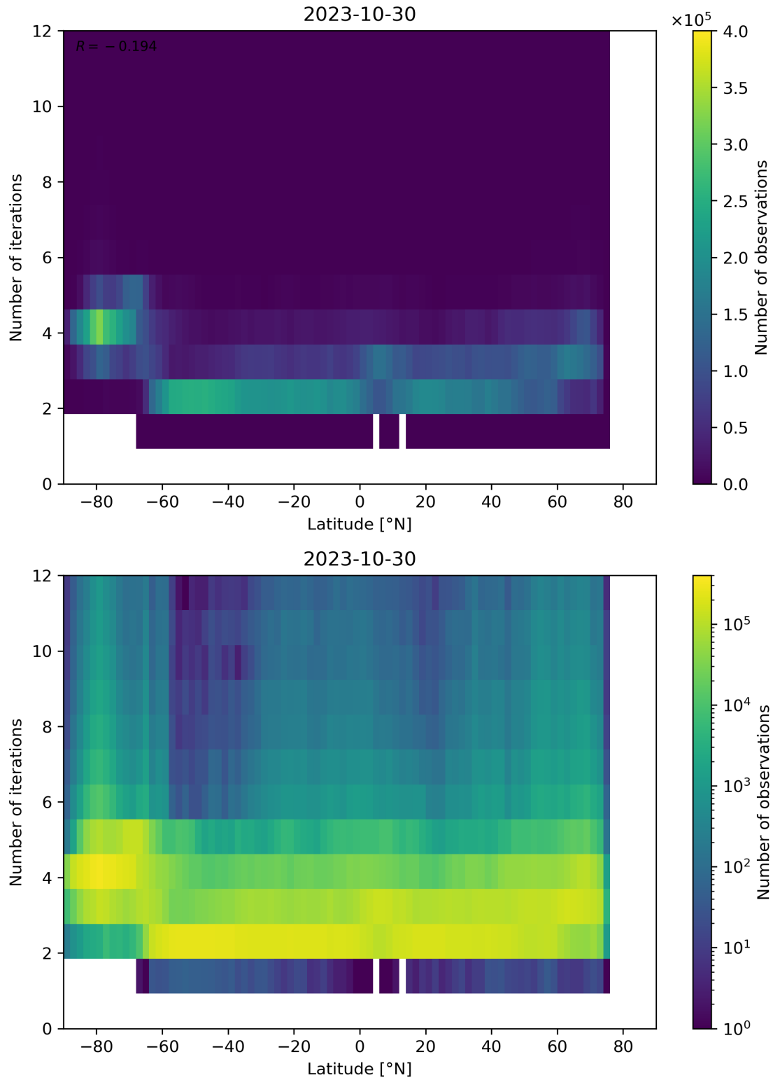
Figure 102: Scatter density plot of “Latitude” against “Number of iterations” for 2023-10-29 to 2023-10-31.
