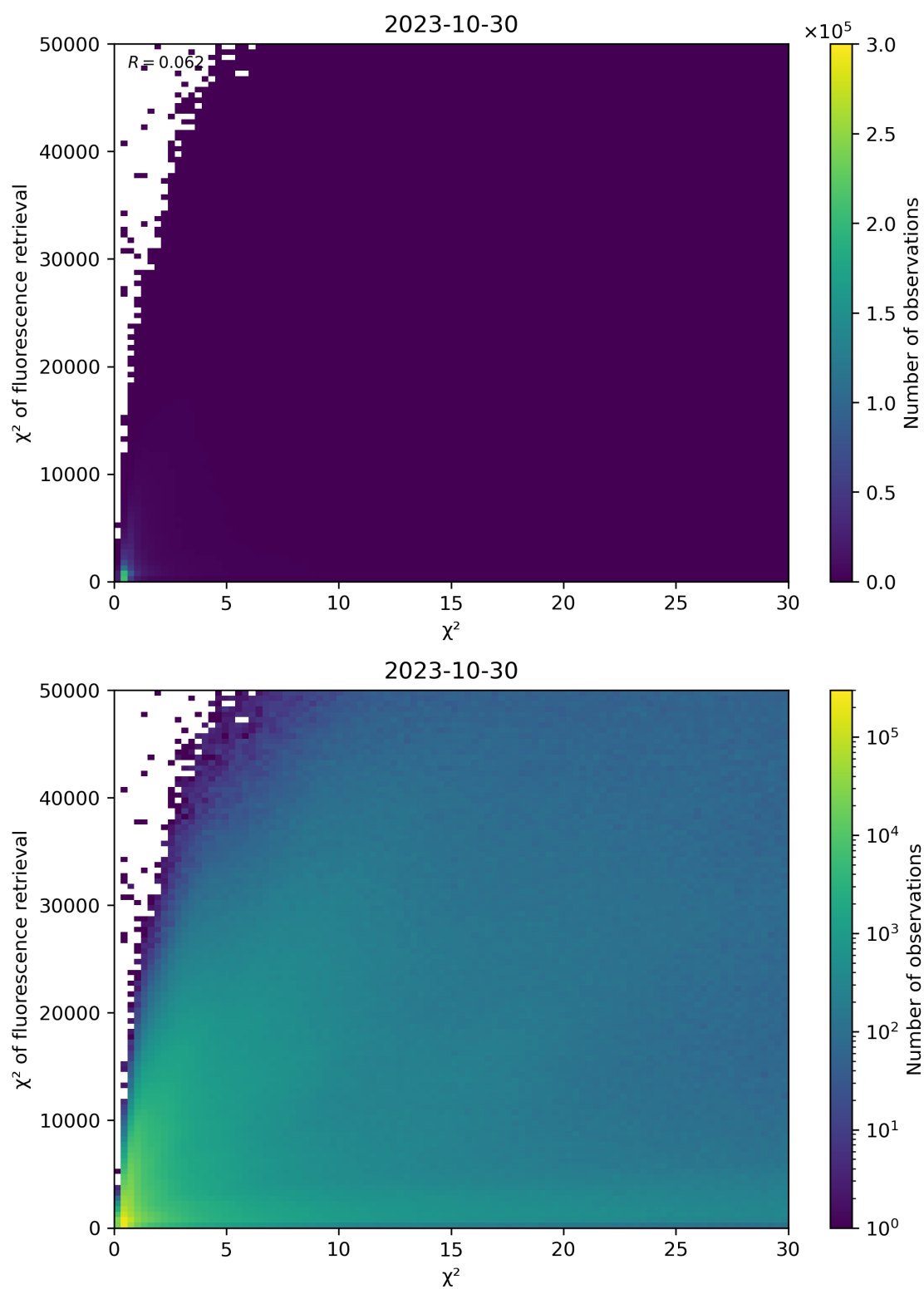
Figure 69: Scatter density plot of “ \chi^2 ” against “ \chi^2 of fluorescence retrieval” for 2023-10-29 to 2023-10-31.
