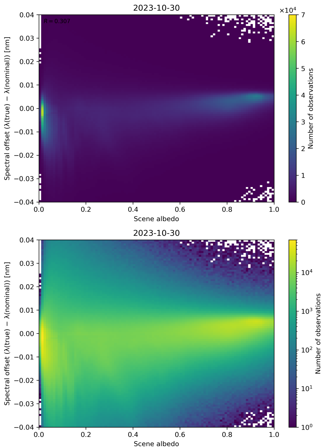
Figure 117: Scatter density plot of “Scene albedo” against “Spectral offset ( \lambda(\text{true}) - \lambda(\text{nominal}) )” for 2023-10-29 to 2023-10-31.
