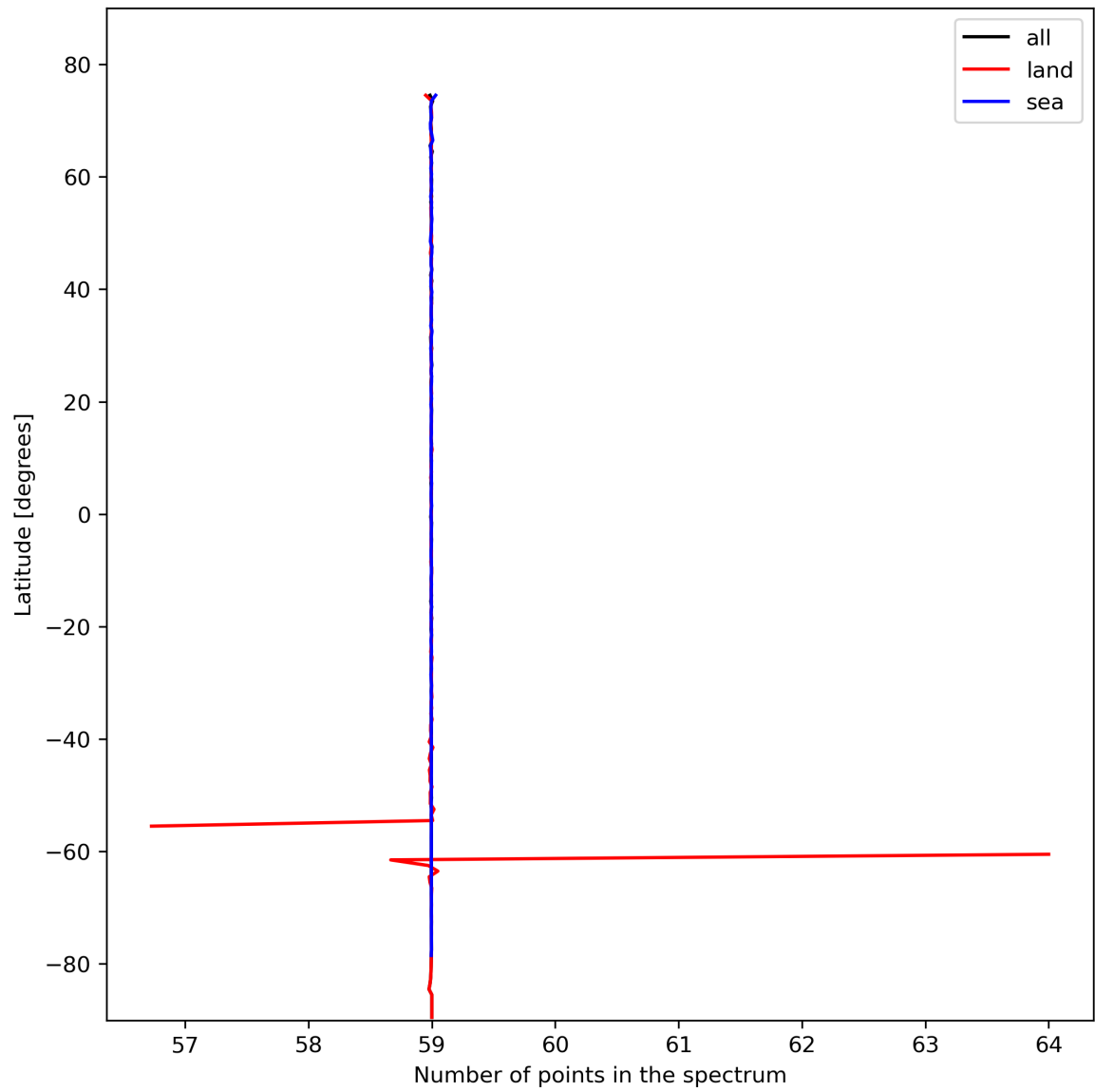
Figure 27: Zonal average of “Number of points in the spectrum” for 2023-10-29 to 2023-10-31.
