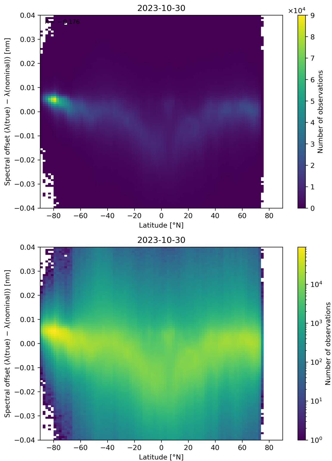
Figure 105: Scatter density plot of “Latitude” against “Spectral offset ( \lambda(\text{true}) - \lambda(\text{nominal}) )” for 2023-10-29 to 2023-10-31.
