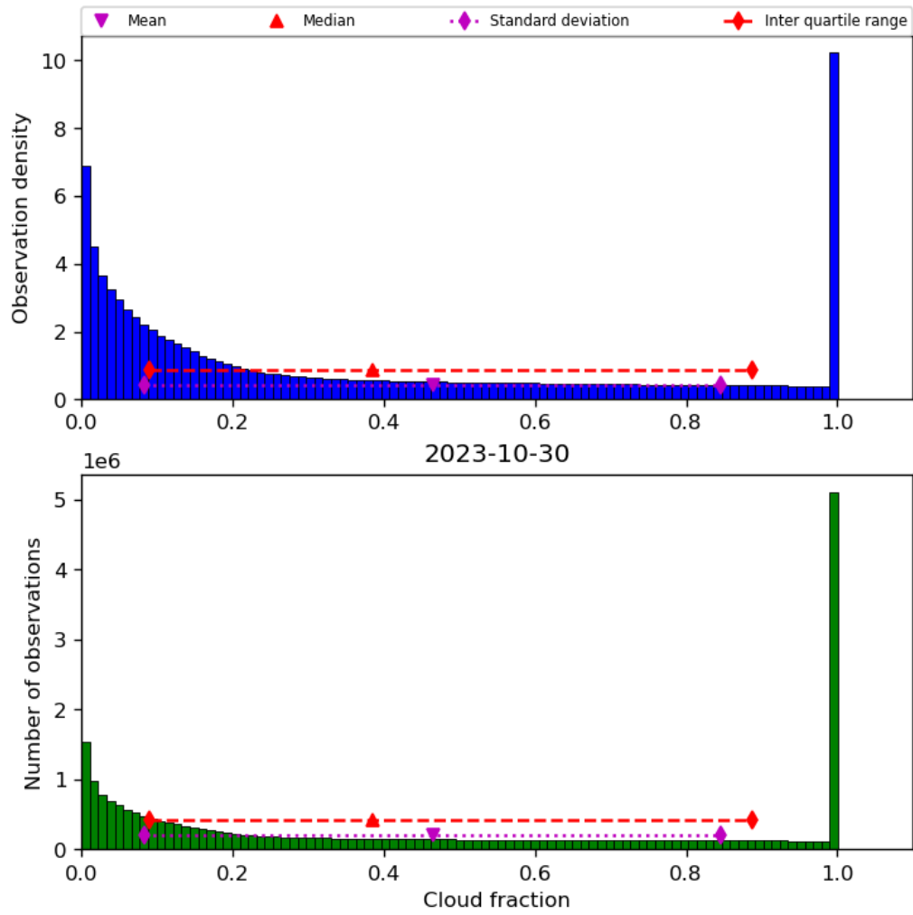
Figure 32: Histogram of “Cloud fraction” for 2023-10-29 to 2023-10-31
