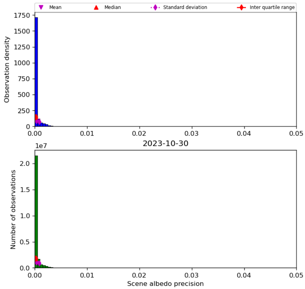
Figure 35: Histogram of “Scene albedo precision” for 2023-10-29 to 2023-10-31
