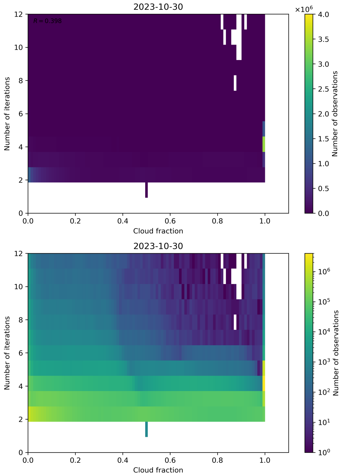
Figure 80: Scatter density plot of “Cloud fraction” against “Number of iterations” for 2023-10-29 to 2023-10-31.
