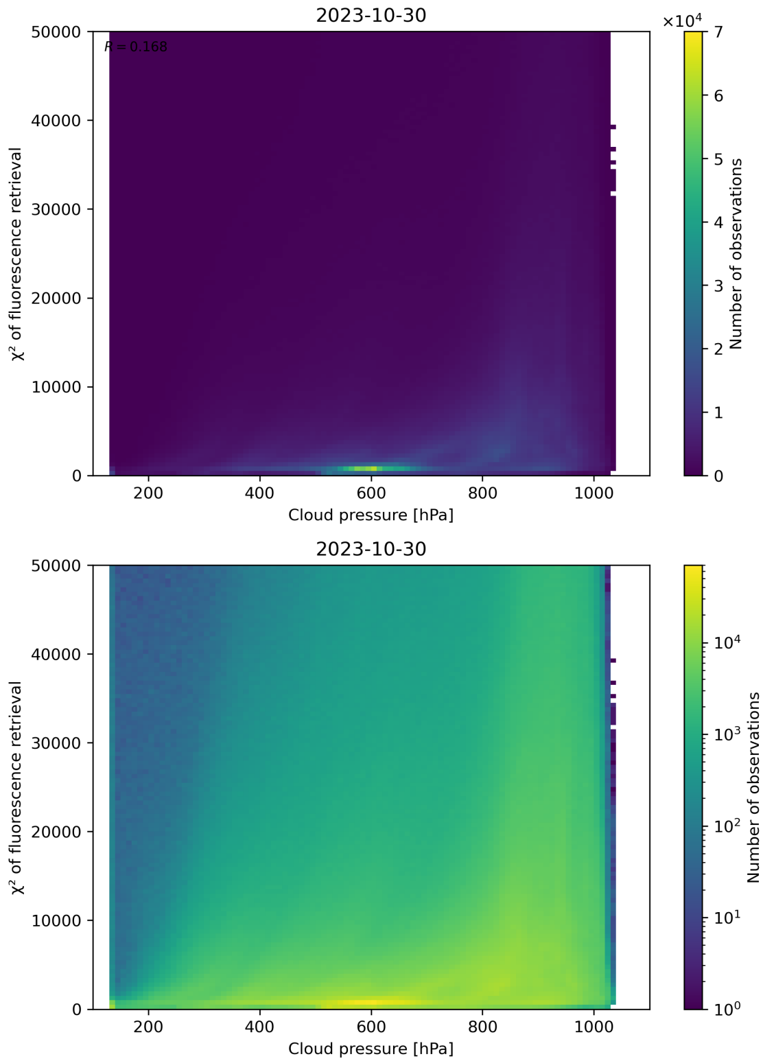
Figure 86: Scatter density plot of “Cloud pressure” against “ \chi^2 of fluorescence retrieval” for 2023-10-29 to 2023-10-31.
