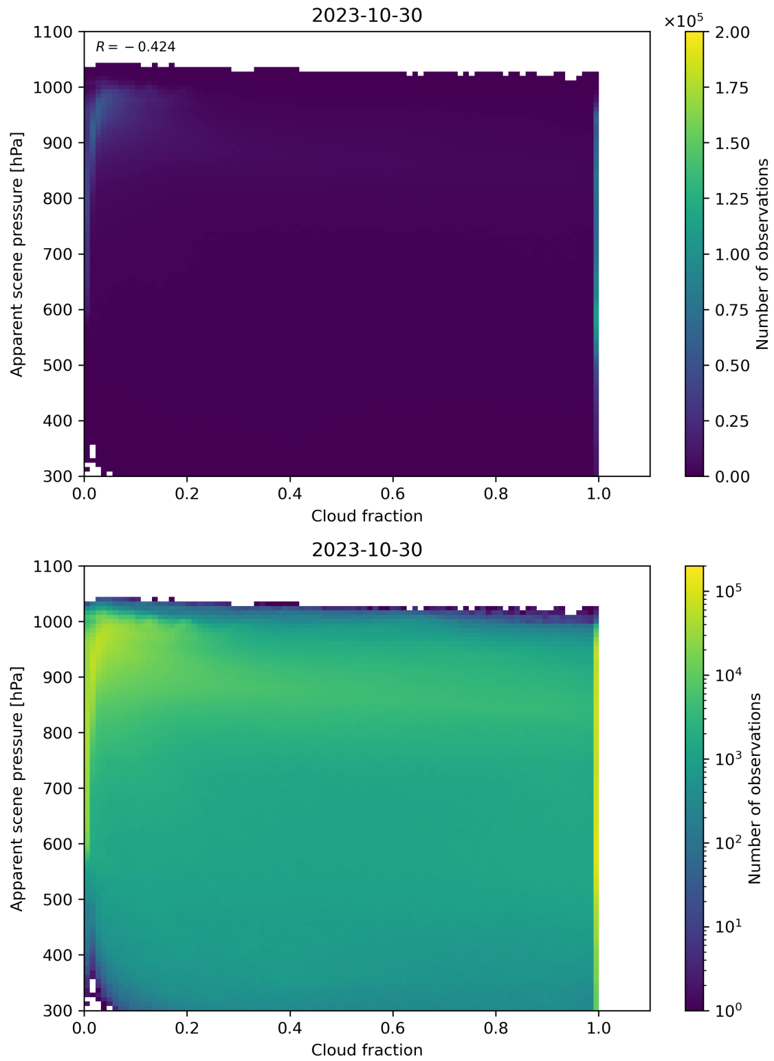
Figure 76: Scatter density plot of “Cloud fraction” against “Apparent scene pressure” for 2023-10-29 to 2023-10-31.
