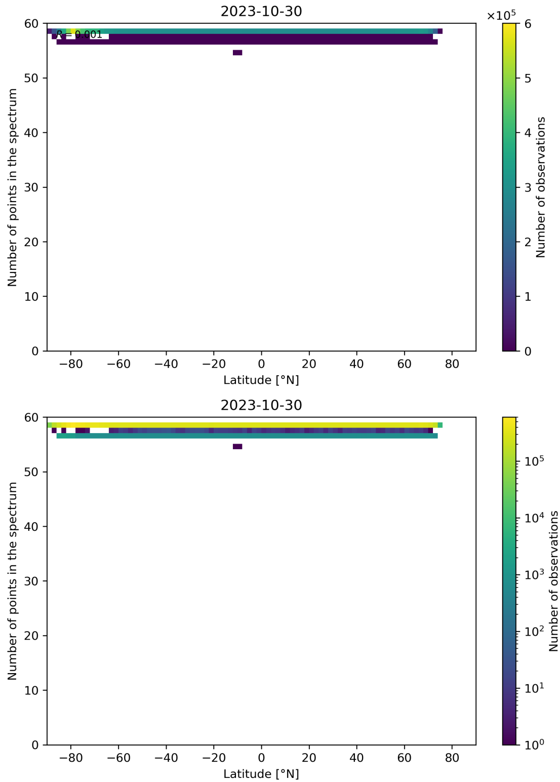
Figure 103: Scatter density plot of “Latitude” against “Number of points in the spectrum” for 2023-10-29 to 2023-10-31.
