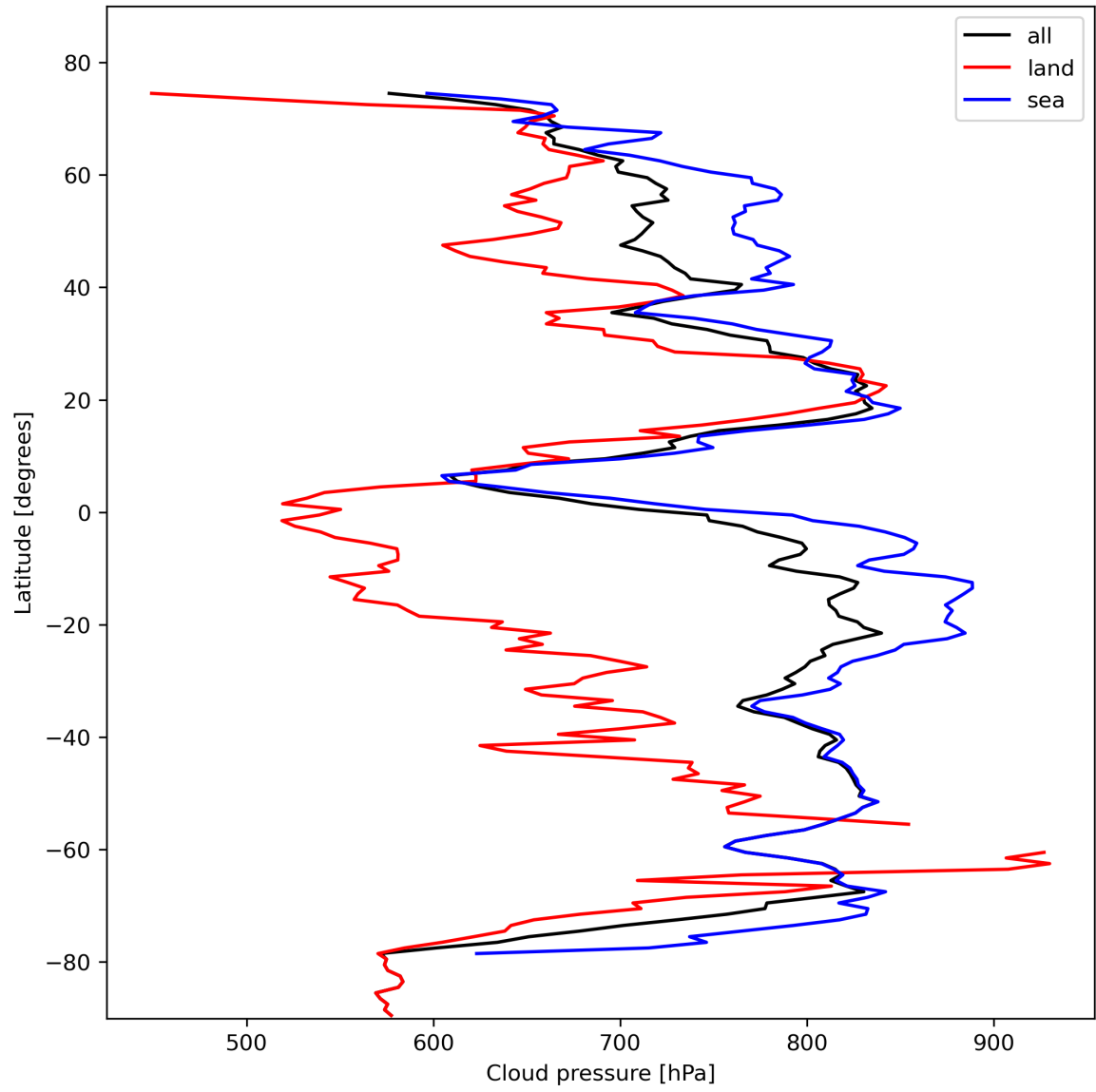
Figure 13: Zonal average of “Cloud pressure” for 2023-10-29 to 2023-10-31.
