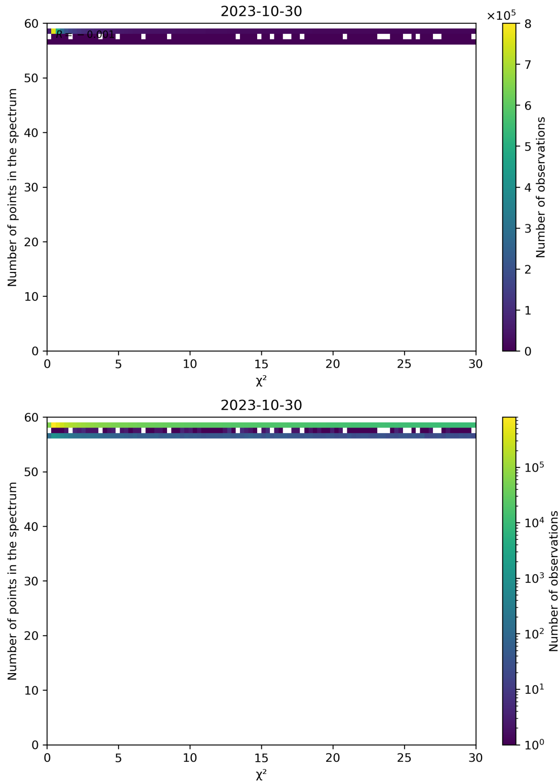
Figure 74: Scatter density plot of “ \chi^2 ” against “Number of points in the spectrum” for 2023-10-29 to 2023-10-31.
