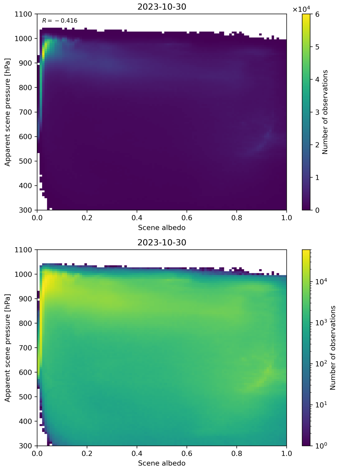
Figure 111: Scatter density plot of “Scene albedo” against “Apparent scene pressure” for 2023-10-29 to 2023-10-31.
