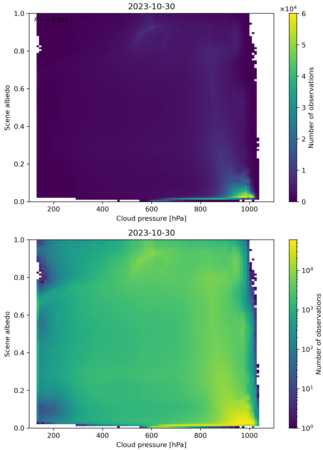
Figure 91: Scatter density plot of “Cloud pressure” against “Scene albedo” for 2023-10-29 to 2023-10-31.
