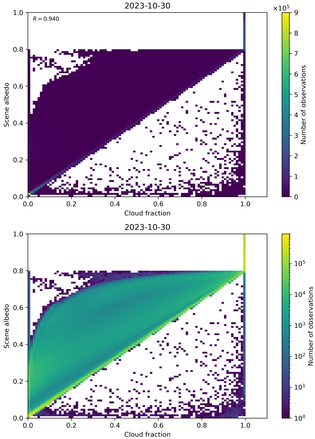
Figure 82: Scatter density plot of “Cloud fraction” against “Scene albedo” for 2023-10-29 to 2023-10-31.
