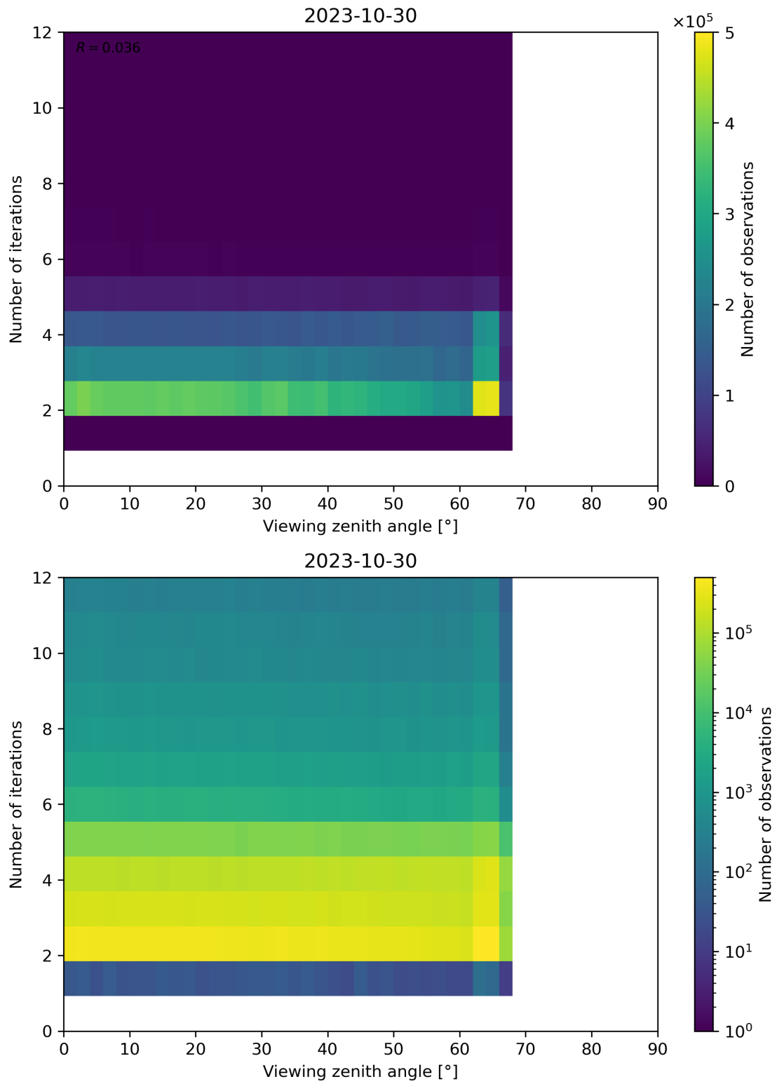
Figure 136: Scatter density plot of “Viewing zenith angle” against “Number of iterations” for 2023-10-29 to 2023-10-31.
