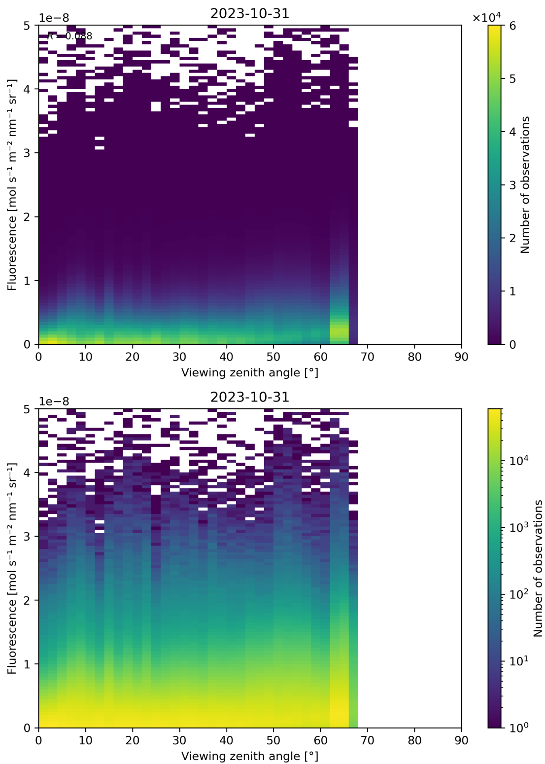
Figure 134: Scatter density plot of “Viewing zenith angle” against “Fluorescence” for 2023-10-30 to 2023-11-01.
