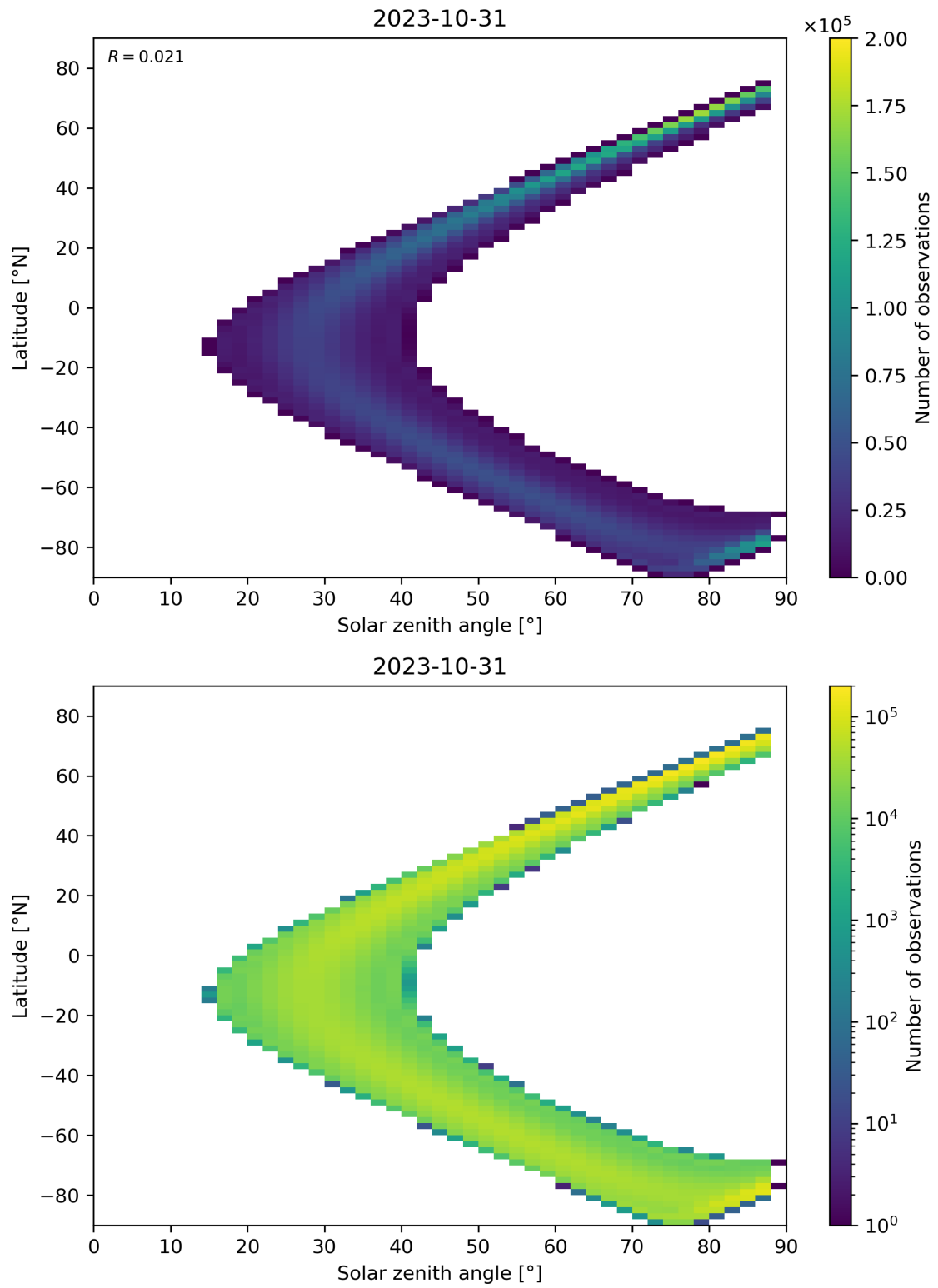
Figure 124: Scatter density plot of “Solar zenith angle” against “Latitude” for 2023-10-30 to 2023-11-01.
