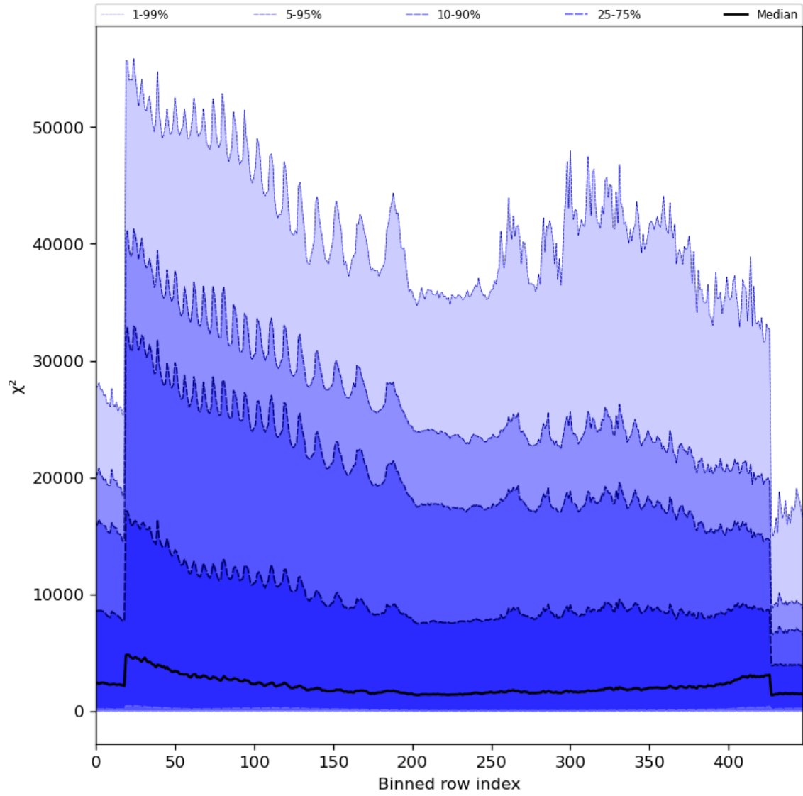
Figure 55: Along track statistics of “ \chi^2 ” for 2023-10-30 to 2023-11-01
