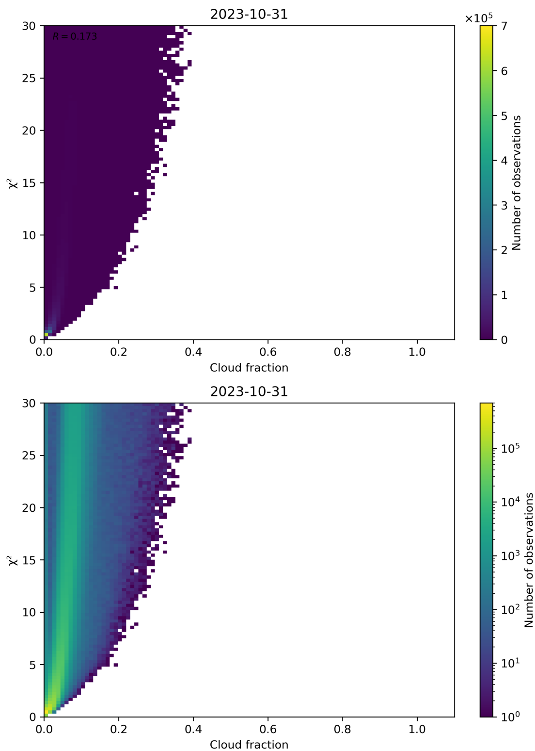
Figure 77: Scatter density plot of “Cloud fraction” against “ \chi^2 ” for 2023-10-30 to 2023-11-01.
