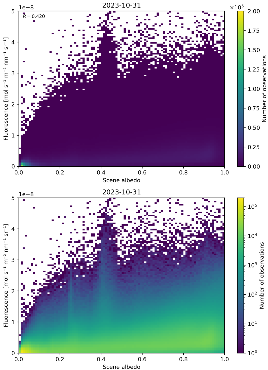
Figure 114: Scatter density plot of “Scene albedo” against “Fluorescence” for 2023-10-30 to 2023-11-01.
