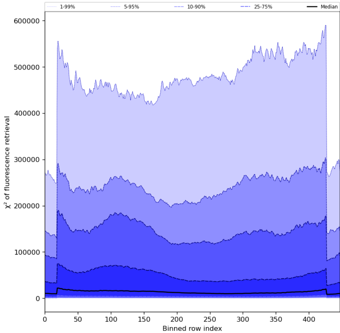
Figure 59: Along track statistics of “ \chi^2 of fluorescence retrieval” for 2023-10-30 to 2023-11-01
