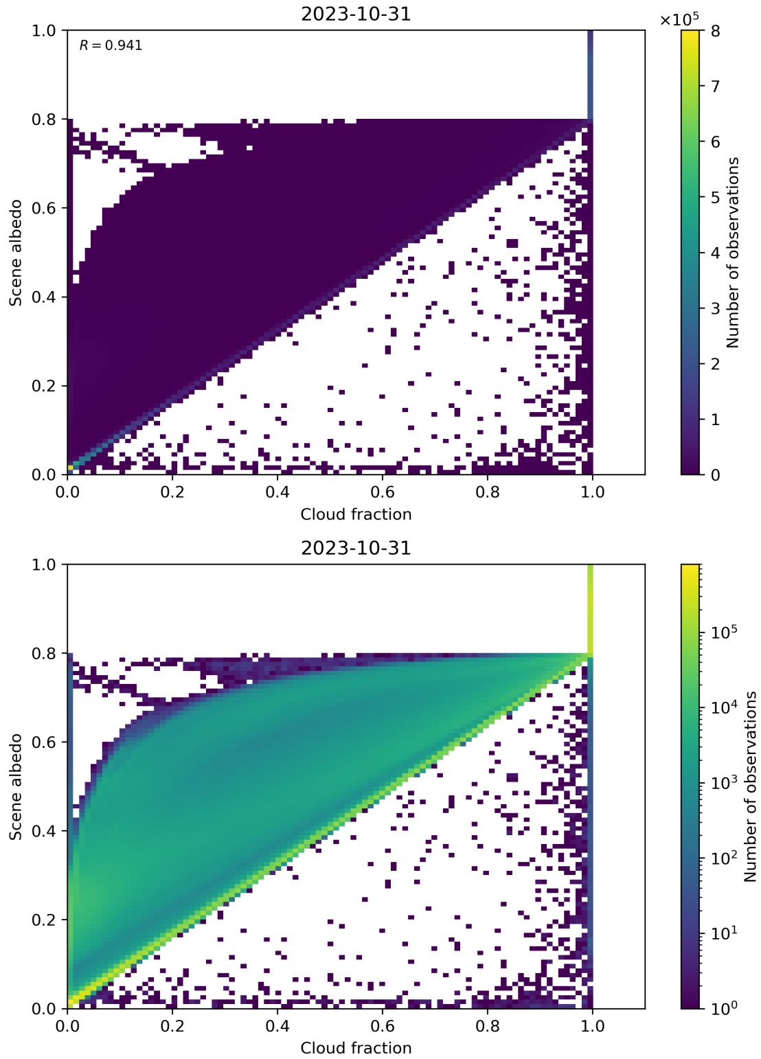
Figure 82: Scatter density plot of “Cloud fraction” against “Scene albedo” for 2023-10-30 to 2023-11-01.
