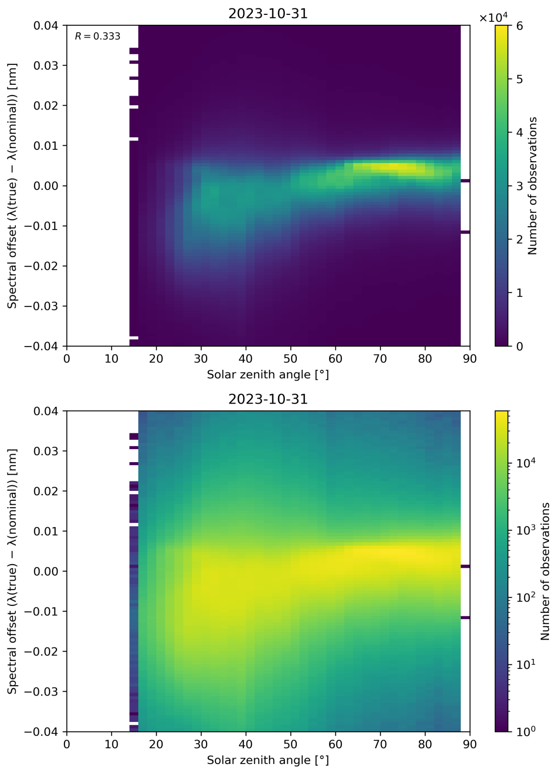
Figure 128: Scatter density plot of “Solar zenith angle” against “Spectral offset ( \lambda(\text{true}) - \lambda(\text{nominal}) )” for 2023-10-30 to 2023-11-01.
