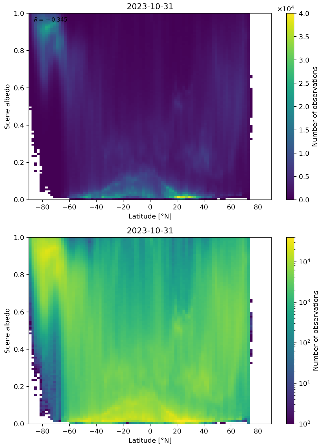
Figure 104: Scatter density plot of “Latitude” against “Scene albedo” for 2023-10-30 to 2023-11-01.
