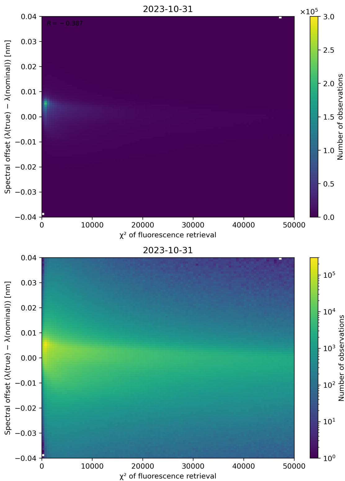
Figure 72: Scatter density plot of " \chi^2 of fluorescence retrieval" against "Spectral offset ( \lambda(\text{true}) - \lambda(\text{nominal})) " for 2023-10-30 to 2023-11-01.
