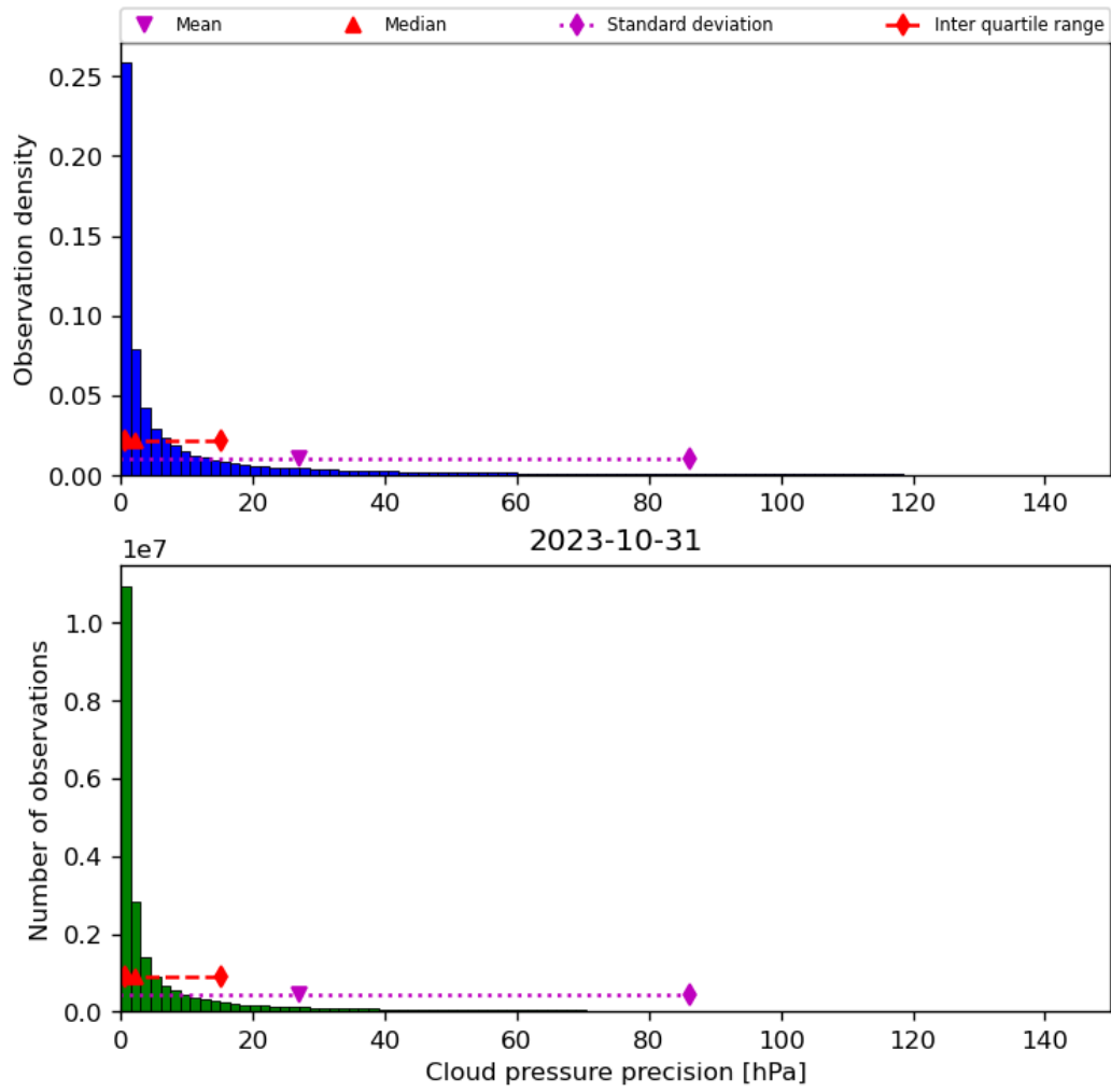
Figure 31: Histogram of “Cloud pressure precision” for 2023-10-30 to 2023-11-01
