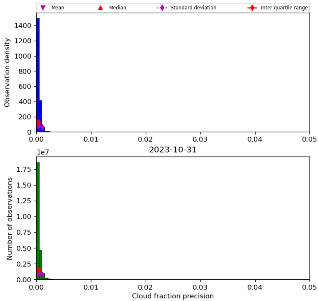
Figure 33: Histogram of “Cloud fraction precision” for 2023-10-30 to 2023-11-01
