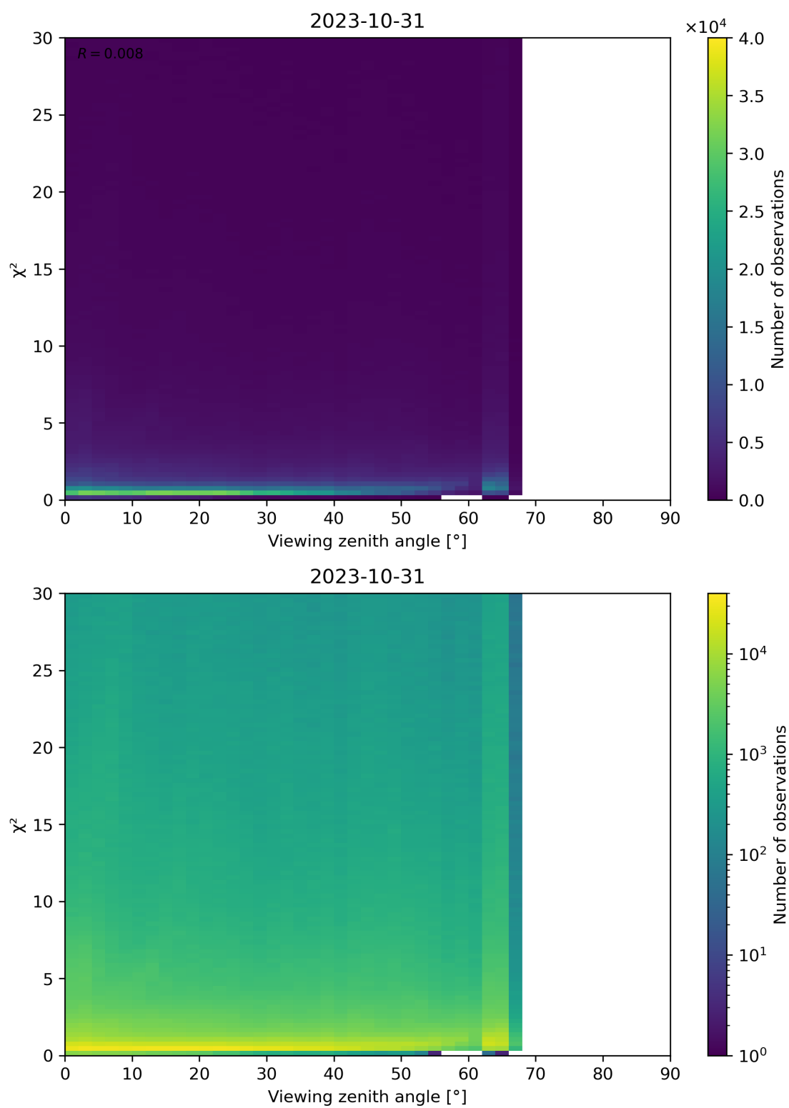
Figure 130: Scatter density plot of “Viewing zenith angle” against “ \chi^2 ” for 2023-10-30 to 2023-11-01.
