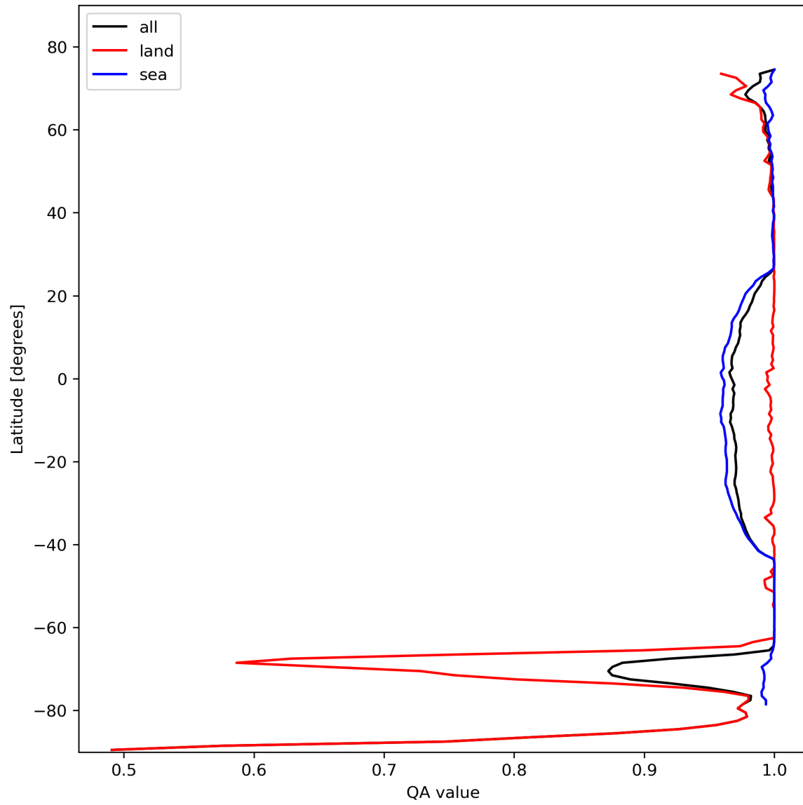
Figure 12: Zonal average of “QA value” for 2023-10-30 to 2023-11-01.
