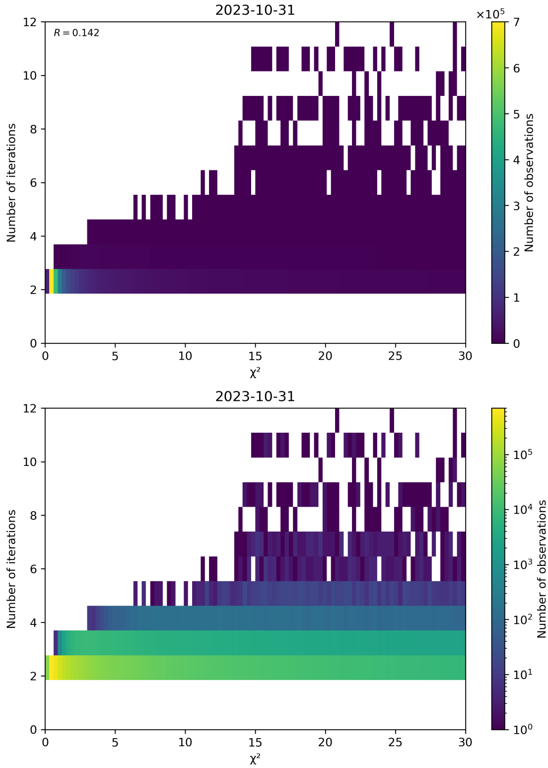
Figure 73: Scatter density plot of “ \chi^2 ” against “Number of iterations” for 2023-10-30 to 2023-11-01.
