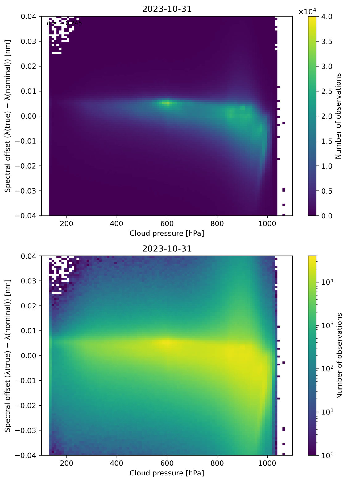
Figure 92: Scatter density plot of “Cloud pressure” against “Spectral offset ( \lambda(\text{true}) - \lambda(\text{nominal}) )” for 2023-10-30 to 2023-11-01.
