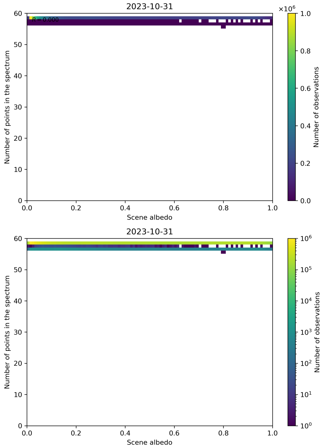
Figure 116: Scatter density plot of “Scene albedo” against “Number of points in the spectrum” for 2023-10-30 to 2023-11-01.
