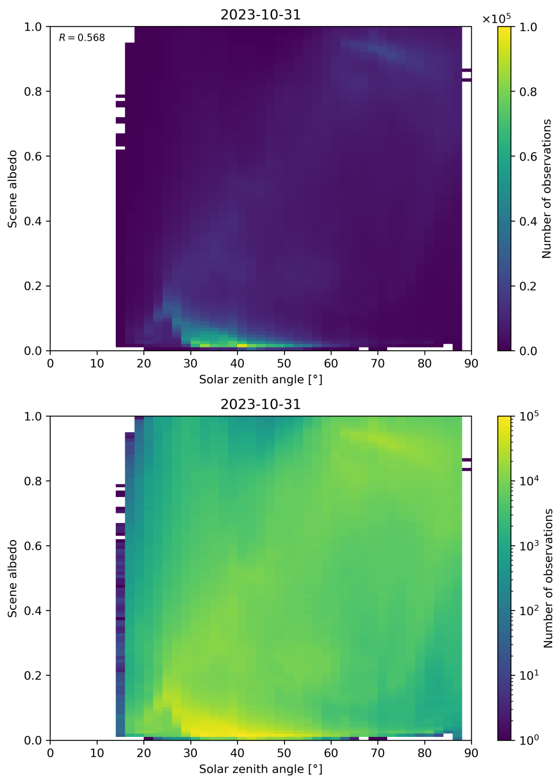
Figure 127: Scatter density plot of “Solar zenith angle” against “Scene albedo” for 2023-10-30 to 2023-11-01.
