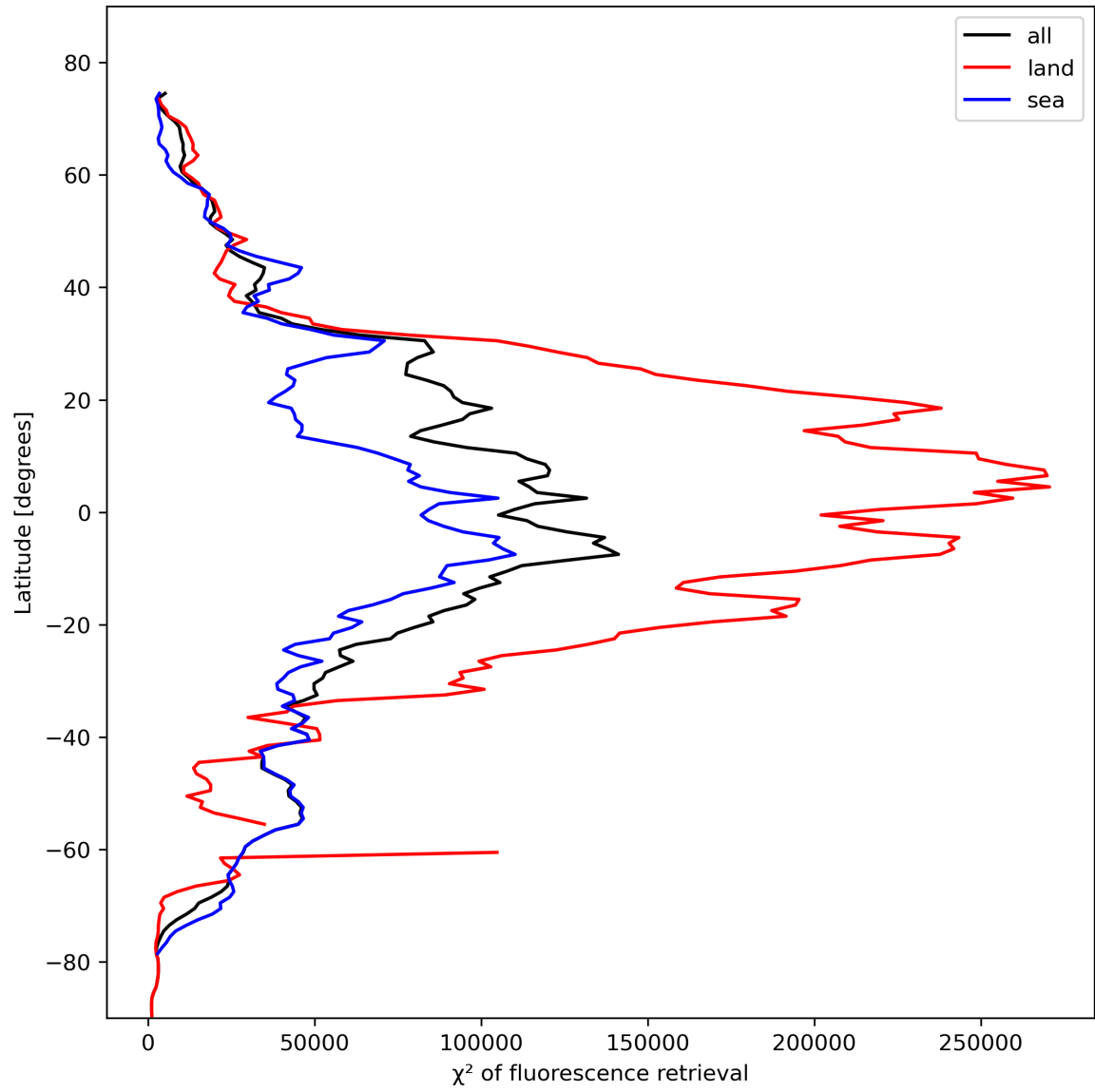
Figure 25: Zonal average of “ \chi^2 of fluorescence retrieval” for 2023-10-30 to 2023-11-01.
