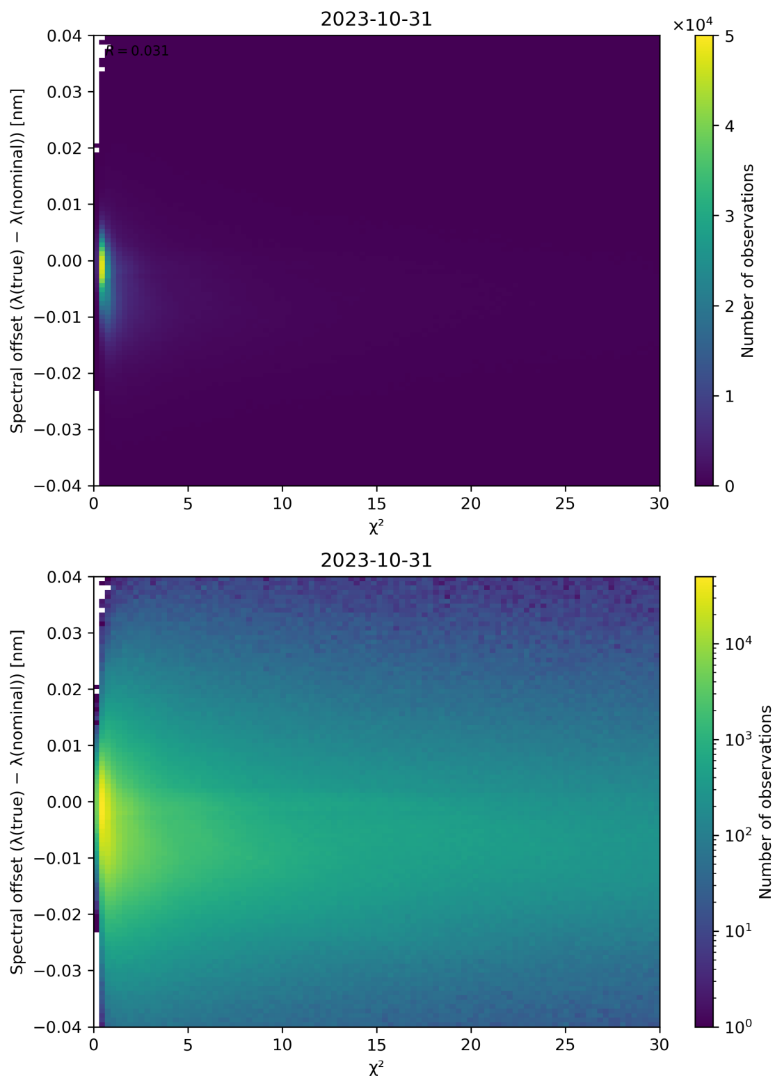
Figure 75: Scatter density plot of “ \chi^2 ” against “Spectral offset ( \lambda(\text{true}) - \lambda(\text{nominal}) )” for 2023-10-30 to 2023-11-01.
