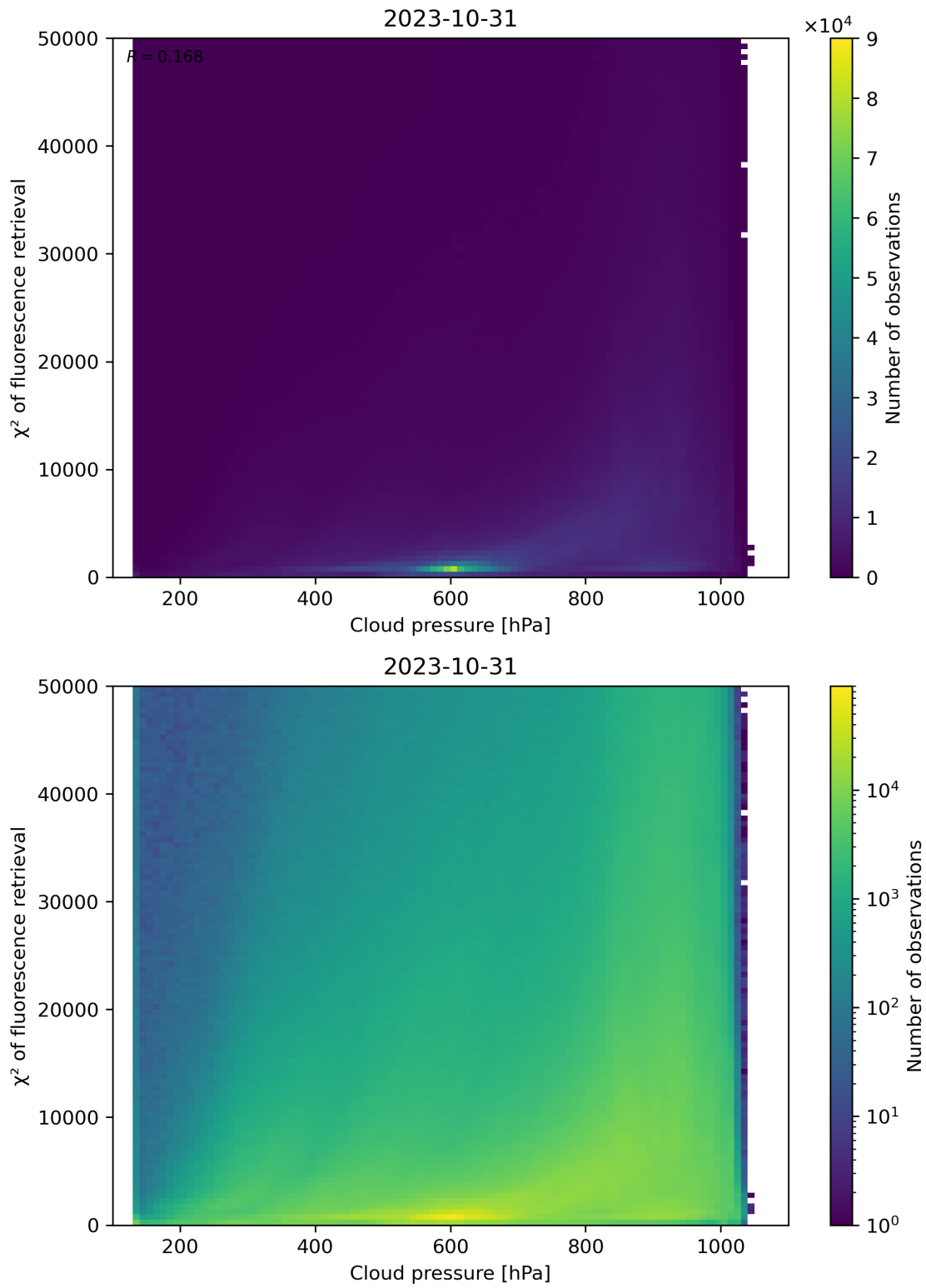
Figure 86: Scatter density plot of “Cloud pressure” against “ \chi^2 of fluorescence retrieval” for 2023-10-30 to 2023-11-01.
