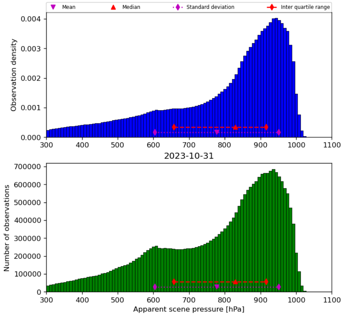
Figure 36: Histogram of “Apparent scene pressure” for 2023-10-30 to 2023-11-01
