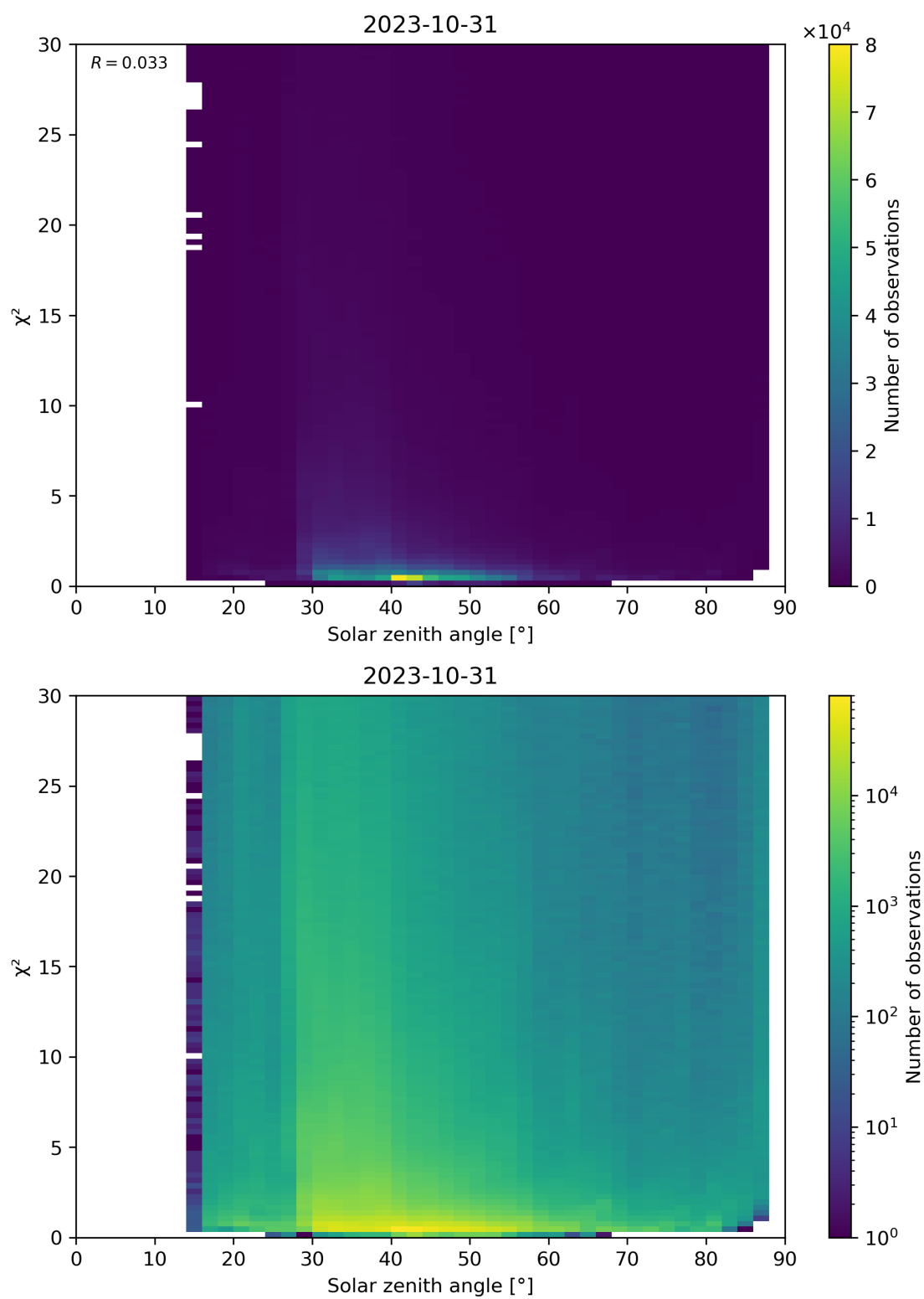
Figure 119: Scatter density plot of “Solar zenith angle” against “ \chi^2 ” for 2023-10-30 to 2023-11-01.
