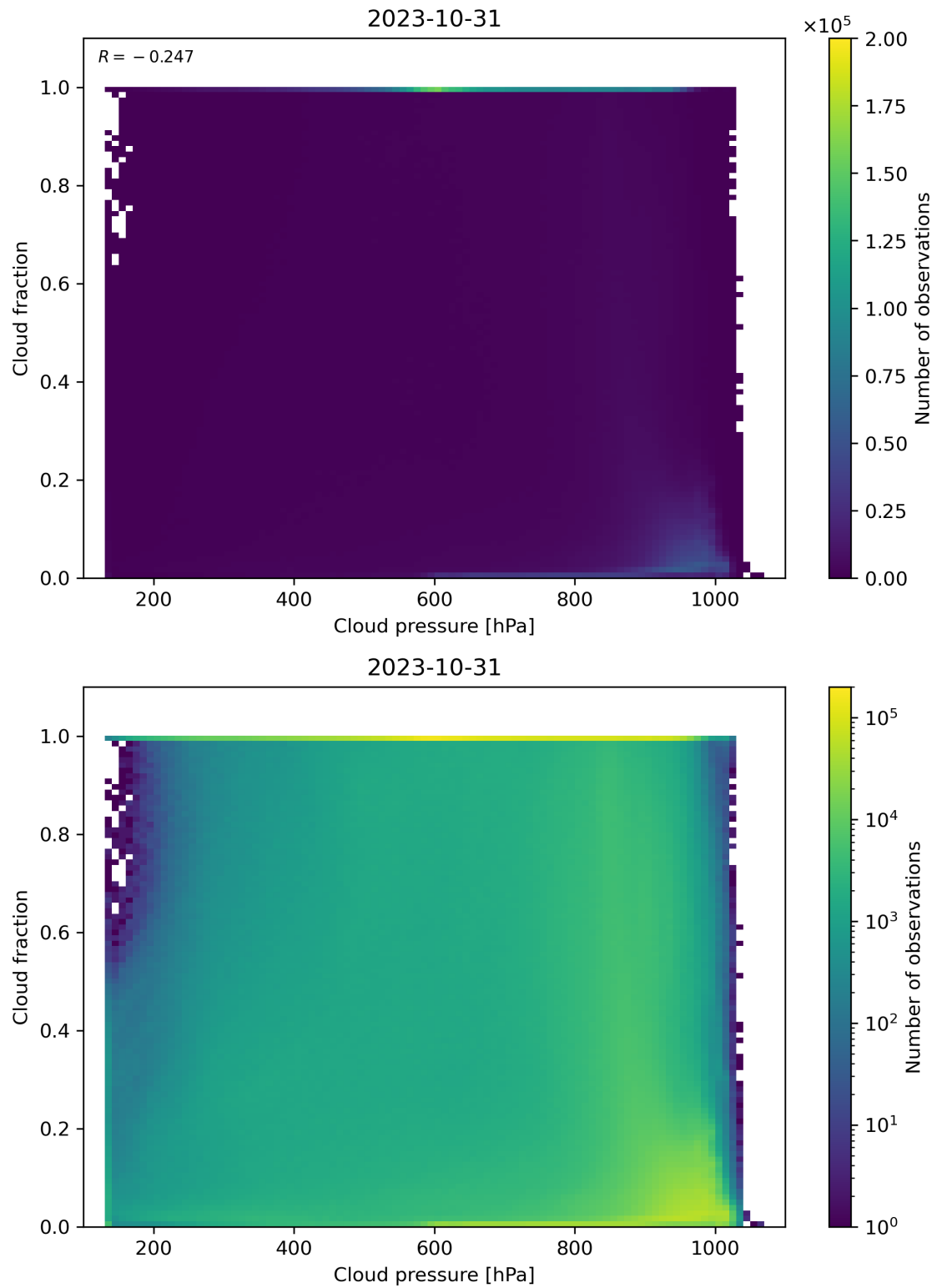
Figure 87: Scatter density plot of “Cloud pressure” against “Cloud fraction” for 2023-10-30 to 2023-11-01.
