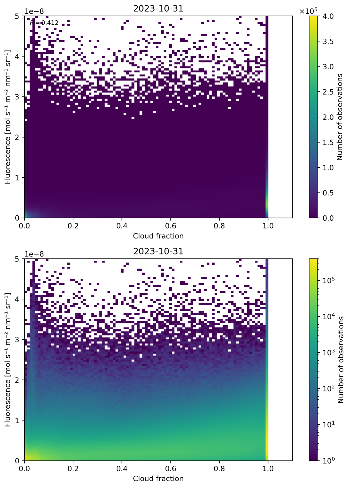
Figure 79: Scatter density plot of “Cloud fraction” against “Fluorescence” for 2023-10-30 to 2023-11-01.
