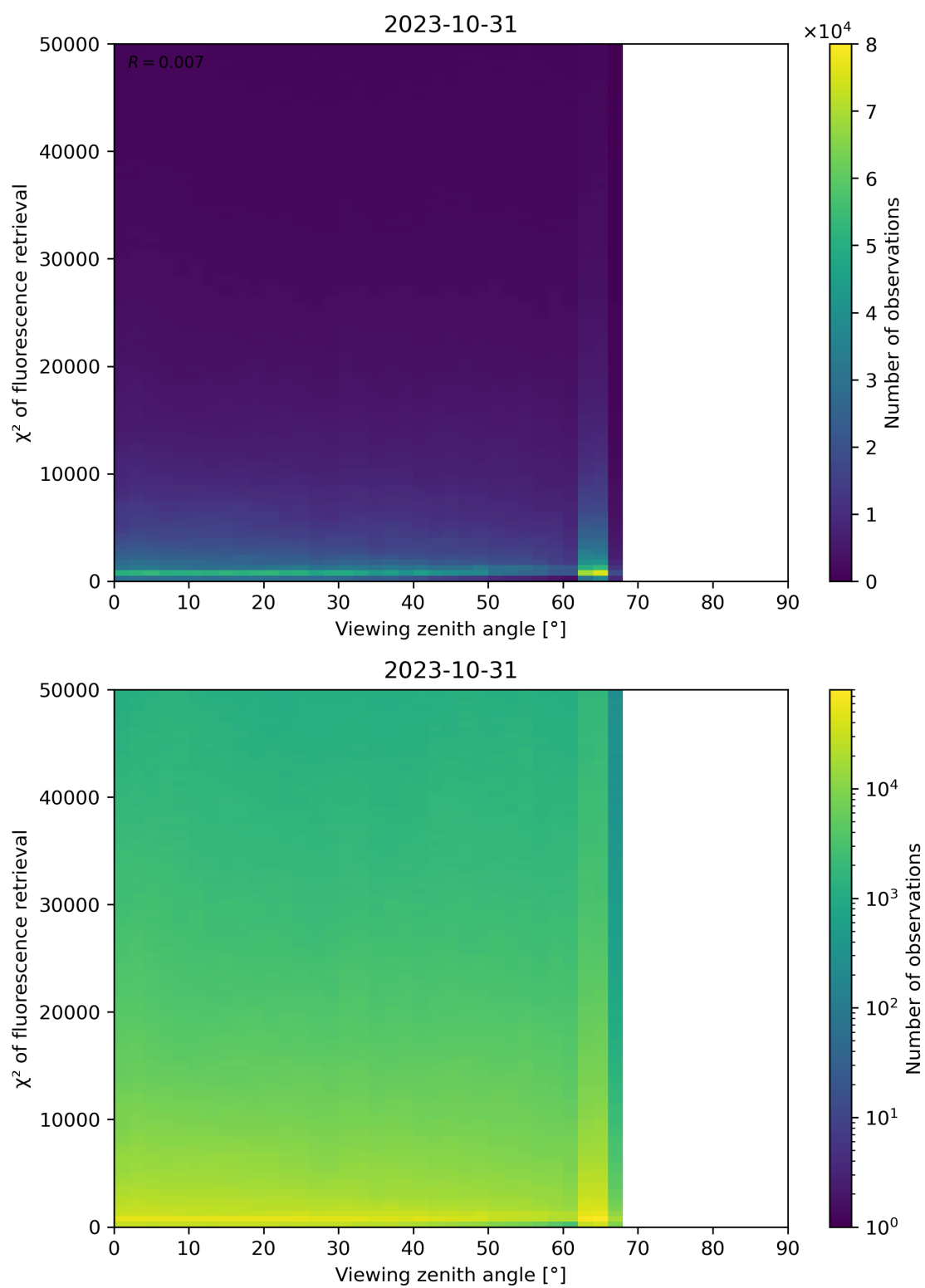
Figure 131: Scatter density plot of “Viewing zenith angle” against “ \chi^2 of fluorescence retrieval” for 2023-10-30 to 2023-11-01.
