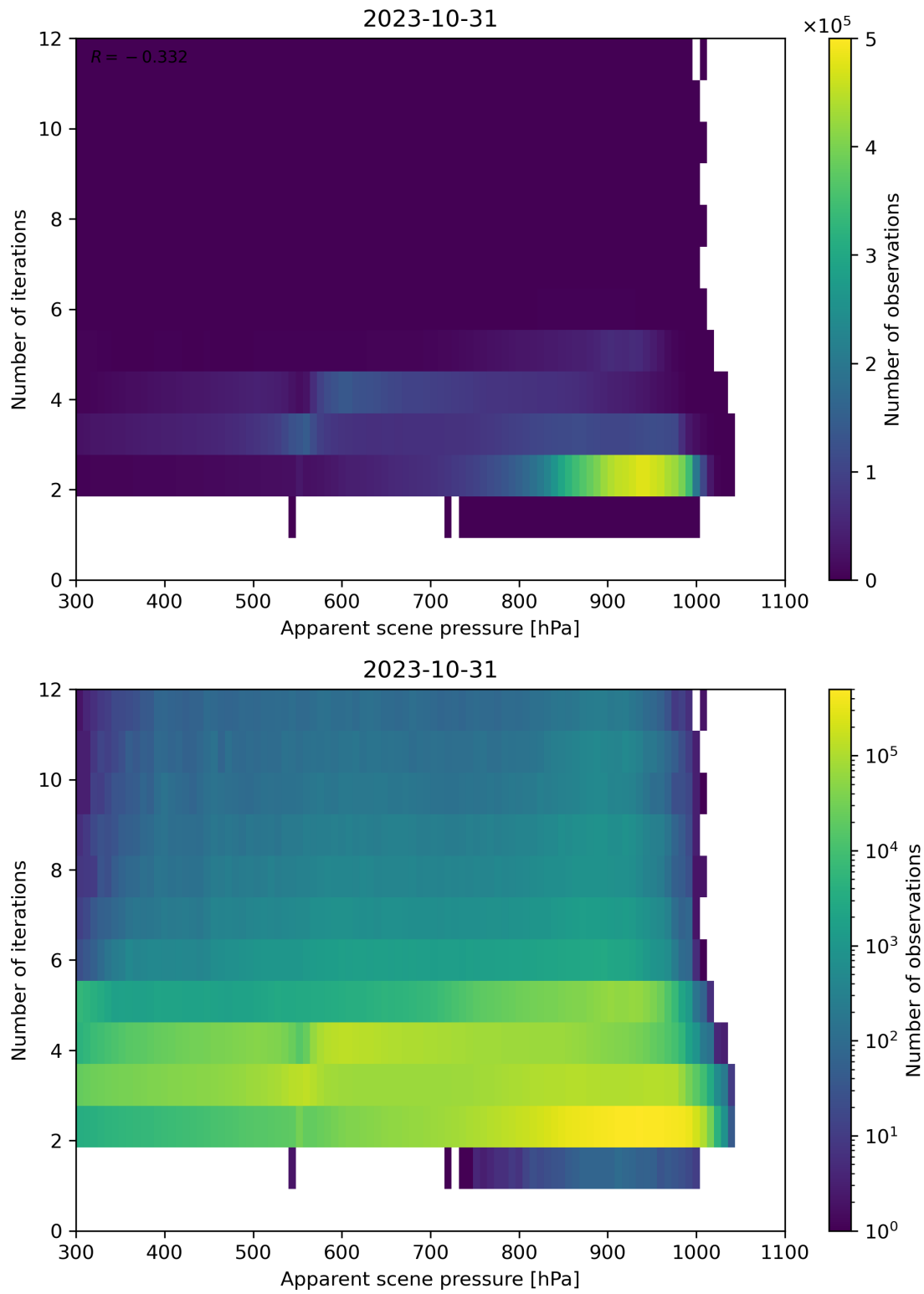
Figure 66: Scatter density plot of “Apparent scene pressure” against “Number of iterations” for 2023-10-30 to 2023-11-01.
