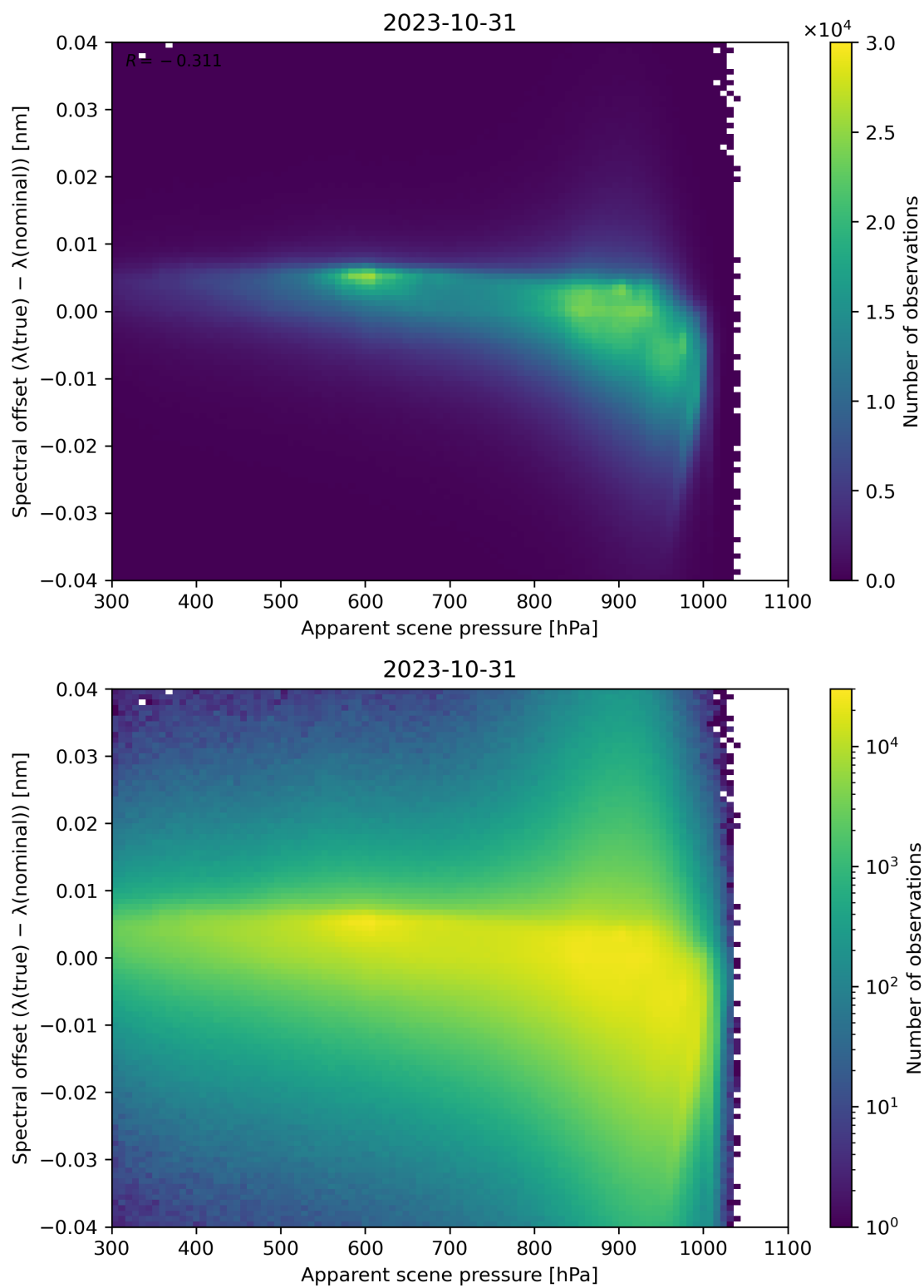
Figure 68: Scatter density plot of “Apparent scene pressure” against “Spectral offset ( \lambda(\text{true}) - \lambda(\text{nominal}) )” for 2023-10-30 to 2023-11-01.
