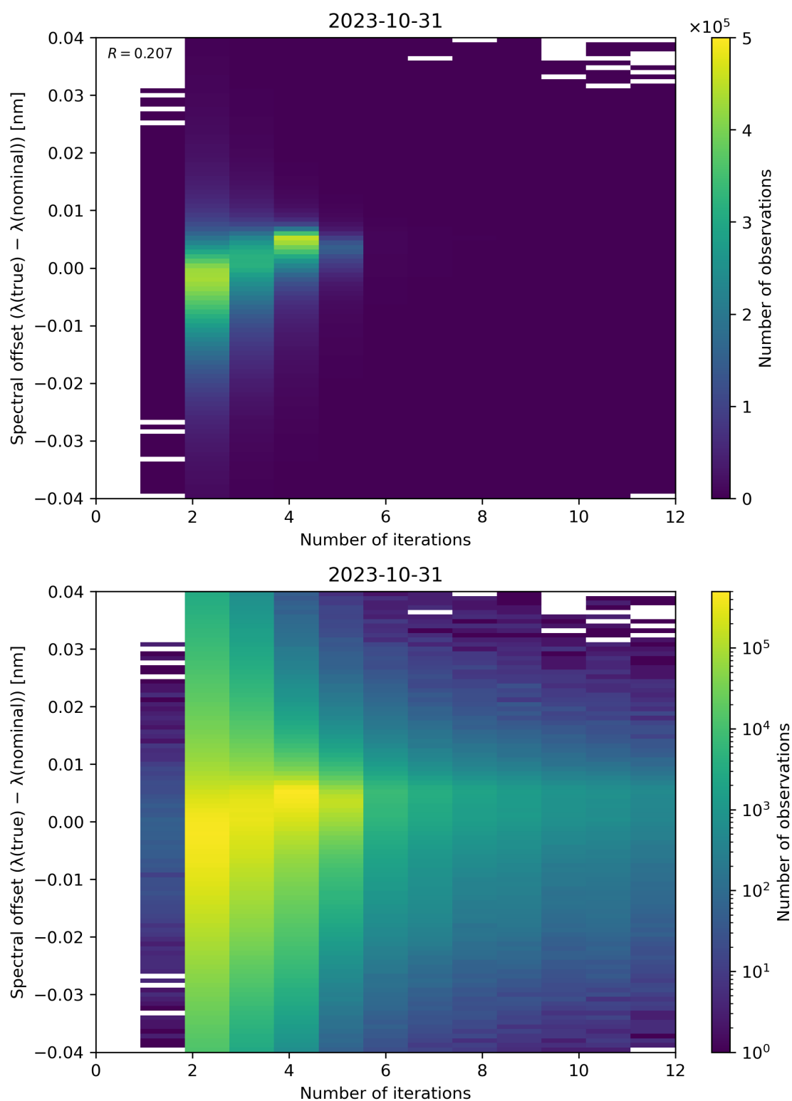
Figure 109: Scatter density plot of “Number of iterations” against “Spectral offset ( \lambda(\text{true}) - \lambda(\text{nominal}) )” for 2023-10-30 to 2023-11-01.
