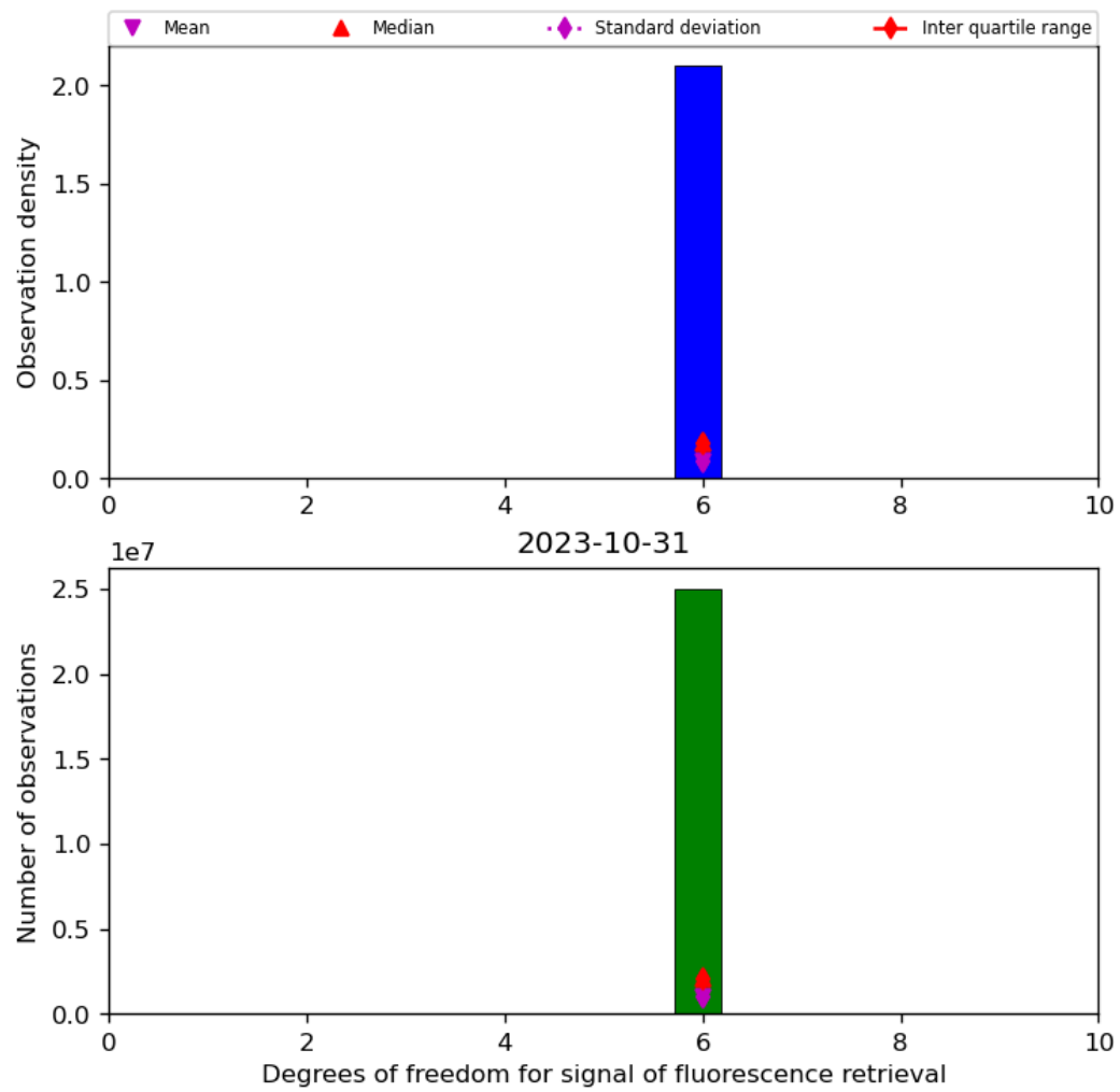
Figure 43: Histogram of “Degrees of freedom for signal of fluorescence retrieval” for 2023-10-30 to 2023-11-01
