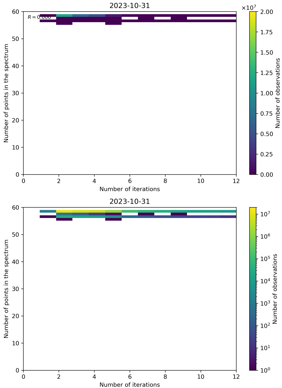
Figure 108: Scatter density plot of “Number of iterations” against “Number of points in the spectrum” for 2023-10-30 to 2023-11-01.
