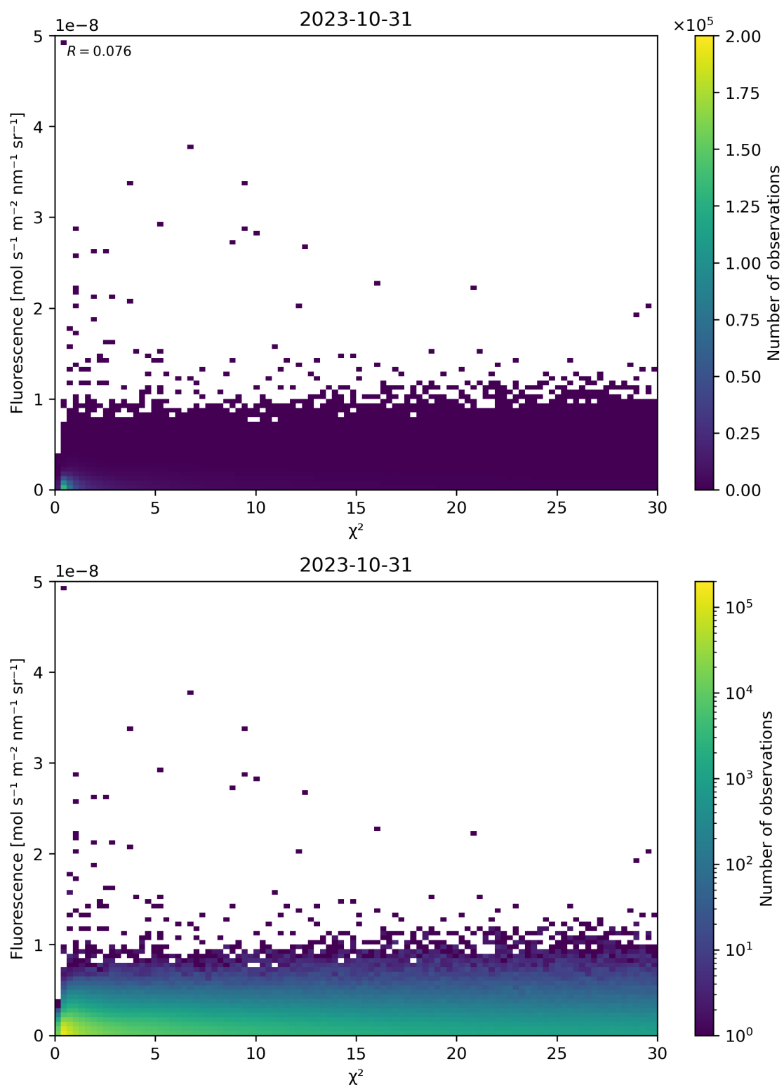
Figure 70: Scatter density plot of “ \chi^2 ” against “Fluorescence” for 2023-10-30 to 2023-11-01.
