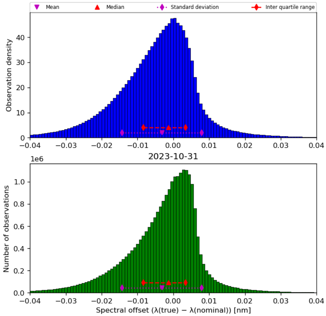
Figure 45: Histogram of “Spectral offset ( \lambda(\text{true}) - \lambda(\text{nominal}) )” for 2023-10-30 to 2023-11-01
