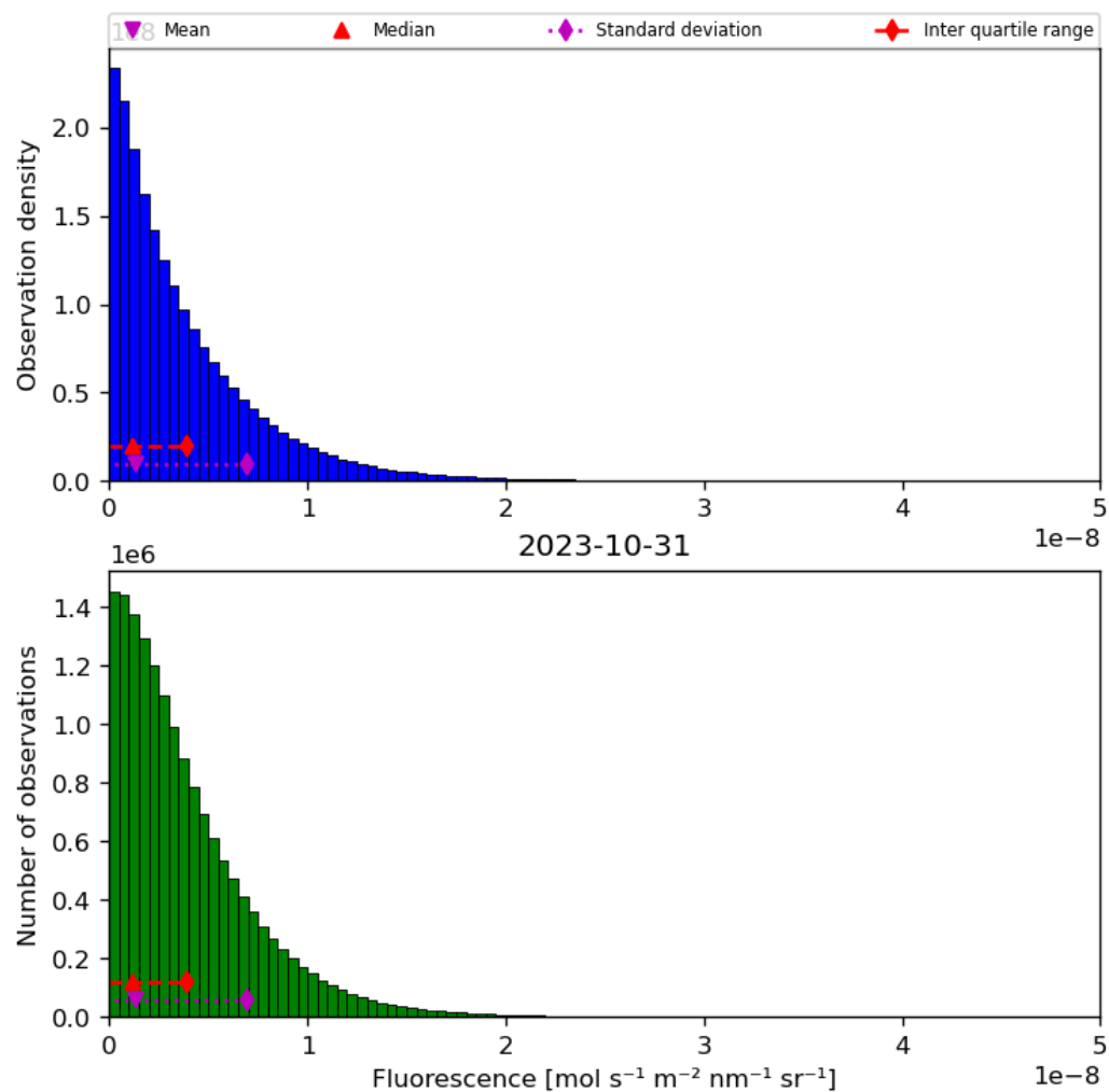
Figure 40: Histogram of “Fluorescence” for 2023-10-30 to 2023-11-01
