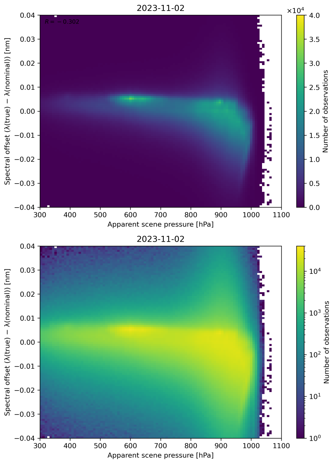
Figure 68: Scatter density plot of “Apparent scene pressure” against “Spectral offset ( \lambda(\text{true}) - \lambda(\text{nominal}) )” for 2023-11-02 to 2023-11-03.
