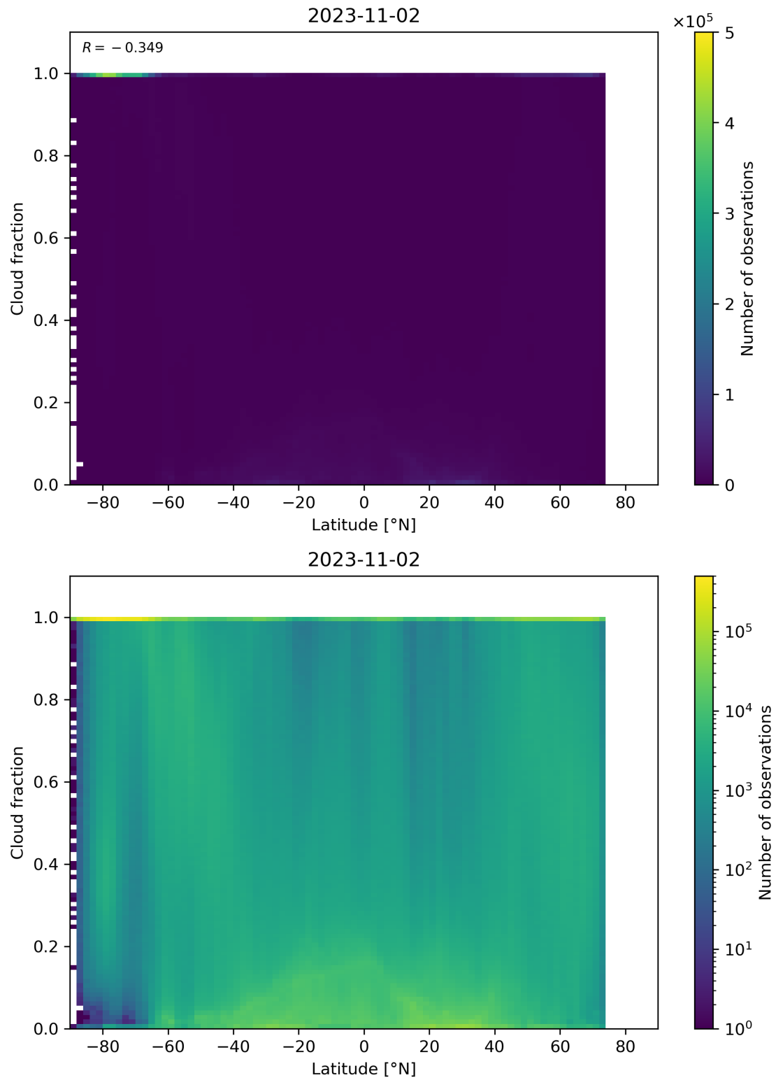
Figure 99: Scatter density plot of “Latitude” against “Cloud fraction” for 2023-11-02 to 2023-11-03.
