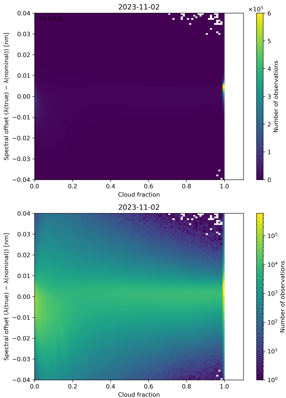
Figure 83: Scatter density plot of “Cloud fraction” against “Spectral offset ( \lambda(\text{true}) - \lambda(\text{nominal}) )” for 2023-11-02 to 2023-11-03.
