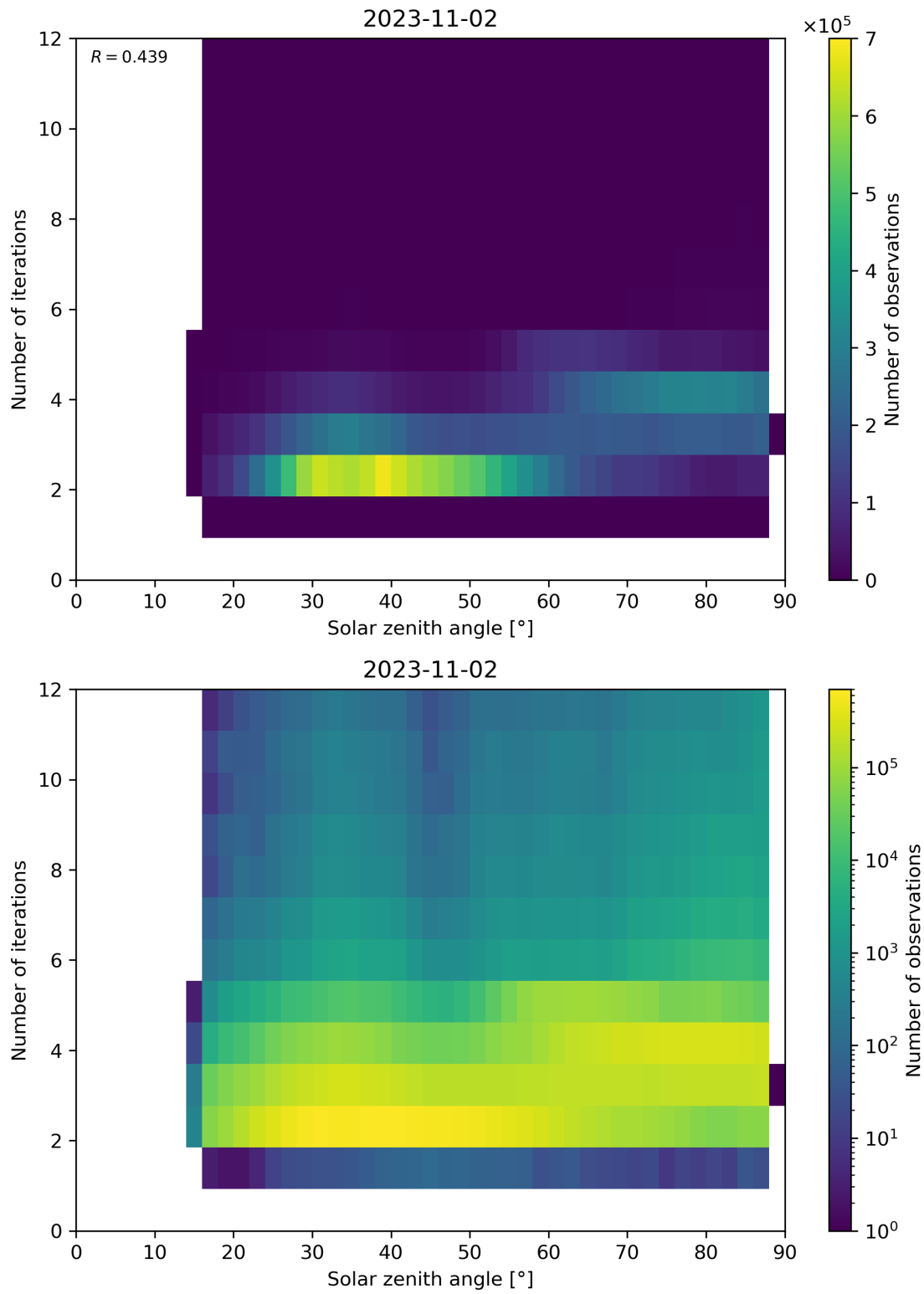
Figure 125: Scatter density plot of “Solar zenith angle” against “Number of iterations” for 2023-11-02 to 2023-11-03.
