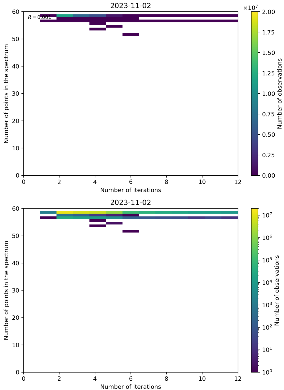
Figure 108: Scatter density plot of “Number of iterations” against “Number of points in the spectrum” for 2023-11-02 to 2023-11-03.
