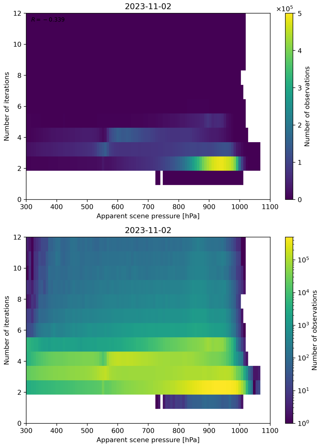
Figure 66: Scatter density plot of “Apparent scene pressure” against “Number of iterations” for 2023-11-02 to 2023-11-03.
