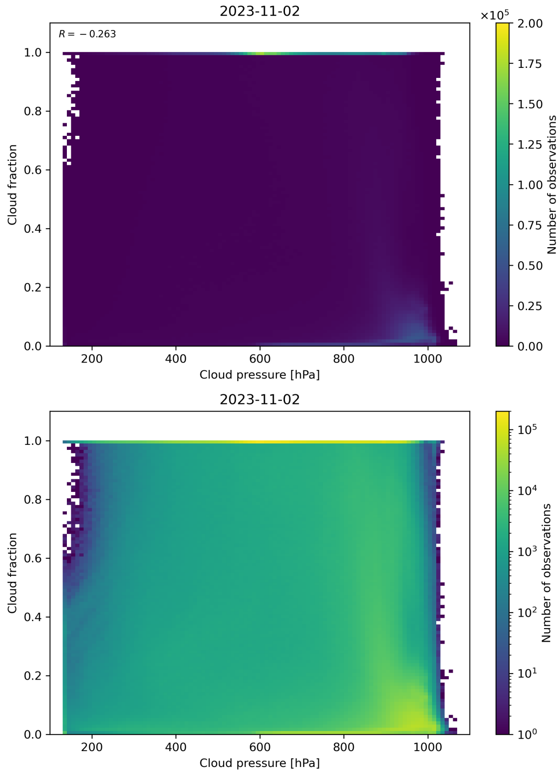
Figure 87: Scatter density plot of “Cloud pressure” against “Cloud fraction” for 2023-11-02 to 2023-11-03.
