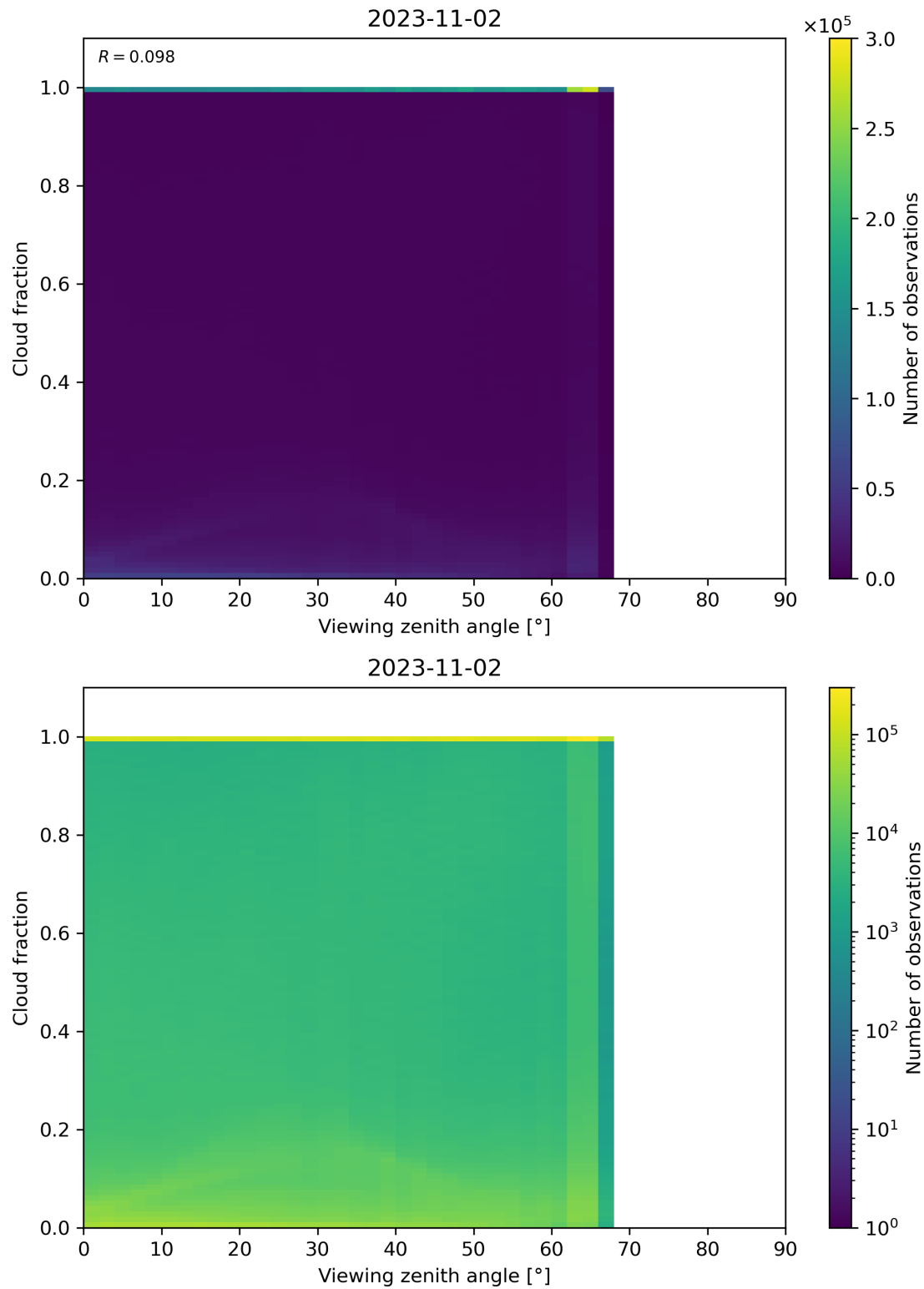
Figure 132: Scatter density plot of “Viewing zenith angle” against “Cloud fraction” for 2023-11-02 to 2023-11-03.
