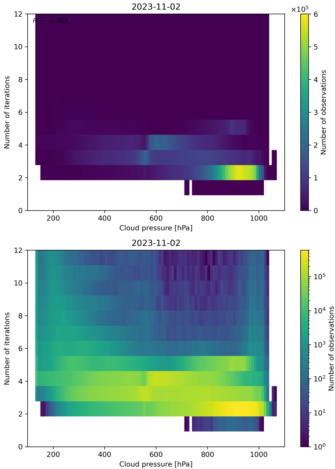
Figure 89: Scatter density plot of “Cloud pressure” against “Number of iterations” for 2023-11-02 to 2023-11-03.
