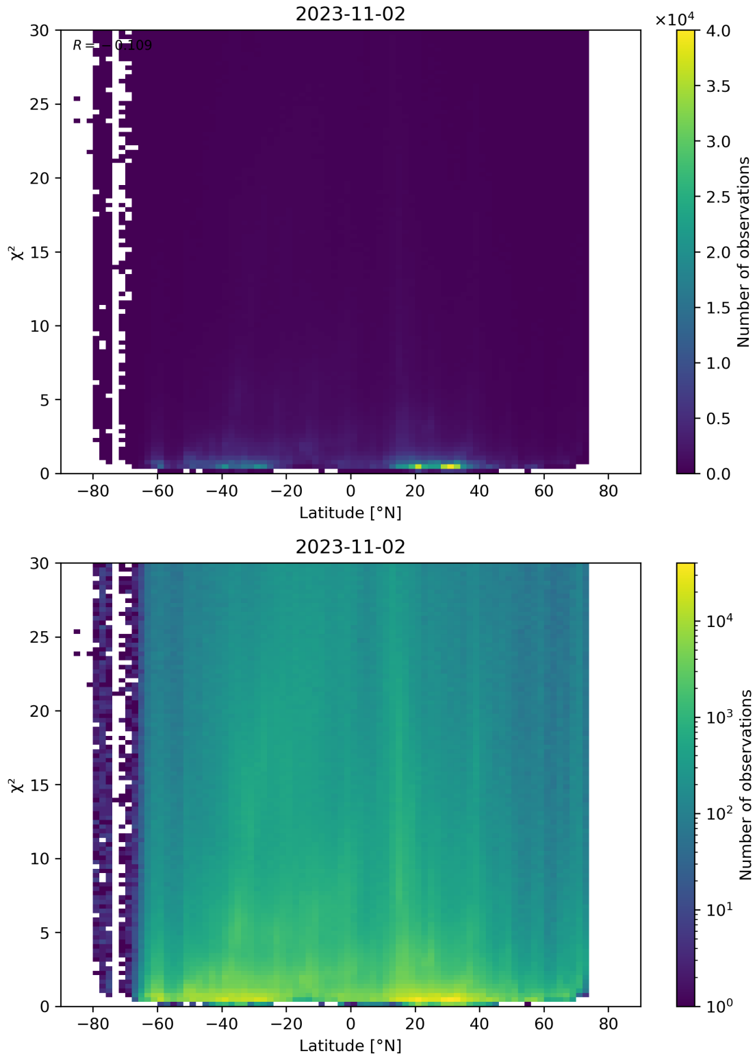
Figure 97: Scatter density plot of “Latitude” against “ \chi^2 ” for 2023-11-02 to 2023-11-03.
