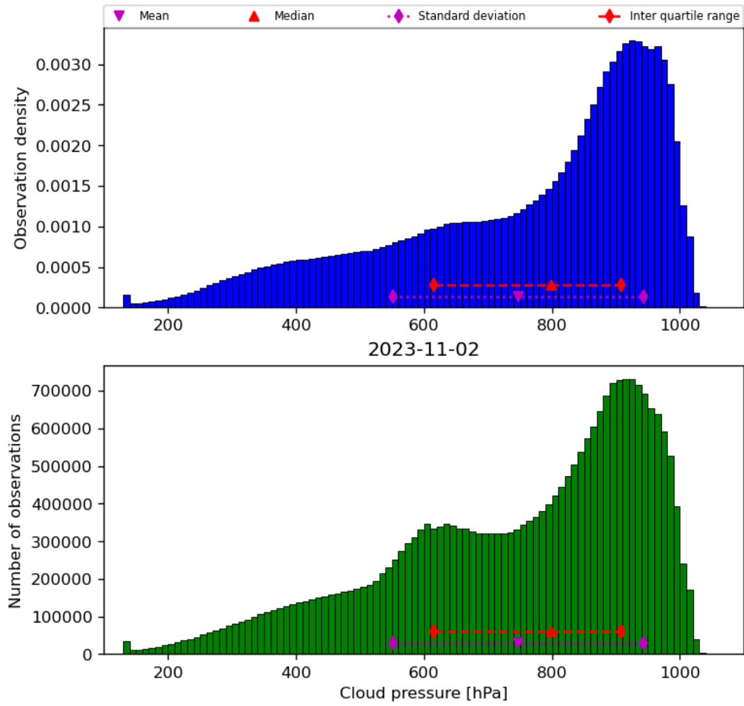
Figure 30: Histogram of “Cloud pressure” for 2023-11-02 to 2023-11-03
