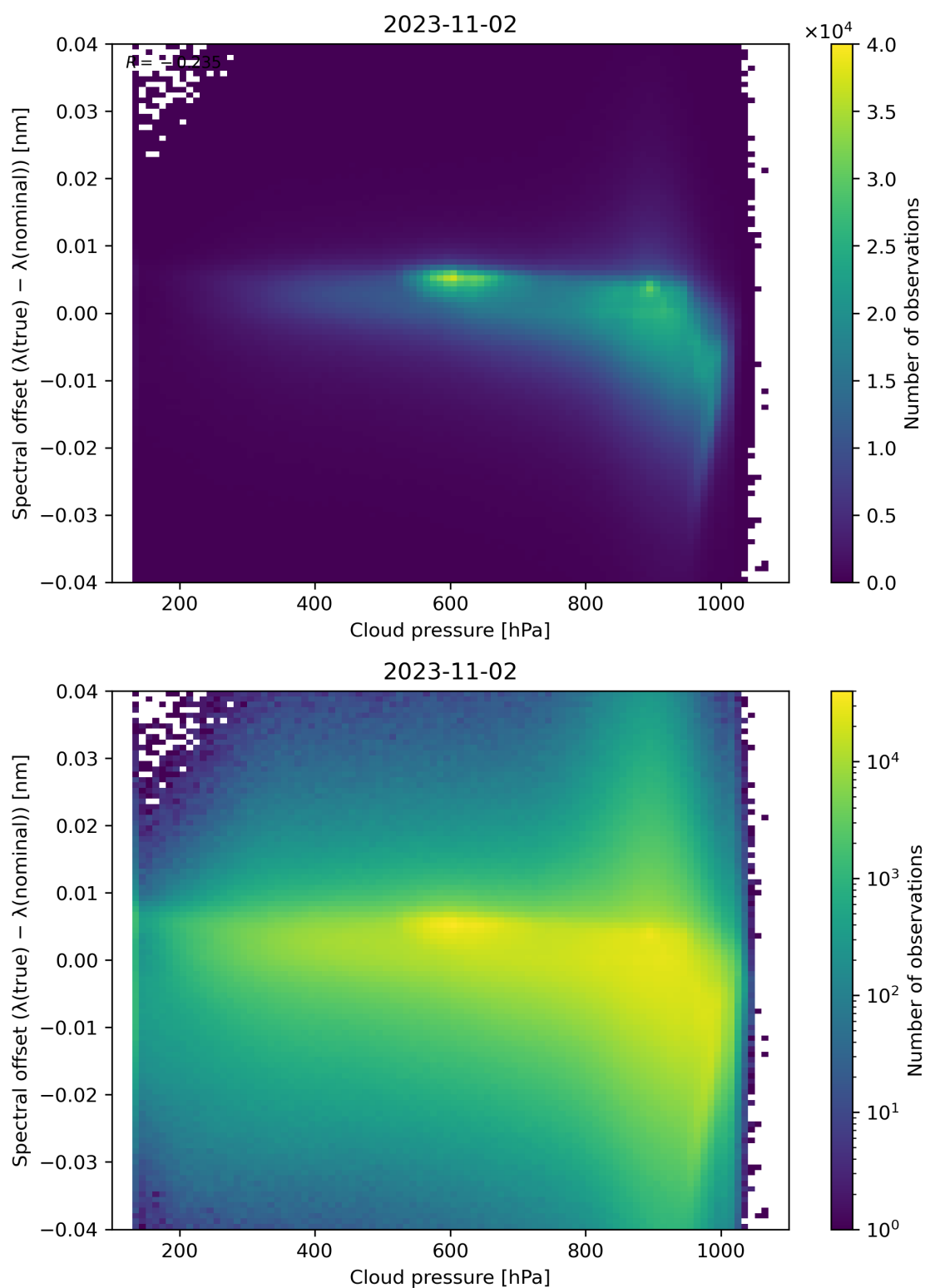
Figure 92: Scatter density plot of “Cloud pressure” against “Spectral offset ( \lambda(\text{true}) - \lambda(\text{nominal}) )” for 2023-11-02 to 2023-11-03.
