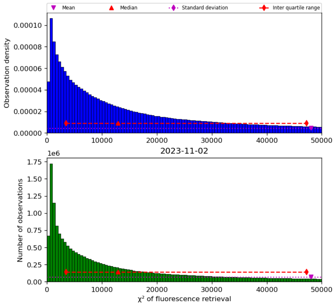
Figure 42: Histogram of “ \chi^2 of fluorescence retrieval” for 2023-11-02 to 2023-11-03
