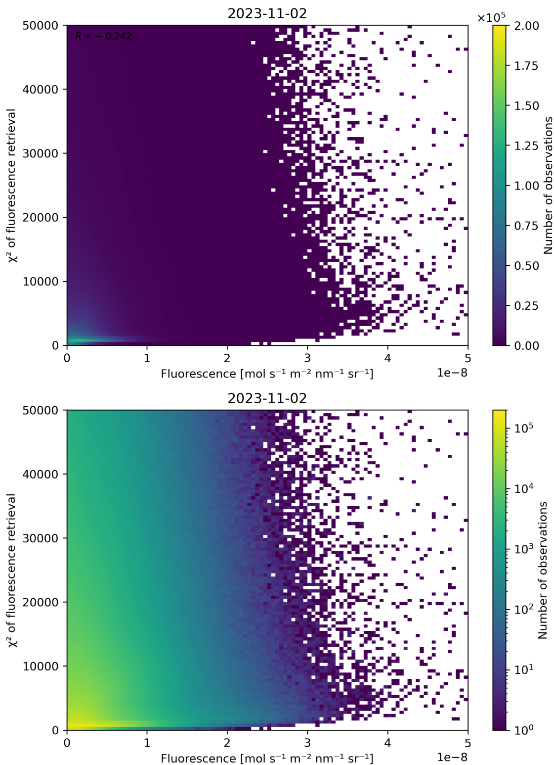
Figure 93: Scatter density plot of “Fluorescence” against “ \chi^2 of fluorescence retrieval” for 2023-11-02 to 2023-11-03.
