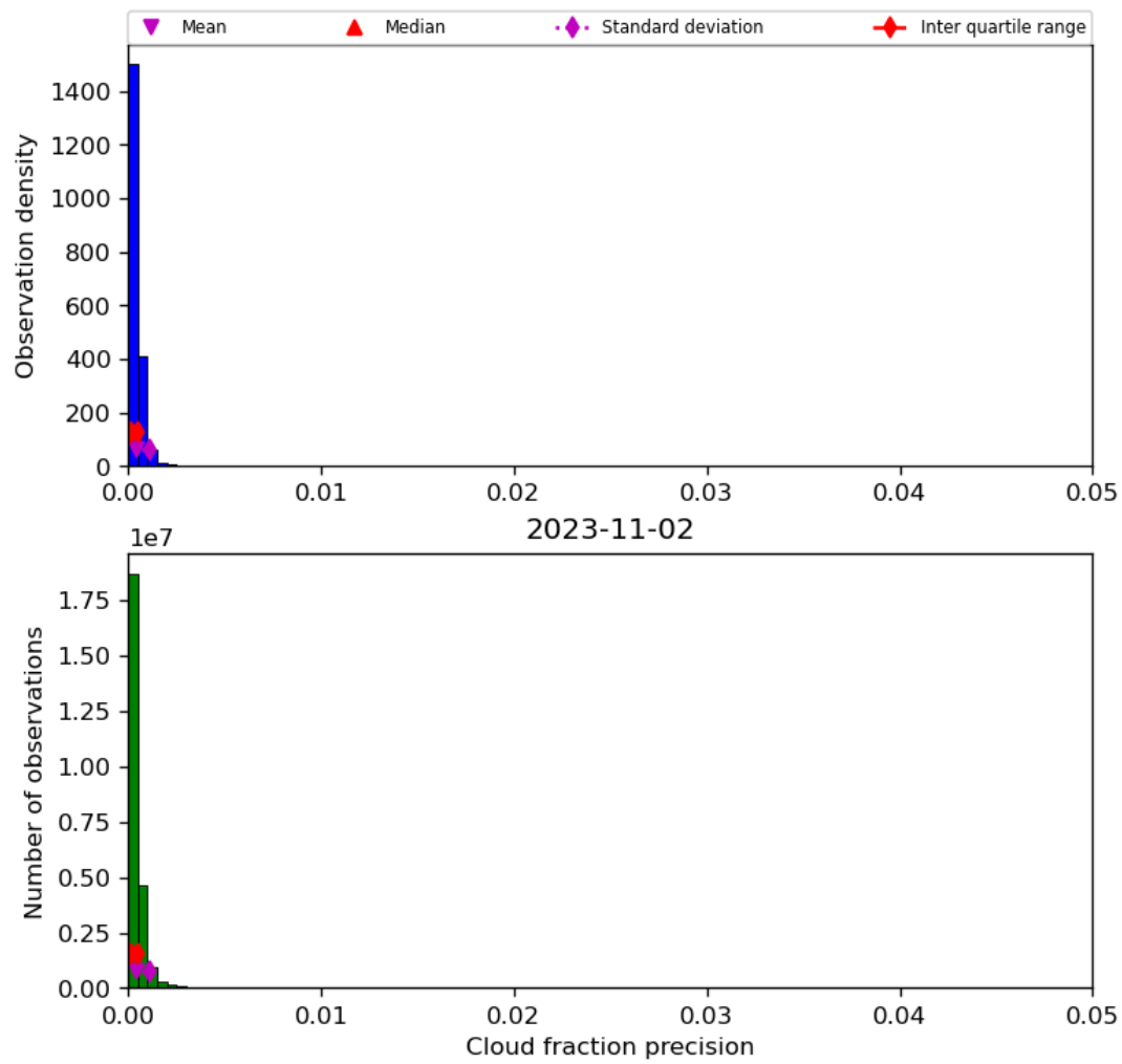
Figure 33: Histogram of “Cloud fraction precision” for 2023-11-02 to 2023-11-03
