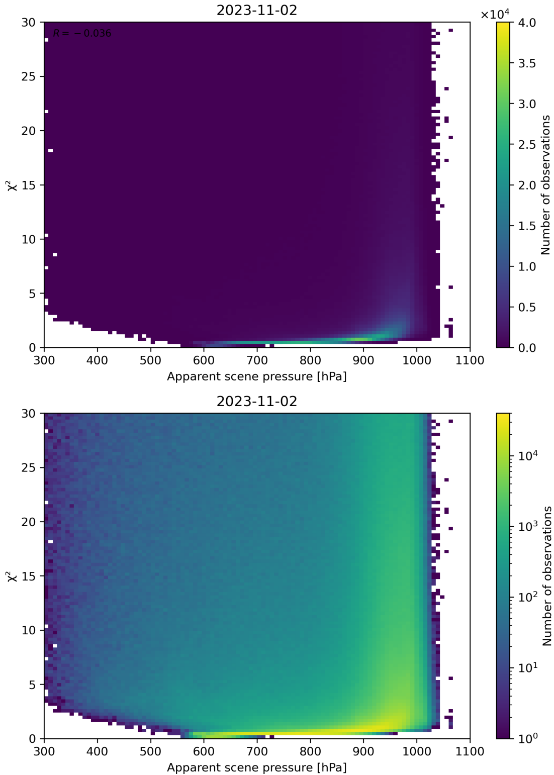
Figure 63: Scatter density plot of “Apparent scene pressure” against “ \chi^2 ” for 2023-11-02 to 2023-11-03.
