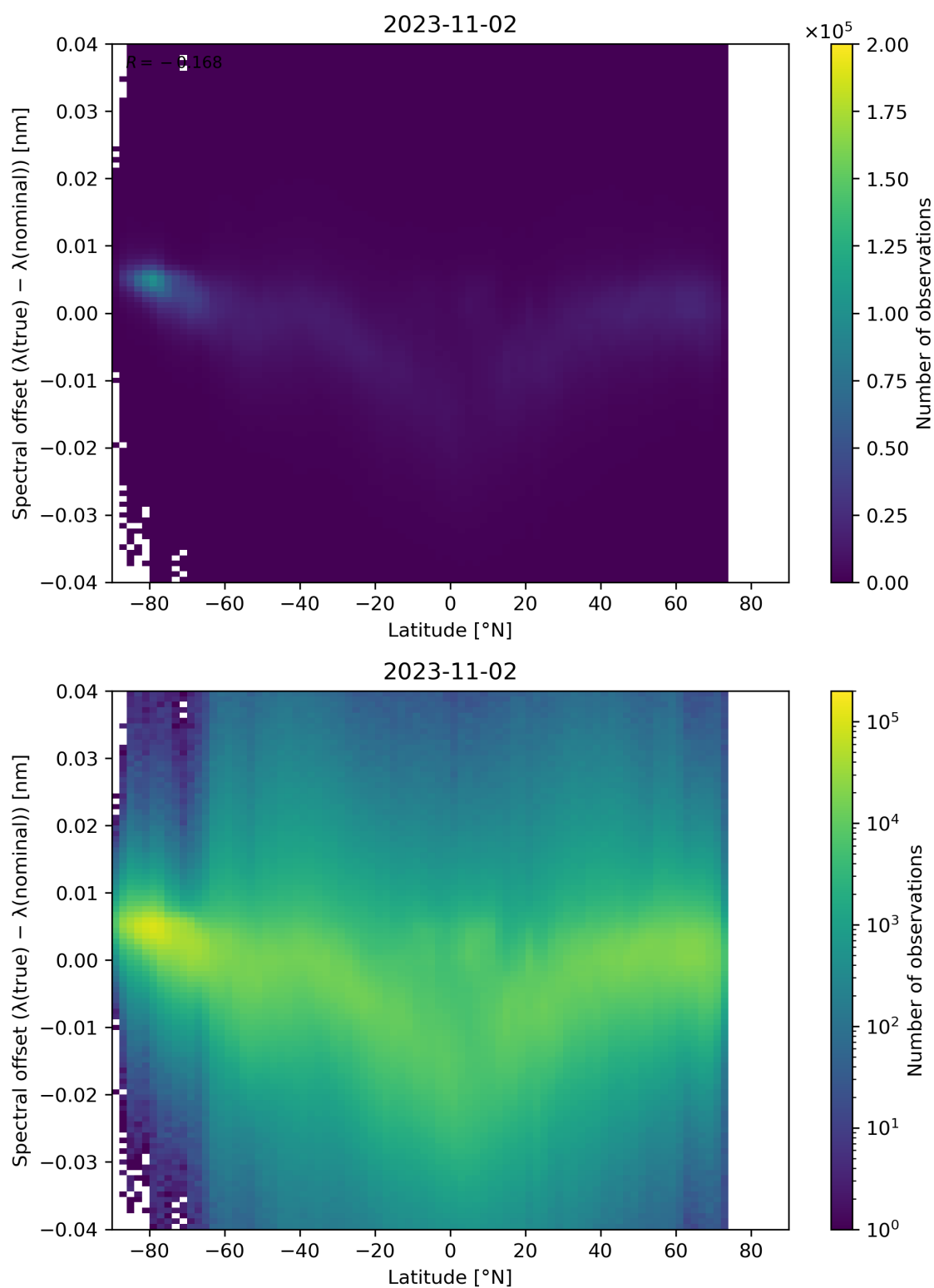
Figure 105: Scatter density plot of “Latitude” against “Spectral offset ( \lambda(\text{true}) - \lambda(\text{nominal}) )” for 2023-11-02 to 2023-11-03.
