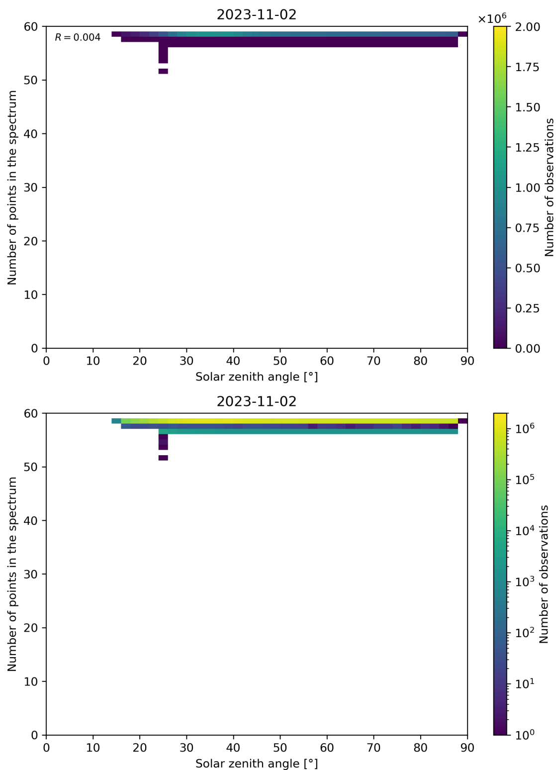
Figure 126: Scatter density plot of “Solar zenith angle” against “Number of points in the spectrum” for 2023-11-02 to 2023-11-03.
