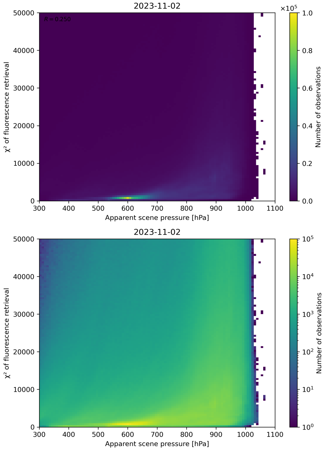
Figure 64: Scatter density plot of “Apparent scene pressure” against “ \chi^2 of fluorescence retrieval” for 2023-11-02 to 2023-11-03.
