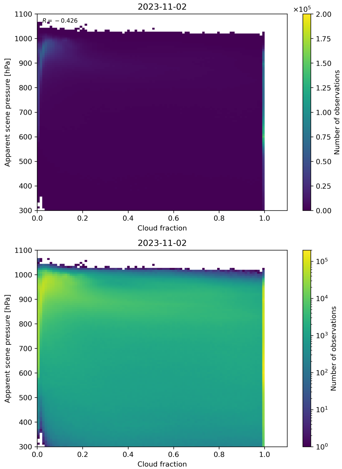
Figure 76: Scatter density plot of “Cloud fraction” against “Apparent scene pressure” for 2023-11-02 to 2023-11-03.
