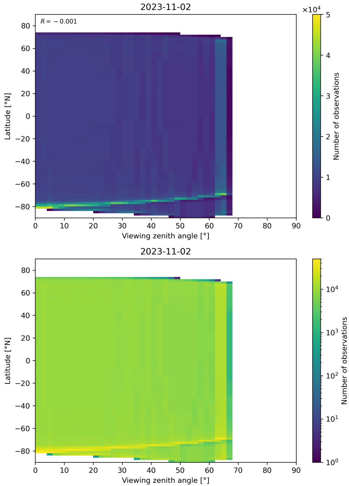
Figure 135: Scatter density plot of “Viewing zenith angle” against “Latitude” for 2023-11-02 to 2023-11-03.
