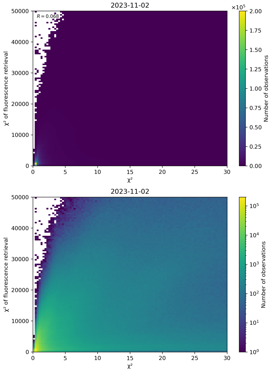
Figure 69: Scatter density plot of “ \chi^2 ” against “ \chi^2 of fluorescence retrieval” for 2023-11-02 to 2023-11-03.
