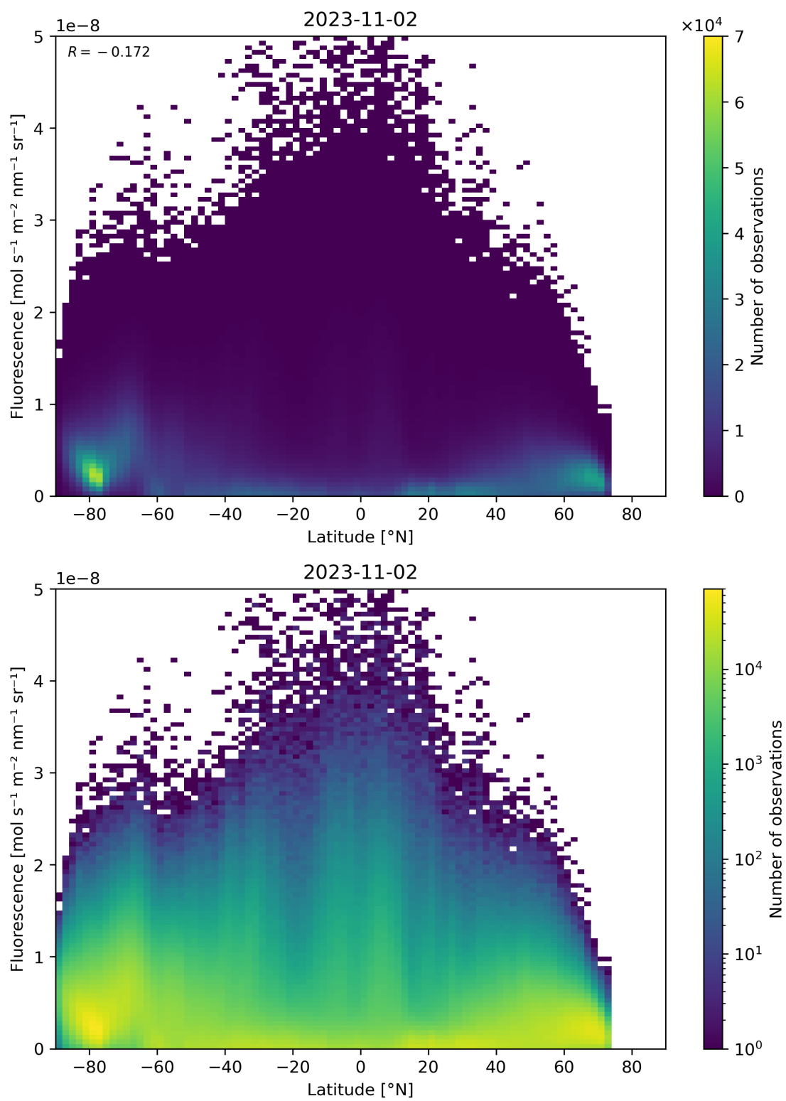
Figure 101: Scatter density plot of “Latitude” against “Fluorescence” for 2023-11-02 to 2023-11-03.
