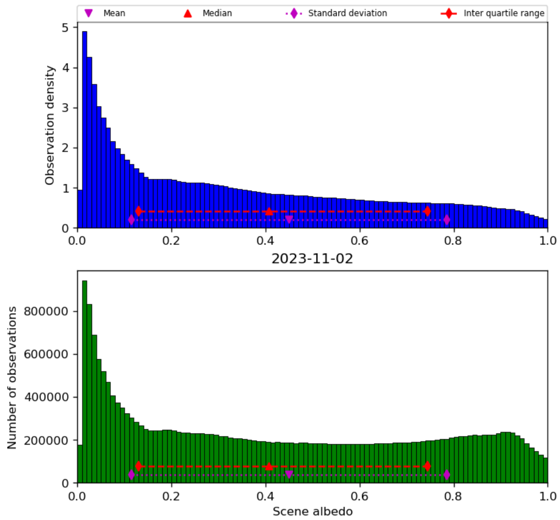
Figure 34: Histogram of “Scene albedo” for 2023-11-02 to 2023-11-03
