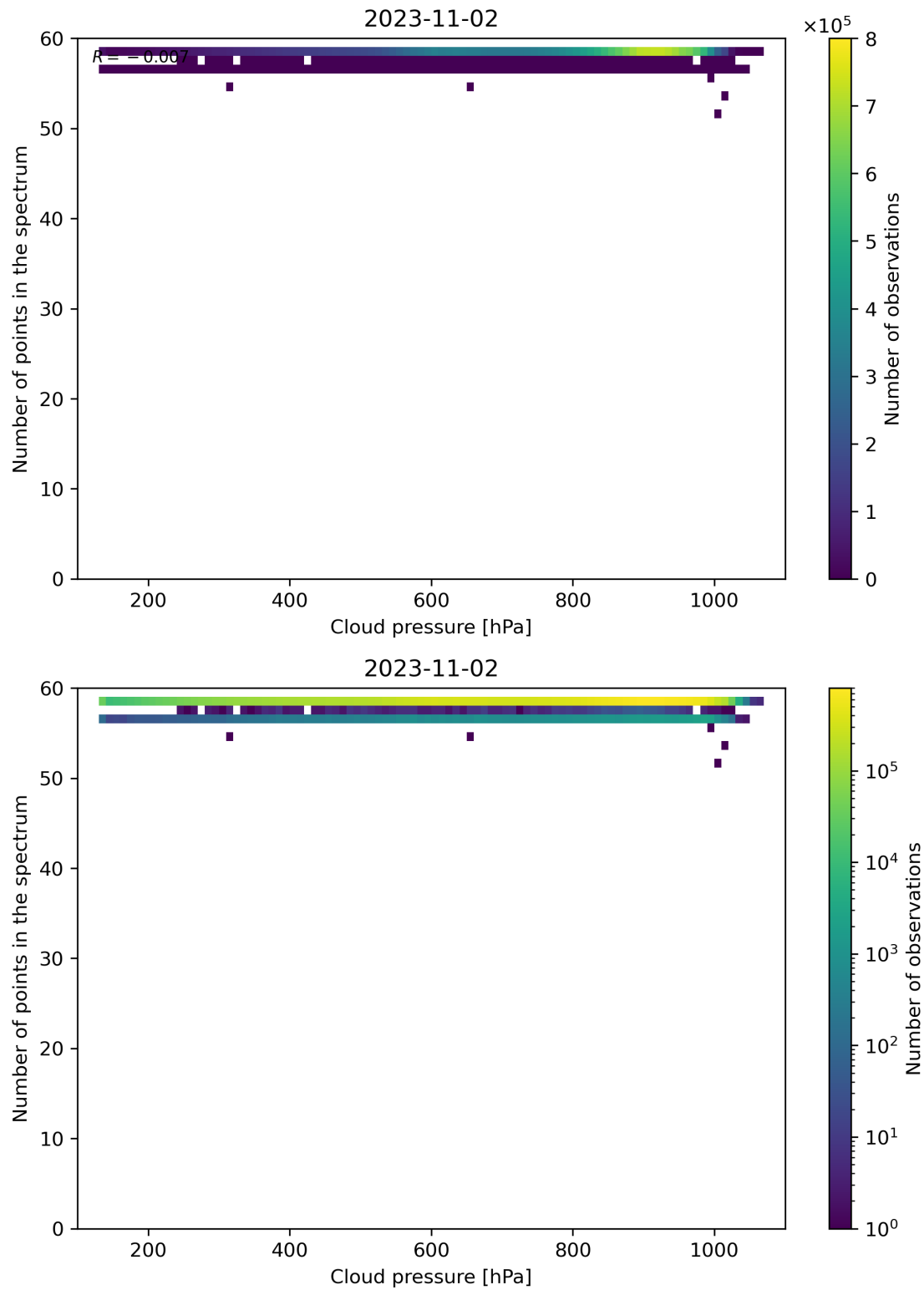
Figure 90: Scatter density plot of “Cloud pressure” against “Number of points in the spectrum” for 2023-11-02 to 2023-11-03.
