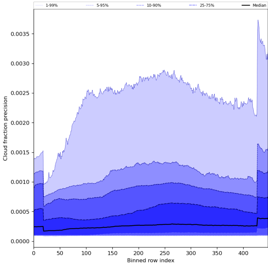
Figure 50: Along track statistics of “Cloud fraction precision” for 2023-11-02 to 2023-11-03
