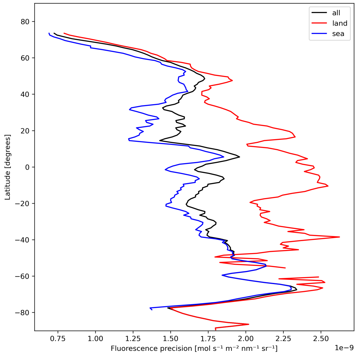
Figure 24: Zonal average of “Fluorescence precision” for 2023-11-02 to 2023-11-03.
