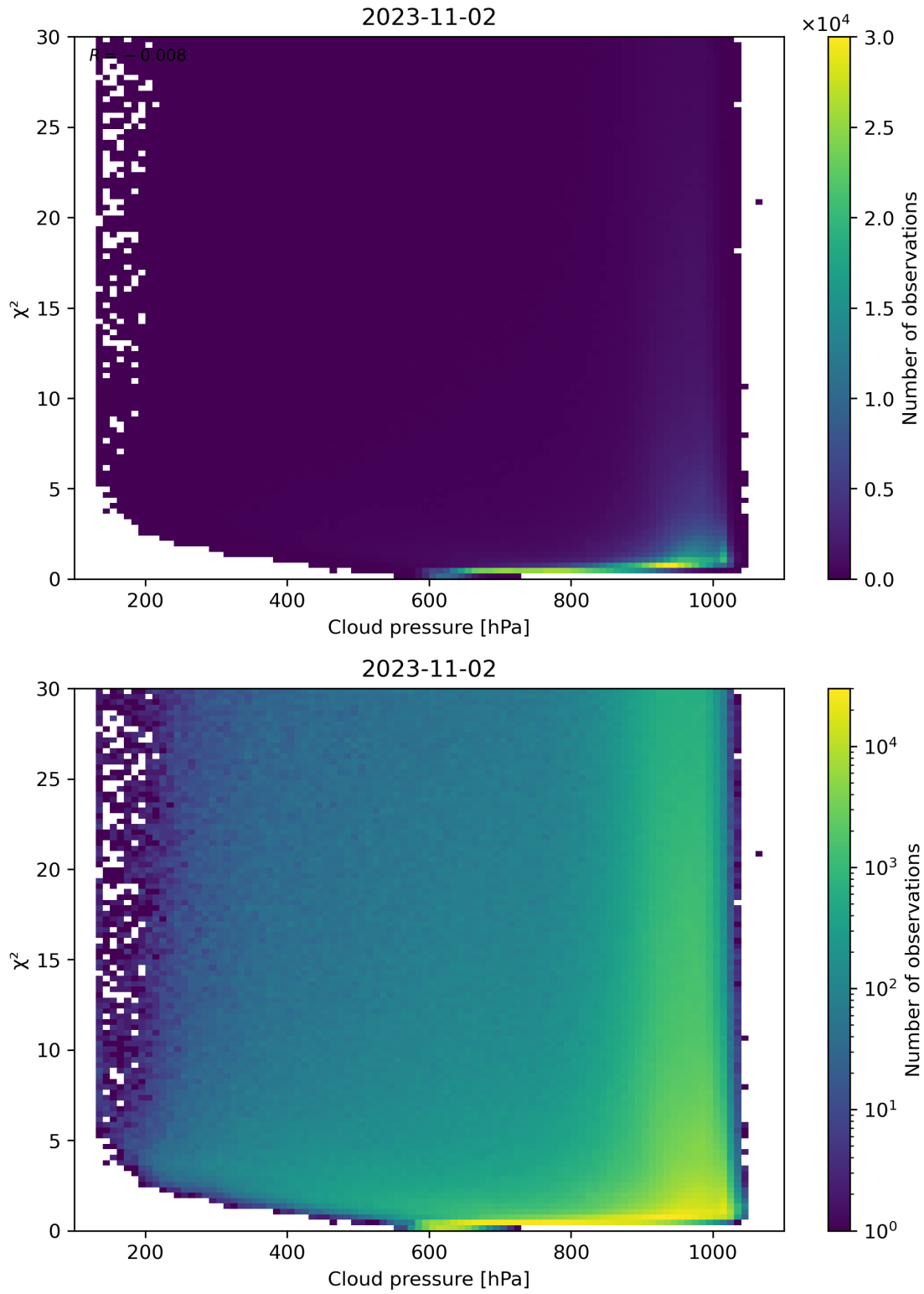
Figure 85: Scatter density plot of “Cloud pressure” against “ \chi^2 ” for 2023-11-02 to 2023-11-03.
