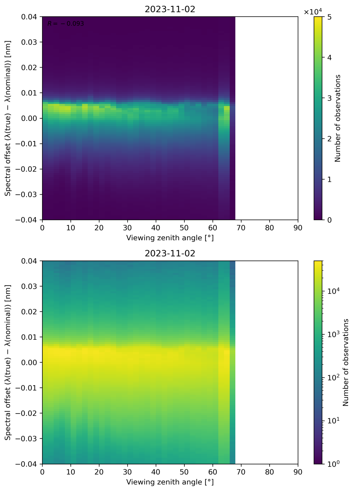
Figure 140: Scatter density plot of “Viewing zenith angle” against “Spectral offset ( \lambda(\text{true}) - \lambda(\text{nominal}) )” for 2023-11-02 to 2023-11-03.
