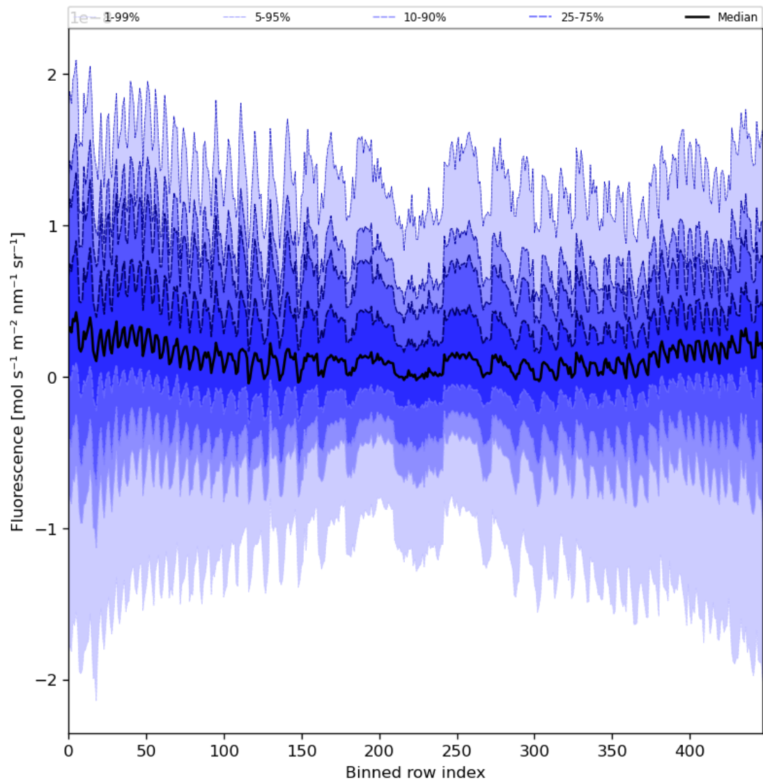
Figure 57: Along track statistics of “Fluorescence” for 2023-11-02 to 2023-11-03
