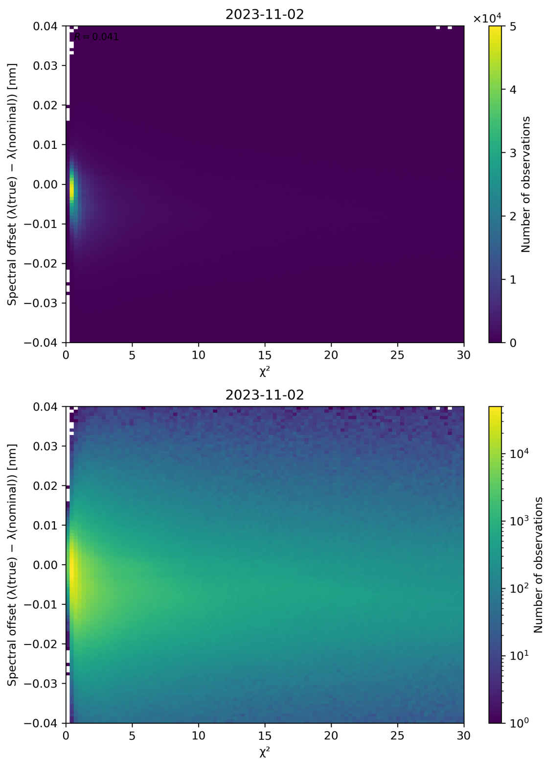
Figure 75: Scatter density plot of “ \chi^2 ” against “Spectral offset ( \lambda(\text{true}) - \lambda(\text{nominal}) )” for 2023-11-02 to 2023-11-03.
