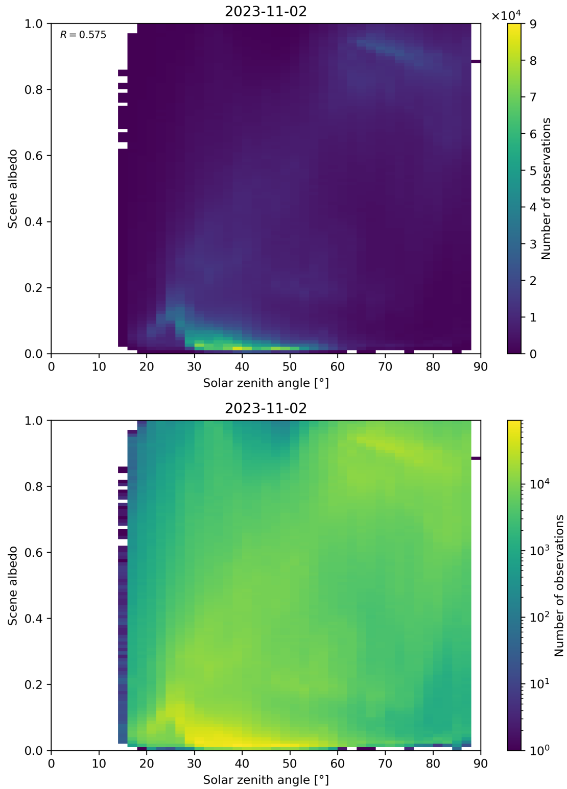
Figure 127: Scatter density plot of “Solar zenith angle” against “Scene albedo” for 2023-11-02 to 2023-11-03.
