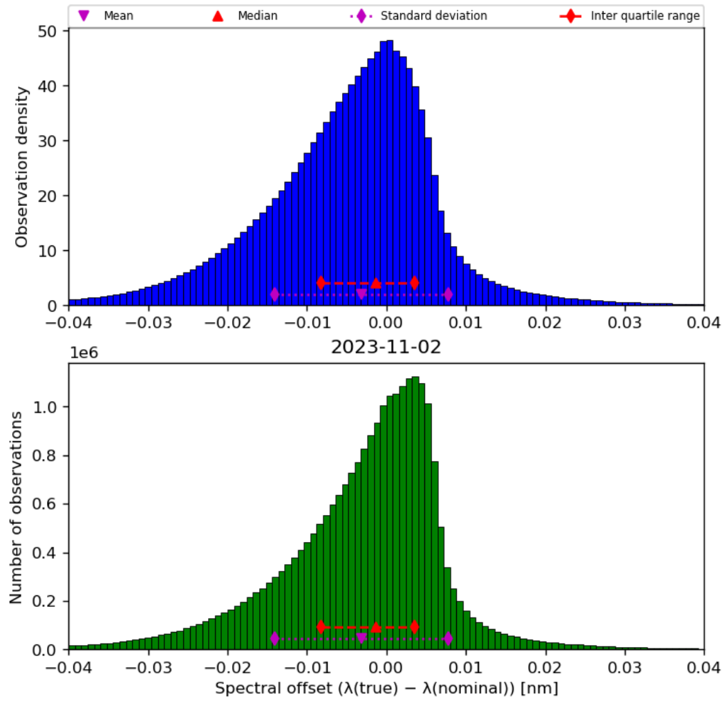
Figure 45: Histogram of “Spectral offset ( \lambda(\text{true}) - \lambda(\text{nominal}) )” for 2023-11-02 to 2023-11-03
