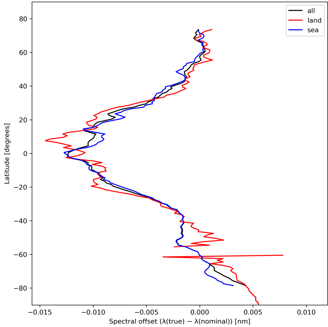
Figure 28: Zonal average of “Spectral offset ( \lambda(\text{true}) - \lambda(\text{nominal}) )” for 2023-11-02 to 2023-11-03.
