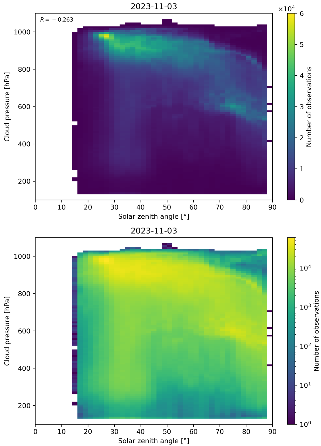
Figure 122: Scatter density plot of “Solar zenith angle” against “Cloud pressure” for 2023-11-02 to 2023-11-04.
