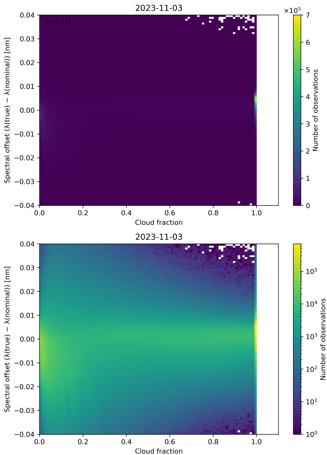
Figure 83: Scatter density plot of “Cloud fraction” against “Spectral offset ( \lambda(\text{true}) - \lambda(\text{nominal}) )” for 2023-11-02 to 2023-11-04.
