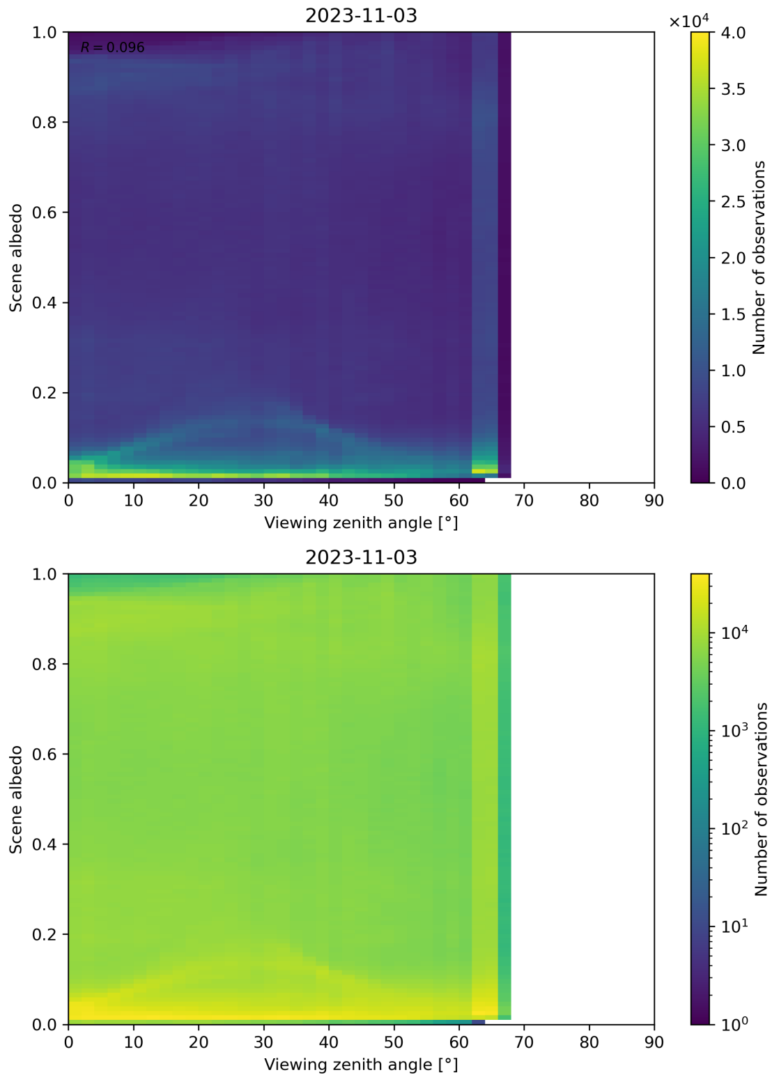
Figure 138: Scatter density plot of “Viewing zenith angle” against “Scene albedo” for 2023-11-02 to 2023-11-04.
