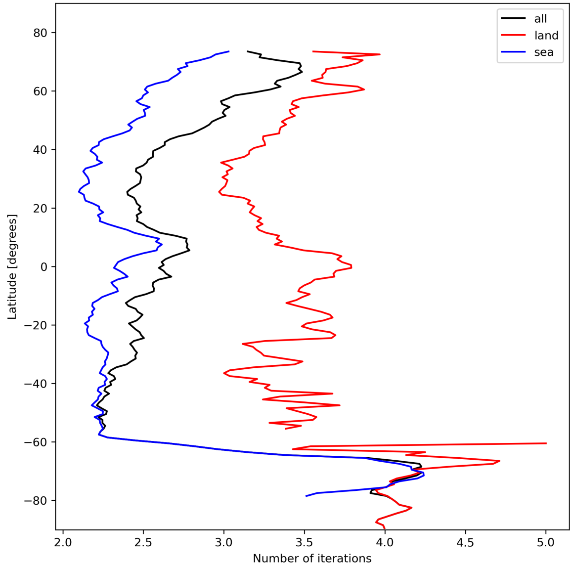
Figure 22: Zonal average of “Number of iterations” for 2023-11-02 to 2023-11-04.
