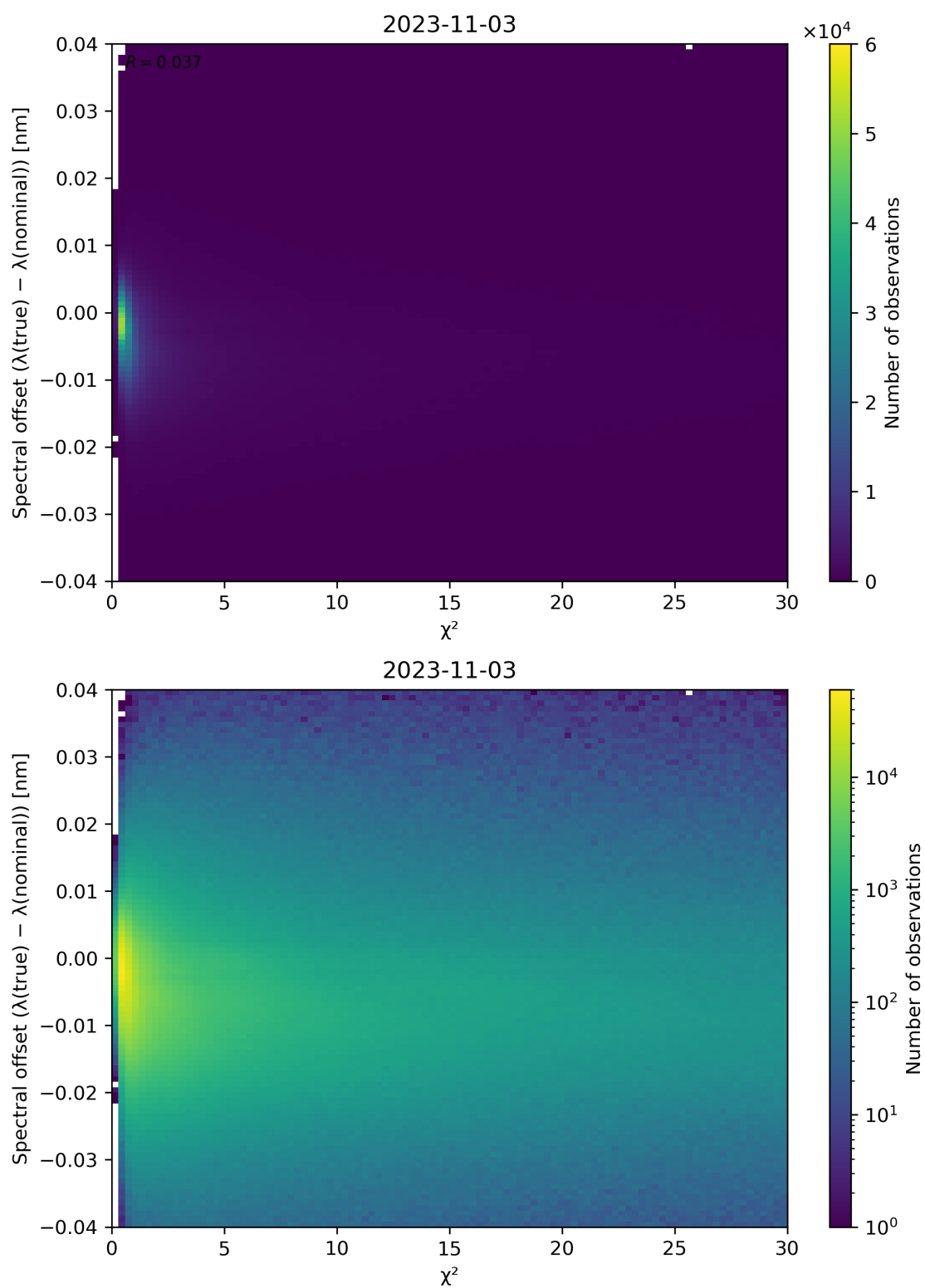
Figure 75: Scatter density plot of “ \chi^2 ” against “Spectral offset ( \lambda(\text{true}) - \lambda(\text{nominal}) )” for 2023-11-02 to 2023-11-04.
