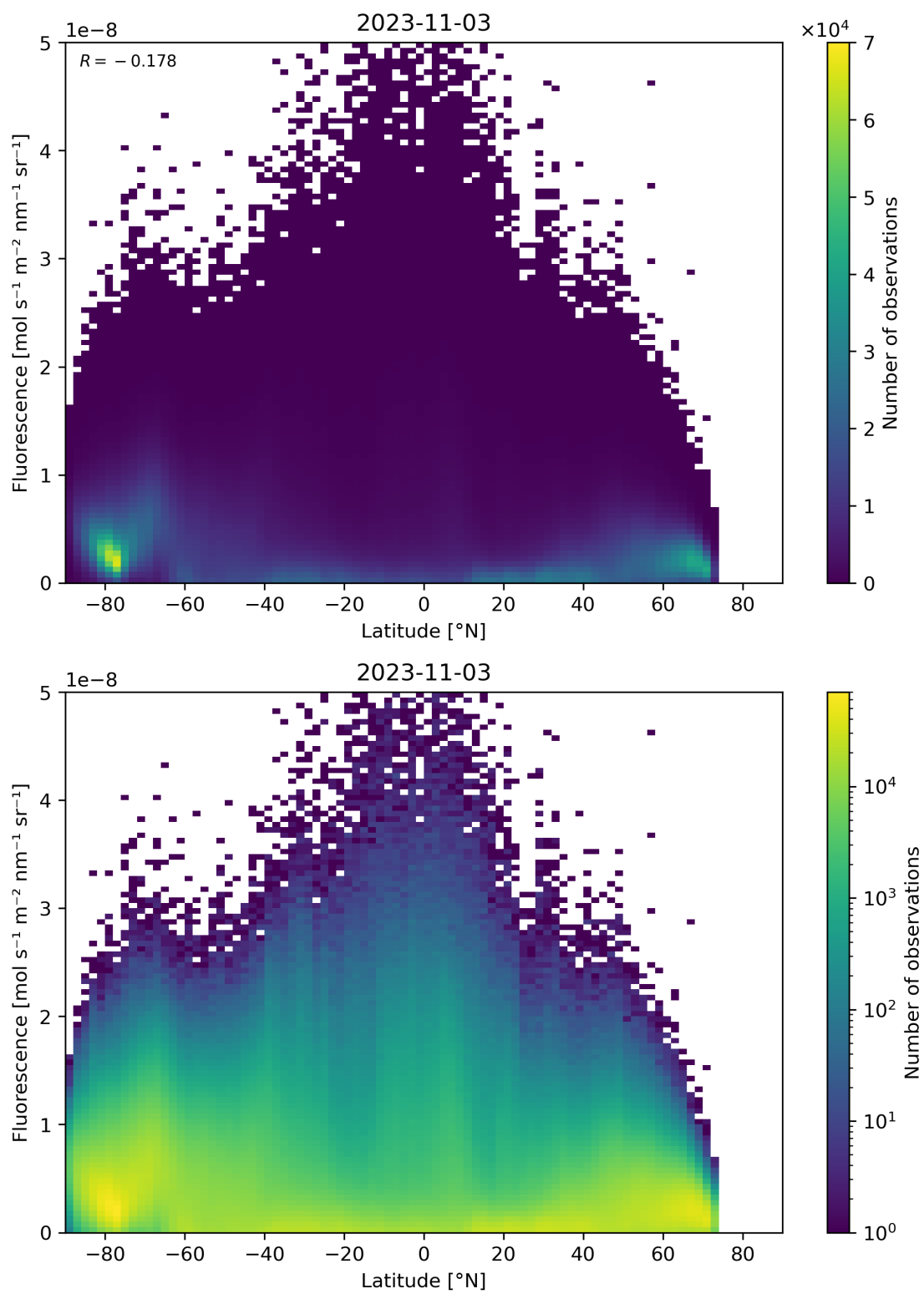
Figure 101: Scatter density plot of “Latitude” against “Fluorescence” for 2023-11-02 to 2023-11-04.
