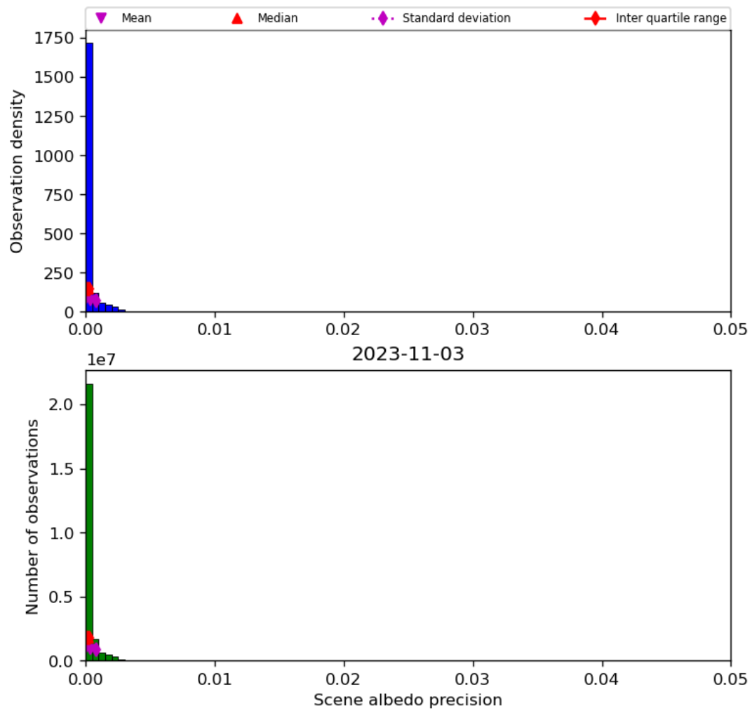
Figure 35: Histogram of “Scene albedo precision” for 2023-11-02 to 2023-11-04
