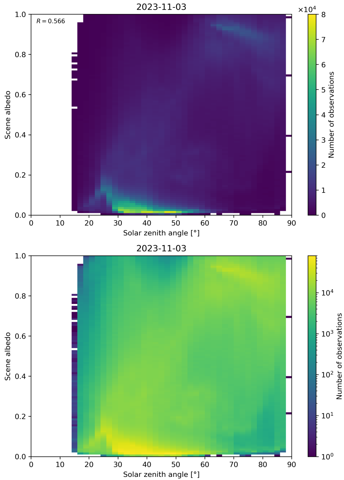
Figure 127: Scatter density plot of “Solar zenith angle” against “Scene albedo” for 2023-11-02 to 2023-11-04.
