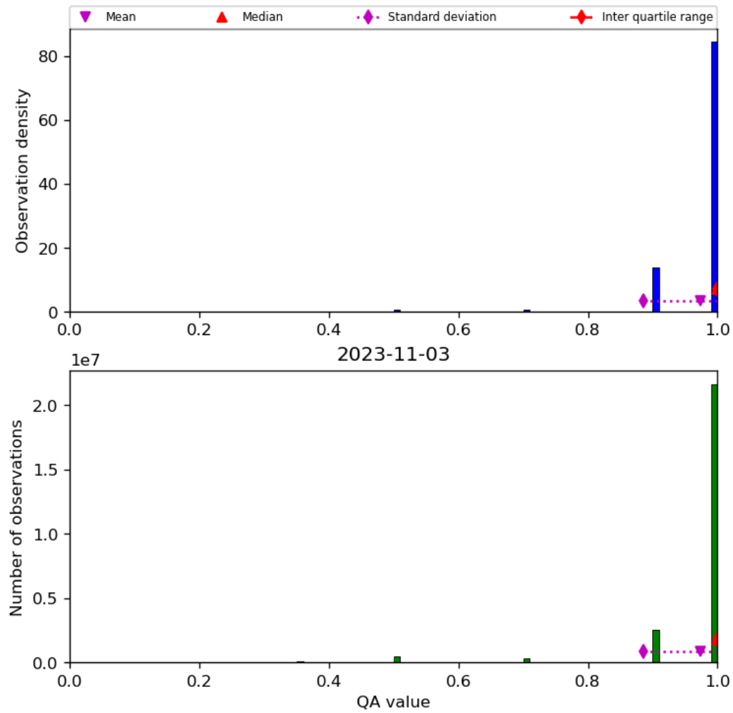
Figure 29: Histogram of “QA value” for 2023-11-02 to 2023-11-04
