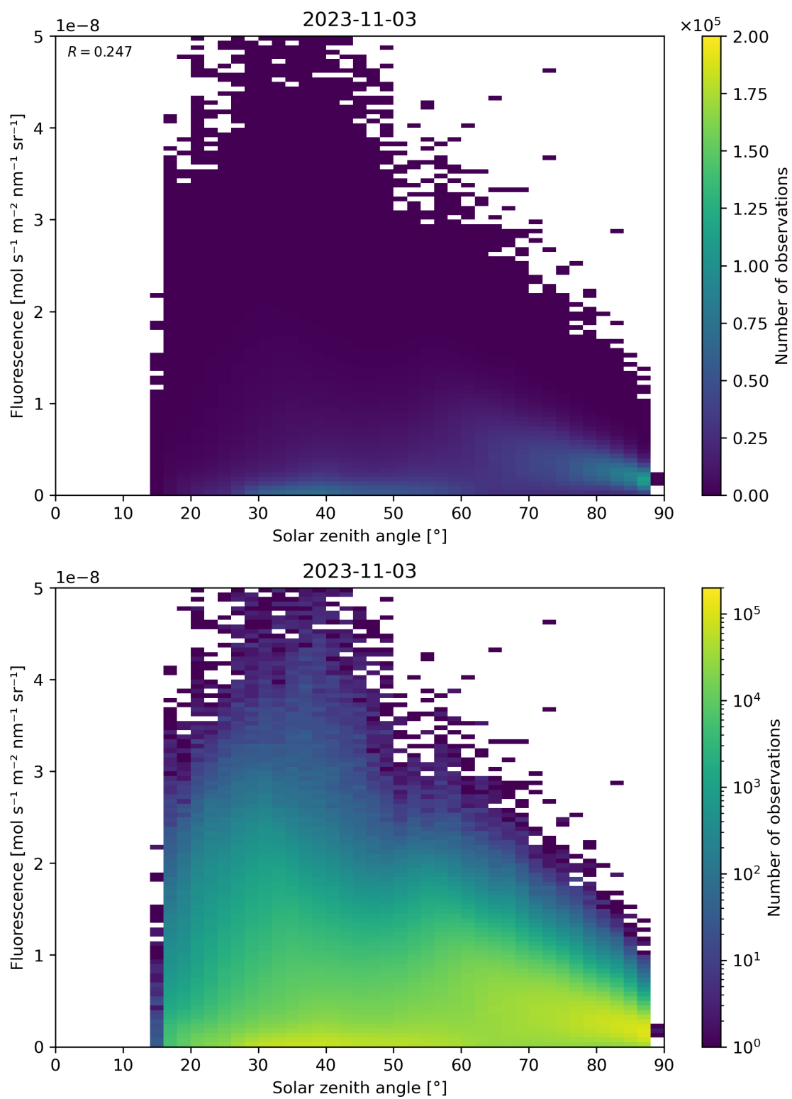
Figure 123: Scatter density plot of “Solar zenith angle” against “Fluorescence” for 2023-11-02 to 2023-11-04.
