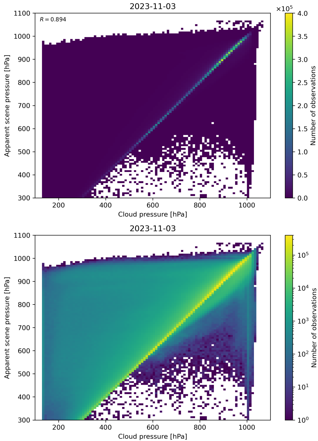
Figure 84: Scatter density plot of “Cloud pressure” against “Apparent scene pressure” for 2023-11-02 to 2023-11-04.
