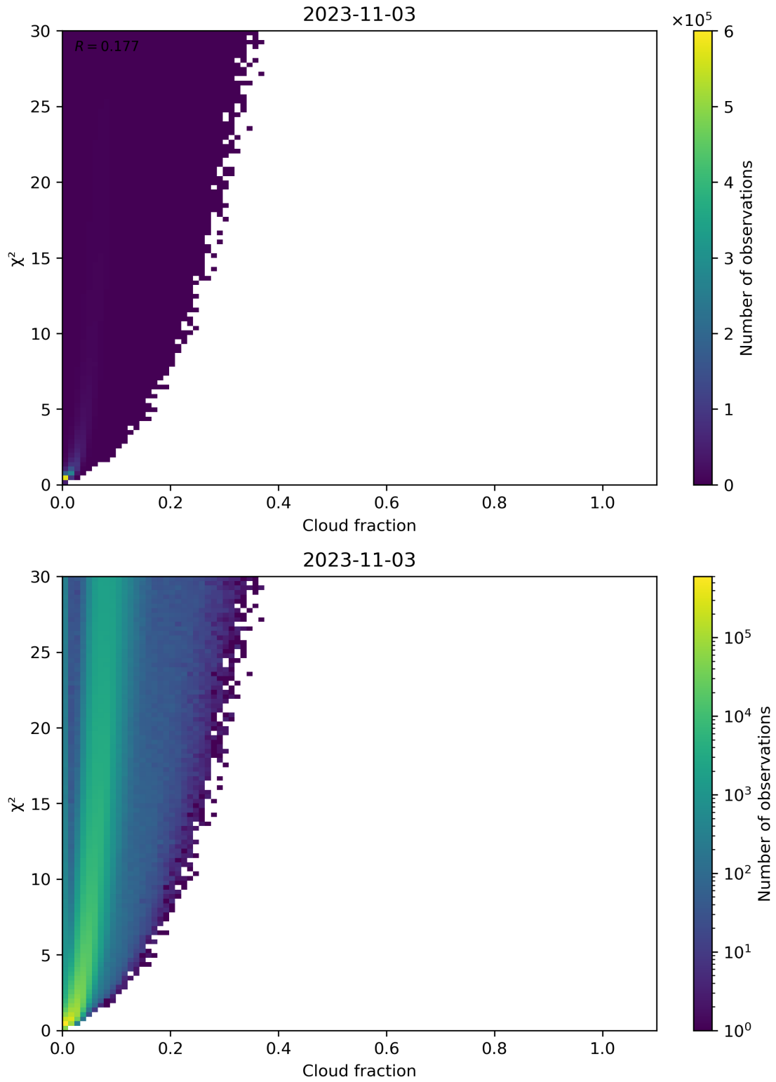
Figure 77: Scatter density plot of “Cloud fraction” against “ \chi^2 ” for 2023-11-02 to 2023-11-04.
