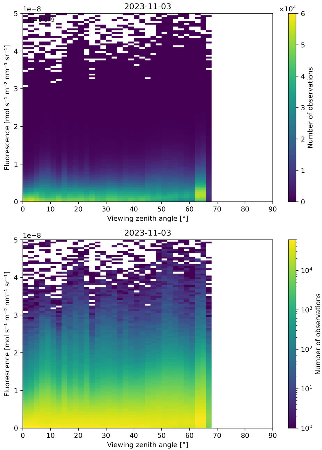
Figure 134: Scatter density plot of “Viewing zenith angle” against “Fluorescence” for 2023-11-02 to 2023-11-04.
