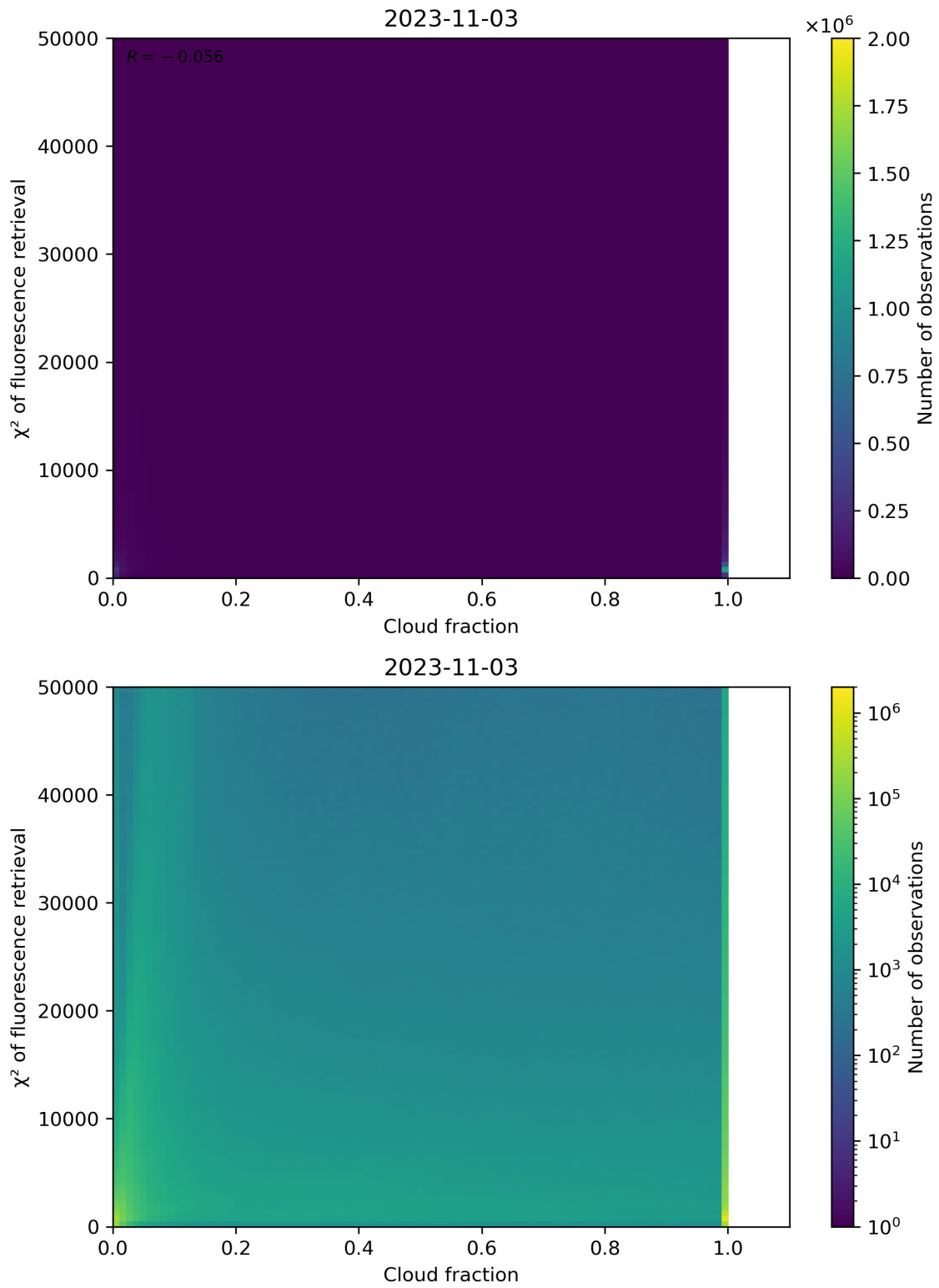
Figure 78: Scatter density plot of “Cloud fraction” against “ \chi^2 of fluorescence retrieval” for 2023-11-02 to 2023-11-04.
