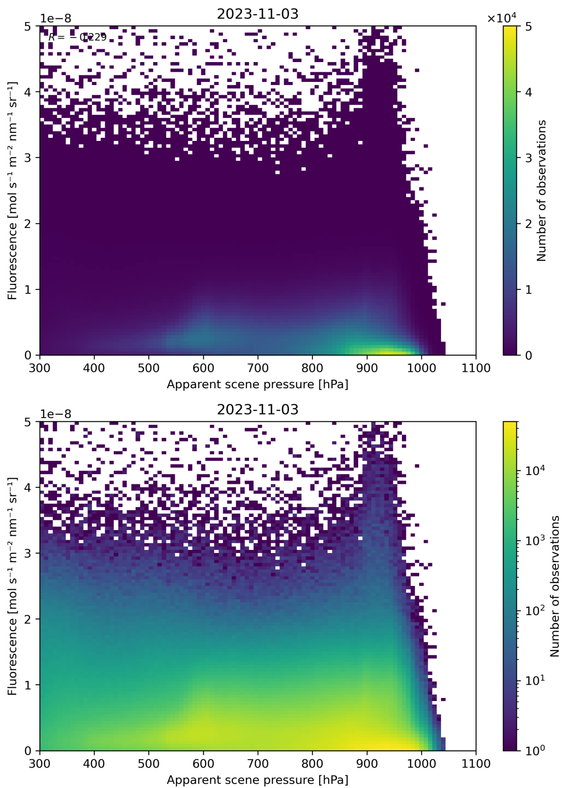
Figure 65: Scatter density plot of “Apparent scene pressure” against “Fluorescence” for 2023-11-02 to 2023-11-04.
