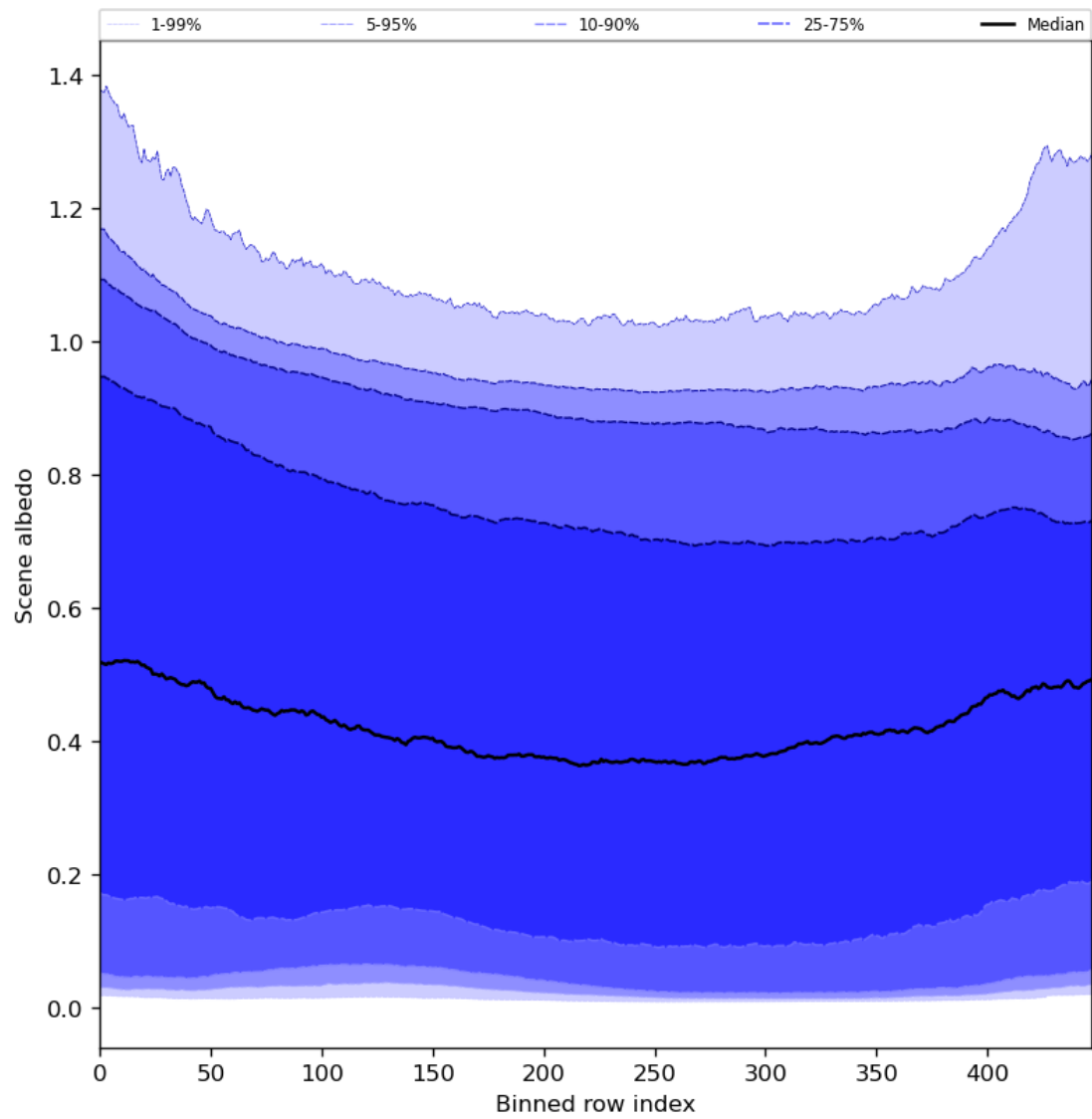
Figure 51: Along track statistics of “Scene albedo” for 2023-11-02 to 2023-11-04
