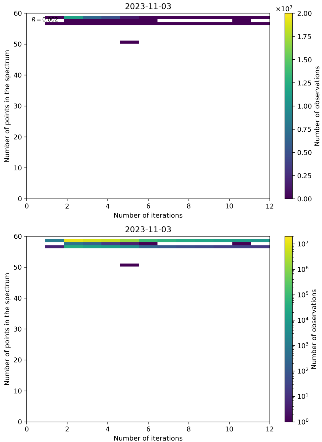
Figure 108: Scatter density plot of “Number of iterations” against “Number of points in the spectrum” for 2023-11-02 to 2023-11-04.
