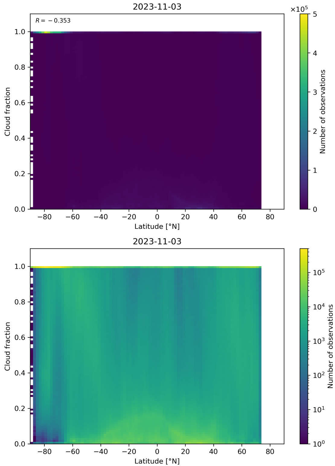
Figure 99: Scatter density plot of “Latitude” against “Cloud fraction” for 2023-11-02 to 2023-11-04.
