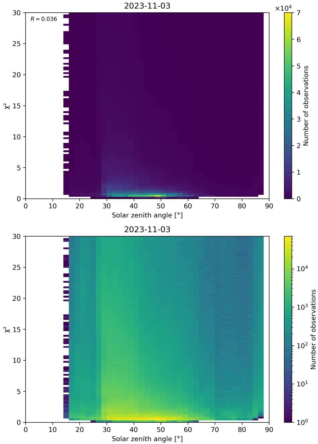
Figure 119: Scatter density plot of “Solar zenith angle” against “ \chi^2 ” for 2023-11-02 to 2023-11-04.
