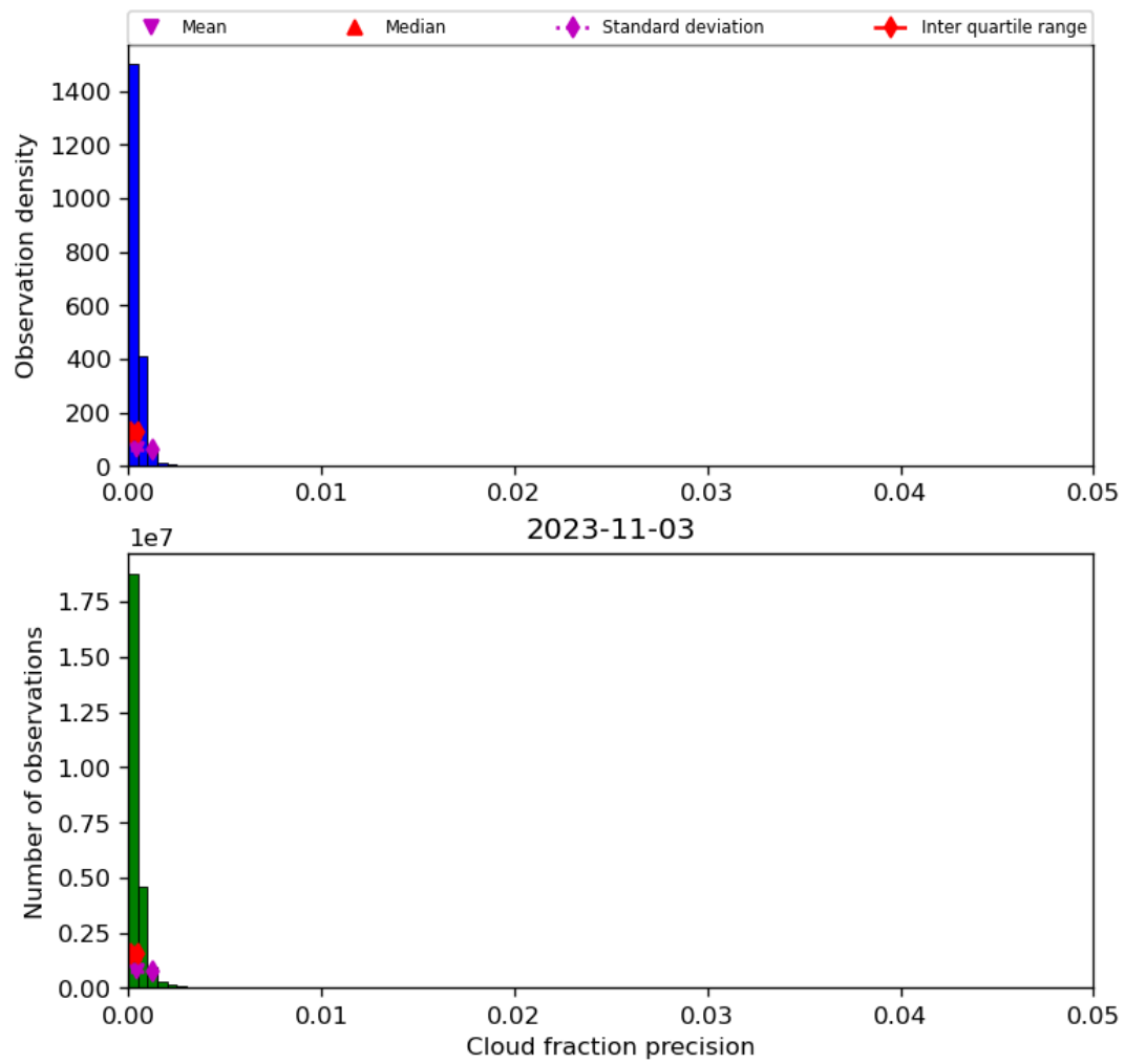
Figure 33: Histogram of “Cloud fraction precision” for 2023-11-02 to 2023-11-04
