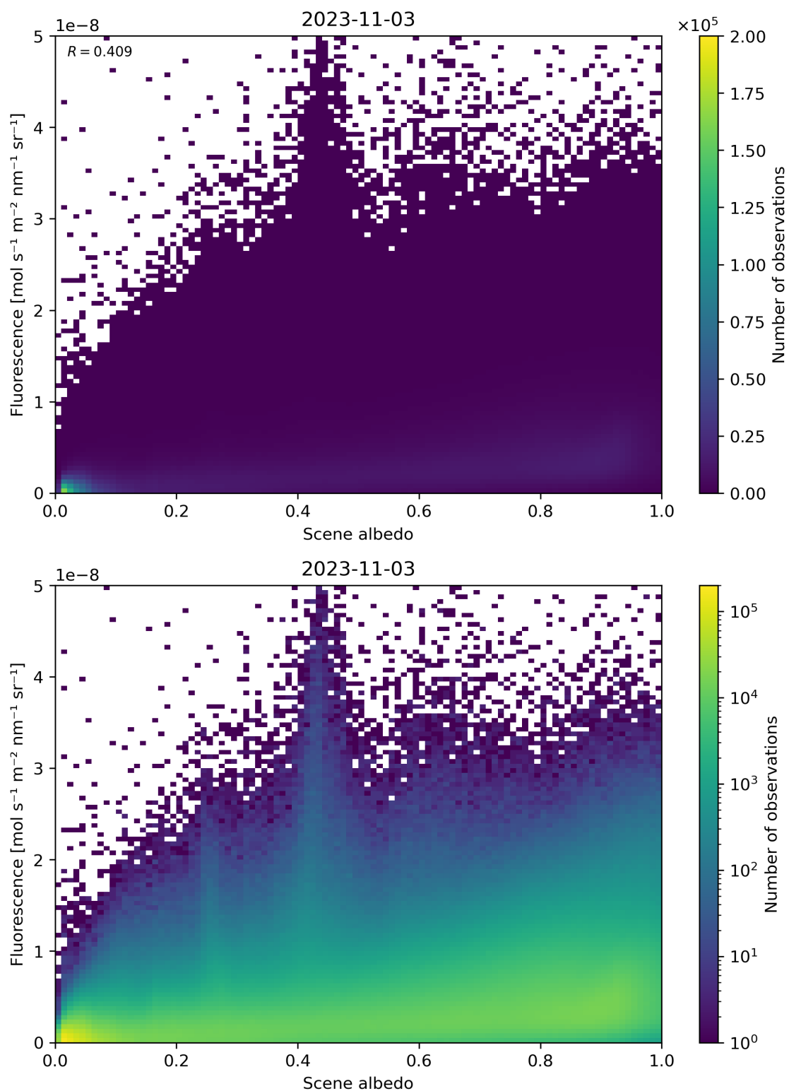
Figure 114: Scatter density plot of “Scene albedo” against “Fluorescence” for 2023-11-02 to 2023-11-04.
