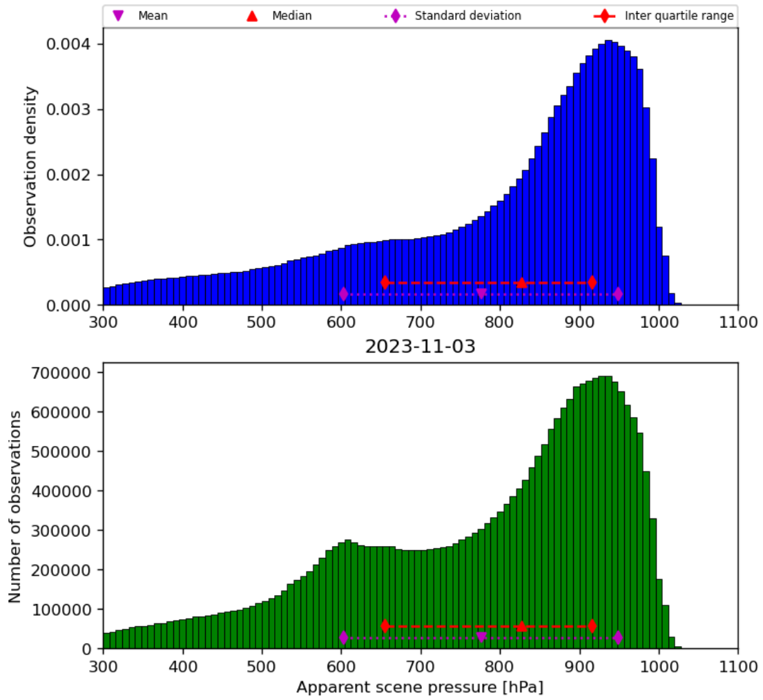
Figure 36: Histogram of “Apparent scene pressure” for 2023-11-02 to 2023-11-04
