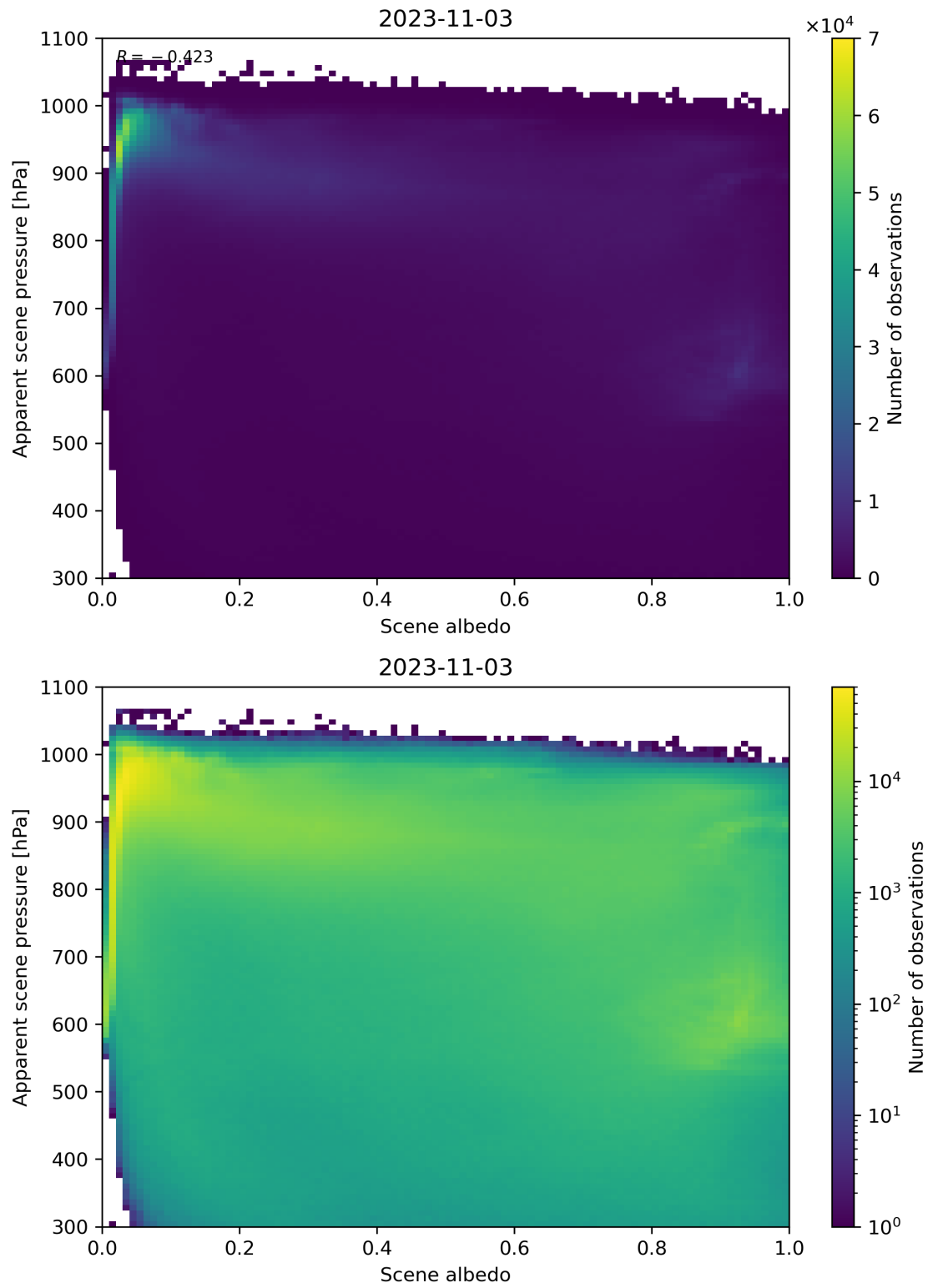
Figure 111: Scatter density plot of “Scene albedo” against “Apparent scene pressure” for 2023-11-02 to 2023-11-04.
