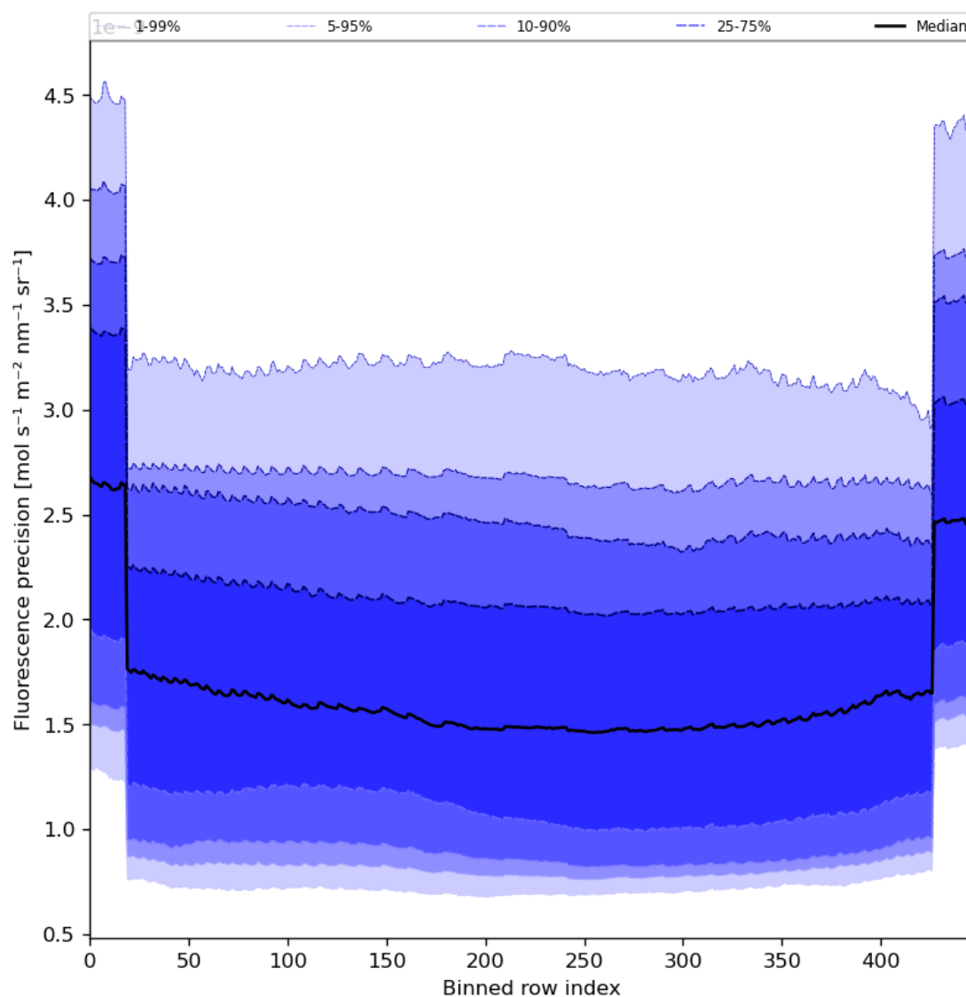
Figure 58: Along track statistics of “Fluorescence precision” for 2023-11-02 to 2023-11-04
