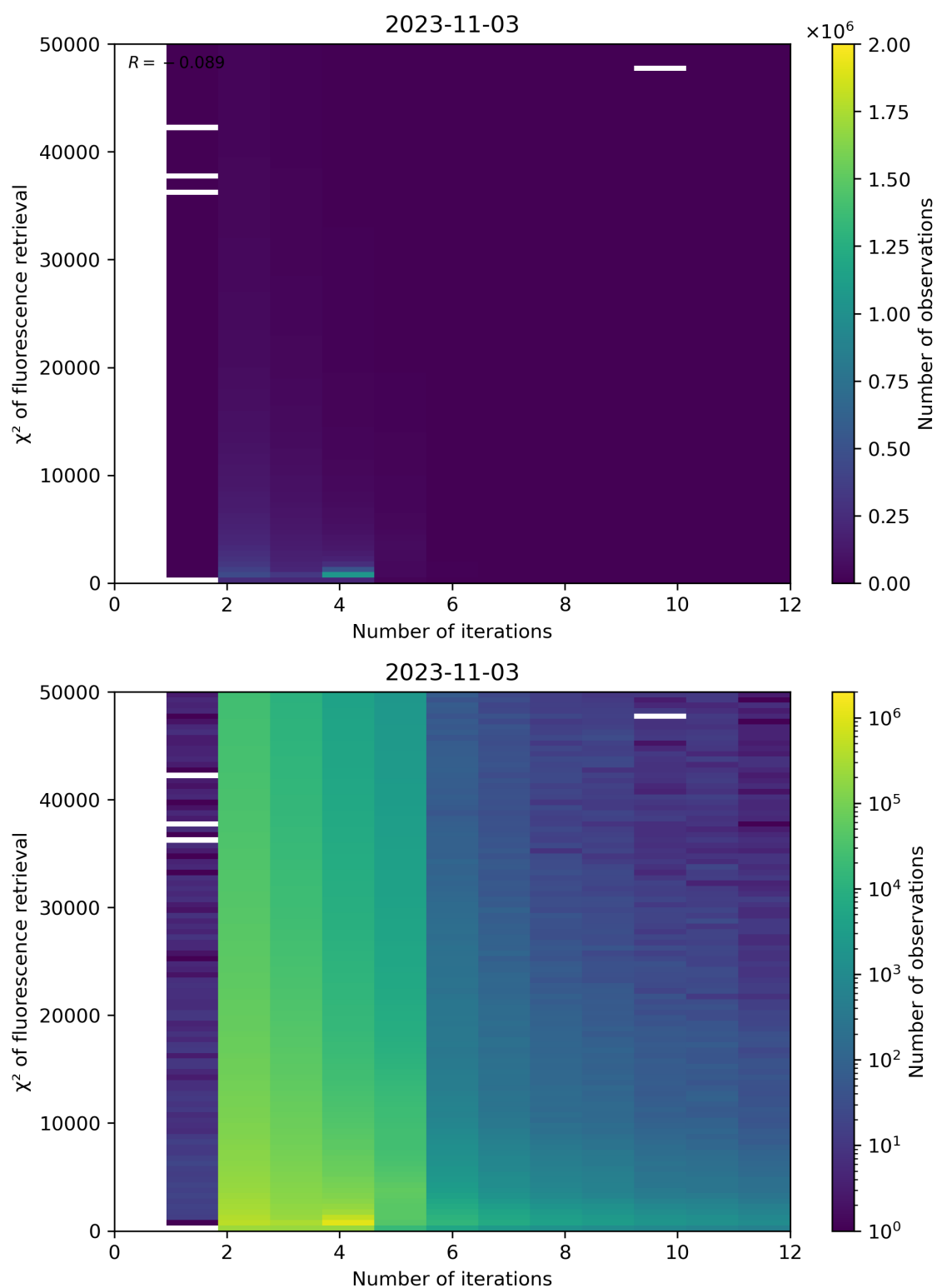
Figure 106: Scatter density plot of “Number of iterations” against “ \chi^2 of fluorescence retrieval” for 2023-11-02 to 2023-11-04.
