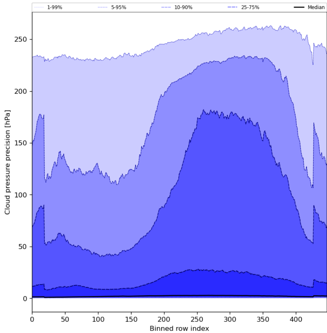
Figure 48: Along track statistics of “Cloud pressure precision” for 2023-11-02 to 2023-11-04
