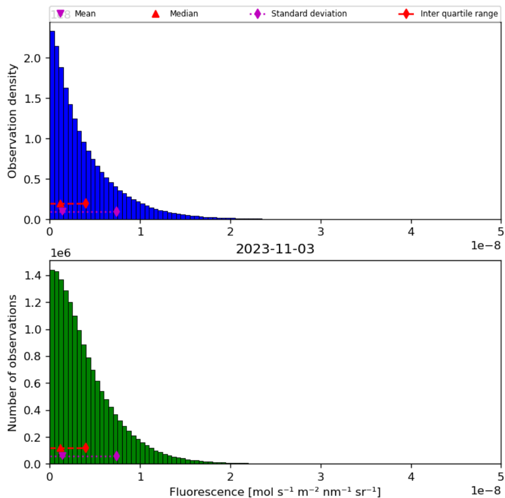
Figure 40: Histogram of “Fluorescence” for 2023-11-02 to 2023-11-04
