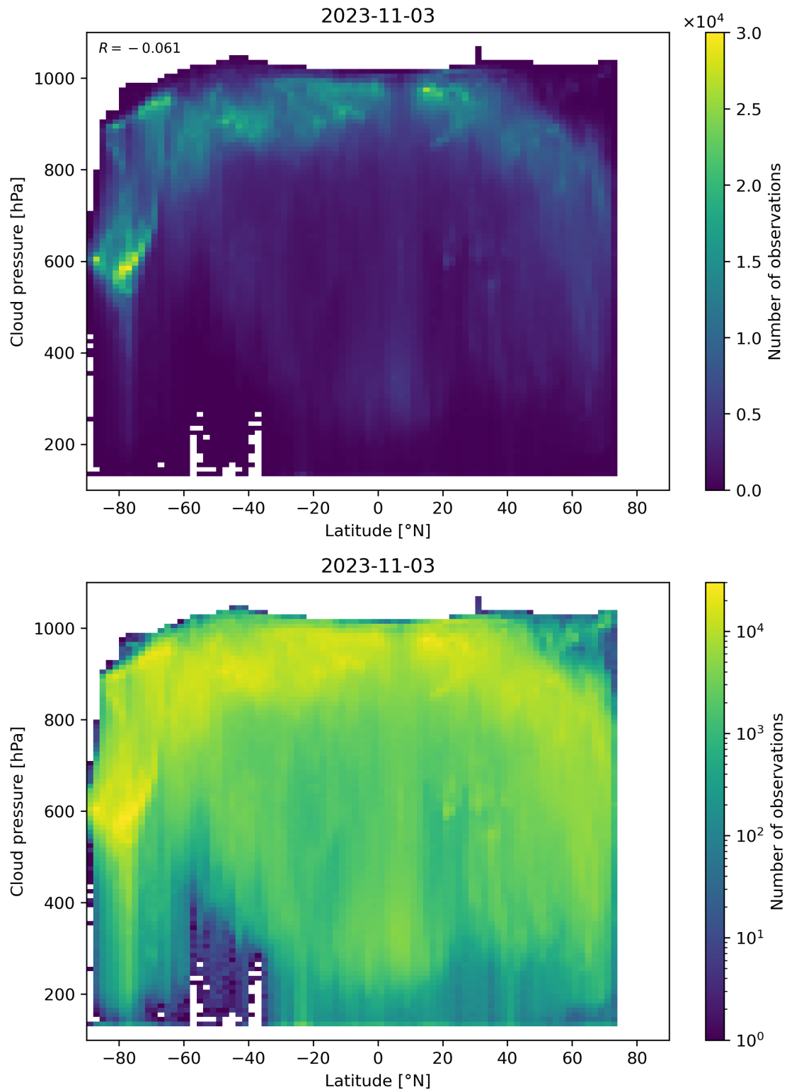
Figure 100: Scatter density plot of “Latitude” against “Cloud pressure” for 2023-11-02 to 2023-11-04.
