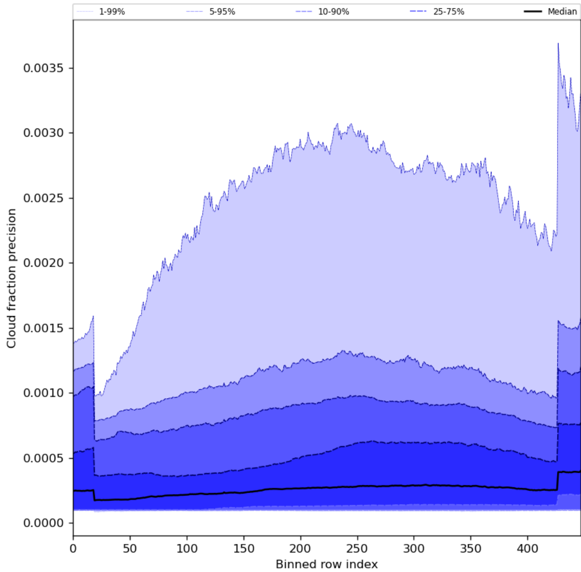
Figure 50: Along track statistics of “Cloud fraction precision” for 2023-11-02 to 2023-11-04
