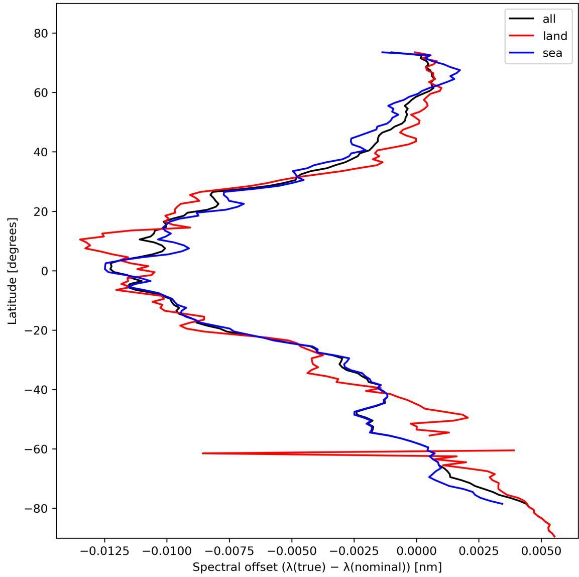
Figure 28: Zonal average of “Spectral offset ( \lambda(\text{true}) - \lambda(\text{nominal}) )” for 2023-11-02 to 2023-11-04.
