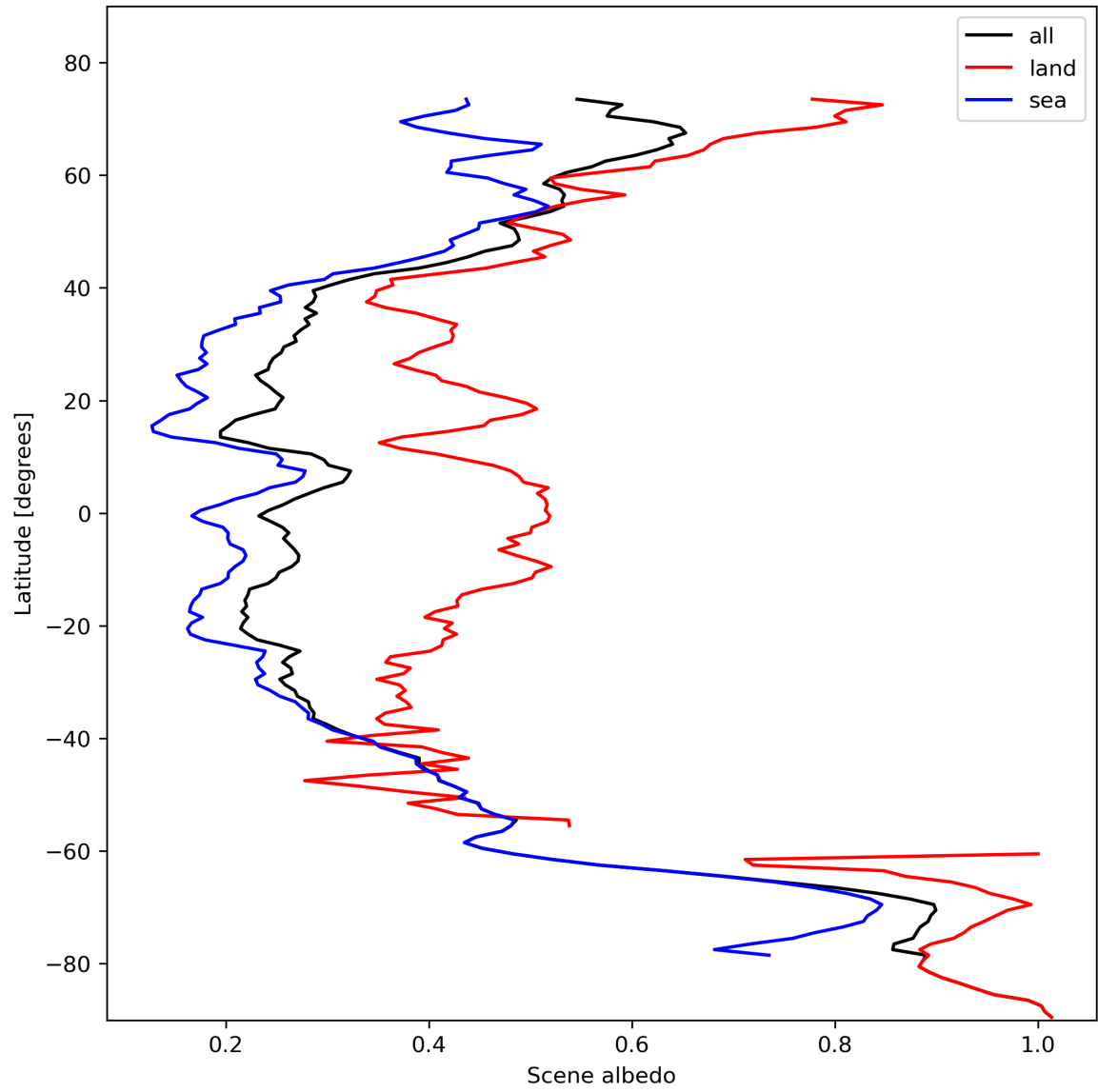
Figure 17: Zonal average of “Scene albedo” for 2023-11-02 to 2023-11-04.
