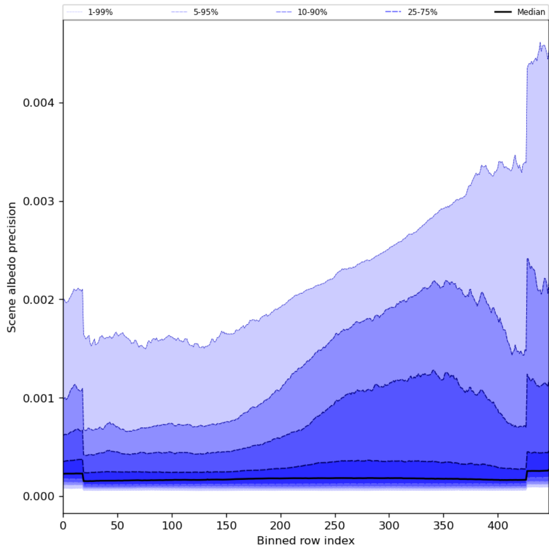
Figure 52: Along track statistics of “Scene albedo precision” for 2023-11-02 to 2023-11-04
