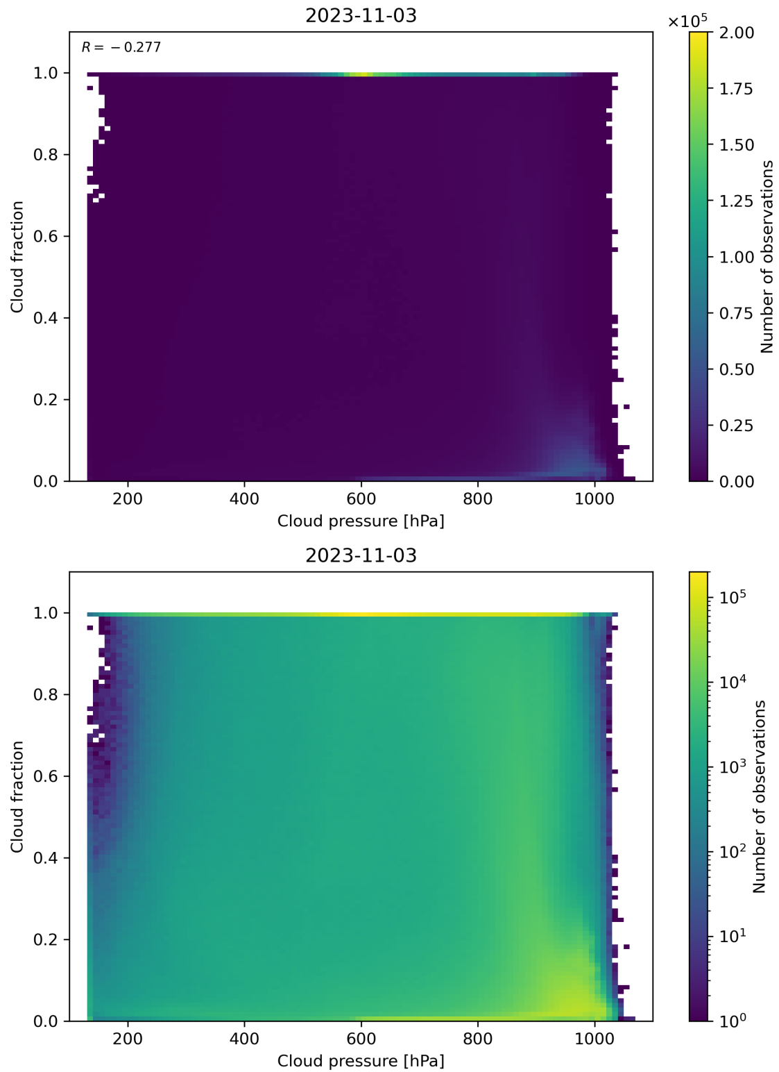
Figure 87: Scatter density plot of “Cloud pressure” against “Cloud fraction” for 2023-11-02 to 2023-11-04.
