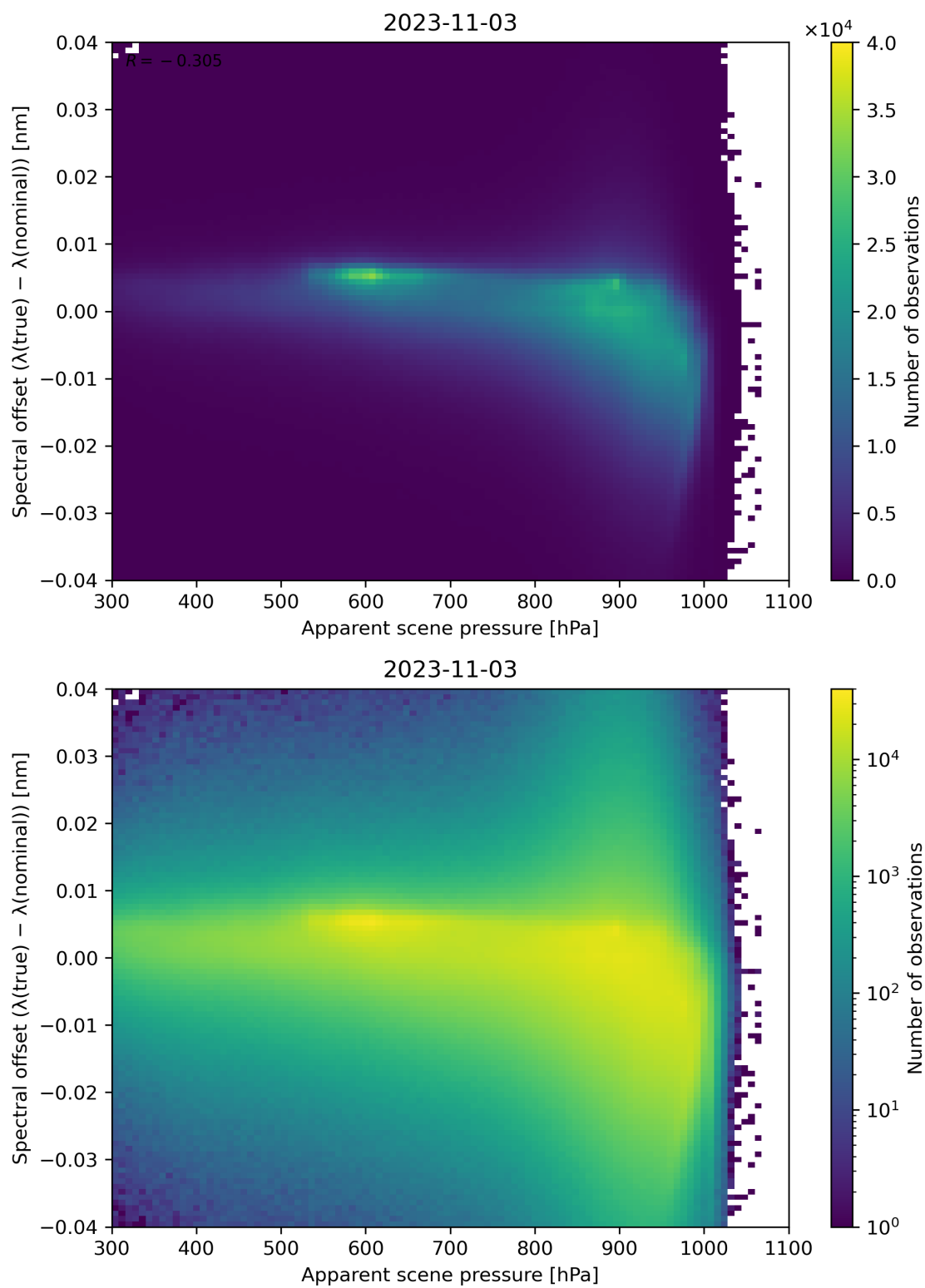
Figure 68: Scatter density plot of “Apparent scene pressure” against “Spectral offset ( \lambda(\text{true}) - \lambda(\text{nominal}) )” for 2023-11-02 to 2023-11-04.
