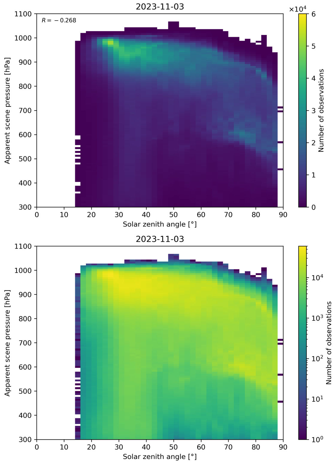
Figure 118: Scatter density plot of “Solar zenith angle” against “Apparent scene pressure” for 2023-11-02 to 2023-11-04.
