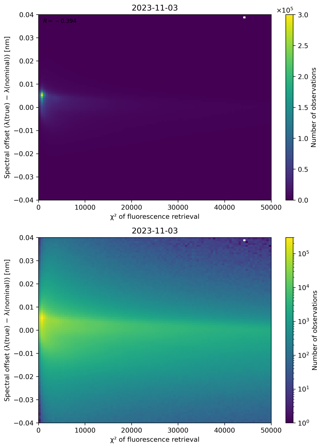
Figure 72: Scatter density plot of " \chi^2 of fluorescence retrieval" against "Spectral offset ( \lambda(\text{true}) - \lambda(\text{nominal})) " for 2023-11-02 to 2023-11-04.
