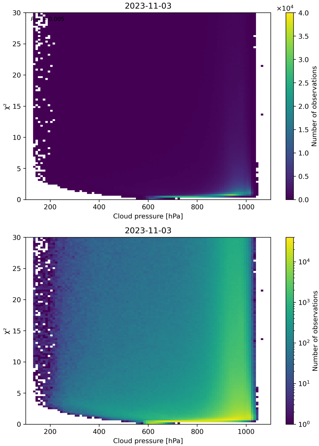
Figure 85: Scatter density plot of “Cloud pressure” against “ \chi^2 ” for 2023-11-02 to 2023-11-04.
