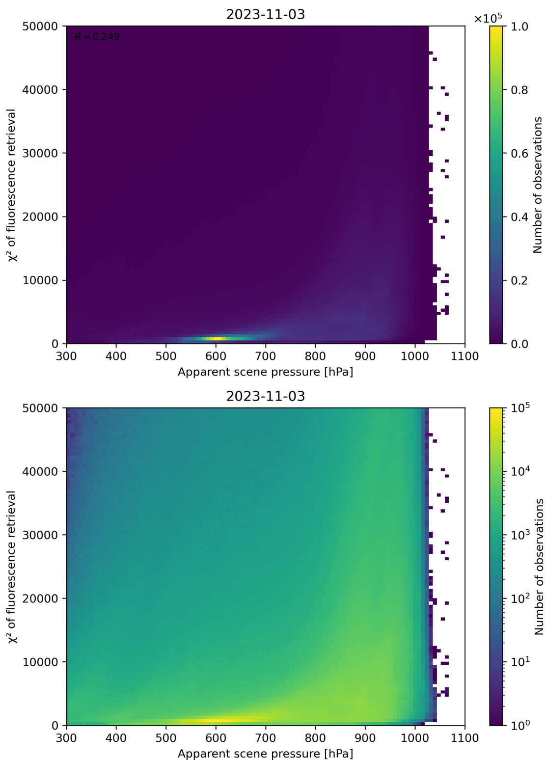
Figure 64: Scatter density plot of “Apparent scene pressure” against “ \chi^2 of fluorescence retrieval” for 2023-11-02 to 2023-11-04.
