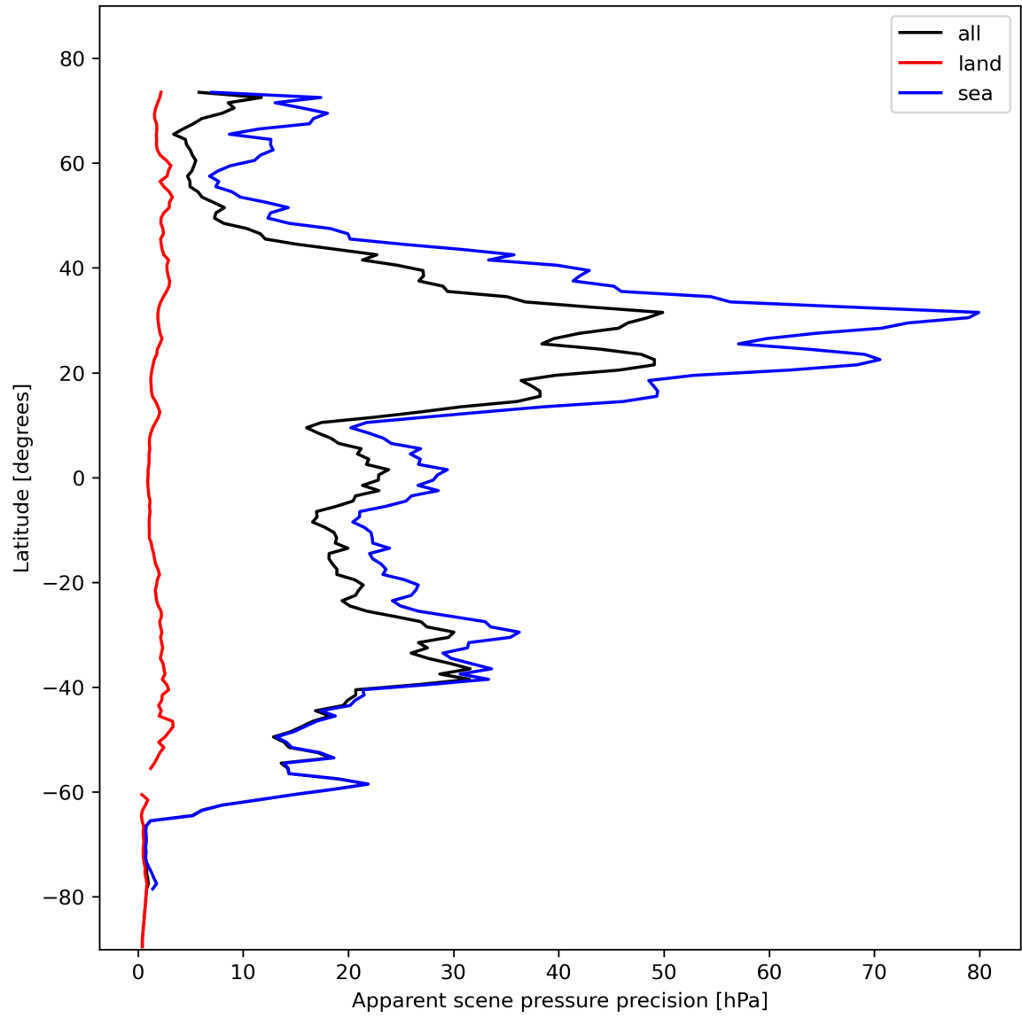
Figure 20: Zonal average of “Apparent scene pressure precision” for 2023-11-02 to 2023-11-04.
