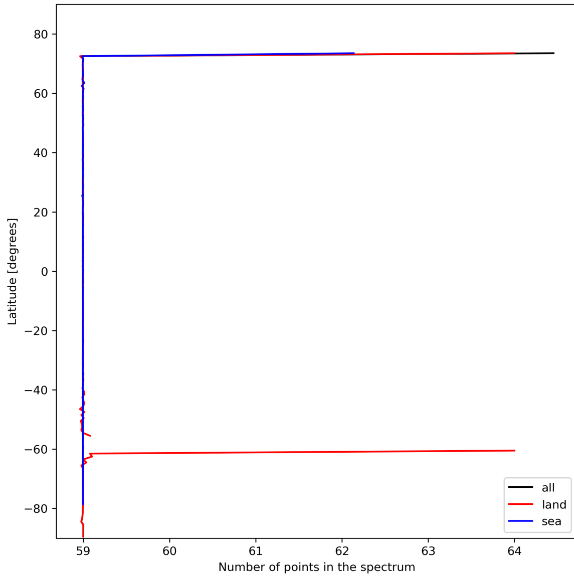
Figure 27: Zonal average of “Number of points in the spectrum” for 2023-11-02 to 2023-11-04.
