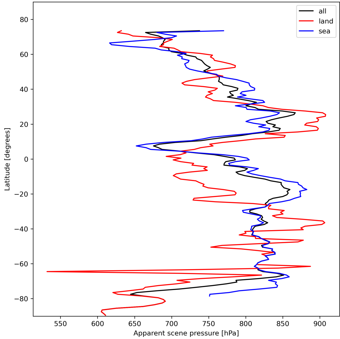
Figure 19: Zonal average of “Apparent scene pressure” for 2023-11-02 to 2023-11-04.
