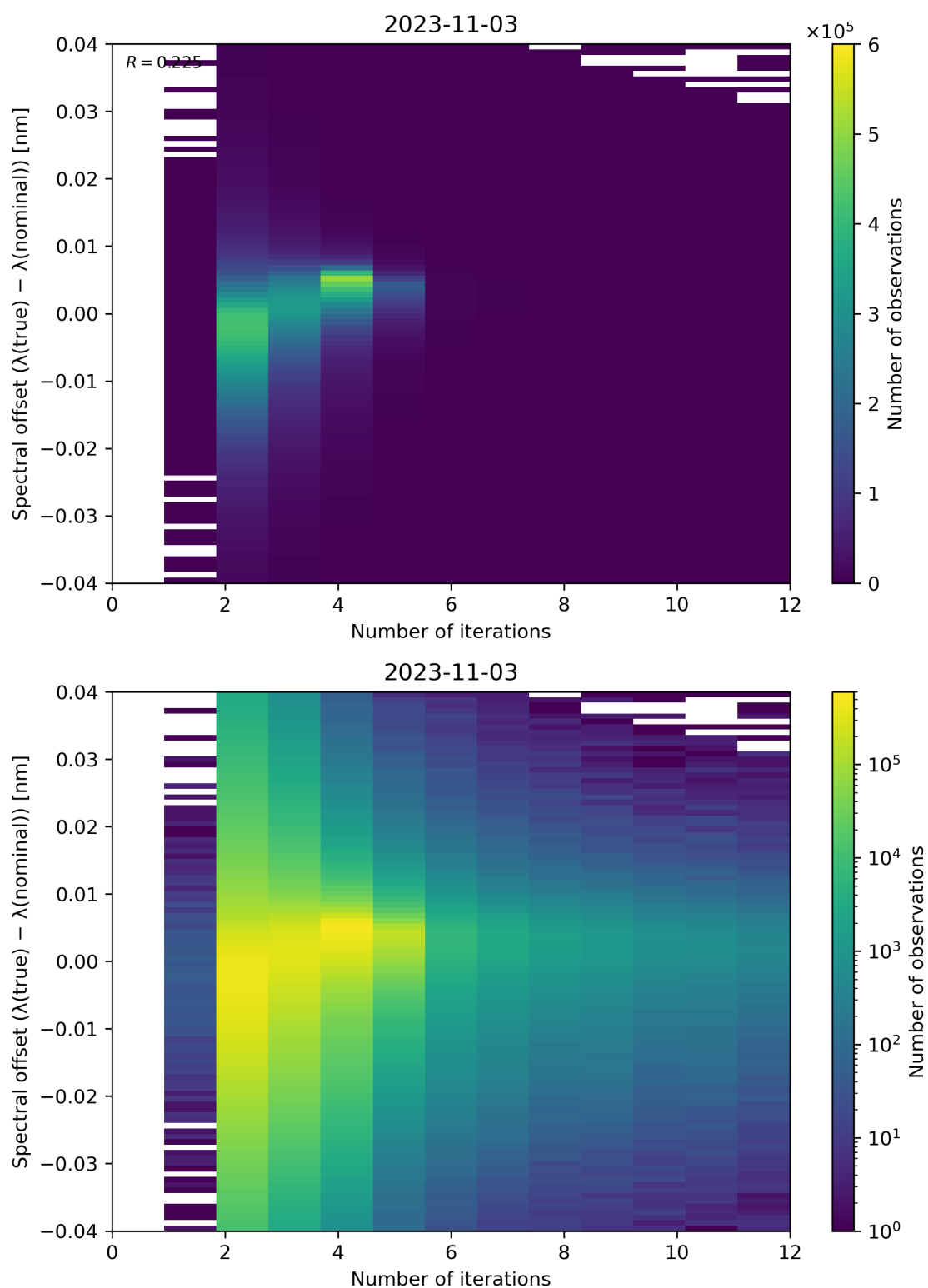
Figure 109: Scatter density plot of “Number of iterations” against “Spectral offset ( \lambda(\text{true}) - \lambda(\text{nominal}) )” for 2023-11-02 to 2023-11-04.
