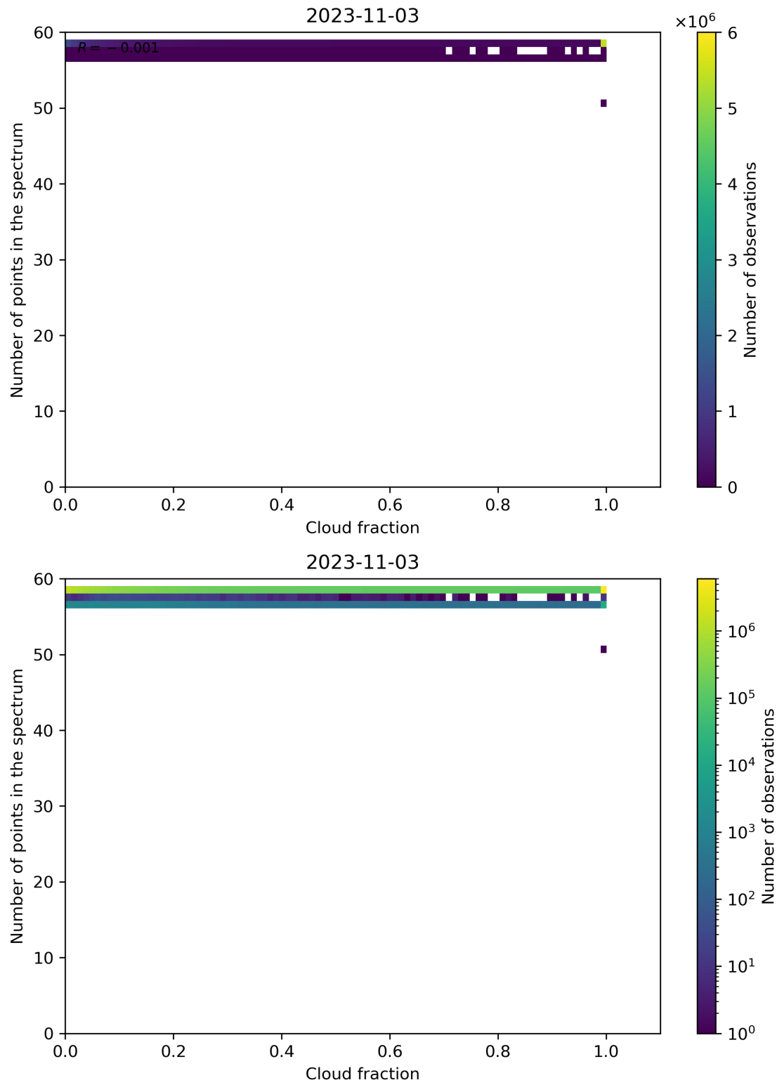
Figure 81: Scatter density plot of “Cloud fraction” against “Number of points in the spectrum” for 2023-11-02 to 2023-11-04.
