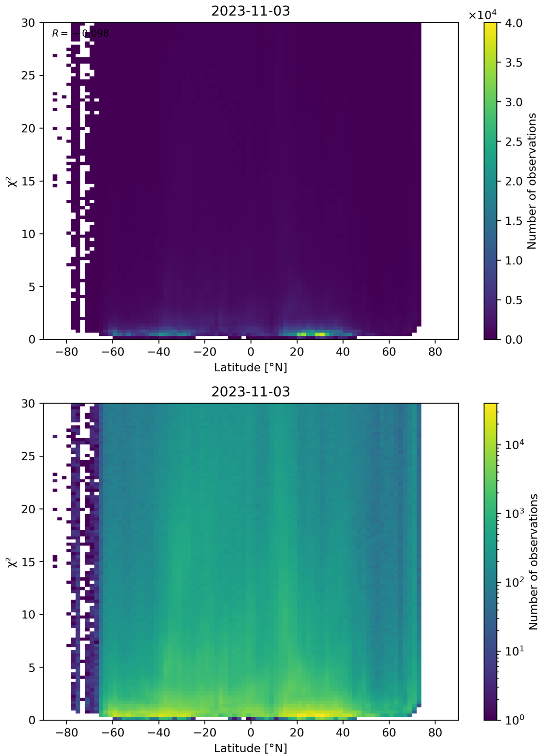
Figure 97: Scatter density plot of “Latitude” against “ \chi^2 ” for 2023-11-02 to 2023-11-04.
