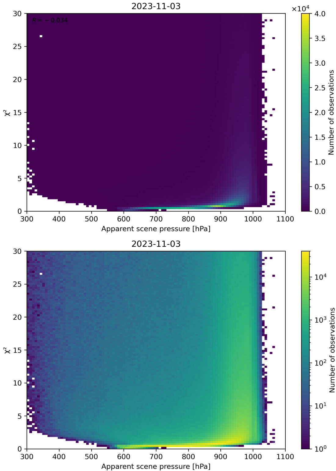
Figure 63: Scatter density plot of “Apparent scene pressure” against “ \chi^2 ” for 2023-11-02 to 2023-11-04.
