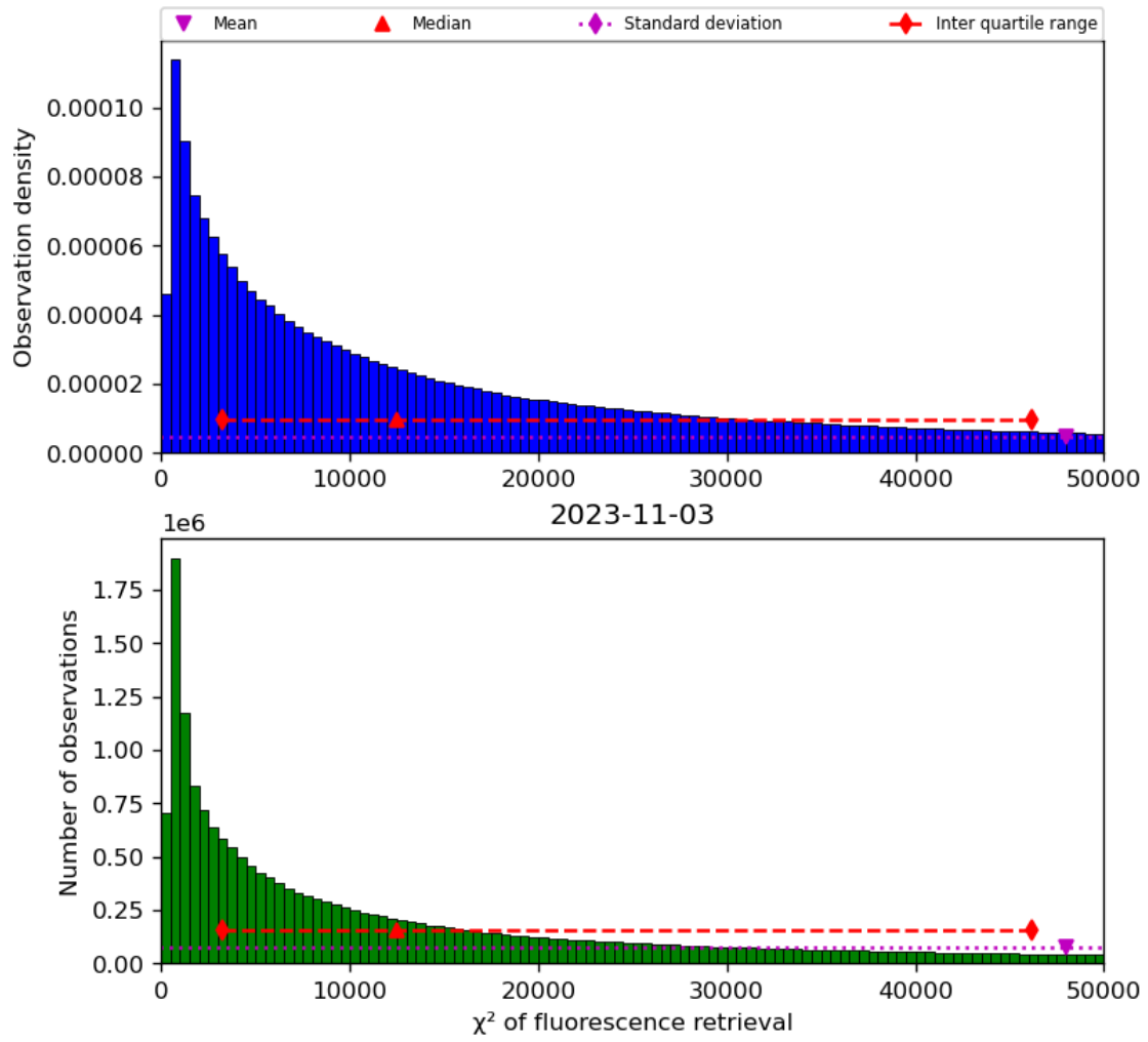
Figure 42: Histogram of “ \chi^2 of fluorescence retrieval” for 2023-11-02 to 2023-11-04
