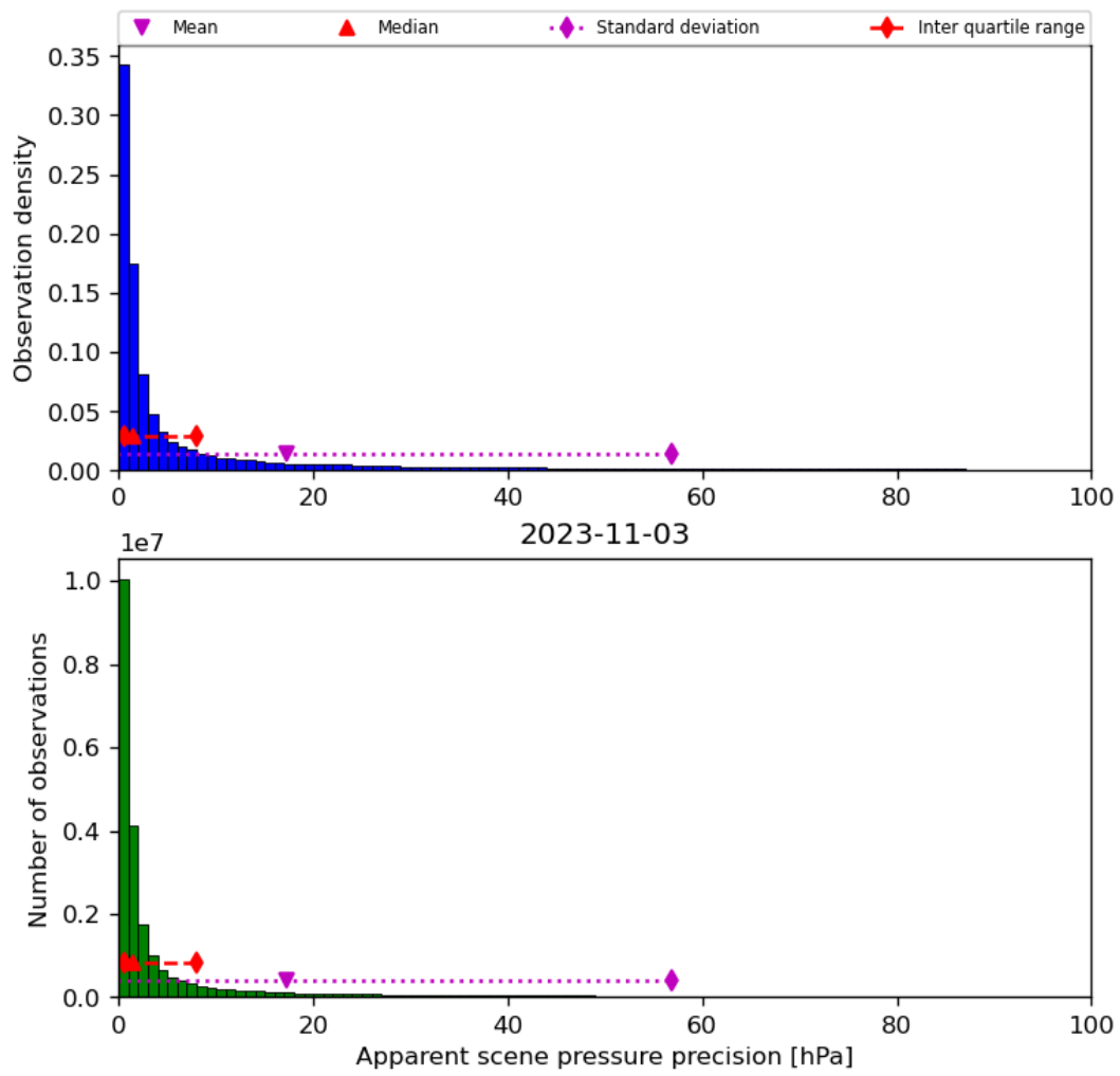
Figure 37: Histogram of “Apparent scene pressure precision” for 2023-11-02 to 2023-11-04
