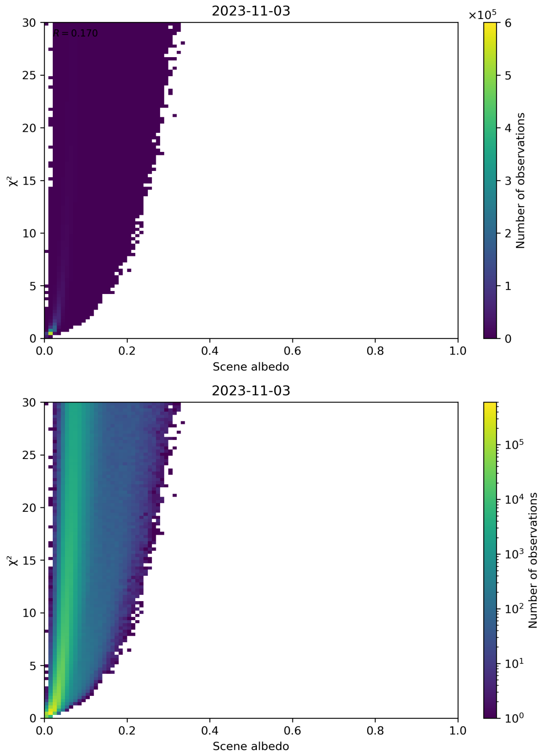
Figure 112: Scatter density plot of “Scene albedo” against “ \chi^2 ” for 2023-11-02 to 2023-11-04.
