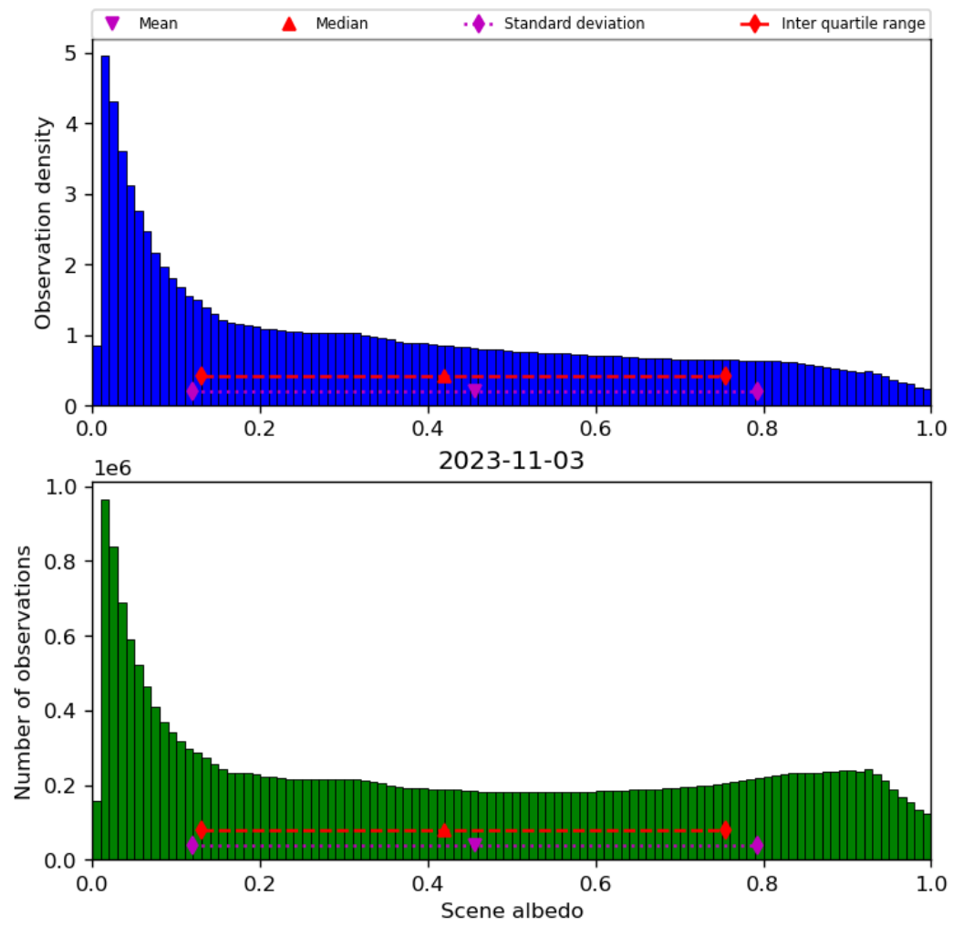
Figure 34: Histogram of “Scene albedo” for 2023-11-02 to 2023-11-04
