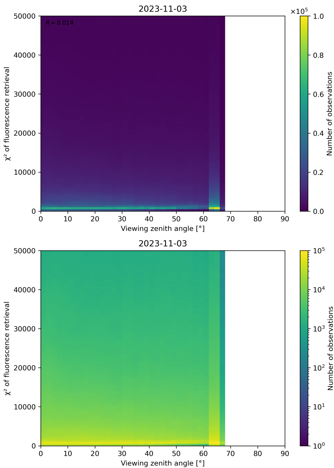
Figure 131: Scatter density plot of “Viewing zenith angle” against “ \chi^2 of fluorescence retrieval” for 2023-11-02 to 2023-11-04.
