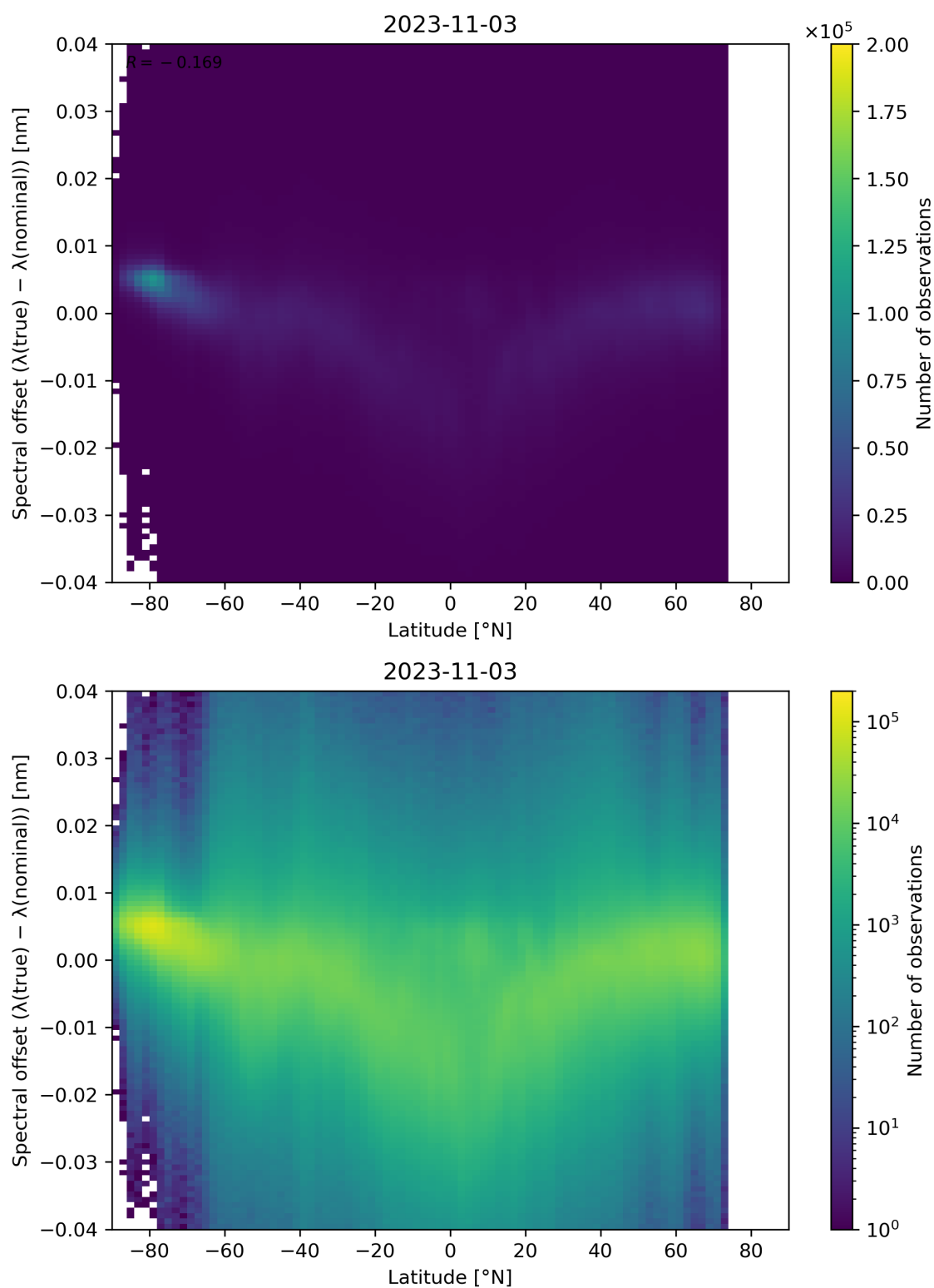
Figure 105: Scatter density plot of “Latitude” against “Spectral offset ( \lambda(\text{true}) - \lambda(\text{nominal}) )” for 2023-11-02 to 2023-11-04.
