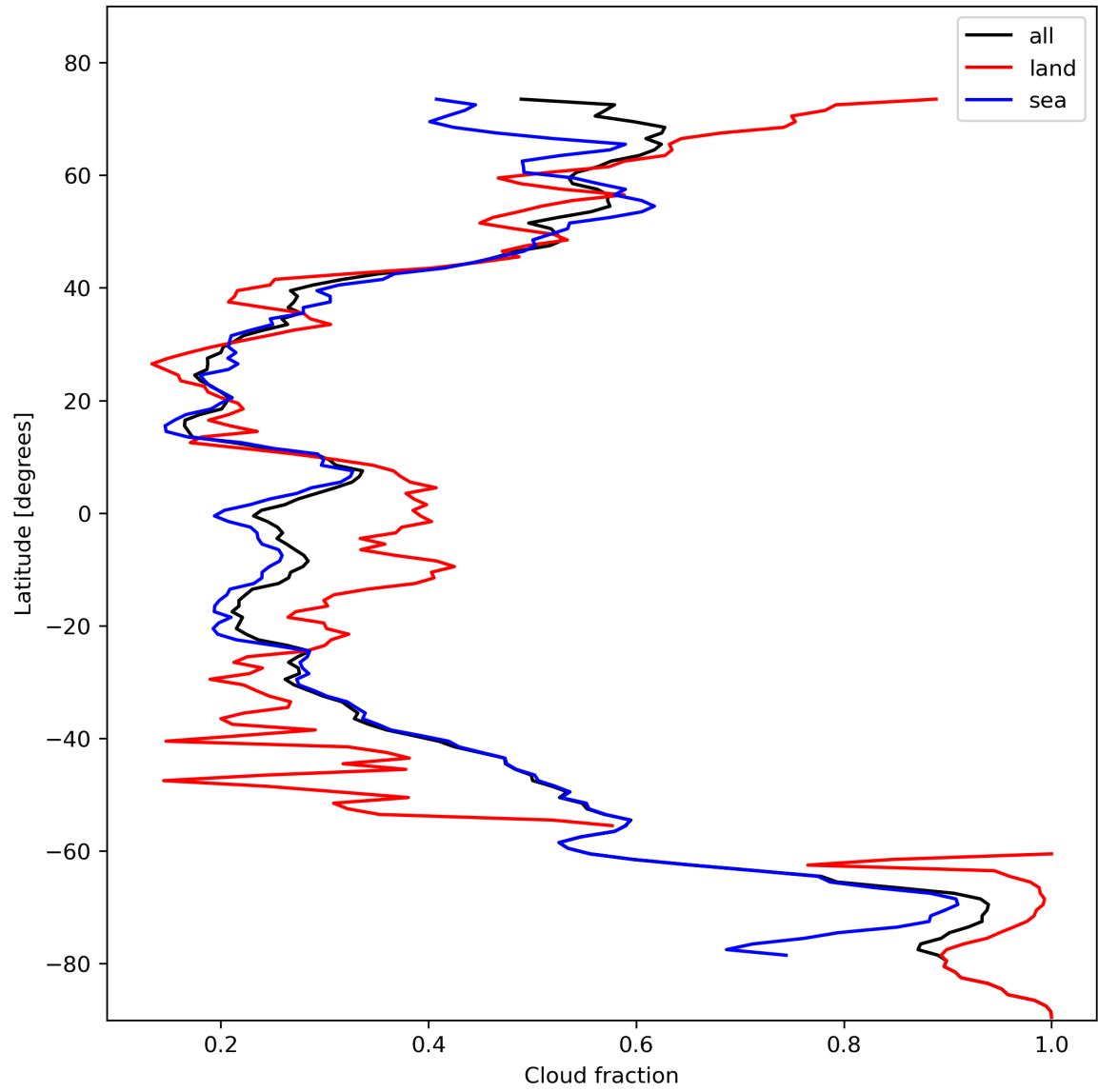
Figure 15: Zonal average of “Cloud fraction” for 2023-11-02 to 2023-11-04.
