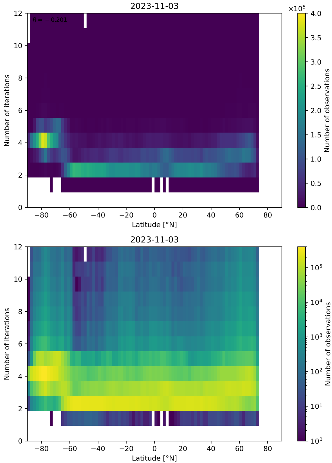
Figure 102: Scatter density plot of “Latitude” against “Number of iterations” for 2023-11-02 to 2023-11-04.
