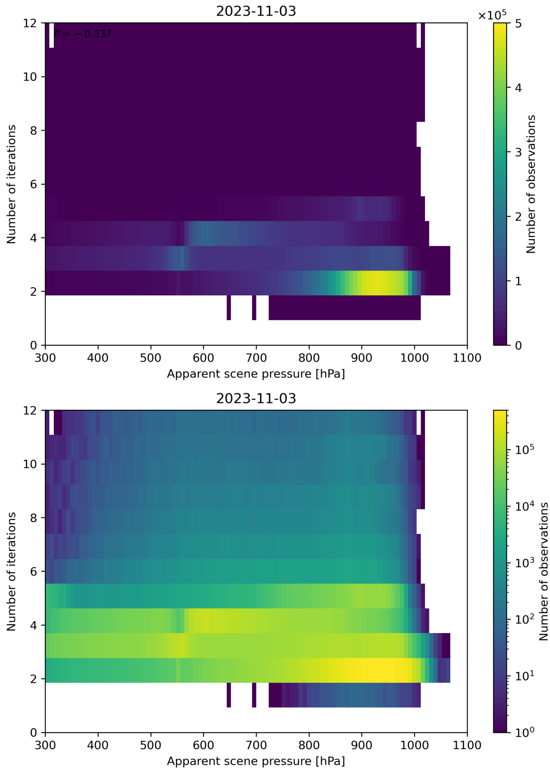
Figure 66: Scatter density plot of “Apparent scene pressure” against “Number of iterations” for 2023-11-02 to 2023-11-04.
