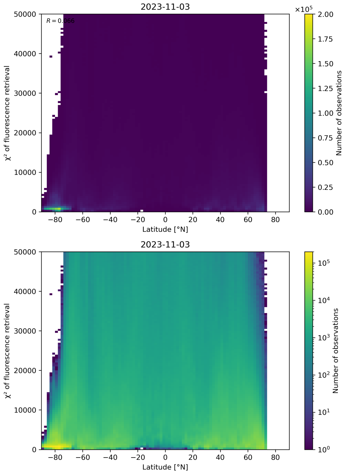
Figure 98: Scatter density plot of “Latitude” against “ \chi^2 of fluorescence retrieval” for 2023-11-02 to 2023-11-04.
