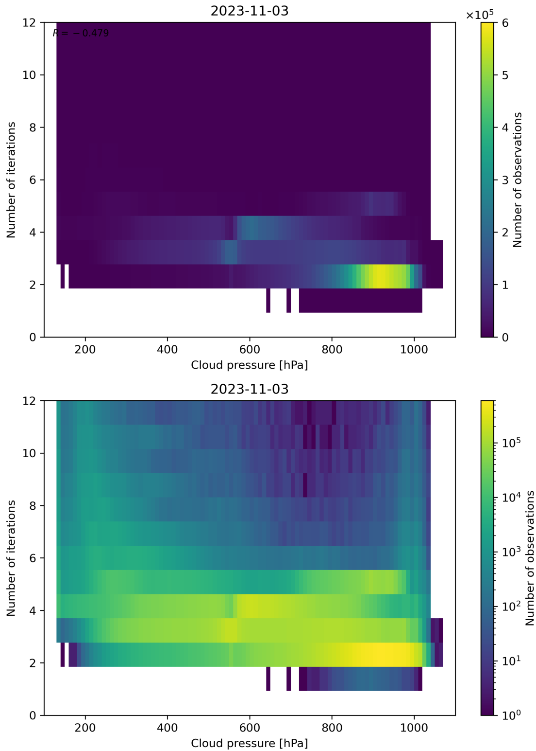
Figure 89: Scatter density plot of “Cloud pressure” against “Number of iterations” for 2023-11-02 to 2023-11-04.
