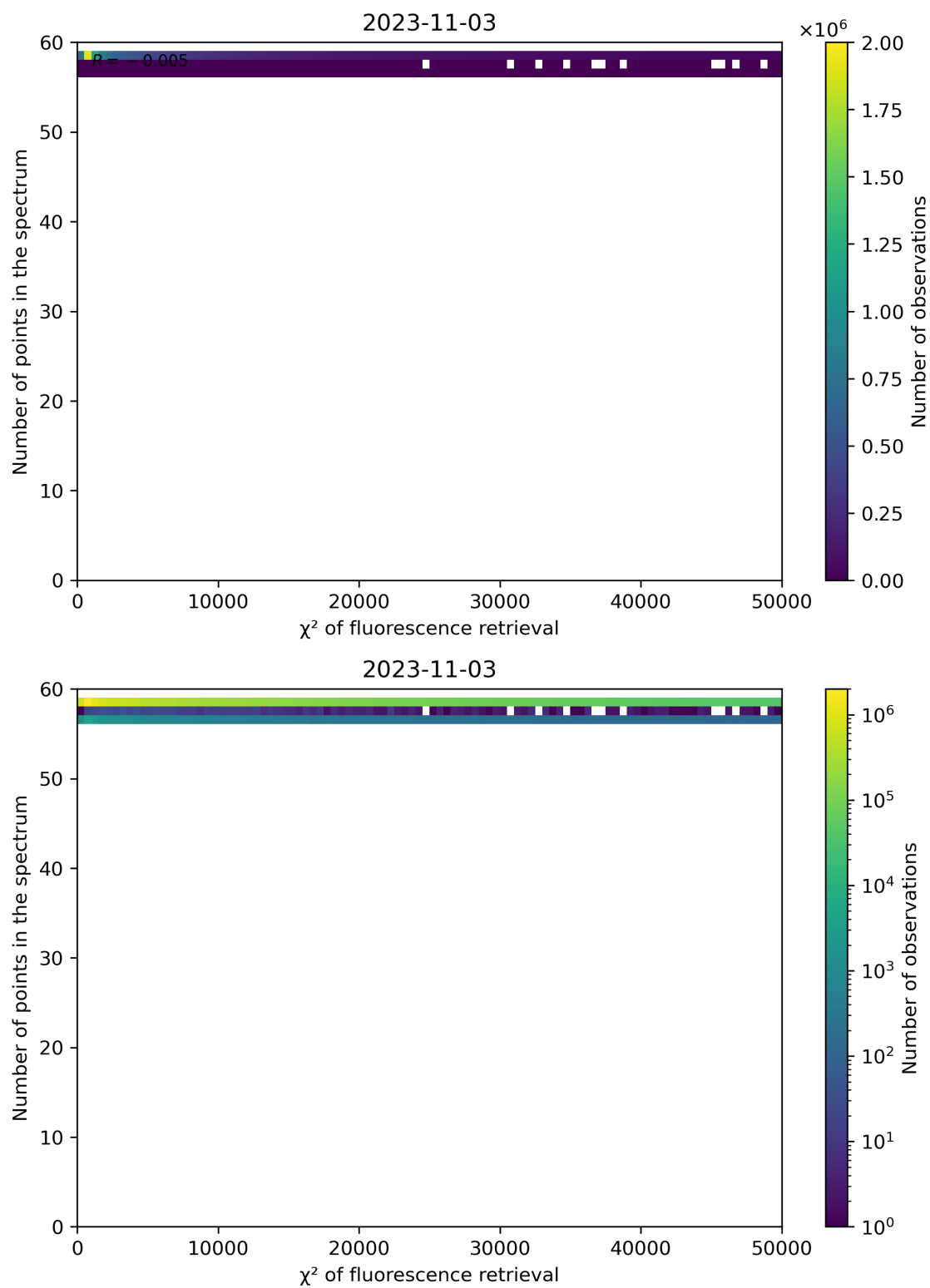
Figure 71: Scatter density plot of " \chi^2 of fluorescence retrieval" against "Number of points in the spectrum" for 2023-11-02 to 2023-11-04.
