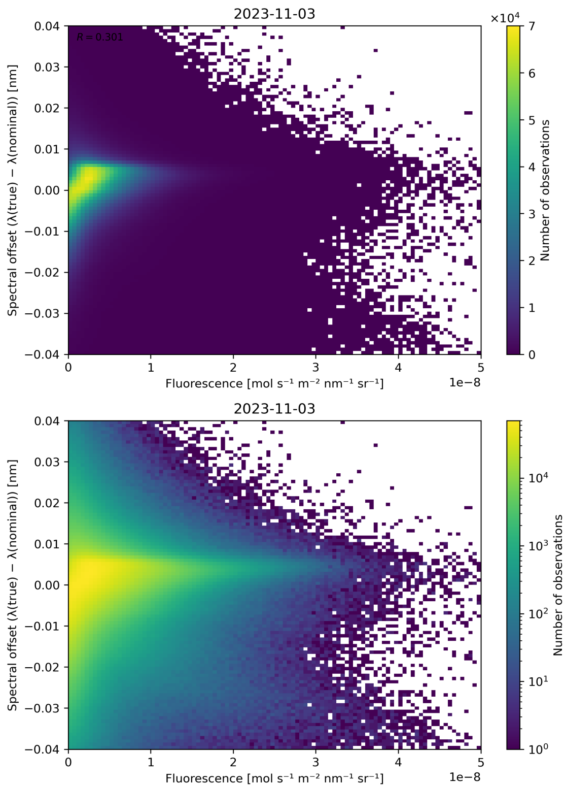
Figure 95: Scatter density plot of “Fluorescence” against “Spectral offset ( \lambda(\text{true}) - \lambda(\text{nominal}) )” for 2023-11-02 to 2023-11-04.
