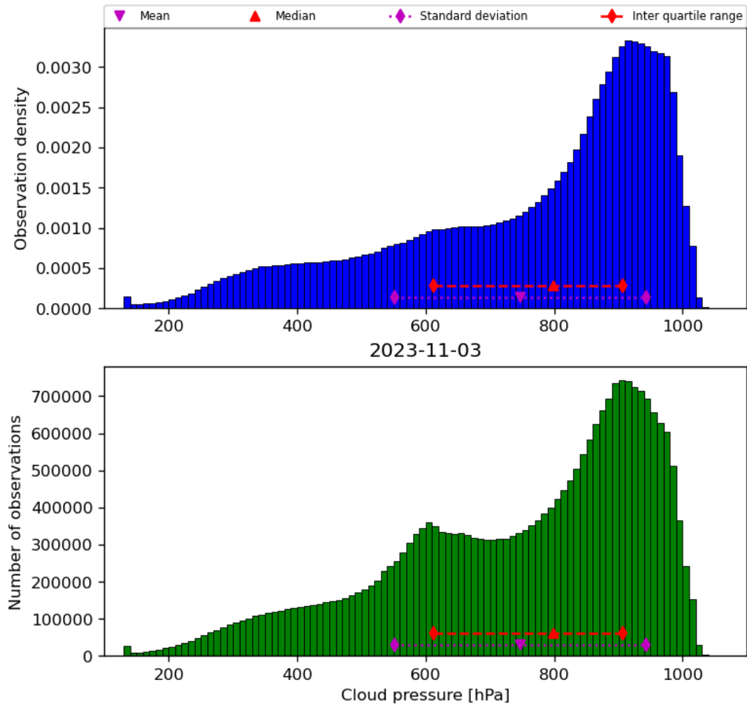
Figure 30: Histogram of “Cloud pressure” for 2023-11-02 to 2023-11-04
