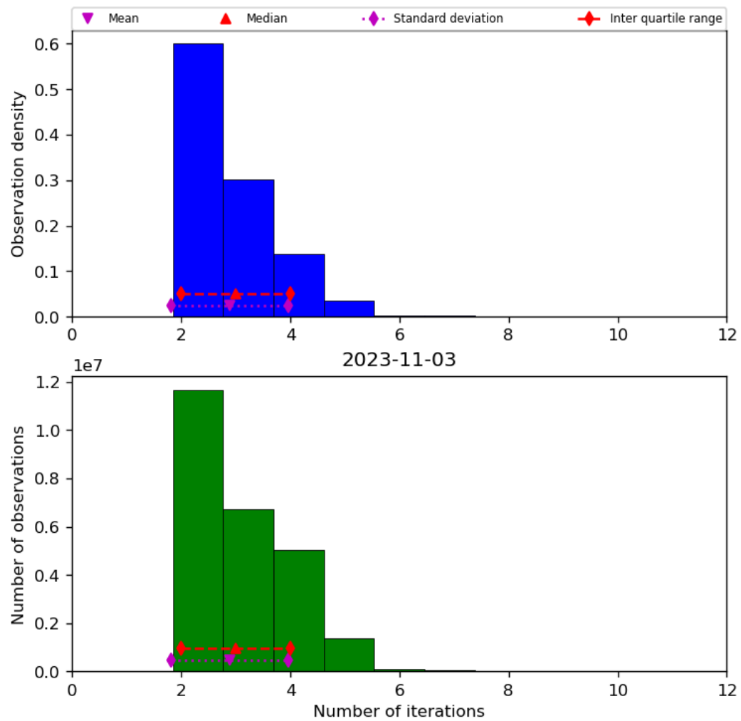
Figure 39: Histogram of “Number of iterations” for 2023-11-02 to 2023-11-04
