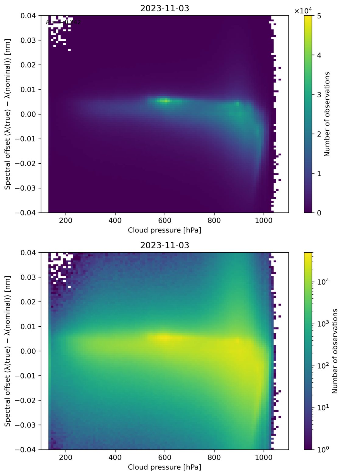
Figure 92: Scatter density plot of “Cloud pressure” against “Spectral offset ( \lambda(\text{true}) - \lambda(\text{nominal}) )” for 2023-11-02 to 2023-11-04.
