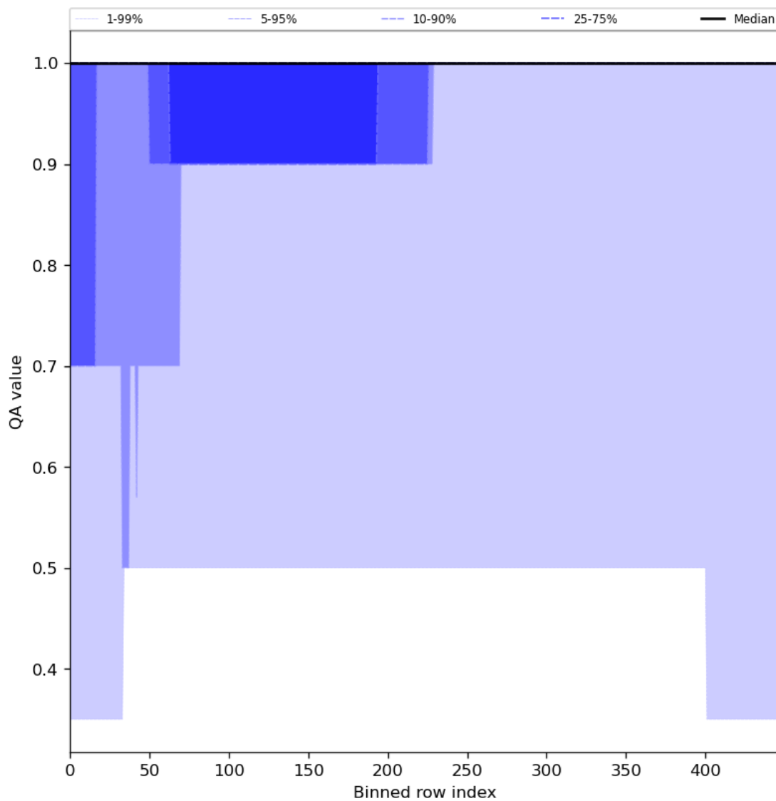
Figure 46: Along track statistics of “QA value” for 2023-11-02 to 2023-11-04
