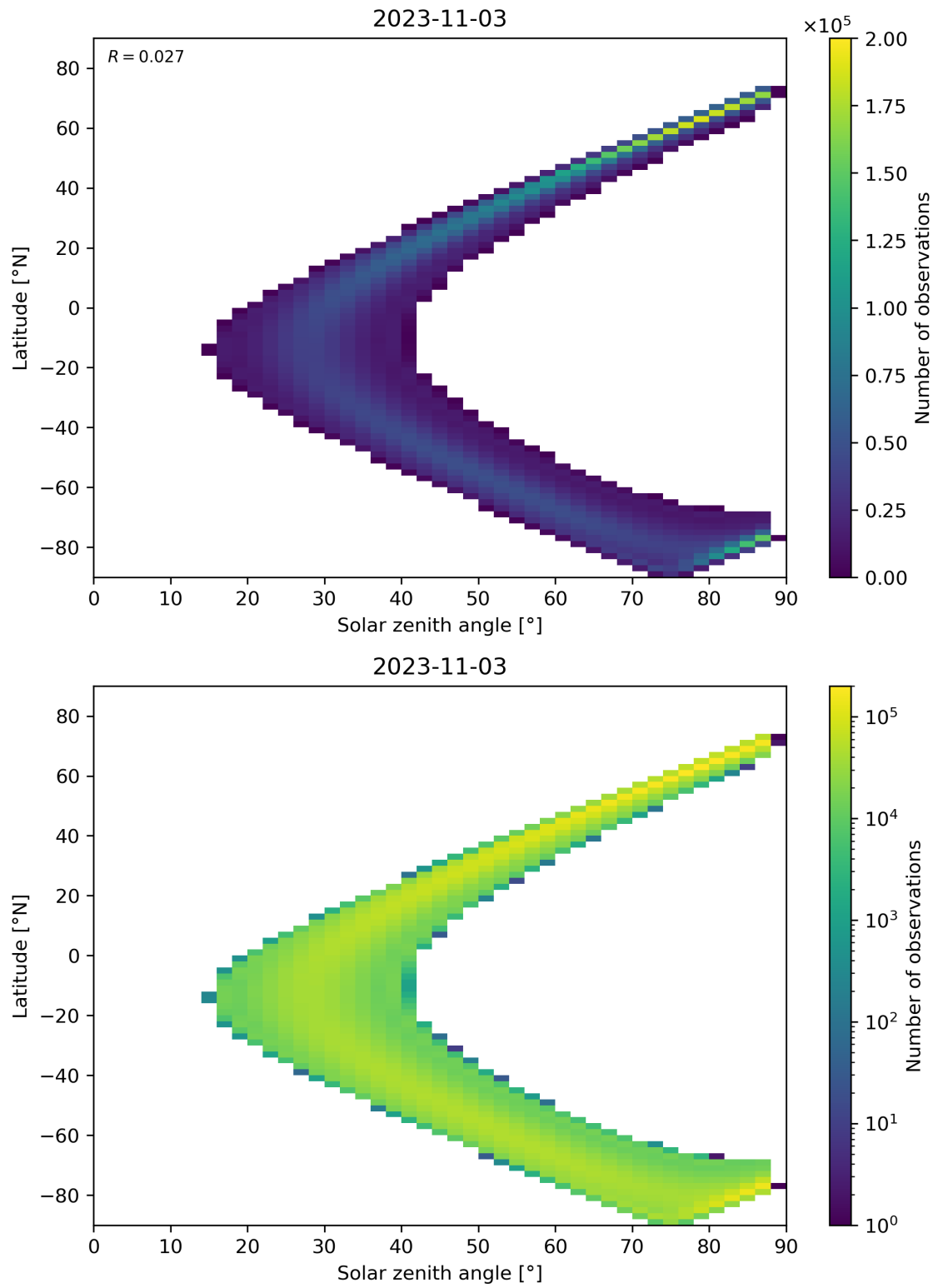
Figure 124: Scatter density plot of “Solar zenith angle” against “Latitude” for 2023-11-02 to 2023-11-04.
