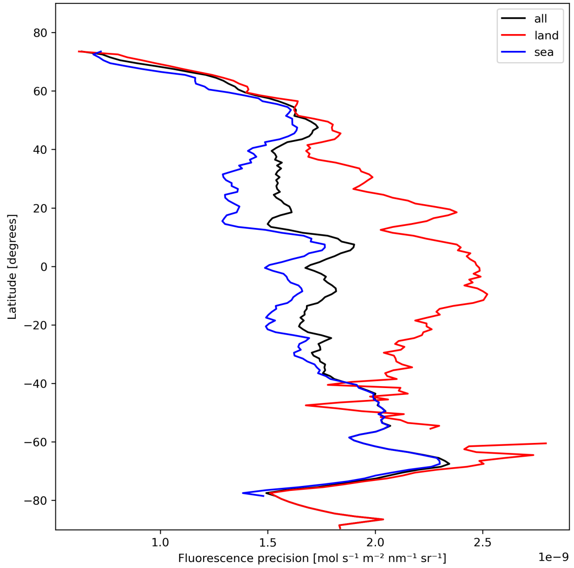
Figure 24: Zonal average of “Fluorescence precision” for 2023-11-02 to 2023-11-04.
