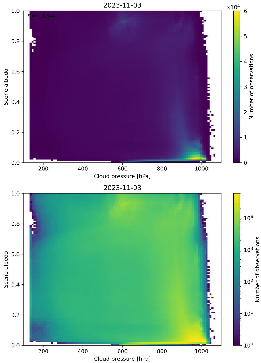
Figure 91: Scatter density plot of “Cloud pressure” against “Scene albedo” for 2023-11-02 to 2023-11-04.
