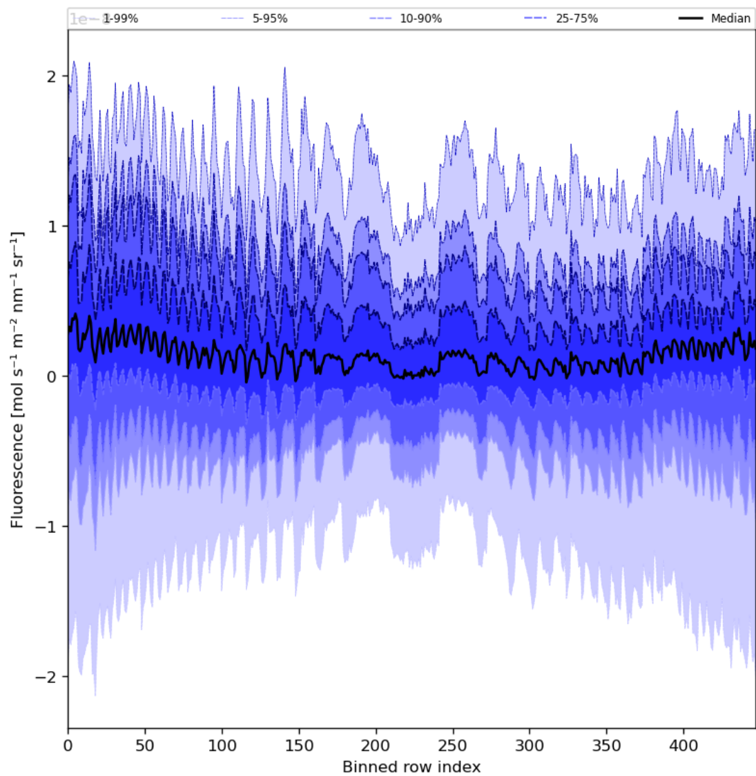
Figure 57: Along track statistics of “Fluorescence” for 2023-11-02 to 2023-11-04
