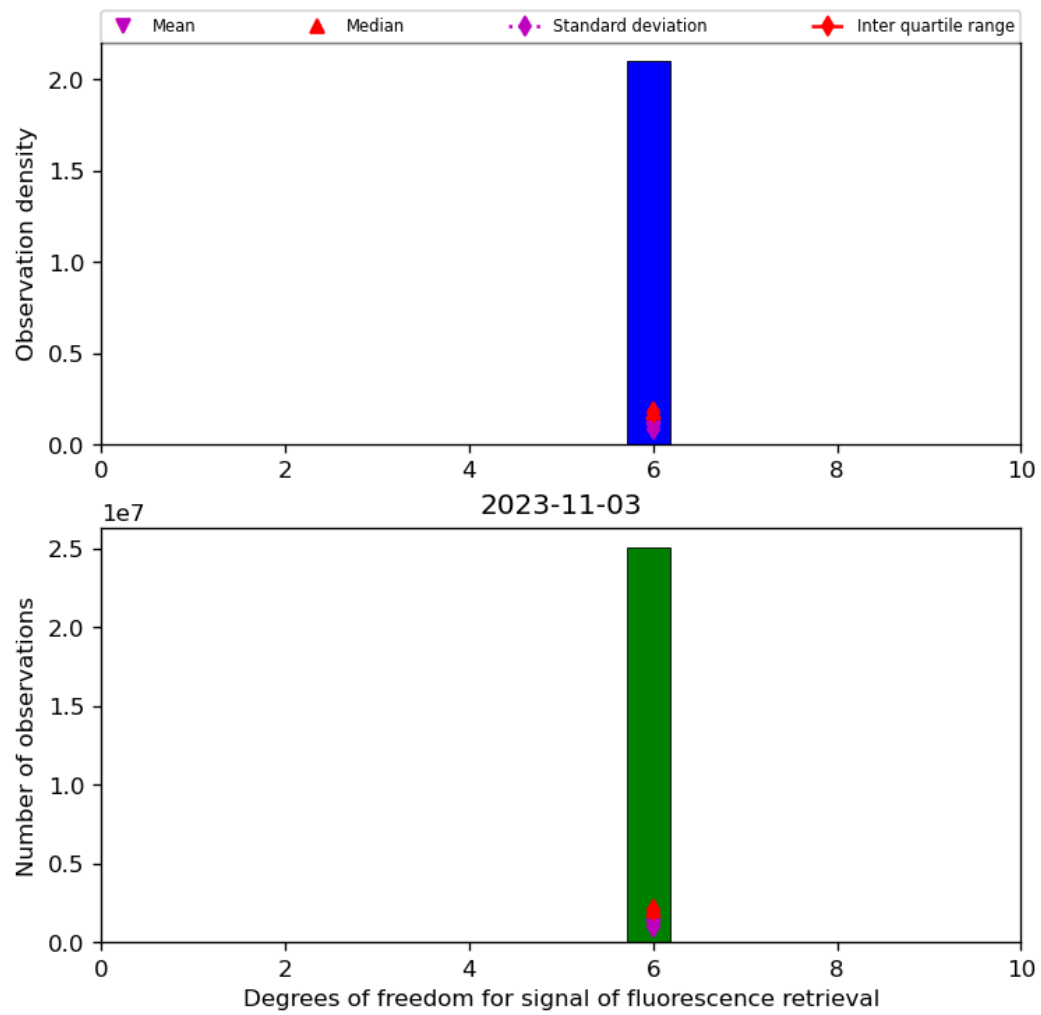
Figure 43: Histogram of “Degrees of freedom for signal of fluorescence retrieval” for 2023-11-02 to 2023-11-04
