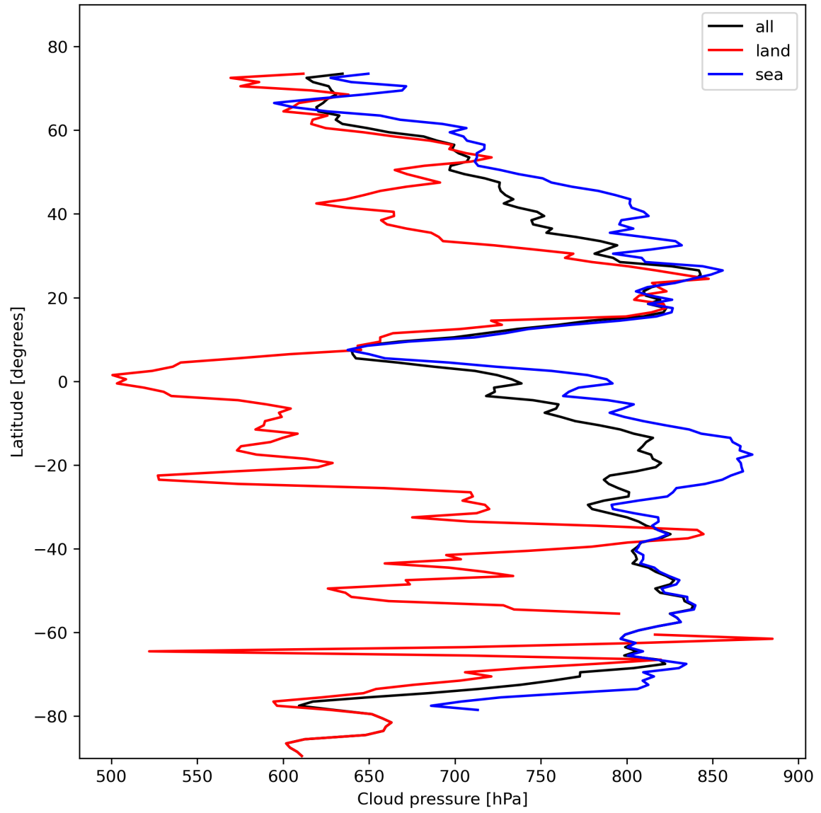
Figure 13: Zonal average of “Cloud pressure” for 2023-11-02 to 2023-11-04.
