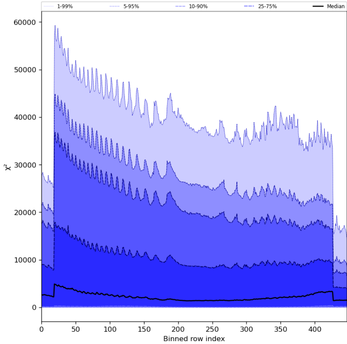
Figure 55: Along track statistics of “ \chi^2 ” for 2023-11-02 to 2023-11-04
