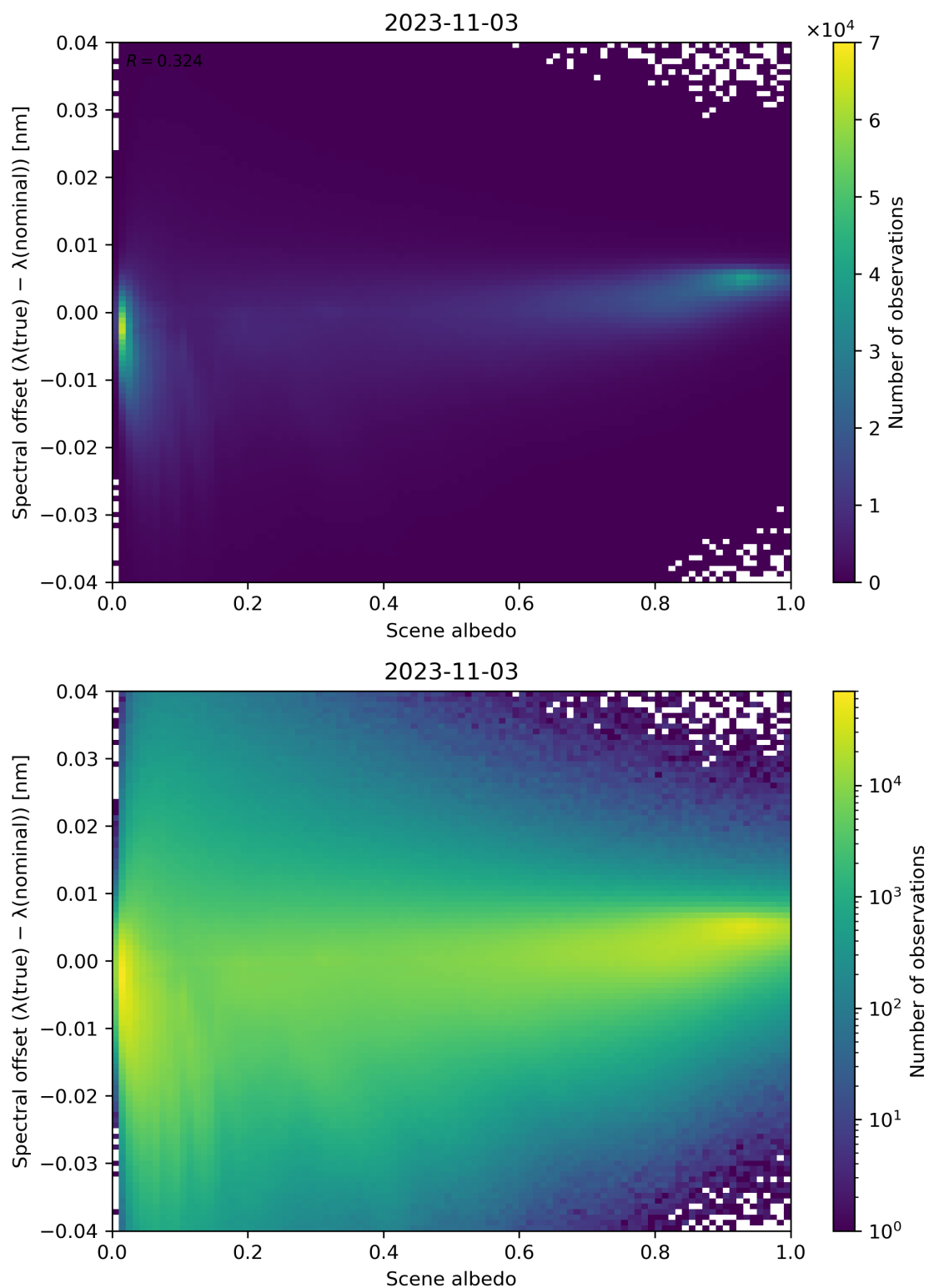
Figure 117: Scatter density plot of “Scene albedo” against “Spectral offset ( \lambda(\text{true}) - \lambda(\text{nominal}) )” for 2023-11-02 to 2023-11-04.
