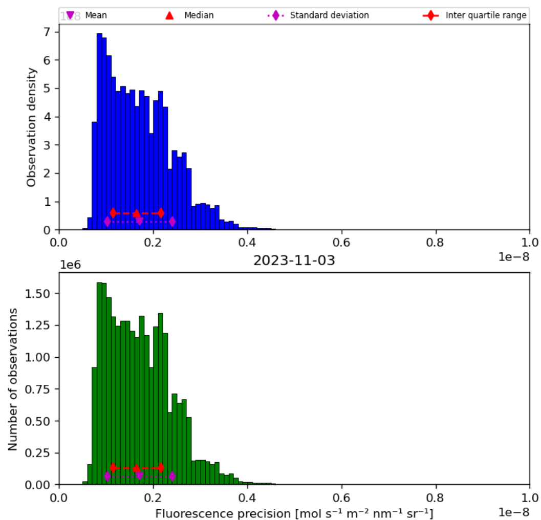
Figure 41: Histogram of “Fluorescence precision” for 2023-11-02 to 2023-11-04
