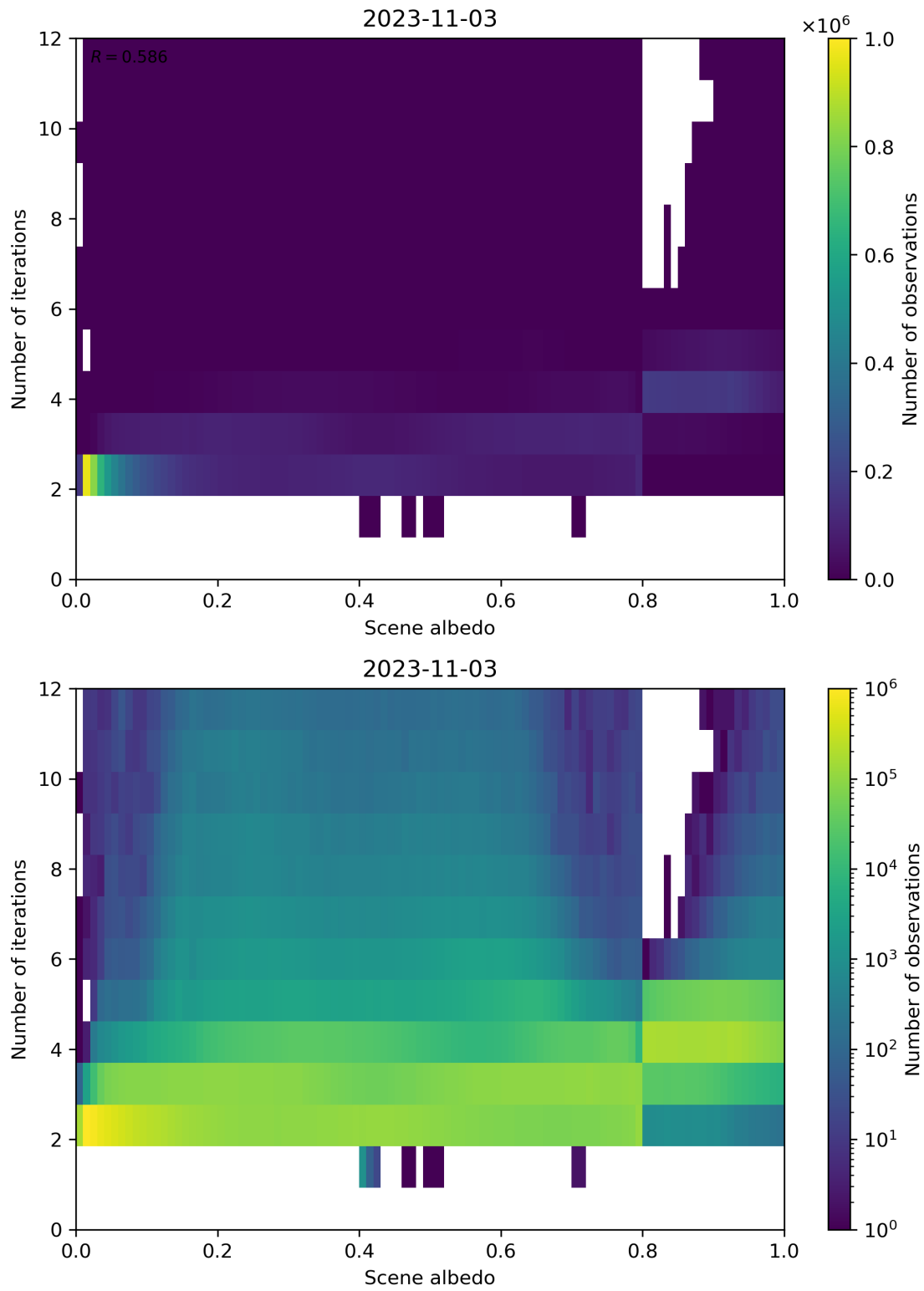
Figure 115: Scatter density plot of “Scene albedo” against “Number of iterations” for 2023-11-02 to 2023-11-04.
