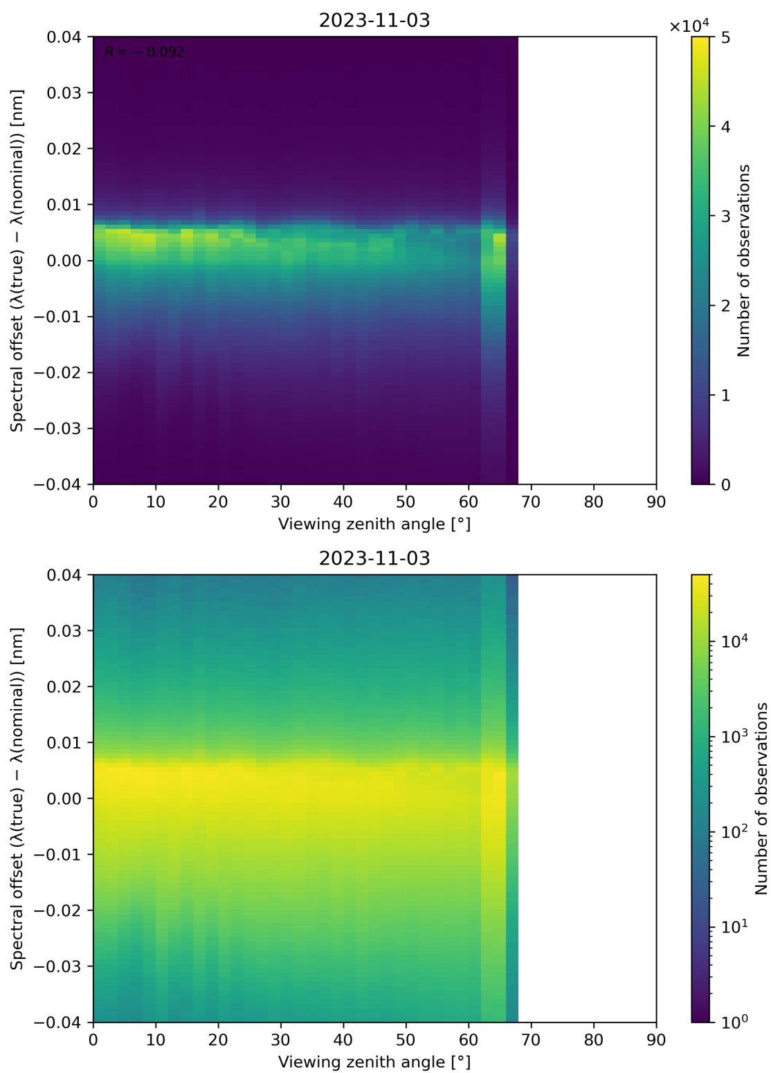
Figure 140: Scatter density plot of “Viewing zenith angle” against “Spectral offset ( \lambda(\text{true}) - \lambda(\text{nominal}) )” for 2023-11-02 to 2023-11-04.
