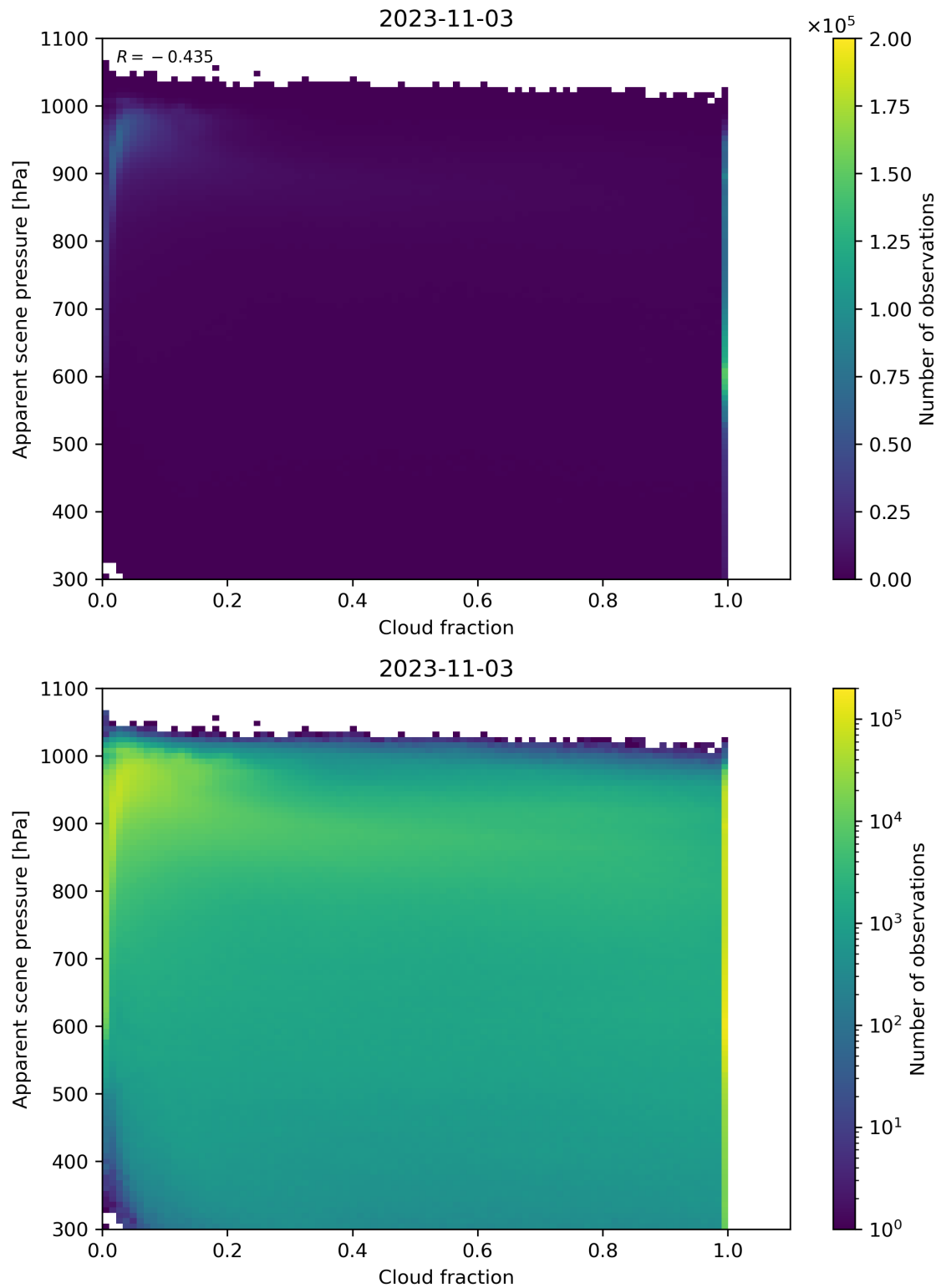
Figure 76: Scatter density plot of “Cloud fraction” against “Apparent scene pressure” for 2023-11-02 to 2023-11-04.
