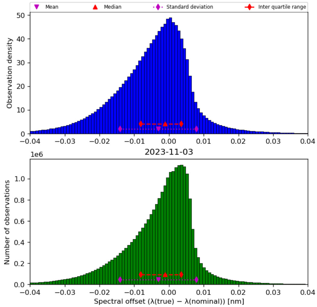
Figure 45: Histogram of “Spectral offset ( \lambda(\text{true}) - \lambda(\text{nominal}) )” for 2023-11-02 to 2023-11-04
