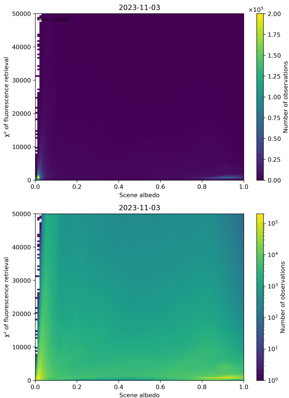
Figure 113: Scatter density plot of “Scene albedo” against “ \chi^2 of fluorescence retrieval” for 2023-11-02 to 2023-11-04.
