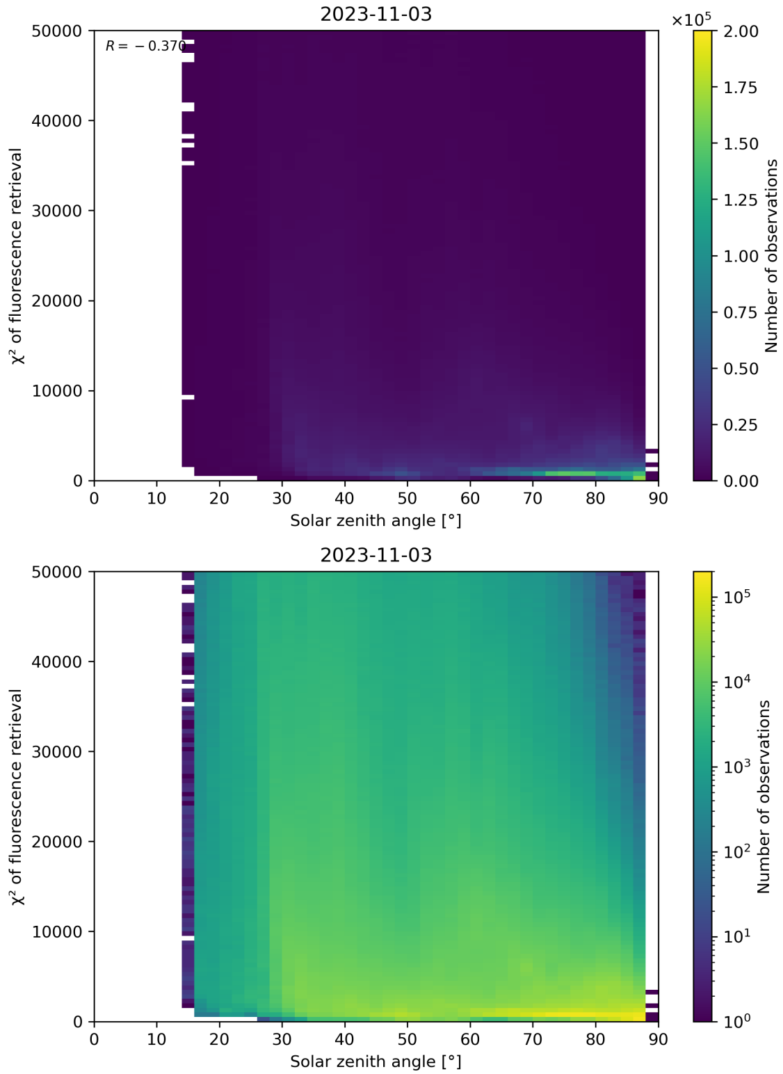
Figure 120: Scatter density plot of “Solar zenith angle” against “ \chi^2 of fluorescence retrieval” for 2023-11-02 to 2023-11-04.
