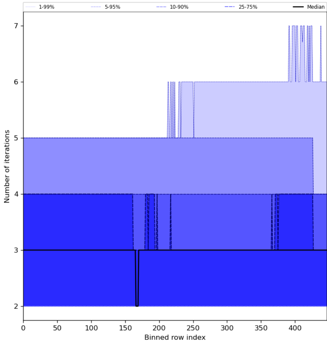
Figure 56: Along track statistics of “Number of iterations” for 2023-11-02 to 2023-11-04
