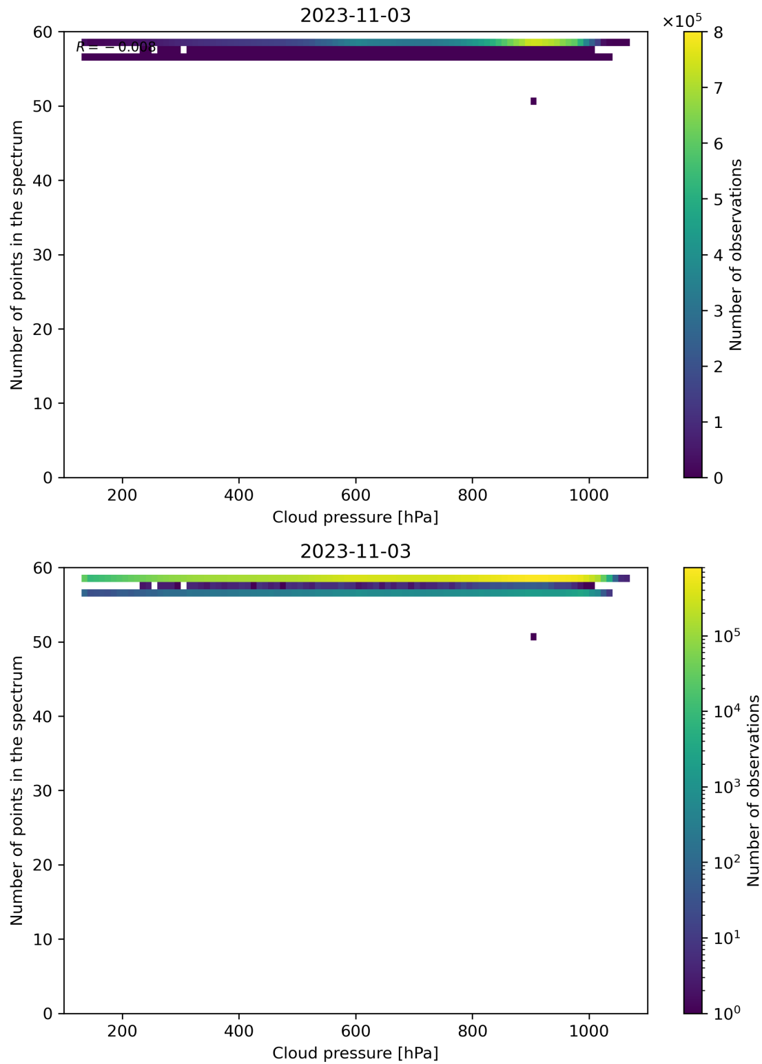
Figure 90: Scatter density plot of “Cloud pressure” against “Number of points in the spectrum” for 2023-11-02 to 2023-11-04.
