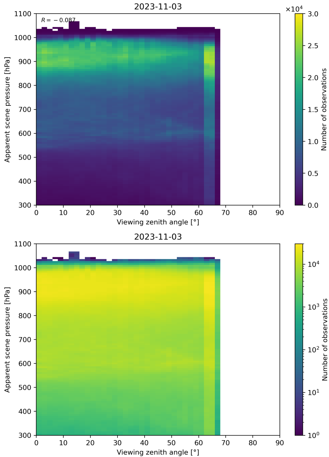
Figure 129: Scatter density plot of “Viewing zenith angle” against “Apparent scene pressure” for 2023-11-02 to 2023-11-04.
