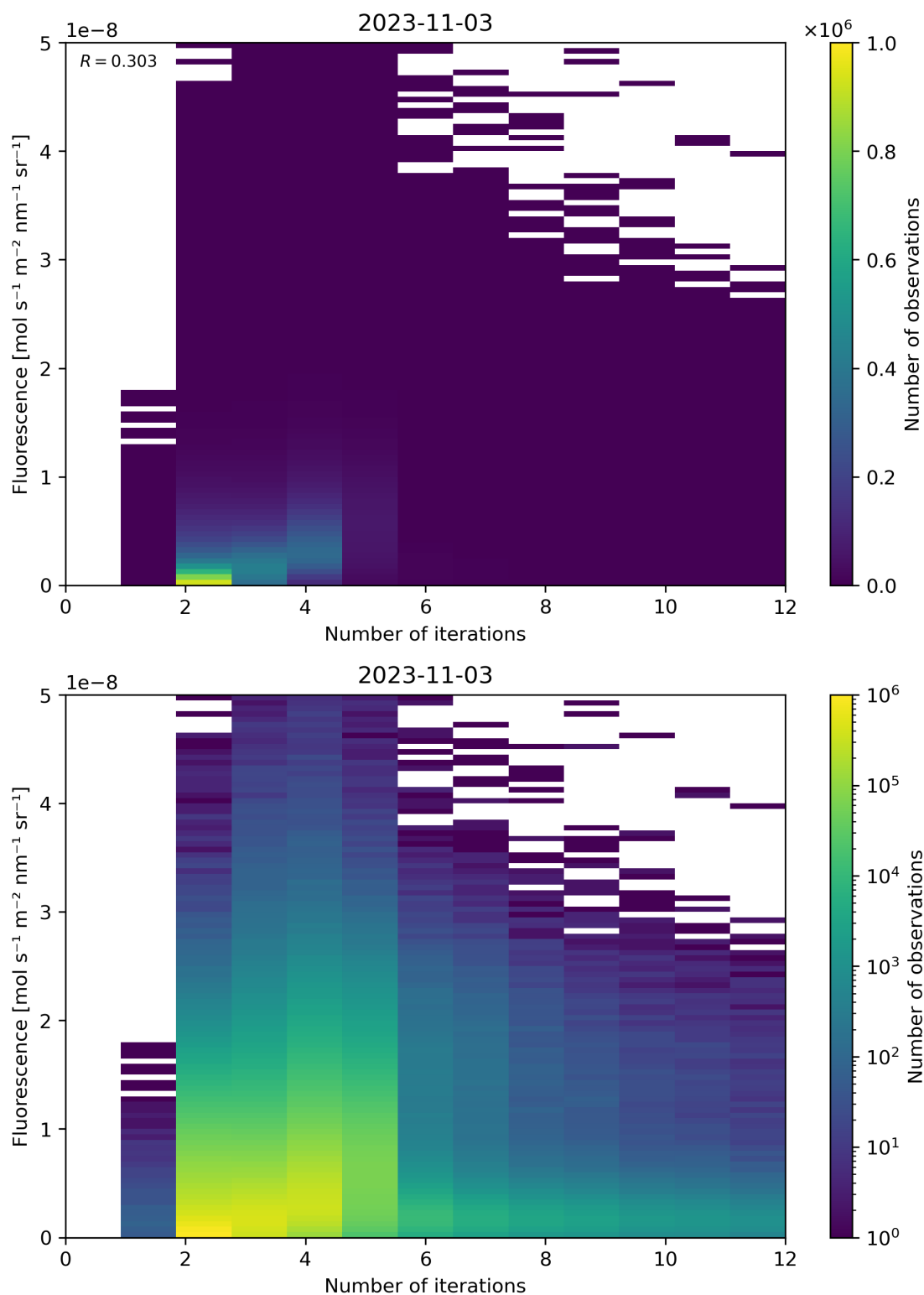
Figure 107: Scatter density plot of “Number of iterations” against “Fluorescence” for 2023-11-02 to 2023-11-04.
