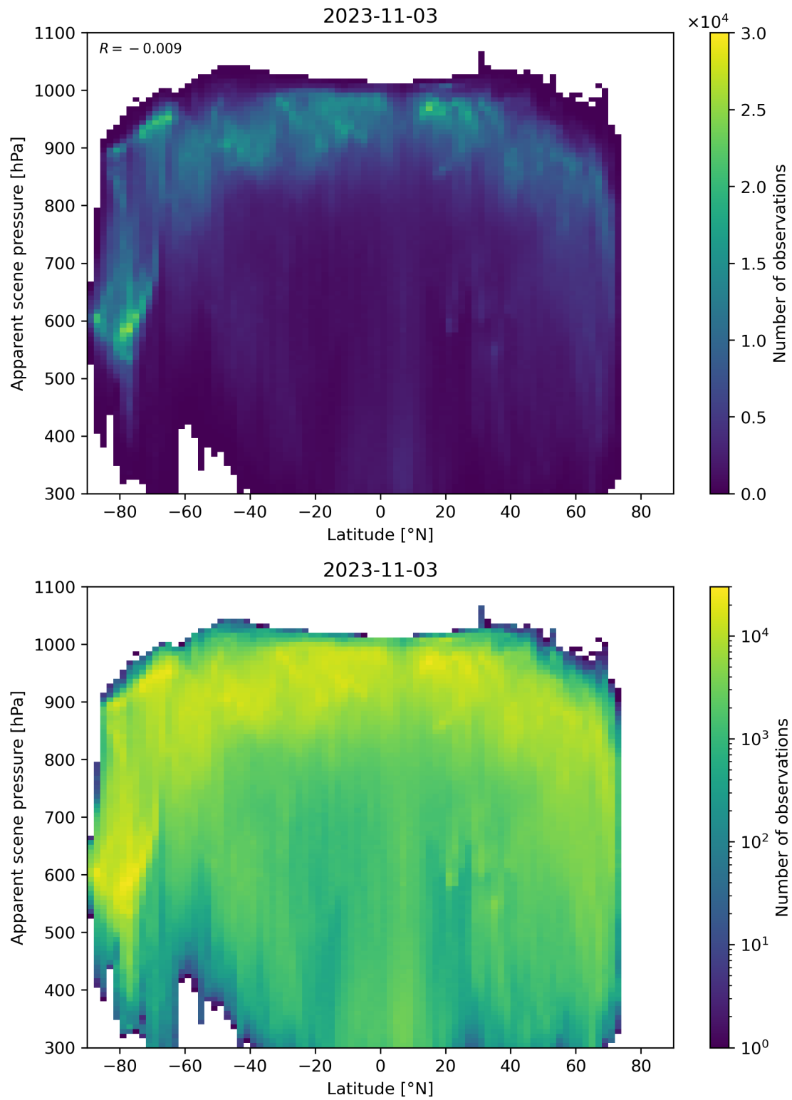
Figure 96: Scatter density plot of “Latitude” against “Apparent scene pressure” for 2023-11-02 to 2023-11-04.
