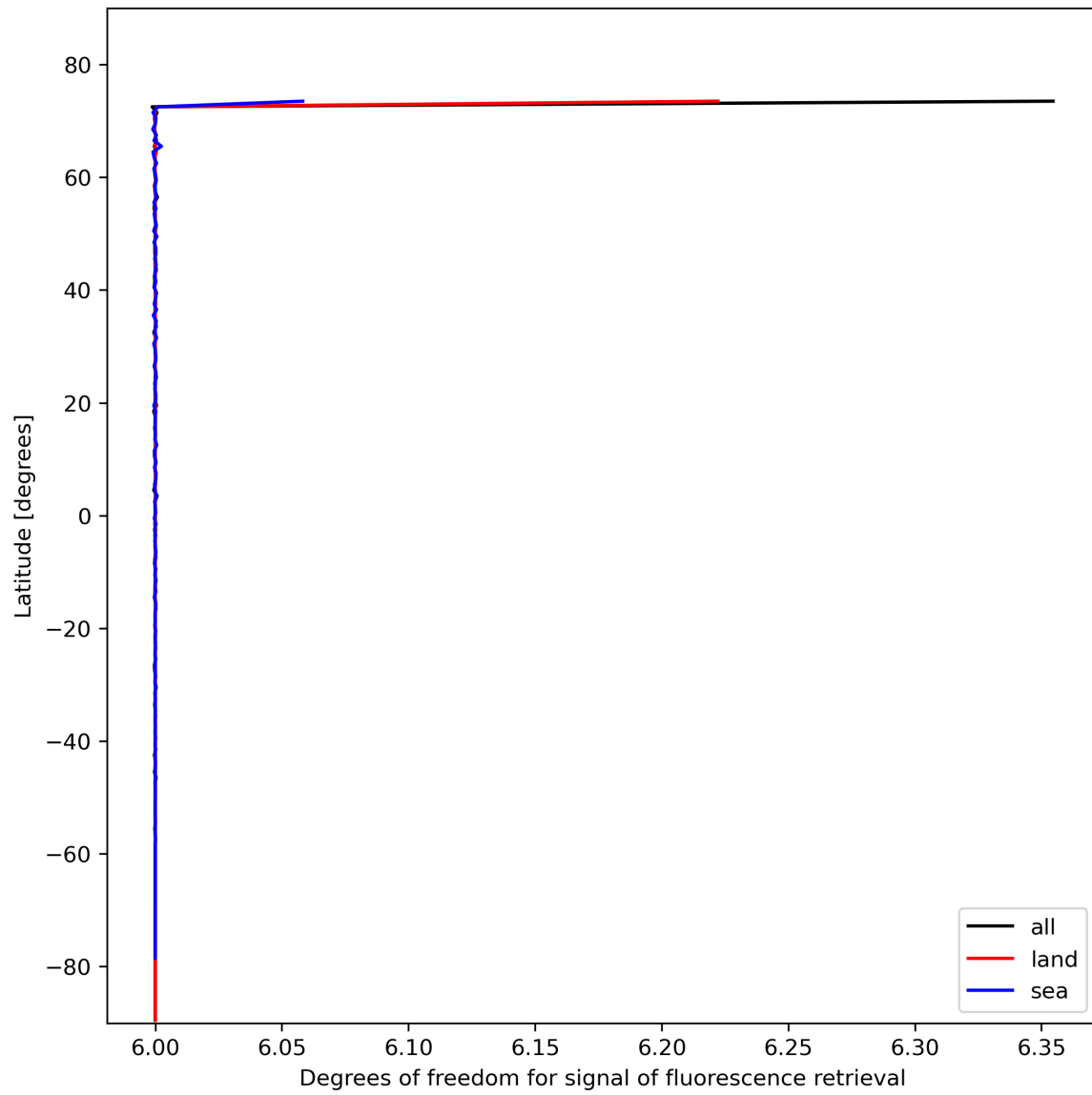
Figure 26: Zonal average of “Degrees of freedom for signal of fluorescence retrieval” for 2023-11-02 to 2023-11-04.
