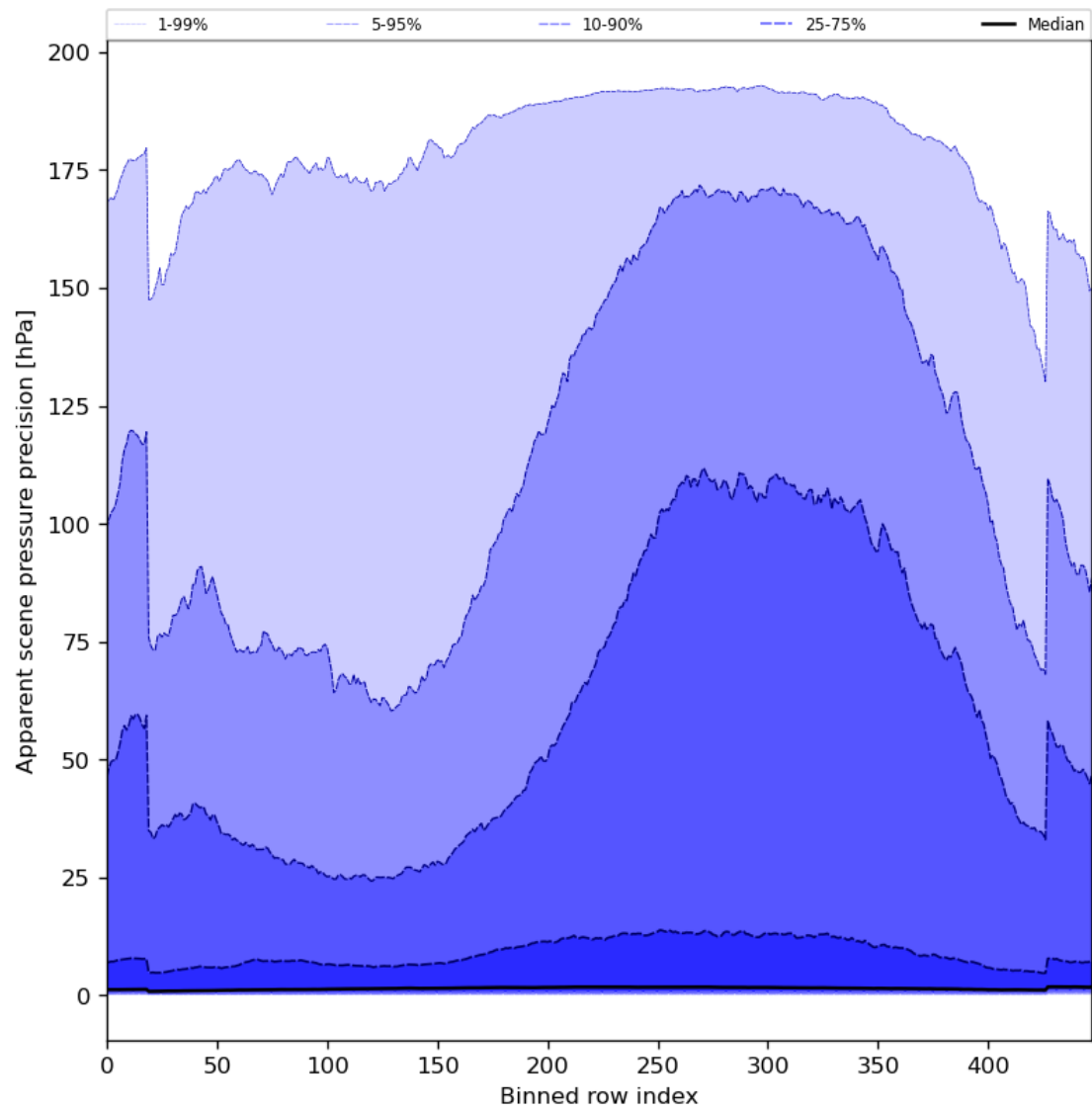
Figure 54: Along track statistics of “Apparent scene pressure precision” for 2023-11-02 to 2023-11-04
