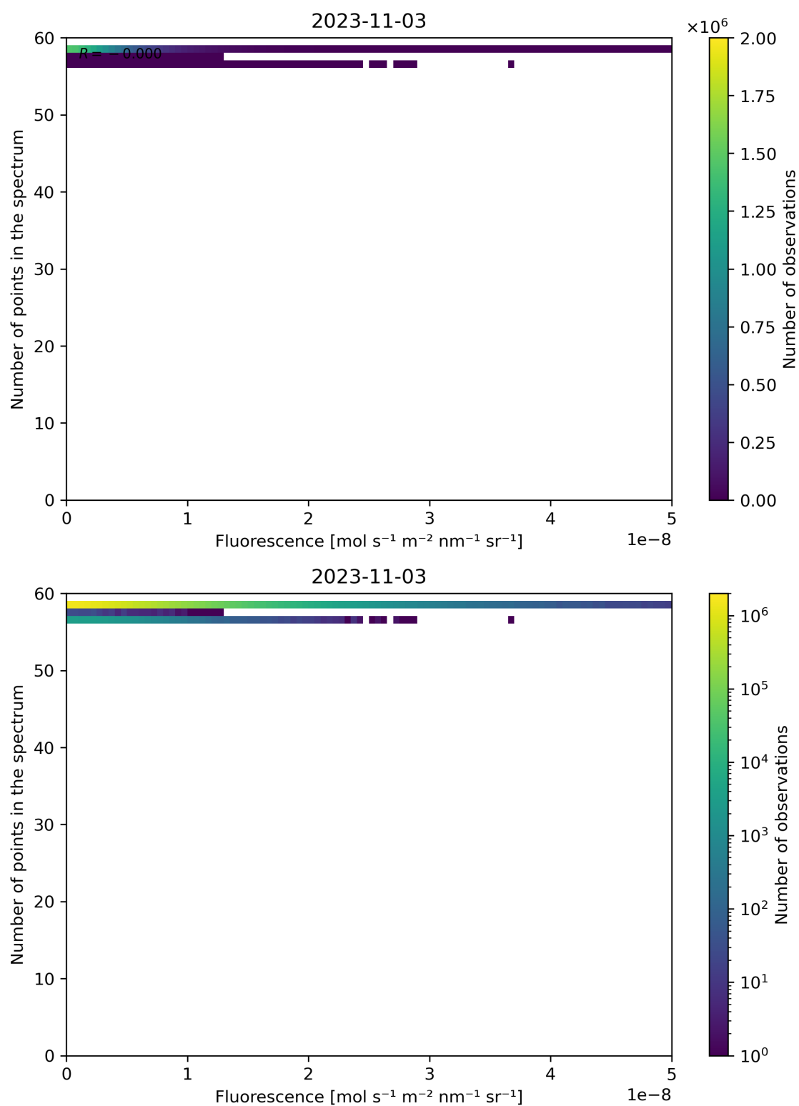
Figure 94: Scatter density plot of “Fluorescence” against “Number of points in the spectrum” for 2023-11-02 to 2023-11-04.
