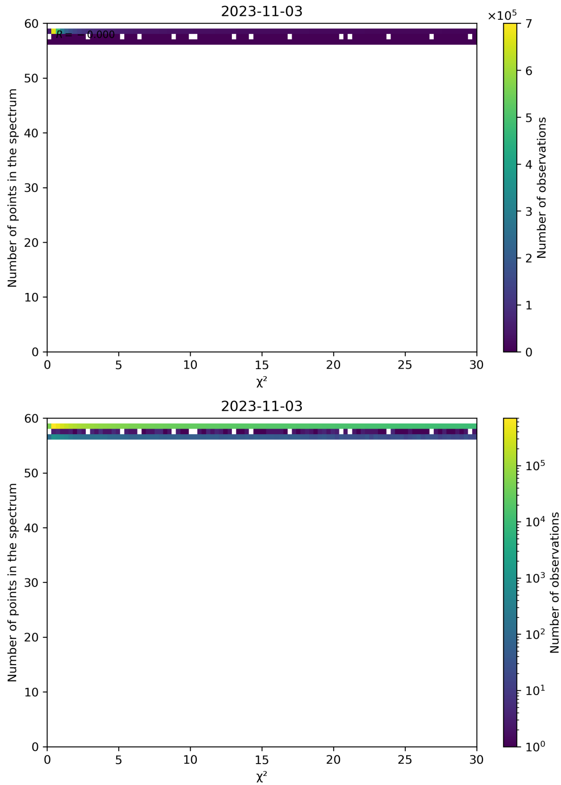
Figure 74: Scatter density plot of " \chi^2 " against "Number of points in the spectrum" for 2023-11-02 to 2023-11-04.
