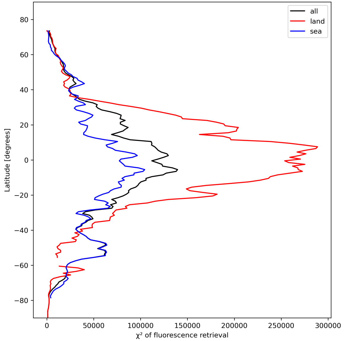
Figure 25: Zonal average of “ \chi^2 of fluorescence retrieval” for 2023-11-02 to 2023-11-04.
