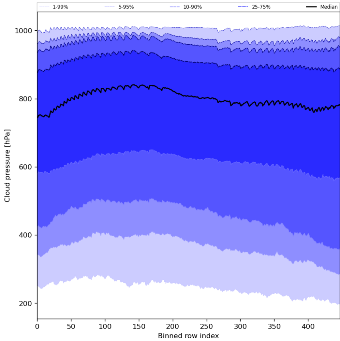
Figure 47: Along track statistics of “Cloud pressure” for 2023-11-02 to 2023-11-04
