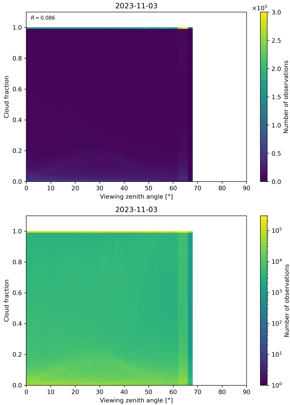
Figure 132: Scatter density plot of “Viewing zenith angle” against “Cloud fraction” for 2023-11-02 to 2023-11-04.
