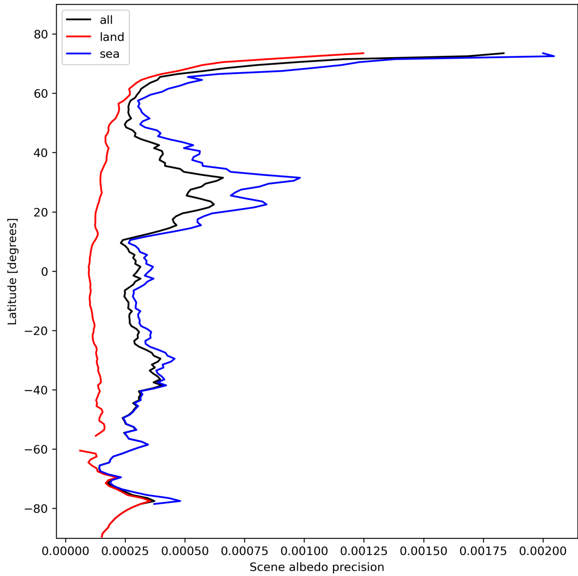
Figure 18: Zonal average of "Scene albedo precision" for 2023-11-02 to 2023-11-04.
