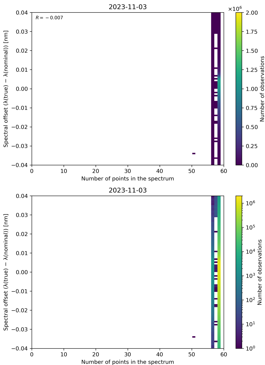
Figure 110: Scatter density plot of “Number of points in the spectrum” against “Spectral offset ( \lambda(\text{true}) - \lambda(\text{nominal}) )” for 2023-11-02 to 2023-11-04.
