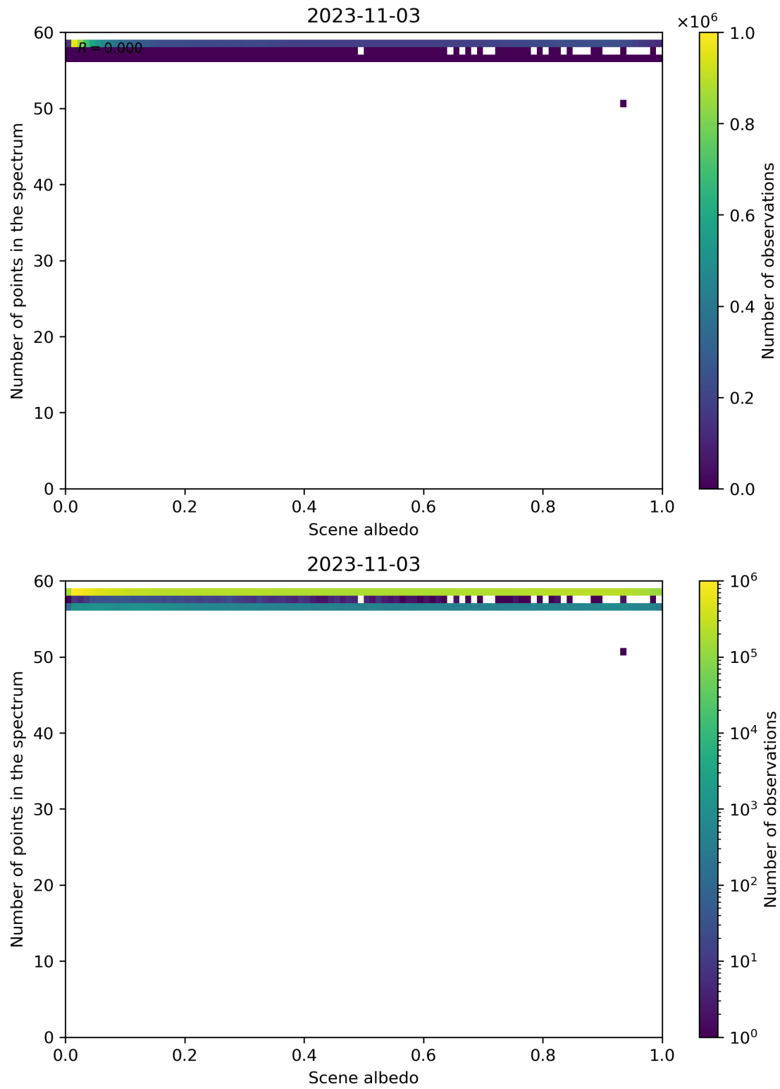
Figure 116: Scatter density plot of “Scene albedo” against “Number of points in the spectrum” for 2023-11-02 to 2023-11-04.
