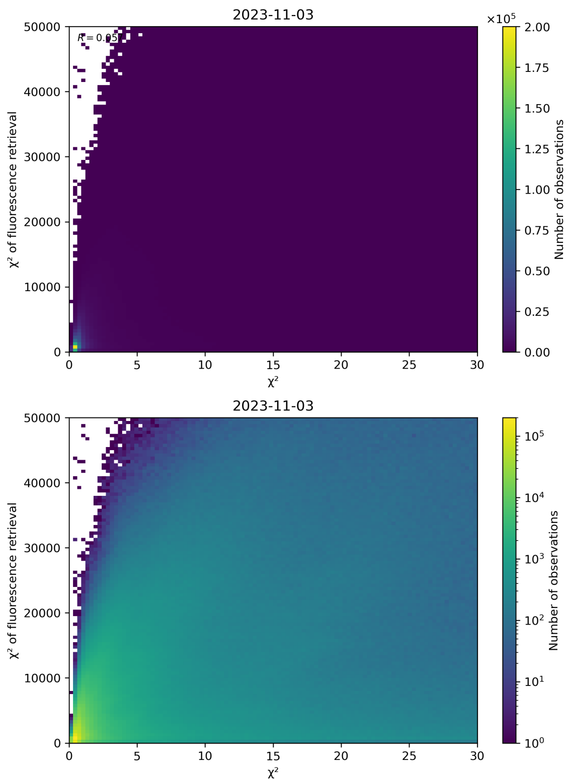
Figure 69: Scatter density plot of “ \chi^2 ” against “ \chi^2 of fluorescence retrieval” for 2023-11-02 to 2023-11-04.
