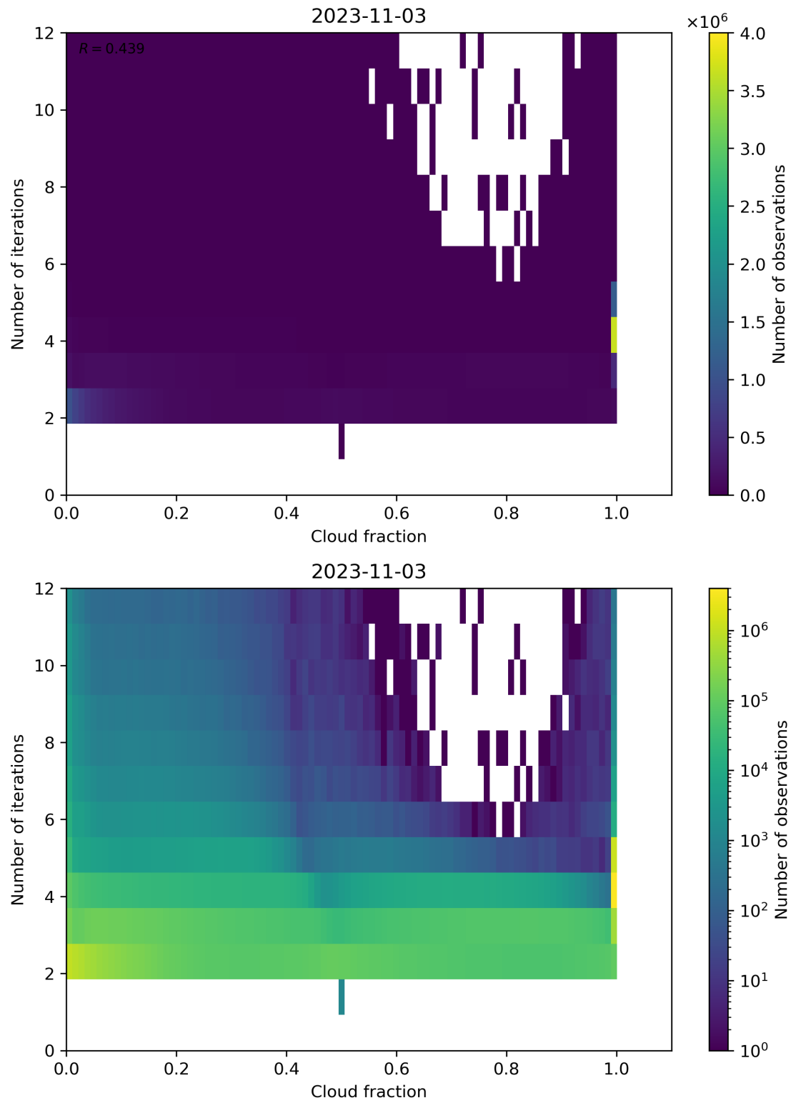
Figure 80: Scatter density plot of “Cloud fraction” against “Number of iterations” for 2023-11-02 to 2023-11-04.
