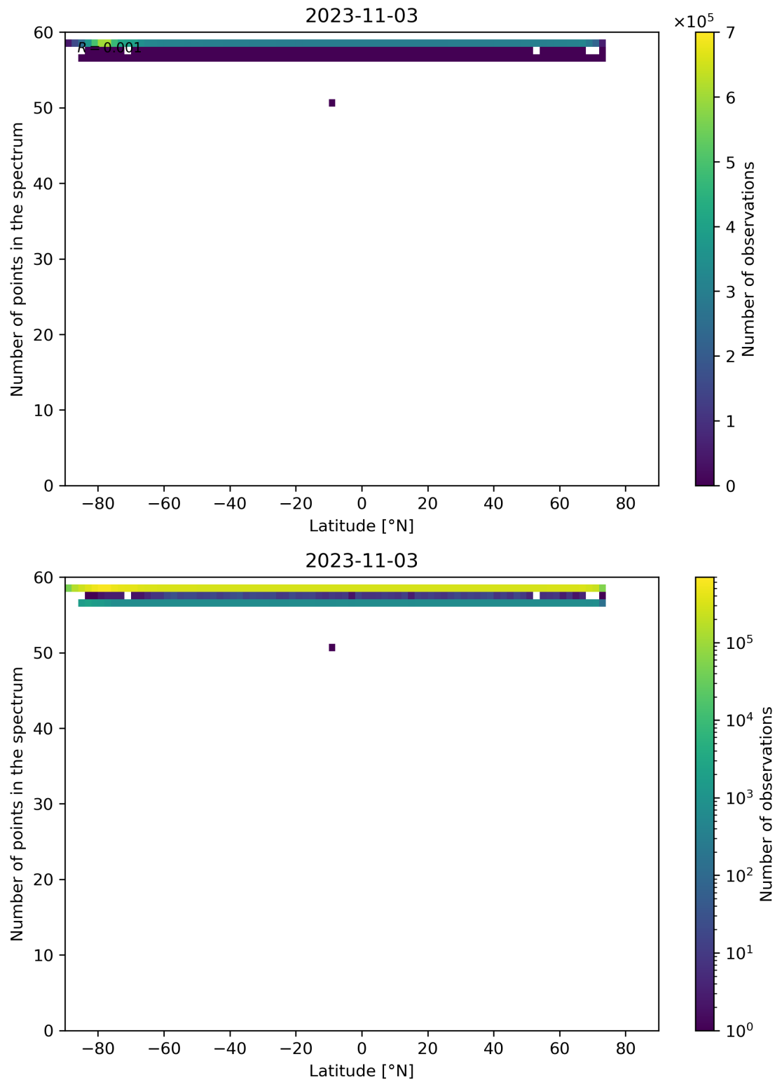
Figure 103: Scatter density plot of “Latitude” against “Number of points in the spectrum” for 2023-11-02 to 2023-11-04.
