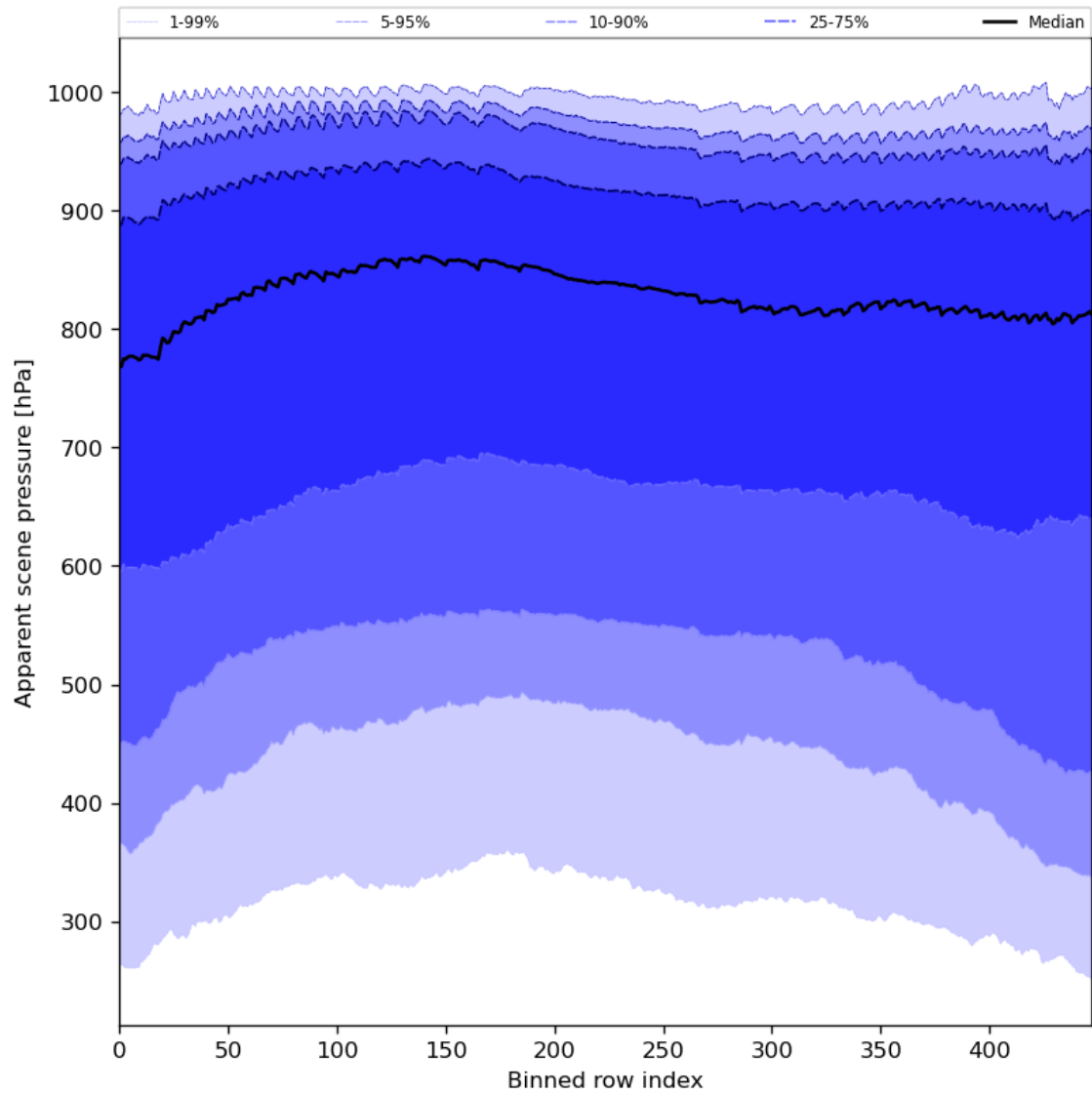
Figure 53: Along track statistics of “Apparent scene pressure” for 2023-11-02 to 2023-11-04
