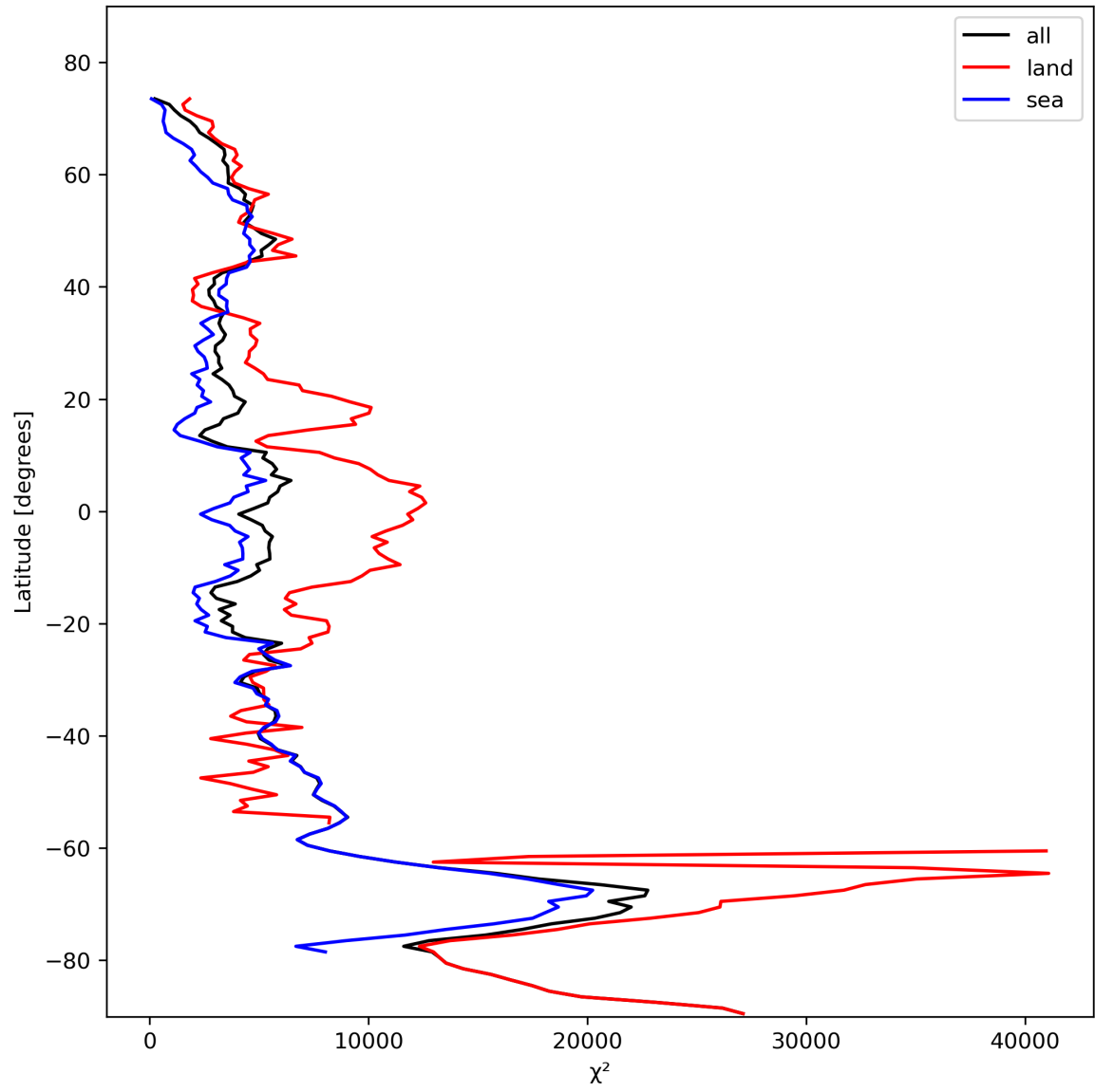
Figure 21: Zonal average of “ \chi^2 ” for 2023-11-02 to 2023-11-04.
