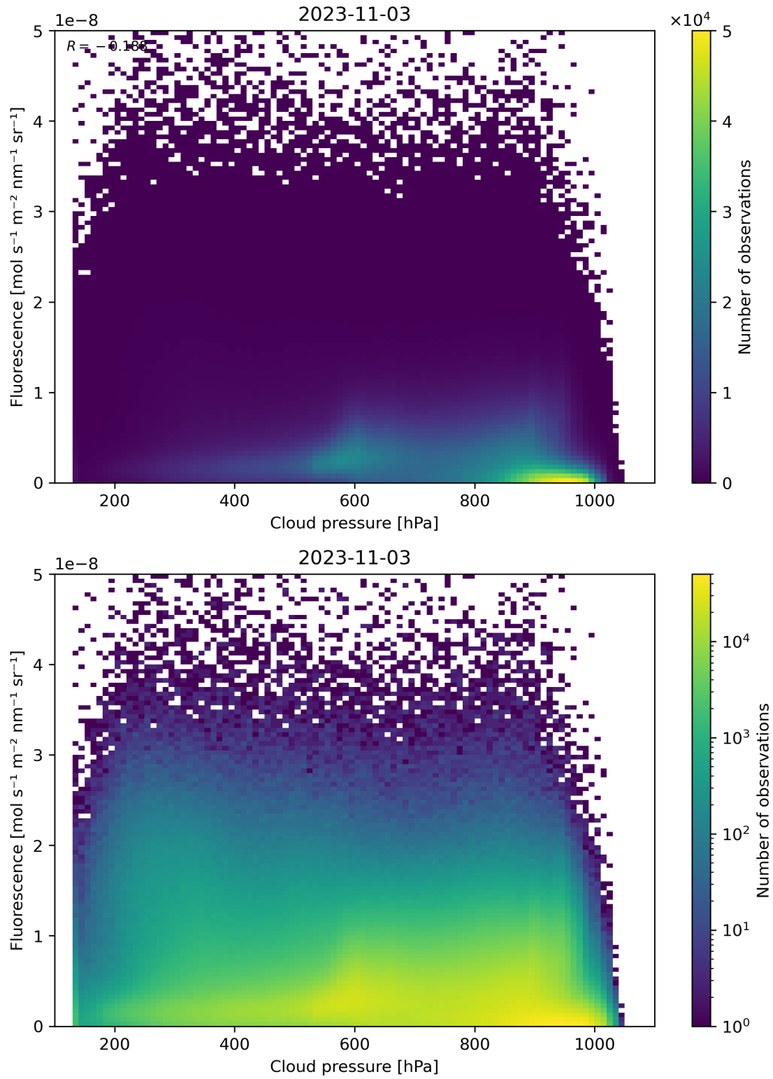
Figure 88: Scatter density plot of “Cloud pressure” against “Fluorescence” for 2023-11-02 to 2023-11-04.
