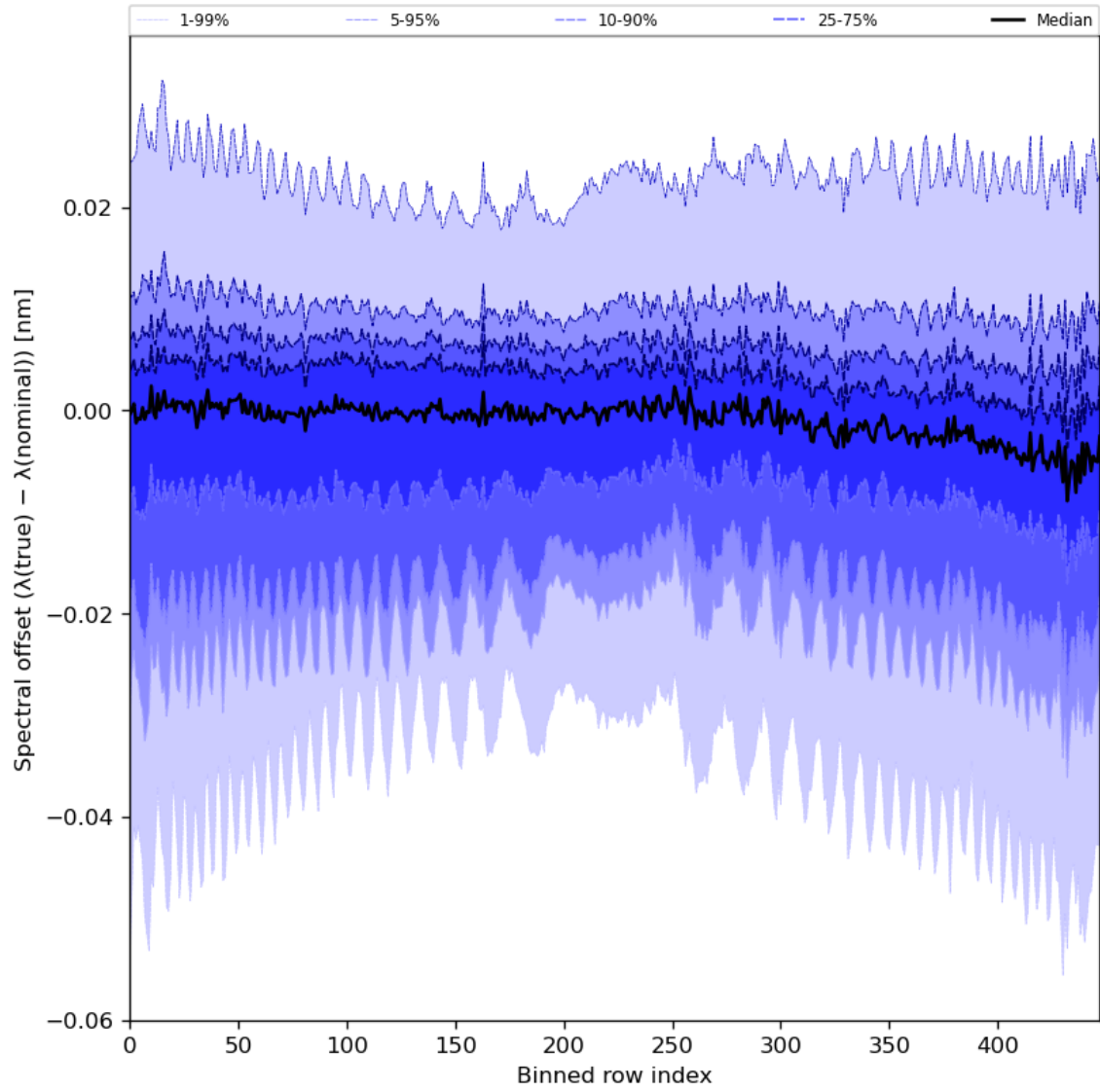
Figure 62: Along track statistics of “Spectral offset ( \lambda(\text{true}) - \lambda(\text{nominal}) )” for 2023-11-02 to 2023-11-04
