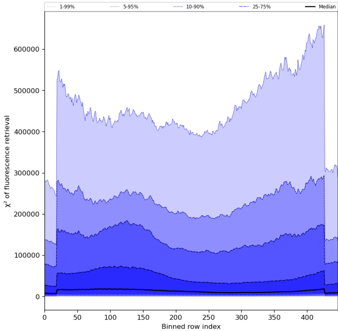
Figure 59: Along track statistics of “ \chi^2 of fluorescence retrieval” for 2023-11-02 to 2023-11-04
