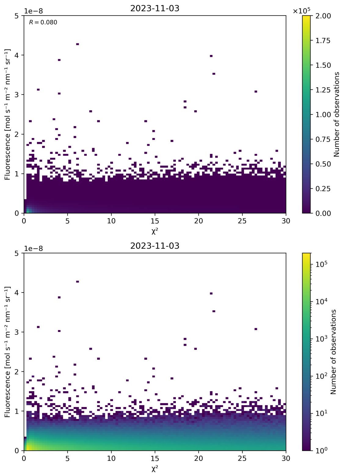
Figure 70: Scatter density plot of “ \chi^2 ” against “Fluorescence” for 2023-11-02 to 2023-11-04.
