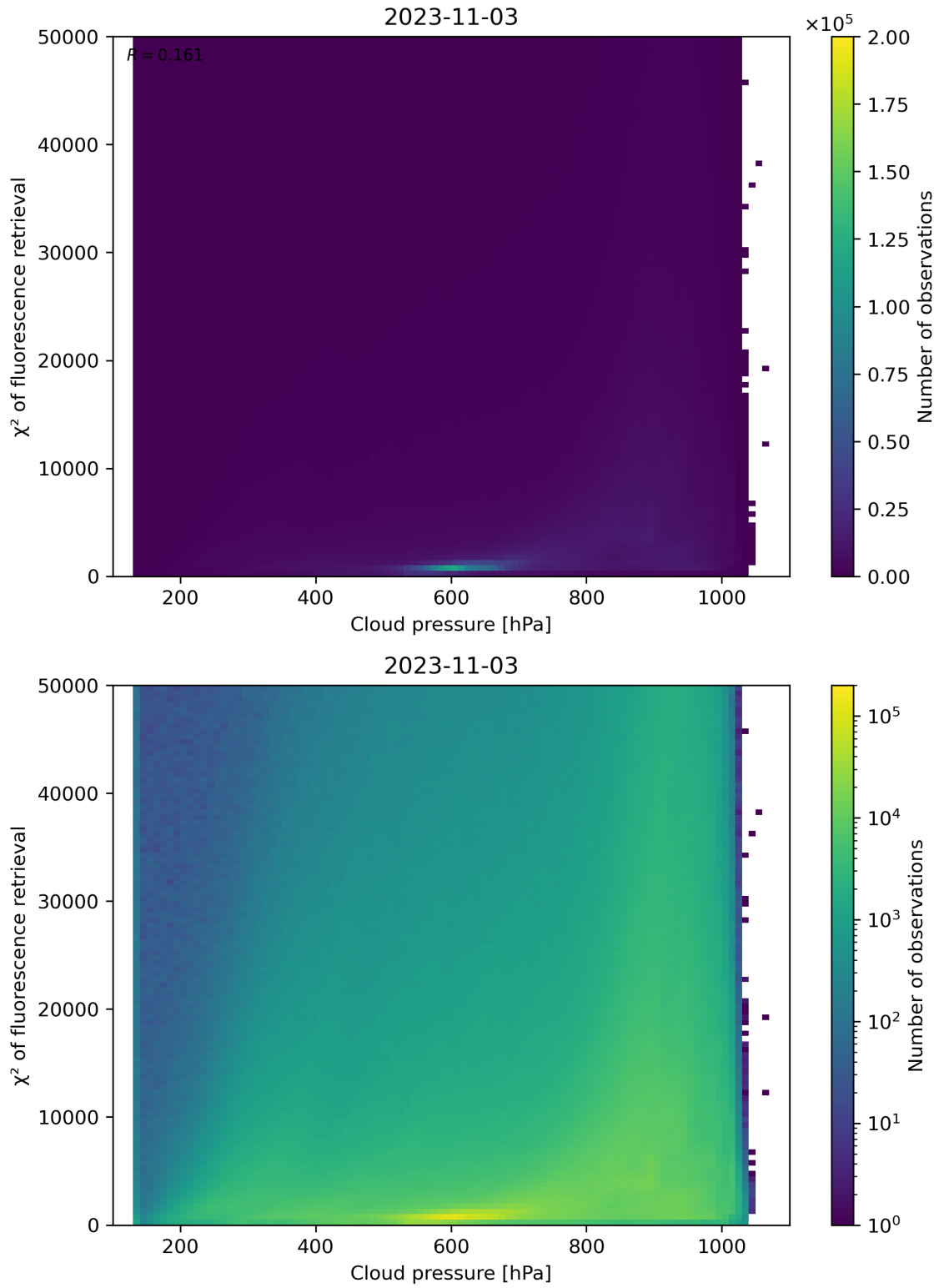
Figure 86: Scatter density plot of “Cloud pressure” against “ \chi^2 of fluorescence retrieval” for 2023-11-02 to 2023-11-04.
