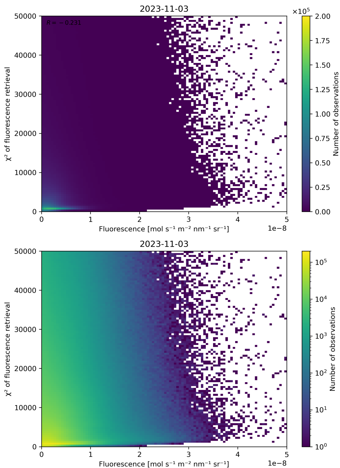
Figure 93: Scatter density plot of “Fluorescence” against “ \chi^2 of fluorescence retrieval” for 2023-11-02 to 2023-11-04.
