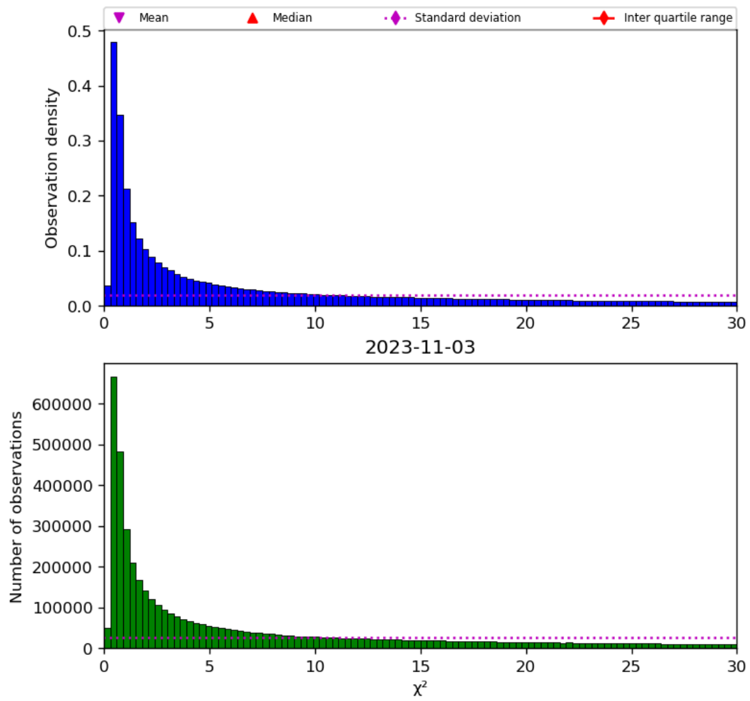
Figure 38: Histogram of " \chi^2 " for 2023-11-02 to 2023-11-04
