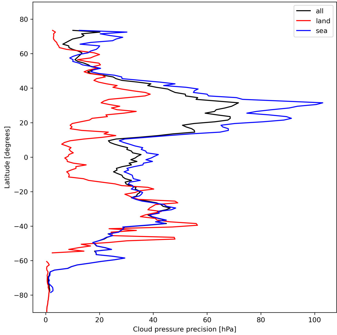
Figure 14: Zonal average of “Cloud pressure precision” for 2023-11-02 to 2023-11-04.
