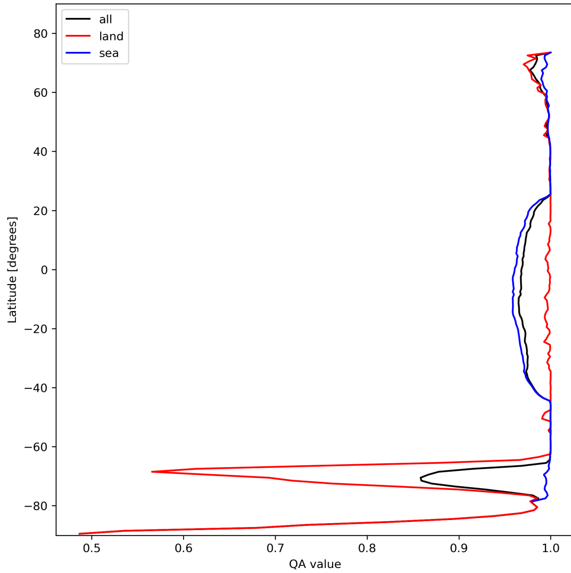
Figure 12: Zonal average of “QA value” for 2023-11-02 to 2023-11-04.
