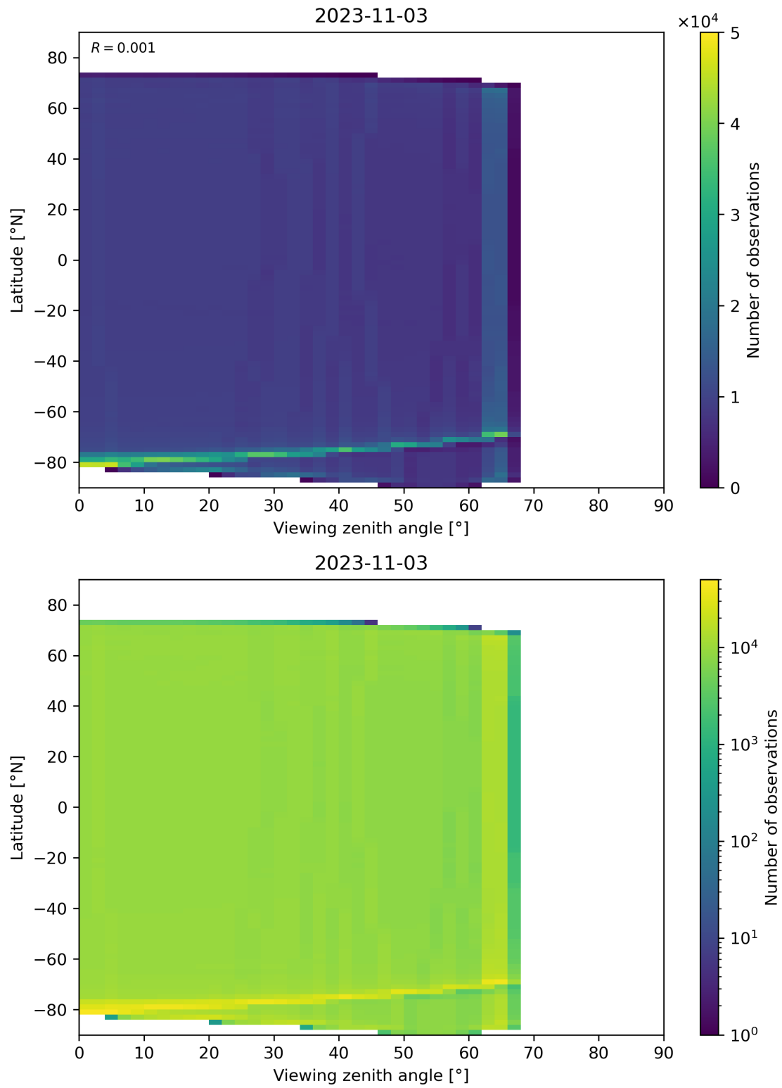
Figure 135: Scatter density plot of “Viewing zenith angle” against “Latitude” for 2023-11-02 to 2023-11-04.
