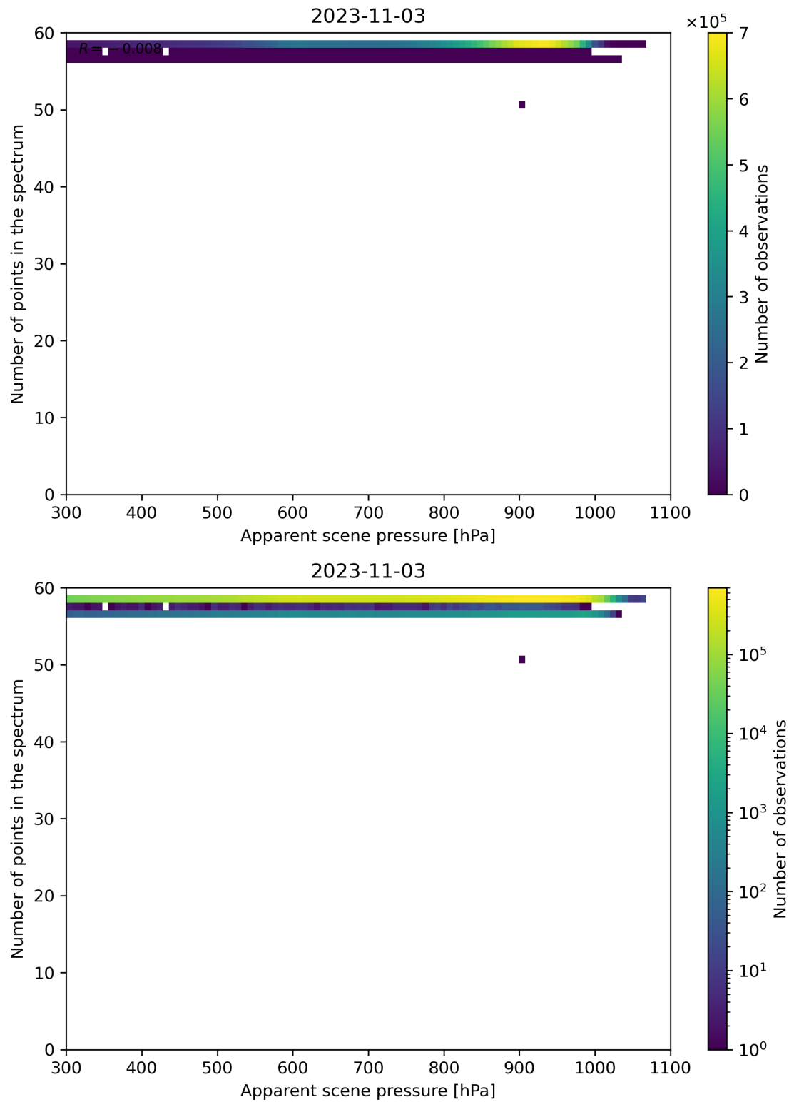
Figure 67: Scatter density plot of “Apparent scene pressure” against “Number of points in the spectrum” for 2023-11-02 to 2023-11-04.
