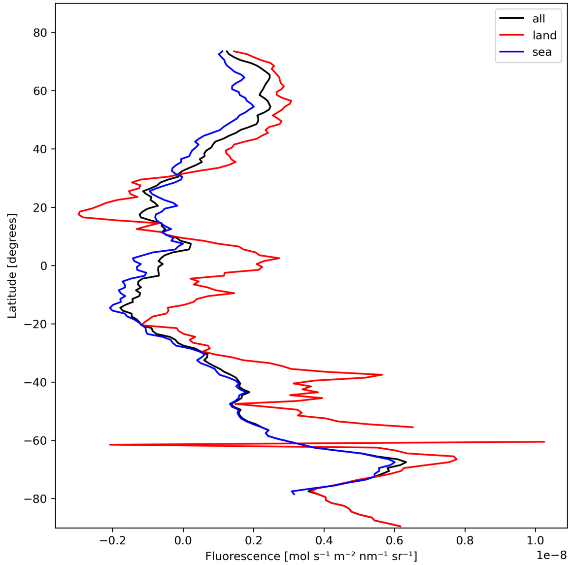
Figure 23: Zonal average of “Fluorescence” for 2023-11-02 to 2023-11-04.
