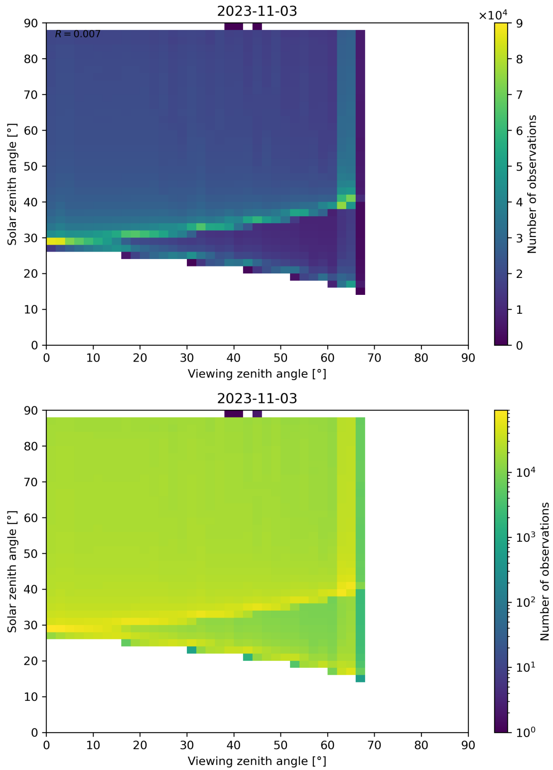
Figure 139: Scatter density plot of “Viewing zenith angle” against “Solar zenith angle” for 2023-11-02 to 2023-11-04.
