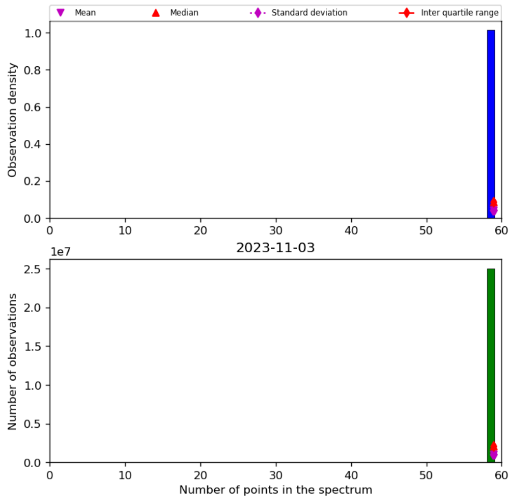
Figure 44: Histogram of “Number of points in the spectrum” for 2023-11-02 to 2023-11-04
