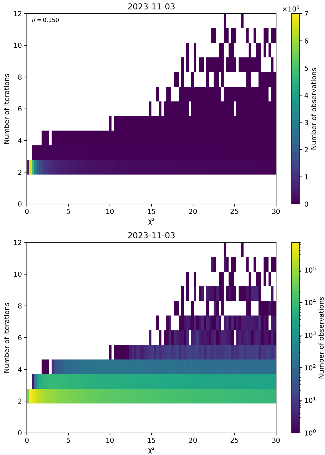
Figure 73: Scatter density plot of “ \chi^2 ” against “Number of iterations” for 2023-11-02 to 2023-11-04.
