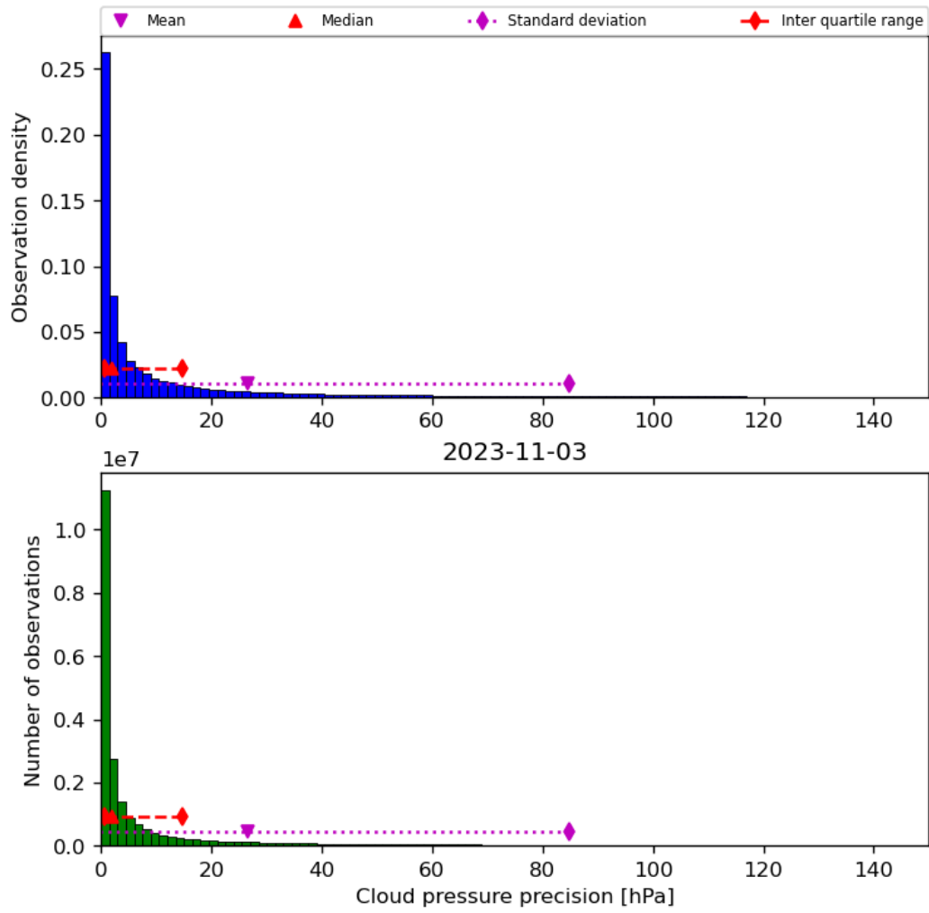
Figure 31: Histogram of “Cloud pressure precision” for 2023-11-02 to 2023-11-04
