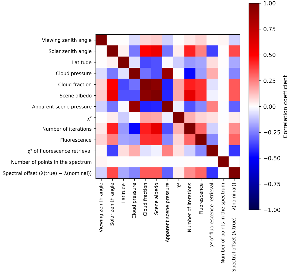
Figure 2: Map of correlation matrix for 2023-11-02 to 2023-11-04.
