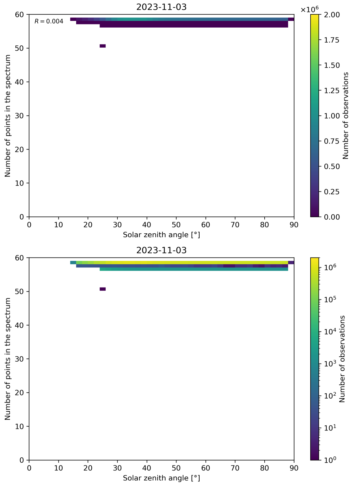
Figure 126: Scatter density plot of “Solar zenith angle” against “Number of points in the spectrum” for 2023-11-02 to 2023-11-04.
