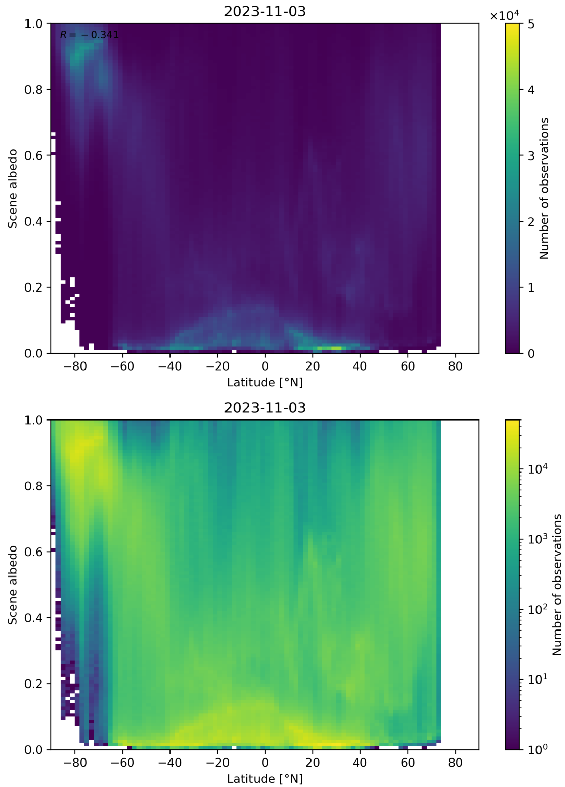
Figure 104: Scatter density plot of “Latitude” against “Scene albedo” for 2023-11-02 to 2023-11-04.
