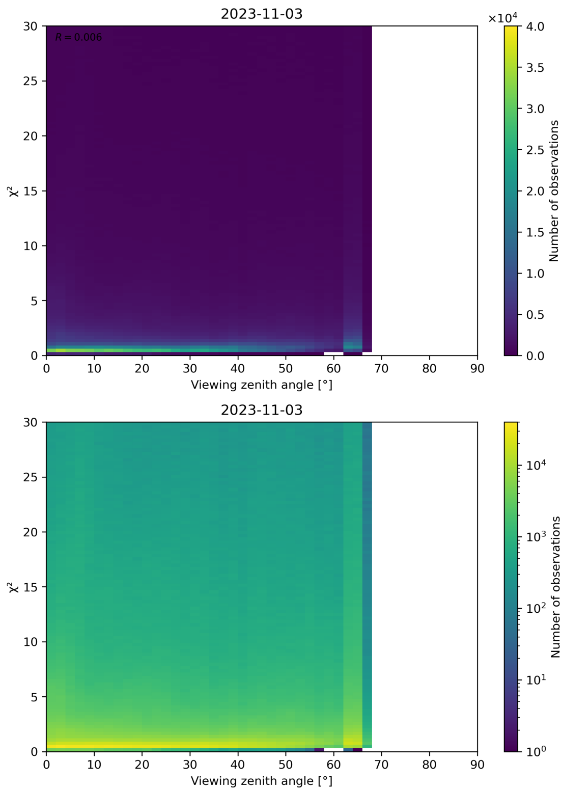
Figure 130: Scatter density plot of “Viewing zenith angle” against “ \chi^2 ” for 2023-11-02 to 2023-11-04.
