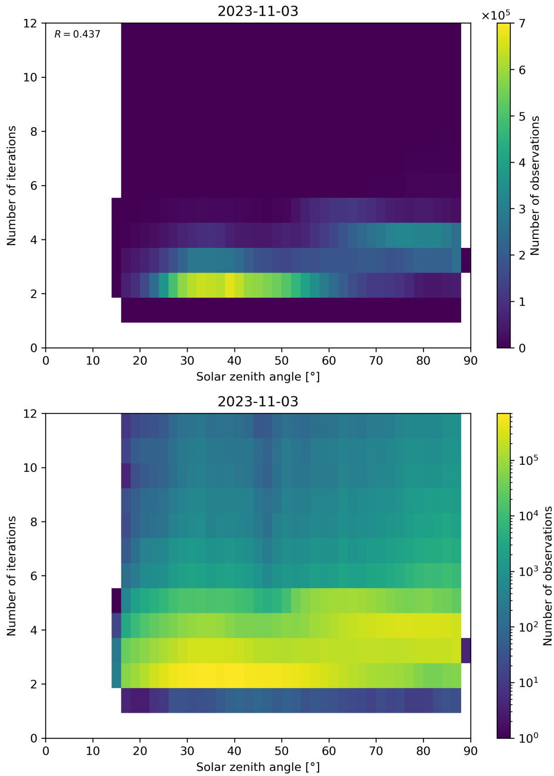
Figure 125: Scatter density plot of “Solar zenith angle” against “Number of iterations” for 2023-11-02 to 2023-11-04.
