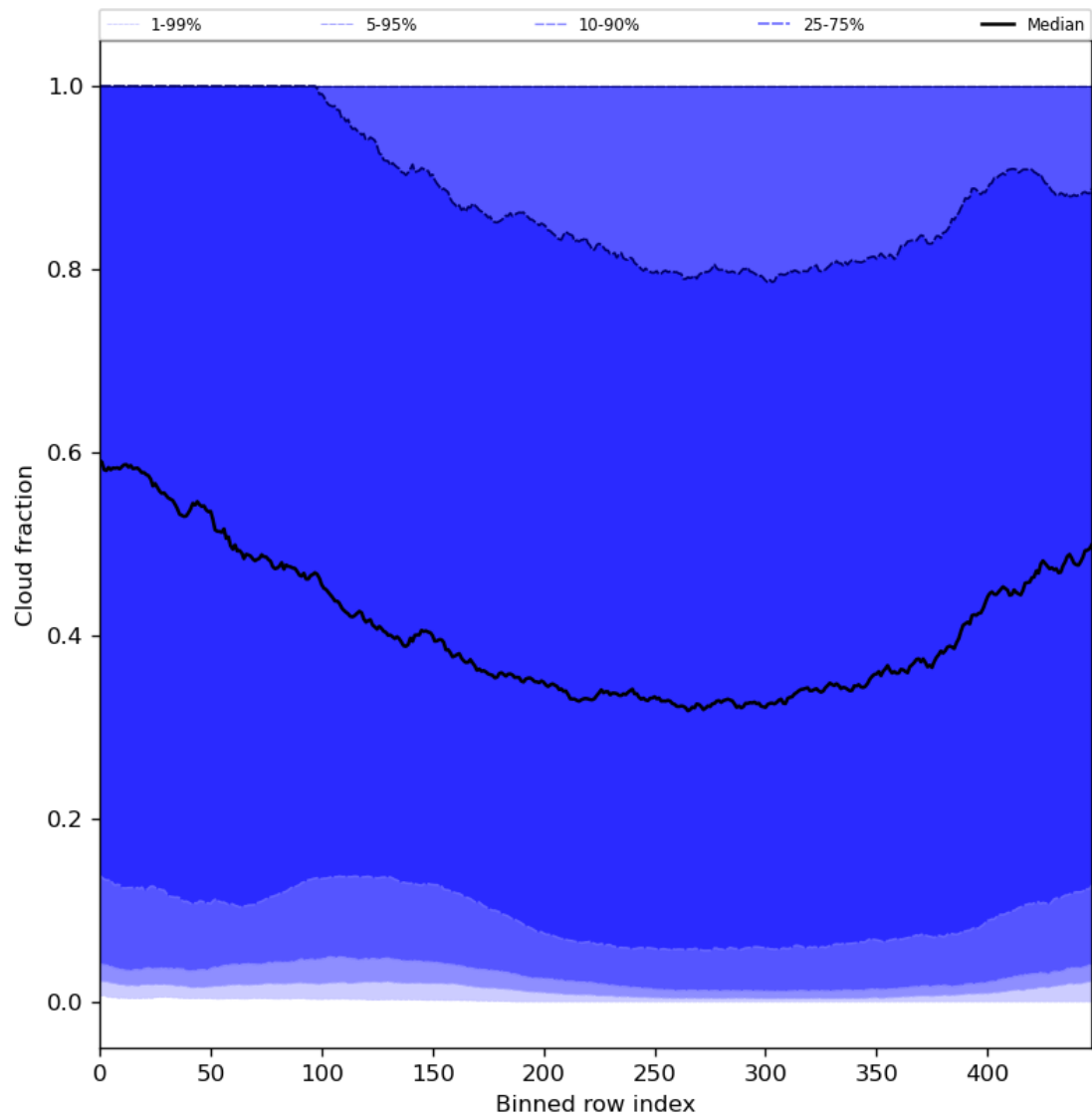
Figure 49: Along track statistics of “Cloud fraction” for 2023-11-02 to 2023-11-04
