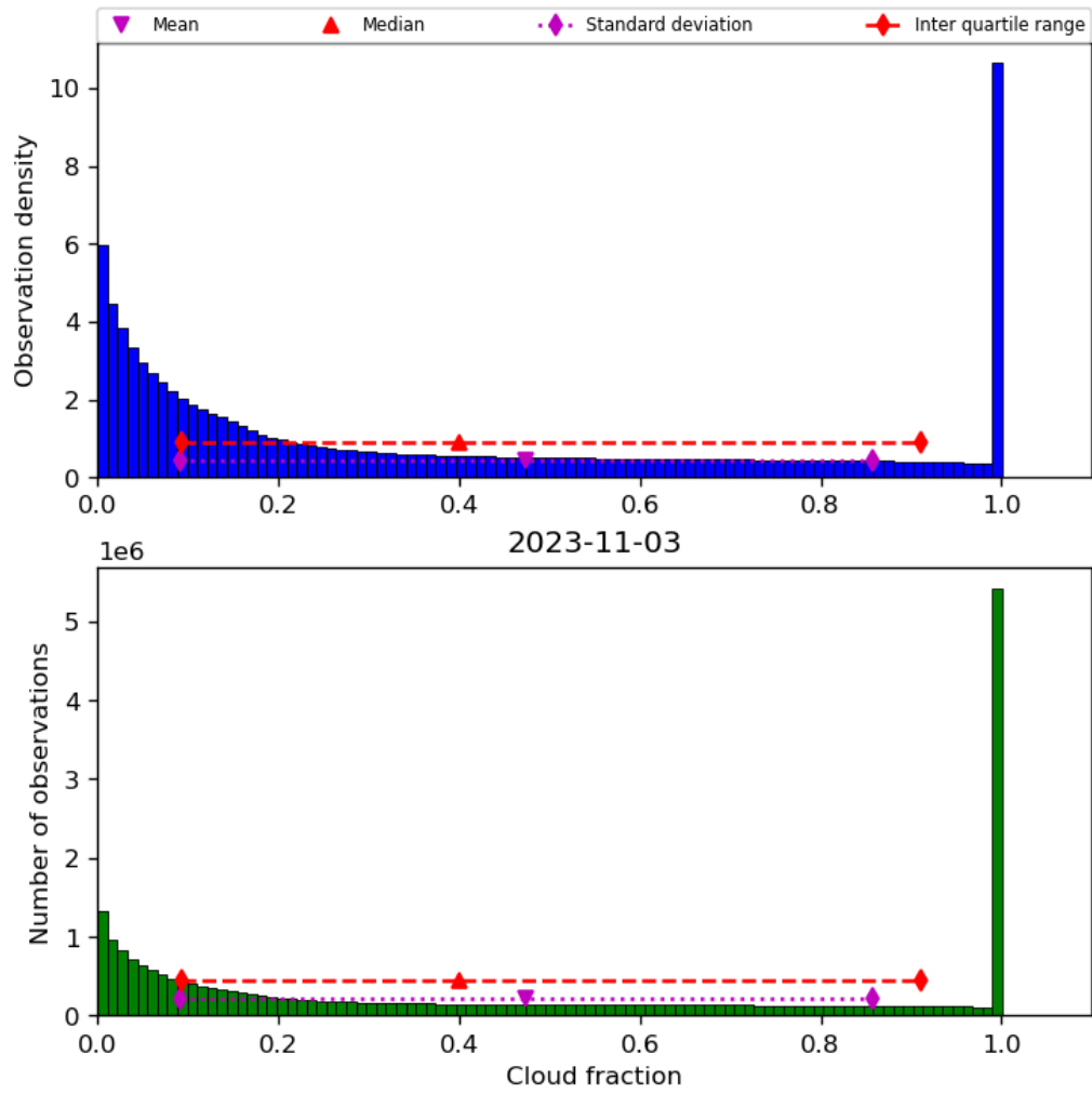
Figure 32: Histogram of “Cloud fraction” for 2023-11-02 to 2023-11-04
