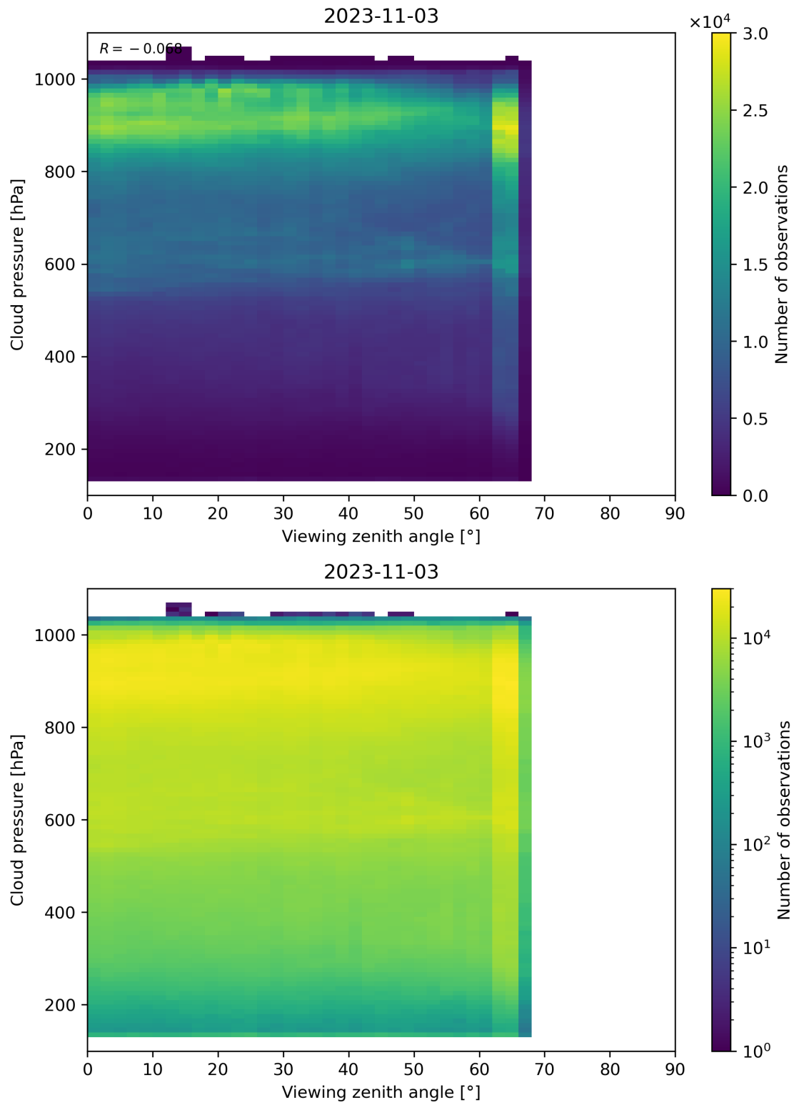
Figure 133: Scatter density plot of “Viewing zenith angle” against “Cloud pressure” for 2023-11-02 to 2023-11-04.
