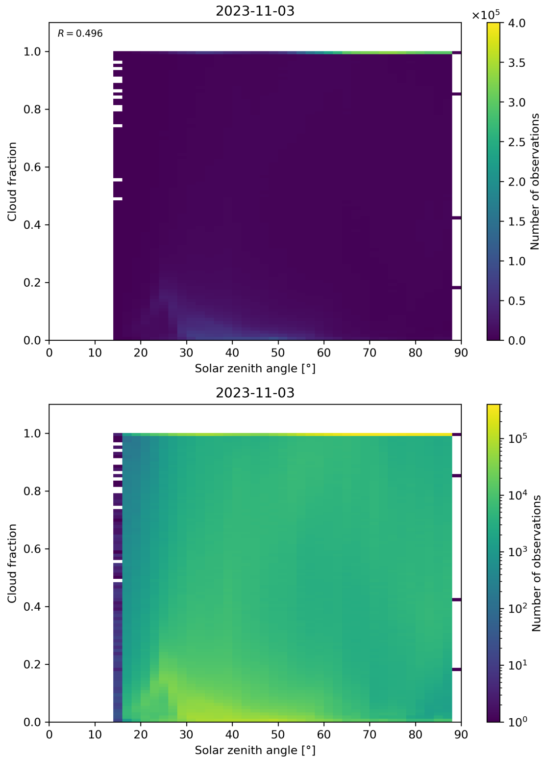
Figure 121: Scatter density plot of “Solar zenith angle” against “Cloud fraction” for 2023-11-02 to 2023-11-04.
