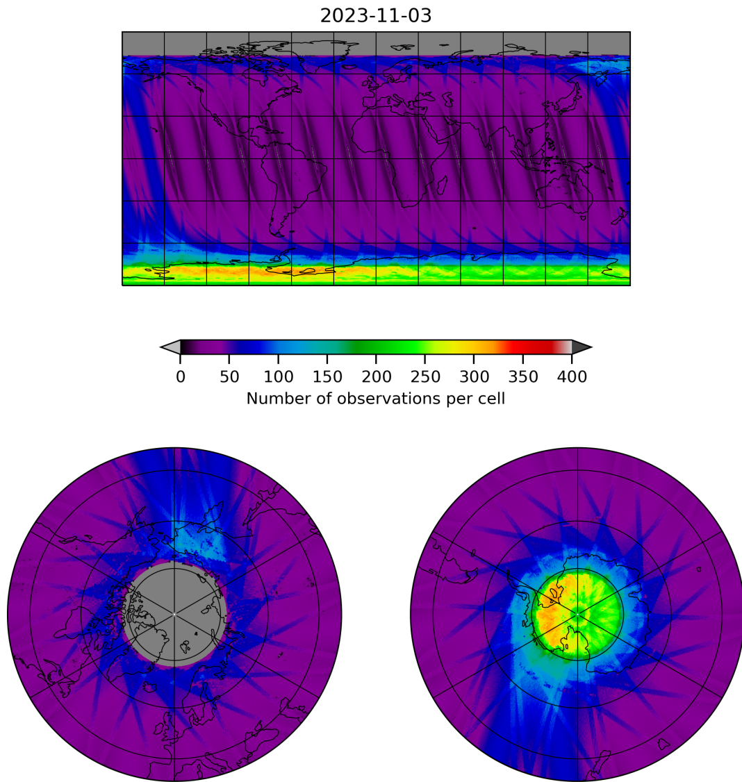
Figure 11: Map of the number of observations for 2023-11-02 to 2023-11-04
