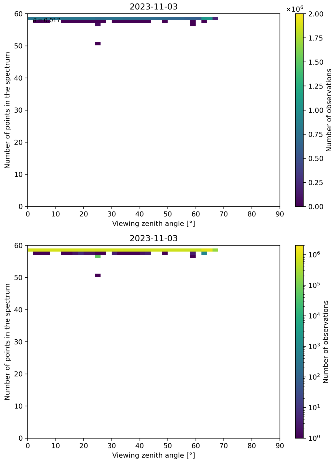
Figure 137: Scatter density plot of “Viewing zenith angle” against “Number of points in the spectrum” for 2023-11-02 to 2023-11-04.
