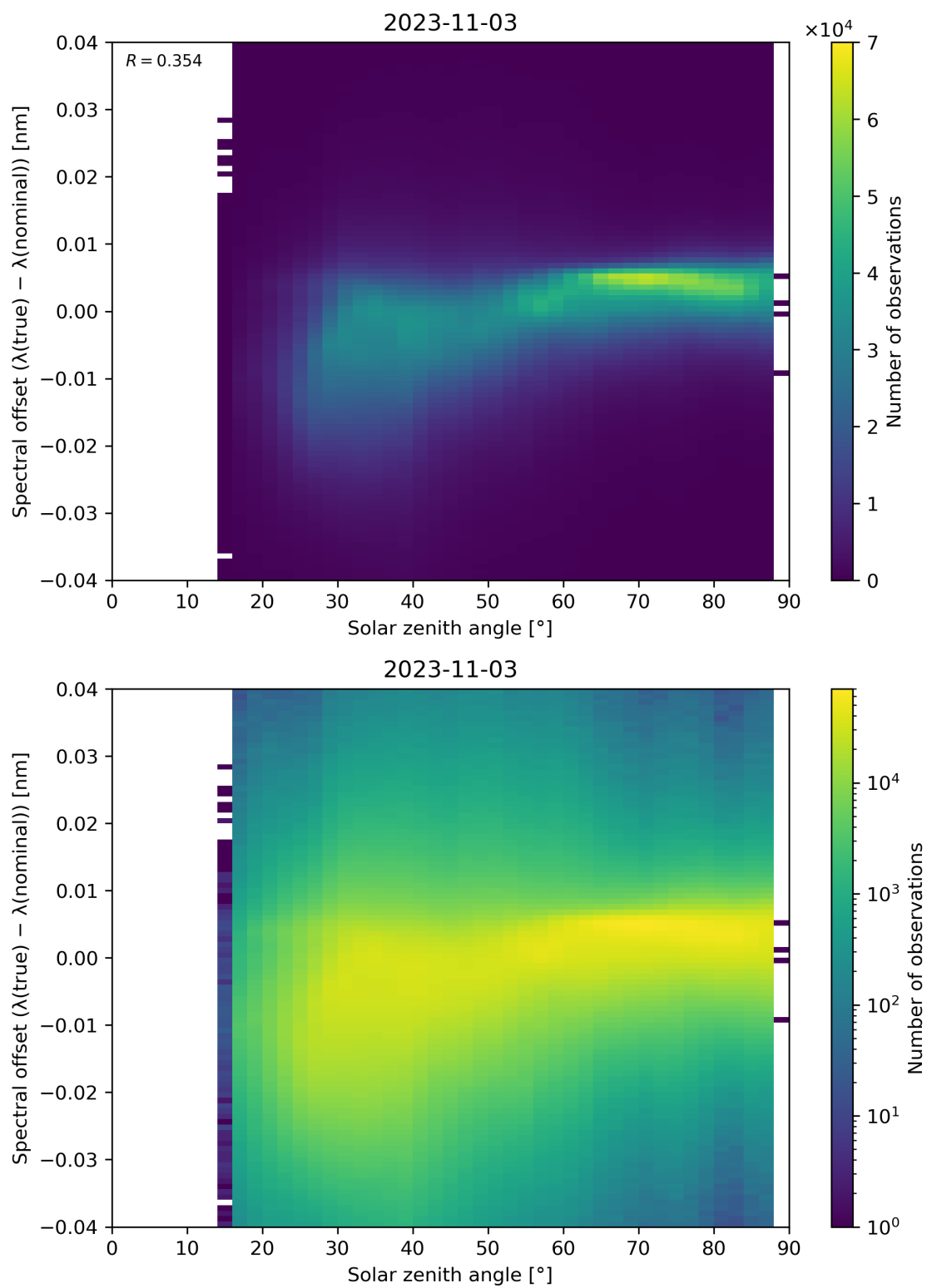
Figure 128: Scatter density plot of “Solar zenith angle” against “Spectral offset ( \lambda(\text{true}) - \lambda(\text{nominal}) )” for 2023-11-02 to 2023-11-04.
