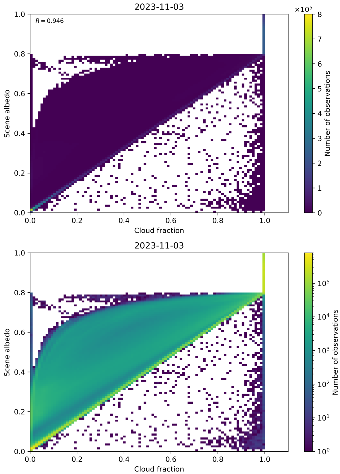
Figure 82: Scatter density plot of “Cloud fraction” against “Scene albedo” for 2023-11-02 to 2023-11-04.
