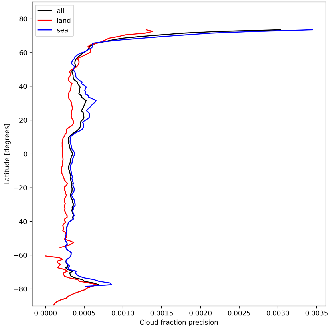
Figure 16: Zonal average of “Cloud fraction precision” for 2023-11-02 to 2023-11-04.
