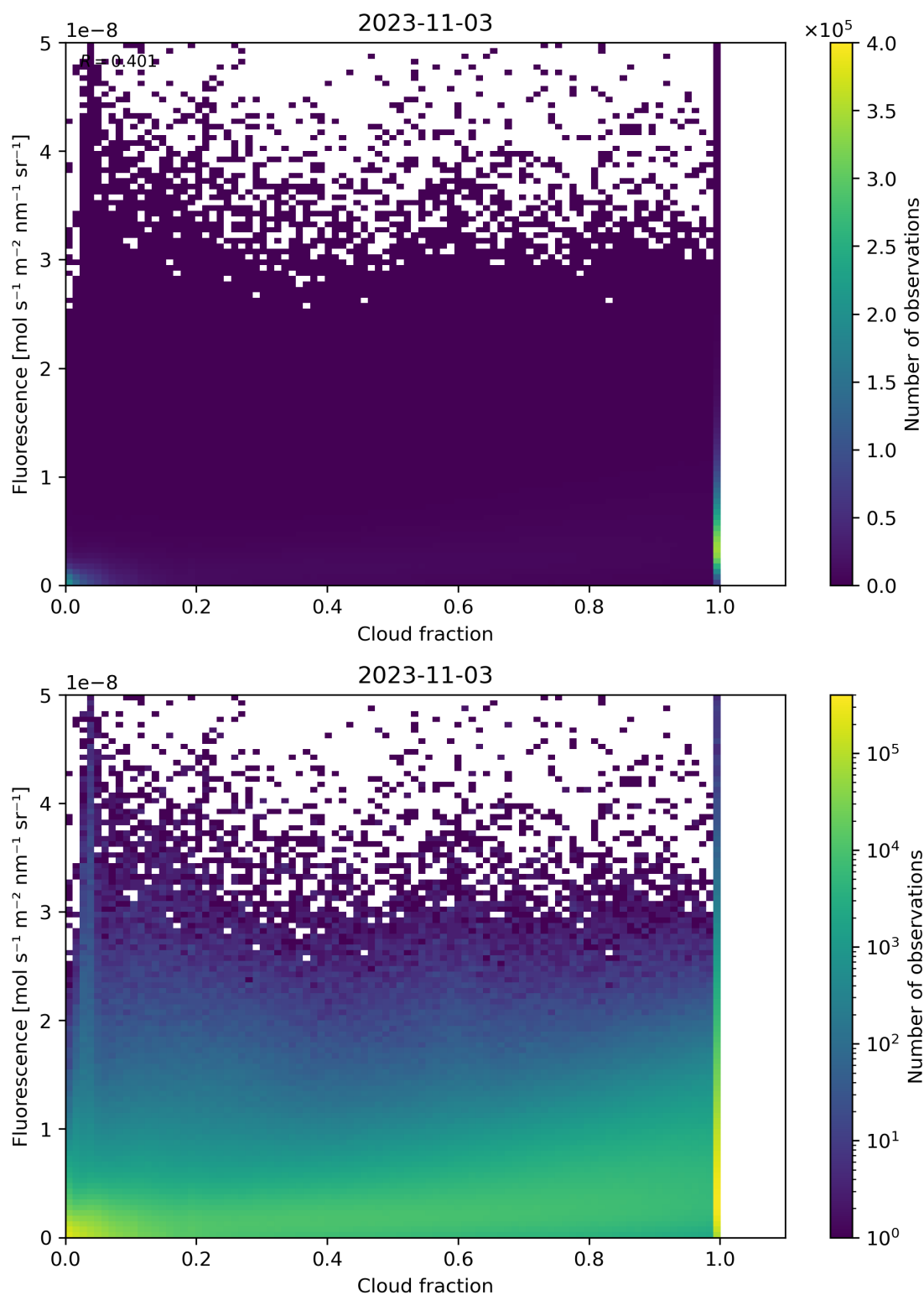
Figure 79: Scatter density plot of “Cloud fraction” against “Fluorescence” for 2023-11-02 to 2023-11-04.
