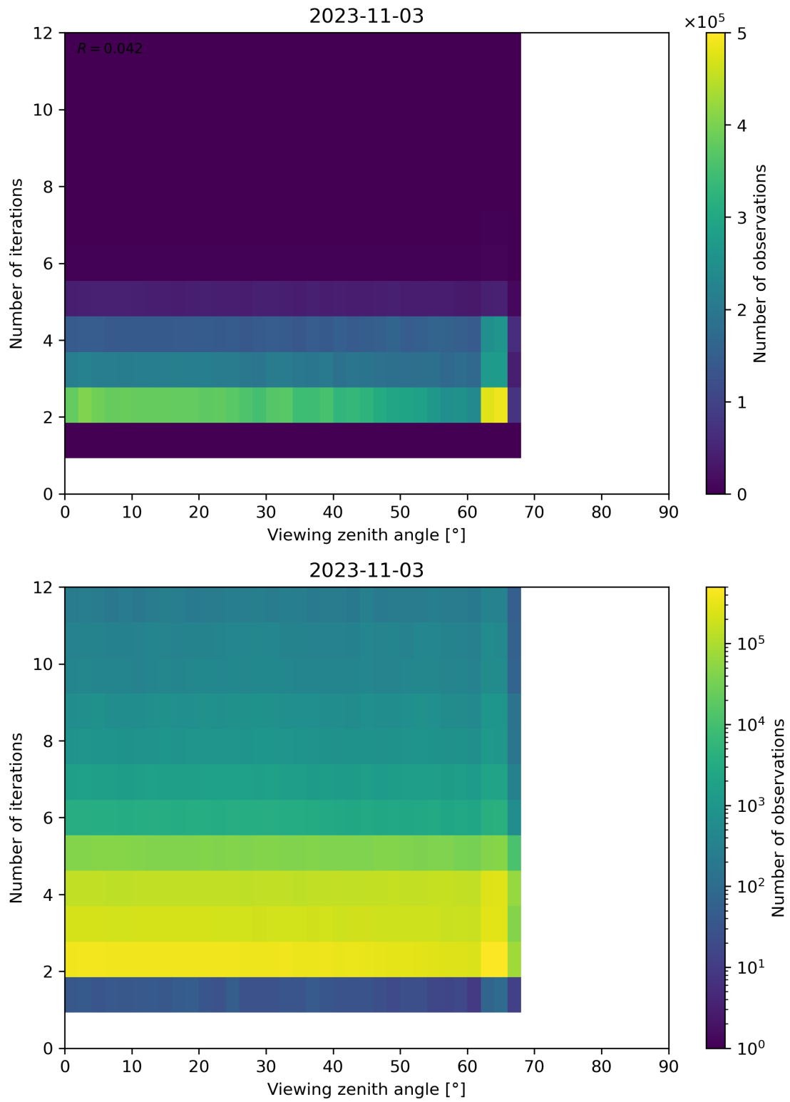
Figure 136: Scatter density plot of “Viewing zenith angle” against “Number of iterations” for 2023-11-02 to 2023-11-04.
