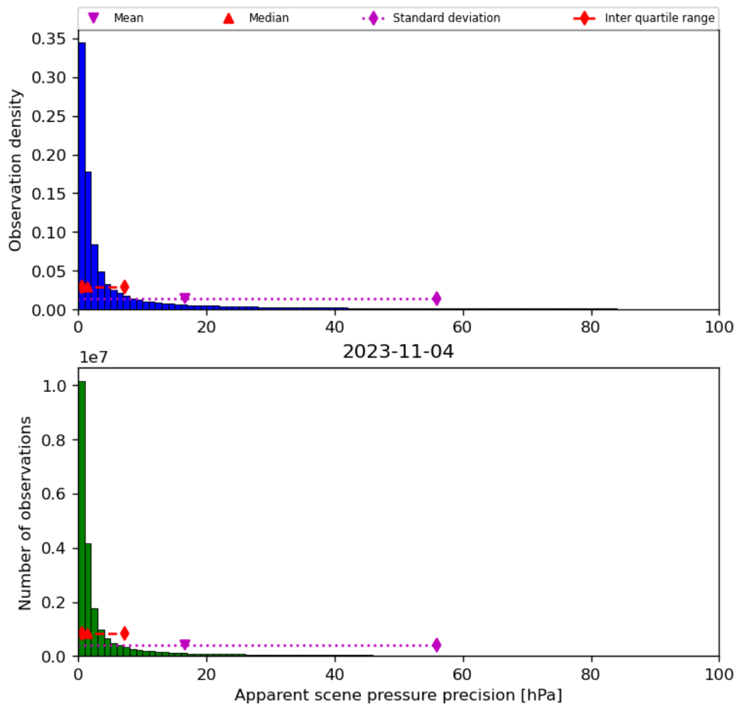
Figure 37: Histogram of “Apparent scene pressure precision” for 2023-11-03 to 2023-11-05
