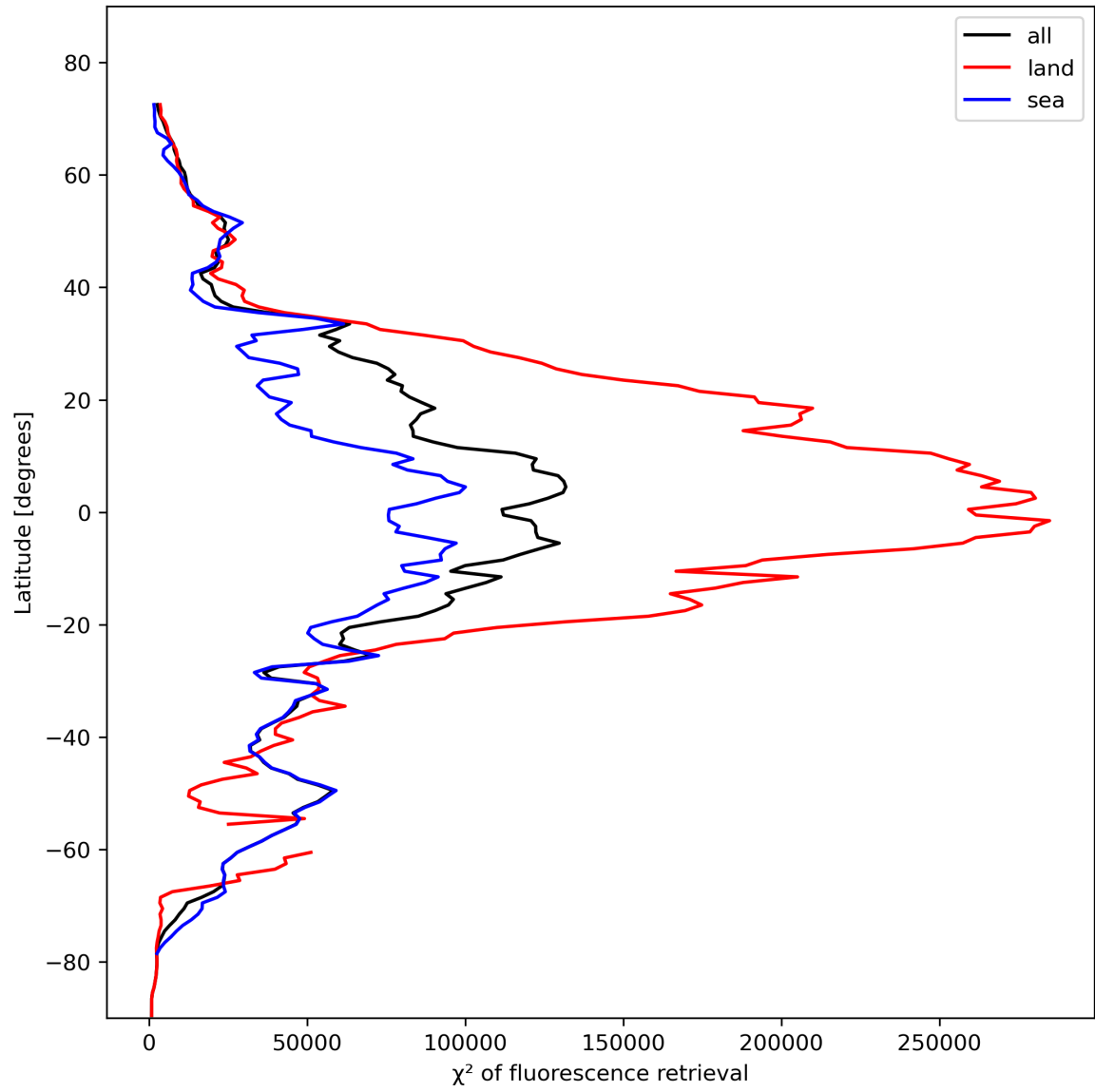
Figure 25: Zonal average of “ \chi^2 of fluorescence retrieval” for 2023-11-03 to 2023-11-05.
