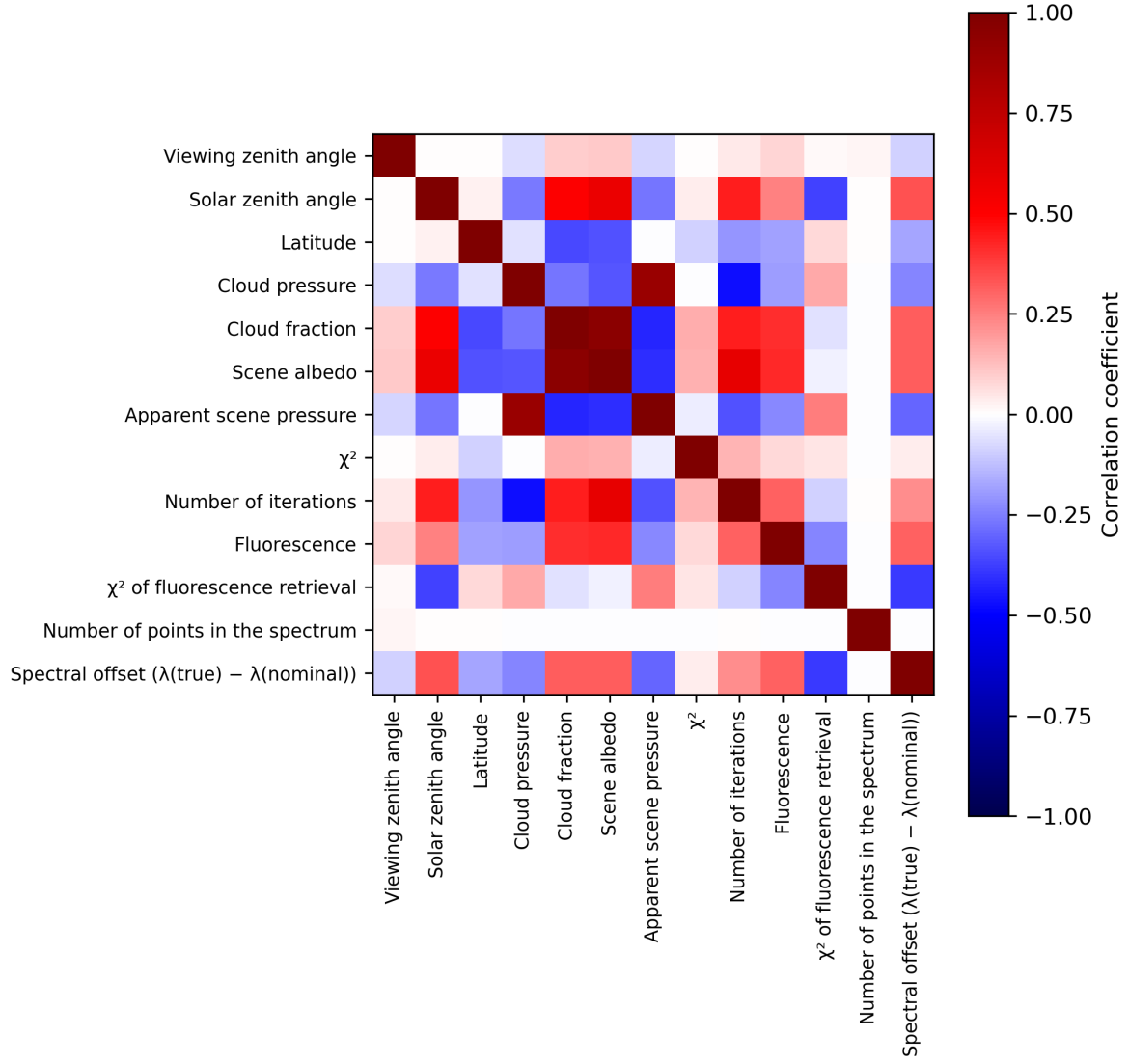
Figure 2: Map of correlation matrix for 2023-11-03 to 2023-11-05.
