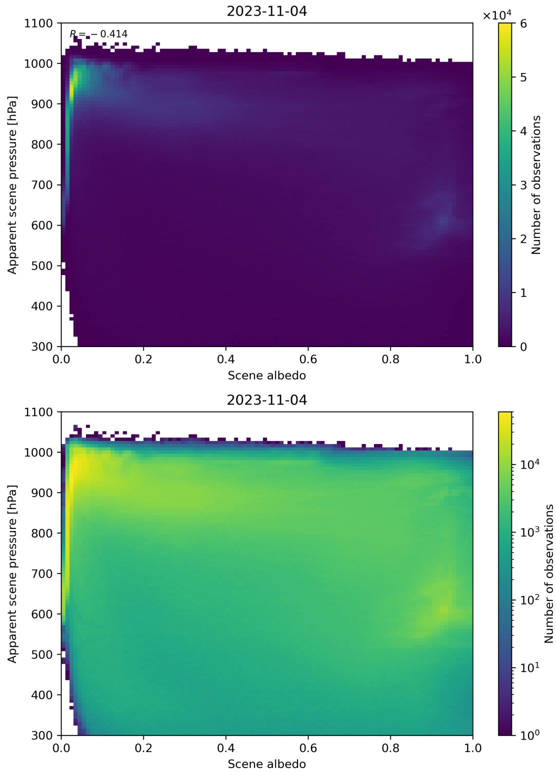
Figure 111: Scatter density plot of “Scene albedo” against “Apparent scene pressure” for 2023-11-03 to 2023-11-05.
