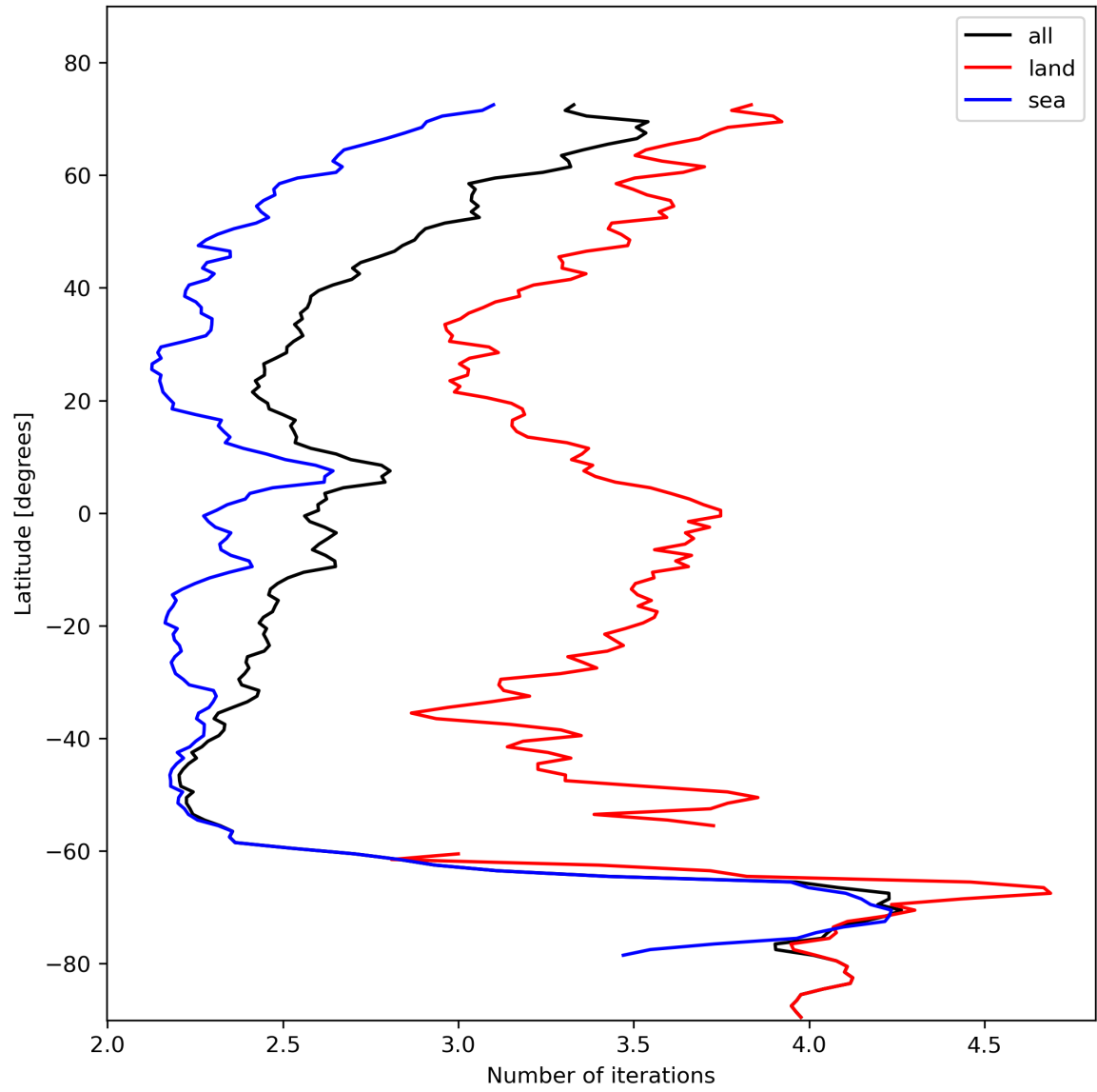
Figure 22: Zonal average of “Number of iterations” for 2023-11-03 to 2023-11-05.
