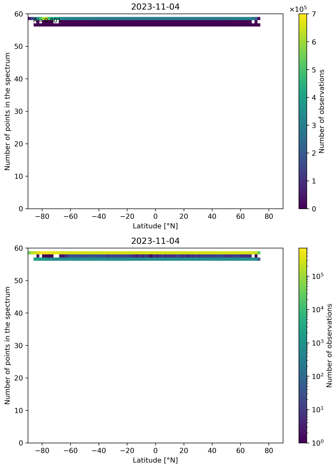
Figure 103: Scatter density plot of “Latitude” against “Number of points in the spectrum” for 2023-11-03 to 2023-11-05.
