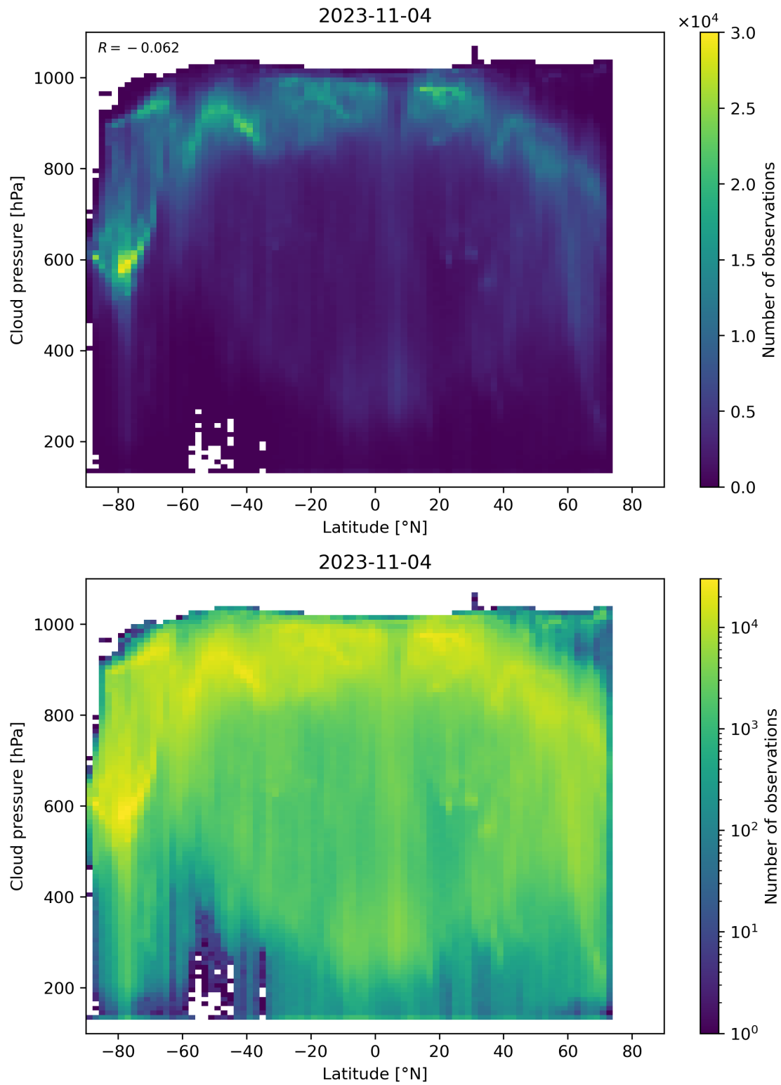
Figure 100: Scatter density plot of “Latitude” against “Cloud pressure” for 2023-11-03 to 2023-11-05.
