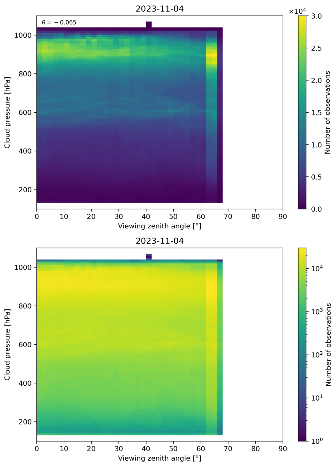
Figure 133: Scatter density plot of “Viewing zenith angle” against “Cloud pressure” for 2023-11-03 to 2023-11-05.
