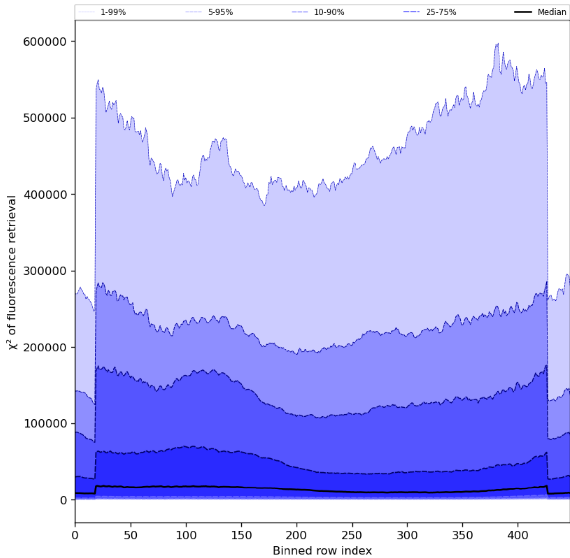
Figure 59: Along track statistics of “ \chi^2 of fluorescence retrieval” for 2023-11-03 to 2023-11-05
