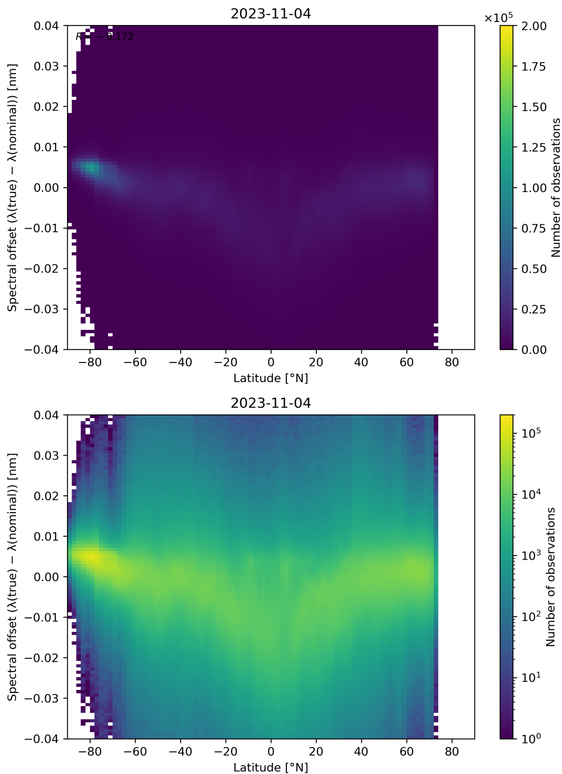
Figure 105: Scatter density plot of “Latitude” against “Spectral offset ( \lambda(\text{true}) - \lambda(\text{nominal}) )” for 2023-11-03 to 2023-11-05.
