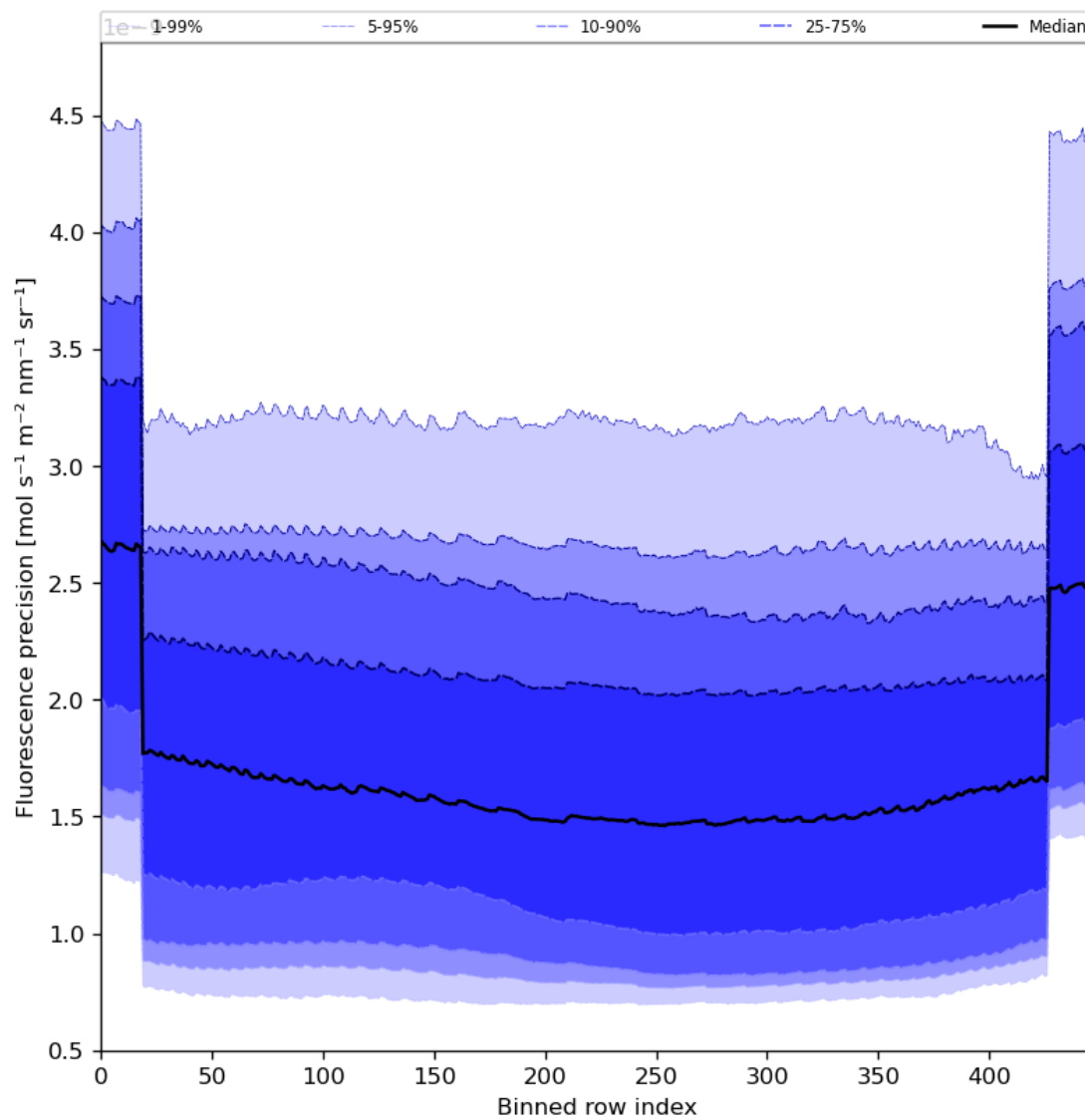
Figure 58: Along track statistics of “Fluorescence precision” for 2023-11-03 to 2023-11-05
