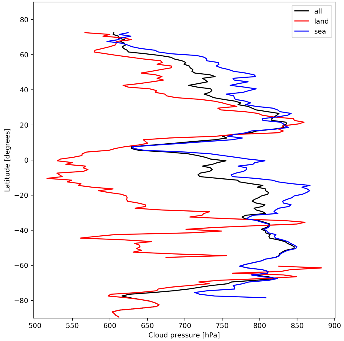
Figure 13: Zonal average of “Cloud pressure” for 2023-11-03 to 2023-11-05.
