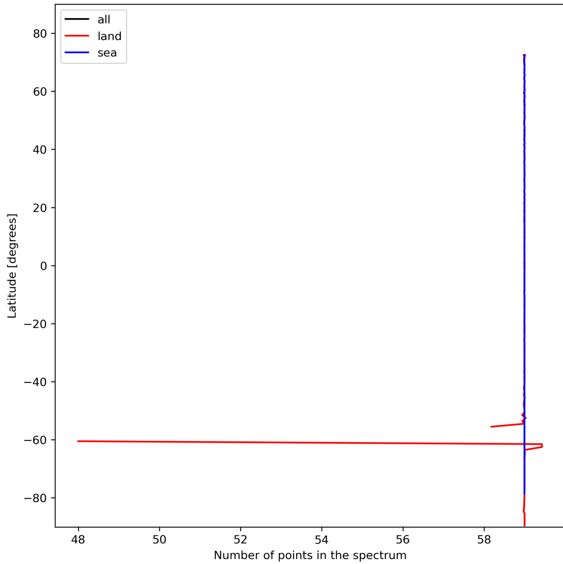
Figure 27: Zonal average of “Number of points in the spectrum” for 2023-11-03 to 2023-11-05.
