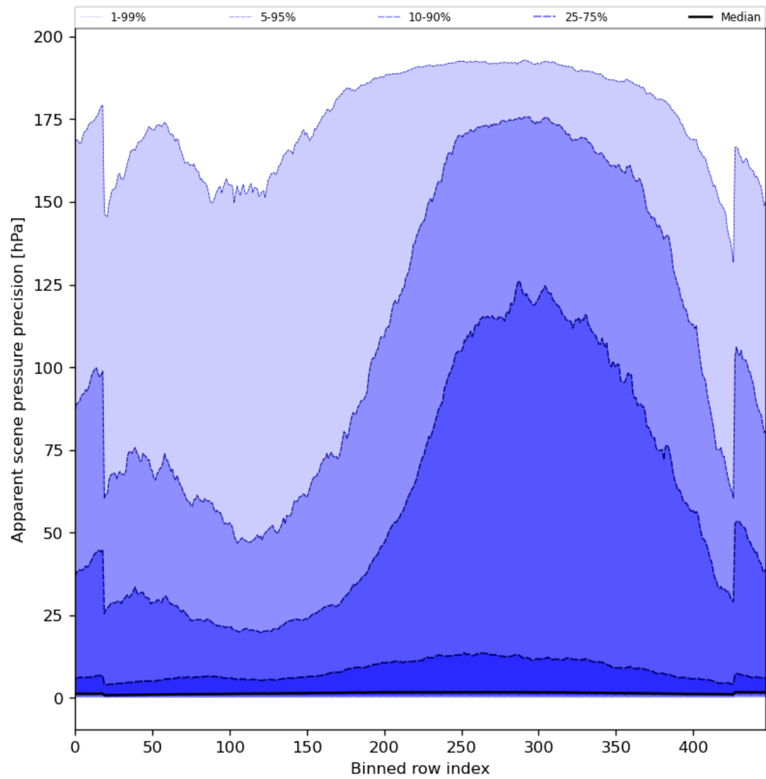
Figure 54: Along track statistics of “Apparent scene pressure precision” for 2023-11-03 to 2023-11-05
