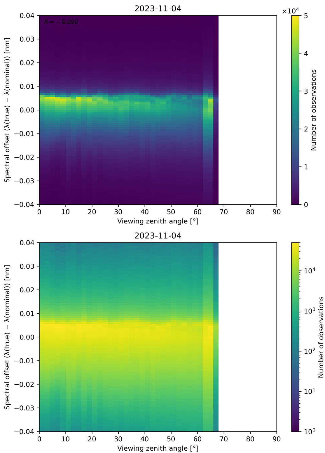
Figure 140: Scatter density plot of “Viewing zenith angle” against “Spectral offset ( \lambda(\text{true}) - \lambda(\text{nominal}) )” for 2023-11-03 to 2023-11-05.
