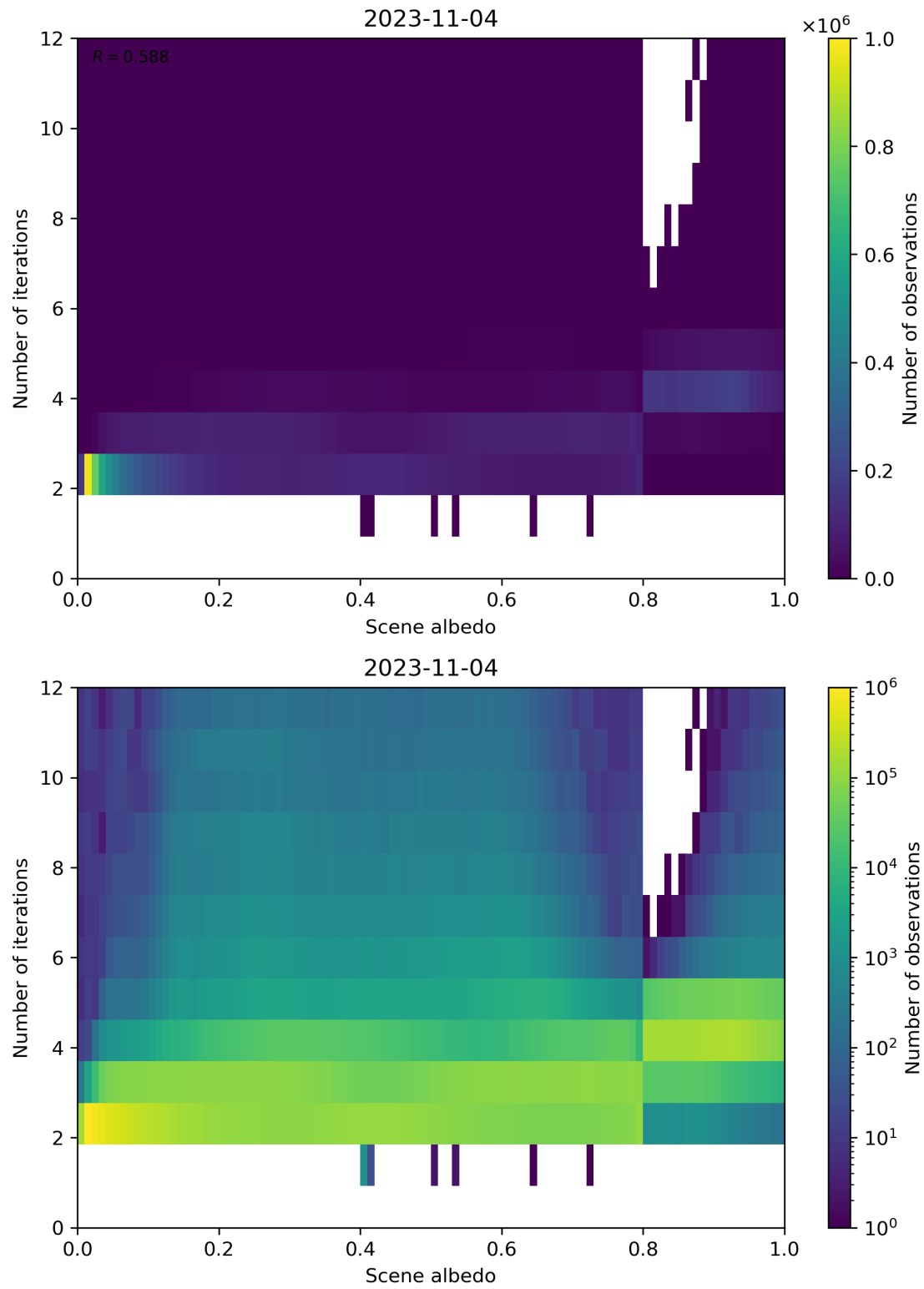
Figure 115: Scatter density plot of “Scene albedo” against “Number of iterations” for 2023-11-03 to 2023-11-05.
