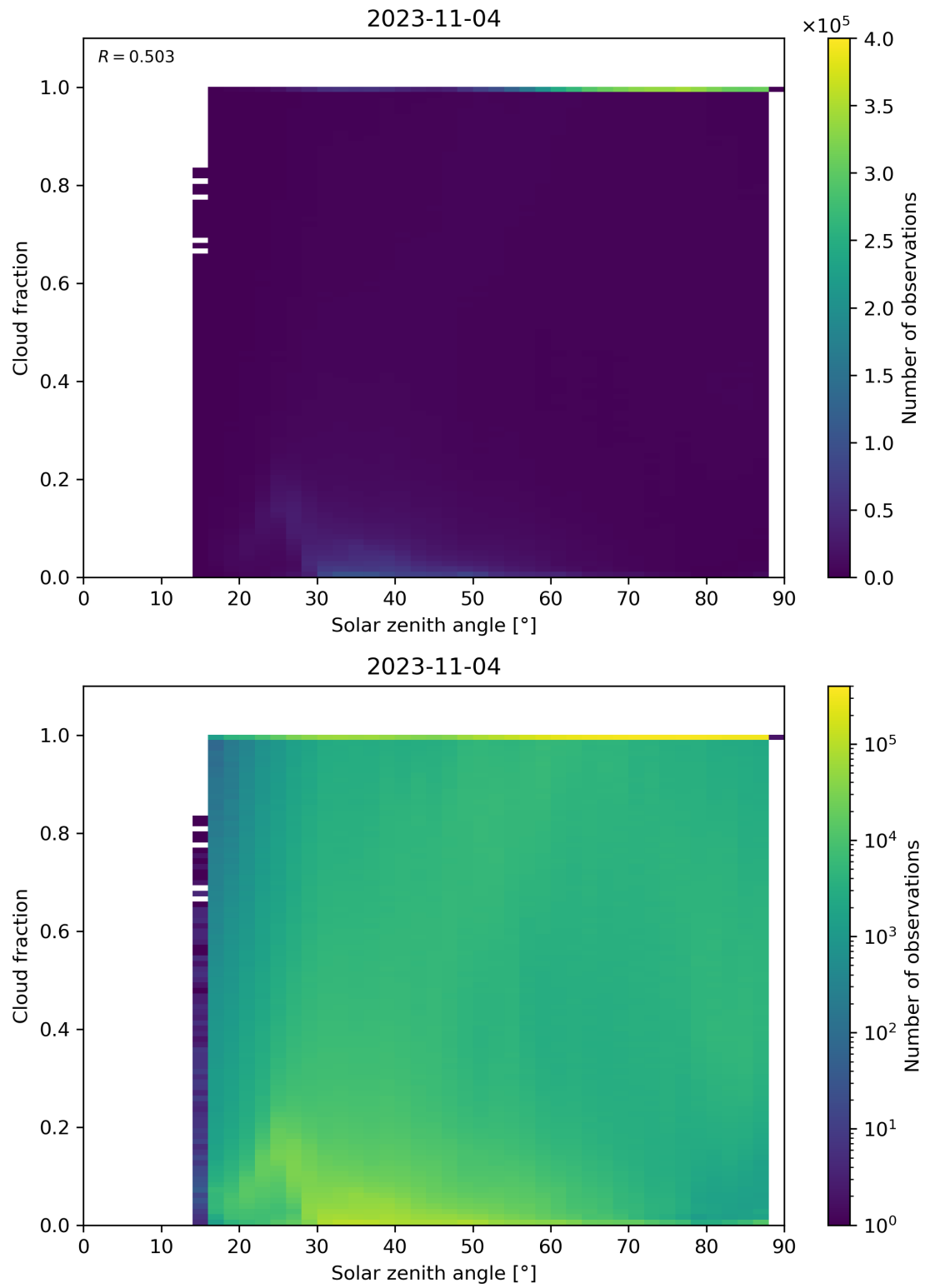
Figure 121: Scatter density plot of “Solar zenith angle” against “Cloud fraction” for 2023-11-03 to 2023-11-05.
