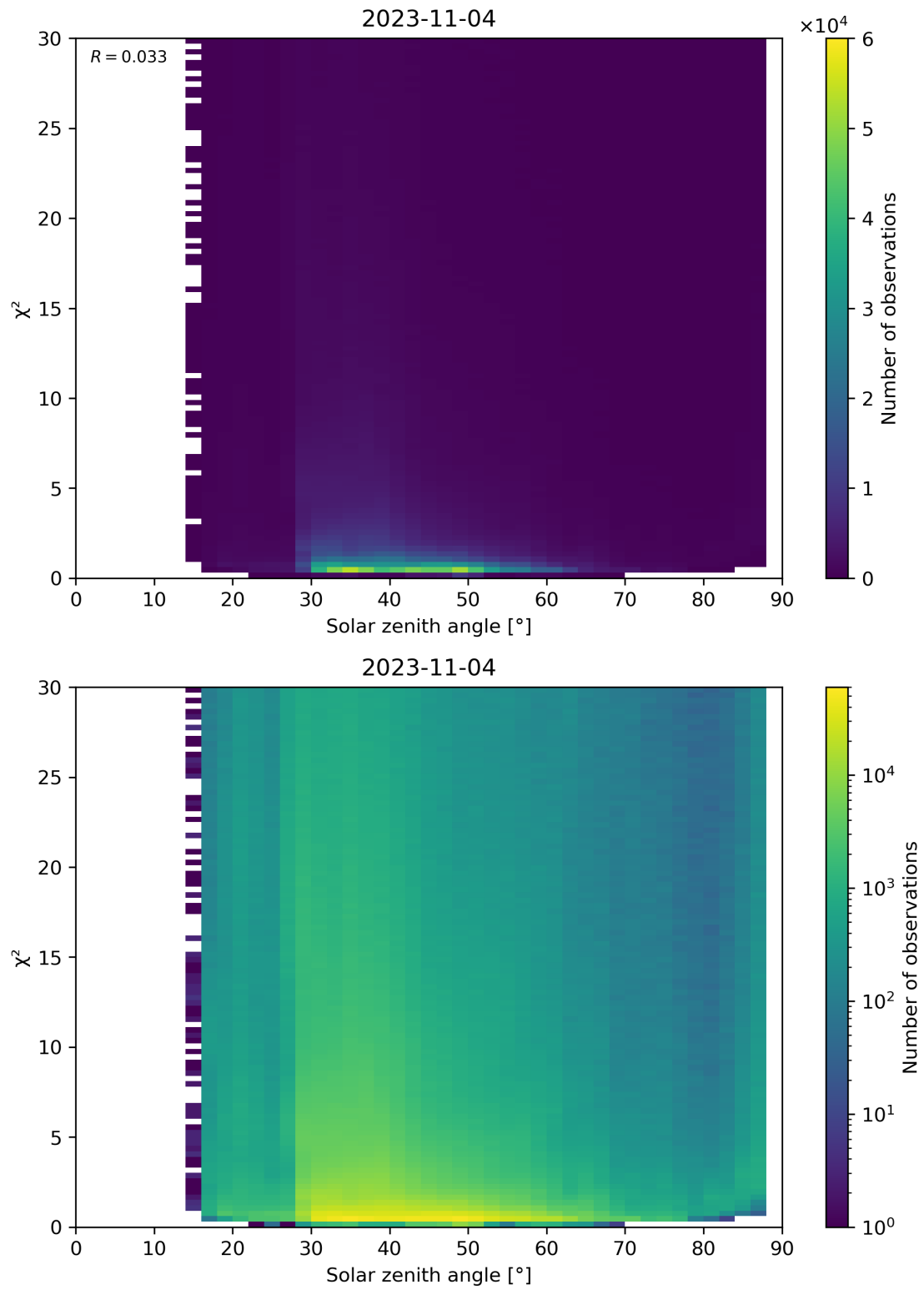
Figure 119: Scatter density plot of “Solar zenith angle” against “ \chi^2 ” for 2023-11-03 to 2023-11-05.
