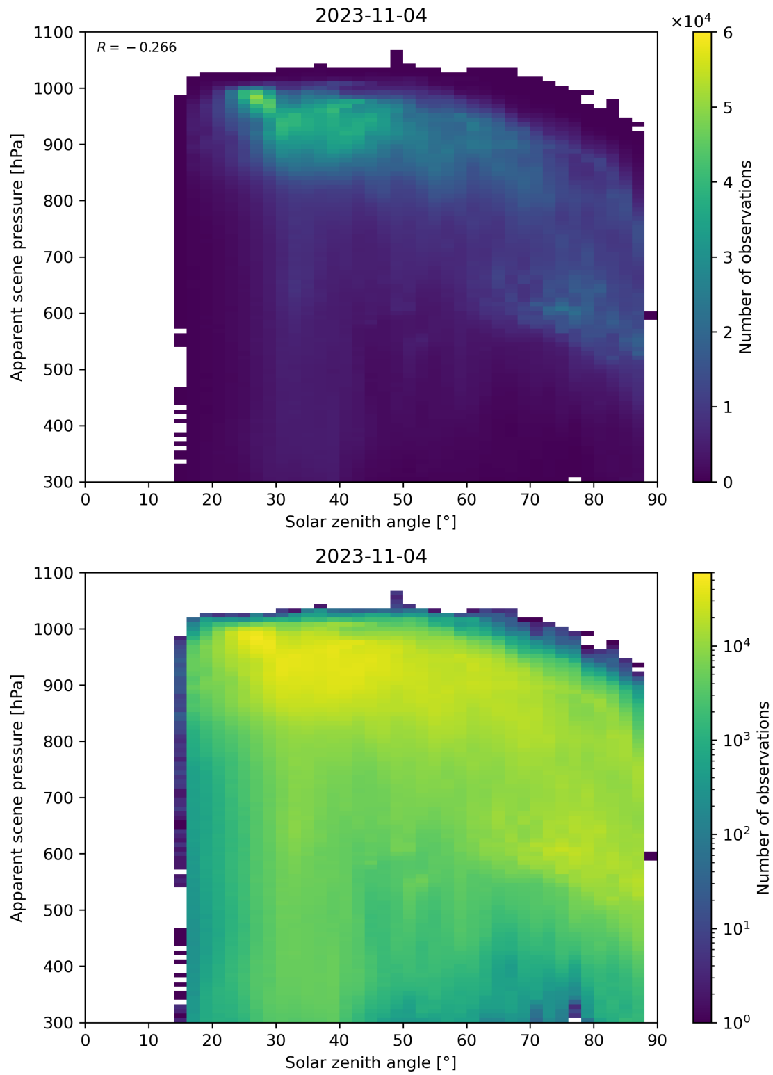
Figure 118: Scatter density plot of “Solar zenith angle” against “Apparent scene pressure” for 2023-11-03 to 2023-11-05.
