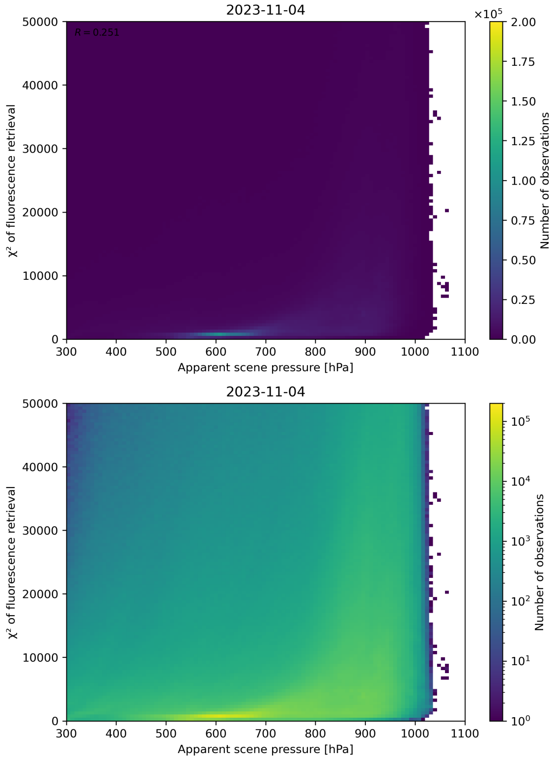
Figure 64: Scatter density plot of “Apparent scene pressure” against “ \chi^2 of fluorescence retrieval” for 2023-11-03 to 2023-11-05.
