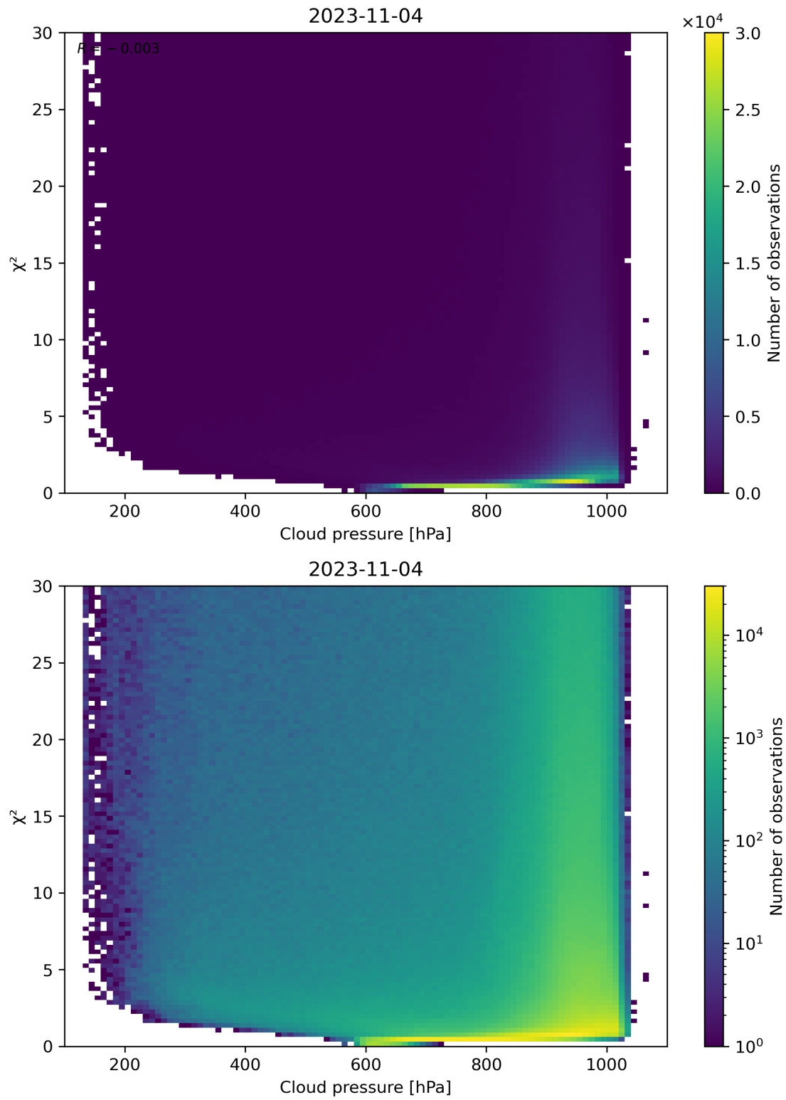
Figure 85: Scatter density plot of “Cloud pressure” against “ \chi^2 ” for 2023-11-03 to 2023-11-05.
