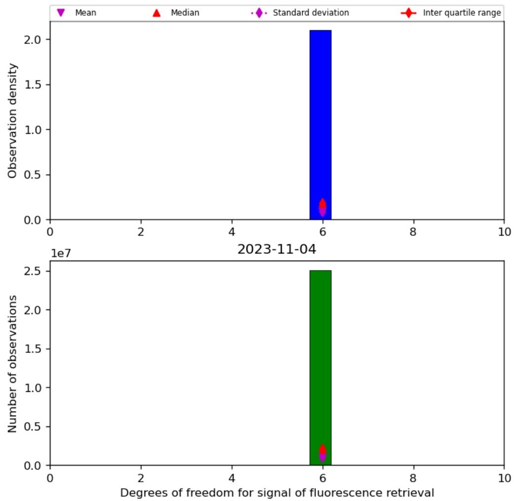
Figure 43: Histogram of “Degrees of freedom for signal of fluorescence retrieval” for 2023-11-03 to 2023-11-05
