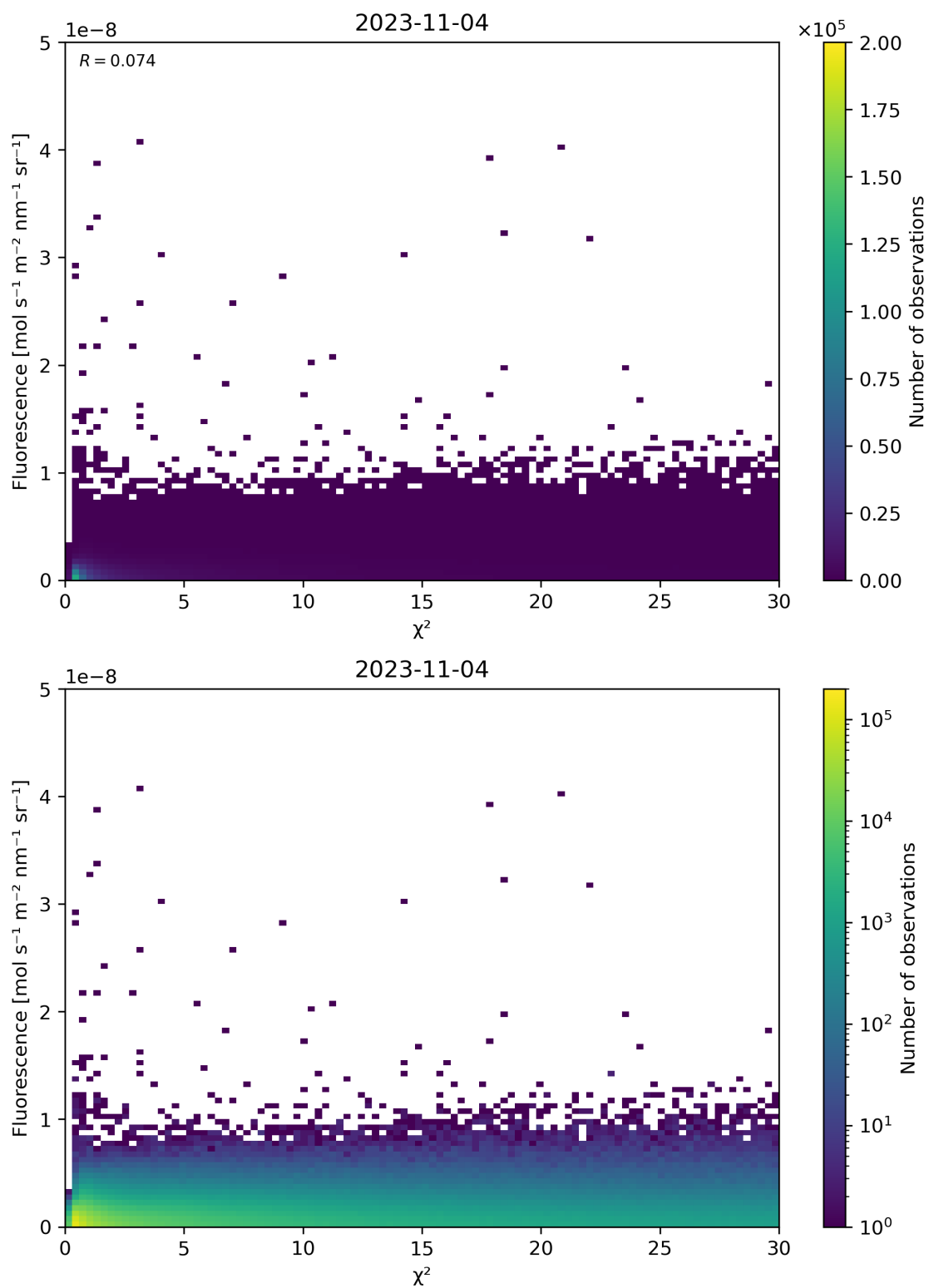
Figure 70: Scatter density plot of “ \chi^2 ” against “Fluorescence” for 2023-11-03 to 2023-11-05.
