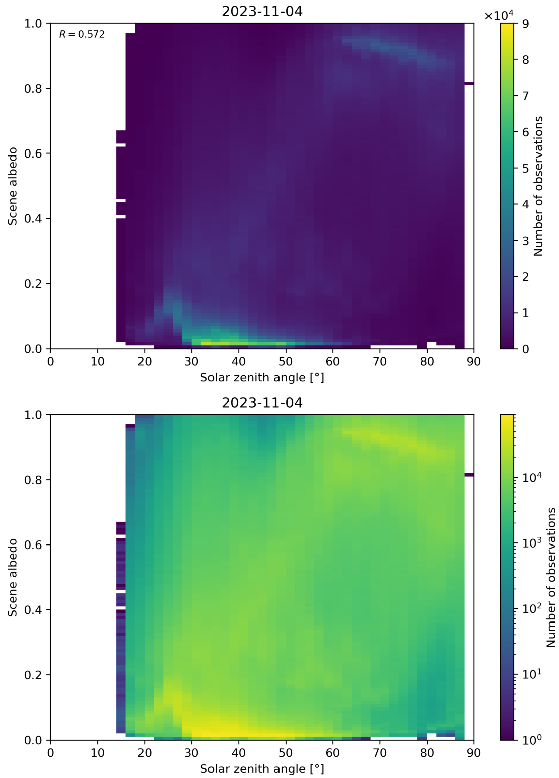
Figure 127: Scatter density plot of “Solar zenith angle” against “Scene albedo” for 2023-11-03 to 2023-11-05.
