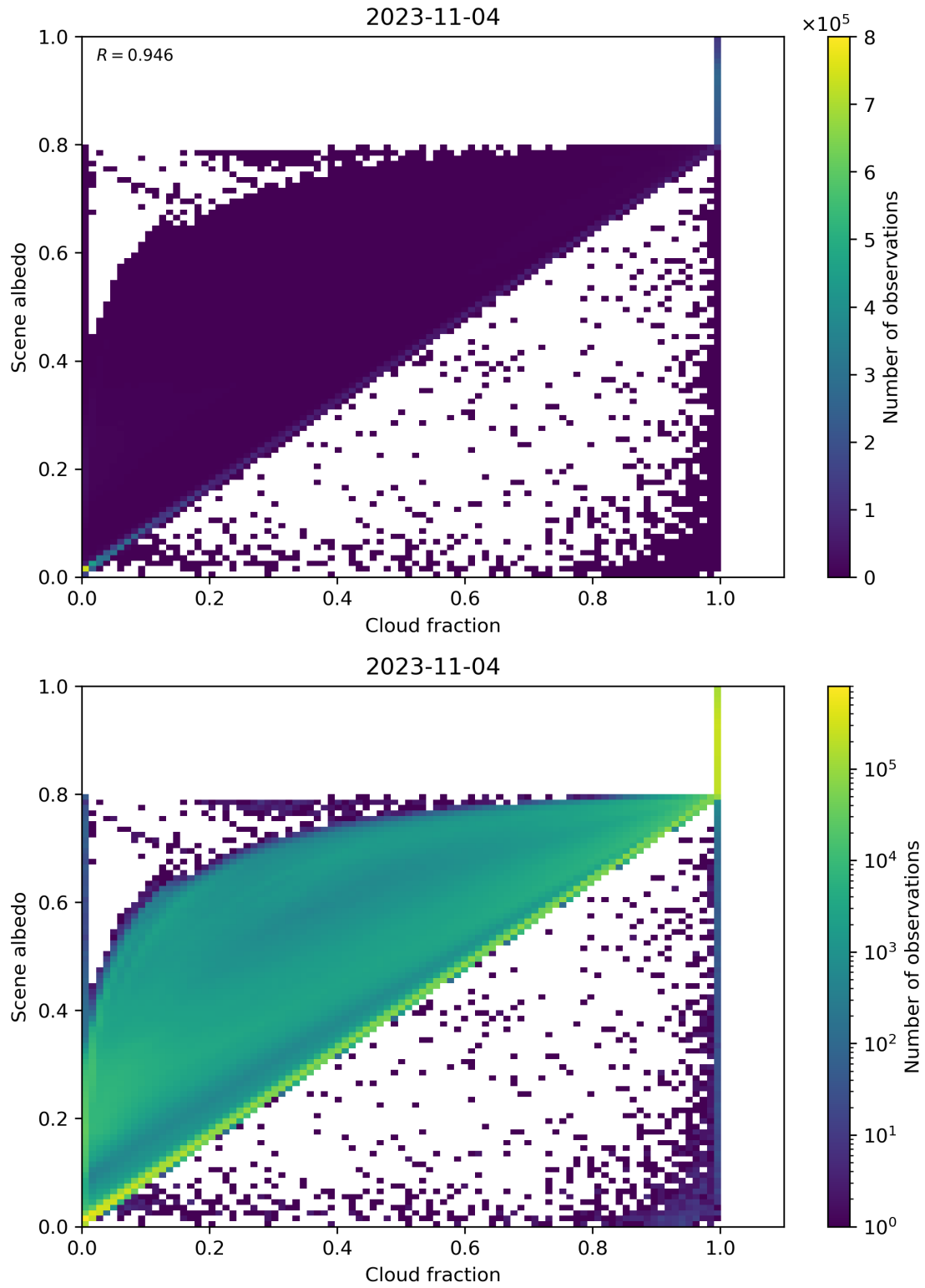
Figure 82: Scatter density plot of “Cloud fraction” against “Scene albedo” for 2023-11-03 to 2023-11-05.
