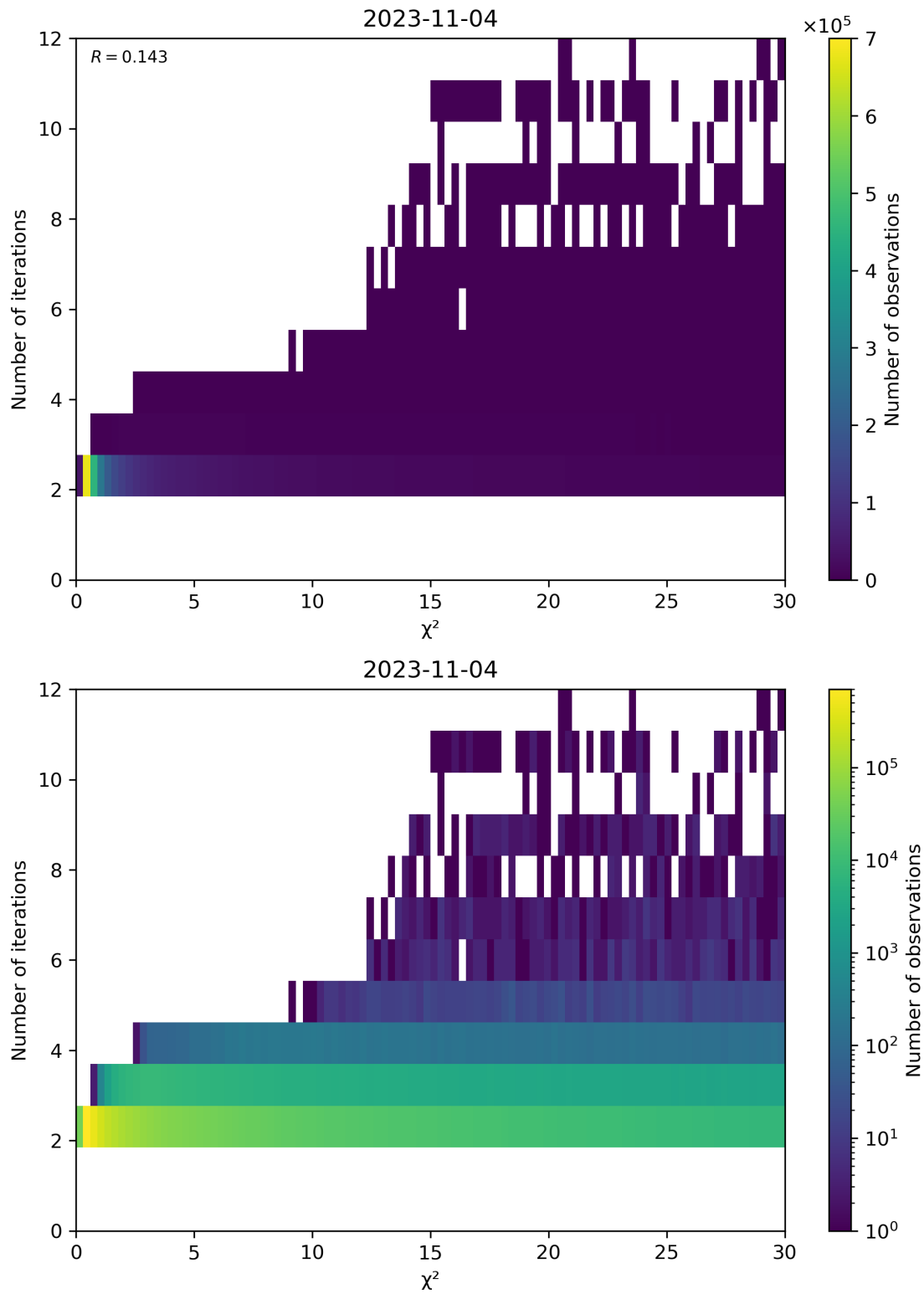
Figure 73: Scatter density plot of “ \chi^2 ” against “Number of iterations” for 2023-11-03 to 2023-11-05.
