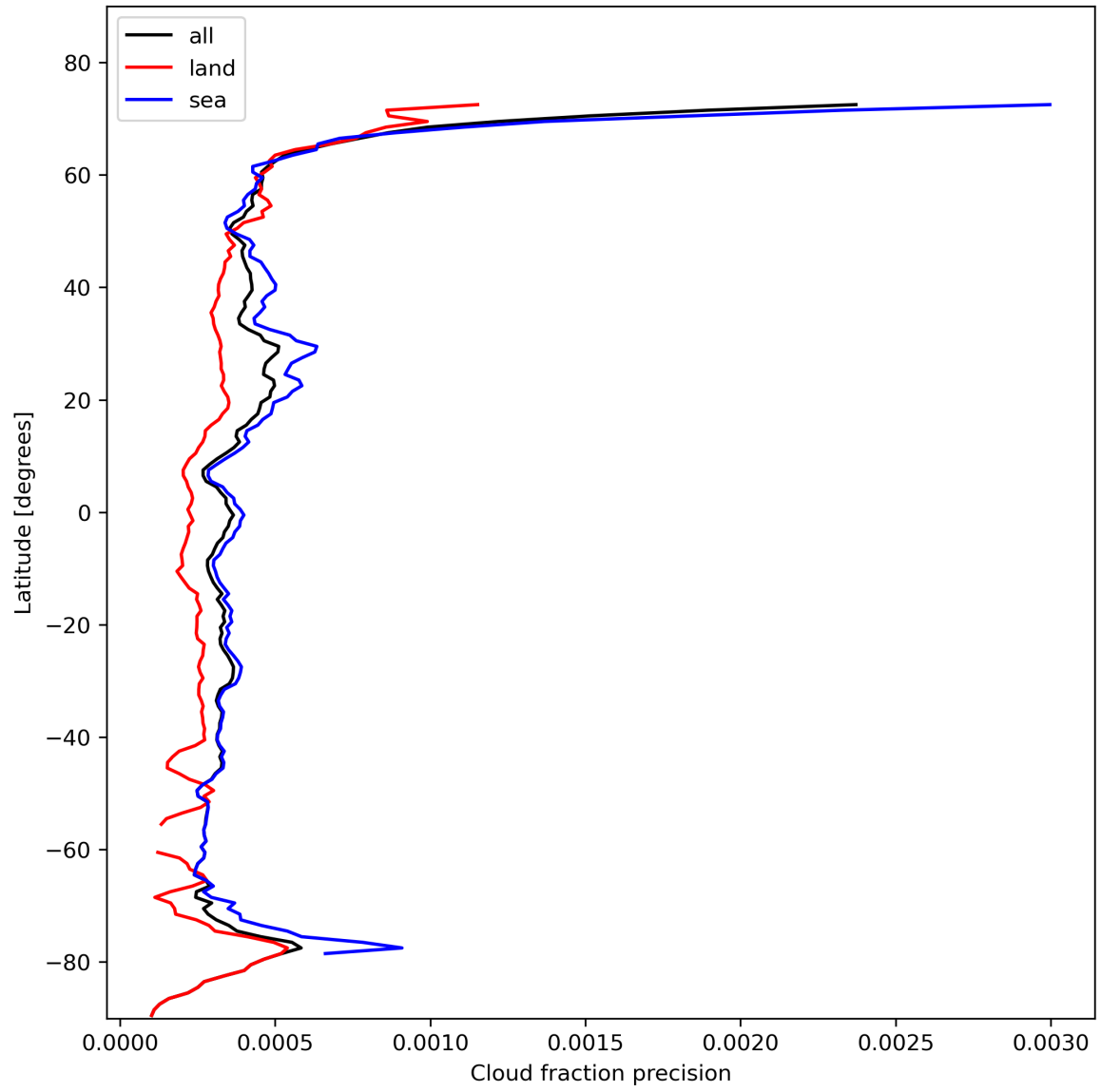
Figure 16: Zonal average of “Cloud fraction precision” for 2023-11-03 to 2023-11-05.
