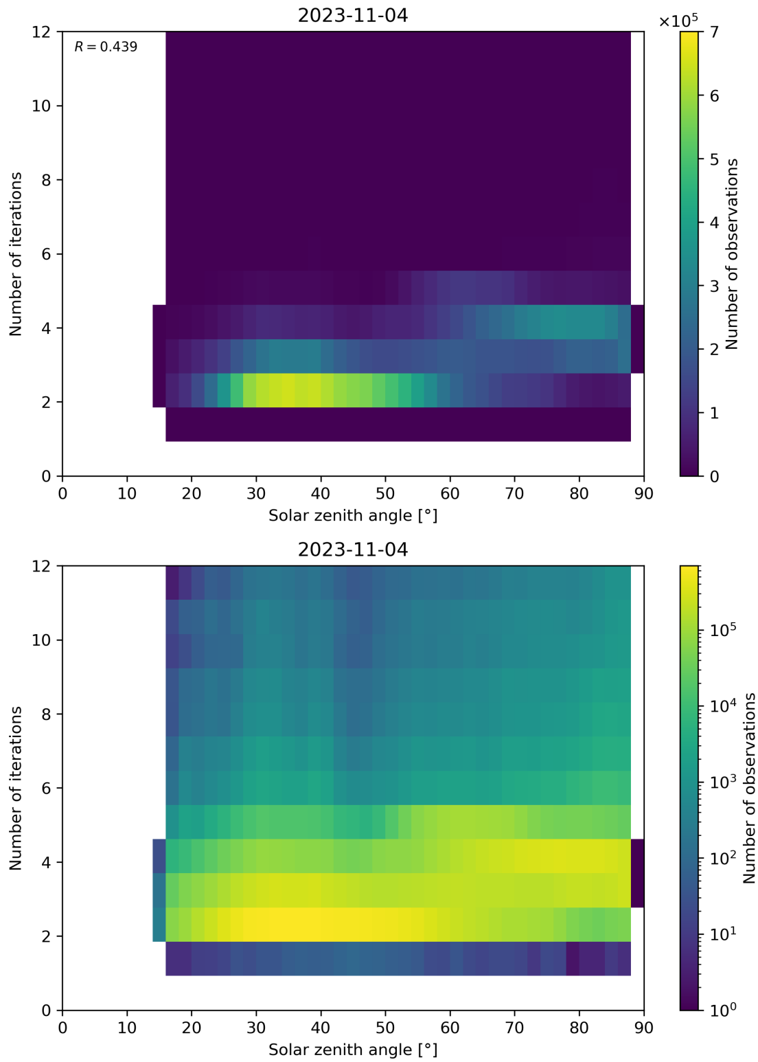
Figure 125: Scatter density plot of “Solar zenith angle” against “Number of iterations” for 2023-11-03 to 2023-11-05.
