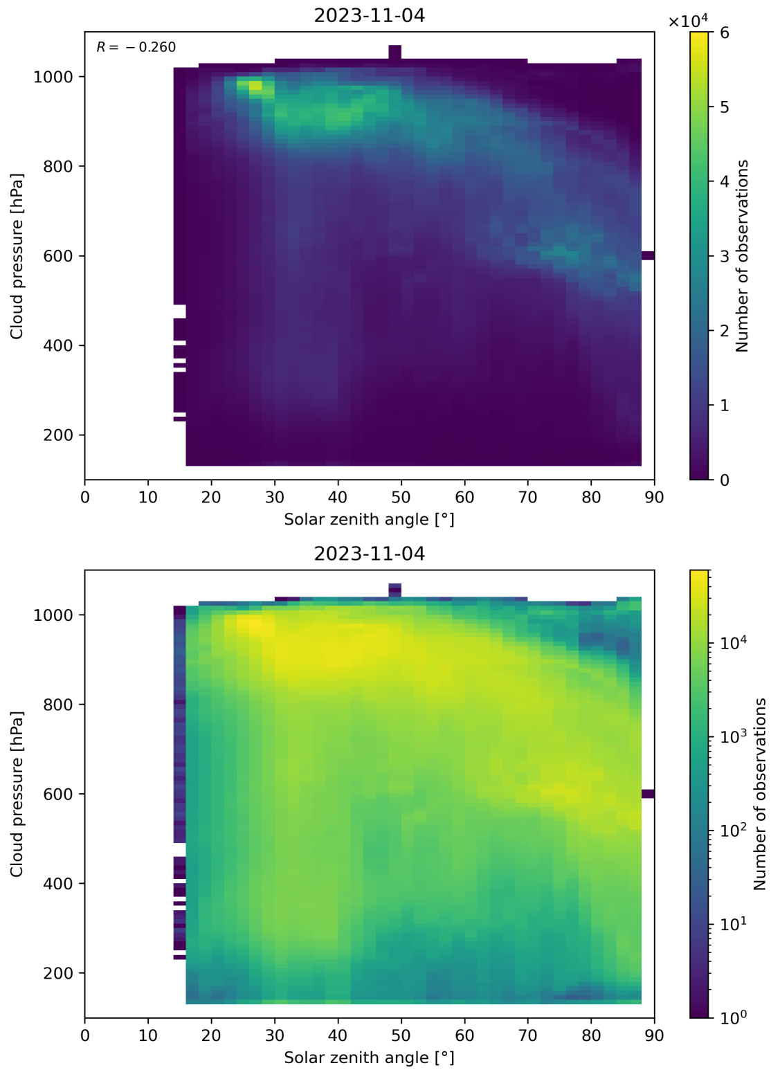
Figure 122: Scatter density plot of “Solar zenith angle” against “Cloud pressure” for 2023-11-03 to 2023-11-05.
