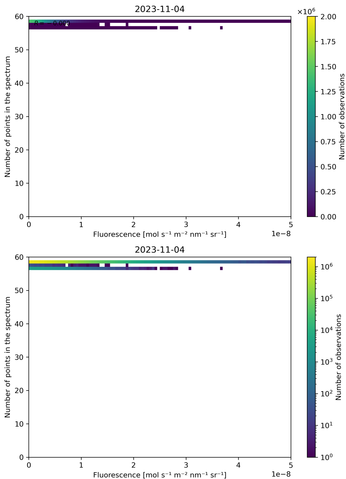
Figure 94: Scatter density plot of “Fluorescence” against “Number of points in the spectrum” for 2023-11-03 to 2023-11-05.
