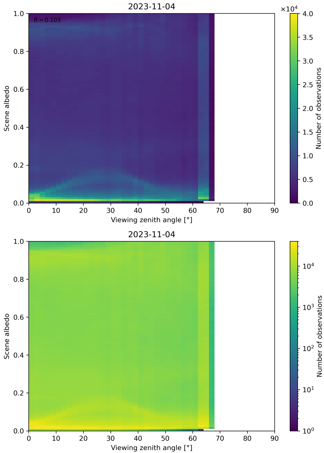
Figure 138: Scatter density plot of “Viewing zenith angle” against “Scene albedo” for 2023-11-03 to 2023-11-05.
