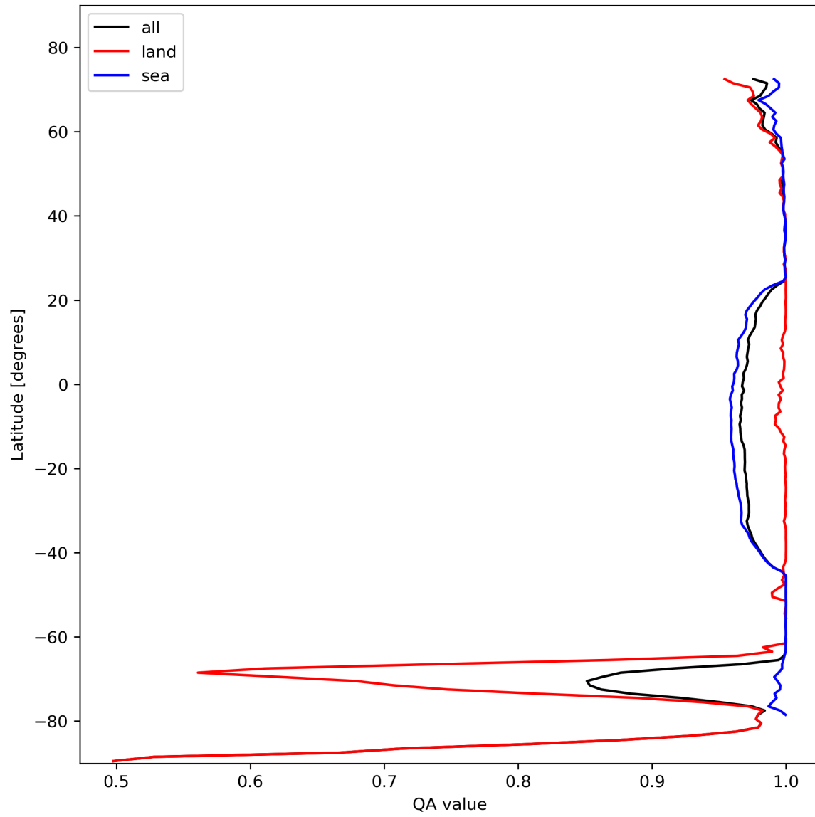
Figure 12: Zonal average of “QA value” for 2023-11-03 to 2023-11-05.
