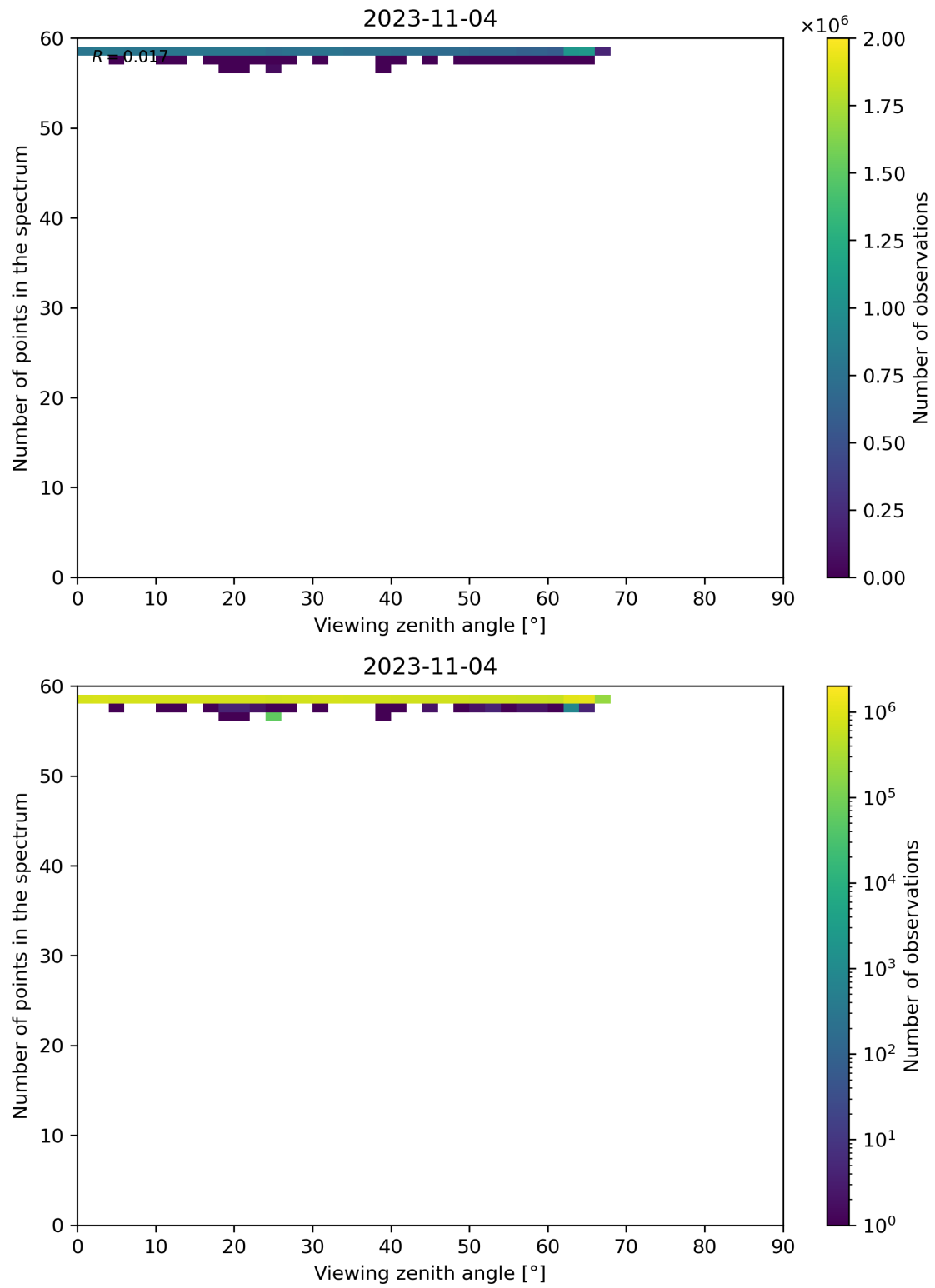
Figure 137: Scatter density plot of “Viewing zenith angle” against “Number of points in the spectrum” for 2023-11-03 to 2023-11-05.
