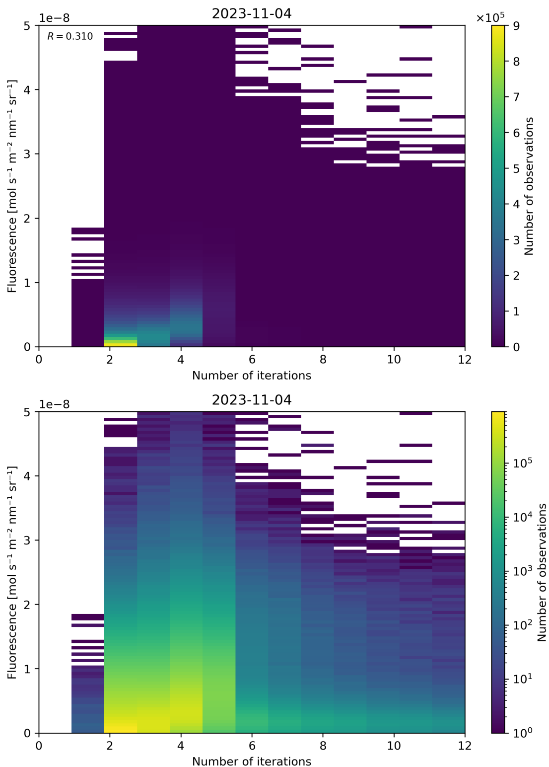
Figure 107: Scatter density plot of “Number of iterations” against “Fluorescence” for 2023-11-03 to 2023-11-05.
