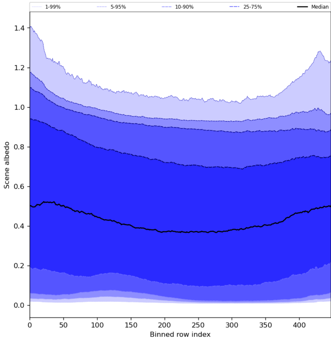
Figure 51: Along track statistics of “Scene albedo” for 2023-11-03 to 2023-11-05
