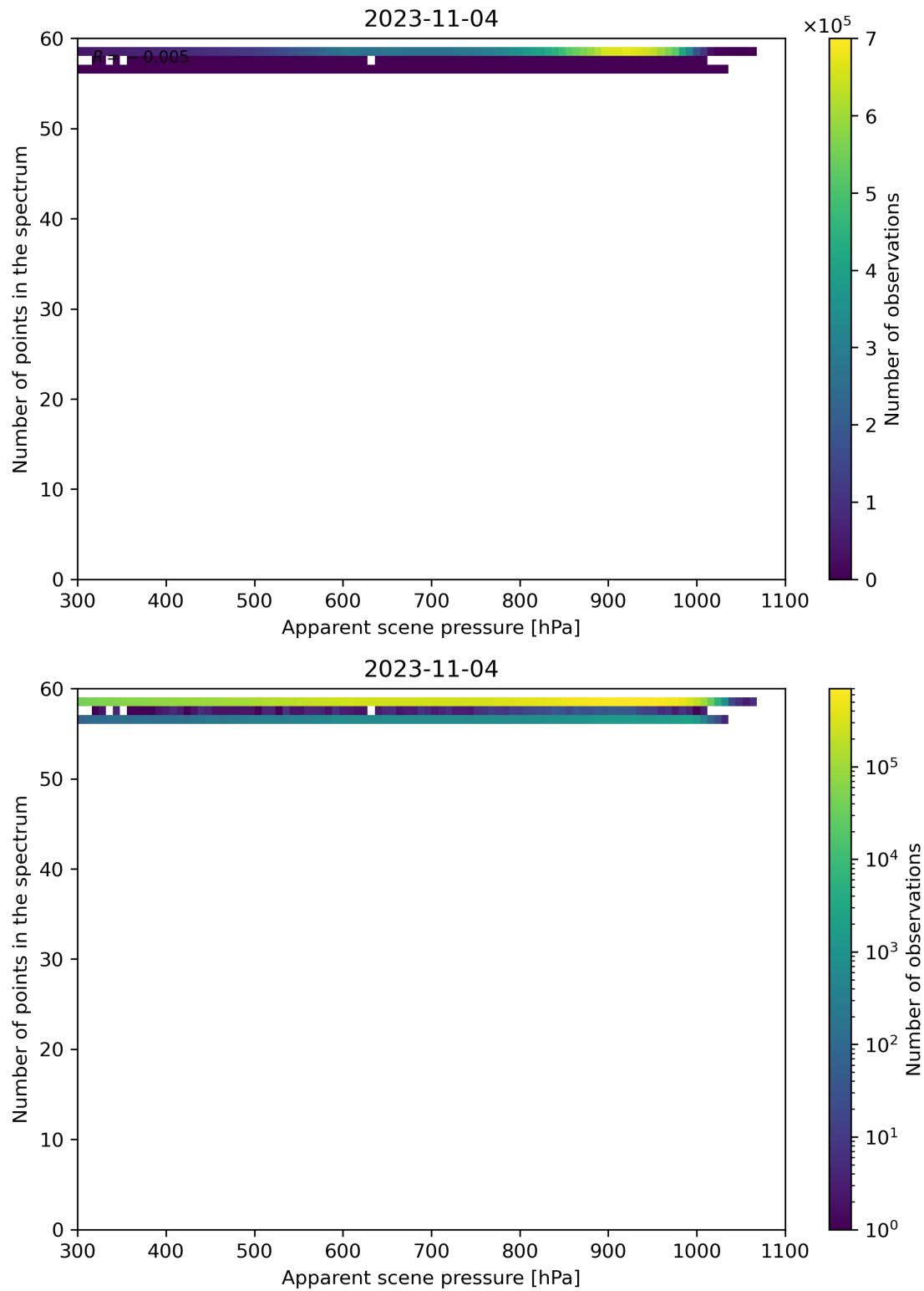
Figure 67: Scatter density plot of “Apparent scene pressure” against “Number of points in the spectrum” for 2023-11-03 to 2023-11-05.
