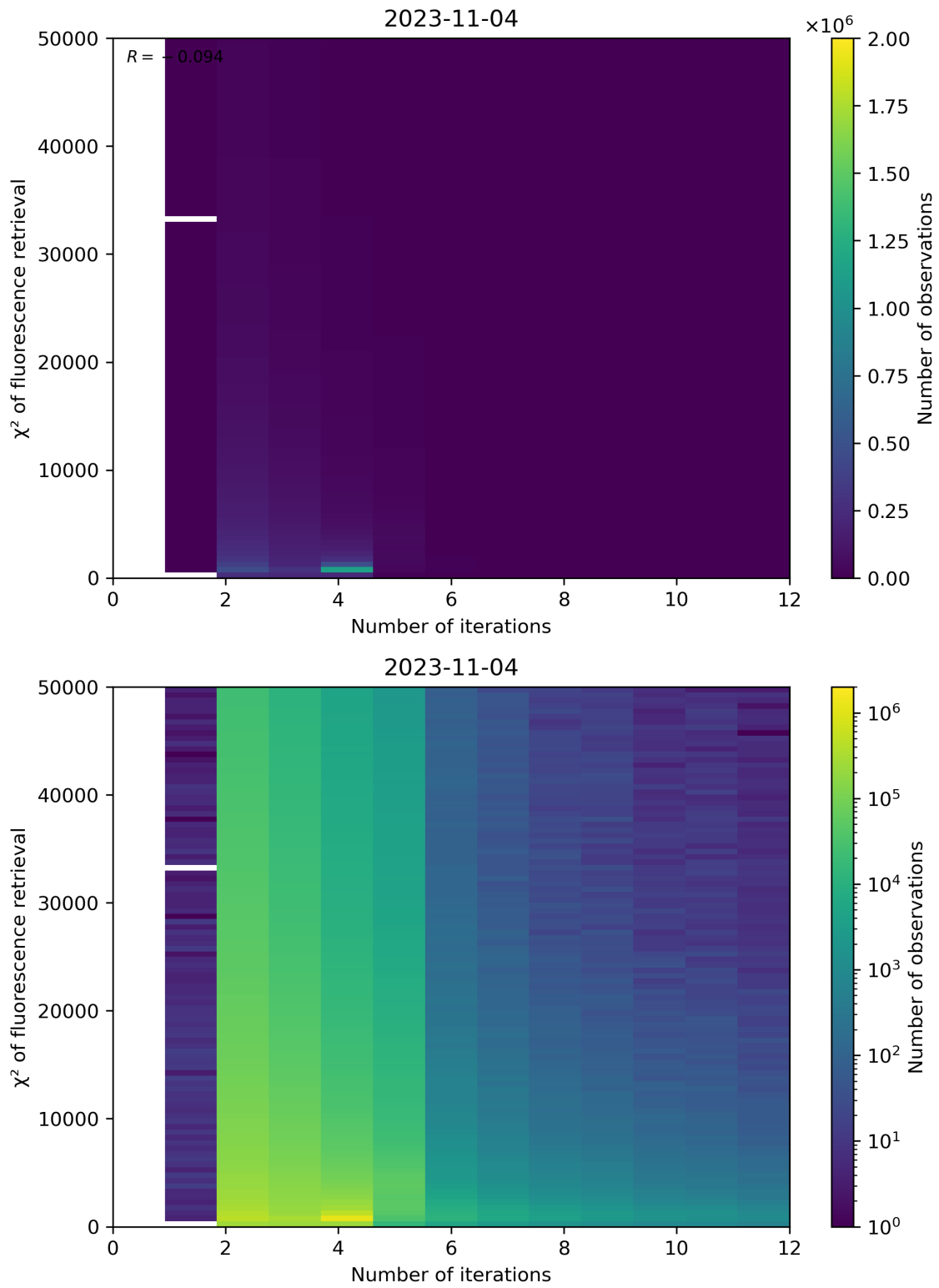
Figure 106: Scatter density plot of “Number of iterations” against “ \chi^2 of fluorescence retrieval” for 2023-11-03 to 2023-11-05.
