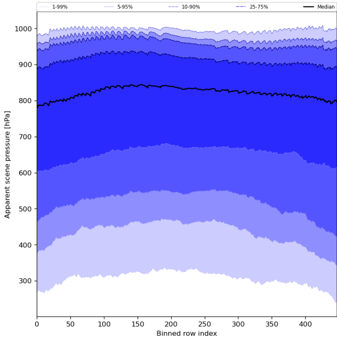
Figure 53: Along track statistics of “Apparent scene pressure” for 2023-11-03 to 2023-11-05
