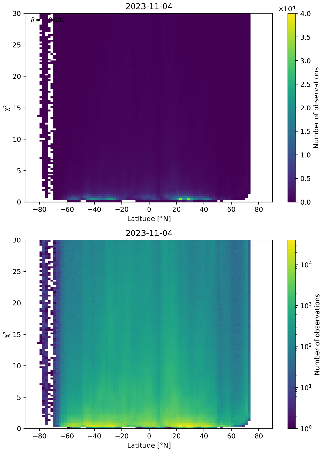
Figure 97: Scatter density plot of “Latitude” against “ \chi^2 ” for 2023-11-03 to 2023-11-05.
