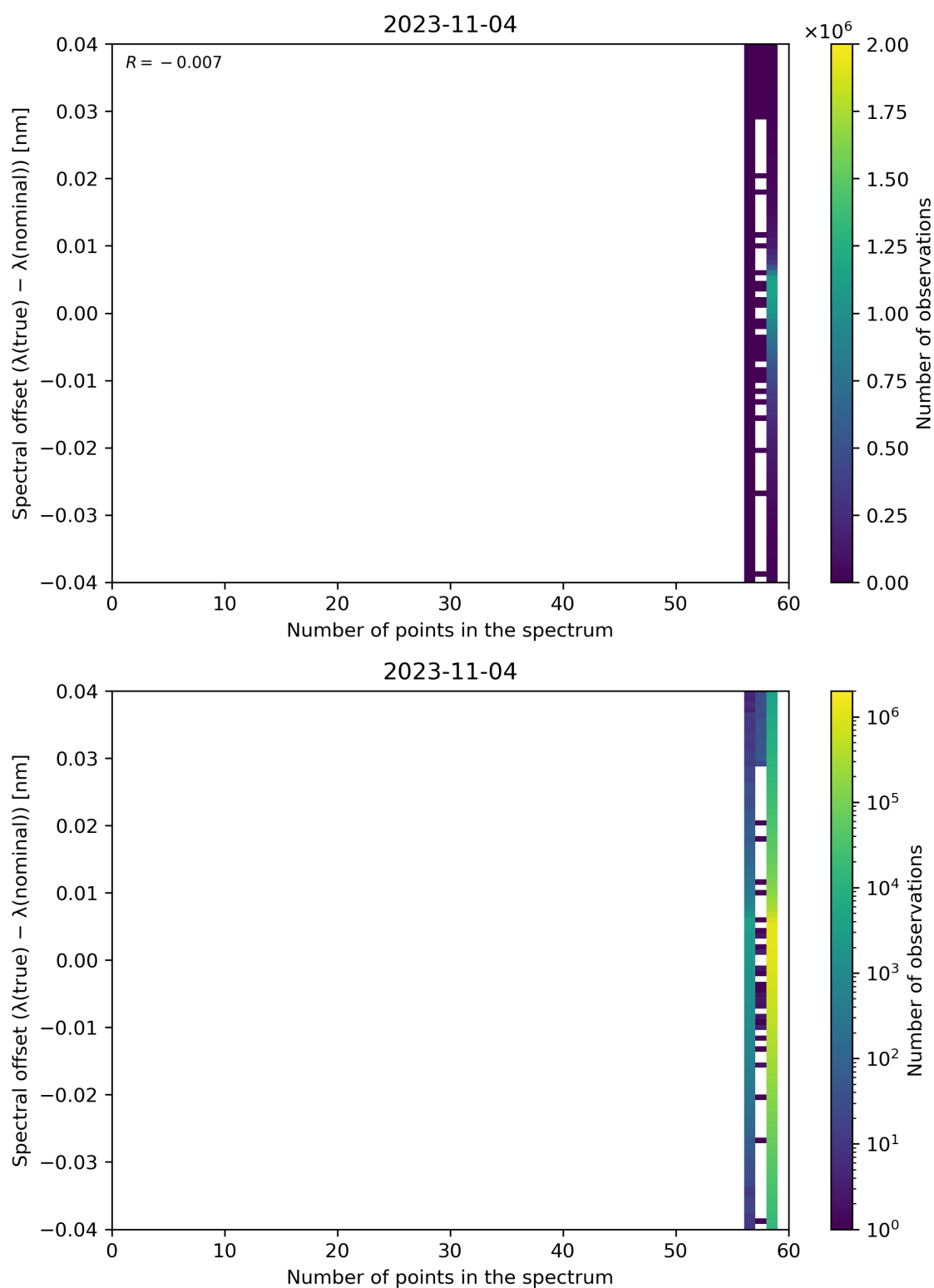
Figure 110: Scatter density plot of “Number of points in the spectrum” against “Spectral offset ( \lambda(\text{true}) - \lambda(\text{nominal}) )” for 2023-11-03 to 2023-11-05.
