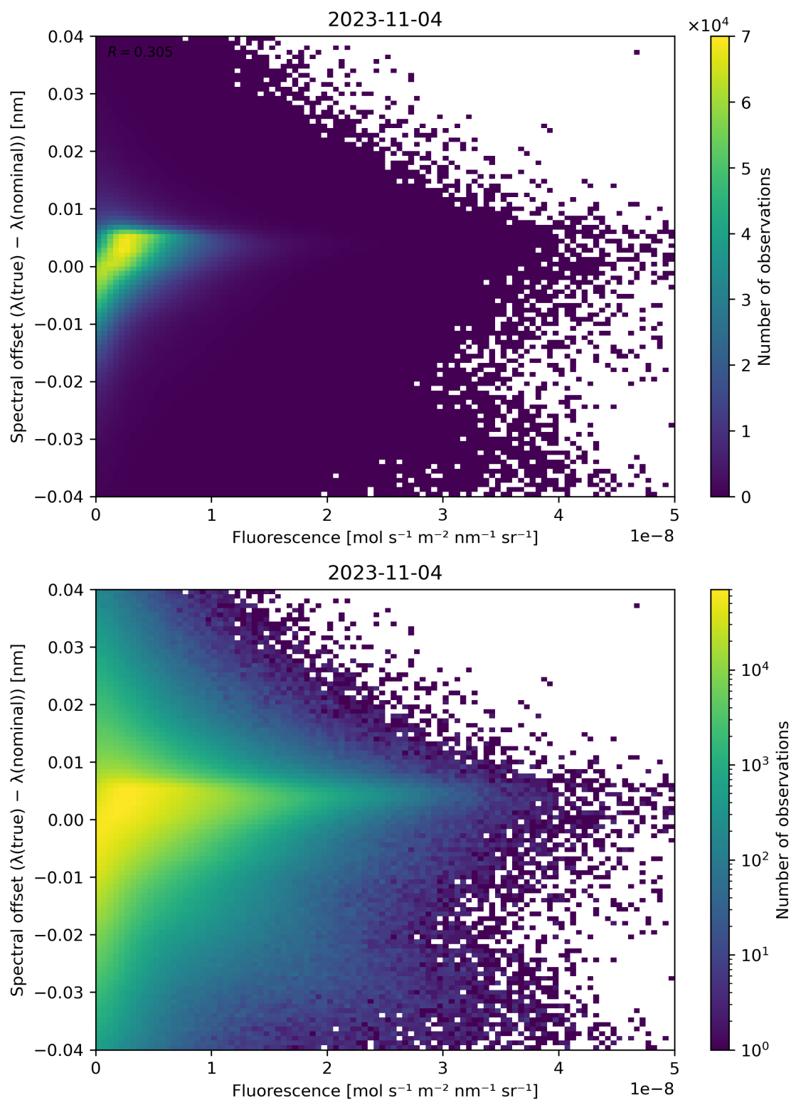
Figure 95: Scatter density plot of “Fluorescence” against “Spectral offset ( \lambda(\text{true}) - \lambda(\text{nominal}) )” for 2023-11-03 to 2023-11-05.
