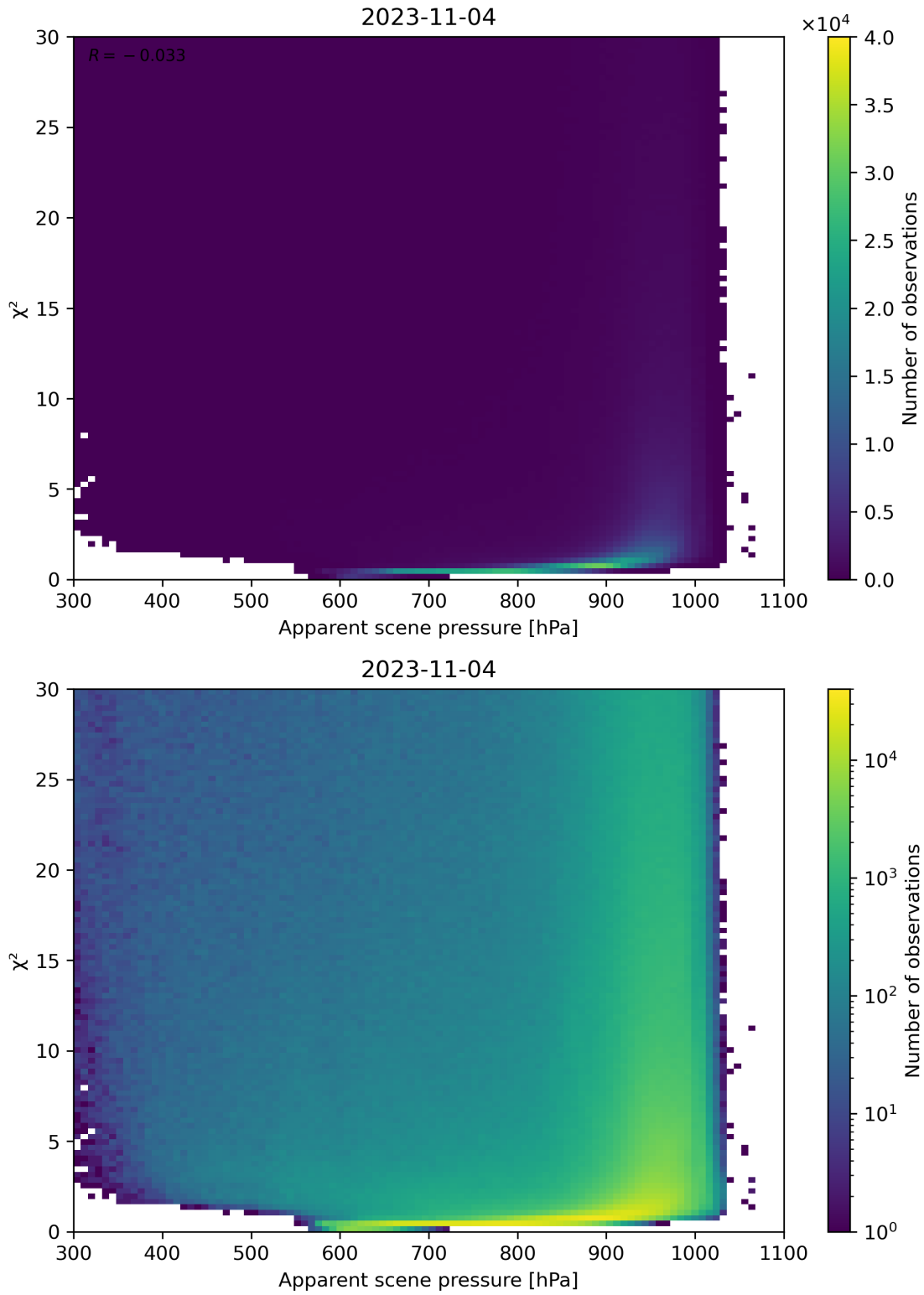
Figure 63: Scatter density plot of “Apparent scene pressure” against “ \chi^2 ” for 2023-11-03 to 2023-11-05.
