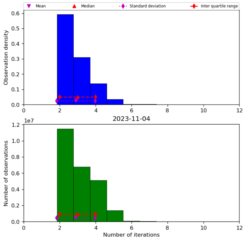
Figure 39: Histogram of “Number of iterations” for 2023-11-03 to 2023-11-05
