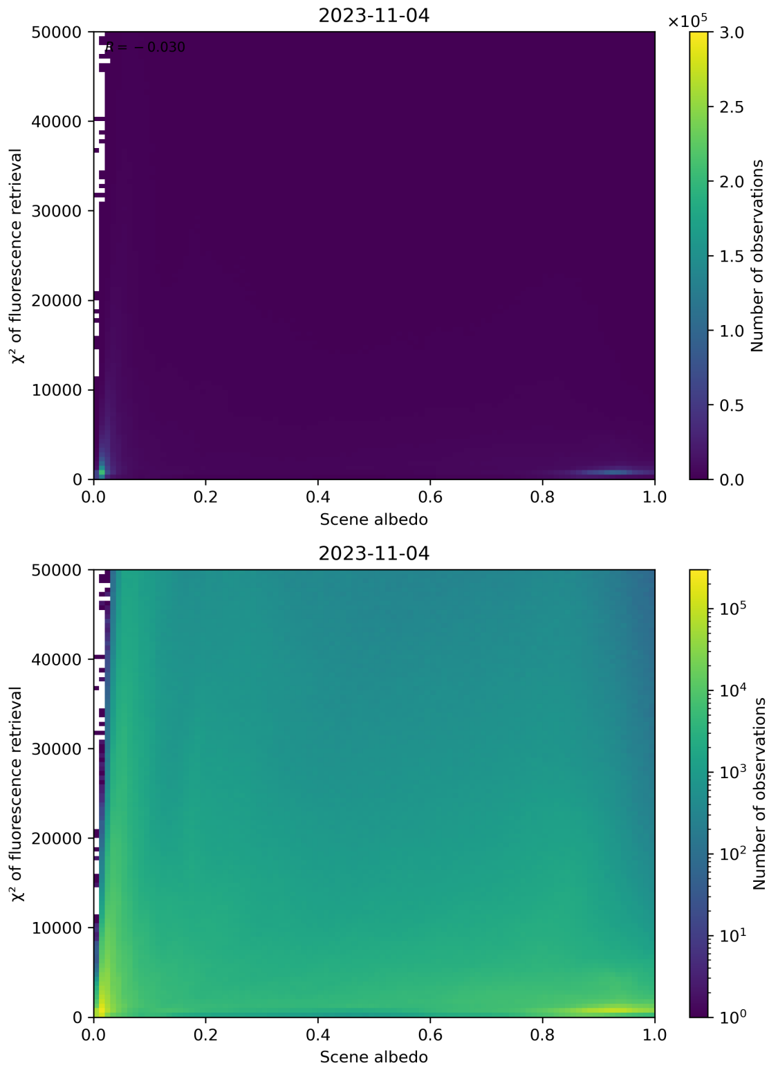
Figure 113: Scatter density plot of “Scene albedo” against “ \chi^2 of fluorescence retrieval” for 2023-11-03 to 2023-11-05.
