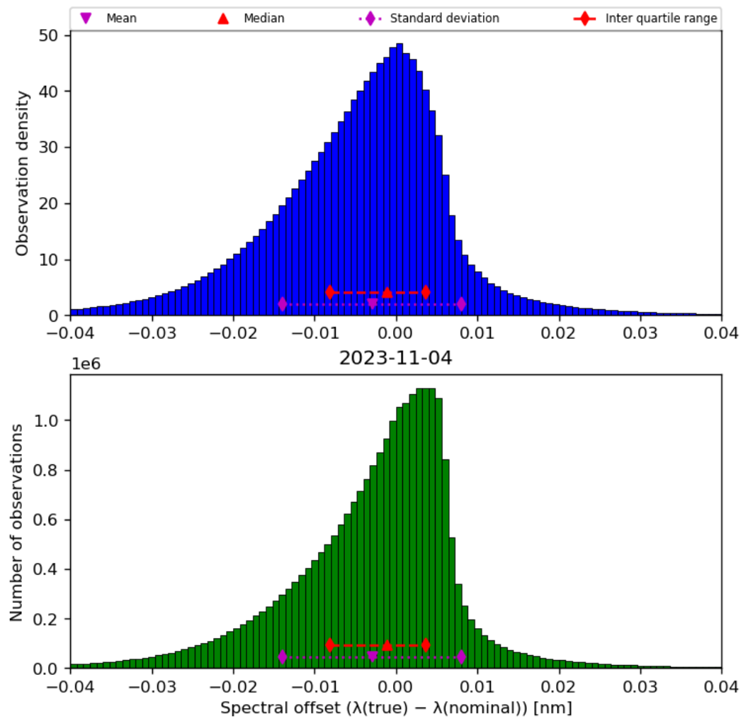
Figure 45: Histogram of “Spectral offset ( \lambda(\text{true}) - \lambda(\text{nominal}) )” for 2023-11-03 to 2023-11-05
