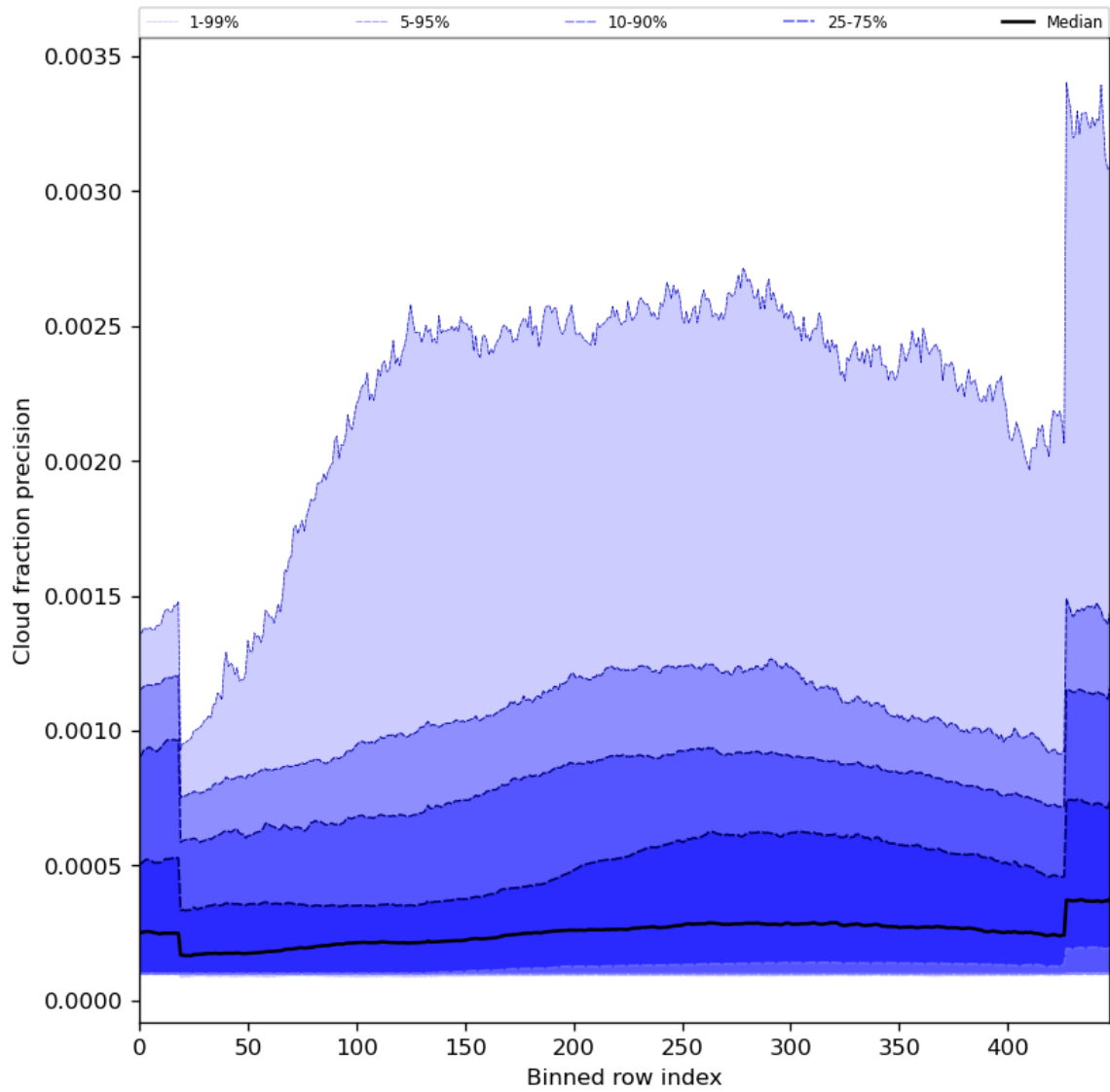
Figure 50: Along track statistics of “Cloud fraction precision” for 2023-11-03 to 2023-11-05
