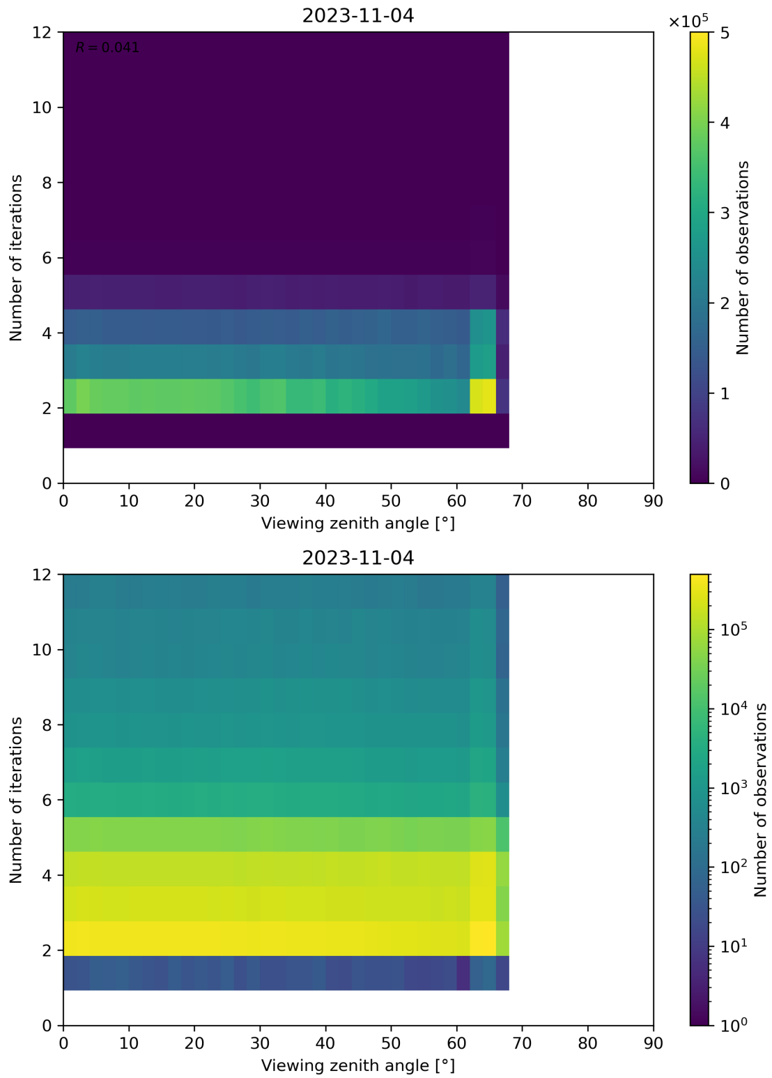
Figure 136: Scatter density plot of “Viewing zenith angle” against “Number of iterations” for 2023-11-03 to 2023-11-05.
