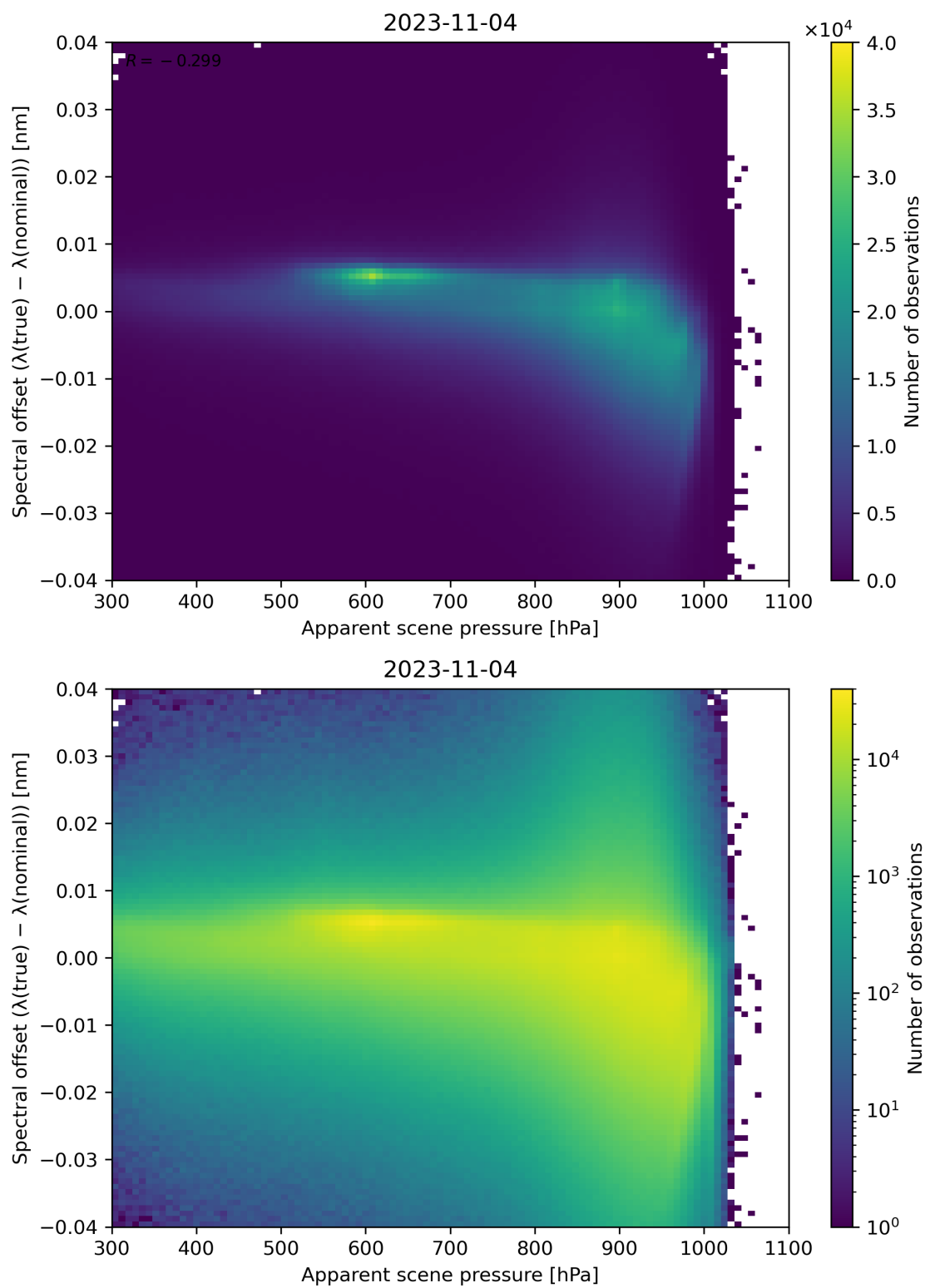
Figure 68: Scatter density plot of “Apparent scene pressure” against “Spectral offset ( \lambda(\text{true}) - \lambda(\text{nominal}) )” for 2023-11-03 to 2023-11-05.
