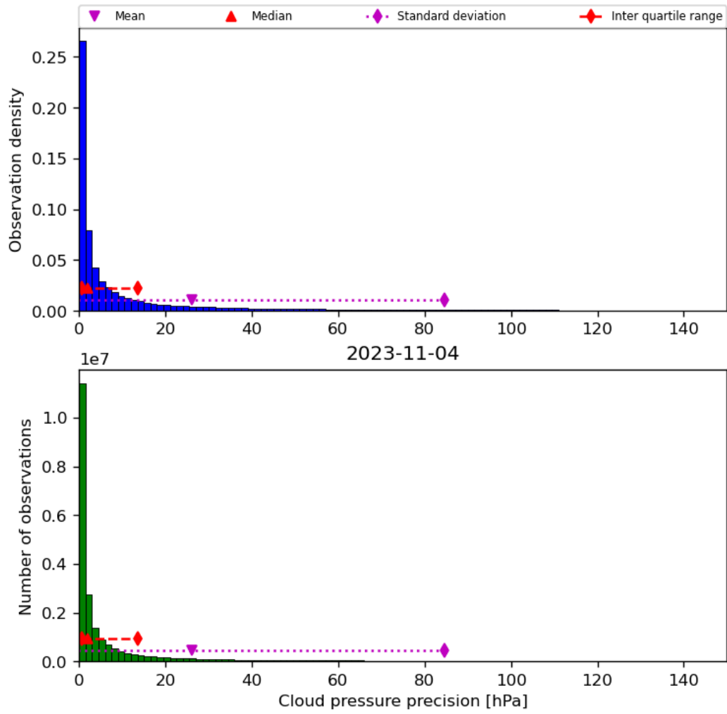
Figure 31: Histogram of “Cloud pressure precision” for 2023-11-03 to 2023-11-05
