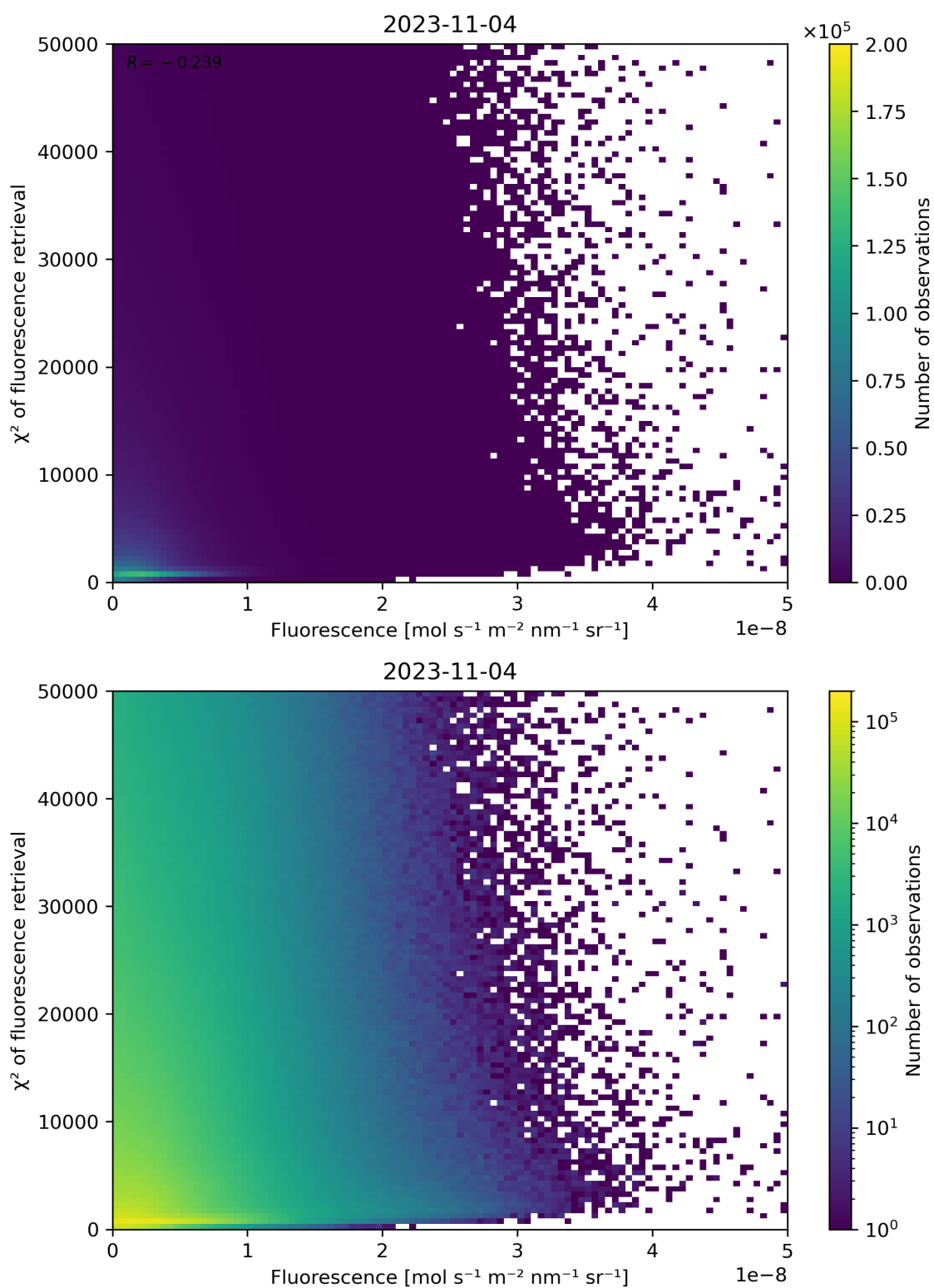
Figure 93: Scatter density plot of “Fluorescence” against “ \chi^2 of fluorescence retrieval” for 2023-11-03 to 2023-11-05.
