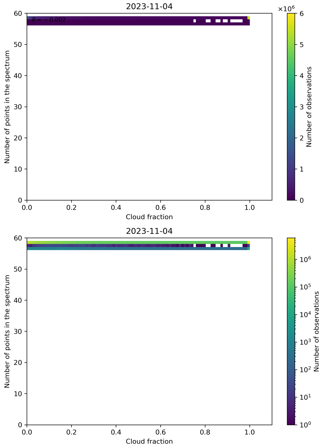
Figure 81: Scatter density plot of “Cloud fraction” against “Number of points in the spectrum” for 2023-11-03 to 2023-11-05.
