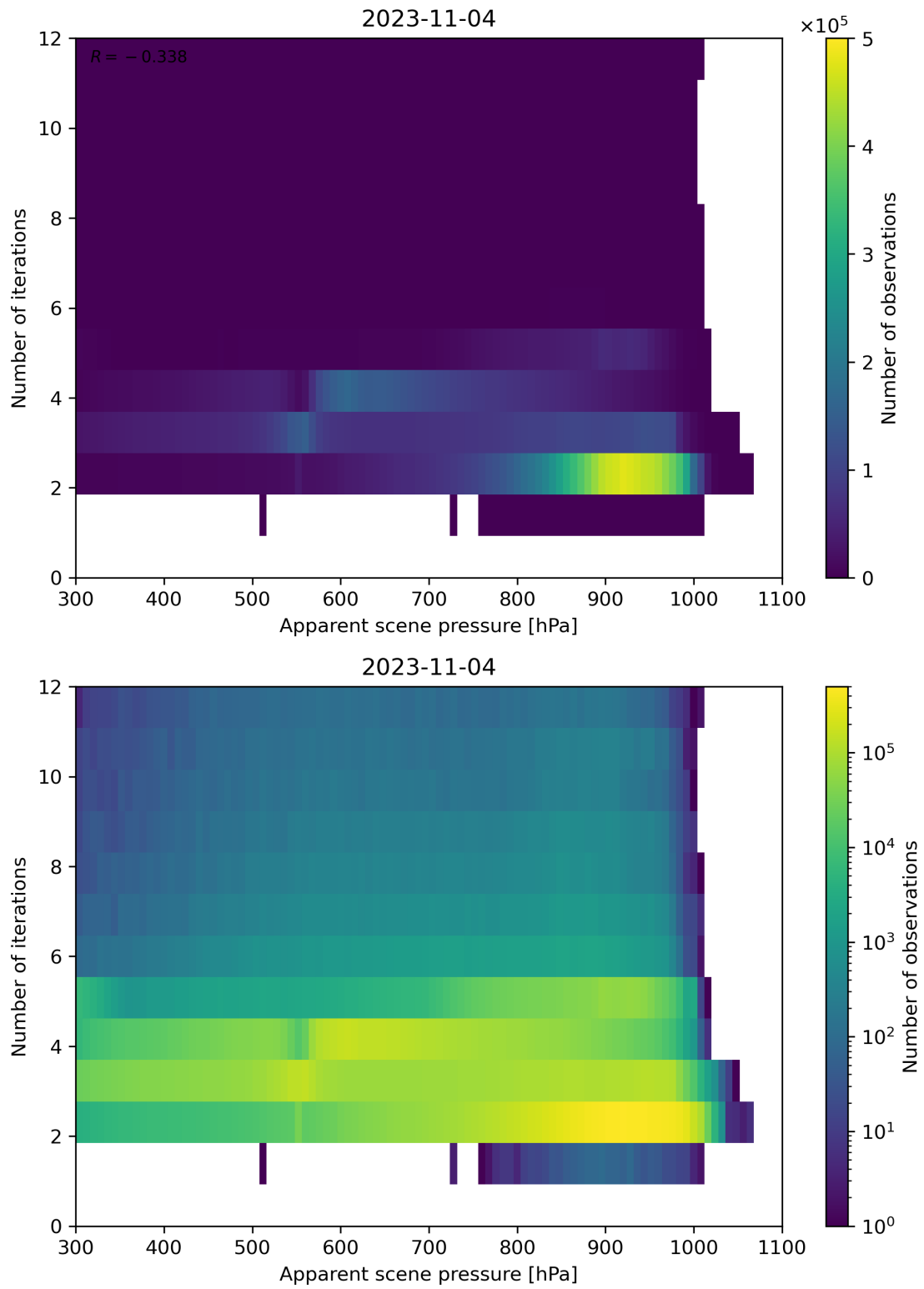
Figure 66: Scatter density plot of “Apparent scene pressure” against “Number of iterations” for 2023-11-03 to 2023-11-05.
