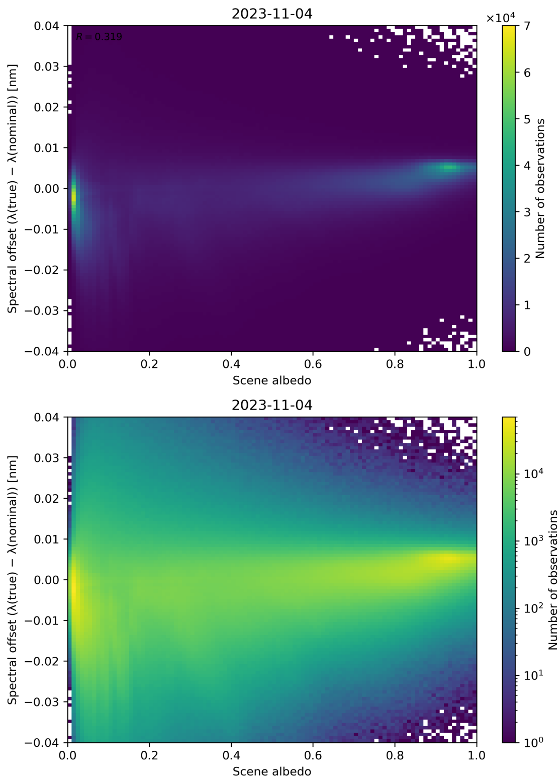
Figure 117: Scatter density plot of “Scene albedo” against “Spectral offset ( \lambda(\text{true}) - \lambda(\text{nominal}) )” for 2023-11-03 to 2023-11-05.
