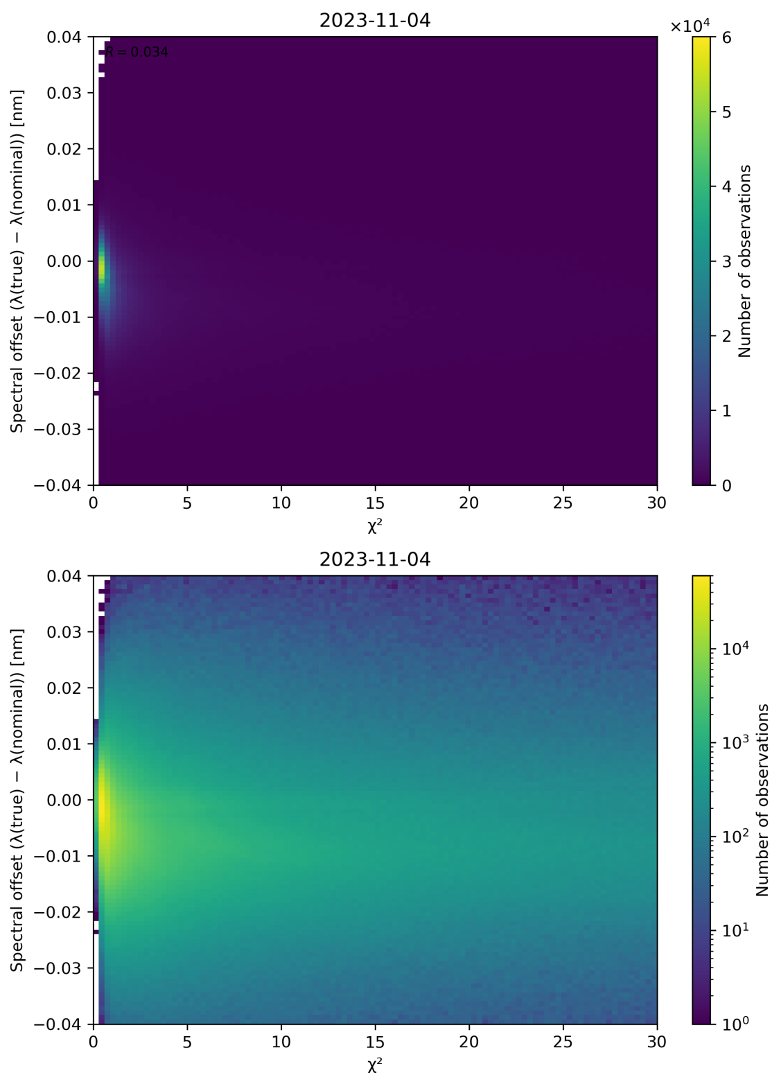
Figure 75: Scatter density plot of “ \chi^2 ” against “Spectral offset ( \lambda(\text{true}) - \lambda(\text{nominal}) )” for 2023-11-03 to 2023-11-05.
