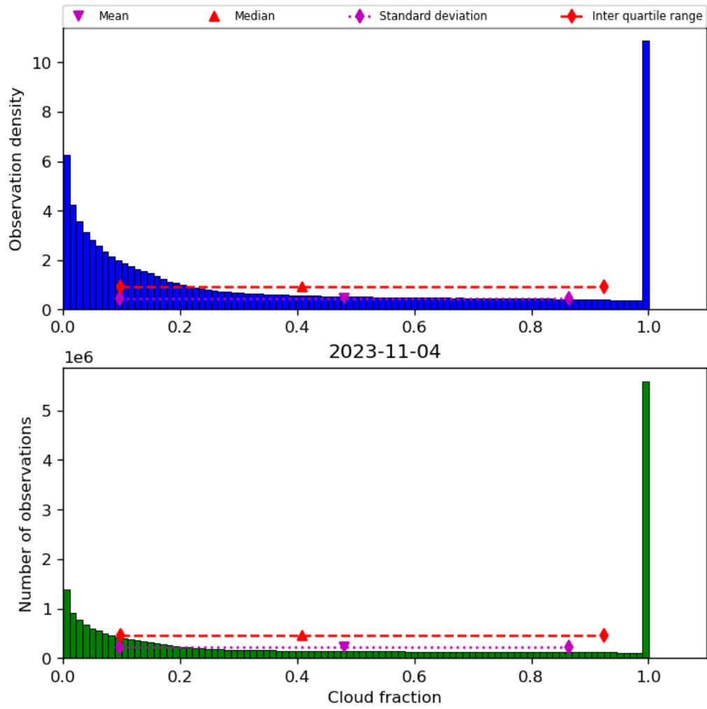
Figure 32: Histogram of “Cloud fraction” for 2023-11-03 to 2023-11-05
