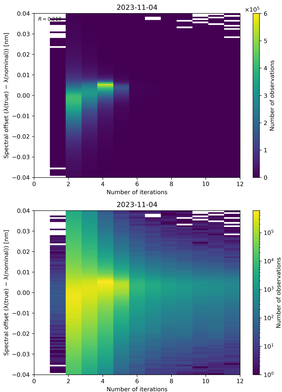
Figure 109: Scatter density plot of “Number of iterations” against “Spectral offset ( \lambda(\text{true}) - \lambda(\text{nominal}) )” for 2023-11-03 to 2023-11-05.
