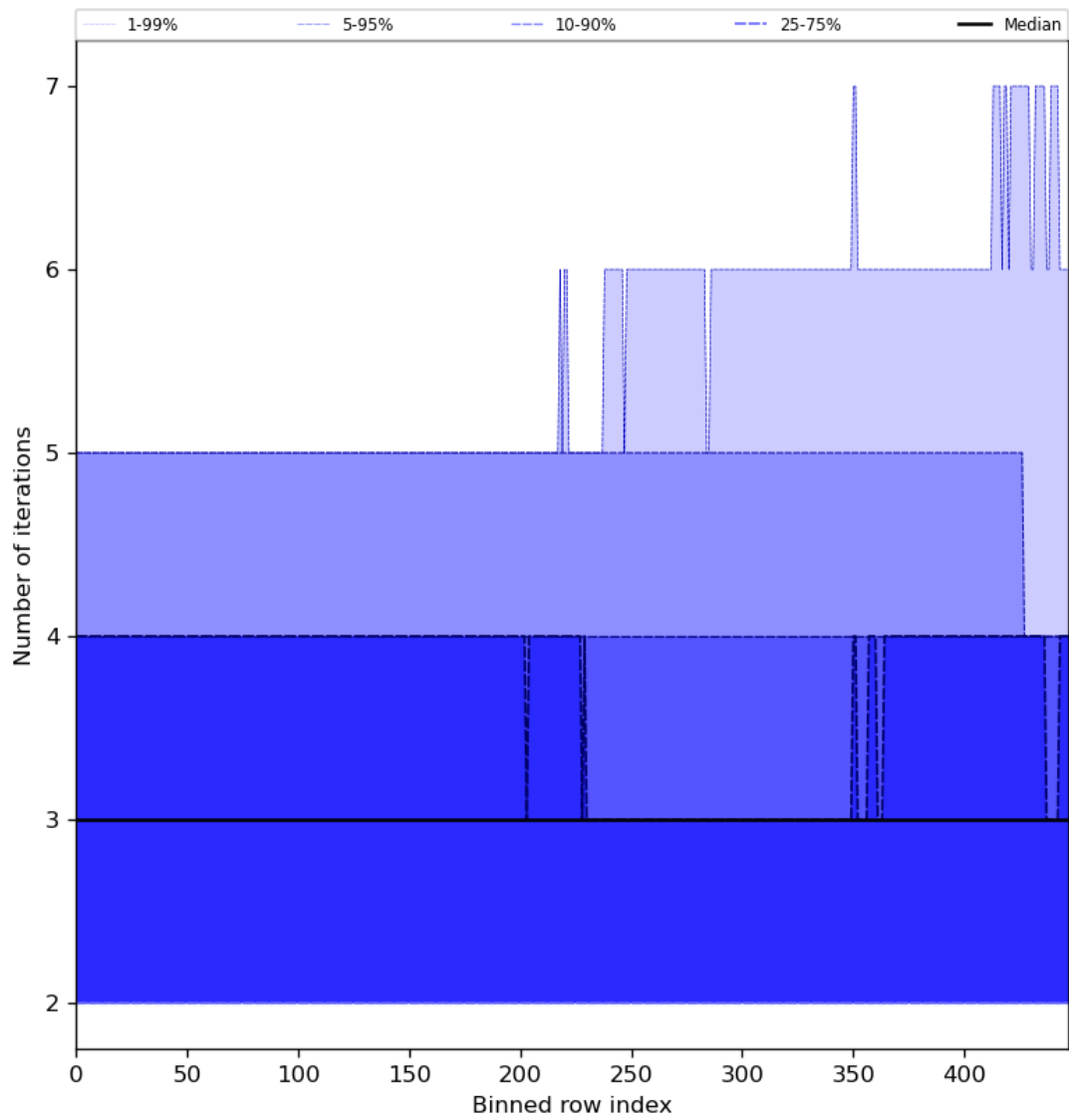
Figure 56: Along track statistics of “Number of iterations” for 2023-11-03 to 2023-11-05
