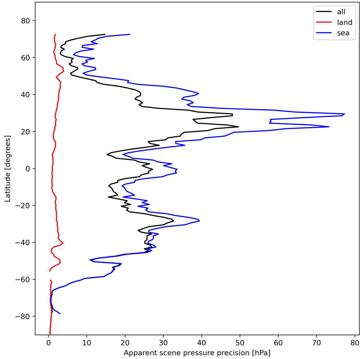
Figure 20: Zonal average of “Apparent scene pressure precision” for 2023-11-03 to 2023-11-05.
