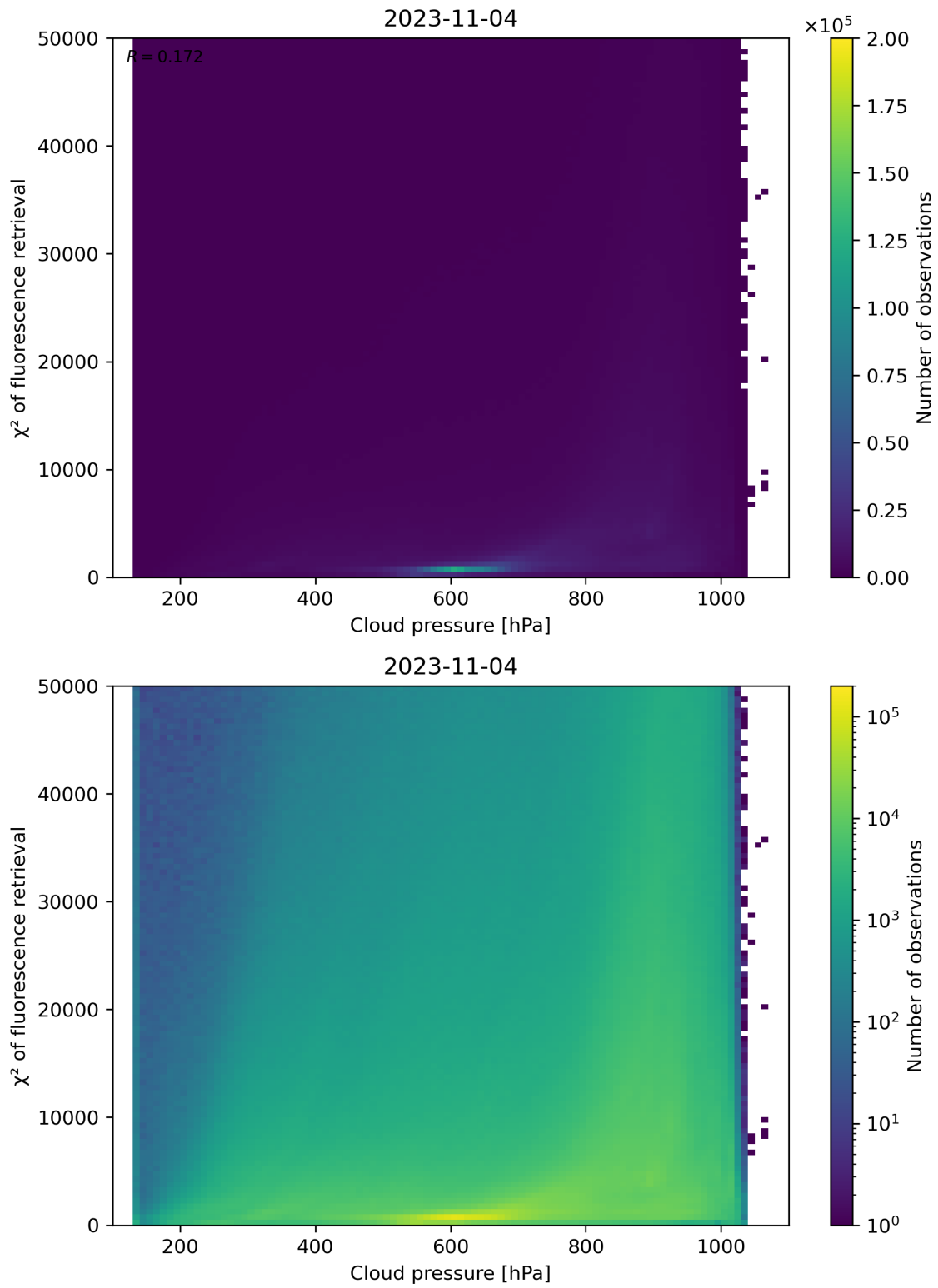
Figure 86: Scatter density plot of “Cloud pressure” against “ \chi^2 of fluorescence retrieval” for 2023-11-03 to 2023-11-05.
