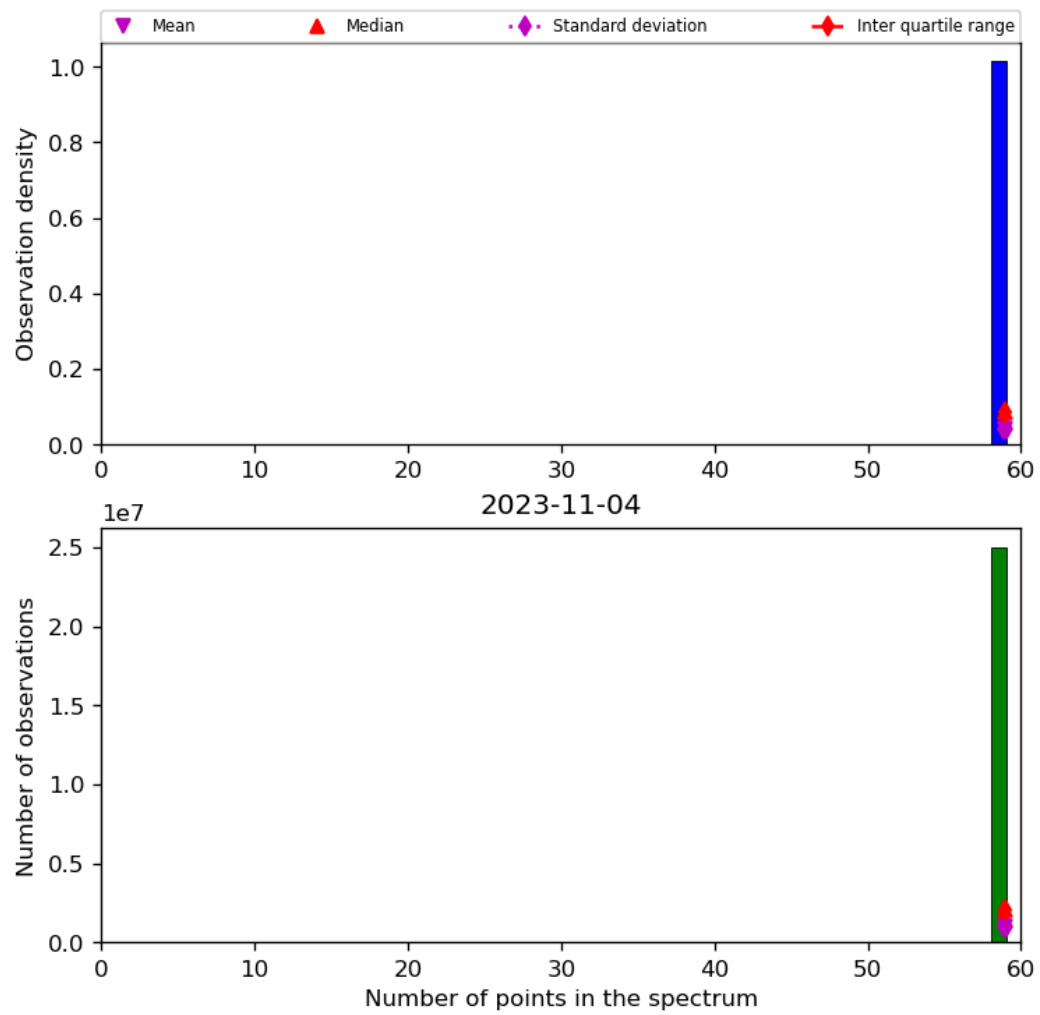
Figure 44: Histogram of “Number of points in the spectrum” for 2023-11-03 to 2023-11-05
