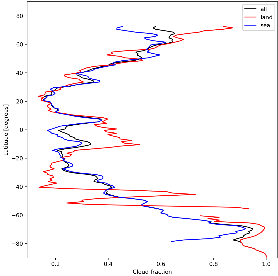
Figure 15: Zonal average of “Cloud fraction” for 2023-11-03 to 2023-11-05.
