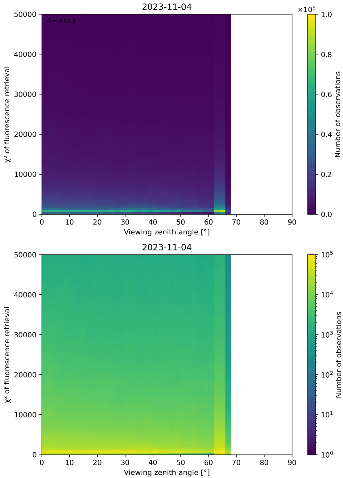
Figure 131: Scatter density plot of “Viewing zenith angle” against “ \chi^2 of fluorescence retrieval” for 2023-11-03 to 2023-11-05.
