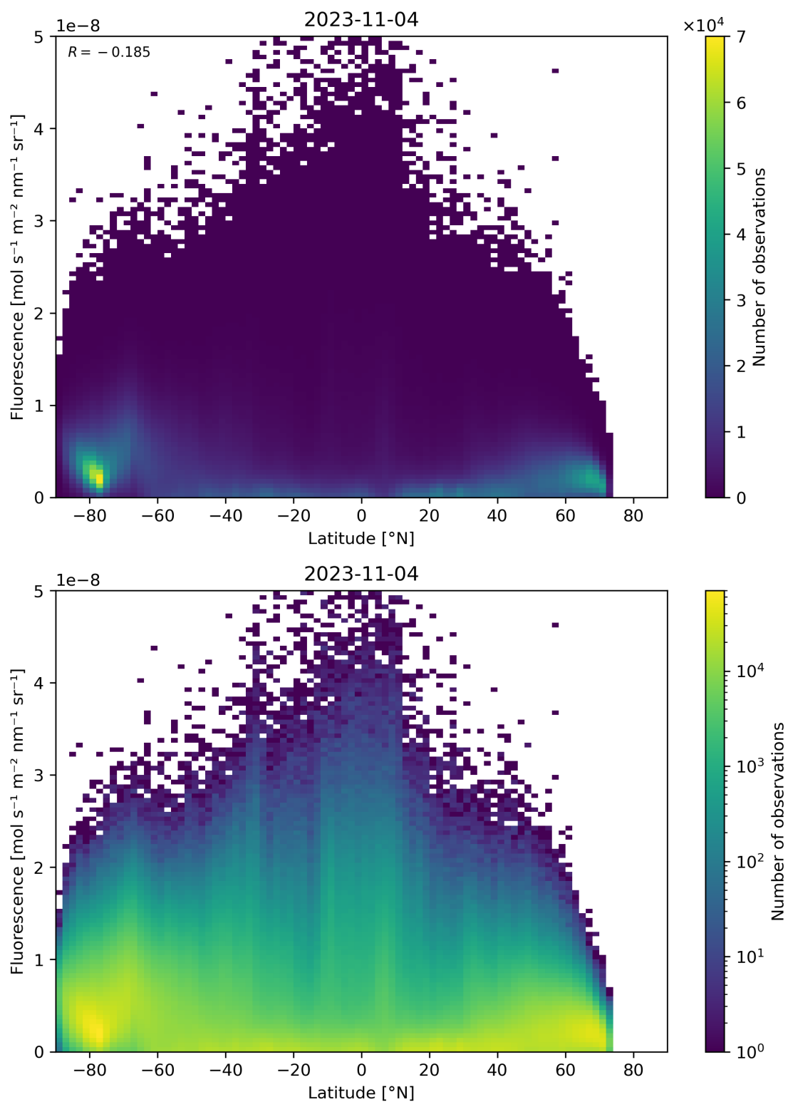
Figure 101: Scatter density plot of “Latitude” against “Fluorescence” for 2023-11-03 to 2023-11-05.
