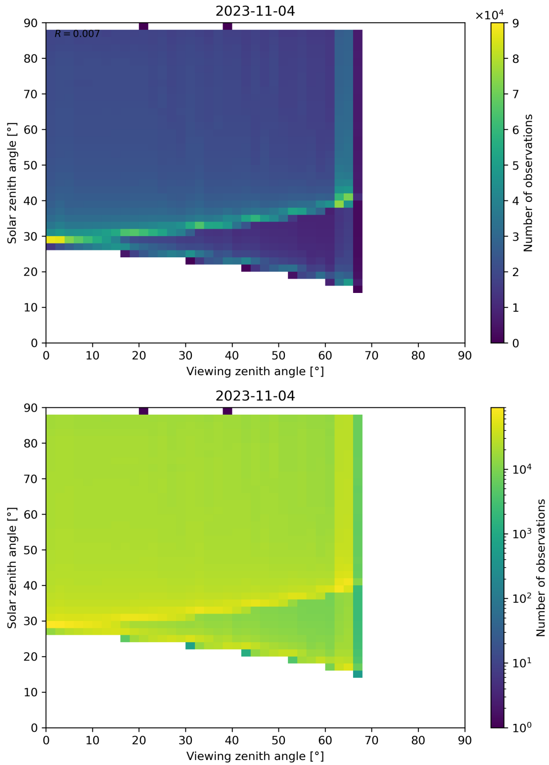
Figure 139: Scatter density plot of “Viewing zenith angle” against “Solar zenith angle” for 2023-11-03 to 2023-11-05.
