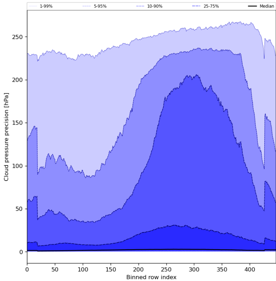
Figure 48: Along track statistics of “Cloud pressure precision” for 2023-11-03 to 2023-11-05
