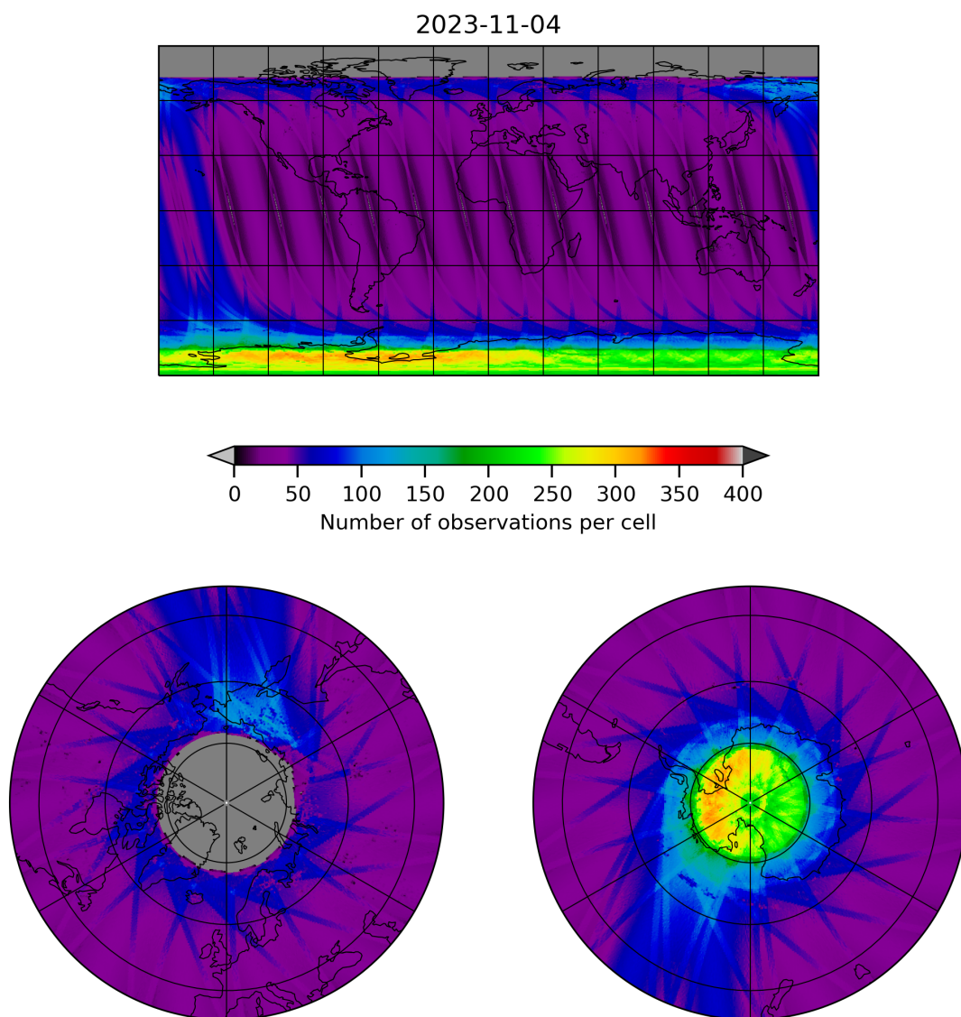
Figure 11: Map of the number of observations for 2023-11-03 to 2023-11-05
