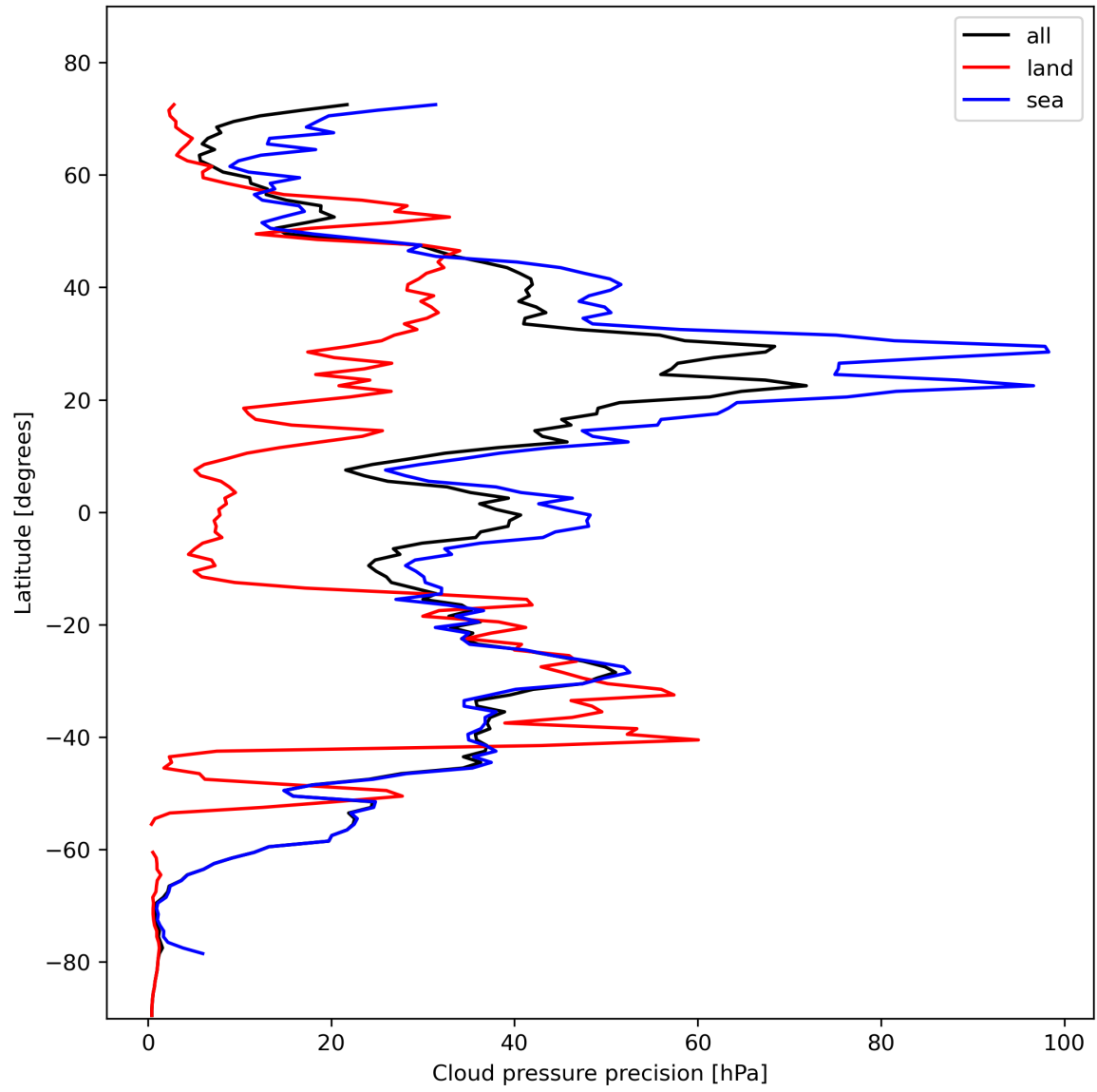
Figure 14: Zonal average of “Cloud pressure precision” for 2023-11-03 to 2023-11-05.
