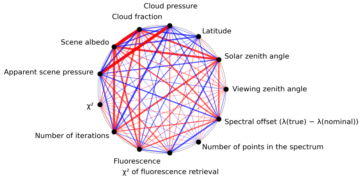
Figure 1: Map of correlation graph for 2023-11-03 to 2023-11-05.
