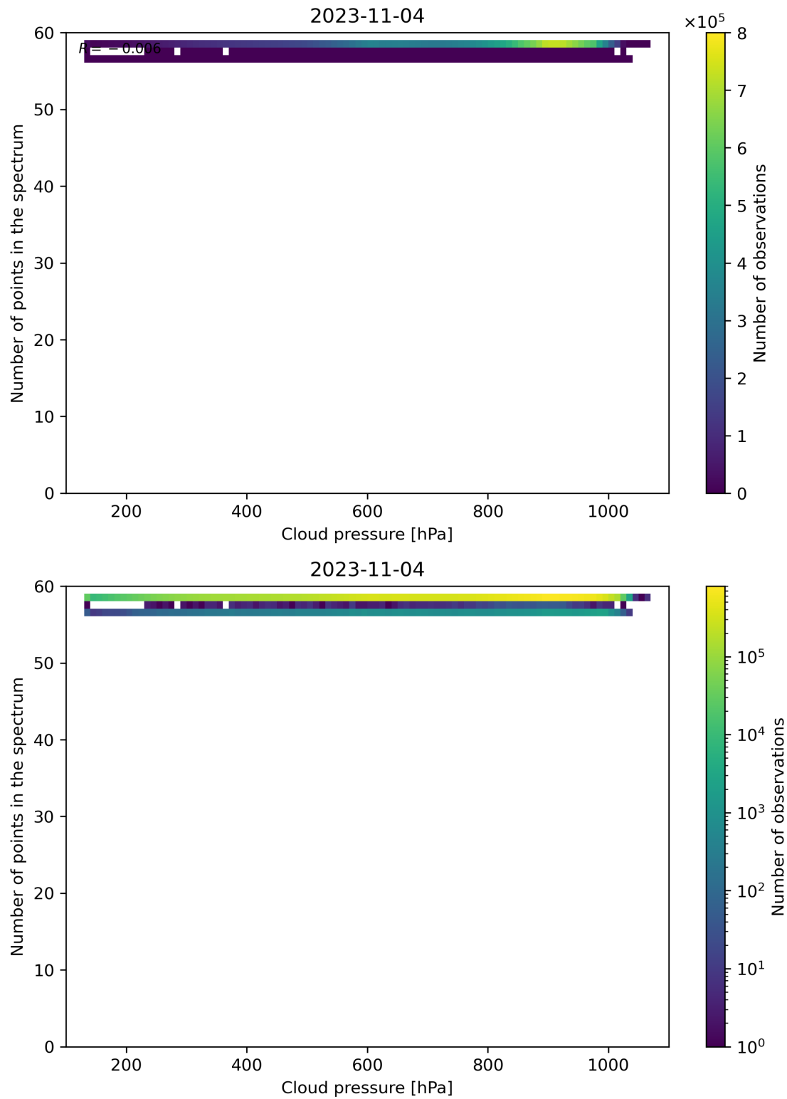
Figure 90: Scatter density plot of “Cloud pressure” against “Number of points in the spectrum” for 2023-11-03 to 2023-11-05.
