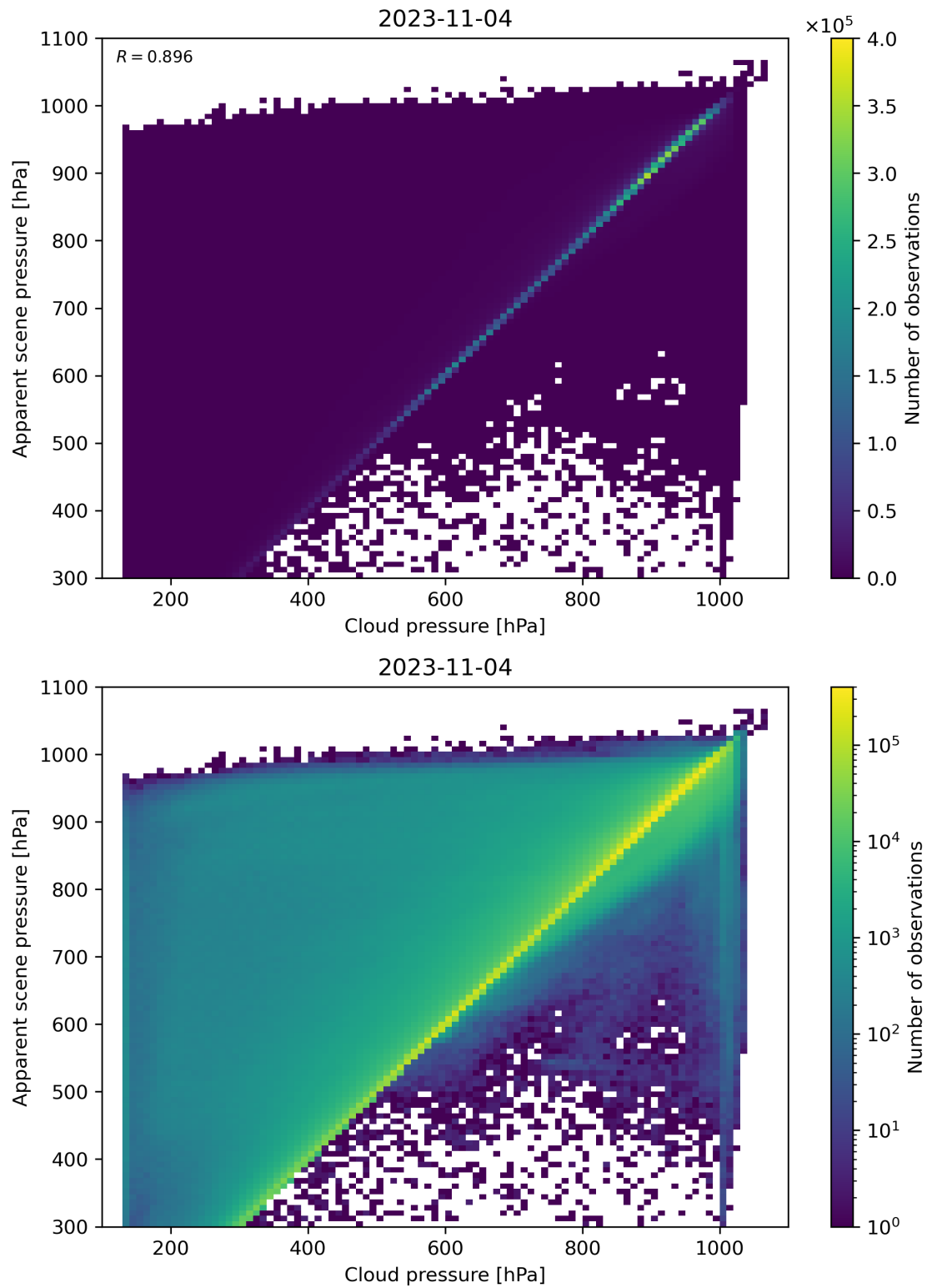
Figure 84: Scatter density plot of “Cloud pressure” against “Apparent scene pressure” for 2023-11-03 to 2023-11-05.
