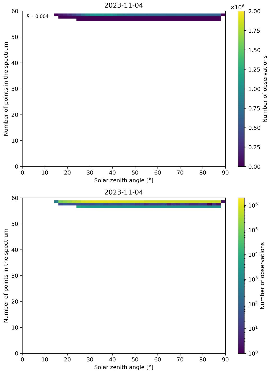
Figure 126: Scatter density plot of “Solar zenith angle” against “Number of points in the spectrum” for 2023-11-03 to 2023-11-05.
