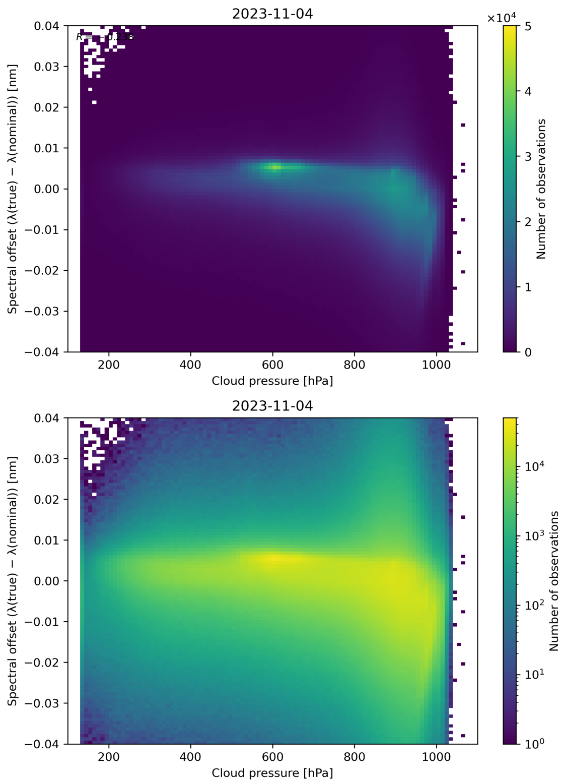
Figure 92: Scatter density plot of “Cloud pressure” against “Spectral offset ( \lambda(\text{true}) - \lambda(\text{nominal}) )” for 2023-11-03 to 2023-11-05.
