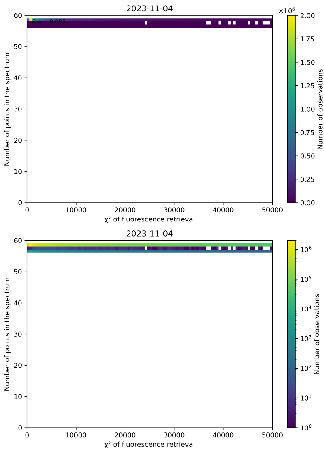
Figure 71: Scatter density plot of " \chi^2 of fluorescence retrieval" against "Number of points in the spectrum" for 2023-11-03 to 2023-11-05.
