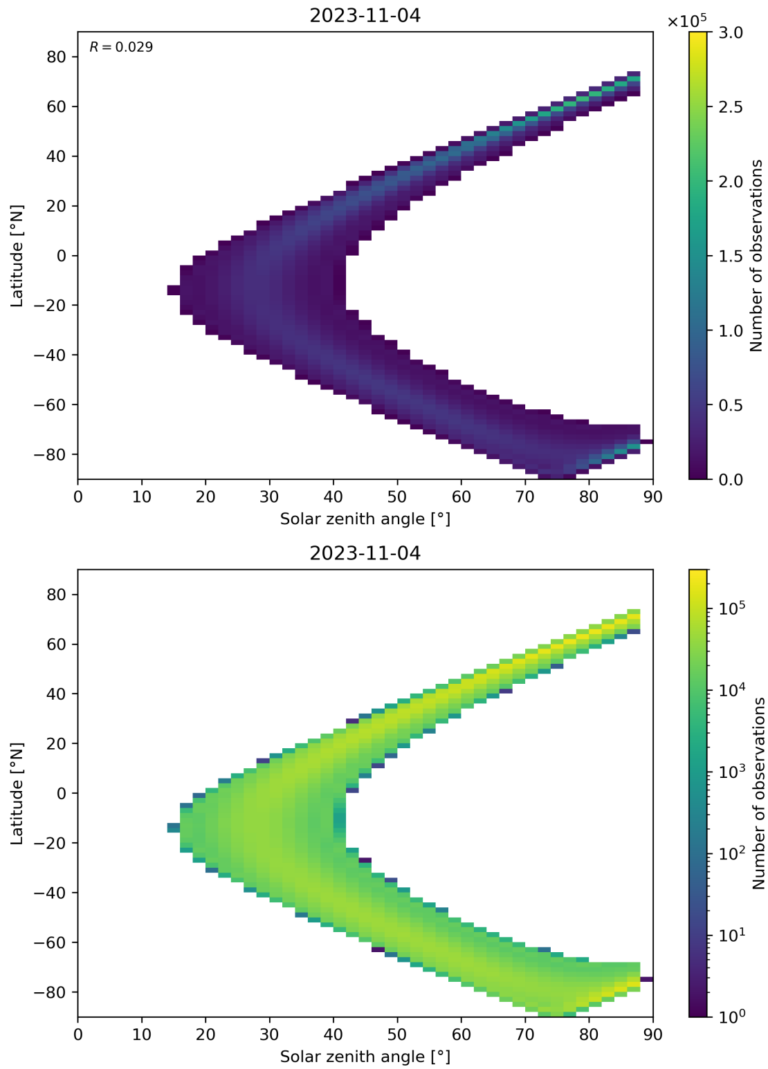
Figure 124: Scatter density plot of “Solar zenith angle” against “Latitude” for 2023-11-03 to 2023-11-05.
