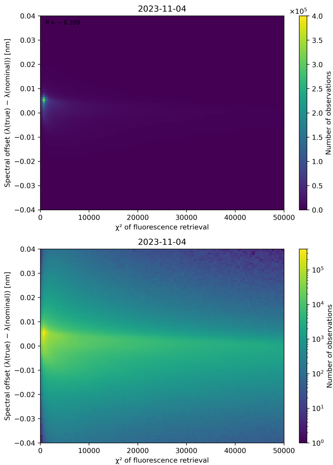
Figure 72: Scatter density plot of " \chi^2 of fluorescence retrieval" against "Spectral offset ( \lambda(\text{true}) - \lambda(\text{nominal})) " for 2023-11-03 to 2023-11-05.
