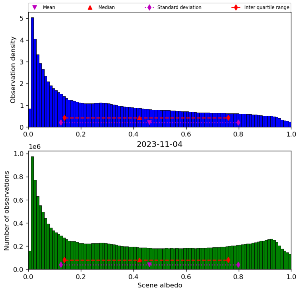
Figure 34: Histogram of “Scene albedo” for 2023-11-03 to 2023-11-05
