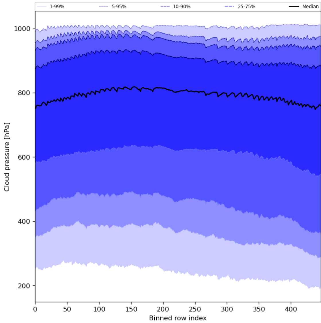
Figure 47: Along track statistics of "Cloud pressure" for 2023-11-03 to 2023-11-05
