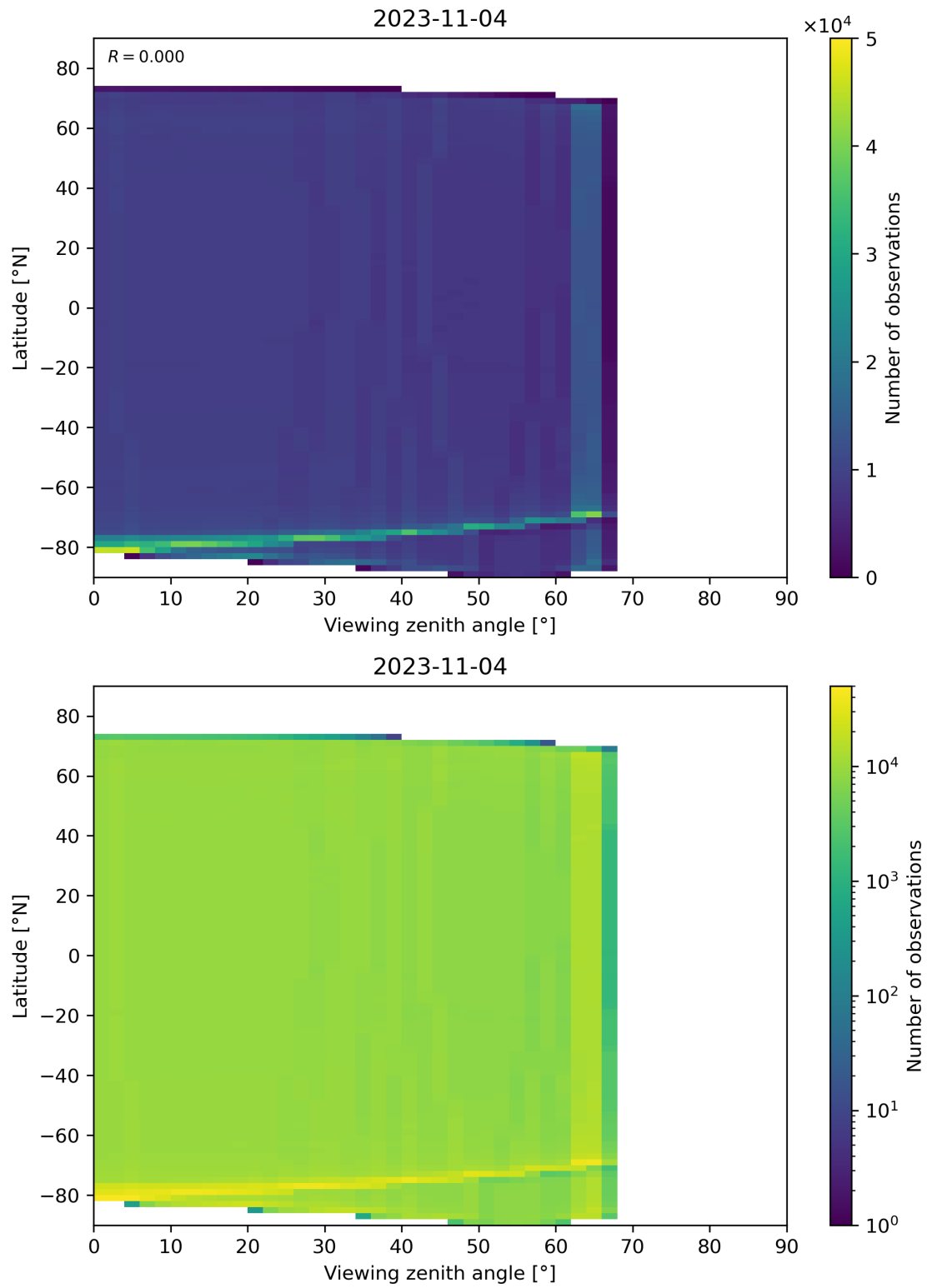
Figure 135: Scatter density plot of “Viewing zenith angle” against “Latitude” for 2023-11-03 to 2023-11-05.
