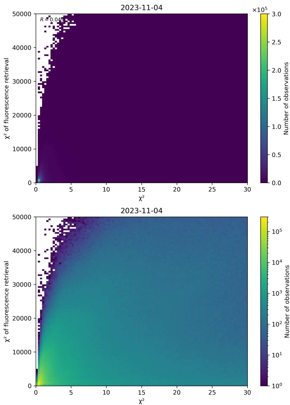
Figure 69: Scatter density plot of “ \chi^2 ” against “ \chi^2 of fluorescence retrieval” for 2023-11-03 to 2023-11-05.
