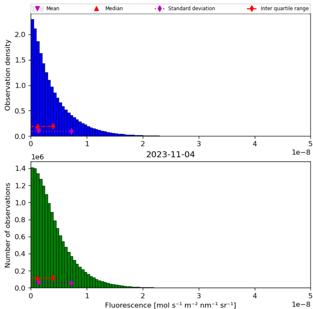
Figure 40: Histogram of “Fluorescence” for 2023-11-03 to 2023-11-05
