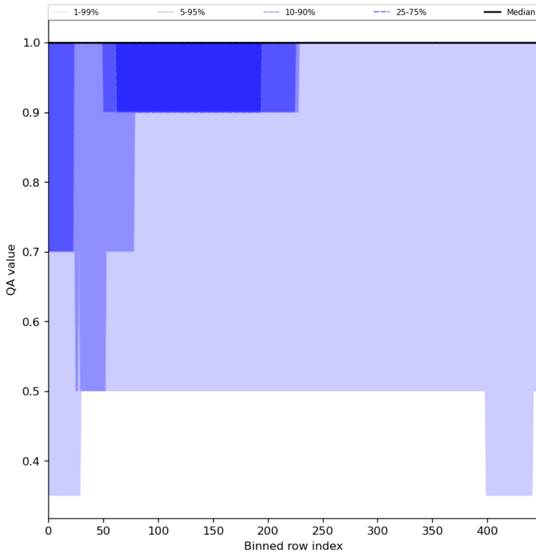
Figure 46: Along track statistics of “QA value” for 2023-11-03 to 2023-11-05
