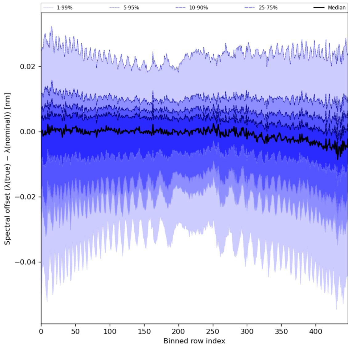
Figure 62: Along track statistics of “Spectral offset ( \lambda(\text{true}) - \lambda(\text{nominal}) )” for 2023-11-03 to 2023-11-05
