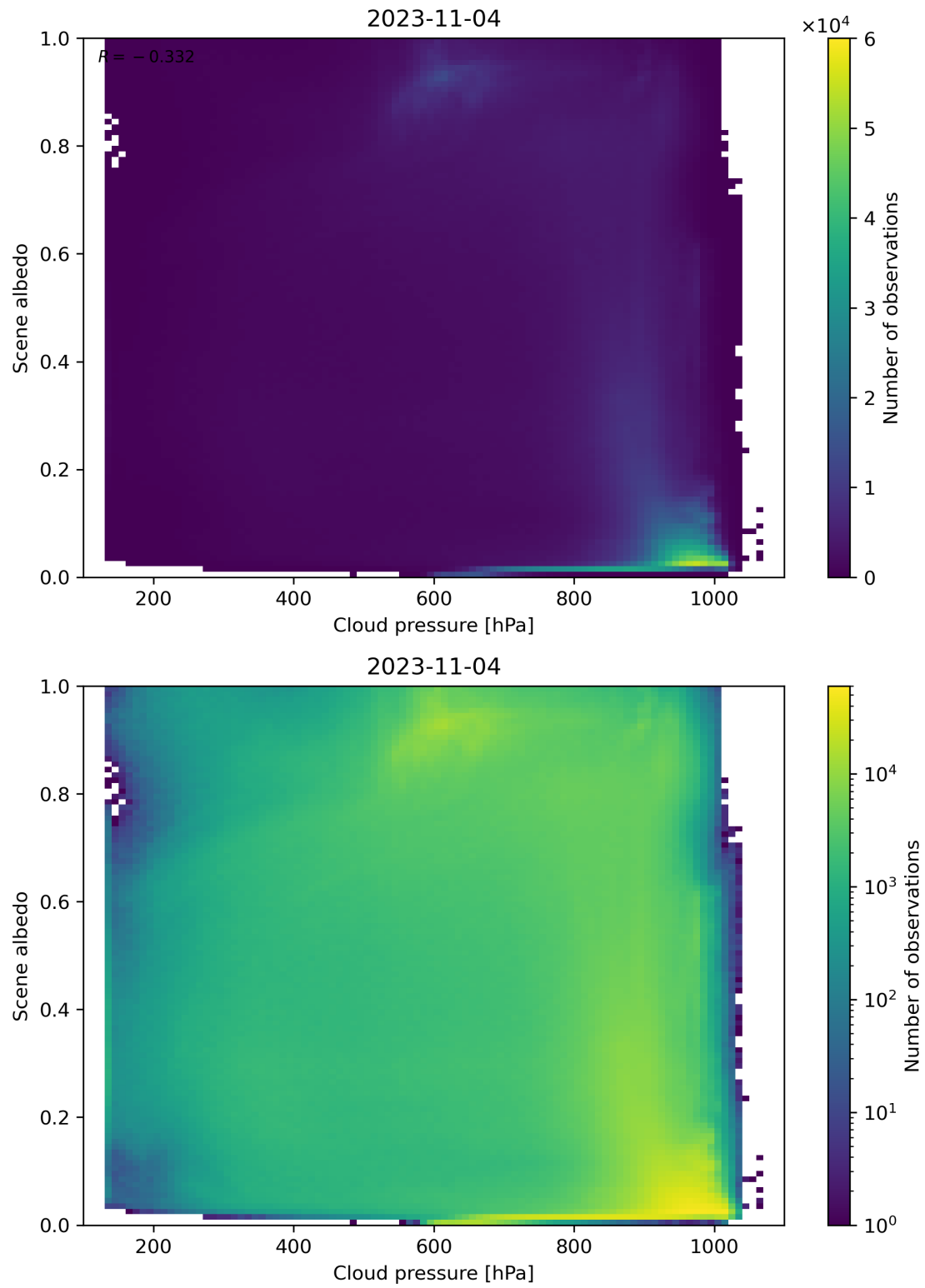
Figure 91: Scatter density plot of “Cloud pressure” against “Scene albedo” for 2023-11-03 to 2023-11-05.
