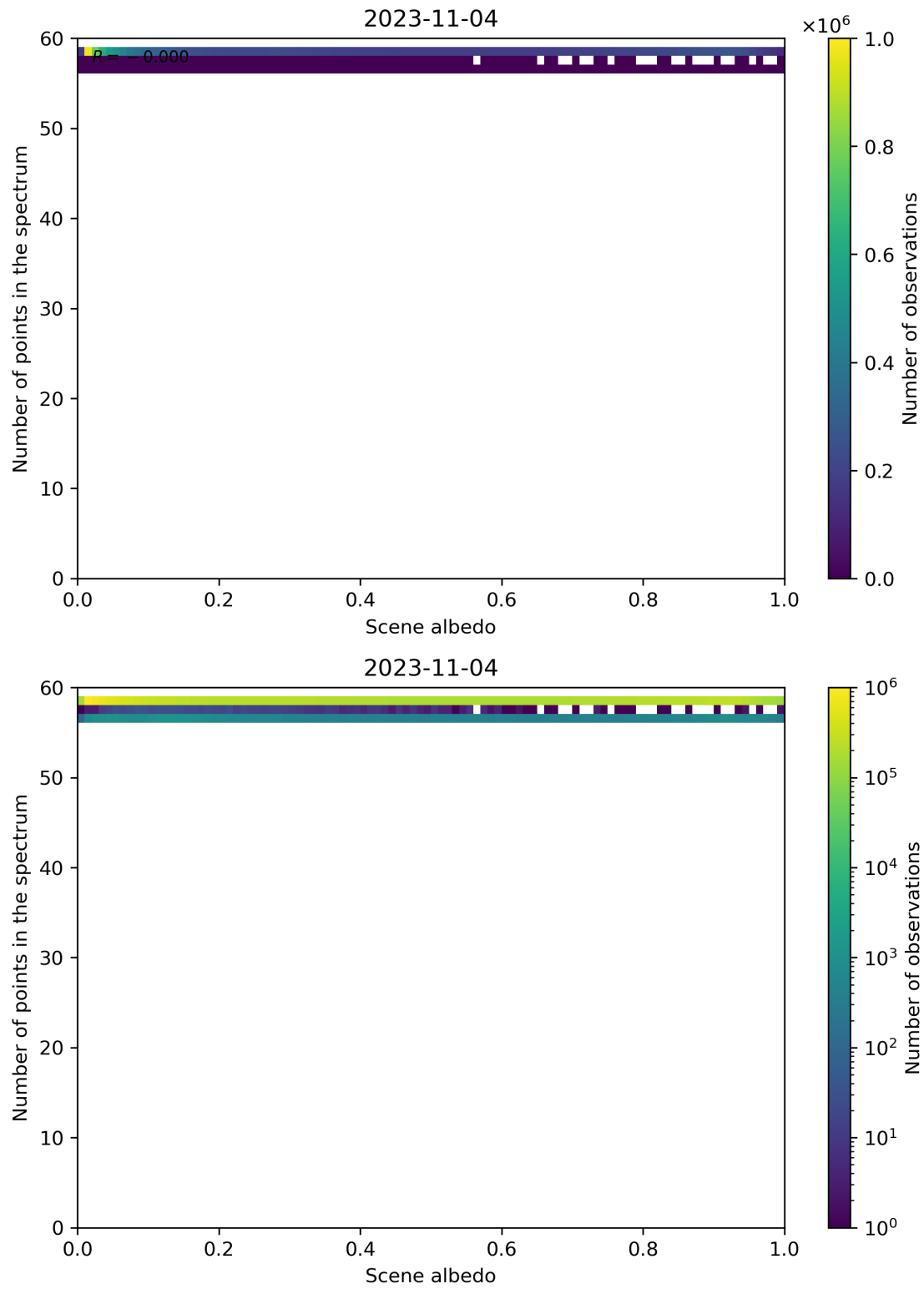
Figure 116: Scatter density plot of “Scene albedo” against “Number of points in the spectrum” for 2023-11-03 to 2023-11-05.
