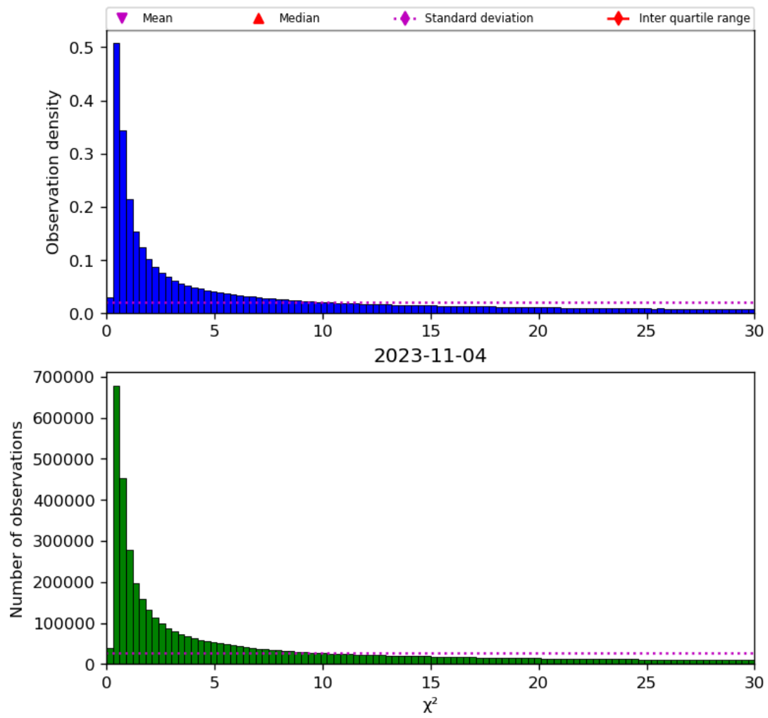
Figure 38: Histogram of " \chi^2 " for 2023-11-03 to 2023-11-05
