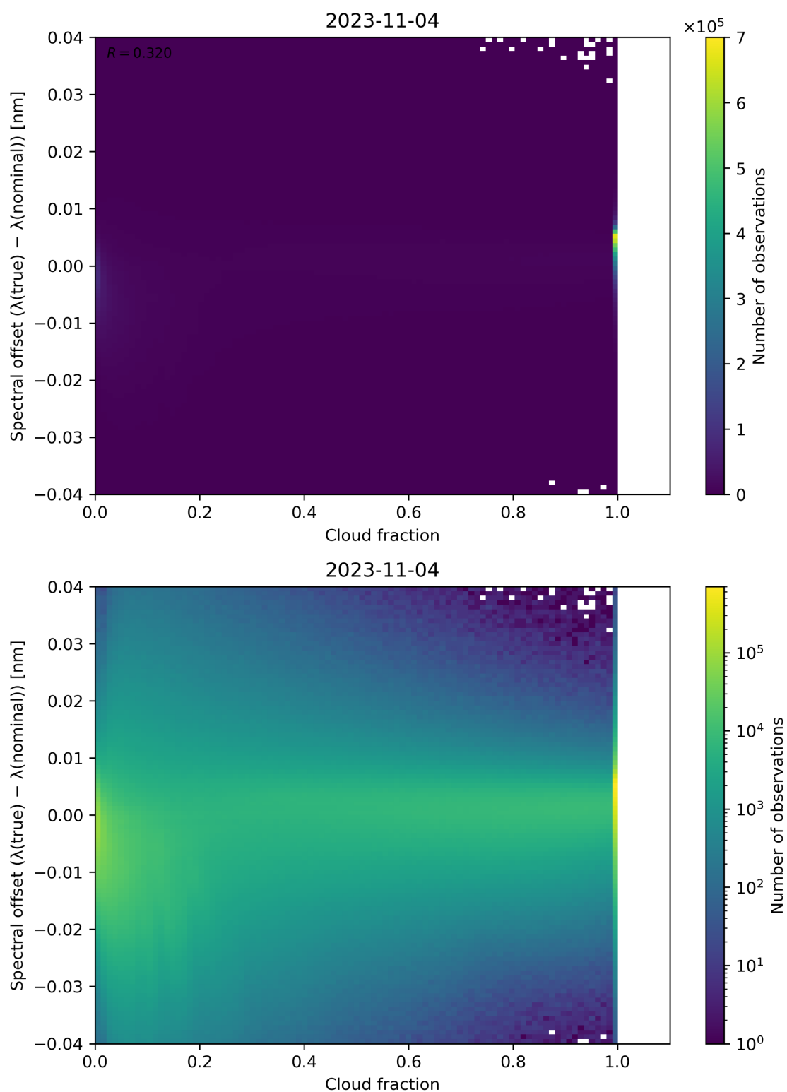
Figure 83: Scatter density plot of “Cloud fraction” against “Spectral offset ( \lambda(\text{true}) - \lambda(\text{nominal}) )” for 2023-11-03 to 2023-11-05.
