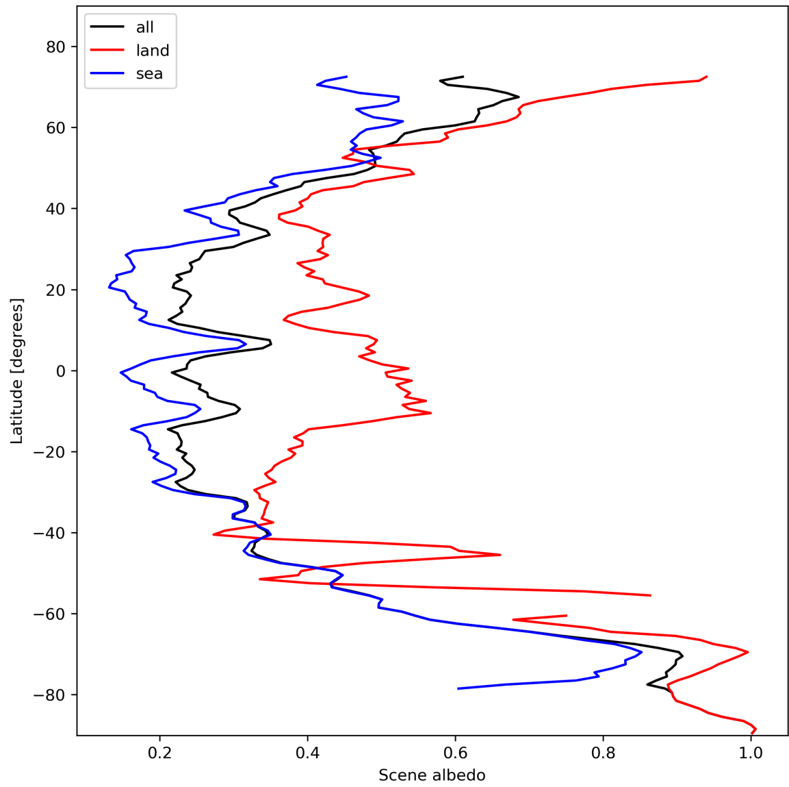
Figure 17: Zonal average of “Scene albedo” for 2023-11-03 to 2023-11-05.
