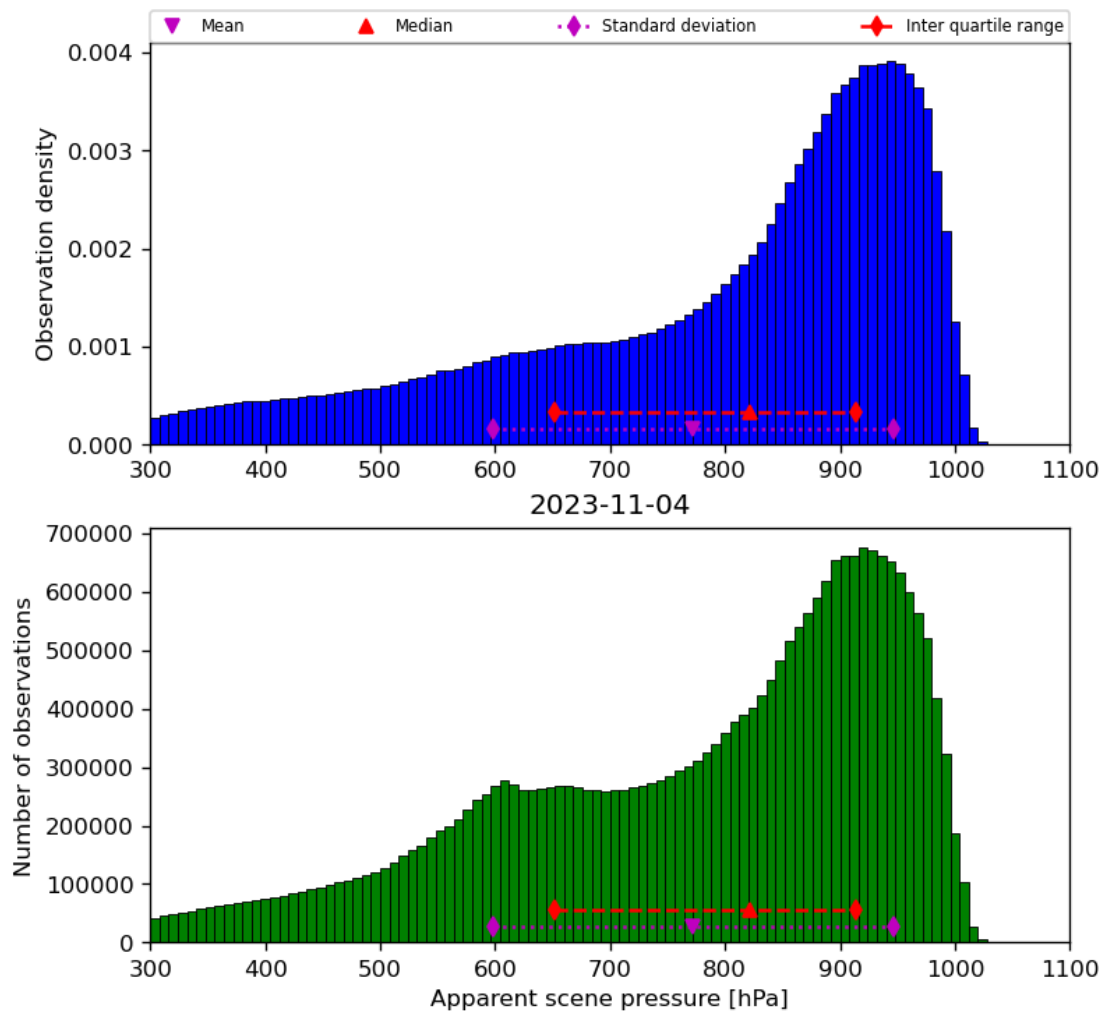
Figure 36: Histogram of “Apparent scene pressure” for 2023-11-03 to 2023-11-05
