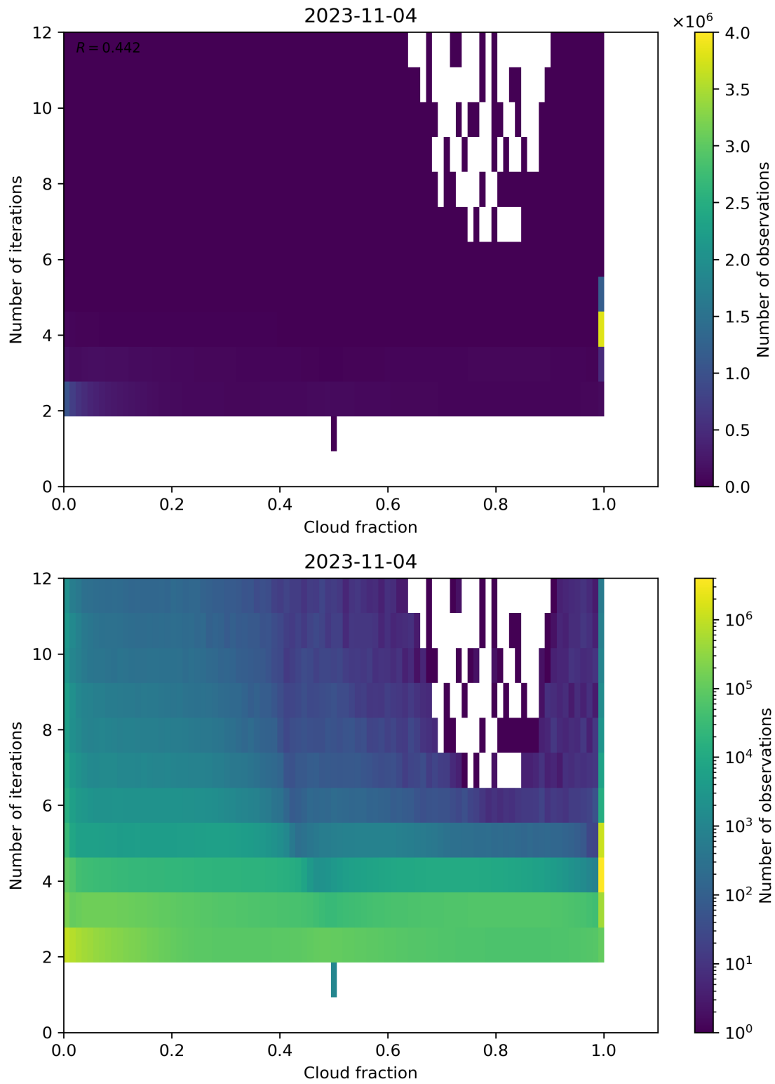
Figure 80: Scatter density plot of “Cloud fraction” against “Number of iterations” for 2023-11-03 to 2023-11-05.
