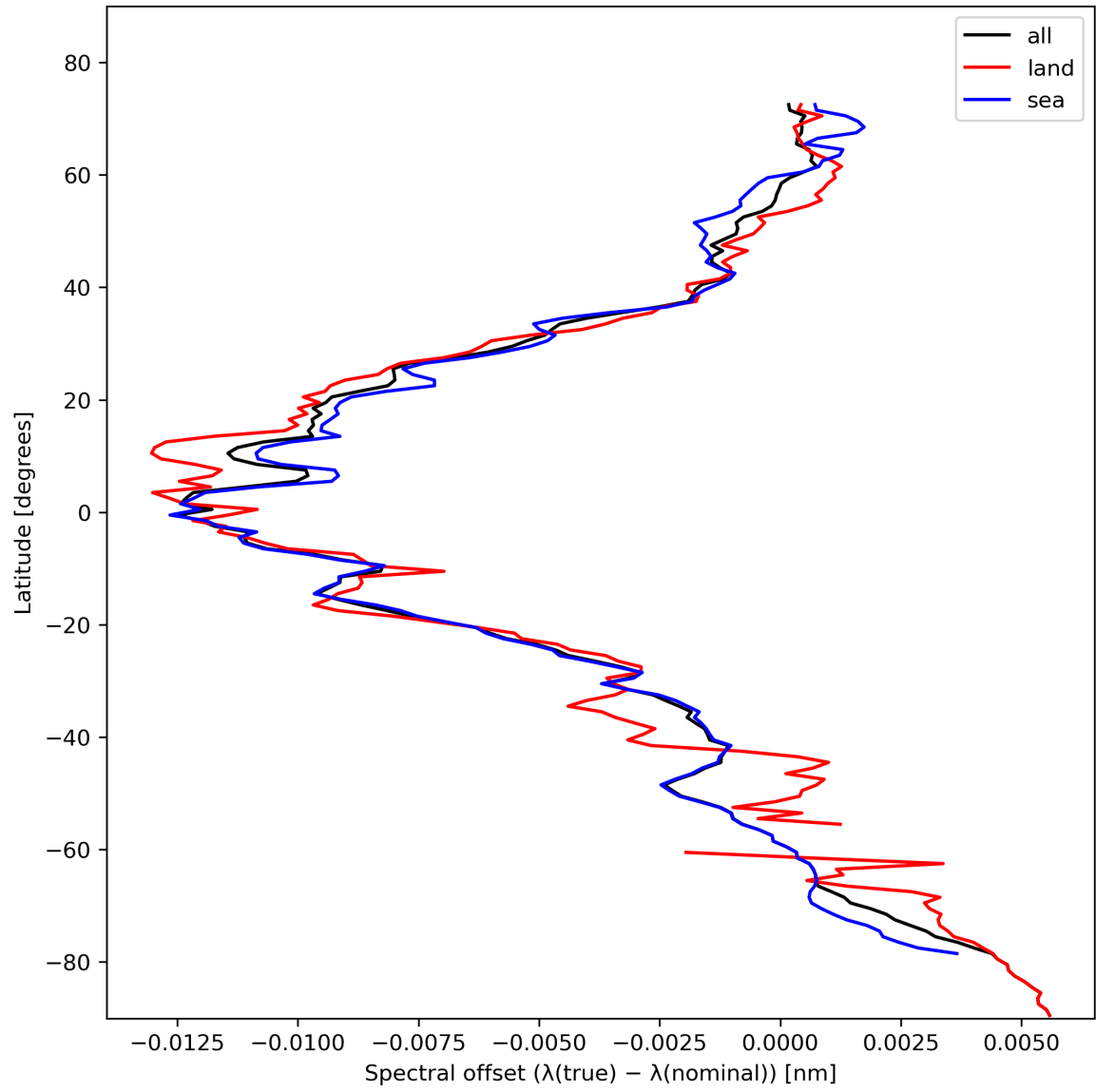
Figure 28: Zonal average of “Spectral offset ( \lambda(\text{true}) - \lambda(\text{nominal}) )” for 2023-11-03 to 2023-11-05.
