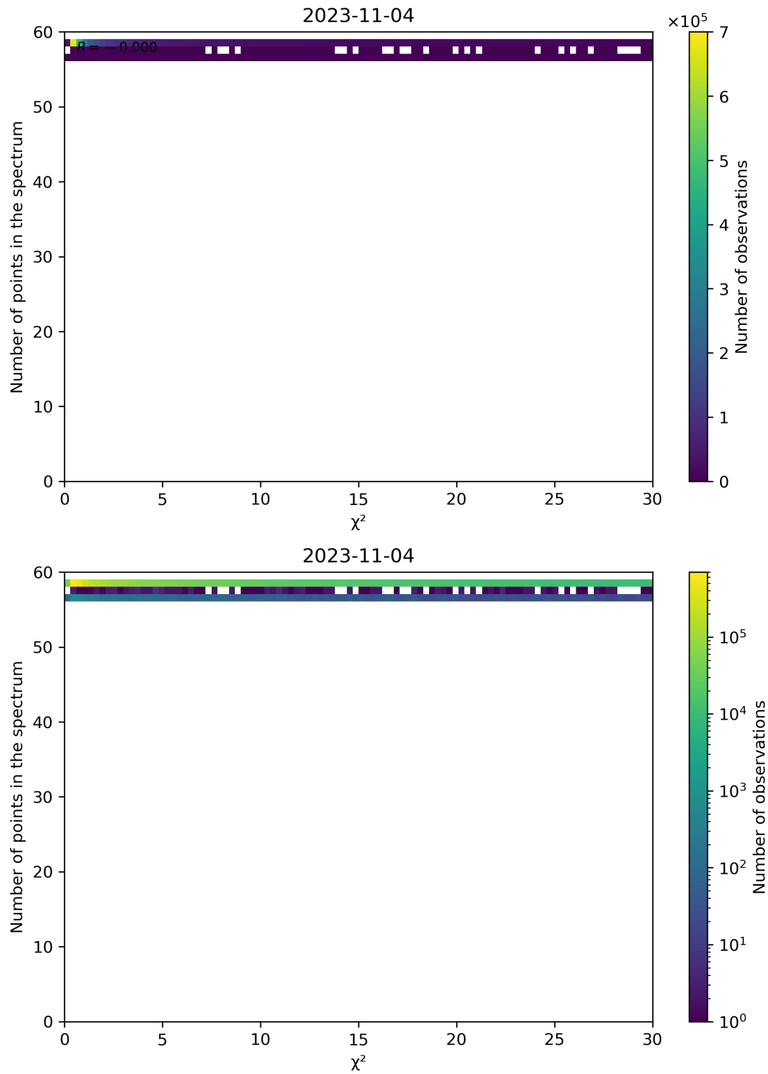
Figure 74: Scatter density plot of " \chi^2 " against "Number of points in the spectrum" for 2023-11-03 to 2023-11-05.
