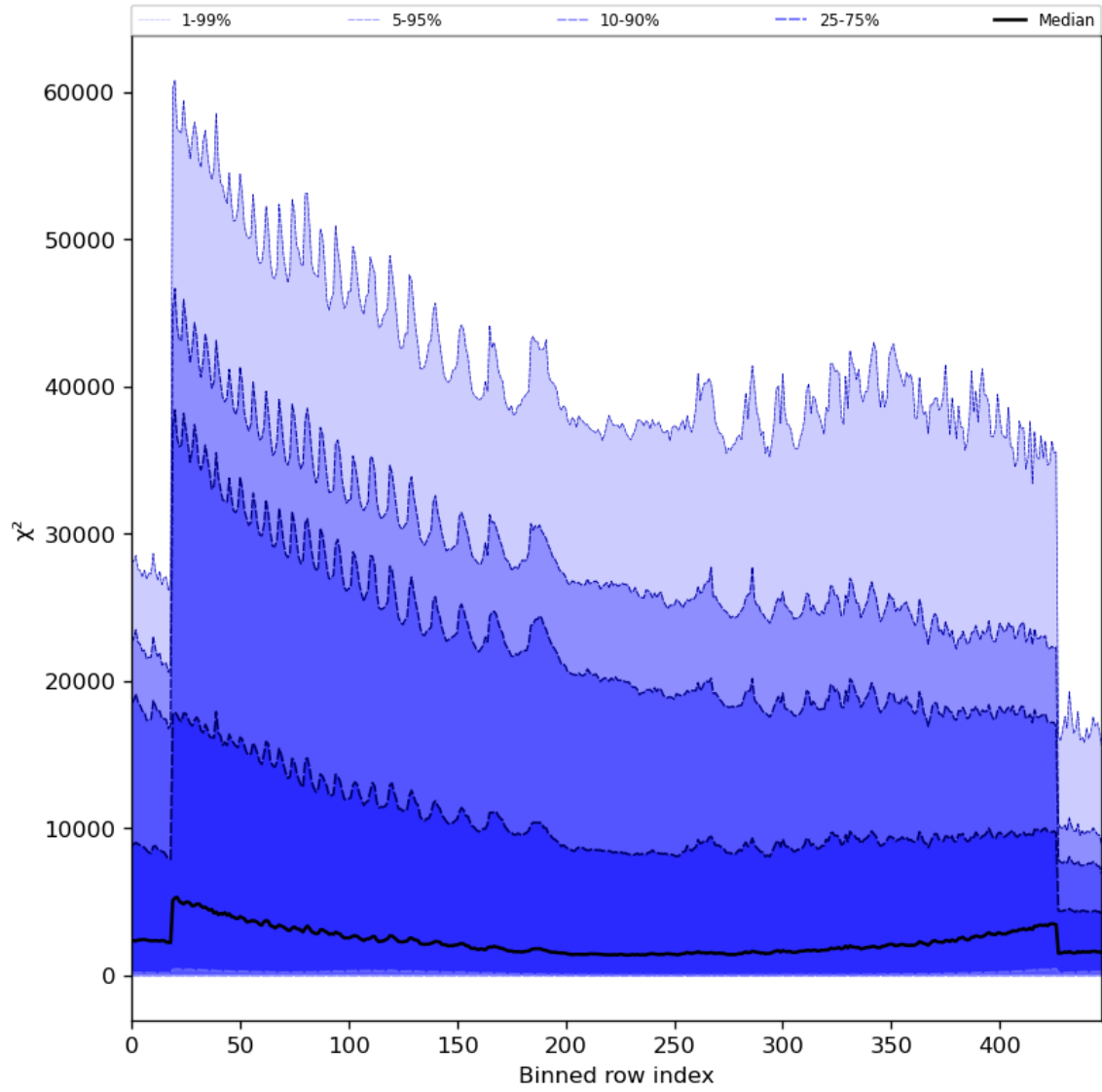
Figure 55: Along track statistics of “ \chi^2 ” for 2023-11-03 to 2023-11-05
