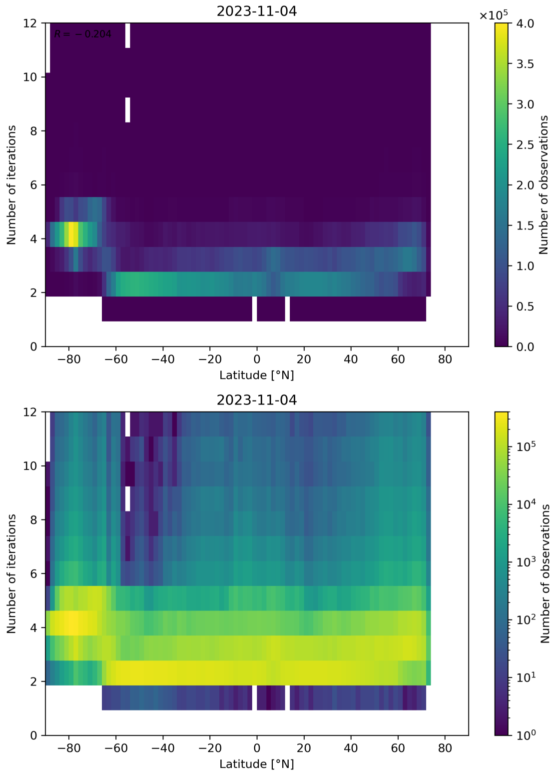
Figure 102: Scatter density plot of “Latitude” against “Number of iterations” for 2023-11-03 to 2023-11-05.
