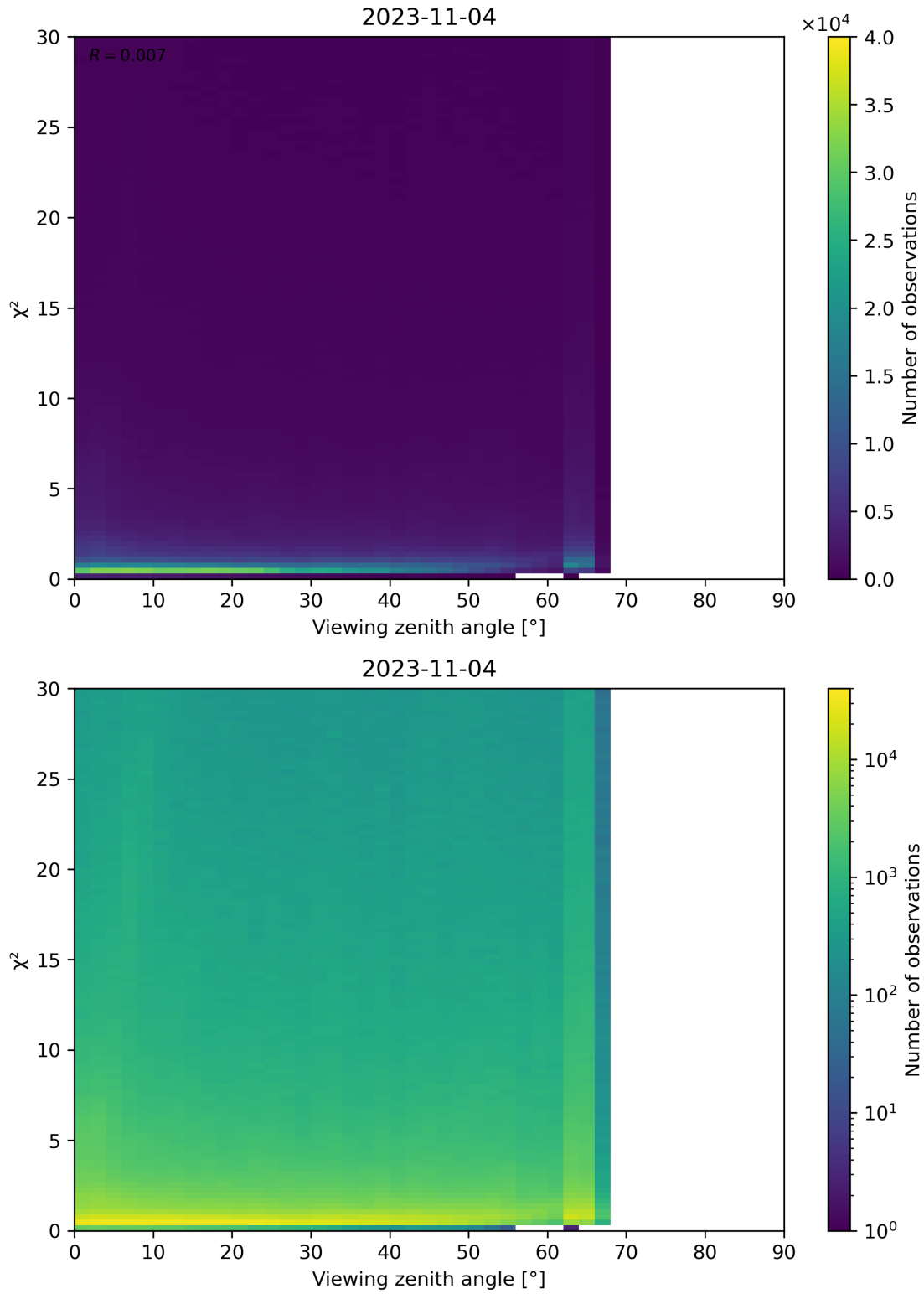
Figure 130: Scatter density plot of “Viewing zenith angle” against “ \chi^2 ” for 2023-11-03 to 2023-11-05.
