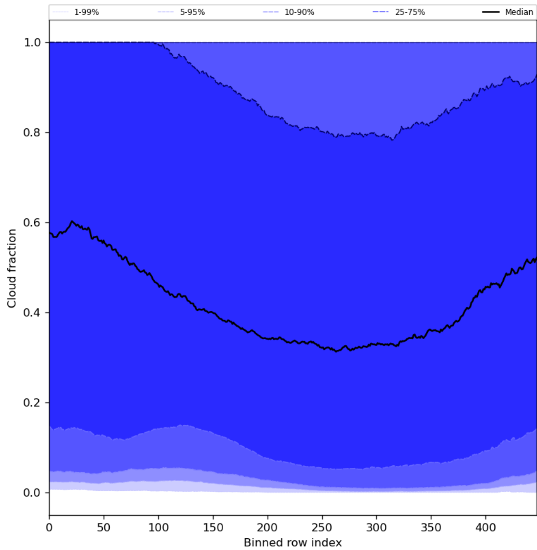
Figure 49: Along track statistics of “Cloud fraction” for 2023-11-03 to 2023-11-05
