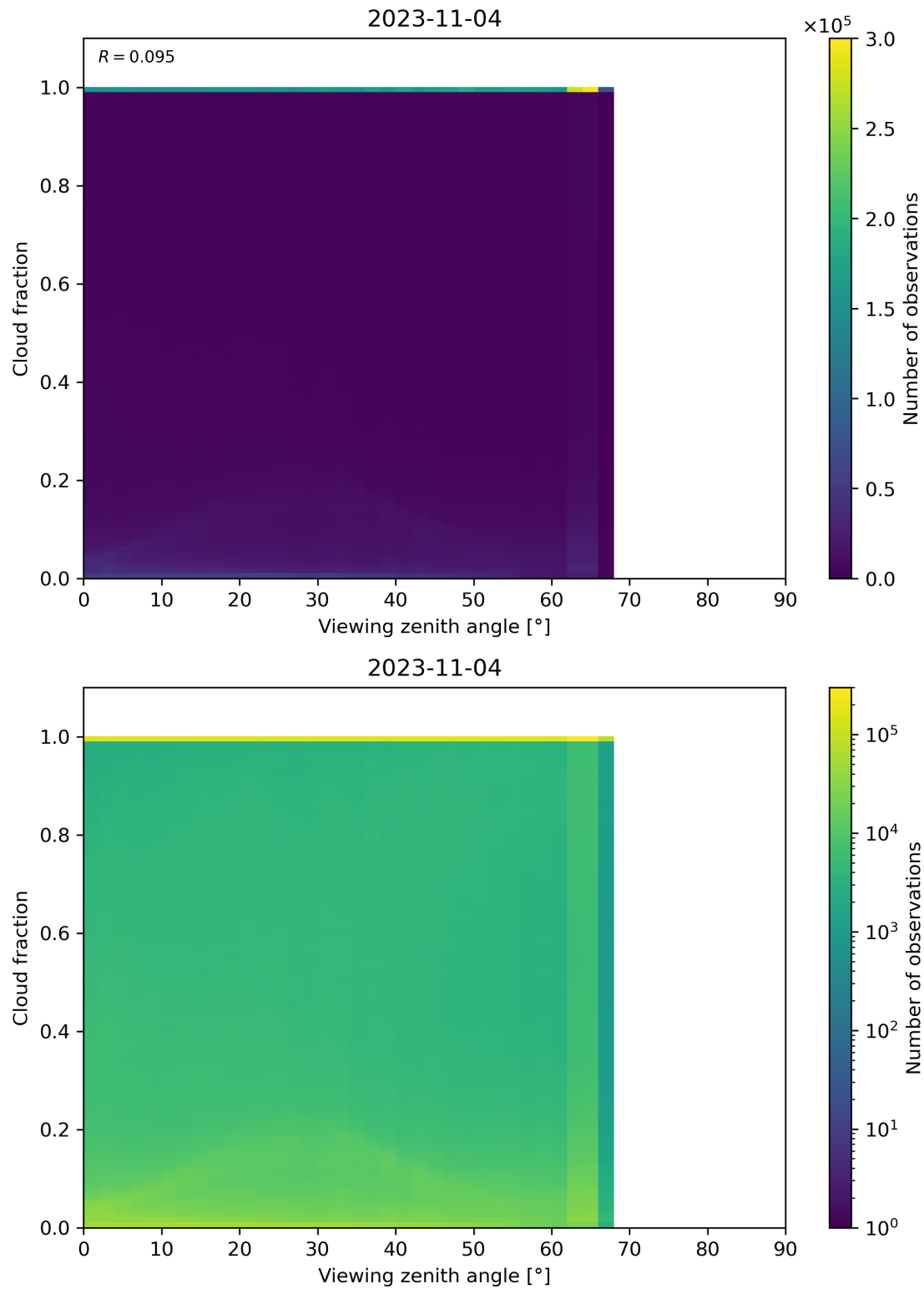
Figure 132: Scatter density plot of “Viewing zenith angle” against “Cloud fraction” for 2023-11-03 to 2023-11-05.
