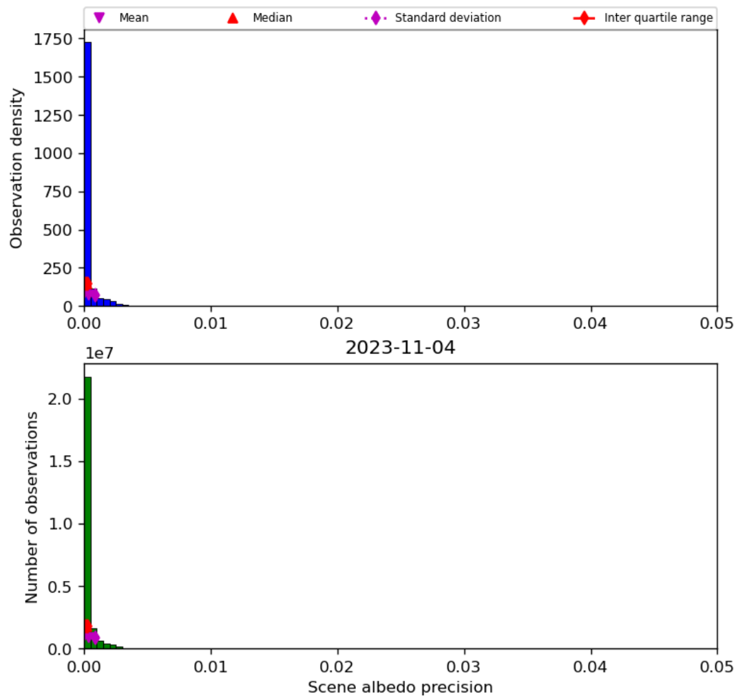
Figure 35: Histogram of “Scene albedo precision” for 2023-11-03 to 2023-11-05
