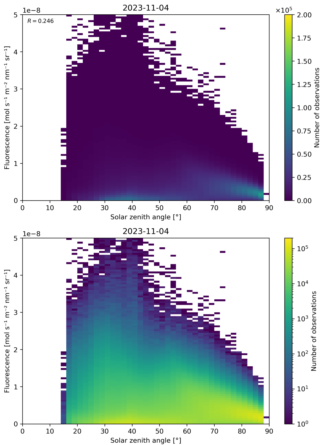
Figure 123: Scatter density plot of “Solar zenith angle” against “Fluorescence” for 2023-11-03 to 2023-11-05.
