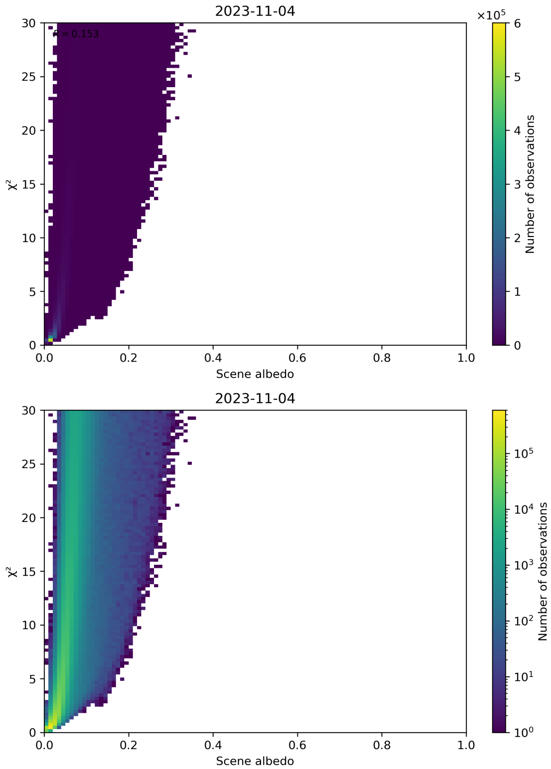
Figure 112: Scatter density plot of “Scene albedo” against “ \chi^2 ” for 2023-11-03 to 2023-11-05.
