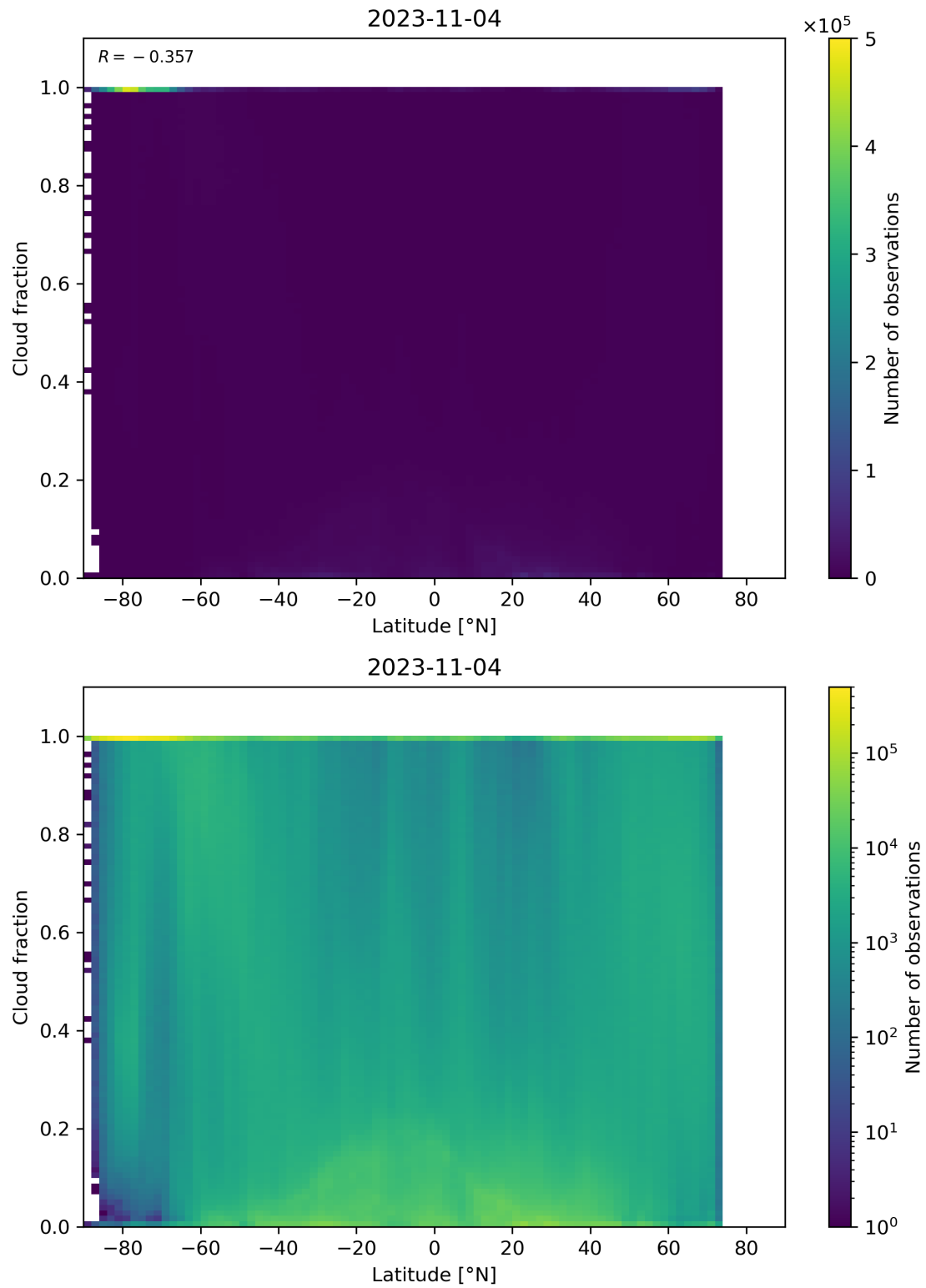
Figure 99: Scatter density plot of “Latitude” against “Cloud fraction” for 2023-11-03 to 2023-11-05.
