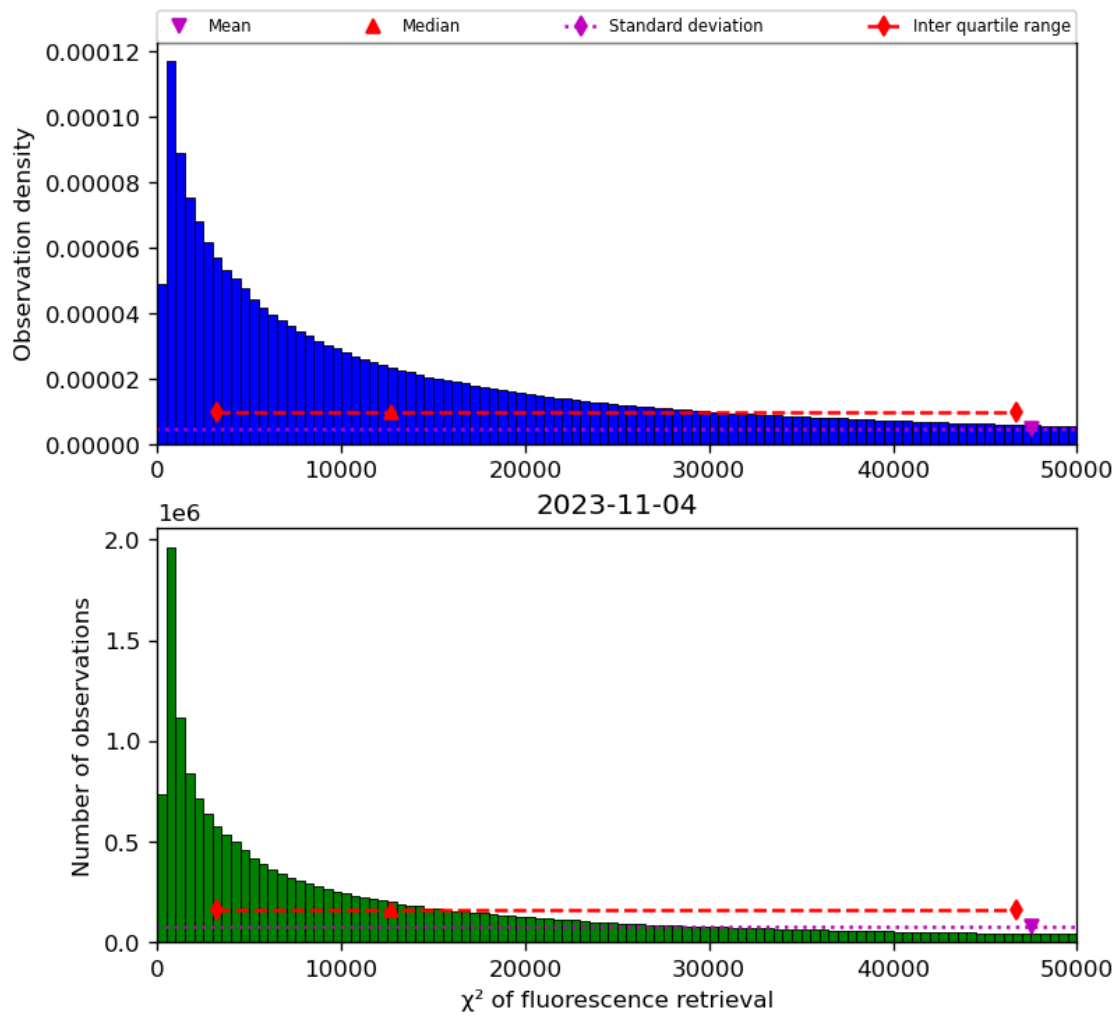
Figure 42: Histogram of “ \chi^2 of fluorescence retrieval” for 2023-11-03 to 2023-11-05
