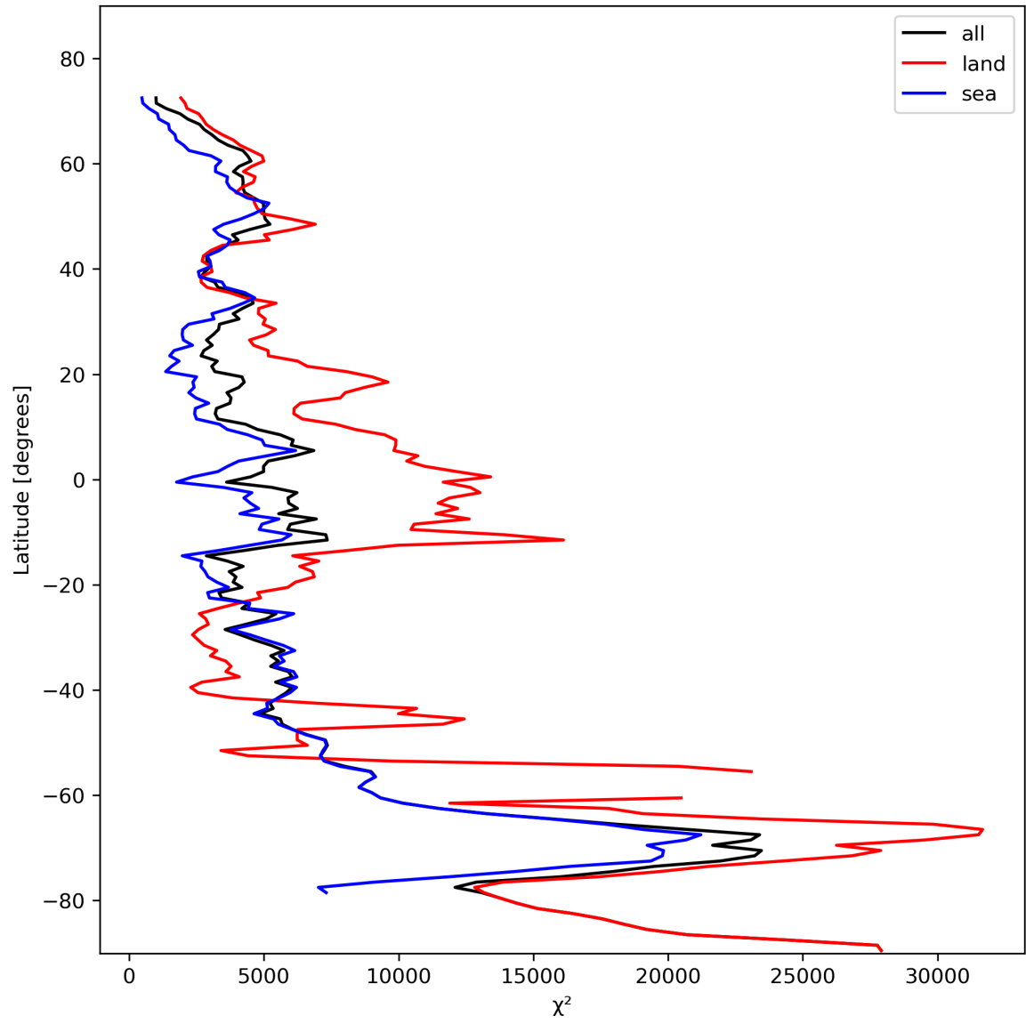
Figure 21: Zonal average of “ \chi^2 ” for 2023-11-03 to 2023-11-05.
