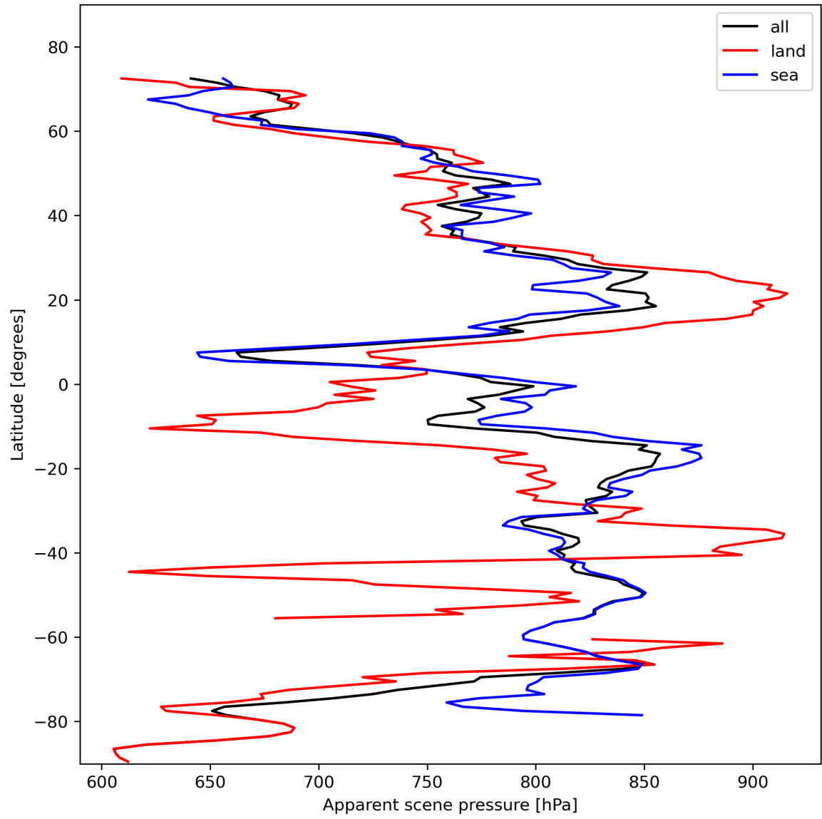
Figure 19: Zonal average of “Apparent scene pressure” for 2023-11-03 to 2023-11-05.
