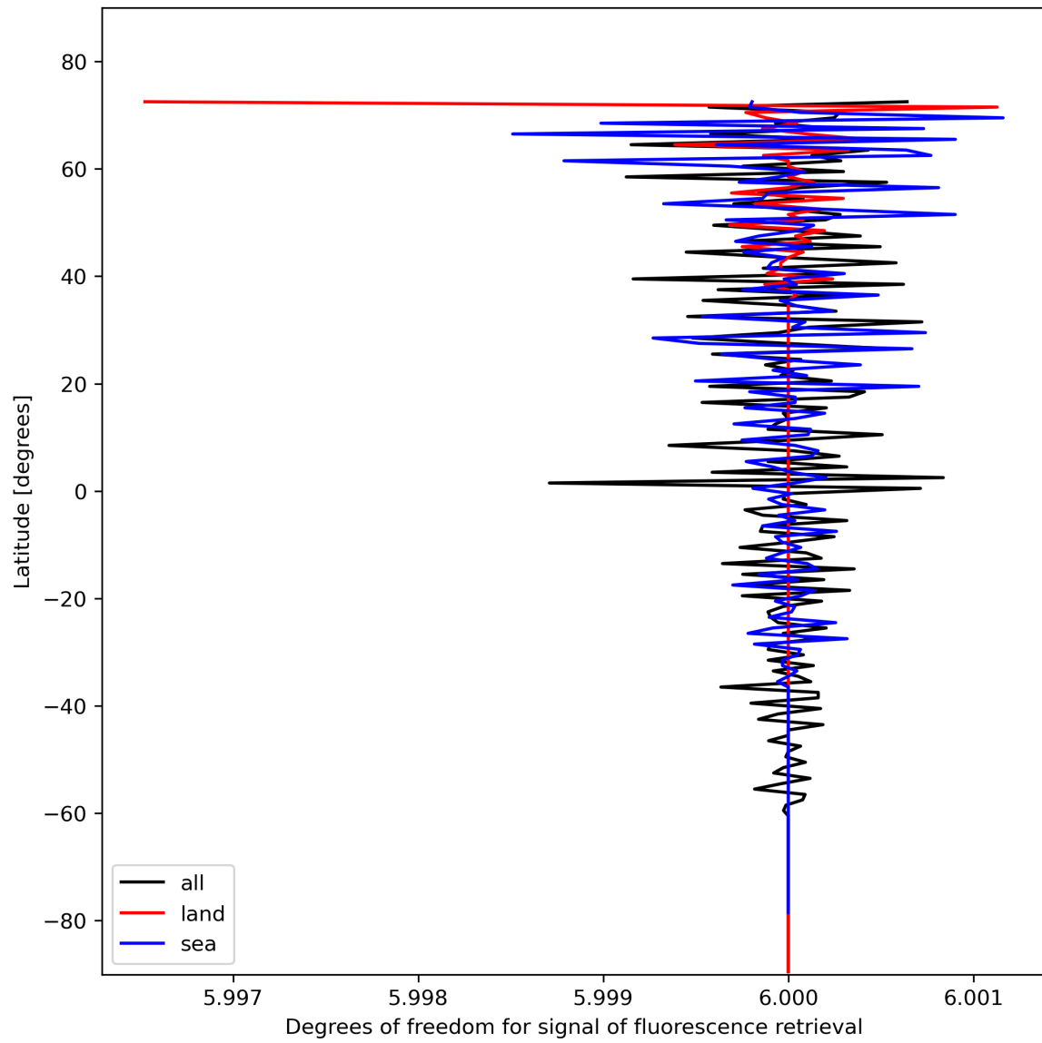
Figure 26: Zonal average of “Degrees of freedom for signal of fluorescence retrieval” for 2023-11-03 to 2023-11-05.
