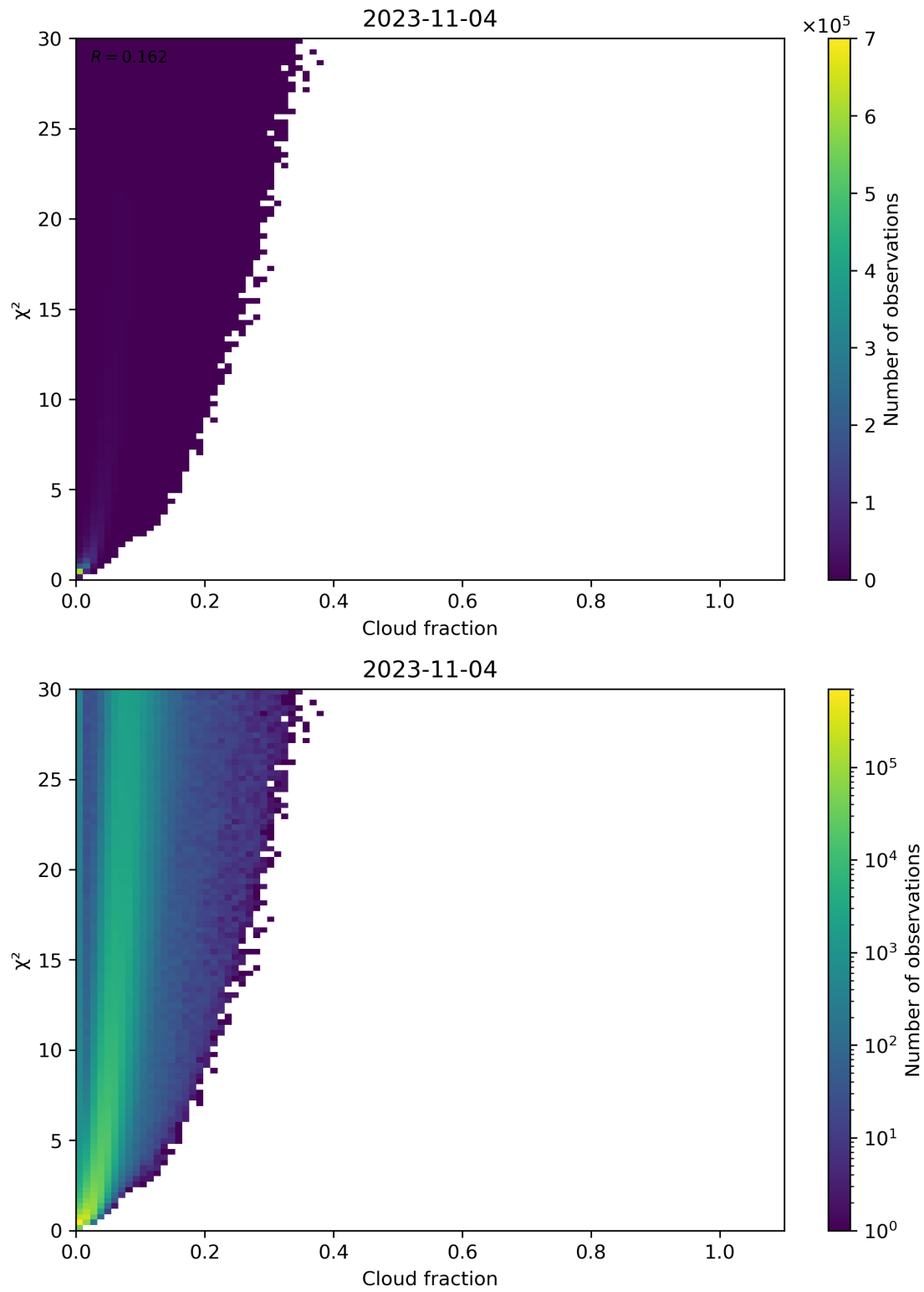
Figure 77: Scatter density plot of “Cloud fraction” against “ \chi^2 ” for 2023-11-03 to 2023-11-05.
