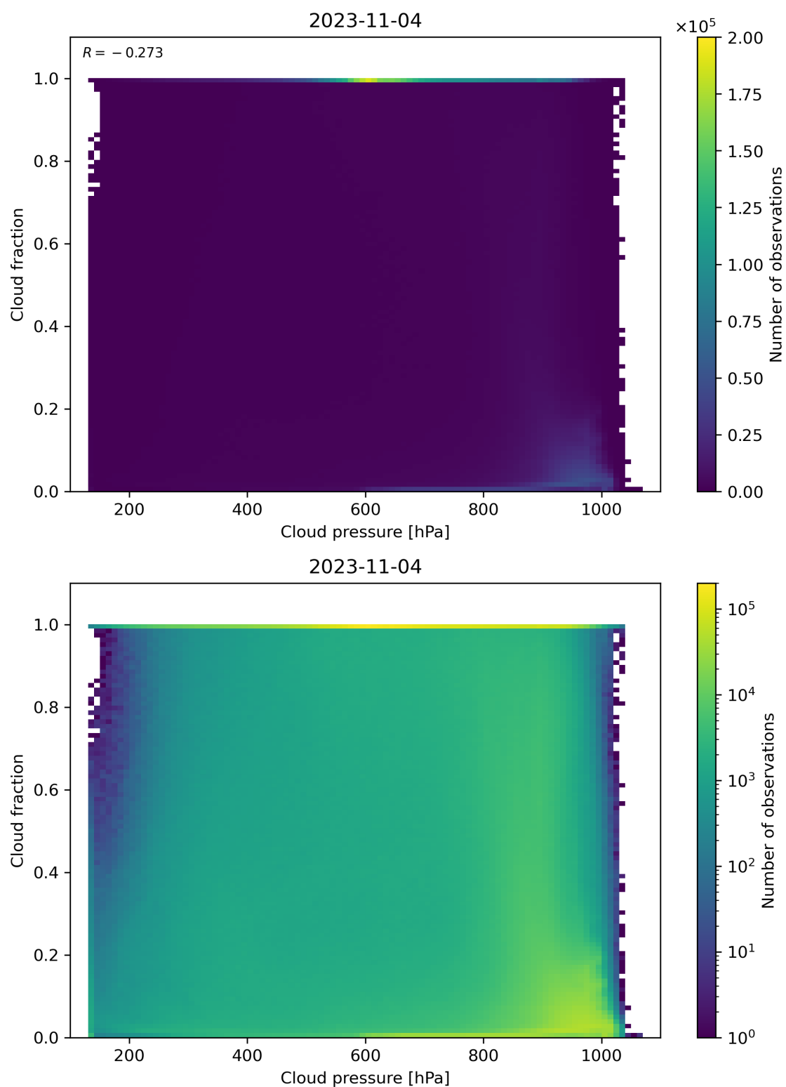
Figure 87: Scatter density plot of “Cloud pressure” against “Cloud fraction” for 2023-11-03 to 2023-11-05.
