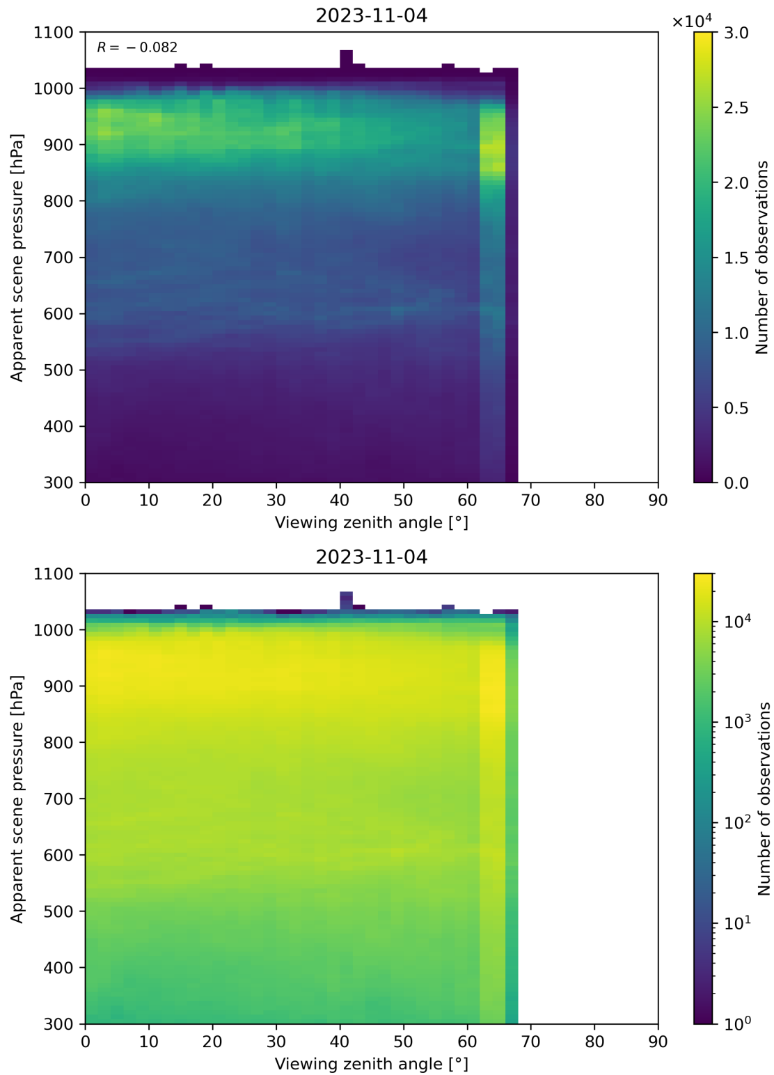
Figure 129: Scatter density plot of “Viewing zenith angle” against “Apparent scene pressure” for 2023-11-03 to 2023-11-05.
