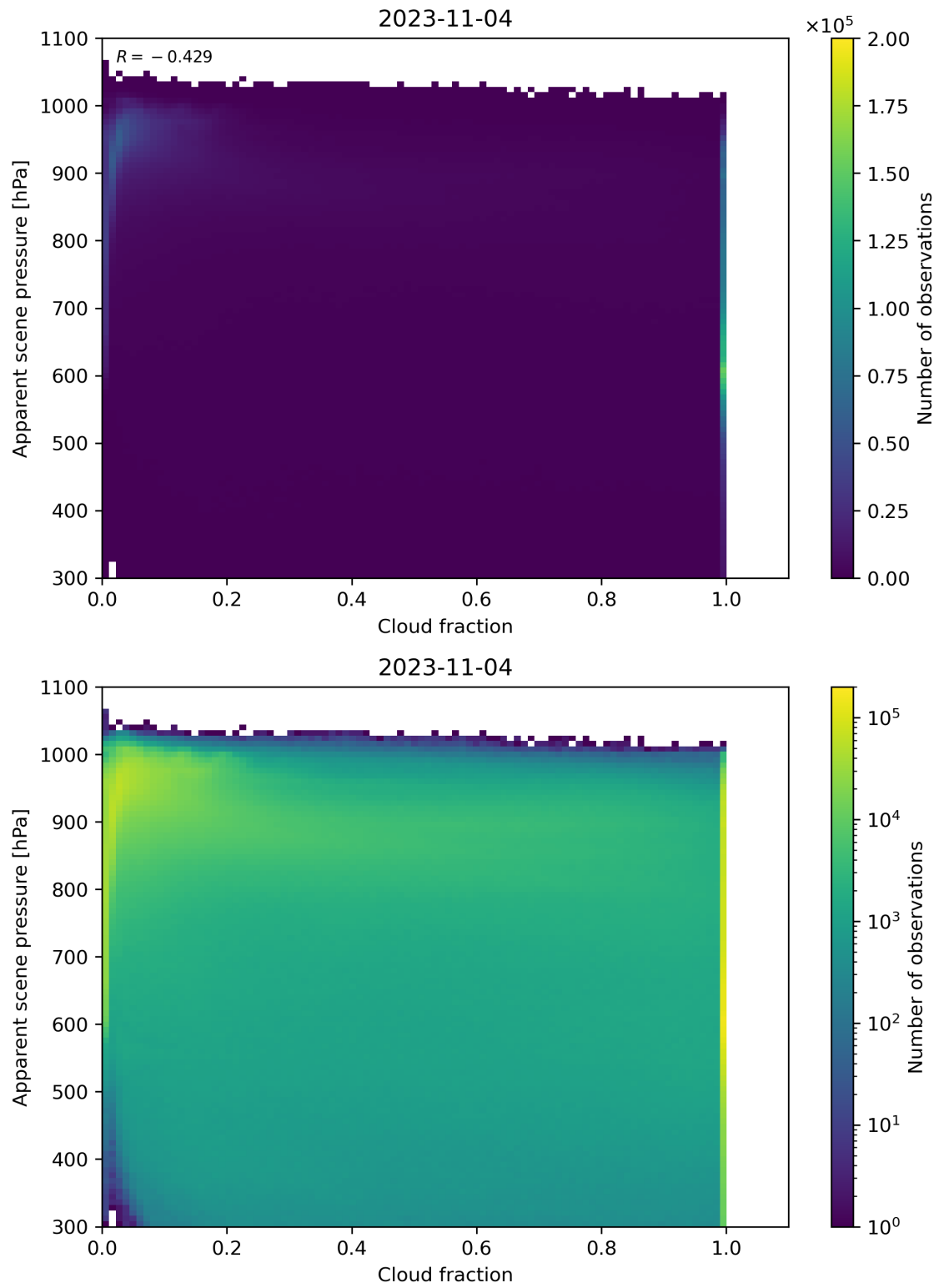
Figure 76: Scatter density plot of “Cloud fraction” against “Apparent scene pressure” for 2023-11-03 to 2023-11-05.
