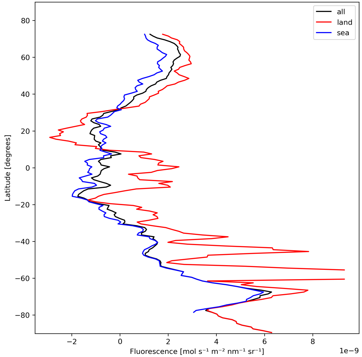
Figure 23: Zonal average of “Fluorescence” for 2023-11-03 to 2023-11-05.
