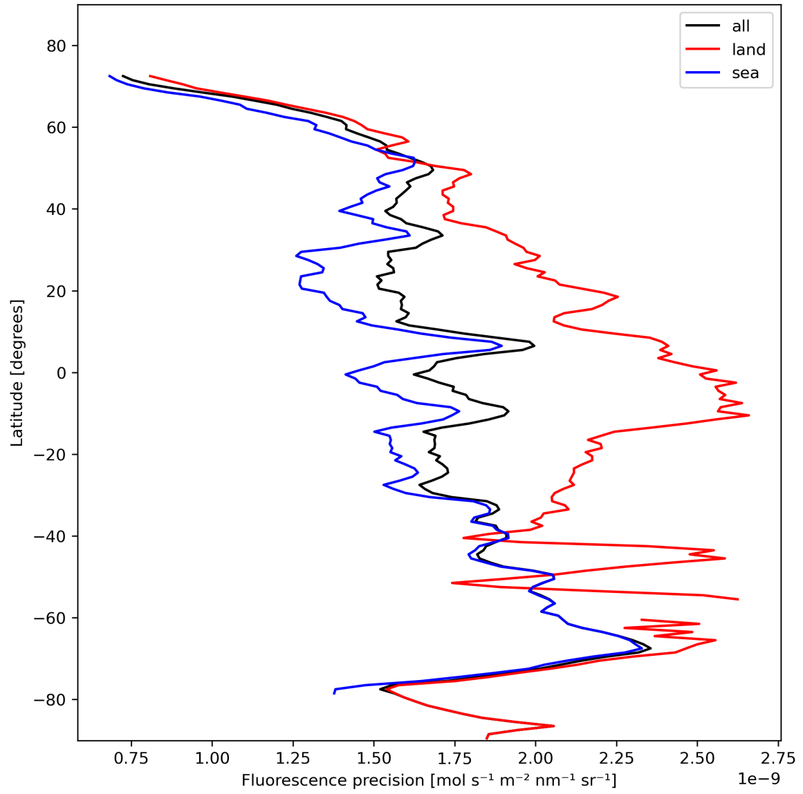
Figure 24: Zonal average of “Fluorescence precision” for 2023-11-03 to 2023-11-05.
