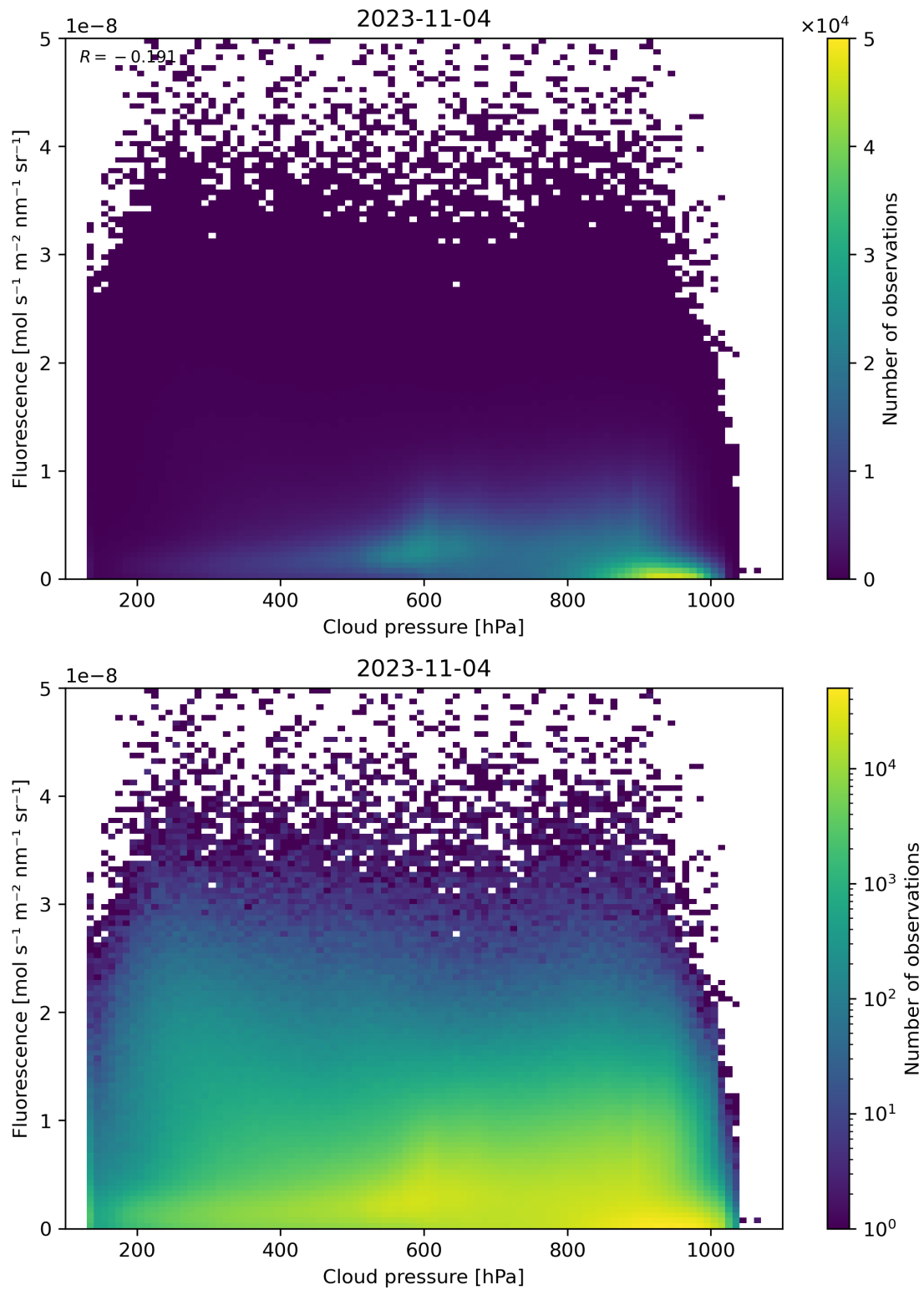
Figure 88: Scatter density plot of “Cloud pressure” against “Fluorescence” for 2023-11-03 to 2023-11-05.
