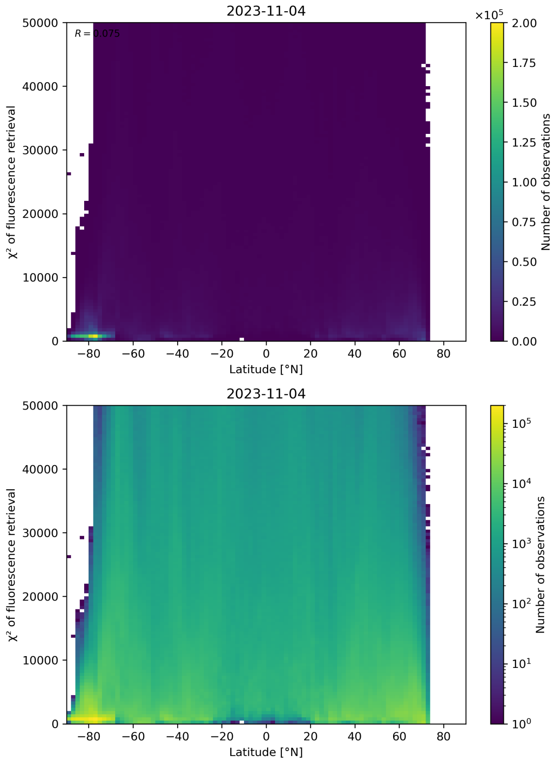
Figure 98: Scatter density plot of “Latitude” against “ \chi^2 of fluorescence retrieval” for 2023-11-03 to 2023-11-05.
