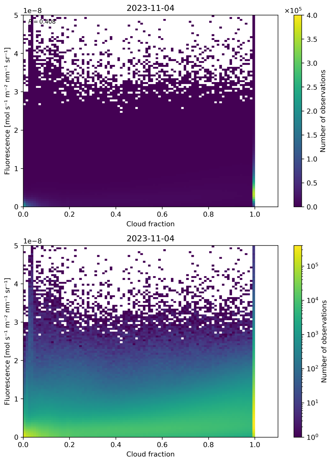
Figure 79: Scatter density plot of “Cloud fraction” against “Fluorescence” for 2023-11-03 to 2023-11-05.
