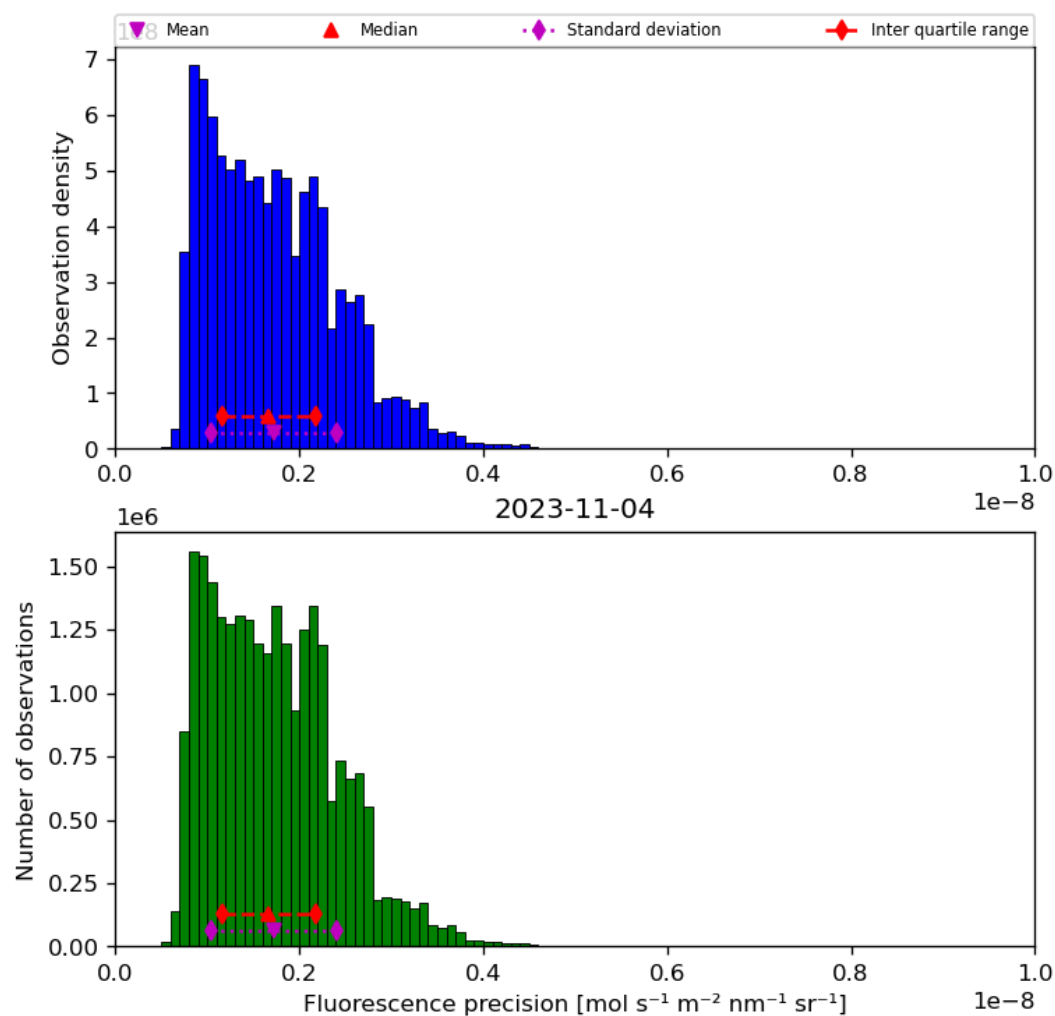
Figure 41: Histogram of “Fluorescence precision” for 2023-11-03 to 2023-11-05
