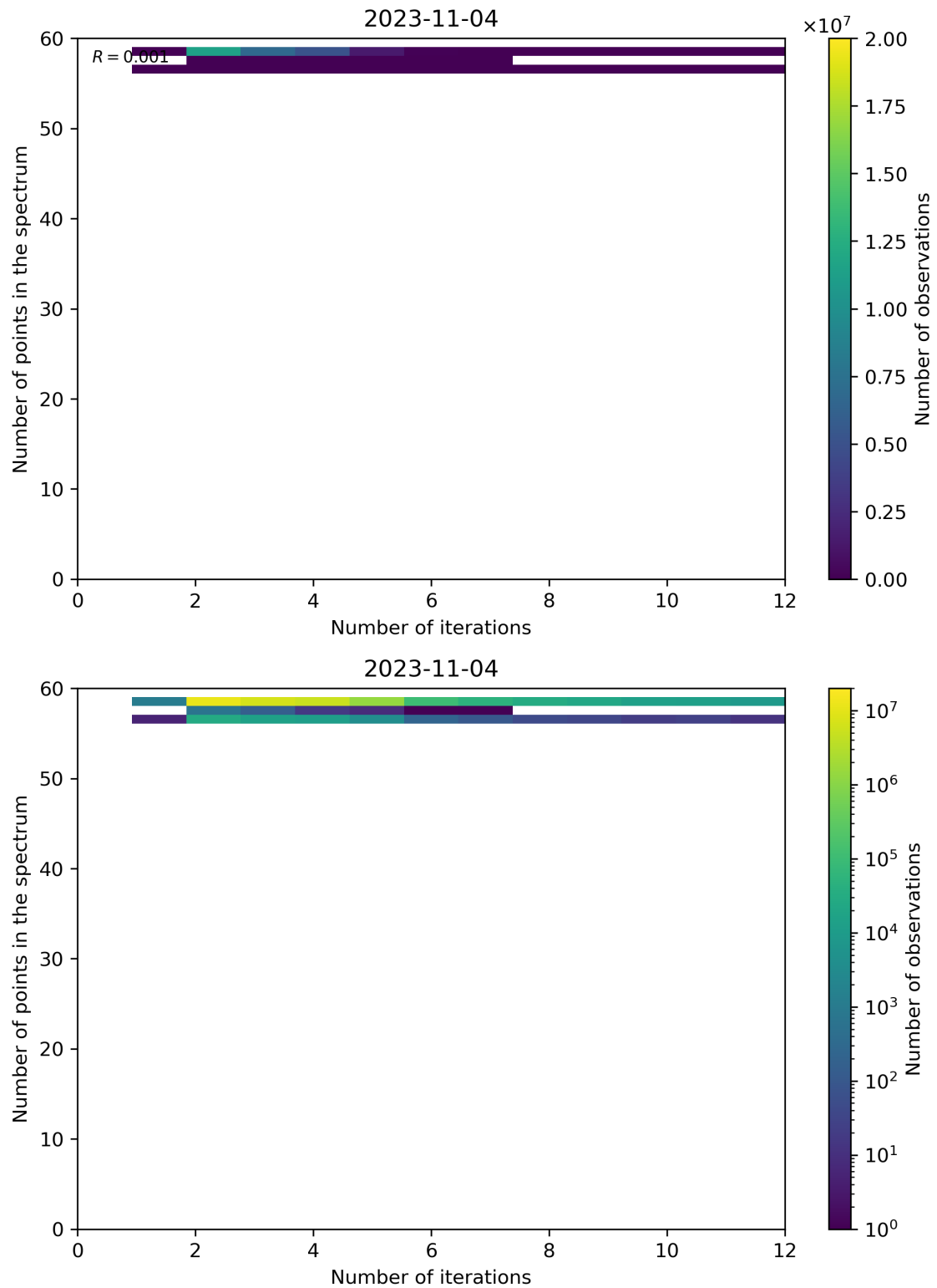
Figure 108: Scatter density plot of “Number of iterations” against “Number of points in the spectrum” for 2023-11-03 to 2023-11-05.
