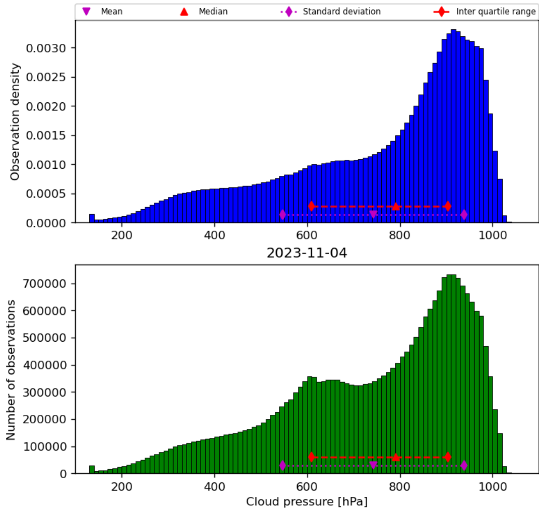
Figure 30: Histogram of “Cloud pressure” for 2023-11-03 to 2023-11-05
