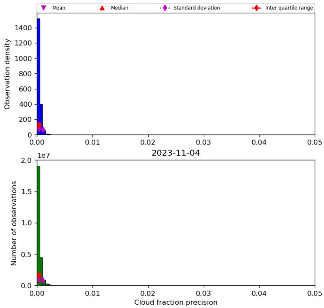
Figure 33: Histogram of “Cloud fraction precision” for 2023-11-03 to 2023-11-05
