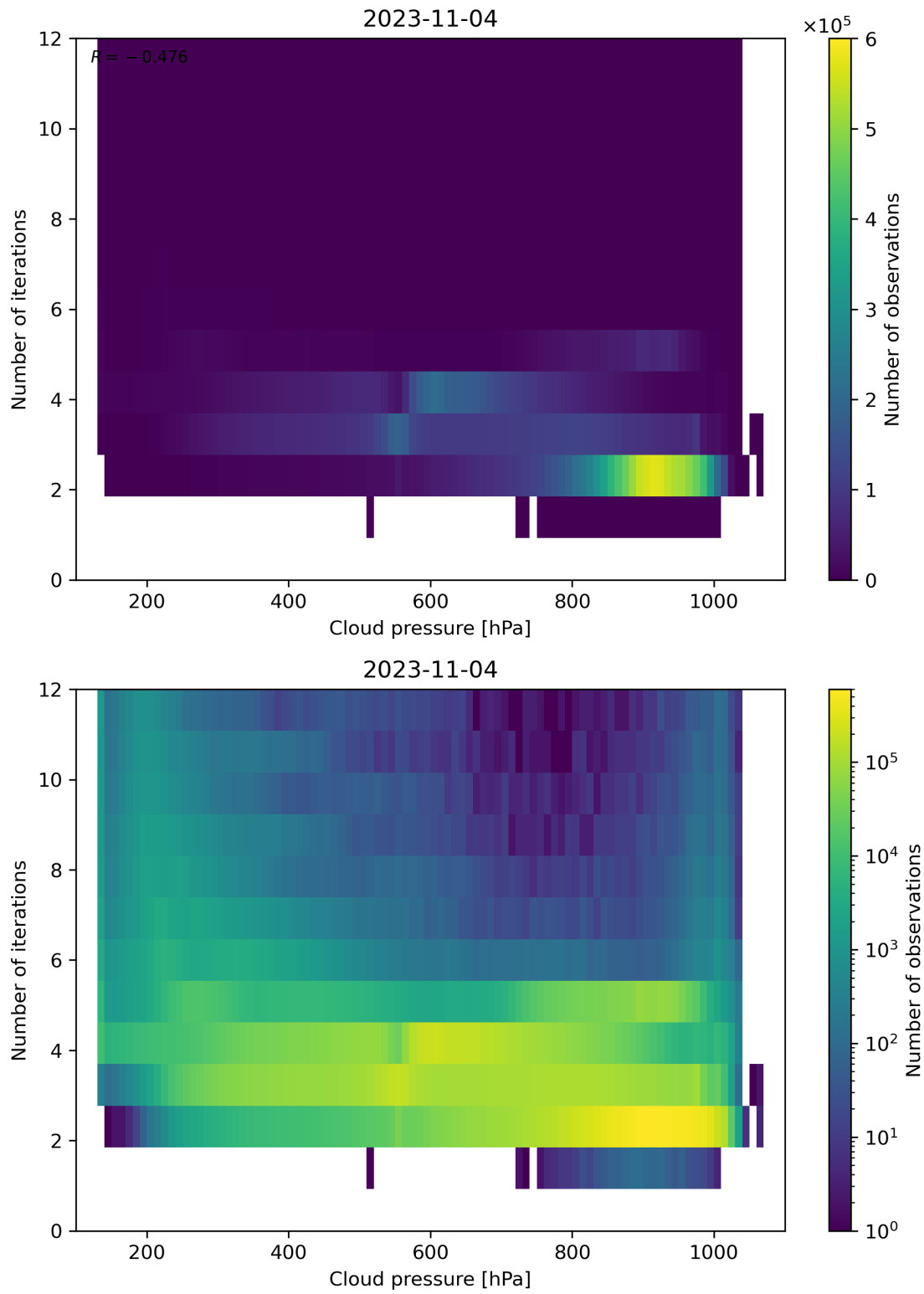
Figure 89: Scatter density plot of “Cloud pressure” against “Number of iterations” for 2023-11-03 to 2023-11-05.
