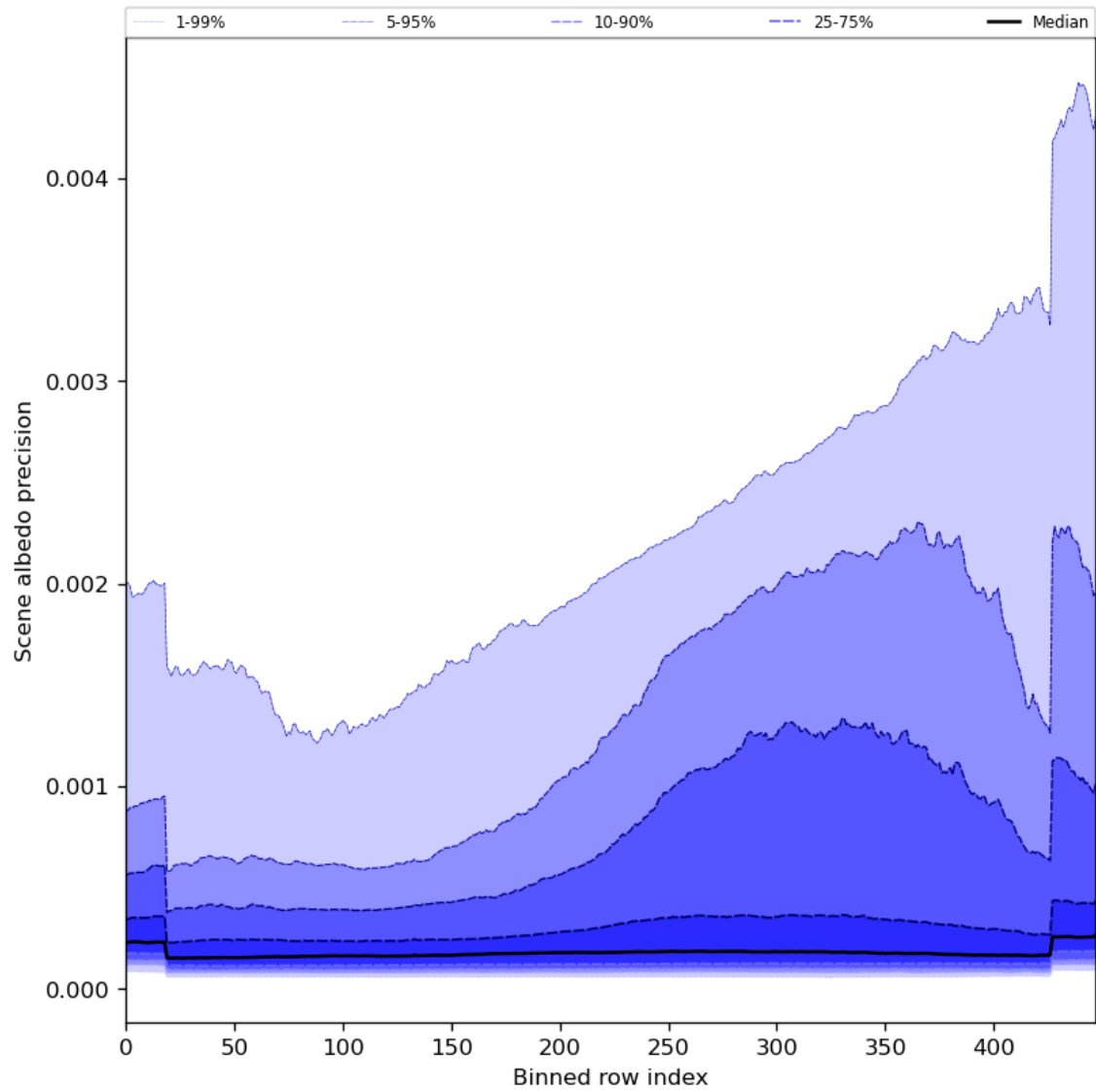
Figure 52: Along track statistics of “Scene albedo precision” for 2023-11-03 to 2023-11-05
