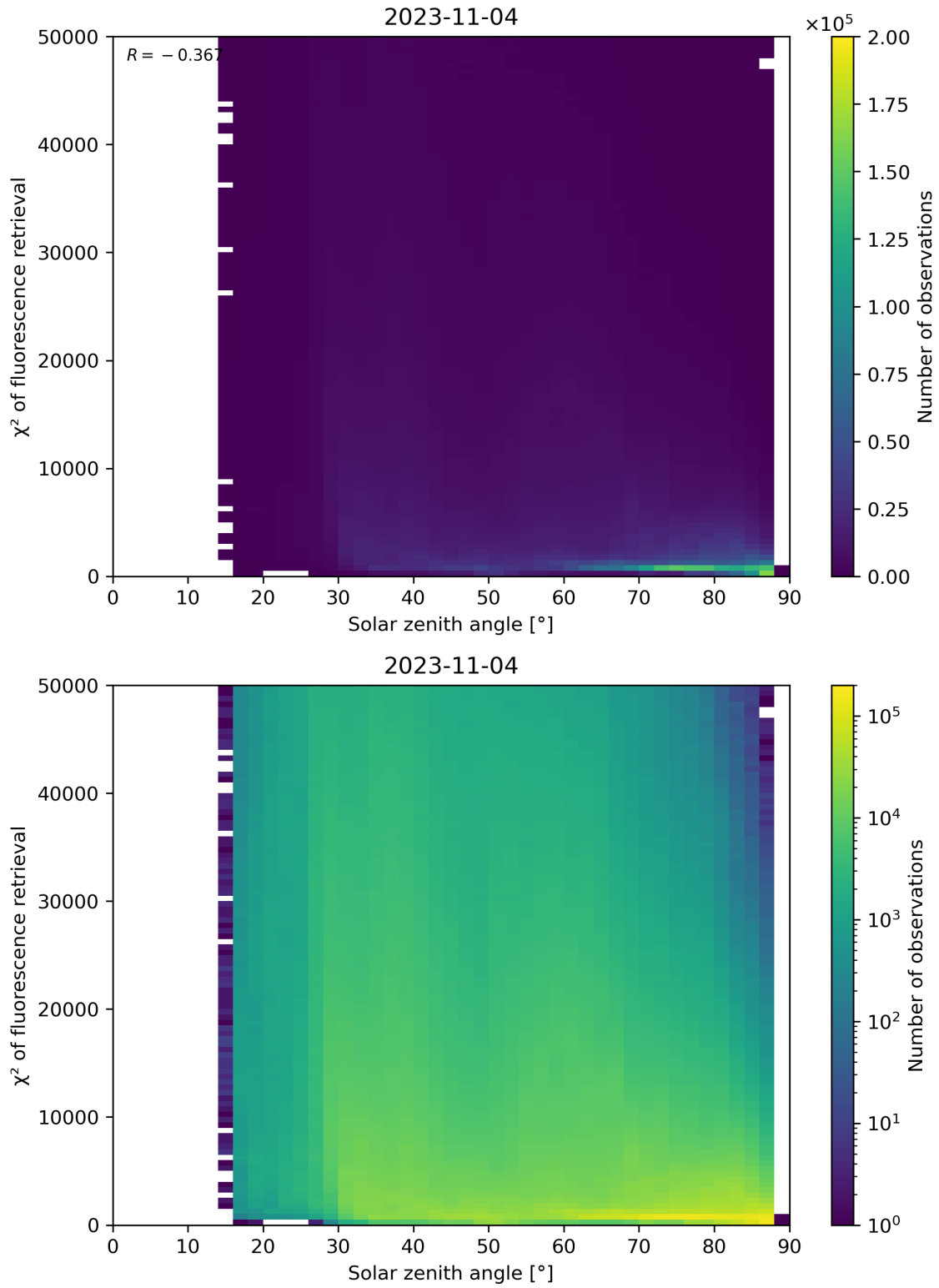
Figure 120: Scatter density plot of “Solar zenith angle” against “ \chi^2 of fluorescence retrieval” for 2023-11-03 to 2023-11-05.
