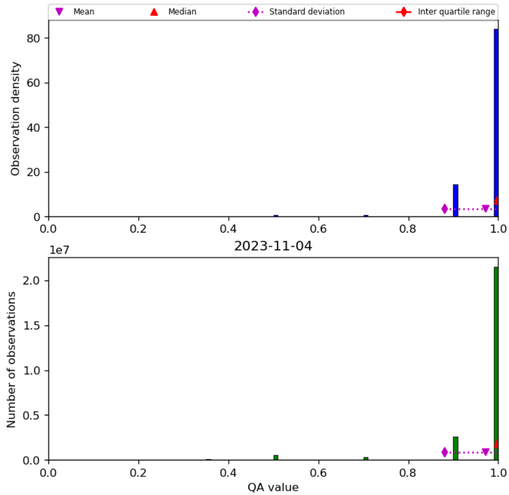
Figure 29: Histogram of “QA value” for 2023-11-03 to 2023-11-05
