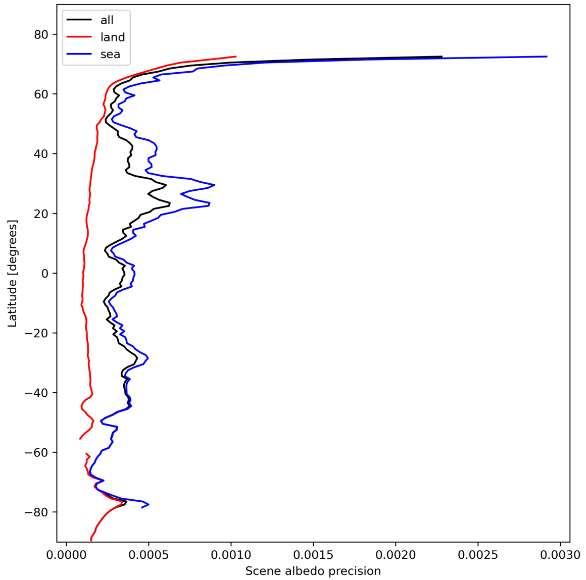
Figure 18: Zonal average of “Scene albedo precision” for 2023-11-03 to 2023-11-05.
