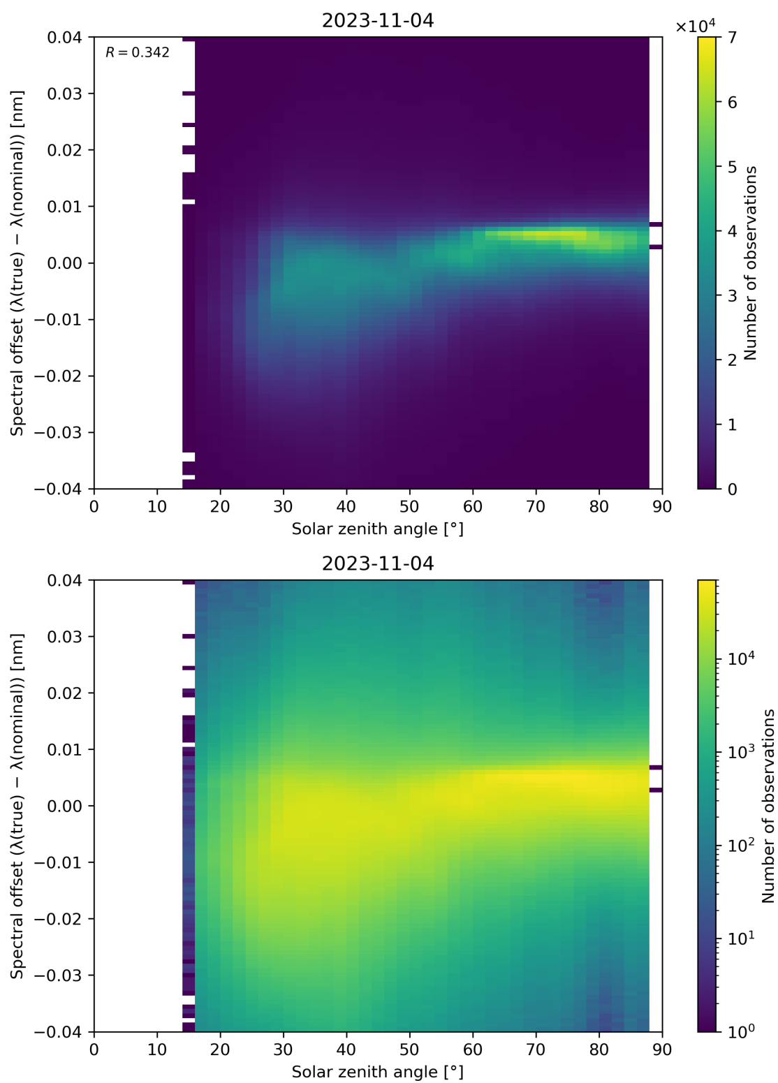
Figure 128: Scatter density plot of “Solar zenith angle” against “Spectral offset ( \lambda(\text{true}) - \lambda(\text{nominal}) )” for 2023-11-03 to 2023-11-05.
