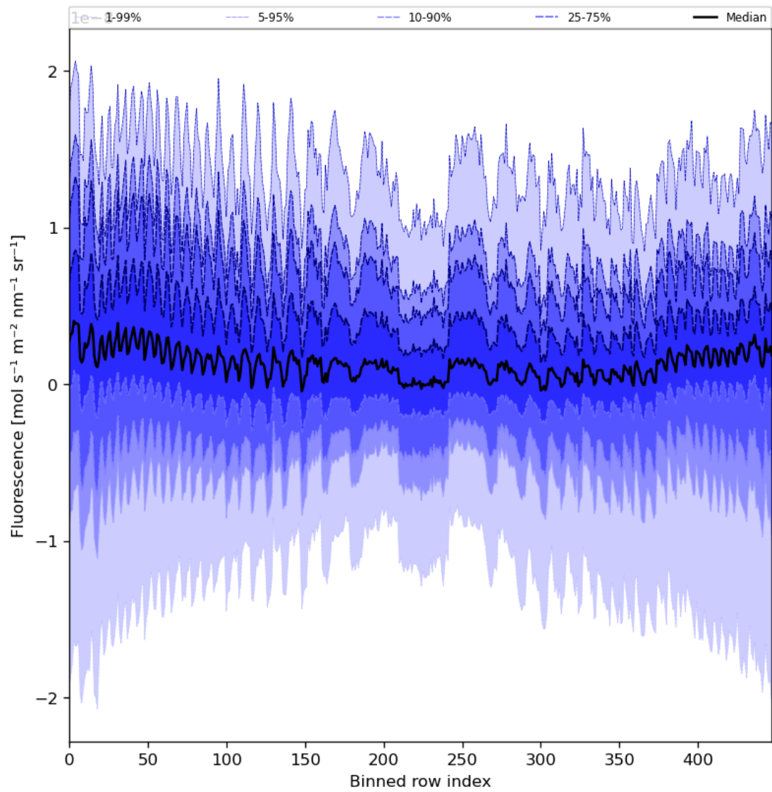
Figure 57: Along track statistics of “Fluorescence” for 2023-11-03 to 2023-11-05
