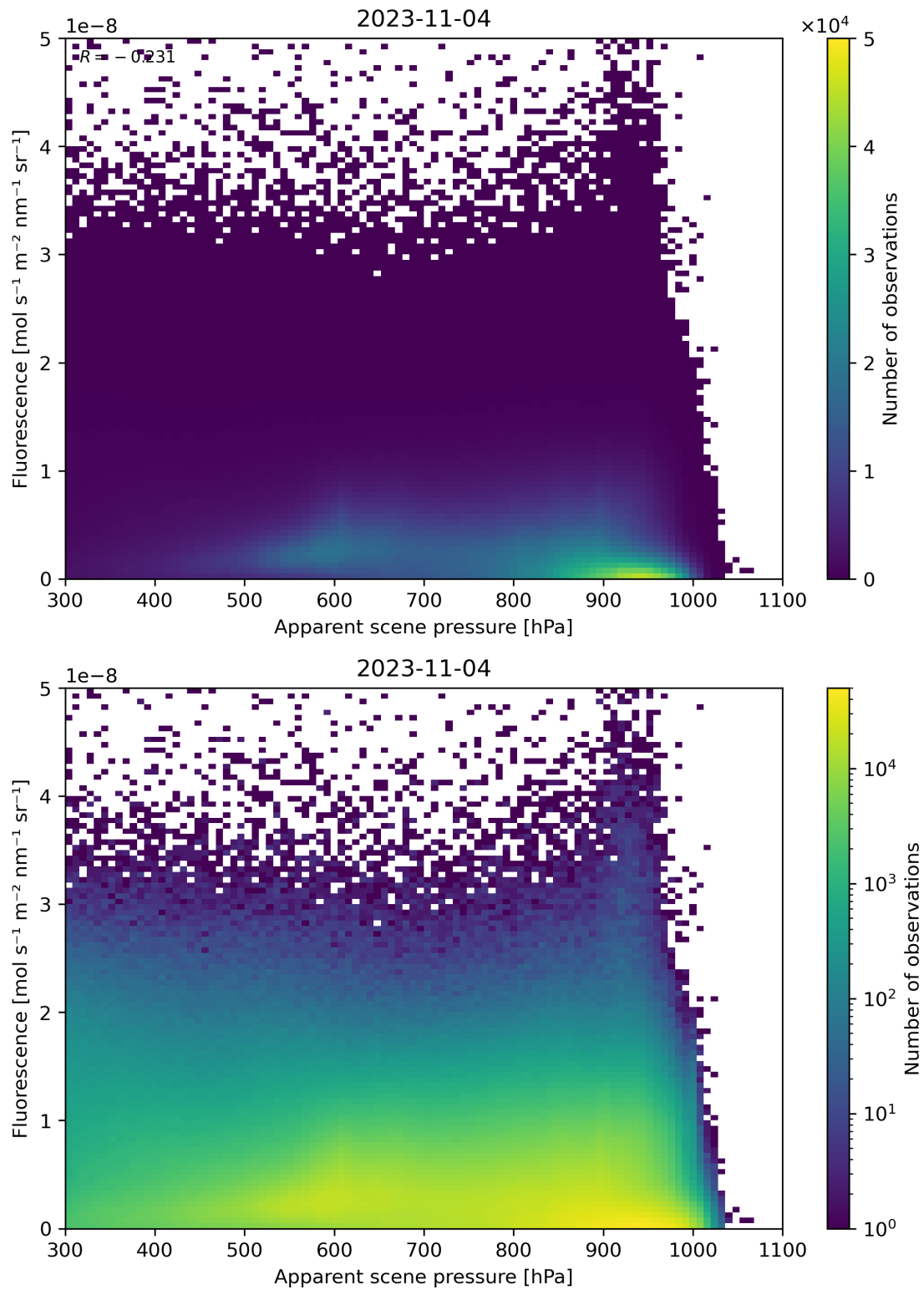
Figure 65: Scatter density plot of “Apparent scene pressure” against “Fluorescence” for 2023-11-03 to 2023-11-05.
