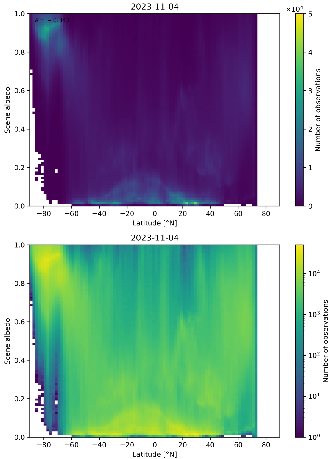
Figure 104: Scatter density plot of “Latitude” against “Scene albedo” for 2023-11-03 to 2023-11-05.
