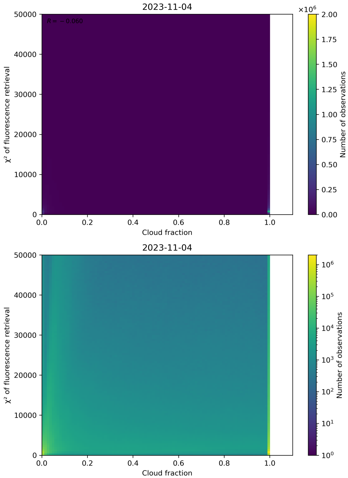
Figure 78: Scatter density plot of “Cloud fraction” against “ \chi^2 of fluorescence retrieval” for 2023-11-03 to 2023-11-05.
