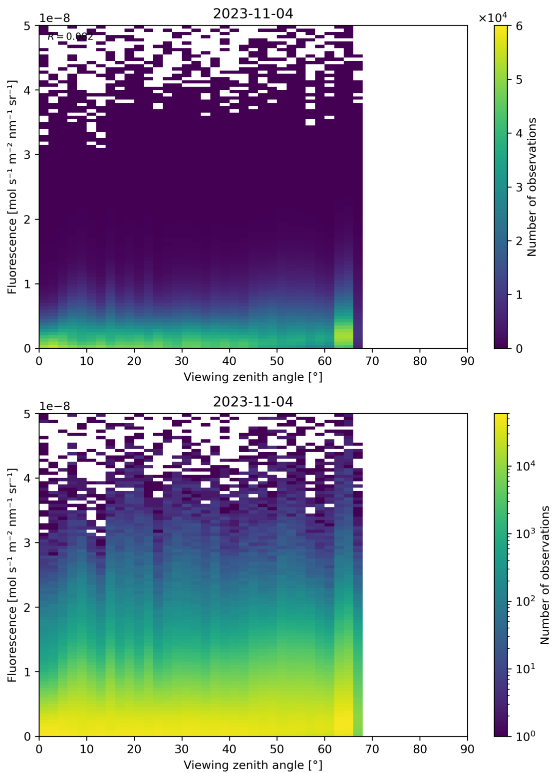
Figure 134: Scatter density plot of “Viewing zenith angle” against “Fluorescence” for 2023-11-03 to 2023-11-05.
