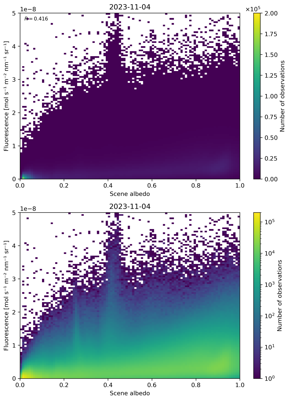
Figure 114: Scatter density plot of "Scene albedo" against "Fluorescence" for 2023-11-03 to 2023-11-05.
