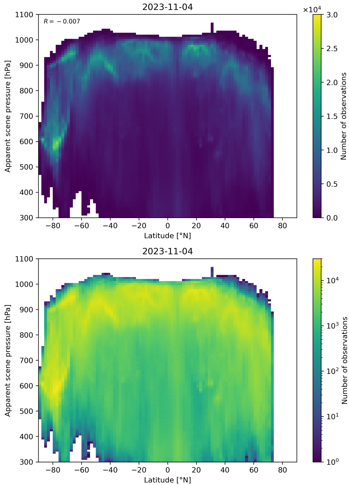
Figure 96: Scatter density plot of “Latitude” against “Apparent scene pressure” for 2023-11-03 to 2023-11-05.
