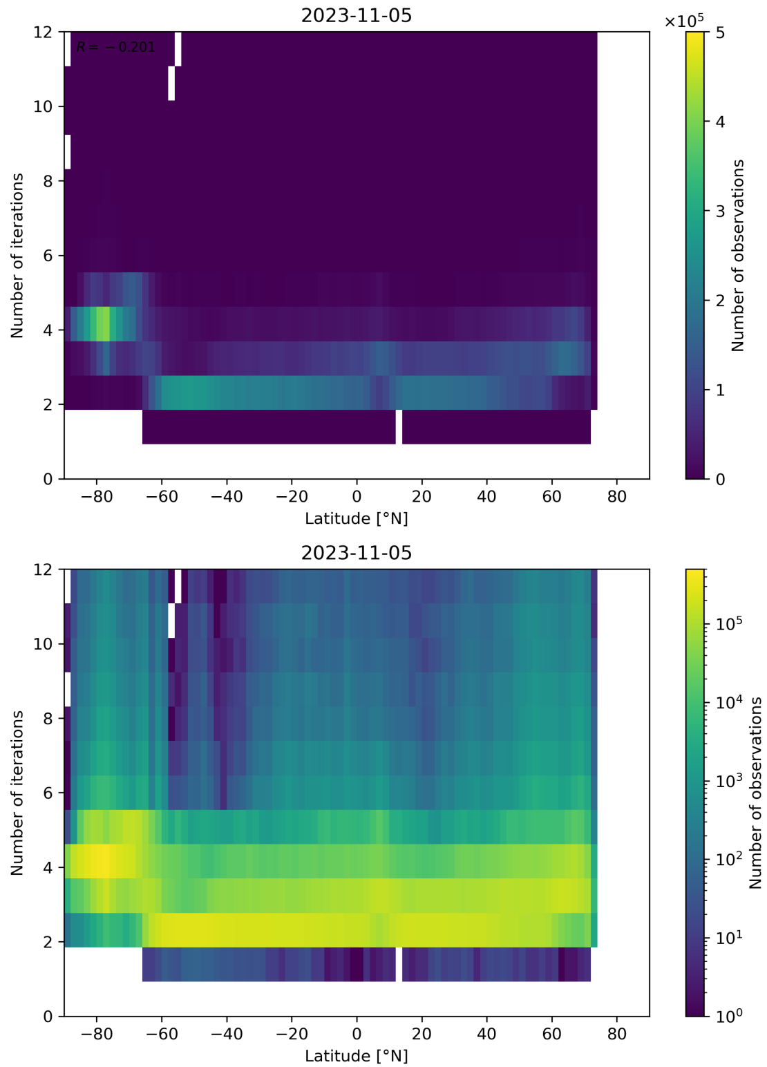
Figure 102: Scatter density plot of “Latitude” against “Number of iterations” for 2023-11-04 to 2023-11-06.
