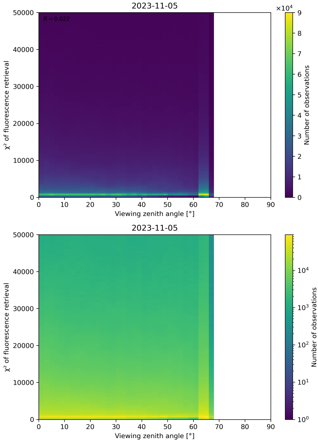
Figure 131: Scatter density plot of “Viewing zenith angle” against “ \chi^2 of fluorescence retrieval” for 2023-11-04 to 2023-11-06.
