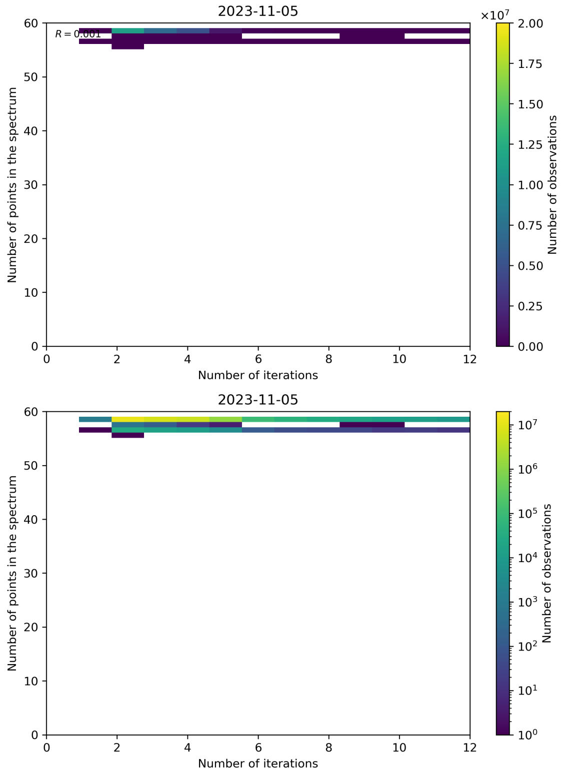
Figure 108: Scatter density plot of “Number of iterations” against “Number of points in the spectrum” for 2023-11-04 to 2023-11-06.
