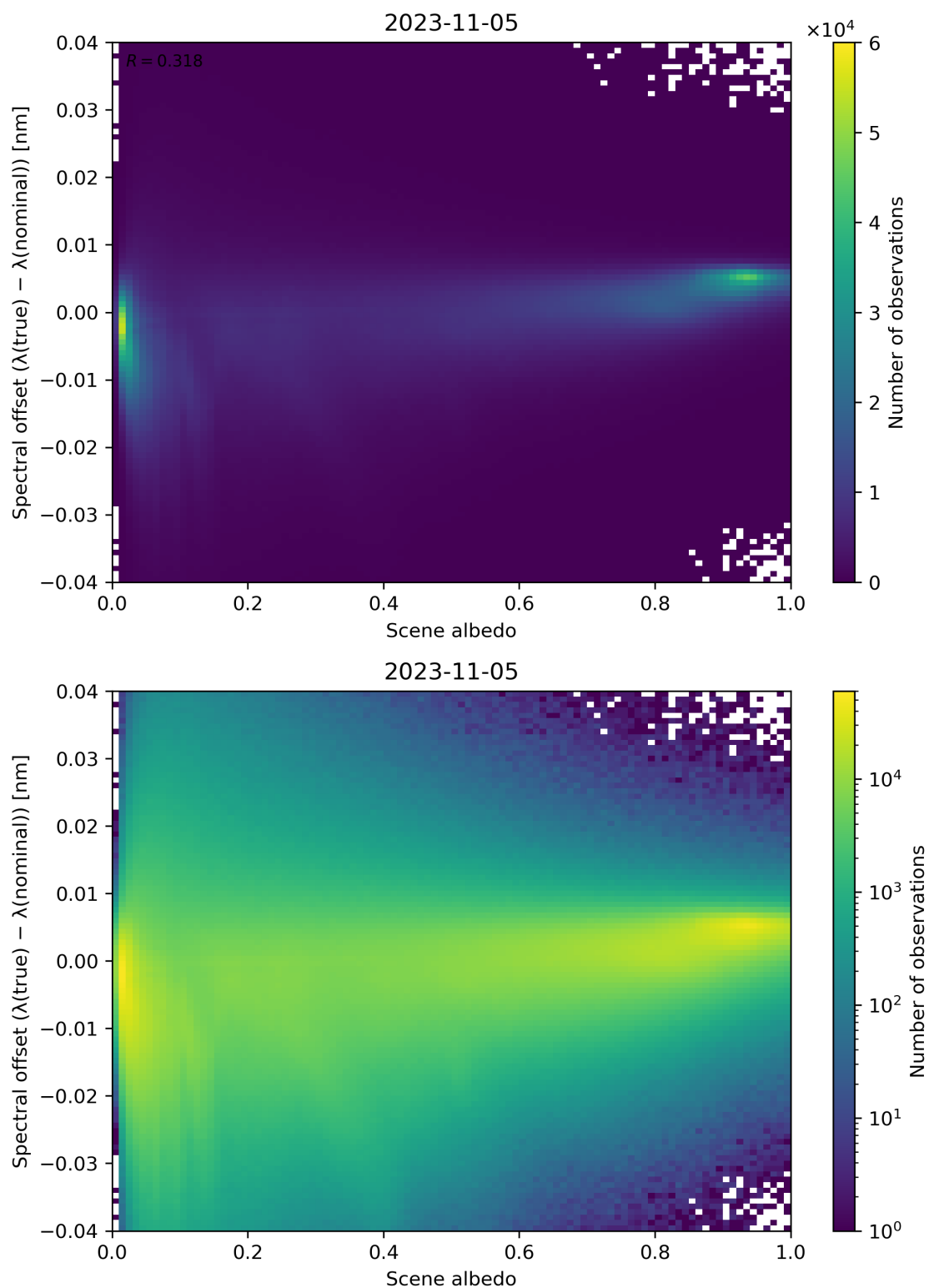
Figure 117: Scatter density plot of “Scene albedo” against “Spectral offset ( \lambda(\text{true}) - \lambda(\text{nominal}) )” for 2023-11-04 to 2023-11-06.
