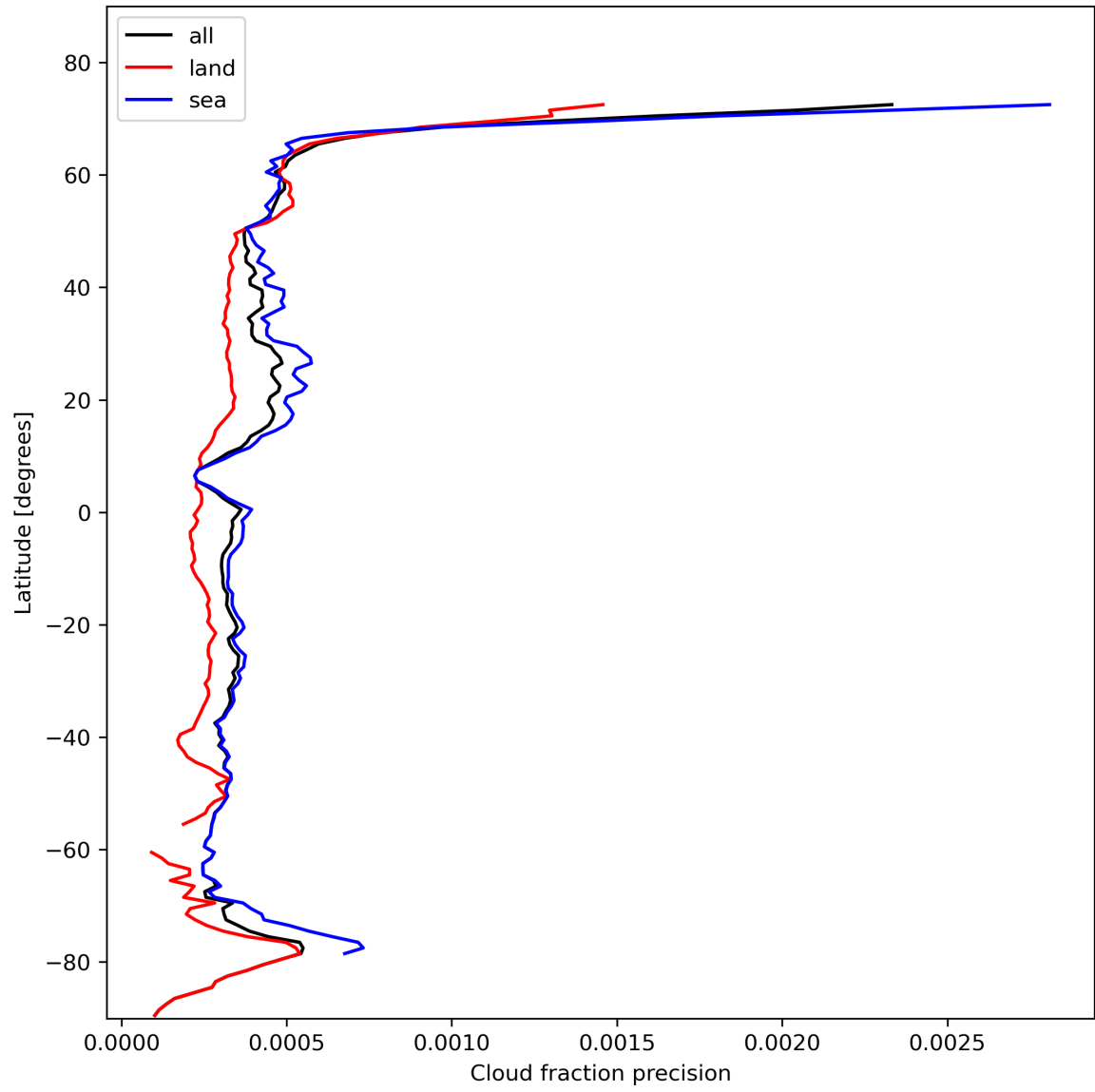
Figure 16: Zonal average of “Cloud fraction precision” for 2023-11-04 to 2023-11-06.
