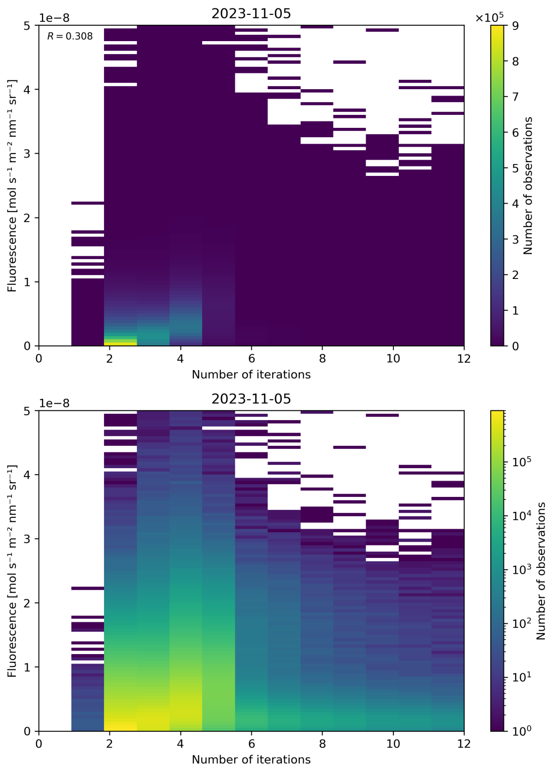
Figure 107: Scatter density plot of “Number of iterations” against “Fluorescence” for 2023-11-04 to 2023-11-06.
