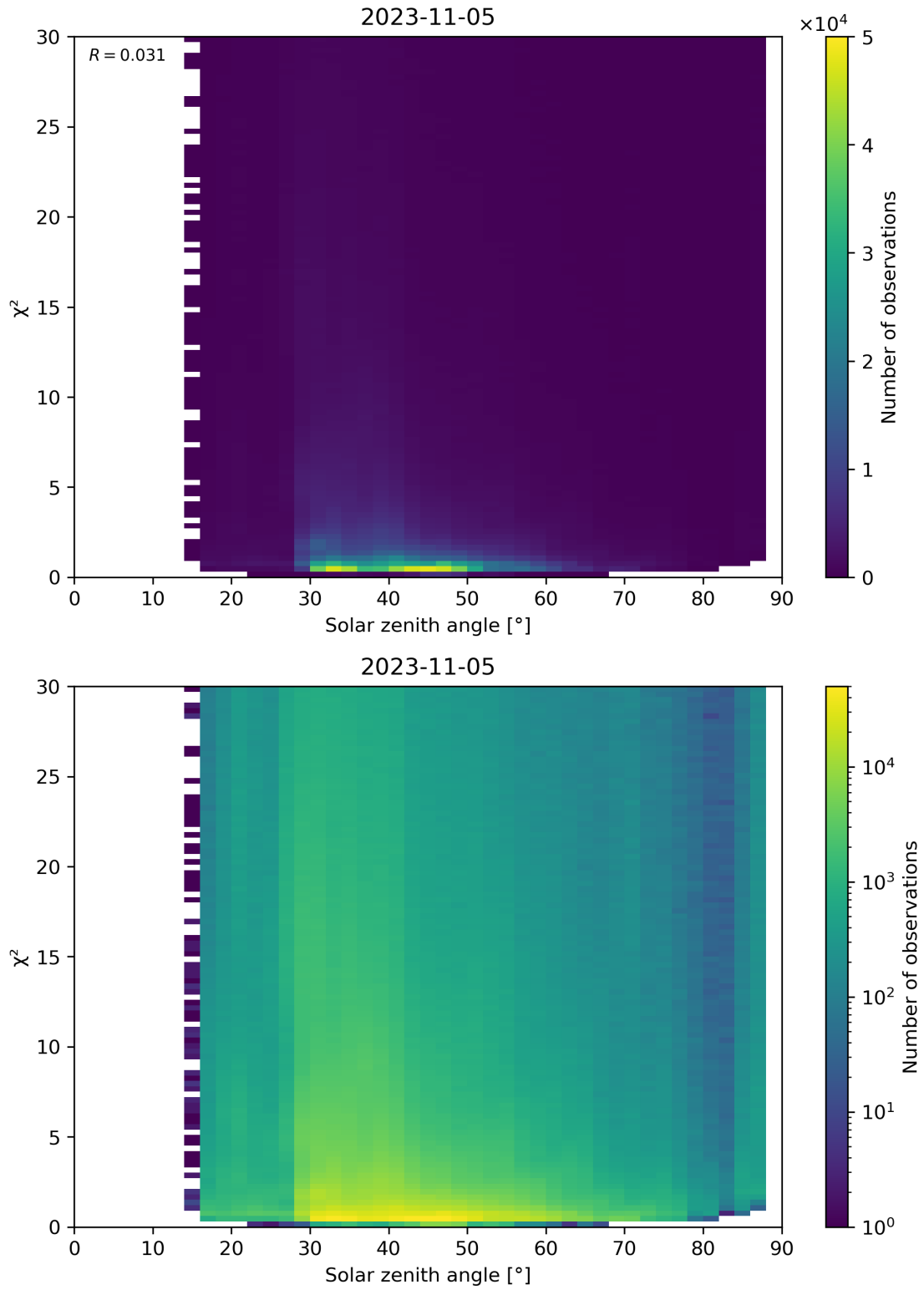
Figure 119: Scatter density plot of “Solar zenith angle” against “ \chi^2 ” for 2023-11-04 to 2023-11-06.
