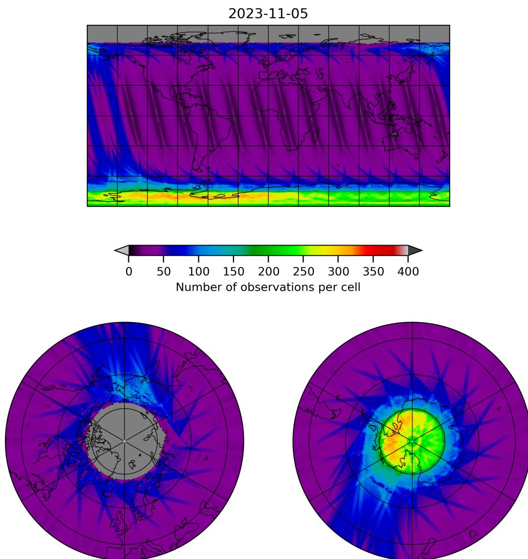
Figure 11: Map of the number of observations for 2023-11-04 to 2023-11-06
