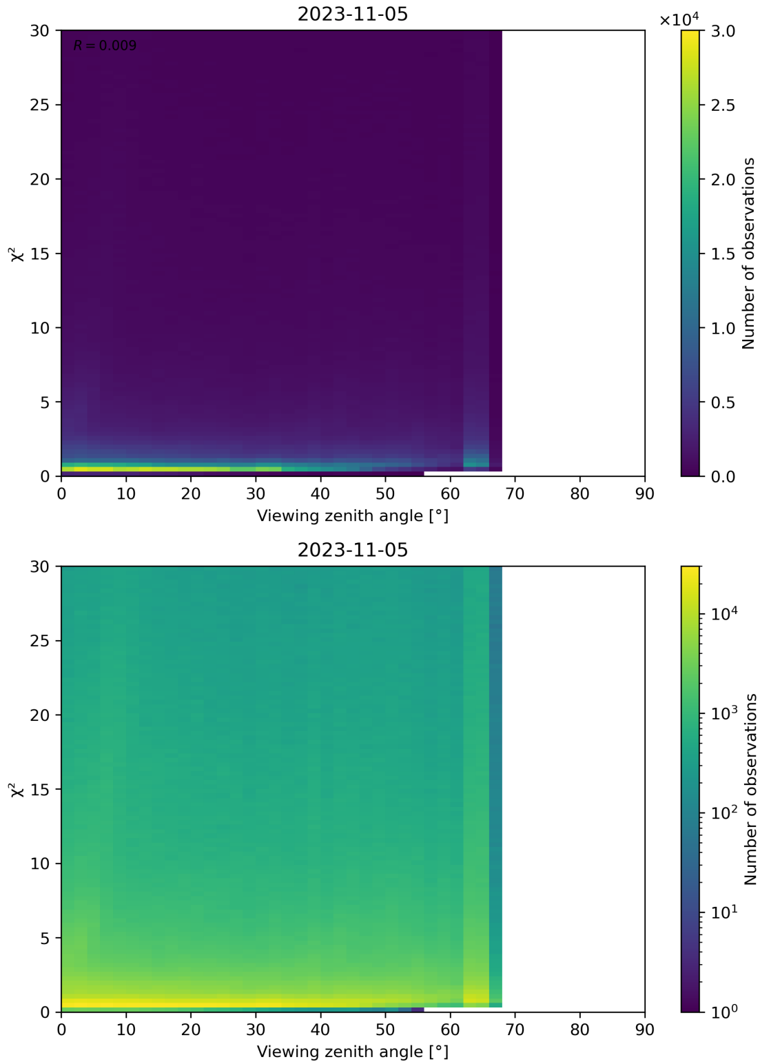
Figure 130: Scatter density plot of “Viewing zenith angle” against “ \chi^2 ” for 2023-11-04 to 2023-11-06.
