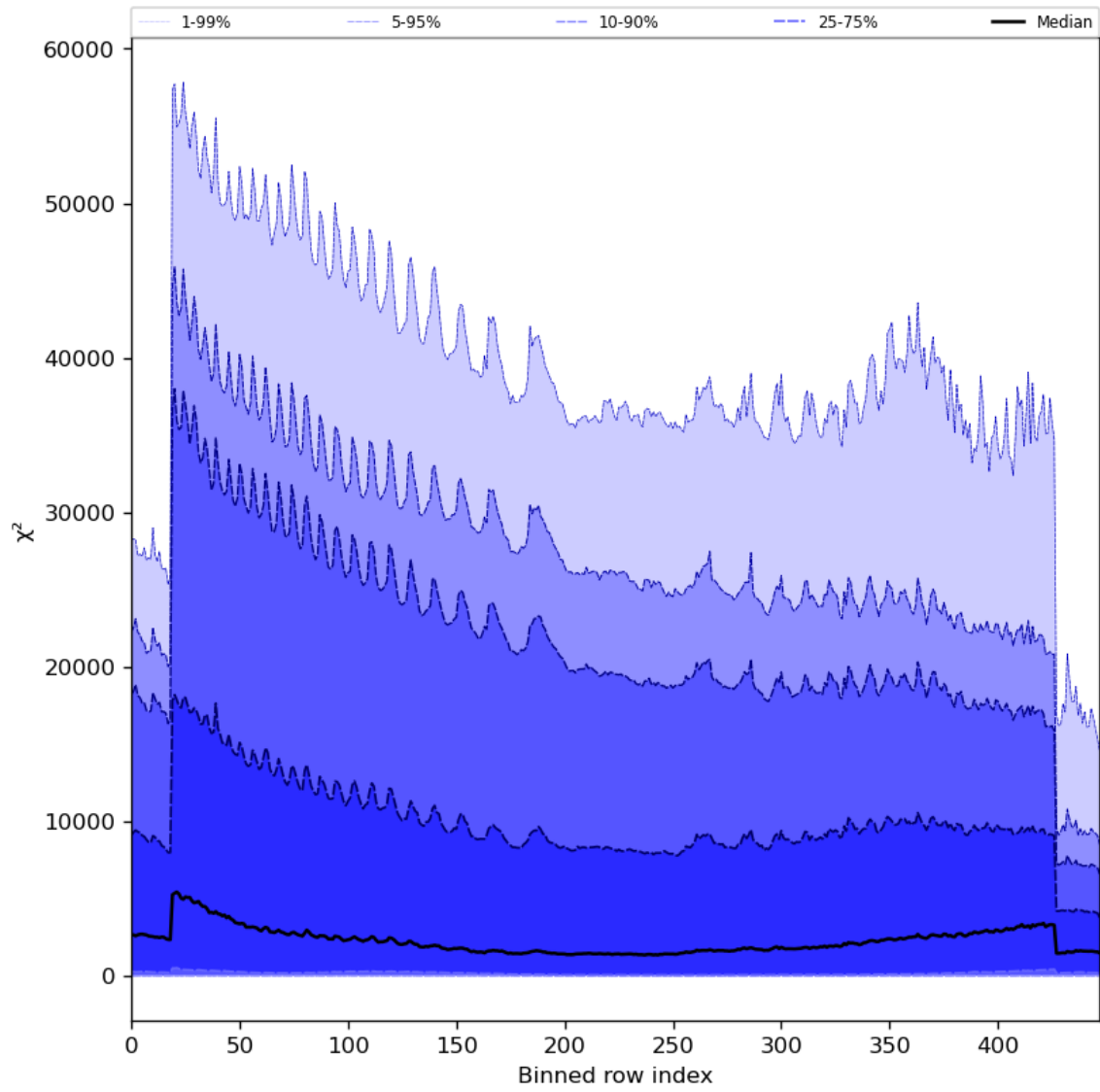
Figure 55: Along track statistics of “ \chi^2 ” for 2023-11-04 to 2023-11-06
