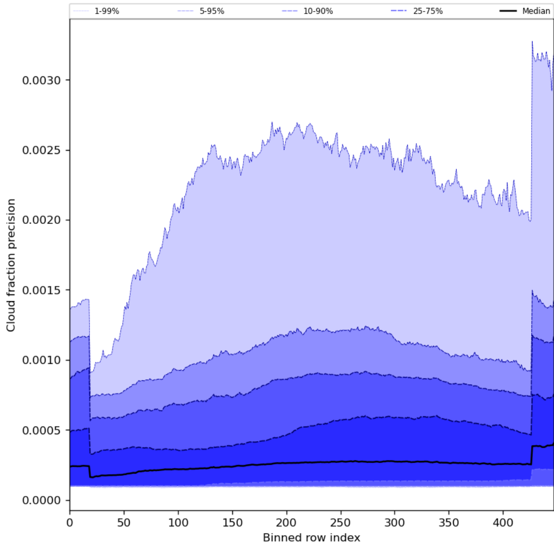
Figure 50: Along track statistics of “Cloud fraction precision” for 2023-11-04 to 2023-11-06
