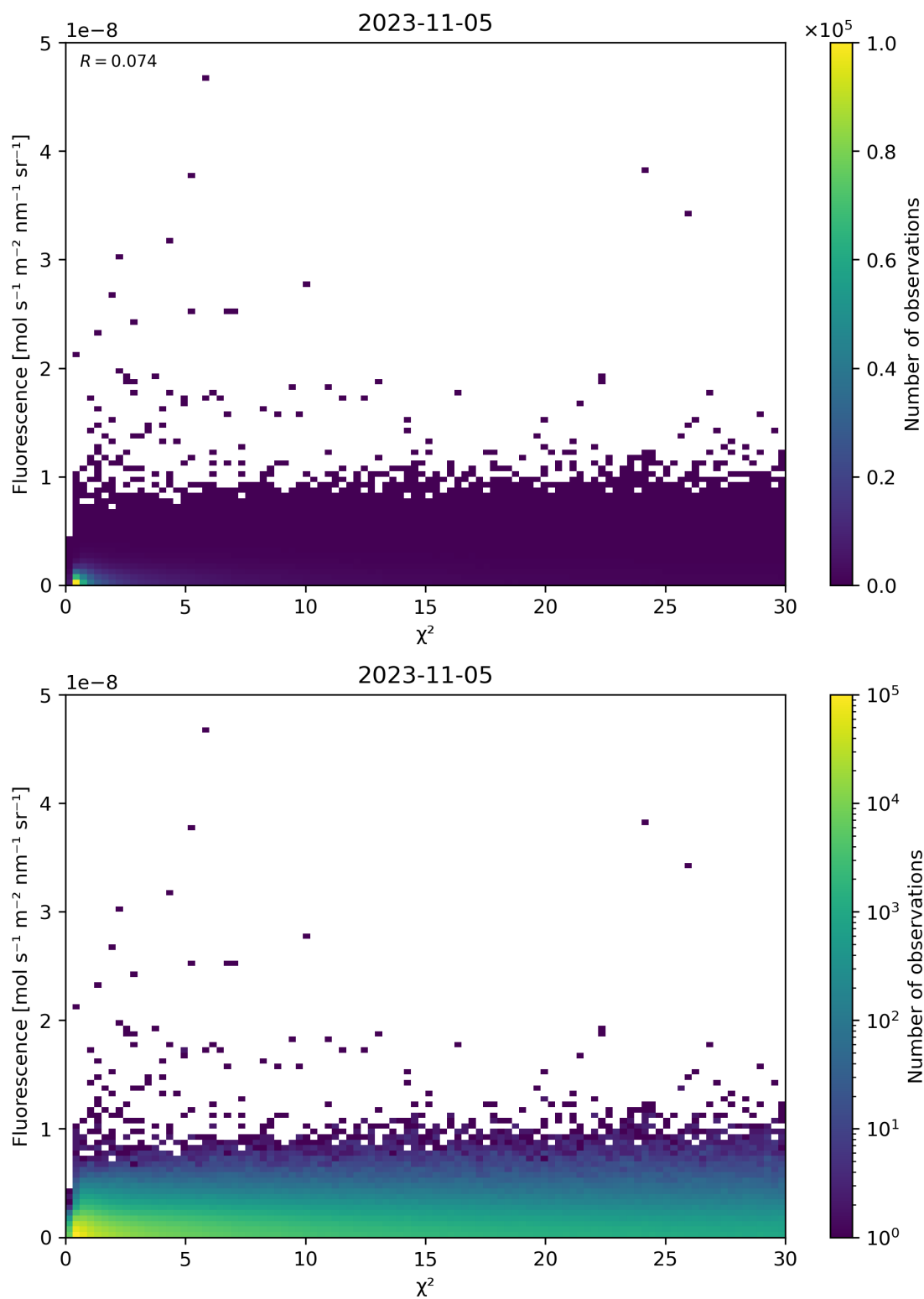
Figure 70: Scatter density plot of “ \chi^2 ” against “Fluorescence” for 2023-11-04 to 2023-11-06.
