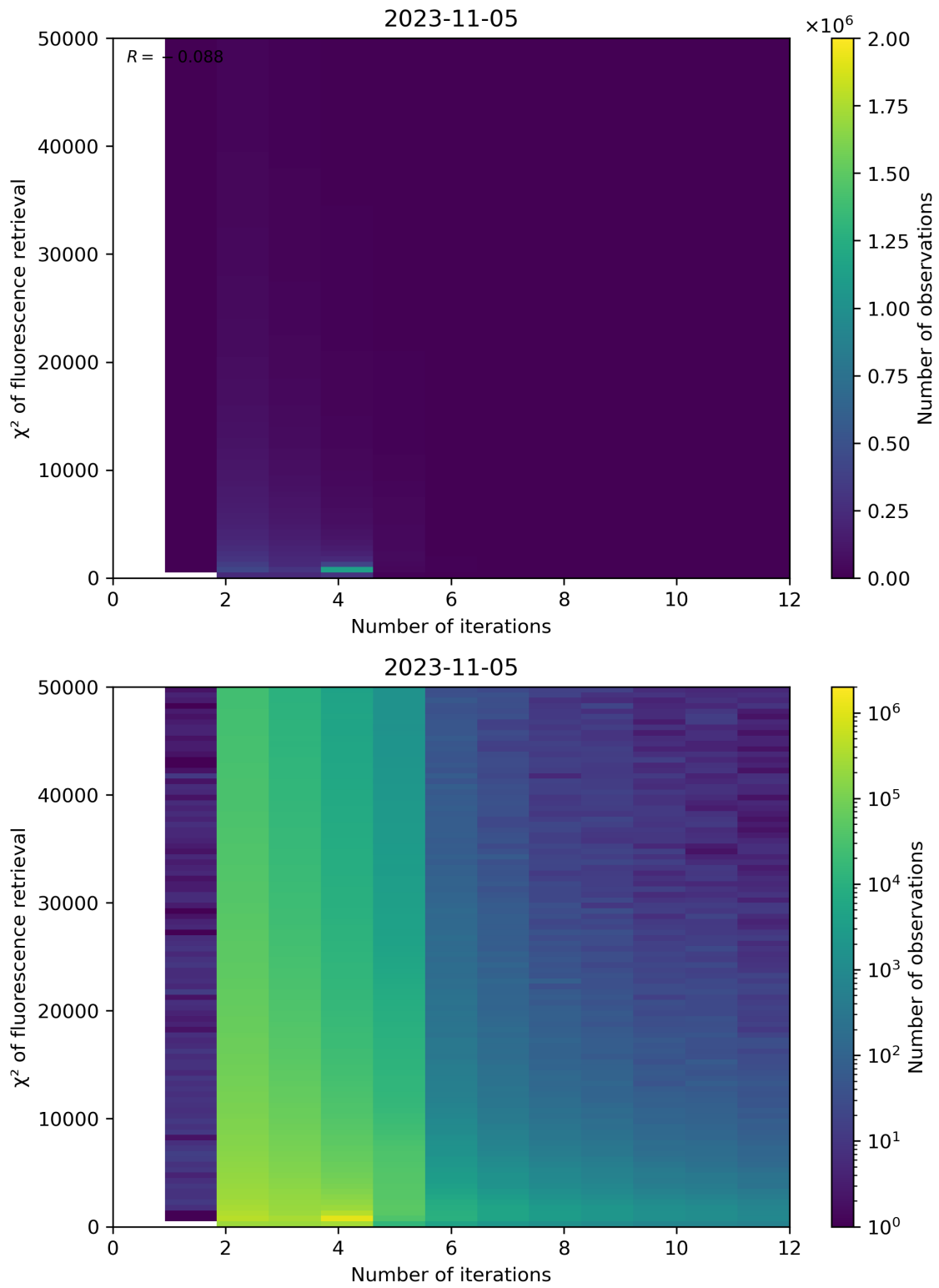
Figure 106: Scatter density plot of “Number of iterations” against “ \chi^2 of fluorescence retrieval” for 2023-11-04 to 2023-11-06.
