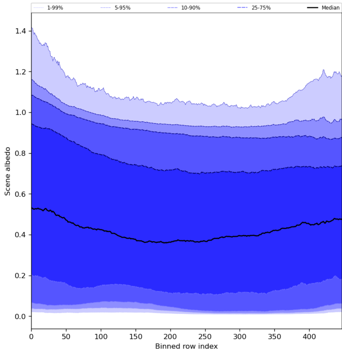
Figure 51: Along track statistics of “Scene albedo” for 2023-11-04 to 2023-11-06
