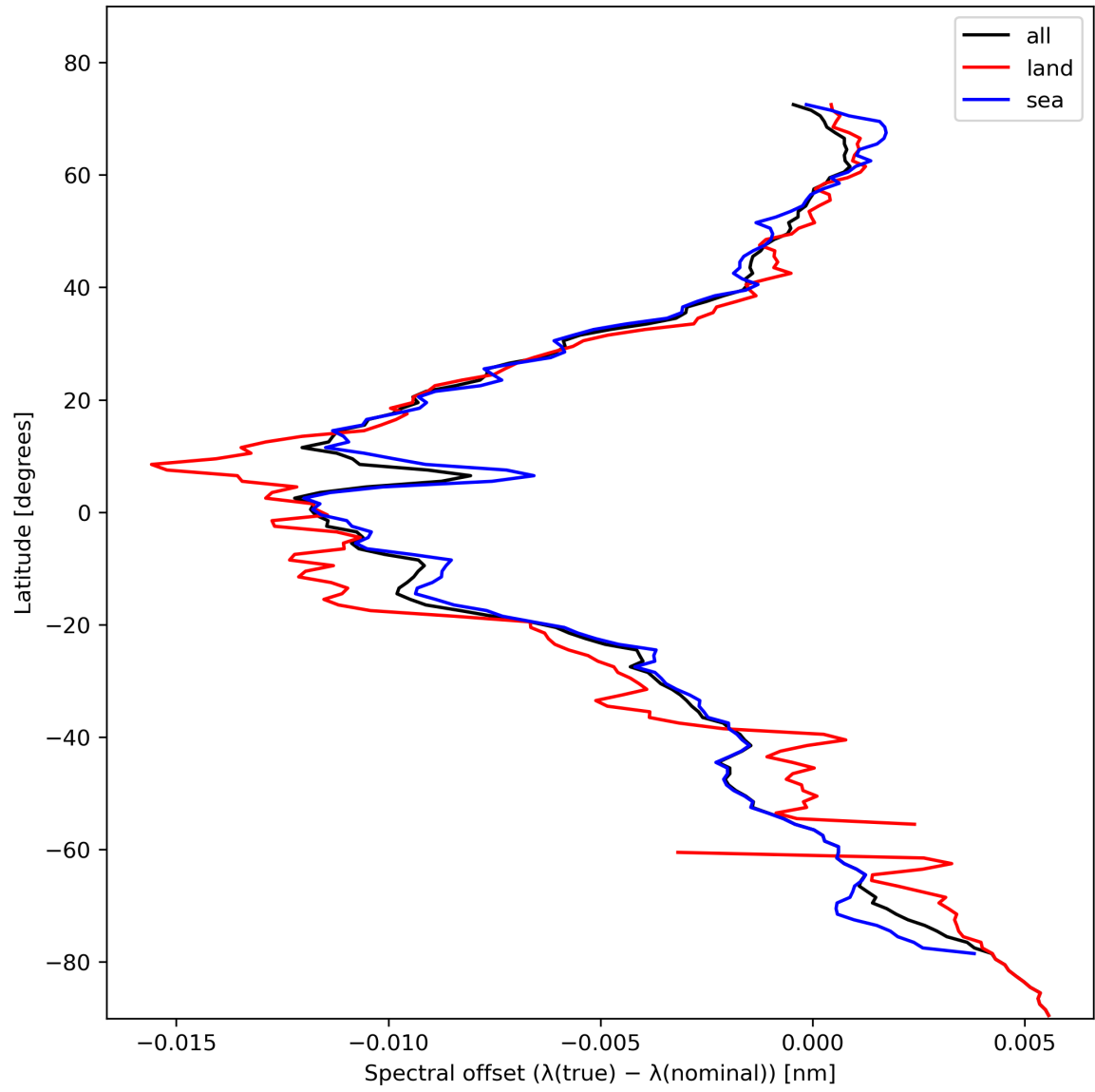
Figure 28: Zonal average of “Spectral offset ( \lambda(\text{true}) - \lambda(\text{nominal}) )” for 2023-11-04 to 2023-11-06.
