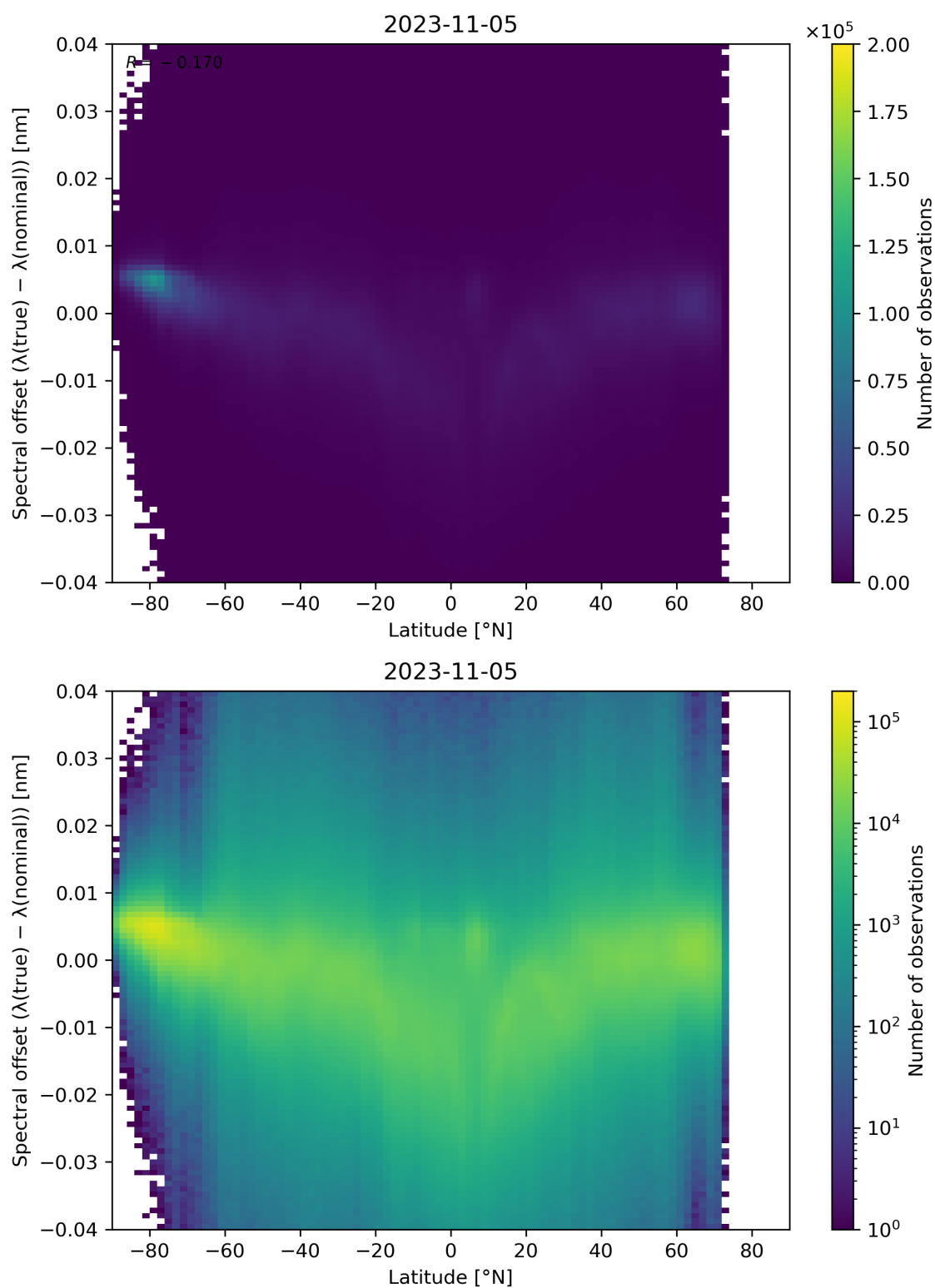
Figure 105: Scatter density plot of “Latitude” against “Spectral offset ( \lambda(\text{true}) - \lambda(\text{nominal}) )” for 2023-11-04 to 2023-11-06.
