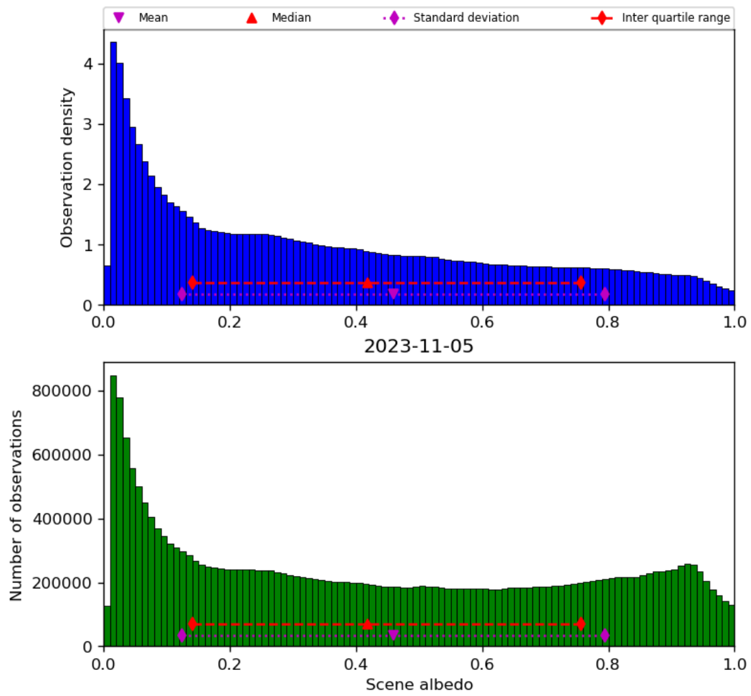
Figure 34: Histogram of “Scene albedo” for 2023-11-04 to 2023-11-06
