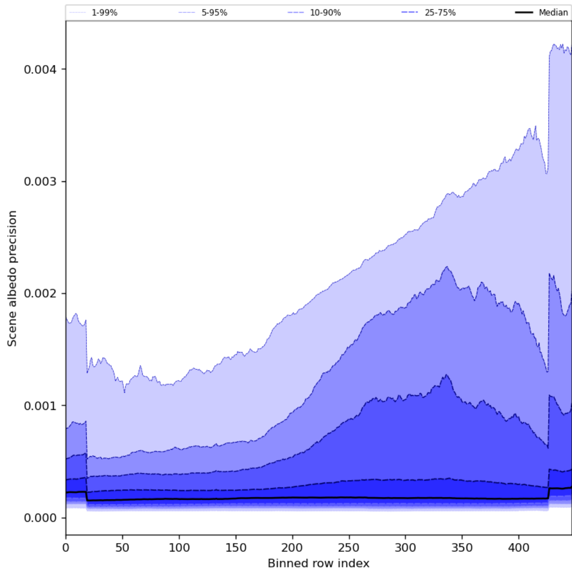
Figure 52: Along track statistics of “Scene albedo precision” for 2023-11-04 to 2023-11-06
