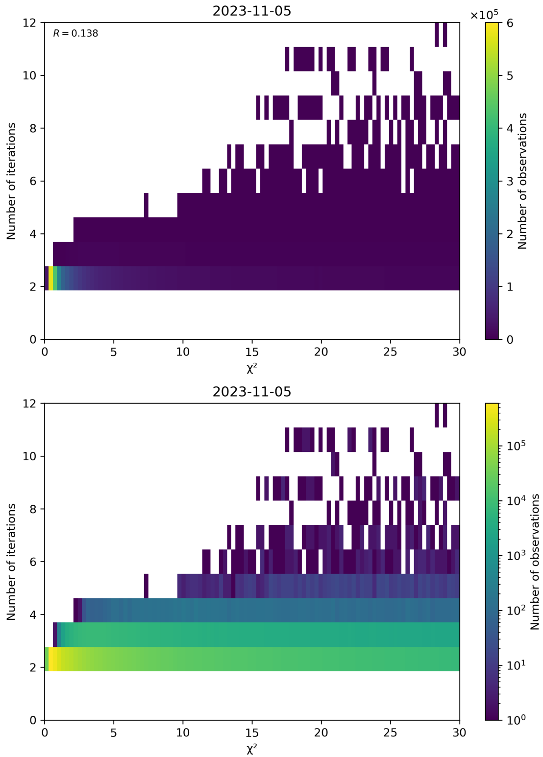
Figure 73: Scatter density plot of “ \chi^2 ” against “Number of iterations” for 2023-11-04 to 2023-11-06.
