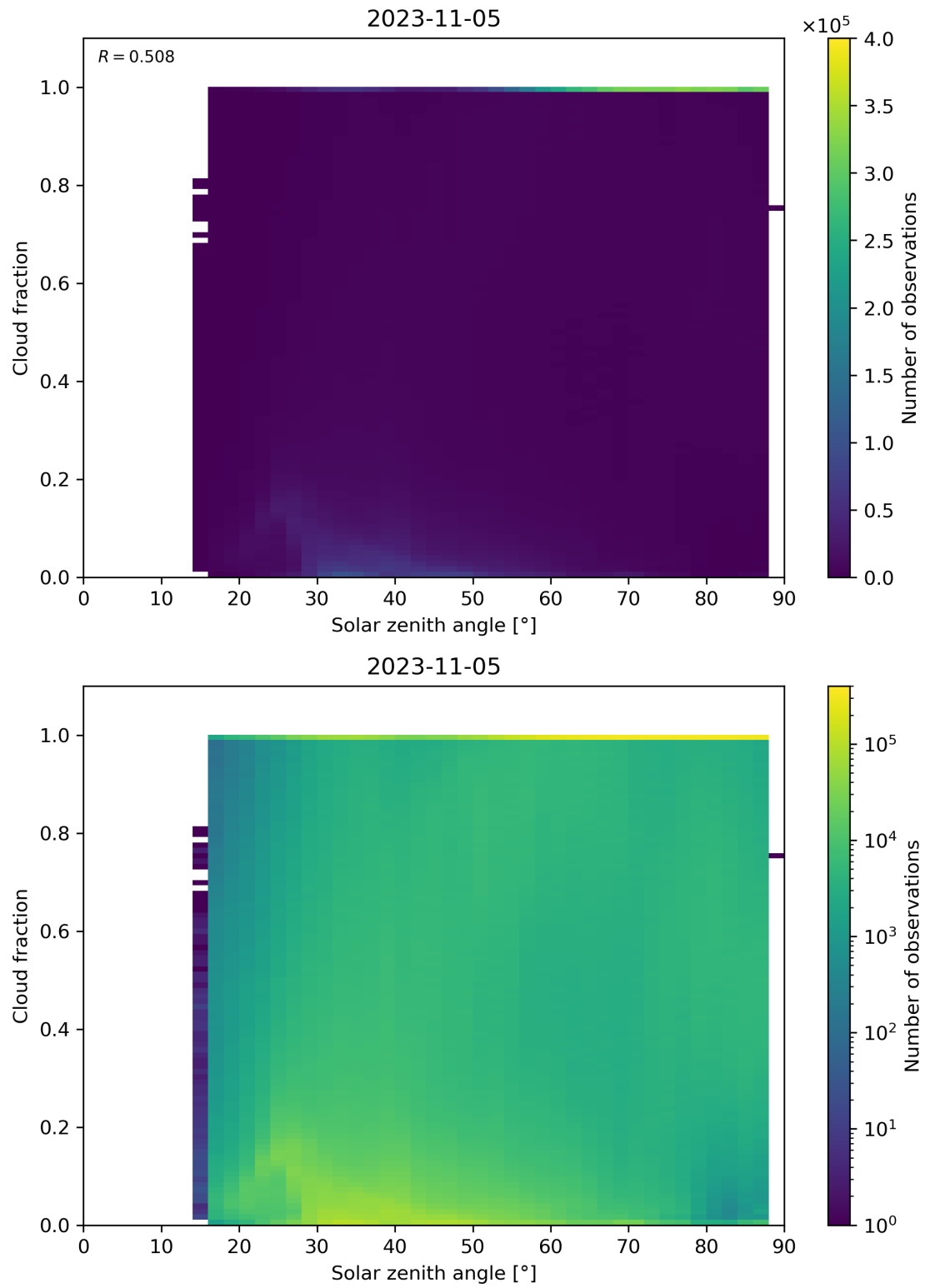
Figure 121: Scatter density plot of “Solar zenith angle” against “Cloud fraction” for 2023-11-04 to 2023-11-06.
