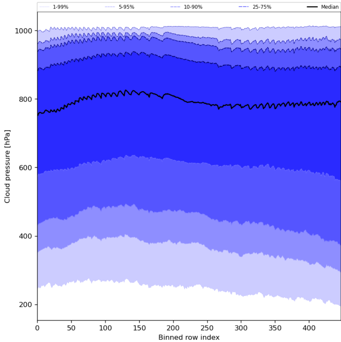
Figure 47: Along track statistics of “Cloud pressure” for 2023-11-04 to 2023-11-06
