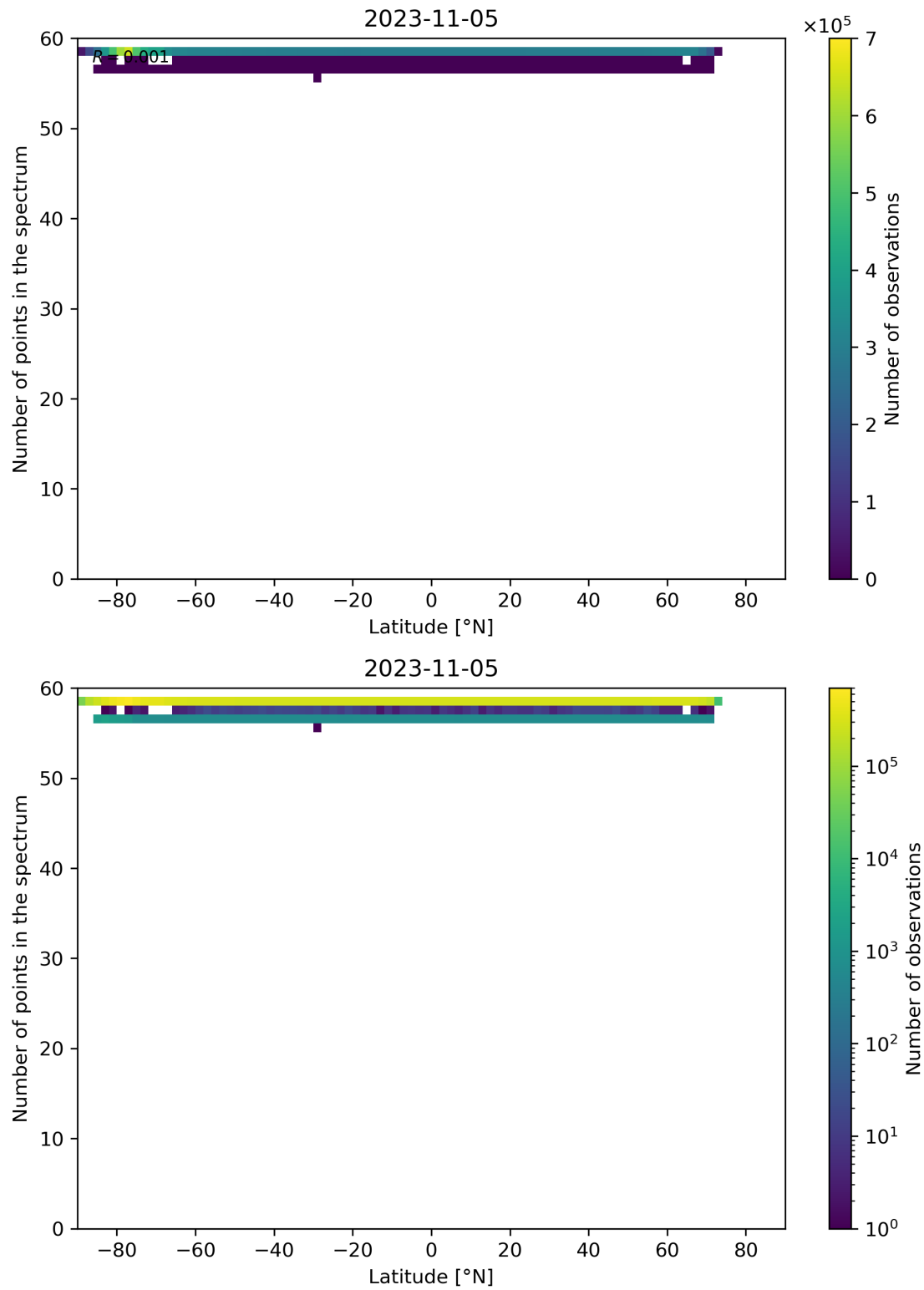
Figure 103: Scatter density plot of “Latitude” against “Number of points in the spectrum” for 2023-11-04 to 2023-11-06.
