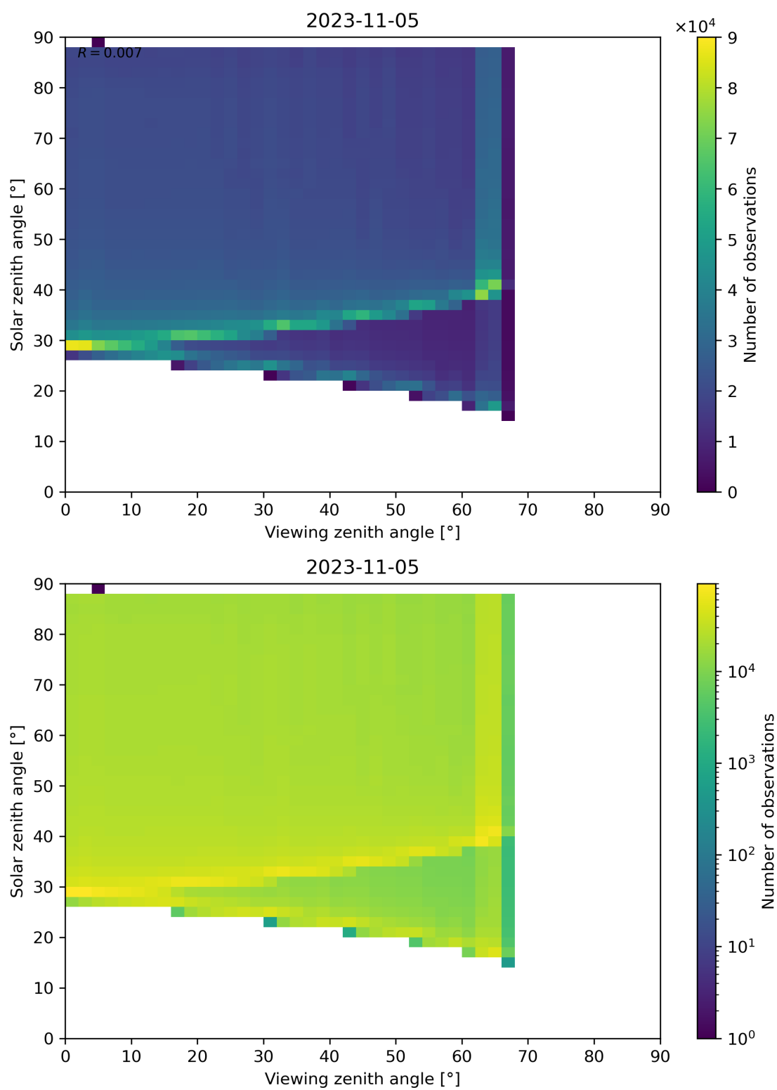
Figure 139: Scatter density plot of “Viewing zenith angle” against “Solar zenith angle” for 2023-11-04 to 2023-11-06.
