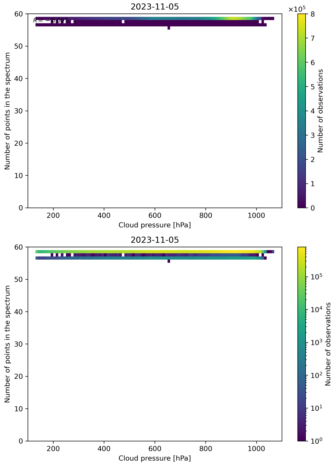
Figure 90: Scatter density plot of “Cloud pressure” against “Number of points in the spectrum” for 2023-11-04 to 2023-11-06.
