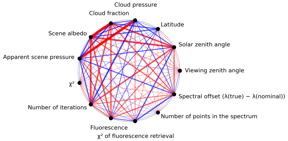
Figure 1: Map of correlation graph for 2023-11-04 to 2023-11-06.
