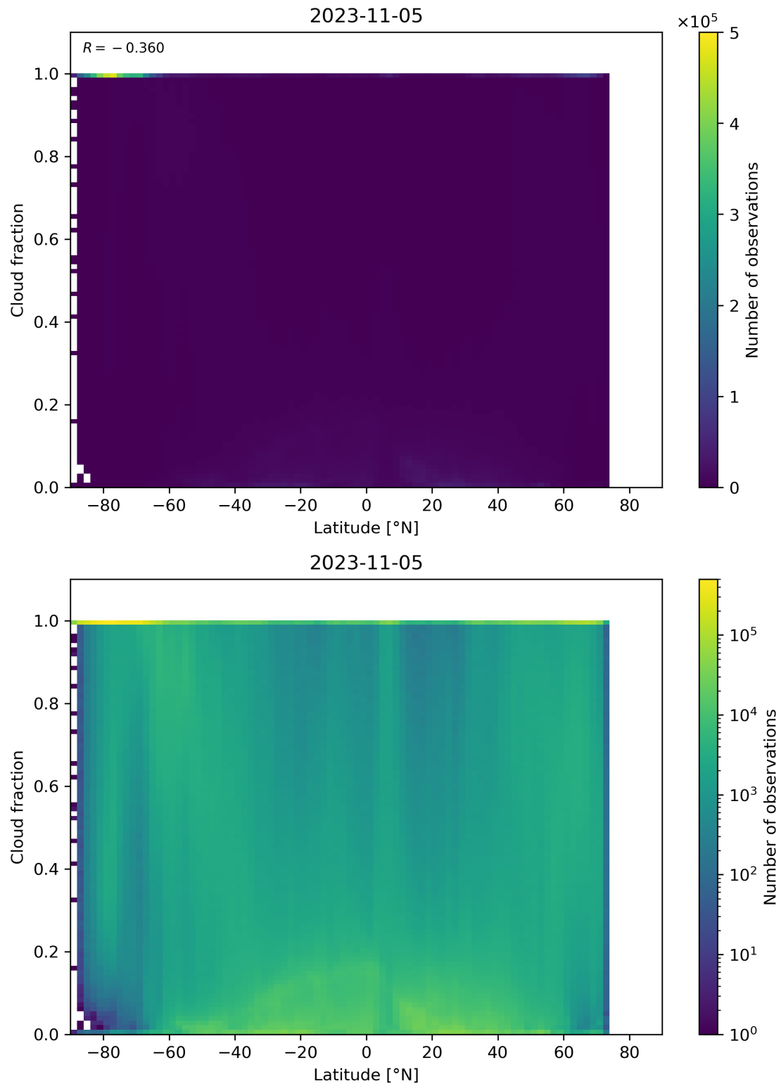
Figure 99: Scatter density plot of “Latitude” against “Cloud fraction” for 2023-11-04 to 2023-11-06.
