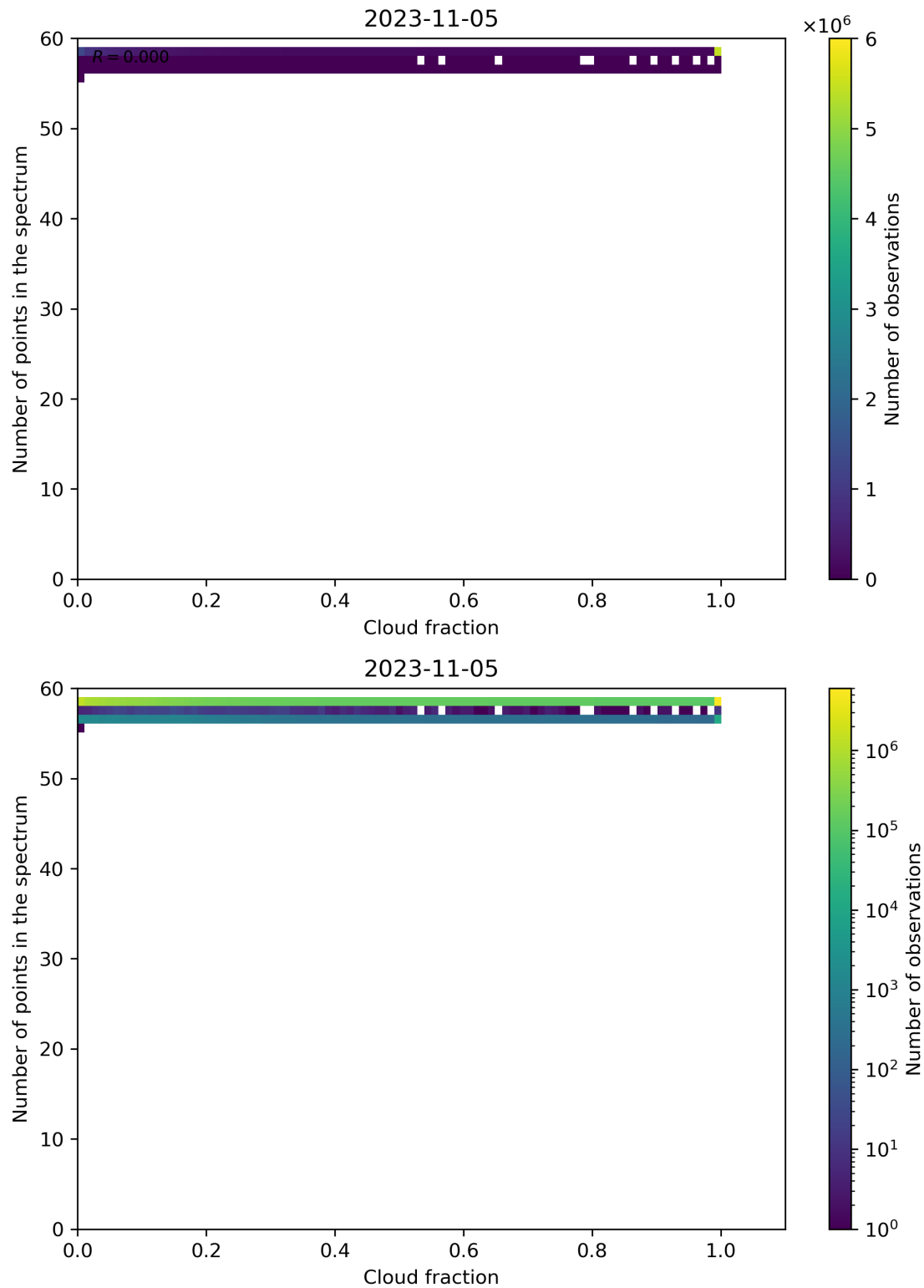
Figure 81: Scatter density plot of “Cloud fraction” against “Number of points in the spectrum” for 2023-11-04 to 2023-11-06.
