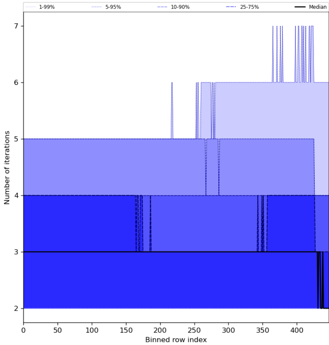
Figure 56: Along track statistics of “Number of iterations” for 2023-11-04 to 2023-11-06
