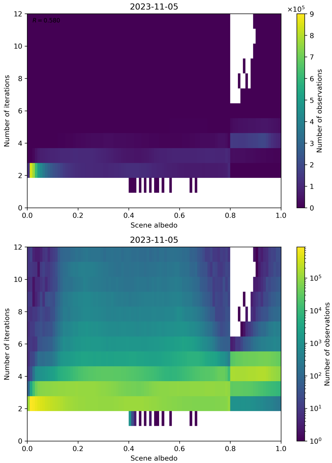
Figure 115: Scatter density plot of “Scene albedo” against “Number of iterations” for 2023-11-04 to 2023-11-06.
