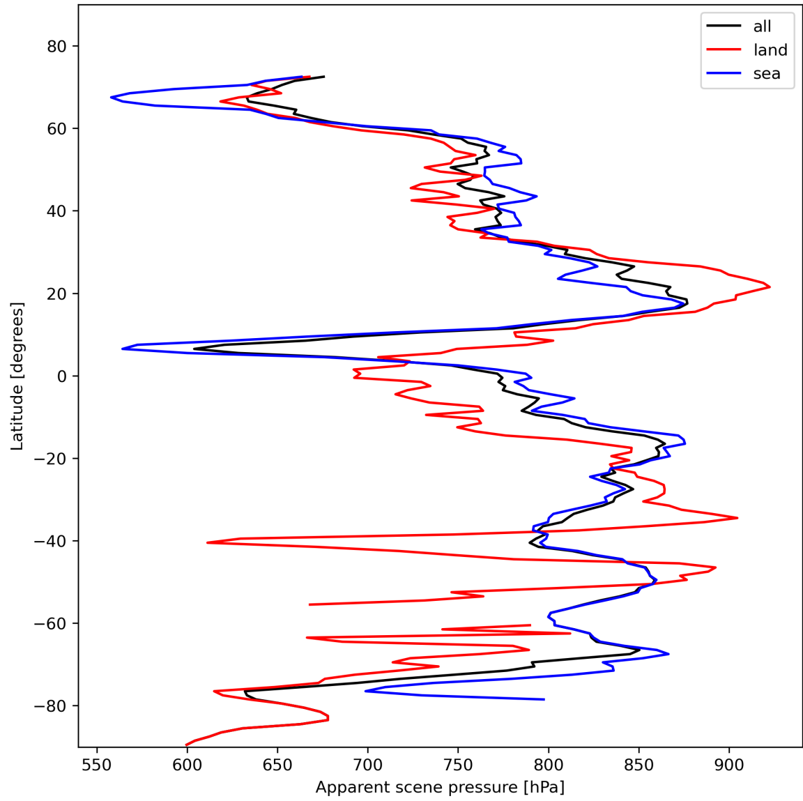
Figure 19: Zonal average of “Apparent scene pressure” for 2023-11-04 to 2023-11-06.
