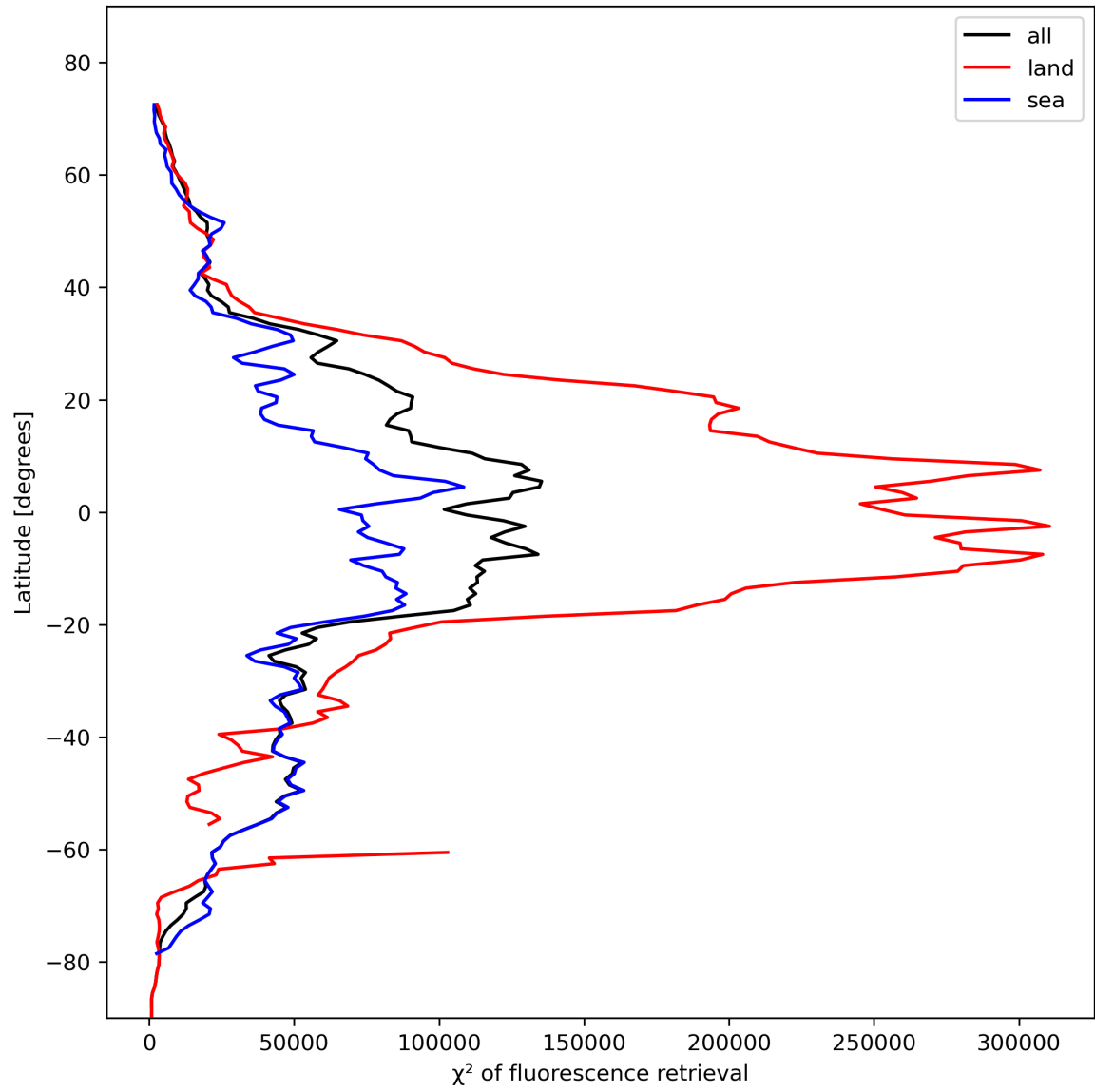
Figure 25: Zonal average of “ \chi^2 of fluorescence retrieval” for 2023-11-04 to 2023-11-06.
