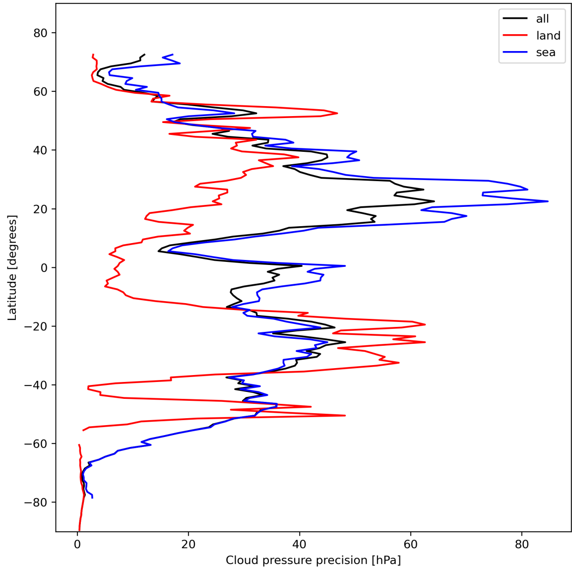
Figure 14: Zonal average of “Cloud pressure precision” for 2023-11-04 to 2023-11-06.
