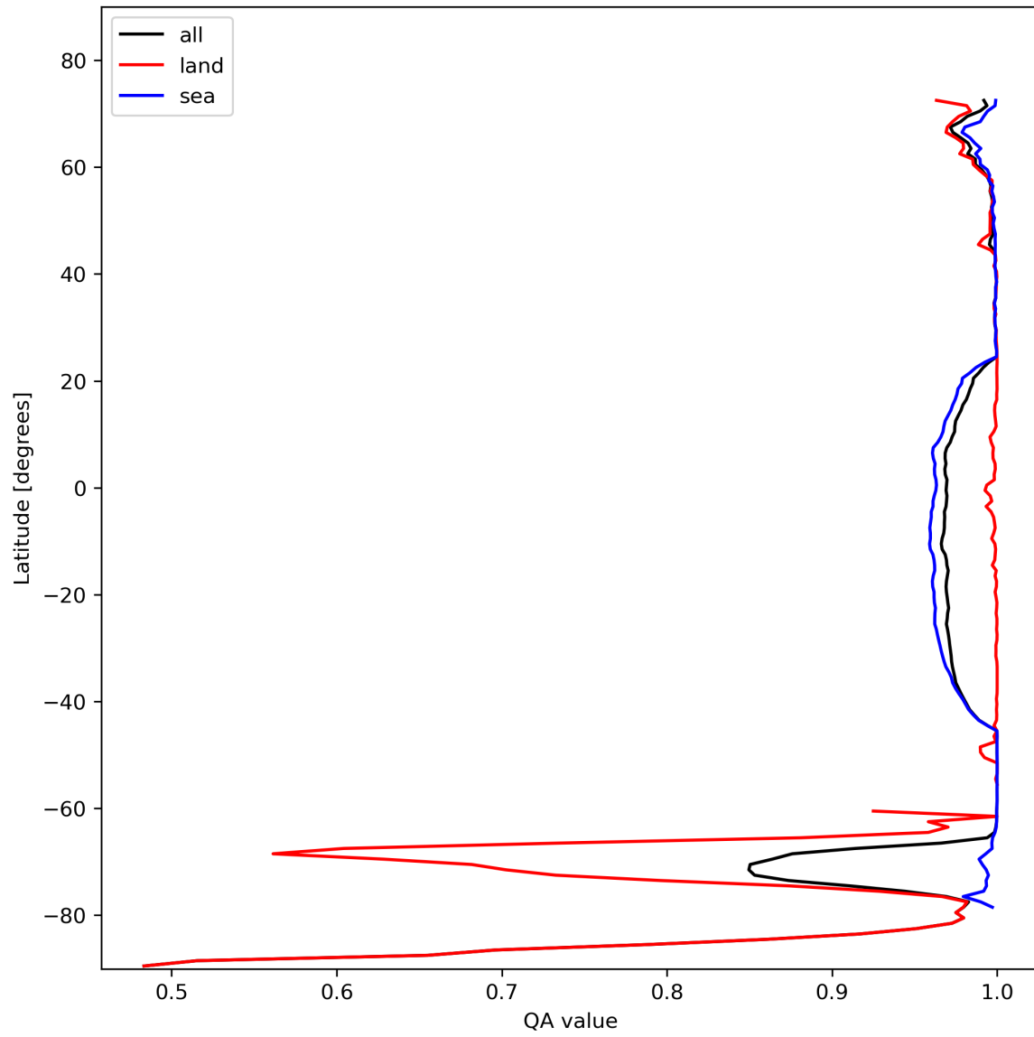
Figure 12: Zonal average of “QA value” for 2023-11-04 to 2023-11-06.
