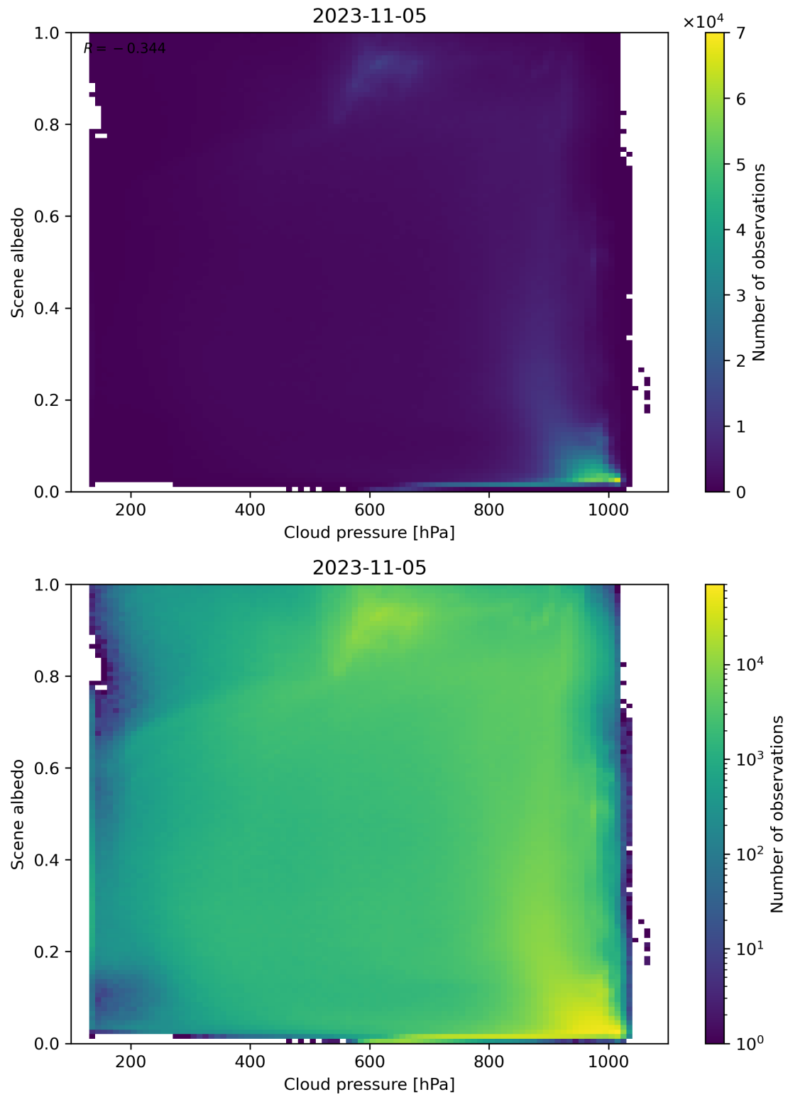
Figure 91: Scatter density plot of “Cloud pressure” against “Scene albedo” for 2023-11-04 to 2023-11-06.
