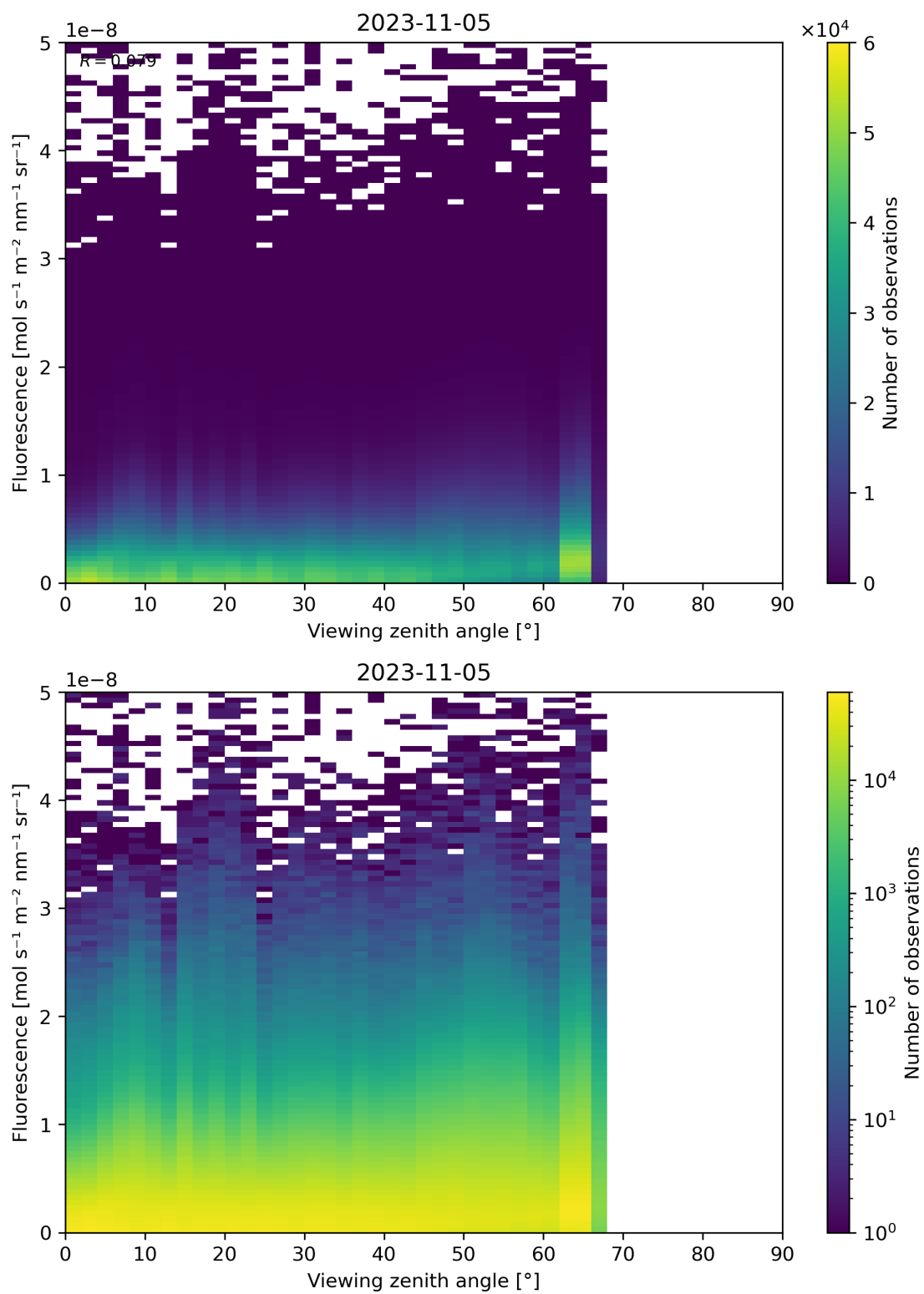
Figure 134: Scatter density plot of “Viewing zenith angle” against “Fluorescence” for 2023-11-04 to 2023-11-06.
