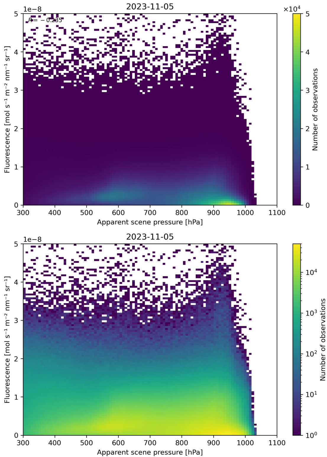
Figure 65: Scatter density plot of “Apparent scene pressure” against “Fluorescence” for 2023-11-04 to 2023-11-06.
