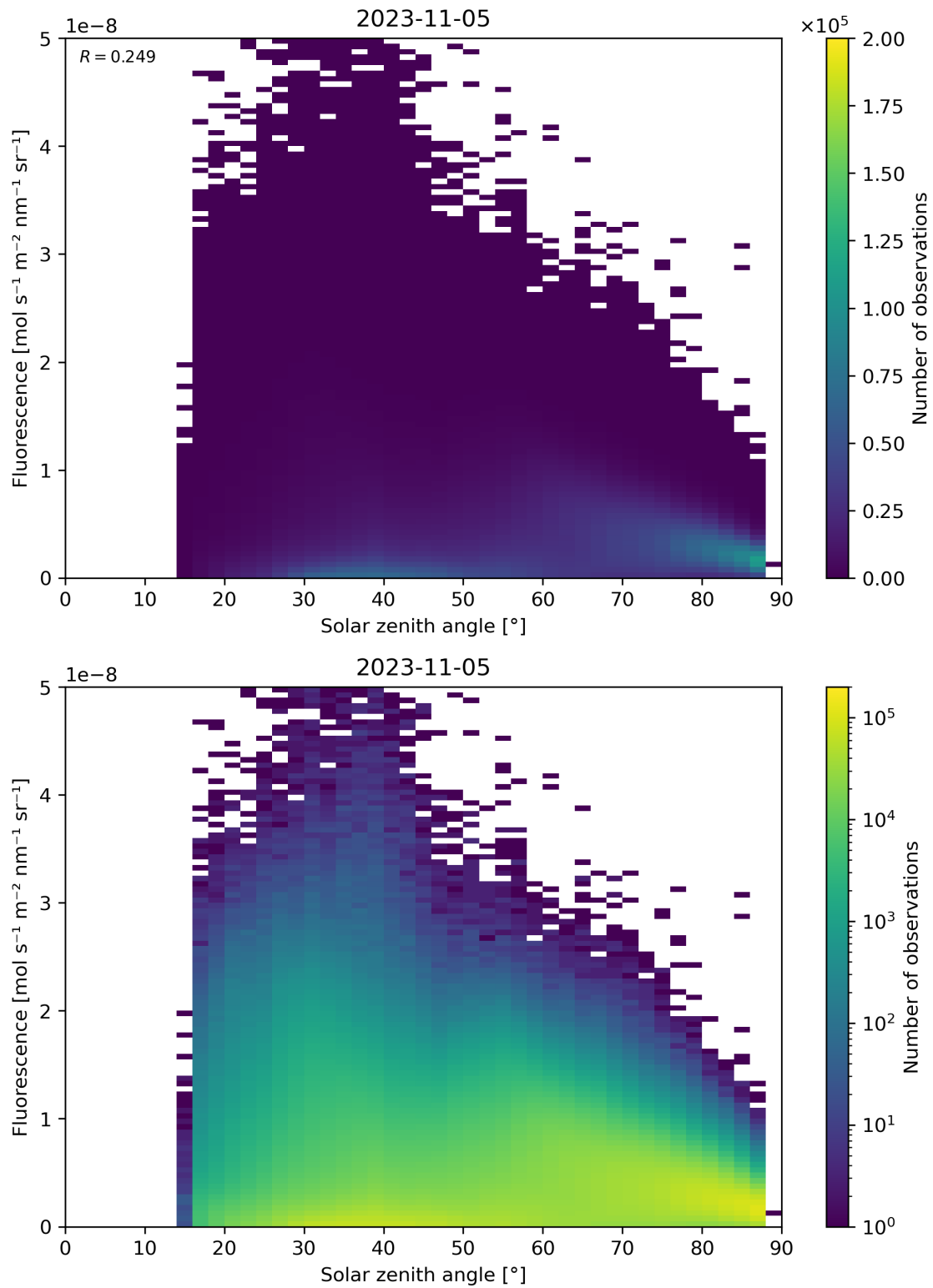
Figure 123: Scatter density plot of “Solar zenith angle” against “Fluorescence” for 2023-11-04 to 2023-11-06.
