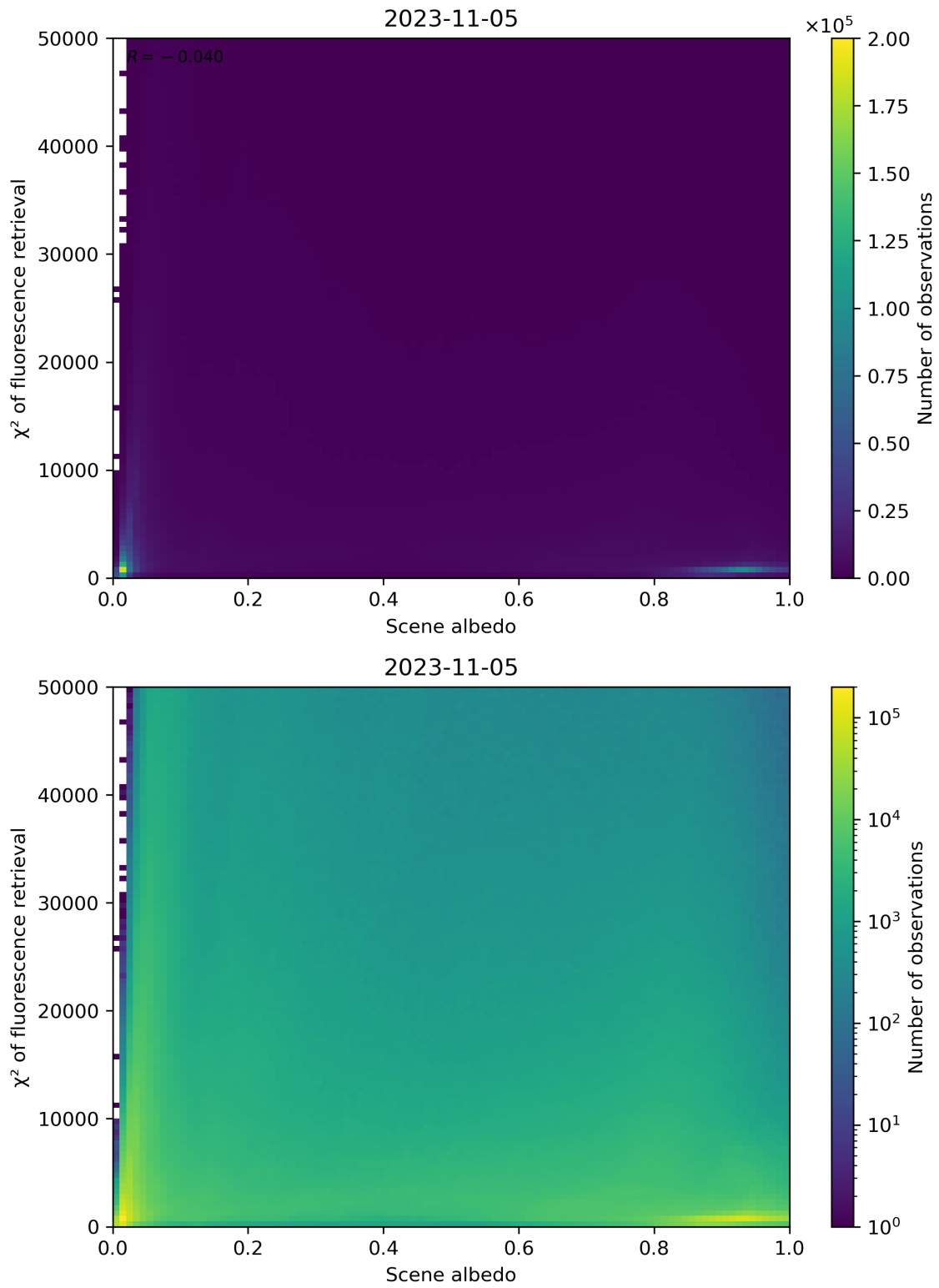
Figure 113: Scatter density plot of “Scene albedo” against “ \chi^2 of fluorescence retrieval” for 2023-11-04 to 2023-11-06.
