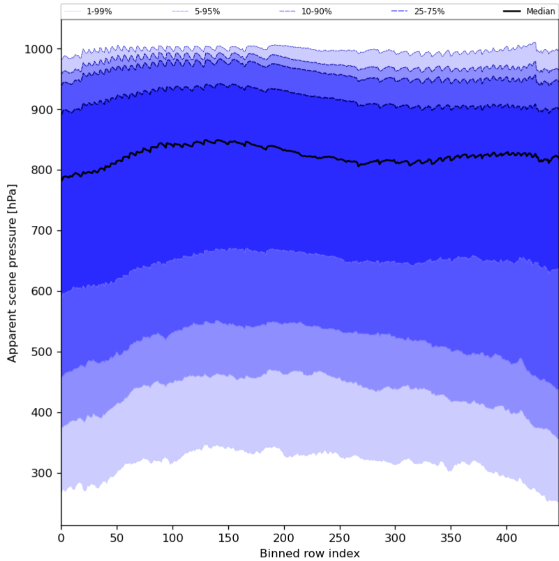
Figure 53: Along track statistics of “Apparent scene pressure” for 2023-11-04 to 2023-11-06
