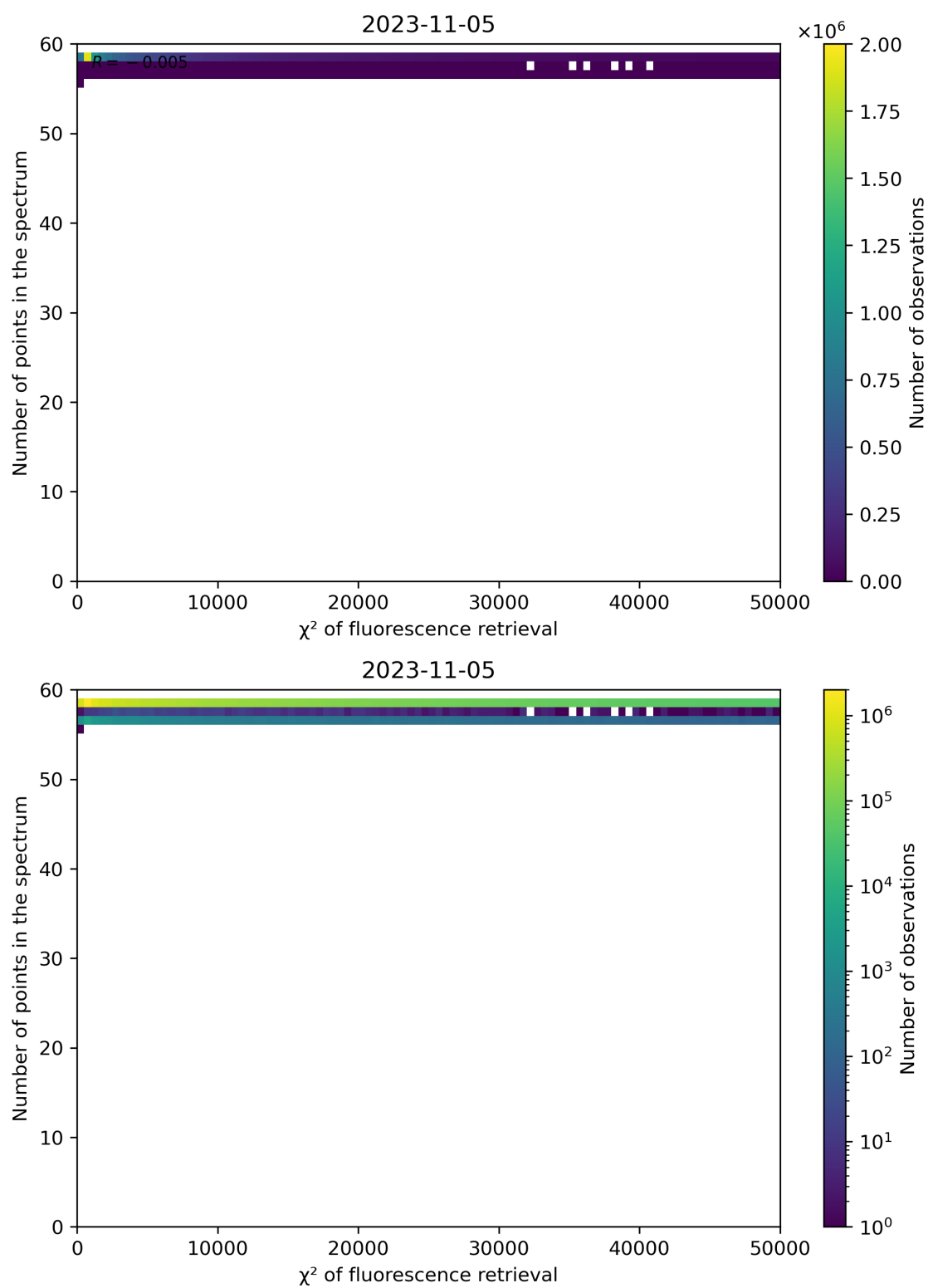
Figure 71: Scatter density plot of " \chi^2 of fluorescence retrieval" against "Number of points in the spectrum" for 2023-11-04 to 2023-11-06.
