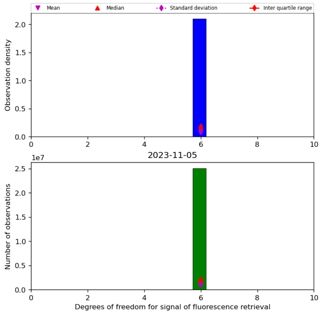
Figure 43: Histogram of “Degrees of freedom for signal of fluorescence retrieval” for 2023-11-04 to 2023-11-06
