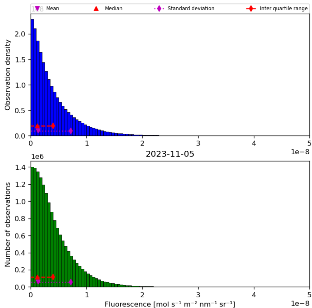
Figure 40: Histogram of “Fluorescence” for 2023-11-04 to 2023-11-06
