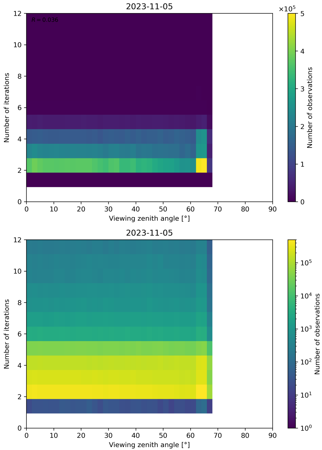
Figure 136: Scatter density plot of “Viewing zenith angle” against “Number of iterations” for 2023-11-04 to 2023-11-06.
