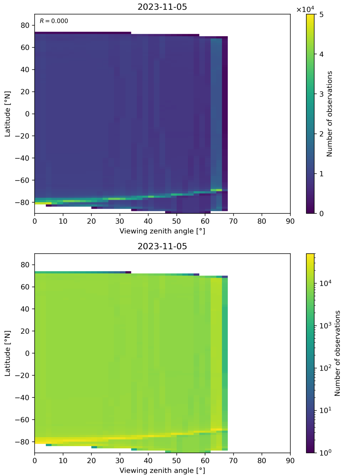
Figure 135: Scatter density plot of “Viewing zenith angle” against “Latitude” for 2023-11-04 to 2023-11-06.
