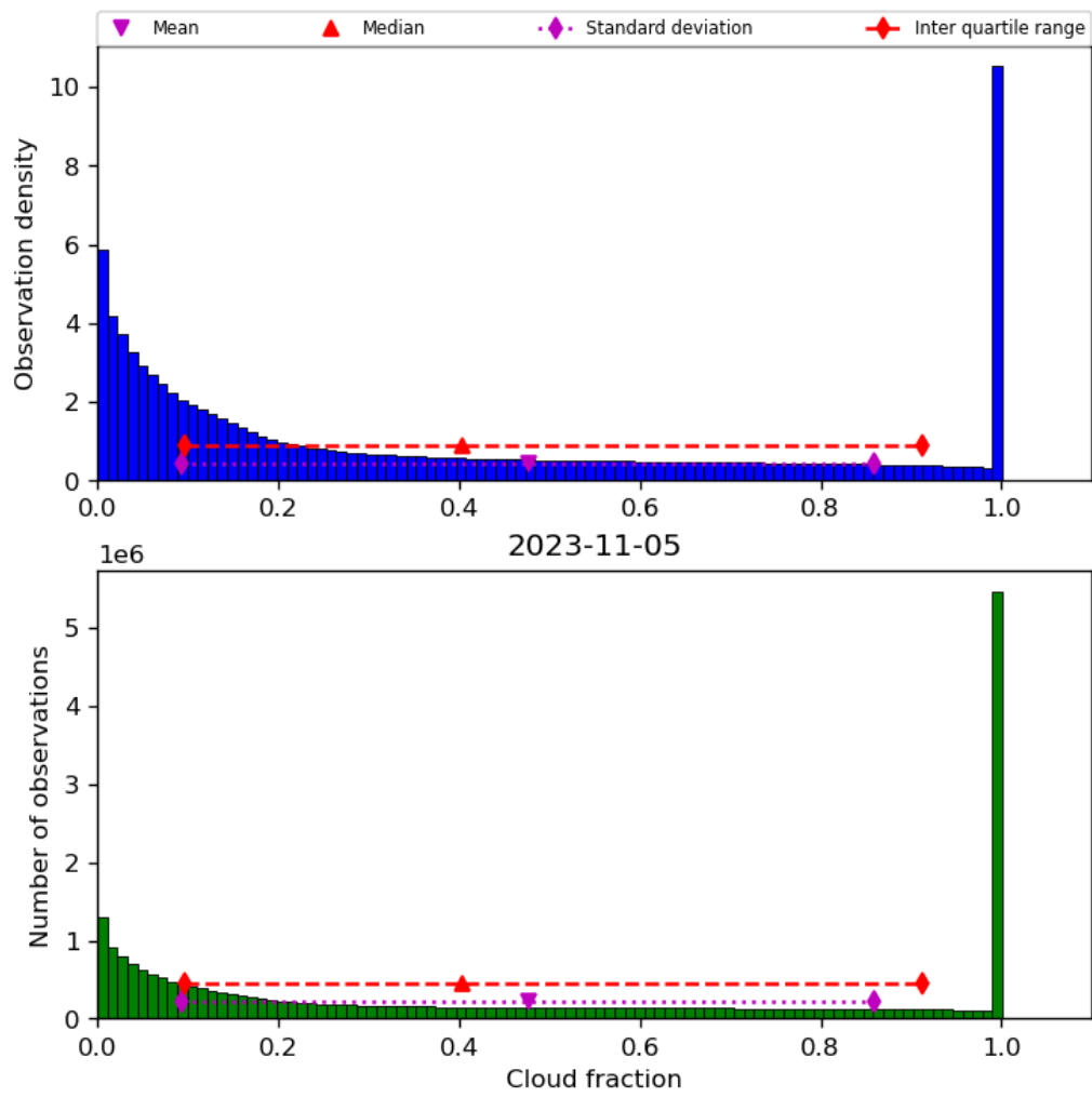
Figure 32: Histogram of “Cloud fraction” for 2023-11-04 to 2023-11-06
