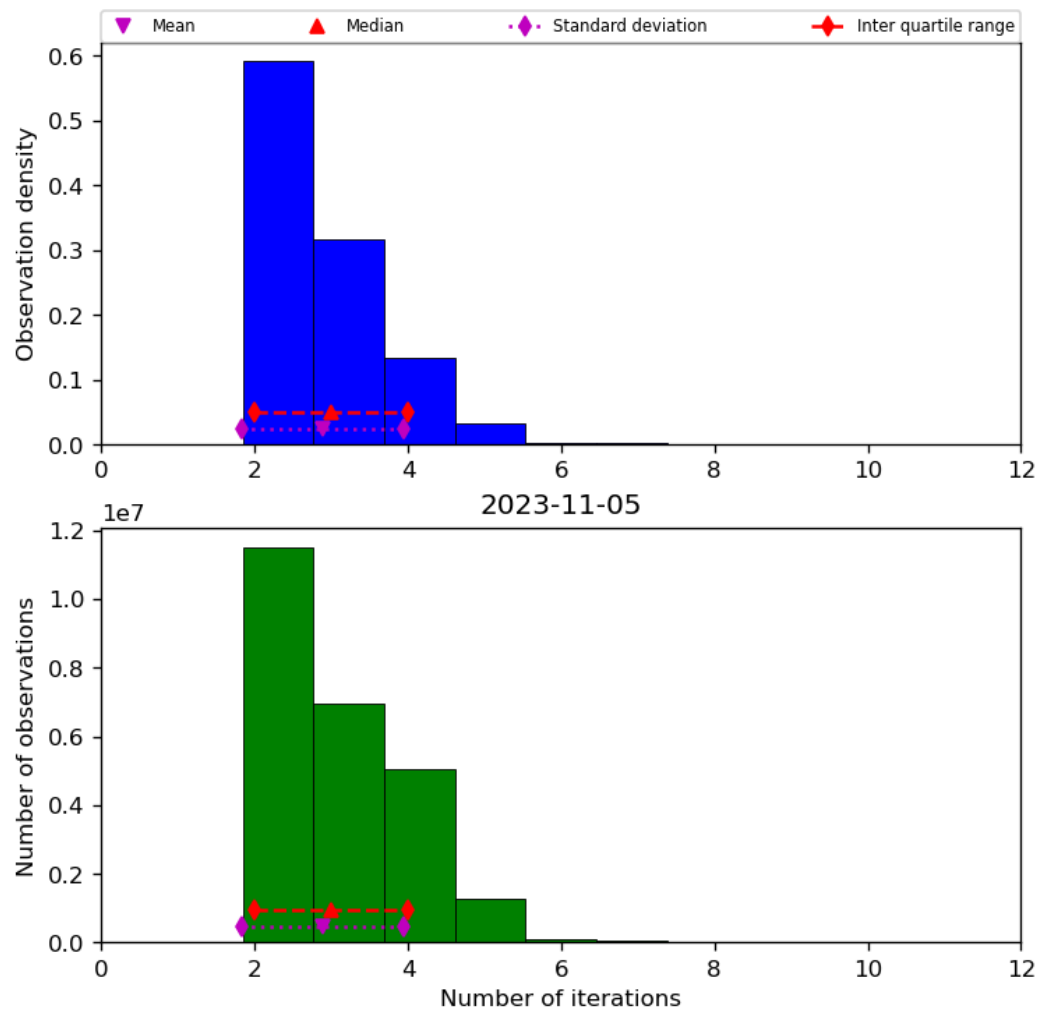
Figure 39: Histogram of “Number of iterations” for 2023-11-04 to 2023-11-06
