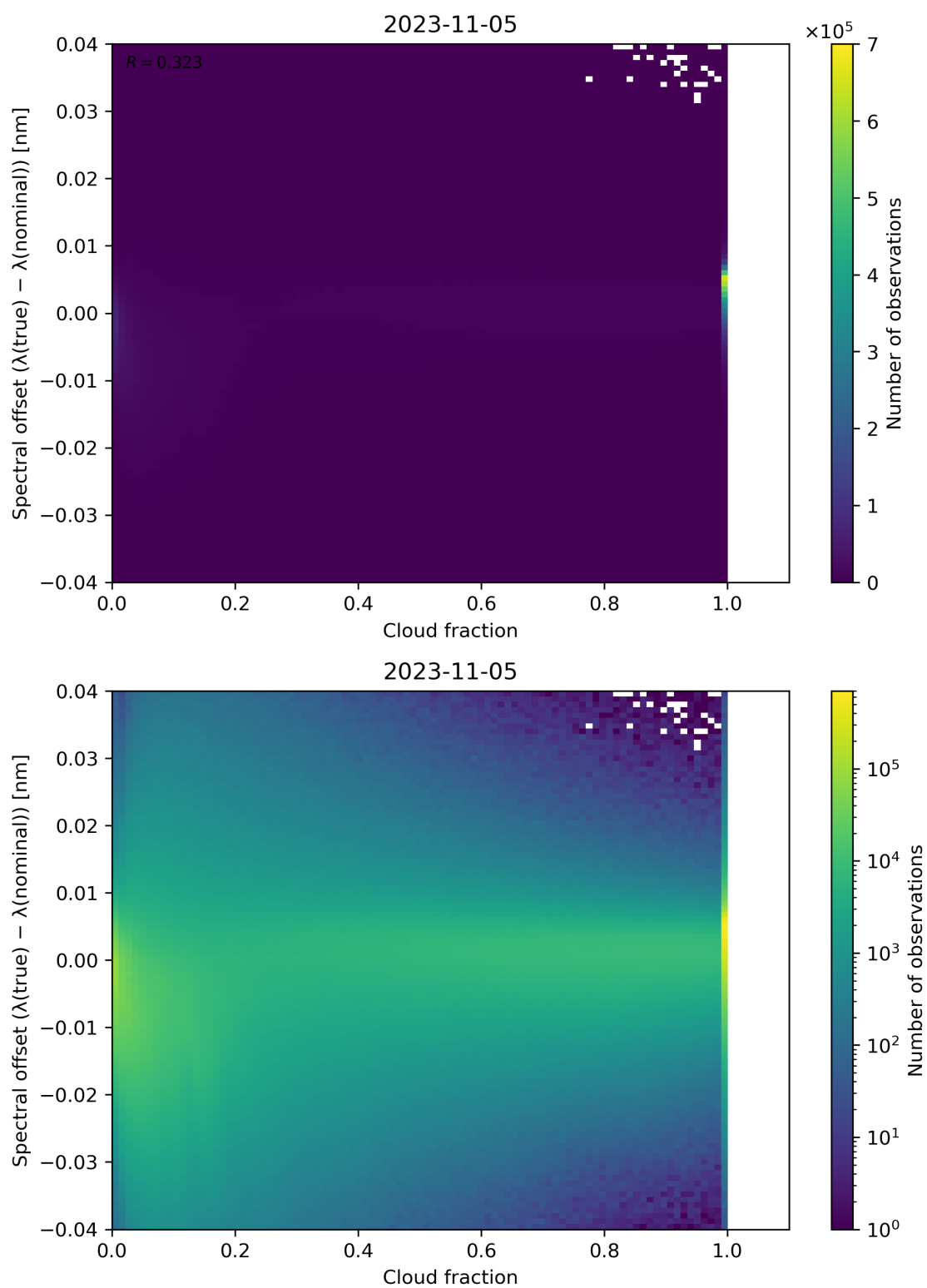
Figure 83: Scatter density plot of “Cloud fraction” against “Spectral offset ( \lambda(\text{true}) - \lambda(\text{nominal}) )” for 2023-11-04 to 2023-11-06.
