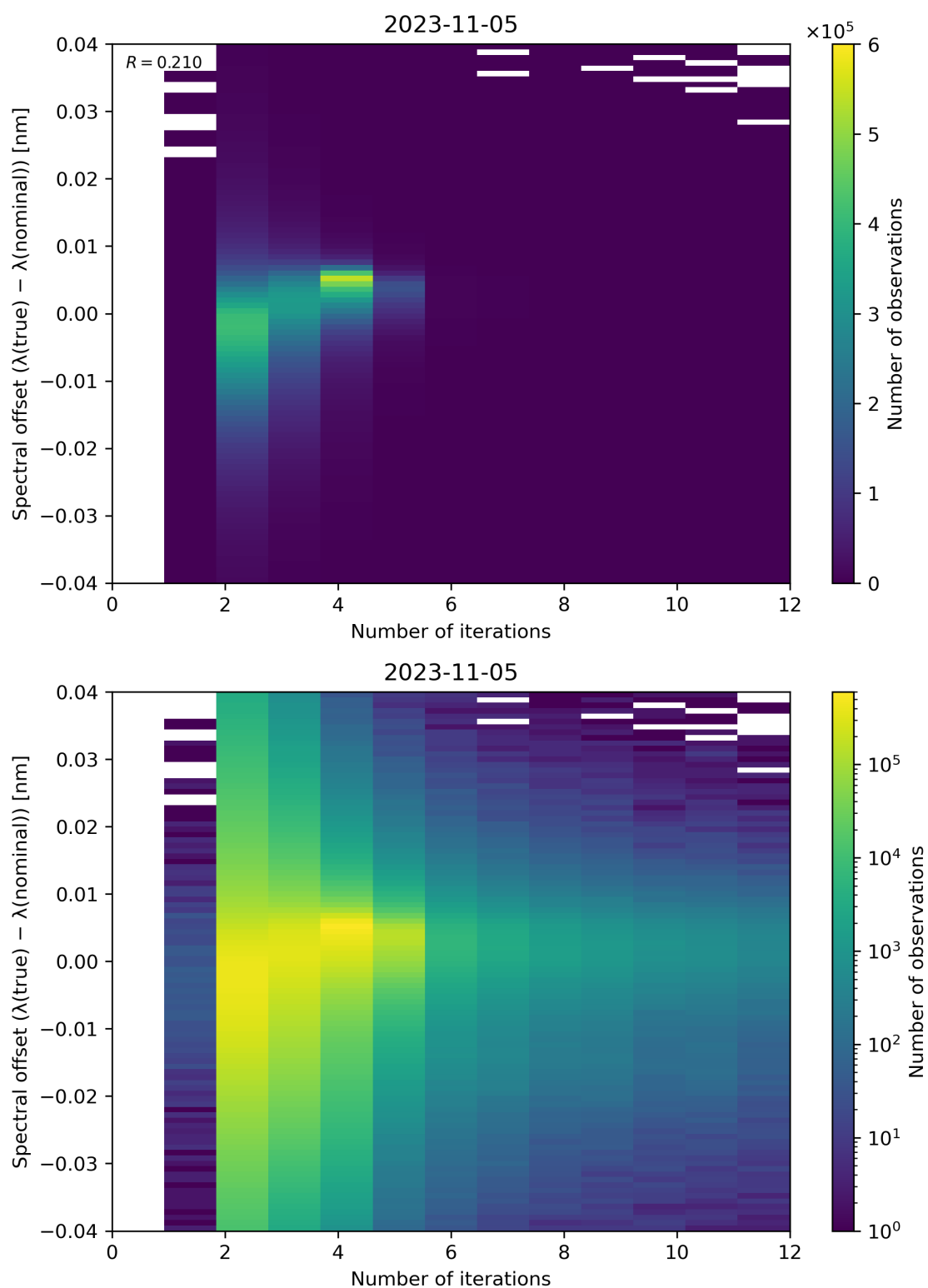
Figure 109: Scatter density plot of “Number of iterations” against “Spectral offset ( \lambda(\text{true}) - \lambda(\text{nominal}) )” for 2023-11-04 to 2023-11-06.
