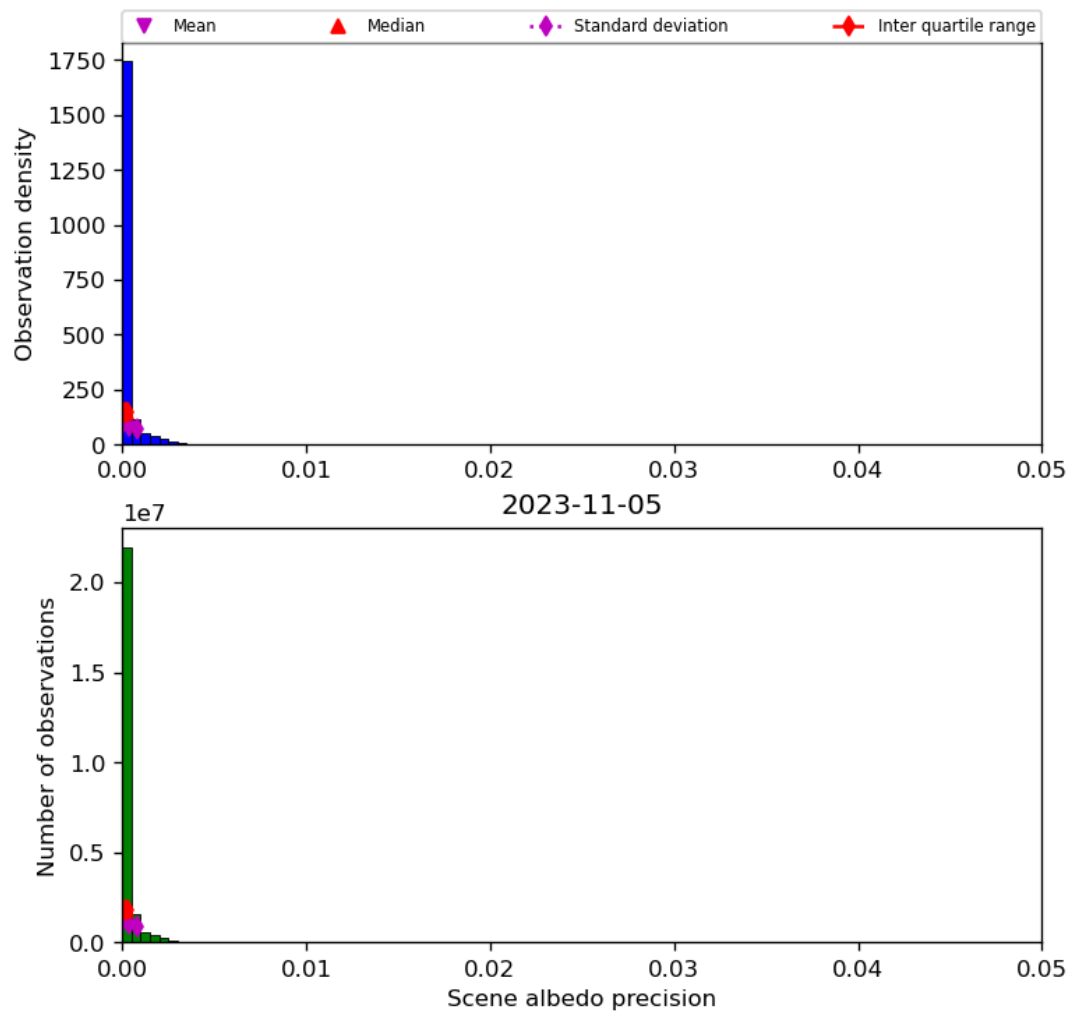
Figure 35: Histogram of “Scene albedo precision” for 2023-11-04 to 2023-11-06
