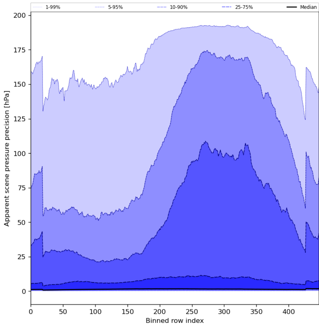
Figure 54: Along track statistics of “Apparent scene pressure precision” for 2023-11-04 to 2023-11-06
