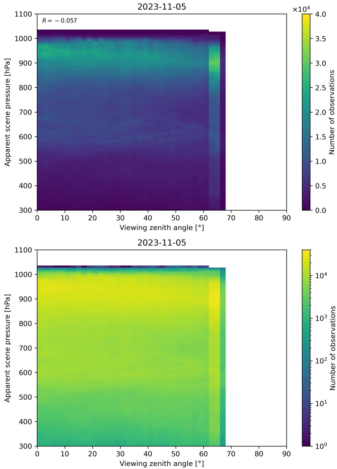
Figure 129: Scatter density plot of “Viewing zenith angle” against “Apparent scene pressure” for 2023-11-04 to 2023-11-06.
