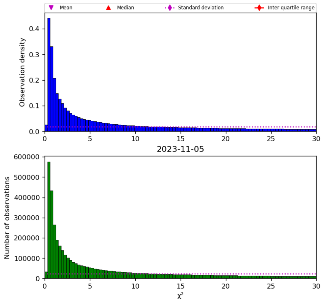
Figure 38: Histogram of “ \chi^2 ” for 2023-11-04 to 2023-11-06
