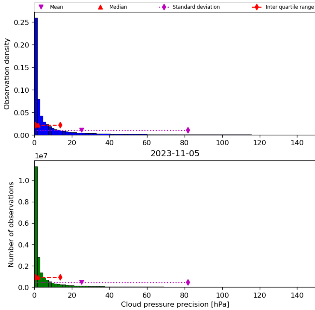
Figure 31: Histogram of “Cloud pressure precision” for 2023-11-04 to 2023-11-06
