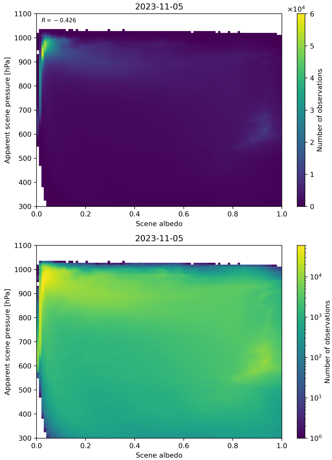
Figure 111: Scatter density plot of “Scene albedo” against “Apparent scene pressure” for 2023-11-04 to 2023-11-06.
