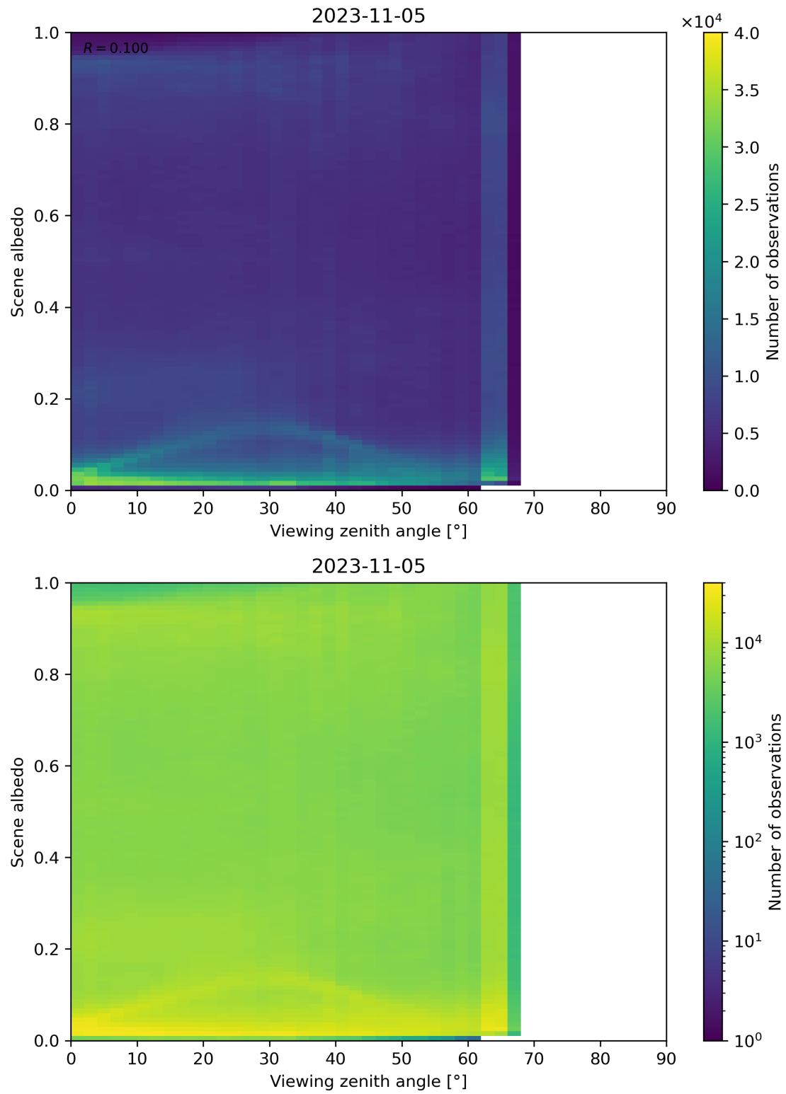
Figure 138: Scatter density plot of “Viewing zenith angle” against “Scene albedo” for 2023-11-04 to 2023-11-06.
