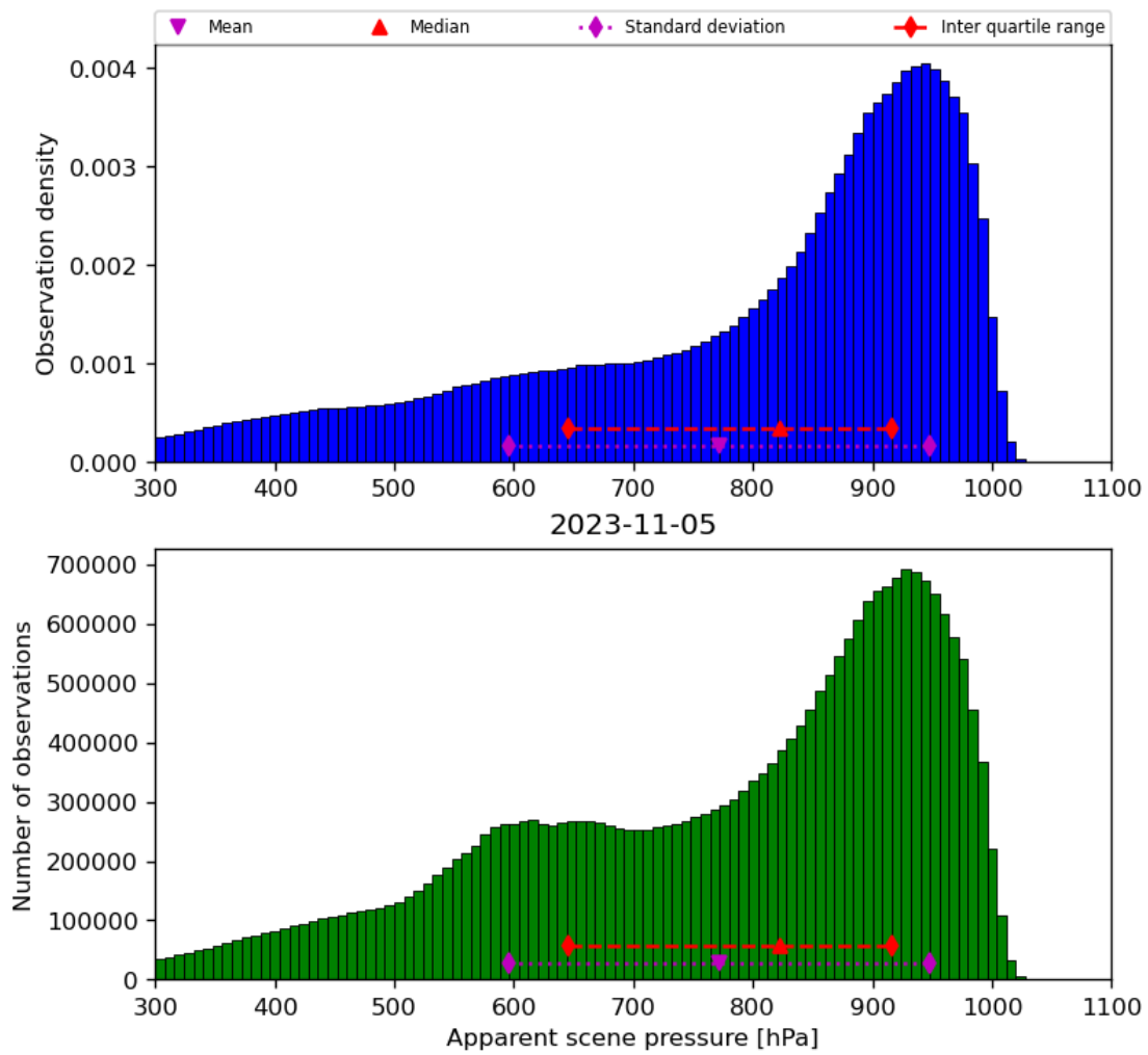
Figure 36: Histogram of “Apparent scene pressure” for 2023-11-04 to 2023-11-06
