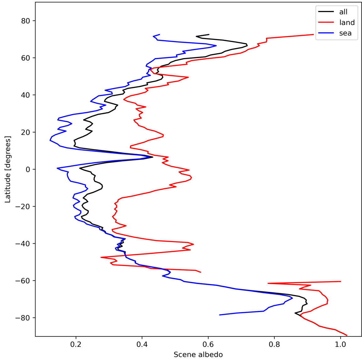
Figure 17: Zonal average of “Scene albedo” for 2023-11-04 to 2023-11-06.
