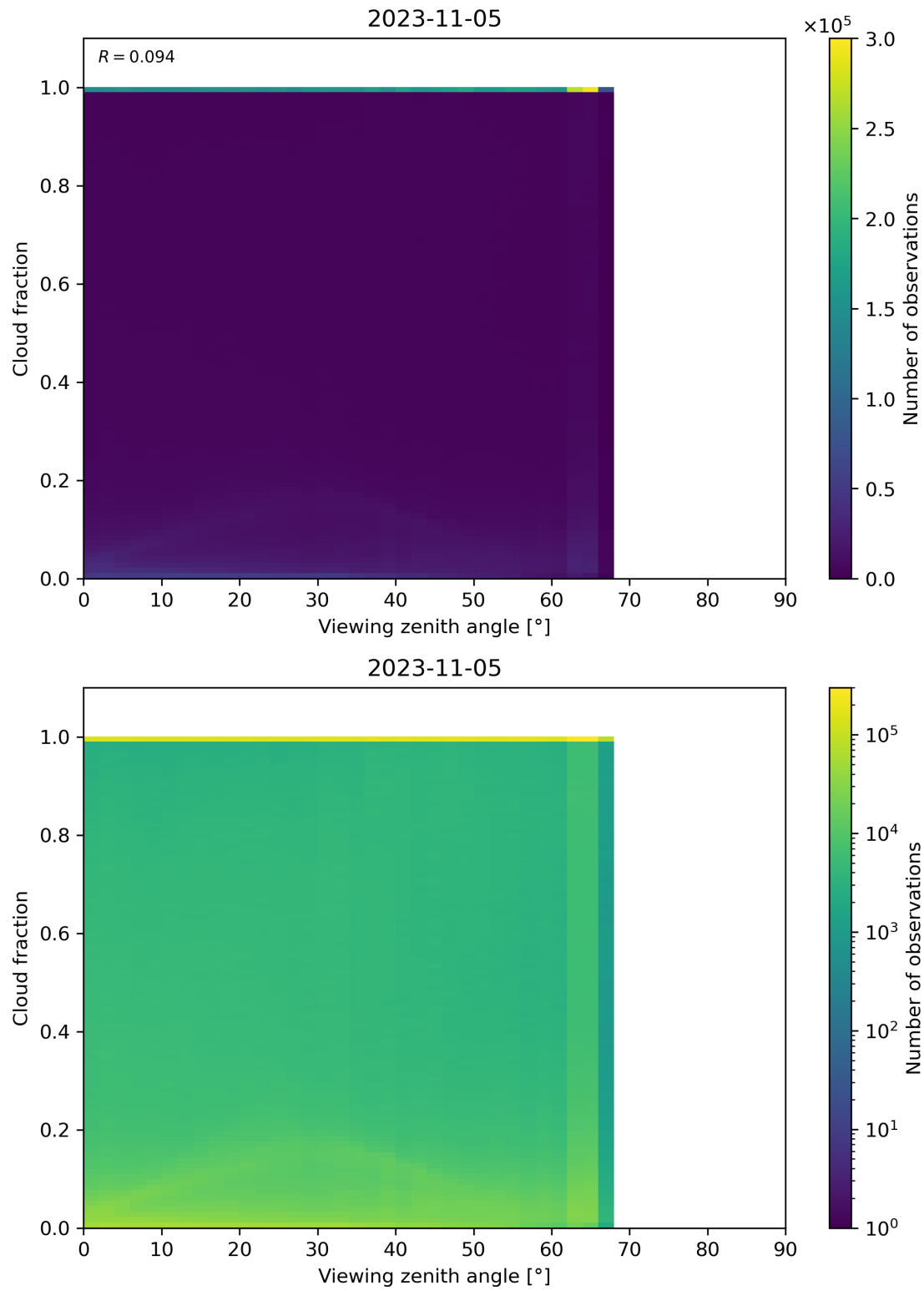
Figure 132: Scatter density plot of “Viewing zenith angle” against “Cloud fraction” for 2023-11-04 to 2023-11-06.
