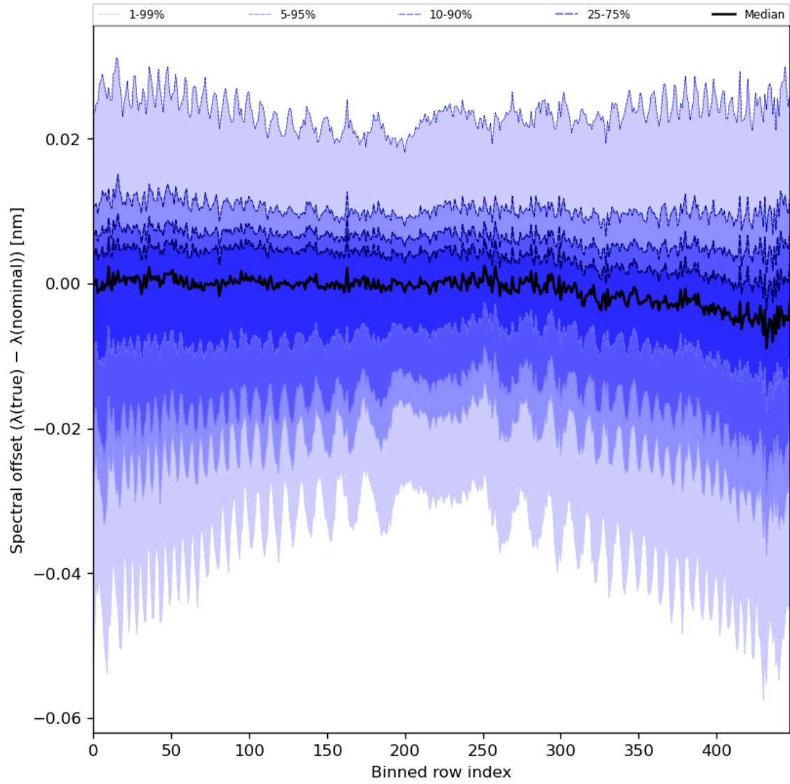
Figure 62: Along track statistics of “Spectral offset ( \lambda(\text{true}) - \lambda(\text{nominal}) )” for 2023-11-04 to 2023-11-06
