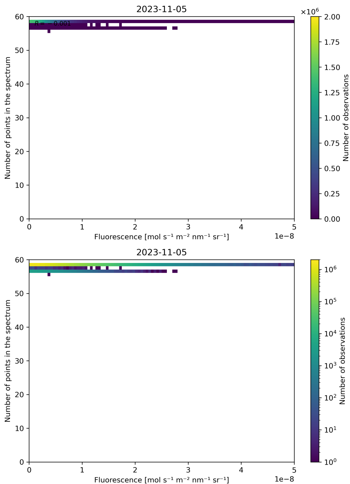
Figure 94: Scatter density plot of “Fluorescence” against “Number of points in the spectrum” for 2023-11-04 to 2023-11-06.
