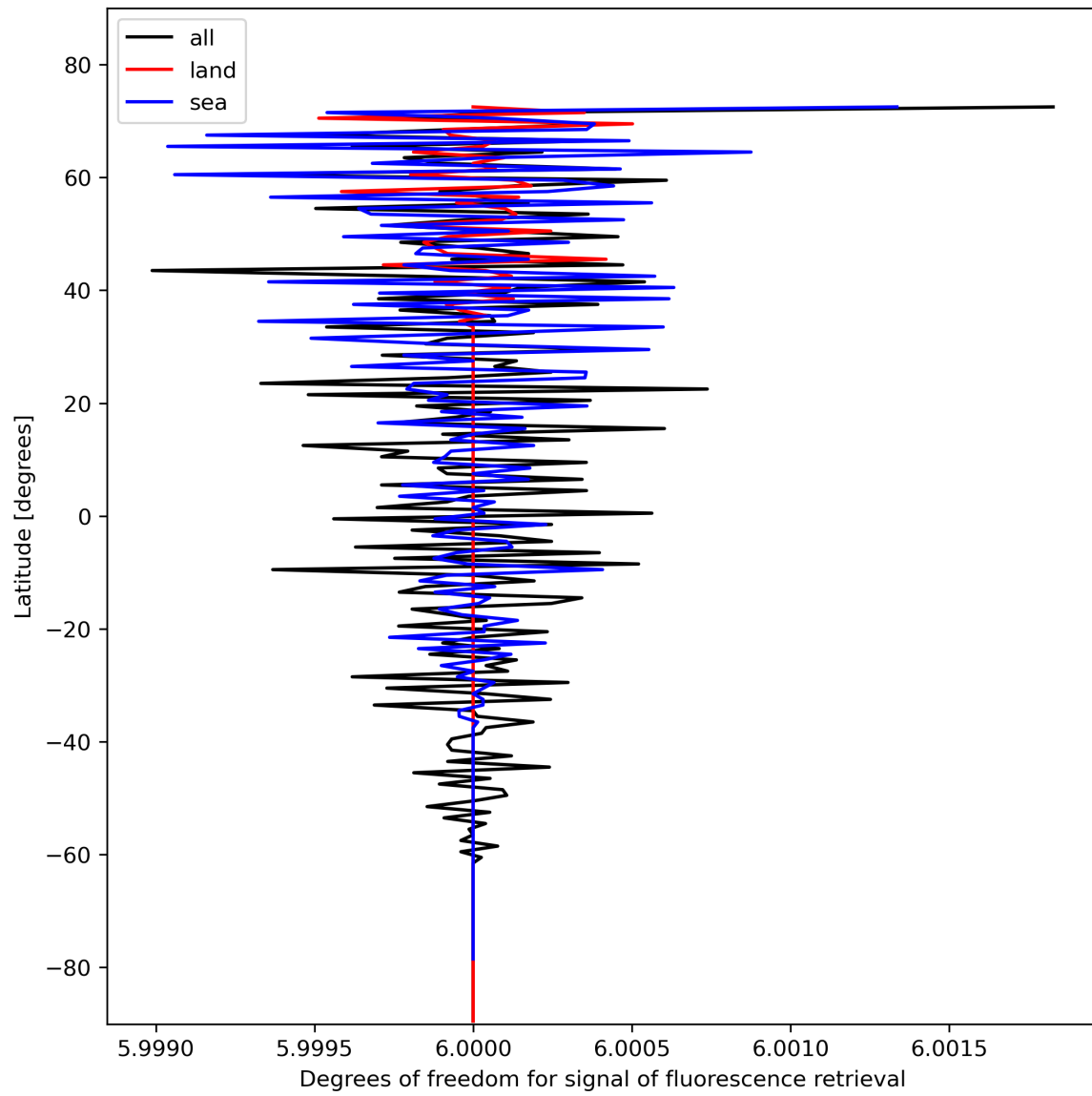
Figure 26: Zonal average of “Degrees of freedom for signal of fluorescence retrieval” for 2023-11-04 to 2023-11-06.
