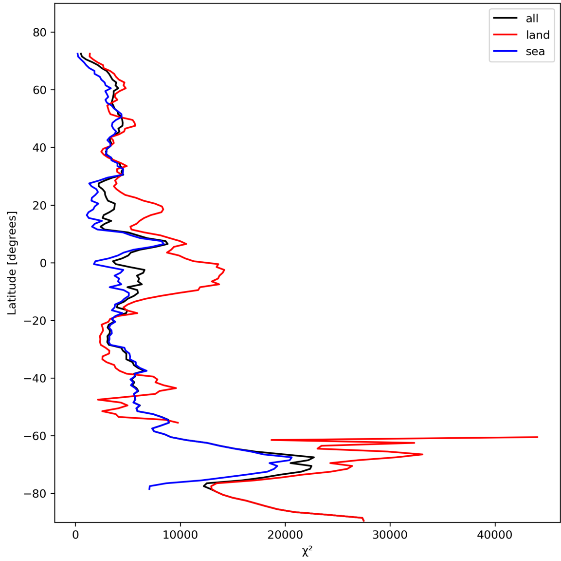
Figure 21: Zonal average of “ \chi^2 ” for 2023-11-04 to 2023-11-06.
