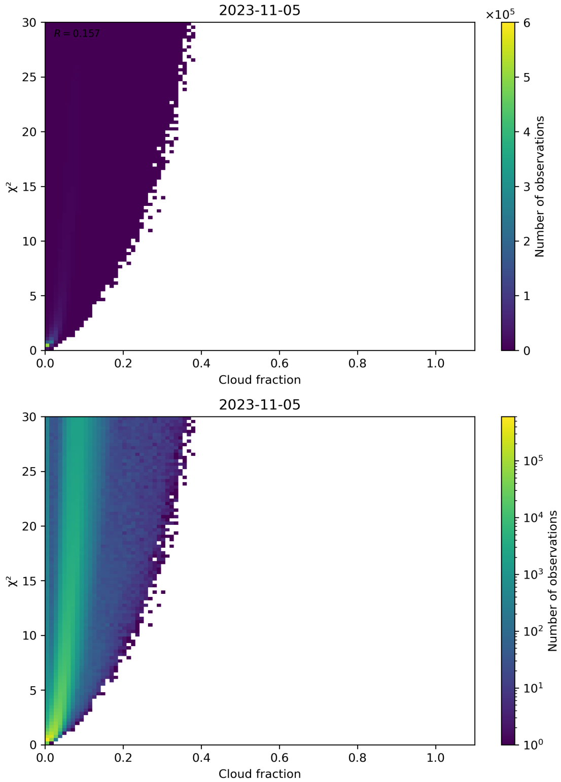
Figure 77: Scatter density plot of “Cloud fraction” against “ \chi^2 ” for 2023-11-04 to 2023-11-06.
