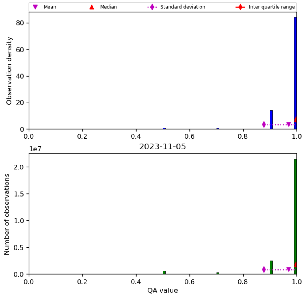
Figure 29: Histogram of “QA value” for 2023-11-04 to 2023-11-06
