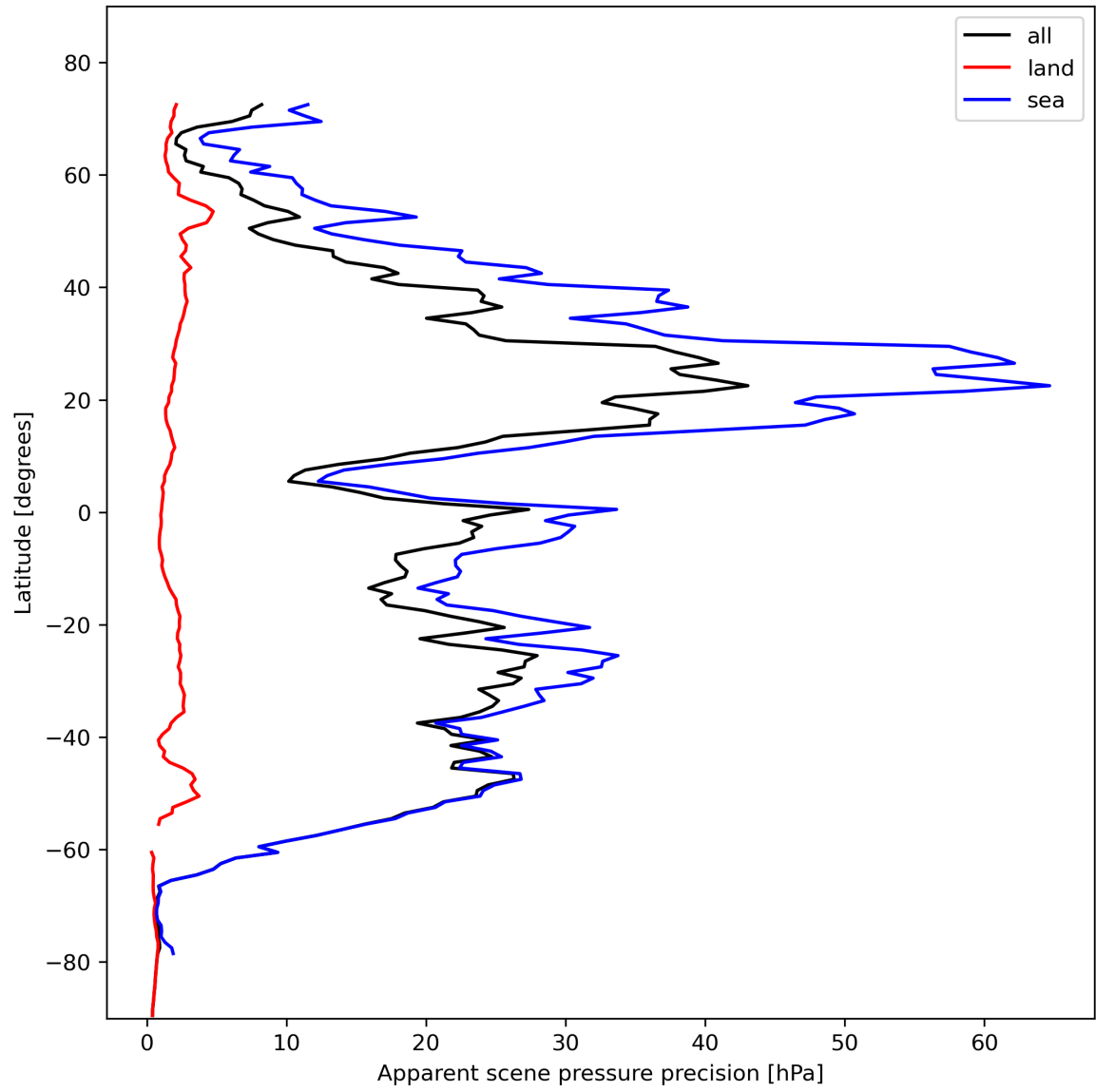
Figure 20: Zonal average of “Apparent scene pressure precision” for 2023-11-04 to 2023-11-06.
