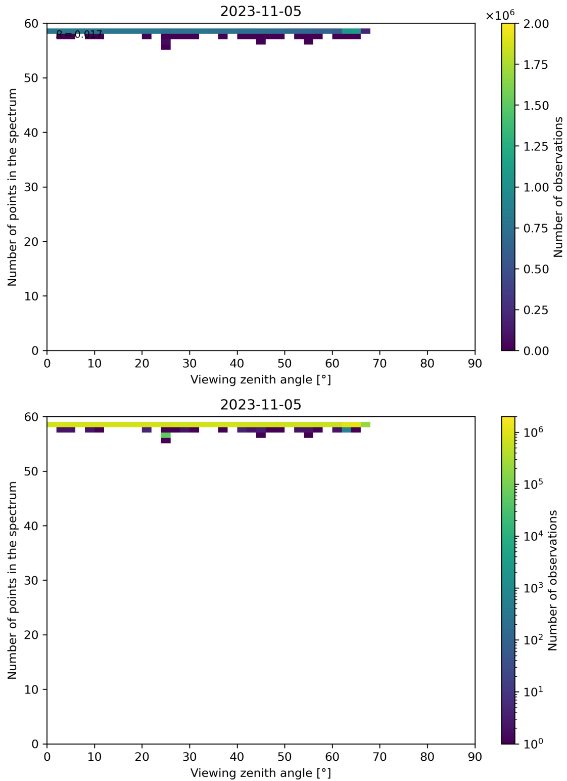
Figure 137: Scatter density plot of “Viewing zenith angle” against “Number of points in the spectrum” for 2023-11-04 to 2023-11-06.
