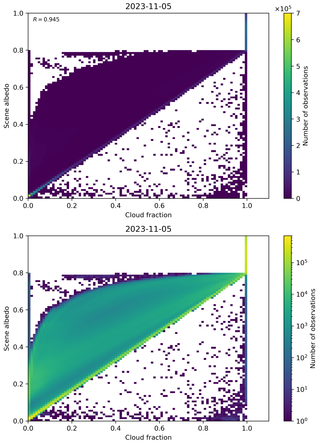
Figure 82: Scatter density plot of “Cloud fraction” against “Scene albedo” for 2023-11-04 to 2023-11-06.
