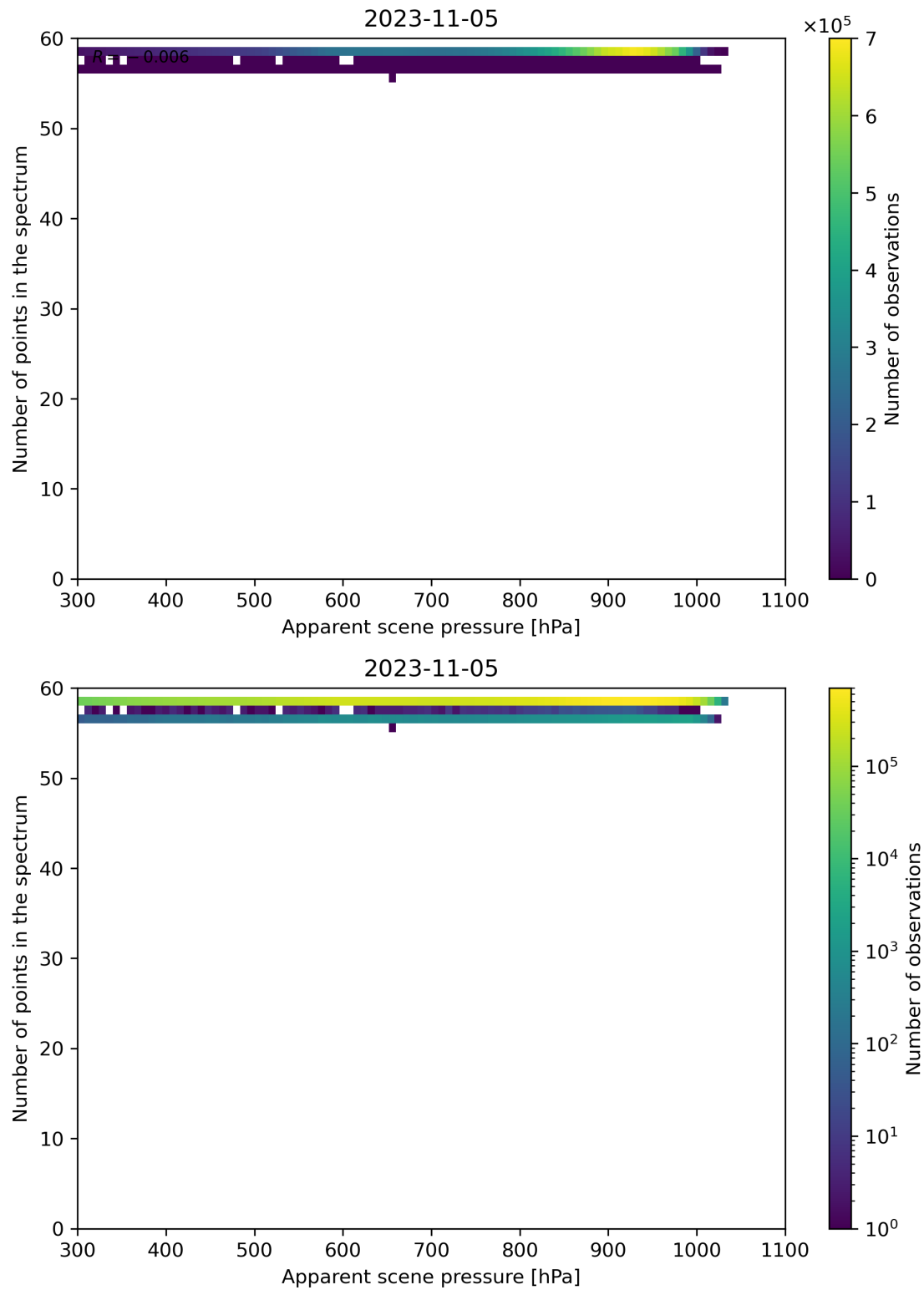
Figure 67: Scatter density plot of “Apparent scene pressure” against “Number of points in the spectrum” for 2023-11-04 to 2023-11-06.
