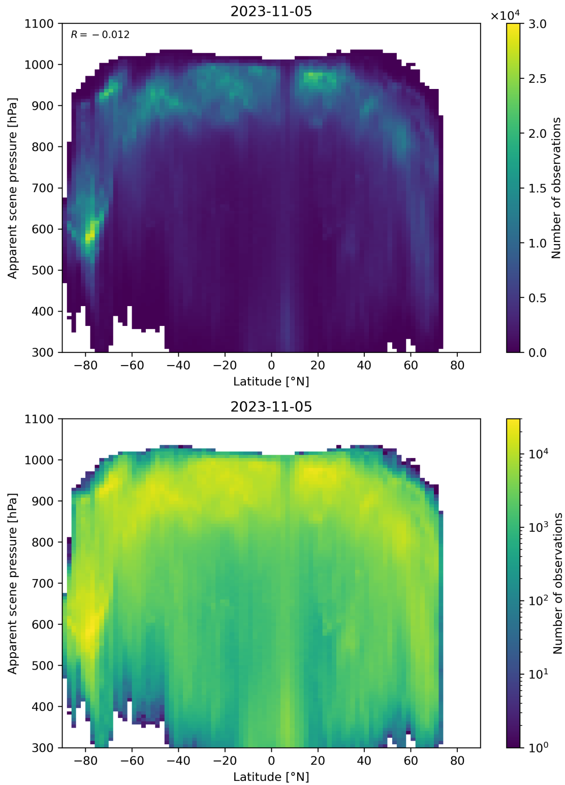
Figure 96: Scatter density plot of “Latitude” against “Apparent scene pressure” for 2023-11-04 to 2023-11-06.
