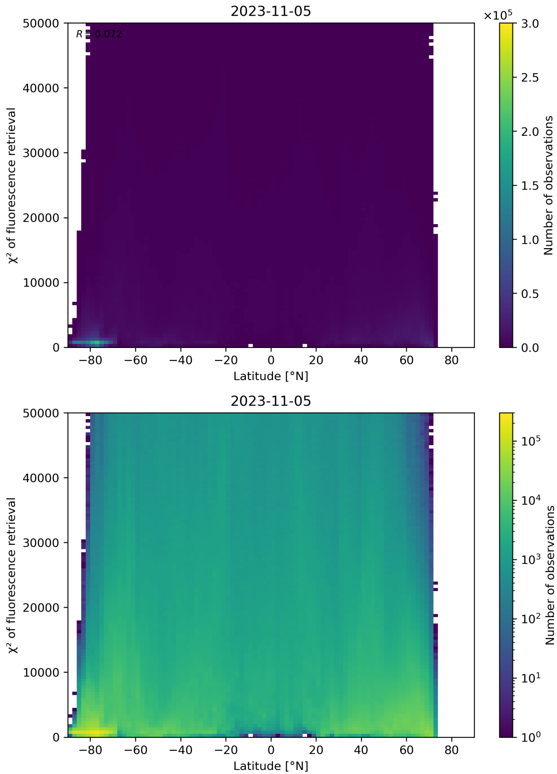
Figure 98: Scatter density plot of “Latitude” against “ \chi^2 of fluorescence retrieval” for 2023-11-04 to 2023-11-06.
