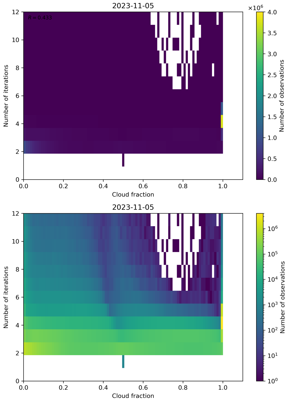
Figure 80: Scatter density plot of “Cloud fraction” against “Number of iterations” for 2023-11-04 to 2023-11-06.
