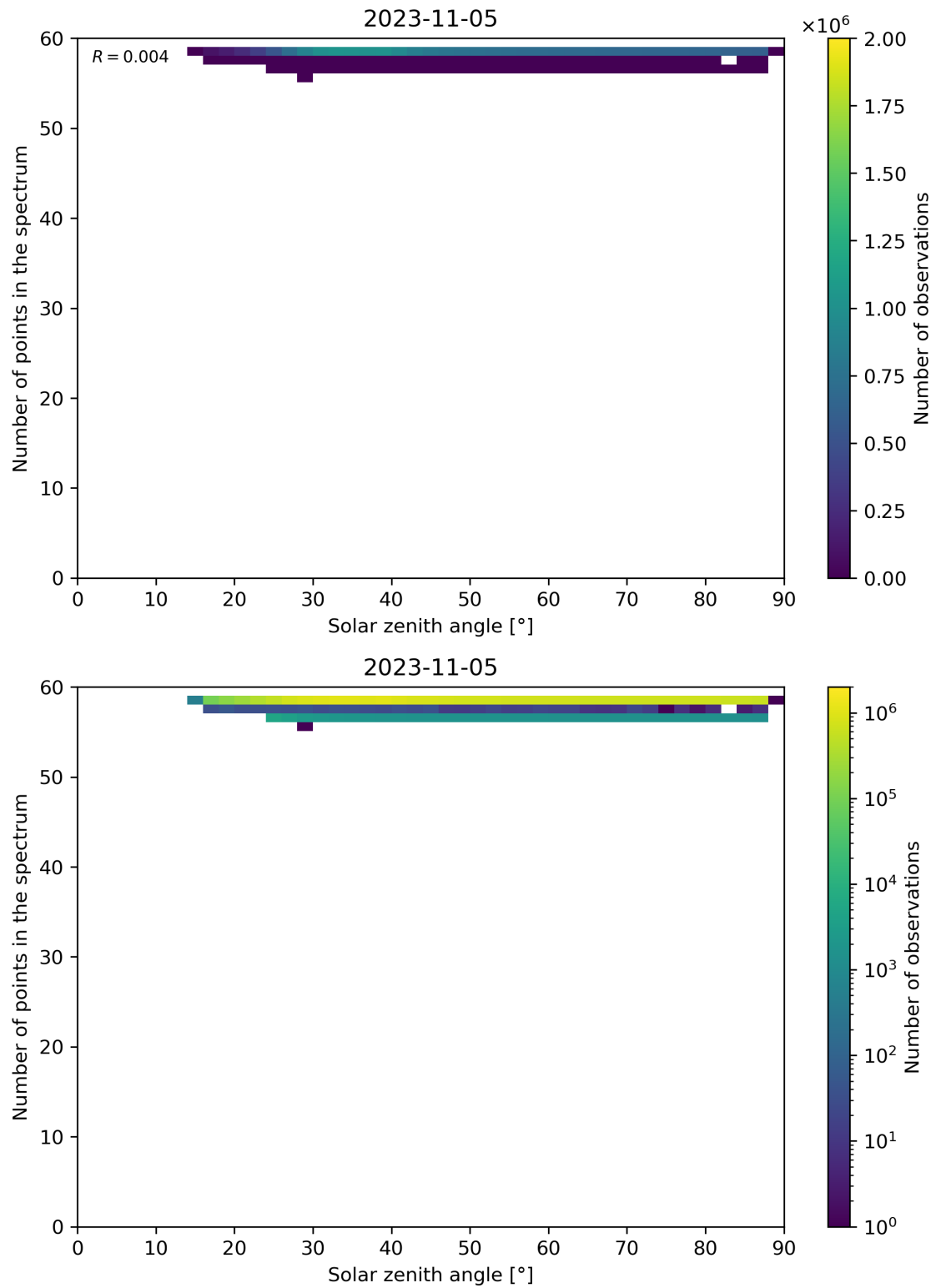
Figure 126: Scatter density plot of “Solar zenith angle” against “Number of points in the spectrum” for 2023-11-04 to 2023-11-06.
