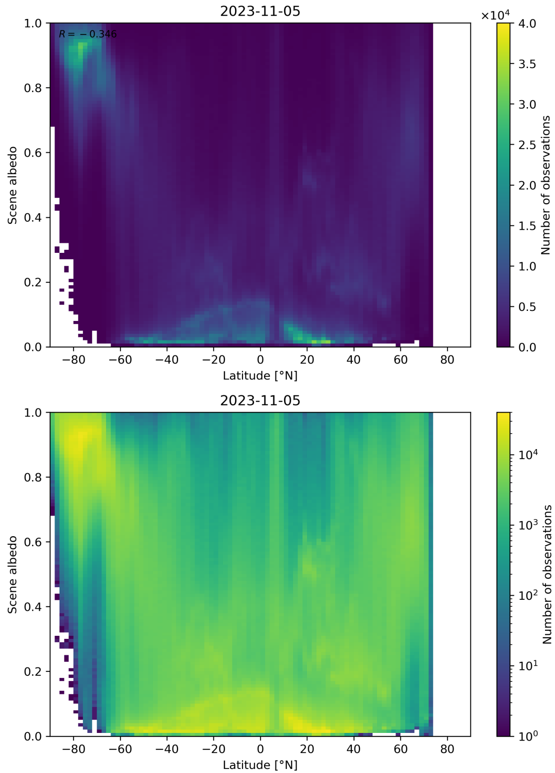
Figure 104: Scatter density plot of “Latitude” against “Scene albedo” for 2023-11-04 to 2023-11-06.
