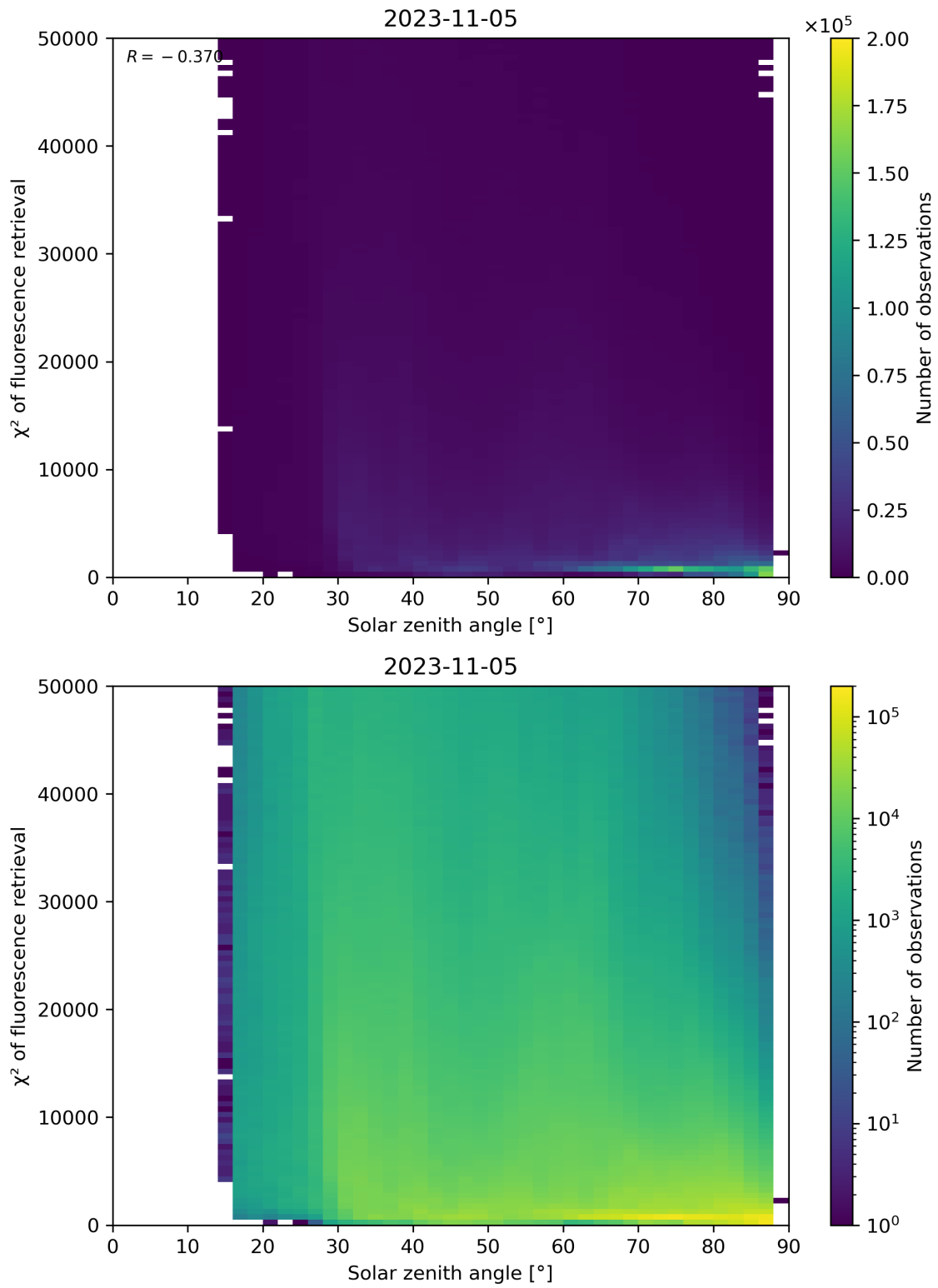
Figure 120: Scatter density plot of “Solar zenith angle” against “ \chi^2 of fluorescence retrieval” for 2023-11-04 to 2023-11-06.
