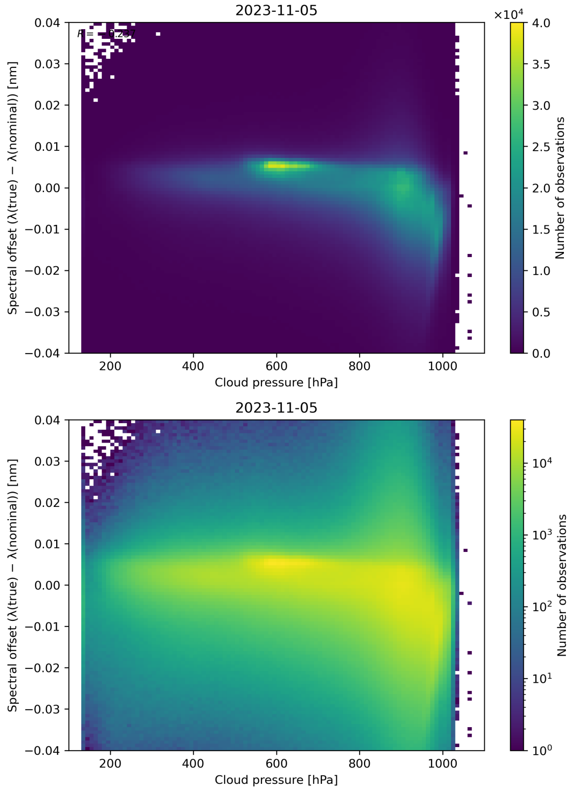
Figure 92: Scatter density plot of “Cloud pressure” against “Spectral offset ( \lambda(\text{true}) - \lambda(\text{nominal}) )” for 2023-11-04 to 2023-11-06.
