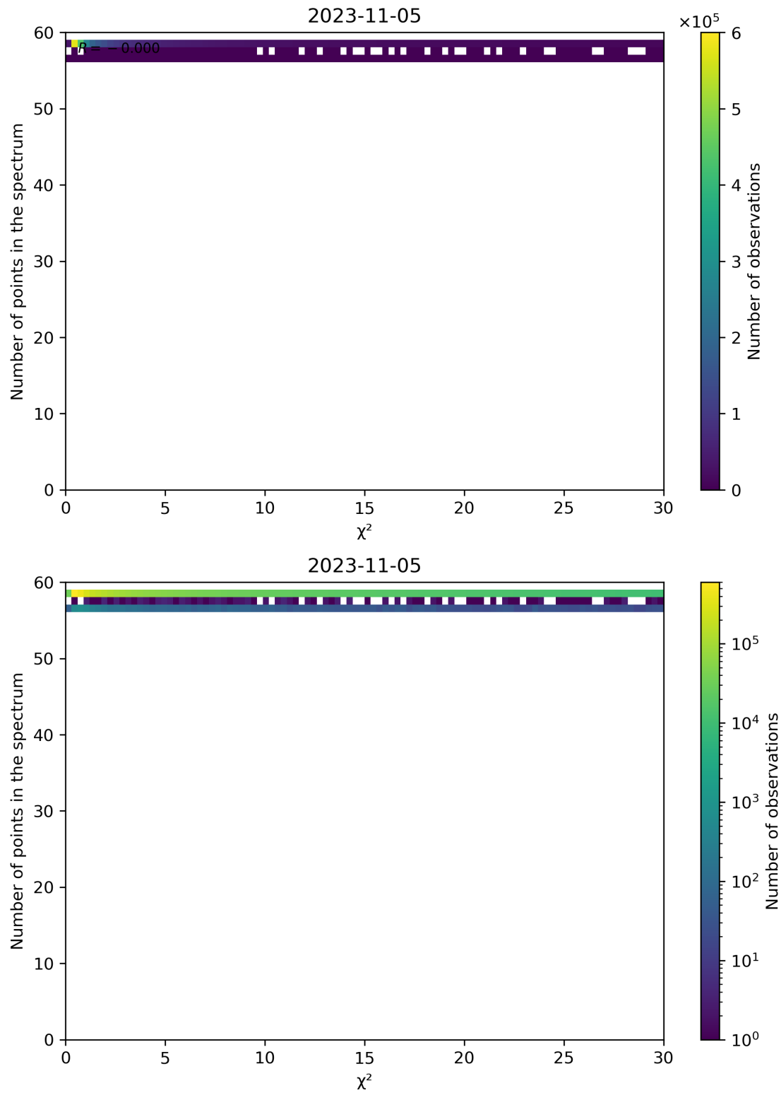
Figure 74: Scatter density plot of " \chi^2 " against "Number of points in the spectrum" for 2023-11-04 to 2023-11-06.
