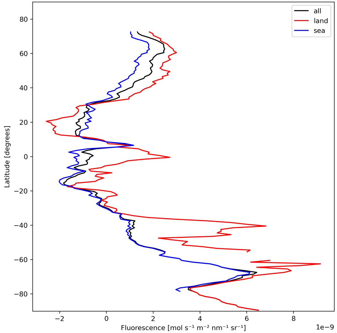
Figure 23: Zonal average of “Fluorescence” for 2023-11-04 to 2023-11-06.
