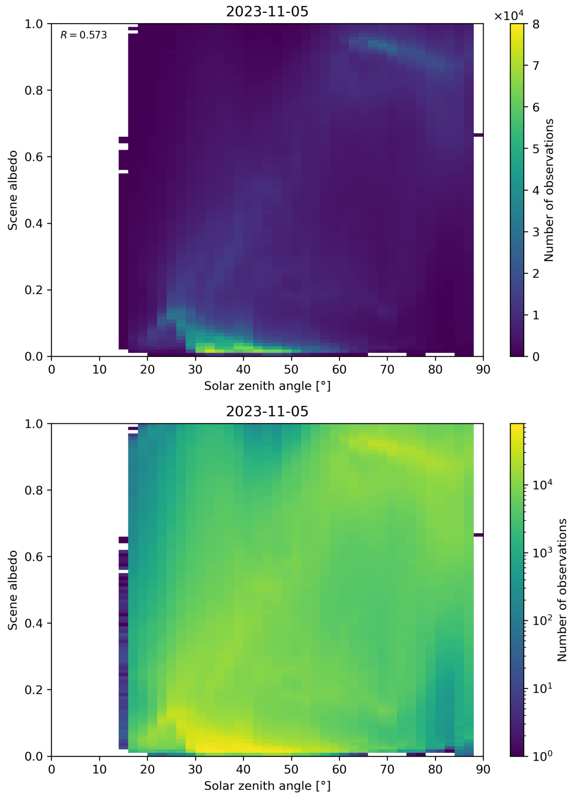
Figure 127: Scatter density plot of “Solar zenith angle” against “Scene albedo” for 2023-11-04 to 2023-11-06.
