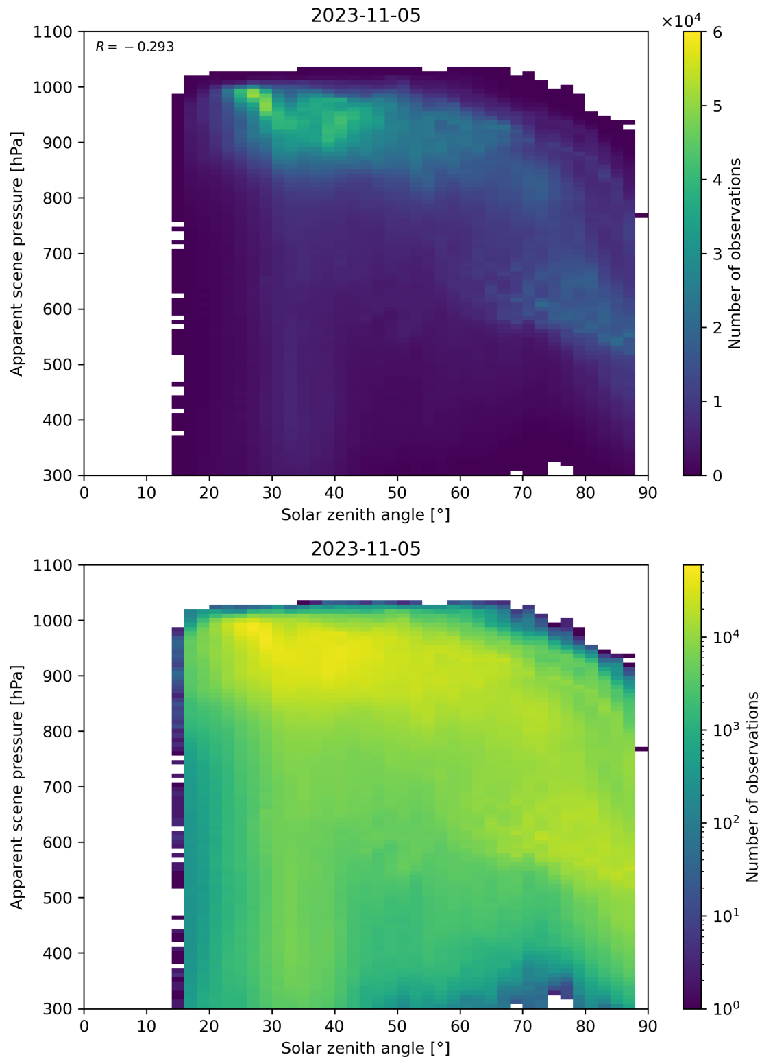
Figure 118: Scatter density plot of “Solar zenith angle” against “Apparent scene pressure” for 2023-11-04 to 2023-11-06.
