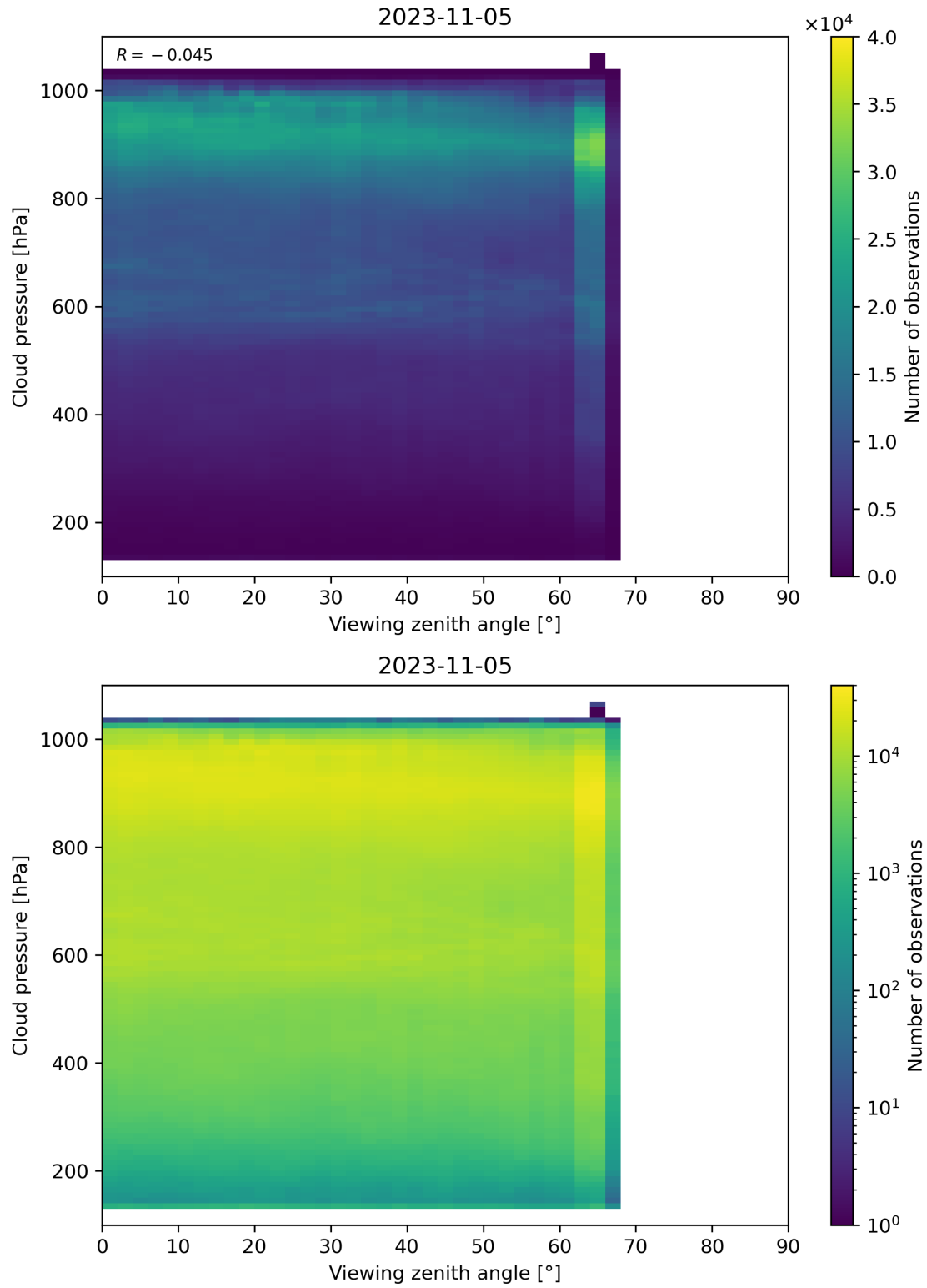
Figure 133: Scatter density plot of “Viewing zenith angle” against “Cloud pressure” for 2023-11-04 to 2023-11-06.
