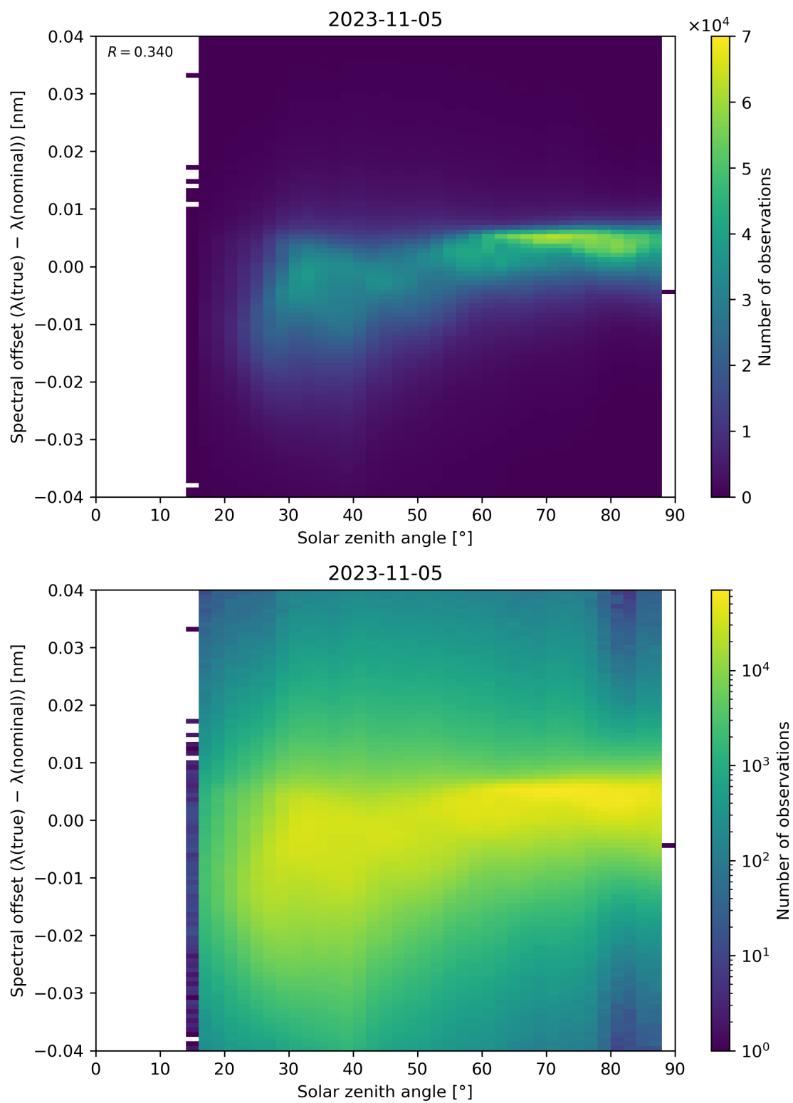
Figure 128: Scatter density plot of “Solar zenith angle” against “Spectral offset ( \lambda(\text{true}) - \lambda(\text{nominal}) )” for 2023-11-04 to 2023-11-06.
