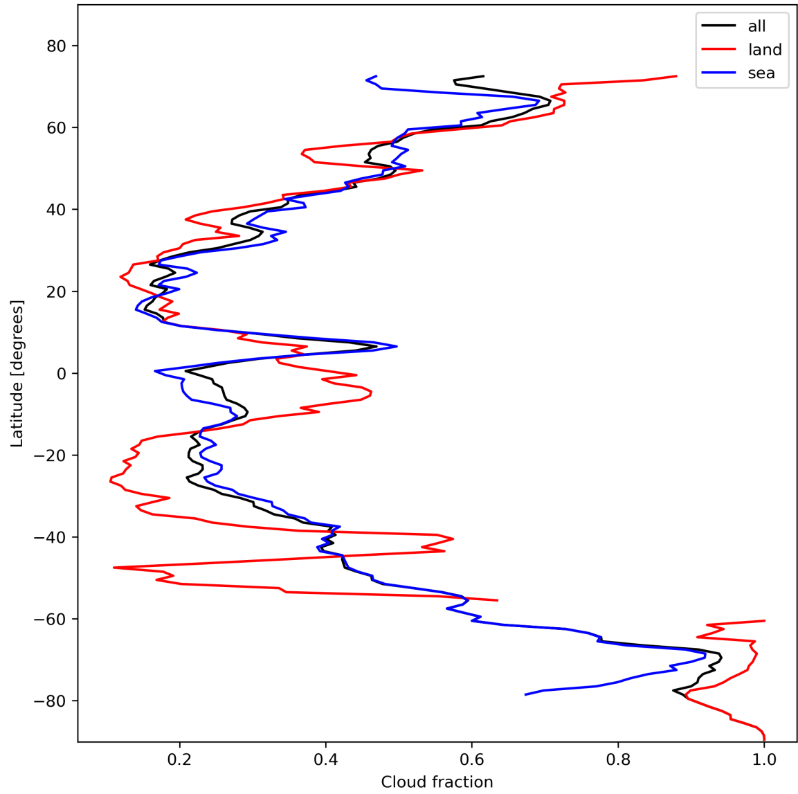
Figure 15: Zonal average of “Cloud fraction” for 2023-11-04 to 2023-11-06.
