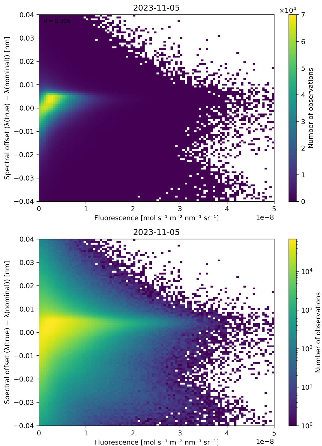
Figure 95: Scatter density plot of “Fluorescence” against “Spectral offset ( \lambda(\text{true}) - \lambda(\text{nominal}) )” for 2023-11-04 to 2023-11-06.
