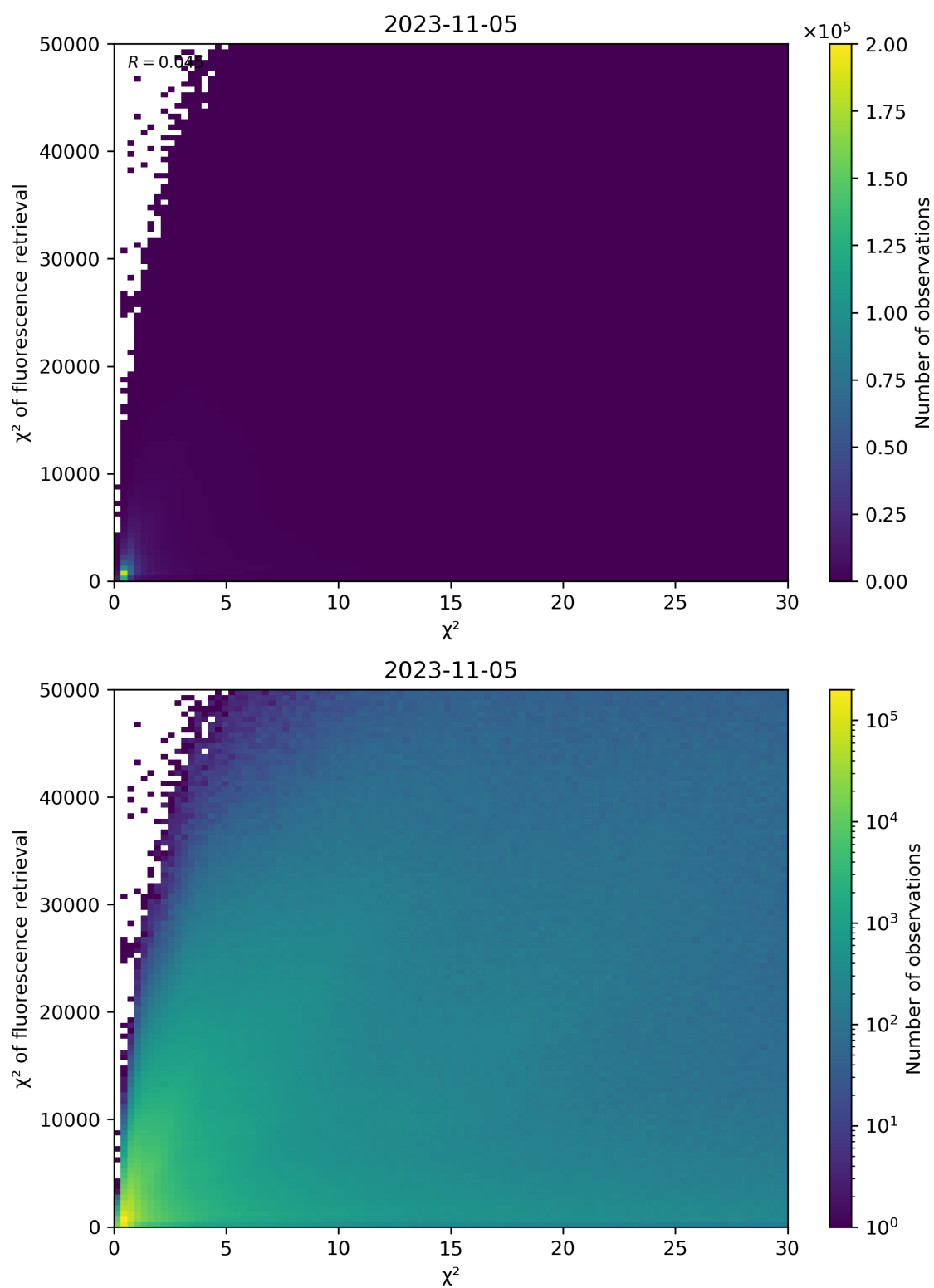
Figure 69: Scatter density plot of “ \chi^2 ” against “ \chi^2 of fluorescence retrieval” for 2023-11-04 to 2023-11-06.
