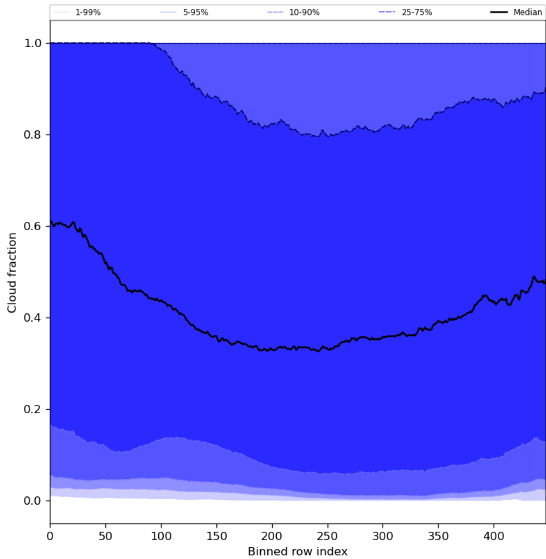
Figure 49: Along track statistics of “Cloud fraction” for 2023-11-04 to 2023-11-06
