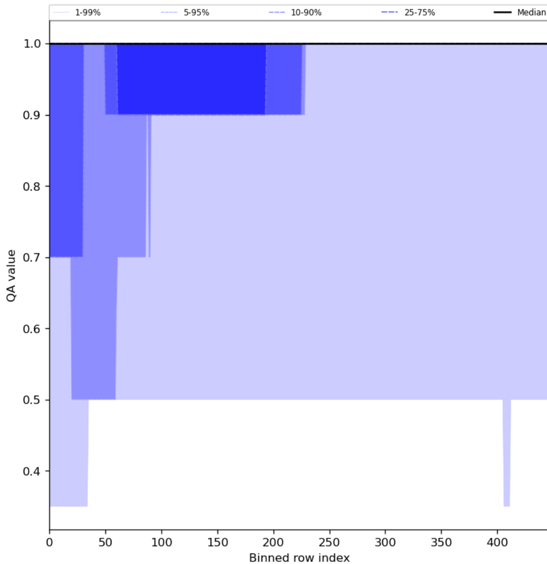
Figure 46: Along track statistics of “QA value” for 2023-11-04 to 2023-11-06
