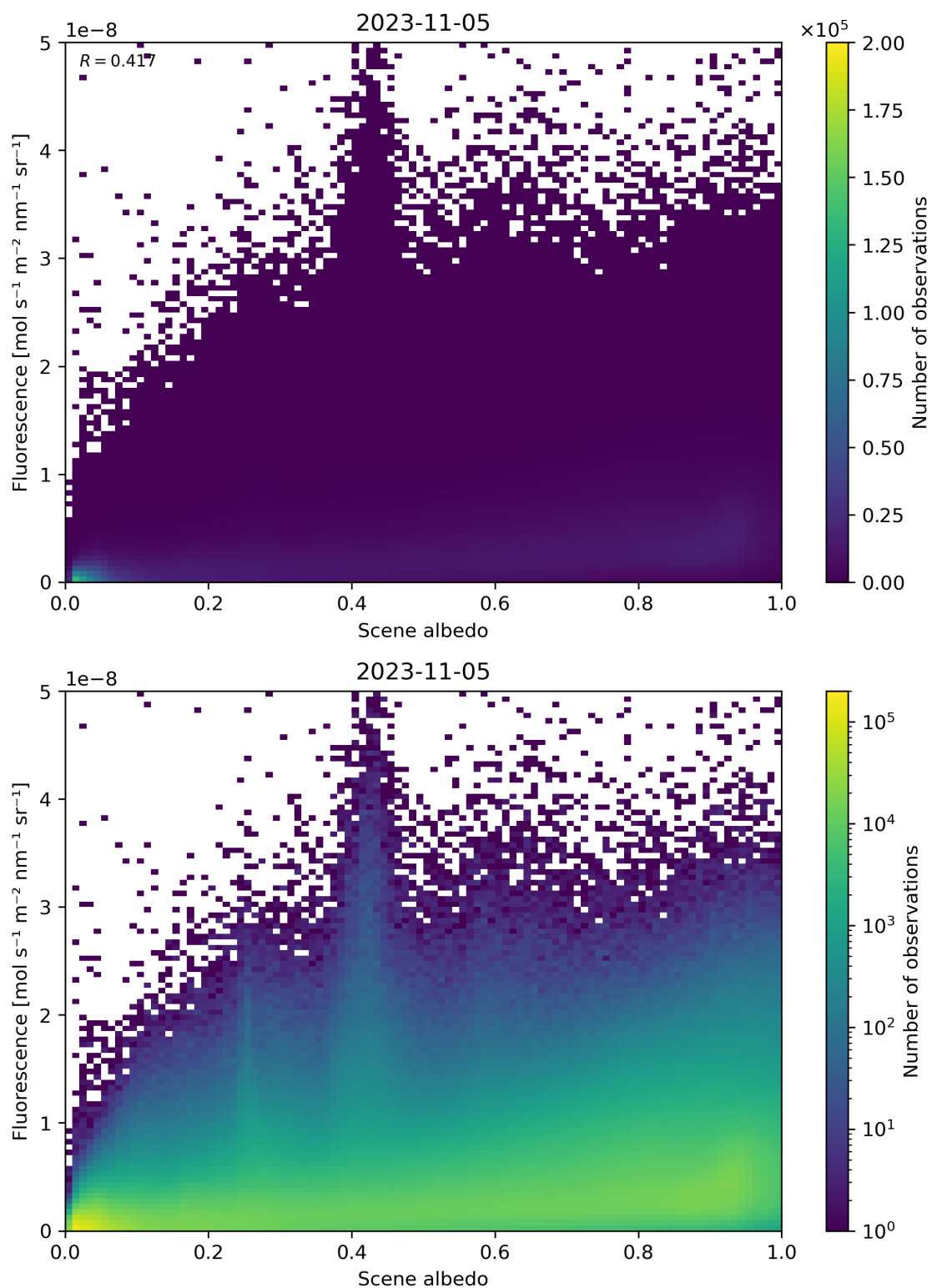
Figure 114: Scatter density plot of “Scene albedo” against “Fluorescence” for 2023-11-04 to 2023-11-06.
