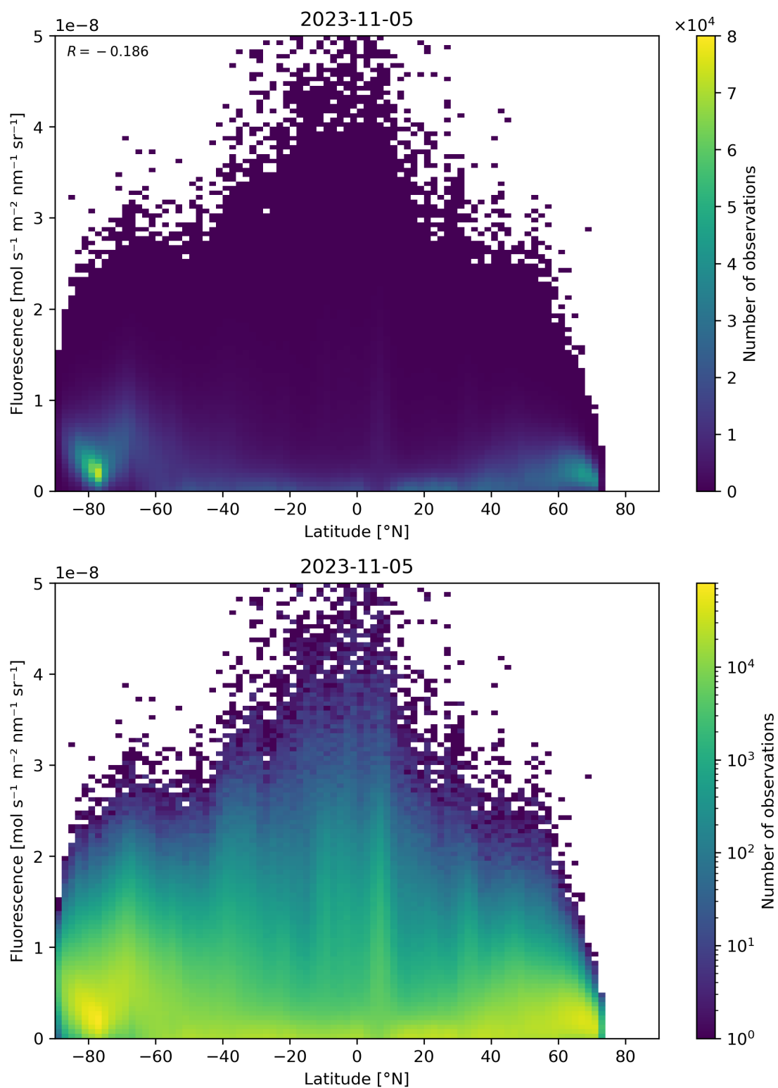
Figure 101: Scatter density plot of “Latitude” against “Fluorescence” for 2023-11-04 to 2023-11-06.
