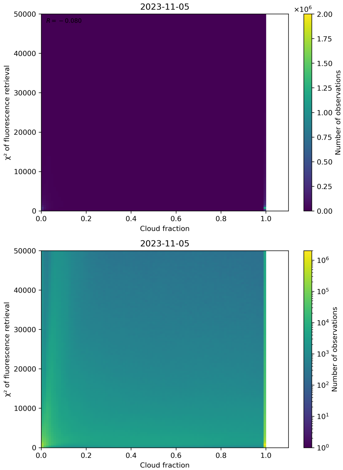
Figure 78: Scatter density plot of “Cloud fraction” against “ \chi^2 of fluorescence retrieval” for 2023-11-04 to 2023-11-06.
