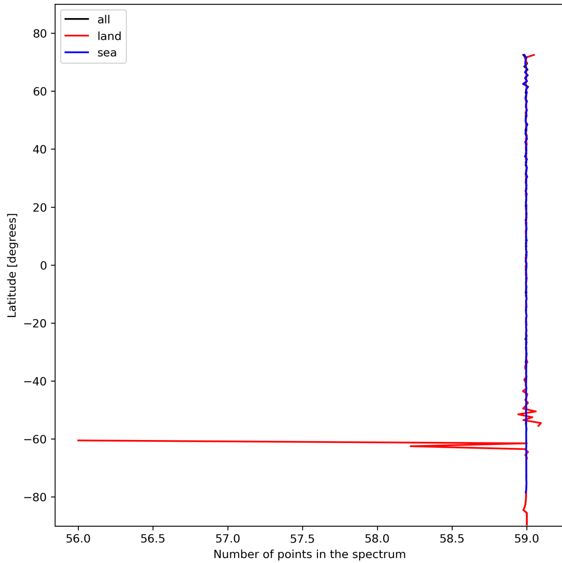
Figure 27: Zonal average of “Number of points in the spectrum” for 2023-11-04 to 2023-11-06.
