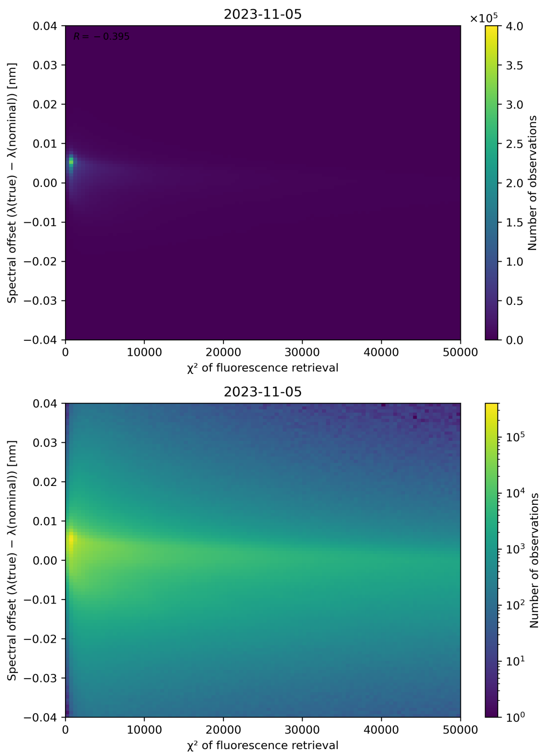
Figure 72: Scatter density plot of " \chi^2 of fluorescence retrieval" against "Spectral offset ( \lambda(\text{true}) - \lambda(\text{nominal}) )" for 2023-11-04 to 2023-11-06.
