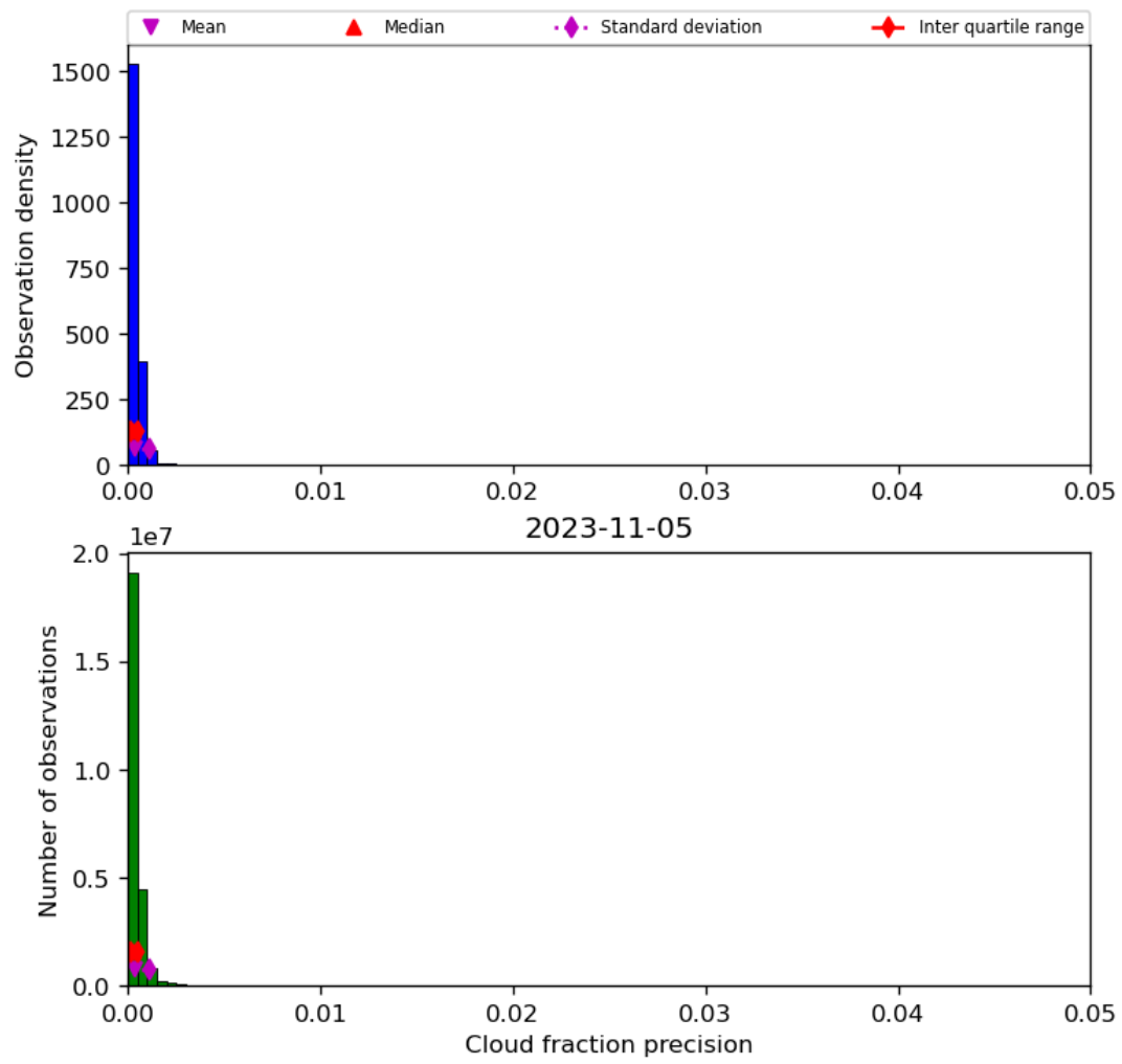
Figure 33: Histogram of “Cloud fraction precision” for 2023-11-04 to 2023-11-06
