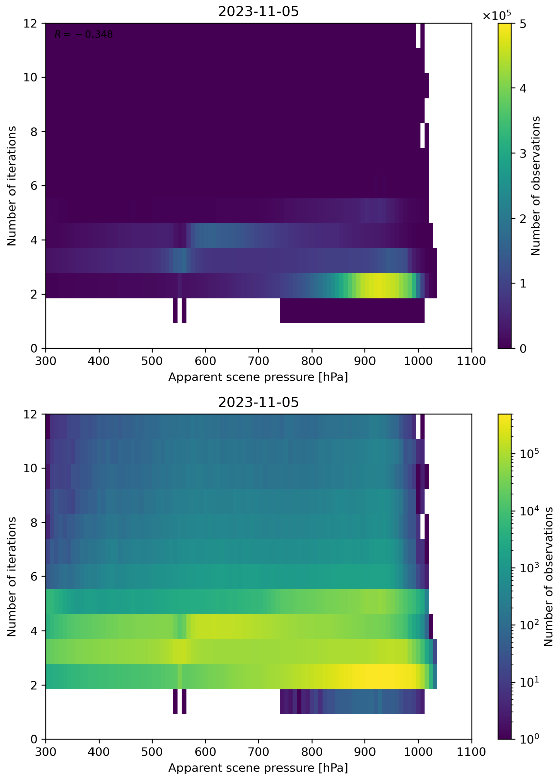
Figure 66: Scatter density plot of “Apparent scene pressure” against “Number of iterations” for 2023-11-04 to 2023-11-06.
