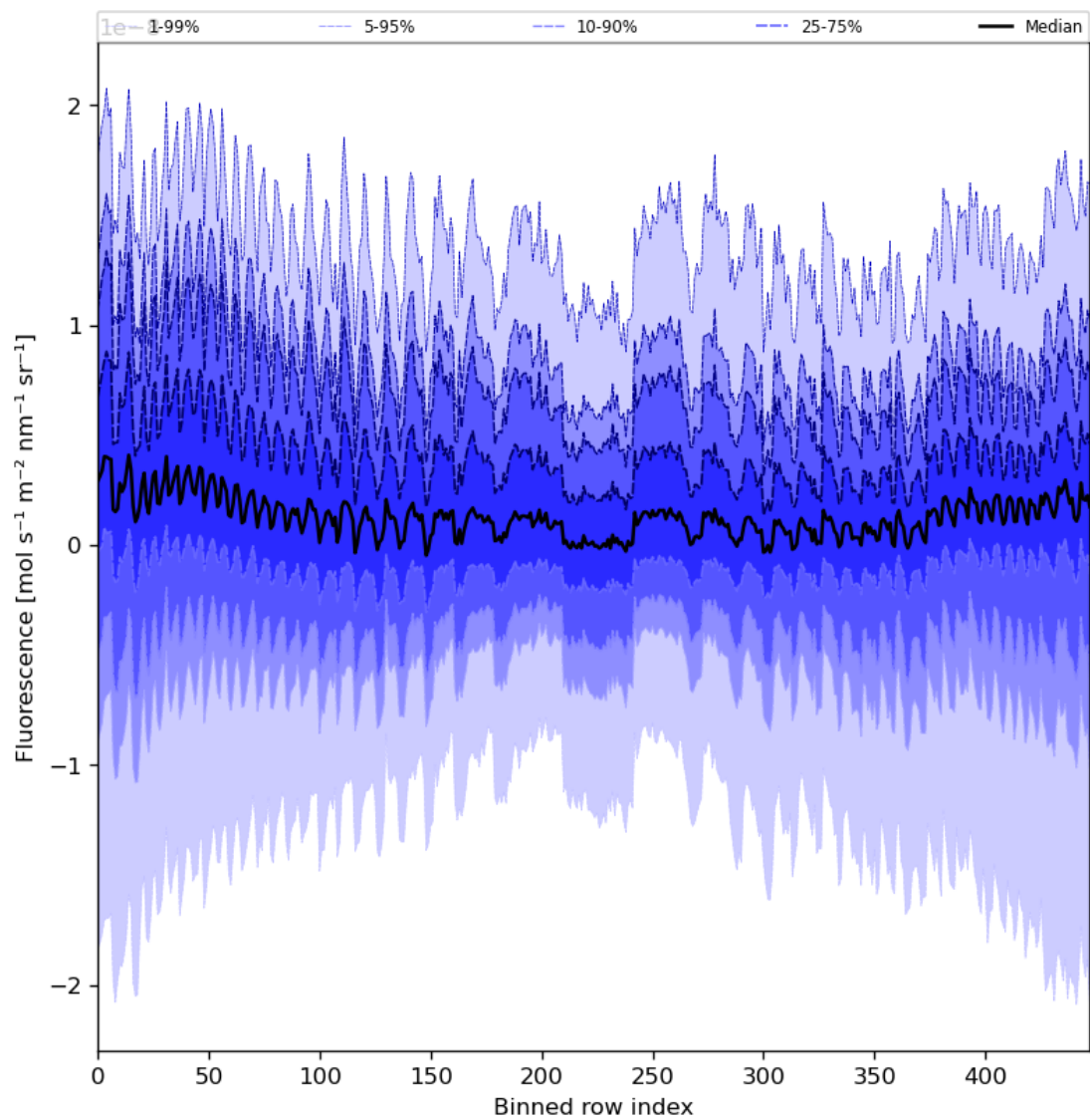
Figure 57: Along track statistics of “Fluorescence” for 2023-11-04 to 2023-11-06
