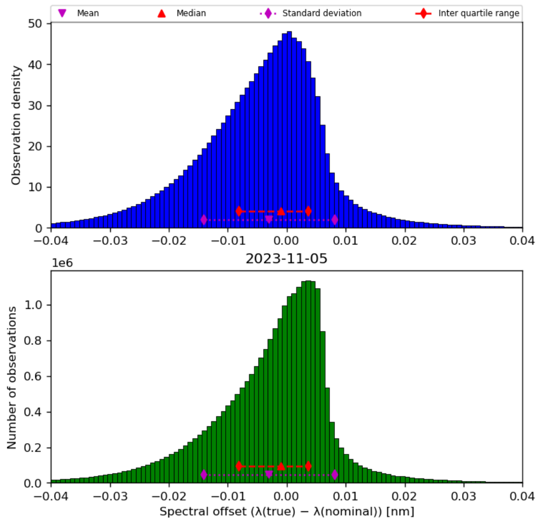
Figure 45: Histogram of “Spectral offset ( \lambda(\text{true}) - \lambda(\text{nominal}) )” for 2023-11-04 to 2023-11-06
