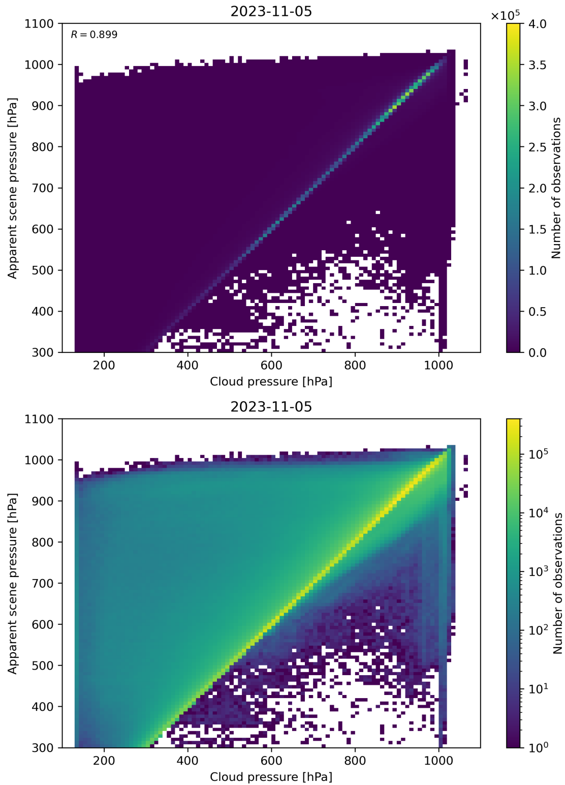
Figure 84: Scatter density plot of “Cloud pressure” against “Apparent scene pressure” for 2023-11-04 to 2023-11-06.
