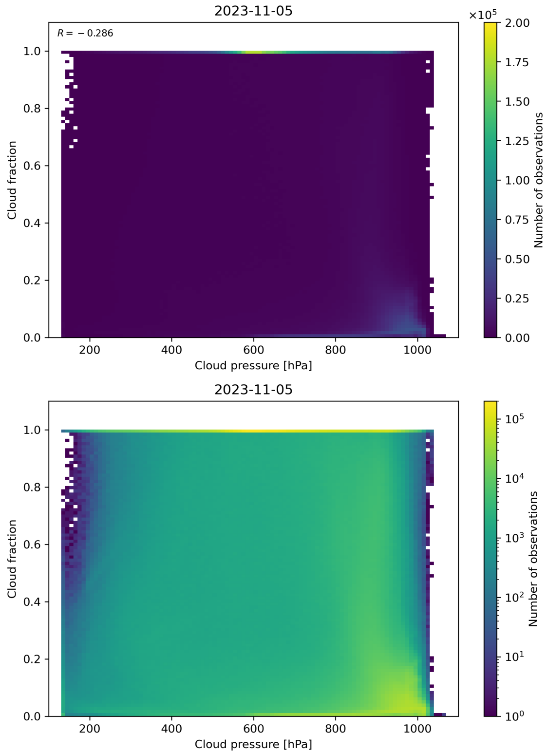
Figure 87: Scatter density plot of “Cloud pressure” against “Cloud fraction” for 2023-11-04 to 2023-11-06.
