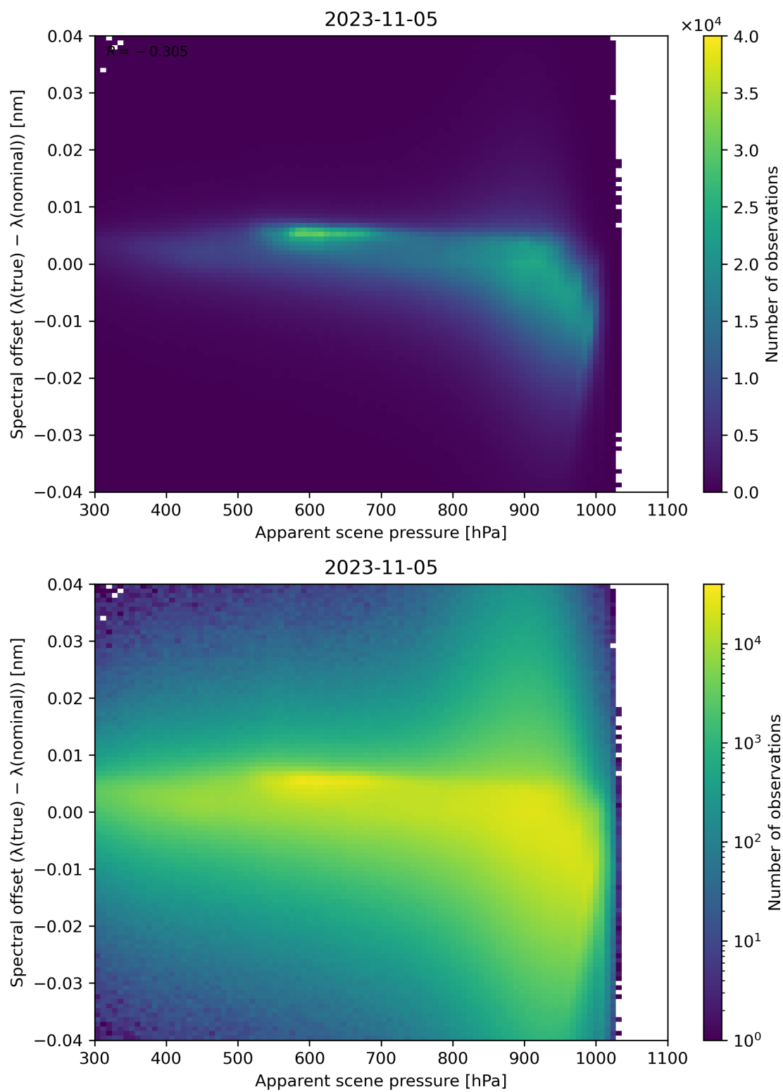
Figure 68: Scatter density plot of “Apparent scene pressure” against “Spectral offset ( \lambda(\text{true}) - \lambda(\text{nominal}) )” for 2023-11-04 to 2023-11-06.
