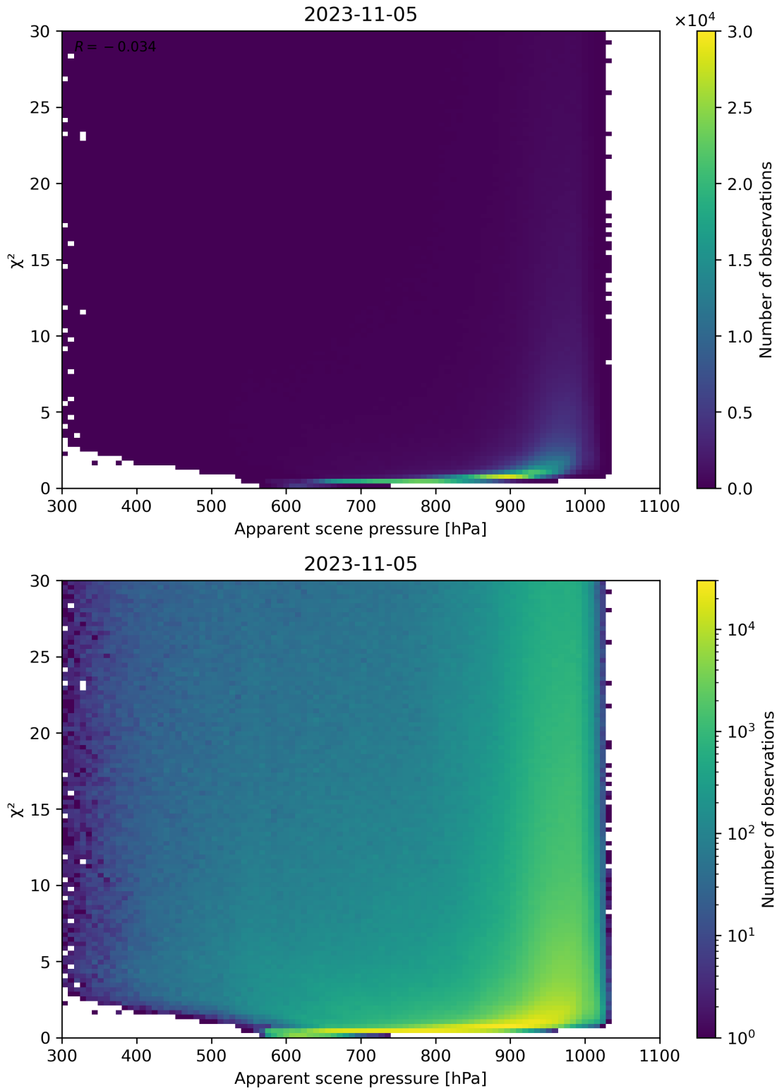
Figure 63: Scatter density plot of “Apparent scene pressure” against “ \chi^2 ” for 2023-11-04 to 2023-11-06.
