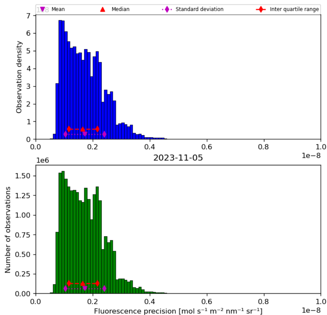
Figure 41: Histogram of “Fluorescence precision” for 2023-11-04 to 2023-11-06
