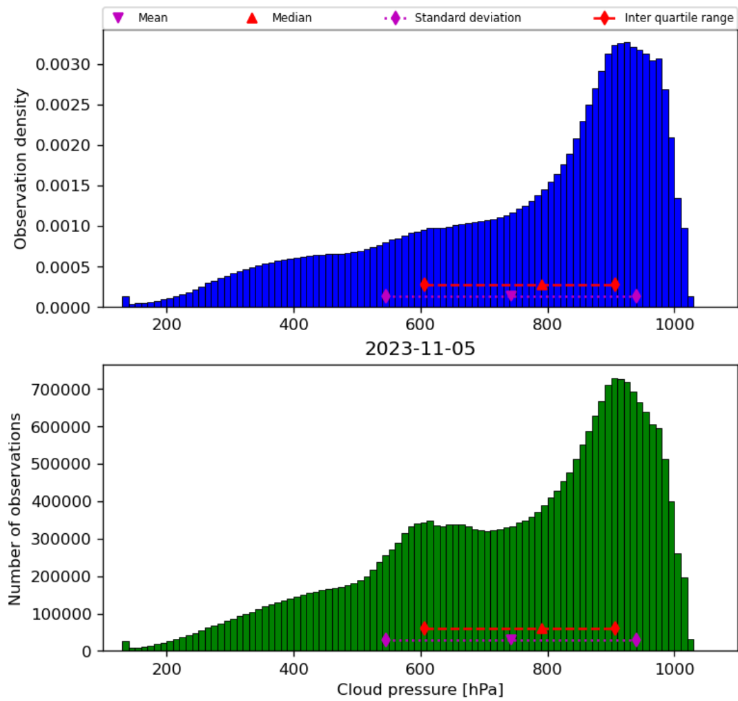
Figure 30: Histogram of “Cloud pressure” for 2023-11-04 to 2023-11-06
