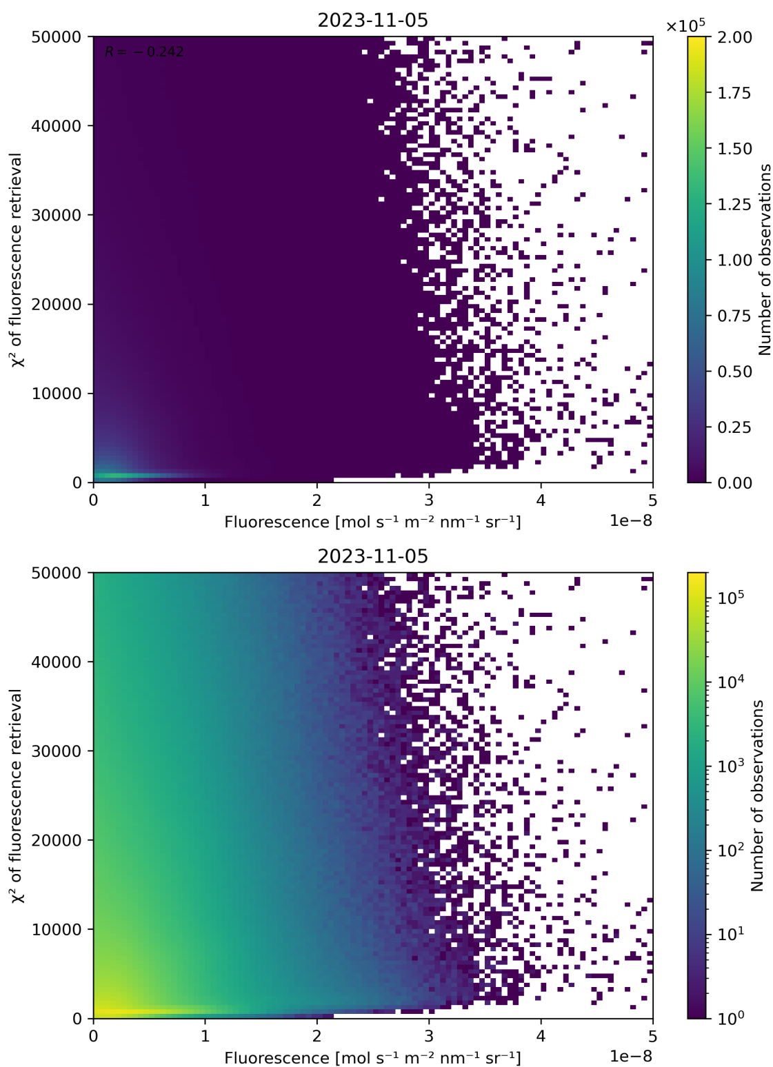
Figure 93: Scatter density plot of “Fluorescence” against “ \chi^2 of fluorescence retrieval” for 2023-11-04 to 2023-11-06.
