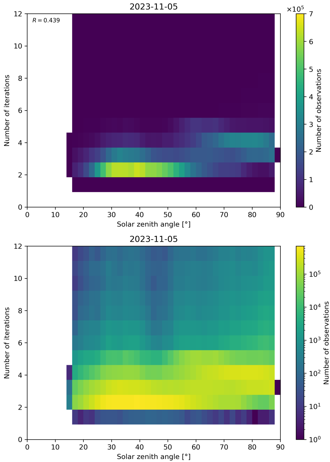
Figure 125: Scatter density plot of “Solar zenith angle” against “Number of iterations” for 2023-11-04 to 2023-11-06.
