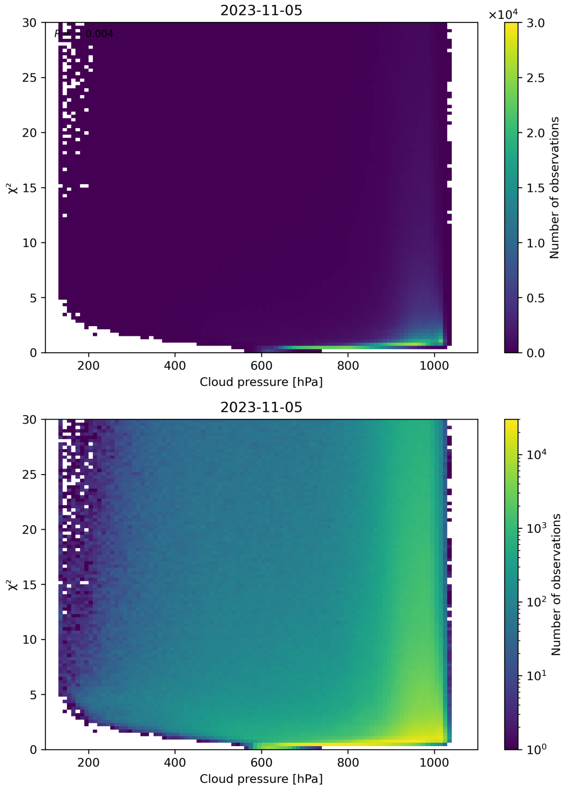
Figure 85: Scatter density plot of “Cloud pressure” against “ \chi^2 ” for 2023-11-04 to 2023-11-06.
