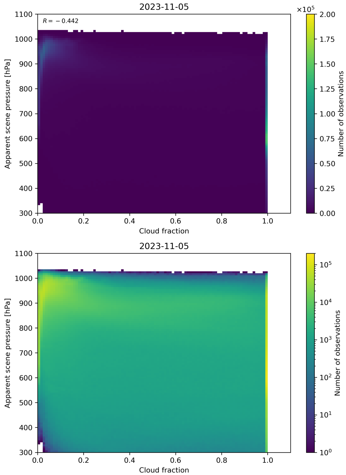
Figure 76: Scatter density plot of “Cloud fraction” against “Apparent scene pressure” for 2023-11-04 to 2023-11-06.
