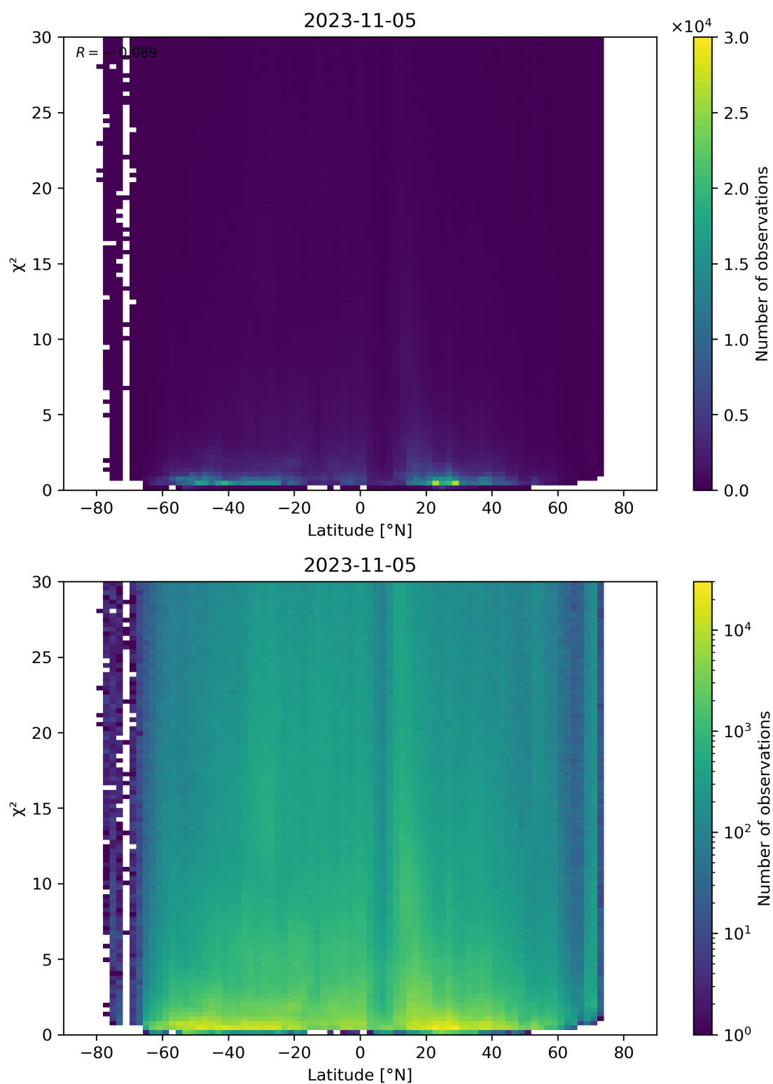
Figure 97: Scatter density plot of “Latitude” against “ \chi^2 ” for 2023-11-04 to 2023-11-06.
