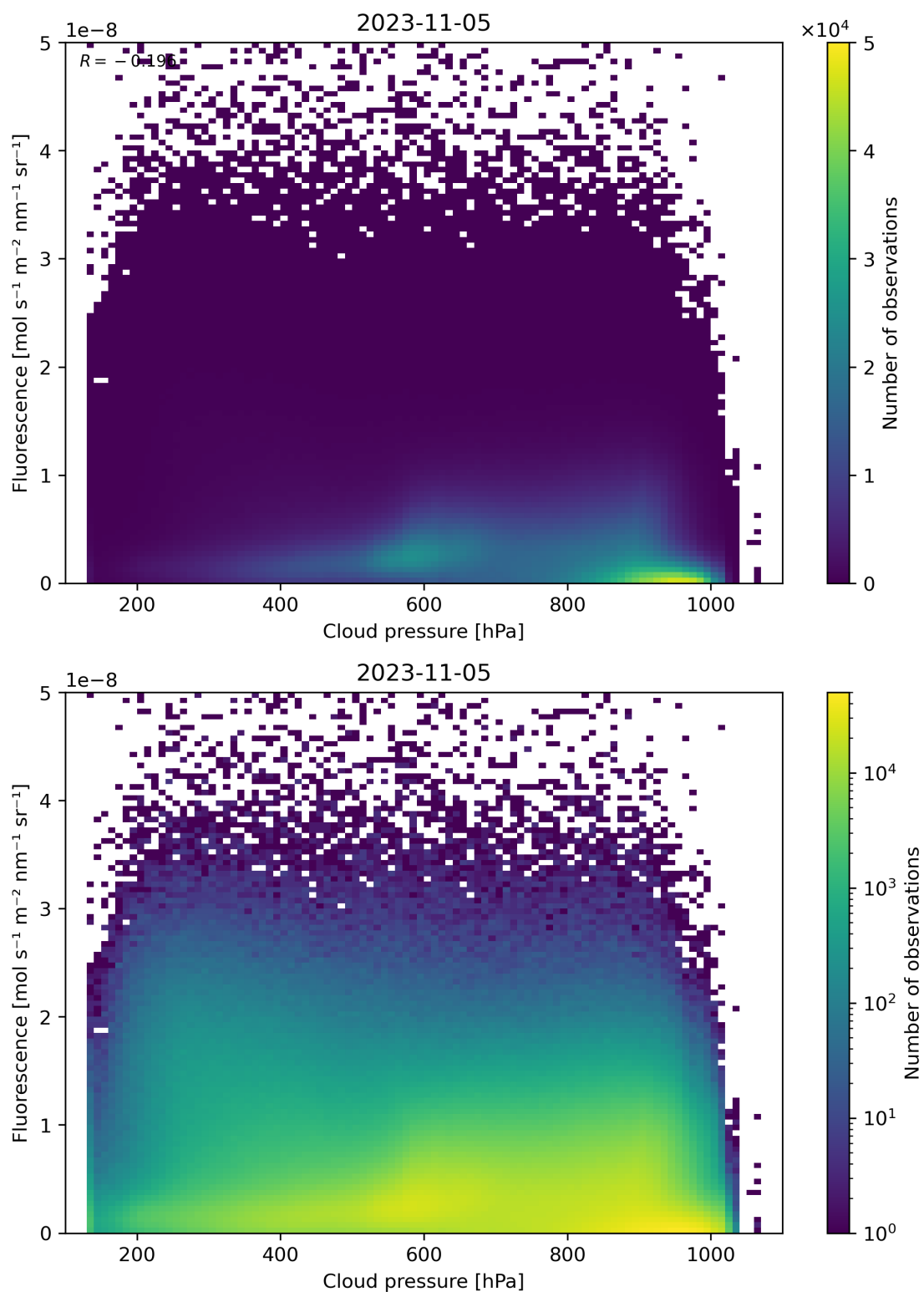
Figure 88: Scatter density plot of “Cloud pressure” against “Fluorescence” for 2023-11-04 to 2023-11-06.
