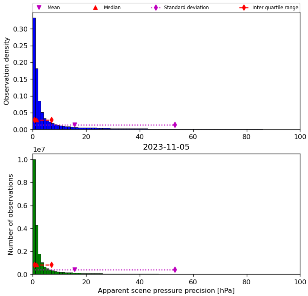
Figure 37: Histogram of “Apparent scene pressure precision” for 2023-11-04 to 2023-11-06
