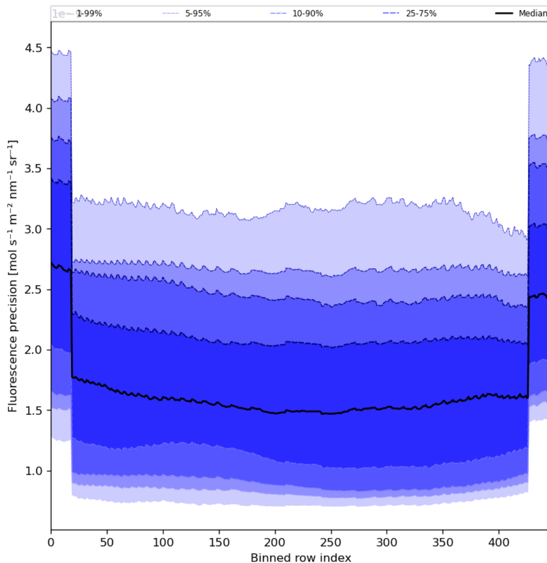
Figure 58: Along track statistics of “Fluorescence precision” for 2023-11-04 to 2023-11-06
