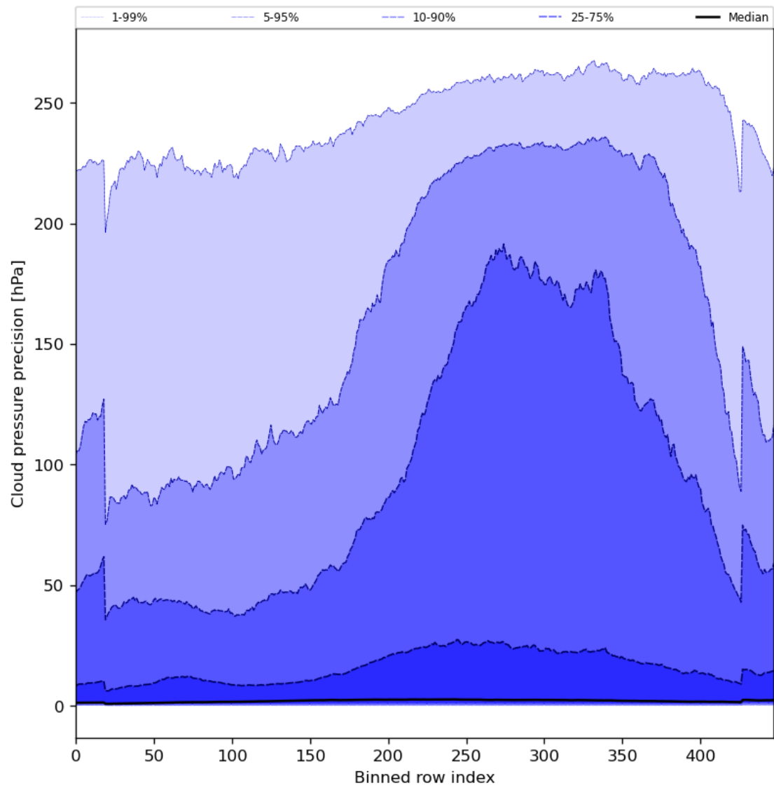
Figure 48: Along track statistics of “Cloud pressure precision” for 2023-11-04 to 2023-11-06
