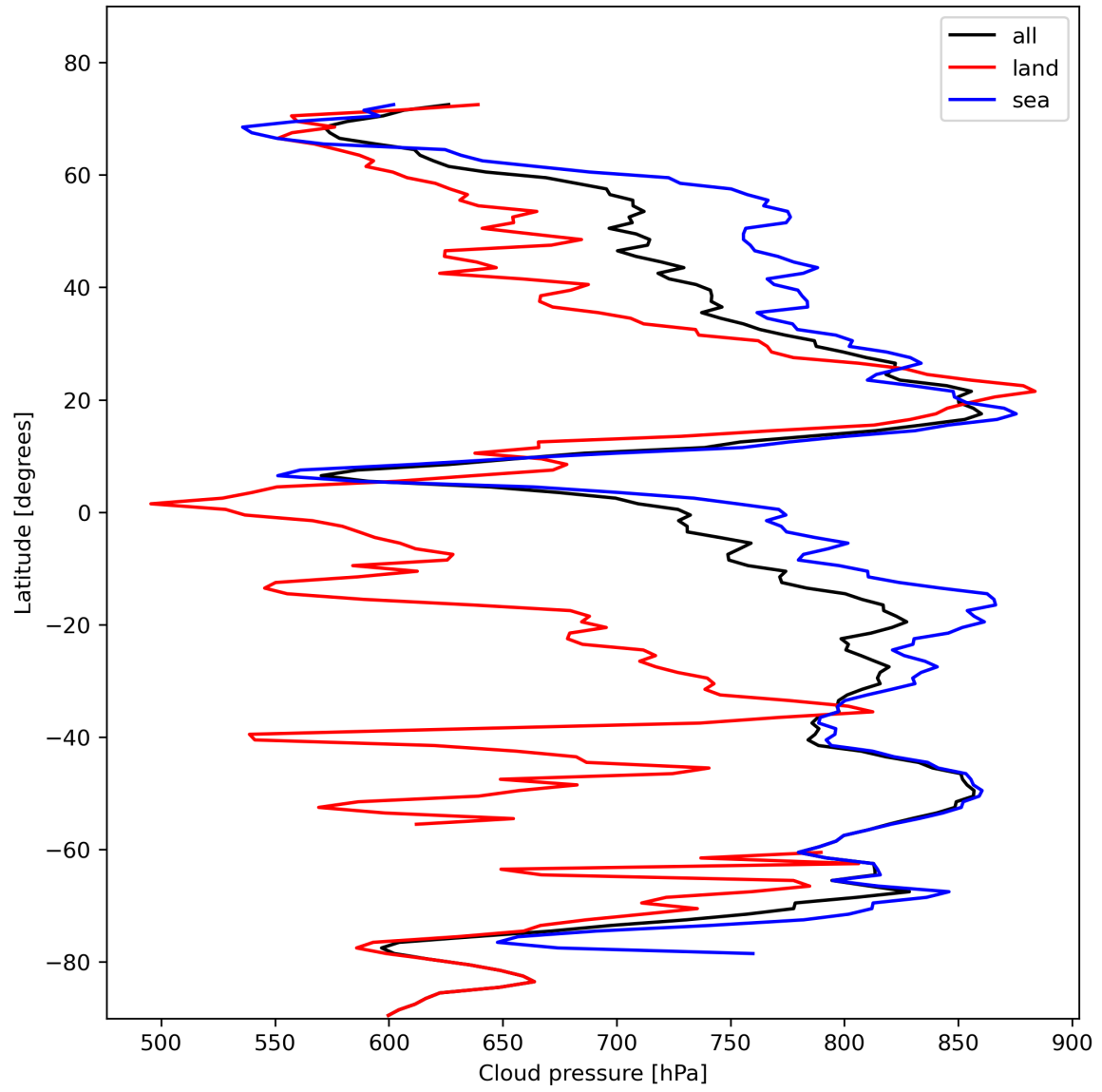
Figure 13: Zonal average of “Cloud pressure” for 2023-11-04 to 2023-11-06.
