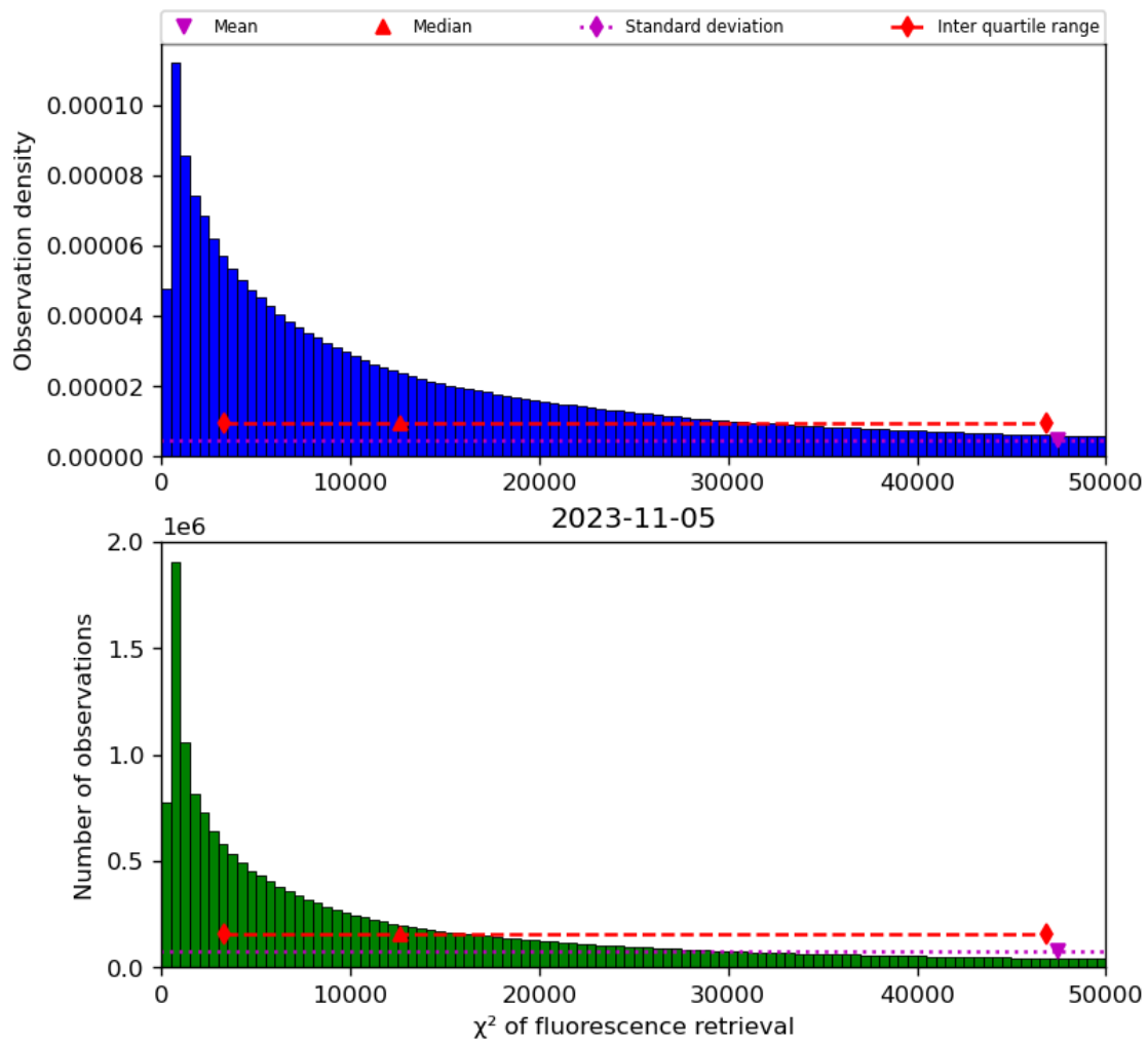
Figure 42: Histogram of “ \chi^2 of fluorescence retrieval” for 2023-11-04 to 2023-11-06
