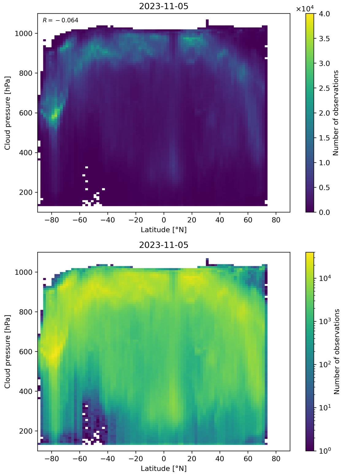
Figure 100: Scatter density plot of “Latitude” against “Cloud pressure” for 2023-11-04 to 2023-11-06.
