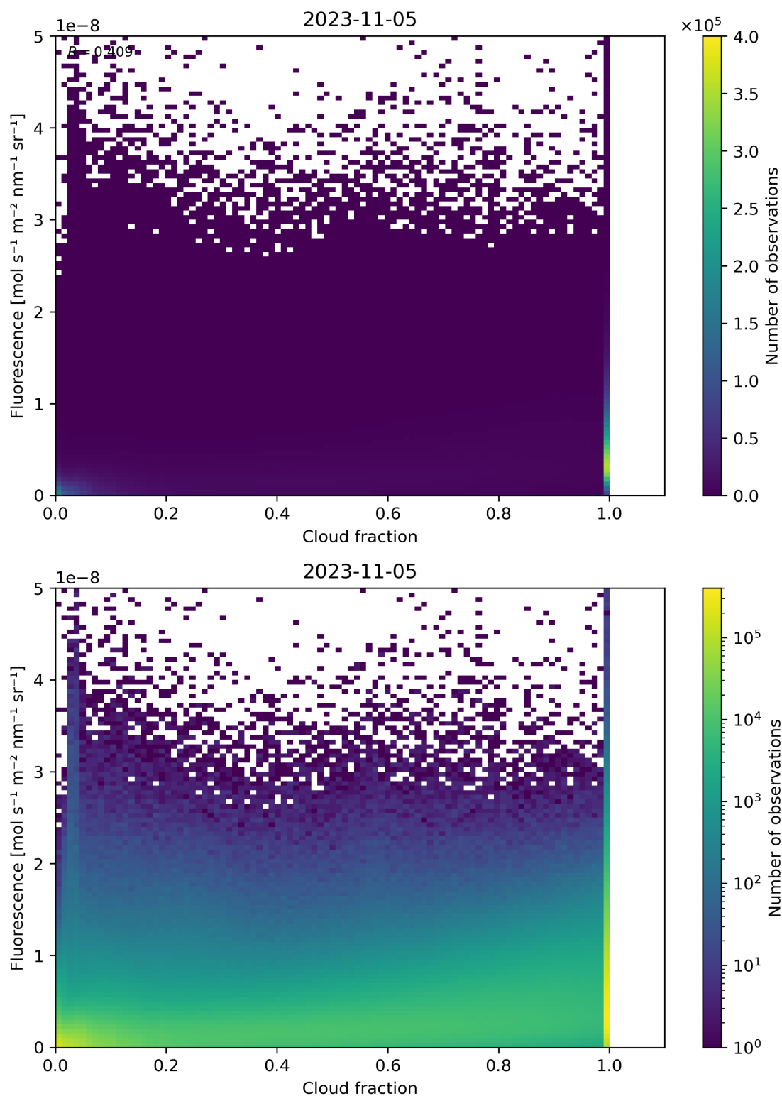
Figure 79: Scatter density plot of “Cloud fraction” against “Fluorescence” for 2023-11-04 to 2023-11-06.
