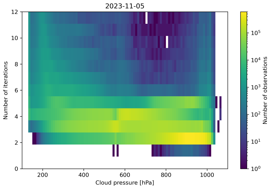
Figure 89: Scatter density plot of “Cloud pressure” against “Number of iterations” for 2023-11-04 to 2023-11-06.
