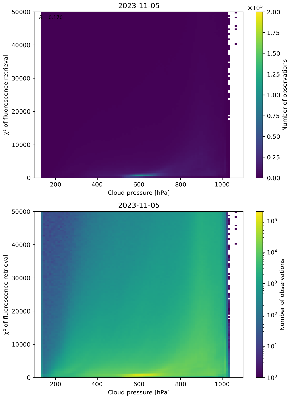
Figure 86: Scatter density plot of “Cloud pressure” against “ \chi^2 of fluorescence retrieval” for 2023-11-04 to 2023-11-06.
