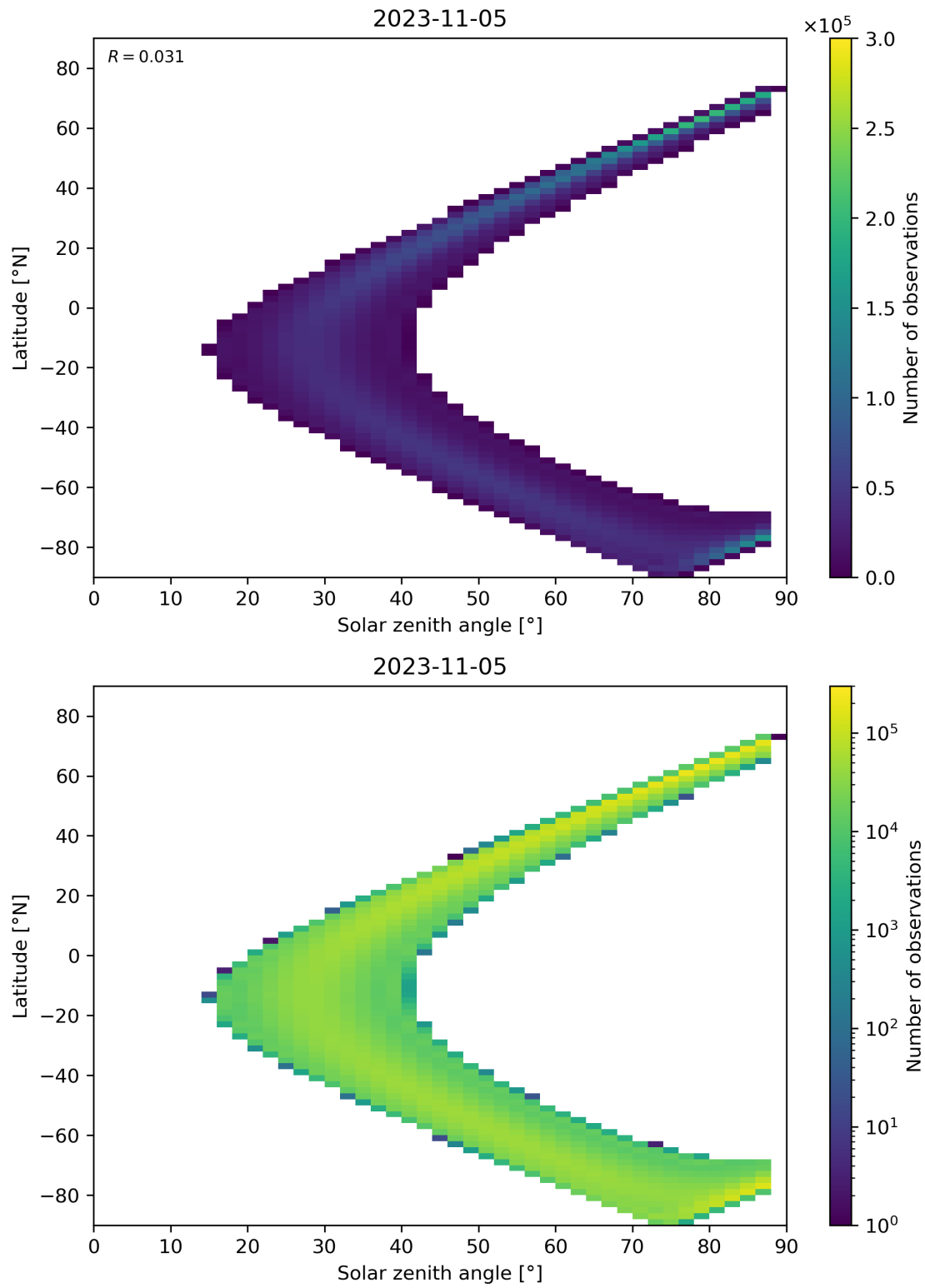
Figure 124: Scatter density plot of “Solar zenith angle” against “Latitude” for 2023-11-04 to 2023-11-06.
