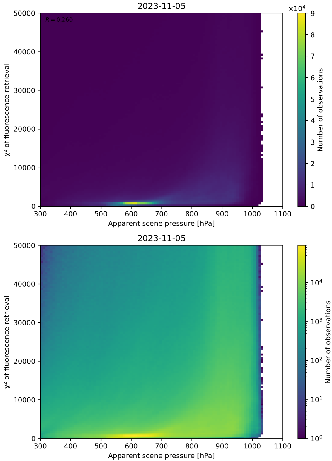
Figure 64: Scatter density plot of “Apparent scene pressure” against “ \chi^2 of fluorescence retrieval” for 2023-11-04 to 2023-11-06.
