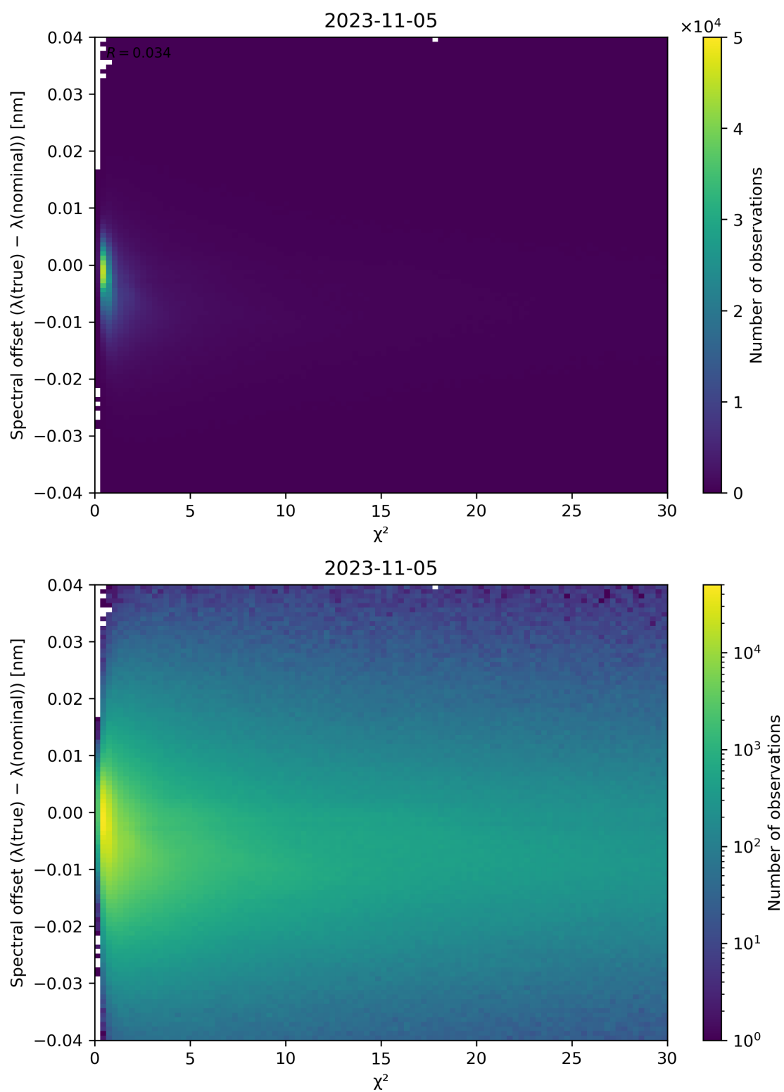
Figure 75: Scatter density plot of “ \chi^2 ” against “Spectral offset ( \lambda(\text{true}) - \lambda(\text{nominal}) )” for 2023-11-04 to 2023-11-06.
