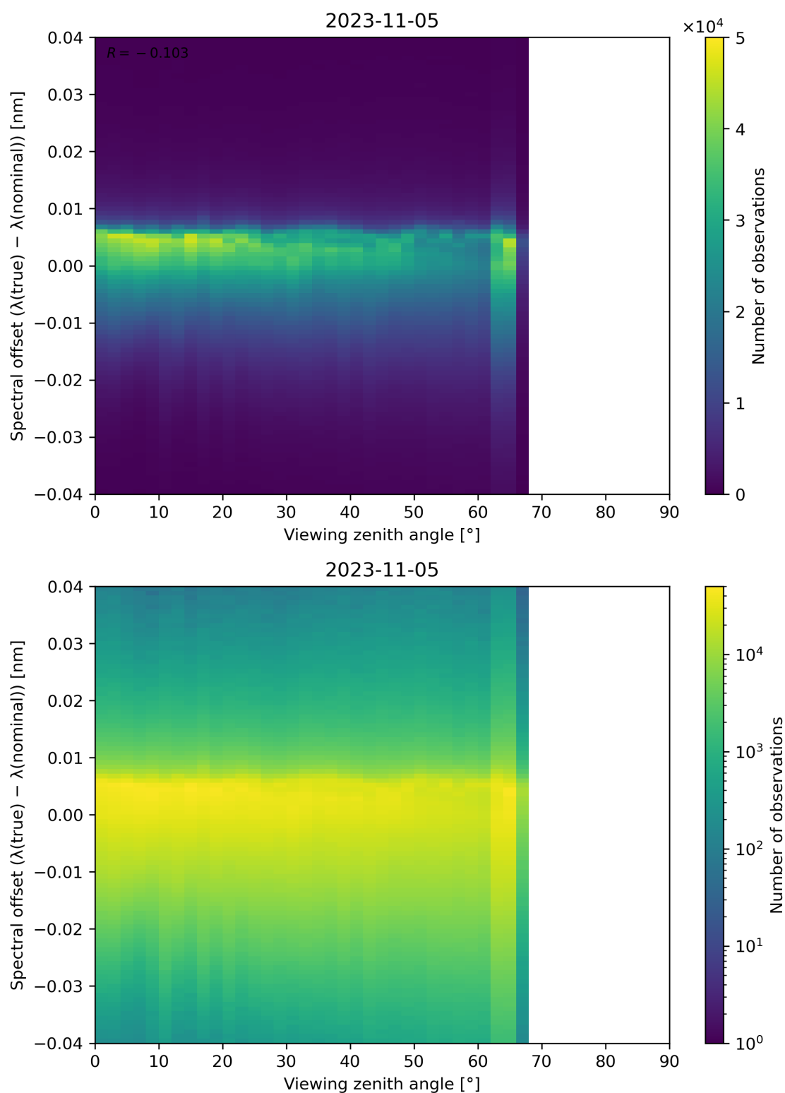
Figure 140: Scatter density plot of “Viewing zenith angle” against “Spectral offset ( \lambda(\text{true}) - \lambda(\text{nominal}) )” for 2023-11-04 to 2023-11-06.
