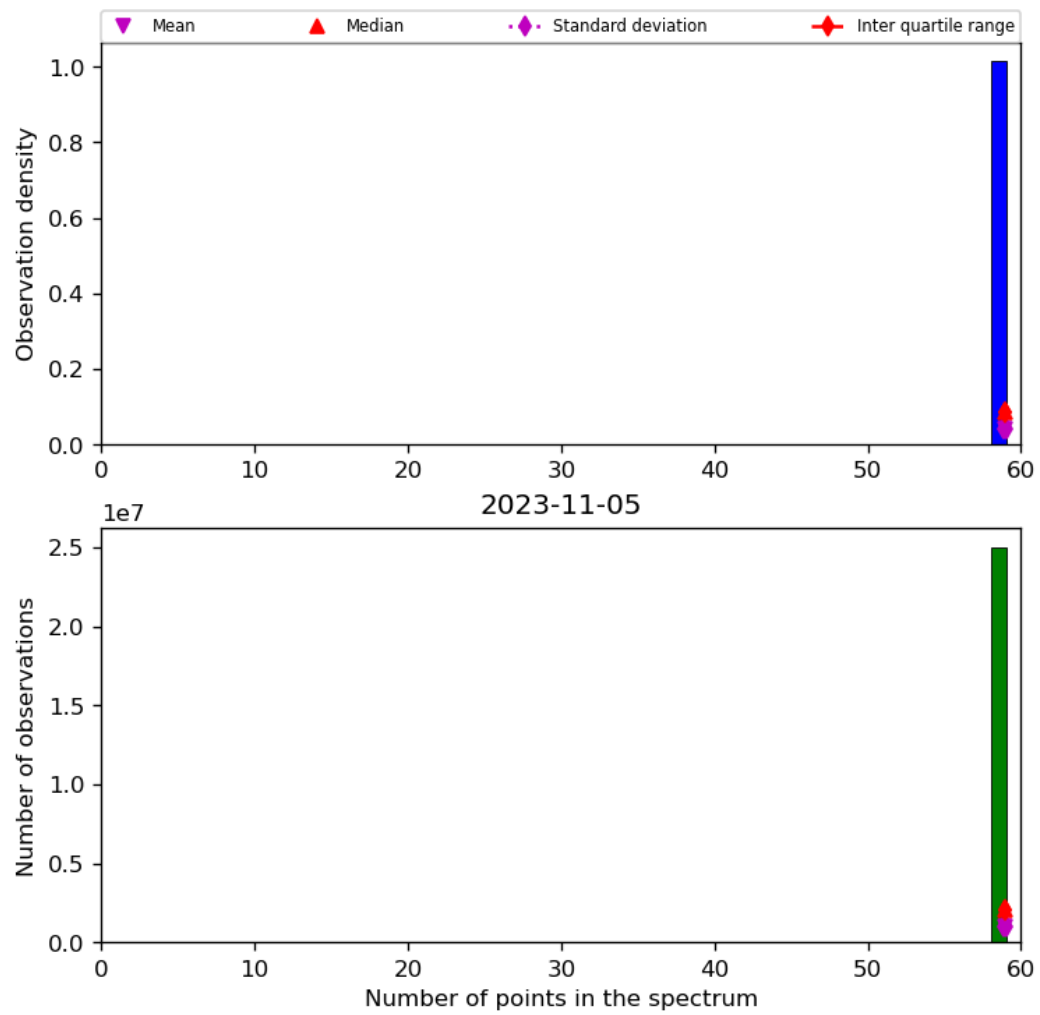
Figure 44: Histogram of "Number of points in the spectrum" for 2023-11-04 to 2023-11-06
