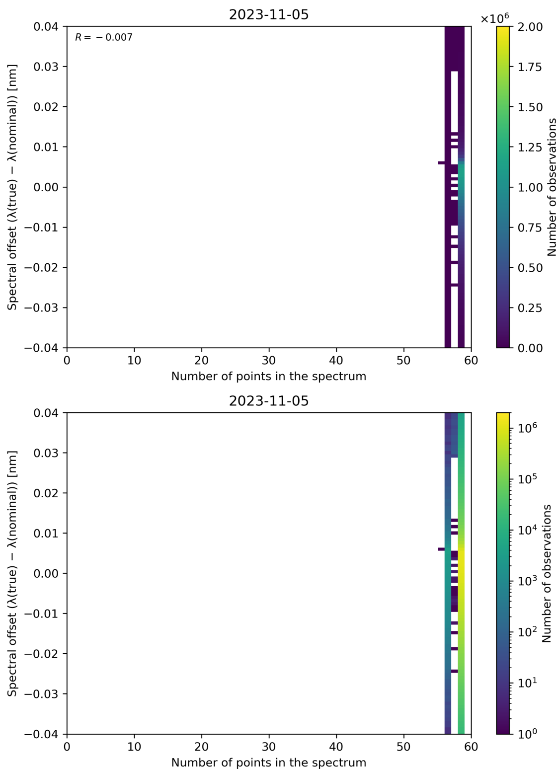
Figure 110: Scatter density plot of “Number of points in the spectrum” against “Spectral offset ( \lambda(\text{true}) - \lambda(\text{nominal}) )” for 2023-11-04 to 2023-11-06.
