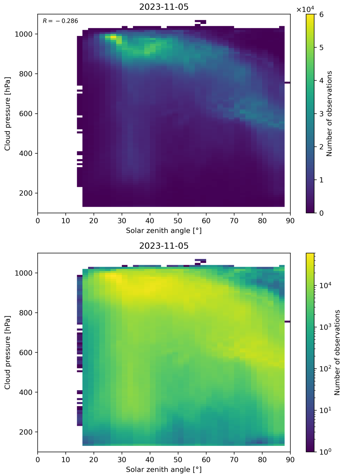
Figure 122: Scatter density plot of “Solar zenith angle” against “Cloud pressure” for 2023-11-04 to 2023-11-06.
