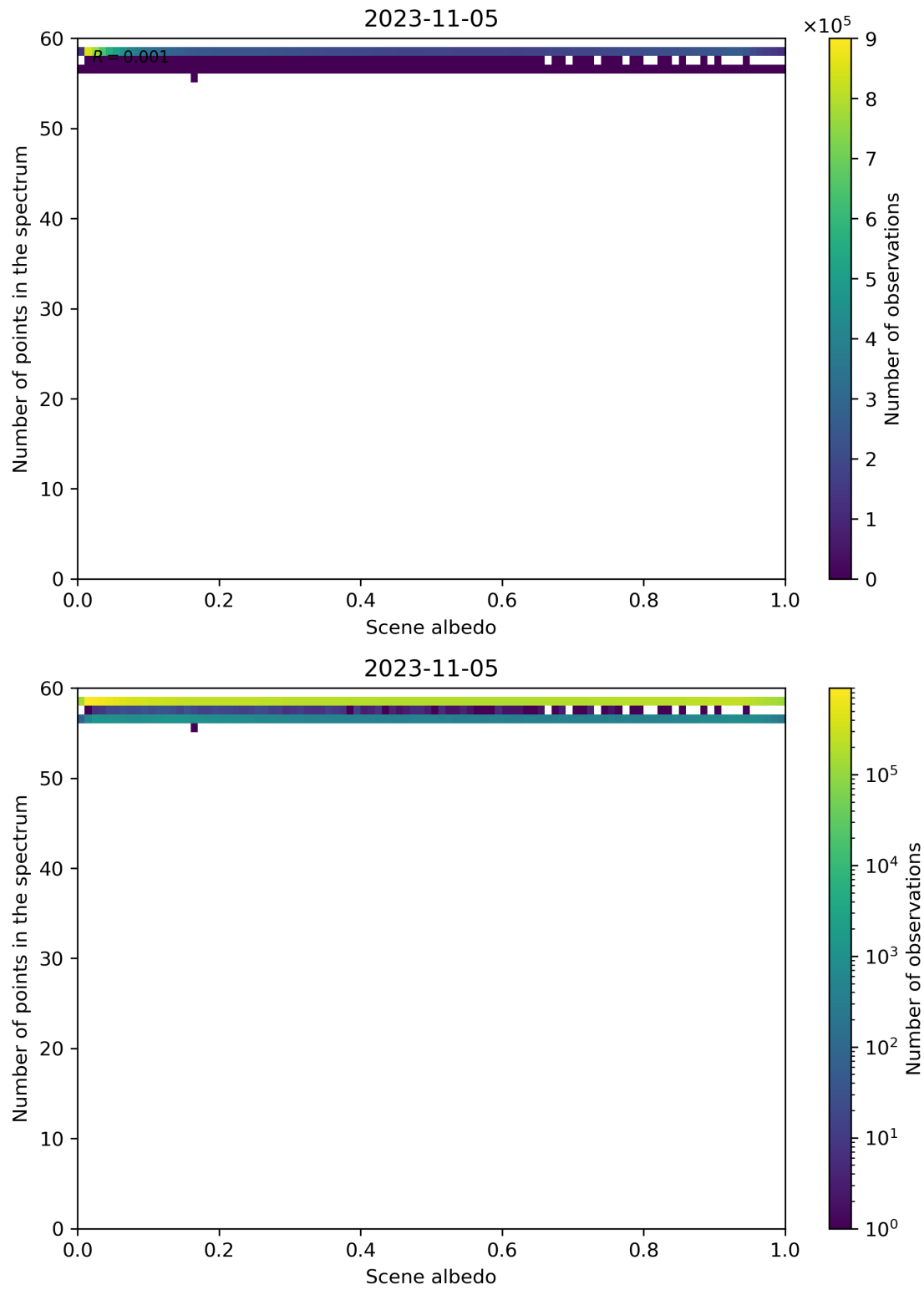
Figure 116: Scatter density plot of “Scene albedo” against “Number of points in the spectrum” for 2023-11-04 to 2023-11-06.
