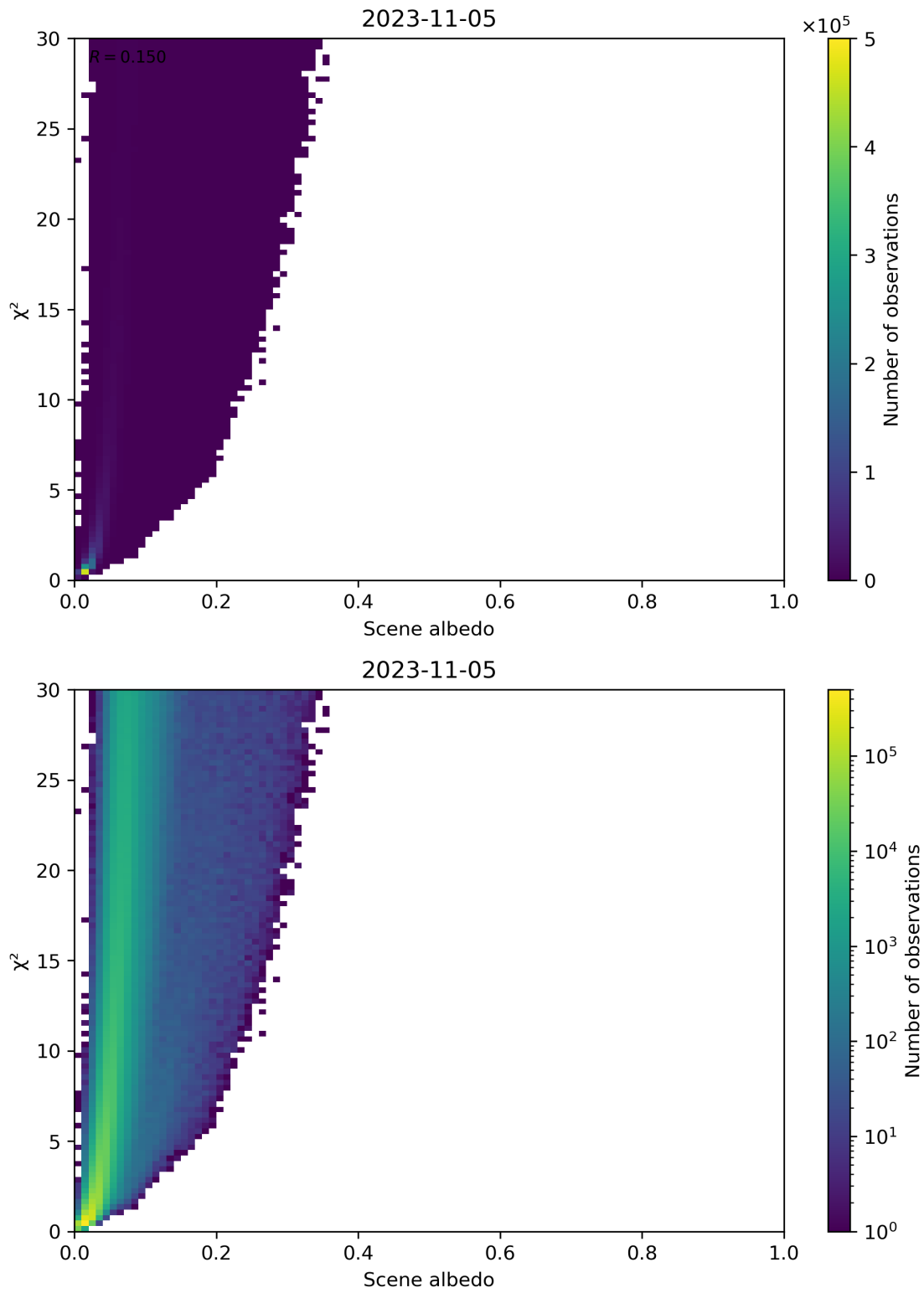
Figure 112: Scatter density plot of “Scene albedo” against “ \chi^2 ” for 2023-11-04 to 2023-11-06.
