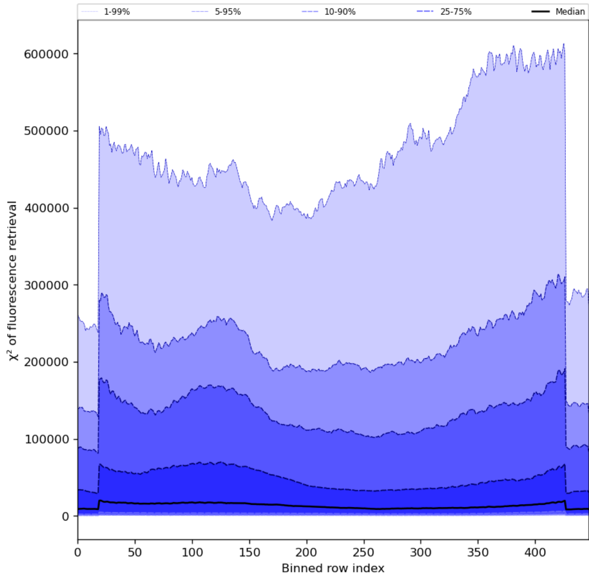
Figure 59: Along track statistics of “ \chi^2 of fluorescence retrieval” for 2023-11-04 to 2023-11-06
