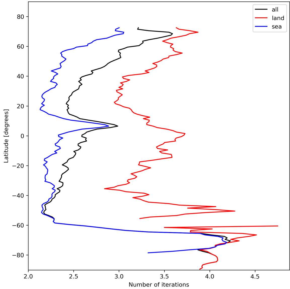
Figure 22: Zonal average of “Number of iterations” for 2023-11-04 to 2023-11-06.
