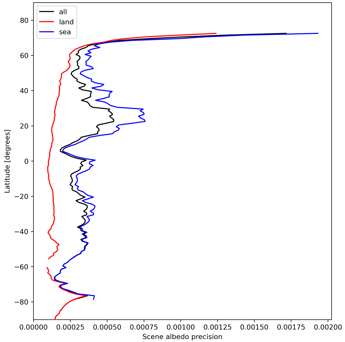
Figure 18: Zonal average of “Scene albedo precision” for 2023-11-04 to 2023-11-06.
