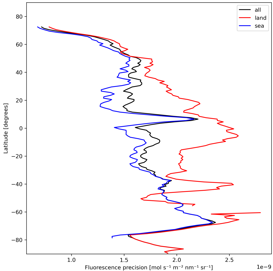
Figure 24: Zonal average of “Fluorescence precision” for 2023-11-04 to 2023-11-06.
