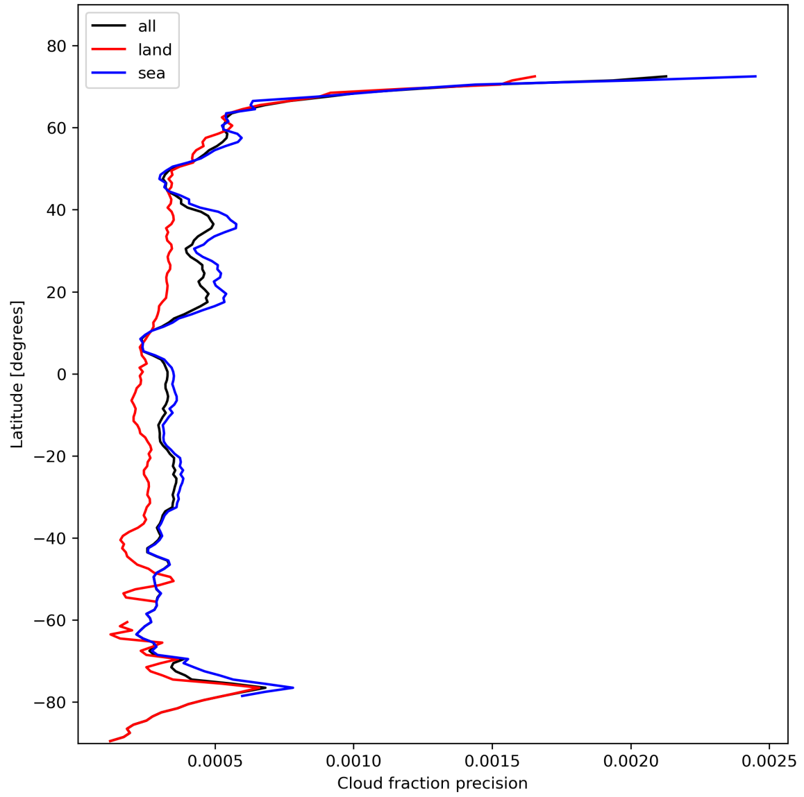
Figure 16: Zonal average of “Cloud fraction precision” for 2023-11-05 to 2023-11-07.
