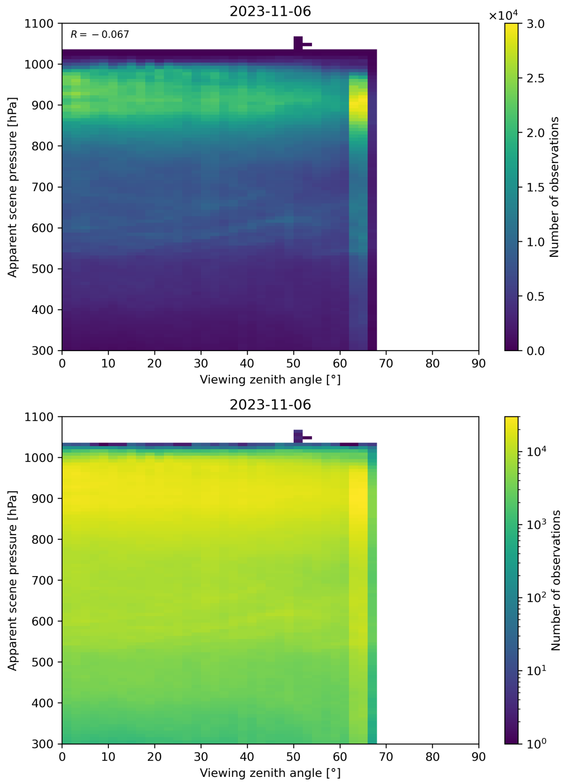
Figure 129: Scatter density plot of “Viewing zenith angle” against “Apparent scene pressure” for 2023-11-05 to 2023-11-07.
