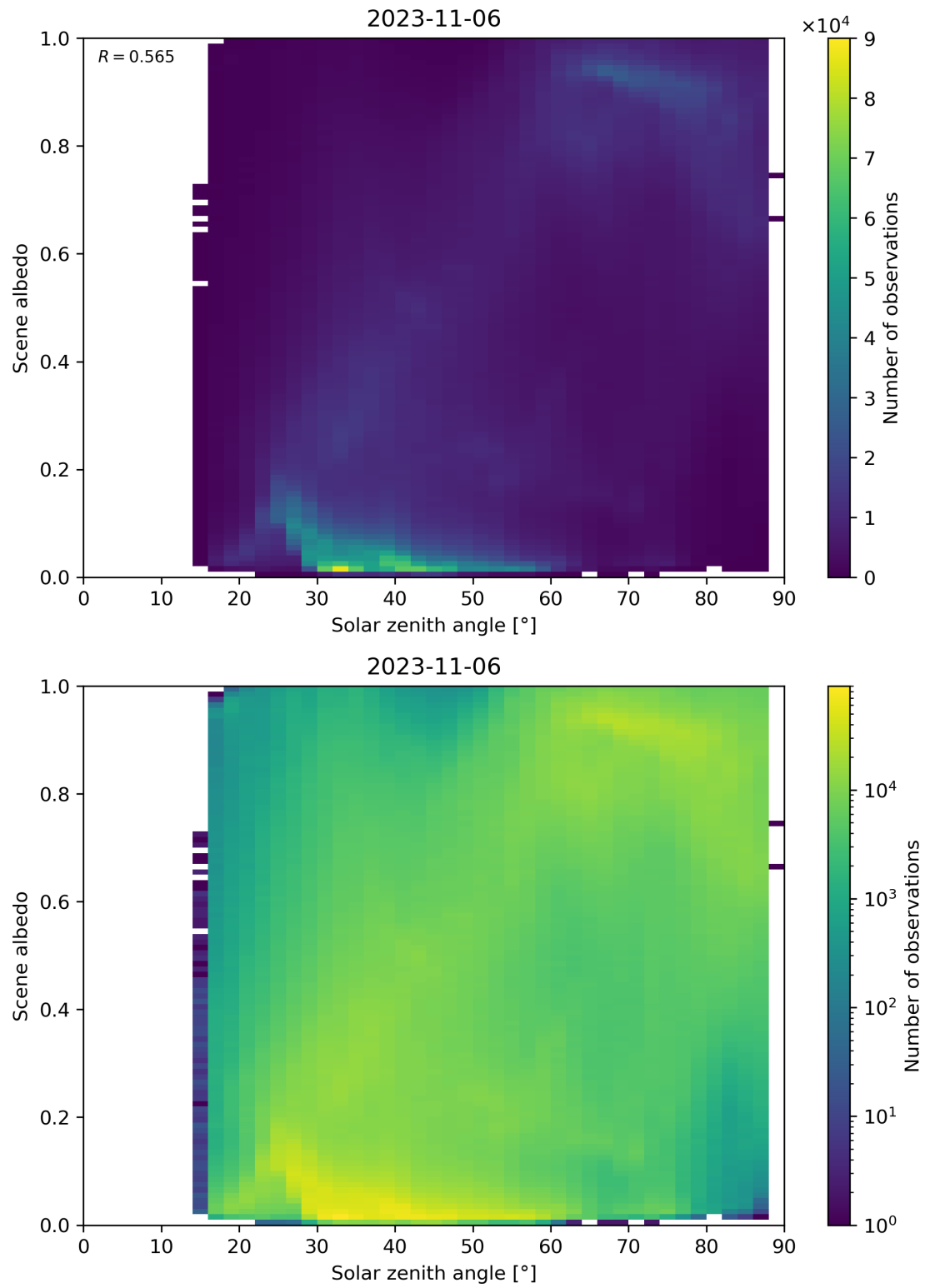
Figure 127: Scatter density plot of “Solar zenith angle” against “Scene albedo” for 2023-11-05 to 2023-11-07.
