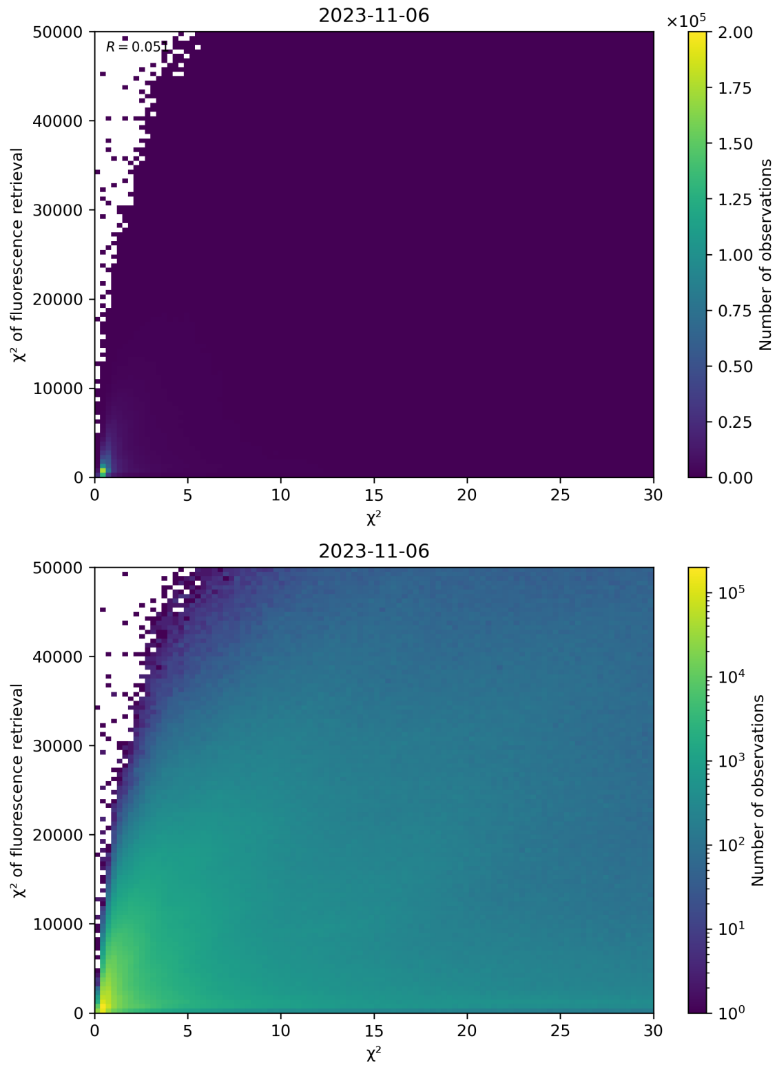
Figure 69: Scatter density plot of “ \chi^2 ” against “ \chi^2 of fluorescence retrieval” for 2023-11-05 to 2023-11-07.
