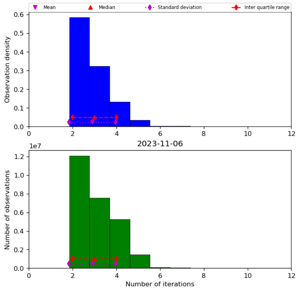
Figure 39: Histogram of “Number of iterations” for 2023-11-05 to 2023-11-07
