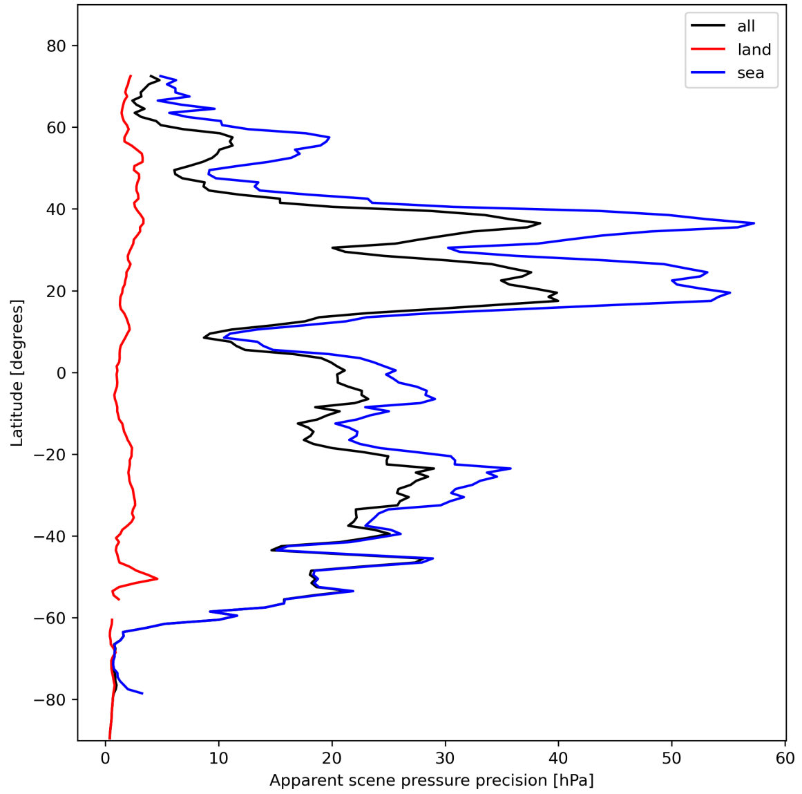
Figure 20: Zonal average of “Apparent scene pressure precision” for 2023-11-05 to 2023-11-07.
