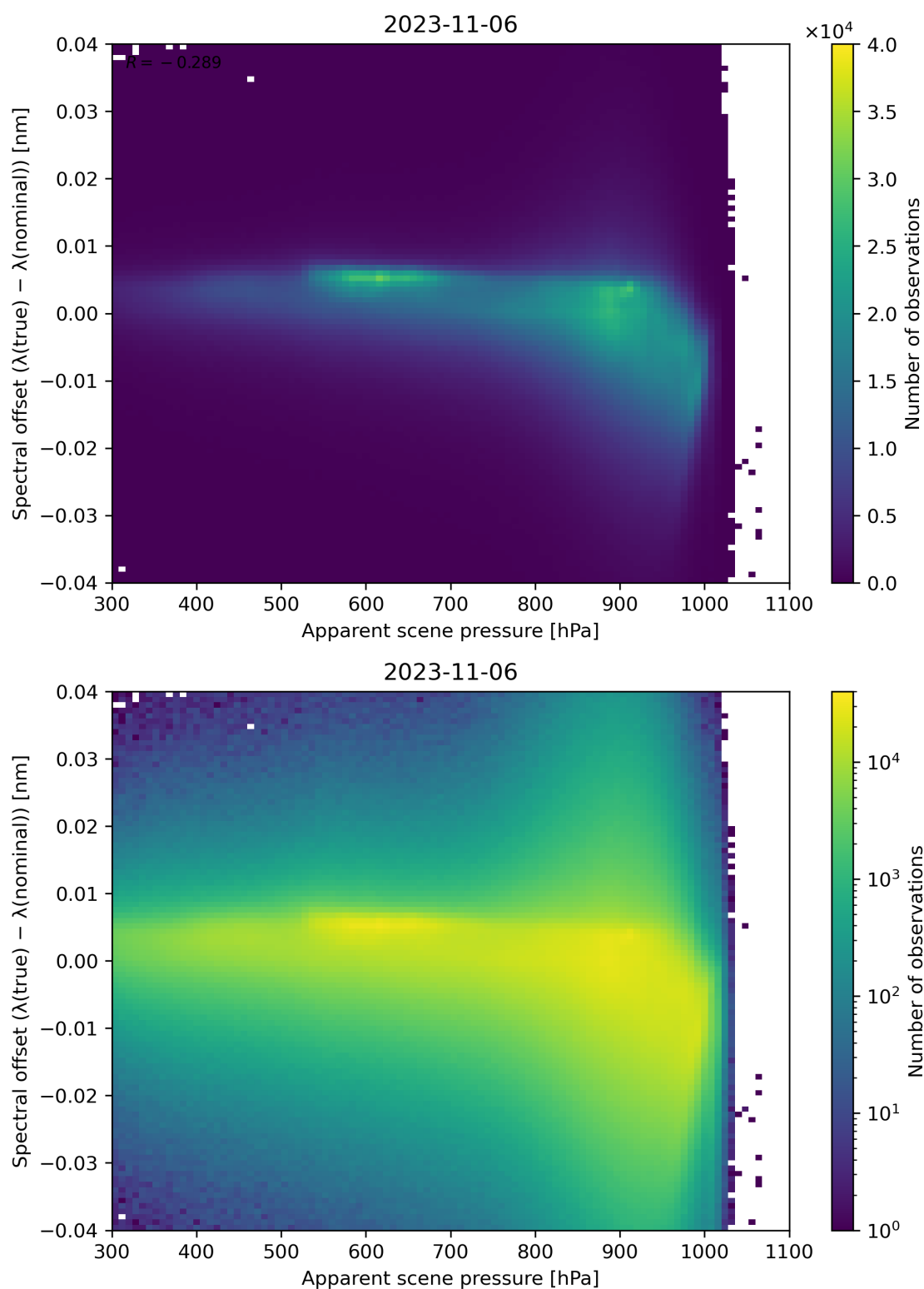
Figure 68: Scatter density plot of “Apparent scene pressure” against “Spectral offset ( \lambda(\text{true}) - \lambda(\text{nominal}) )” for 2023-11-05 to 2023-11-07.
