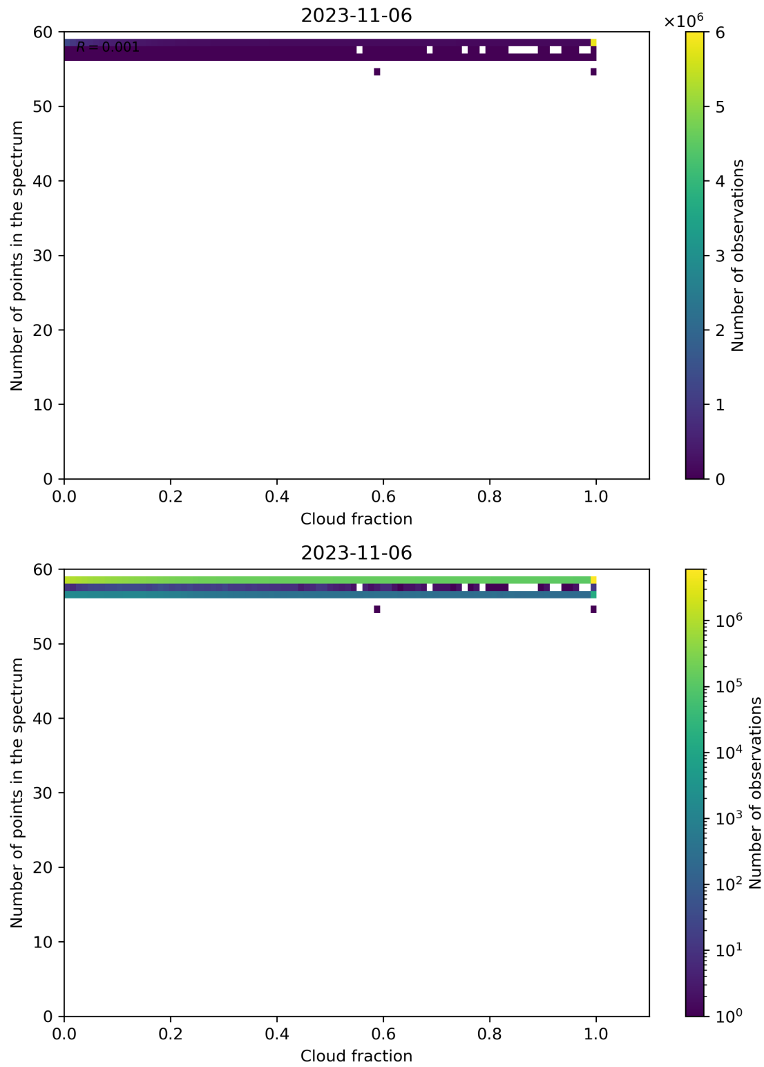
Figure 81: Scatter density plot of “Cloud fraction” against “Number of points in the spectrum” for 2023-11-05 to 2023-11-07.
