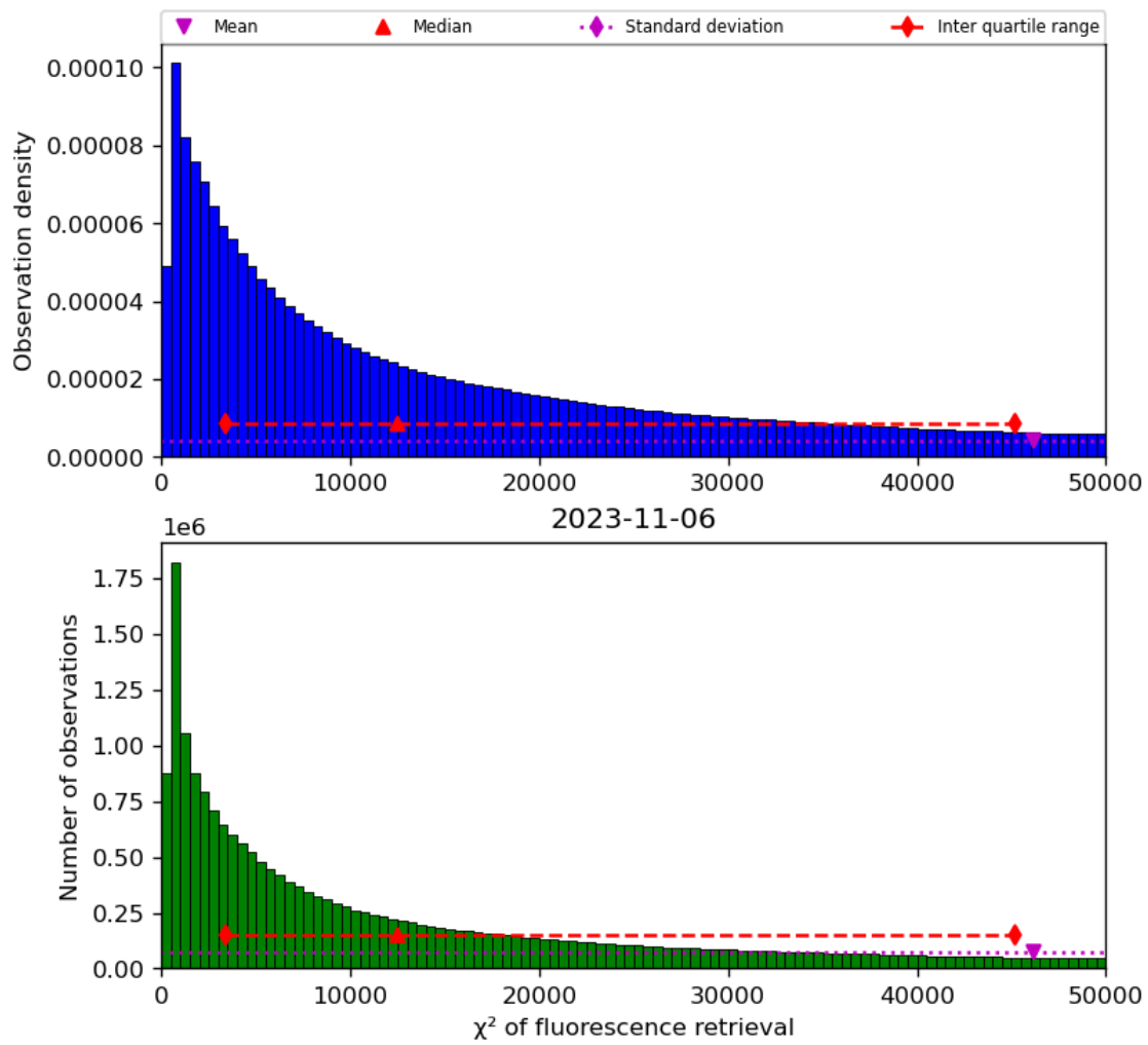
Figure 42: Histogram of “ \chi^2 of fluorescence retrieval” for 2023-11-05 to 2023-11-07
