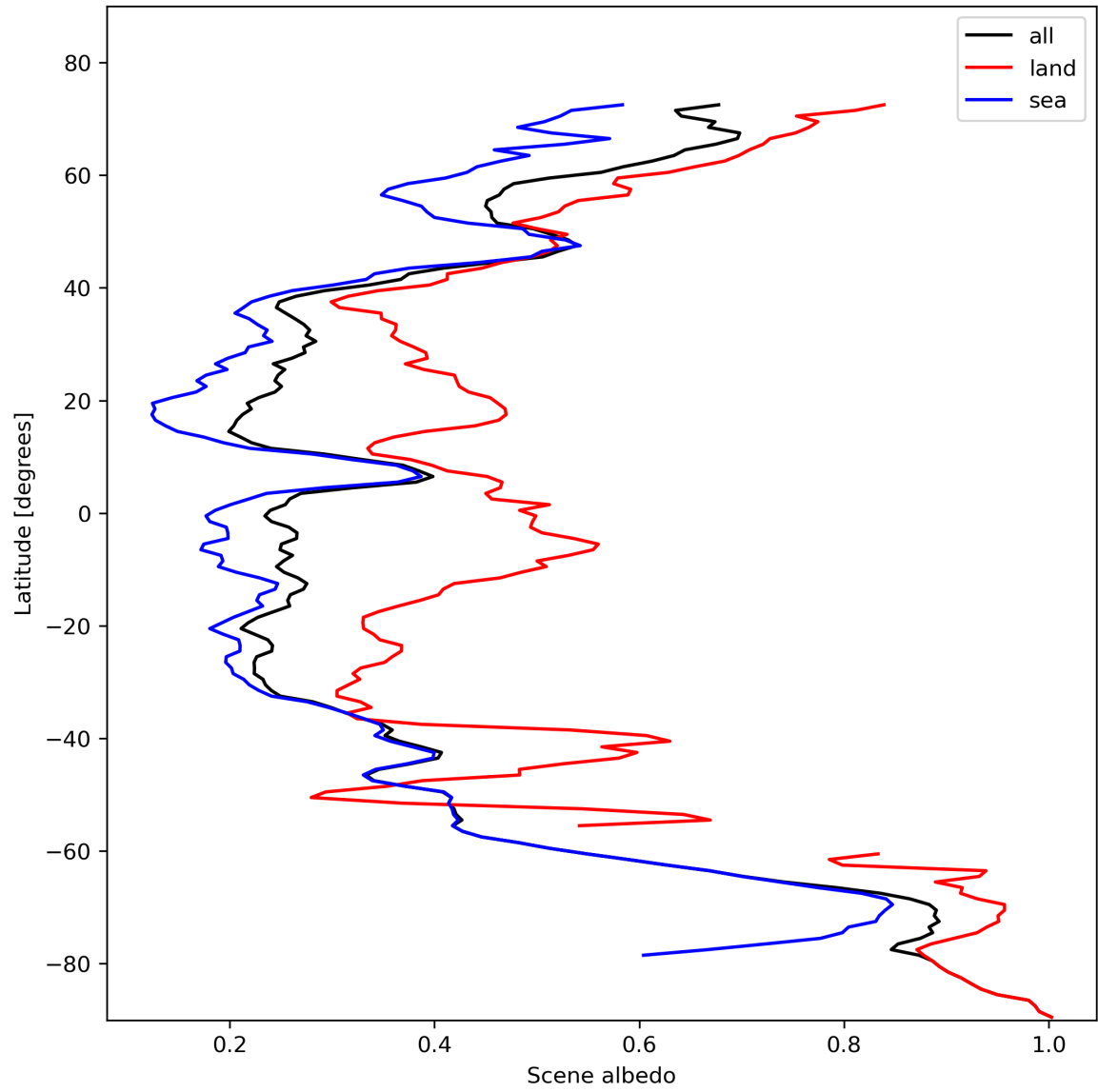
Figure 17: Zonal average of “Scene albedo” for 2023-11-05 to 2023-11-07.
