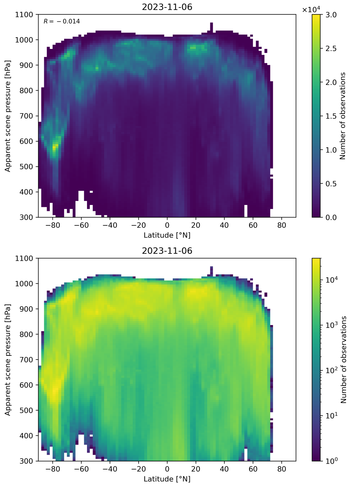
Figure 96: Scatter density plot of “Latitude” against “Apparent scene pressure” for 2023-11-05 to 2023-11-07.
