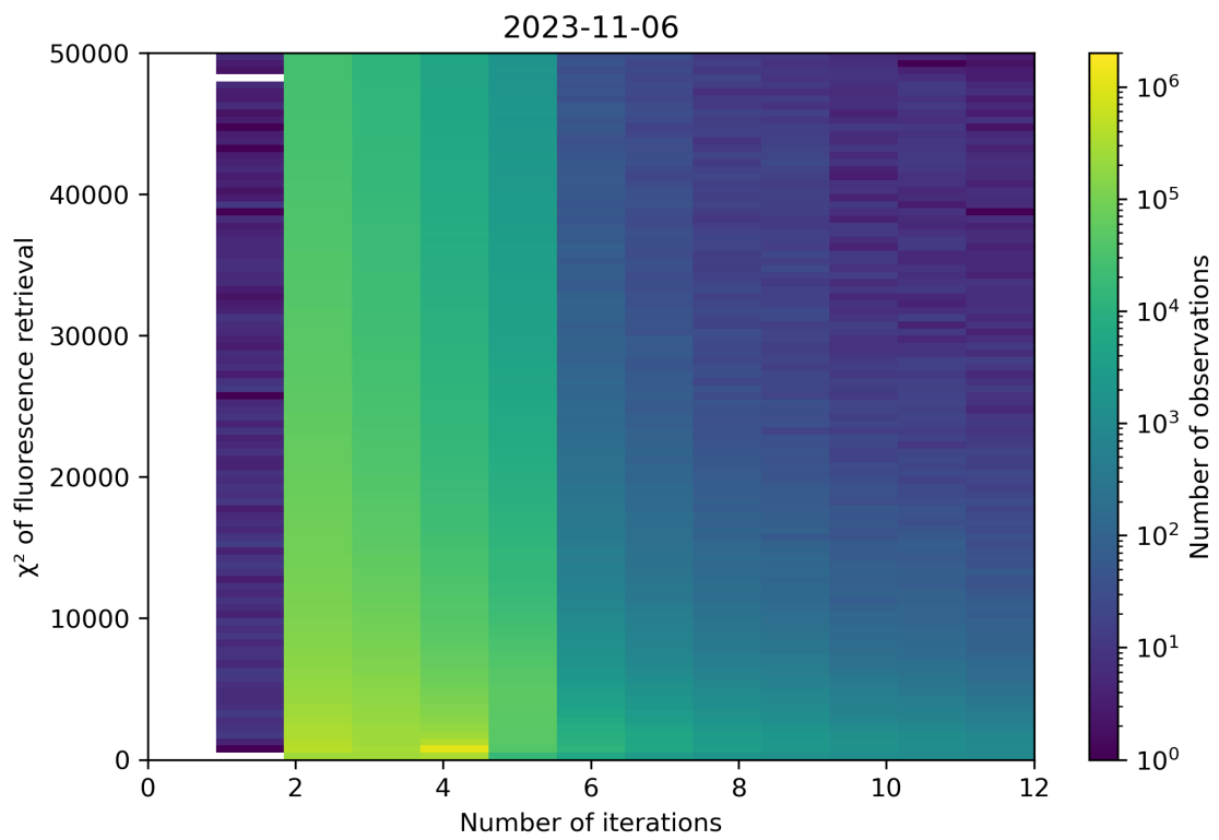
Figure 106: Scatter density plot of “Number of iterations” against “ \chi^2 of fluorescence retrieval” for 2023-11-05 to 2023-11-07.
