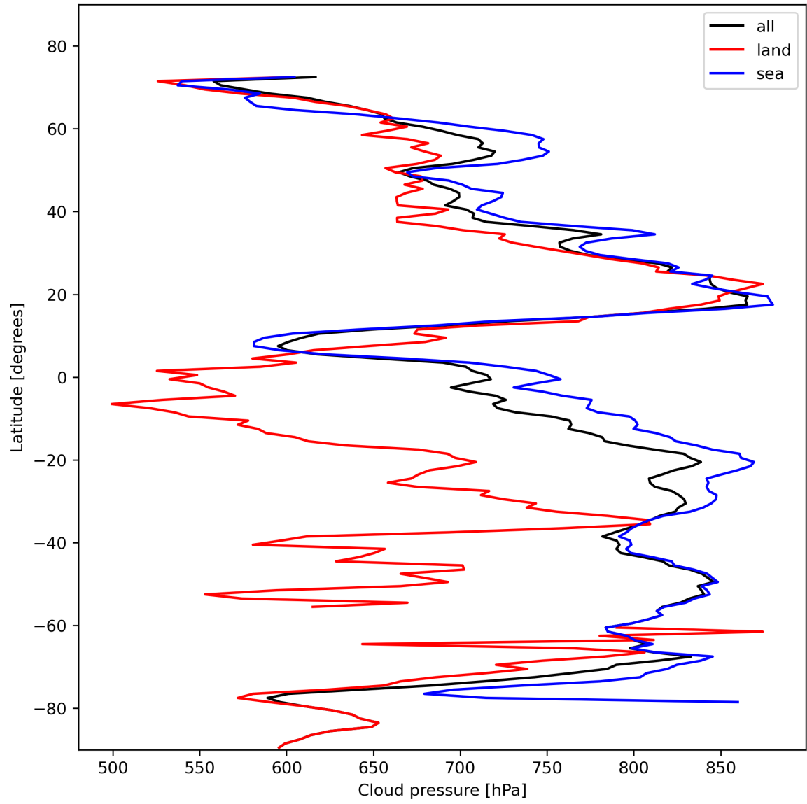
Figure 13: Zonal average of “Cloud pressure” for 2023-11-05 to 2023-11-07.
