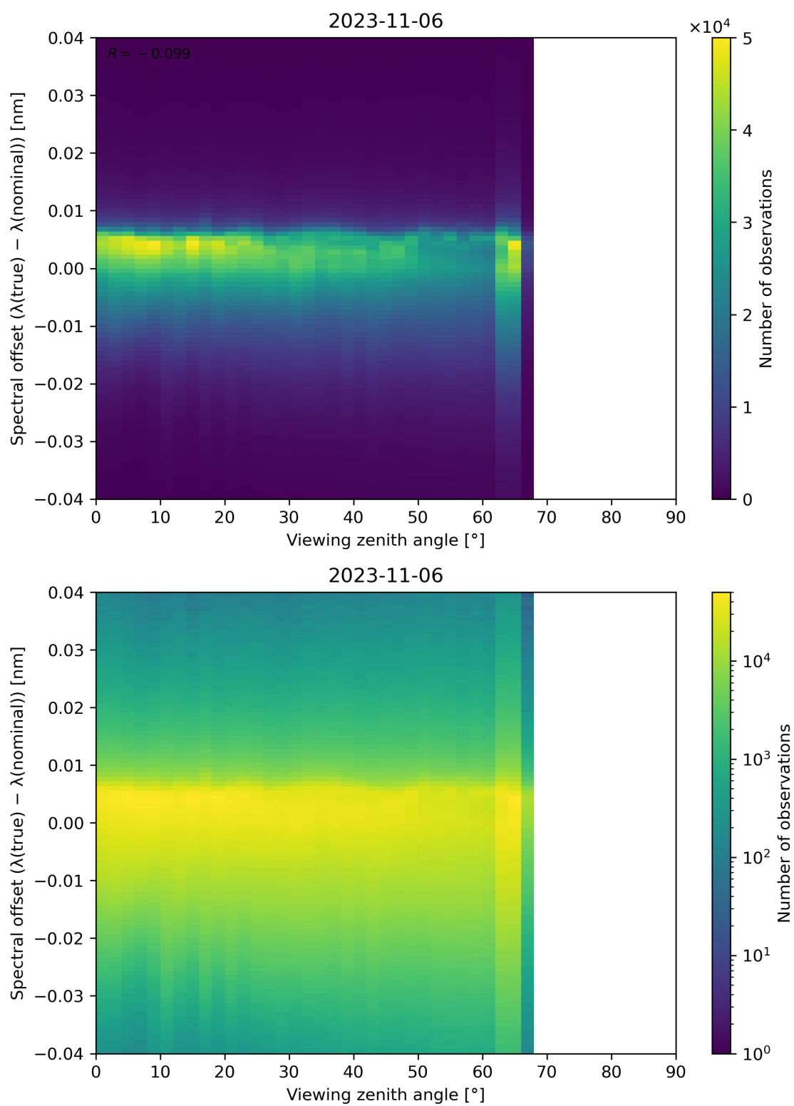
Figure 140: Scatter density plot of “Viewing zenith angle” against “Spectral offset ( \lambda(\text{true}) - \lambda(\text{nominal}) )” for 2023-11-05 to 2023-11-07.
