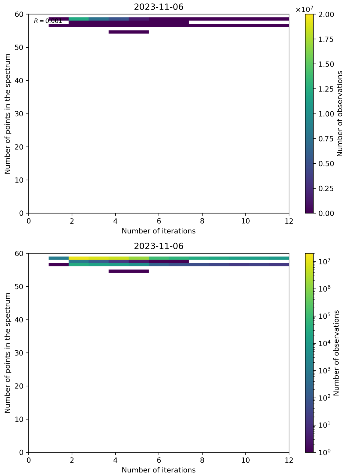
Figure 108: Scatter density plot of “Number of iterations” against “Number of points in the spectrum” for 2023-11-05 to 2023-11-07.
