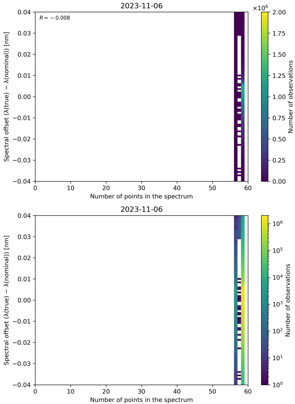
Figure 110: Scatter density plot of “Number of points in the spectrum” against “Spectral offset ( \lambda(\text{true}) - \lambda(\text{nominal}) )” for 2023-11-05 to 2023-11-07.
