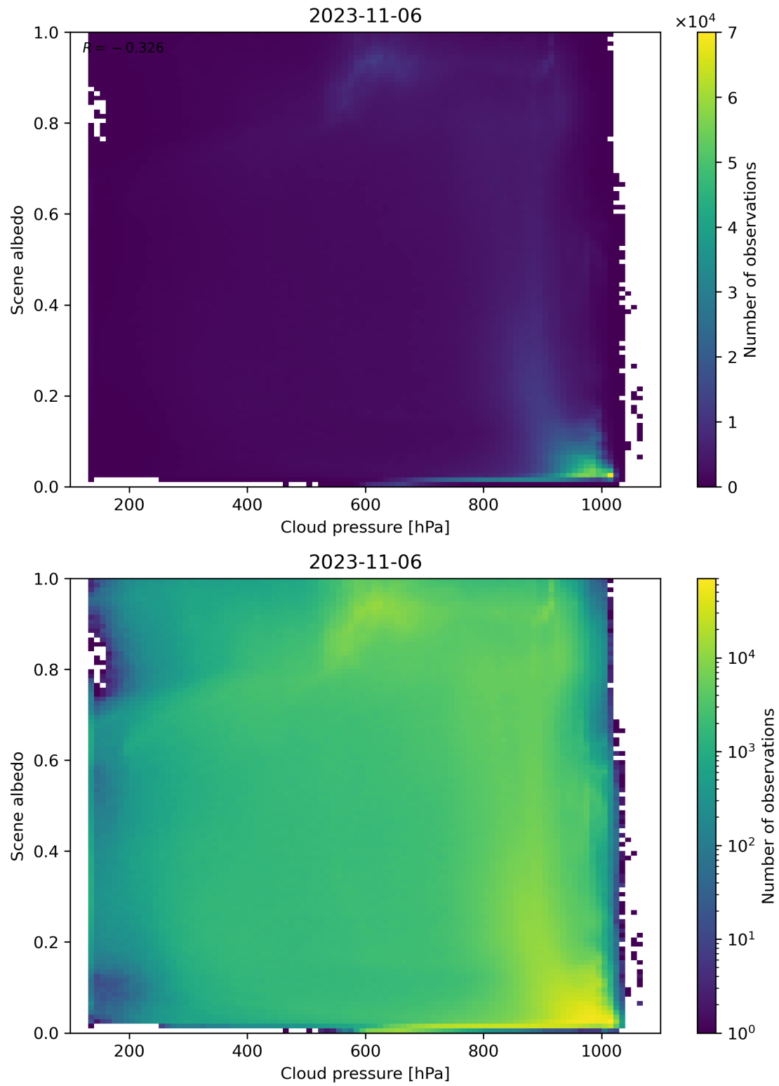
Figure 91: Scatter density plot of “Cloud pressure” against “Scene albedo” for 2023-11-05 to 2023-11-07.
