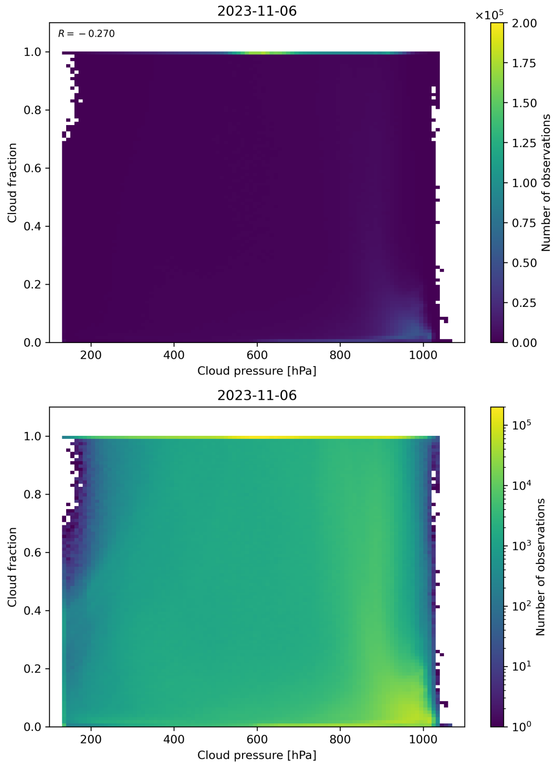
Figure 87: Scatter density plot of “Cloud pressure” against “Cloud fraction” for 2023-11-05 to 2023-11-07.
