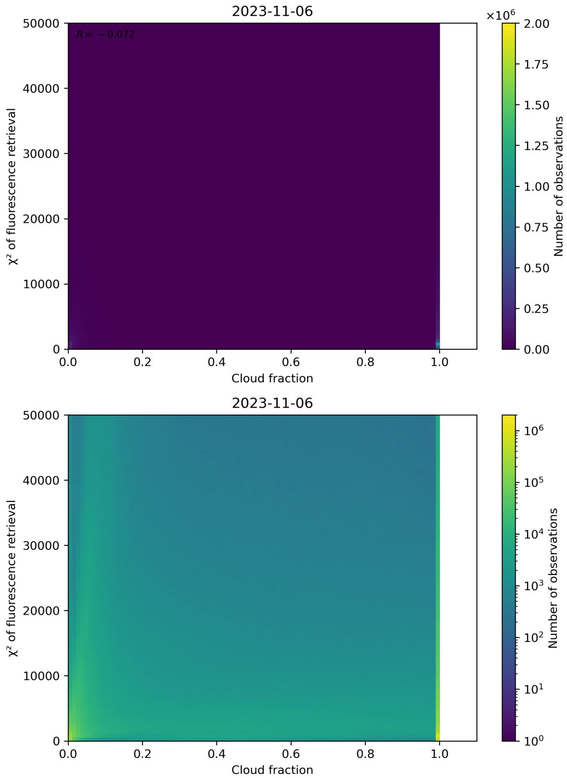
Figure 78: Scatter density plot of “Cloud fraction” against “ \chi^2 of fluorescence retrieval” for 2023-11-05 to 2023-11-07.
