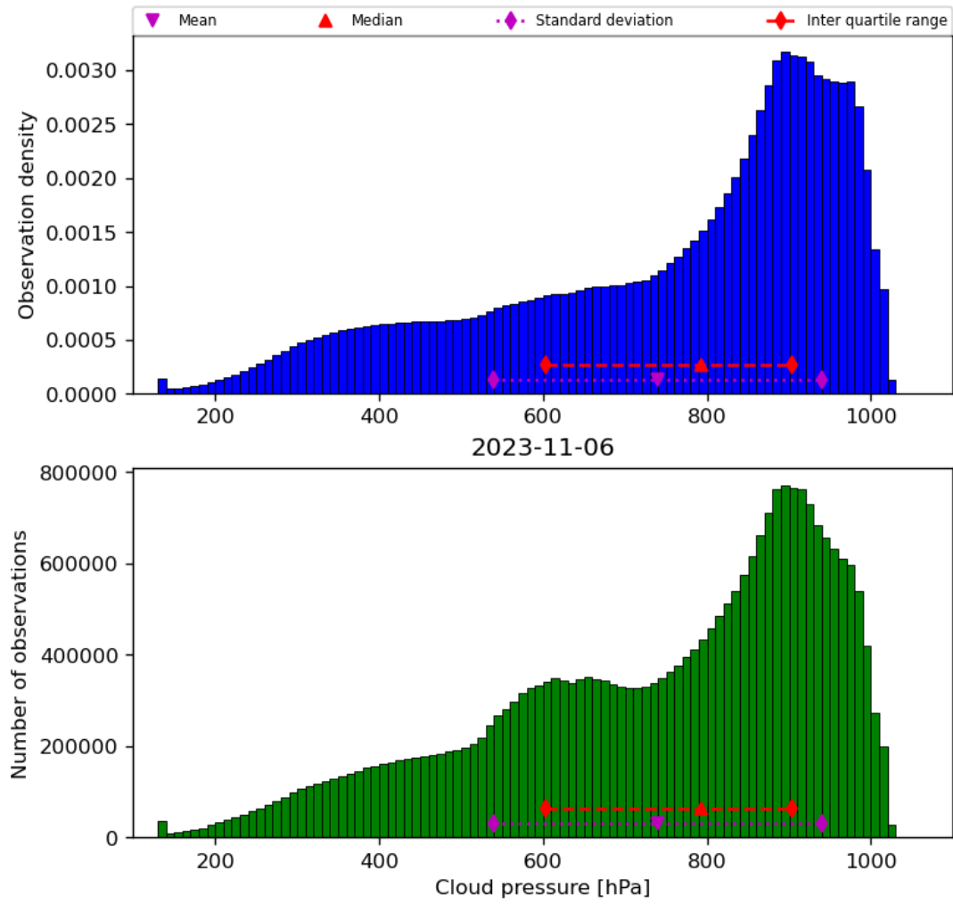
Figure 30: Histogram of “Cloud pressure” for 2023-11-05 to 2023-11-07
