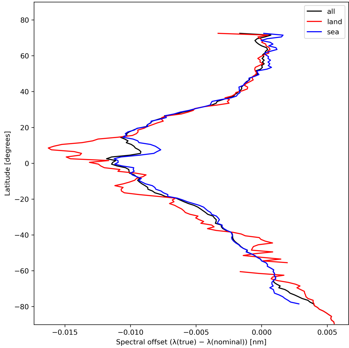
Figure 28: Zonal average of “Spectral offset ( \lambda(\text{true}) - \lambda(\text{nominal}) )” for 2023-11-05 to 2023-11-07.
