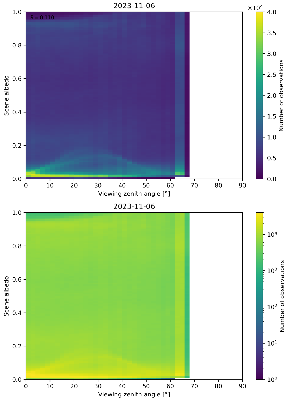
Figure 138: Scatter density plot of “Viewing zenith angle” against “Scene albedo” for 2023-11-05 to 2023-11-07.
