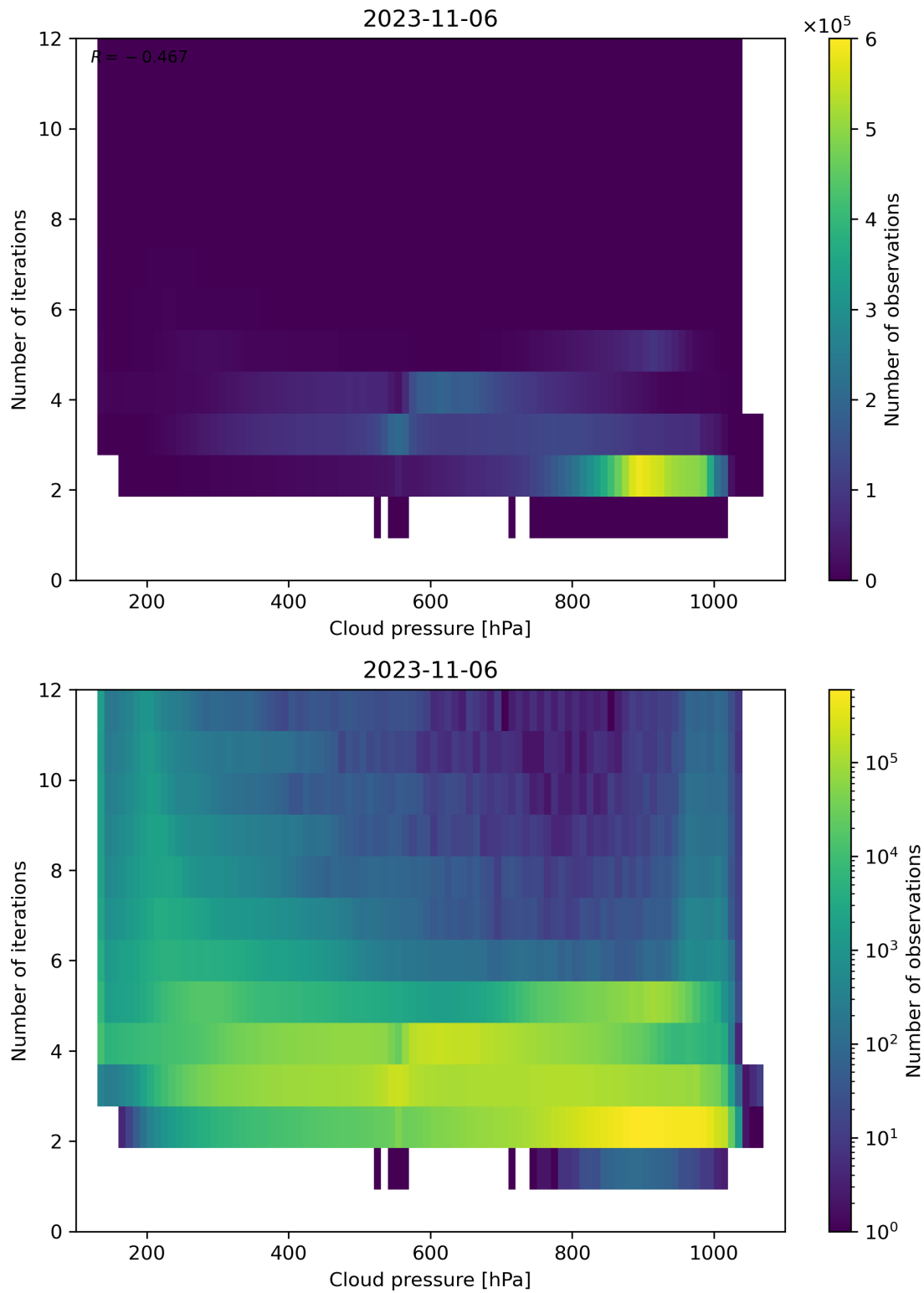
Figure 89: Scatter density plot of “Cloud pressure” against “Number of iterations” for 2023-11-05 to 2023-11-07.
