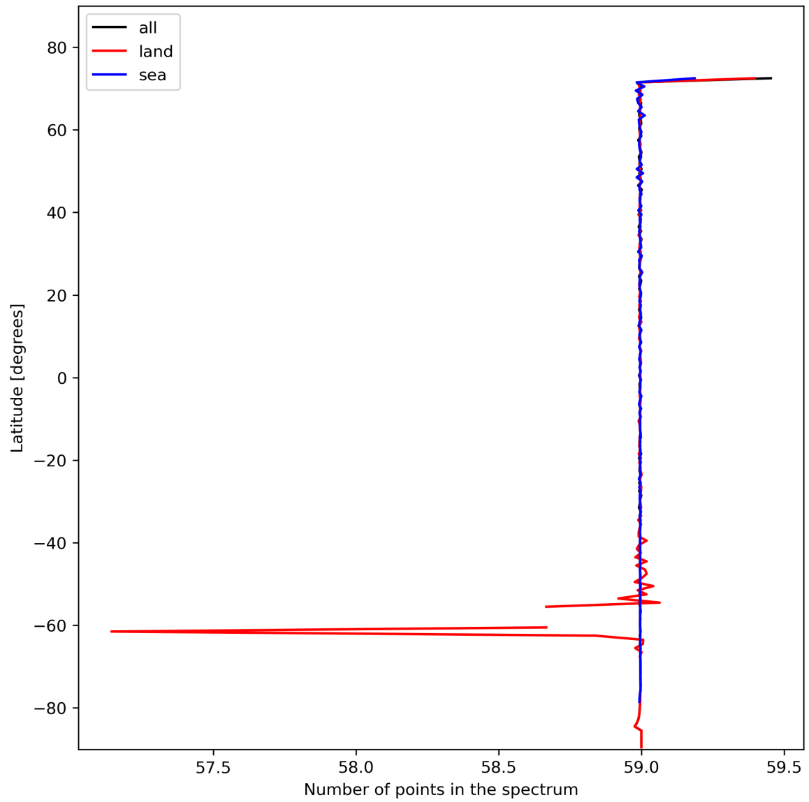
Figure 27: Zonal average of “Number of points in the spectrum” for 2023-11-05 to 2023-11-07.
