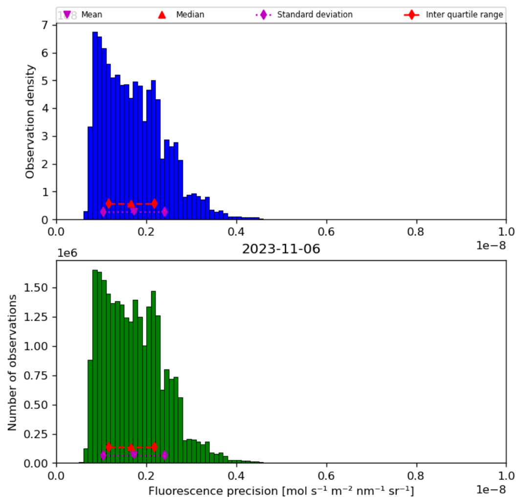
Figure 41: Histogram of “Fluorescence precision” for 2023-11-05 to 2023-11-07
