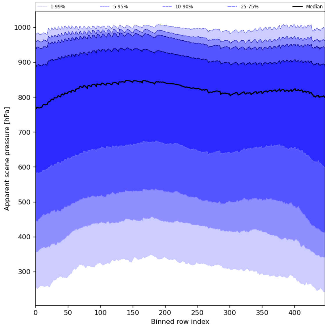
Figure 53: Along track statistics of “Apparent scene pressure” for 2023-11-05 to 2023-11-07
