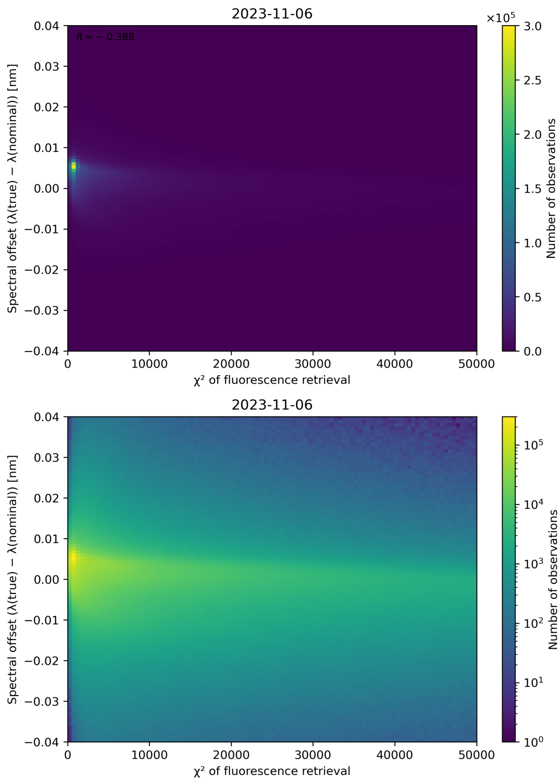
Figure 72: Scatter density plot of " \chi^2 of fluorescence retrieval" against "Spectral offset ( \lambda(\text{true}) - \lambda(\text{nominal}) )" for 2023-11-05 to 2023-11-07.
