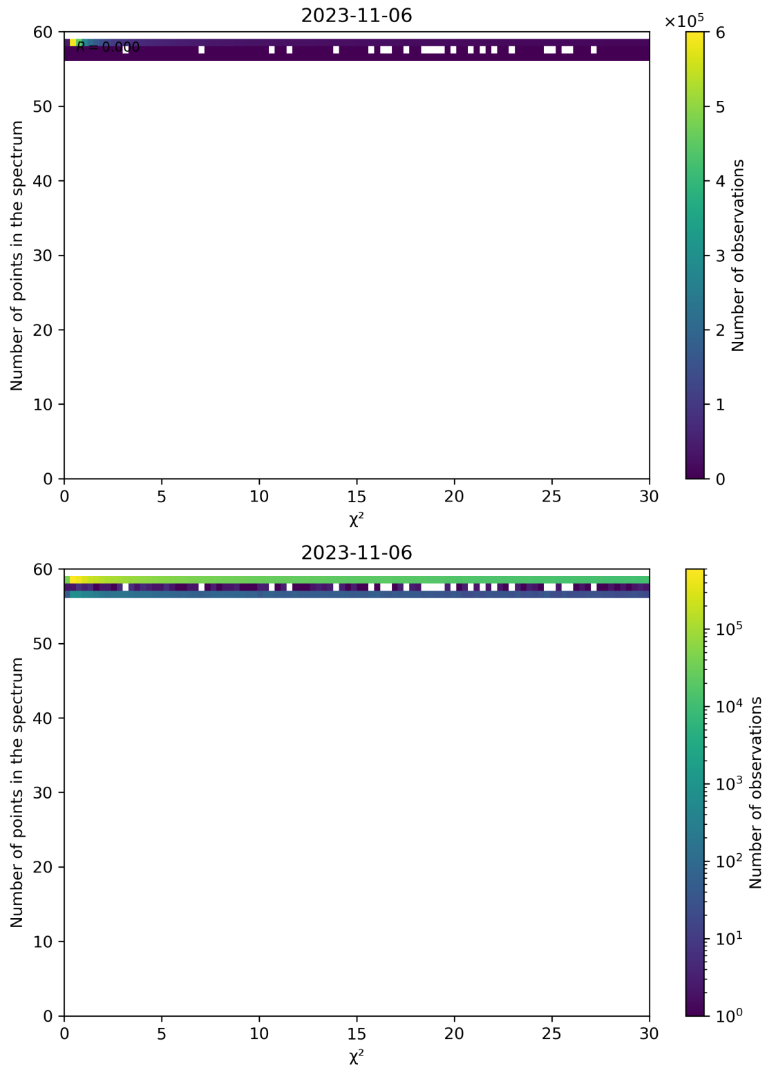
Figure 74: Scatter density plot of " \chi^2 " against "Number of points in the spectrum" for 2023-11-05 to 2023-11-07.
