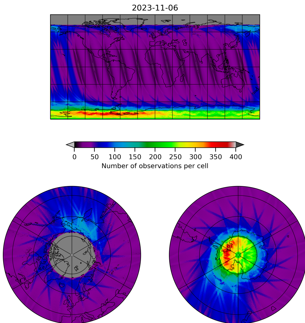
Figure 11: Map of the number of observations for 2023-11-05 to 2023-11-07
