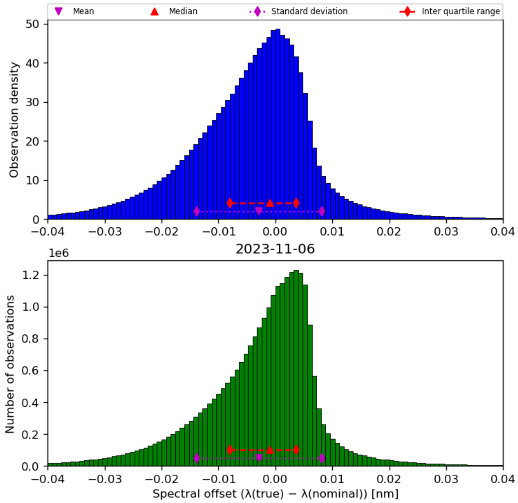
Figure 45: Histogram of “Spectral offset ( \lambda(\text{true}) - \lambda(\text{nominal}) )” for 2023-11-05 to 2023-11-07
