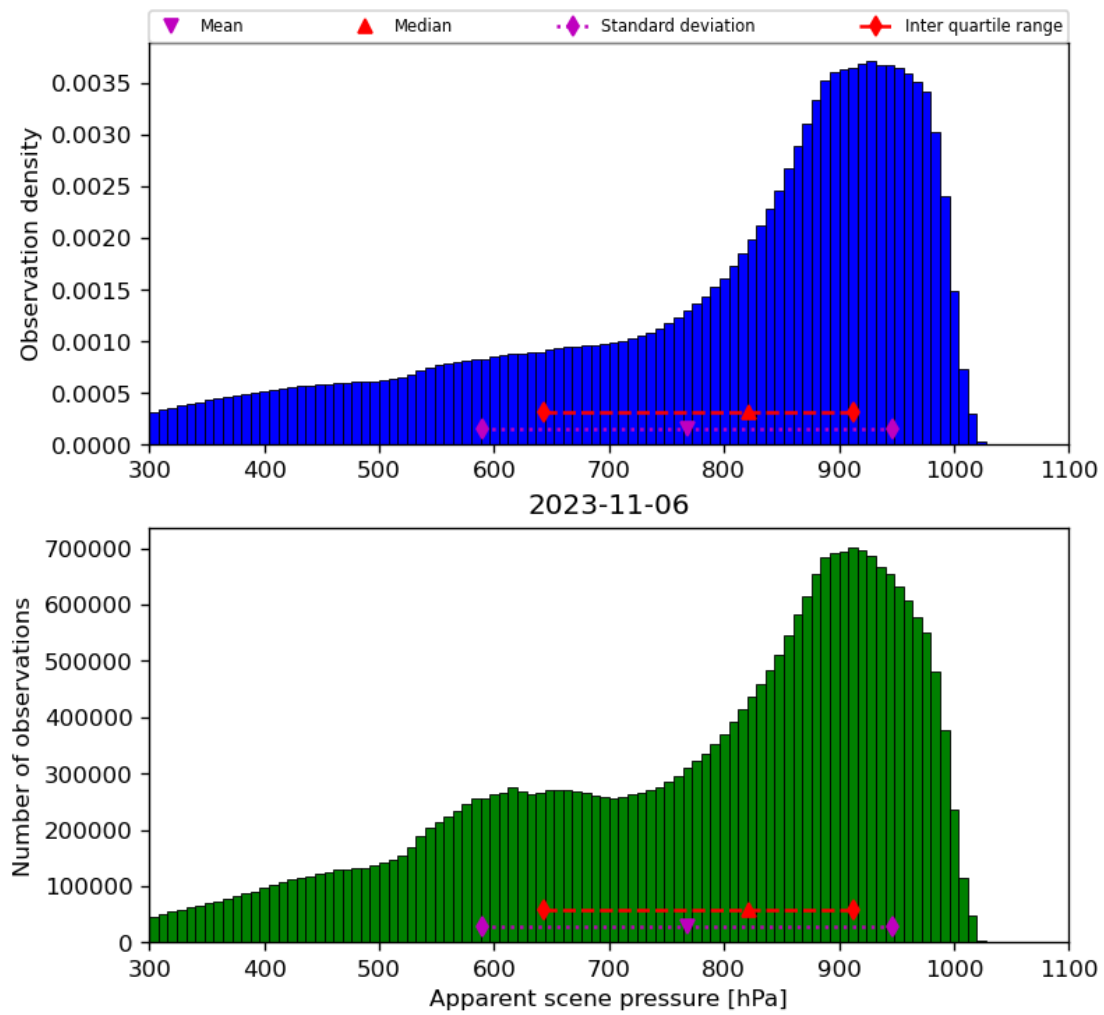
Figure 36: Histogram of “Apparent scene pressure” for 2023-11-05 to 2023-11-07
