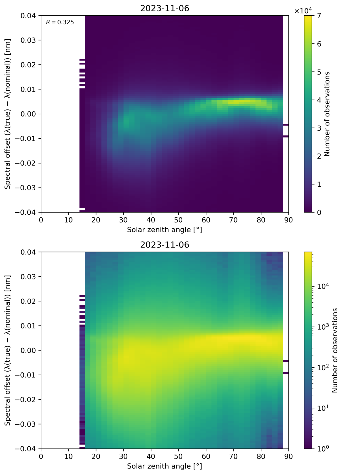
Figure 128: Scatter density plot of “Solar zenith angle” against “Spectral offset ( \lambda(\text{true}) - \lambda(\text{nominal}) )” for 2023-11-05 to 2023-11-07.
