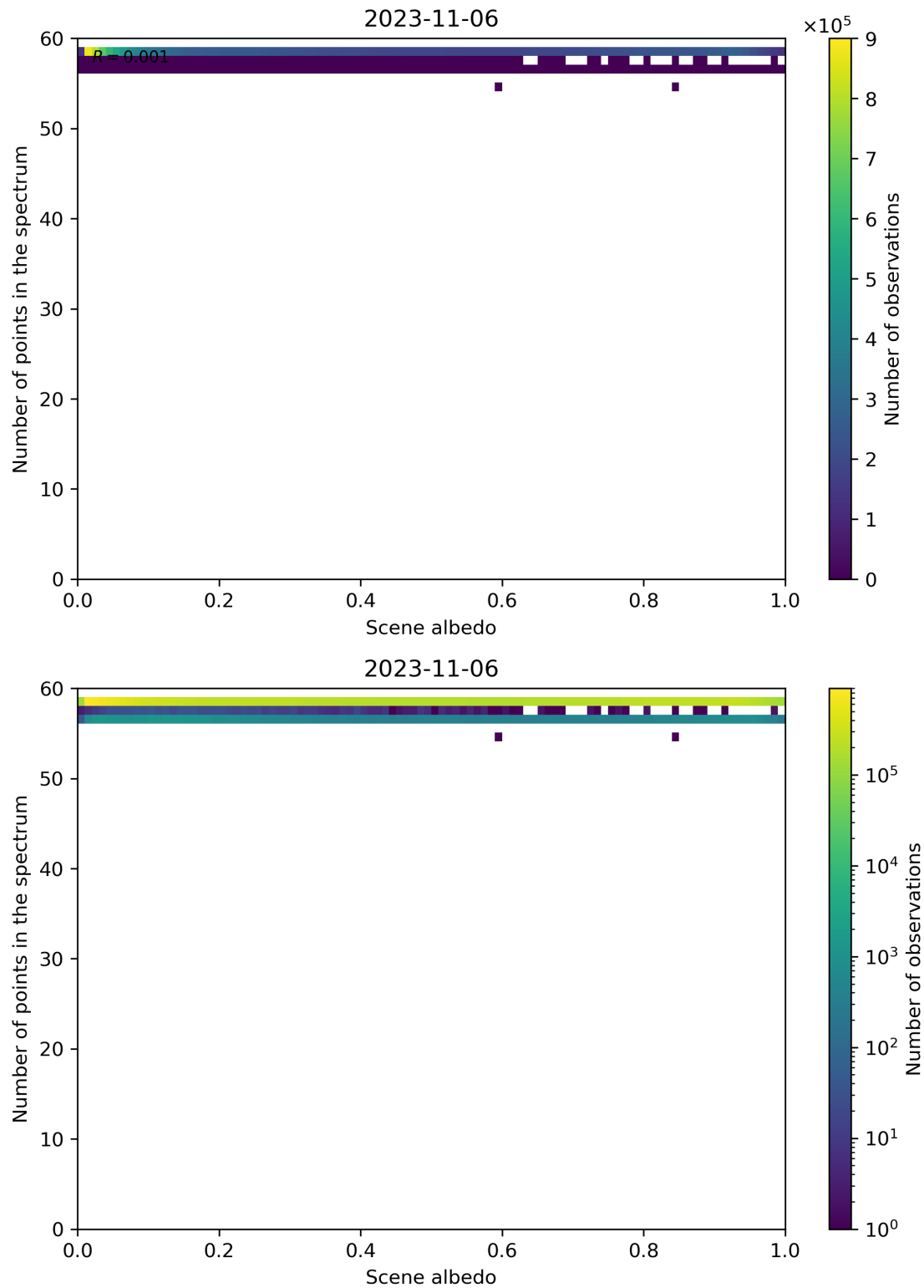
Figure 116: Scatter density plot of “Scene albedo” against “Number of points in the spectrum” for 2023-11-05 to 2023-11-07.
