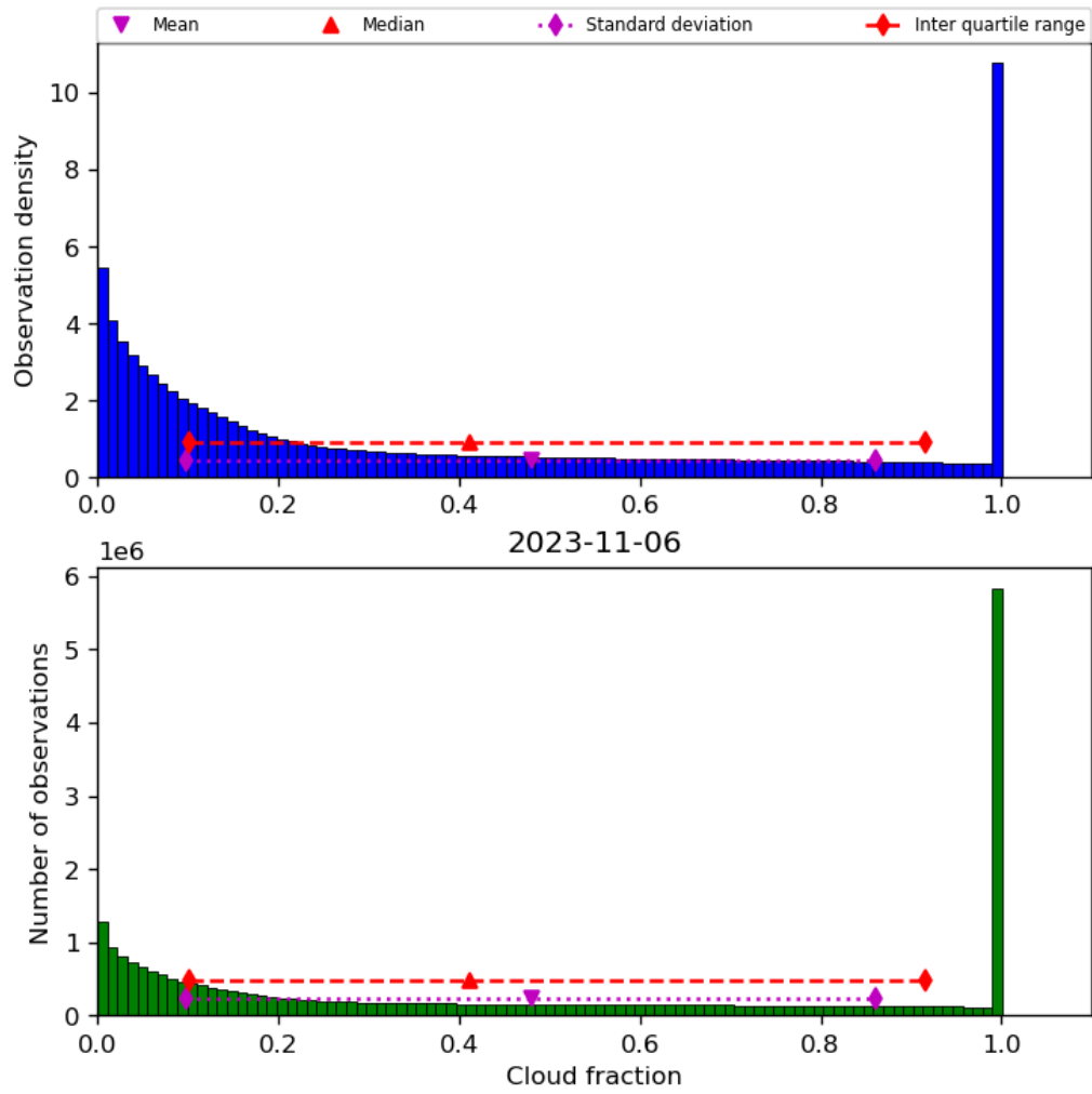
Figure 32: Histogram of “Cloud fraction” for 2023-11-05 to 2023-11-07
