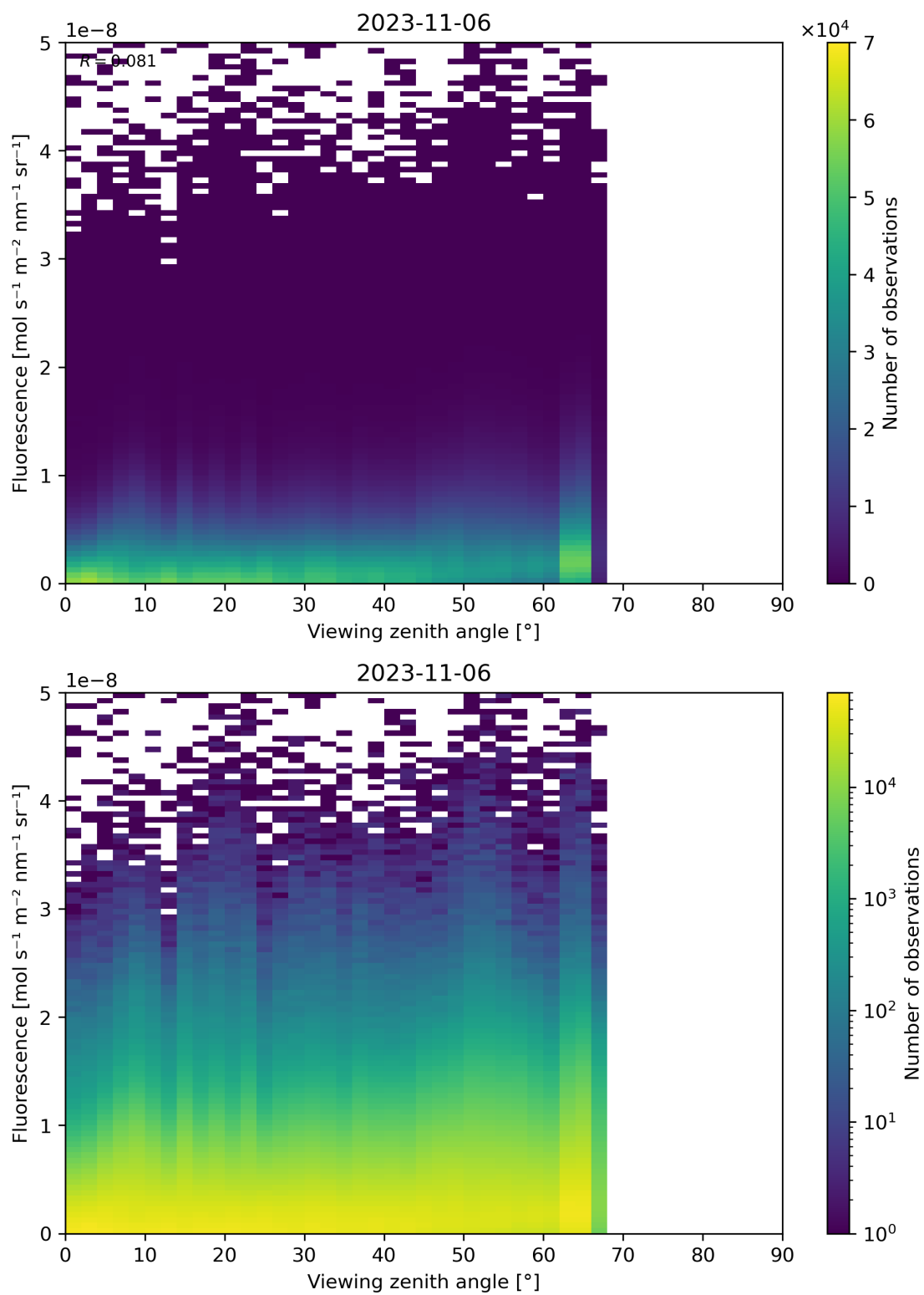
Figure 134: Scatter density plot of “Viewing zenith angle” against “Fluorescence” for 2023-11-05 to 2023-11-07.
