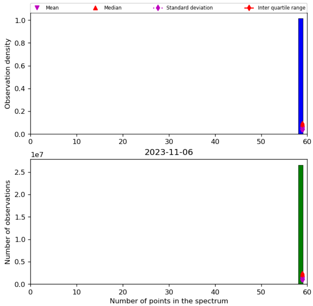
Figure 44: Histogram of "Number of points in the spectrum" for 2023-11-05 to 2023-11-07
