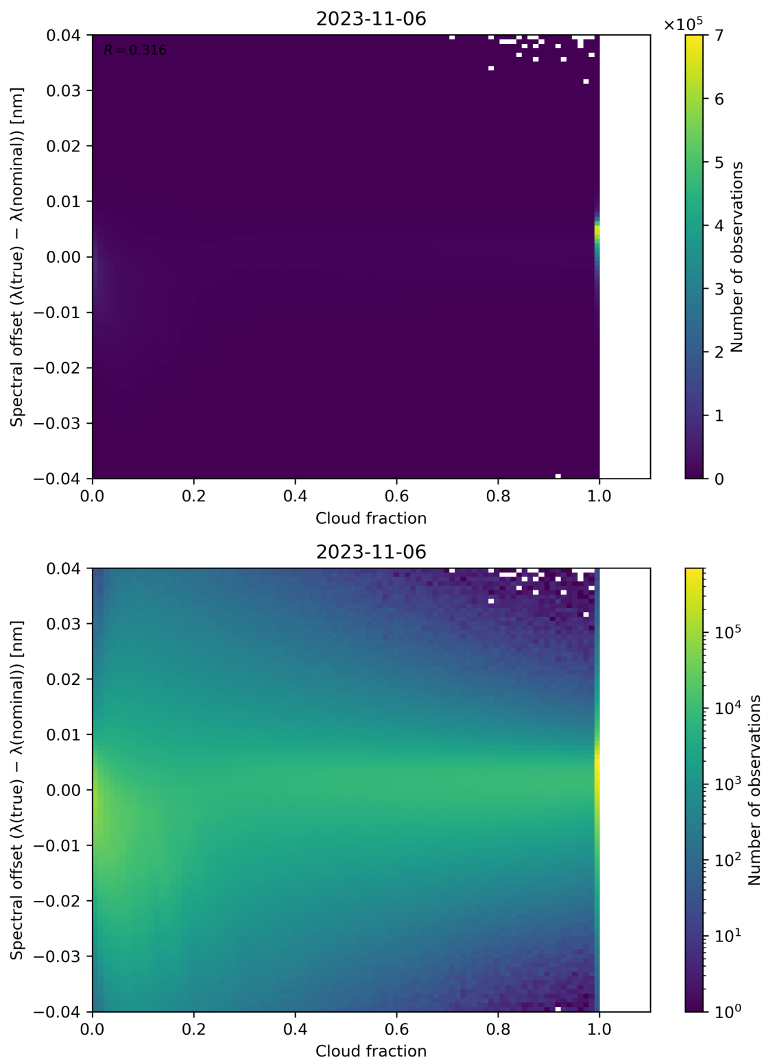
Figure 83: Scatter density plot of “Cloud fraction” against “Spectral offset ( \lambda(\text{true}) - \lambda(\text{nominal}) )” for 2023-11-05 to 2023-11-07.
