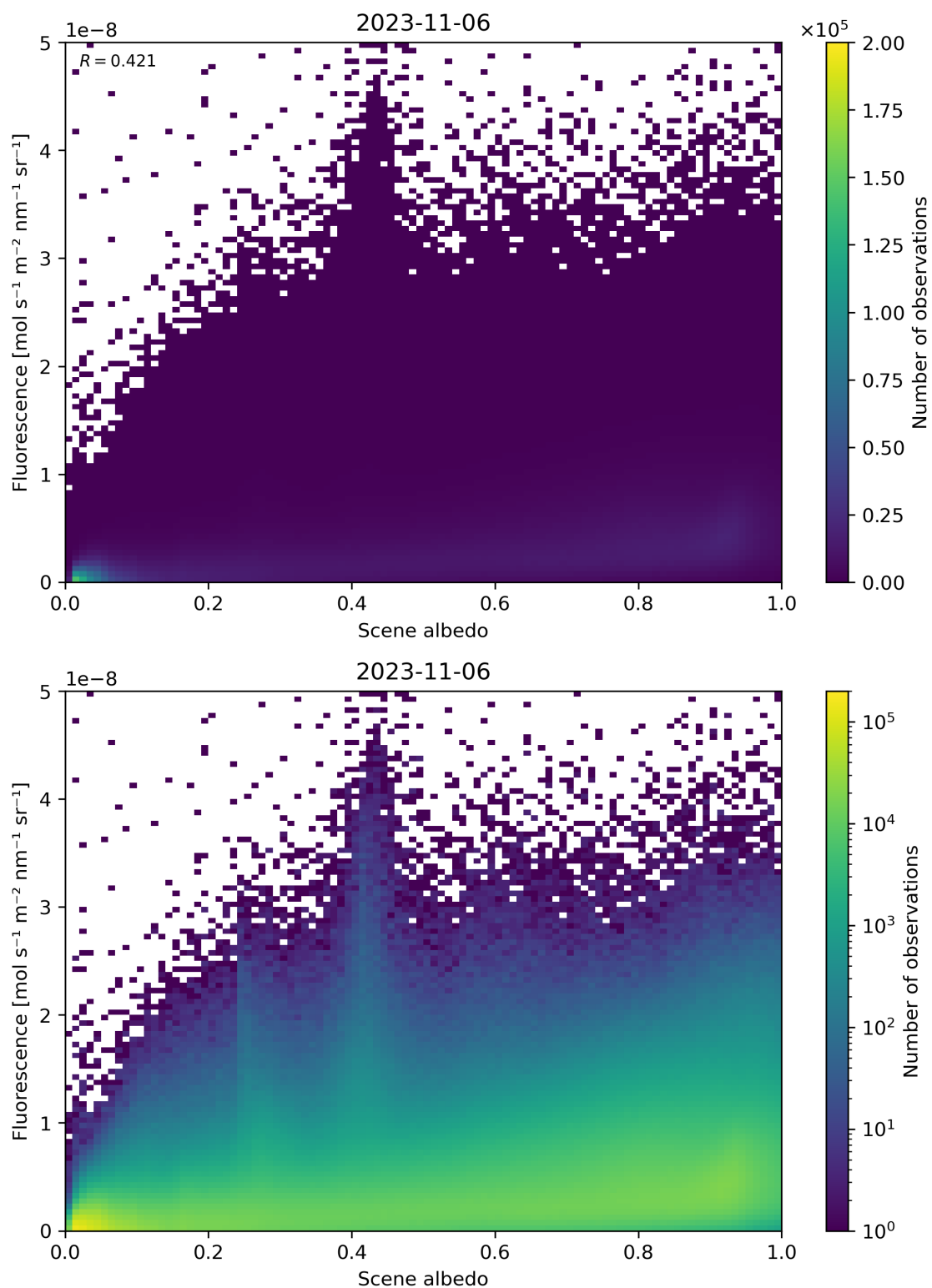
Figure 114: Scatter density plot of “Scene albedo” against “Fluorescence” for 2023-11-05 to 2023-11-07.
