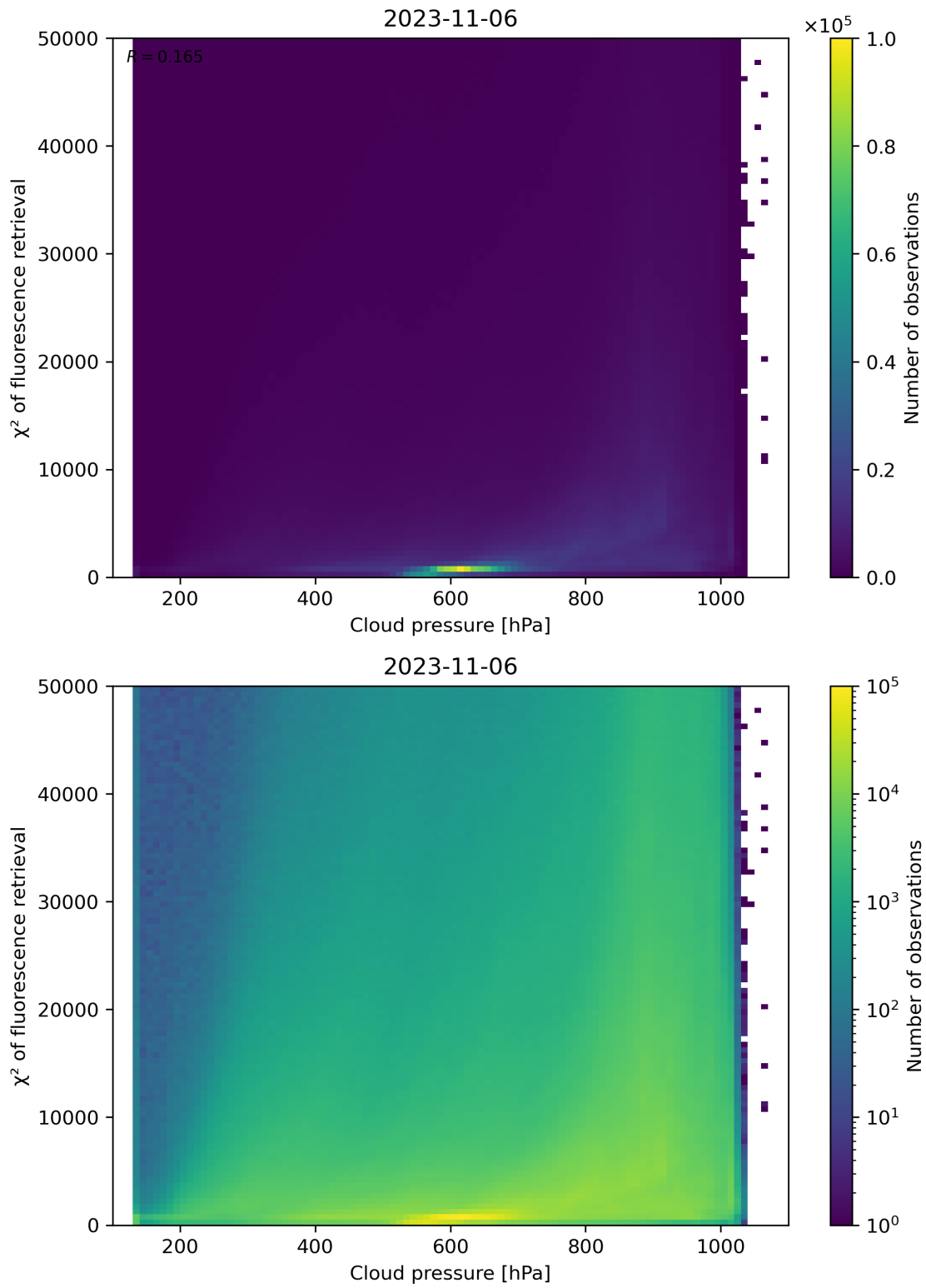
Figure 86: Scatter density plot of “Cloud pressure” against “ \chi^2 of fluorescence retrieval” for 2023-11-05 to 2023-11-07.
