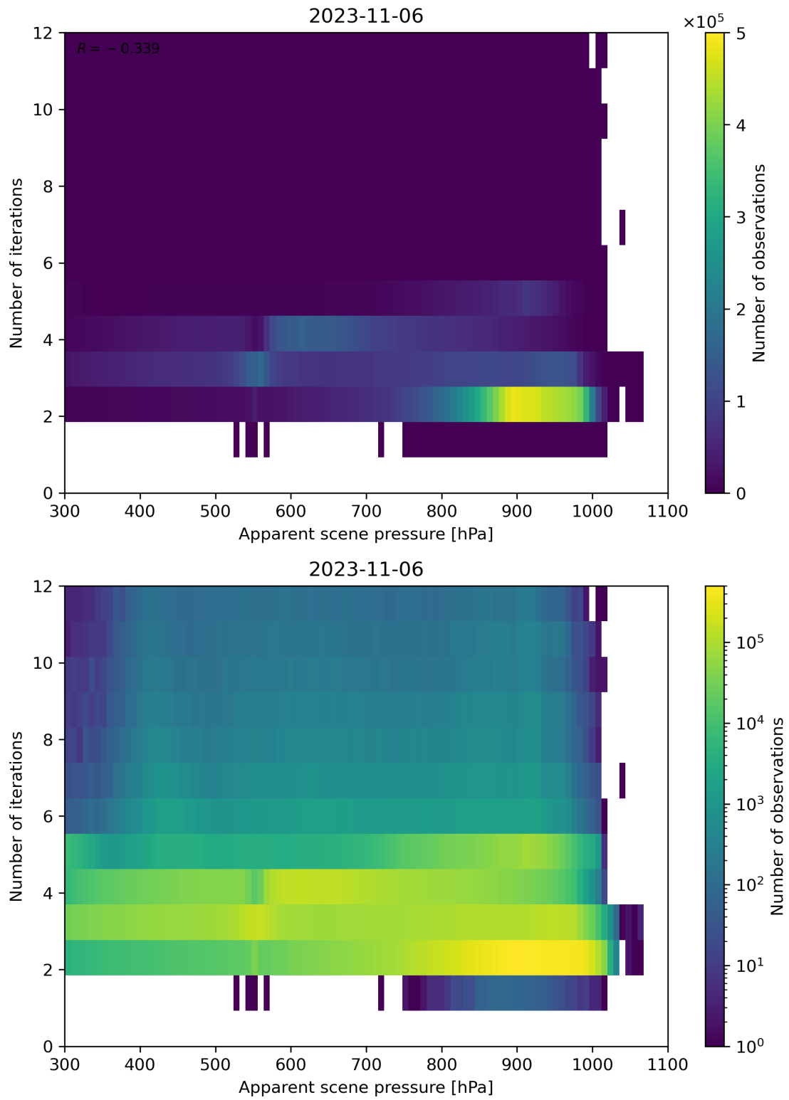
Figure 66: Scatter density plot of “Apparent scene pressure” against “Number of iterations” for 2023-11-05 to 2023-11-07.
