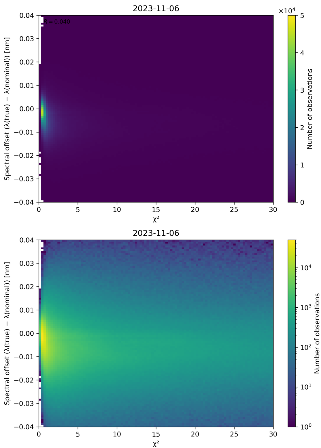
Figure 75: Scatter density plot of “ \chi^2 ” against “Spectral offset ( \lambda(\text{true}) - \lambda(\text{nominal}) )” for 2023-11-05 to 2023-11-07.
