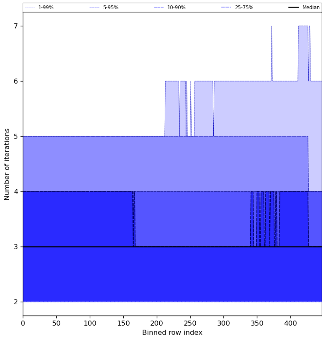
Figure 56: Along track statistics of “Number of iterations” for 2023-11-05 to 2023-11-07
