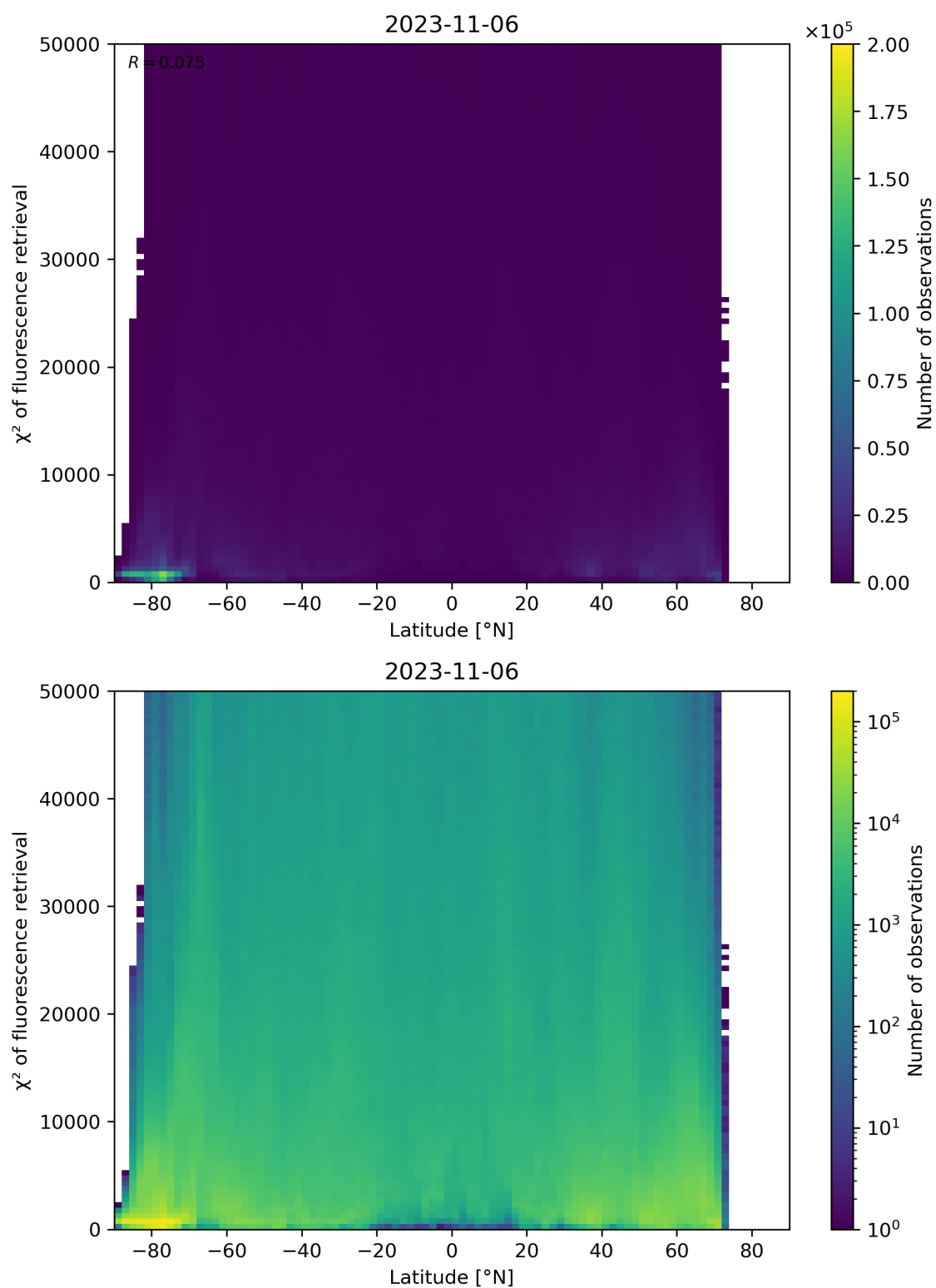
Figure 98: Scatter density plot of “Latitude” against “ \chi^2 of fluorescence retrieval” for 2023-11-05 to 2023-11-07.
