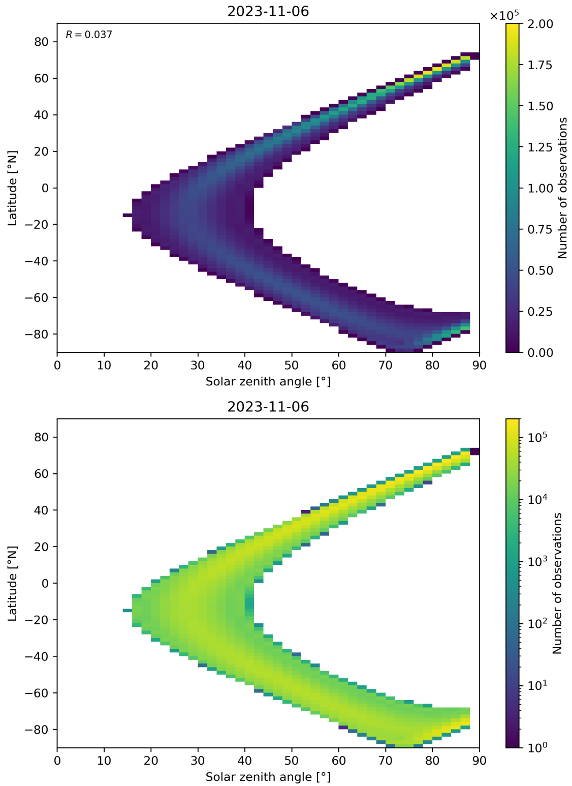
Figure 124: Scatter density plot of “Solar zenith angle” against “Latitude” for 2023-11-05 to 2023-11-07.
