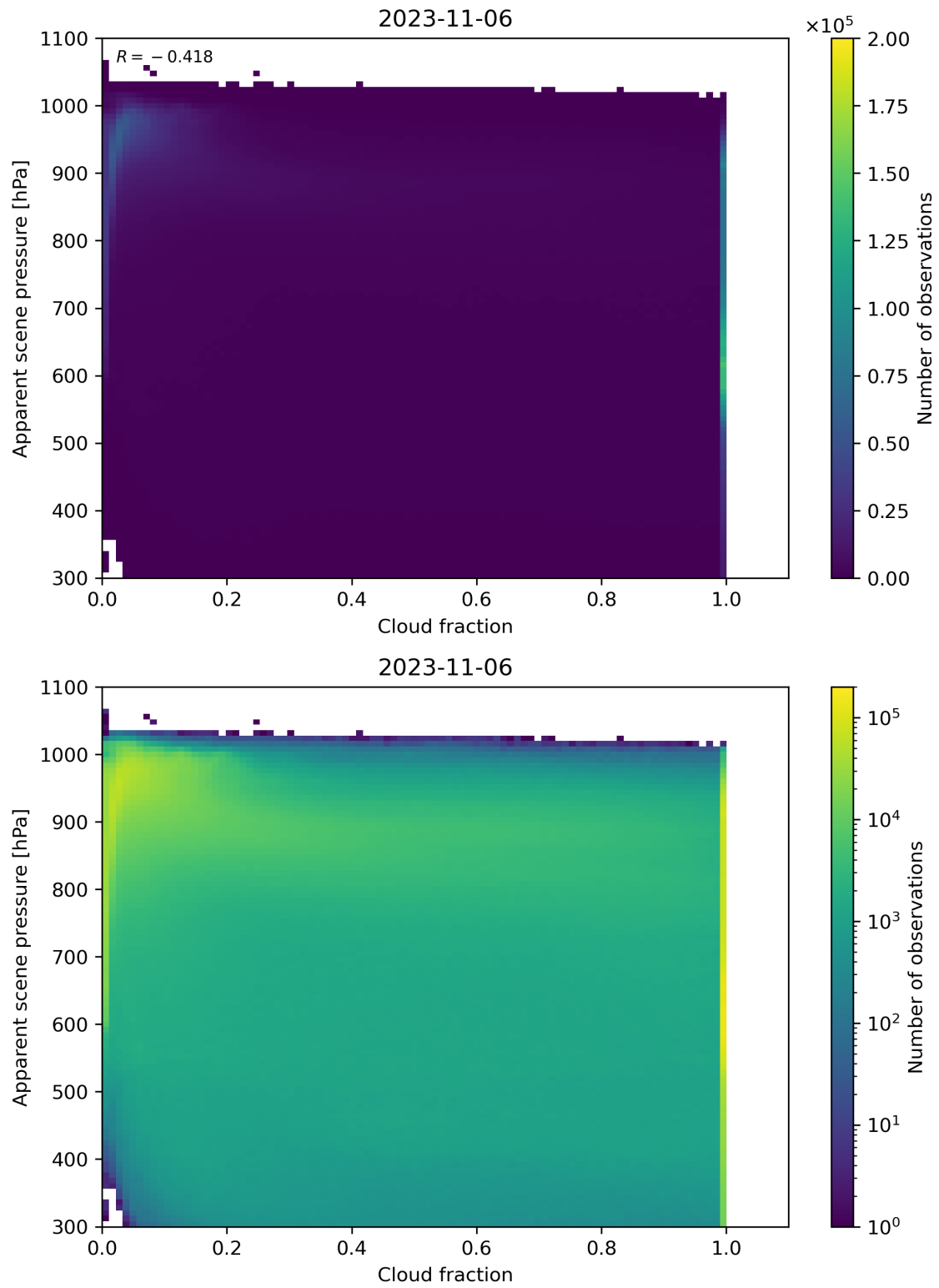
Figure 76: Scatter density plot of “Cloud fraction” against “Apparent scene pressure” for 2023-11-05 to 2023-11-07.
