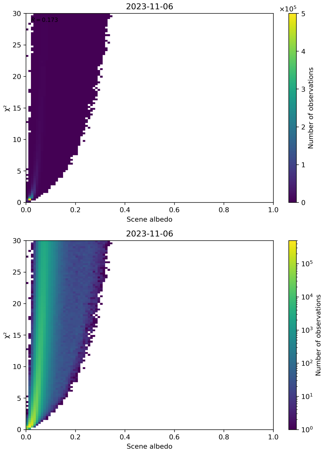
Figure 112: Scatter density plot of “Scene albedo” against “ \chi^2 ” for 2023-11-05 to 2023-11-07.
