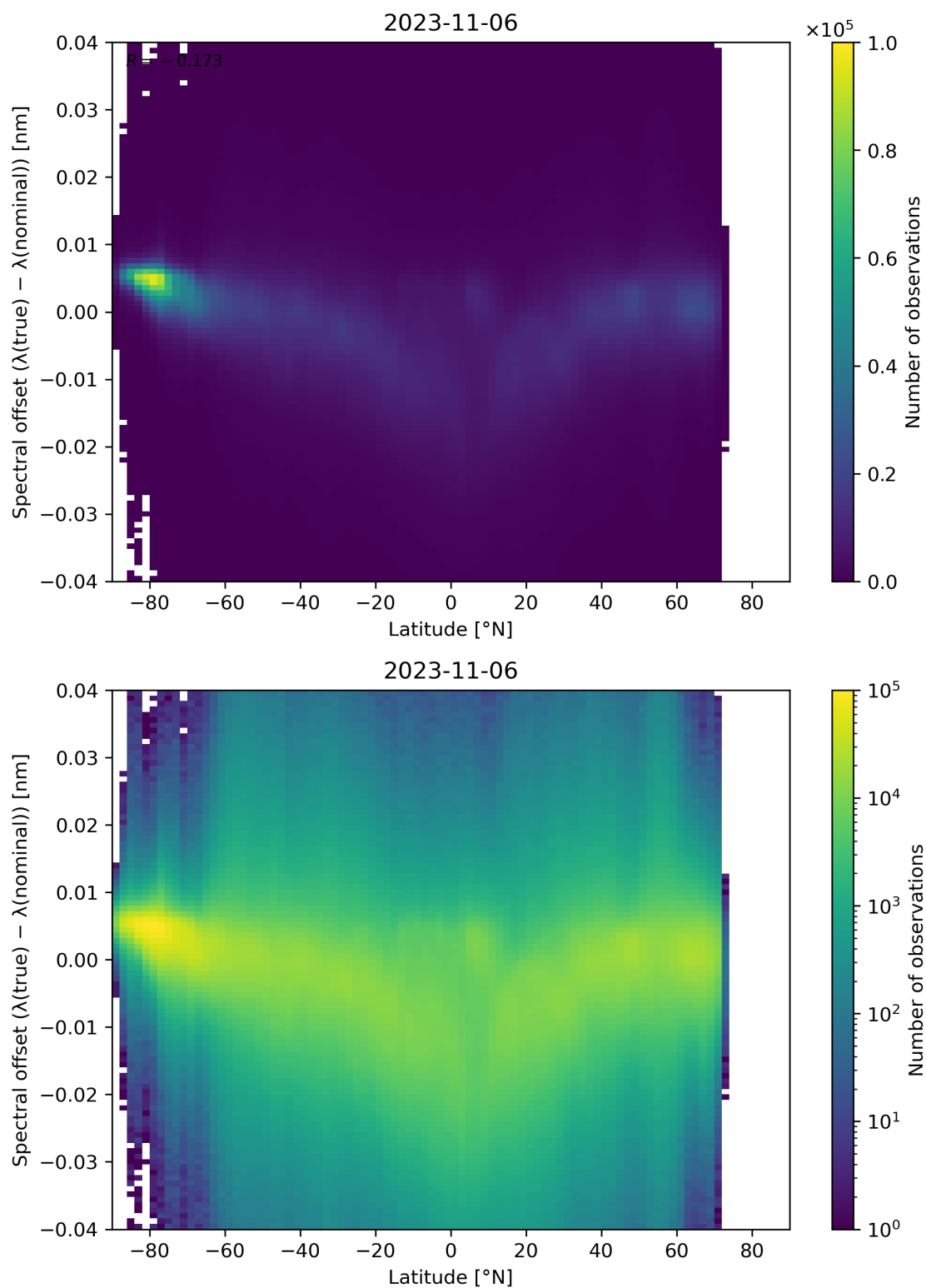
Figure 105: Scatter density plot of “Latitude” against “Spectral offset ( \lambda(\text{true}) - \lambda(\text{nominal}) )” for 2023-11-05 to 2023-11-07.
