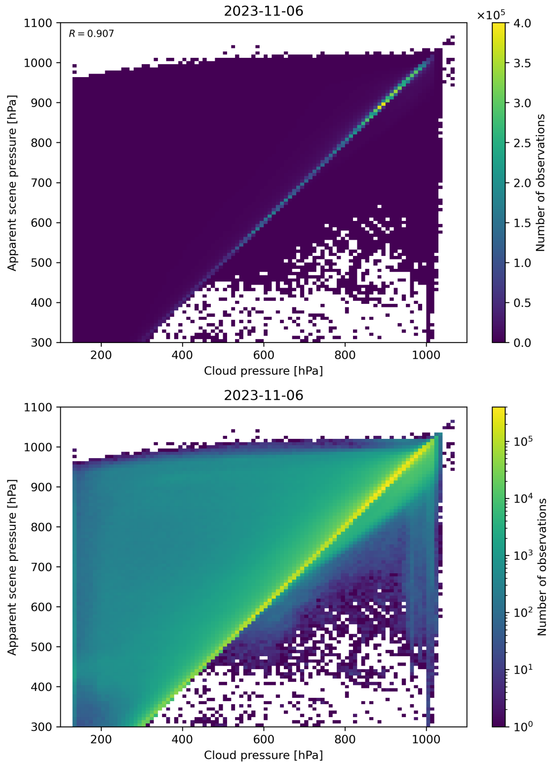
Figure 84: Scatter density plot of “Cloud pressure” against “Apparent scene pressure” for 2023-11-05 to 2023-11-07.
