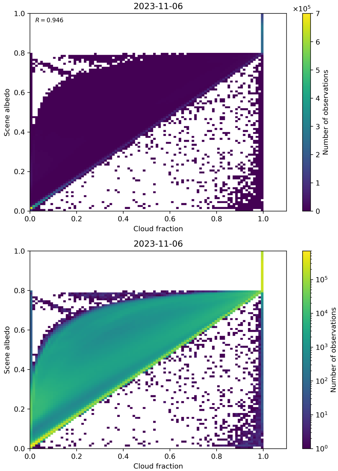
Figure 82: Scatter density plot of “Cloud fraction” against “Scene albedo” for 2023-11-05 to 2023-11-07.
