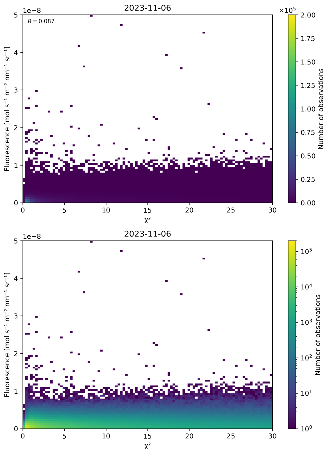
Figure 70: Scatter density plot of “ \chi^2 ” against “Fluorescence” for 2023-11-05 to 2023-11-07.
