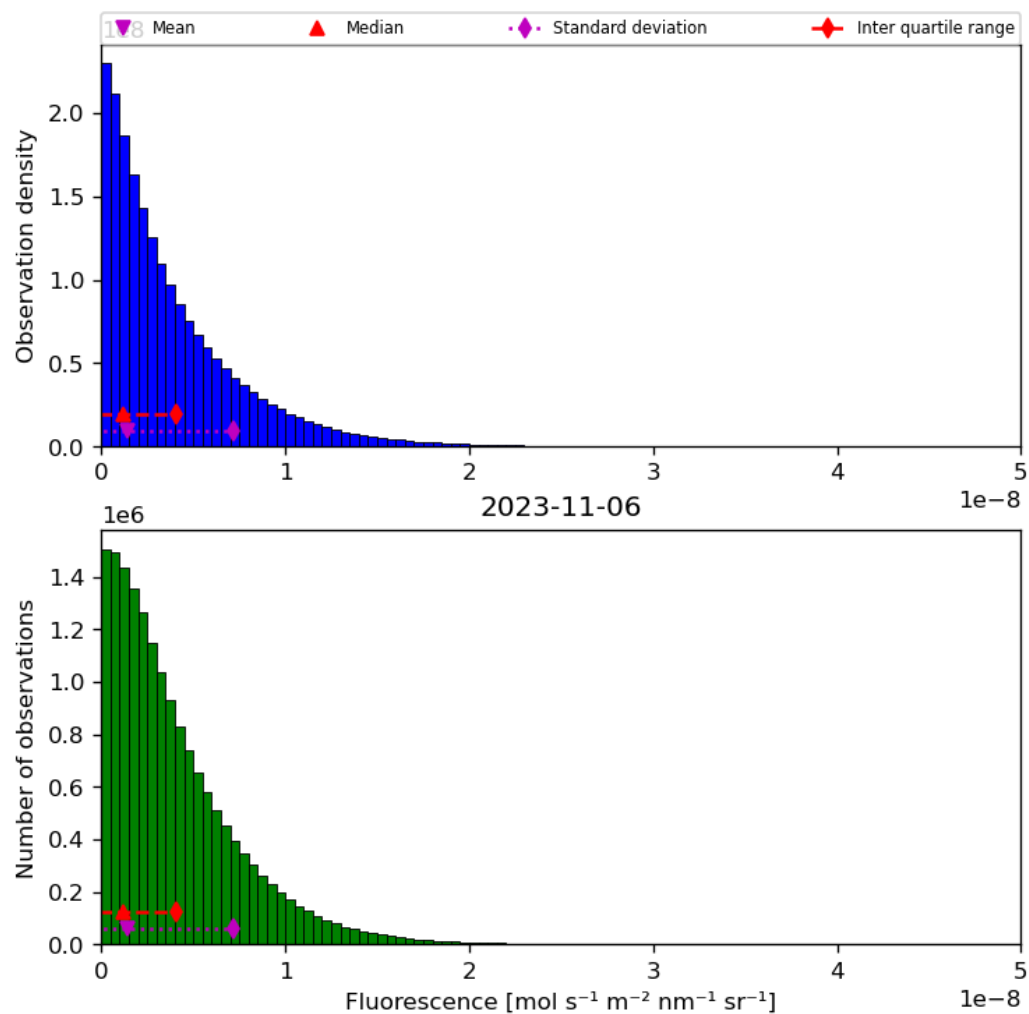
Figure 40: Histogram of “Fluorescence” for 2023-11-05 to 2023-11-07
