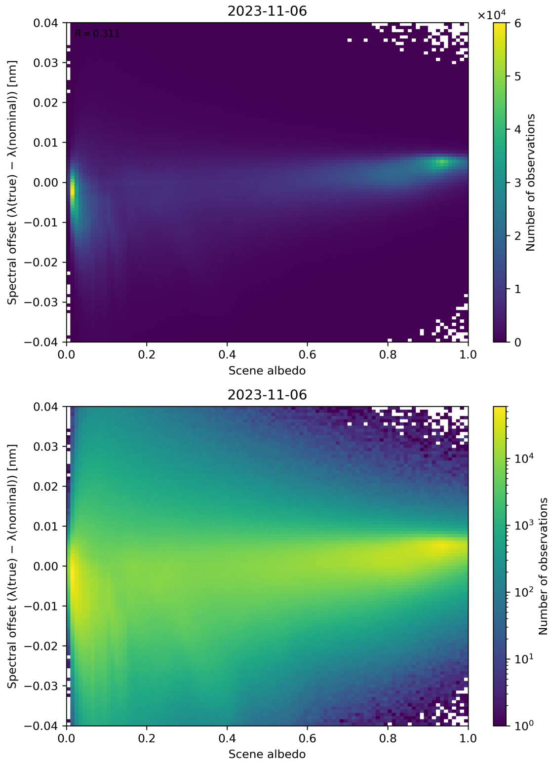
Figure 117: Scatter density plot of “Scene albedo” against “Spectral offset ( \lambda(\text{true}) - \lambda(\text{nominal}) )” for 2023-11-05 to 2023-11-07.
