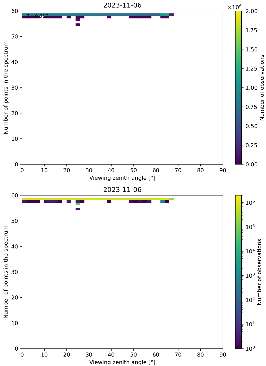
Figure 137: Scatter density plot of “Viewing zenith angle” against “Number of points in the spectrum” for 2023-11-05 to 2023-11-07.
