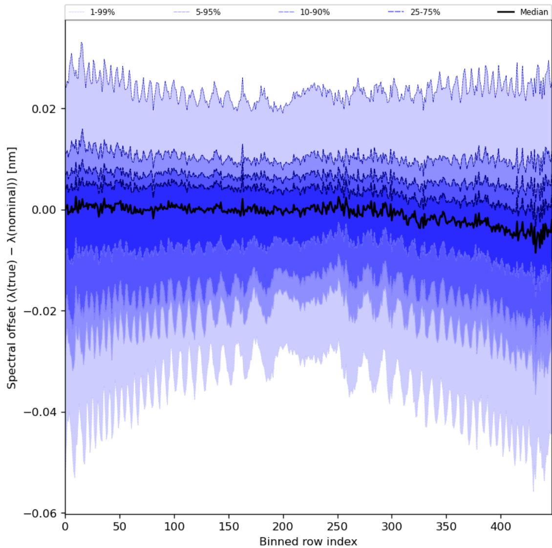
Figure 62: Along track statistics of “Spectral offset ( \lambda(\text{true}) - \lambda(\text{nominal}) )” for 2023-11-05 to 2023-11-07
