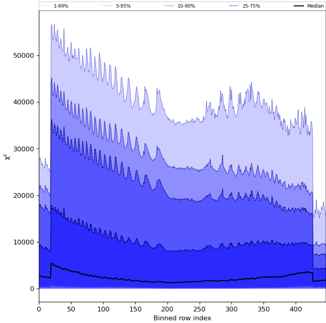
Figure 55: Along track statistics of “ \chi^2 ” for 2023-11-05 to 2023-11-07
