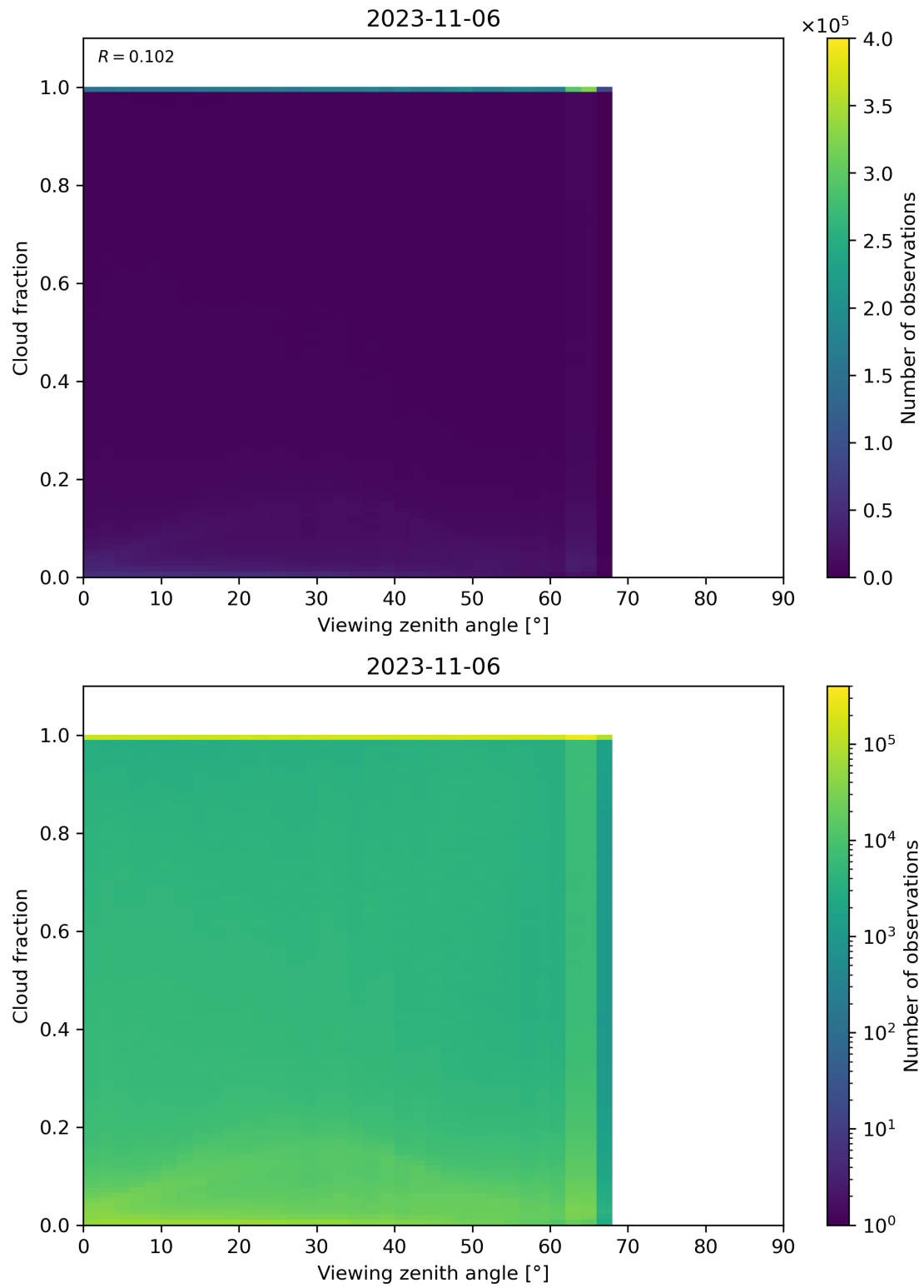
Figure 132: Scatter density plot of “Viewing zenith angle” against “Cloud fraction” for 2023-11-05 to 2023-11-07.
