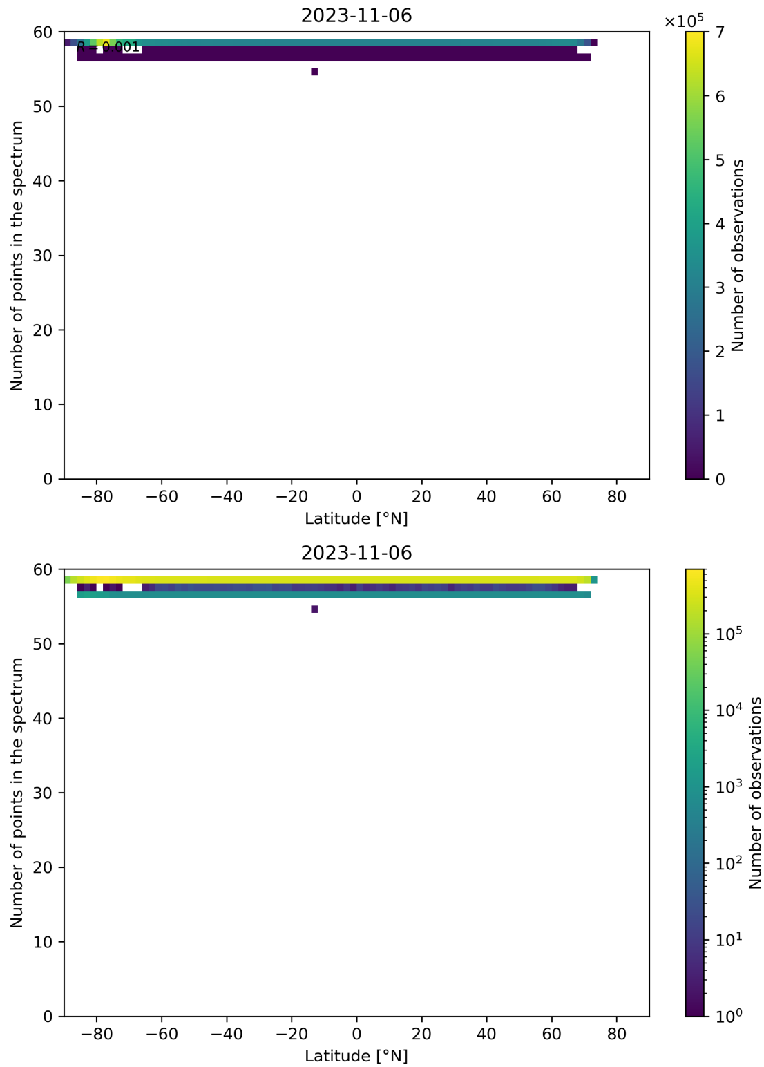
Figure 103: Scatter density plot of “Latitude” against “Number of points in the spectrum” for 2023-11-05 to 2023-11-07.
