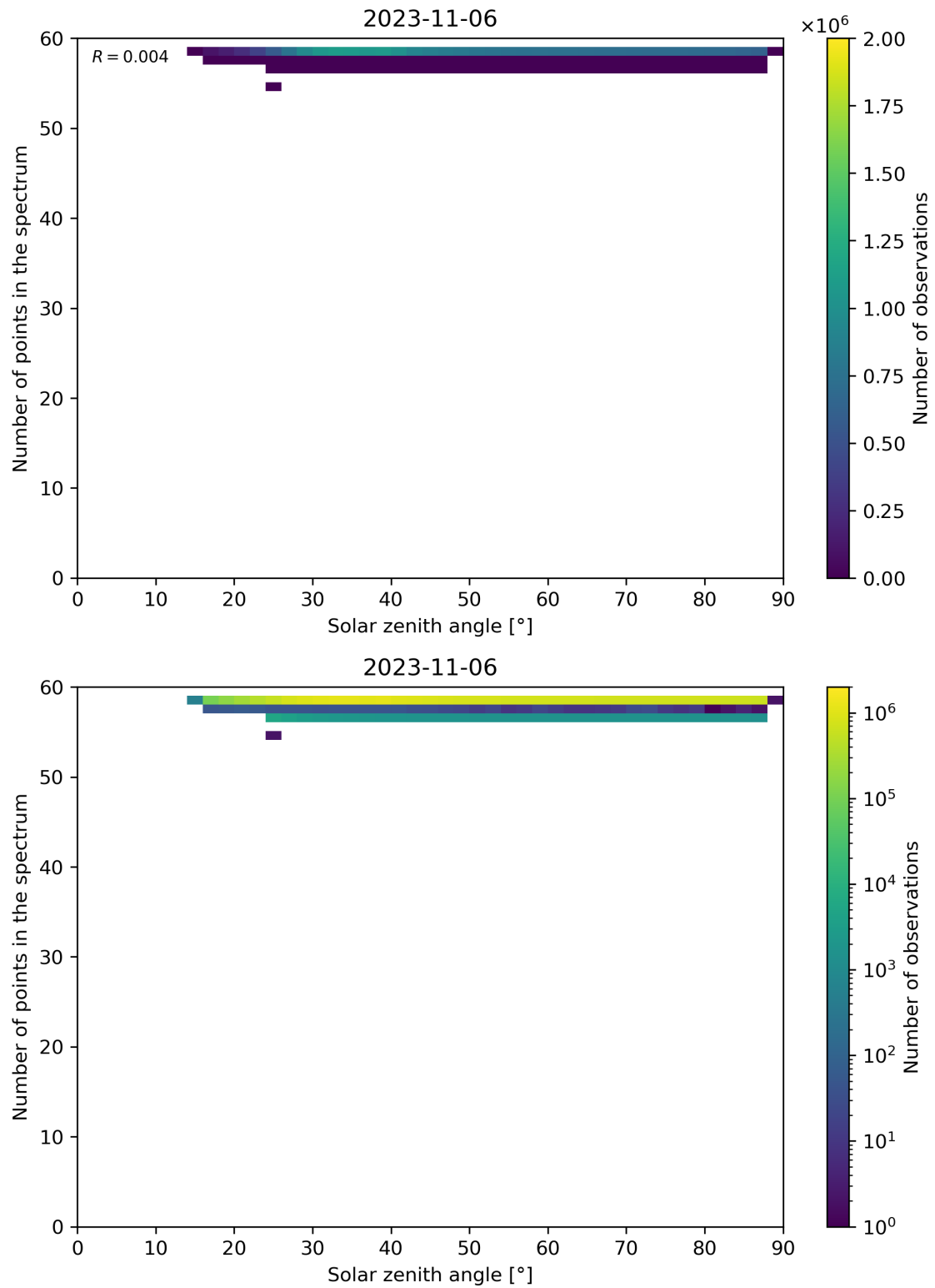
Figure 126: Scatter density plot of “Solar zenith angle” against “Number of points in the spectrum” for 2023-11-05 to 2023-11-07.
