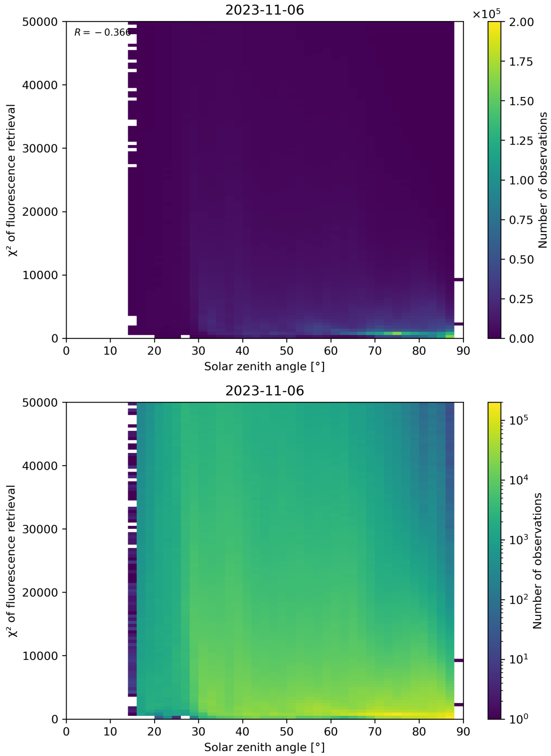
Figure 120: Scatter density plot of “Solar zenith angle” against “ \chi^2 of fluorescence retrieval” for 2023-11-05 to 2023-11-07.
