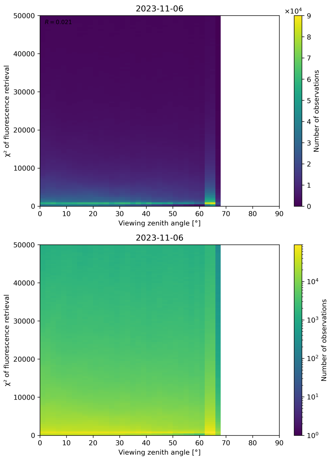
Figure 131: Scatter density plot of “Viewing zenith angle” against “ \chi^2 of fluorescence retrieval” for 2023-11-05 to 2023-11-07.
