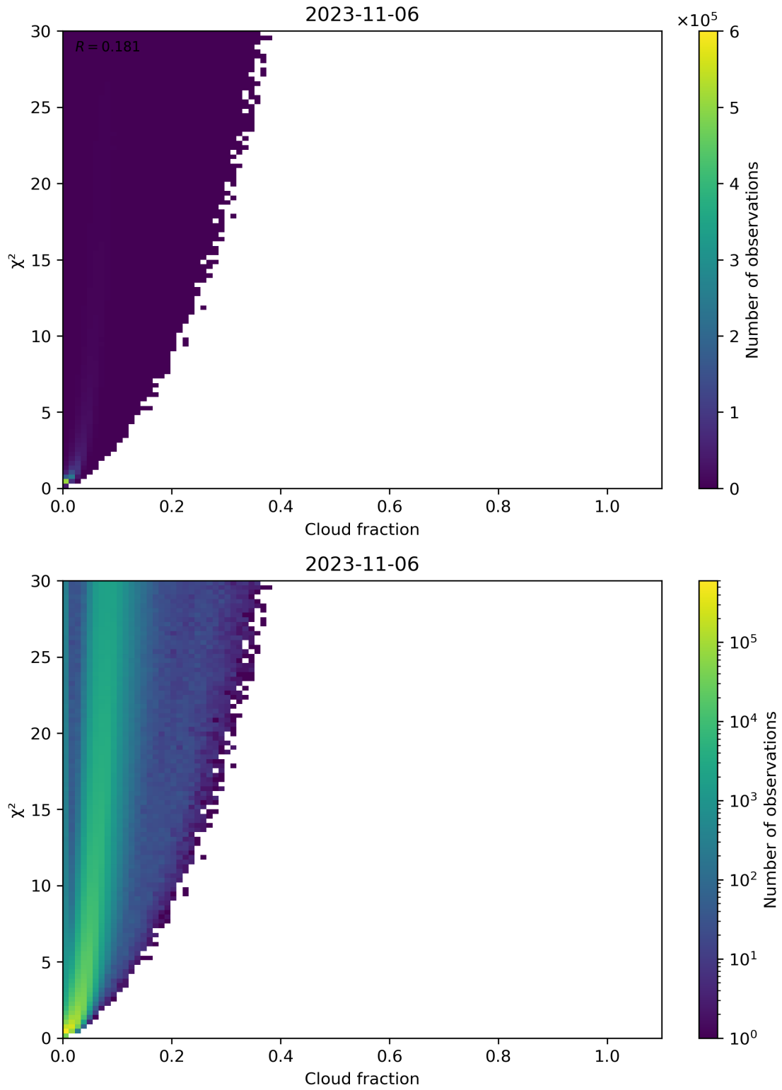
Figure 77: Scatter density plot of “Cloud fraction” against “ \chi^2 ” for 2023-11-05 to 2023-11-07.
