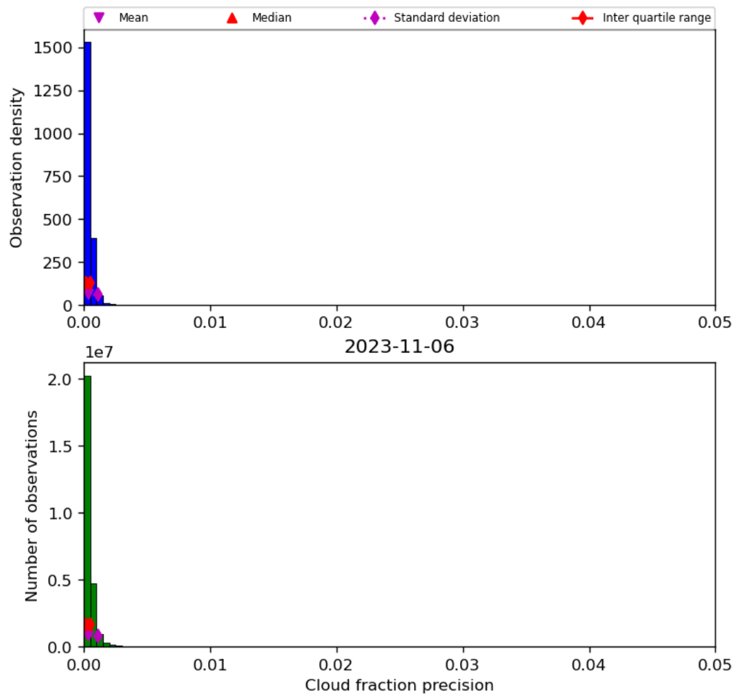
Figure 33: Histogram of “Cloud fraction precision” for 2023-11-05 to 2023-11-07
