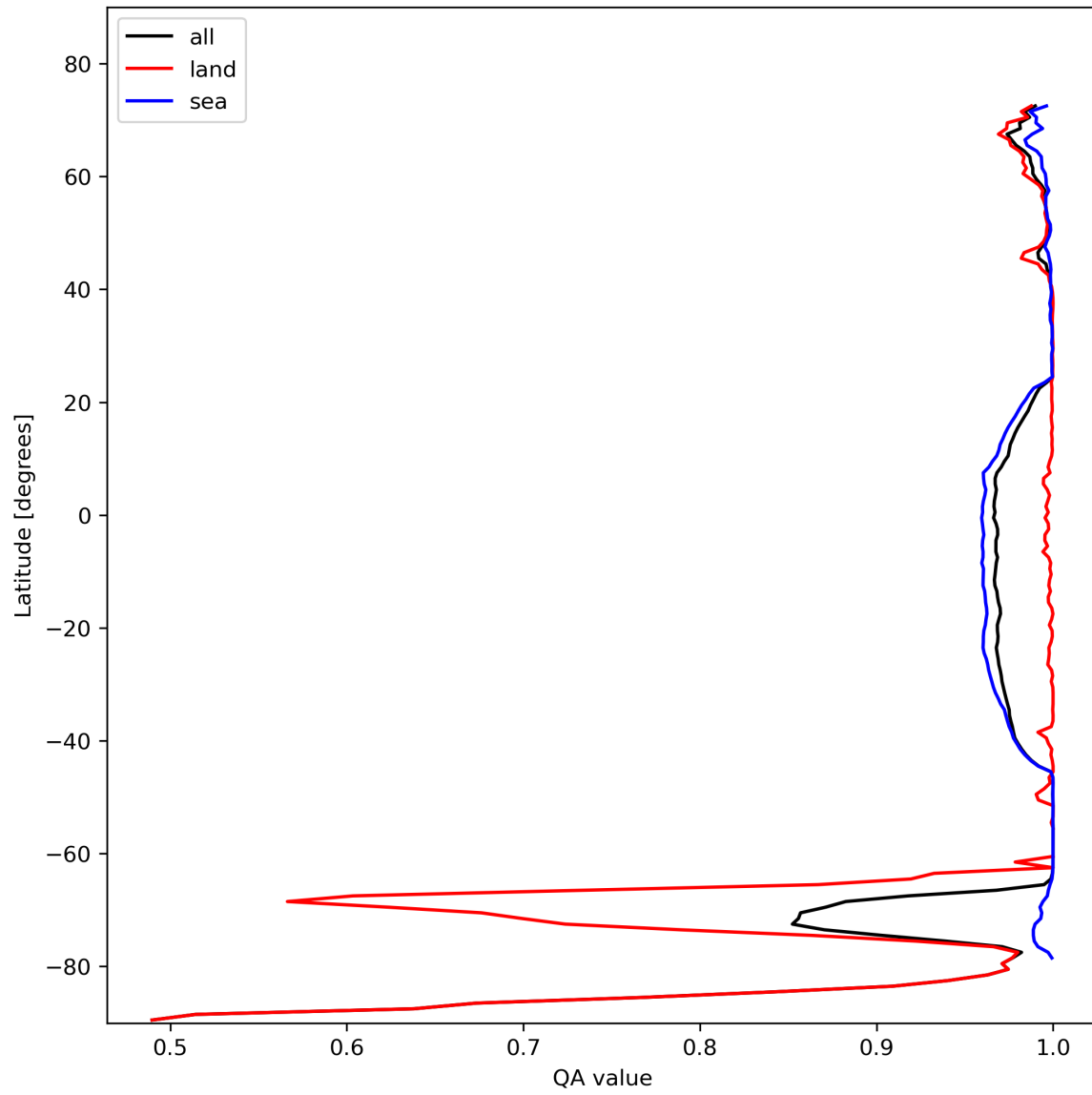
Figure 12: Zonal average of “QA value” for 2023-11-05 to 2023-11-07.
