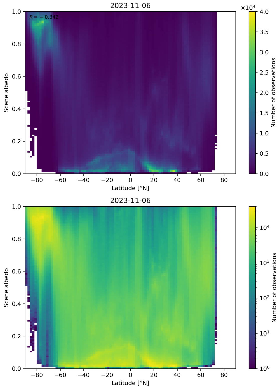
Figure 104: Scatter density plot of “Latitude” against “Scene albedo” for 2023-11-05 to 2023-11-07.
