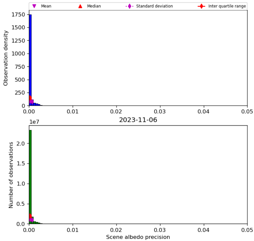
Figure 35: Histogram of “Scene albedo precision” for 2023-11-05 to 2023-11-07
