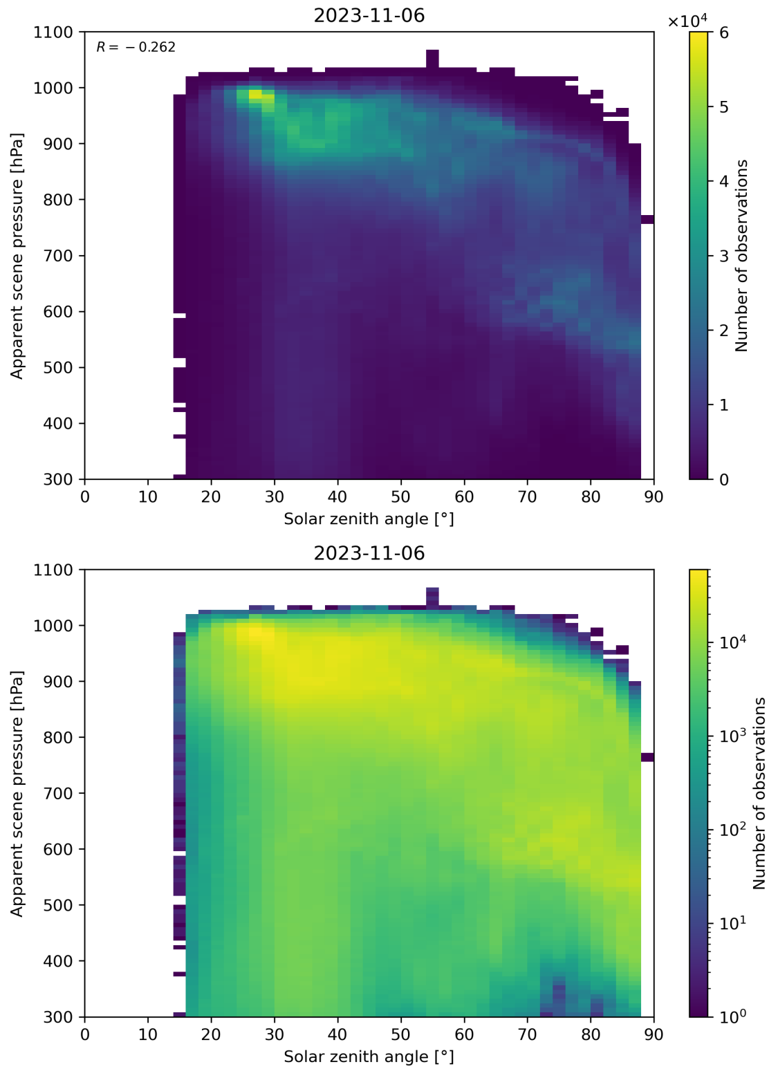
Figure 118: Scatter density plot of “Solar zenith angle” against “Apparent scene pressure” for 2023-11-05 to 2023-11-07.
