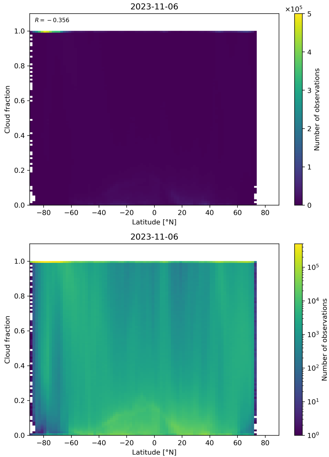
Figure 99: Scatter density plot of “Latitude” against “Cloud fraction” for 2023-11-05 to 2023-11-07.
