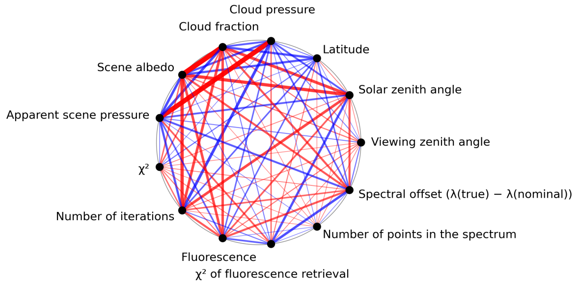
Figure 1: Map of correlation graph for 2023-11-05 to 2023-11-07.
