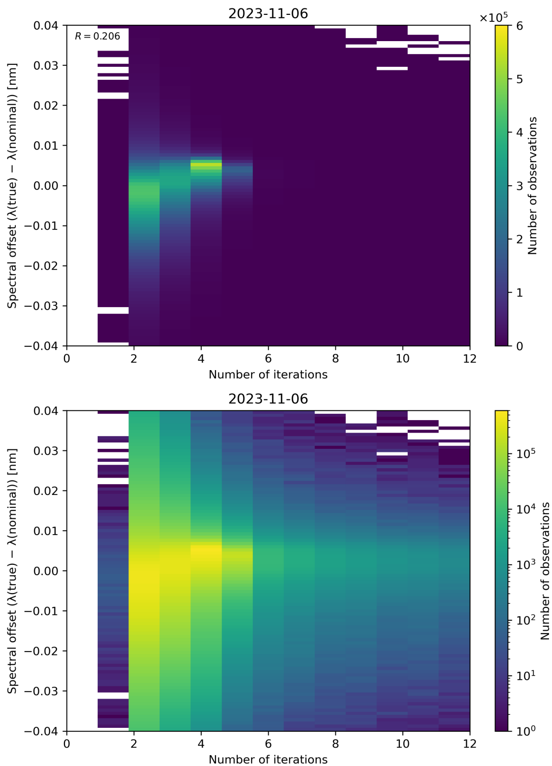
Figure 109: Scatter density plot of “Number of iterations” against “Spectral offset ( \lambda(\text{true}) - \lambda(\text{nominal}) )” for 2023-11-05 to 2023-11-07.
