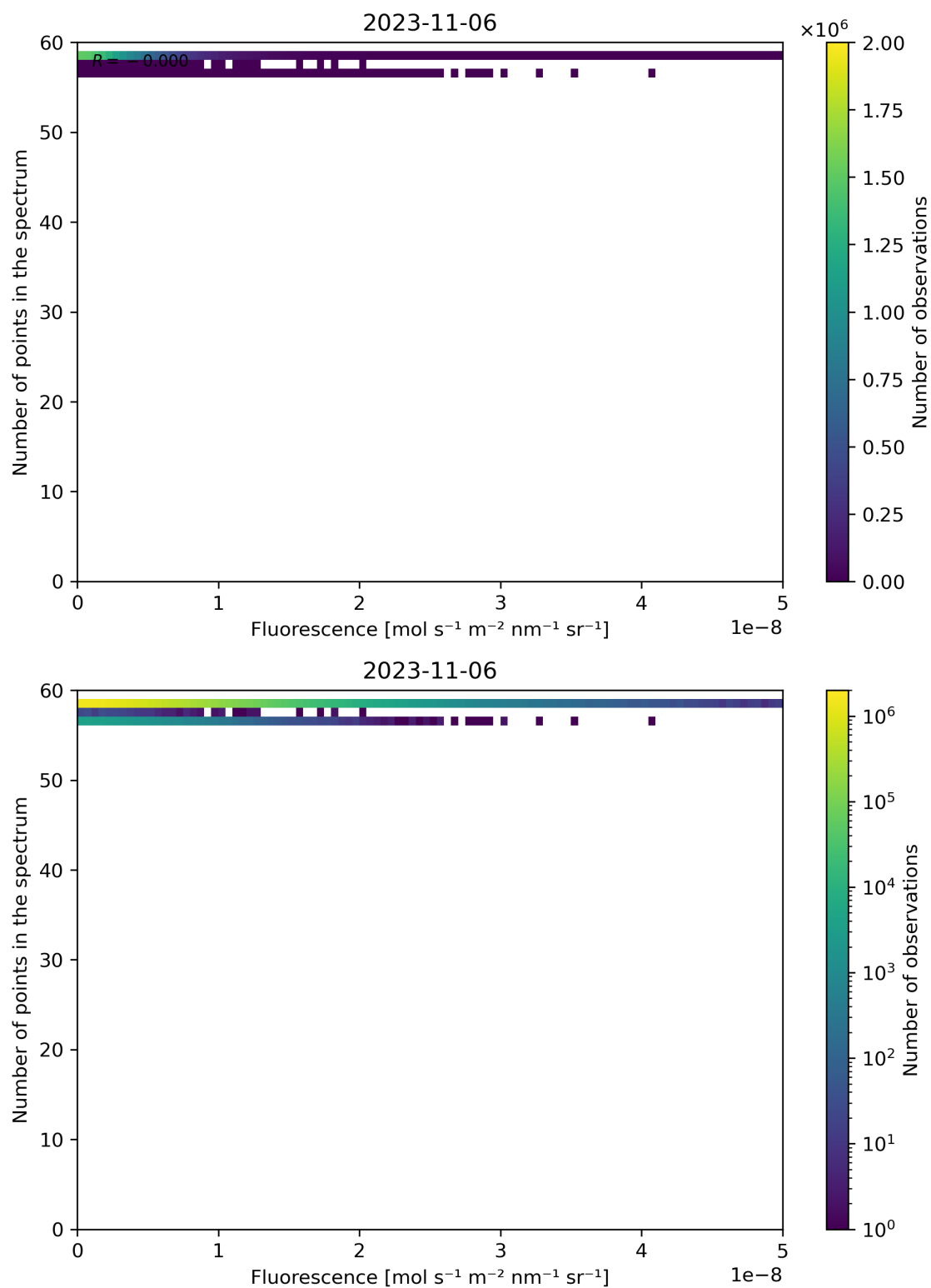
Figure 94: Scatter density plot of “Fluorescence” against “Number of points in the spectrum” for 2023-11-05 to 2023-11-07.
