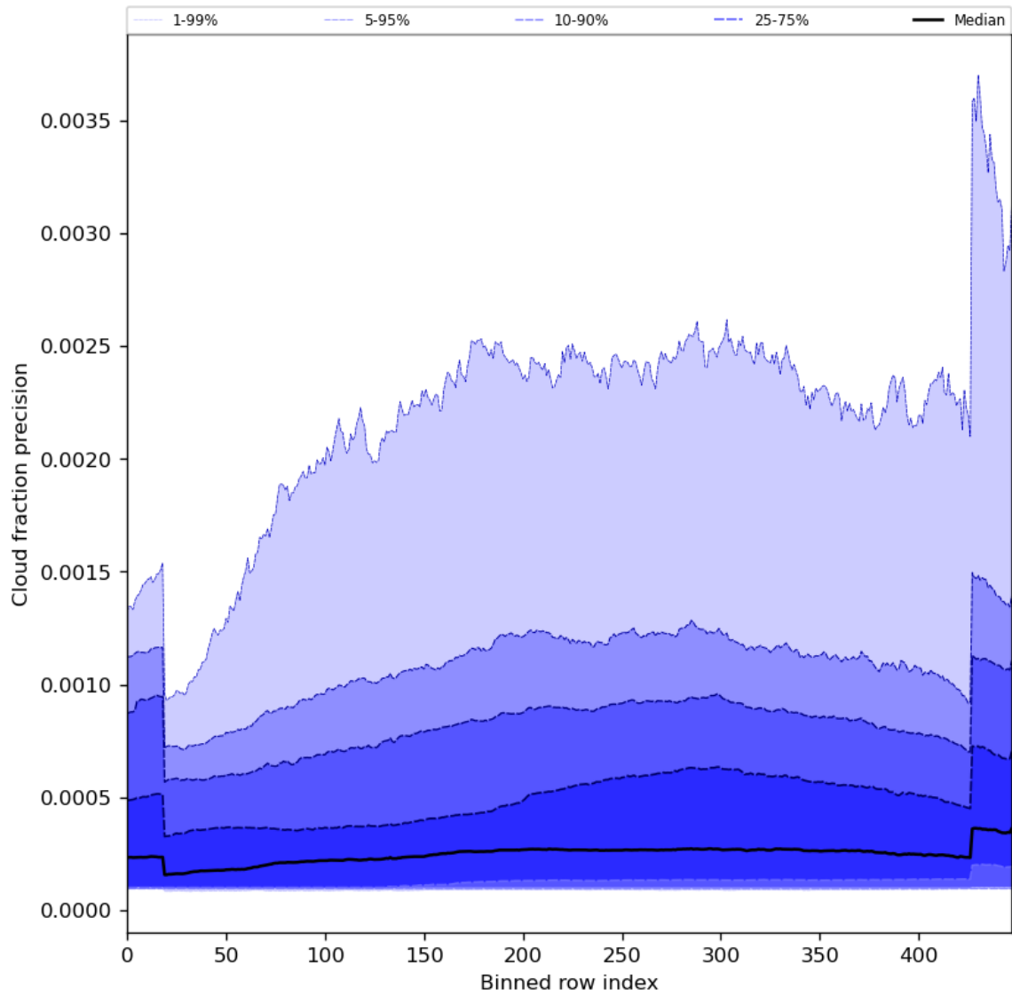
Figure 50: Along track statistics of “Cloud fraction precision” for 2023-11-05 to 2023-11-07
