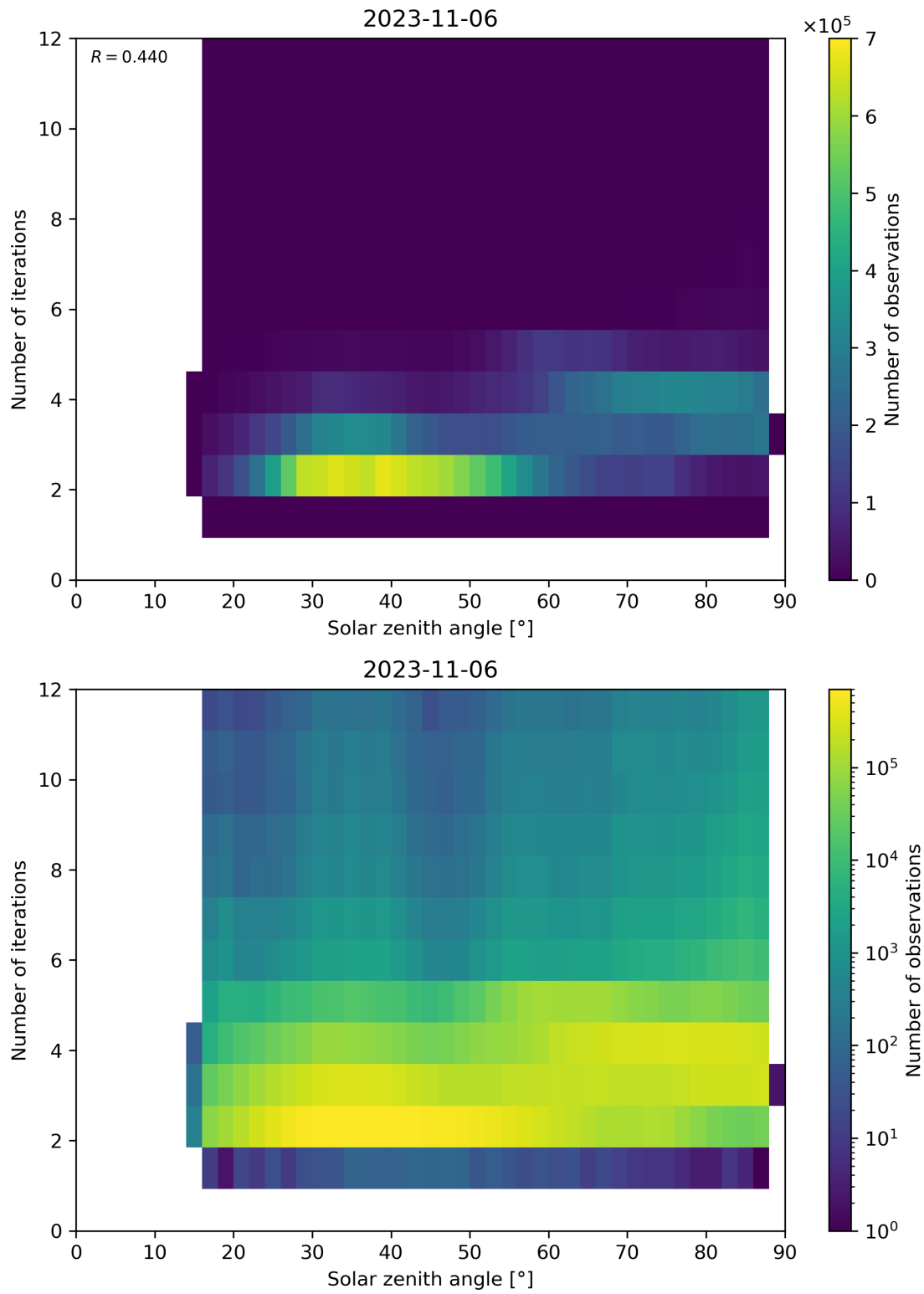
Figure 125: Scatter density plot of “Solar zenith angle” against “Number of iterations” for 2023-11-05 to 2023-11-07.
