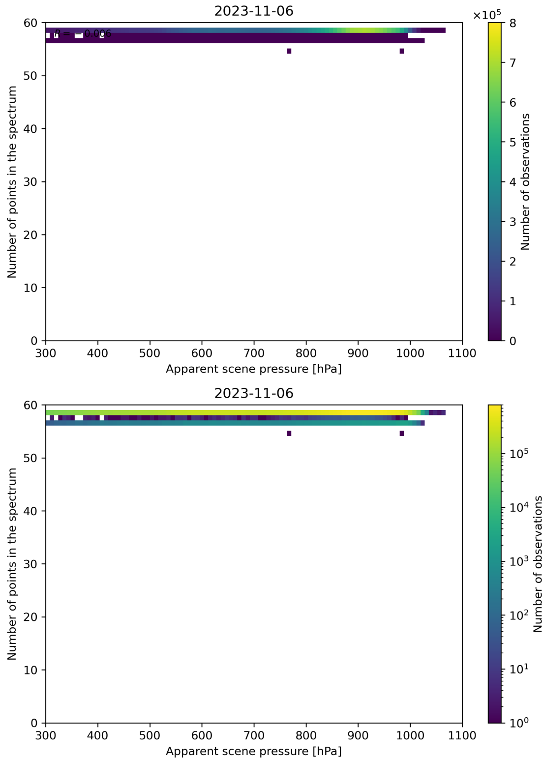
Figure 67: Scatter density plot of “Apparent scene pressure” against “Number of points in the spectrum” for 2023-11-05 to 2023-11-07.
