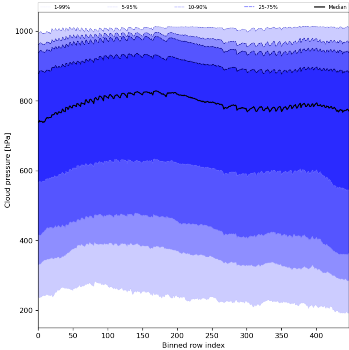
Figure 47: Along track statistics of “Cloud pressure” for 2023-11-05 to 2023-11-07
