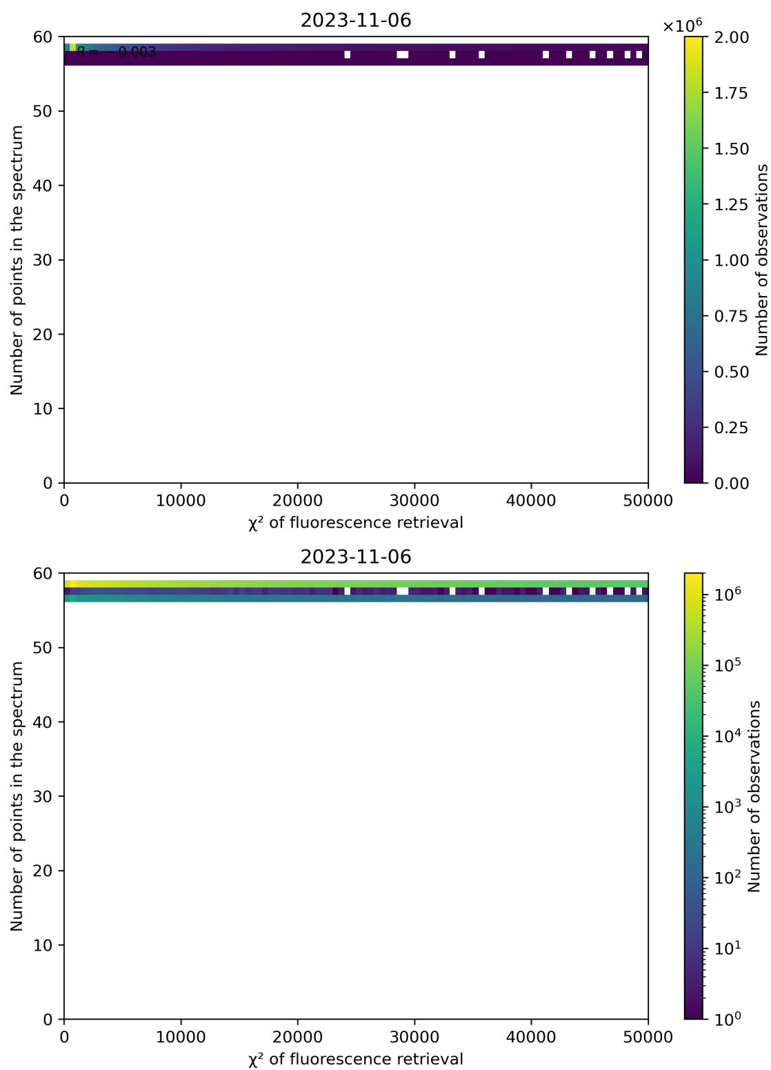
Figure 71: Scatter density plot of " \chi^2 of fluorescence retrieval" against "Number of points in the spectrum" for 2023-11-05 to 2023-11-07.
