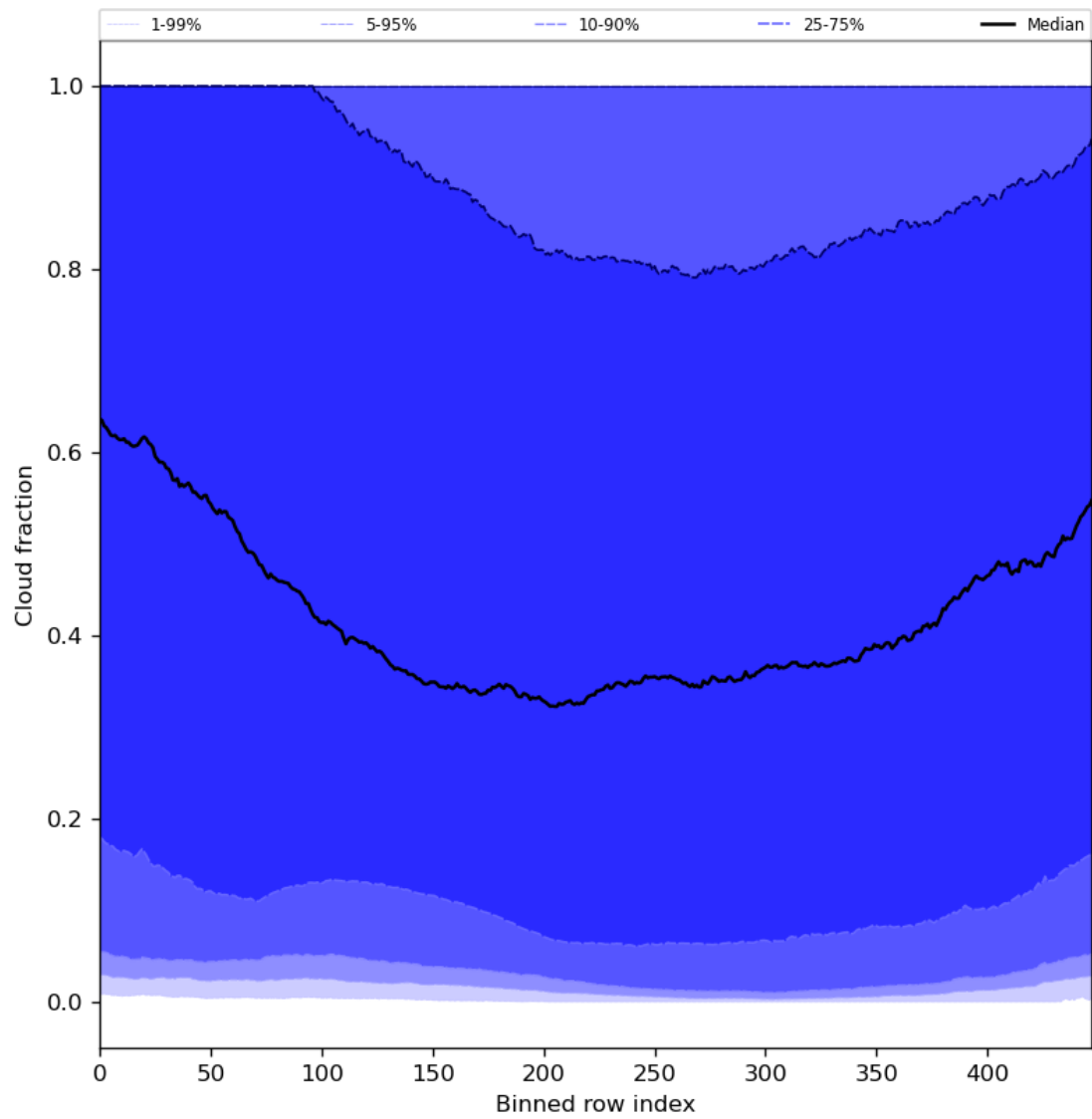
Figure 49: Along track statistics of “Cloud fraction” for 2023-11-05 to 2023-11-07
