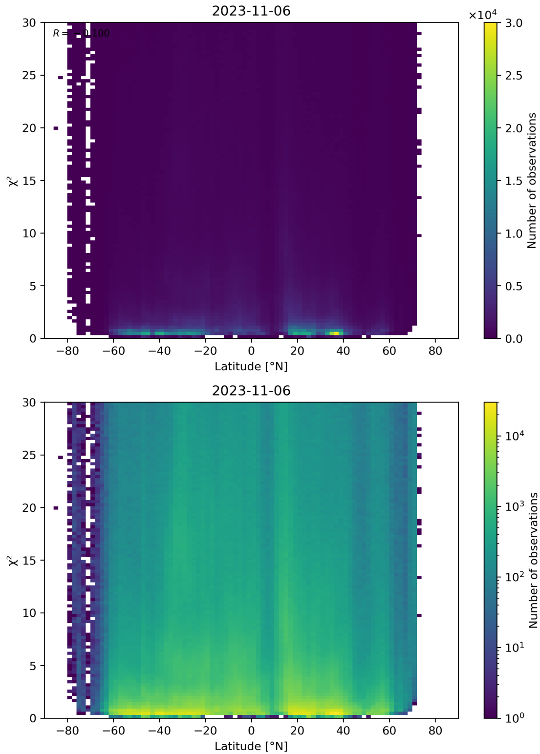
Figure 97: Scatter density plot of “Latitude” against “ \chi^2 ” for 2023-11-05 to 2023-11-07.
