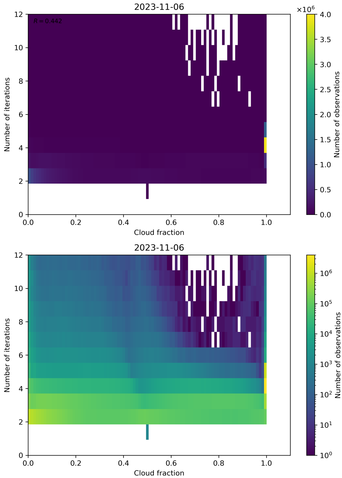
Figure 80: Scatter density plot of “Cloud fraction” against “Number of iterations” for 2023-11-05 to 2023-11-07.
