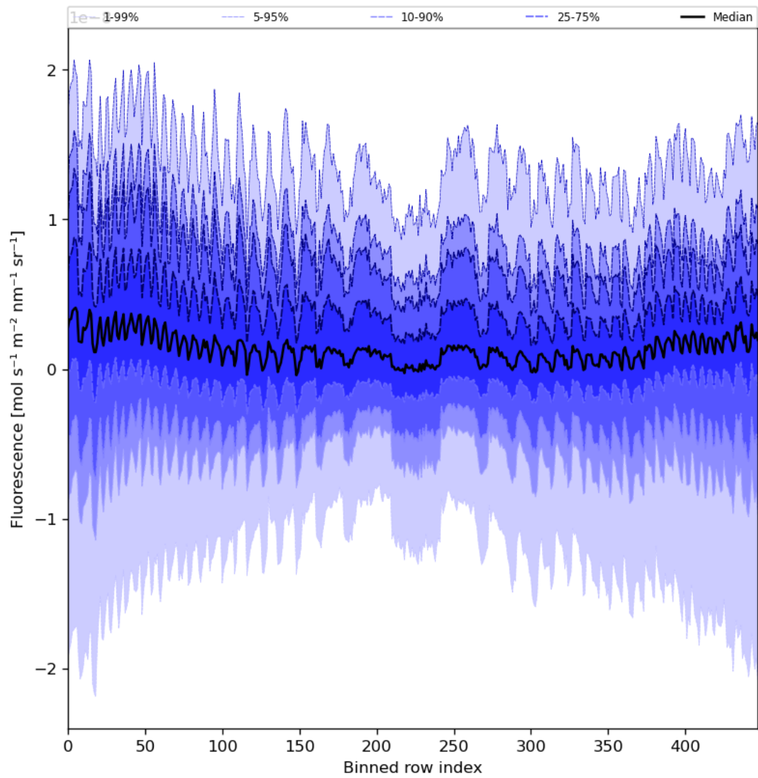
Figure 57: Along track statistics of “Fluorescence” for 2023-11-05 to 2023-11-07
