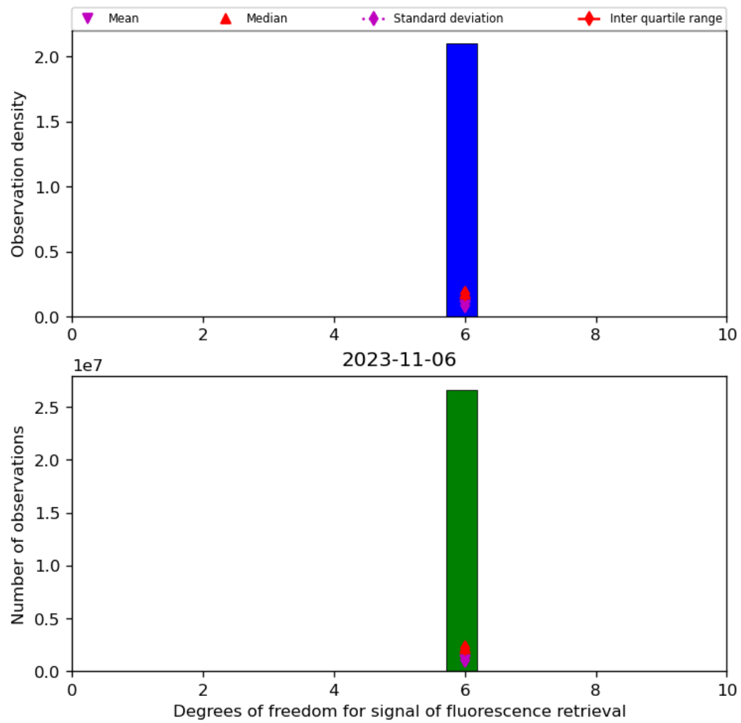
Figure 43: Histogram of “Degrees of freedom for signal of fluorescence retrieval” for 2023-11-05 to 2023-11-07
