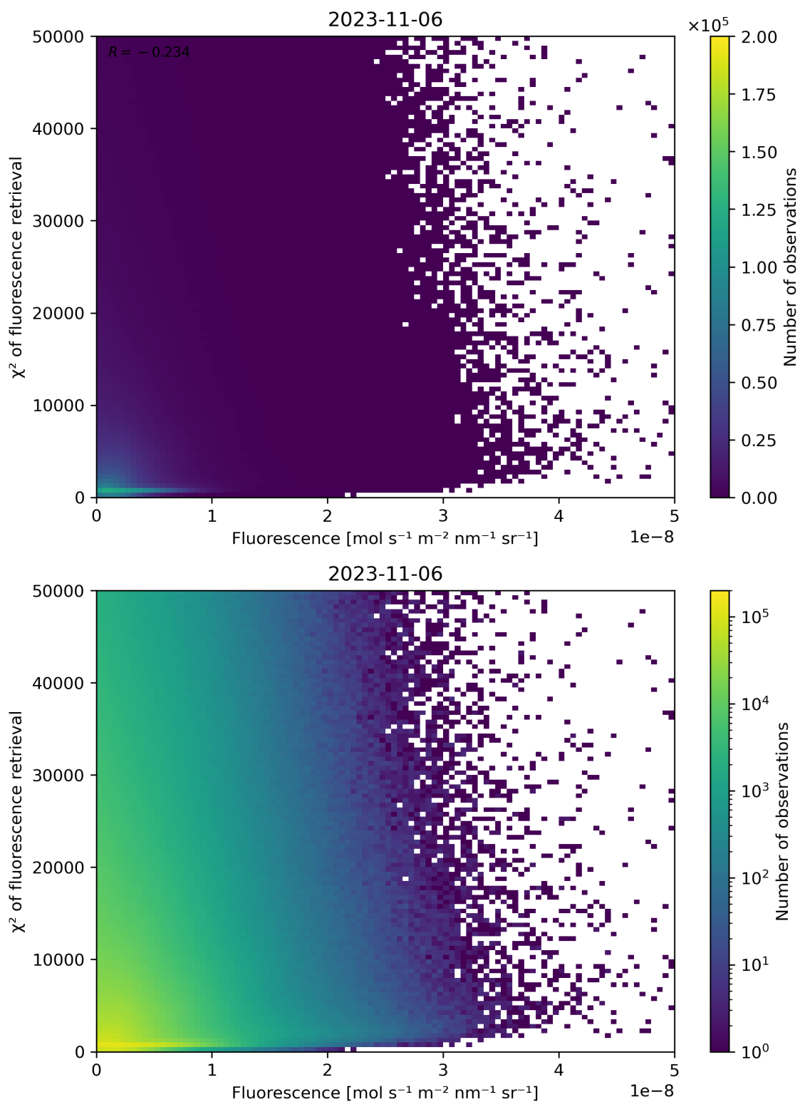
Figure 93: Scatter density plot of “Fluorescence” against “ \chi^2 of fluorescence retrieval” for 2023-11-05 to 2023-11-07.
