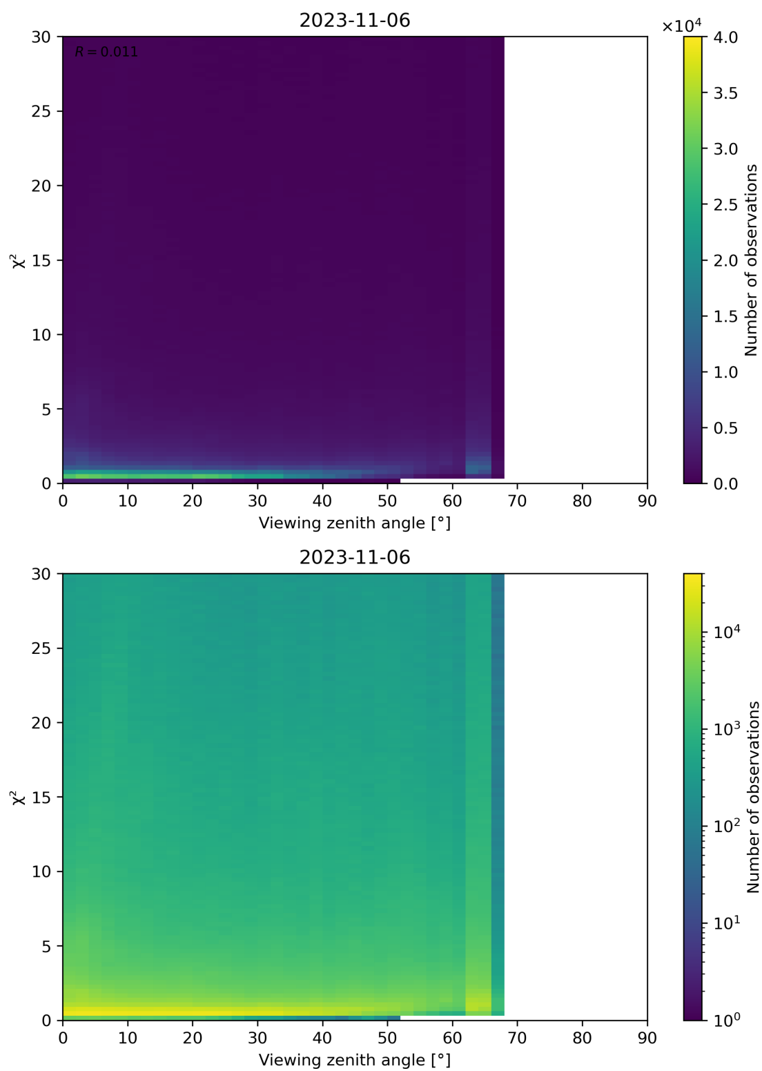
Figure 130: Scatter density plot of “Viewing zenith angle” against “ \chi^2 ” for 2023-11-05 to 2023-11-07.
