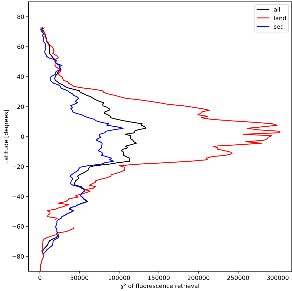
Figure 25: Zonal average of “ \chi^2 of fluorescence retrieval” for 2023-11-05 to 2023-11-07.
