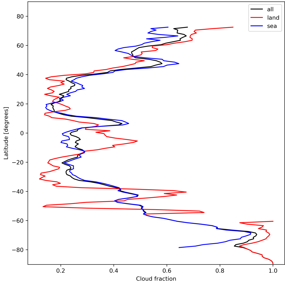
Figure 15: Zonal average of “Cloud fraction” for 2023-11-05 to 2023-11-07.
