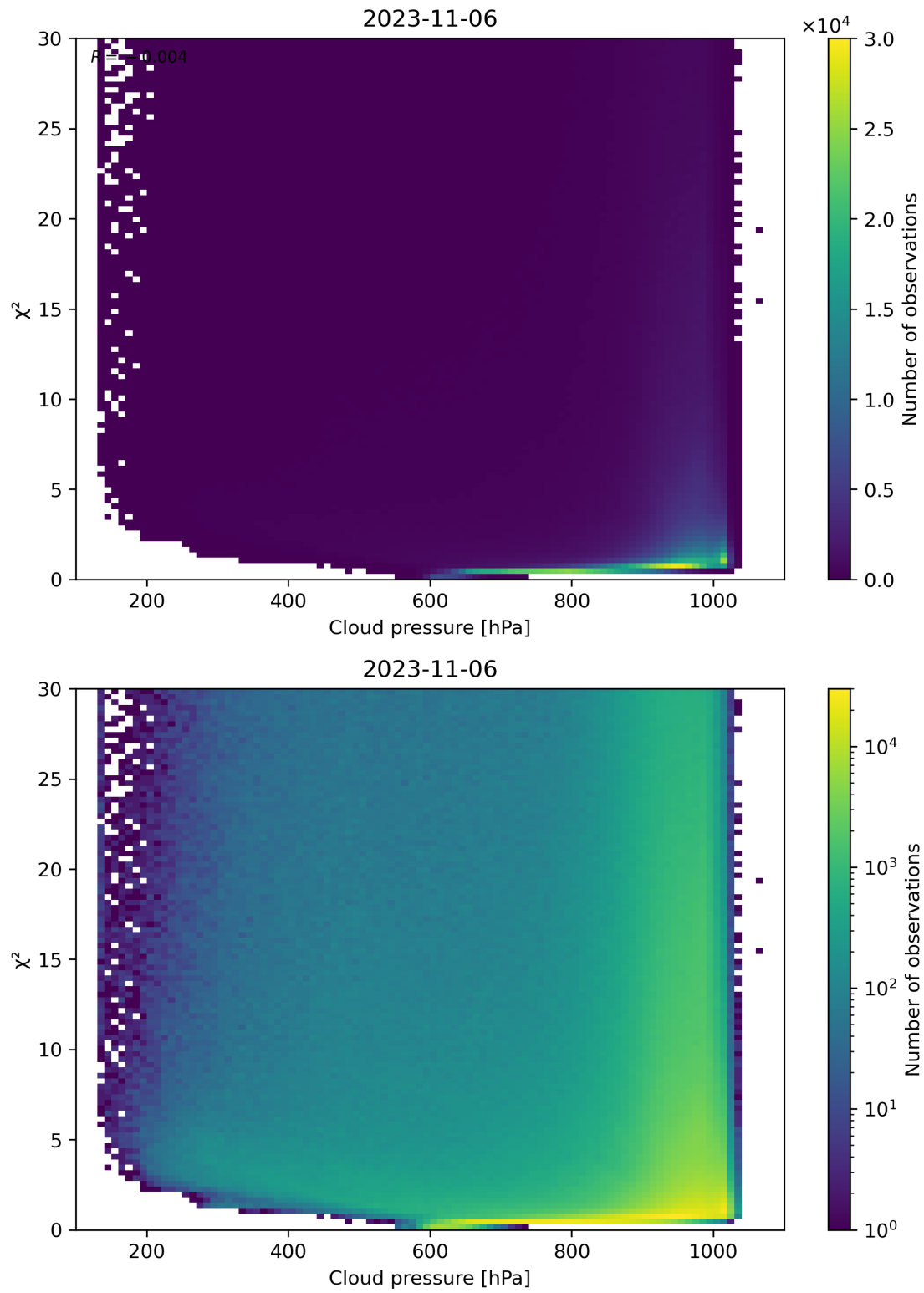
Figure 85: Scatter density plot of “Cloud pressure” against “ \chi^2 ” for 2023-11-05 to 2023-11-07.
