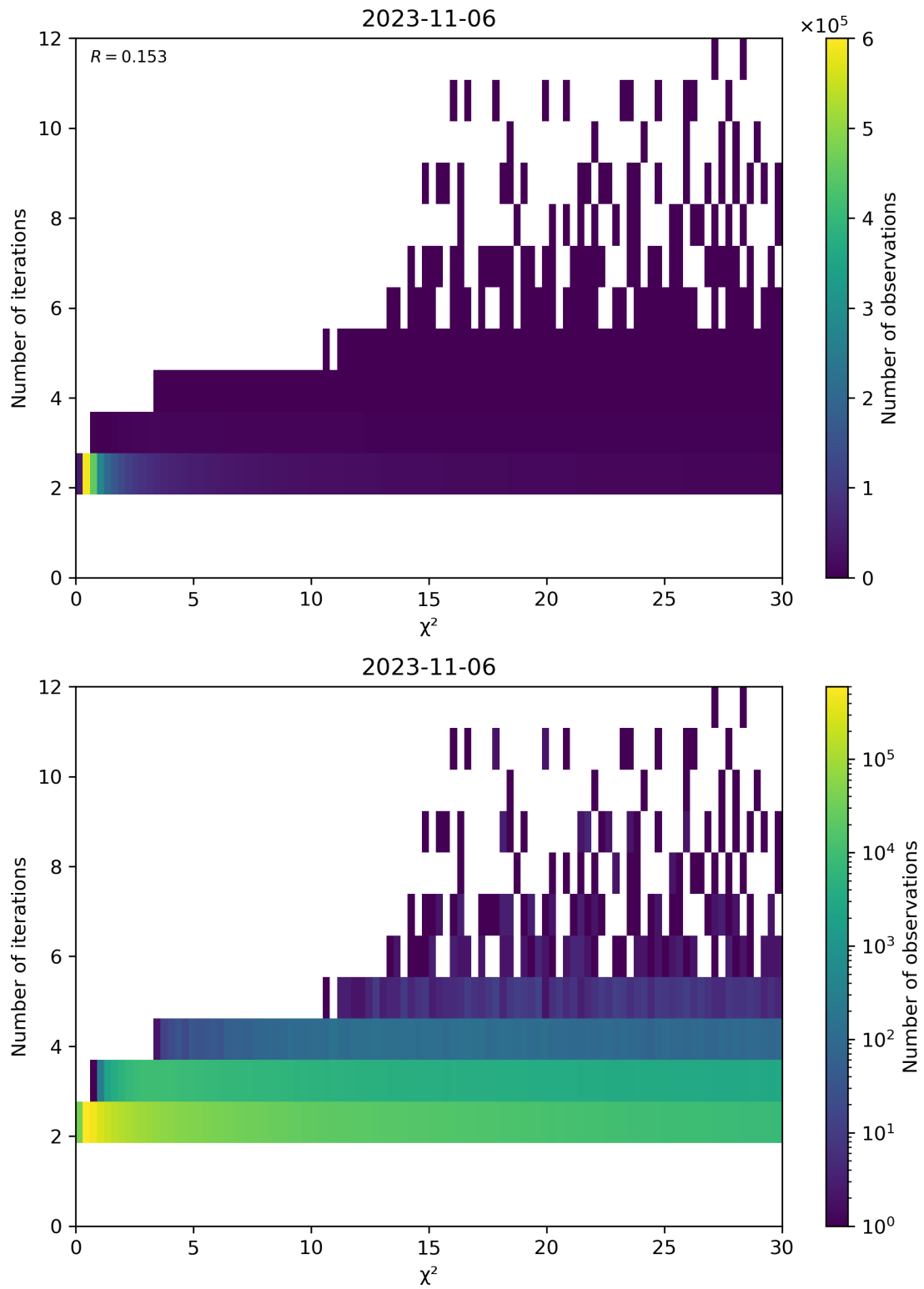
Figure 73: Scatter density plot of “ \chi^2 ” against “Number of iterations” for 2023-11-05 to 2023-11-07.
