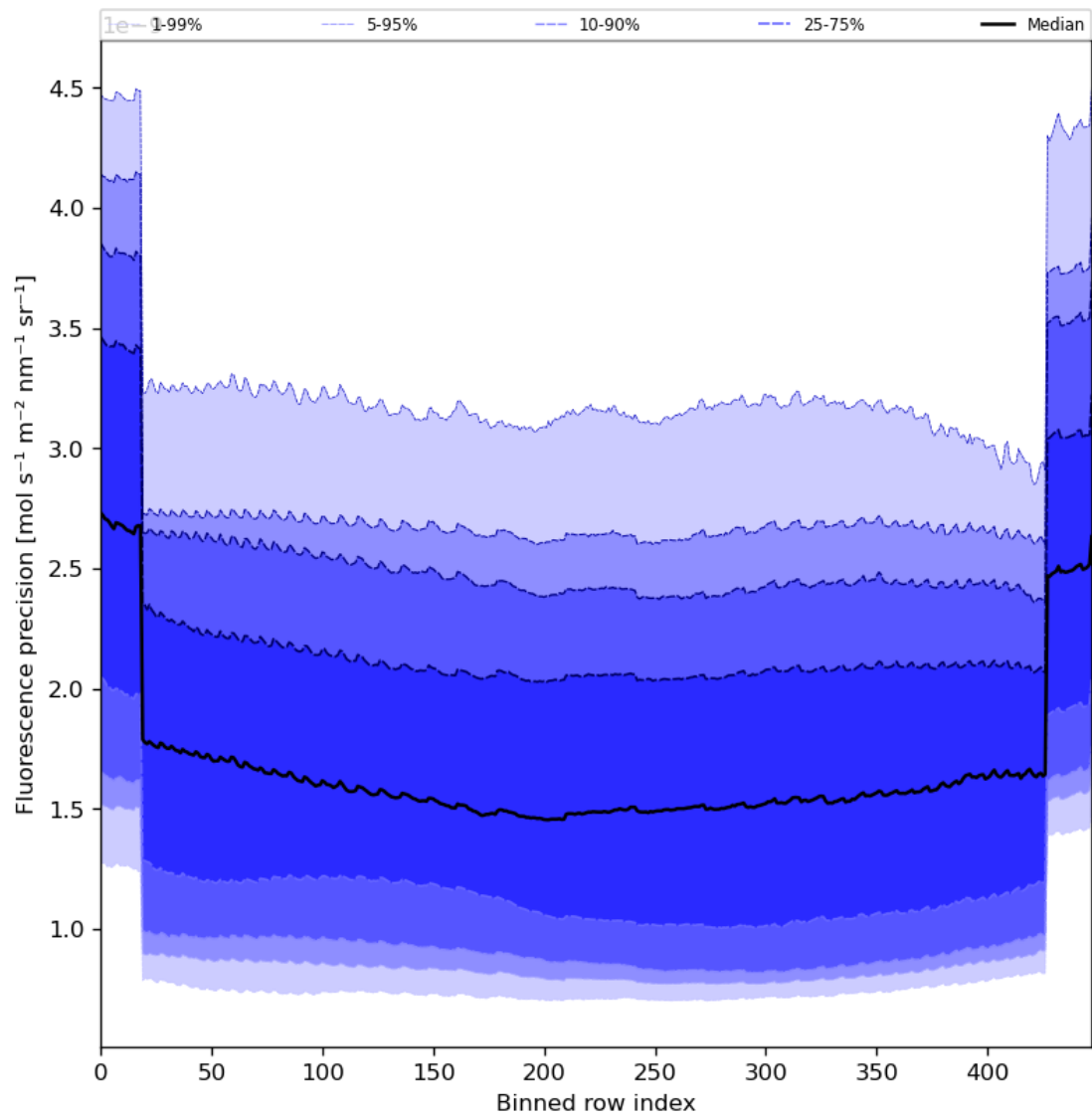
Figure 58: Along track statistics of “Fluorescence precision” for 2023-11-05 to 2023-11-07
