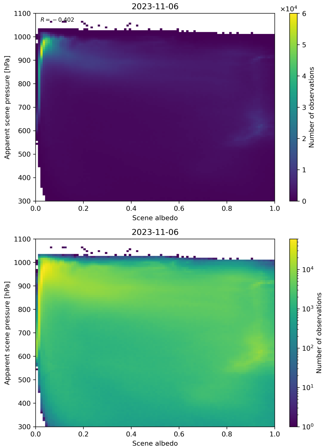
Figure 111: Scatter density plot of “Scene albedo” against “Apparent scene pressure” for 2023-11-05 to 2023-11-07.
