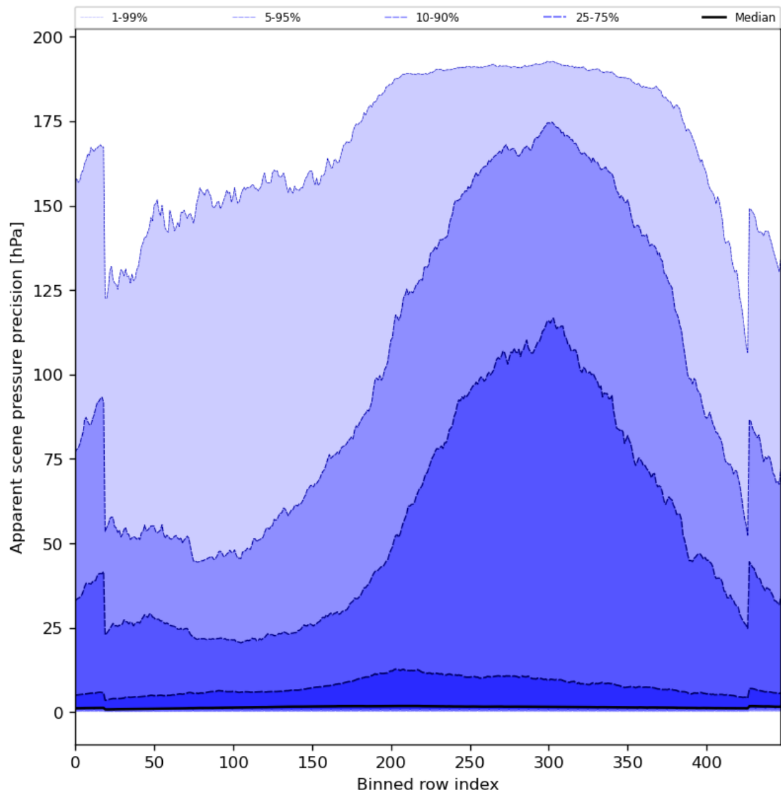
Figure 54: Along track statistics of “Apparent scene pressure precision” for 2023-11-05 to 2023-11-07
