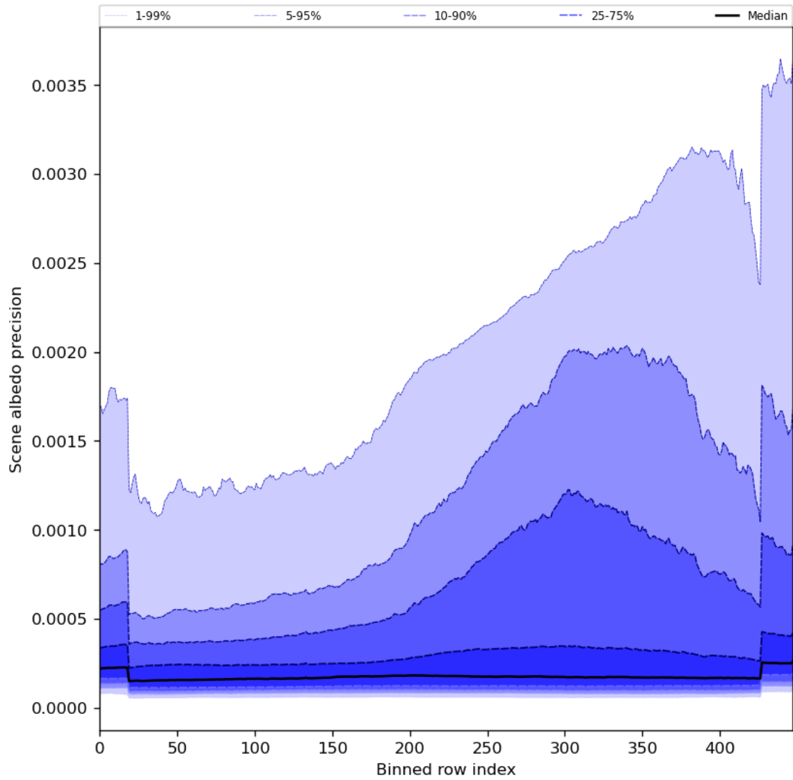
Figure 52: Along track statistics of “Scene albedo precision” for 2023-11-05 to 2023-11-07
