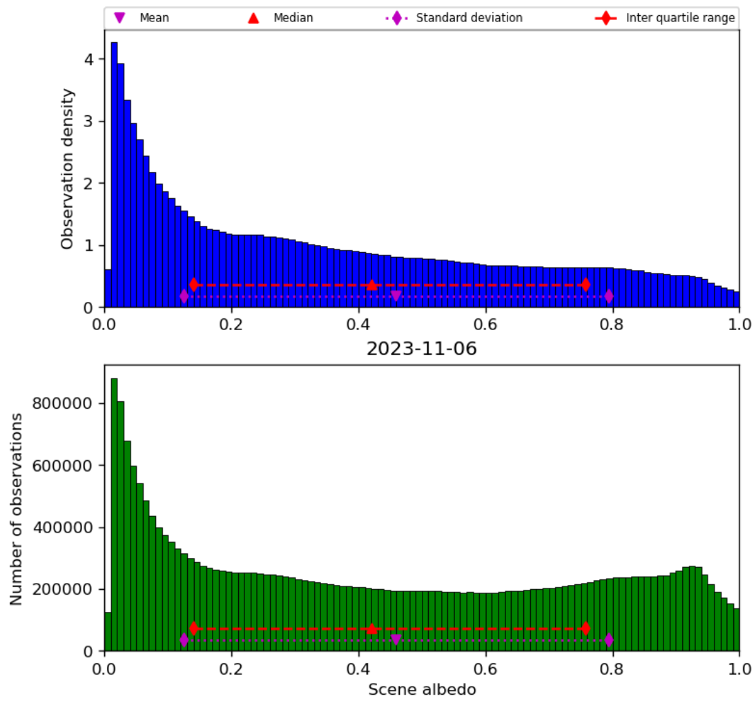
Figure 34: Histogram of “Scene albedo” for 2023-11-05 to 2023-11-07
