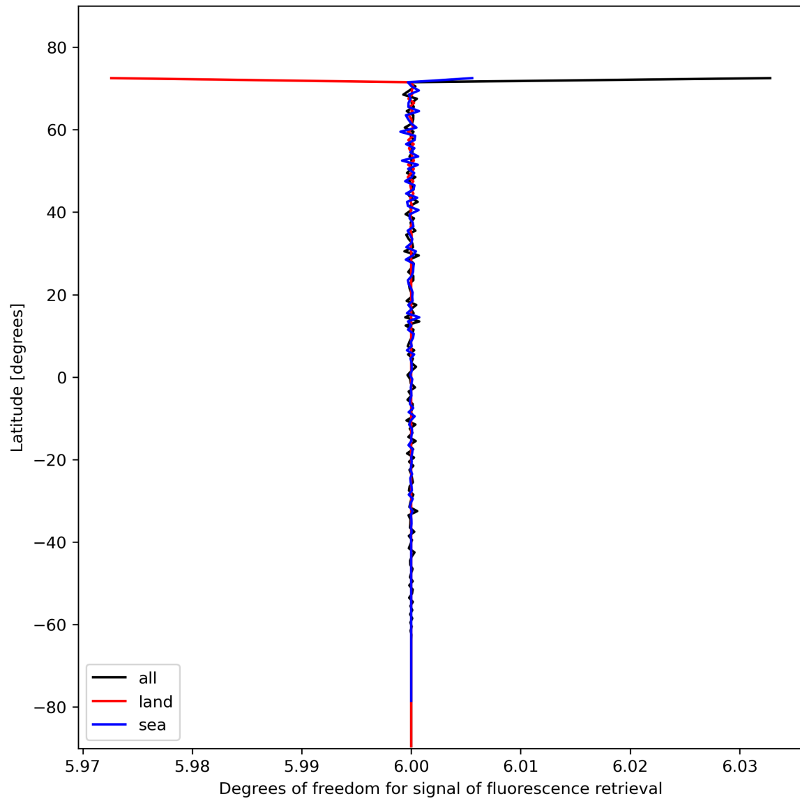
Figure 26: Zonal average of “Degrees of freedom for signal of fluorescence retrieval” for 2023-11-05 to 2023-11-07.
