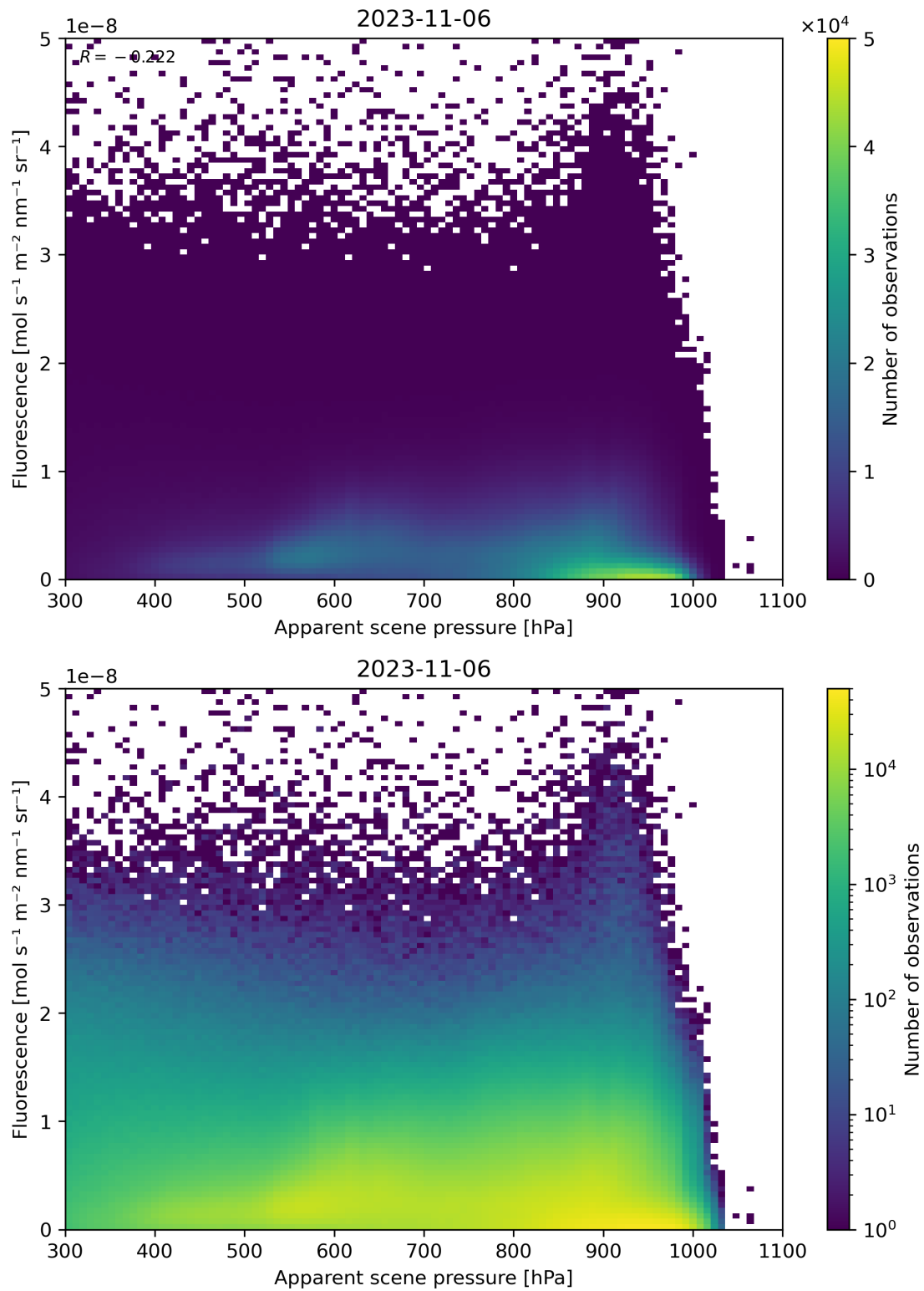
Figure 65: Scatter density plot of “Apparent scene pressure” against “Fluorescence” for 2023-11-05 to 2023-11-07.
