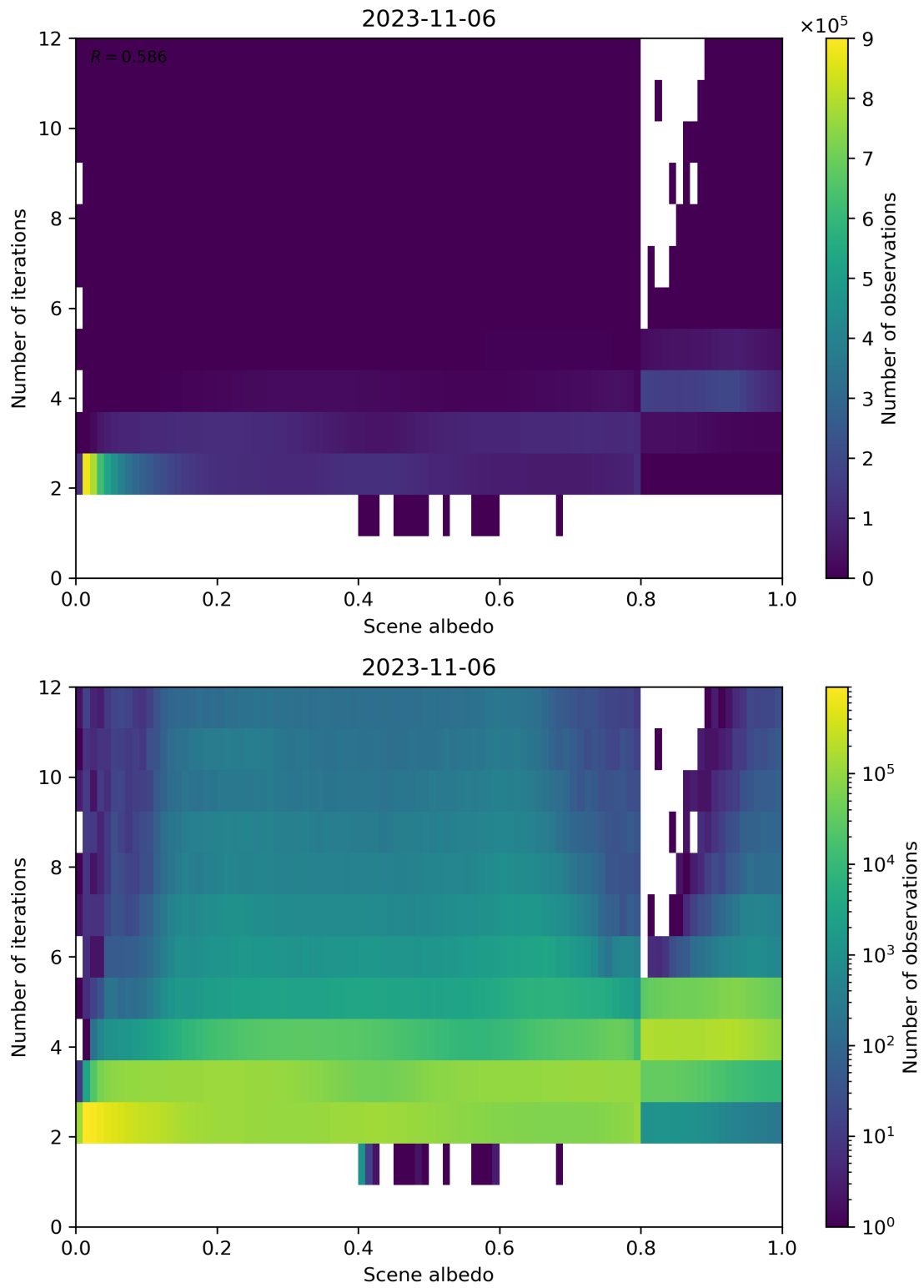
Figure 115: Scatter density plot of “Scene albedo” against “Number of iterations” for 2023-11-05 to 2023-11-07.
