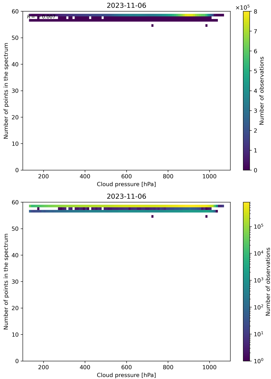
Figure 90: Scatter density plot of “Cloud pressure” against “Number of points in the spectrum” for 2023-11-05 to 2023-11-07.
