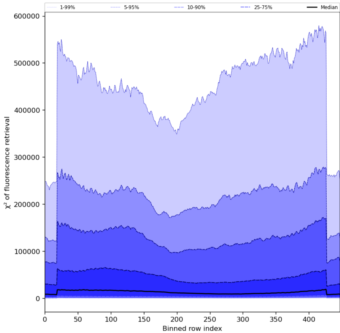
Figure 59: Along track statistics of “ \chi^2 of fluorescence retrieval” for 2023-11-05 to 2023-11-07
