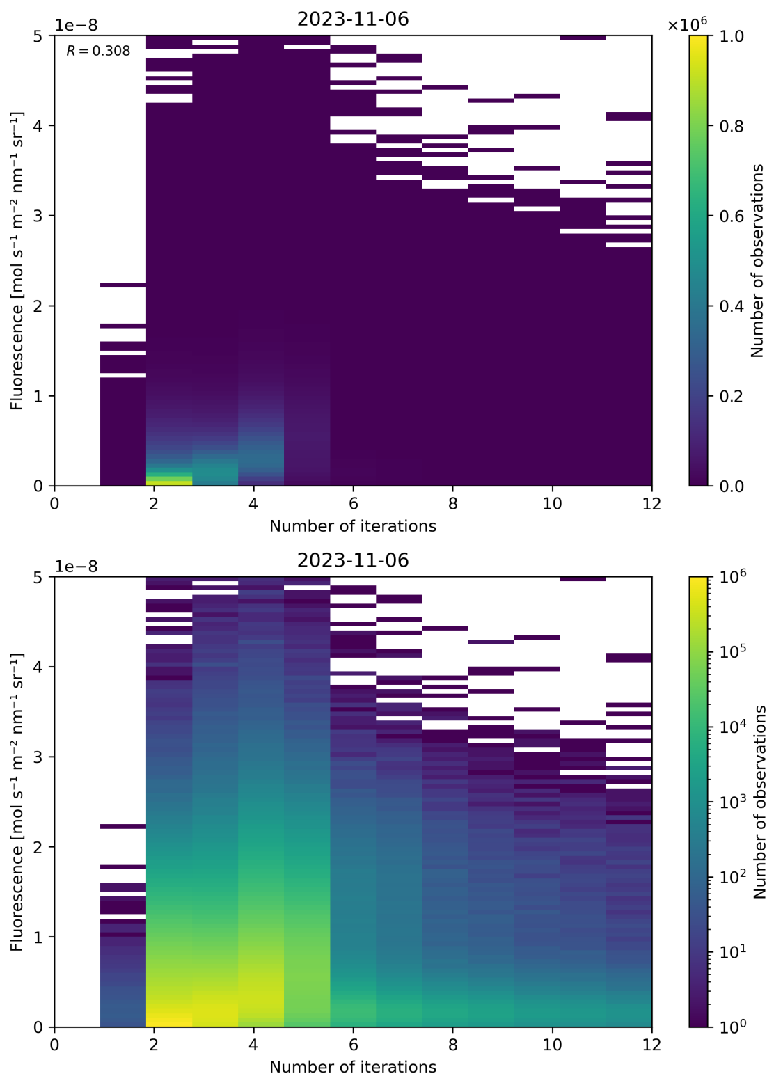
Figure 107: Scatter density plot of “Number of iterations” against “Fluorescence” for 2023-11-05 to 2023-11-07.
