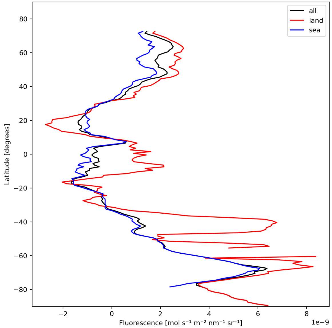
Figure 23: Zonal average of “Fluorescence” for 2023-11-05 to 2023-11-07.
