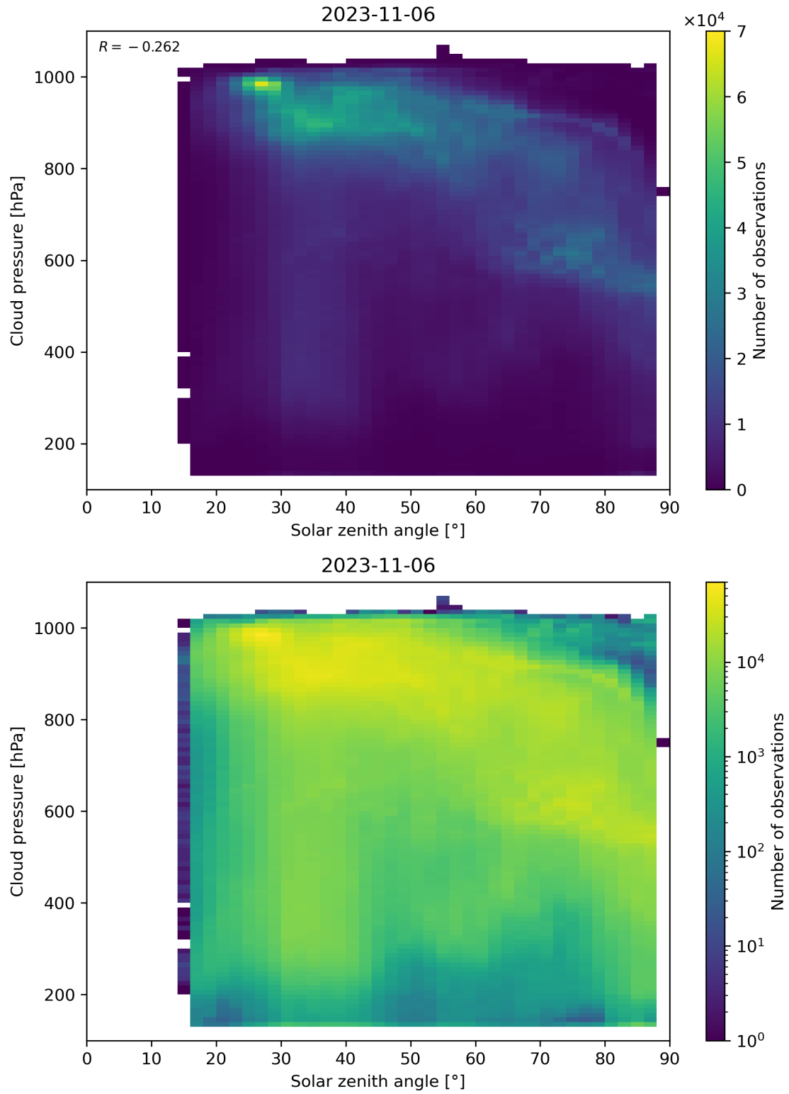
Figure 122: Scatter density plot of “Solar zenith angle” against “Cloud pressure” for 2023-11-05 to 2023-11-07.
