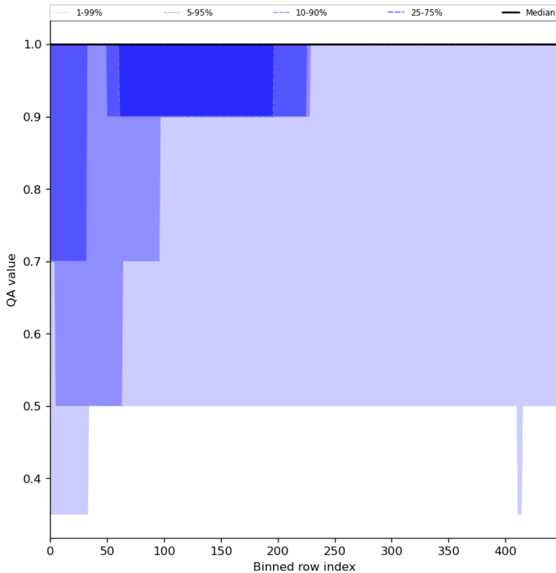
Figure 46: Along track statistics of “QA value” for 2023-11-05 to 2023-11-07
