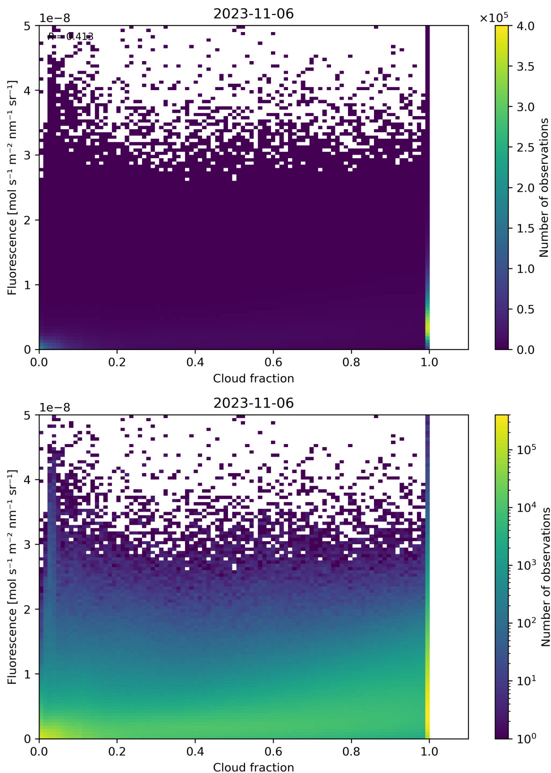
Figure 79: Scatter density plot of “Cloud fraction” against “Fluorescence” for 2023-11-05 to 2023-11-07.
