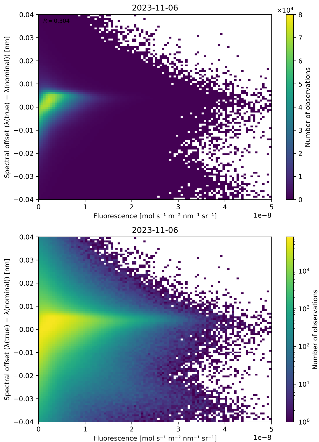
Figure 95: Scatter density plot of “Fluorescence” against “Spectral offset ( \lambda(\text{true}) - \lambda(\text{nominal}) )” for 2023-11-05 to 2023-11-07.
