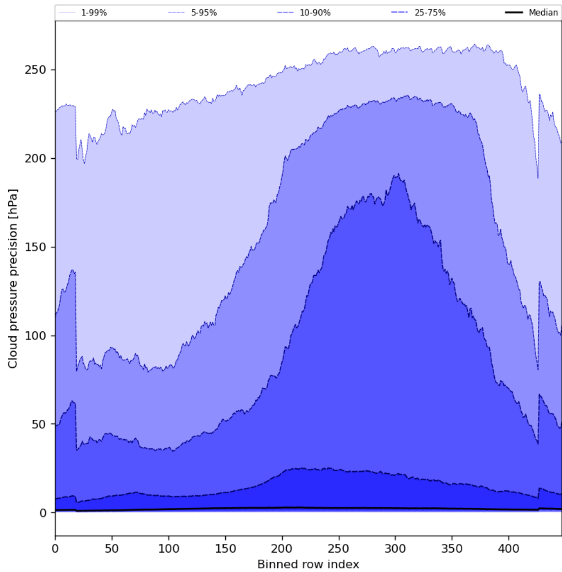
Figure 48: Along track statistics of “Cloud pressure precision” for 2023-11-05 to 2023-11-07
