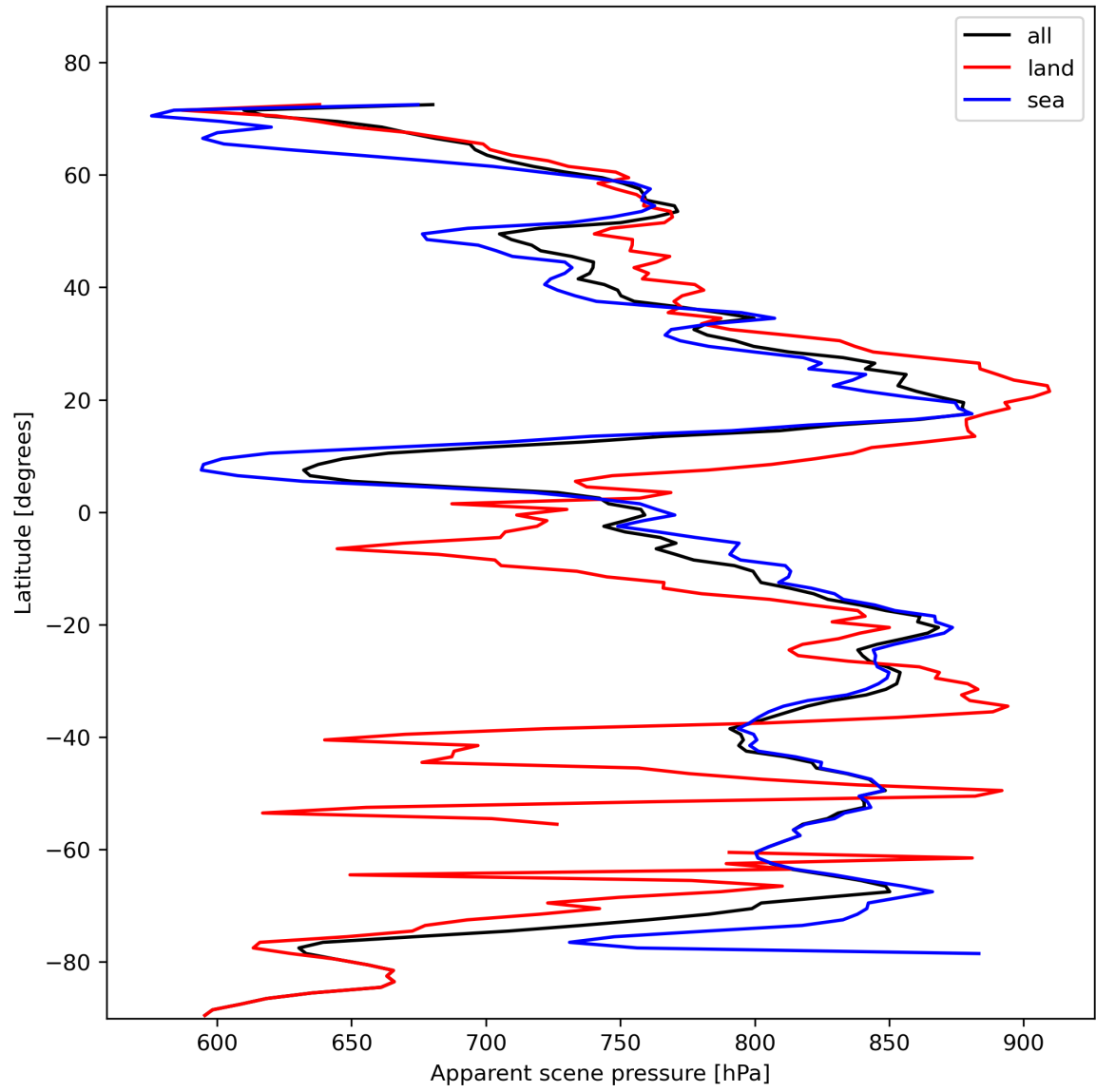
Figure 19: Zonal average of “Apparent scene pressure” for 2023-11-05 to 2023-11-07.
