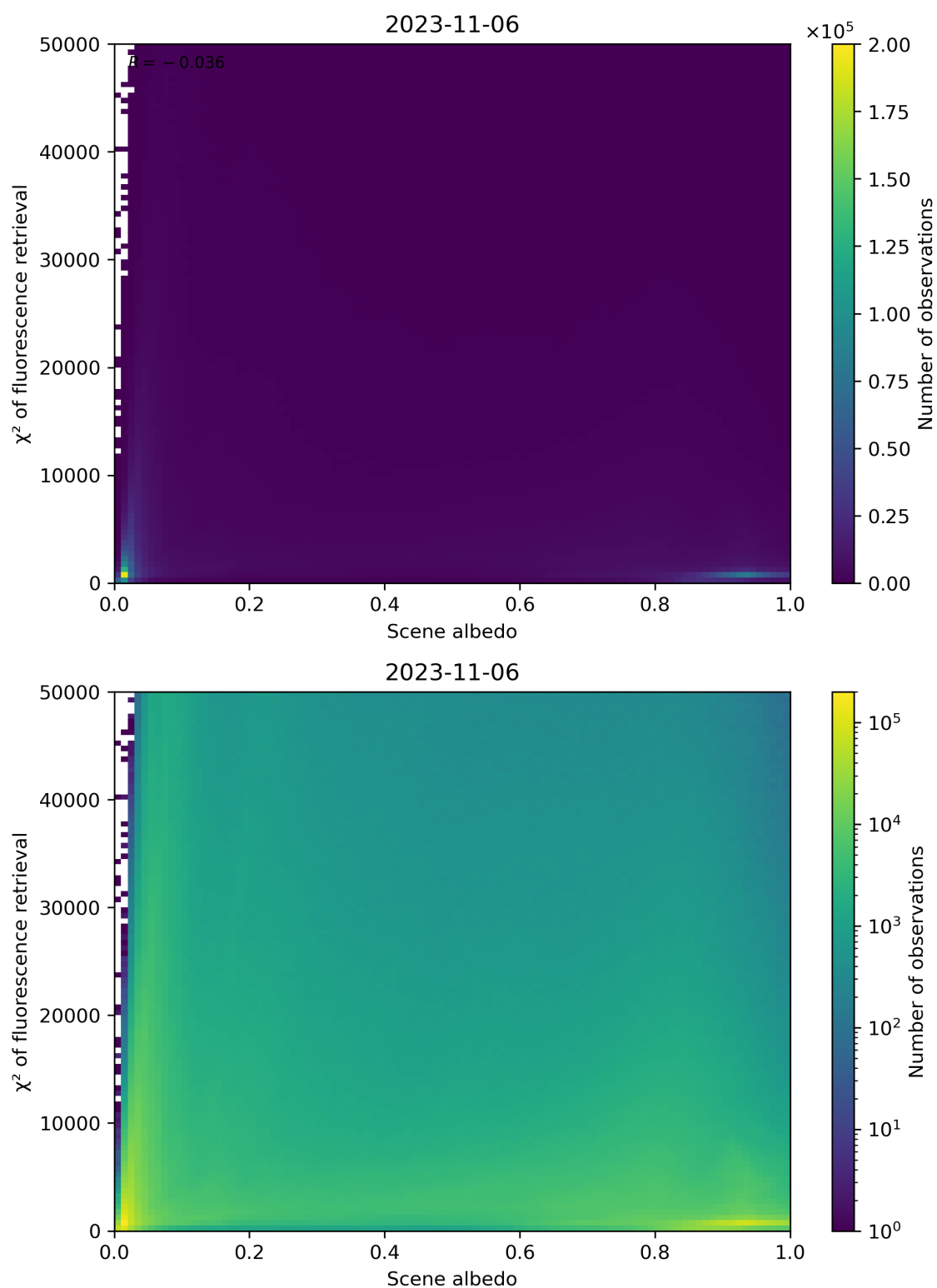
Figure 113: Scatter density plot of “Scene albedo” against “ \chi^2 of fluorescence retrieval” for 2023-11-05 to 2023-11-07.
