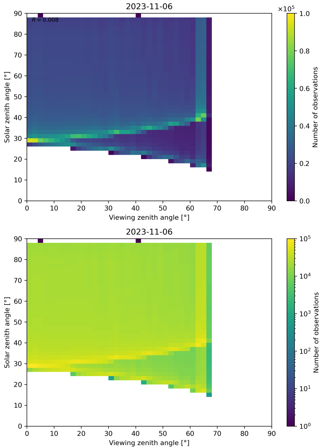
Figure 139: Scatter density plot of “Viewing zenith angle” against “Solar zenith angle” for 2023-11-05 to 2023-11-07.
