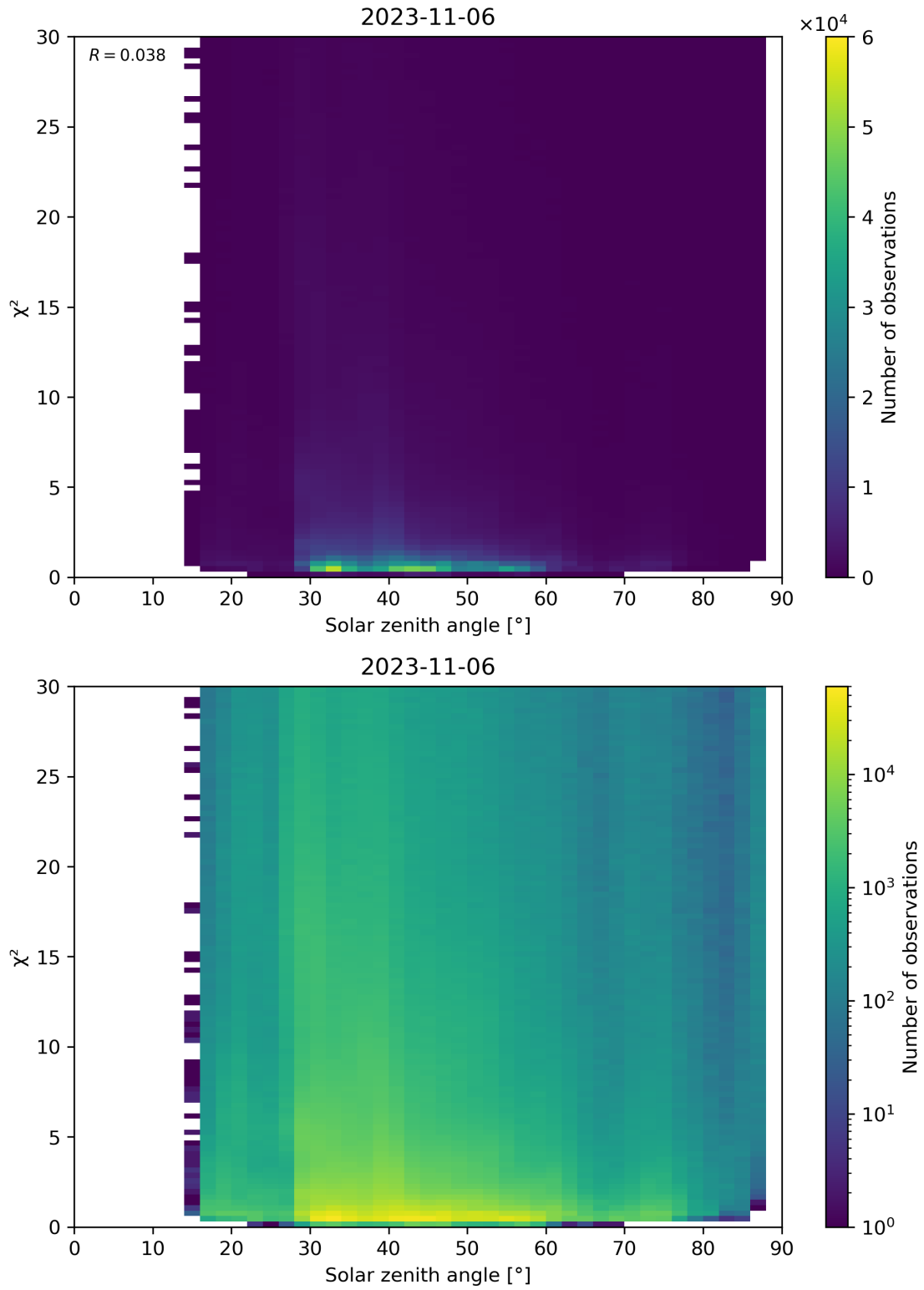
Figure 119: Scatter density plot of “Solar zenith angle” against “ \chi^2 ” for 2023-11-05 to 2023-11-07.
