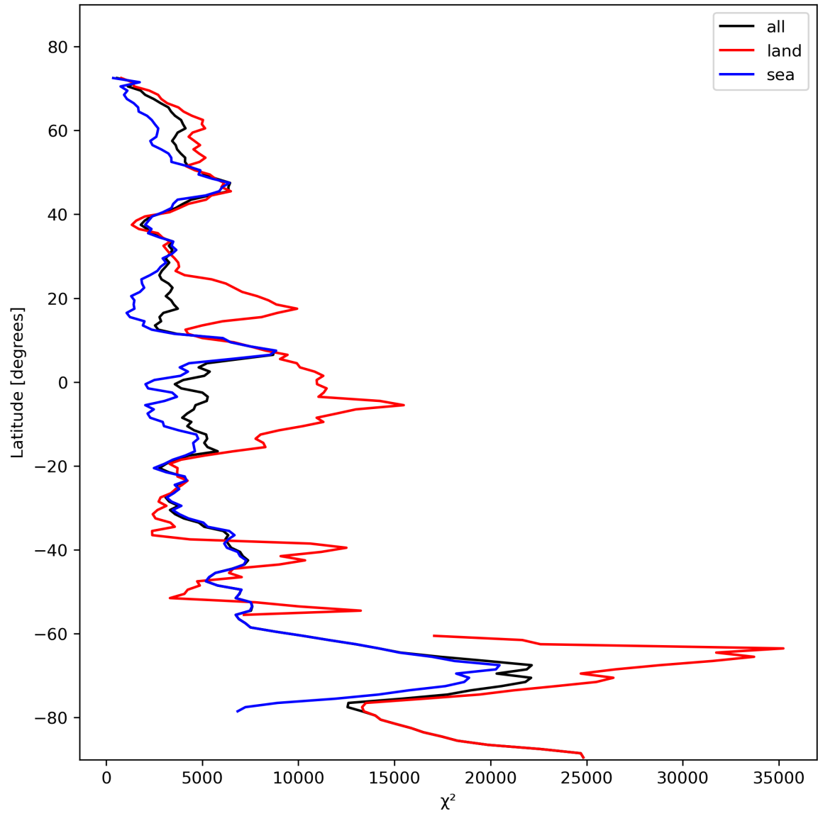
Figure 21: Zonal average of “ \chi^2 ” for 2023-11-05 to 2023-11-07.
