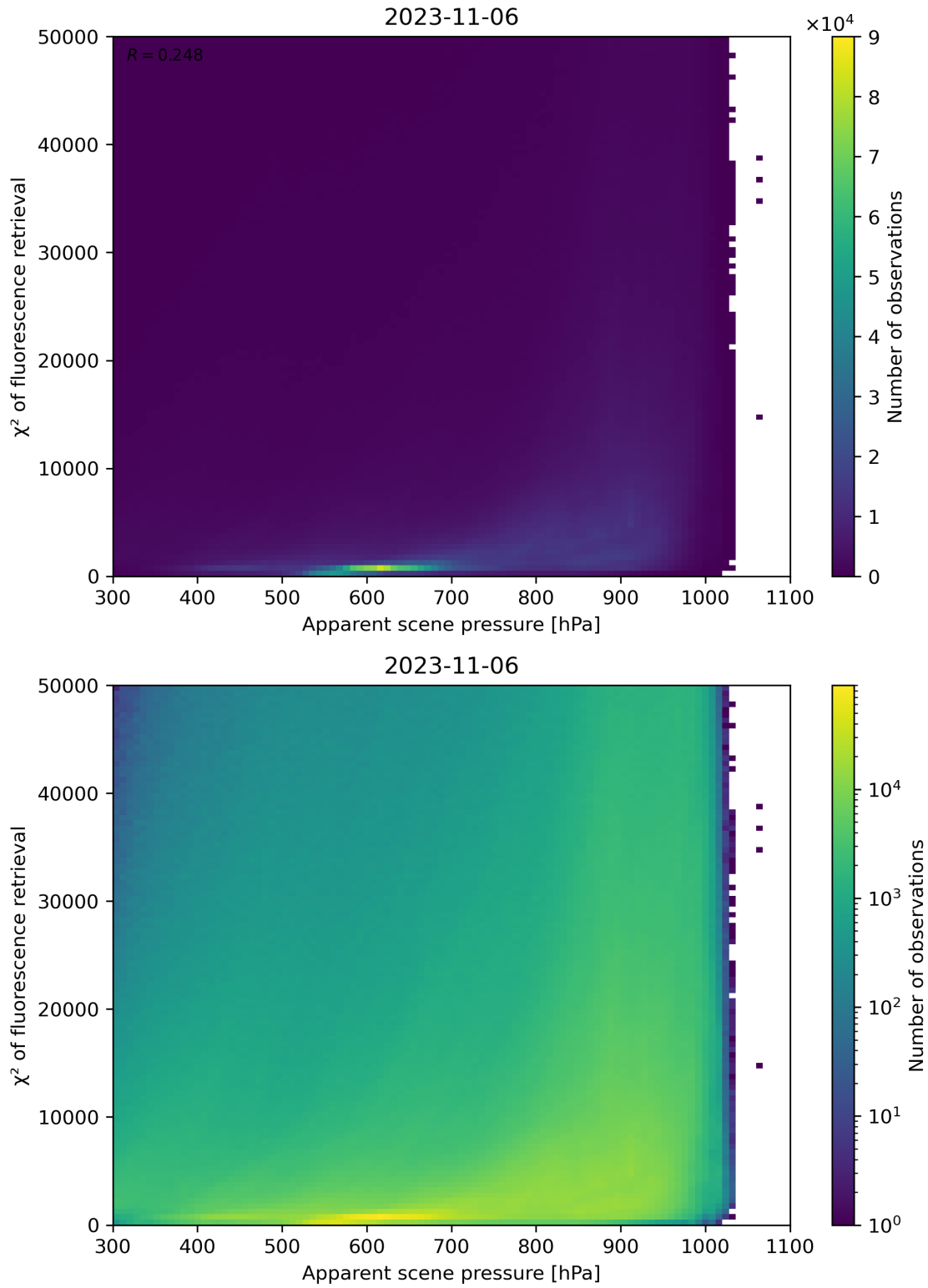
Figure 64: Scatter density plot of “Apparent scene pressure” against “ \chi^2 of fluorescence retrieval” for 2023-11-05 to 2023-11-07.
