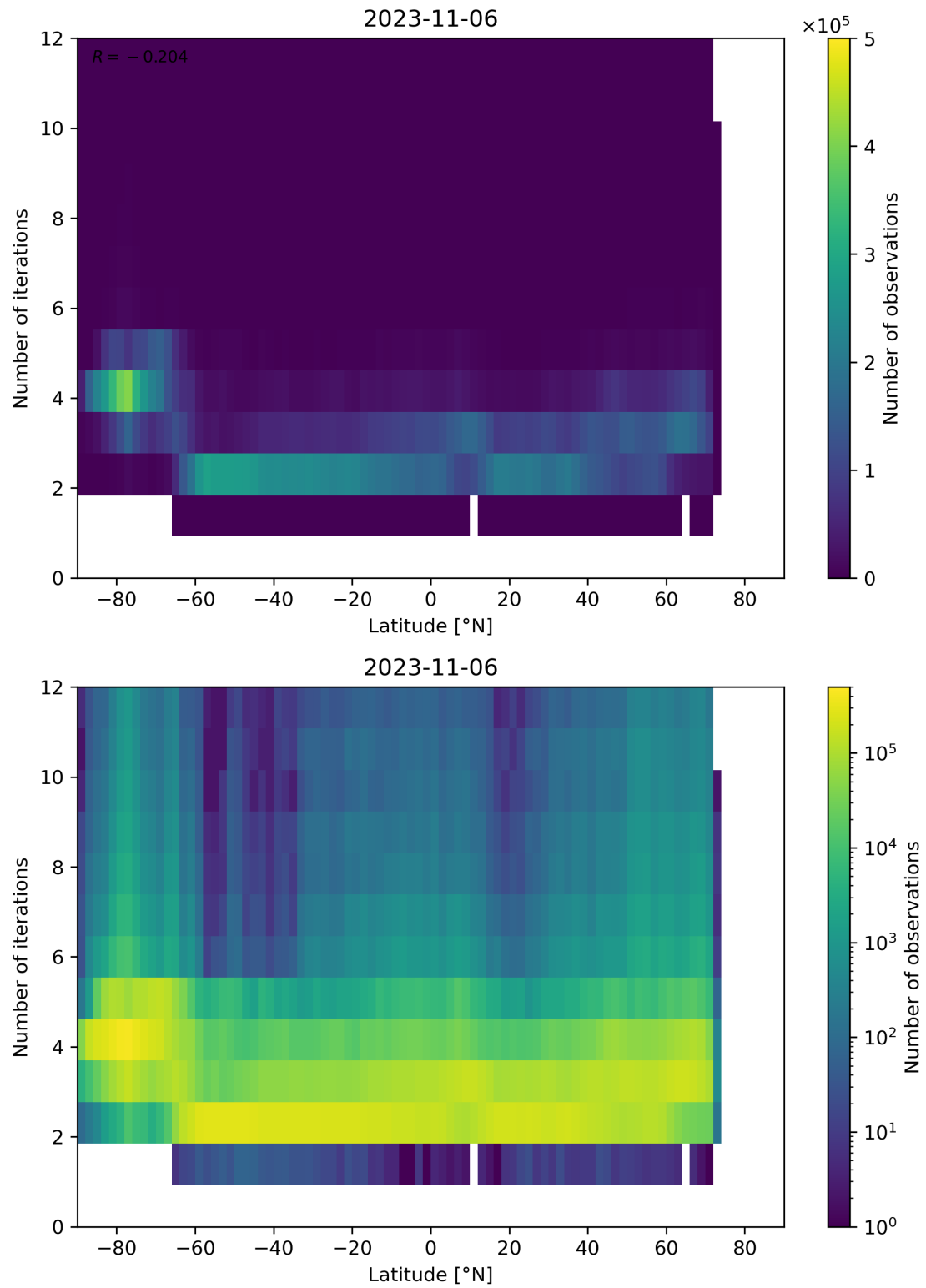
Figure 102: Scatter density plot of “Latitude” against “Number of iterations” for 2023-11-05 to 2023-11-07.
