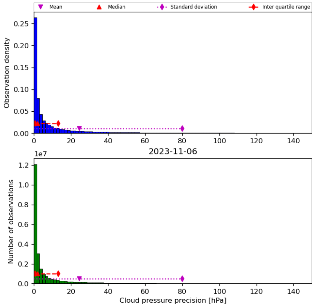
Figure 31: Histogram of “Cloud pressure precision” for 2023-11-05 to 2023-11-07
