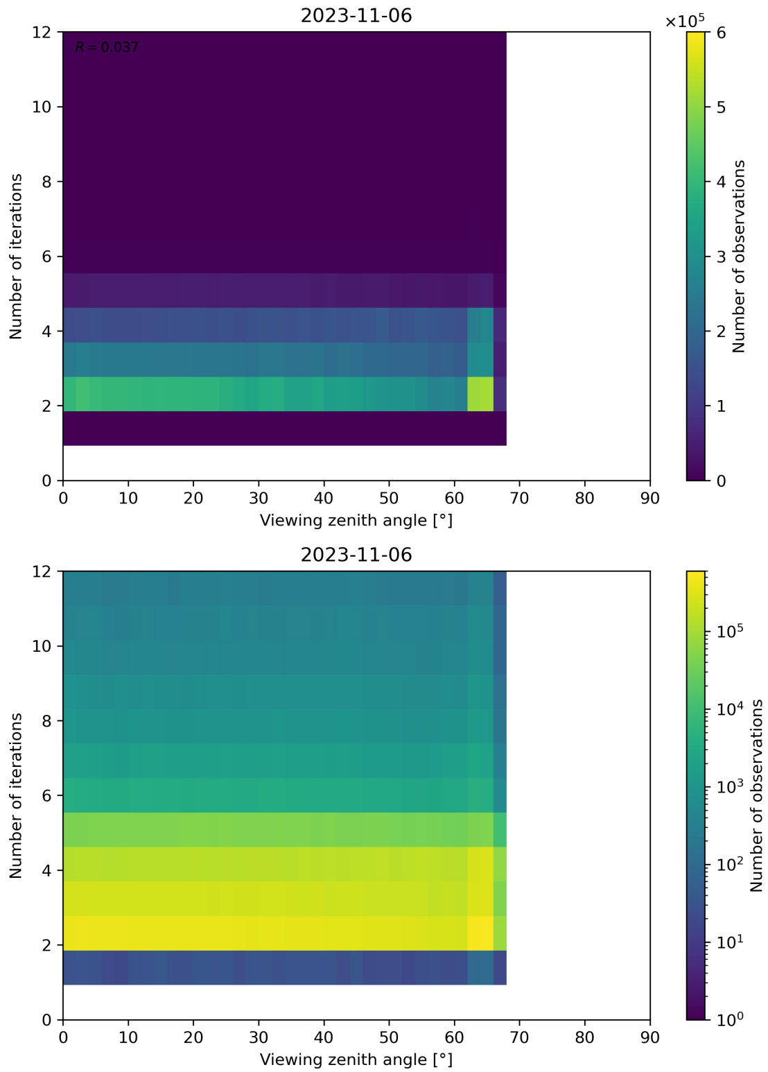
Figure 136: Scatter density plot of “Viewing zenith angle” against “Number of iterations” for 2023-11-05 to 2023-11-07.
