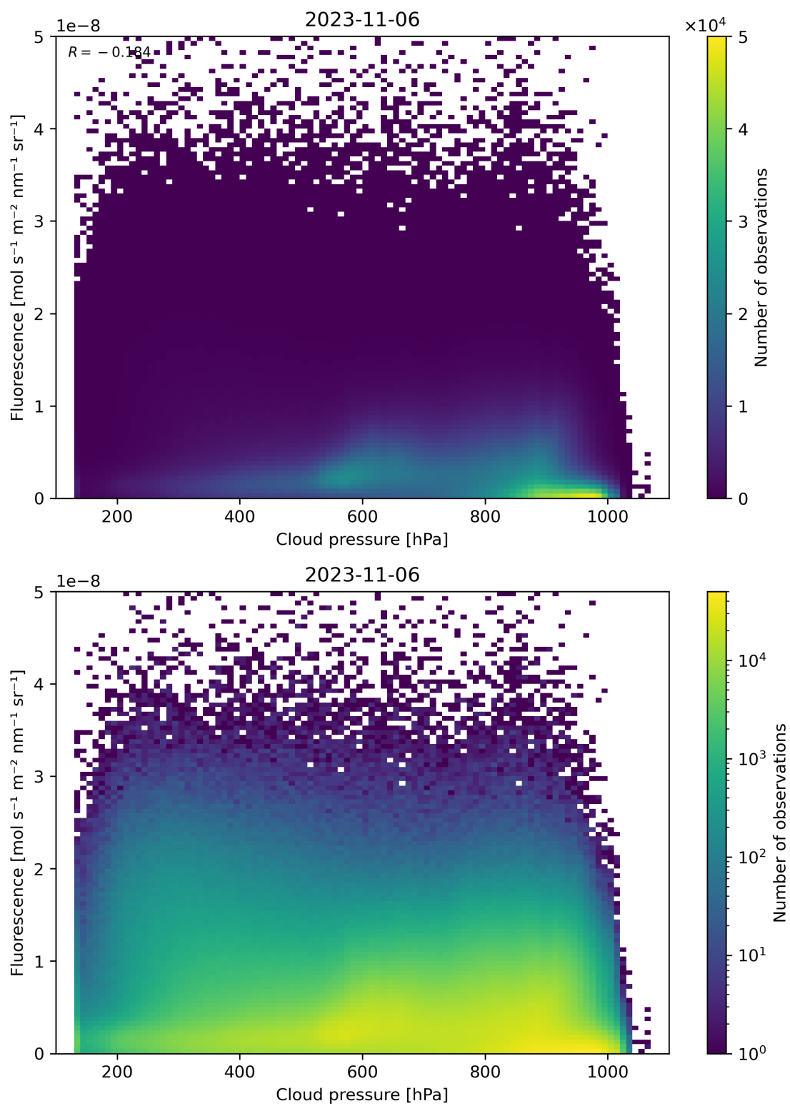
Figure 88: Scatter density plot of “Cloud pressure” against “Fluorescence” for 2023-11-05 to 2023-11-07.
