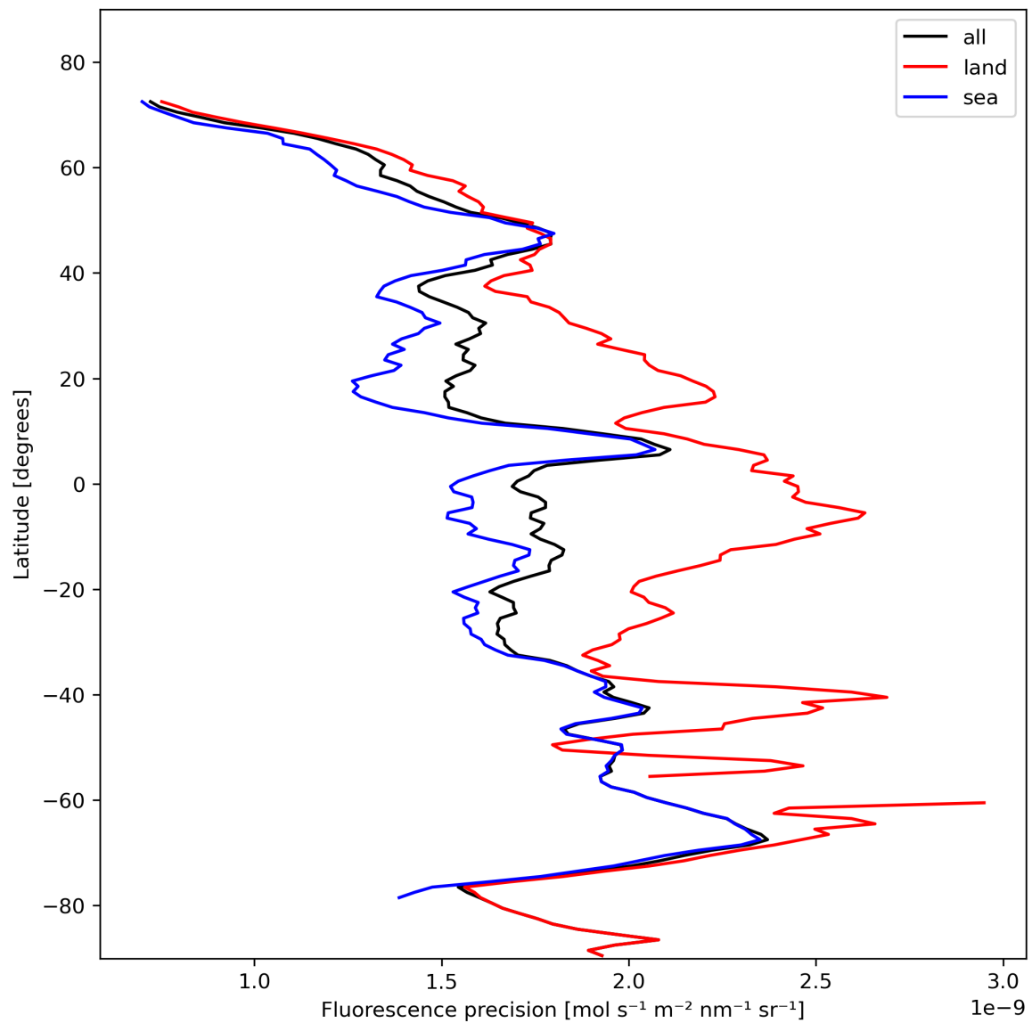
Figure 24: Zonal average of "Fluorescence precision" for 2023-11-05 to 2023-11-07.
