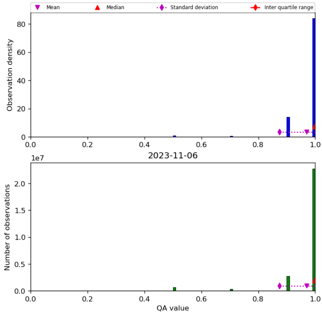
Figure 29: Histogram of “QA value” for 2023-11-05 to 2023-11-07
