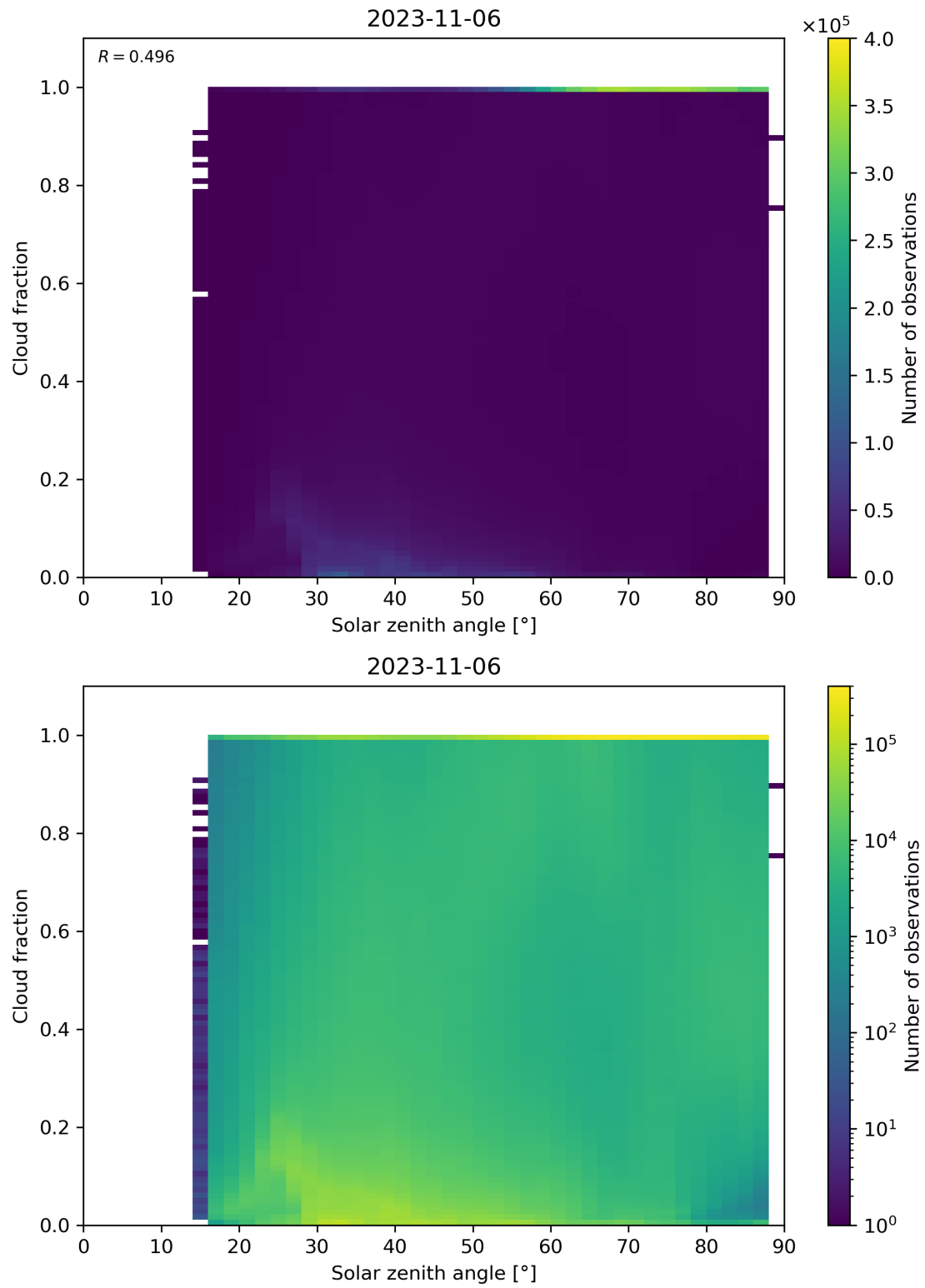
Figure 121: Scatter density plot of “Solar zenith angle” against “Cloud fraction” for 2023-11-05 to 2023-11-07.
