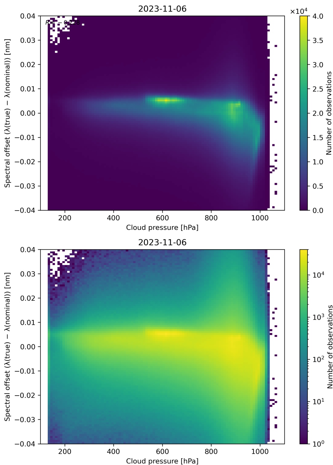
Figure 92: Scatter density plot of “Cloud pressure” against “Spectral offset ( \lambda(\text{true}) - \lambda(\text{nominal}) )” for 2023-11-05 to 2023-11-07.
