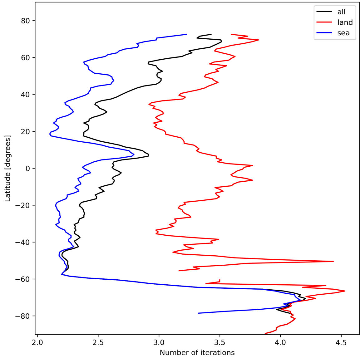
Figure 22: Zonal average of “Number of iterations” for 2023-11-05 to 2023-11-07.
