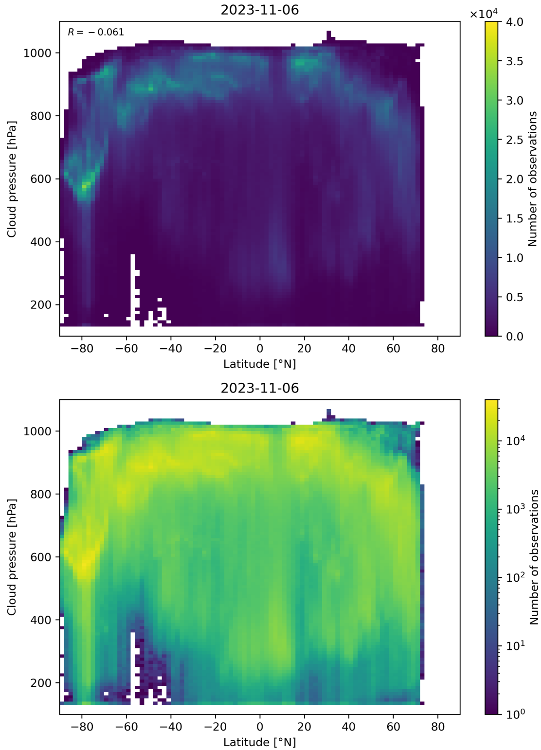
Figure 100: Scatter density plot of “Latitude” against “Cloud pressure” for 2023-11-05 to 2023-11-07.
