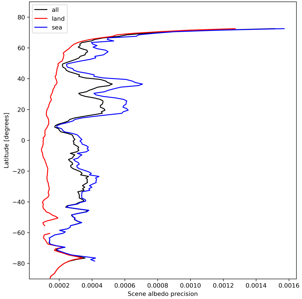
Figure 18: Zonal average of "Scene albedo precision" for 2023-11-05 to 2023-11-07.
