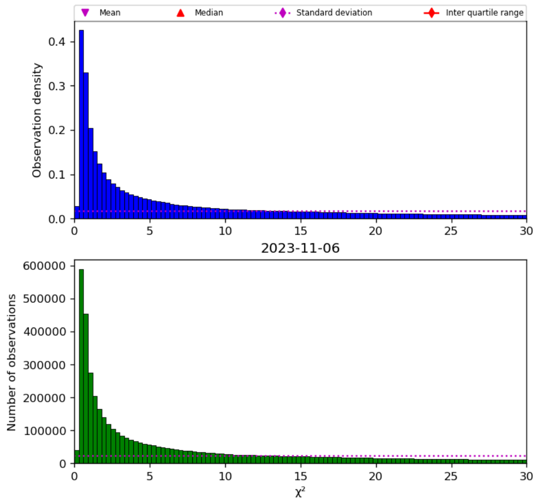
Figure 38: Histogram of “ \chi^2 ” for 2023-11-05 to 2023-11-07
