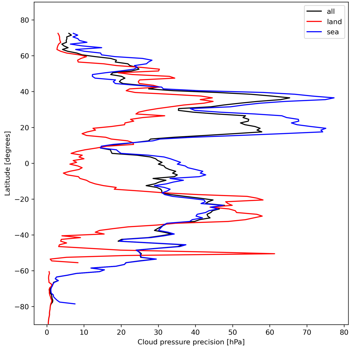
Figure 14: Zonal average of “Cloud pressure precision” for 2023-11-05 to 2023-11-07.
