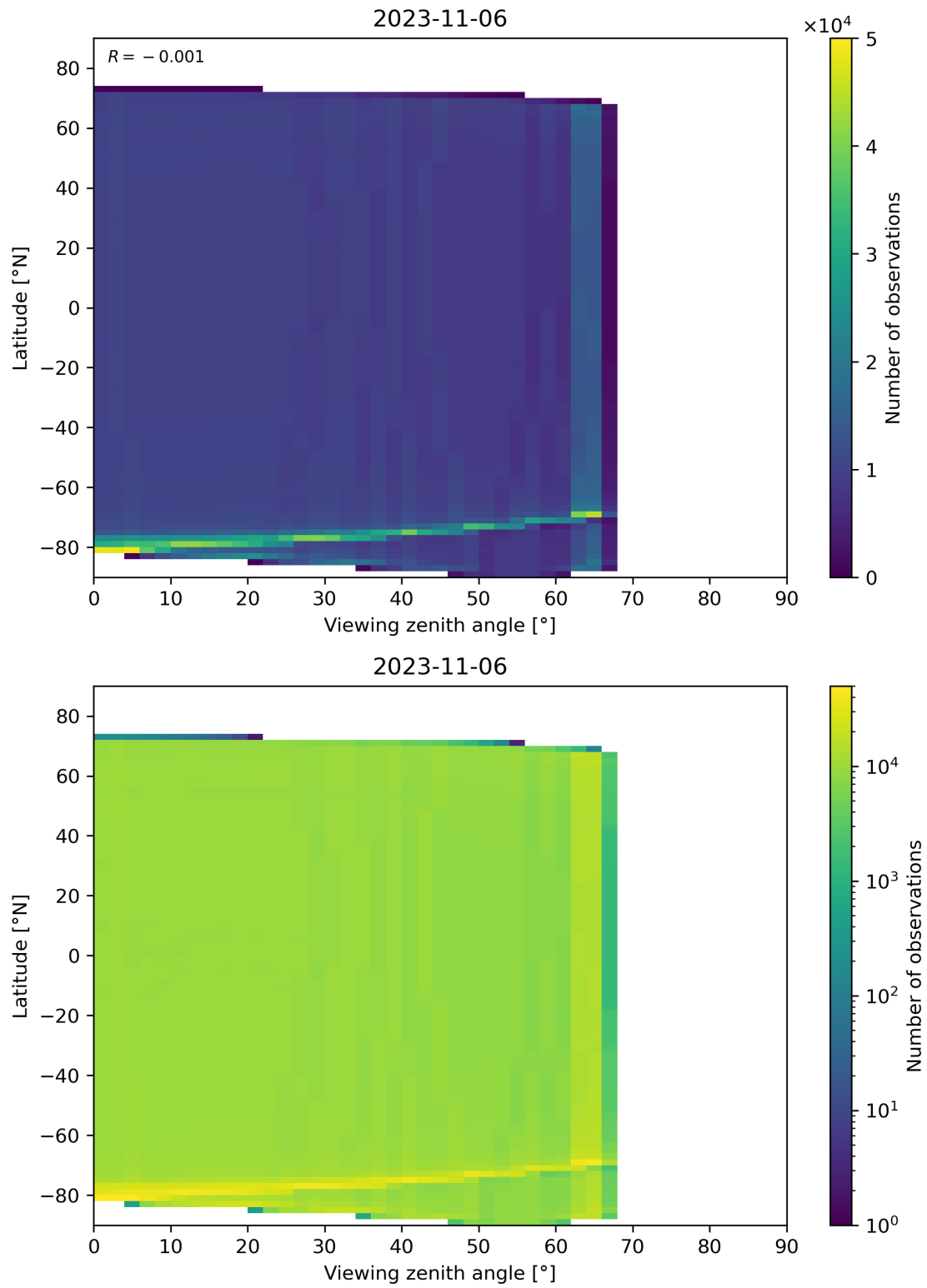
Figure 135: Scatter density plot of “Viewing zenith angle” against “Latitude” for 2023-11-05 to 2023-11-07.
