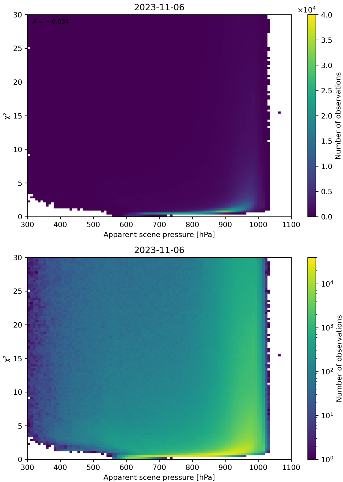
Figure 63: Scatter density plot of “Apparent scene pressure” against “ \chi^2 ” for 2023-11-05 to 2023-11-07.
