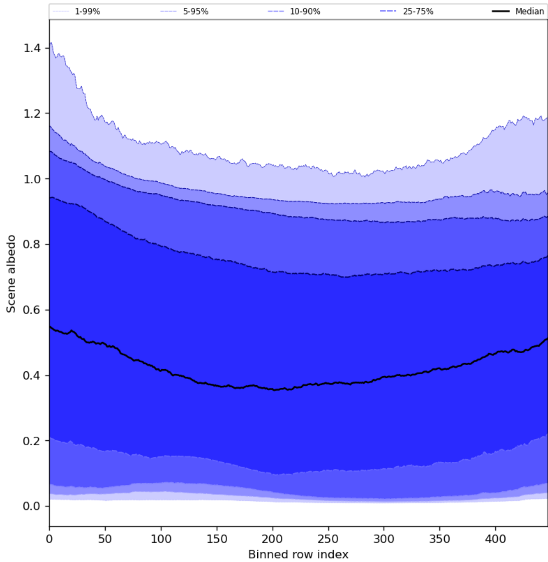
Figure 51: Along track statistics of “Scene albedo” for 2023-11-05 to 2023-11-07
