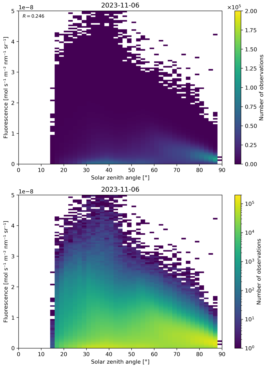
Figure 123: Scatter density plot of “Solar zenith angle” against “Fluorescence” for 2023-11-05 to 2023-11-07.
