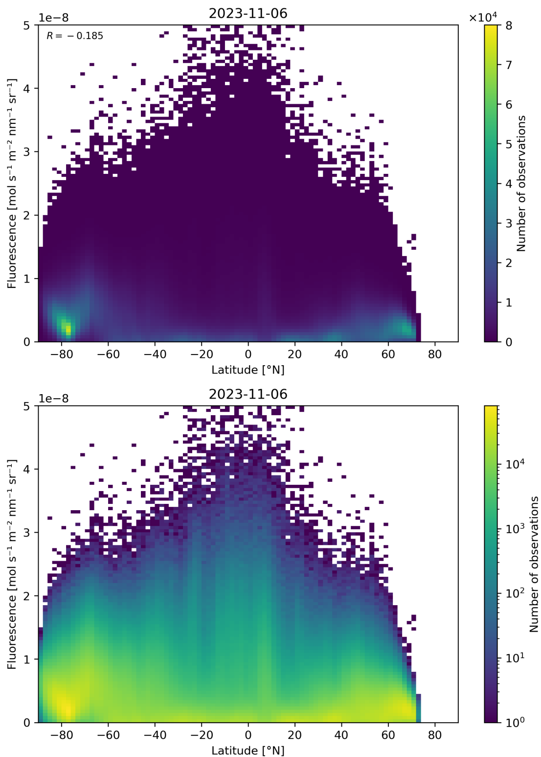
Figure 101: Scatter density plot of “Latitude” against “Fluorescence” for 2023-11-05 to 2023-11-07.
