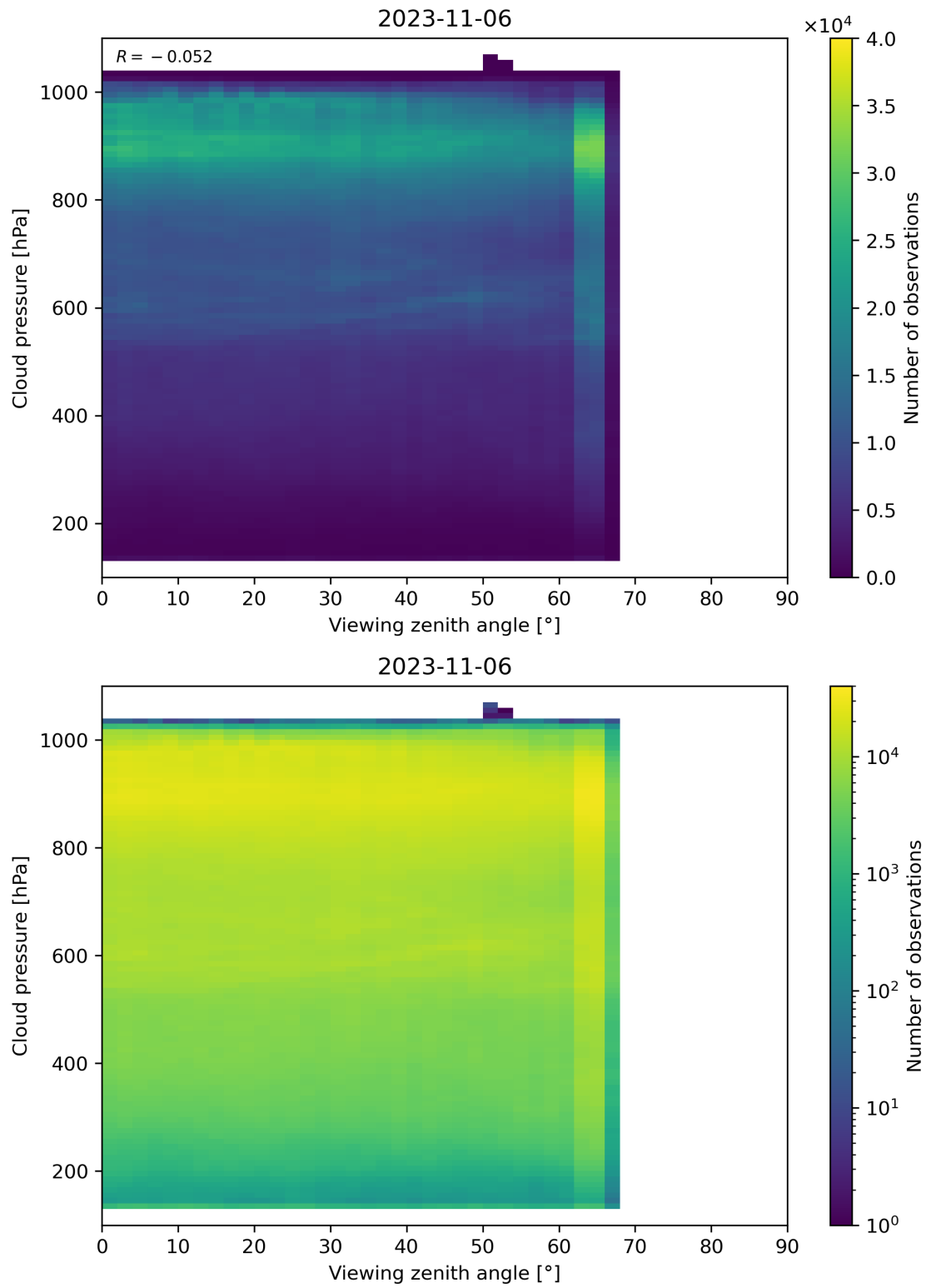
Figure 133: Scatter density plot of “Viewing zenith angle” against “Cloud pressure” for 2023-11-05 to 2023-11-07.
