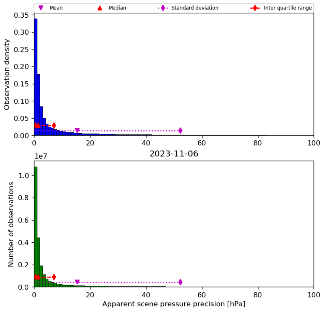
Figure 37: Histogram of “Apparent scene pressure precision” for 2023-11-05 to 2023-11-07
