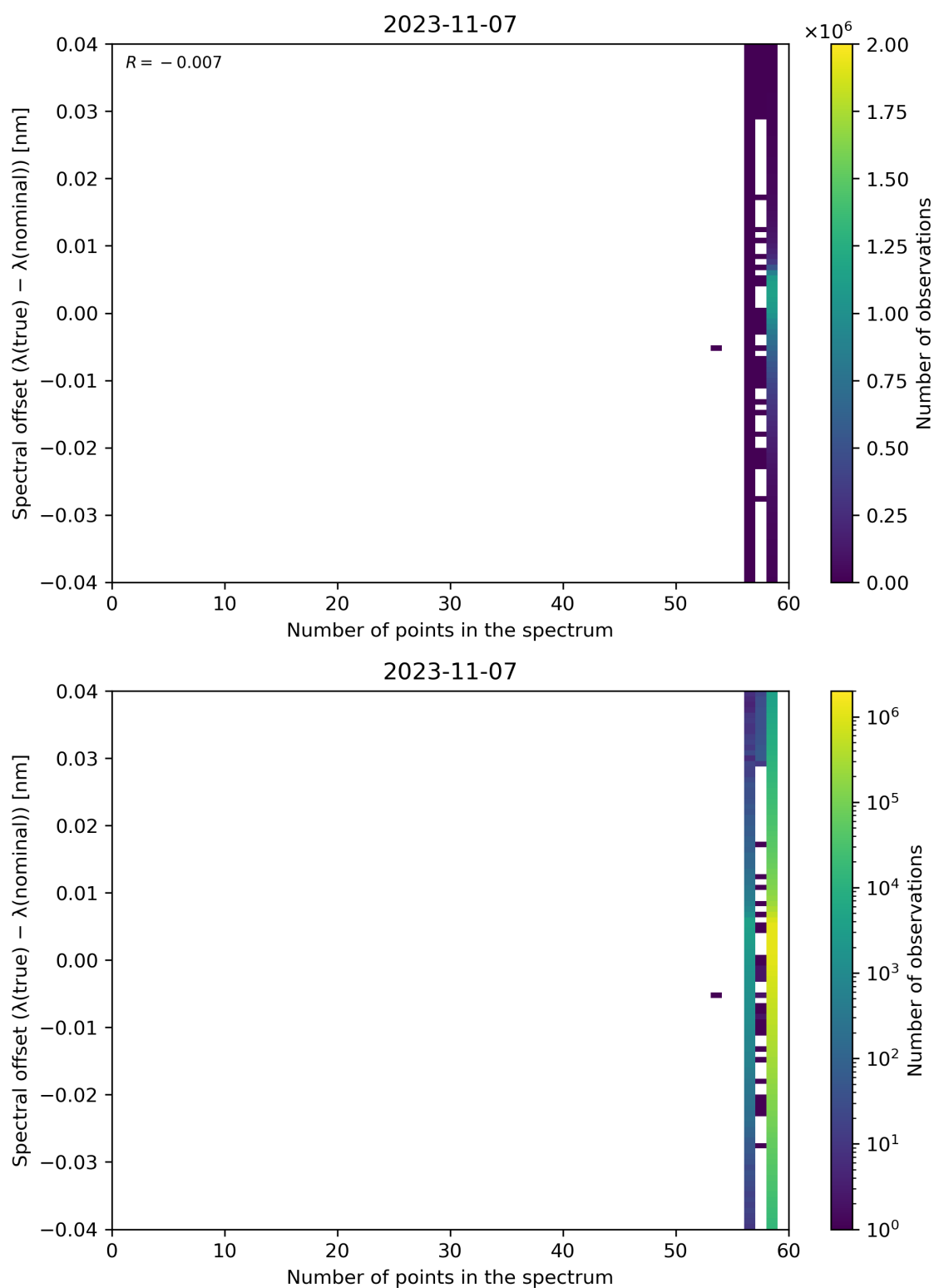
Figure 110: Scatter density plot of “Number of points in the spectrum” against “Spectral offset ( \lambda(\text{true}) - \lambda(\text{nominal}) )” for 2023-11-07 to 2023-11-08.
