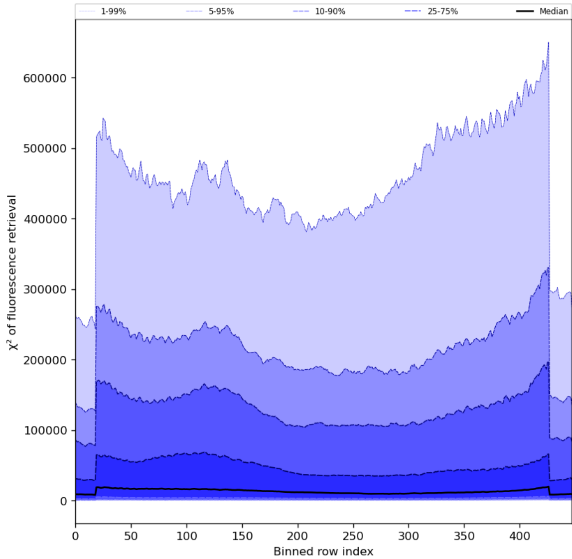
Figure 59: Along track statistics of “ \chi^2 of fluorescence retrieval” for 2023-11-07 to 2023-11-08
