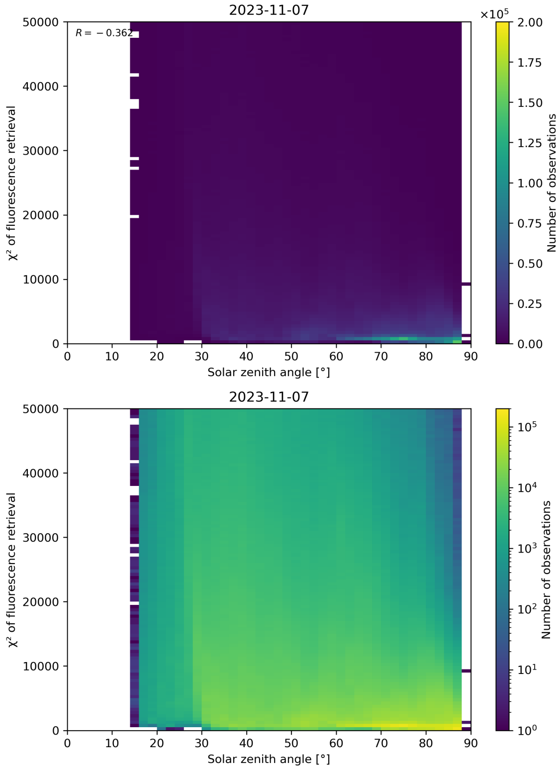
Figure 120: Scatter density plot of “Solar zenith angle” against “ \chi^2 of fluorescence retrieval” for 2023-11-07 to 2023-11-08.
