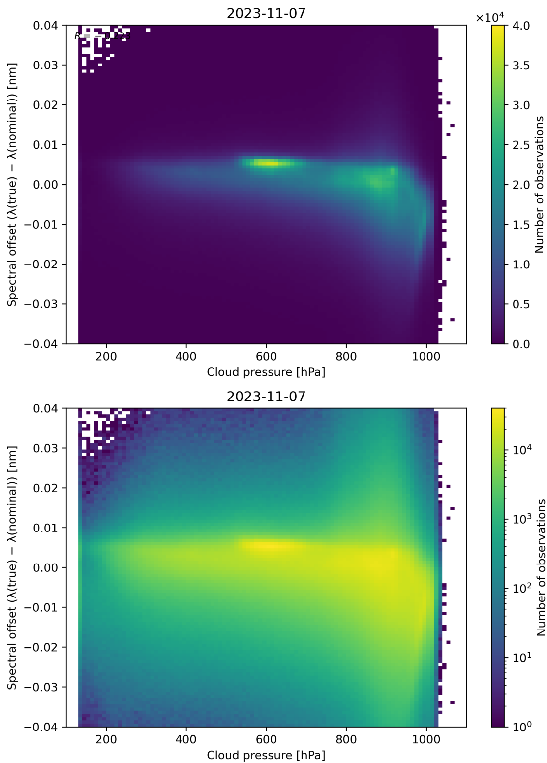
Figure 92: Scatter density plot of “Cloud pressure” against “Spectral offset ( \lambda(\text{true}) - \lambda(\text{nominal}) )” for 2023-11-07 to 2023-11-08.
