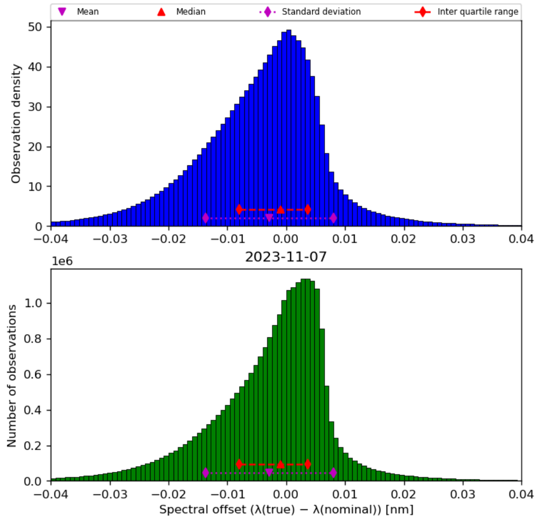
Figure 45: Histogram of “Spectral offset ( \lambda(\text{true}) - \lambda(\text{nominal}) )” for 2023-11-07 to 2023-11-08
