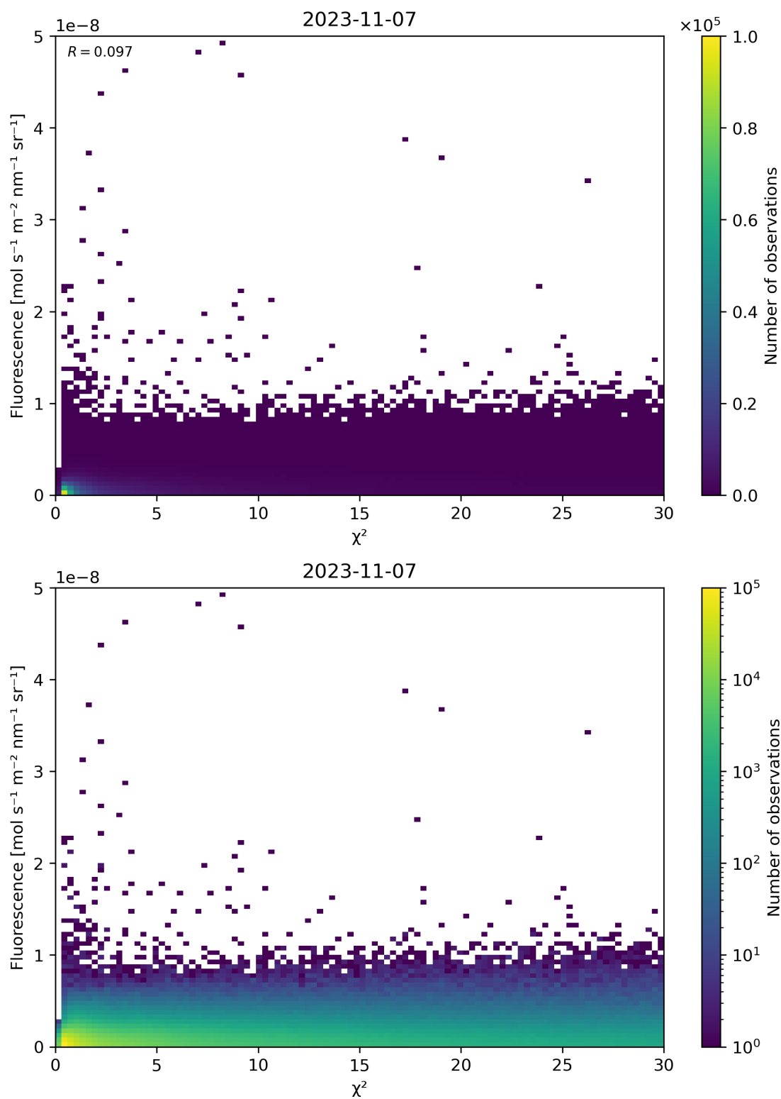
Figure 70: Scatter density plot of “ \chi^2 ” against “Fluorescence” for 2023-11-07 to 2023-11-08.
