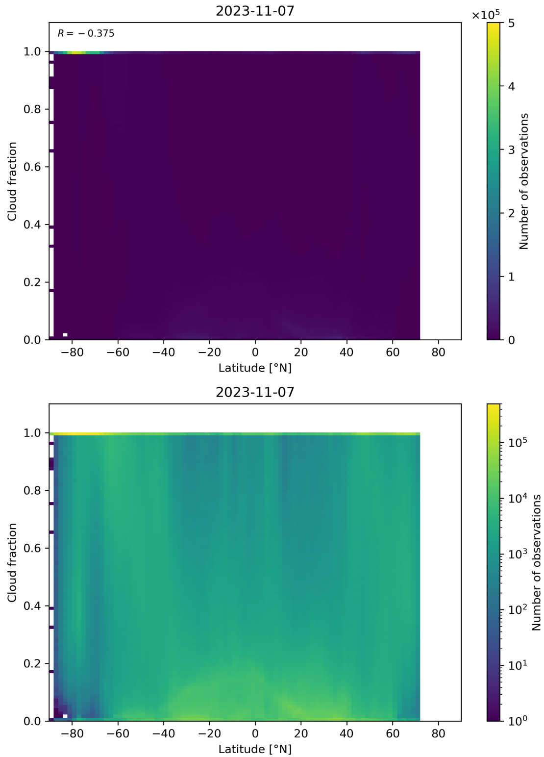
Figure 99: Scatter density plot of “Latitude” against “Cloud fraction” for 2023-11-07 to 2023-11-08.
