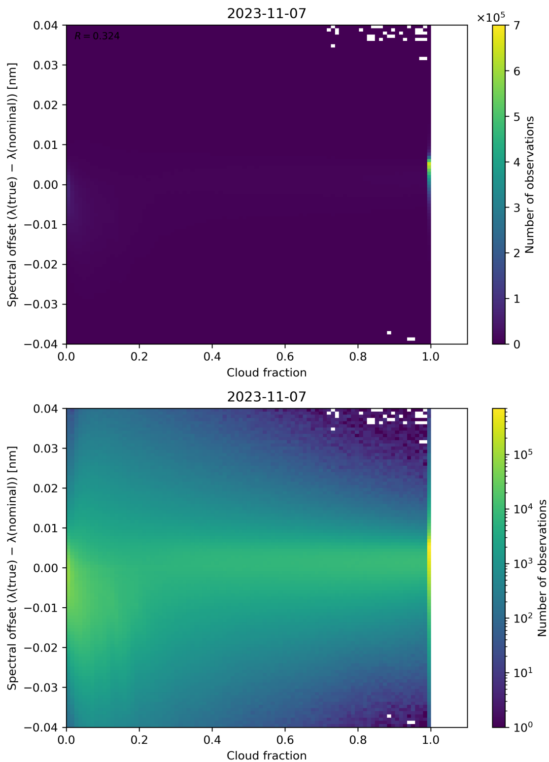
Figure 83: Scatter density plot of “Cloud fraction” against “Spectral offset ( \lambda(\text{true}) - \lambda(\text{nominal}) )” for 2023-11-07 to 2023-11-08.
