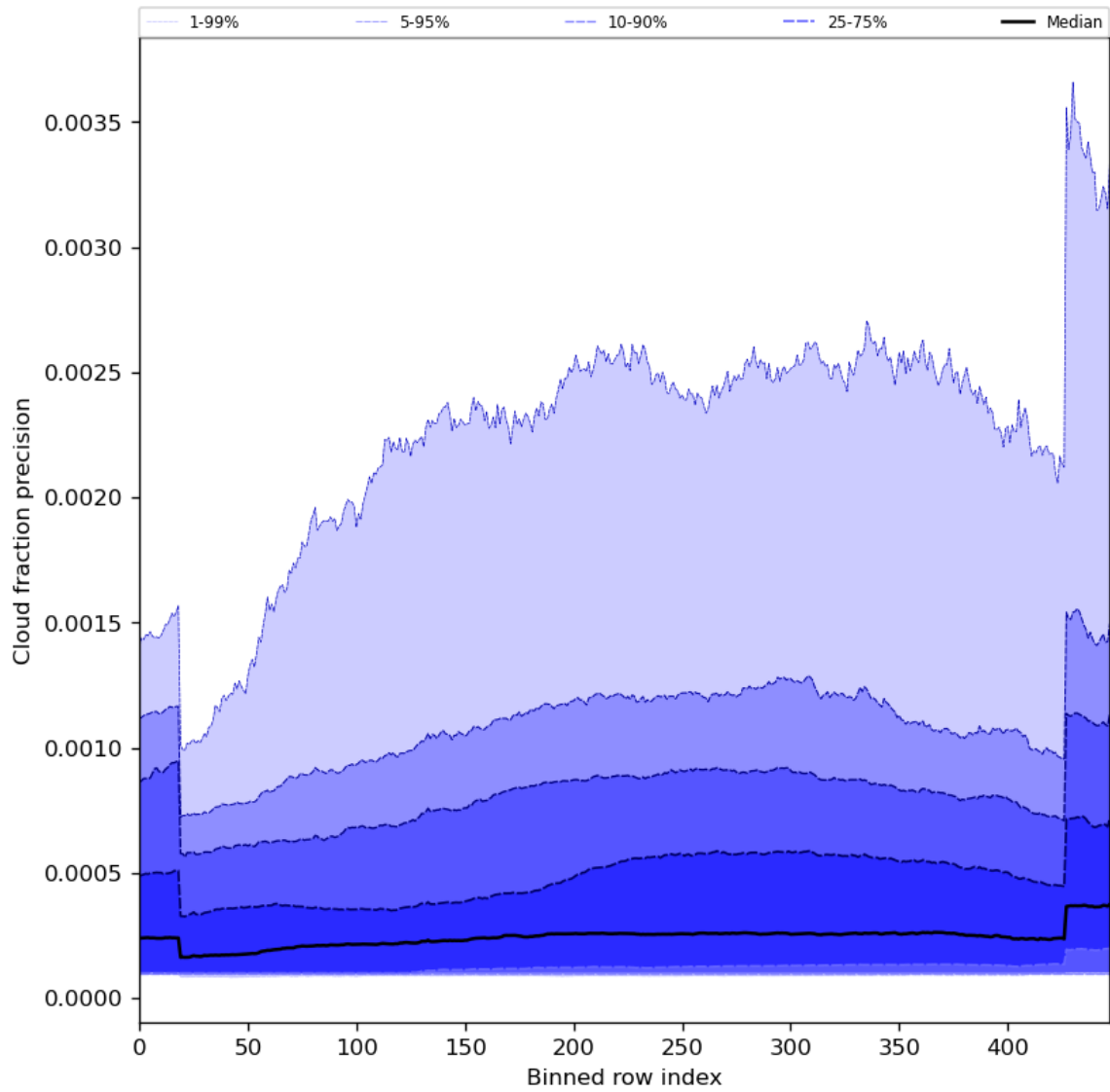
Figure 50: Along track statistics of “Cloud fraction precision” for 2023-11-07 to 2023-11-08
