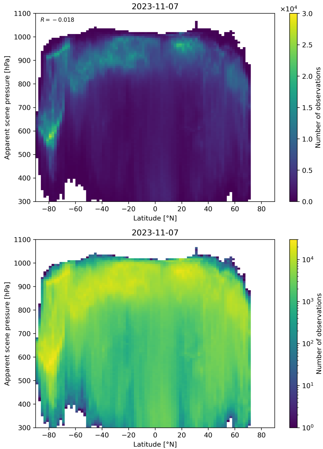
Figure 96: Scatter density plot of “Latitude” against “Apparent scene pressure” for 2023-11-07 to 2023-11-08.
