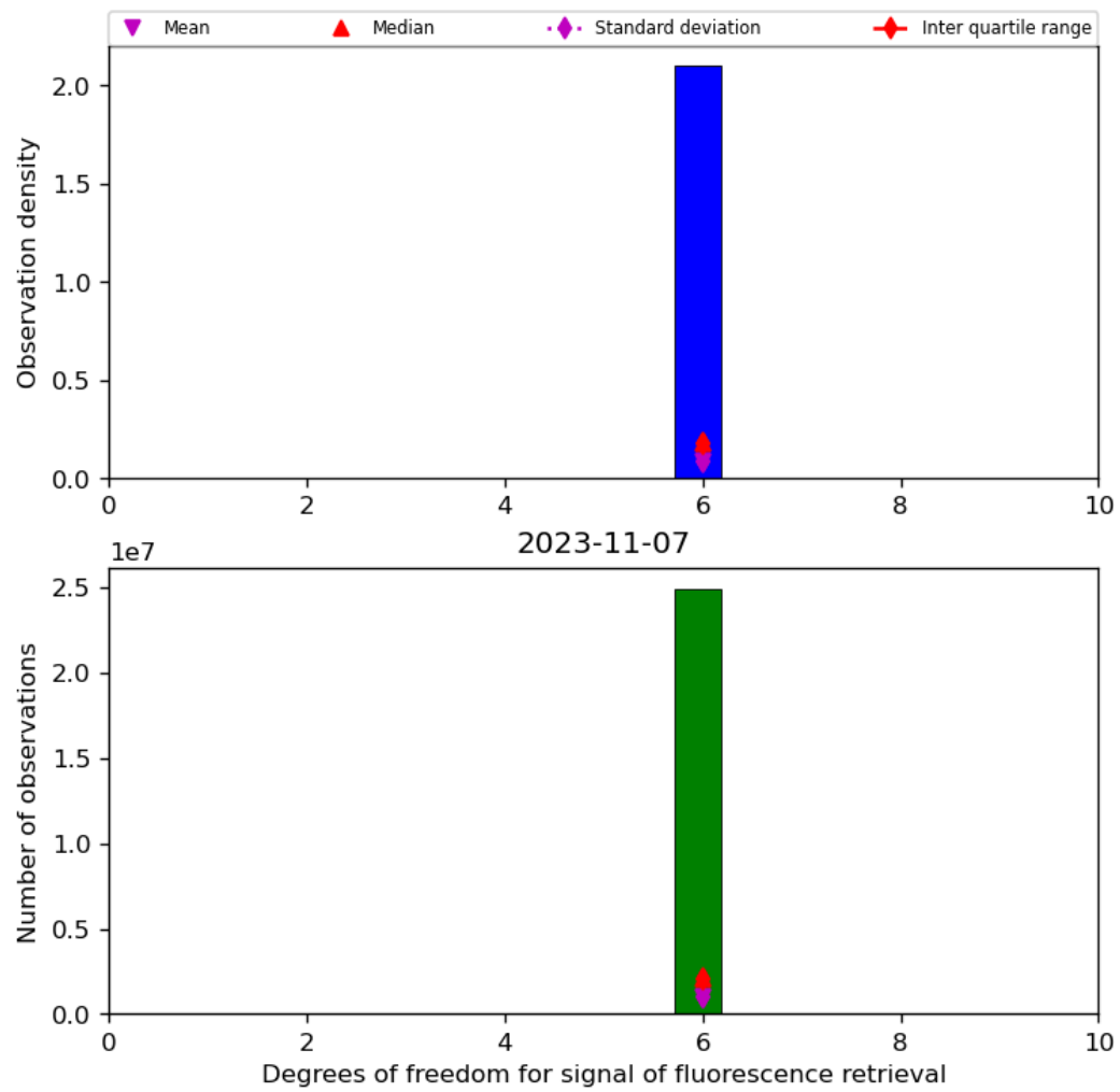
Figure 43: Histogram of “Degrees of freedom for signal of fluorescence retrieval” for 2023-11-07 to 2023-11-08
