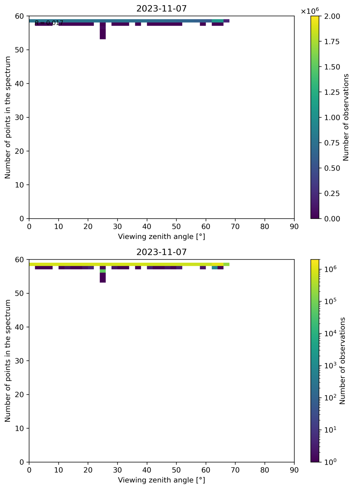
Figure 137: Scatter density plot of “Viewing zenith angle” against “Number of points in the spectrum” for 2023-11-07 to 2023-11-08.
