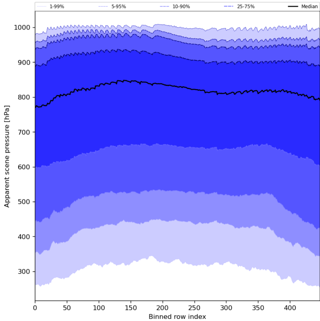
Figure 53: Along track statistics of “Apparent scene pressure” for 2023-11-07 to 2023-11-08
