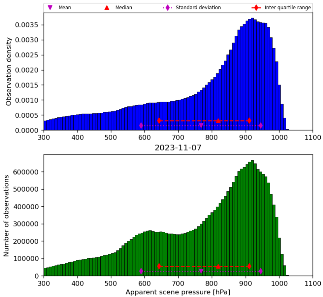
Figure 36: Histogram of “Apparent scene pressure” for 2023-11-07 to 2023-11-08
