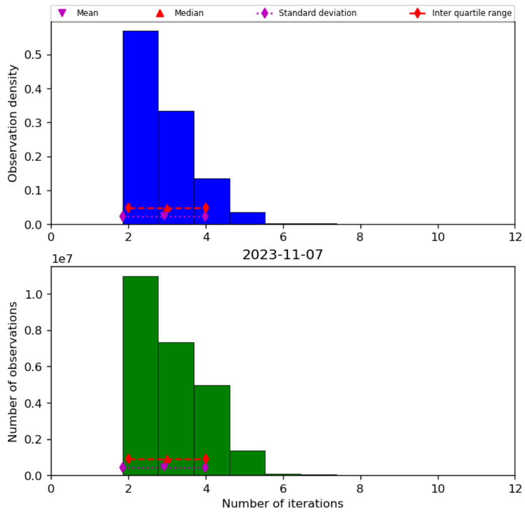
Figure 39: Histogram of “Number of iterations” for 2023-11-07 to 2023-11-08
