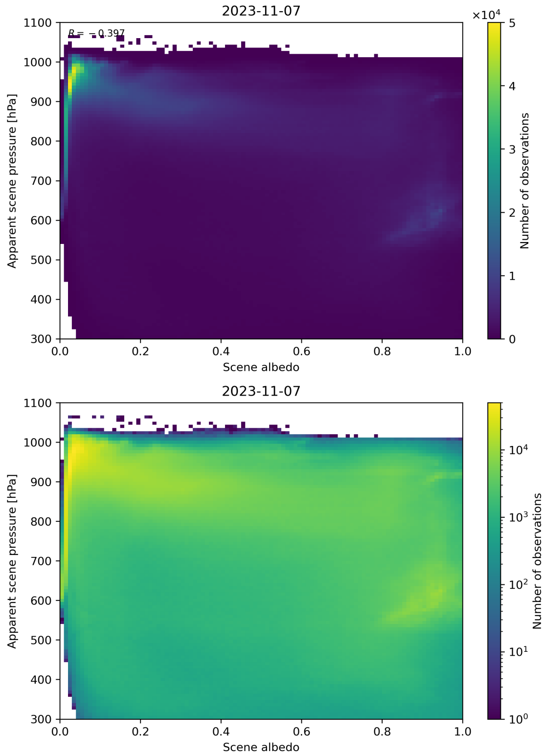
Figure 111: Scatter density plot of “Scene albedo” against “Apparent scene pressure” for 2023-11-07 to 2023-11-08.
