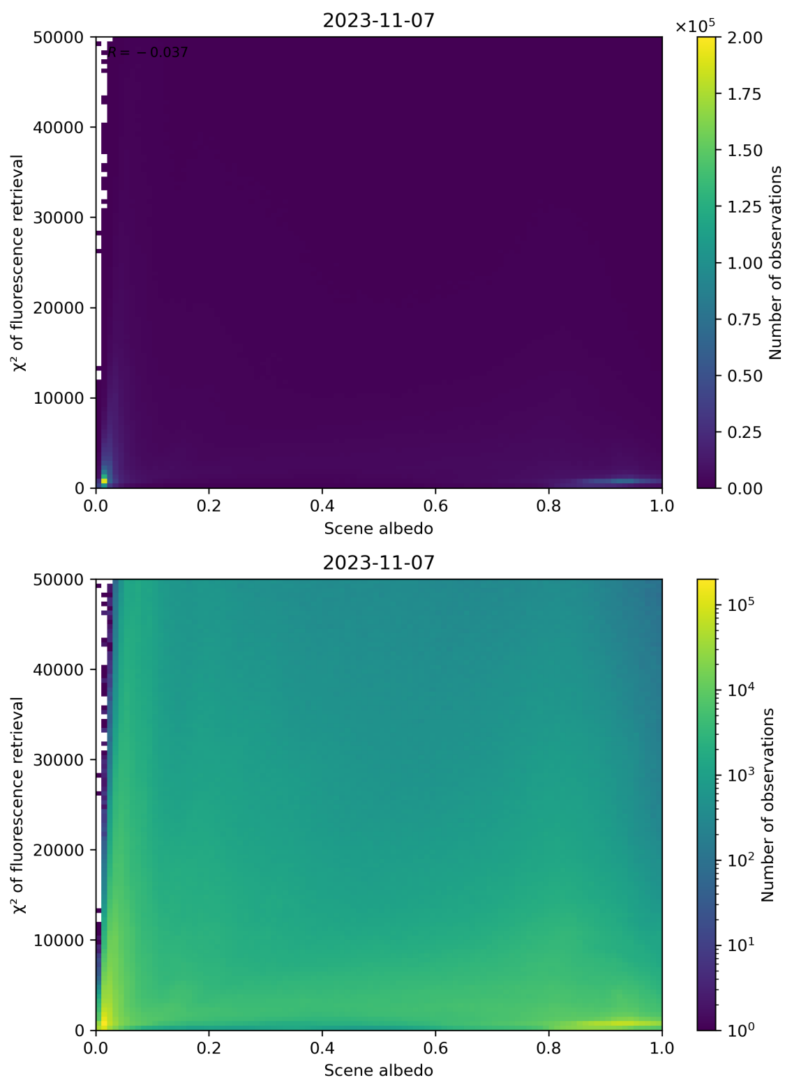
Figure 113: Scatter density plot of “Scene albedo” against “ \chi^2 of fluorescence retrieval” for 2023-11-07 to 2023-11-08.
