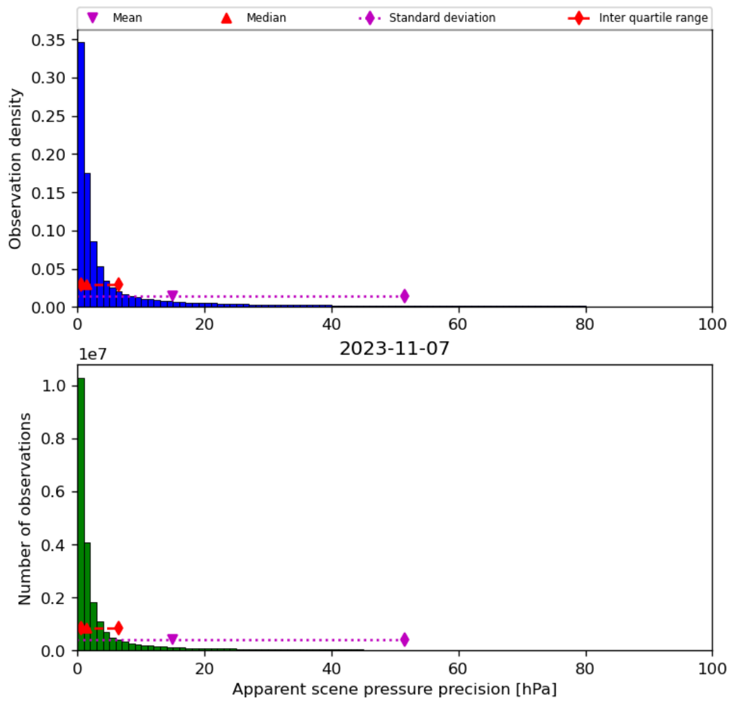
Figure 37: Histogram of “Apparent scene pressure precision” for 2023-11-07 to 2023-11-08
