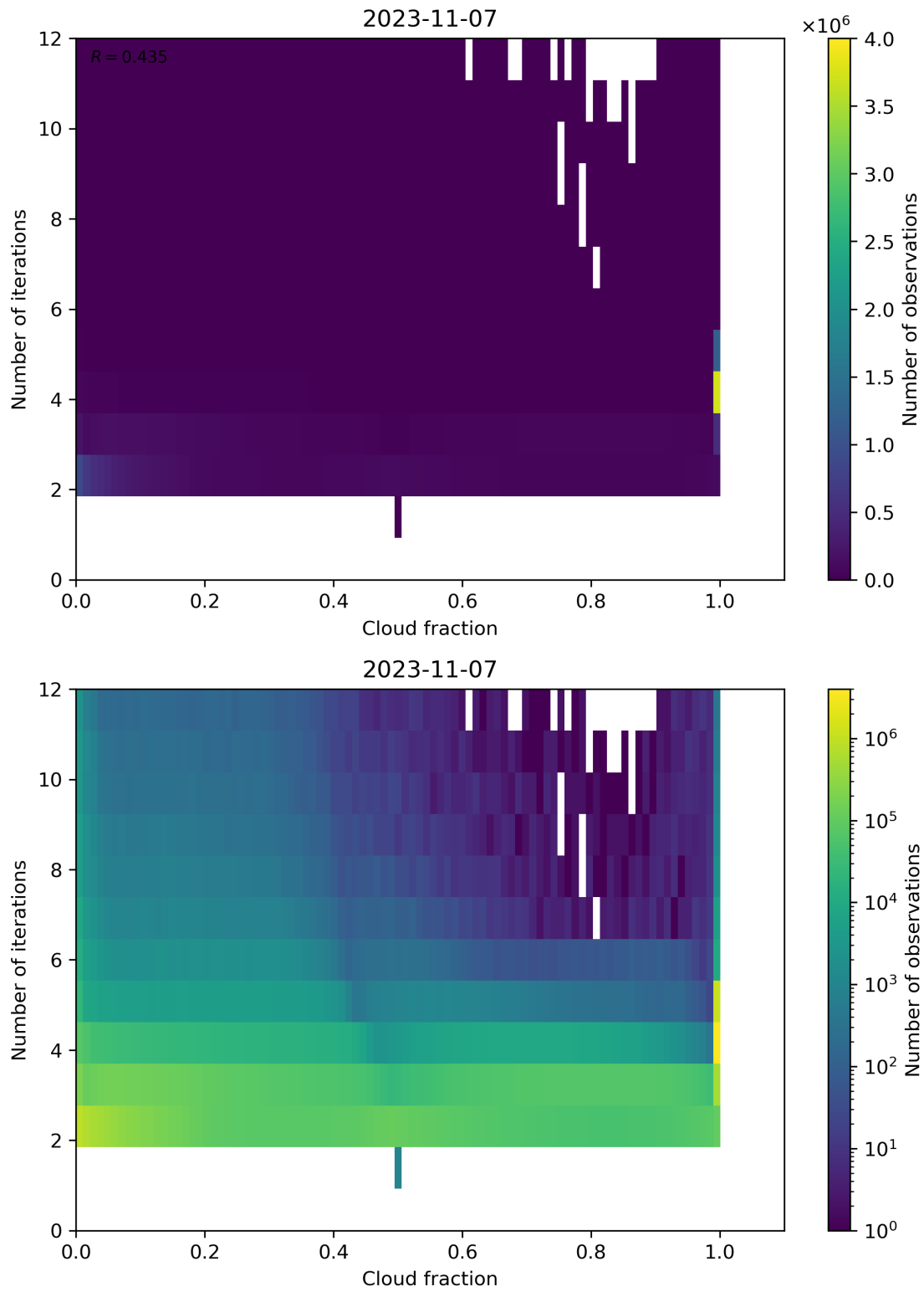
Figure 80: Scatter density plot of “Cloud fraction” against “Number of iterations” for 2023-11-07 to 2023-11-08.
