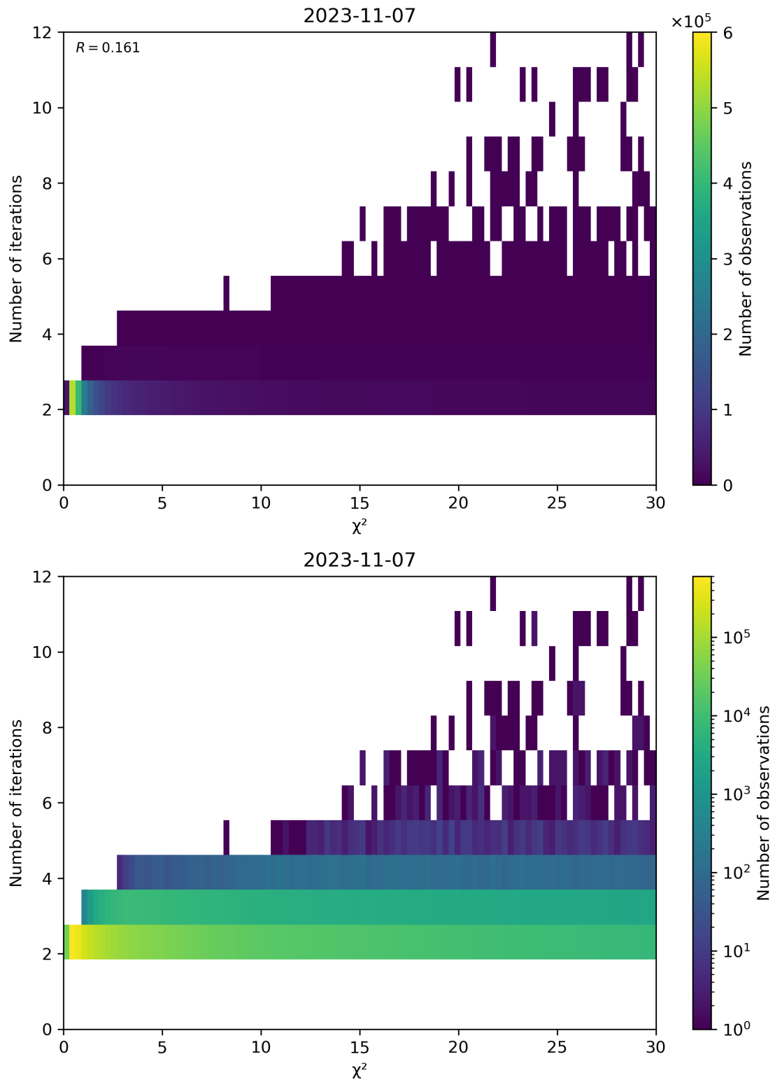
Figure 73: Scatter density plot of “ \chi^2 ” against “Number of iterations” for 2023-11-07 to 2023-11-08.
