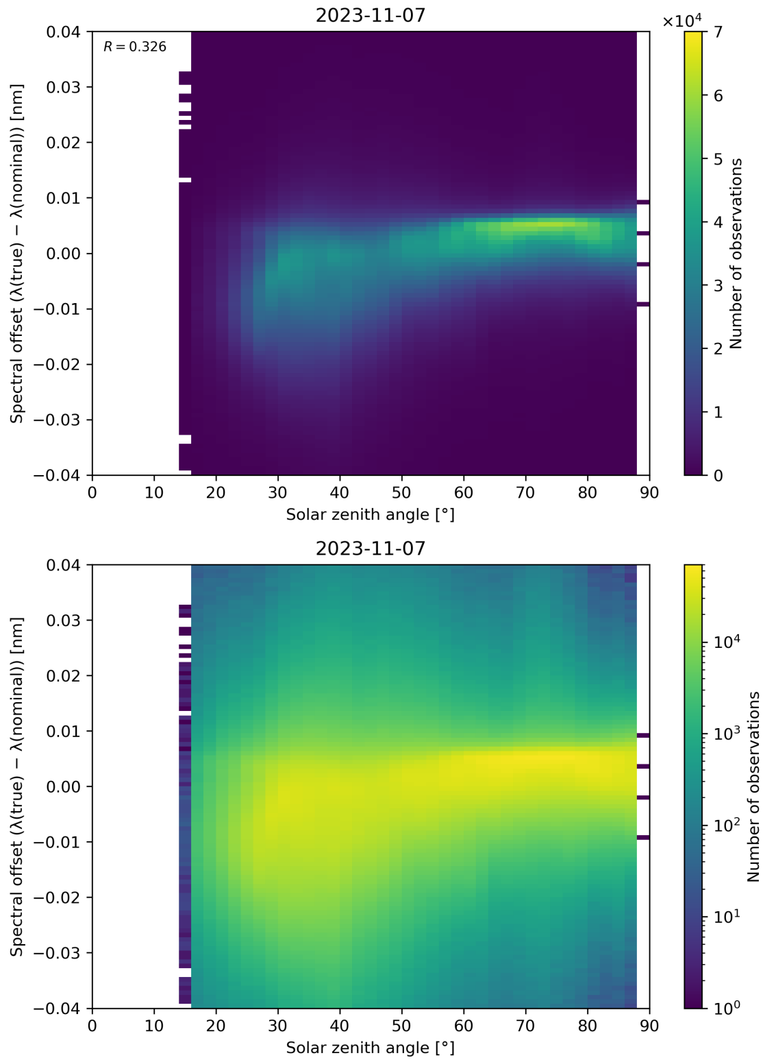
Figure 128: Scatter density plot of “Solar zenith angle” against “Spectral offset ( \lambda(\text{true}) - \lambda(\text{nominal}) )” for 2023-11-07 to 2023-11-08.
