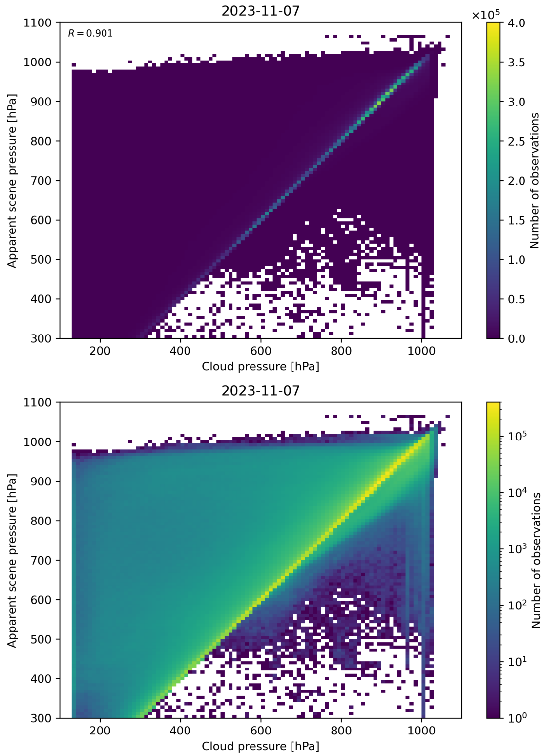
Figure 84: Scatter density plot of “Cloud pressure” against “Apparent scene pressure” for 2023-11-07 to 2023-11-08.
