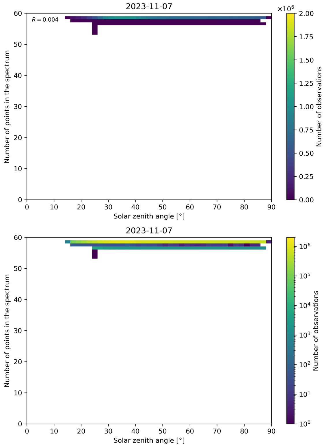
Figure 126: Scatter density plot of “Solar zenith angle” against “Number of points in the spectrum” for 2023-11-07 to 2023-11-08.
