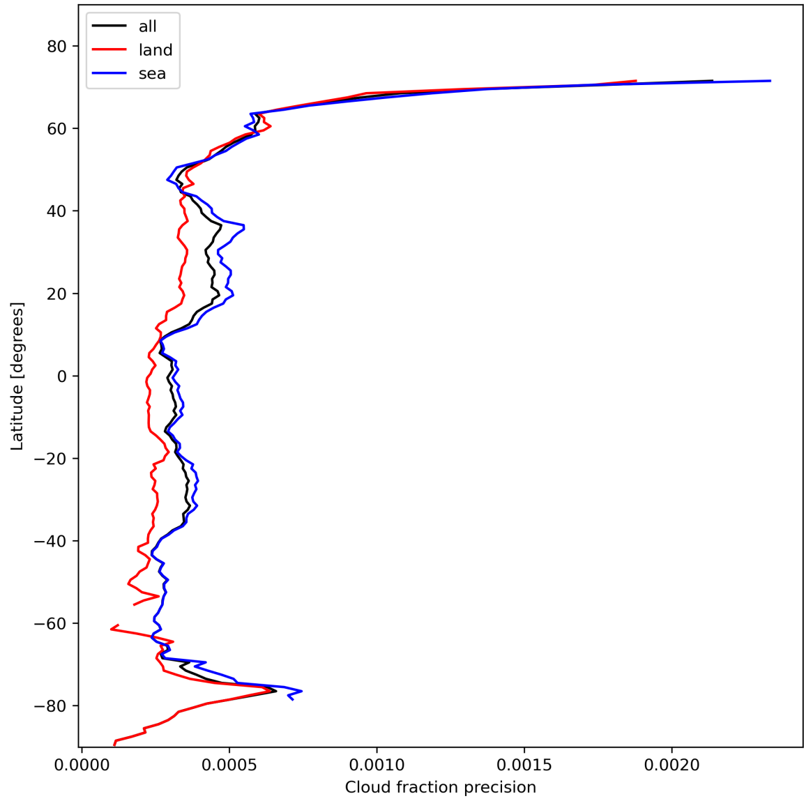
Figure 16: Zonal average of “Cloud fraction precision” for 2023-11-07 to 2023-11-08.
