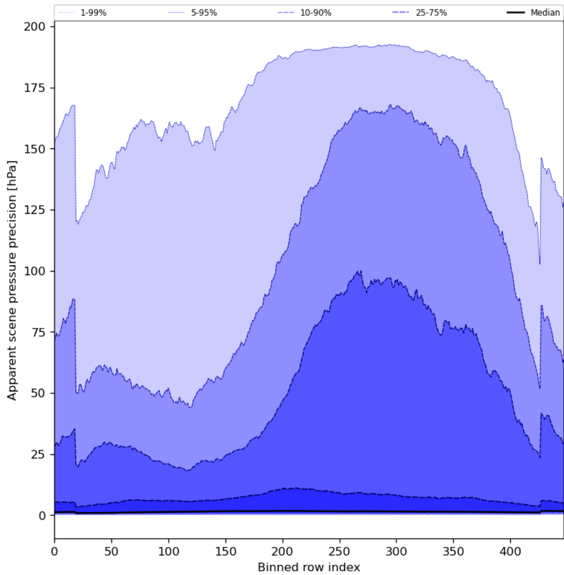
Figure 54: Along track statistics of “Apparent scene pressure precision” for 2023-11-07 to 2023-11-08
