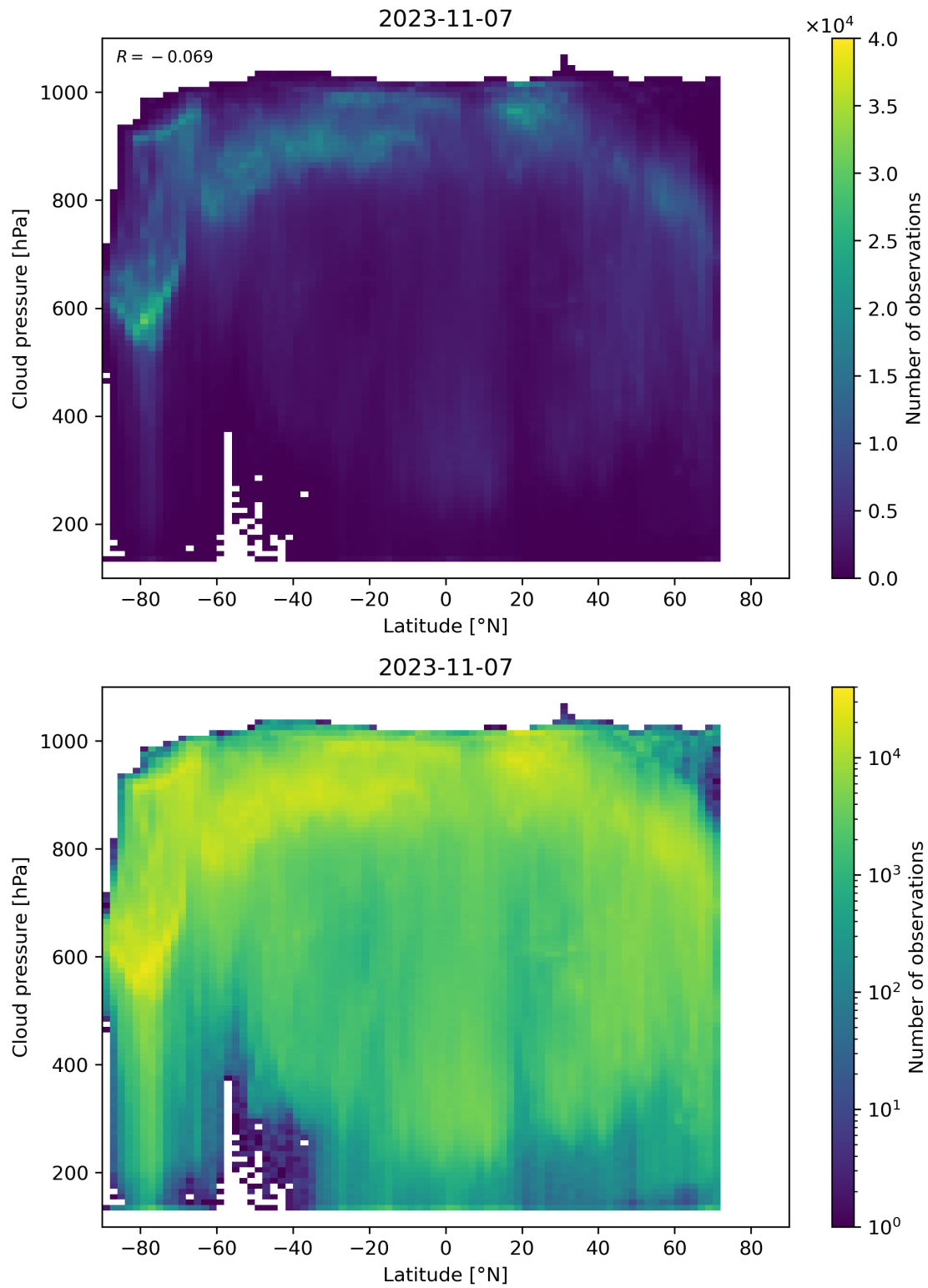
Figure 100: Scatter density plot of “Latitude” against “Cloud pressure” for 2023-11-07 to 2023-11-08.
