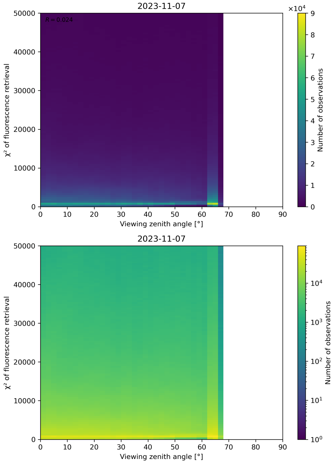
Figure 131: Scatter density plot of “Viewing zenith angle” against “ \chi^2 of fluorescence retrieval” for 2023-11-07 to 2023-11-08.
