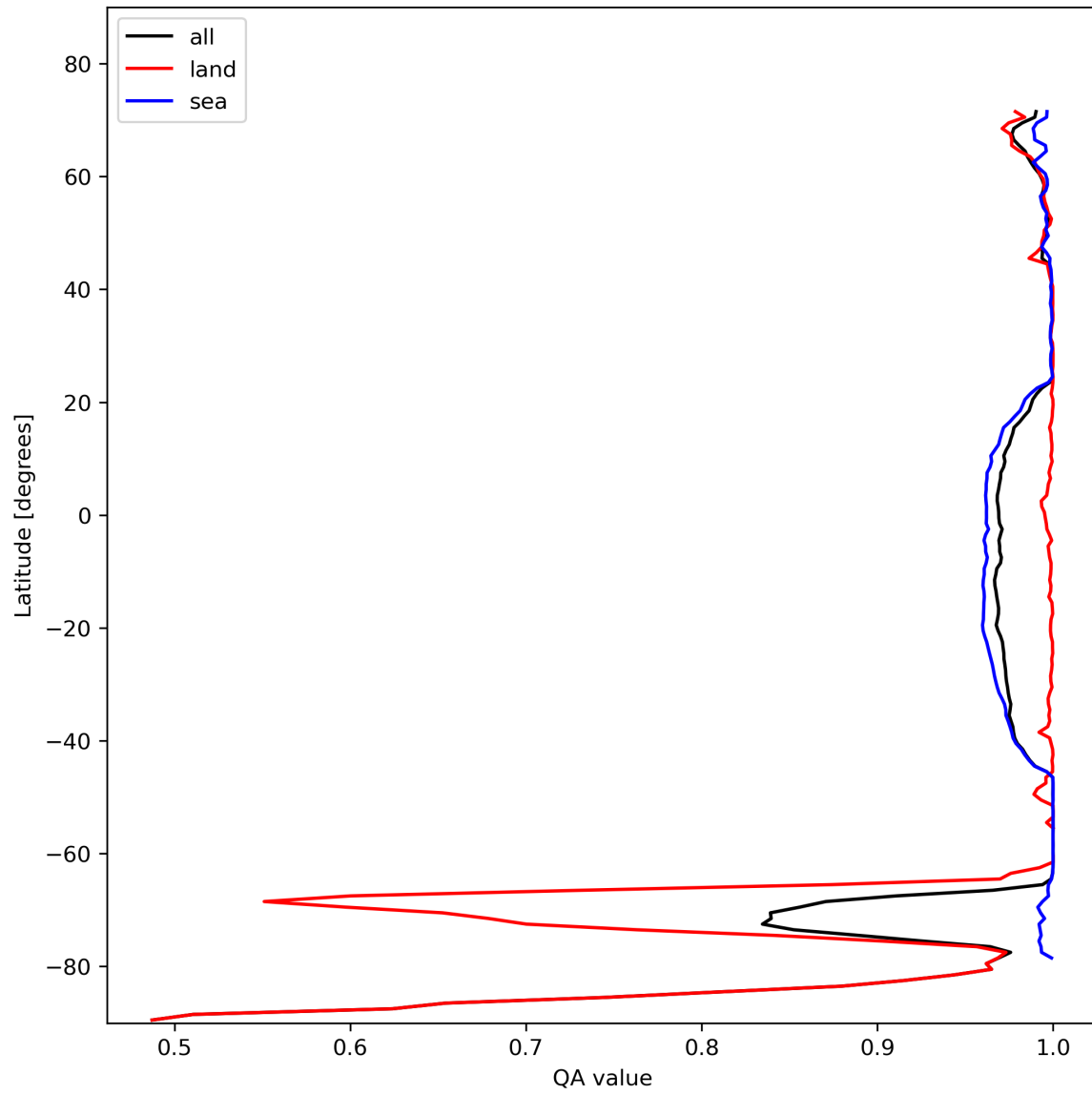
Figure 12: Zonal average of “QA value” for 2023-11-07 to 2023-11-08.
