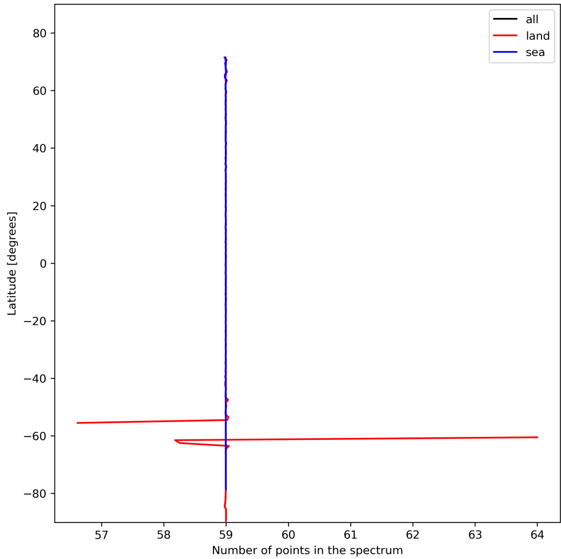
Figure 27: Zonal average of “Number of points in the spectrum” for 2023-11-07 to 2023-11-08.
