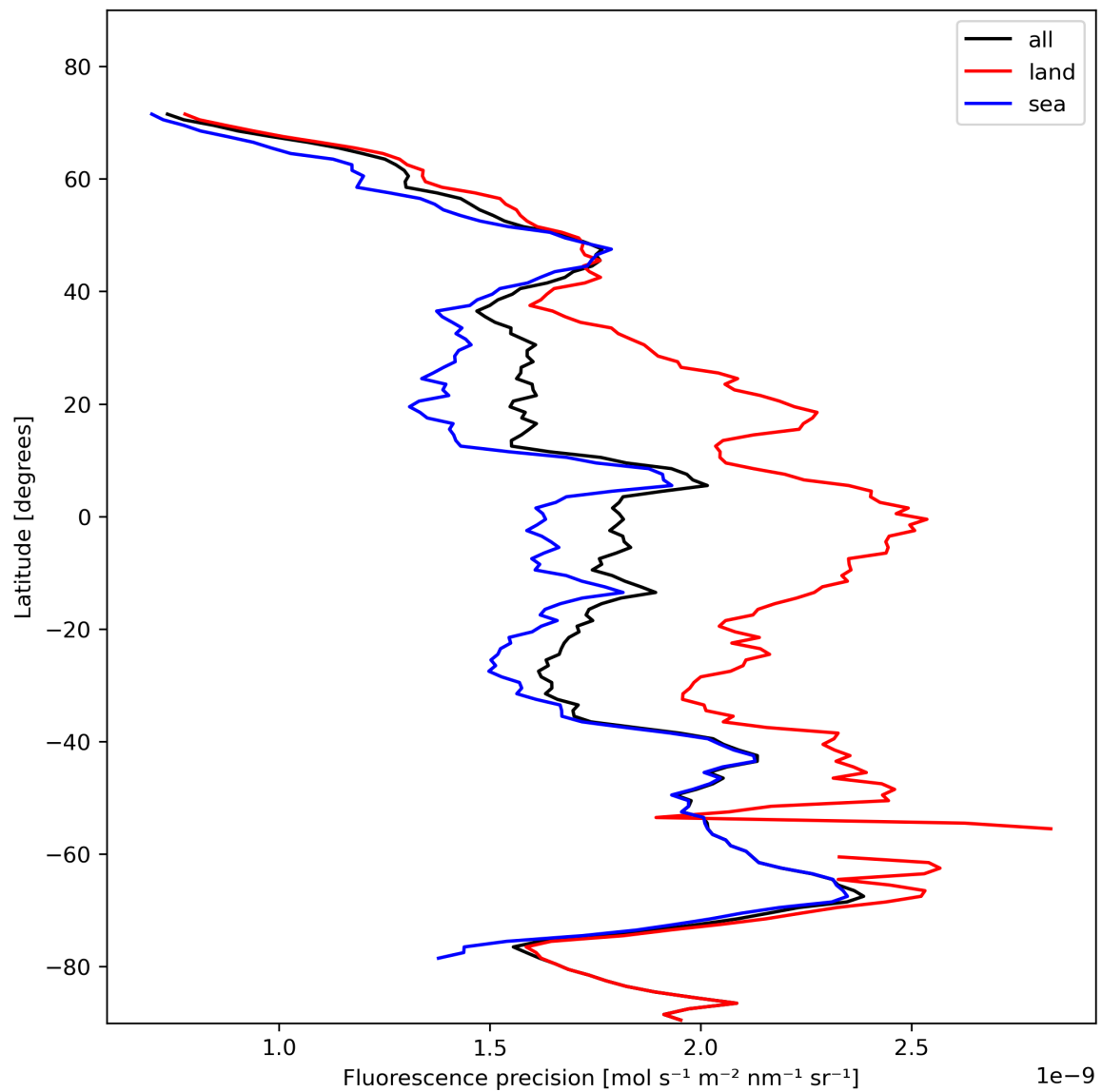
Figure 24: Zonal average of “Fluorescence precision” for 2023-11-07 to 2023-11-08.
