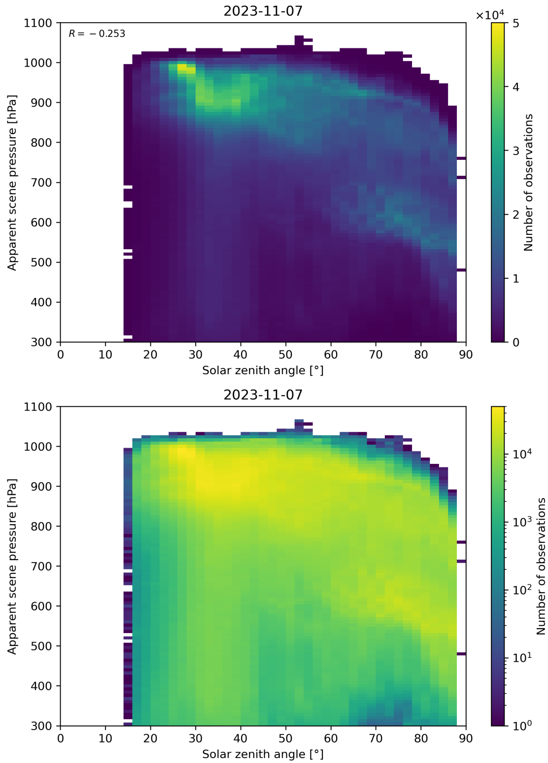
Figure 118: Scatter density plot of “Solar zenith angle” against “Apparent scene pressure” for 2023-11-07 to 2023-11-08.
