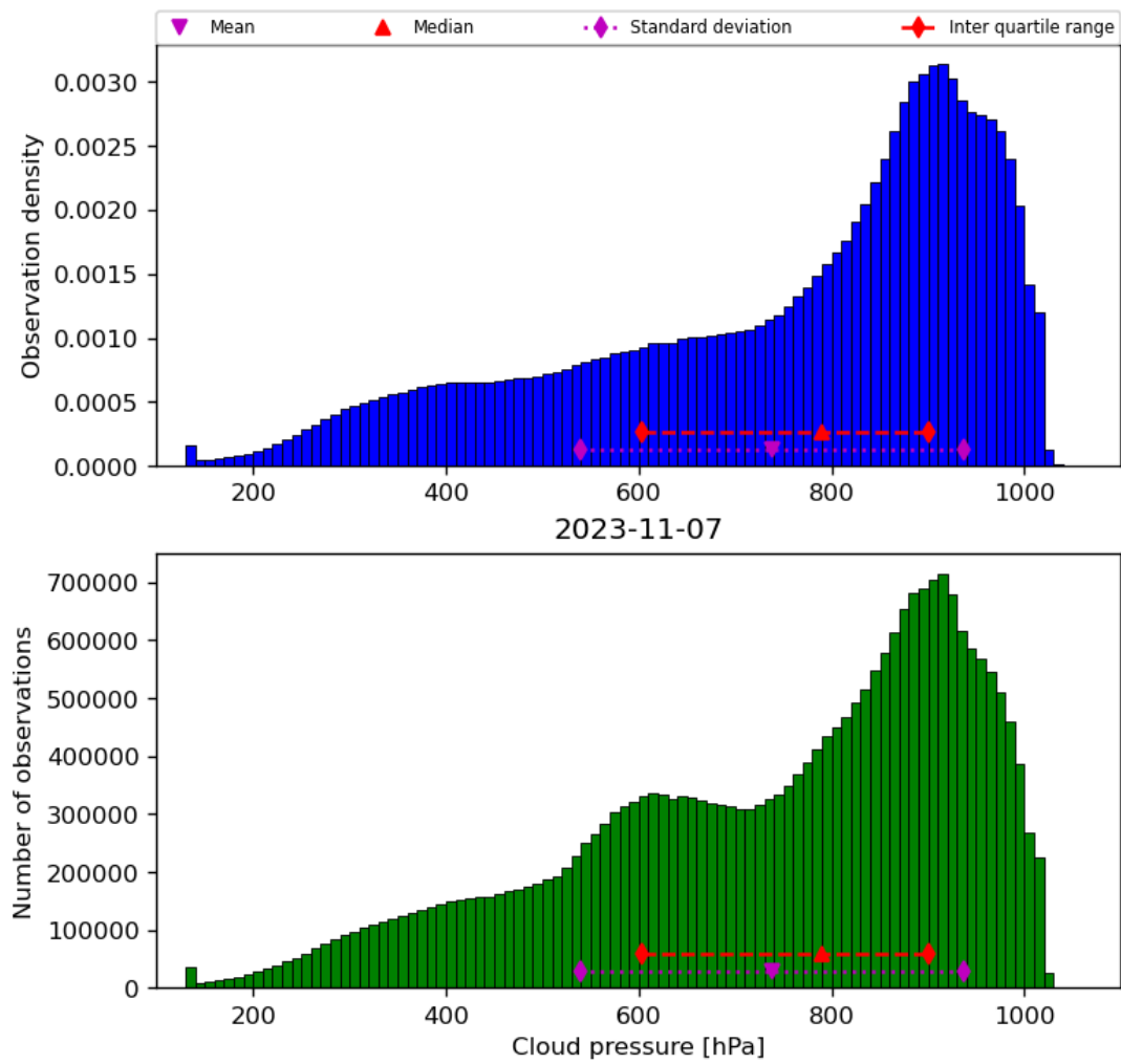
Figure 30: Histogram of “Cloud pressure” for 2023-11-07 to 2023-11-08
