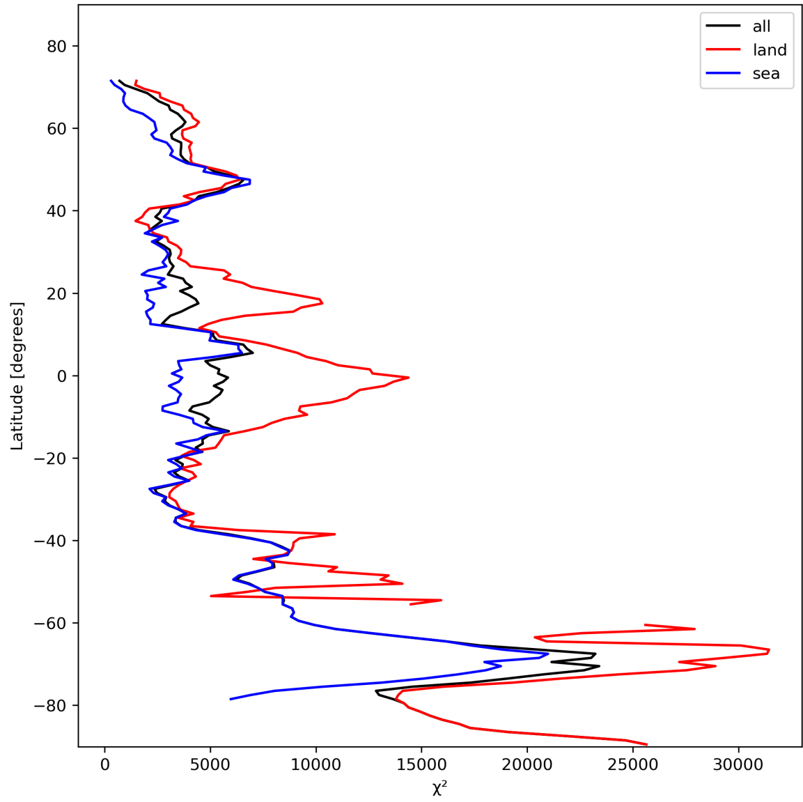
Figure 21: Zonal average of “ \chi^2 ” for 2023-11-07 to 2023-11-08.
