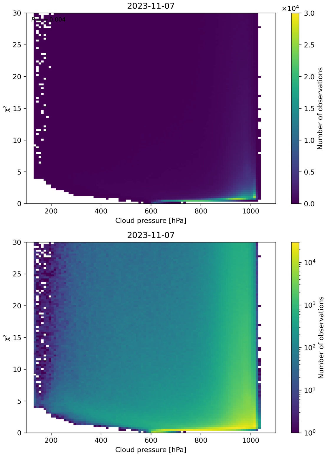
Figure 85: Scatter density plot of “Cloud pressure” against “ \chi^2 ” for 2023-11-07 to 2023-11-08.
