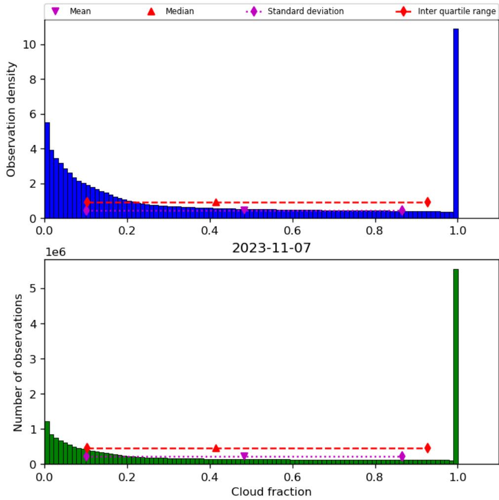
Figure 32: Histogram of “Cloud fraction” for 2023-11-07 to 2023-11-08
