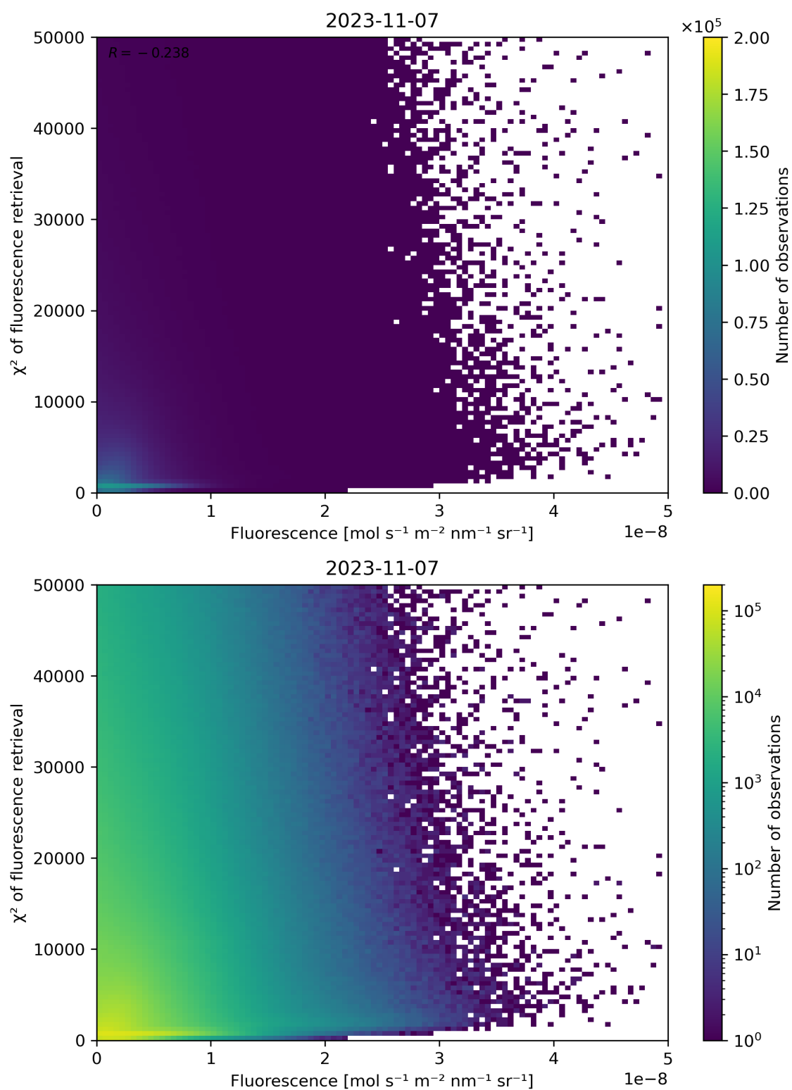
Figure 93: Scatter density plot of “Fluorescence” against “ \chi^2 of fluorescence retrieval” for 2023-11-07 to 2023-11-08.
