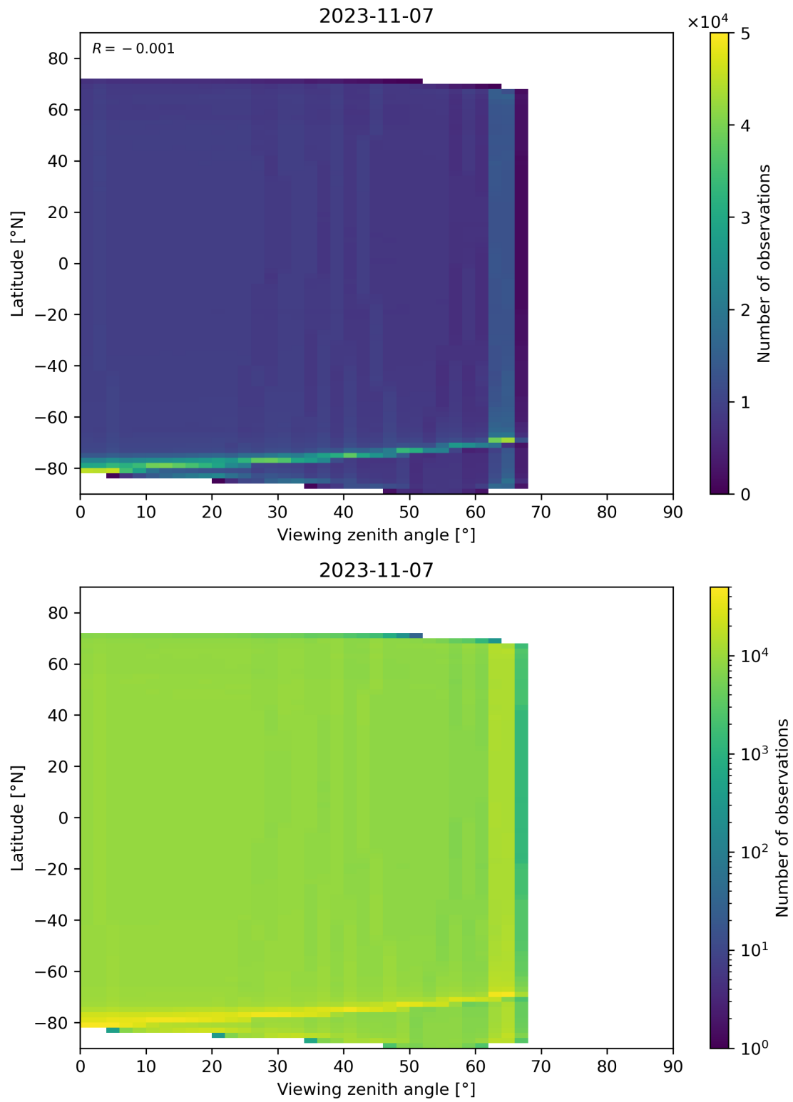
Figure 135: Scatter density plot of “Viewing zenith angle” against “Latitude” for 2023-11-07 to 2023-11-08.
