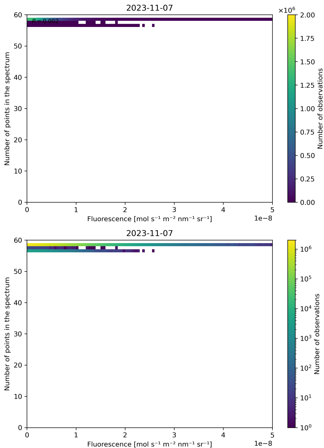
Figure 94: Scatter density plot of “Fluorescence” against “Number of points in the spectrum” for 2023-11-07 to 2023-11-08.
