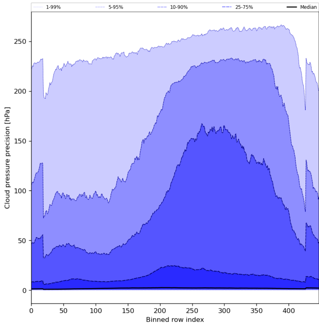
Figure 48: Along track statistics of “Cloud pressure precision” for 2023-11-07 to 2023-11-08
