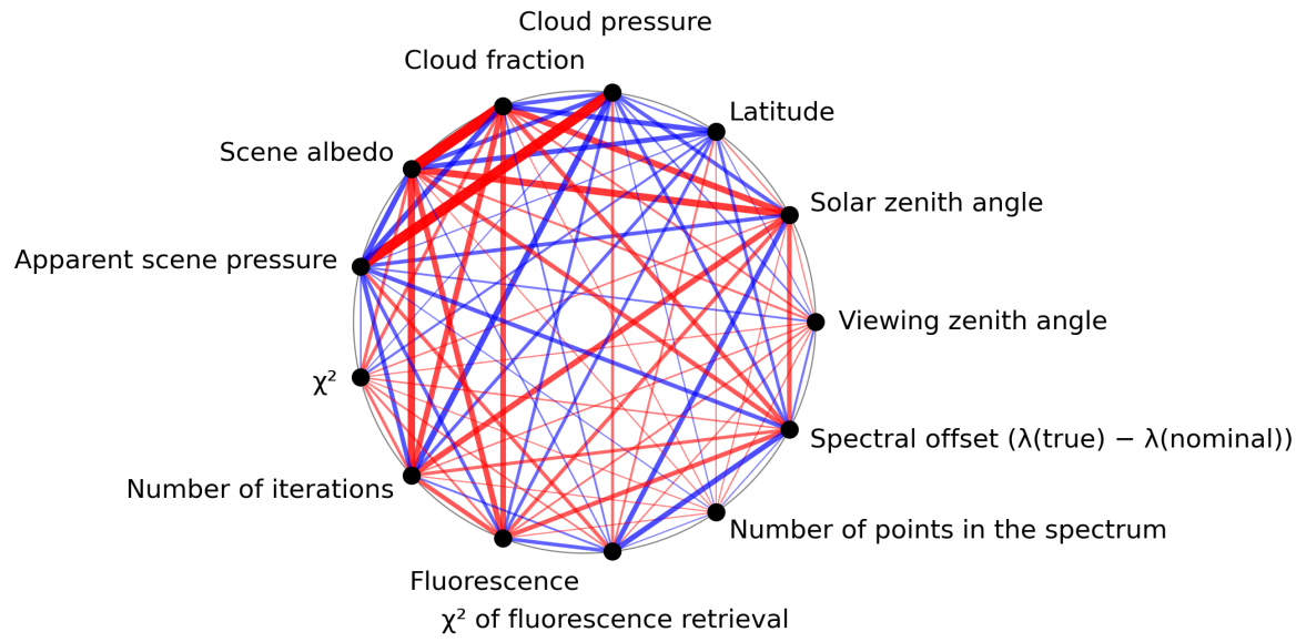
Figure 1: Map of correlation graph for 2023-11-07 to 2023-11-08.
