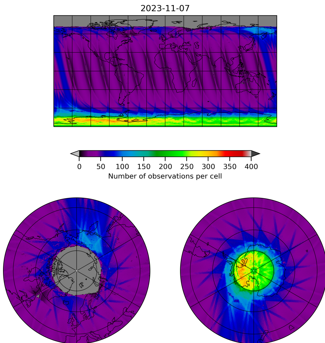
Figure 11: Map of the number of observations for 2023-11-07 to 2023-11-08
