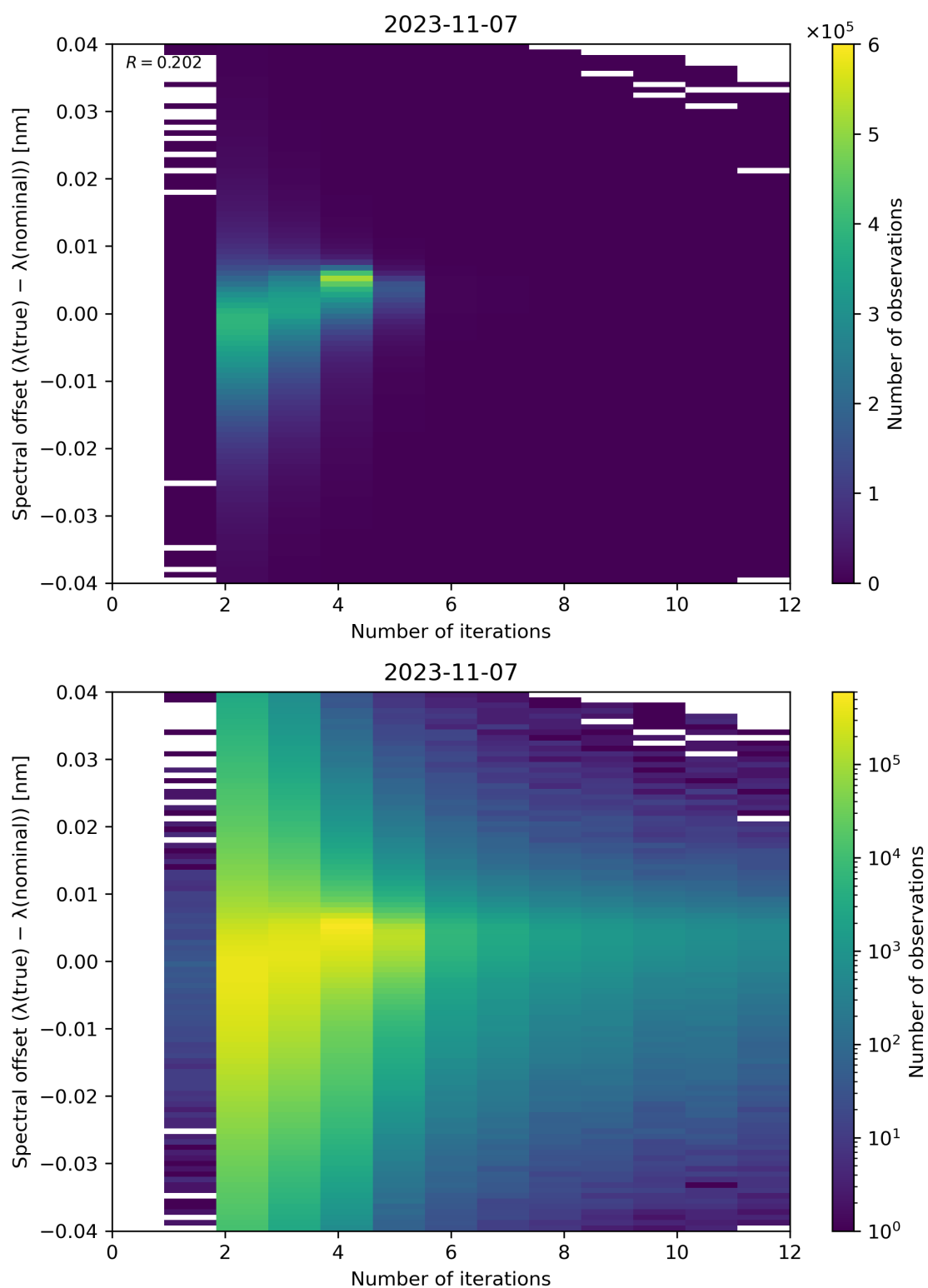
Figure 109: Scatter density plot of “Number of iterations” against “Spectral offset ( \lambda(\text{true}) - \lambda(\text{nominal}) )” for 2023-11-07 to 2023-11-08.
