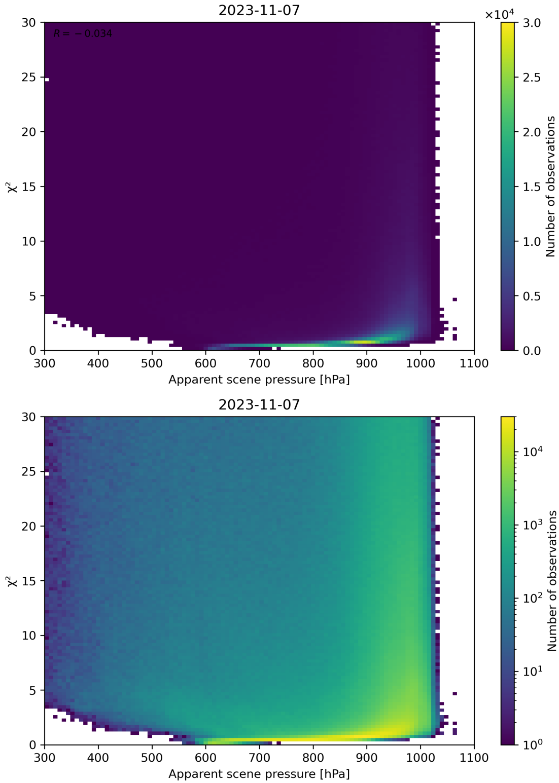
Figure 63: Scatter density plot of “Apparent scene pressure” against “ \chi^2 ” for 2023-11-07 to 2023-11-08.
