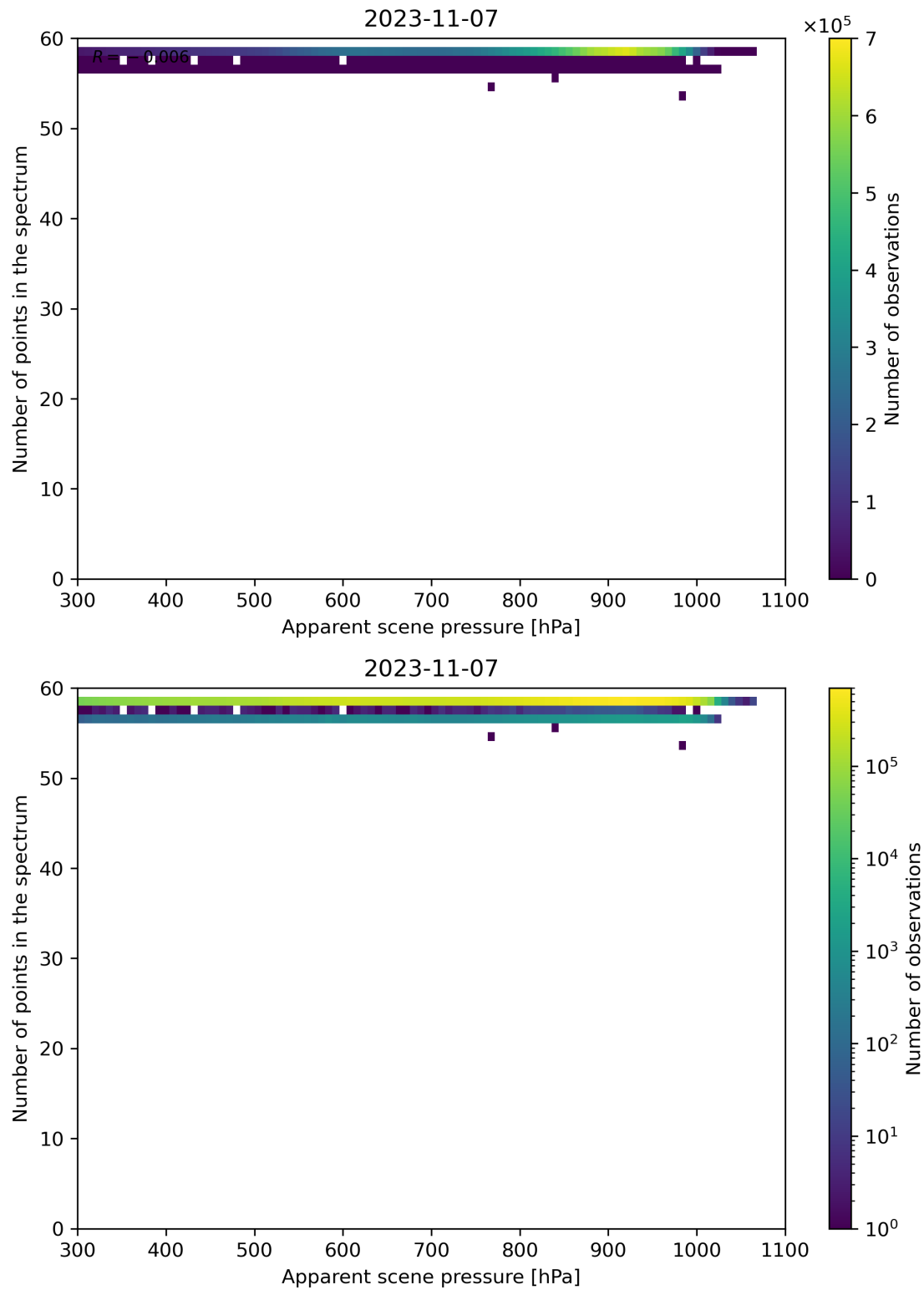
Figure 67: Scatter density plot of “Apparent scene pressure” against “Number of points in the spectrum” for 2023-11-07 to 2023-11-08.
