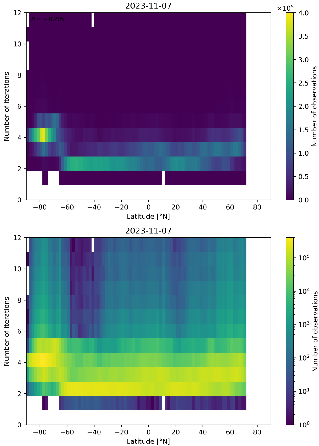
Figure 102: Scatter density plot of “Latitude” against “Number of iterations” for 2023-11-07 to 2023-11-08.
