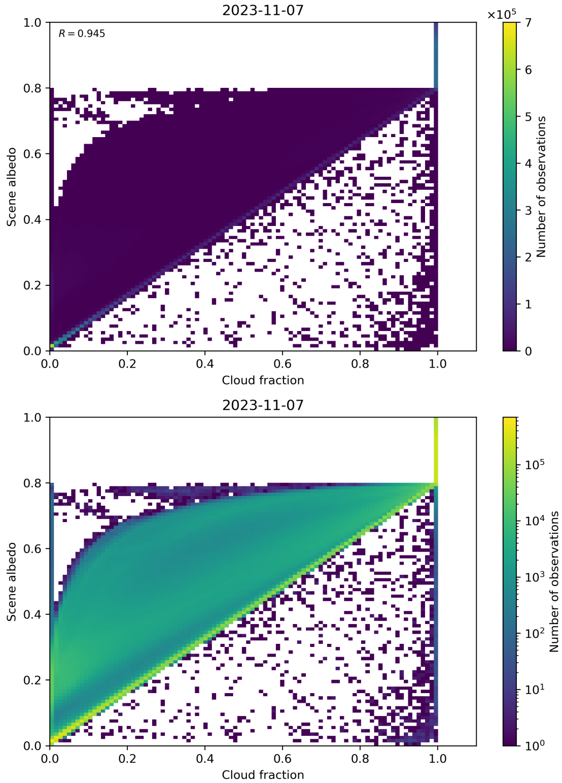
Figure 82: Scatter density plot of “Cloud fraction” against “Scene albedo” for 2023-11-07 to 2023-11-08.
