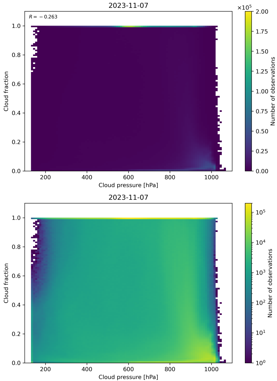
Figure 87: Scatter density plot of “Cloud pressure” against “Cloud fraction” for 2023-11-07 to 2023-11-08.
