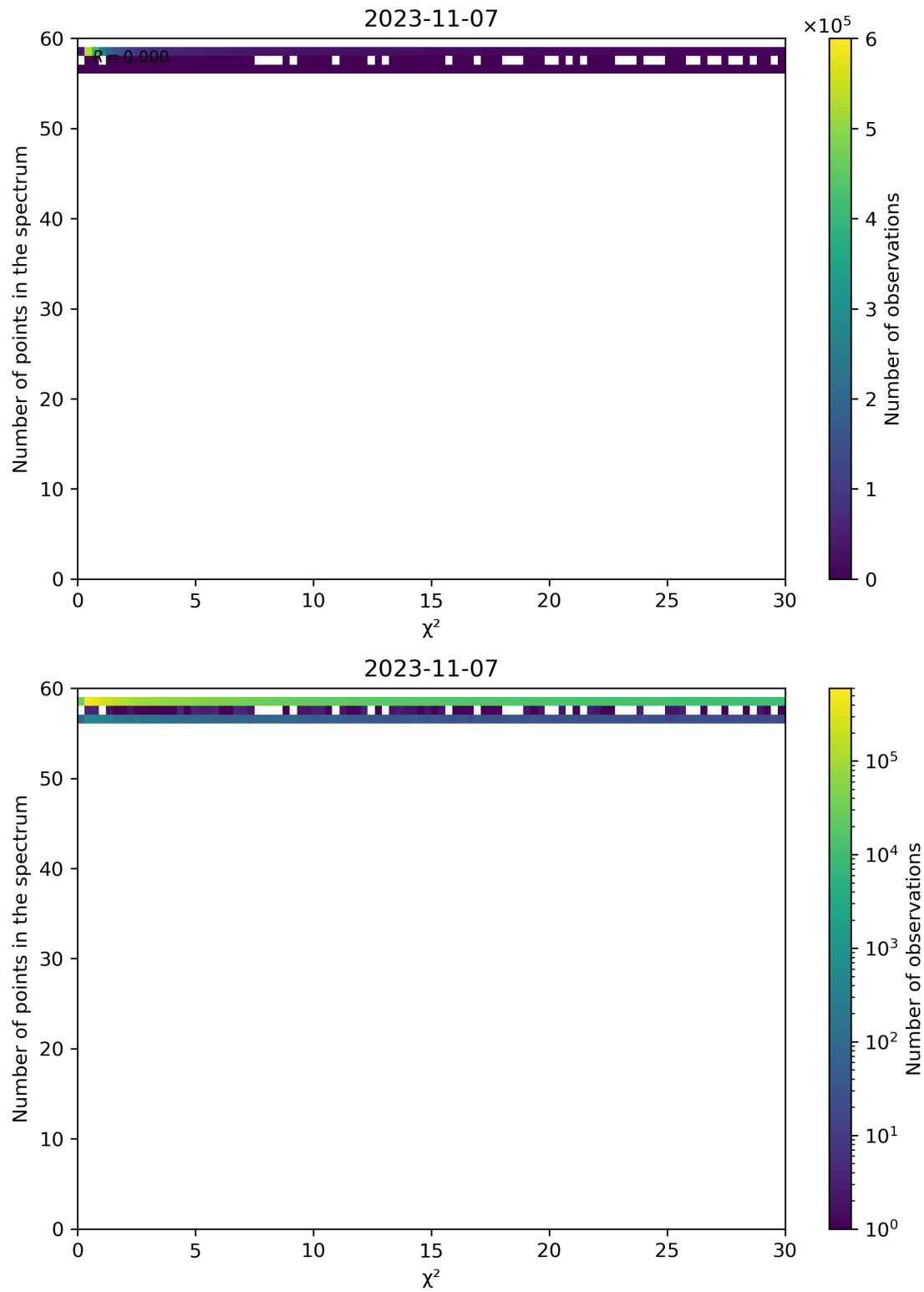
Figure 74: Scatter density plot of " \chi^2 " against "Number of points in the spectrum" for 2023-11-07 to 2023-11-08.
