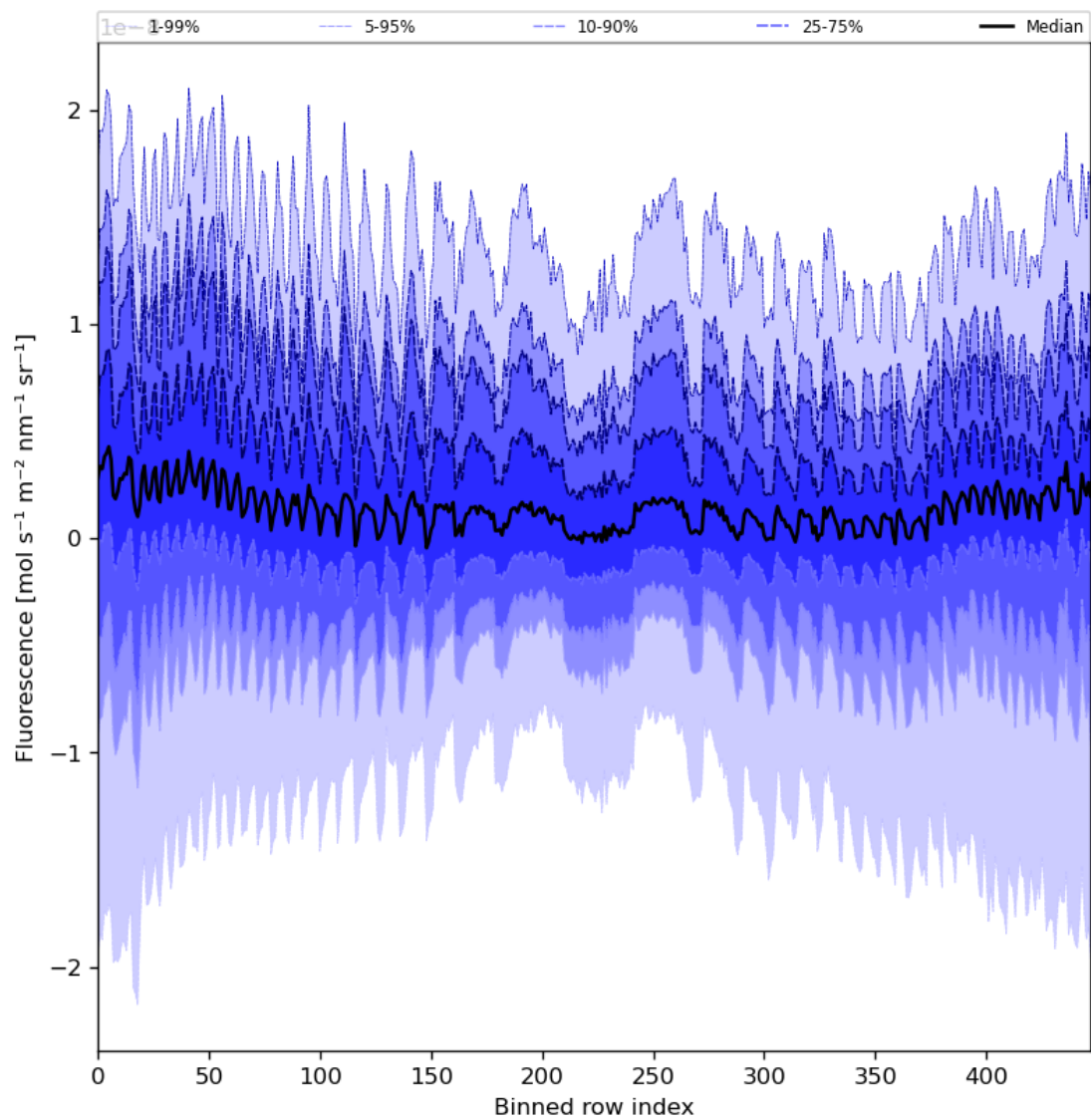
Figure 57: Along track statistics of “Fluorescence” for 2023-11-07 to 2023-11-08
