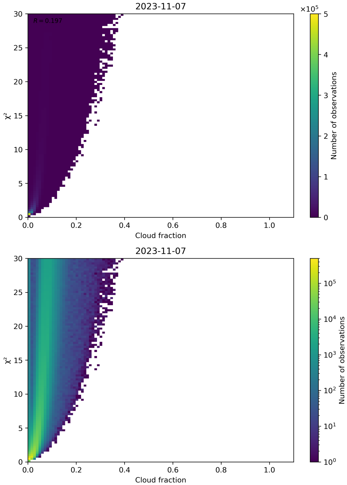
Figure 77: Scatter density plot of “Cloud fraction” against “ \chi^2 ” for 2023-11-07 to 2023-11-08.
