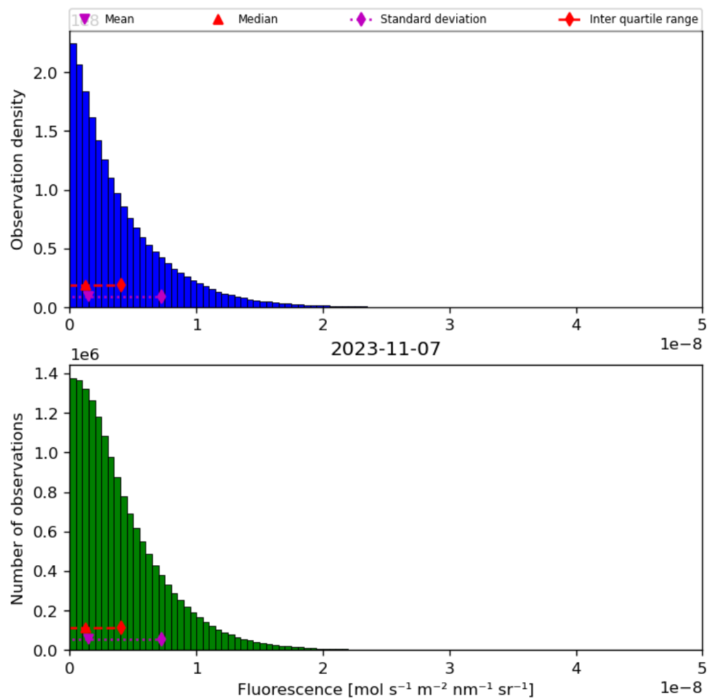
Figure 40: Histogram of “Fluorescence” for 2023-11-07 to 2023-11-08
