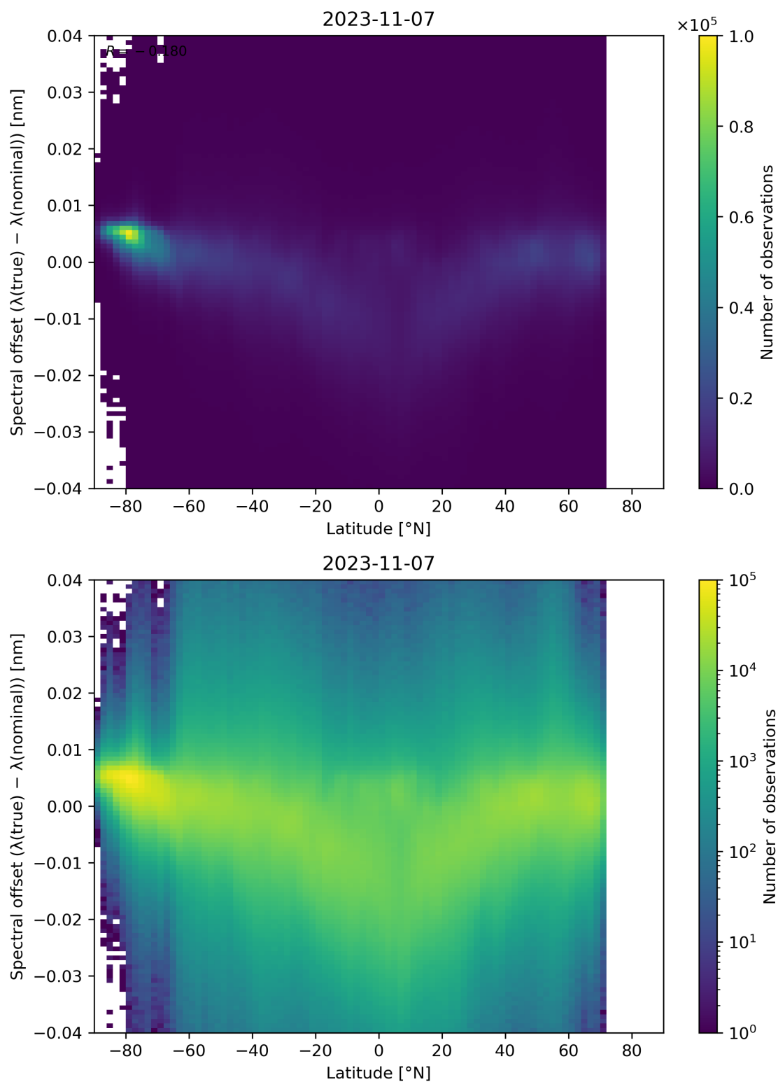
Figure 105: Scatter density plot of “Latitude” against “Spectral offset ( \lambda(\text{true}) - \lambda(\text{nominal}) )” for 2023-11-07 to 2023-11-08.
