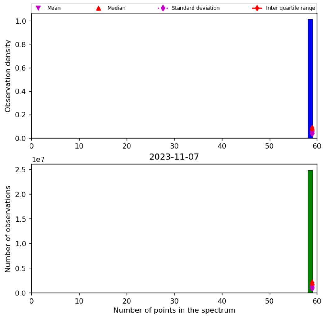
Figure 44: Histogram of “Number of points in the spectrum” for 2023-11-07 to 2023-11-08
