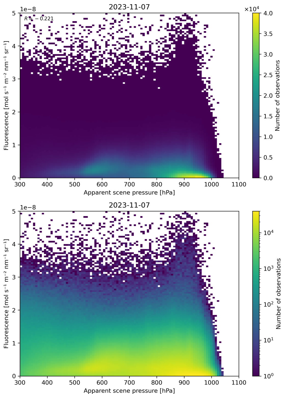
Figure 65: Scatter density plot of “Apparent scene pressure” against “Fluorescence” for 2023-11-07 to 2023-11-08.
