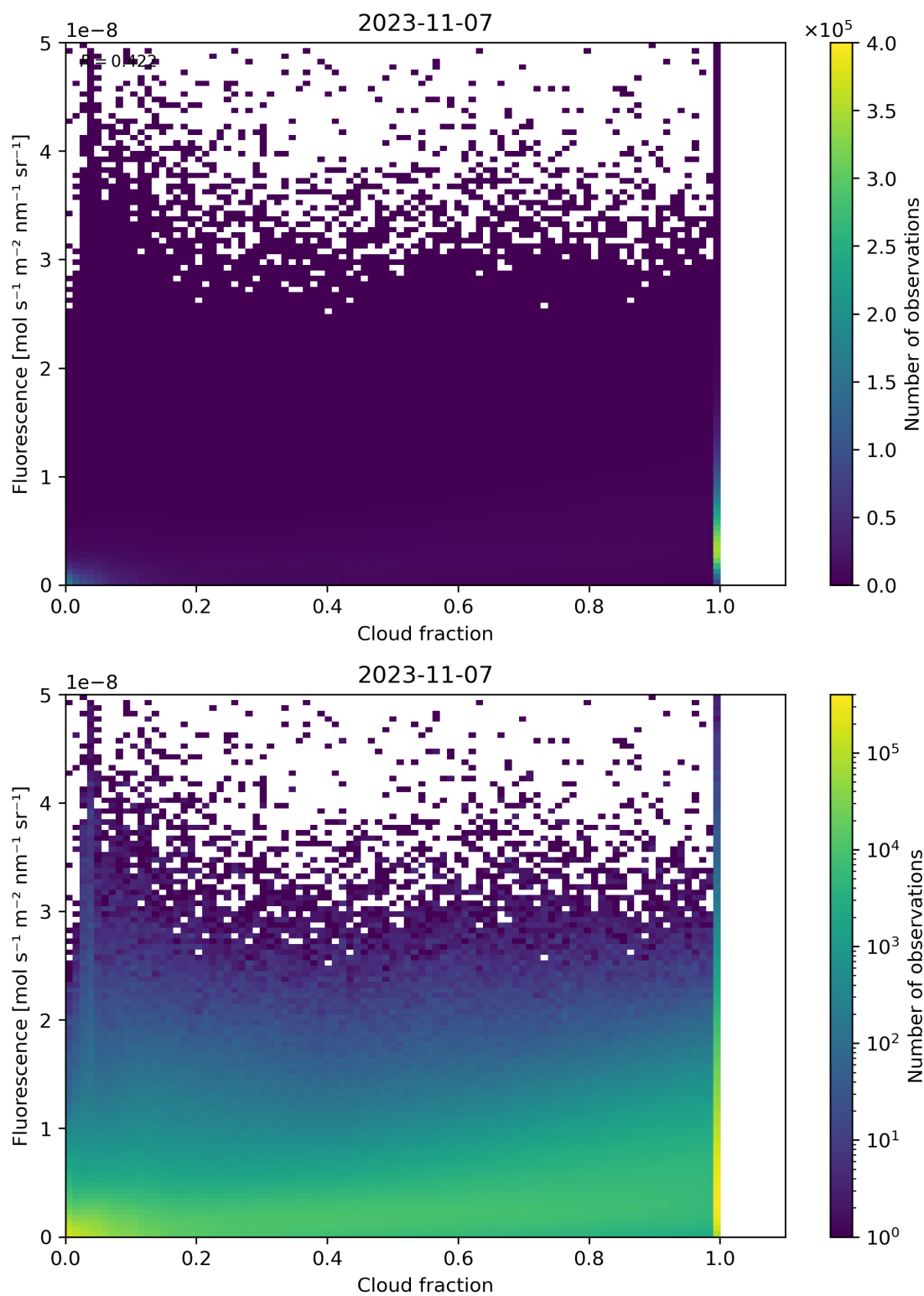
Figure 79: Scatter density plot of “Cloud fraction” against “Fluorescence” for 2023-11-07 to 2023-11-08.
