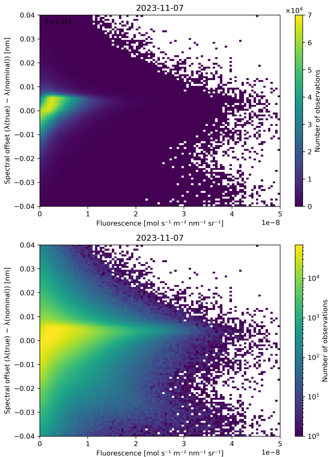
Figure 95: Scatter density plot of “Fluorescence” against “Spectral offset ( \lambda(\text{true}) - \lambda(\text{nominal}) )” for 2023-11-07 to 2023-11-08.
