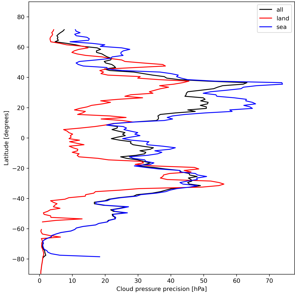
Figure 14: Zonal average of “Cloud pressure precision” for 2023-11-07 to 2023-11-08.
