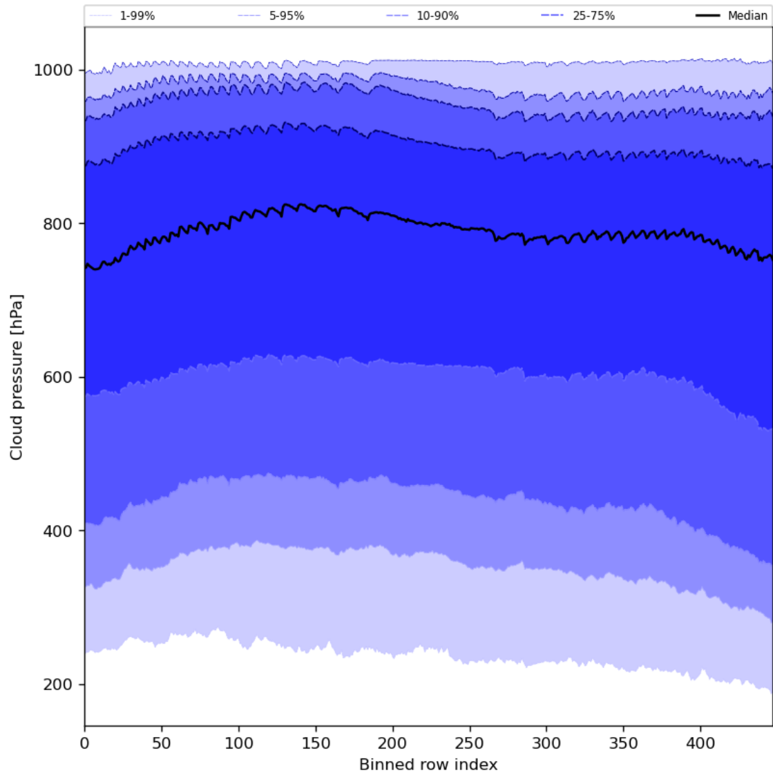
Figure 47: Along track statistics of “Cloud pressure” for 2023-11-07 to 2023-11-08
