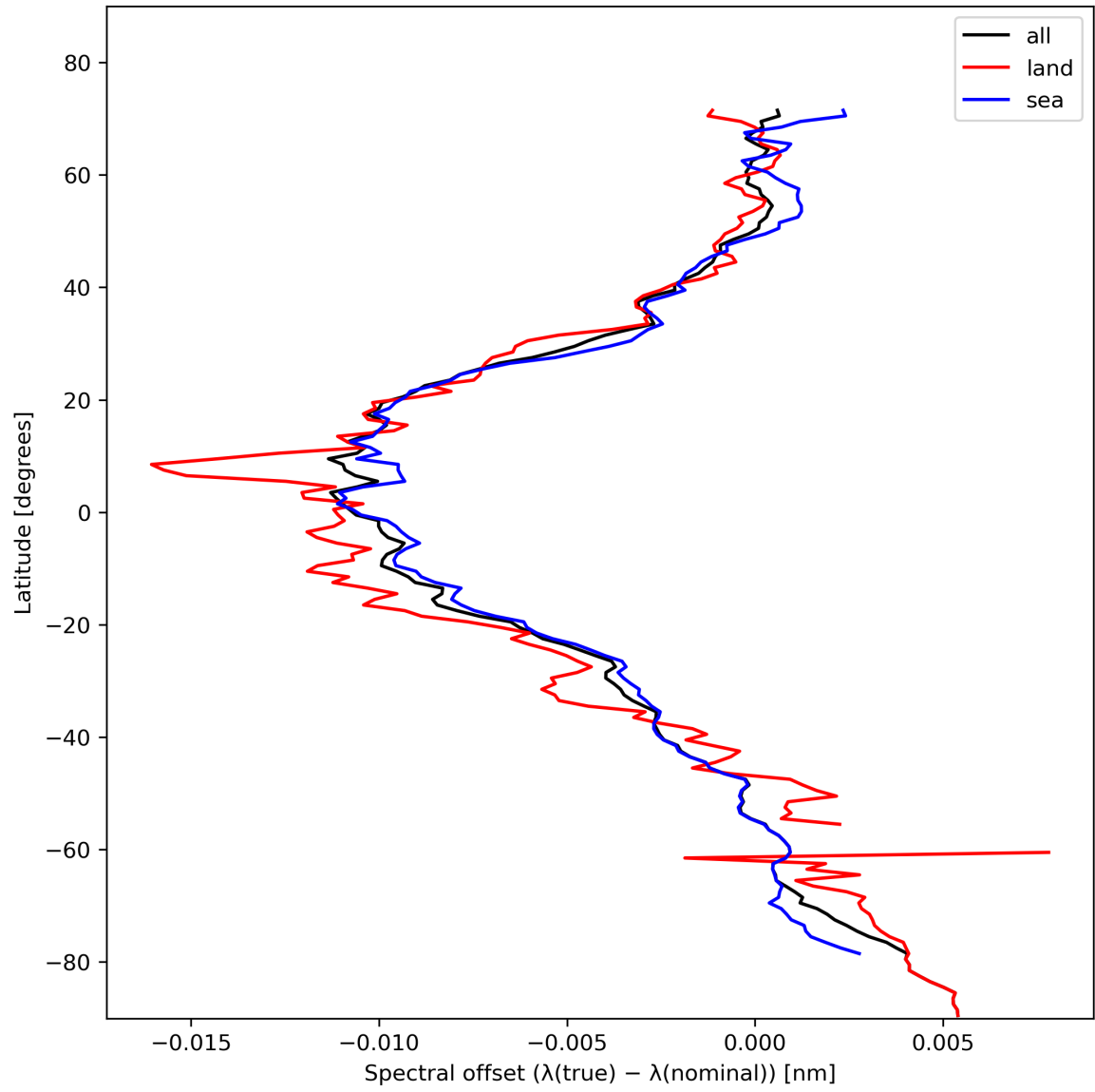
Figure 28: Zonal average of “Spectral offset ( \lambda(\text{true}) - \lambda(\text{nominal}) )” for 2023-11-07 to 2023-11-08.
