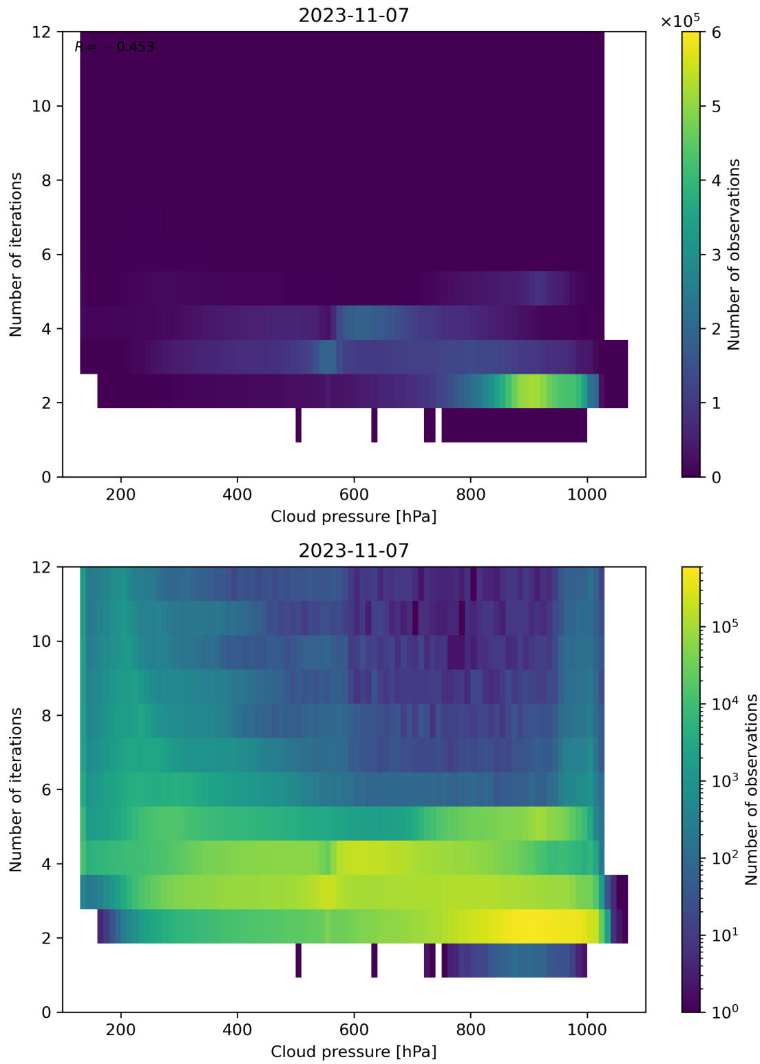
Figure 89: Scatter density plot of “Cloud pressure” against “Number of iterations” for 2023-11-07 to 2023-11-08.
