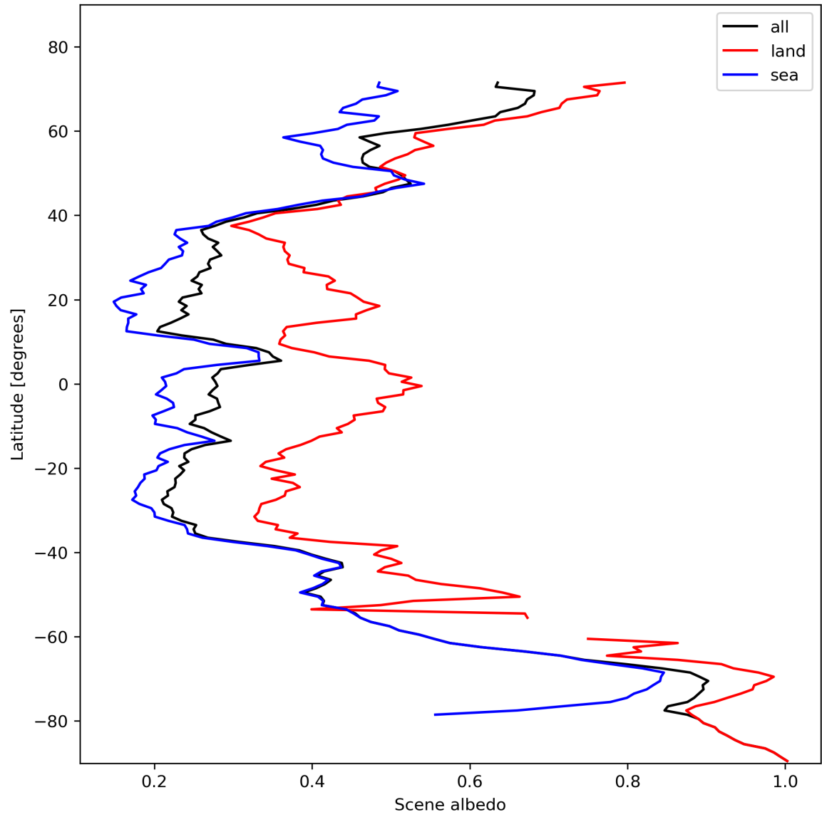
Figure 17: Zonal average of “Scene albedo” for 2023-11-07 to 2023-11-08.
