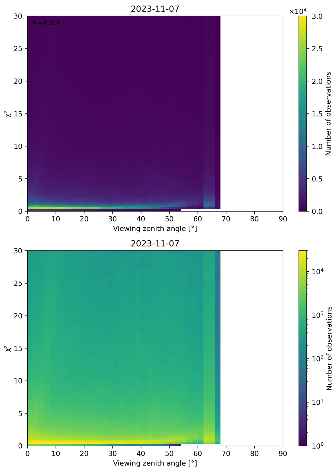
Figure 130: Scatter density plot of “Viewing zenith angle” against “ \chi^2 ” for 2023-11-07 to 2023-11-08.
