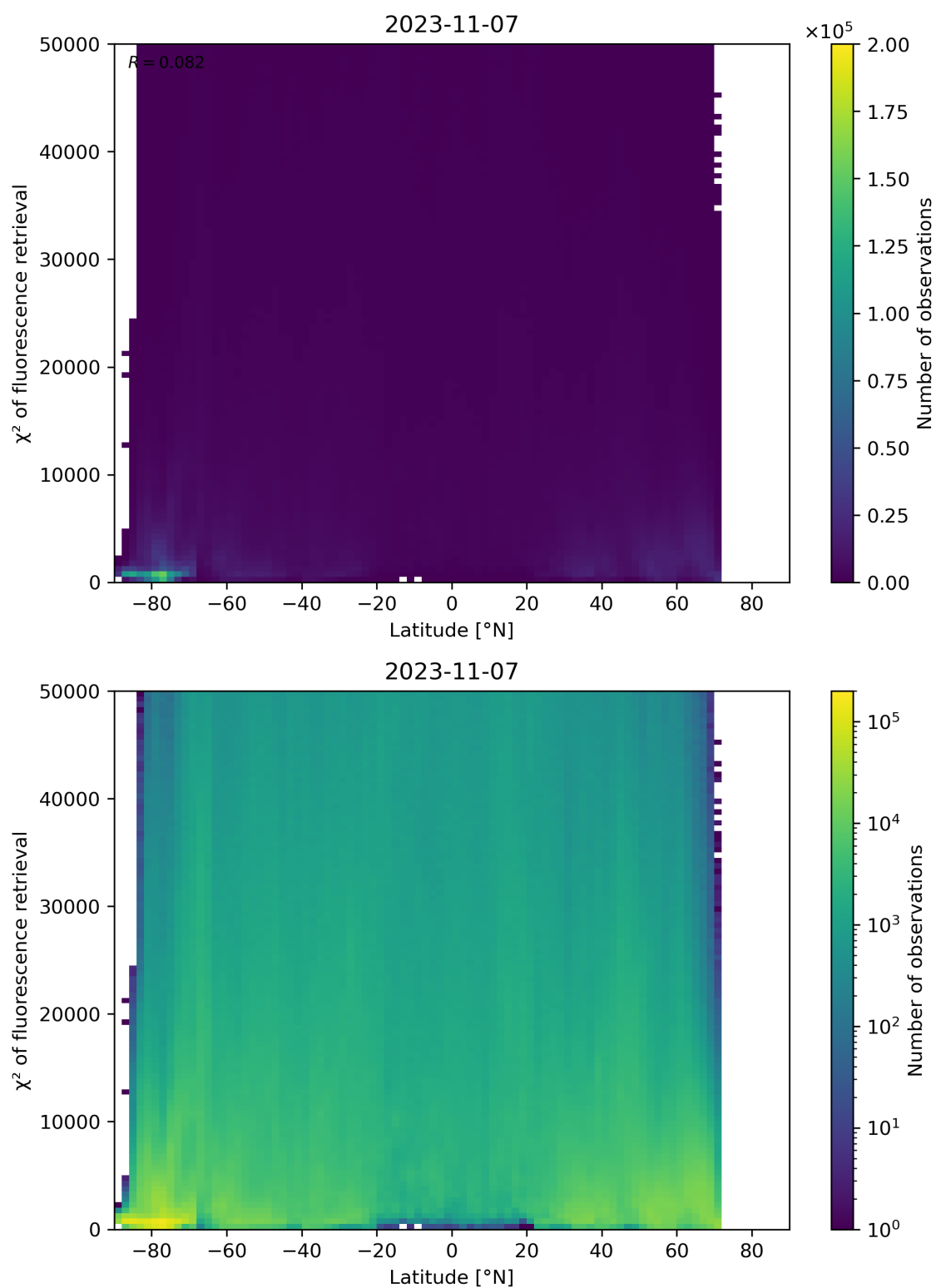
Figure 98: Scatter density plot of “Latitude” against “ \chi^2 of fluorescence retrieval” for 2023-11-07 to 2023-11-08.
