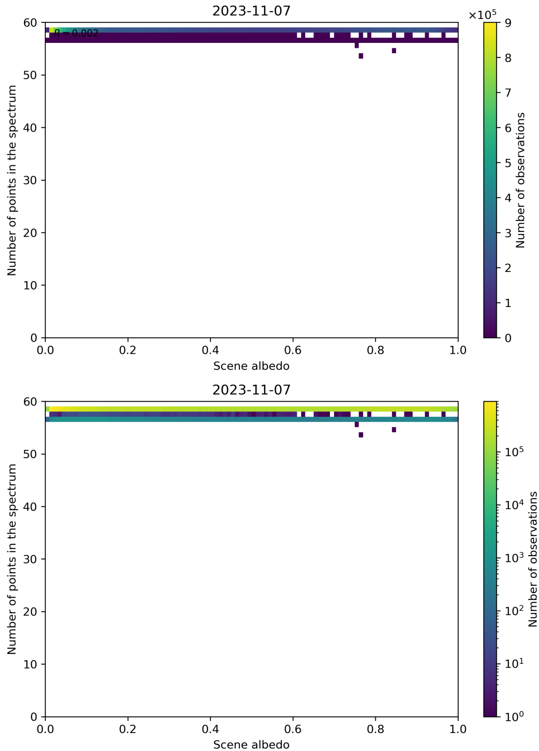
Figure 116: Scatter density plot of “Scene albedo” against “Number of points in the spectrum” for 2023-11-07 to 2023-11-08.
