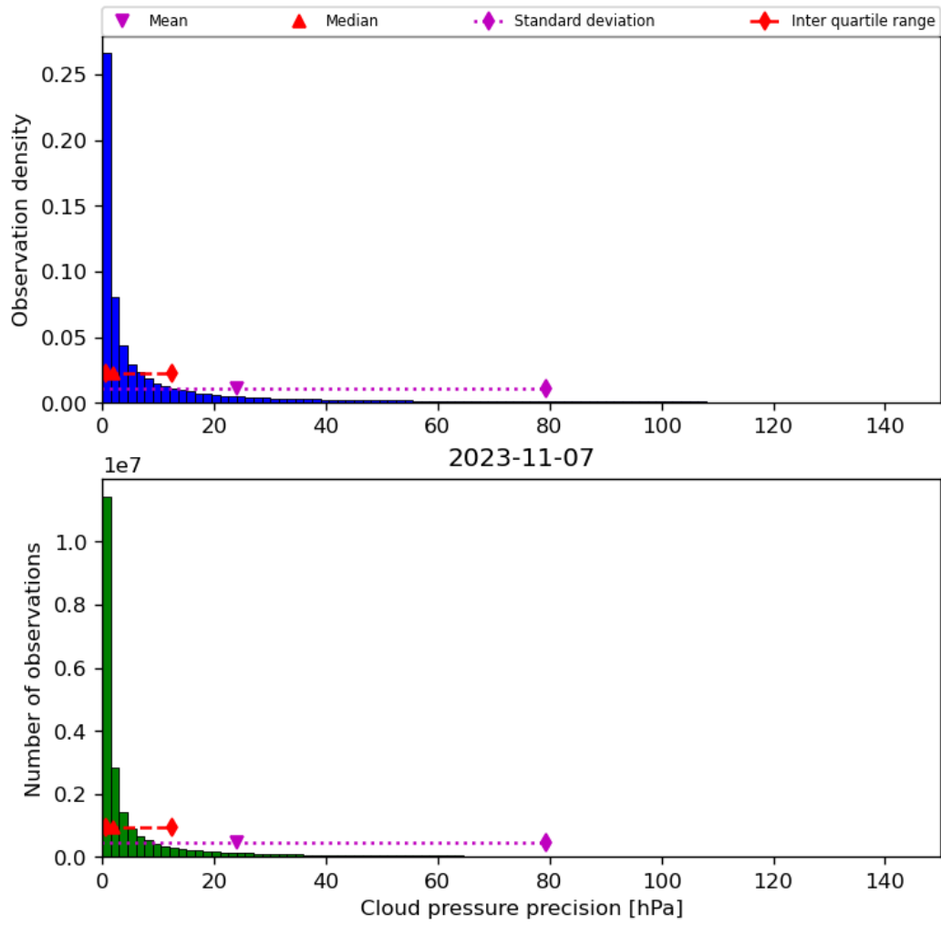
Figure 31: Histogram of “Cloud pressure precision” for 2023-11-07 to 2023-11-08
