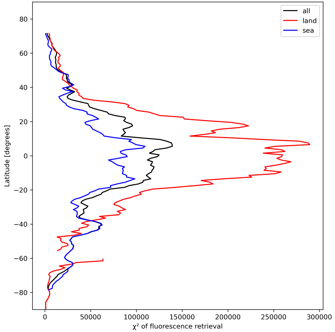
Figure 25: Zonal average of “ \chi^2 of fluorescence retrieval” for 2023-11-07 to 2023-11-08.
