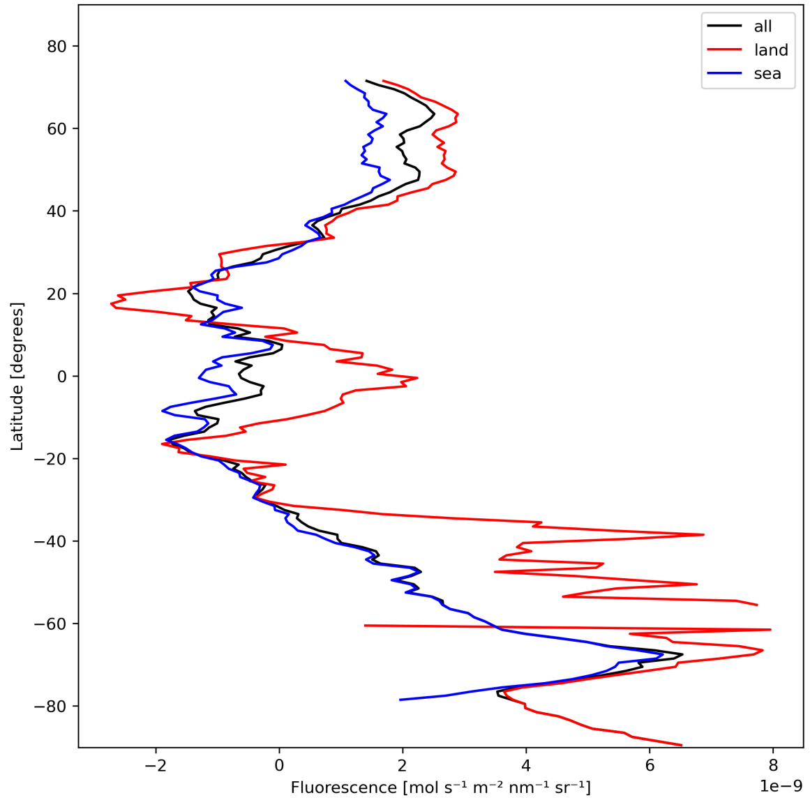
Figure 23: Zonal average of “Fluorescence” for 2023-11-07 to 2023-11-08.
