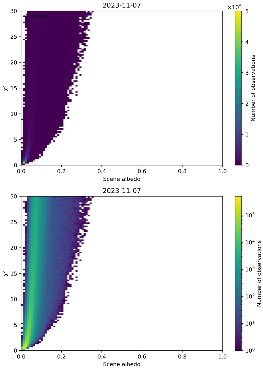
Figure 112: Scatter density plot of “Scene albedo” against “ \chi^2 ” for 2023-11-07 to 2023-11-08.
