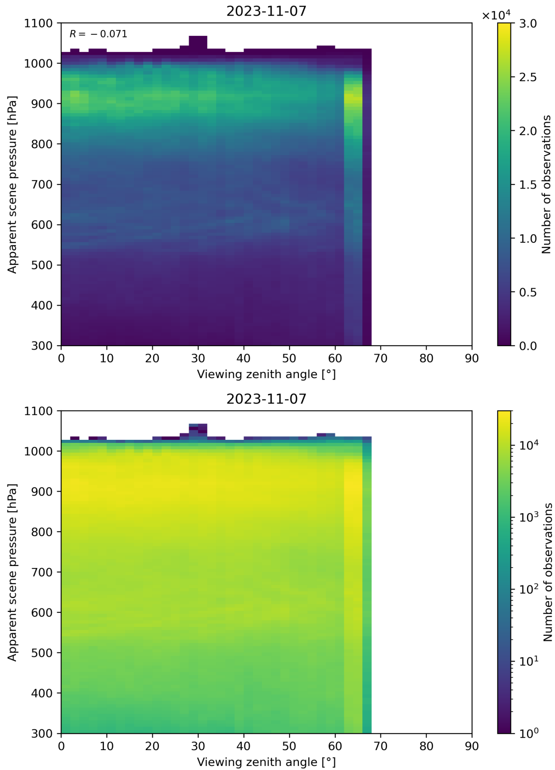
Figure 129: Scatter density plot of “Viewing zenith angle” against “Apparent scene pressure” for 2023-11-07 to 2023-11-08.
