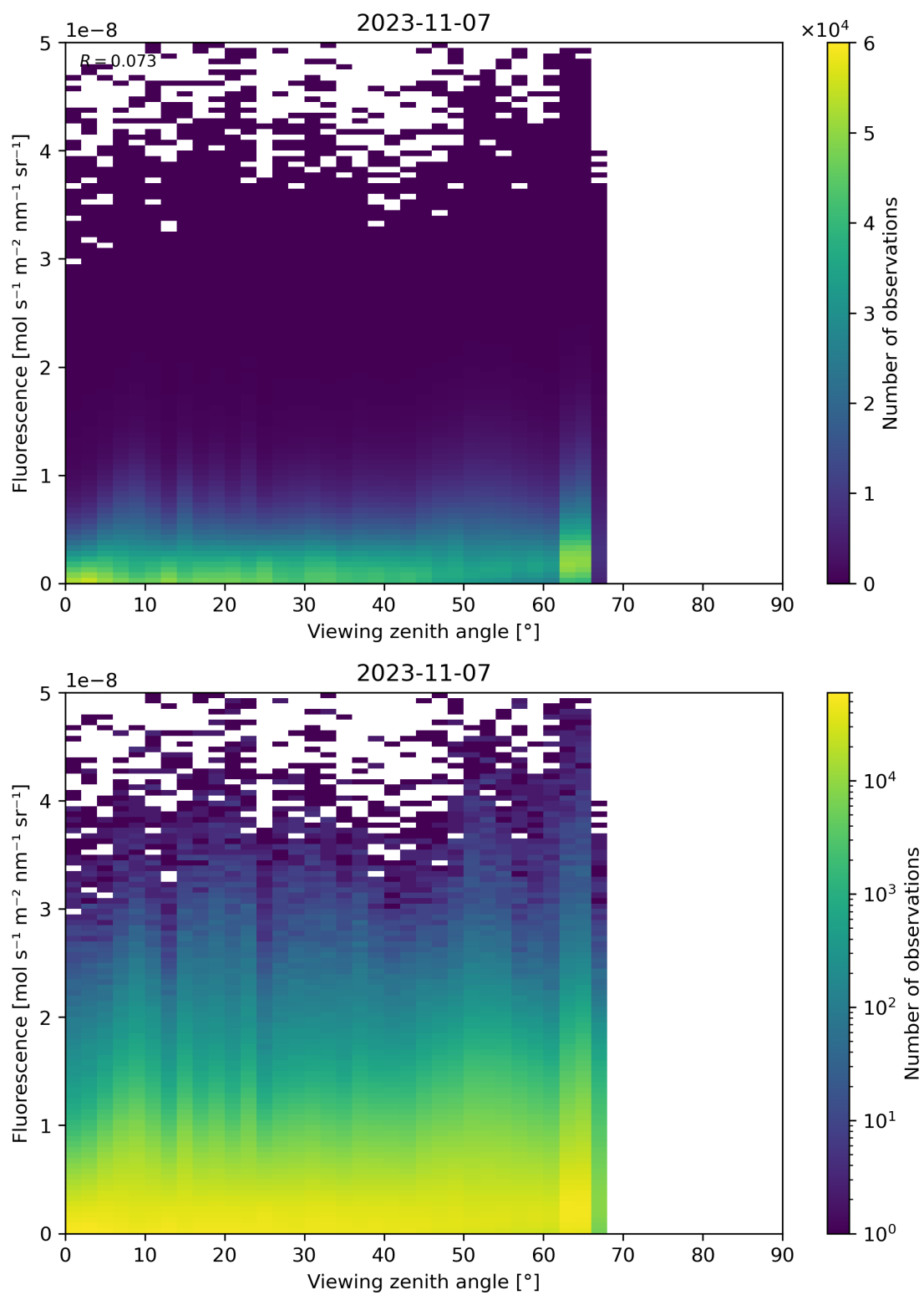
Figure 134: Scatter density plot of “Viewing zenith angle” against “Fluorescence” for 2023-11-07 to 2023-11-08.
