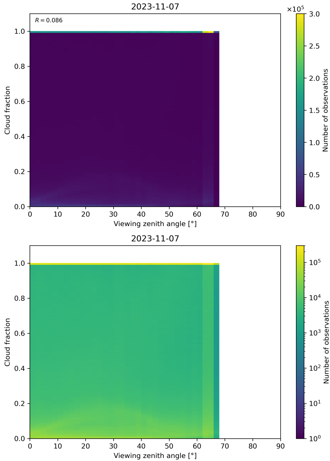
Figure 132: Scatter density plot of “Viewing zenith angle” against “Cloud fraction” for 2023-11-07 to 2023-11-08.
