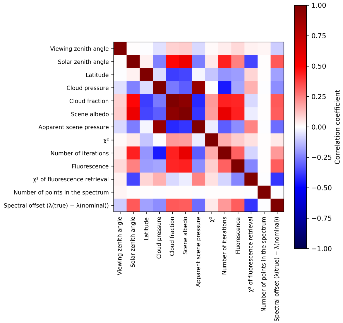
Figure 2: Map of correlation matrix for 2023-11-07 to 2023-11-08.
