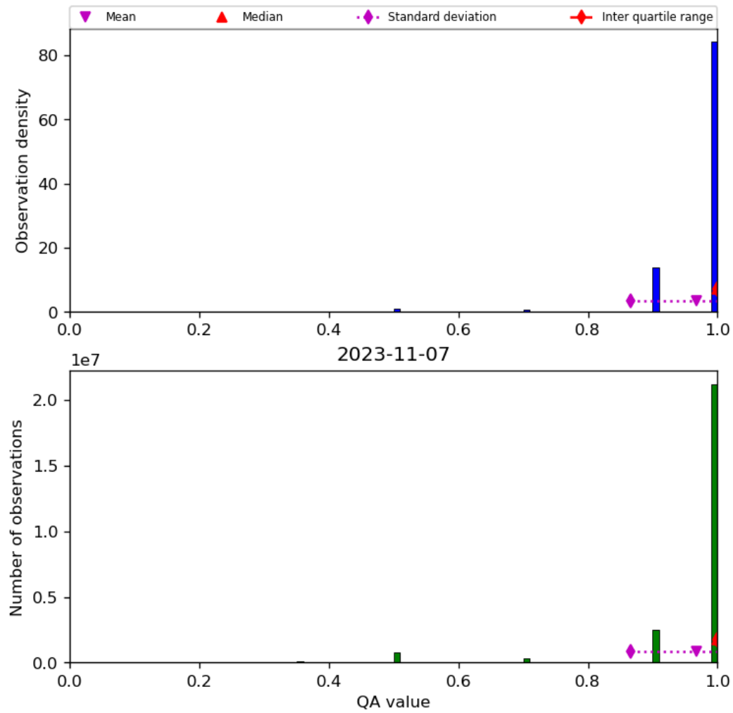
Figure 29: Histogram of “QA value” for 2023-11-07 to 2023-11-08
