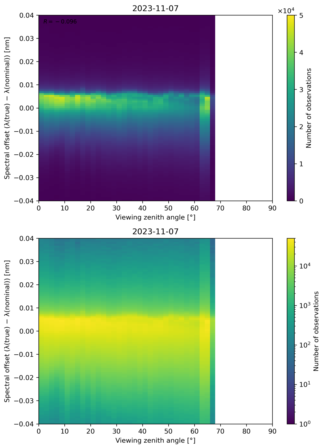
Figure 140: Scatter density plot of “Viewing zenith angle” against “Spectral offset ( \lambda(\text{true}) - \lambda(\text{nominal}) )” for 2023-11-07 to 2023-11-08.
