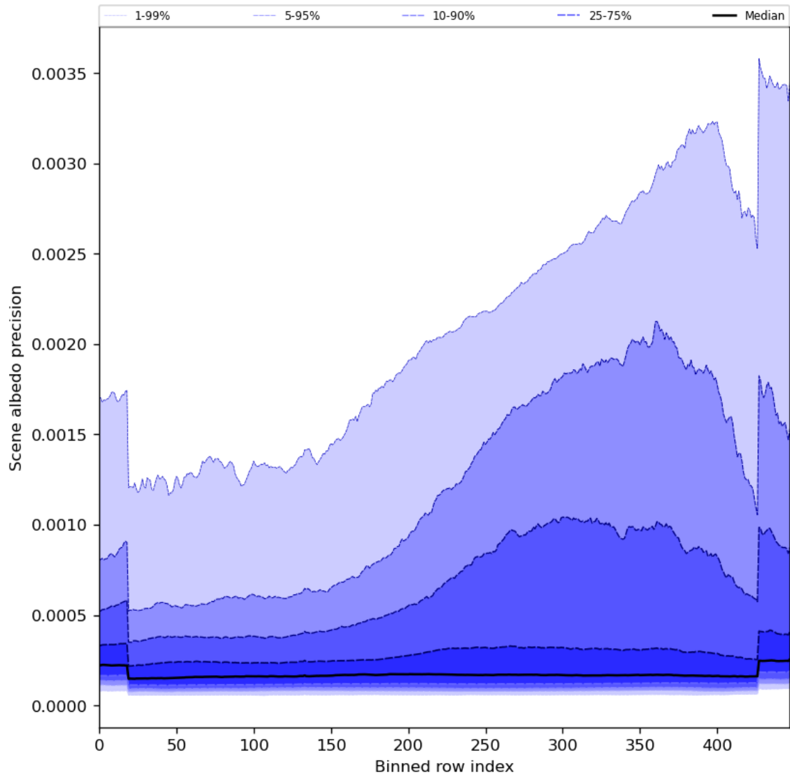
Figure 52: Along track statistics of “Scene albedo precision” for 2023-11-07 to 2023-11-08
