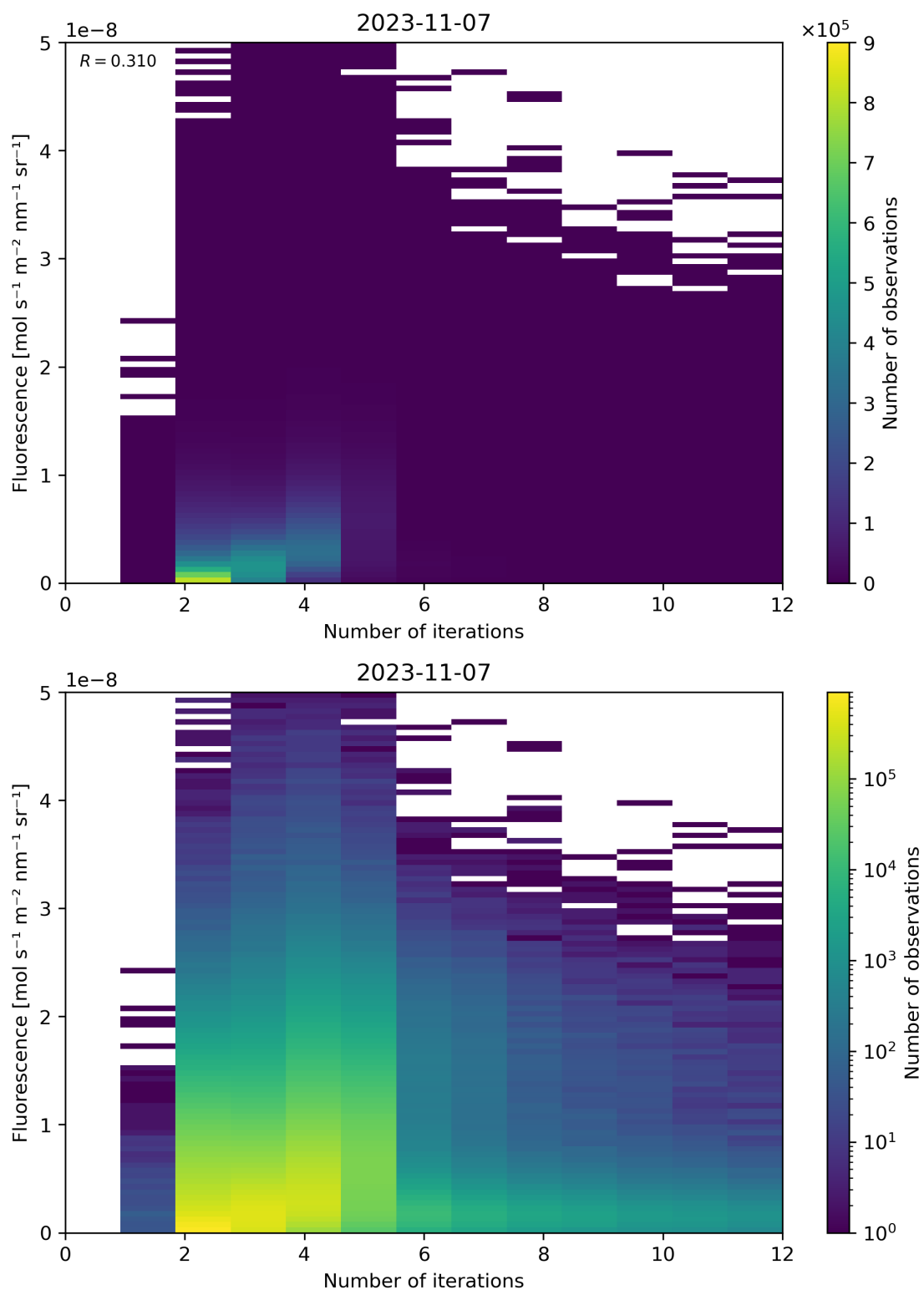
Figure 107: Scatter density plot of “Number of iterations” against “Fluorescence” for 2023-11-07 to 2023-11-08.
