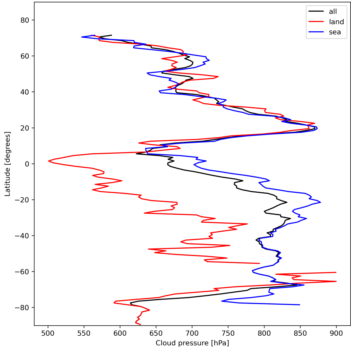
Figure 13: Zonal average of “Cloud pressure” for 2023-11-07 to 2023-11-08.
