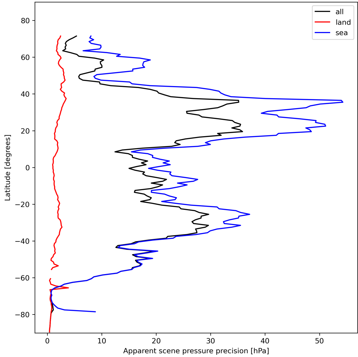
Figure 20: Zonal average of “Apparent scene pressure precision” for 2023-11-07 to 2023-11-08.
