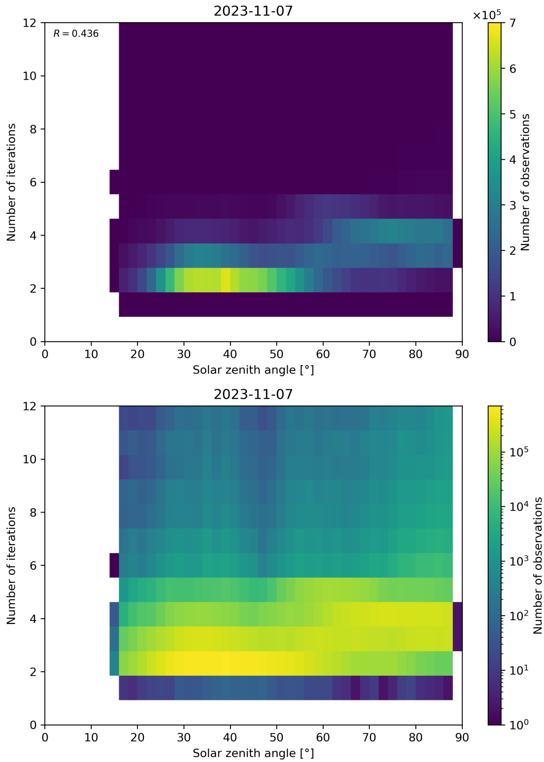
Figure 125: Scatter density plot of “Solar zenith angle” against “Number of iterations” for 2023-11-07 to 2023-11-08.
