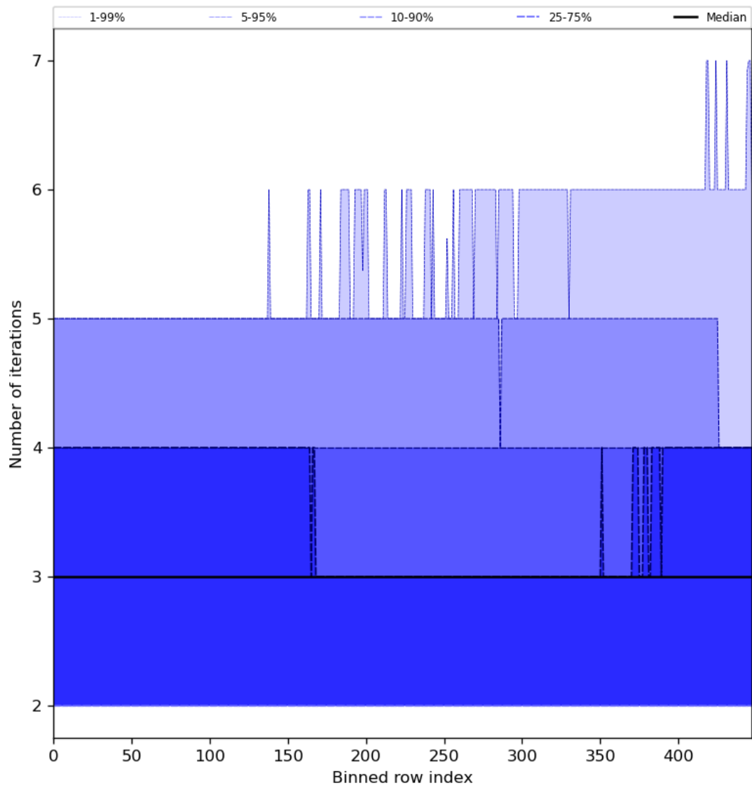
Figure 56: Along track statistics of “Number of iterations” for 2023-11-07 to 2023-11-08
