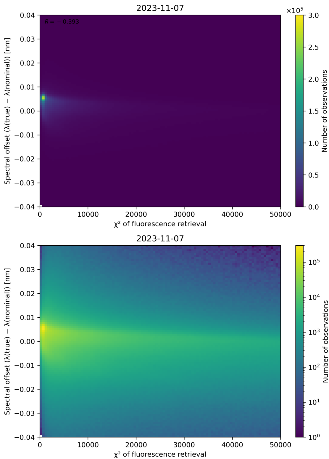
Figure 72: Scatter density plot of " \chi^2 of fluorescence retrieval" against "Spectral offset ( \lambda(\text{true}) - \lambda(\text{nominal}) )" for 2023-11-07 to 2023-11-08.
