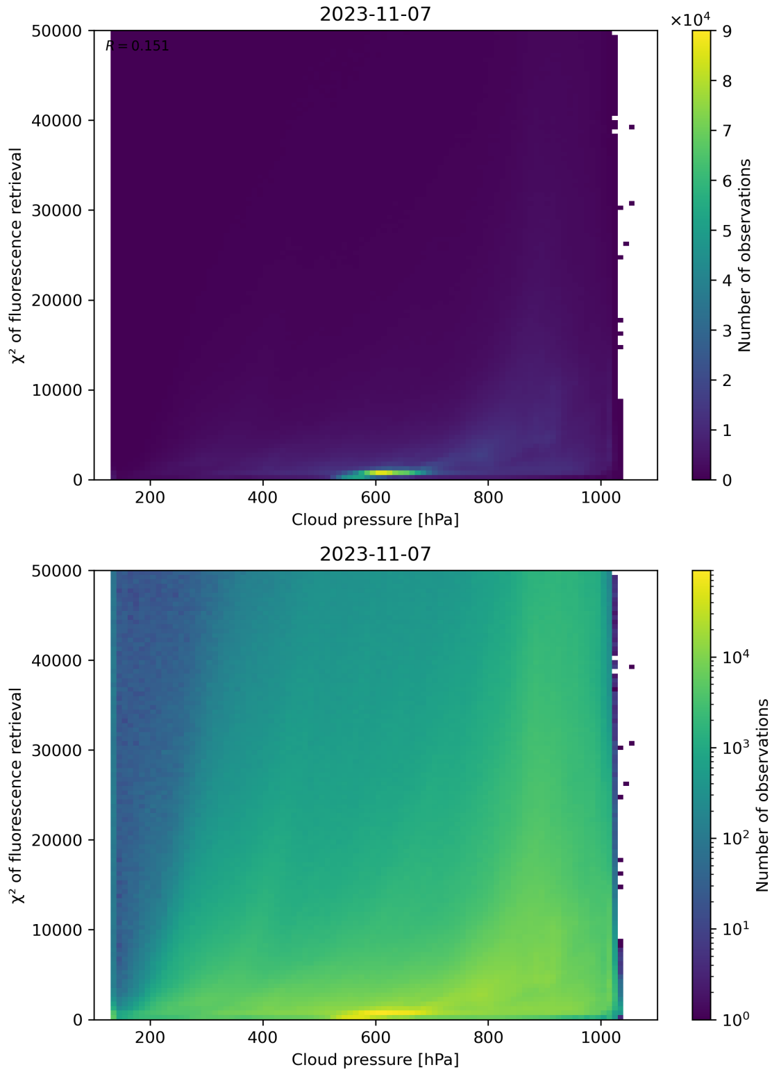
Figure 86: Scatter density plot of “Cloud pressure” against “ \chi^2 of fluorescence retrieval” for 2023-11-07 to 2023-11-08.
