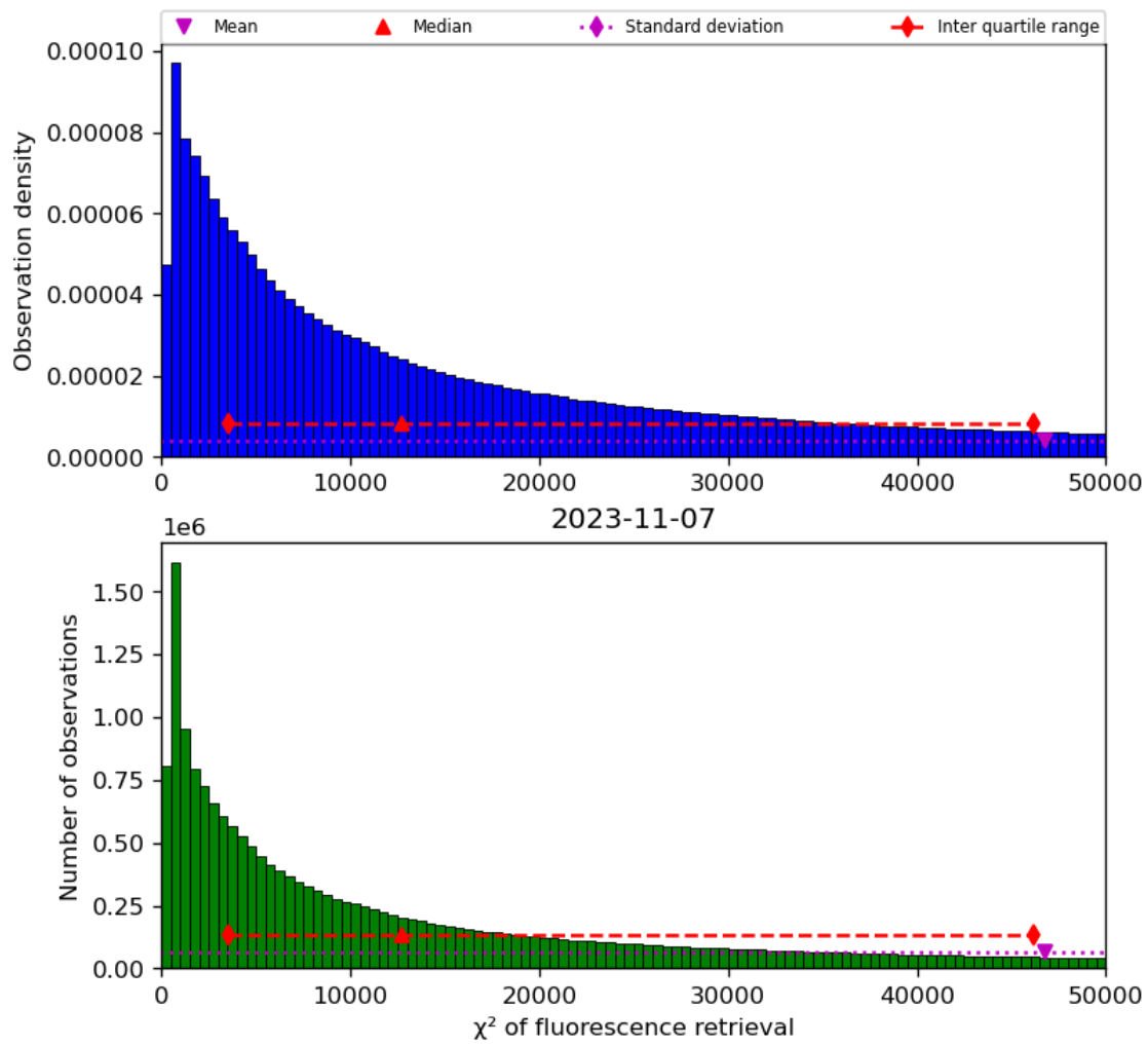
Figure 42: Histogram of “ \chi^2 of fluorescence retrieval” for 2023-11-07 to 2023-11-08
