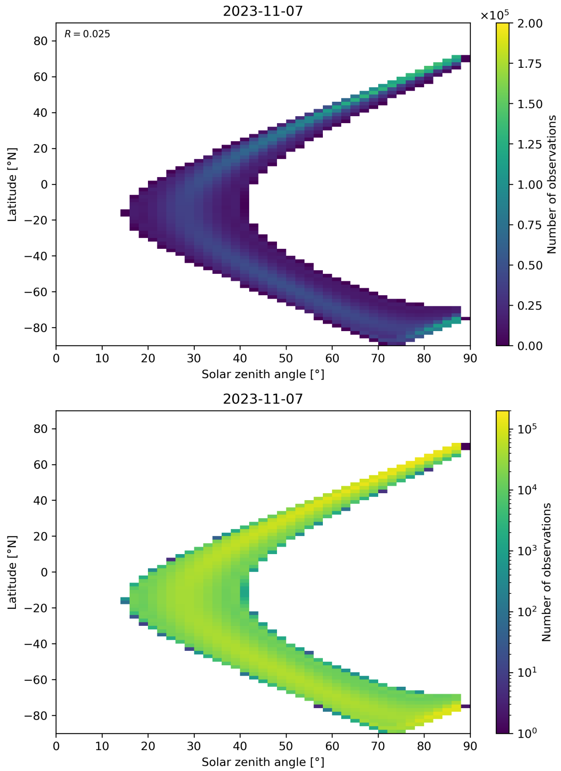
Figure 124: Scatter density plot of “Solar zenith angle” against “Latitude” for 2023-11-07 to 2023-11-08.
