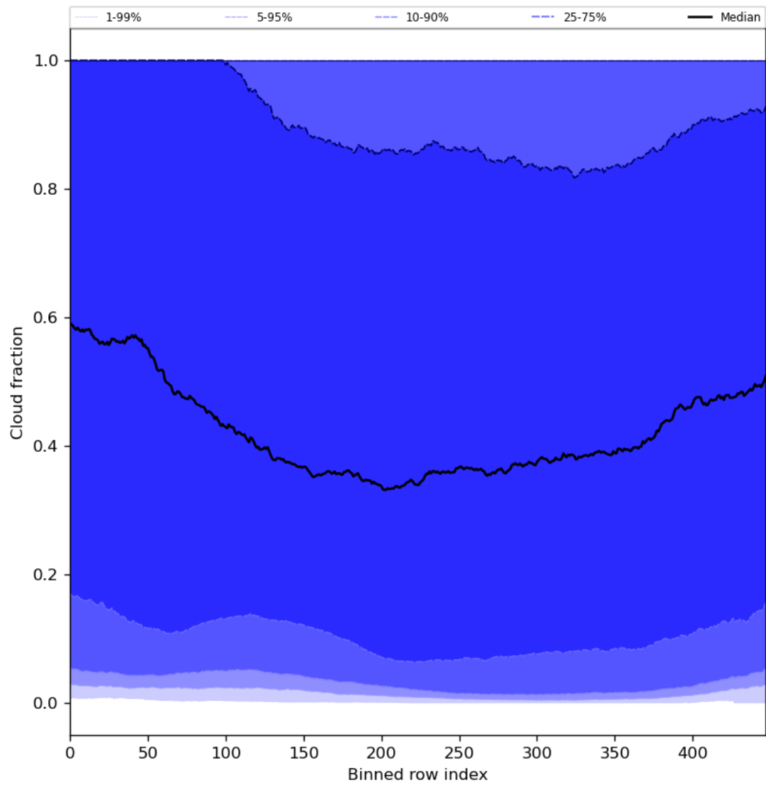
Figure 49: Along track statistics of “Cloud fraction” for 2023-11-07 to 2023-11-08
