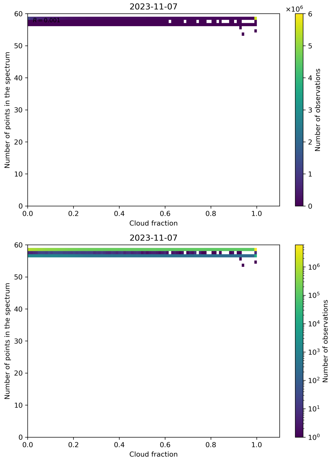
Figure 81: Scatter density plot of “Cloud fraction” against “Number of points in the spectrum” for 2023-11-07 to 2023-11-08.
