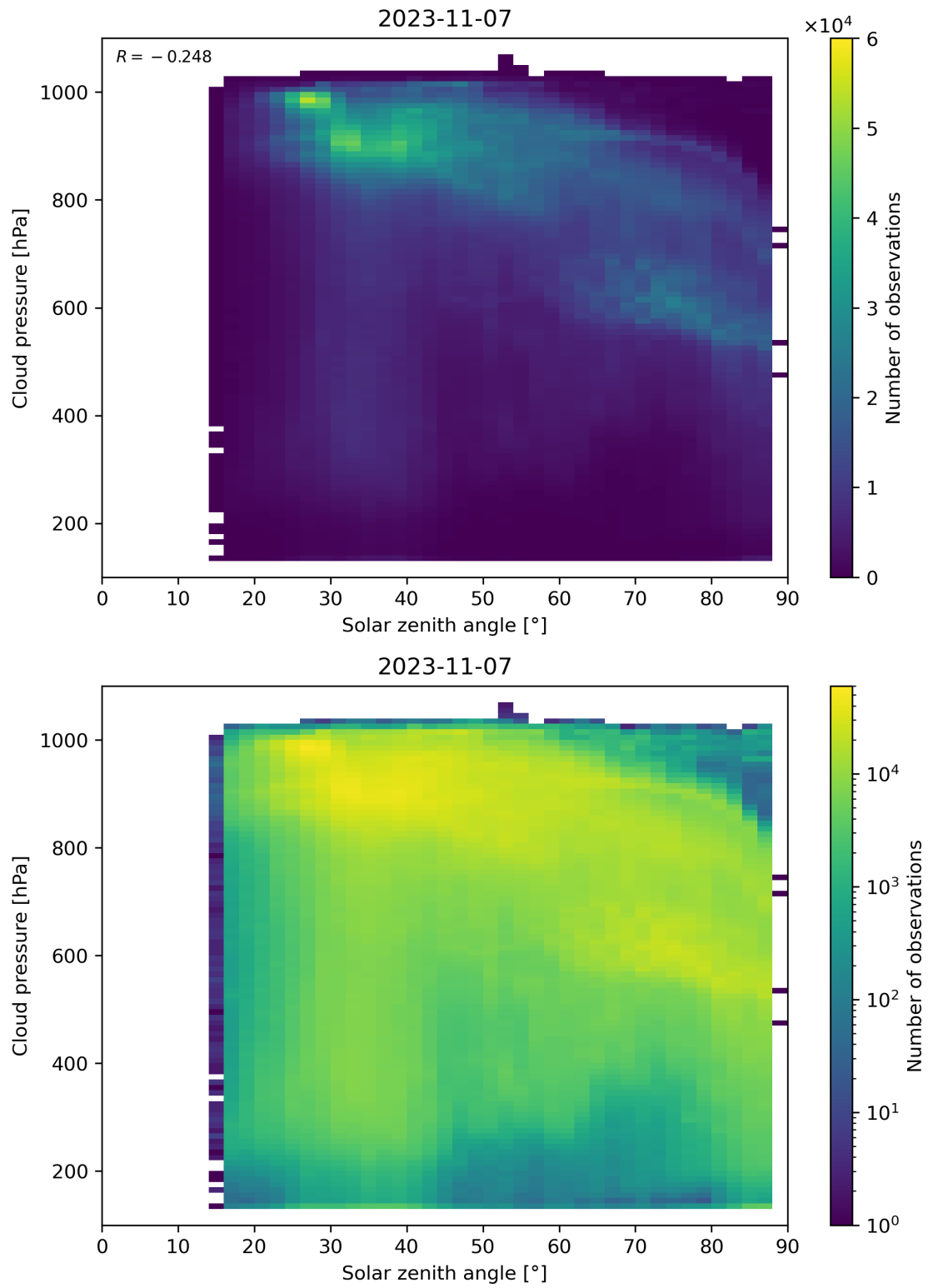
Figure 122: Scatter density plot of “Solar zenith angle” against “Cloud pressure” for 2023-11-07 to 2023-11-08.
