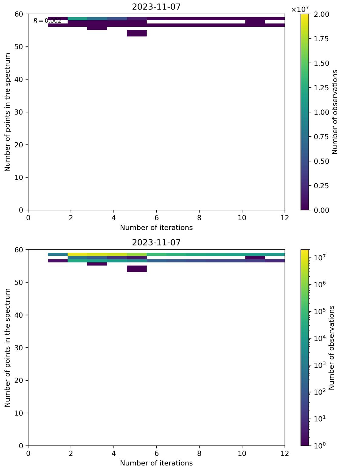
Figure 108: Scatter density plot of “Number of iterations” against “Number of points in the spectrum” for 2023-11-07 to 2023-11-08.
