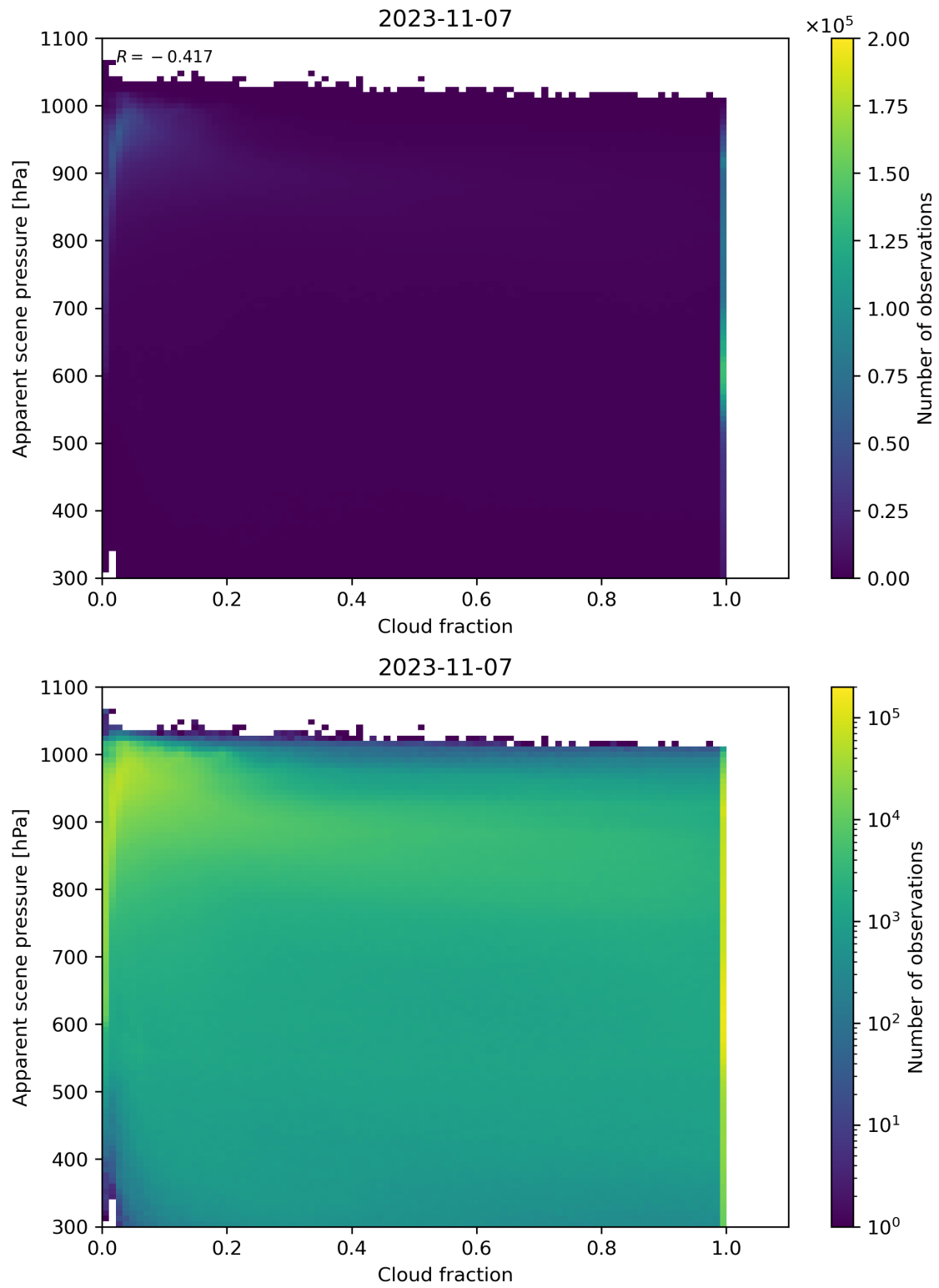
Figure 76: Scatter density plot of “Cloud fraction” against “Apparent scene pressure” for 2023-11-07 to 2023-11-08.
