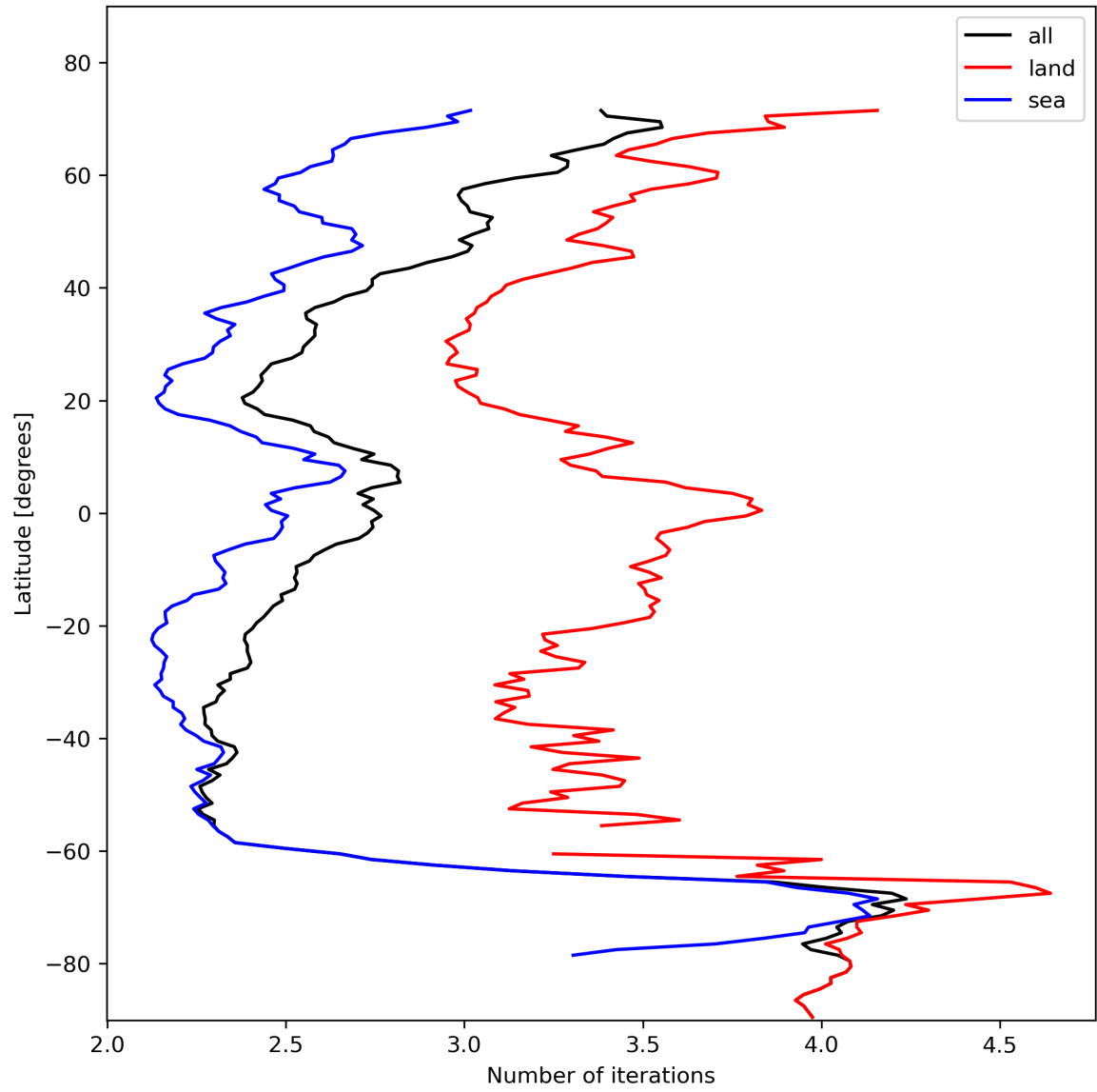
Figure 22: Zonal average of “Number of iterations” for 2023-11-07 to 2023-11-08.
