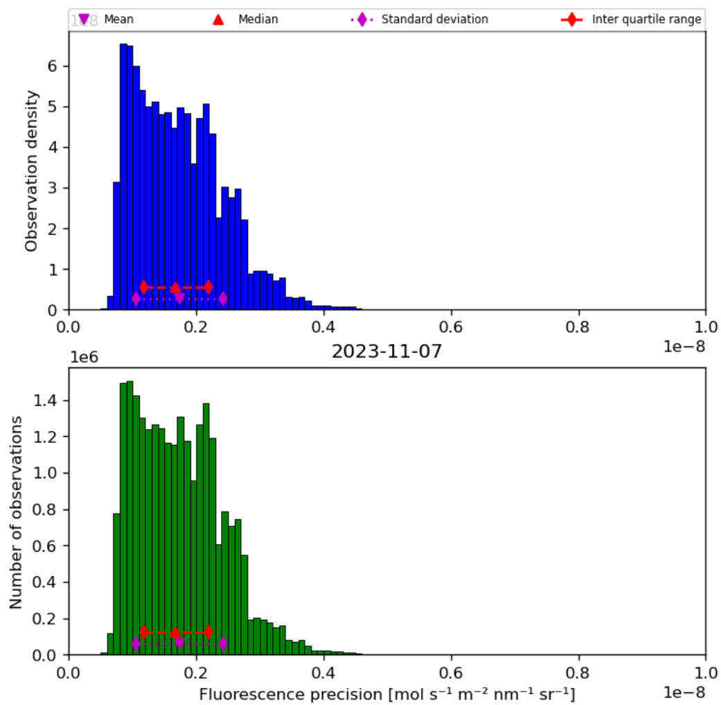
Figure 41: Histogram of “Fluorescence precision” for 2023-11-07 to 2023-11-08
