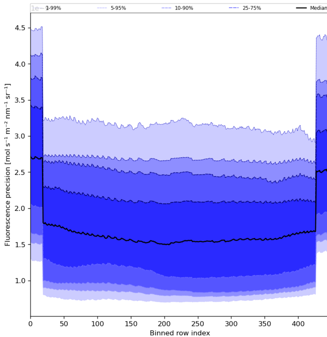
Figure 58: Along track statistics of “Fluorescence precision” for 2023-11-07 to 2023-11-08
