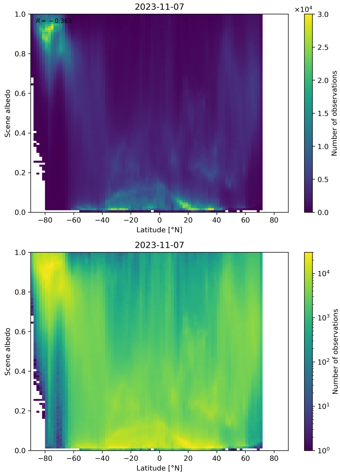
Figure 104: Scatter density plot of “Latitude” against “Scene albedo” for 2023-11-07 to 2023-11-08.
