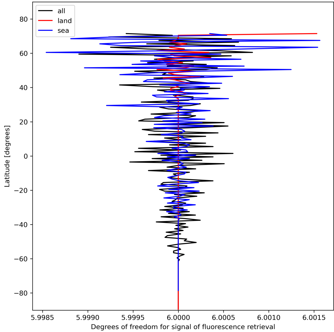
Figure 26: Zonal average of “Degrees of freedom for signal of fluorescence retrieval” for 2023-11-07 to 2023-11-08.
