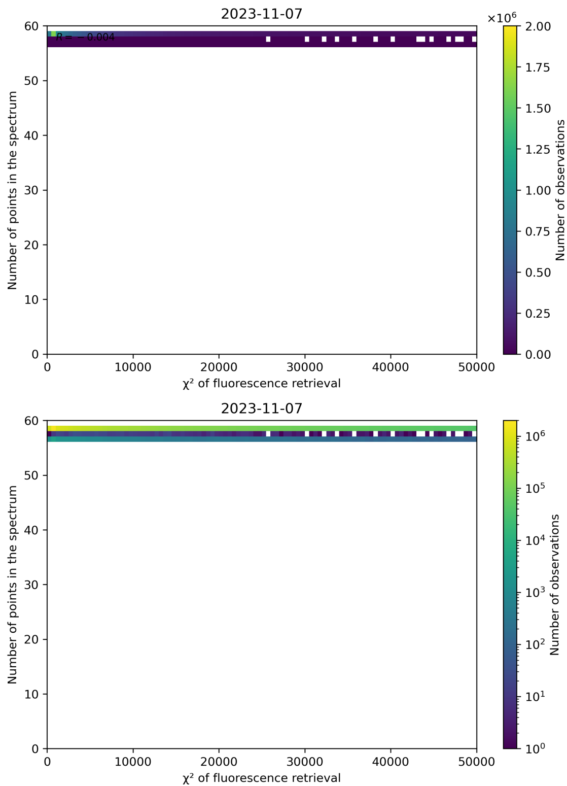
Figure 71: Scatter density plot of " \chi^2 of fluorescence retrieval" against "Number of points in the spectrum" for 2023-11-07 to 2023-11-08.
