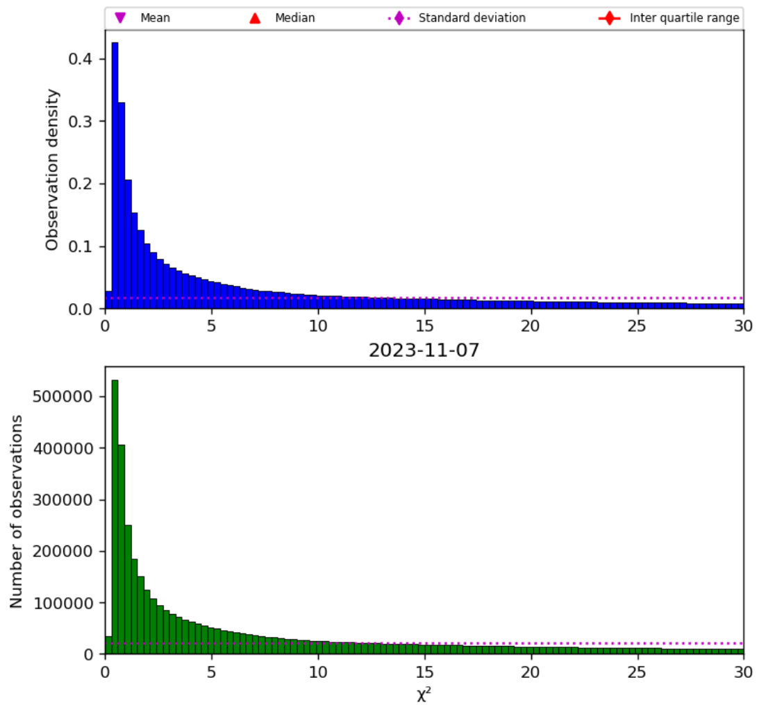
Figure 38: Histogram of " \chi^2 " for 2023-11-07 to 2023-11-08
