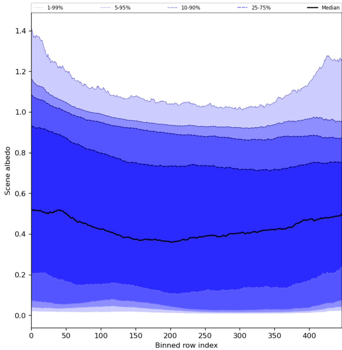
Figure 51: Along track statistics of “Scene albedo” for 2023-11-07 to 2023-11-08
