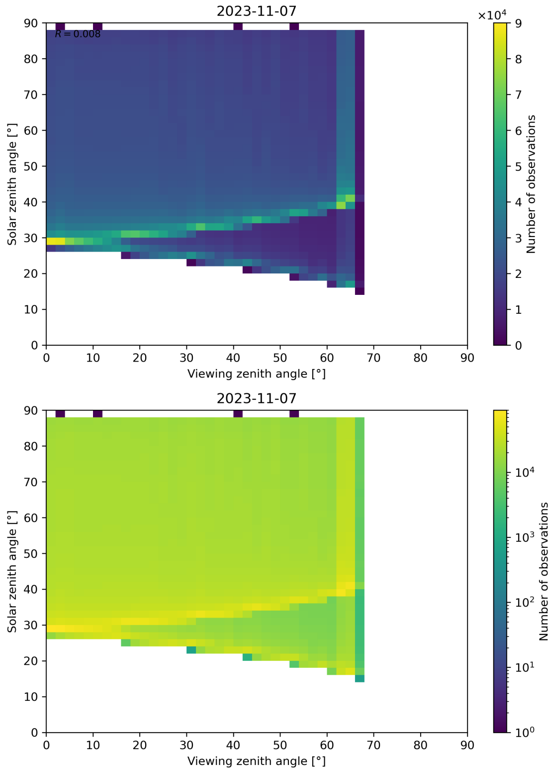
Figure 139: Scatter density plot of “Viewing zenith angle” against “Solar zenith angle” for 2023-11-07 to 2023-11-08.
