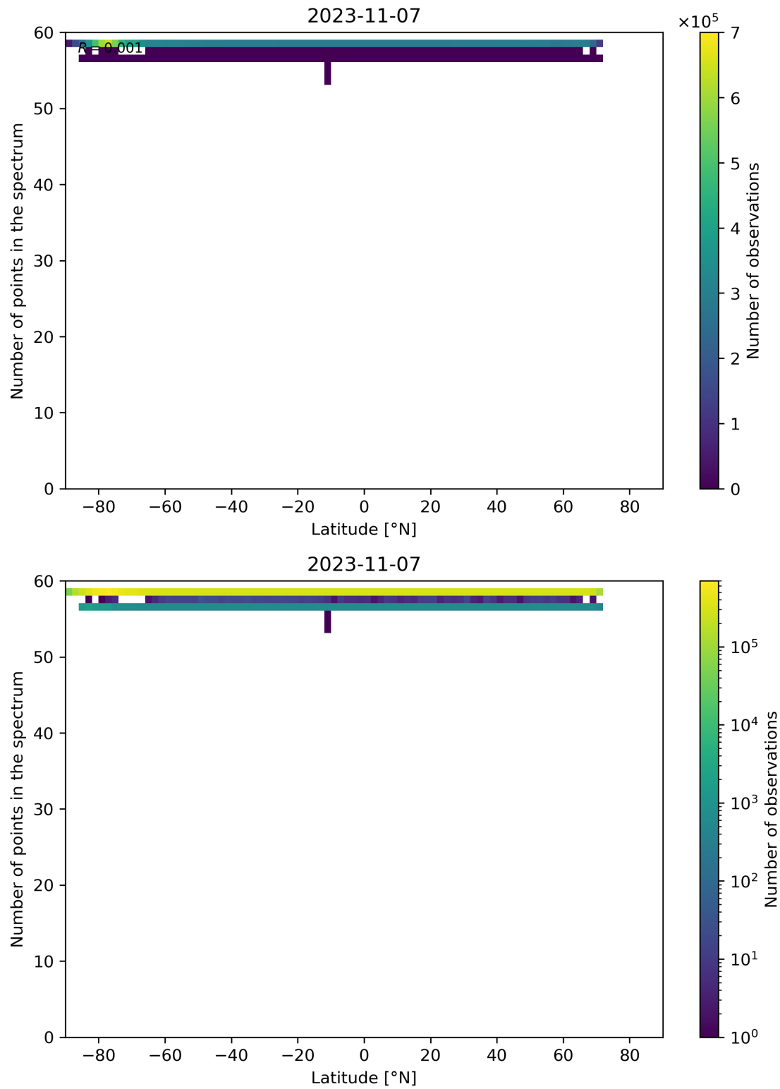
Figure 103: Scatter density plot of “Latitude” against “Number of points in the spectrum” for 2023-11-07 to 2023-11-08.
