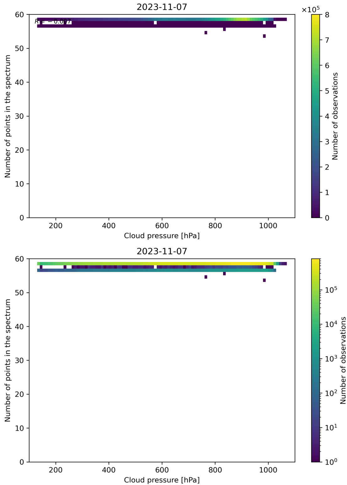
Figure 90: Scatter density plot of “Cloud pressure” against “Number of points in the spectrum” for 2023-11-07 to 2023-11-08.
