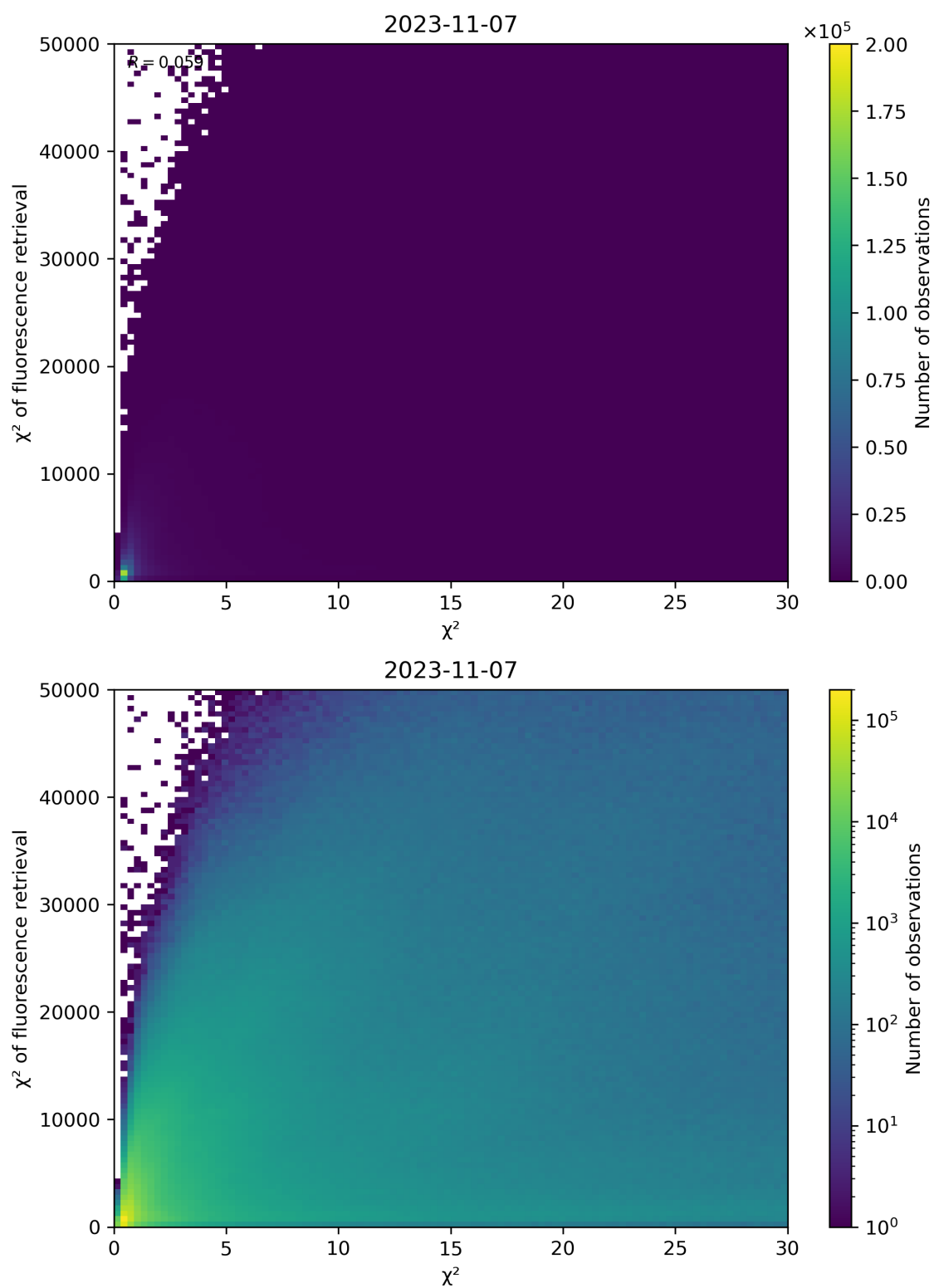
Figure 69: Scatter density plot of “ \chi^2 ” against “ \chi^2 of fluorescence retrieval” for 2023-11-07 to 2023-11-08.
