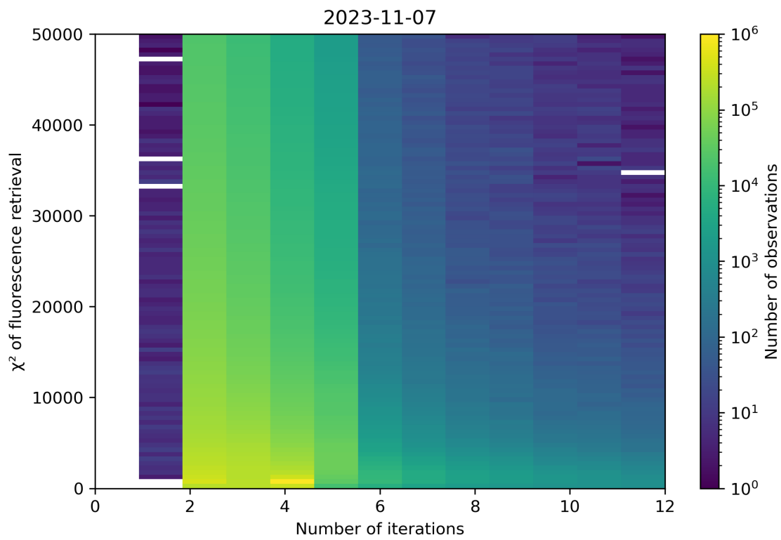
Figure 106: Scatter density plot of “Number of iterations” against “ \chi^2 of fluorescence retrieval” for 2023-11-07 to 2023-11-08.
