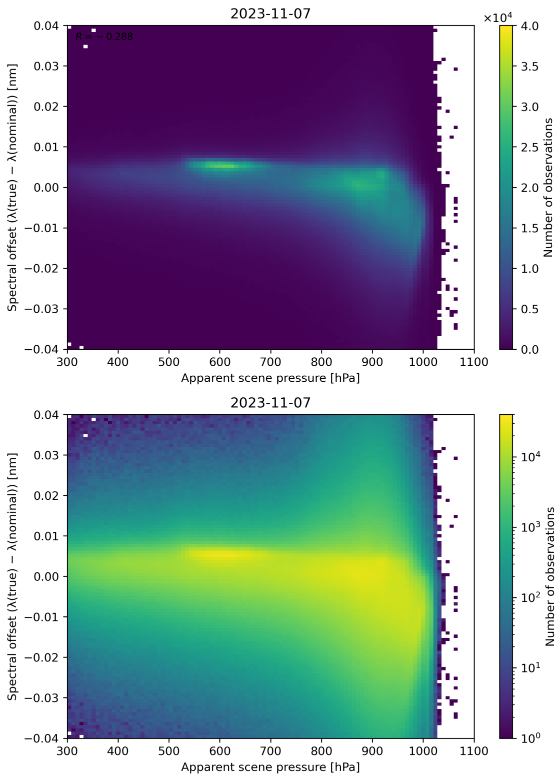
Figure 68: Scatter density plot of “Apparent scene pressure” against “Spectral offset ( \lambda(\text{true}) - \lambda(\text{nominal}) )” for 2023-11-07 to 2023-11-08.
