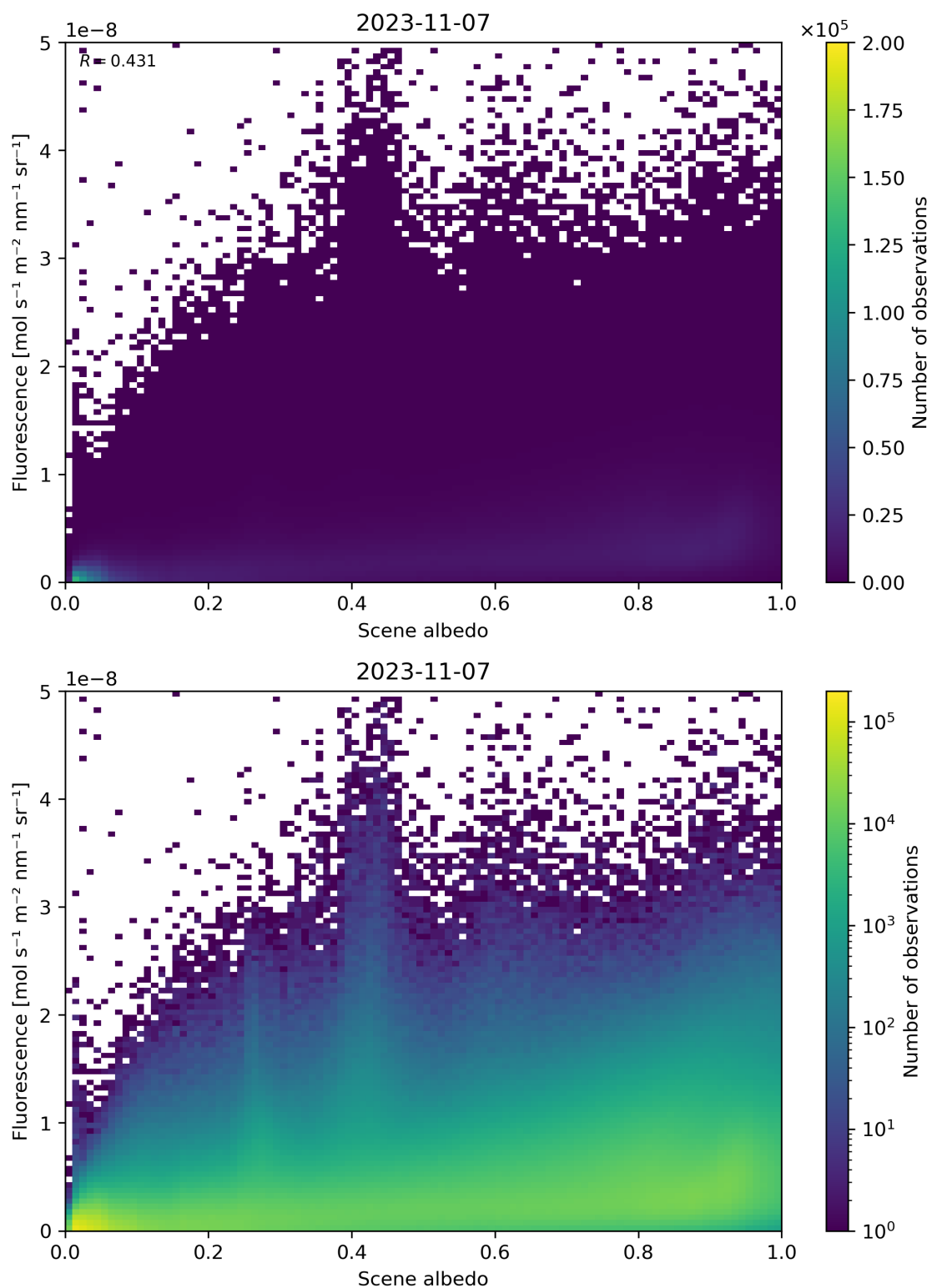
Figure 114: Scatter density plot of “Scene albedo” against “Fluorescence” for 2023-11-07 to 2023-11-08.
