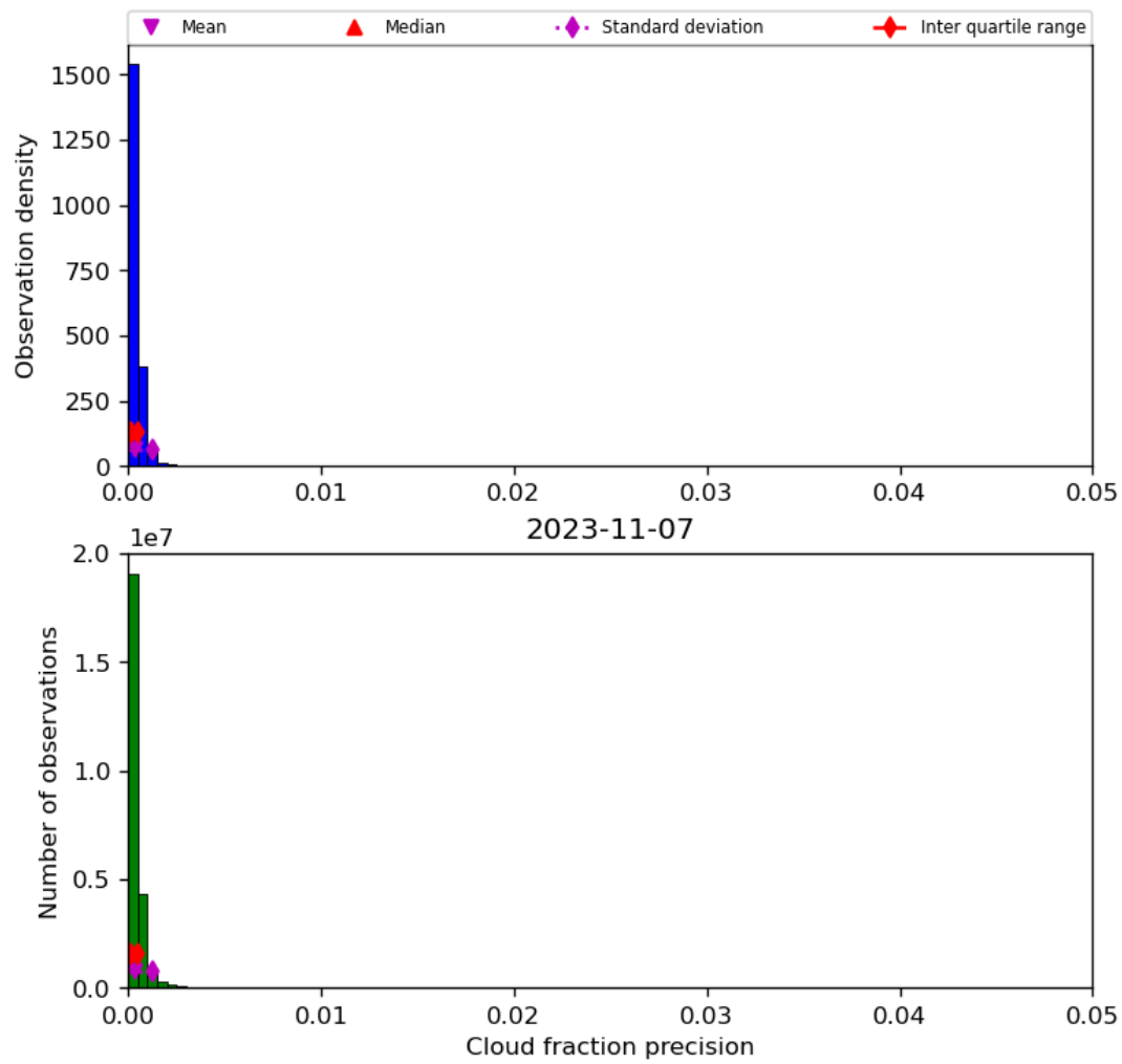
Figure 33: Histogram of “Cloud fraction precision” for 2023-11-07 to 2023-11-08
