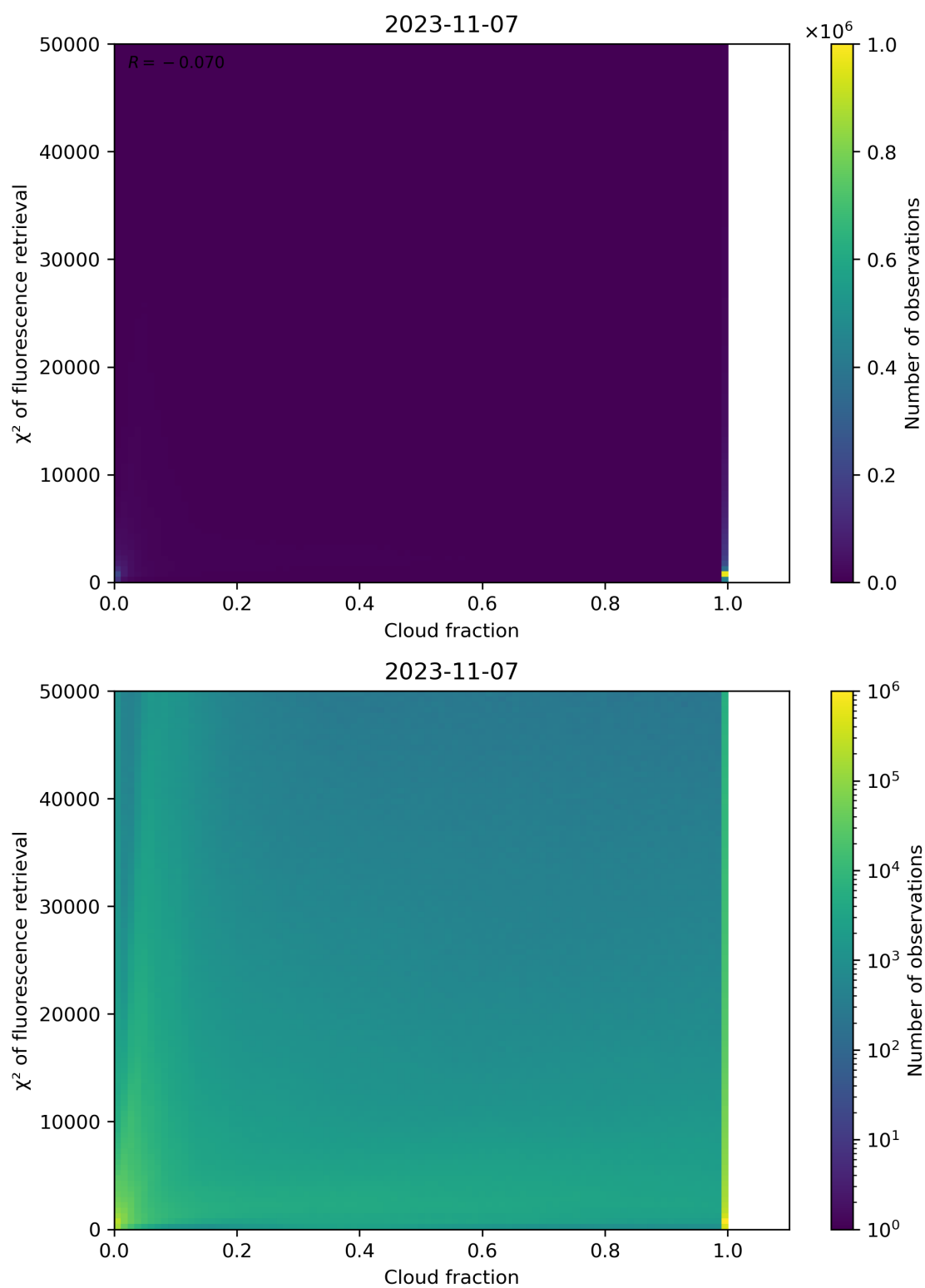
Figure 78: Scatter density plot of “Cloud fraction” against “ \chi^2 of fluorescence retrieval” for 2023-11-07 to 2023-11-08.
