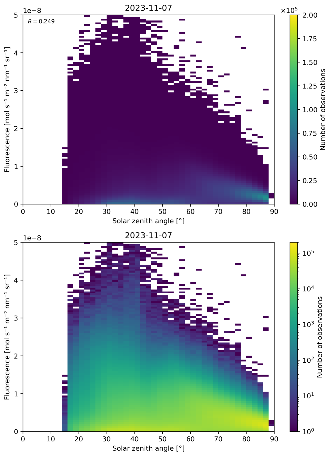
Figure 123: Scatter density plot of “Solar zenith angle” against “Fluorescence” for 2023-11-07 to 2023-11-08.
