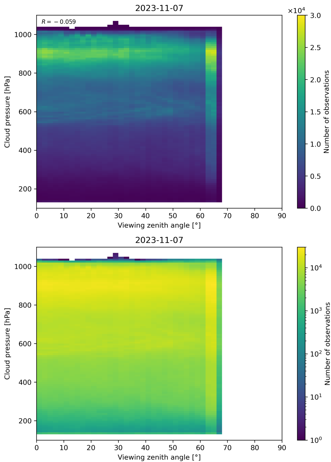
Figure 133: Scatter density plot of “Viewing zenith angle” against “Cloud pressure” for 2023-11-07 to 2023-11-08.
