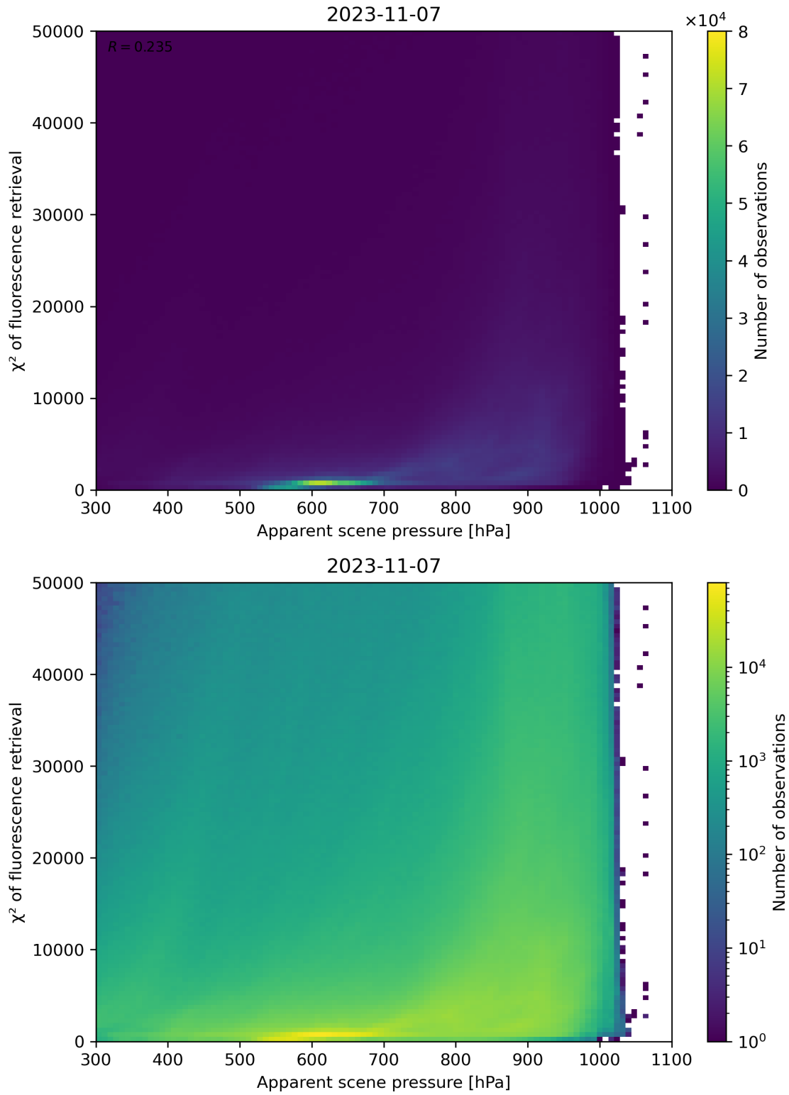
Figure 64: Scatter density plot of “Apparent scene pressure” against “ \chi^2 of fluorescence retrieval” for 2023-11-07 to 2023-11-08.
