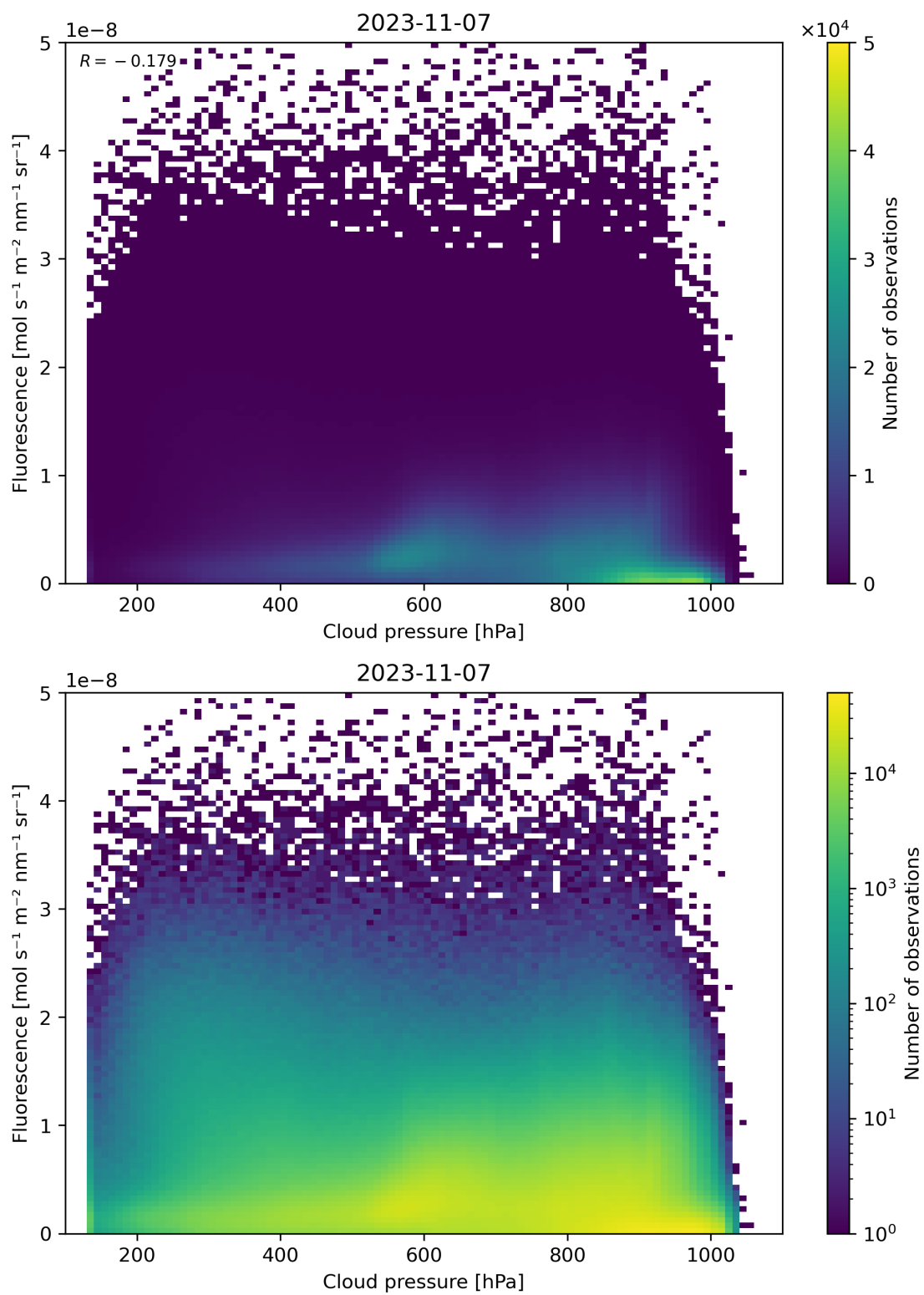
Figure 88: Scatter density plot of “Cloud pressure” against “Fluorescence” for 2023-11-07 to 2023-11-08.
