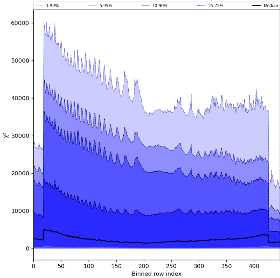
Figure 55: Along track statistics of “ \chi^2 ” for 2023-11-07 to 2023-11-08
