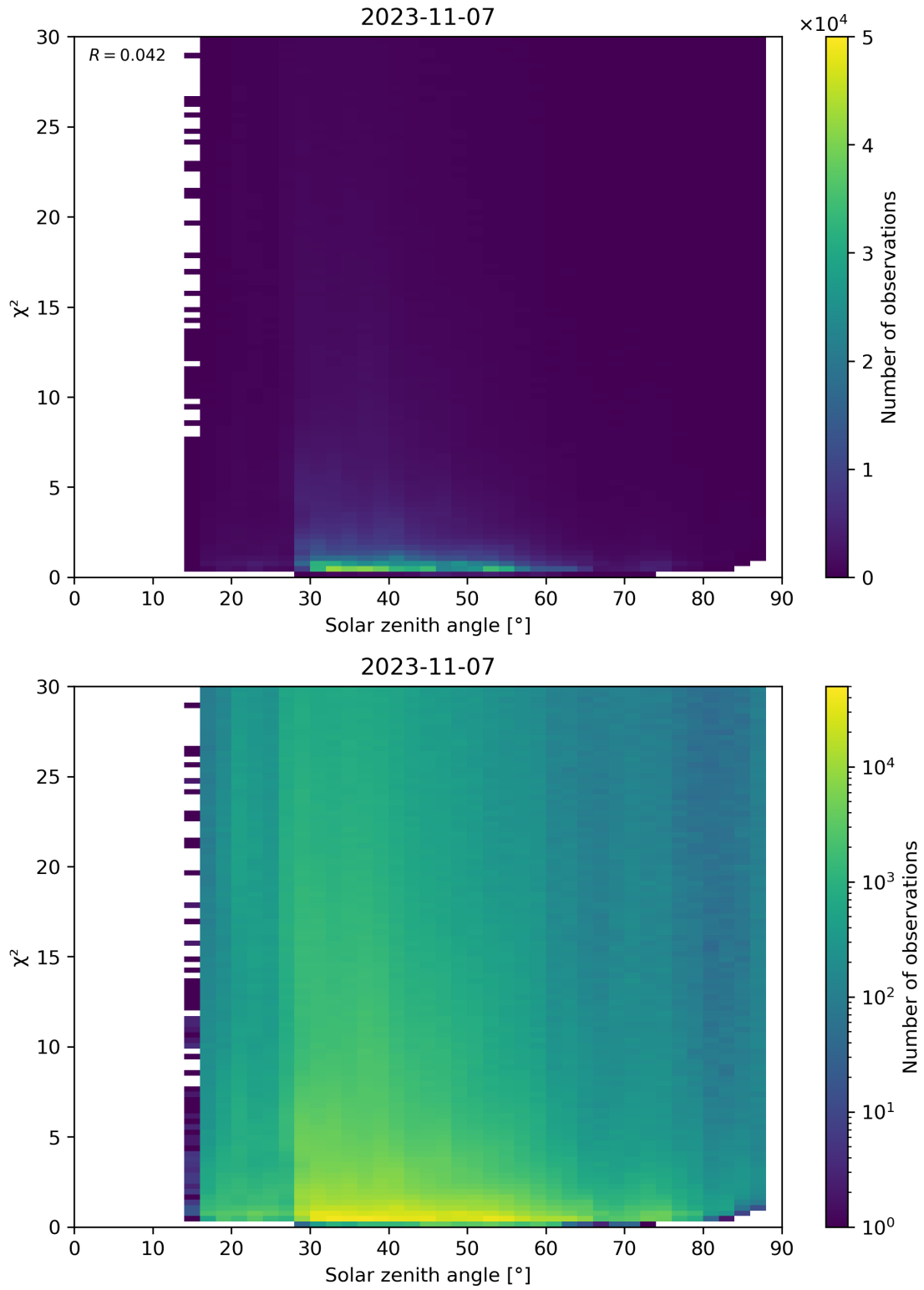
Figure 119: Scatter density plot of “Solar zenith angle” against “ \chi^2 ” for 2023-11-07 to 2023-11-08.
