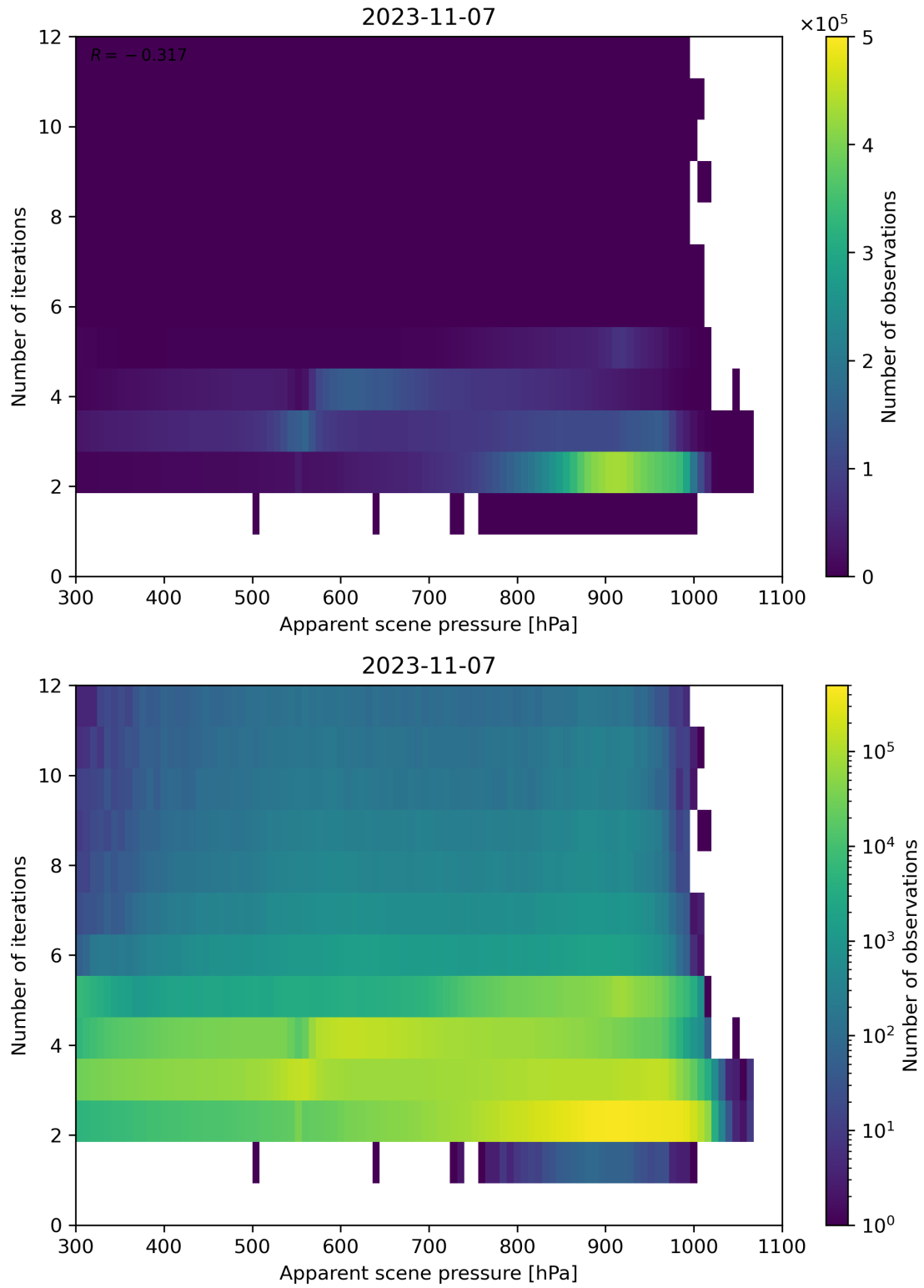
Figure 66: Scatter density plot of “Apparent scene pressure” against “Number of iterations” for 2023-11-07 to 2023-11-08.
