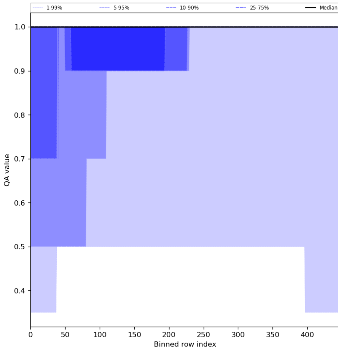
Figure 46: Along track statistics of “QA value” for 2023-11-07 to 2023-11-08
