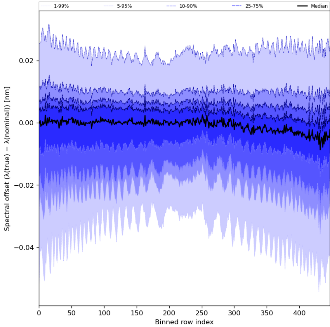
Figure 62: Along track statistics of “Spectral offset ( \lambda(\text{true}) - \lambda(\text{nominal}) )” for 2023-11-07 to 2023-11-08
