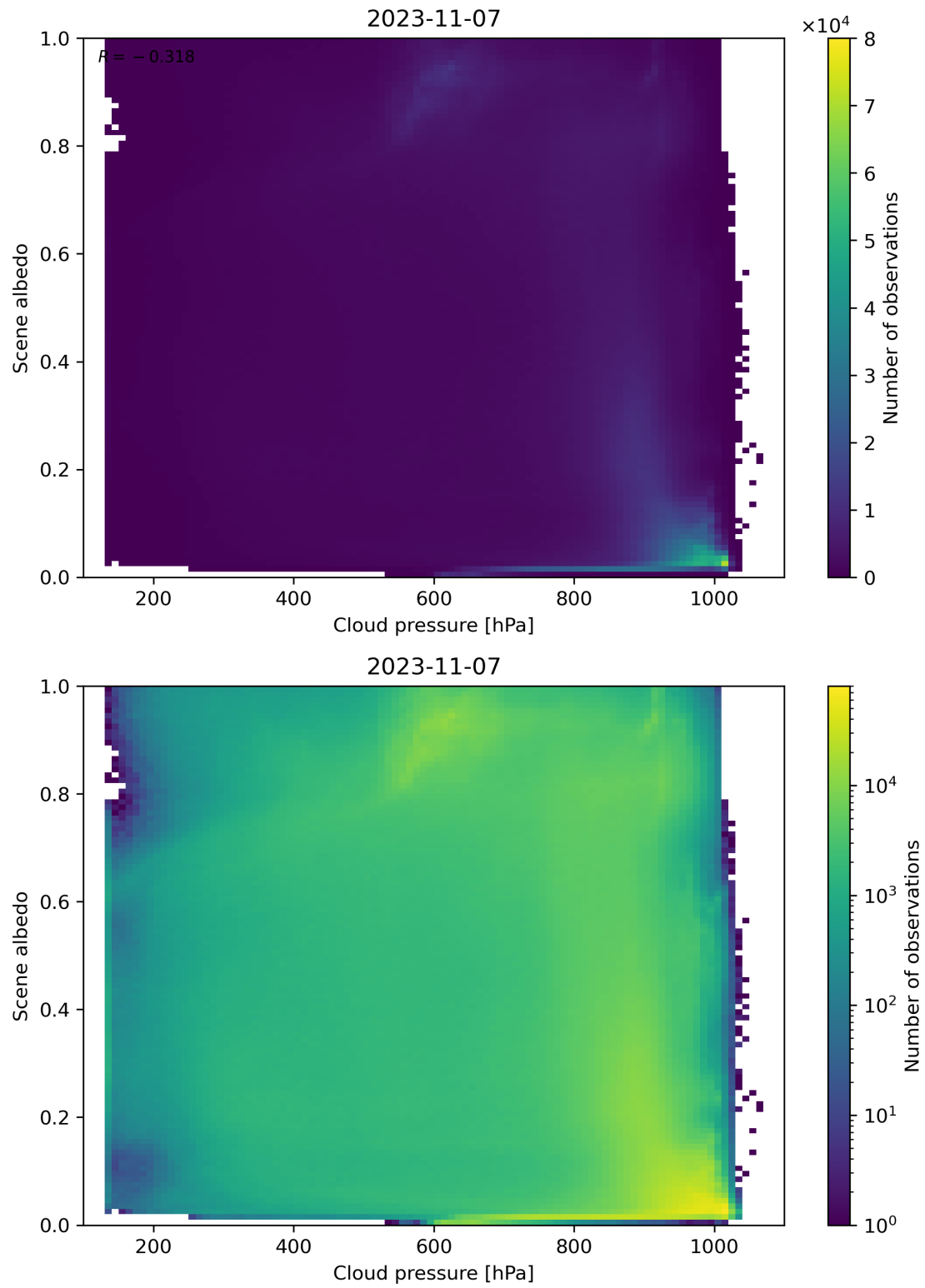
Figure 91: Scatter density plot of “Cloud pressure” against “Scene albedo” for 2023-11-07 to 2023-11-08.
