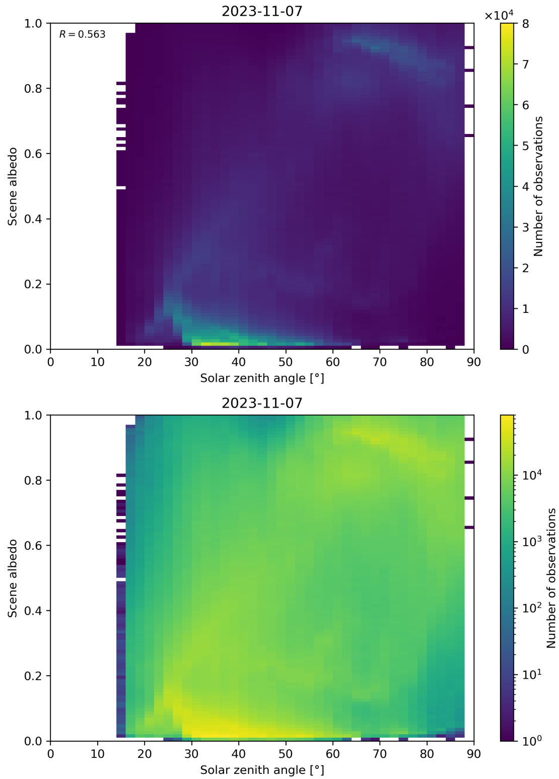
Figure 127: Scatter density plot of “Solar zenith angle” against “Scene albedo” for 2023-11-07 to 2023-11-08.
