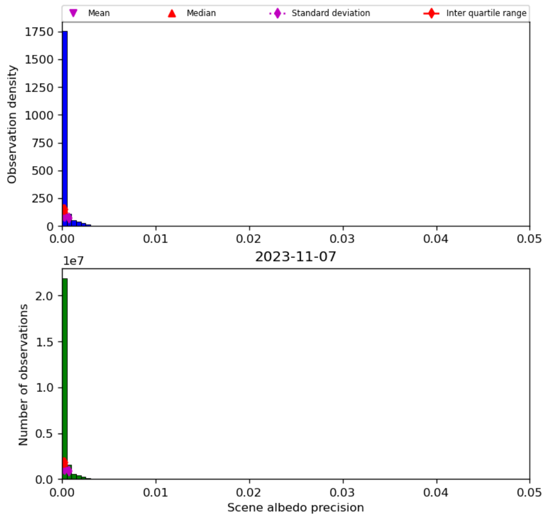
Figure 35: Histogram of “Scene albedo precision” for 2023-11-07 to 2023-11-08
