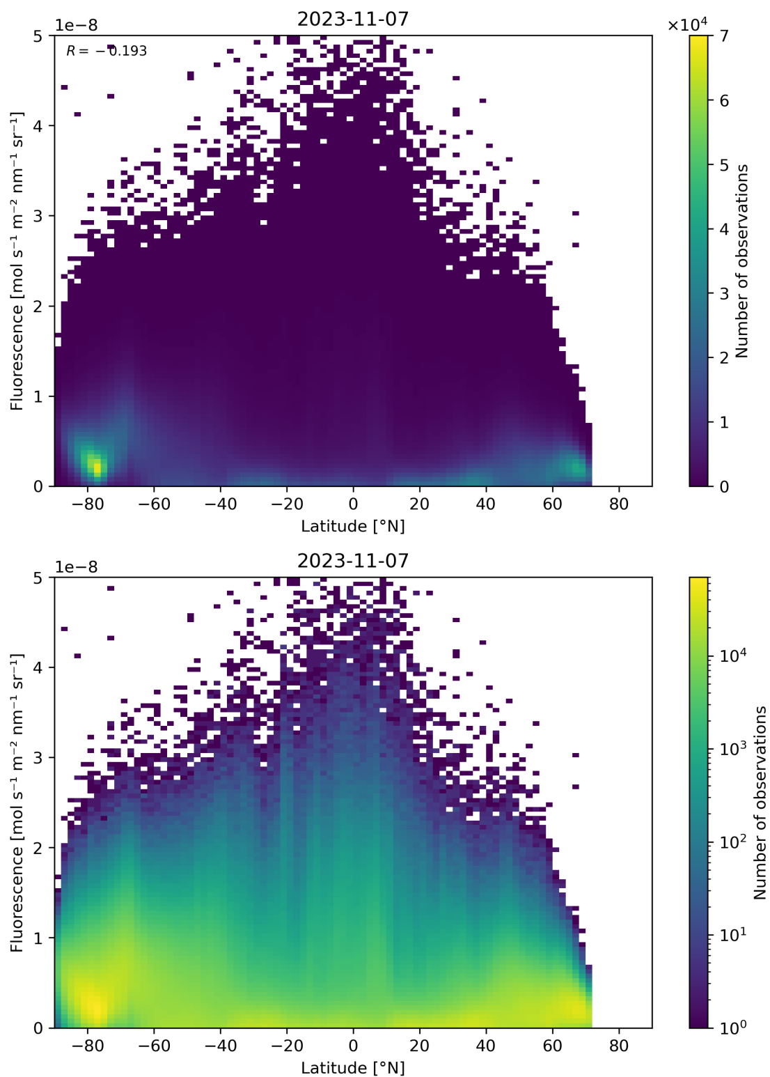
Figure 101: Scatter density plot of “Latitude” against “Fluorescence” for 2023-11-07 to 2023-11-08.
