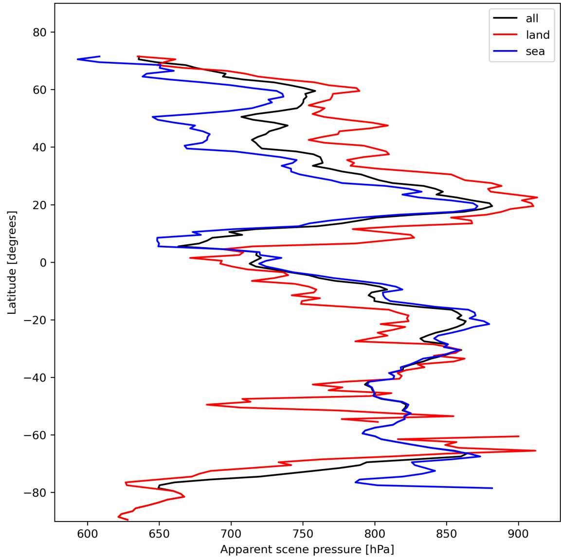
Figure 19: Zonal average of “Apparent scene pressure” for 2023-11-07 to 2023-11-08.
