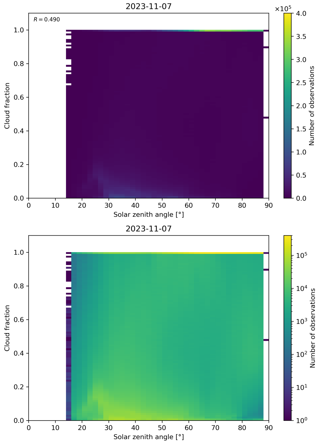
Figure 121: Scatter density plot of “Solar zenith angle” against “Cloud fraction” for 2023-11-07 to 2023-11-08.
