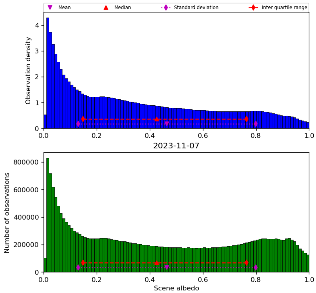
Figure 34: Histogram of “Scene albedo” for 2023-11-07 to 2023-11-08
