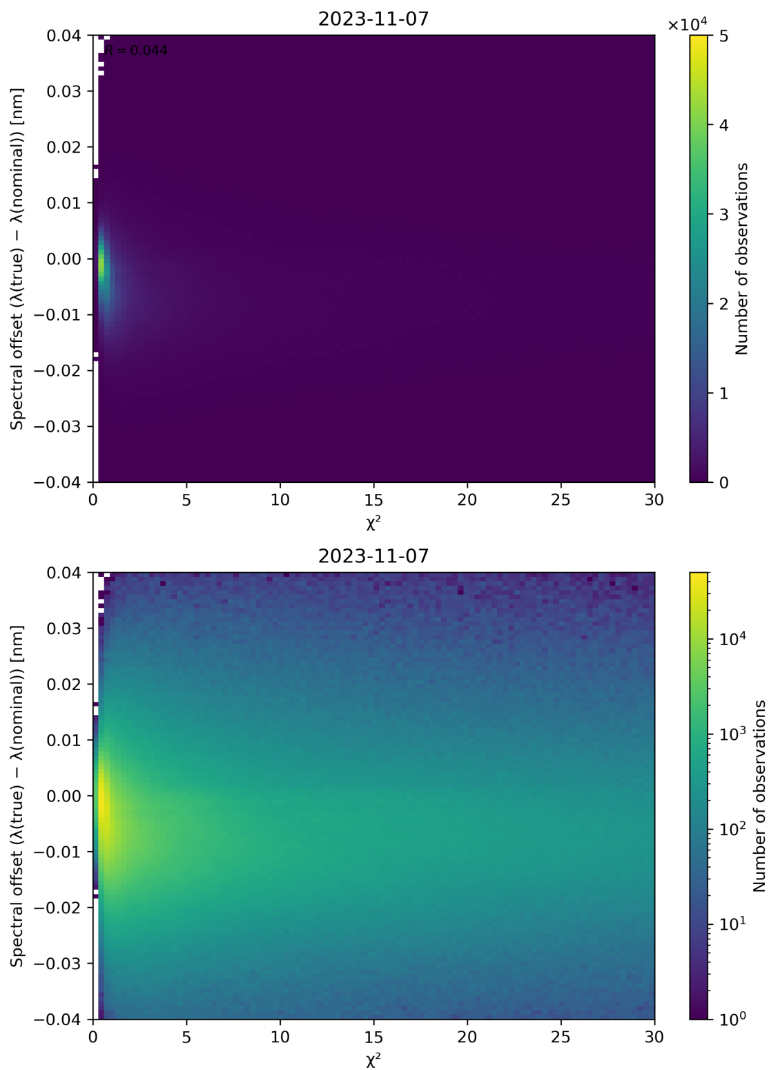
Figure 75: Scatter density plot of “ \chi^2 ” against “Spectral offset ( \lambda(\text{true}) - \lambda(\text{nominal}) )” for 2023-11-07 to 2023-11-08.
