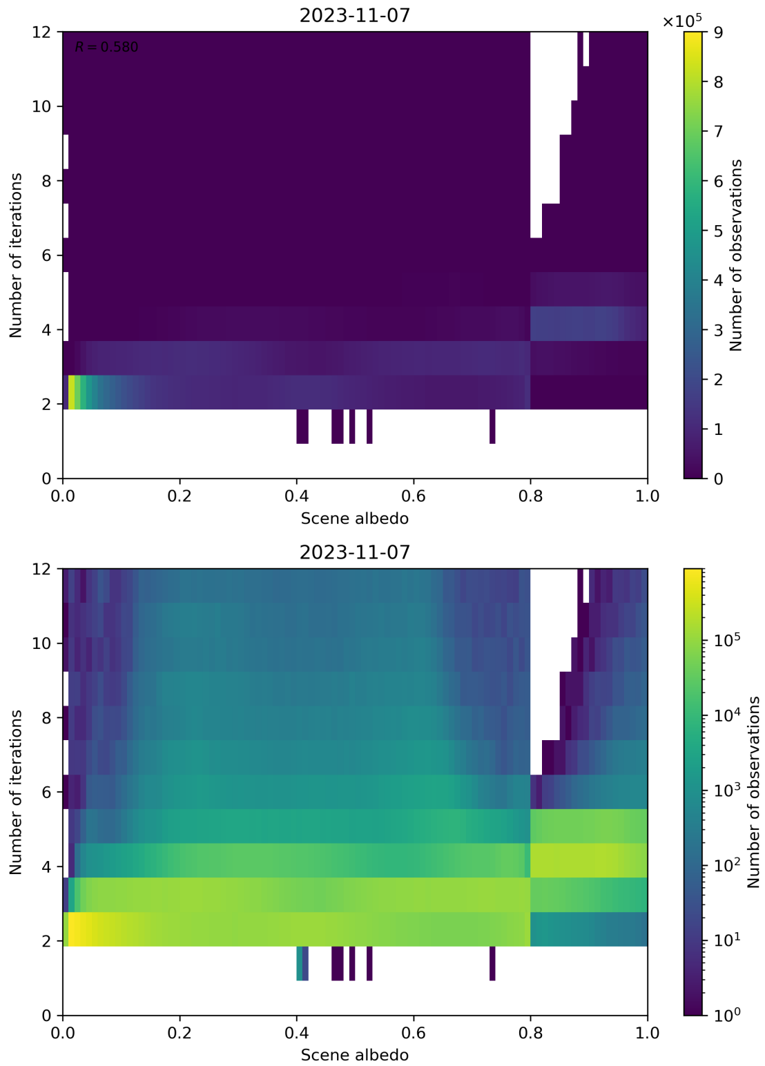
Figure 115: Scatter density plot of “Scene albedo” against “Number of iterations” for 2023-11-07 to 2023-11-08.
