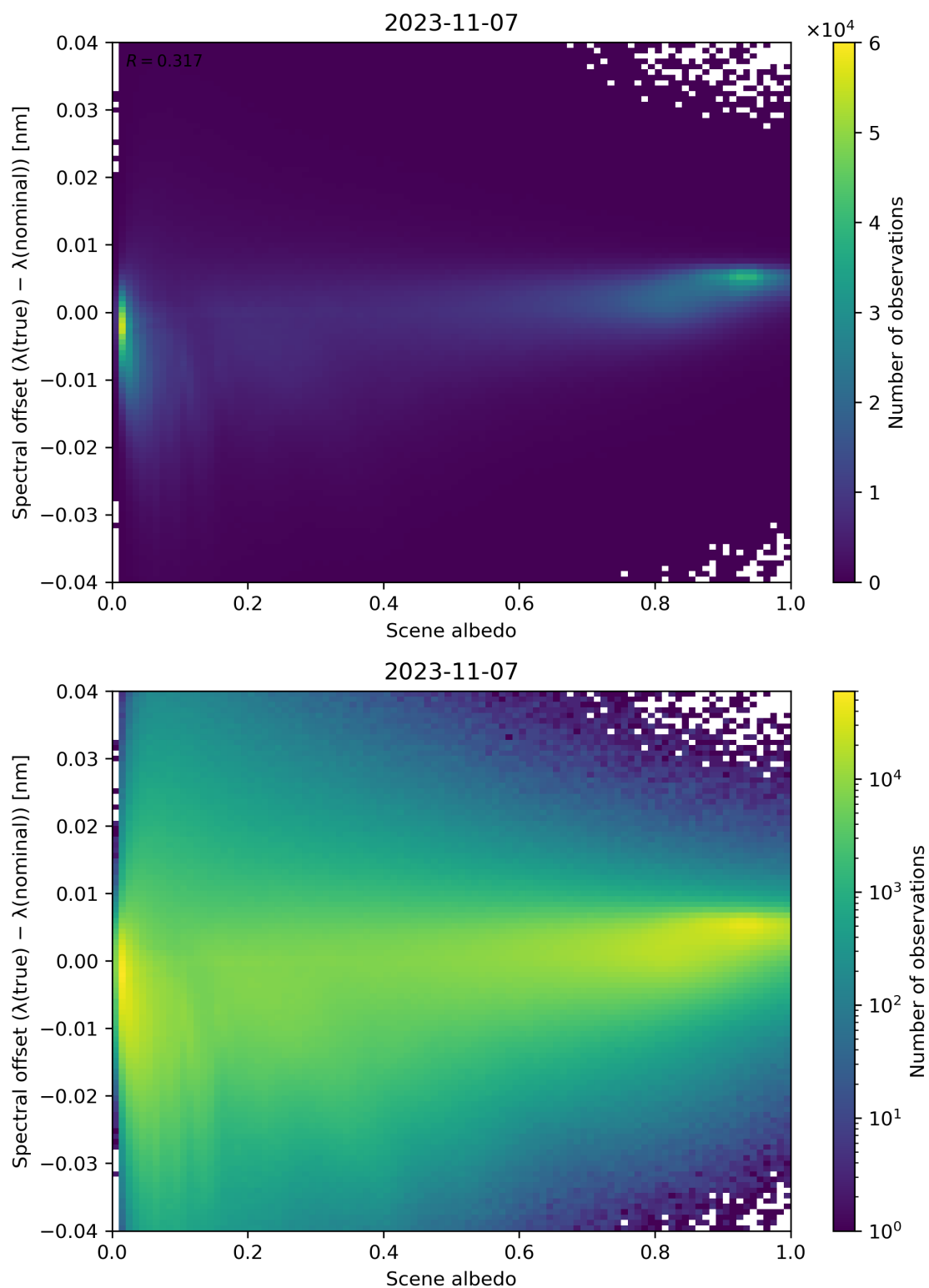
Figure 117: Scatter density plot of “Scene albedo” against “Spectral offset ( \lambda(\text{true}) - \lambda(\text{nominal}) )” for 2023-11-07 to 2023-11-08.
