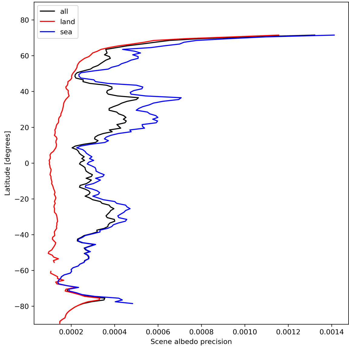
Figure 18: Zonal average of “Scene albedo precision” for 2023-11-07 to 2023-11-08.
