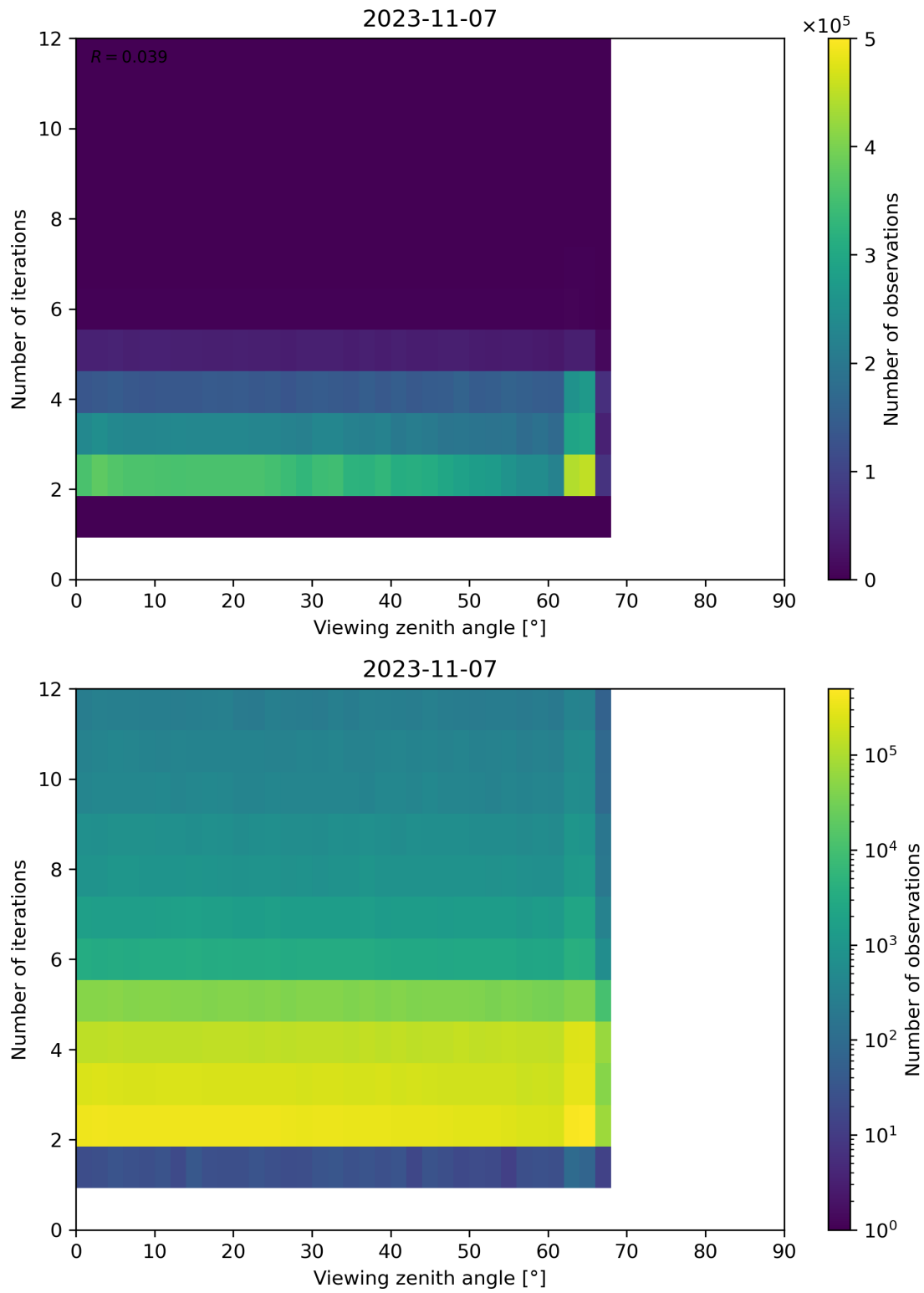
Figure 136: Scatter density plot of “Viewing zenith angle” against “Number of iterations” for 2023-11-07 to 2023-11-08.
