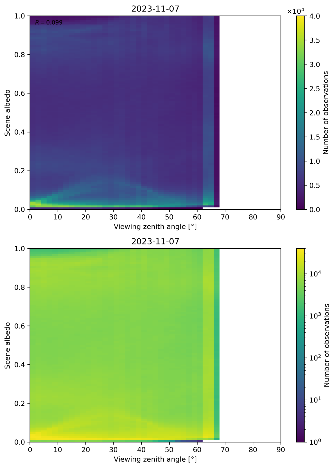
Figure 138: Scatter density plot of “Viewing zenith angle” against “Scene albedo” for 2023-11-07 to 2023-11-08.
