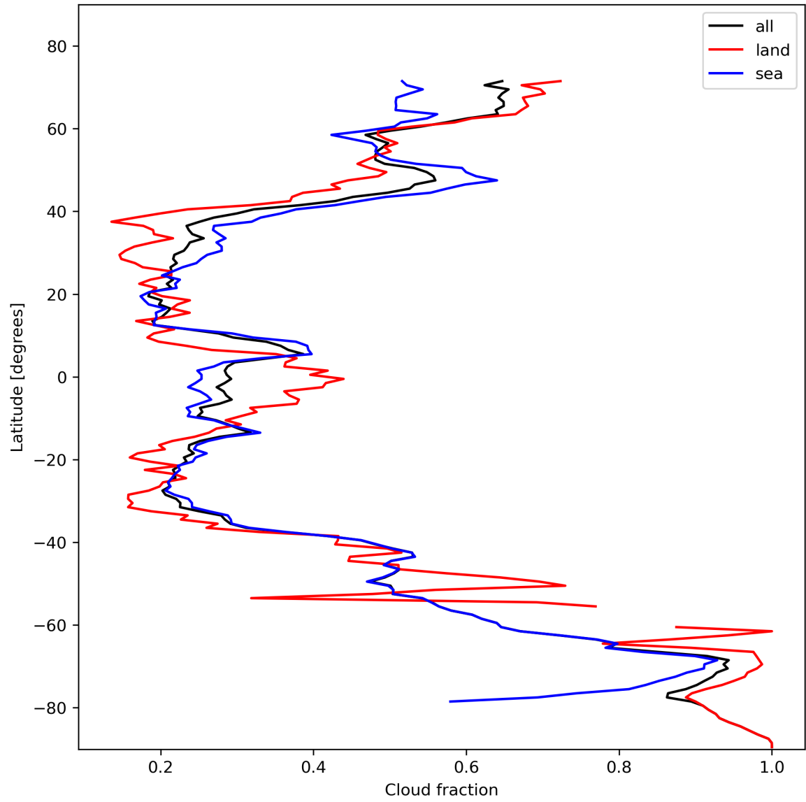
Figure 15: Zonal average of “Cloud fraction” for 2023-11-07 to 2023-11-08.
