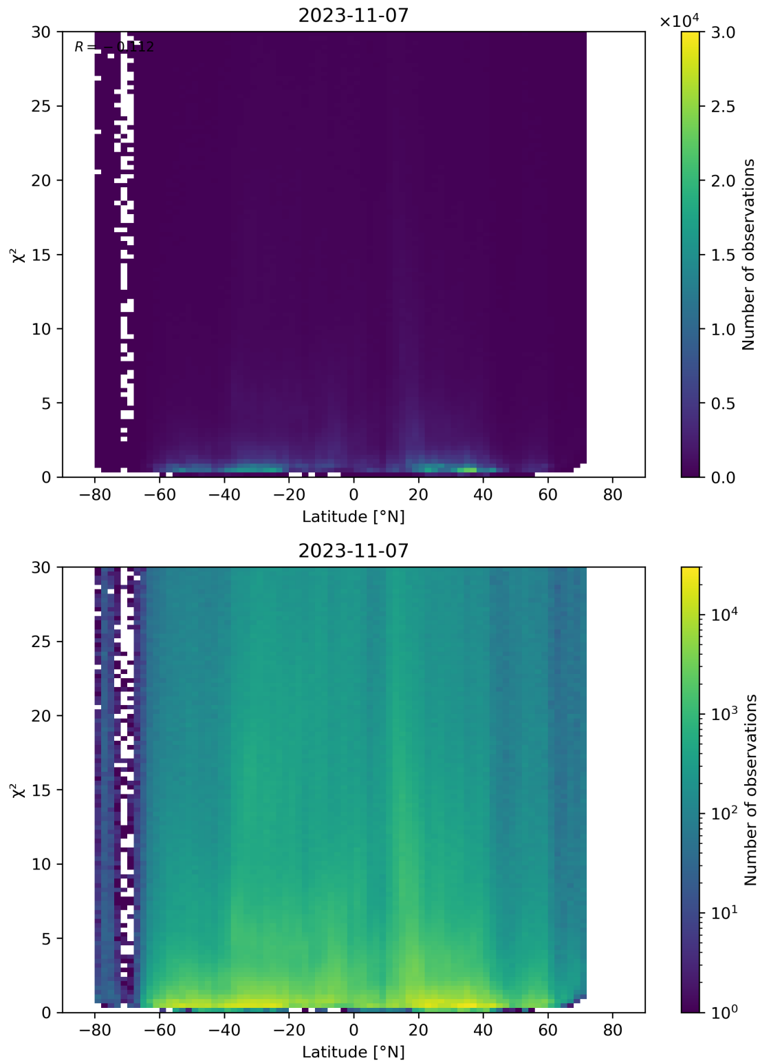
Figure 97: Scatter density plot of “Latitude” against “ \chi^2 ” for 2023-11-07 to 2023-11-08.
