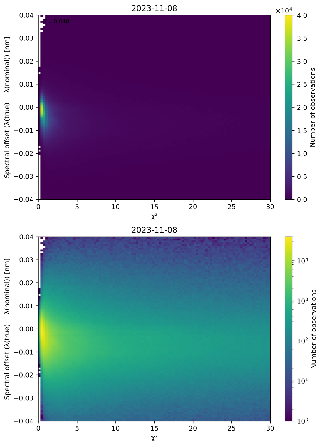
Figure 75: Scatter density plot of “ \chi^2 ” against “Spectral offset ( \lambda(\text{true}) - \lambda(\text{nominal}) )” for 2023-11-07 to 2023-11-09.
