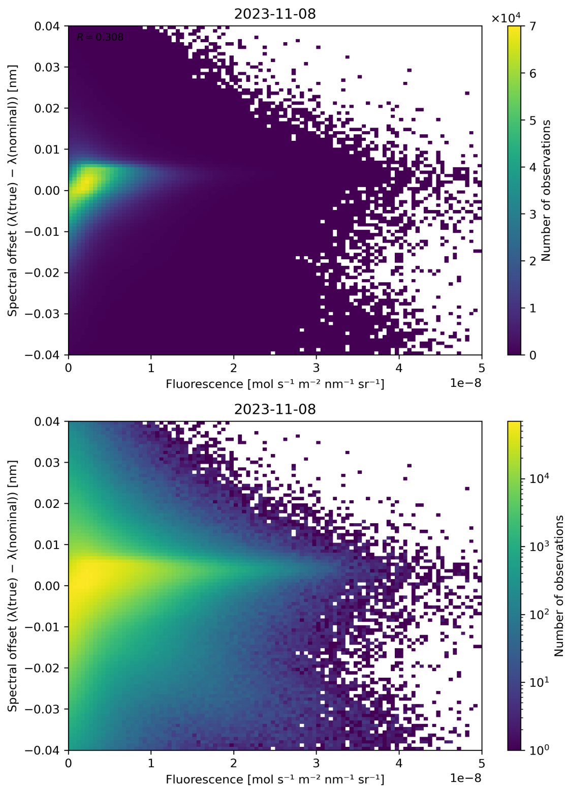
Figure 95: Scatter density plot of “Fluorescence” against “Spectral offset ( \lambda(\text{true}) - \lambda(\text{nominal}) )” for 2023-11-07 to 2023-11-09.
