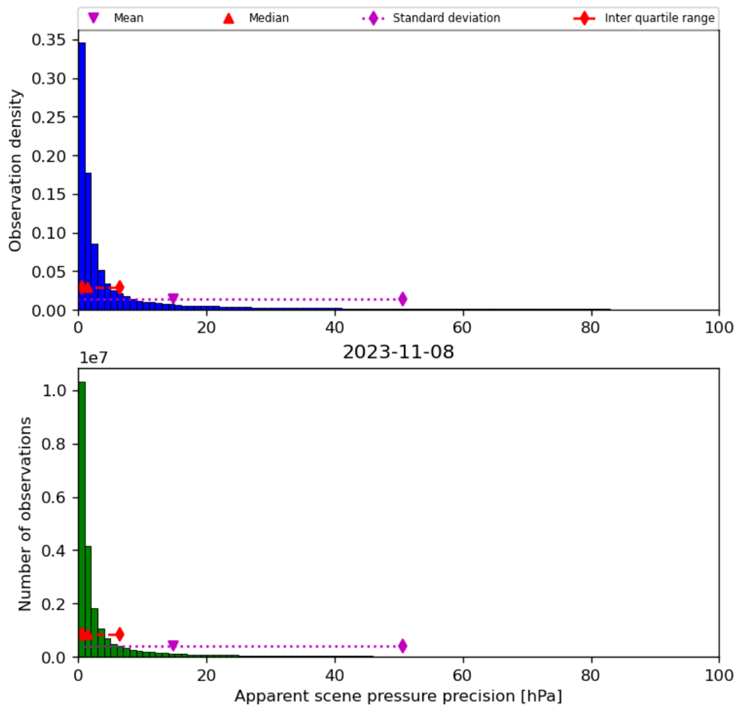
Figure 37: Histogram of “Apparent scene pressure precision” for 2023-11-07 to 2023-11-09
