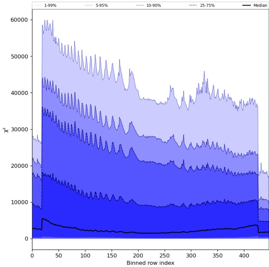
Figure 55: Along track statistics of “ \chi^2 ” for 2023-11-07 to 2023-11-09
