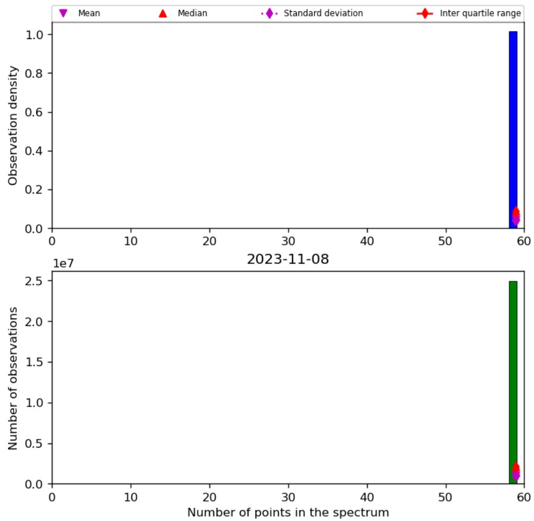
Figure 44: Histogram of “Number of points in the spectrum” for 2023-11-07 to 2023-11-09
