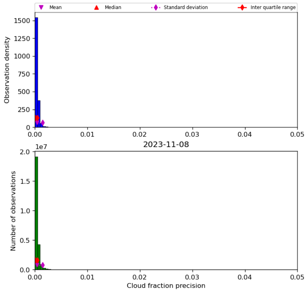
Figure 33: Histogram of “Cloud fraction precision” for 2023-11-07 to 2023-11-09
