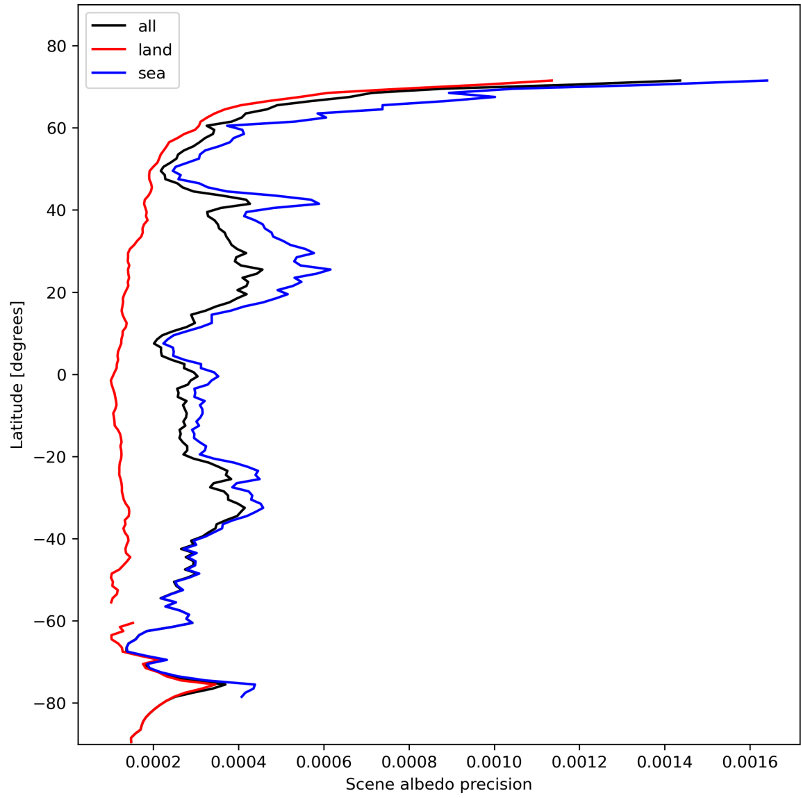
Figure 18: Zonal average of “Scene albedo precision” for 2023-11-07 to 2023-11-09.
