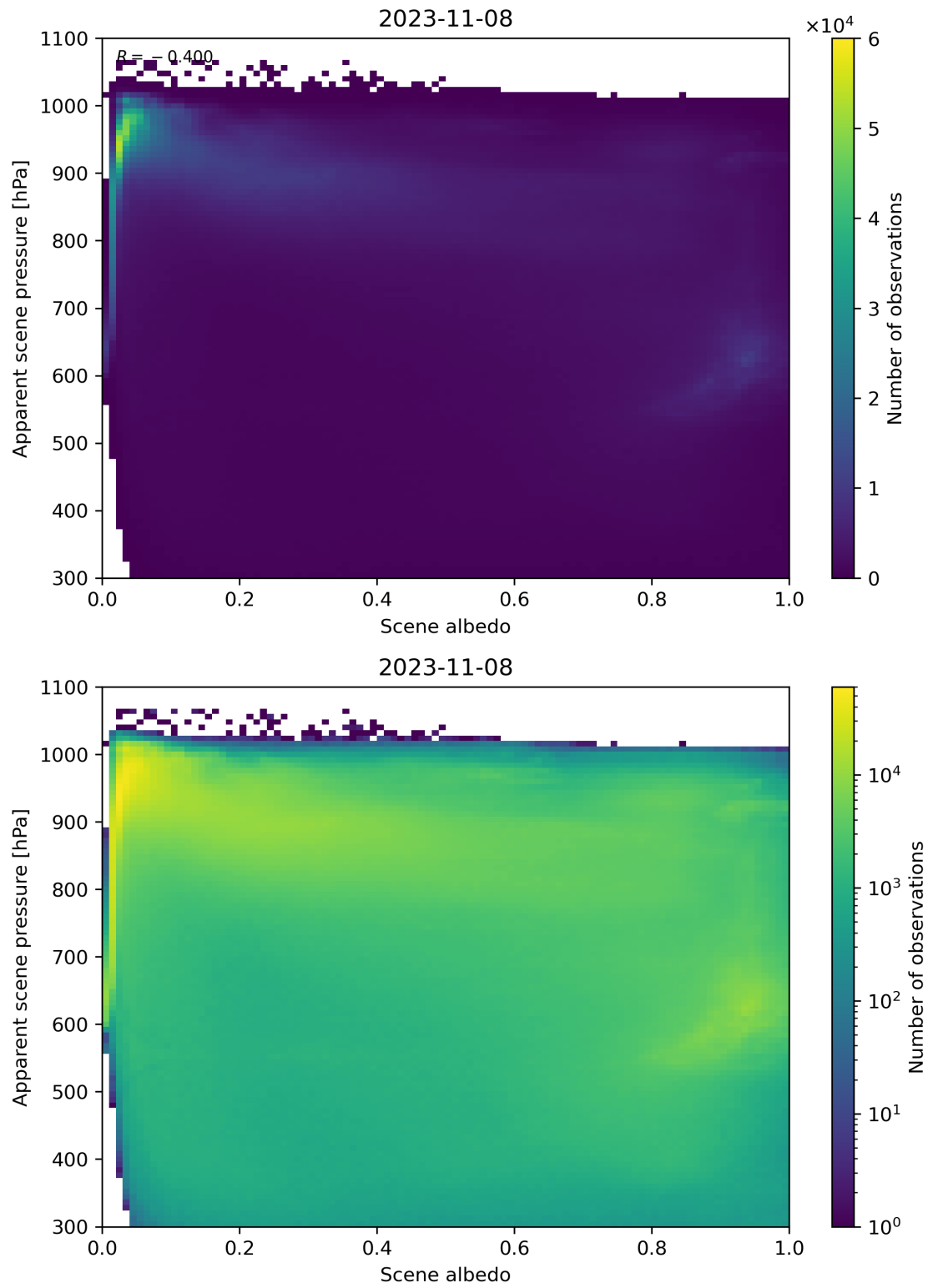
Figure 111: Scatter density plot of “Scene albedo” against “Apparent scene pressure” for 2023-11-07 to 2023-11-09.
