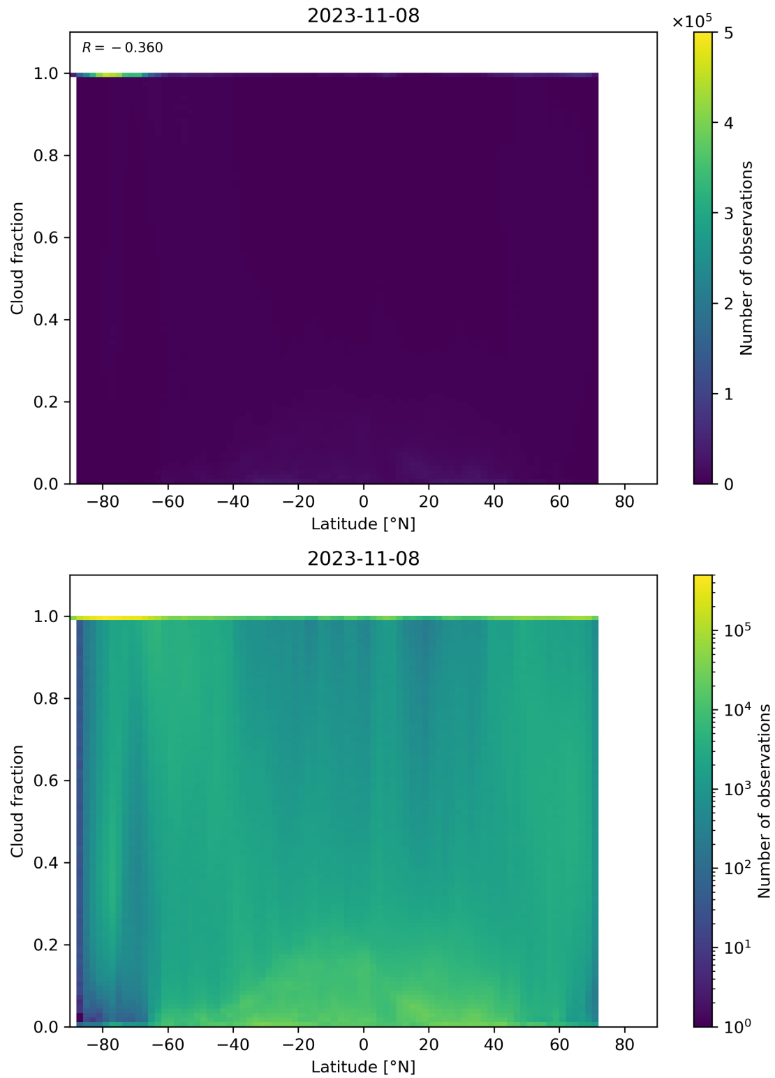
Figure 99: Scatter density plot of “Latitude” against “Cloud fraction” for 2023-11-07 to 2023-11-09.
