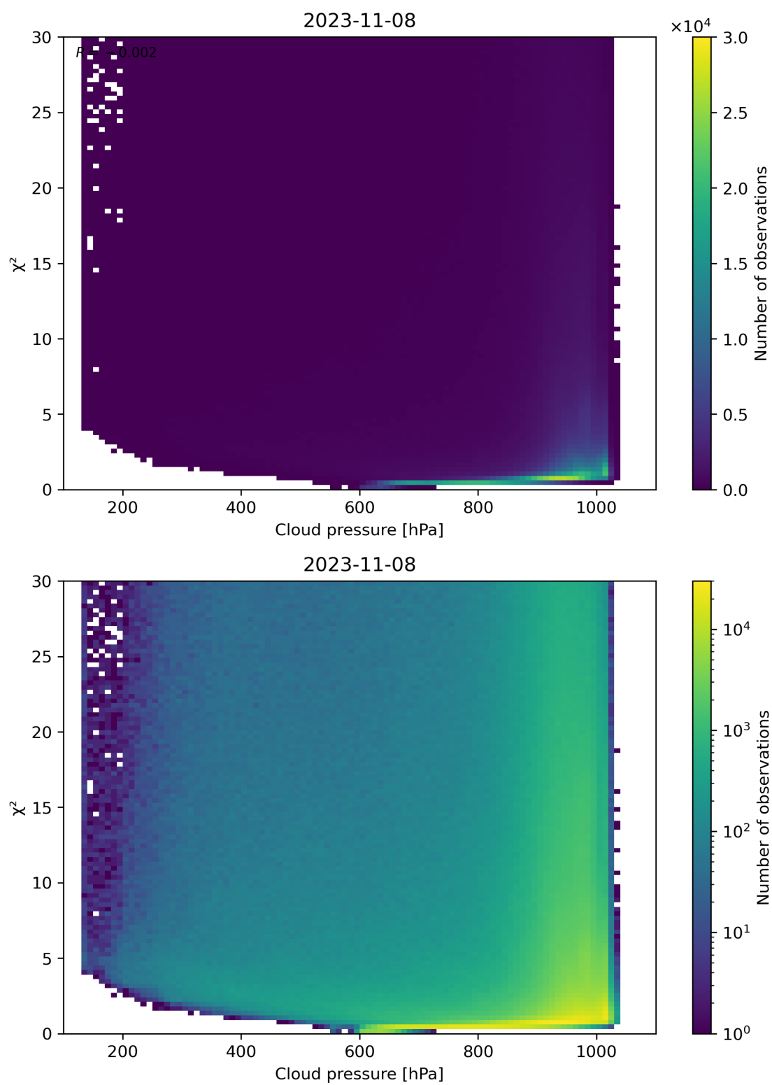
Figure 85: Scatter density plot of “Cloud pressure” against “ \chi^2 ” for 2023-11-07 to 2023-11-09.
