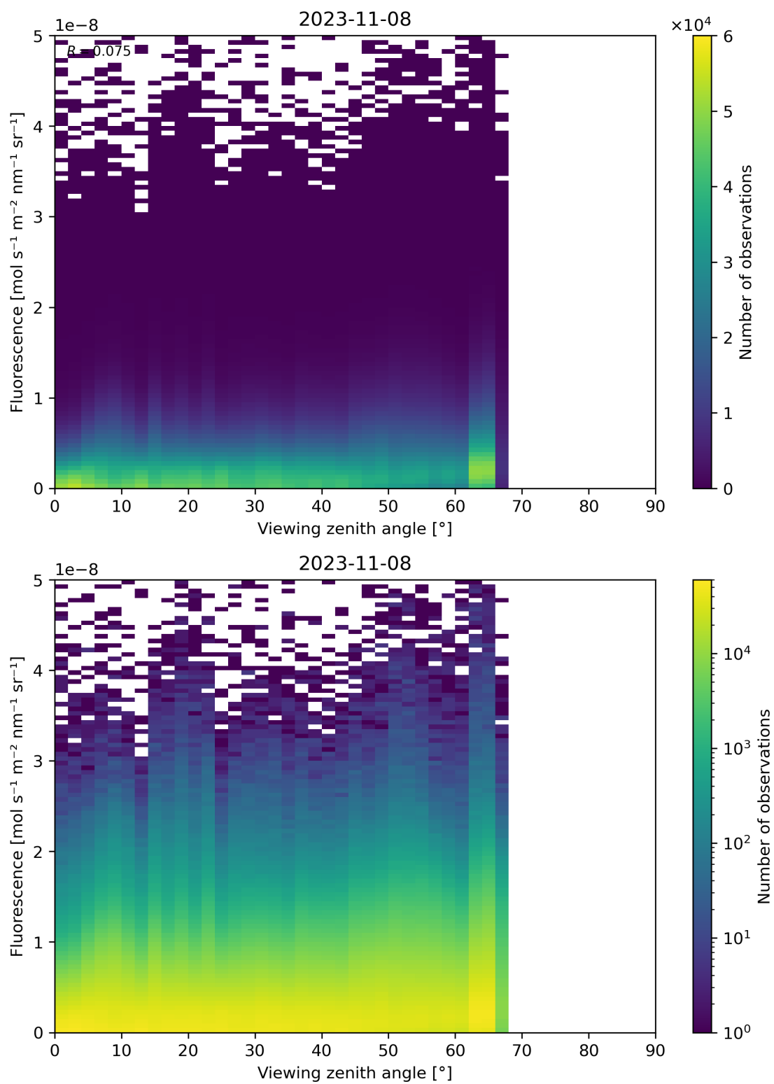
Figure 134: Scatter density plot of “Viewing zenith angle” against “Fluorescence” for 2023-11-07 to 2023-11-09.
