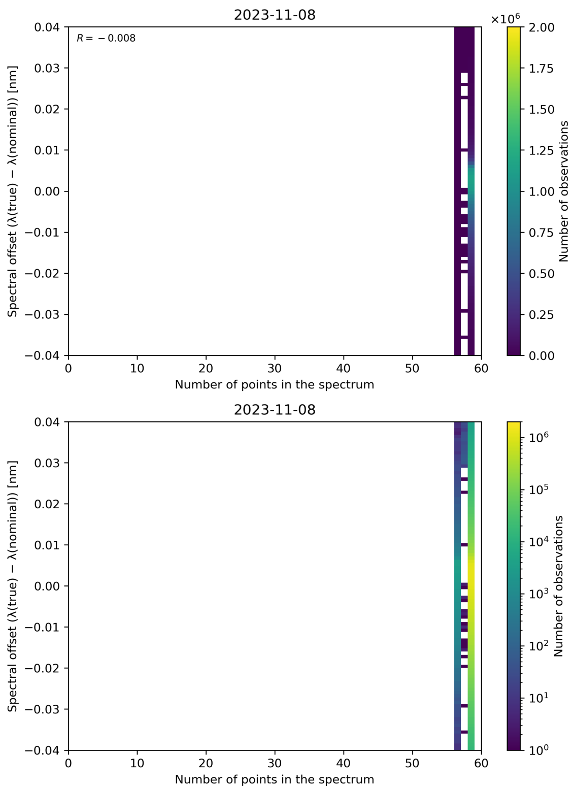
Figure 110: Scatter density plot of “Number of points in the spectrum” against “Spectral offset ( \lambda(\text{true}) - \lambda(\text{nominal}) )” for 2023-11-07 to 2023-11-09.
