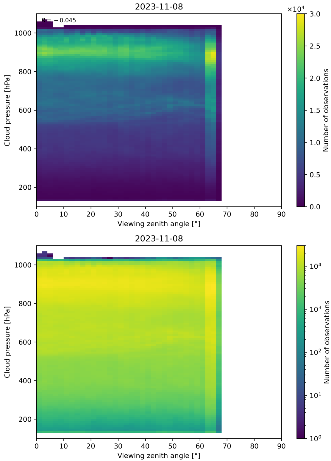
Figure 133: Scatter density plot of “Viewing zenith angle” against “Cloud pressure” for 2023-11-07 to 2023-11-09.
