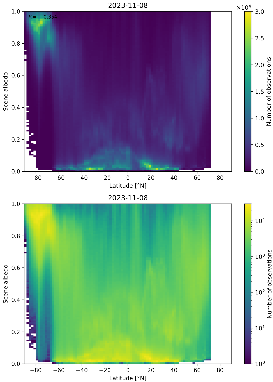
Figure 104: Scatter density plot of “Latitude” against “Scene albedo” for 2023-11-07 to 2023-11-09.
