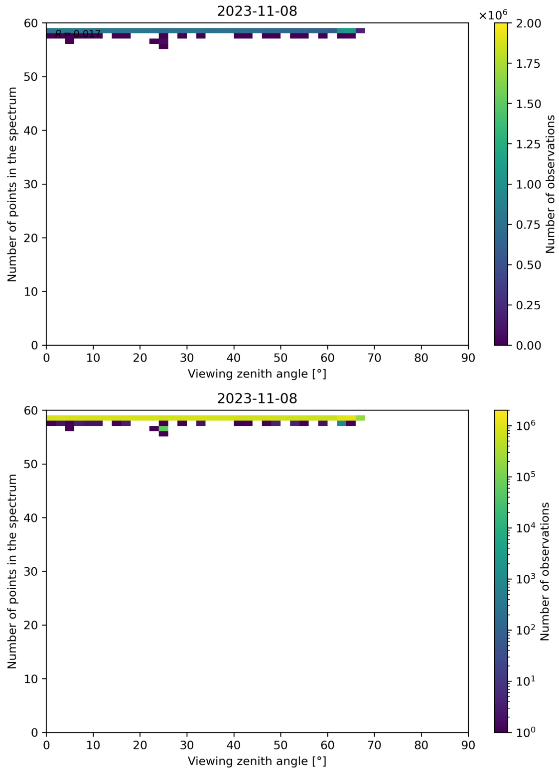
Figure 137: Scatter density plot of “Viewing zenith angle” against “Number of points in the spectrum” for 2023-11-07 to 2023-11-09.
