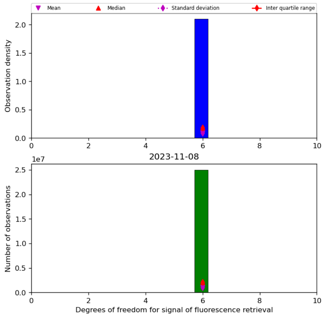
Figure 43: Histogram of “Degrees of freedom for signal of fluorescence retrieval” for 2023-11-07 to 2023-11-09
