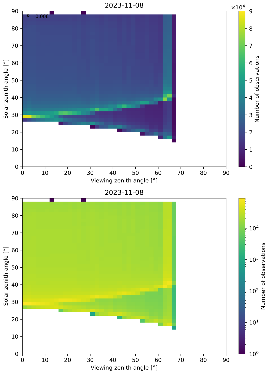
Figure 139: Scatter density plot of “Viewing zenith angle” against “Solar zenith angle” for 2023-11-07 to 2023-11-09.
