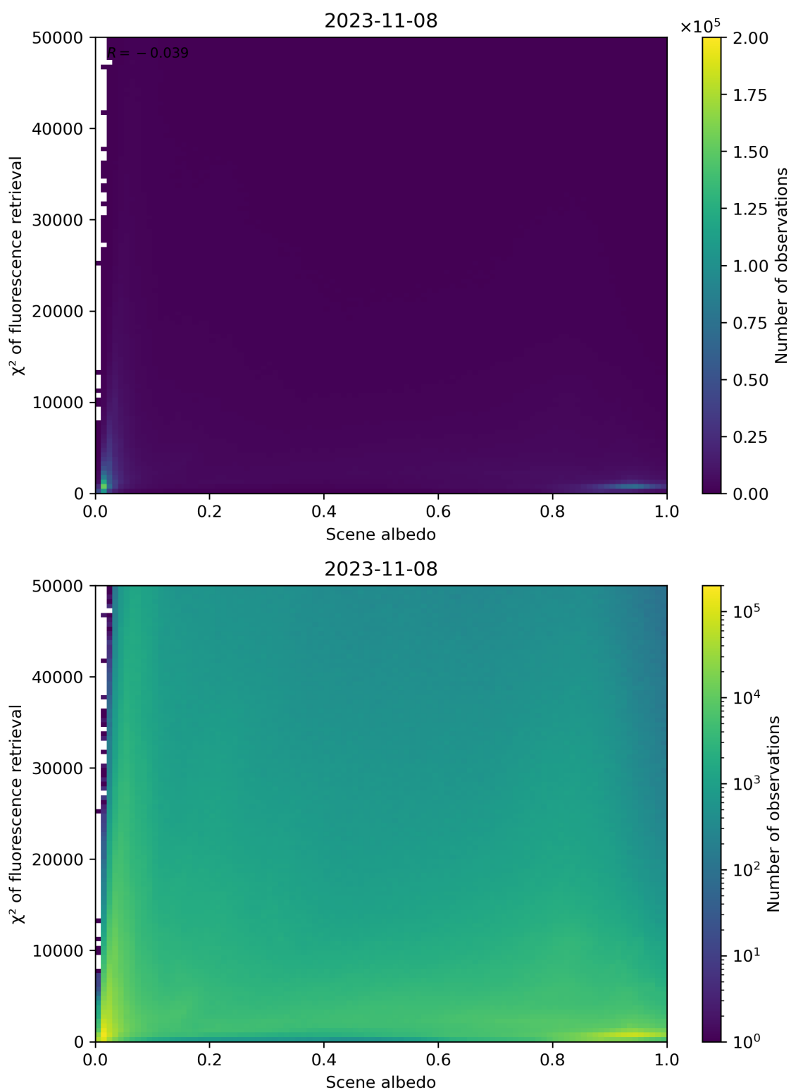
Figure 113: Scatter density plot of “Scene albedo” against “ \chi^2 of fluorescence retrieval” for 2023-11-07 to 2023-11-09.
