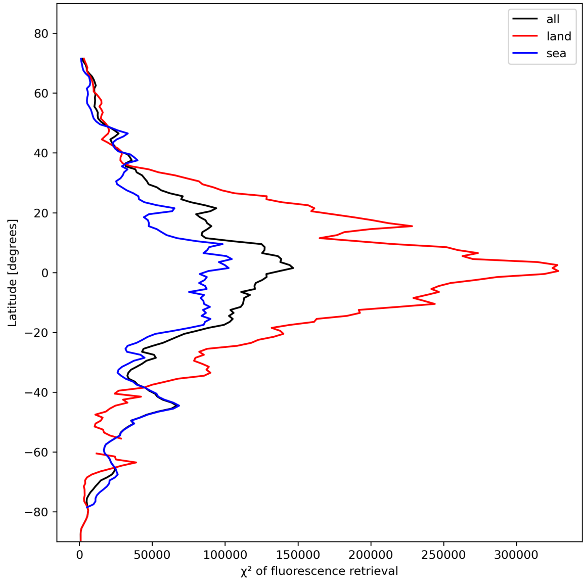
Figure 25: Zonal average of “ \chi^2 of fluorescence retrieval” for 2023-11-07 to 2023-11-09.
