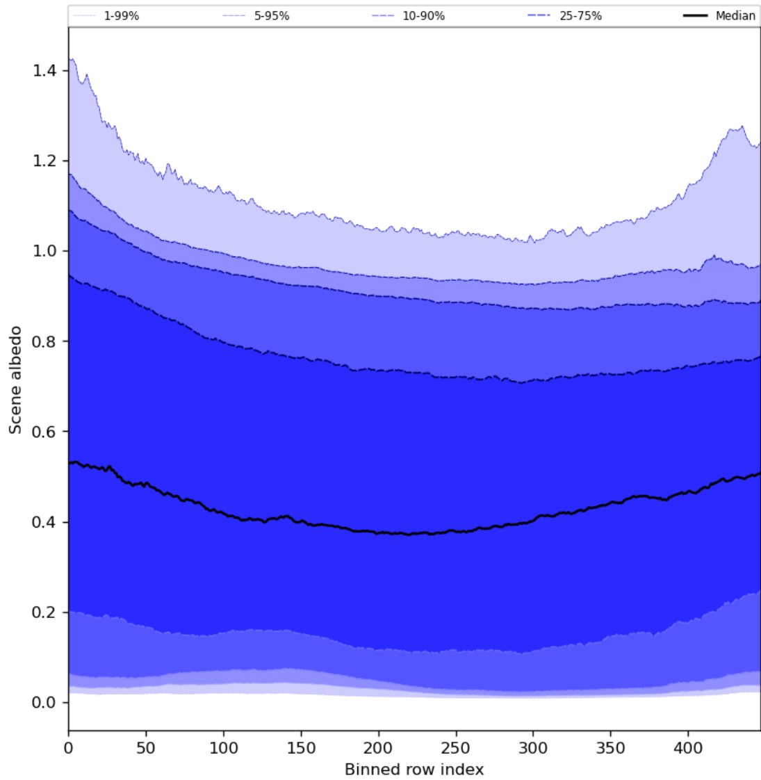
Figure 51: Along track statistics of “Scene albedo” for 2023-11-07 to 2023-11-09
