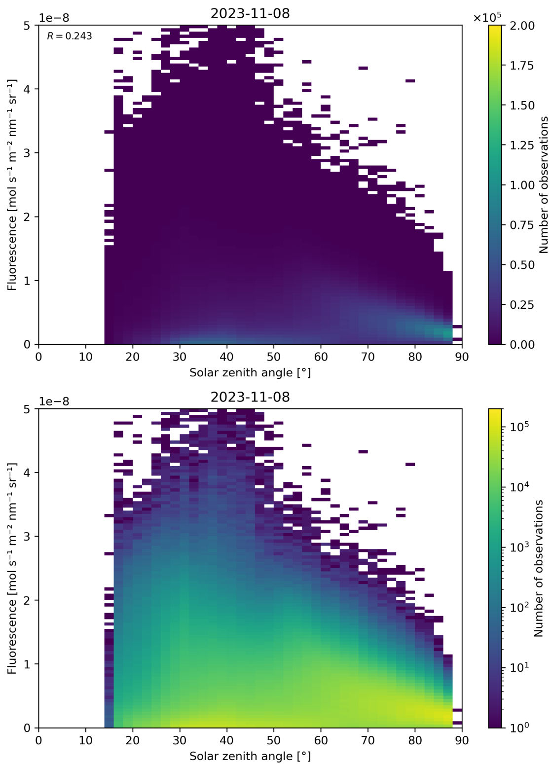
Figure 123: Scatter density plot of “Solar zenith angle” against “Fluorescence” for 2023-11-07 to 2023-11-09.
