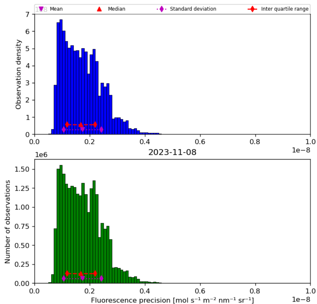
Figure 41: Histogram of “Fluorescence precision” for 2023-11-07 to 2023-11-09
