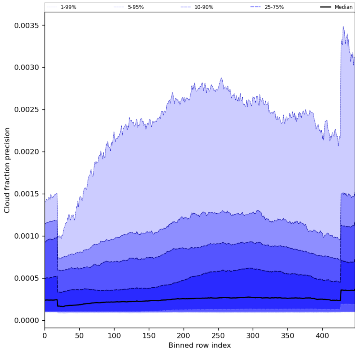
Figure 50: Along track statistics of “Cloud fraction precision” for 2023-11-07 to 2023-11-09
