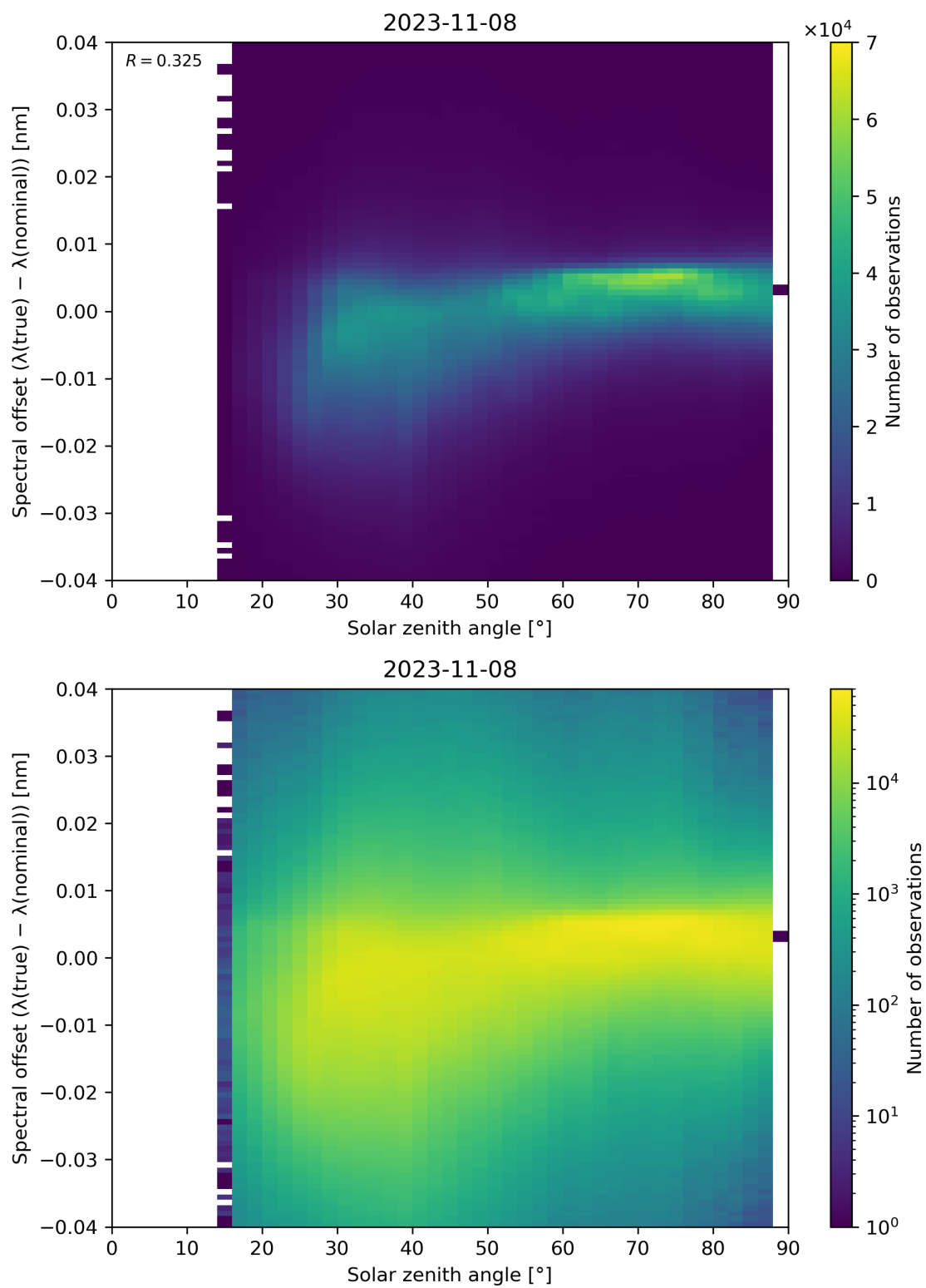
Figure 128: Scatter density plot of “Solar zenith angle” against “Spectral offset ( \lambda(\text{true}) - \lambda(\text{nominal}) )” for 2023-11-07 to 2023-11-09.
