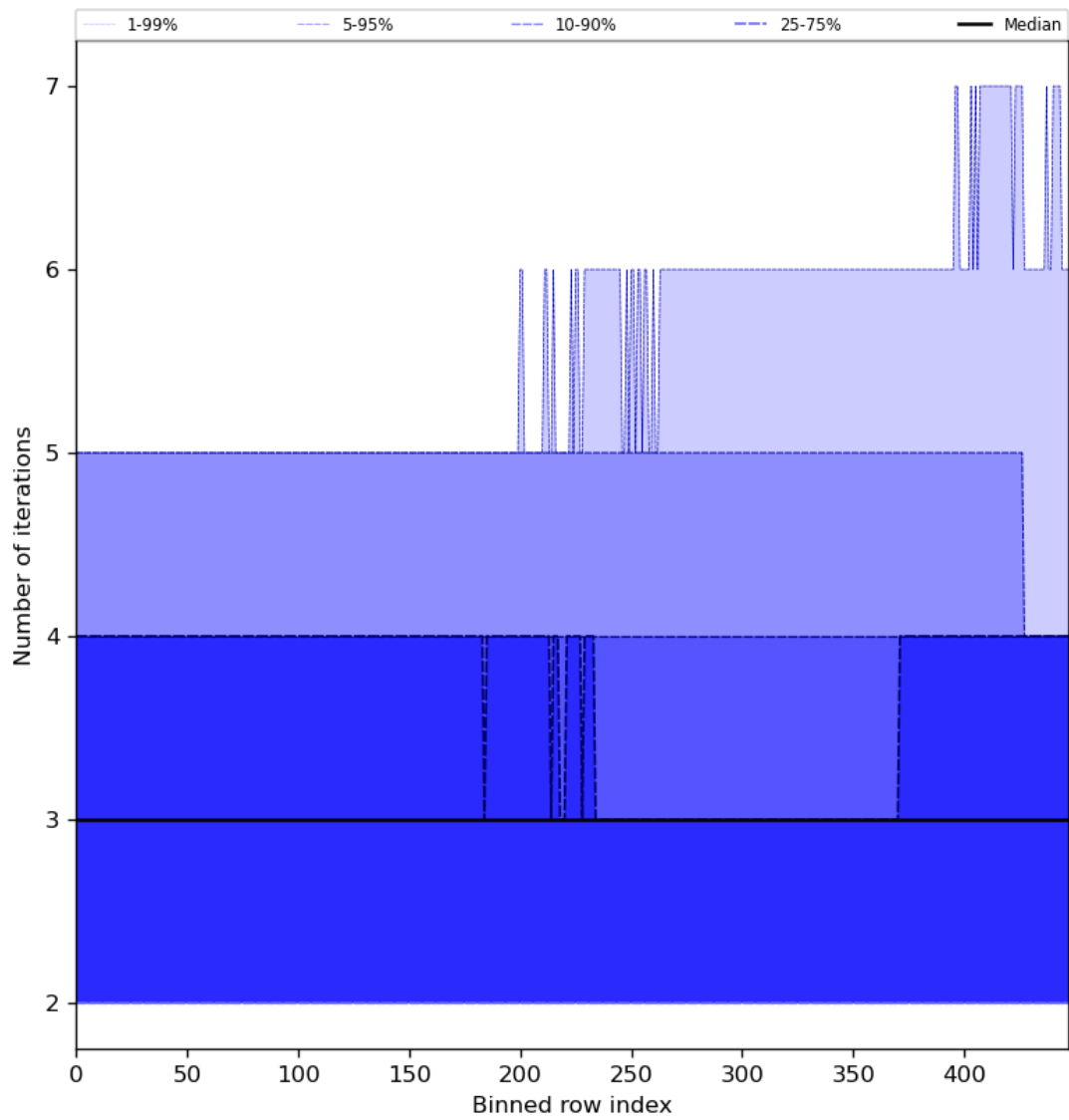
Figure 56: Along track statistics of “Number of iterations” for 2023-11-07 to 2023-11-09
