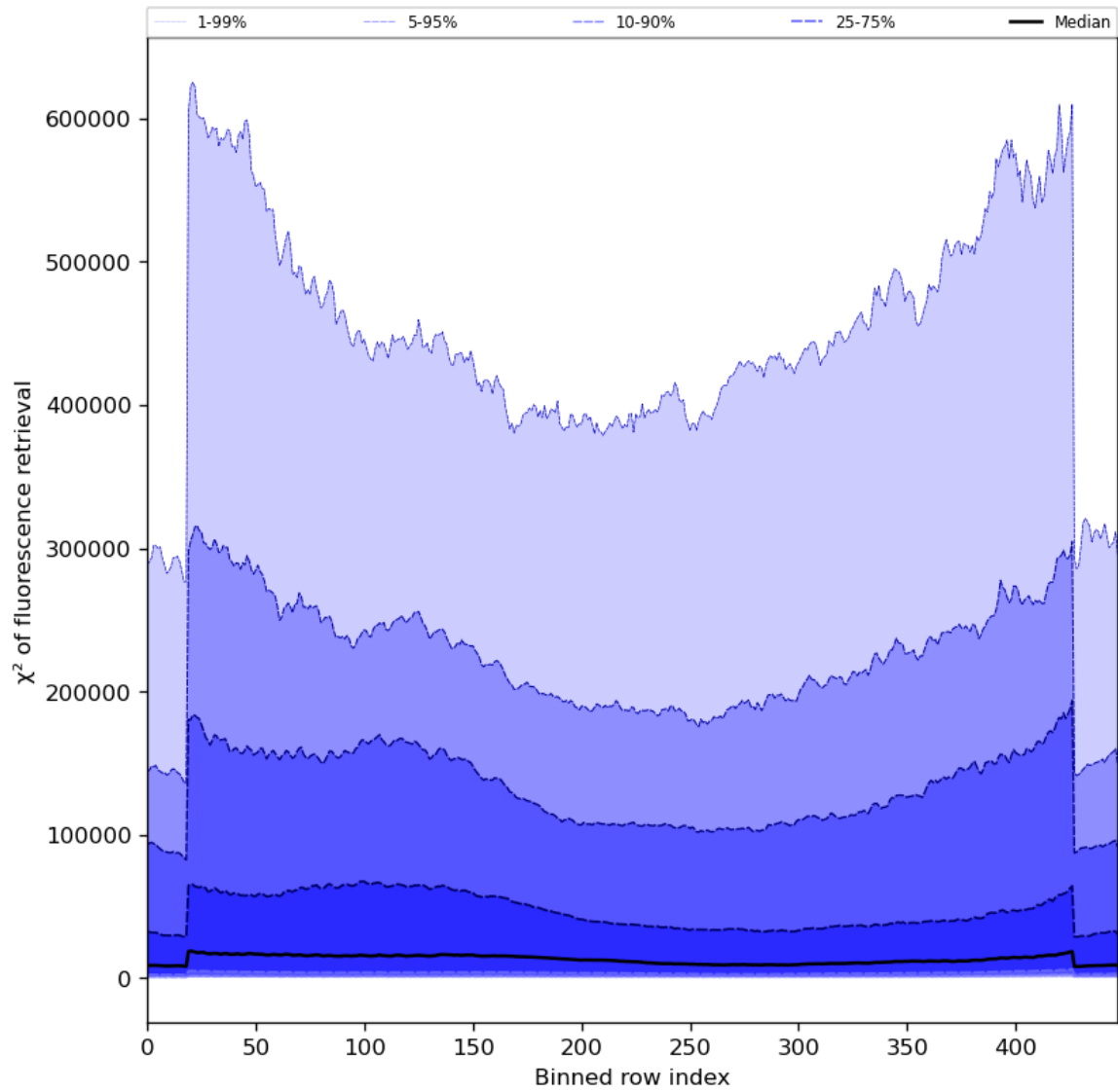
Figure 59: Along track statistics of “ \chi^2 of fluorescence retrieval” for 2023-11-07 to 2023-11-09
