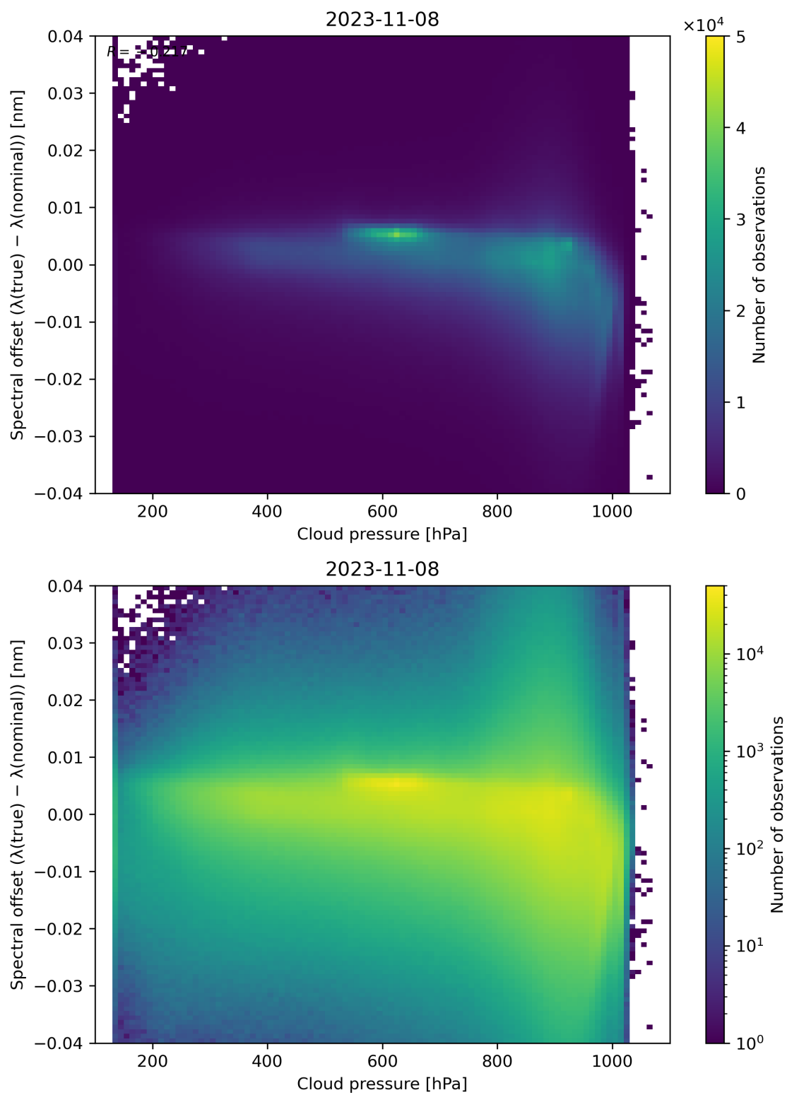
Figure 92: Scatter density plot of “Cloud pressure” against “Spectral offset ( \lambda(\text{true}) - \lambda(\text{nominal}) )” for 2023-11-07 to 2023-11-09.
