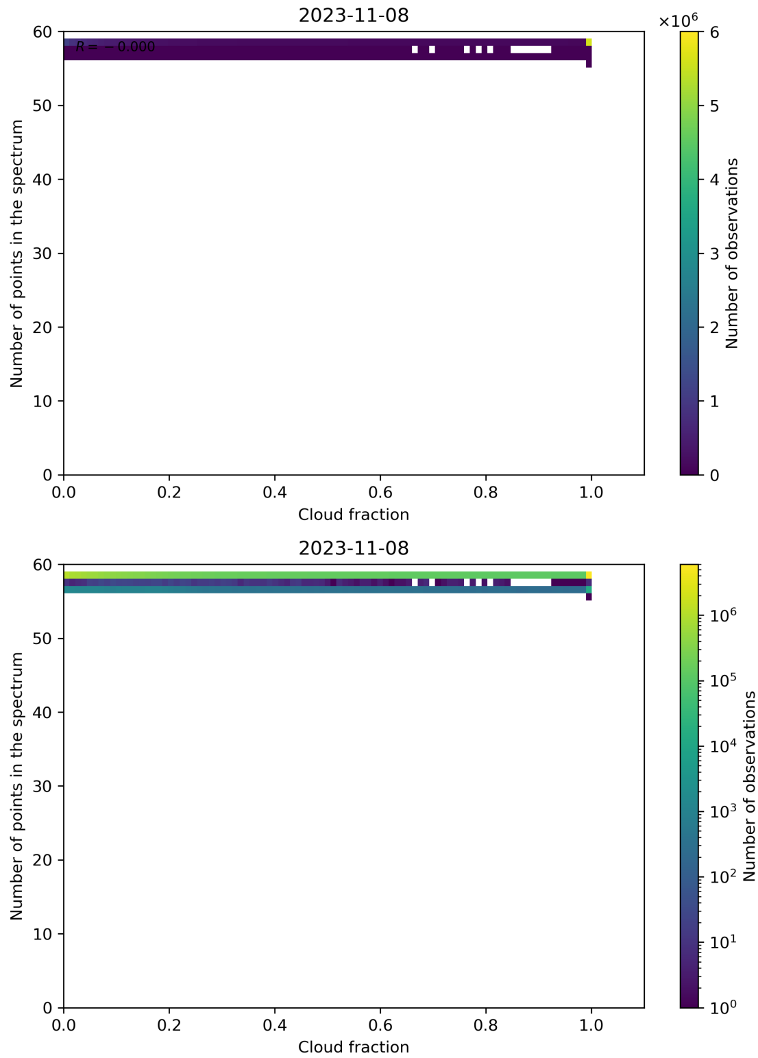
Figure 81: Scatter density plot of “Cloud fraction” against “Number of points in the spectrum” for 2023-11-07 to 2023-11-09.
