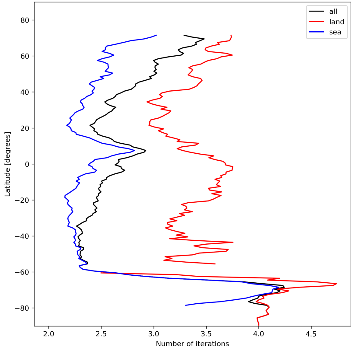
Figure 22: Zonal average of “Number of iterations” for 2023-11-07 to 2023-11-09.
