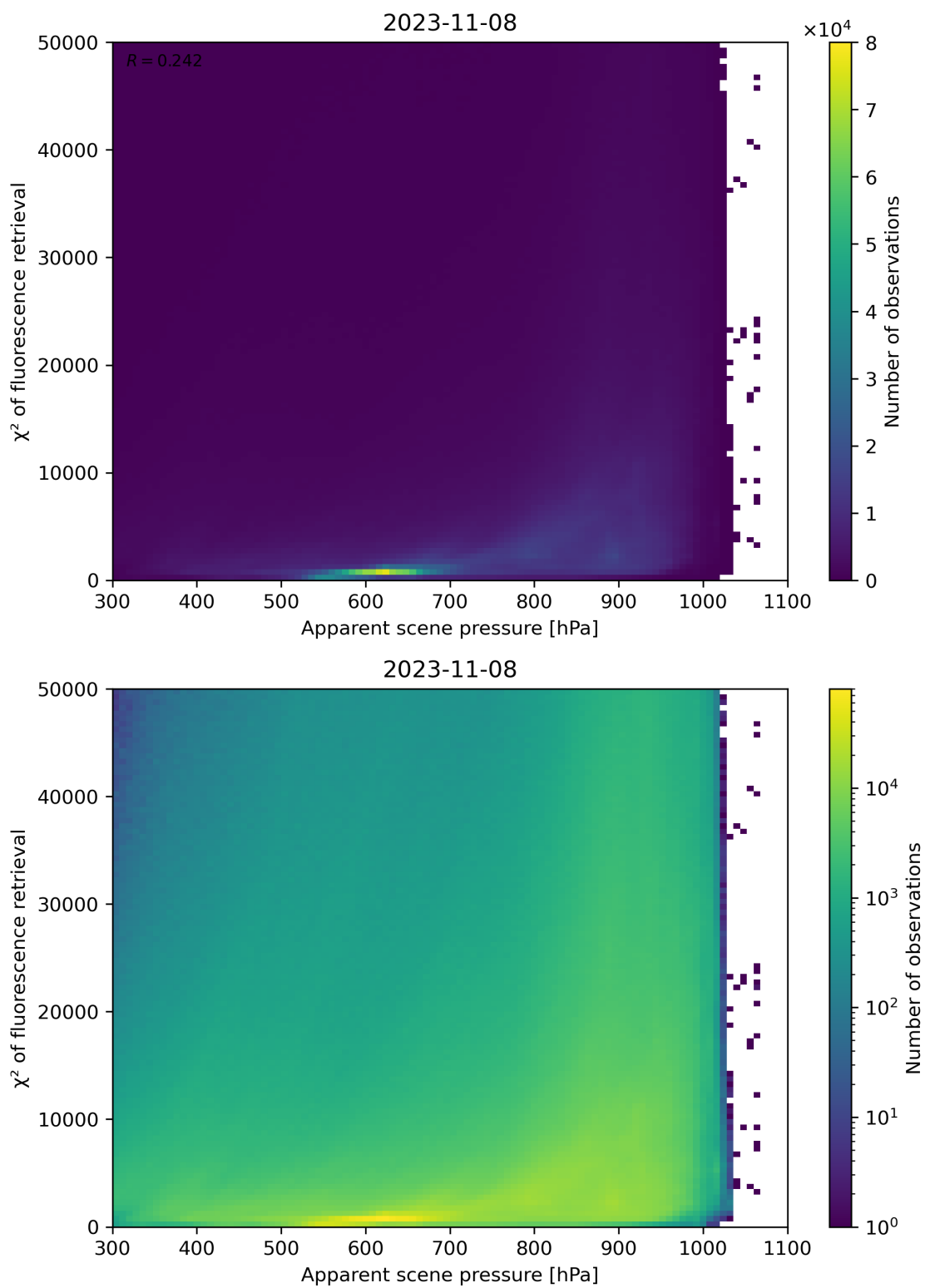
Figure 64: Scatter density plot of “Apparent scene pressure” against “ \chi^2 of fluorescence retrieval” for 2023-11-07 to 2023-11-09.
