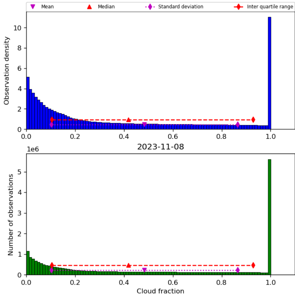
Figure 32: Histogram of “Cloud fraction” for 2023-11-07 to 2023-11-09
