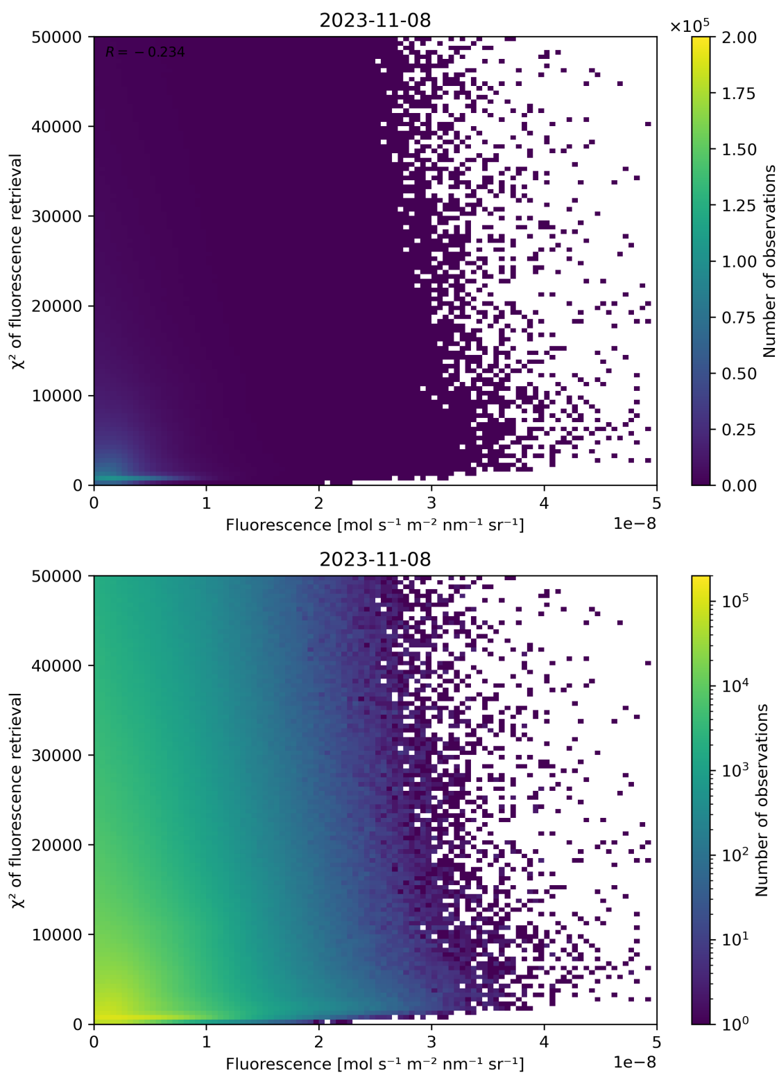
Figure 93: Scatter density plot of “Fluorescence” against “ \chi^2 of fluorescence retrieval” for 2023-11-07 to 2023-11-09.
