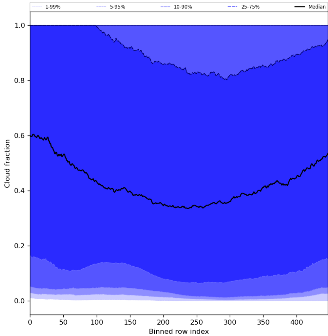
Figure 49: Along track statistics of “Cloud fraction” for 2023-11-07 to 2023-11-09
