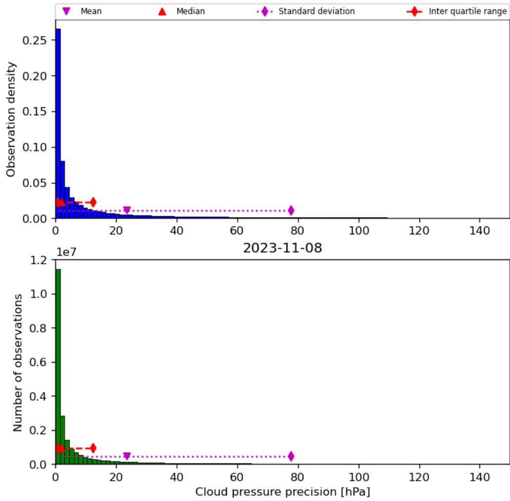
Figure 31: Histogram of “Cloud pressure precision” for 2023-11-07 to 2023-11-09
