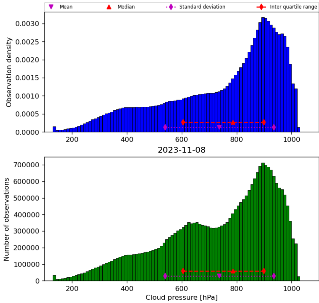
Figure 30: Histogram of “Cloud pressure” for 2023-11-07 to 2023-11-09
