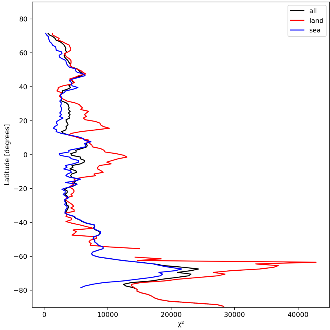
Figure 21: Zonal average of “ \chi^2 ” for 2023-11-07 to 2023-11-09.
