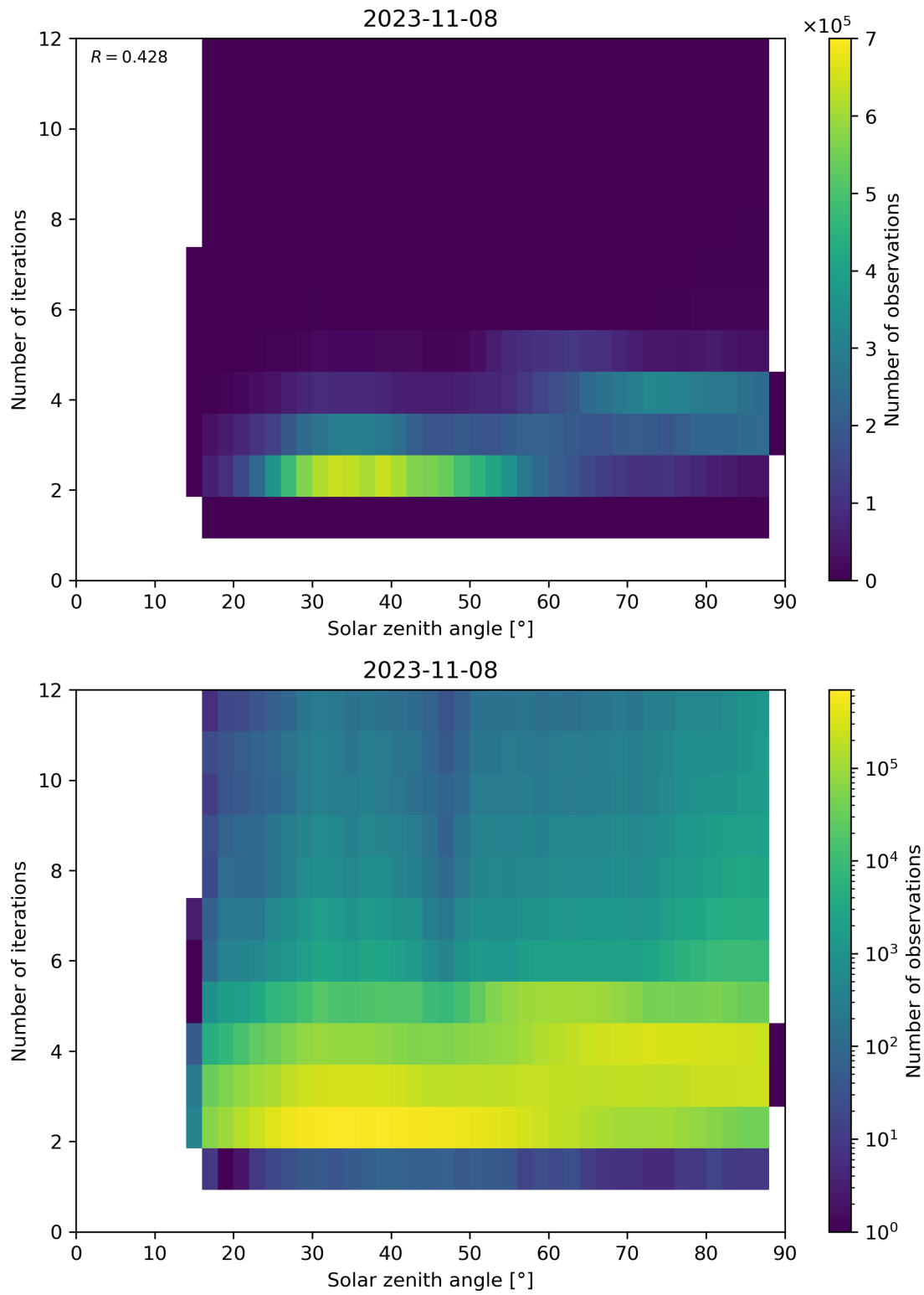
Figure 125: Scatter density plot of “Solar zenith angle” against “Number of iterations” for 2023-11-07 to 2023-11-09.
