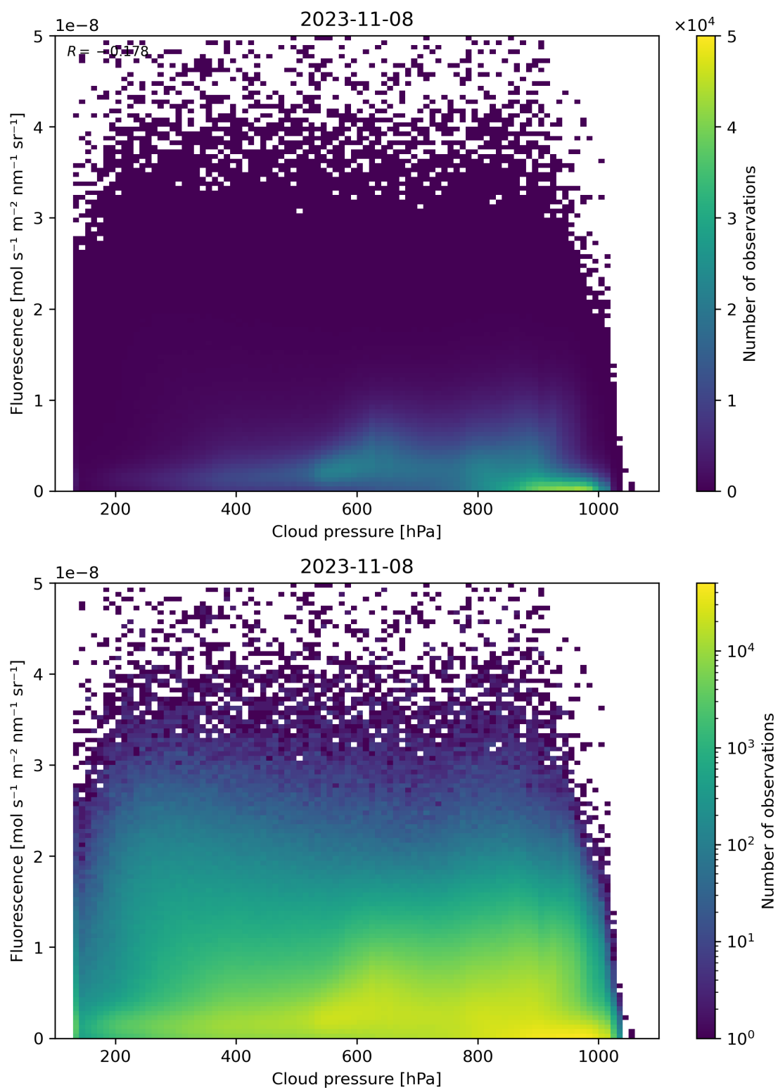
Figure 88: Scatter density plot of “Cloud pressure” against “Fluorescence” for 2023-11-07 to 2023-11-09.
