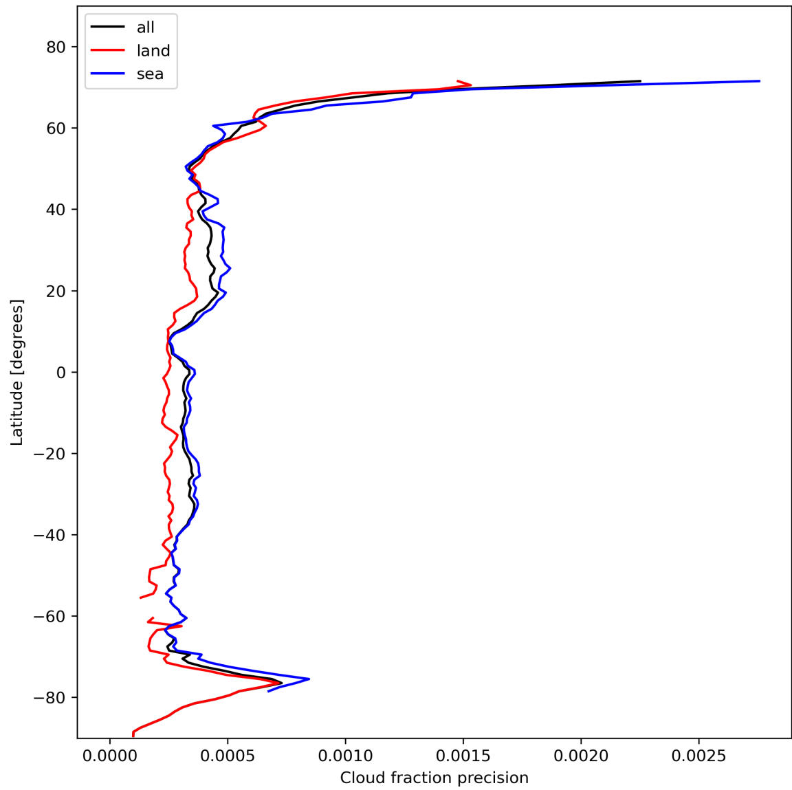
Figure 16: Zonal average of “Cloud fraction precision” for 2023-11-07 to 2023-11-09.
