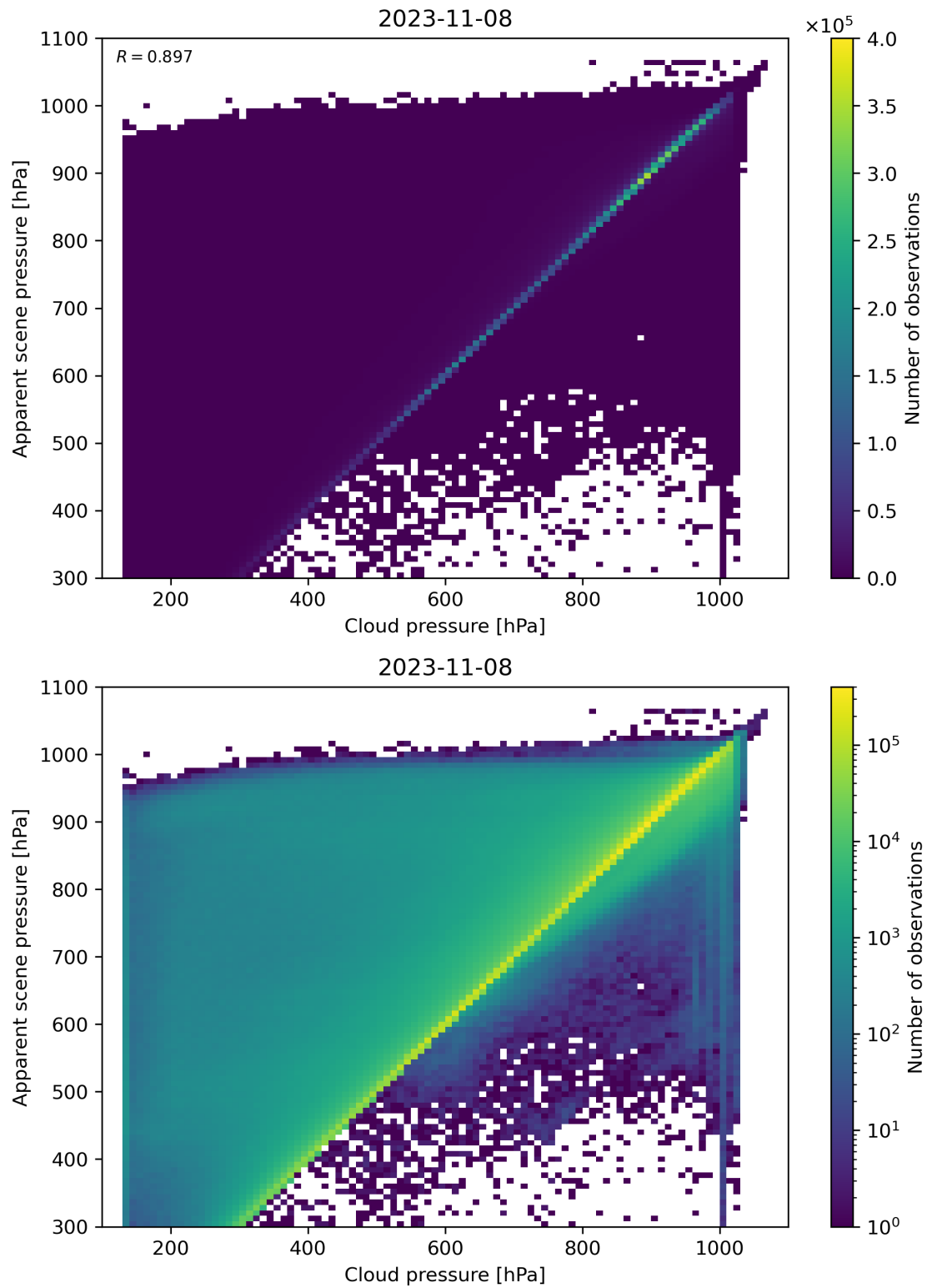
Figure 84: Scatter density plot of “Cloud pressure” against “Apparent scene pressure” for 2023-11-07 to 2023-11-09.
