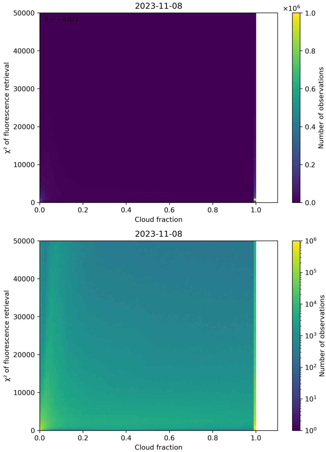
Figure 78: Scatter density plot of “Cloud fraction” against “ \chi^2 of fluorescence retrieval” for 2023-11-07 to 2023-11-09.
