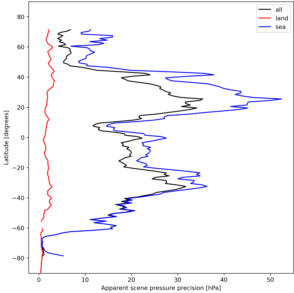
Figure 20: Zonal average of “Apparent scene pressure precision” for 2023-11-07 to 2023-11-09.
