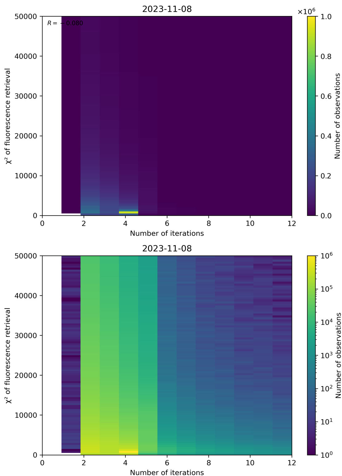
Figure 106: Scatter density plot of “Number of iterations” against “ \chi^2 of fluorescence retrieval” for 2023-11-07 to 2023-11-09.
