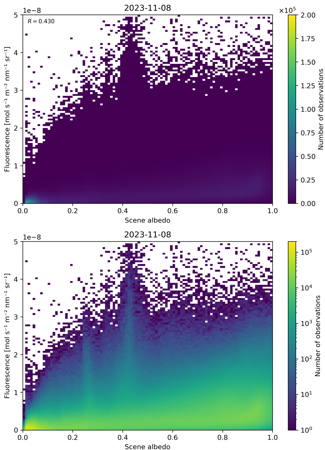
Figure 114: Scatter density plot of “Scene albedo” against “Fluorescence” for 2023-11-07 to 2023-11-09.
