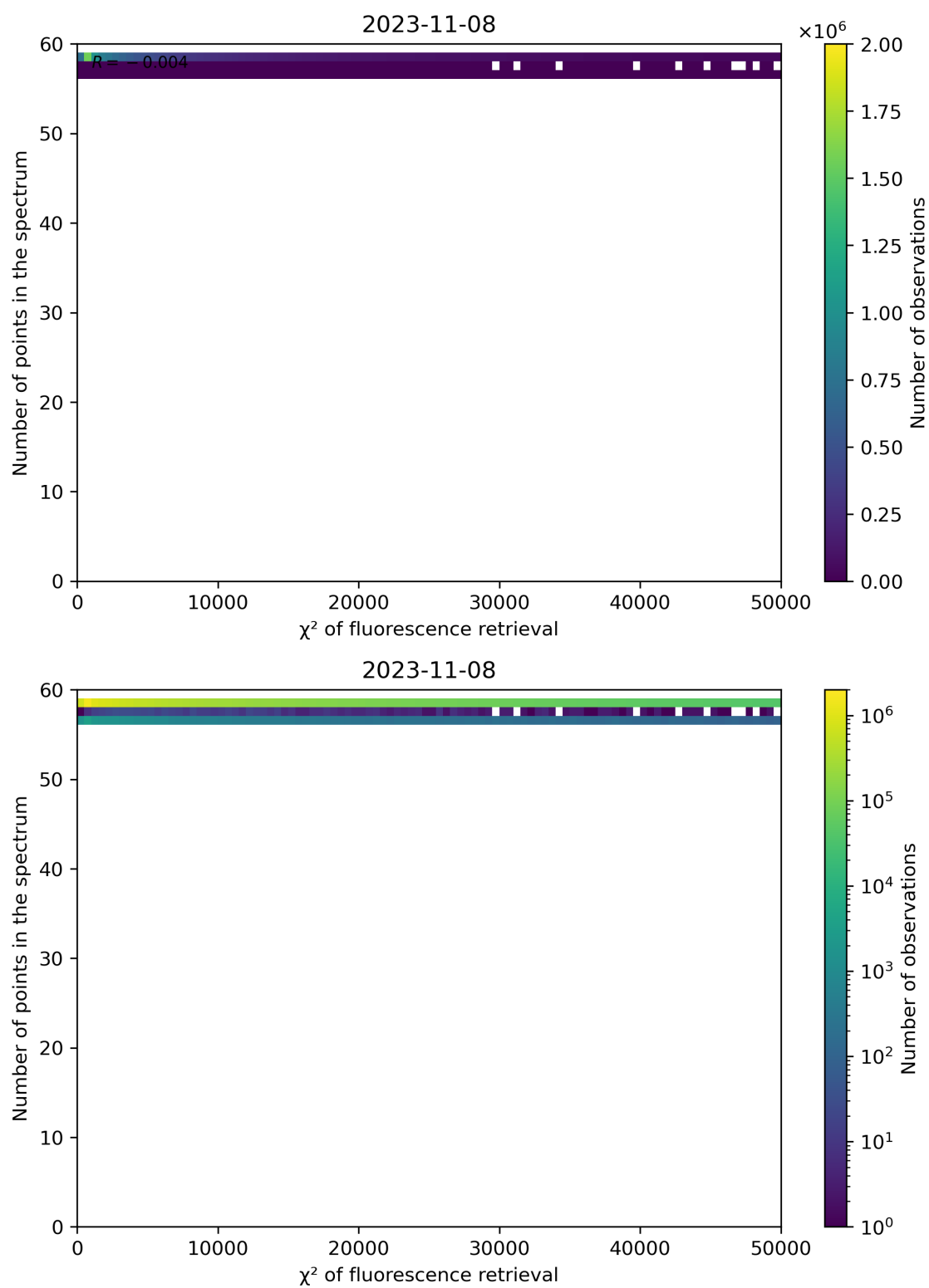
Figure 71: Scatter density plot of " \chi^2 of fluorescence retrieval" against "Number of points in the spectrum" for 2023-11-07 to 2023-11-09.
