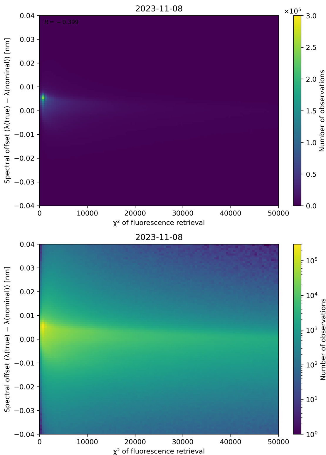
Figure 72: Scatter density plot of " \chi^2 of fluorescence retrieval" against "Spectral offset ( \lambda(\text{true}) - \lambda(\text{nominal}) )" for 2023-11-07 to 2023-11-09.
