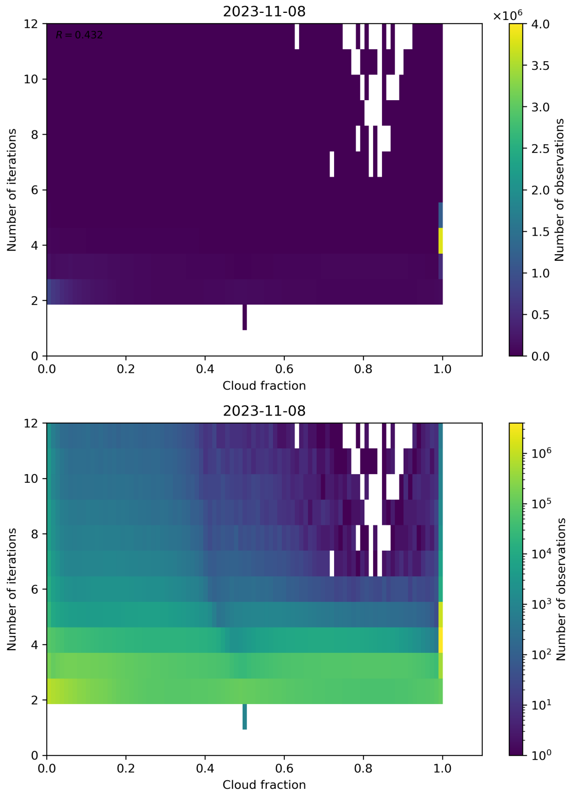
Figure 80: Scatter density plot of “Cloud fraction” against “Number of iterations” for 2023-11-07 to 2023-11-09.
