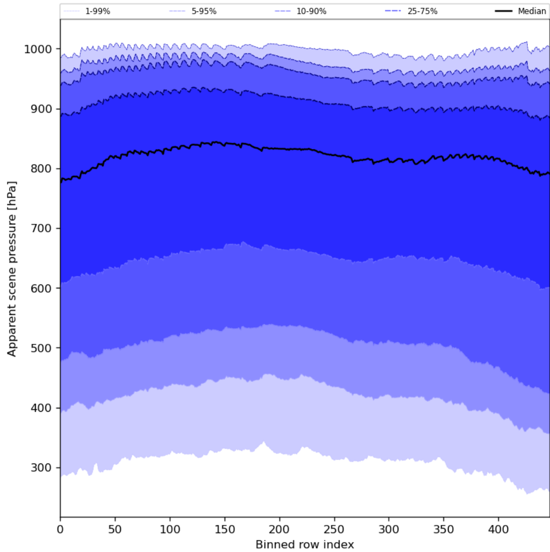
Figure 53: Along track statistics of “Apparent scene pressure” for 2023-11-07 to 2023-11-09
