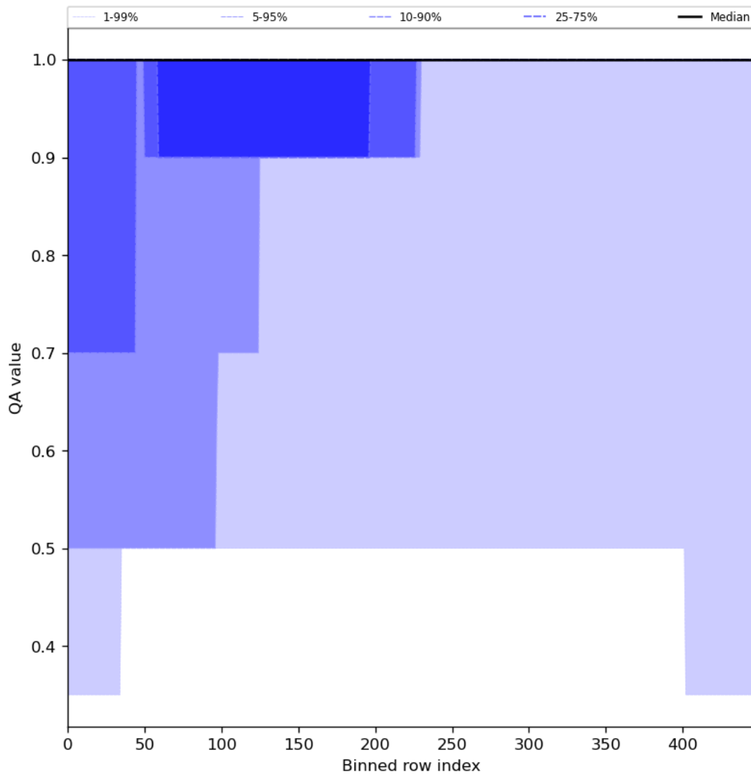
Figure 46: Along track statistics of “QA value” for 2023-11-07 to 2023-11-09
