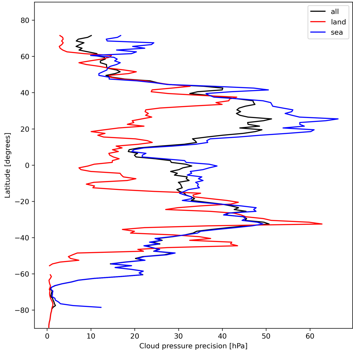
Figure 14: Zonal average of “Cloud pressure precision” for 2023-11-07 to 2023-11-09.
