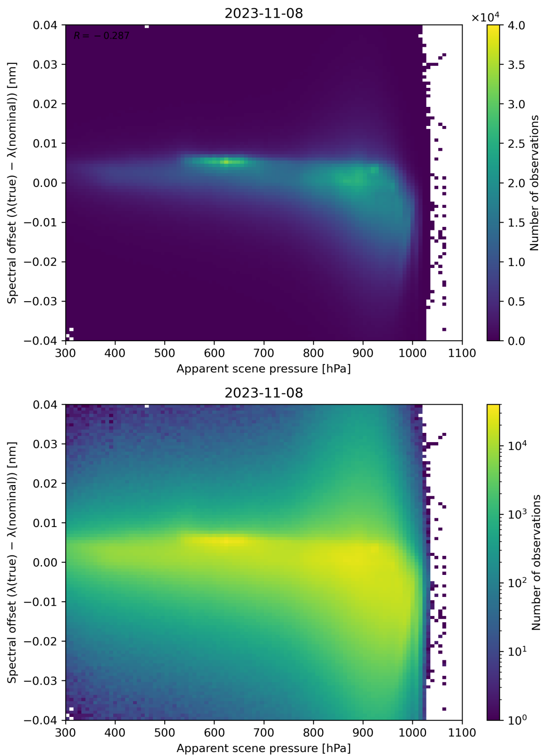
Figure 68: Scatter density plot of “Apparent scene pressure” against “Spectral offset ( \lambda(\text{true}) - \lambda(\text{nominal}) )” for 2023-11-07 to 2023-11-09.
