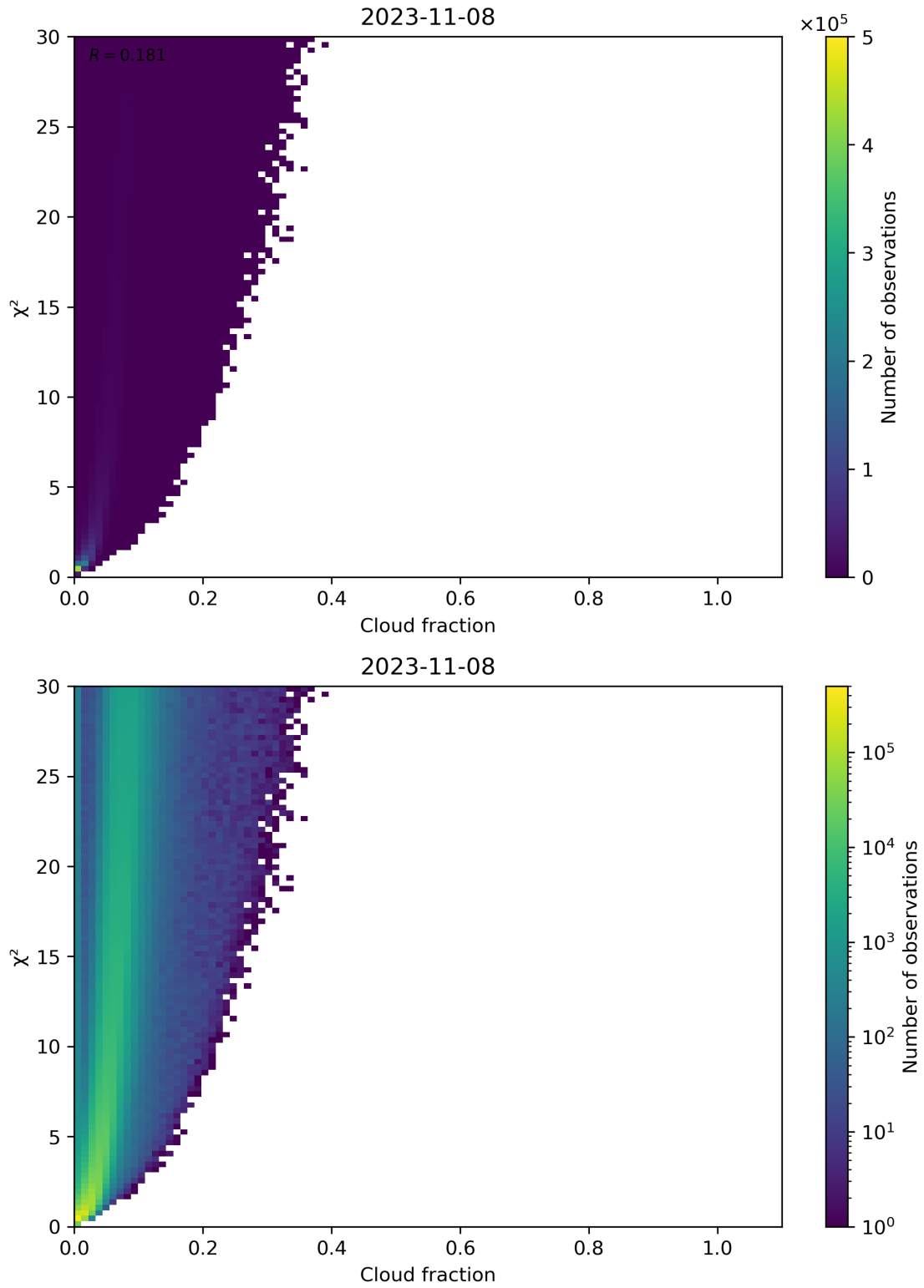
Figure 77: Scatter density plot of “Cloud fraction” against “ \chi^2 ” for 2023-11-07 to 2023-11-09.
