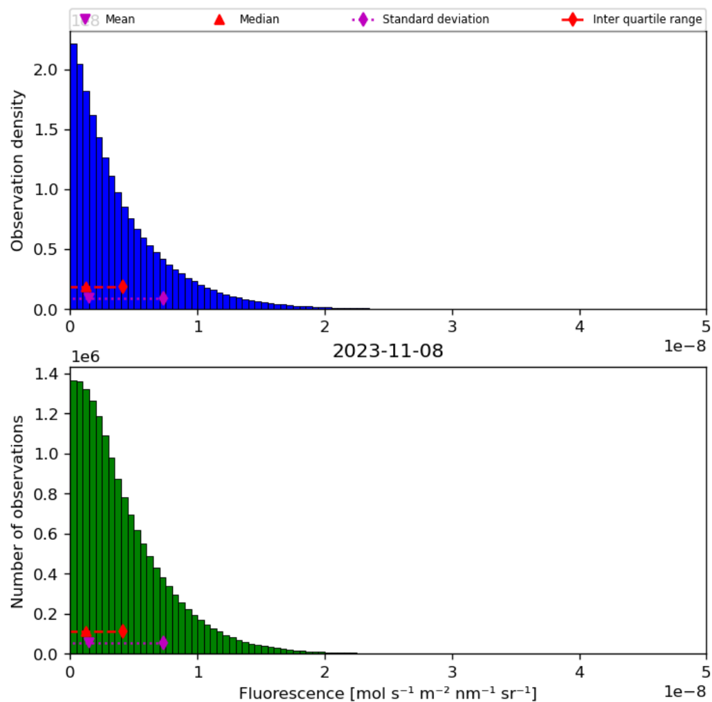
Figure 40: Histogram of “Fluorescence” for 2023-11-07 to 2023-11-09
