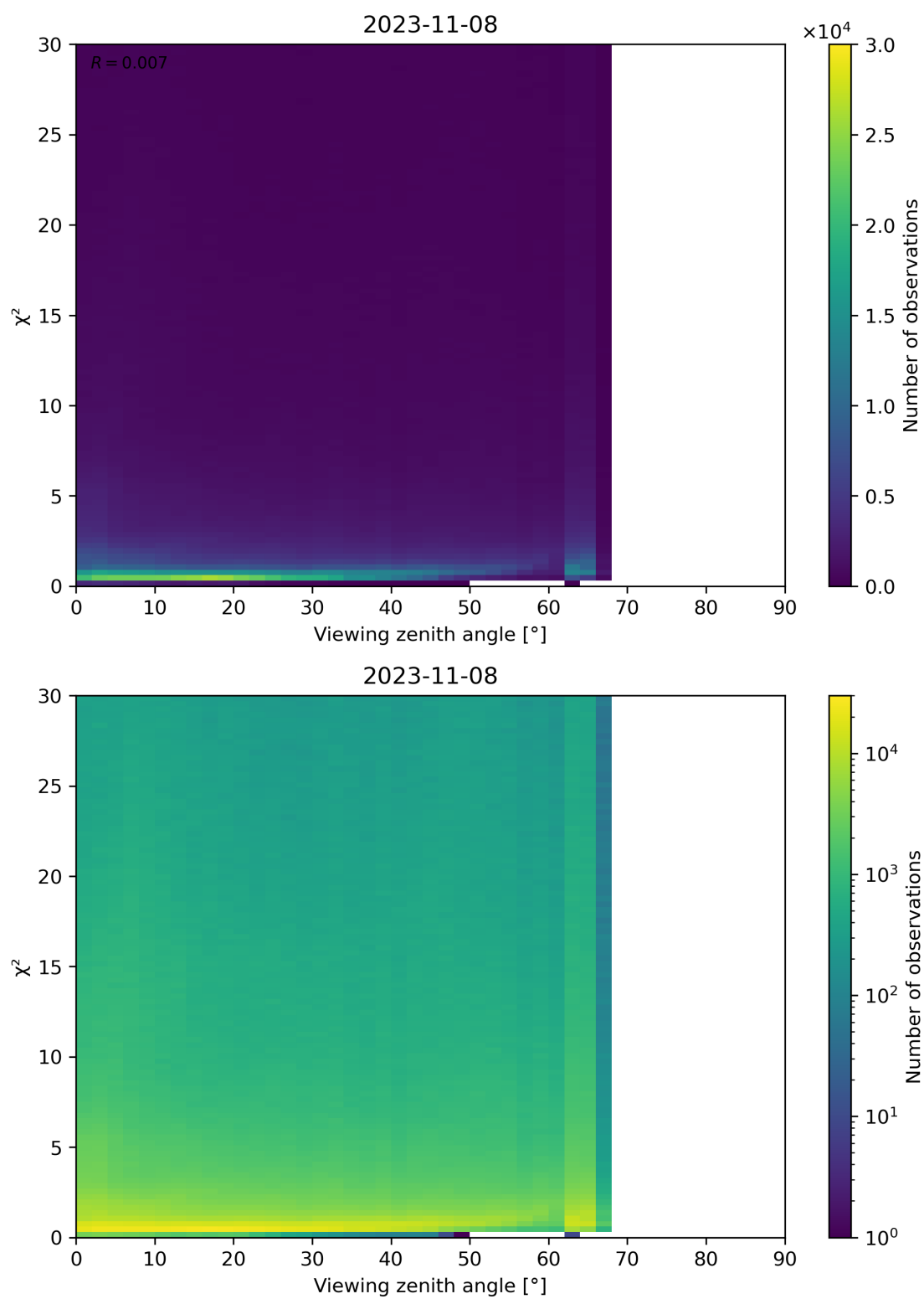
Figure 130: Scatter density plot of “Viewing zenith angle” against “ \chi^2 ” for 2023-11-07 to 2023-11-09.
