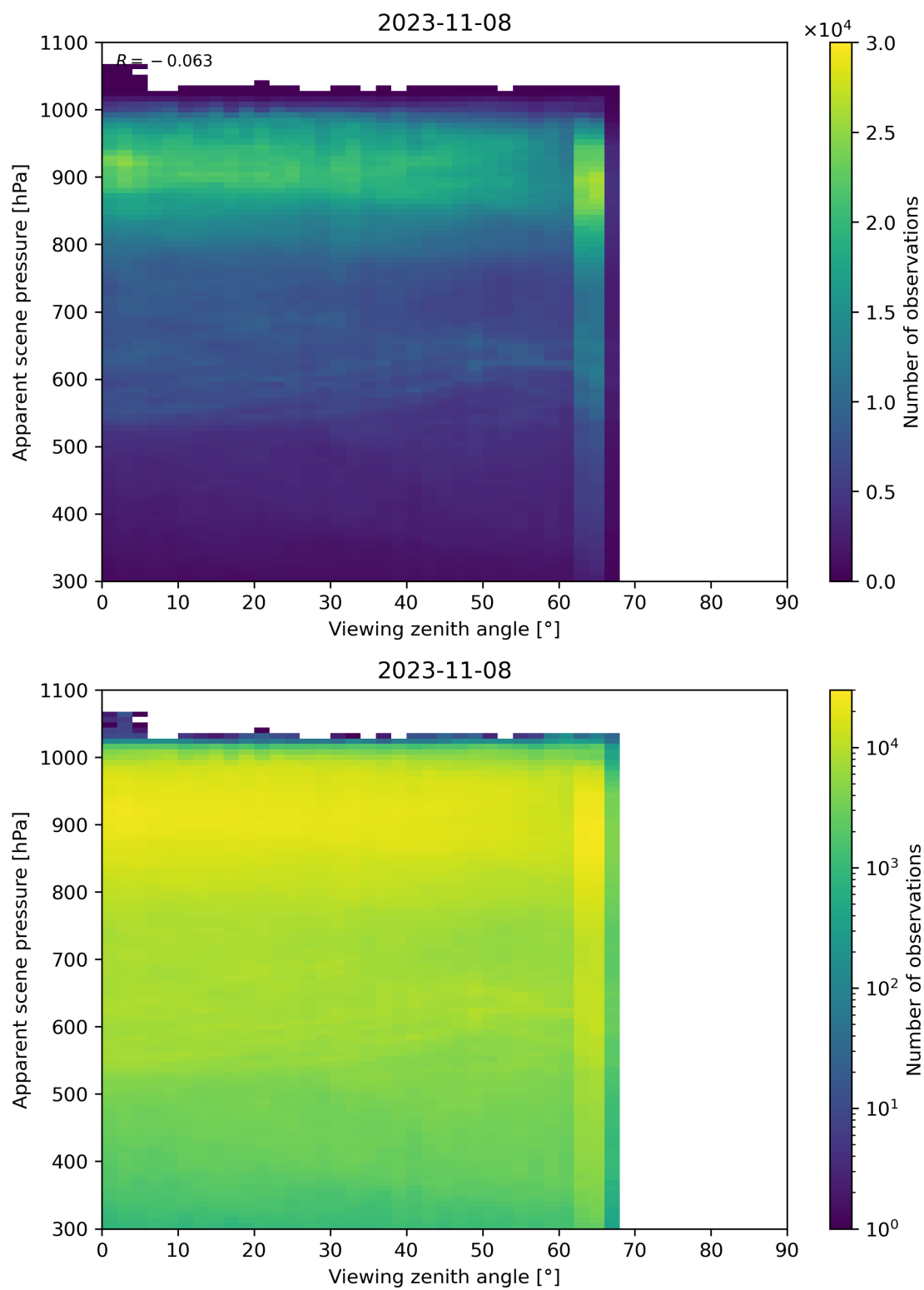
Figure 129: Scatter density plot of “Viewing zenith angle” against “Apparent scene pressure” for 2023-11-07 to 2023-11-09.
