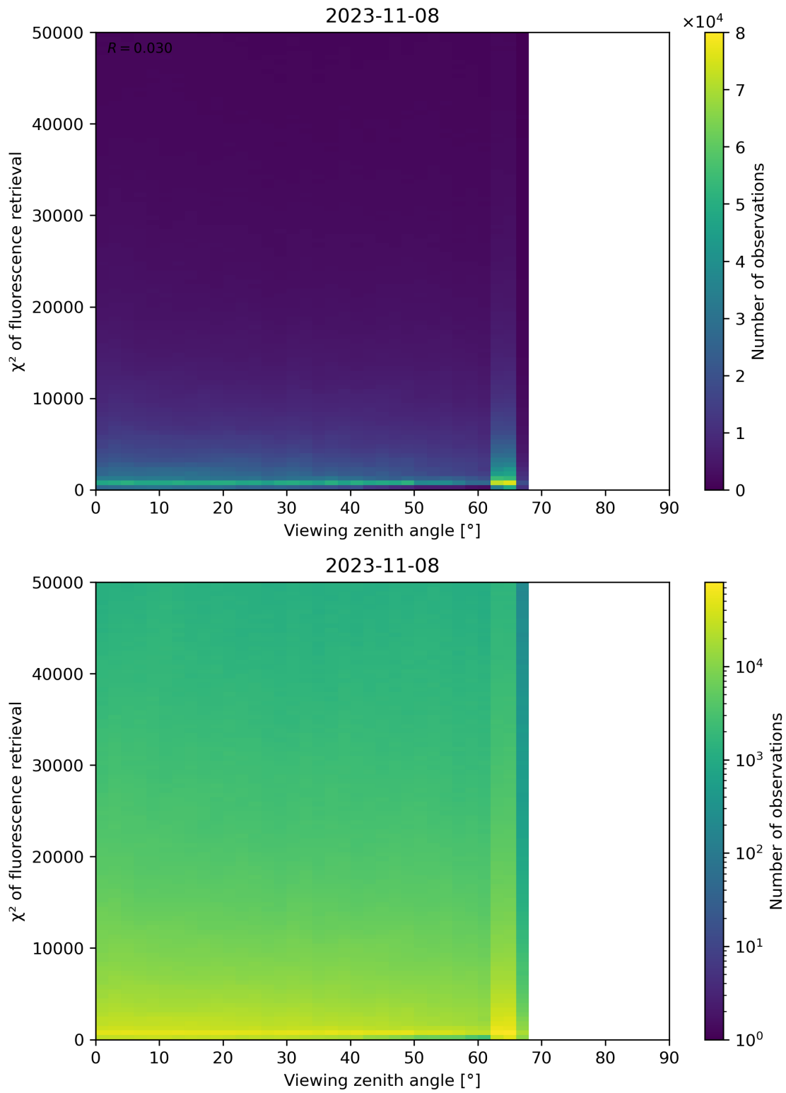
Figure 131: Scatter density plot of “Viewing zenith angle” against “ \chi^2 of fluorescence retrieval” for 2023-11-07 to 2023-11-09.
