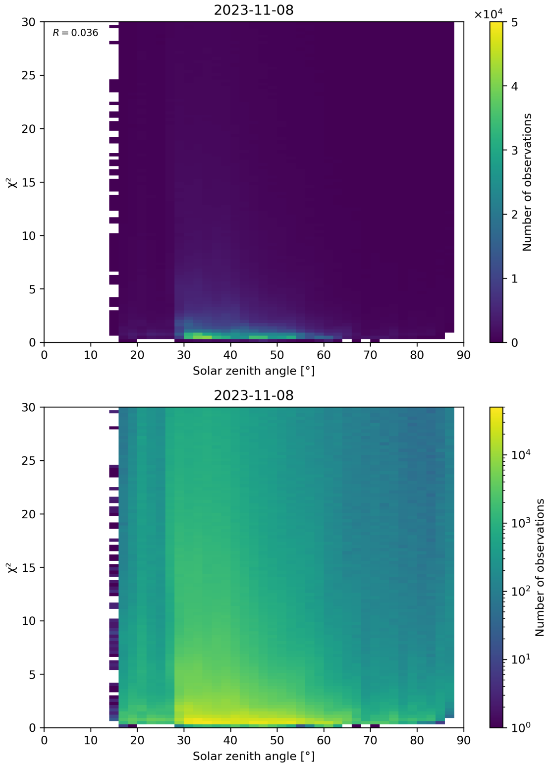
Figure 119: Scatter density plot of “Solar zenith angle” against “ \chi^2 ” for 2023-11-07 to 2023-11-09.
