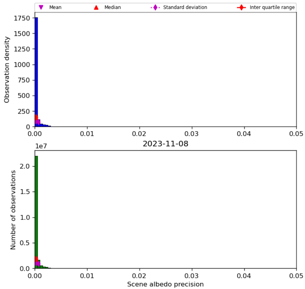
Figure 35: Histogram of “Scene albedo precision” for 2023-11-07 to 2023-11-09
