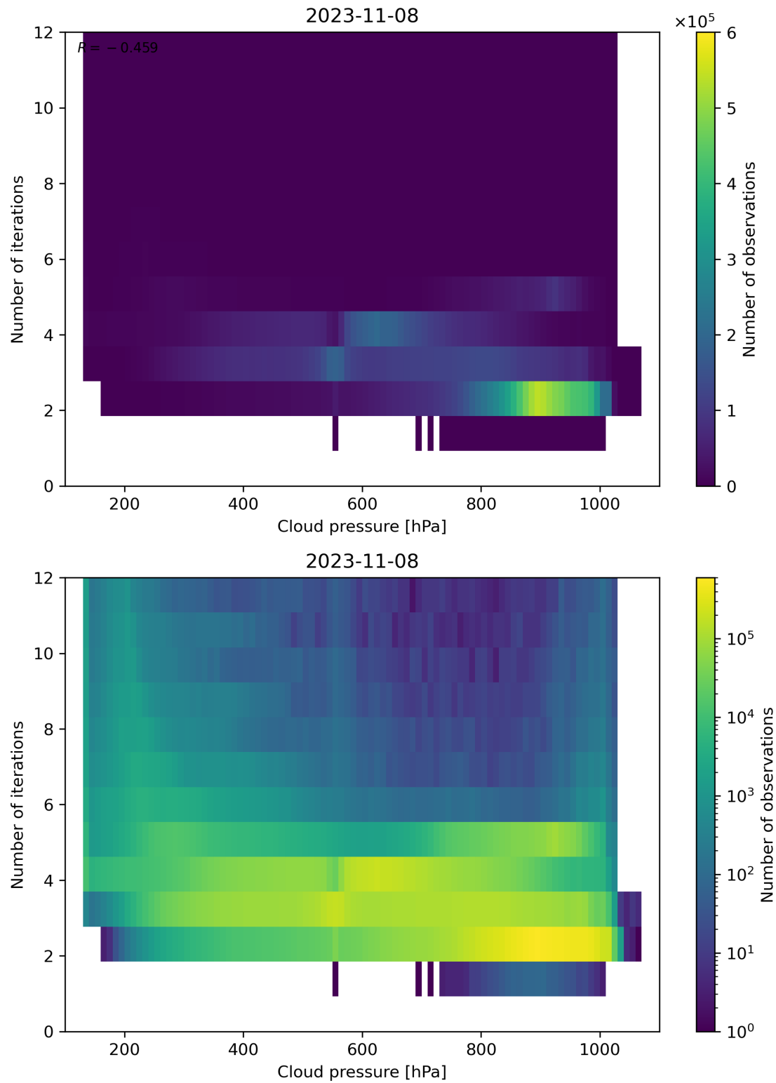
Figure 89: Scatter density plot of “Cloud pressure” against “Number of iterations” for 2023-11-07 to 2023-11-09.
