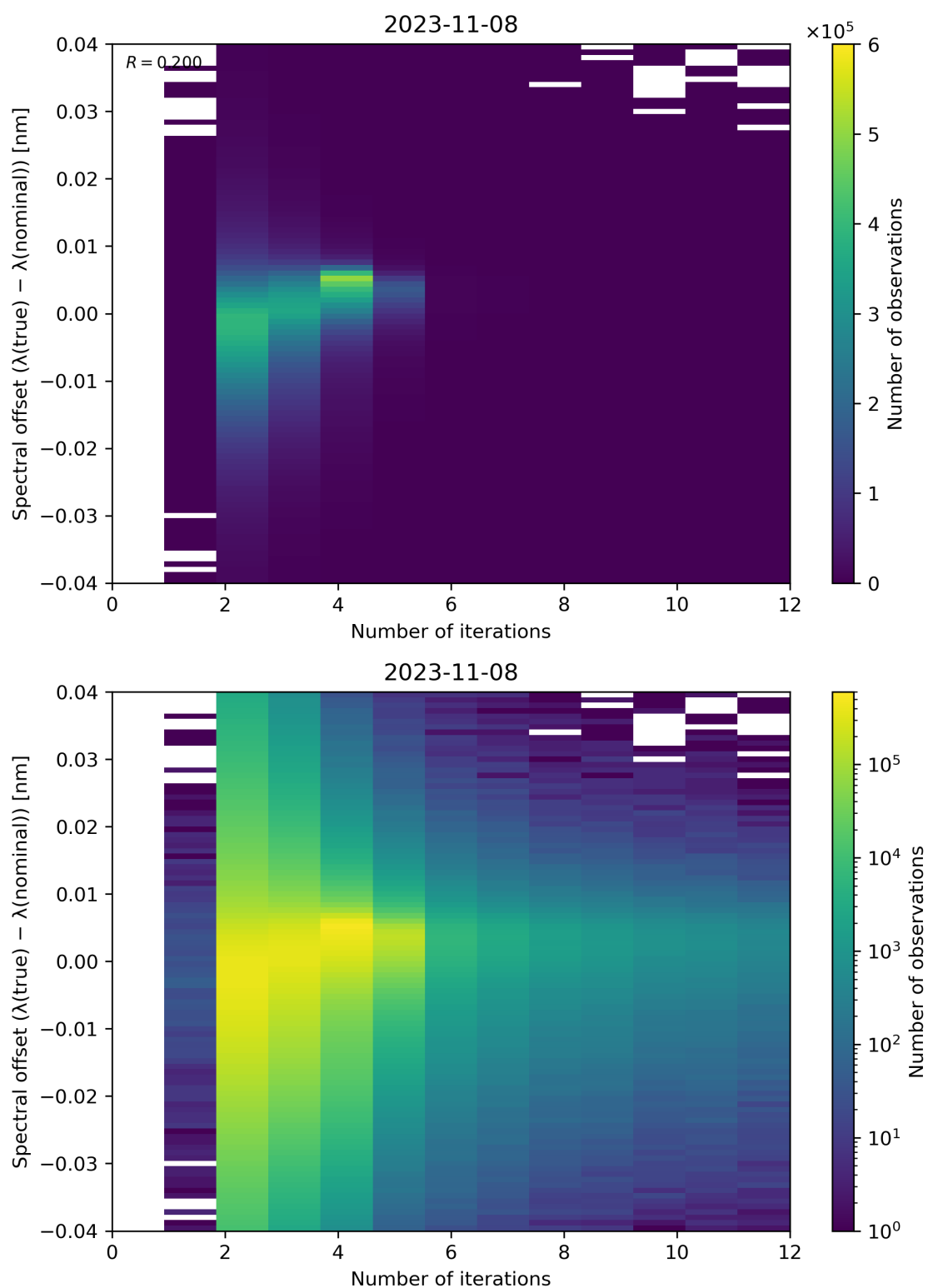
Figure 109: Scatter density plot of “Number of iterations” against “Spectral offset ( \lambda(\text{true}) - \lambda(\text{nominal}) )” for 2023-11-07 to 2023-11-09.
