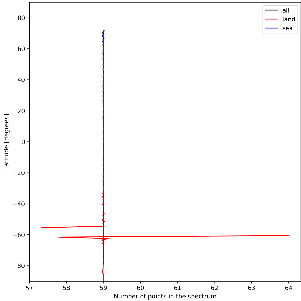
Figure 27: Zonal average of “Number of points in the spectrum” for 2023-11-07 to 2023-11-09.
