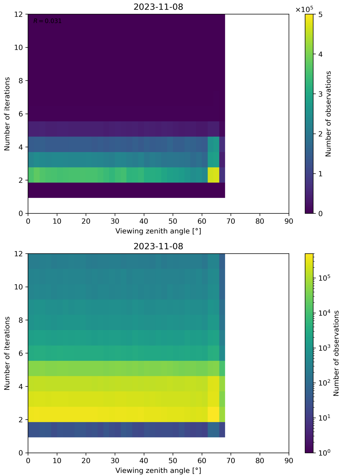
Figure 136: Scatter density plot of “Viewing zenith angle” against “Number of iterations” for 2023-11-07 to 2023-11-09.
