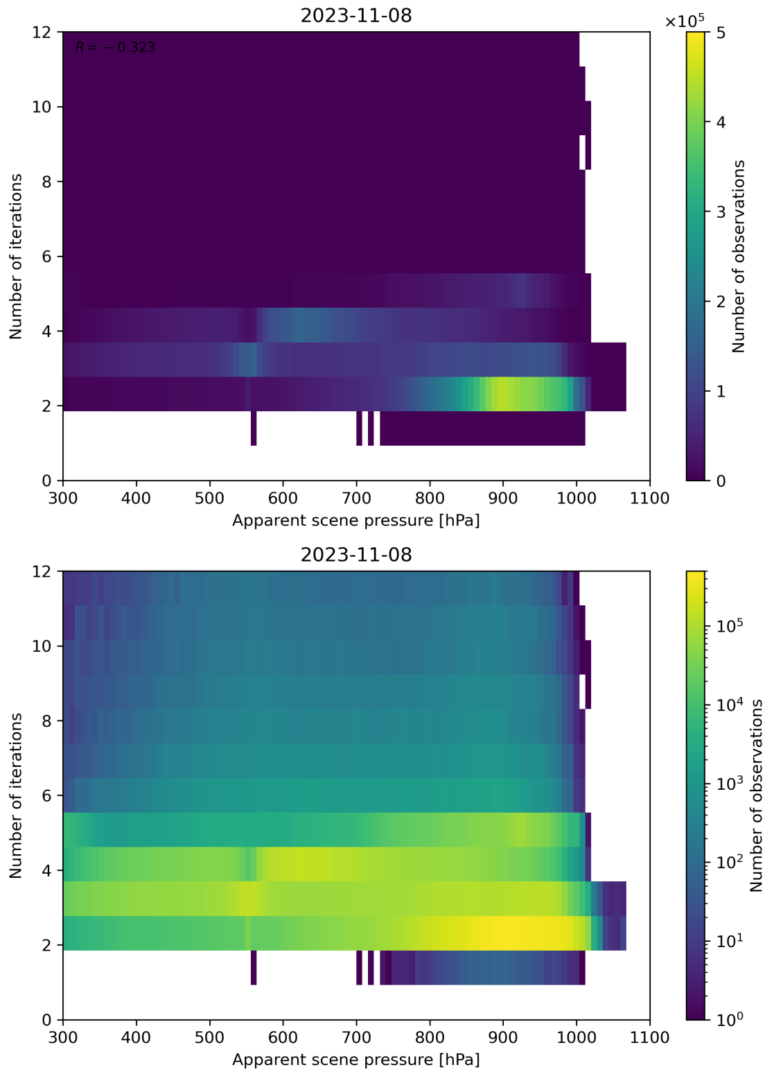
Figure 66: Scatter density plot of “Apparent scene pressure” against “Number of iterations” for 2023-11-07 to 2023-11-09.
