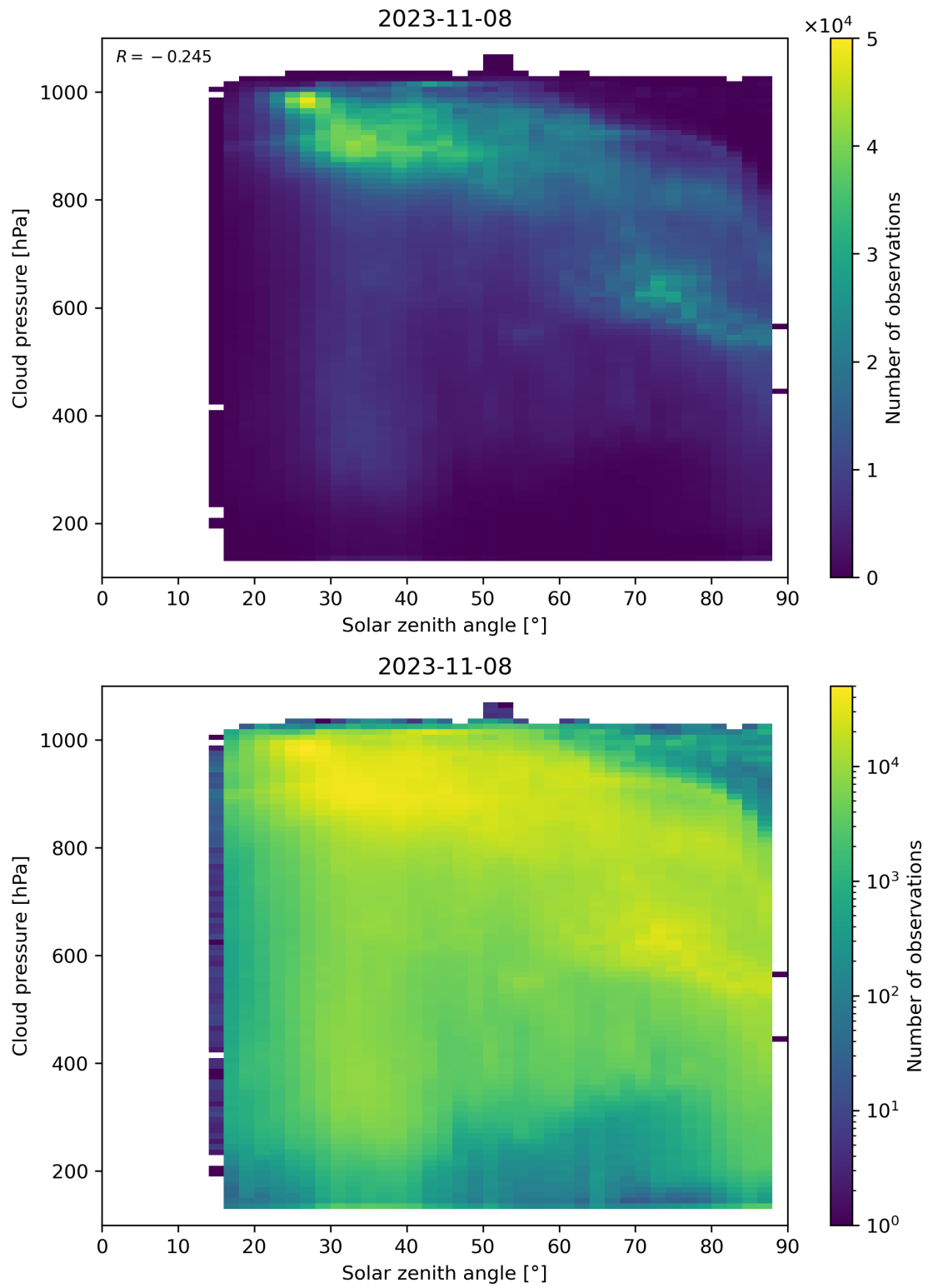
Figure 122: Scatter density plot of “Solar zenith angle” against “Cloud pressure” for 2023-11-07 to 2023-11-09.
