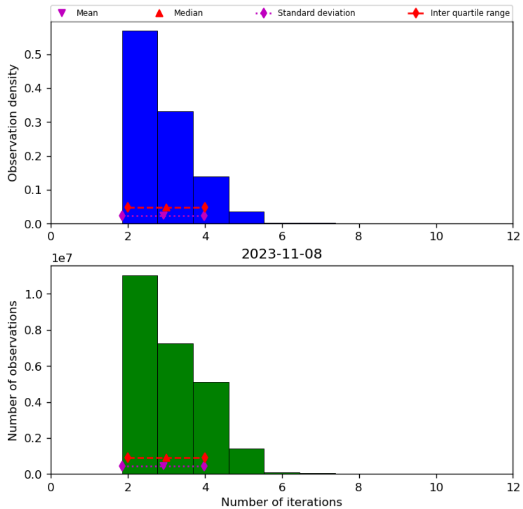
Figure 39: Histogram of “Number of iterations” for 2023-11-07 to 2023-11-09
