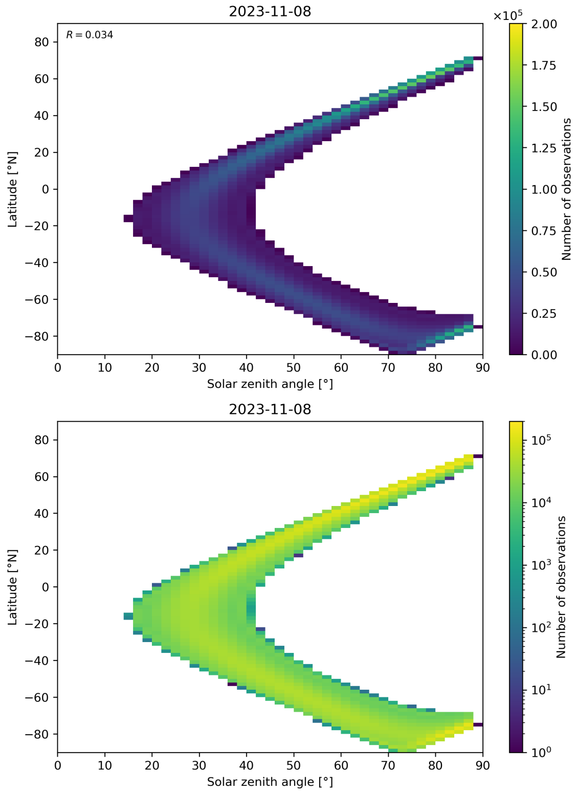
Figure 124: Scatter density plot of “Solar zenith angle” against “Latitude” for 2023-11-07 to 2023-11-09.
