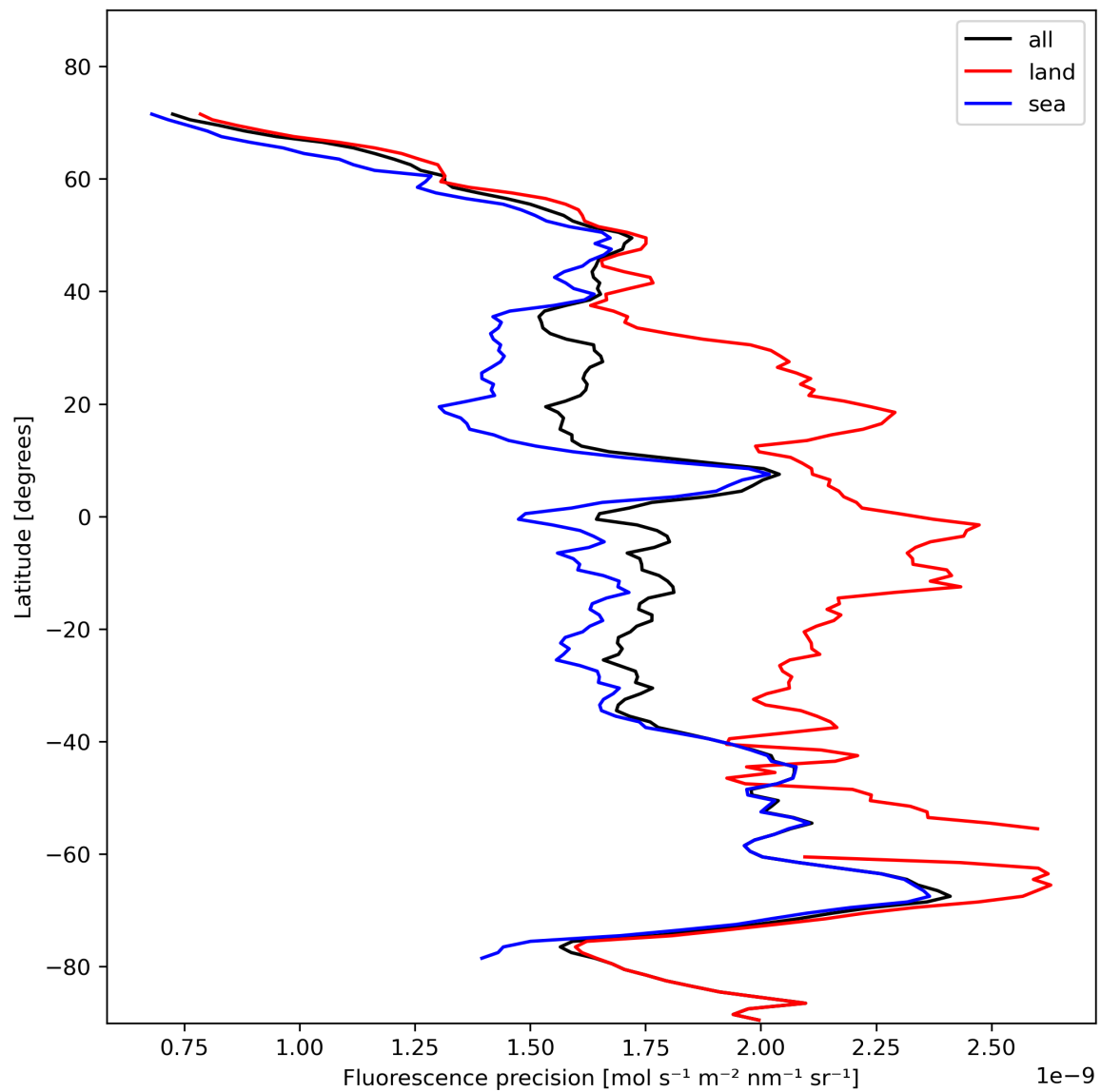
Figure 24: Zonal average of “Fluorescence precision” for 2023-11-07 to 2023-11-09.
