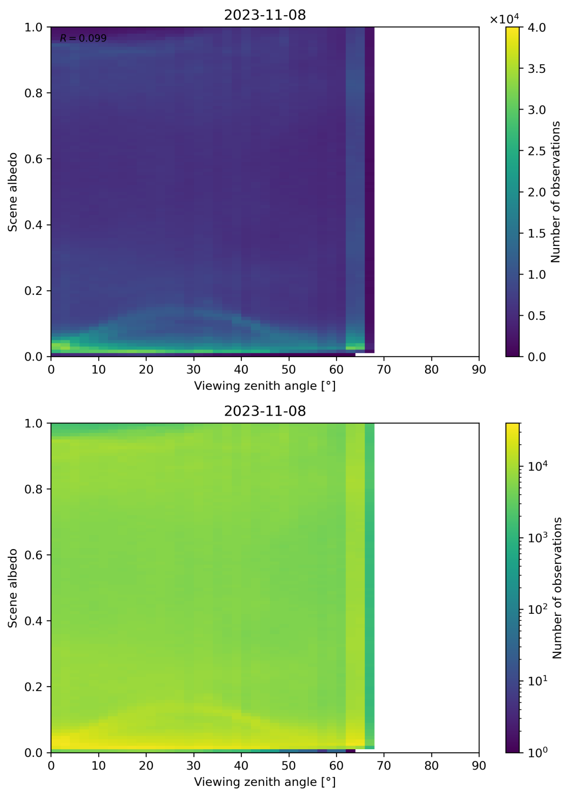
Figure 138: Scatter density plot of “Viewing zenith angle” against “Scene albedo” for 2023-11-07 to 2023-11-09.
