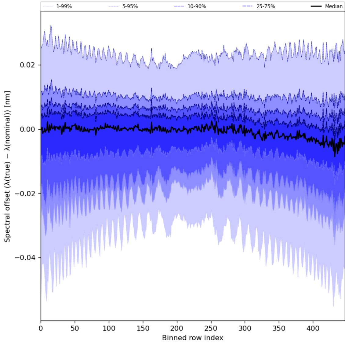
Figure 62: Along track statistics of “Spectral offset ( \lambda(\text{true}) - \lambda(\text{nominal}) )” for 2023-11-07 to 2023-11-09
