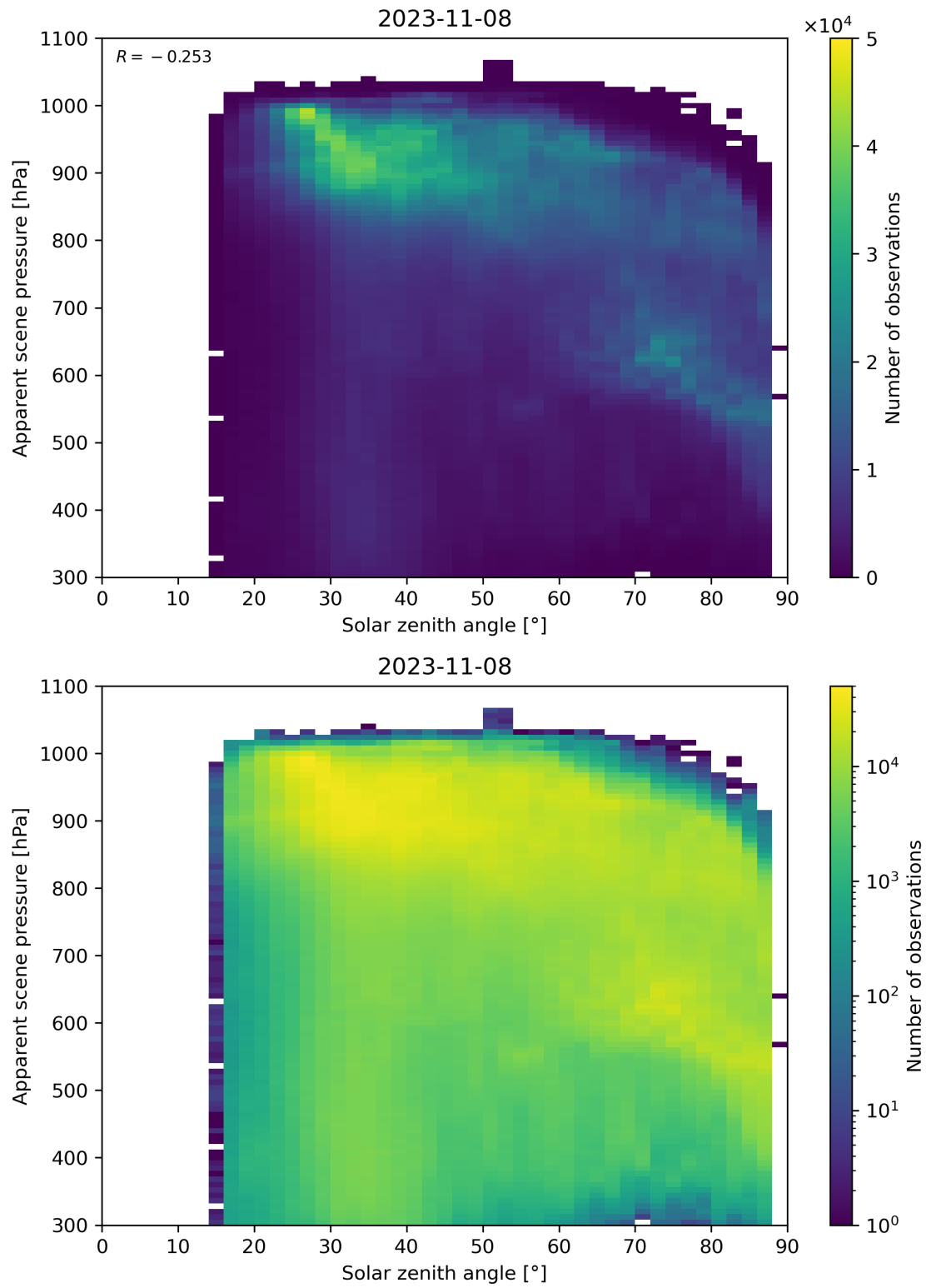
Figure 118: Scatter density plot of “Solar zenith angle” against “Apparent scene pressure” for 2023-11-07 to 2023-11-09.
