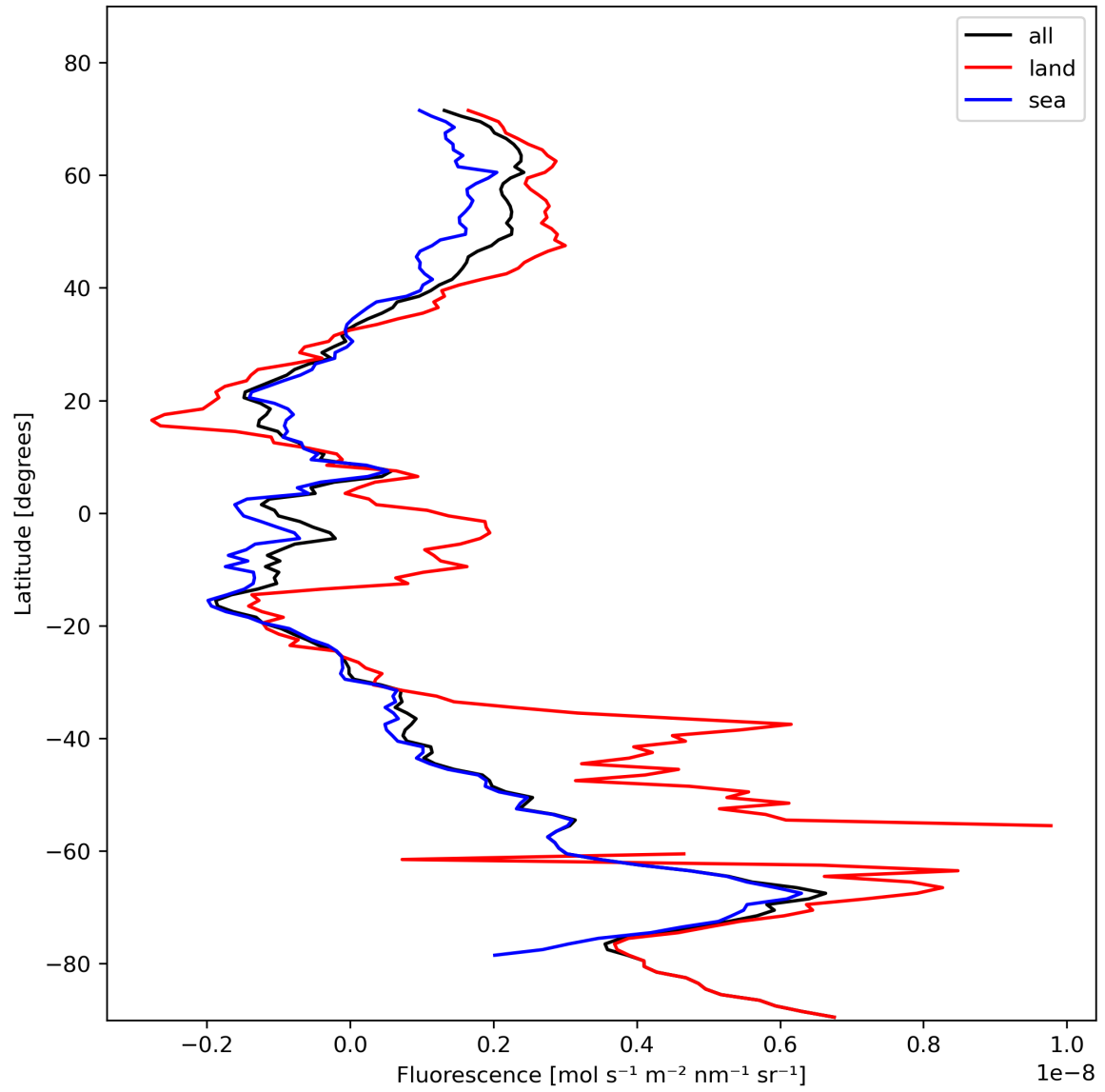
Figure 23: Zonal average of “Fluorescence” for 2023-11-07 to 2023-11-09.
