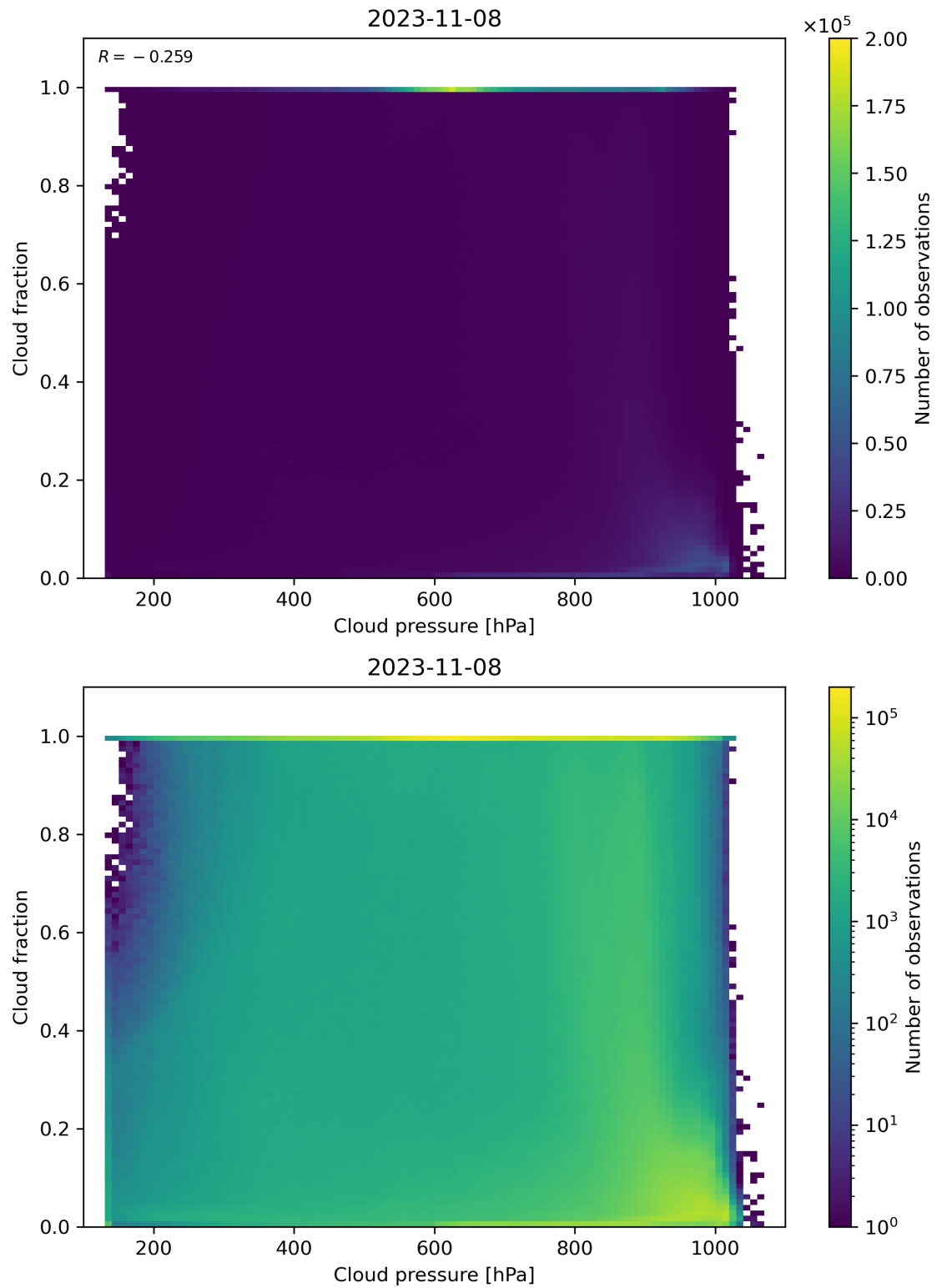
Figure 87: Scatter density plot of “Cloud pressure” against “Cloud fraction” for 2023-11-07 to 2023-11-09.
