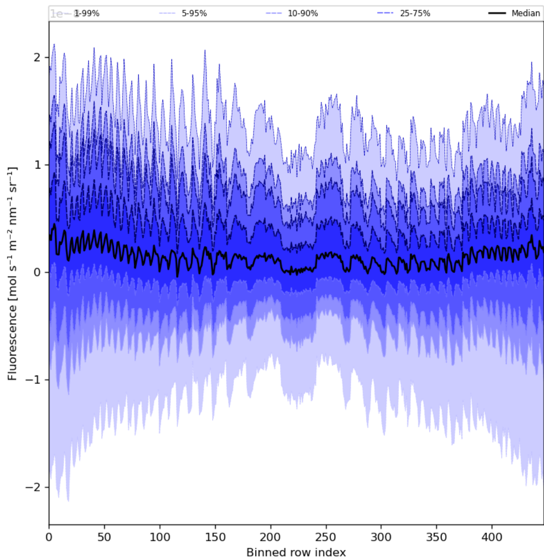
Figure 57: Along track statistics of “Fluorescence” for 2023-11-07 to 2023-11-09
