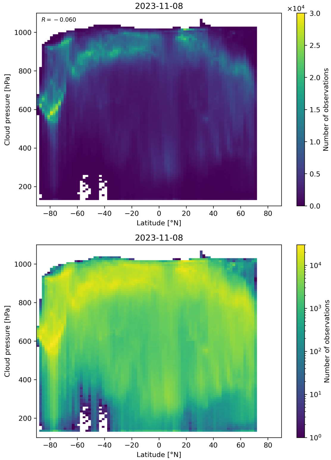
Figure 100: Scatter density plot of “Latitude” against “Cloud pressure” for 2023-11-07 to 2023-11-09.
