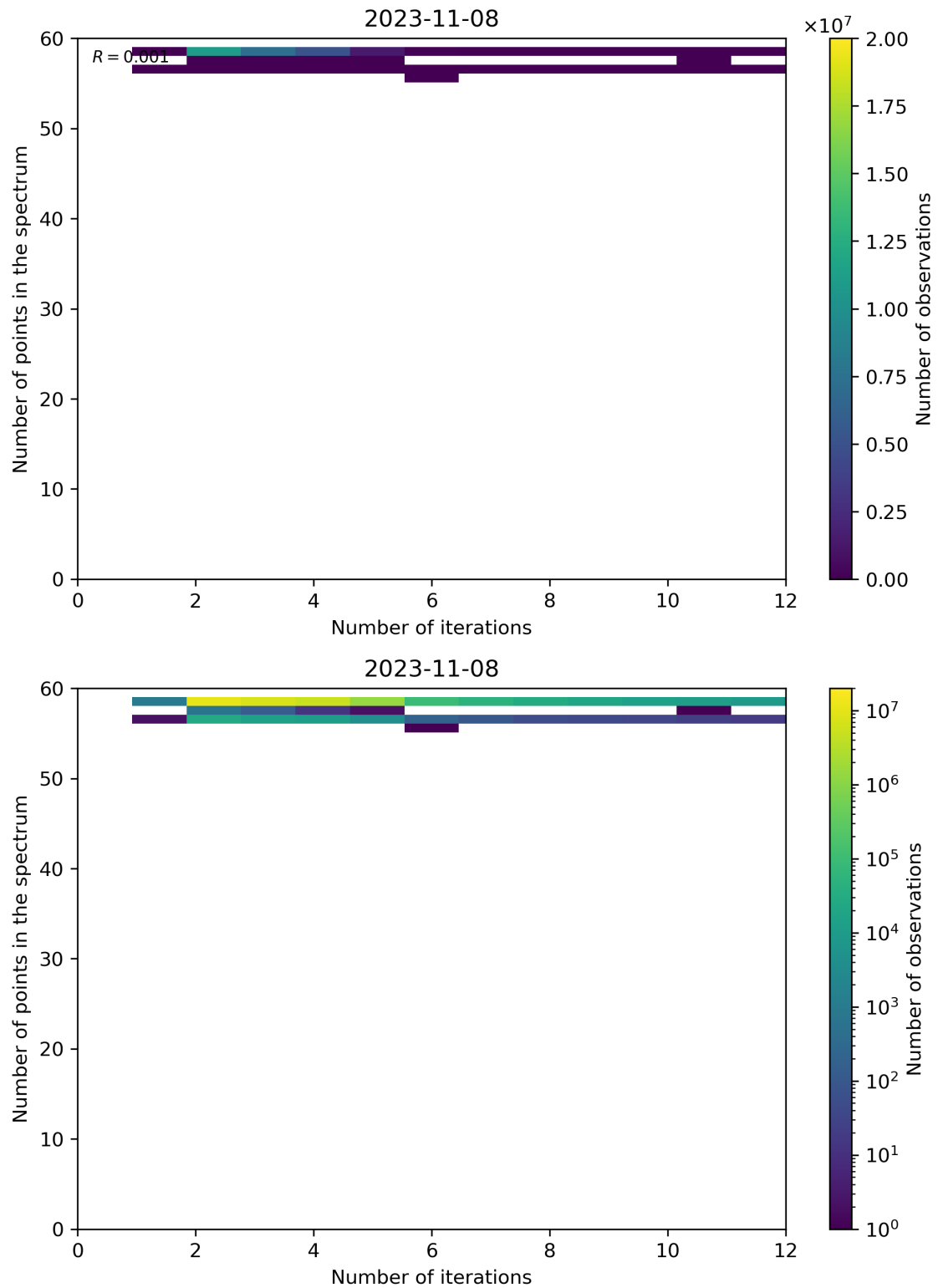
Figure 108: Scatter density plot of “Number of iterations” against “Number of points in the spectrum” for 2023-11-07 to 2023-11-09.
