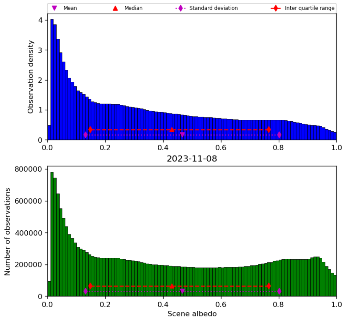
Figure 34: Histogram of “Scene albedo” for 2023-11-07 to 2023-11-09
