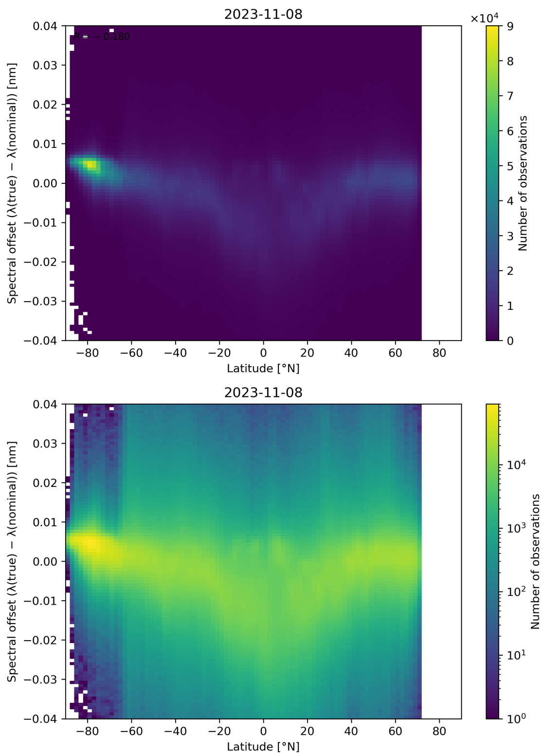
Figure 105: Scatter density plot of “Latitude” against “Spectral offset ( \lambda(\text{true}) - \lambda(\text{nominal}) )” for 2023-11-07 to 2023-11-09.
