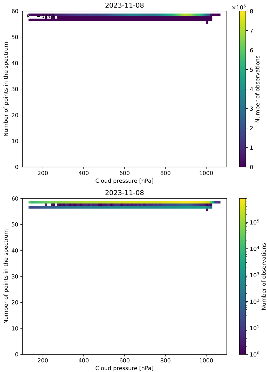
Figure 90: Scatter density plot of “Cloud pressure” against “Number of points in the spectrum” for 2023-11-07 to 2023-11-09.
