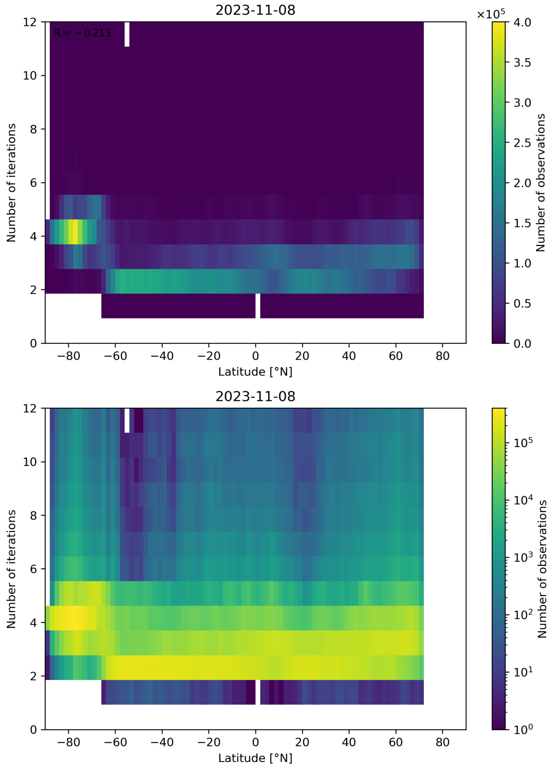
Figure 102: Scatter density plot of “Latitude” against “Number of iterations” for 2023-11-07 to 2023-11-09.
