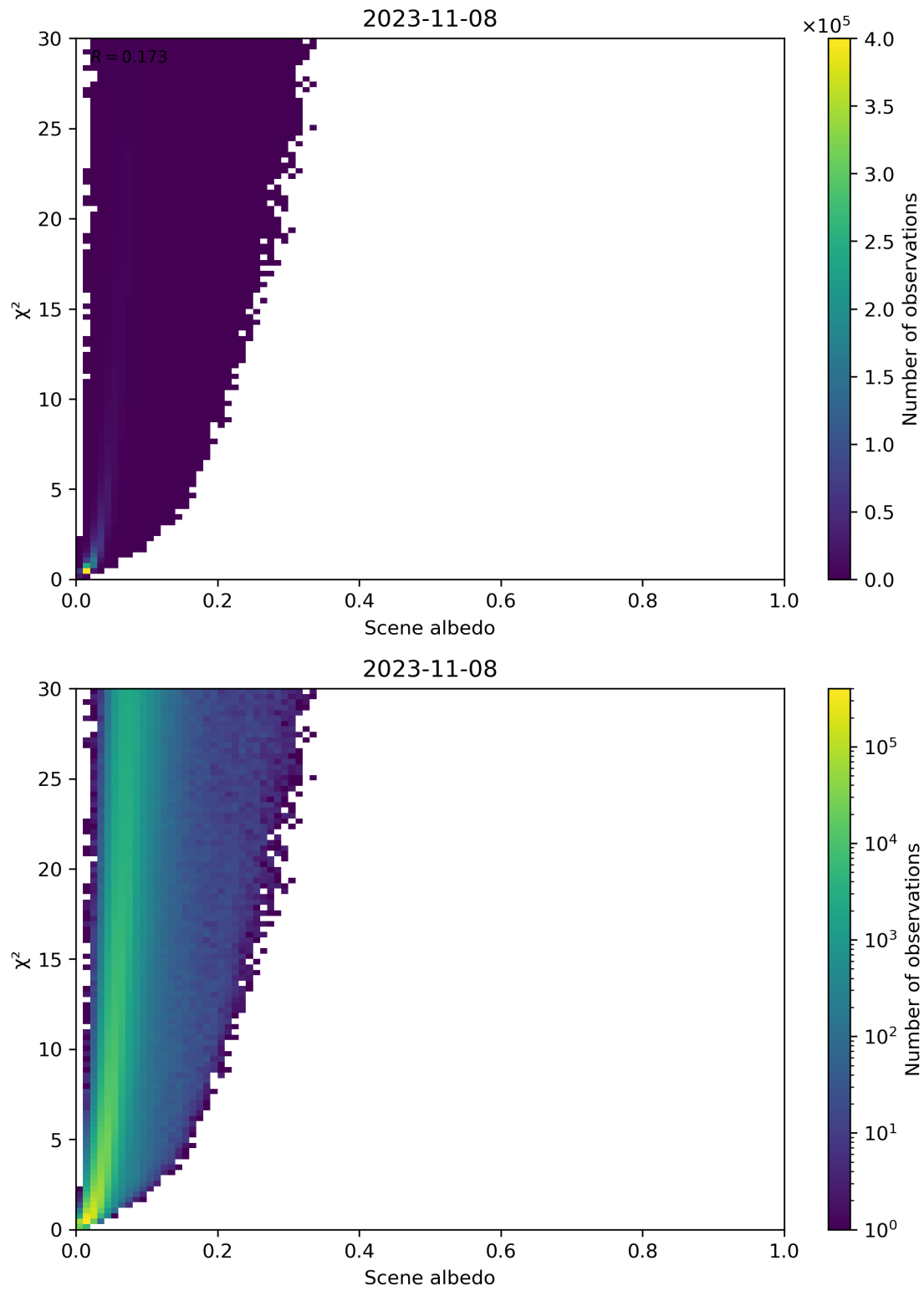
Figure 112: Scatter density plot of “Scene albedo” against “ \chi^2 ” for 2023-11-07 to 2023-11-09.
