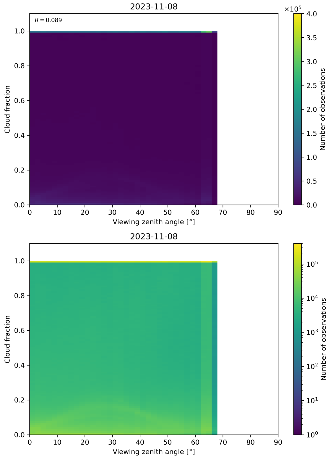
Figure 132: Scatter density plot of “Viewing zenith angle” against “Cloud fraction” for 2023-11-07 to 2023-11-09.
