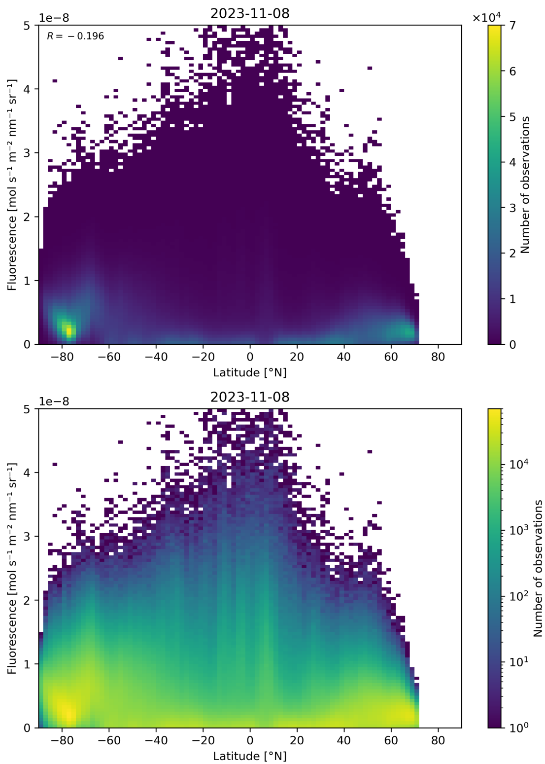
Figure 101: Scatter density plot of “Latitude” against “Fluorescence” for 2023-11-07 to 2023-11-09.
