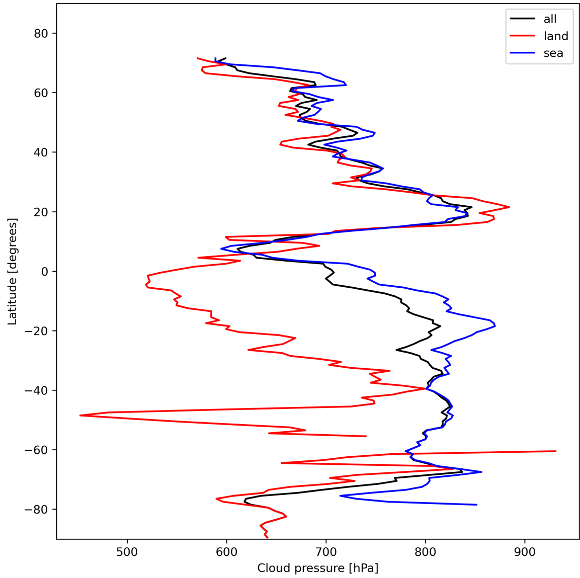
Figure 13: Zonal average of “Cloud pressure” for 2023-11-07 to 2023-11-09.
