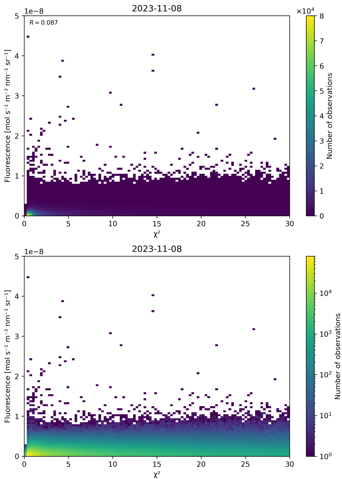
Figure 70: Scatter density plot of “ \chi^2 ” against “Fluorescence” for 2023-11-07 to 2023-11-09.
