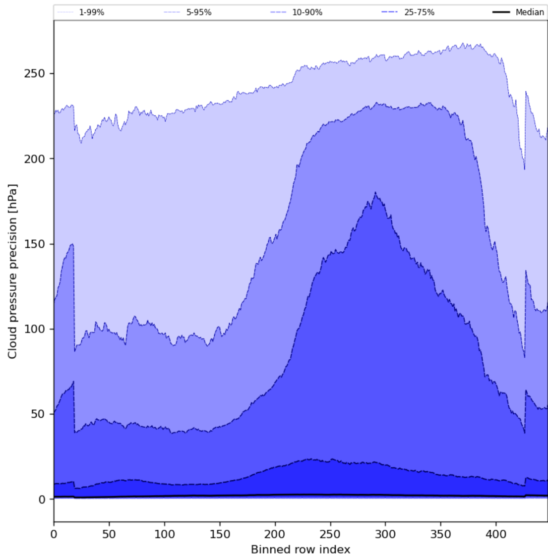
Figure 48: Along track statistics of “Cloud pressure precision” for 2023-11-07 to 2023-11-09
