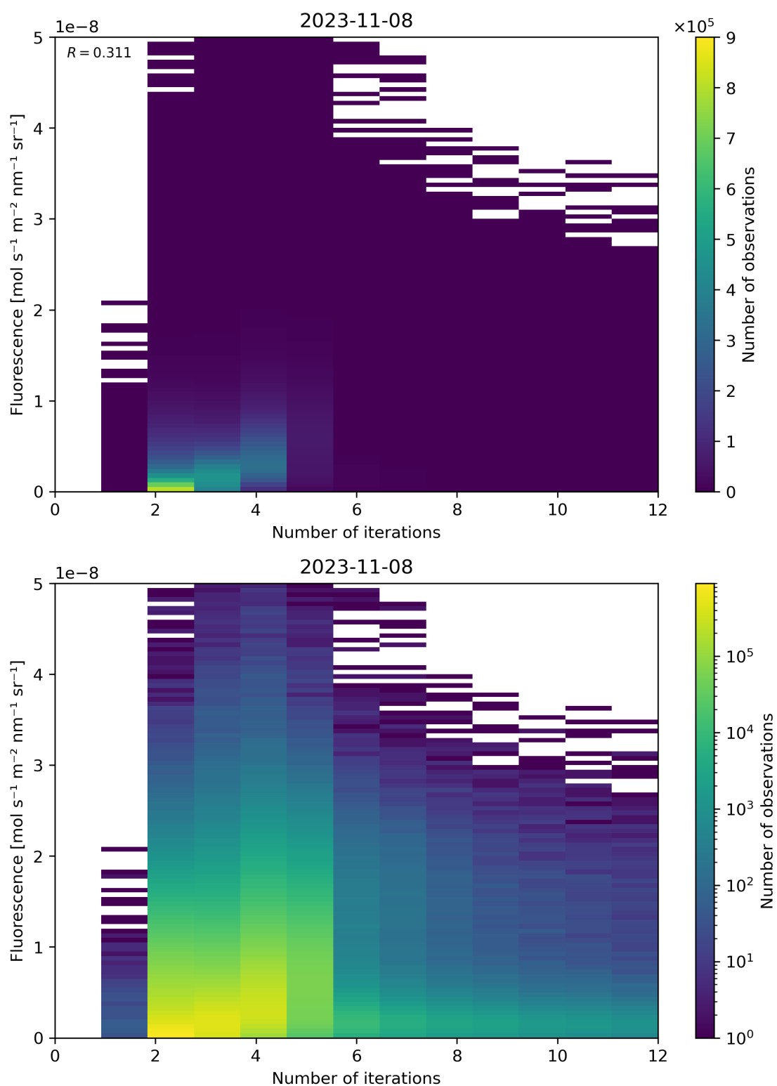
Figure 107: Scatter density plot of “Number of iterations” against “Fluorescence” for 2023-11-07 to 2023-11-09.
