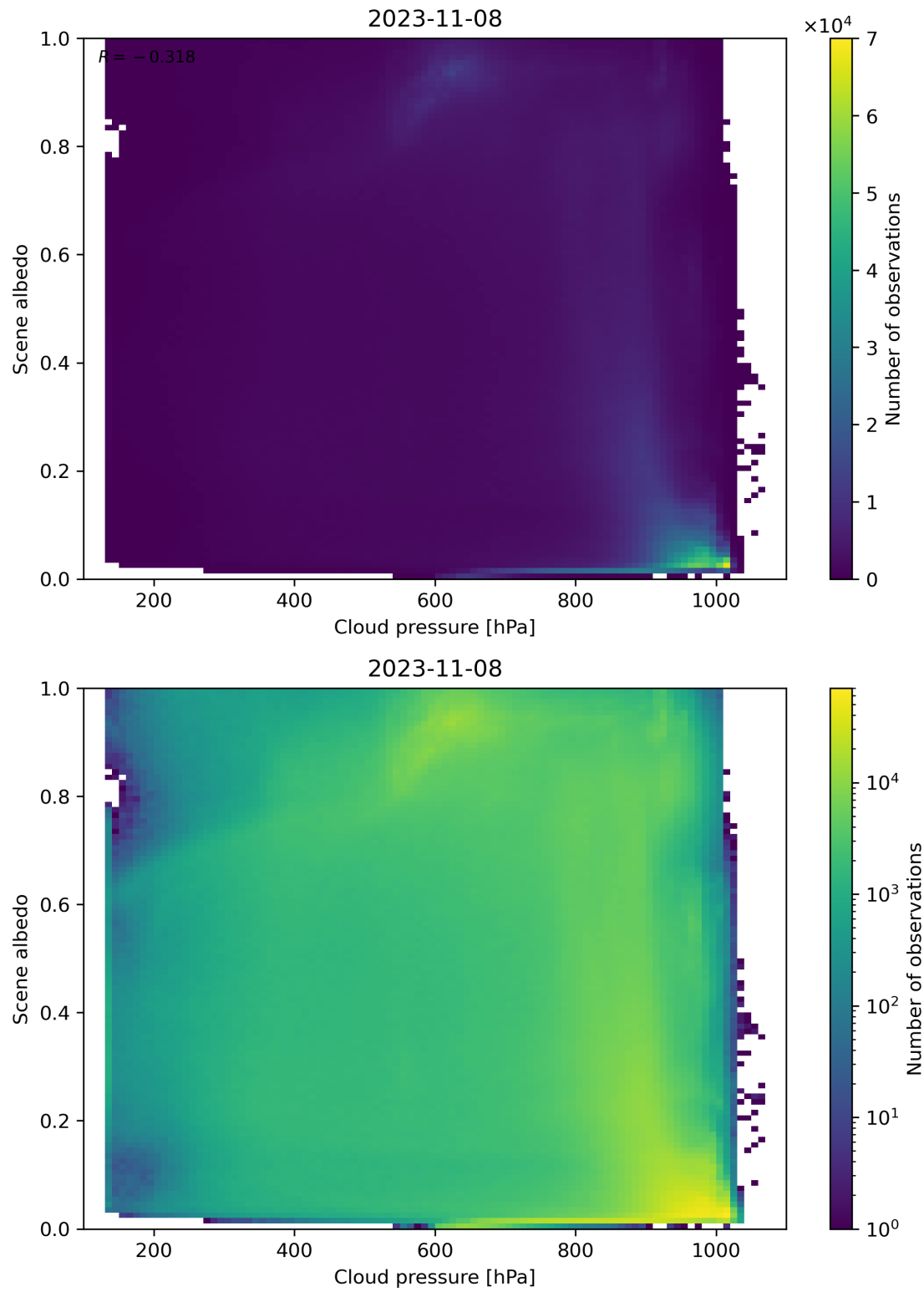
Figure 91: Scatter density plot of “Cloud pressure” against “Scene albedo” for 2023-11-07 to 2023-11-09.
