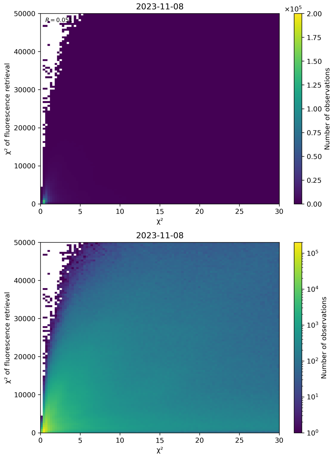
Figure 69: Scatter density plot of “ \chi^2 ” against “ \chi^2 of fluorescence retrieval” for 2023-11-07 to 2023-11-09.
