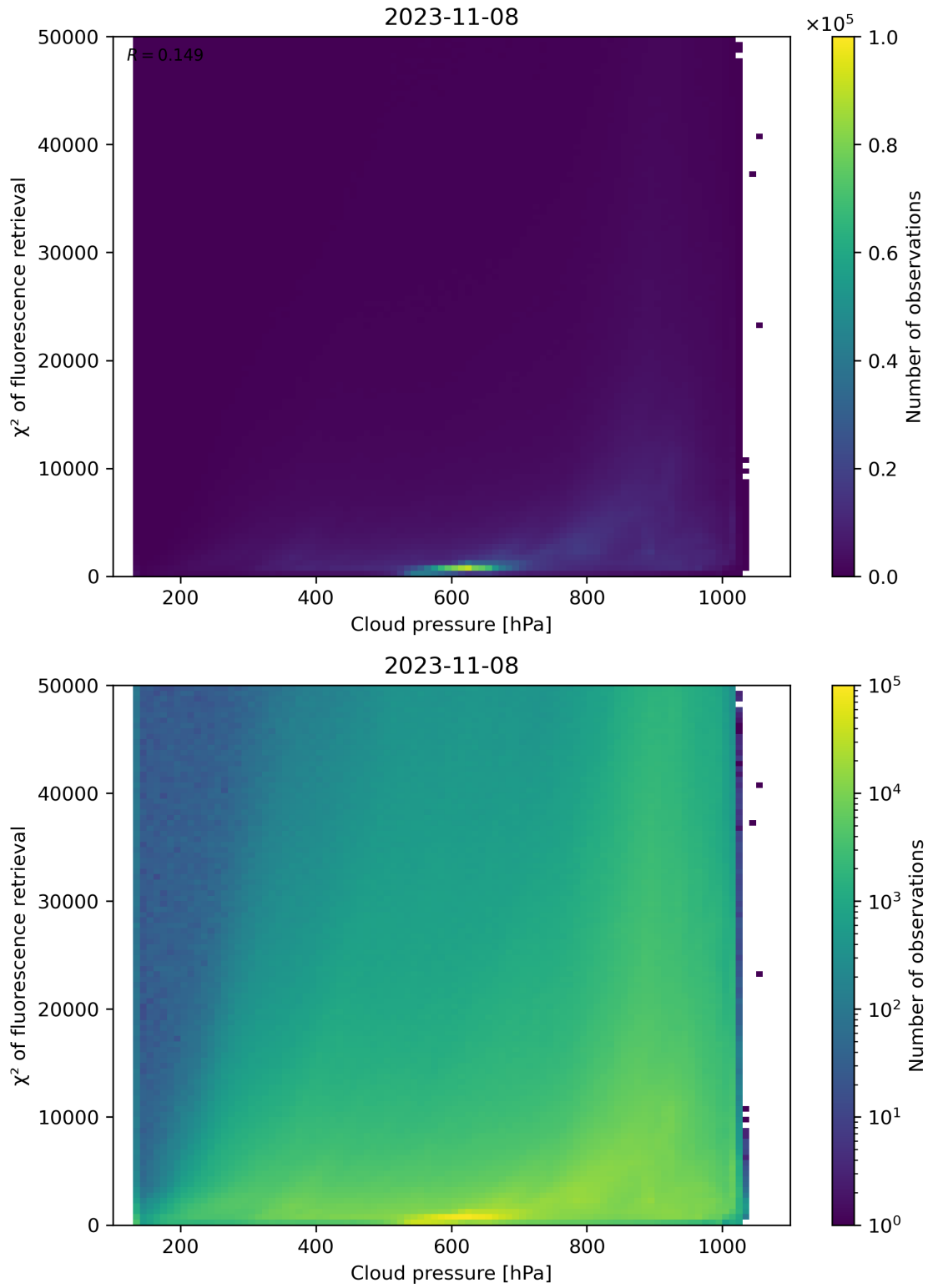
Figure 86: Scatter density plot of “Cloud pressure” against “ \chi^2 of fluorescence retrieval” for 2023-11-07 to 2023-11-09.
