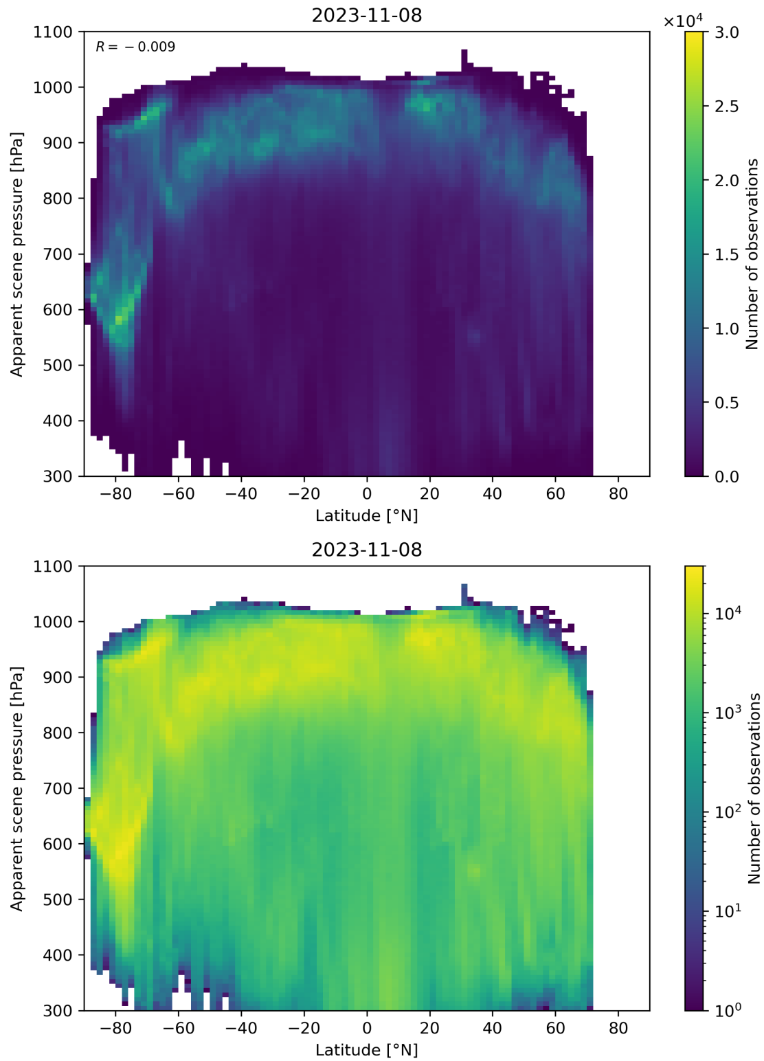
Figure 96: Scatter density plot of “Latitude” against “Apparent scene pressure” for 2023-11-07 to 2023-11-09.
