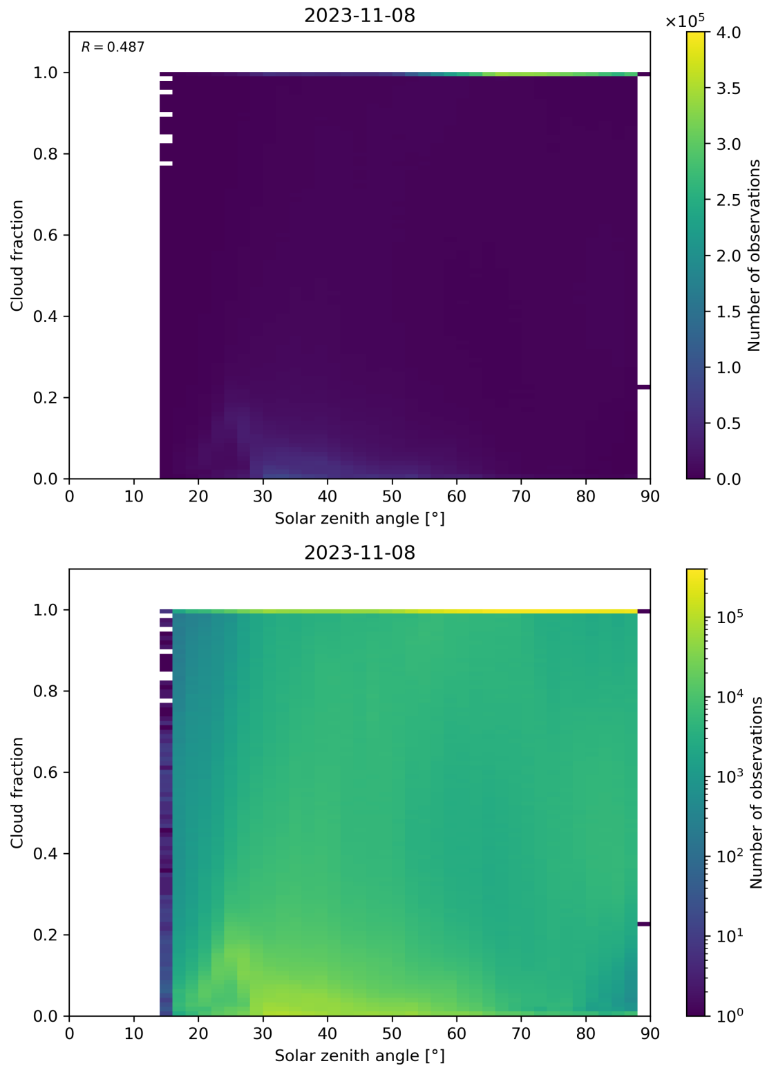
Figure 121: Scatter density plot of “Solar zenith angle” against “Cloud fraction” for 2023-11-07 to 2023-11-09.
