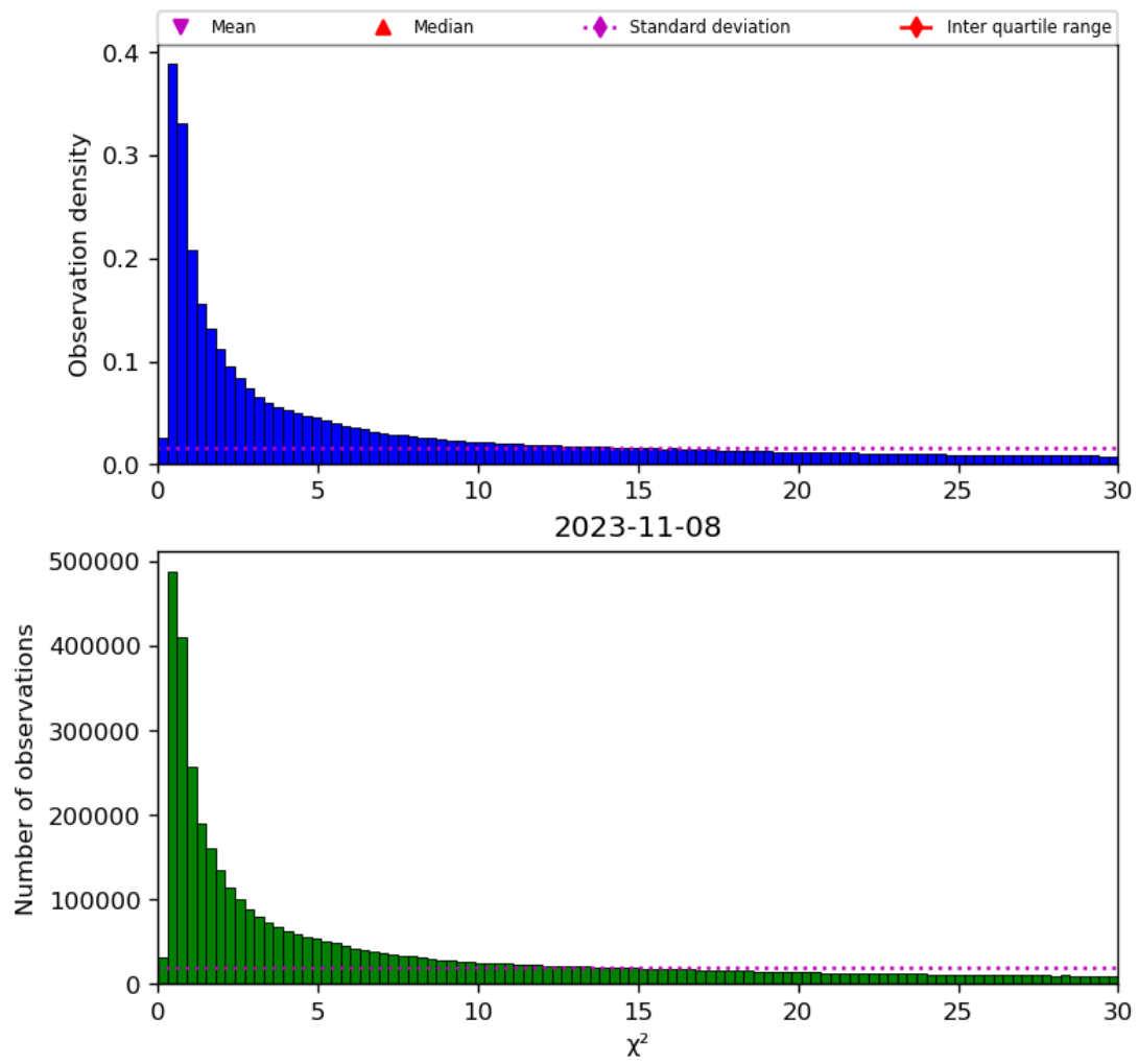
Figure 38: Histogram of “ \chi^2 ” for 2023-11-07 to 2023-11-09
