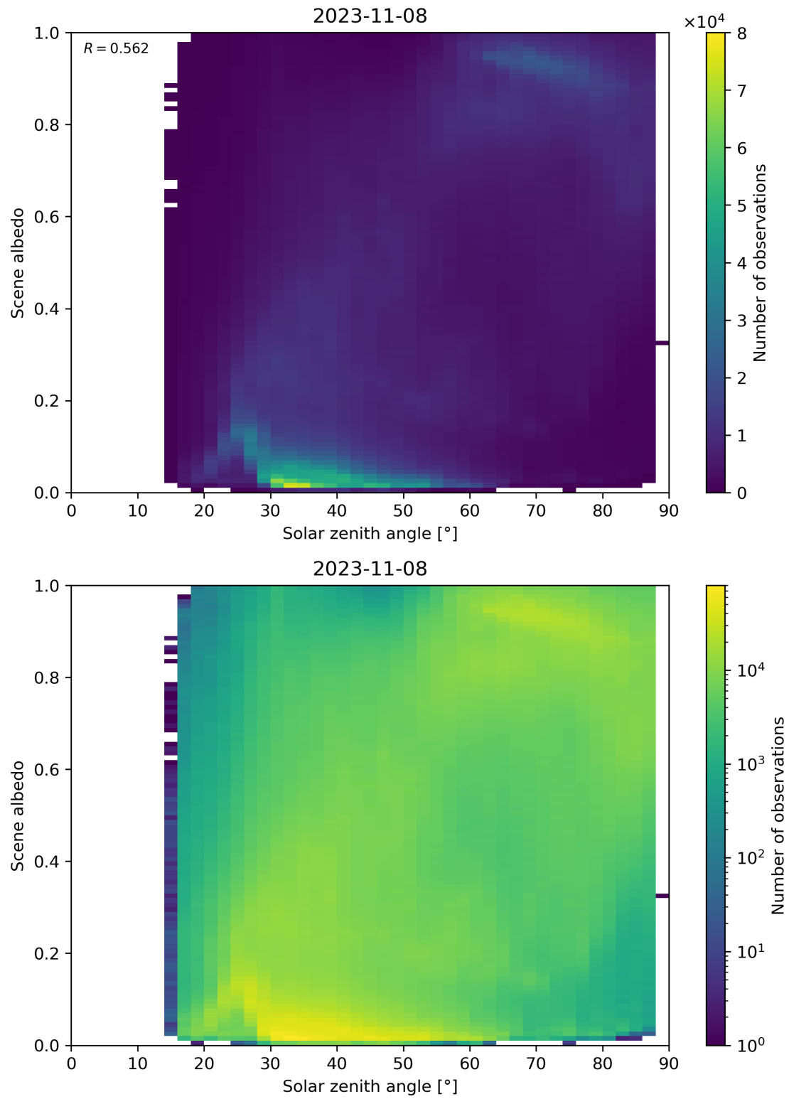
Figure 127: Scatter density plot of “Solar zenith angle” against “Scene albedo” for 2023-11-07 to 2023-11-09.
