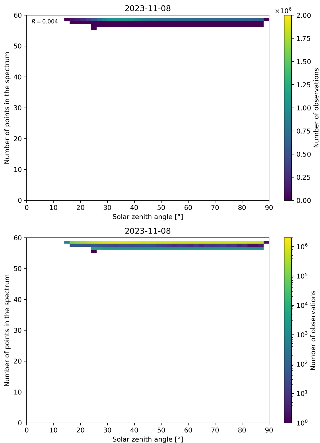
Figure 126: Scatter density plot of “Solar zenith angle” against “Number of points in the spectrum” for 2023-11-07 to 2023-11-09.
