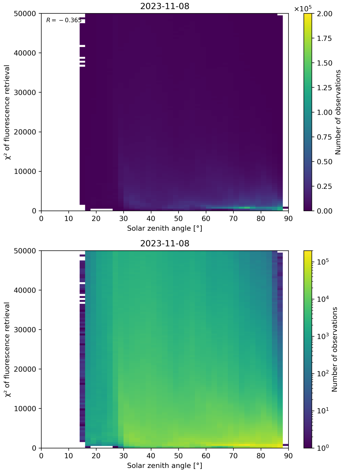
Figure 120: Scatter density plot of “Solar zenith angle” against “ \chi^2 of fluorescence retrieval” for 2023-11-07 to 2023-11-09.
