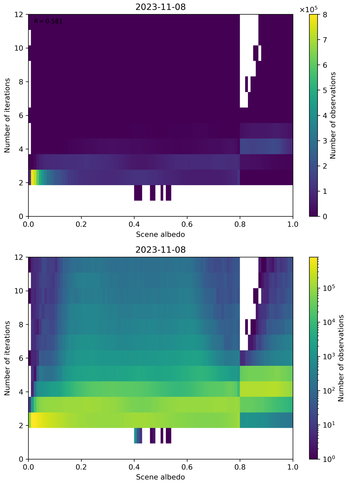
Figure 115: Scatter density plot of “Scene albedo” against “Number of iterations” for 2023-11-07 to 2023-11-09.
