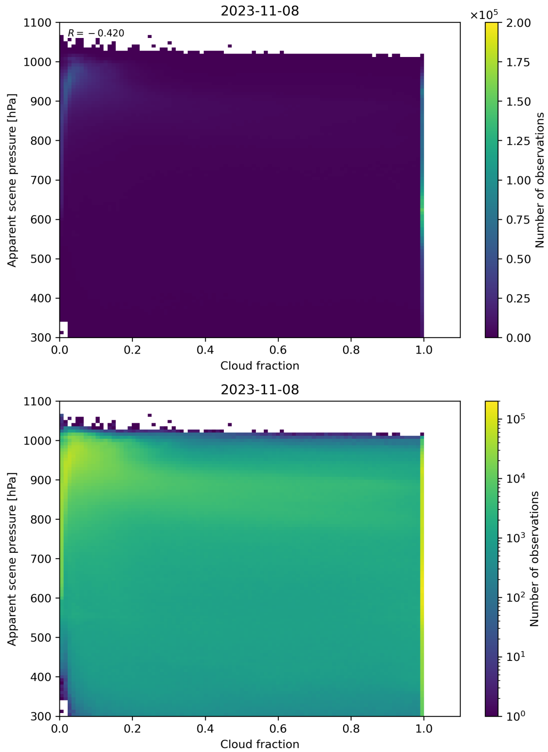
Figure 76: Scatter density plot of “Cloud fraction” against “Apparent scene pressure” for 2023-11-07 to 2023-11-09.
