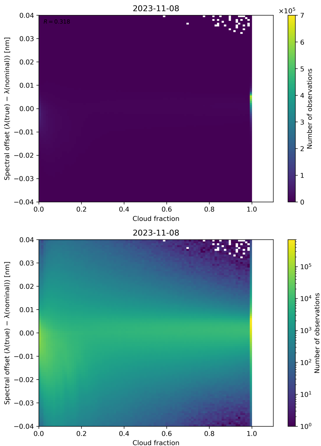
Figure 83: Scatter density plot of “Cloud fraction” against “Spectral offset ( \lambda(\text{true}) - \lambda(\text{nominal}) )” for 2023-11-07 to 2023-11-09.
