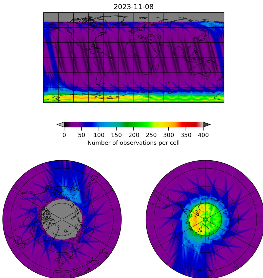
Figure 11: Map of the number of observations for 2023-11-07 to 2023-11-09
