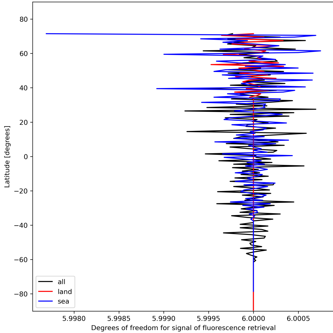
Figure 26: Zonal average of “Degrees of freedom for signal of fluorescence retrieval” for 2023-11-07 to 2023-11-09.
