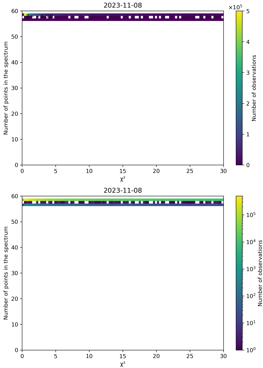
Figure 74: Scatter density plot of " \chi^2 " against "Number of points in the spectrum" for 2023-11-07 to 2023-11-09.
