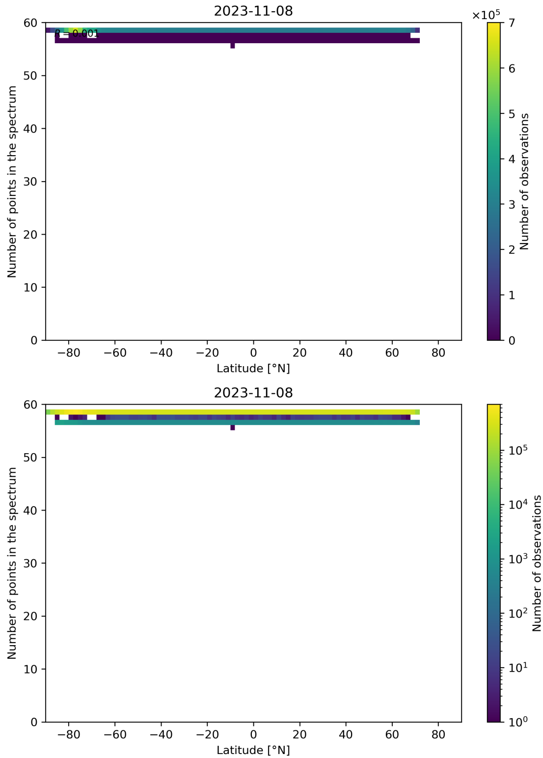
Figure 103: Scatter density plot of “Latitude” against “Number of points in the spectrum” for 2023-11-07 to 2023-11-09.
