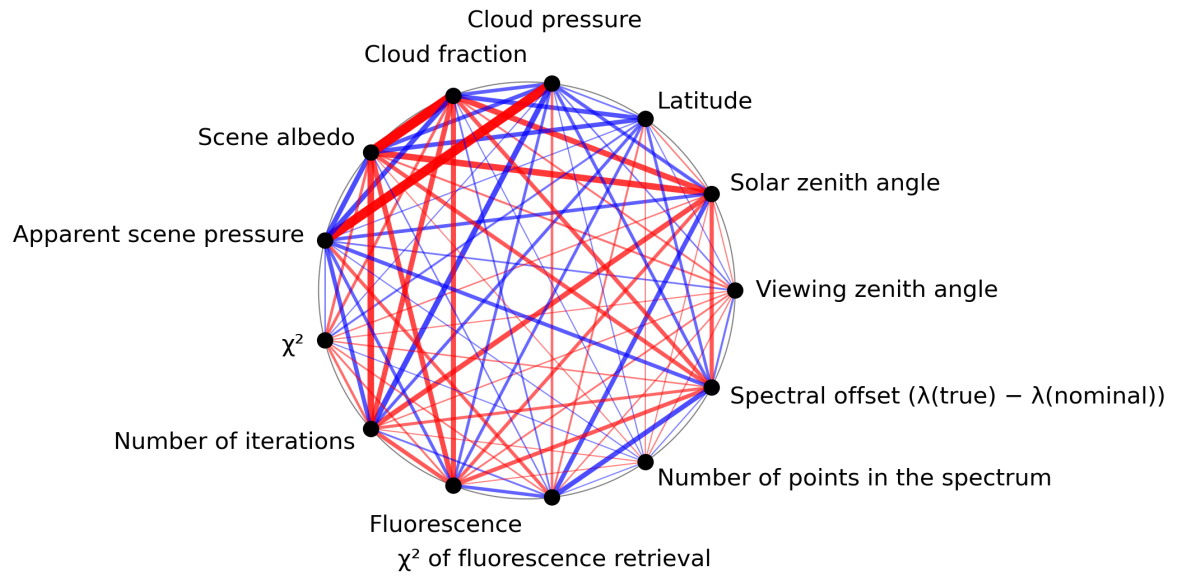
Figure 1: Map of correlation graph for 2023-11-07 to 2023-11-09.
