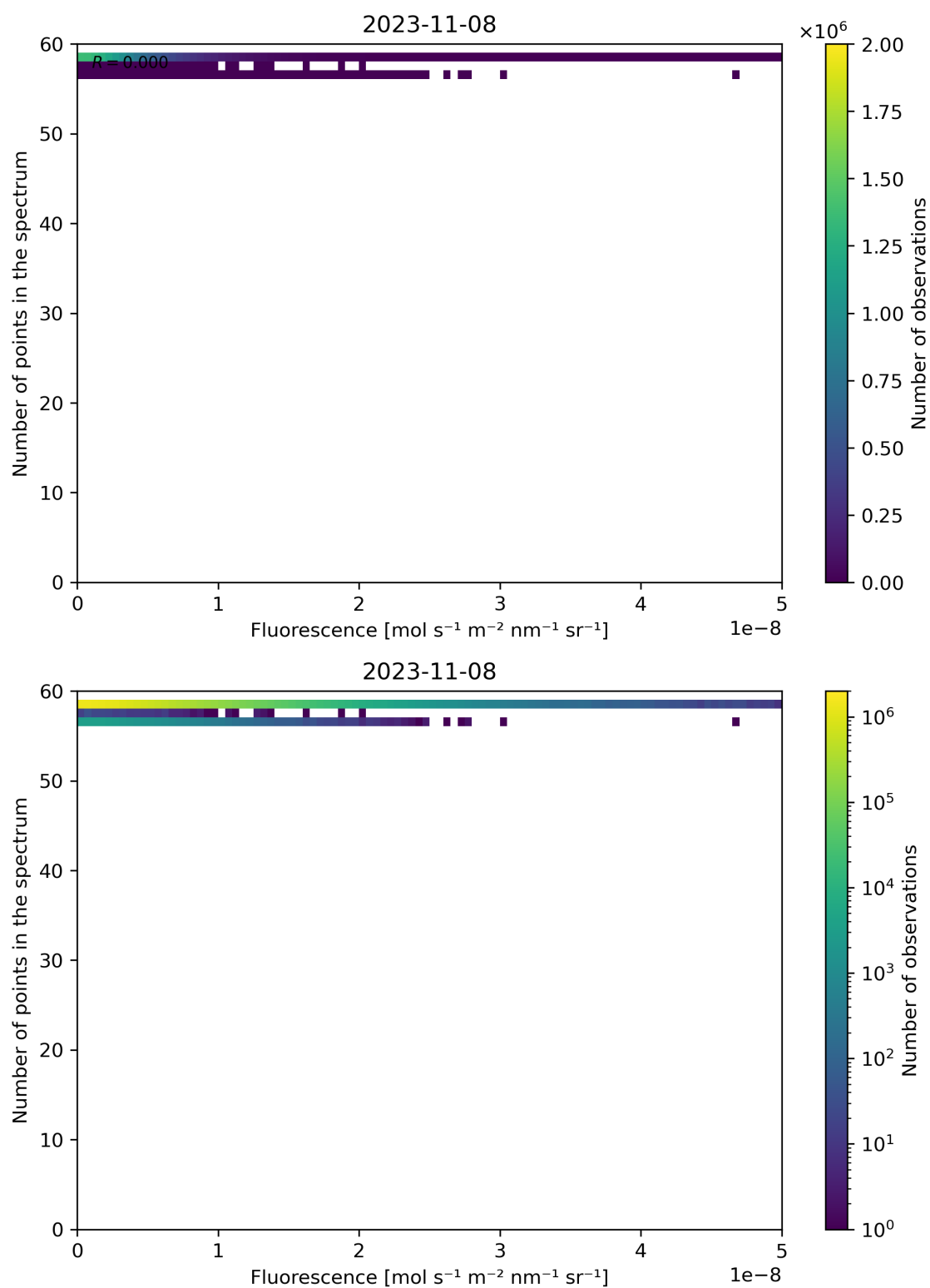
Figure 94: Scatter density plot of “Fluorescence” against “Number of points in the spectrum” for 2023-11-07 to 2023-11-09.
