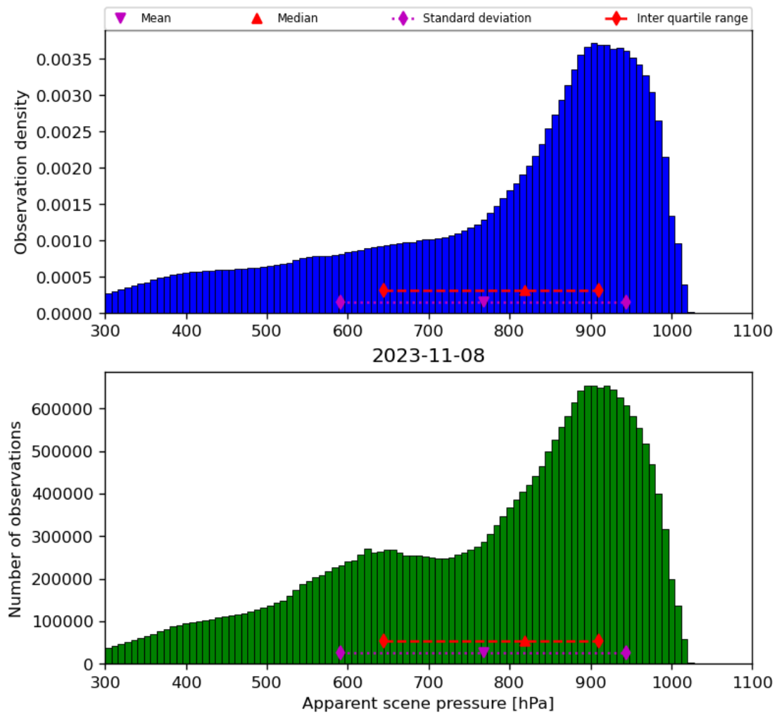
Figure 36: Histogram of “Apparent scene pressure” for 2023-11-07 to 2023-11-09
