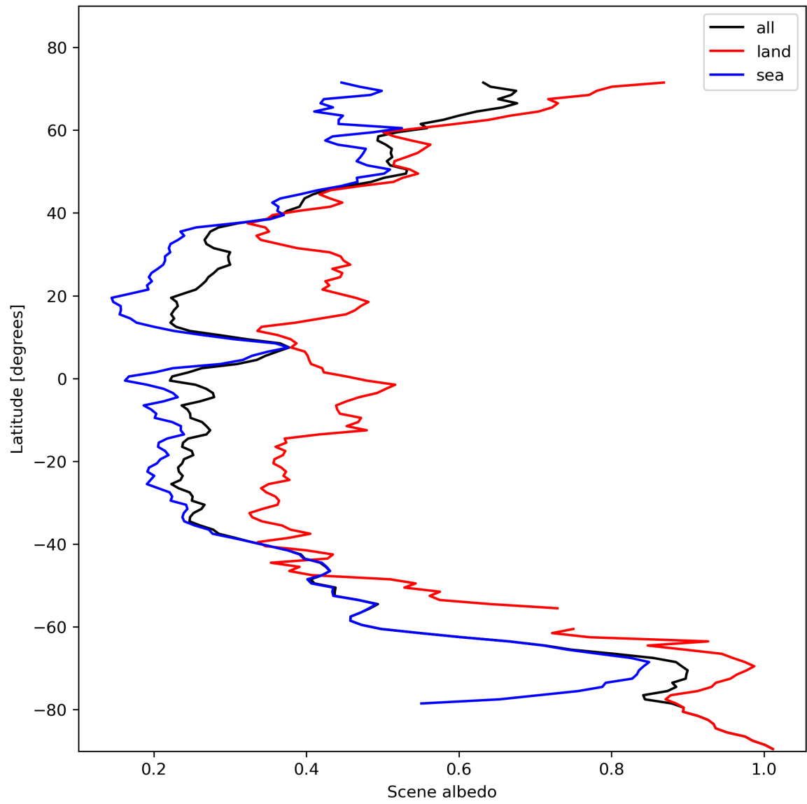
Figure 17: Zonal average of “Scene albedo” for 2023-11-07 to 2023-11-09.
