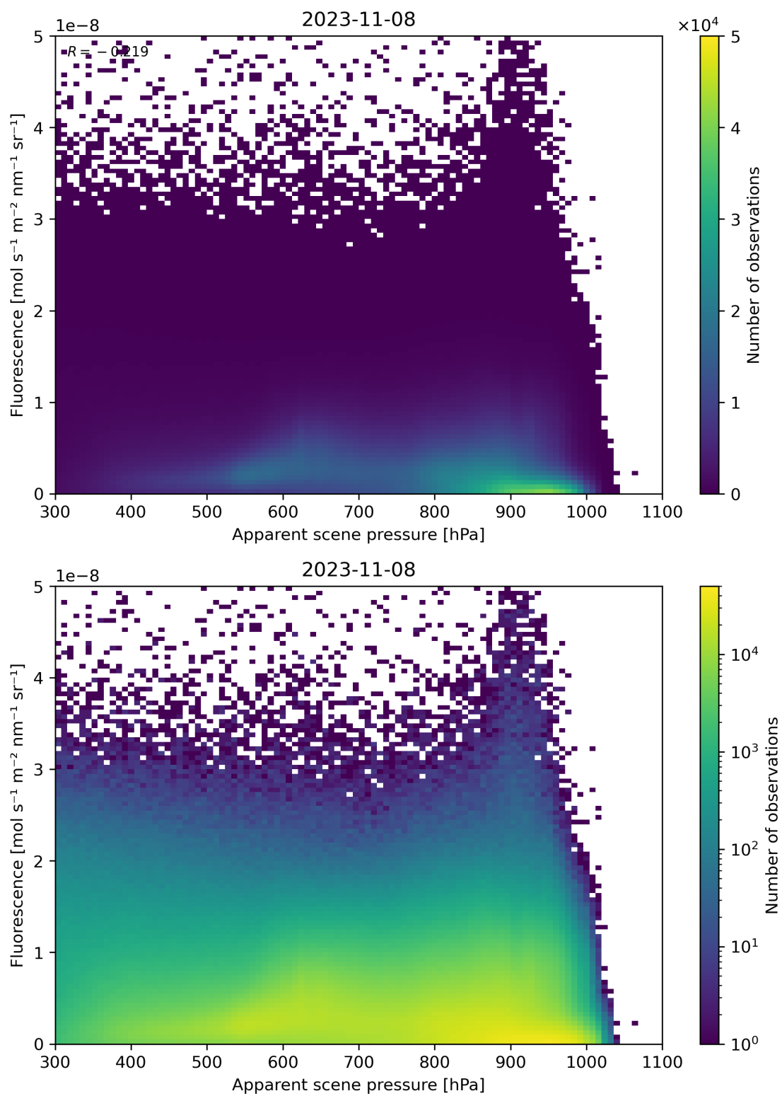
Figure 65: Scatter density plot of “Apparent scene pressure” against “Fluorescence” for 2023-11-07 to 2023-11-09.
