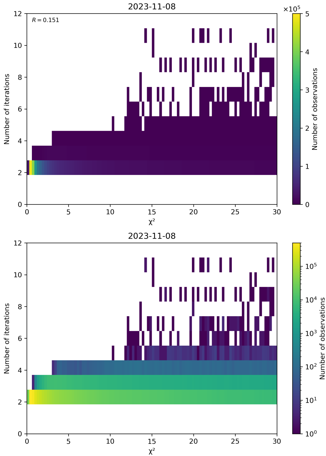
Figure 73: Scatter density plot of “ \chi^2 ” against “Number of iterations” for 2023-11-07 to 2023-11-09.
