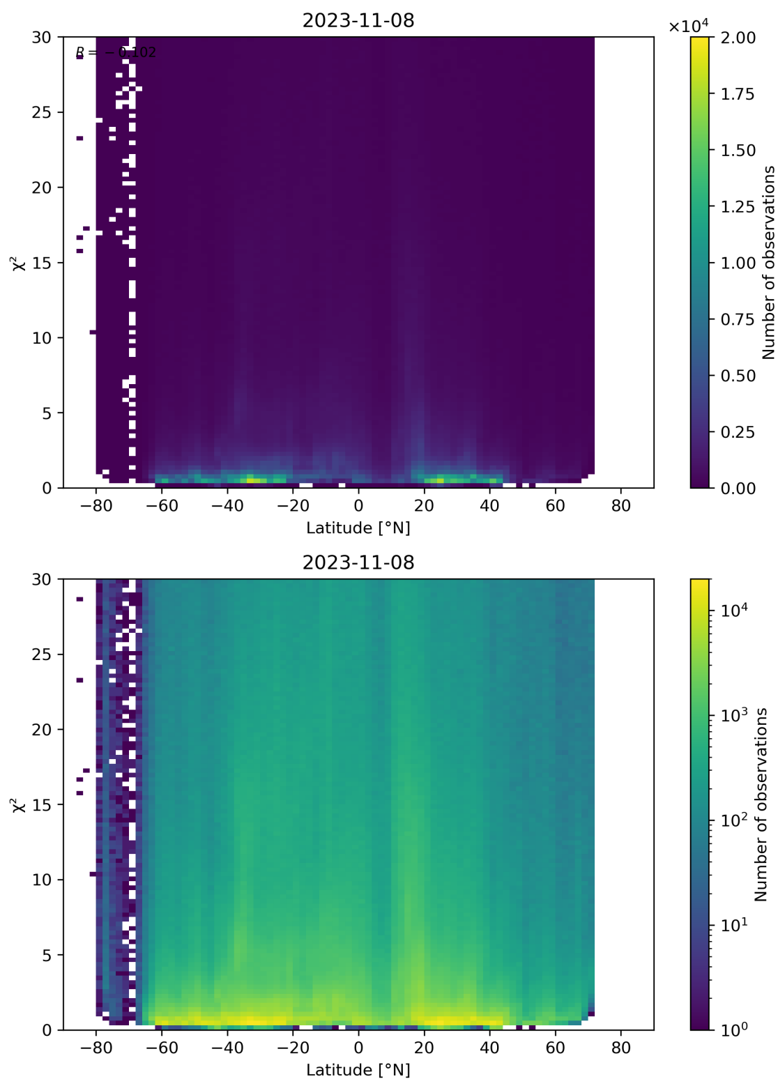
Figure 97: Scatter density plot of “Latitude” against “ \chi^2 ” for 2023-11-07 to 2023-11-09.
