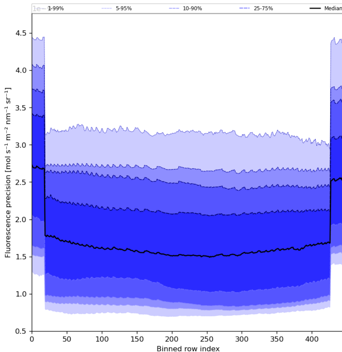
Figure 58: Along track statistics of “Fluorescence precision” for 2023-11-07 to 2023-11-09
