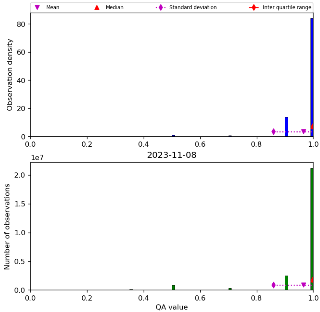
Figure 29: Histogram of “QA value” for 2023-11-07 to 2023-11-09
