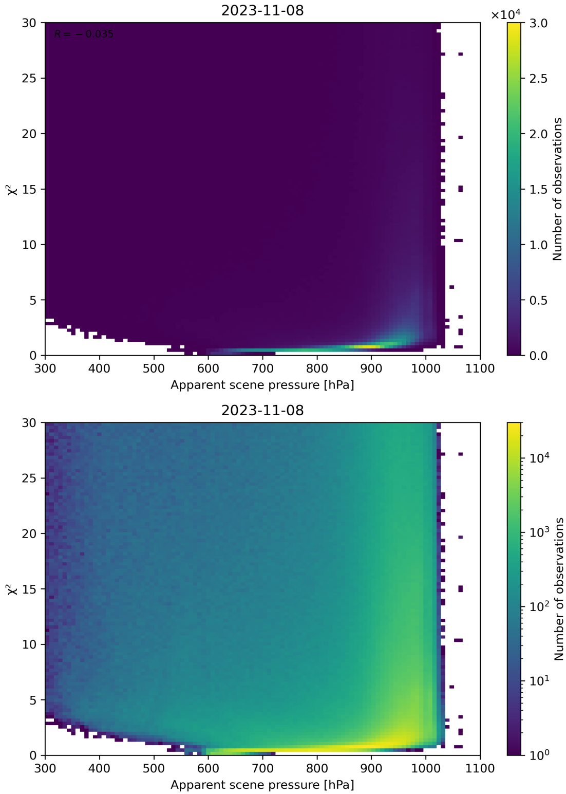
Figure 63: Scatter density plot of “Apparent scene pressure” against “ \chi^2 ” for 2023-11-07 to 2023-11-09.
