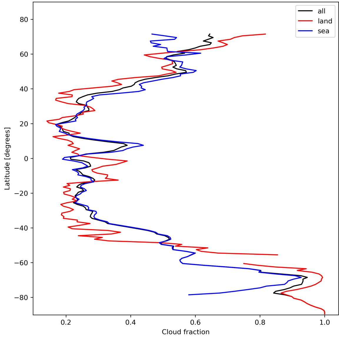
Figure 15: Zonal average of “Cloud fraction” for 2023-11-07 to 2023-11-09.
