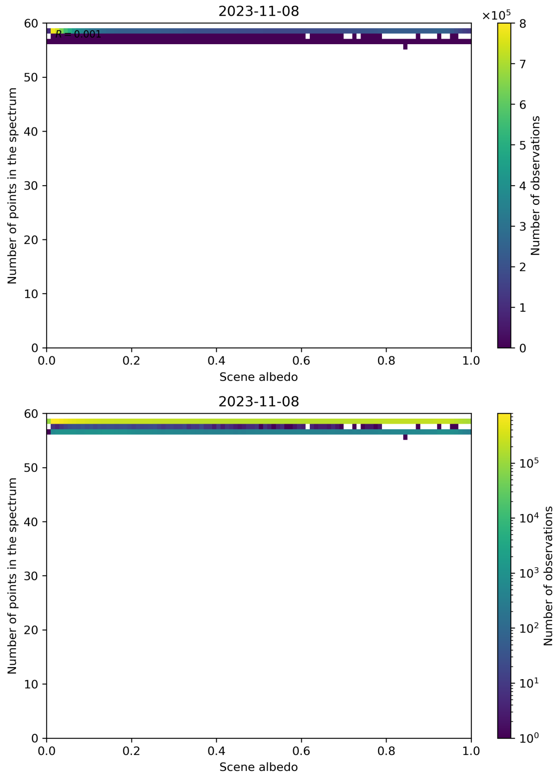
Figure 116: Scatter density plot of “Scene albedo” against “Number of points in the spectrum” for 2023-11-07 to 2023-11-09.
