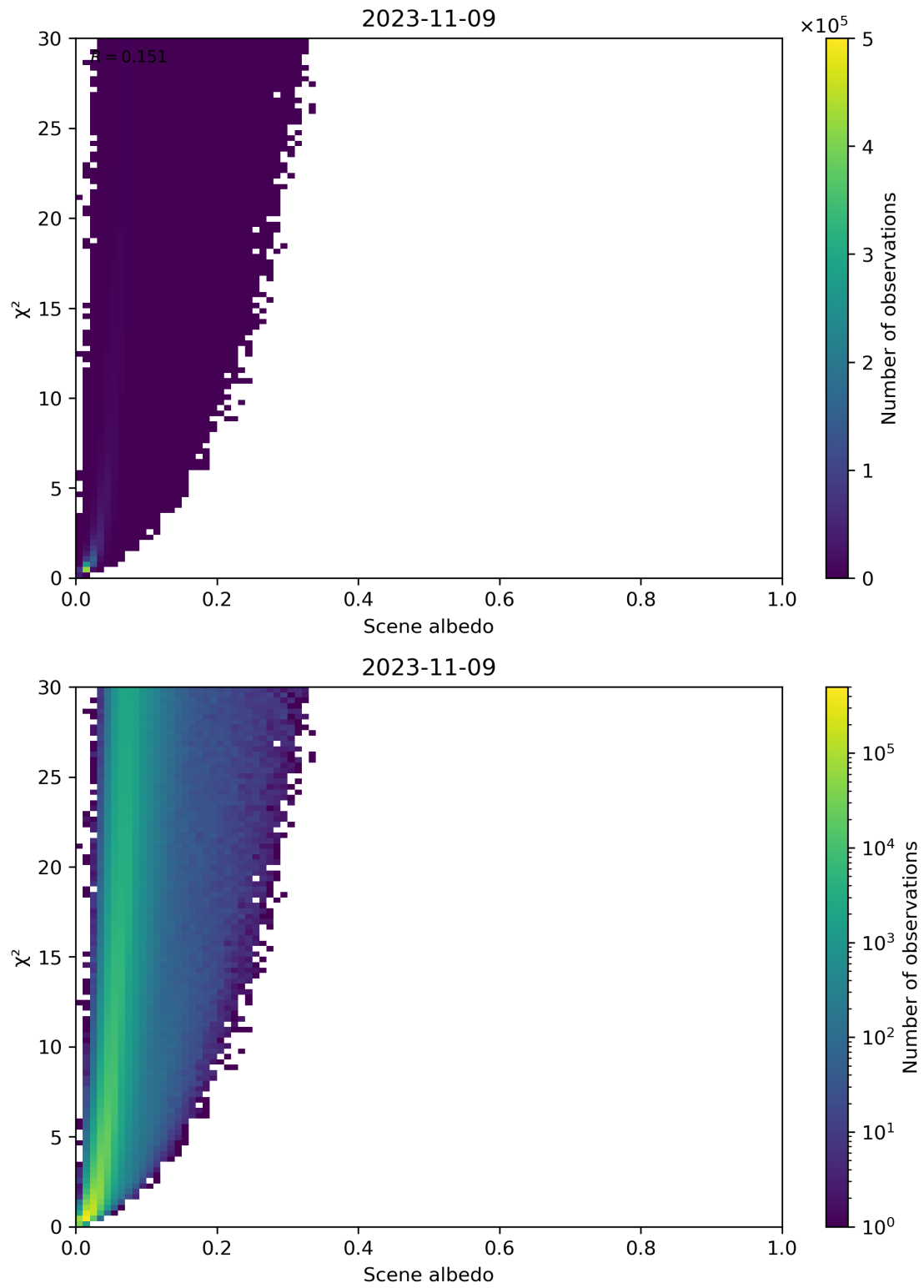
Figure 112: Scatter density plot of “Scene albedo” against “ \chi^2 ” for 2023-11-08 to 2023-11-10.
