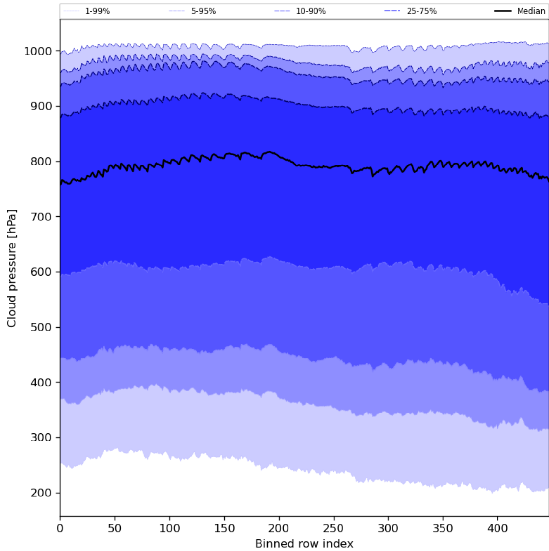
Figure 47: Along track statistics of “Cloud pressure” for 2023-11-08 to 2023-11-10
