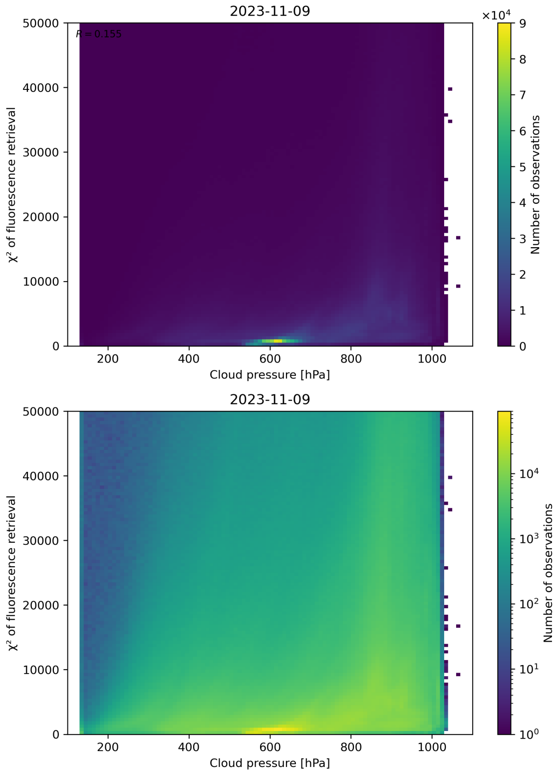
Figure 86: Scatter density plot of “Cloud pressure” against “ \chi^2 of fluorescence retrieval” for 2023-11-08 to 2023-11-10.
