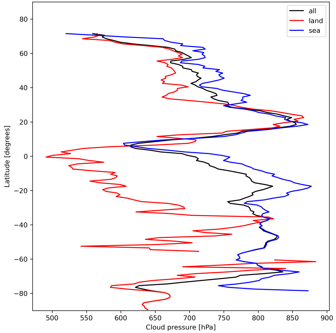
Figure 13: Zonal average of “Cloud pressure” for 2023-11-08 to 2023-11-10.
