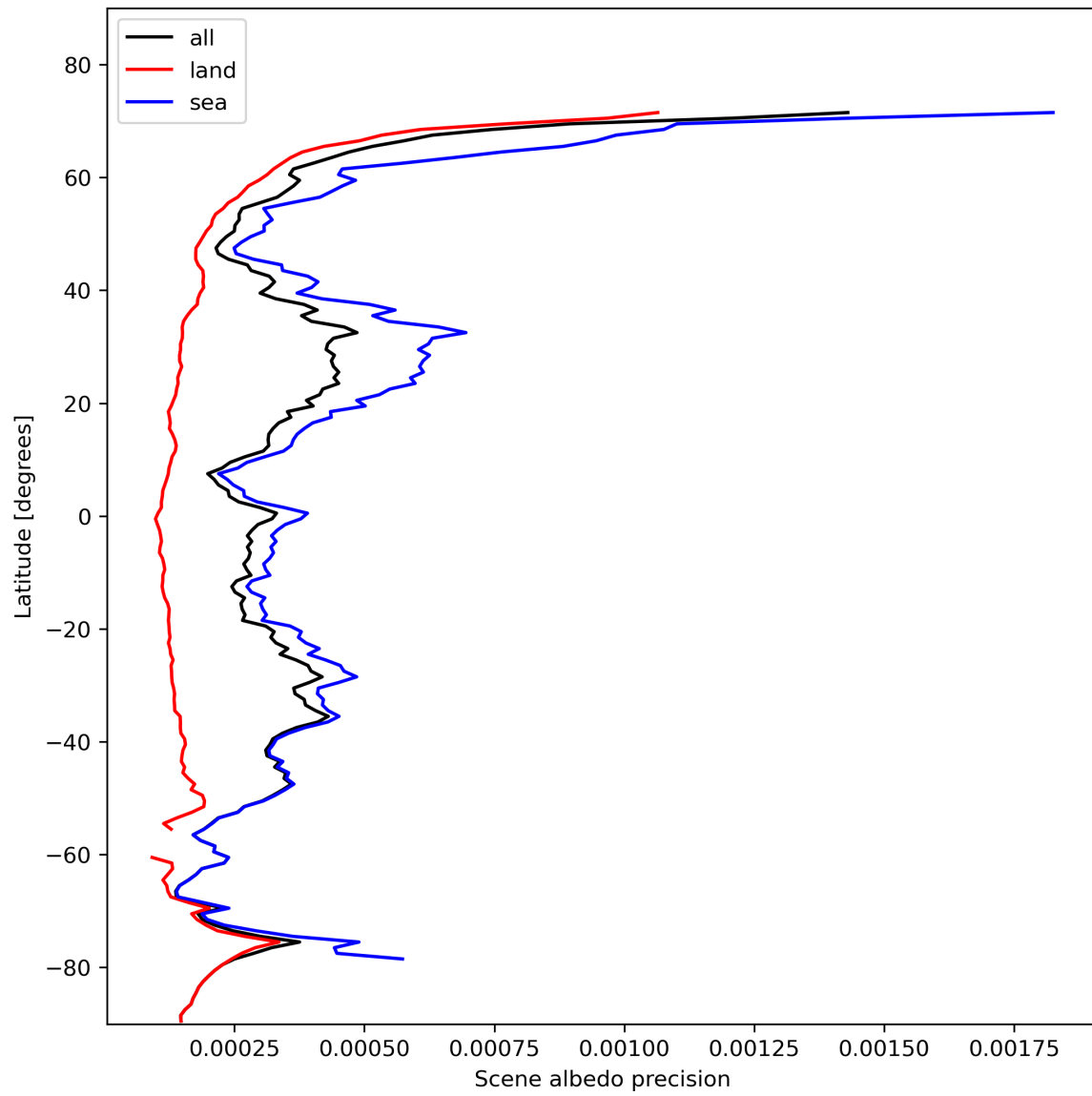
Figure 18: Zonal average of “Scene albedo precision” for 2023-11-08 to 2023-11-10.
