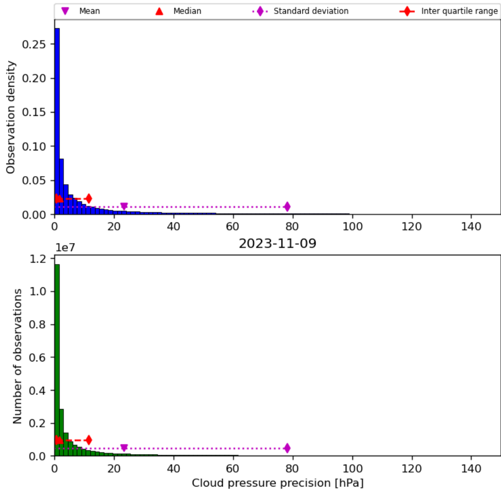
Figure 31: Histogram of “Cloud pressure precision” for 2023-11-08 to 2023-11-10
