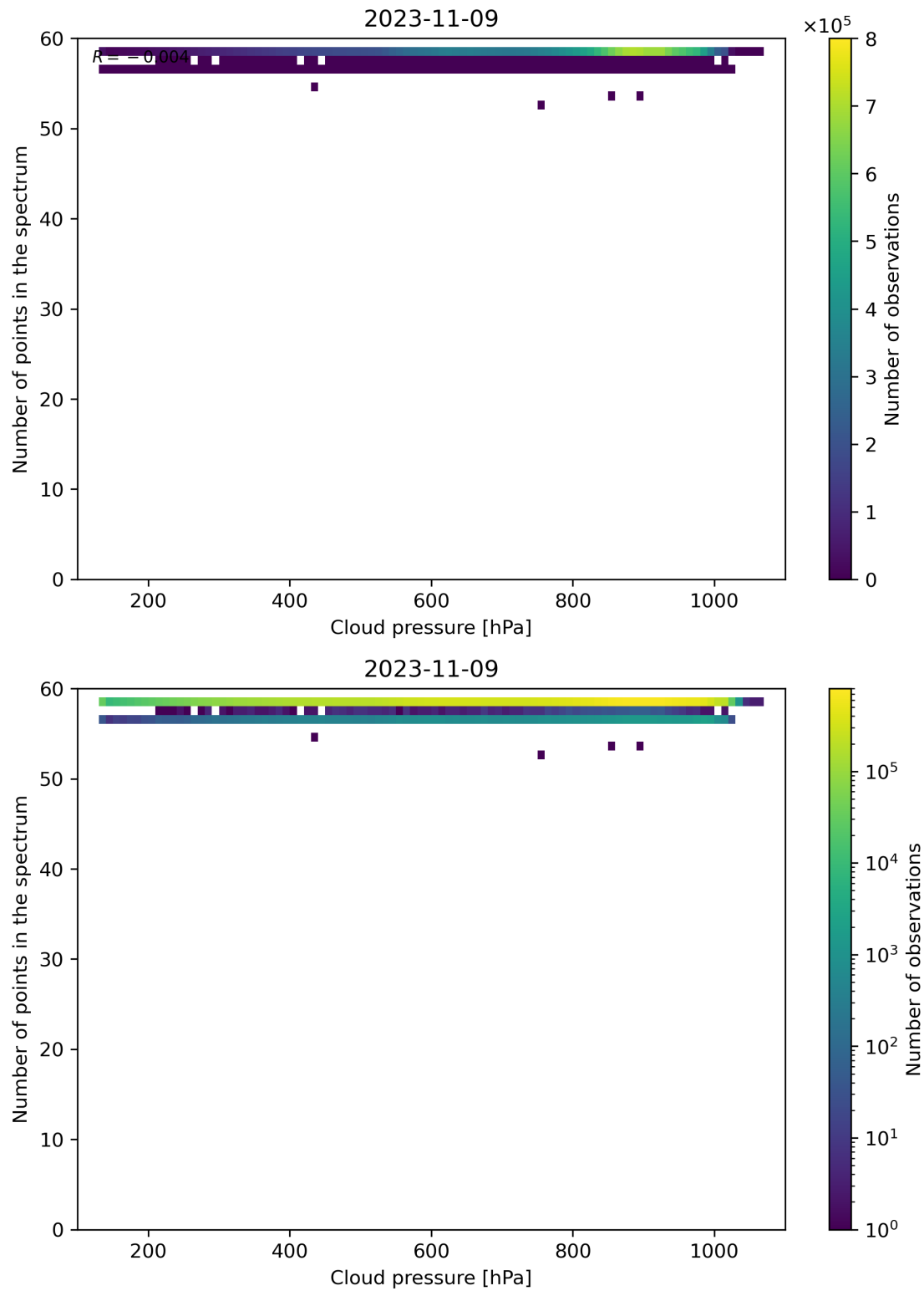
Figure 90: Scatter density plot of “Cloud pressure” against “Number of points in the spectrum” for 2023-11-08 to 2023-11-10.
