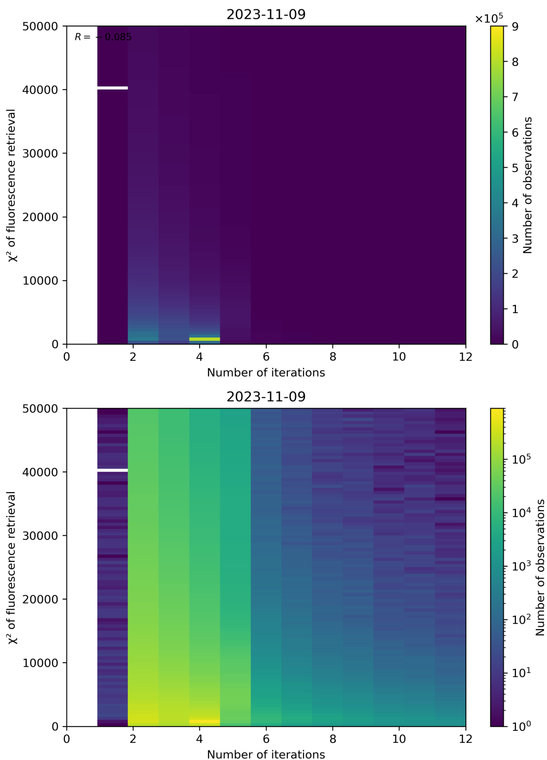
Figure 106: Scatter density plot of “Number of iterations” against “ \chi^2 of fluorescence retrieval” for 2023-11-08 to 2023-11-10.
