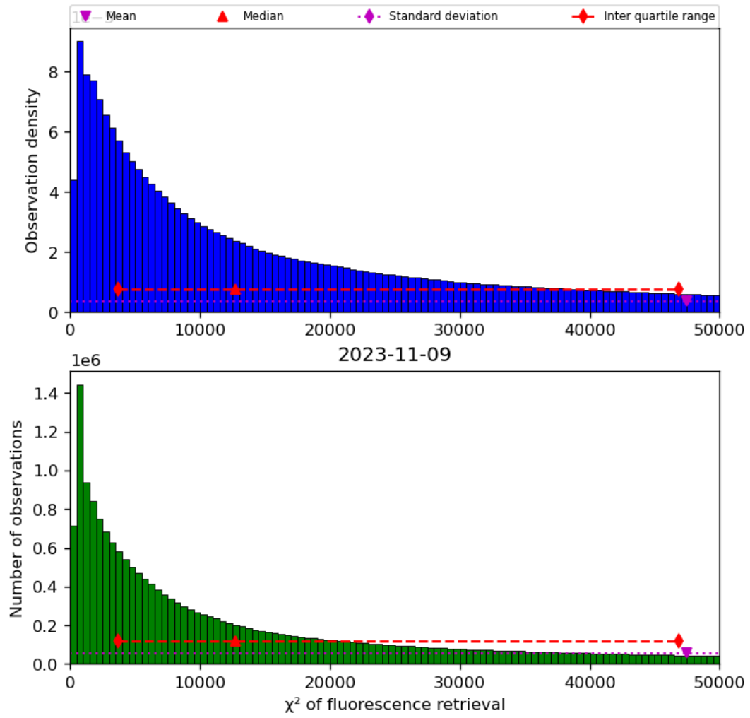
Figure 42: Histogram of “ \chi^2 of fluorescence retrieval” for 2023-11-08 to 2023-11-10
