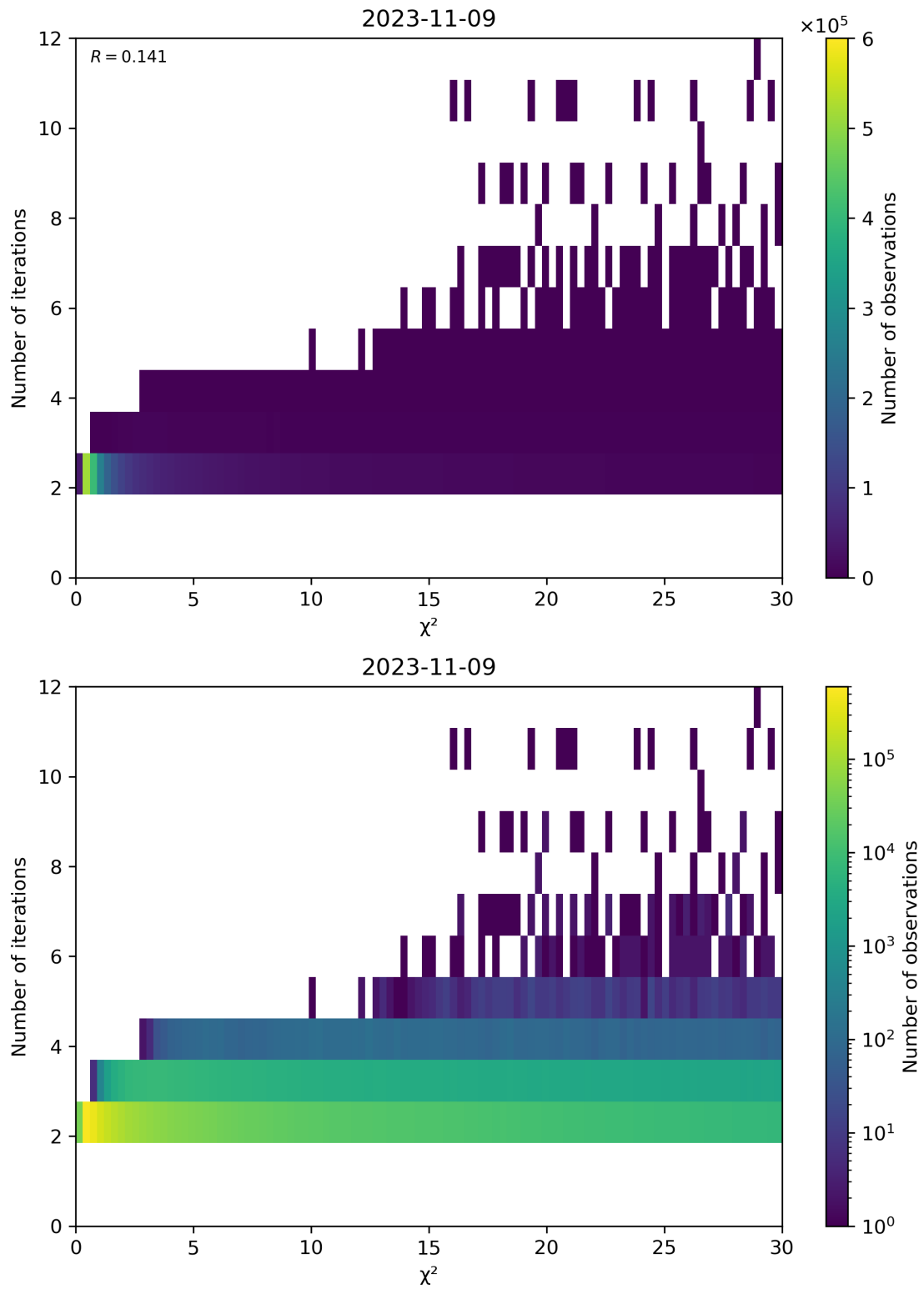
Figure 73: Scatter density plot of “ \chi^2 ” against “Number of iterations” for 2023-11-08 to 2023-11-10.
