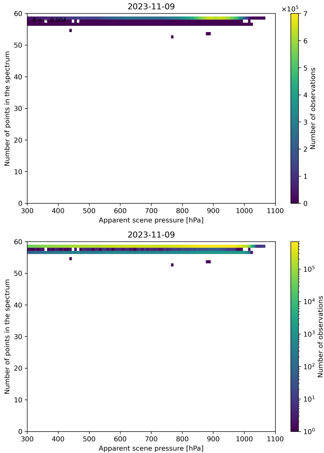
Figure 67: Scatter density plot of “Apparent scene pressure” against “Number of points in the spectrum” for 2023-11-08 to 2023-11-10.
