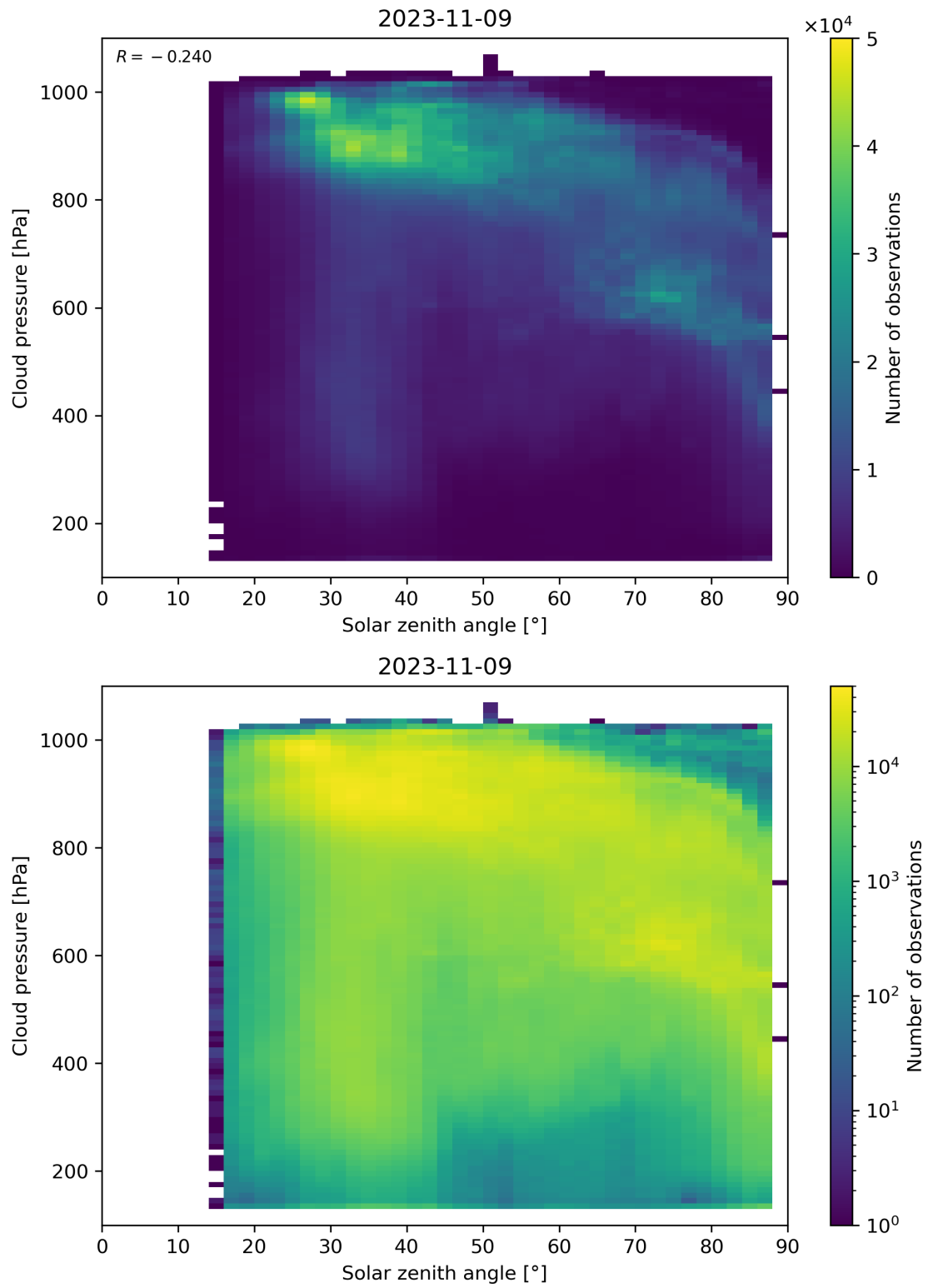
Figure 122: Scatter density plot of “Solar zenith angle” against “Cloud pressure” for 2023-11-08 to 2023-11-10.
