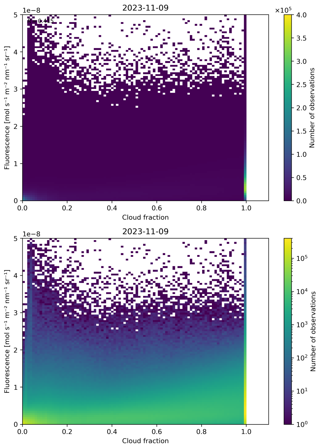
Figure 79: Scatter density plot of “Cloud fraction” against “Fluorescence” for 2023-11-08 to 2023-11-10.
