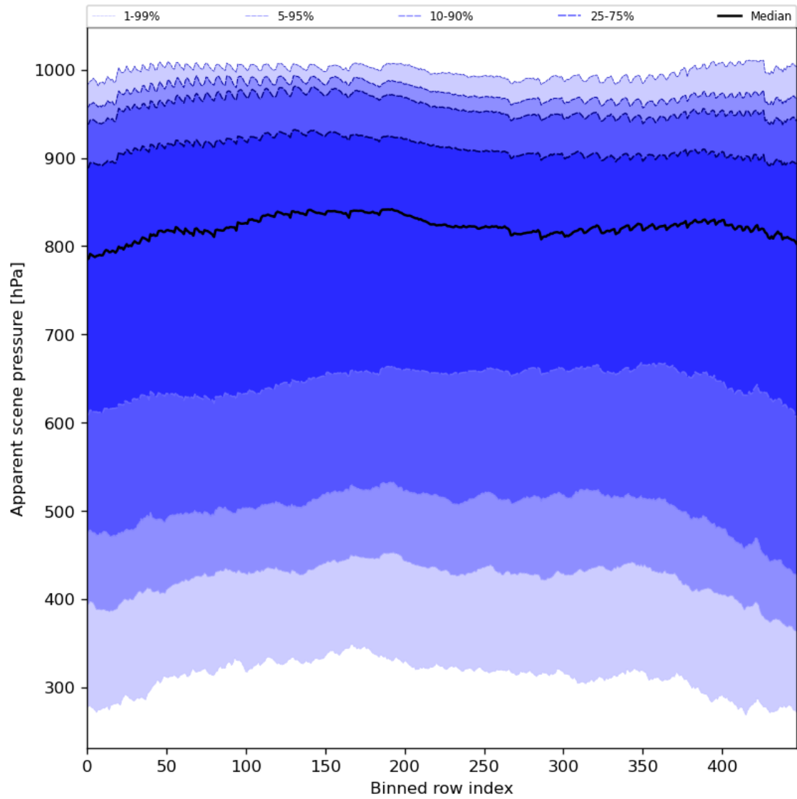
Figure 53: Along track statistics of “Apparent scene pressure” for 2023-11-08 to 2023-11-10
