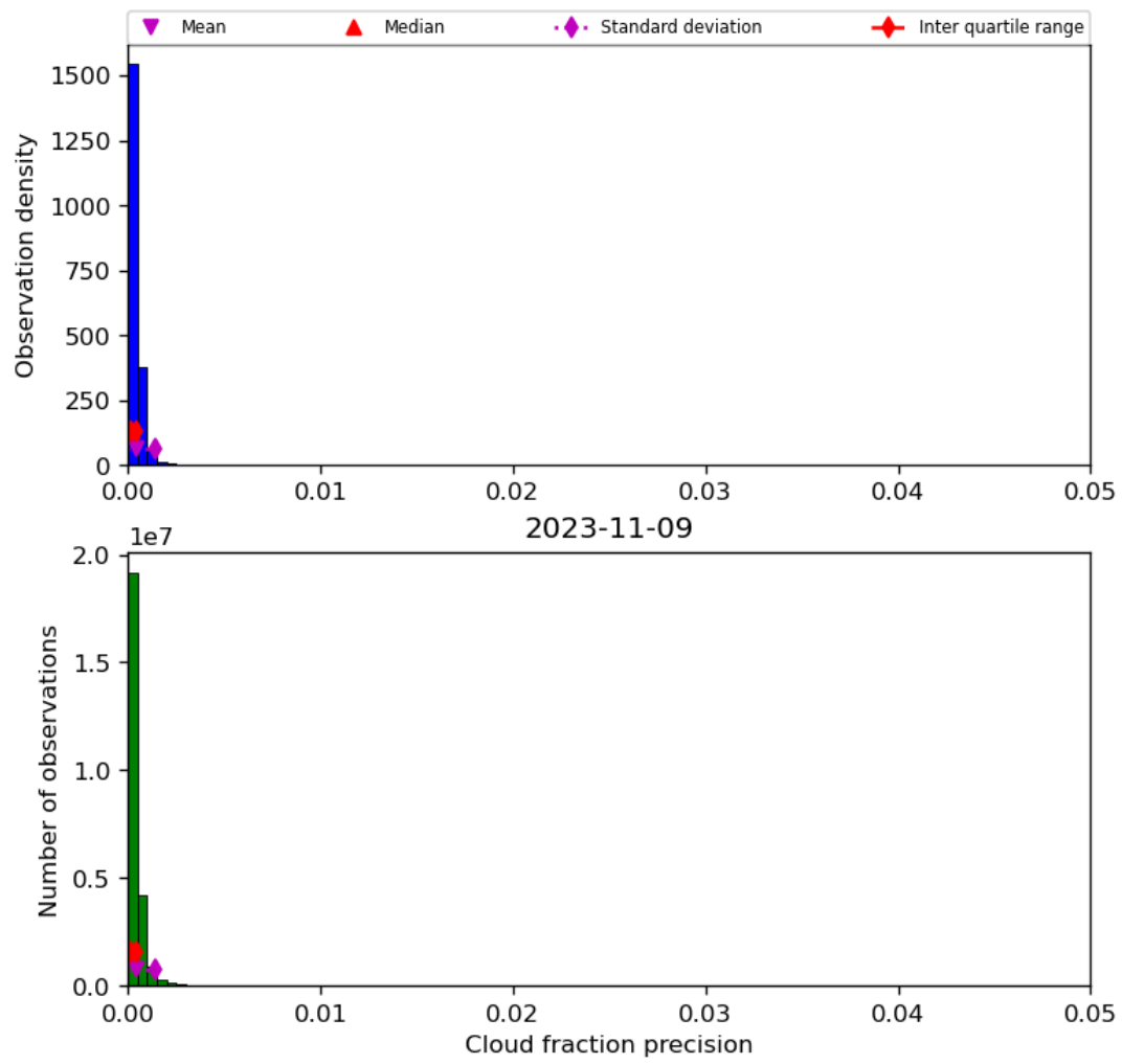
Figure 33: Histogram of “Cloud fraction precision” for 2023-11-08 to 2023-11-10
