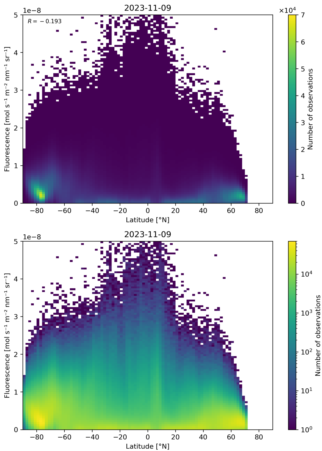
Figure 101: Scatter density plot of “Latitude” against “Fluorescence” for 2023-11-08 to 2023-11-10.
