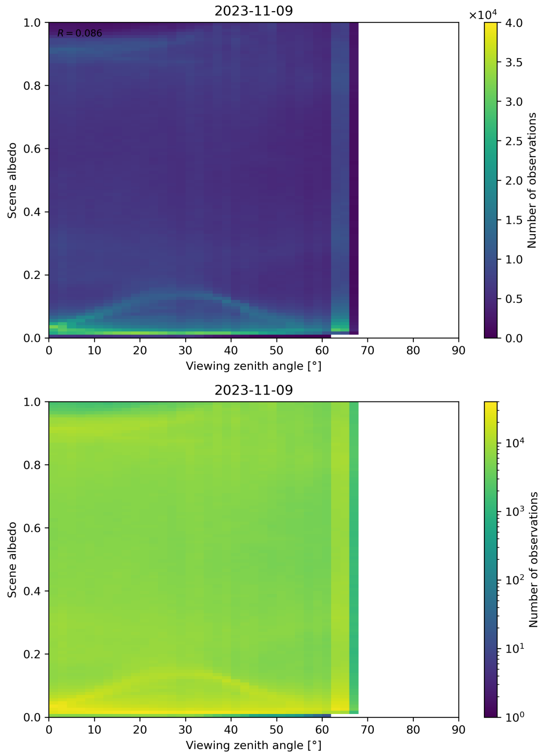
Figure 138: Scatter density plot of “Viewing zenith angle” against “Scene albedo” for 2023-11-08 to 2023-11-10.
