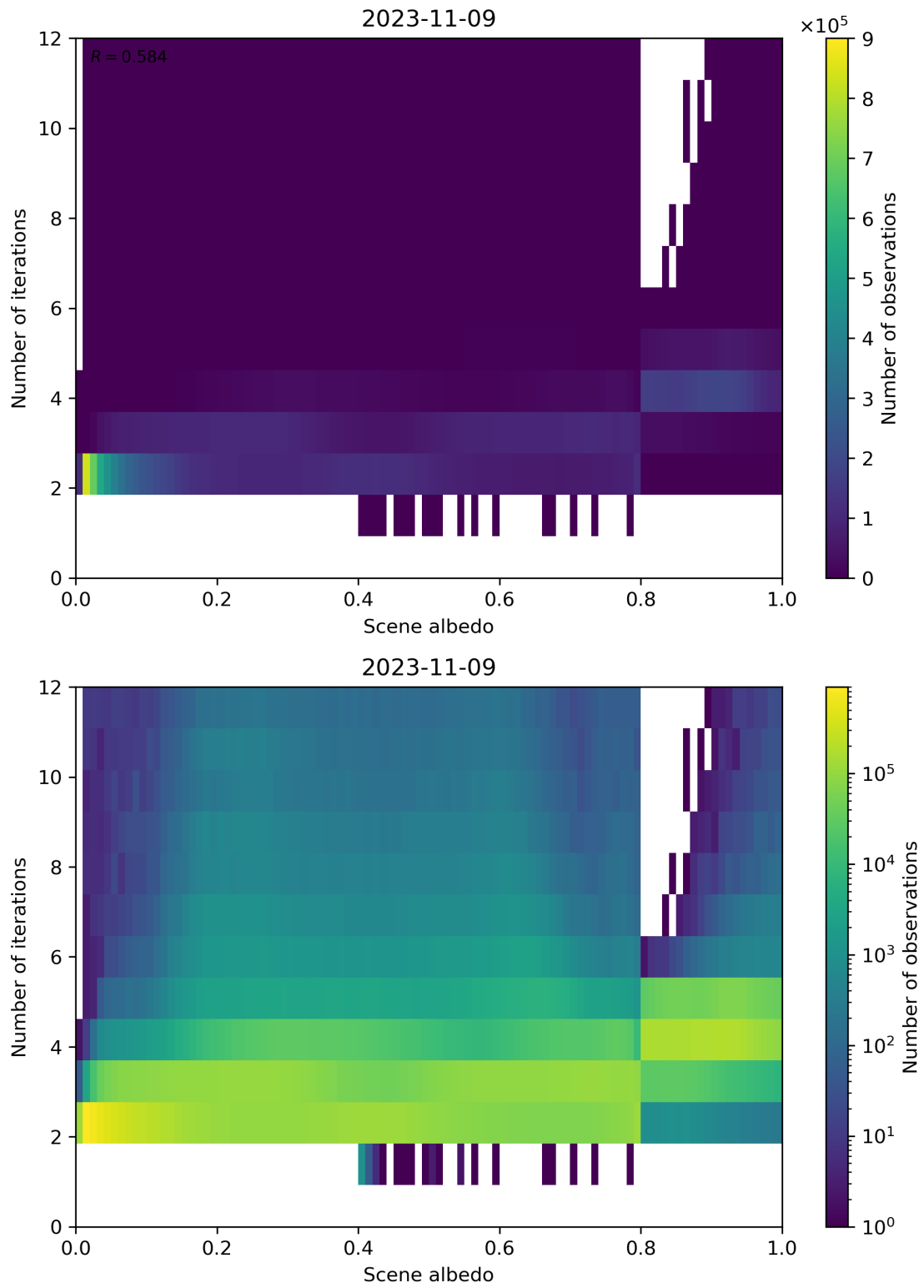
Figure 115: Scatter density plot of “Scene albedo” against “Number of iterations” for 2023-11-08 to 2023-11-10.
