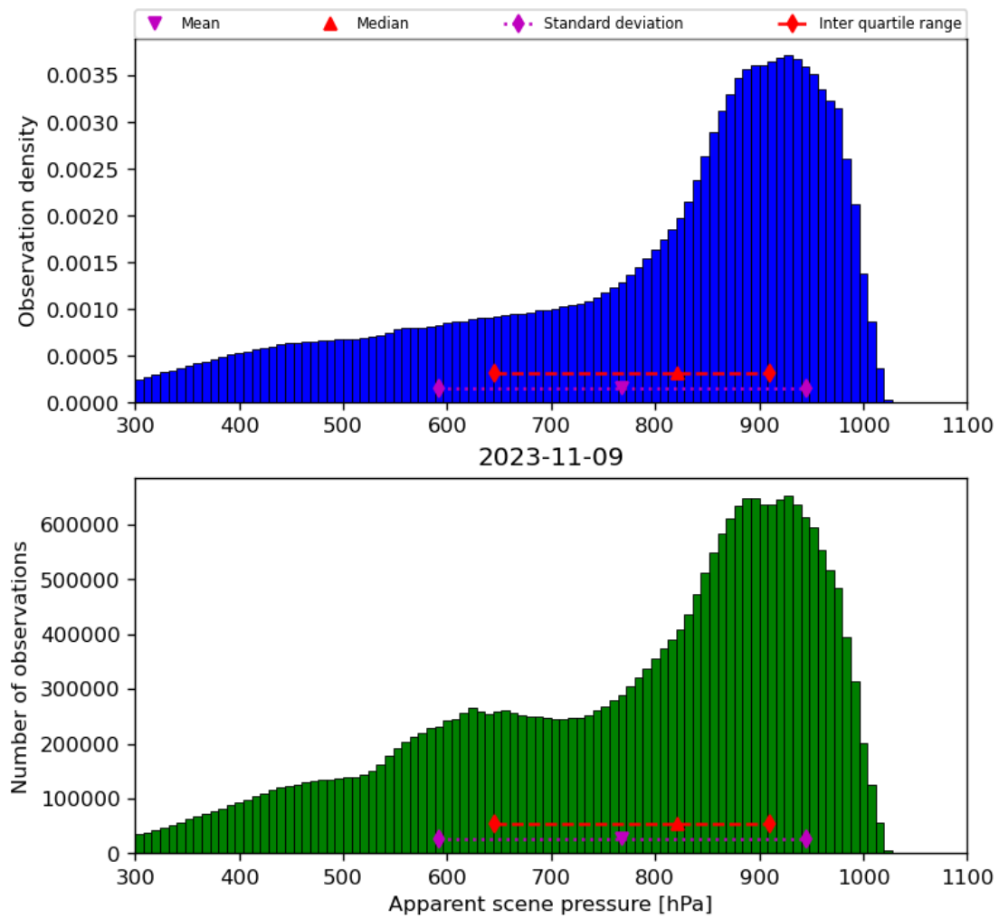
Figure 36: Histogram of “Apparent scene pressure” for 2023-11-08 to 2023-11-10
