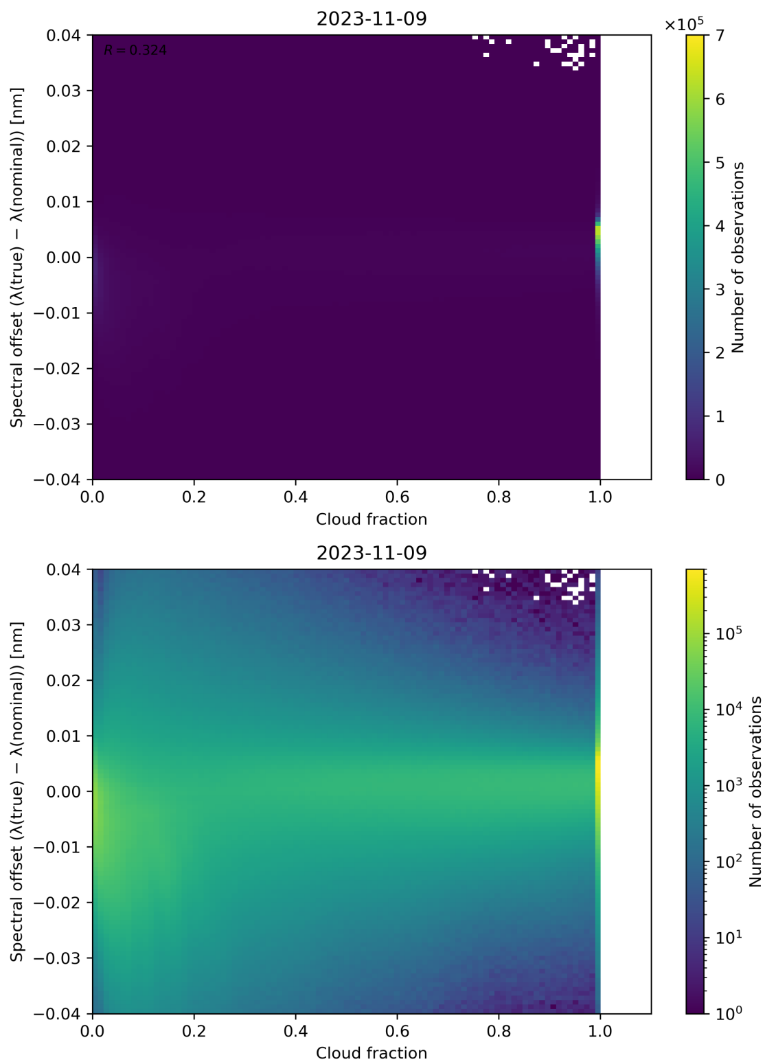
Figure 83: Scatter density plot of “Cloud fraction” against “Spectral offset ( \lambda(\text{true}) - \lambda(\text{nominal}) )” for 2023-11-08 to 2023-11-10.
