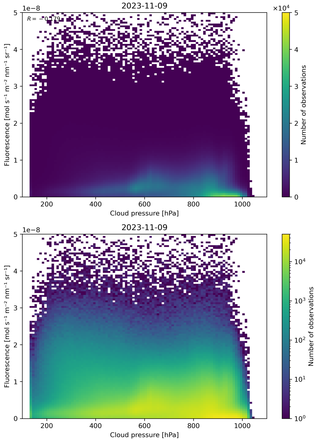
Figure 88: Scatter density plot of “Cloud pressure” against “Fluorescence” for 2023-11-08 to 2023-11-10.
