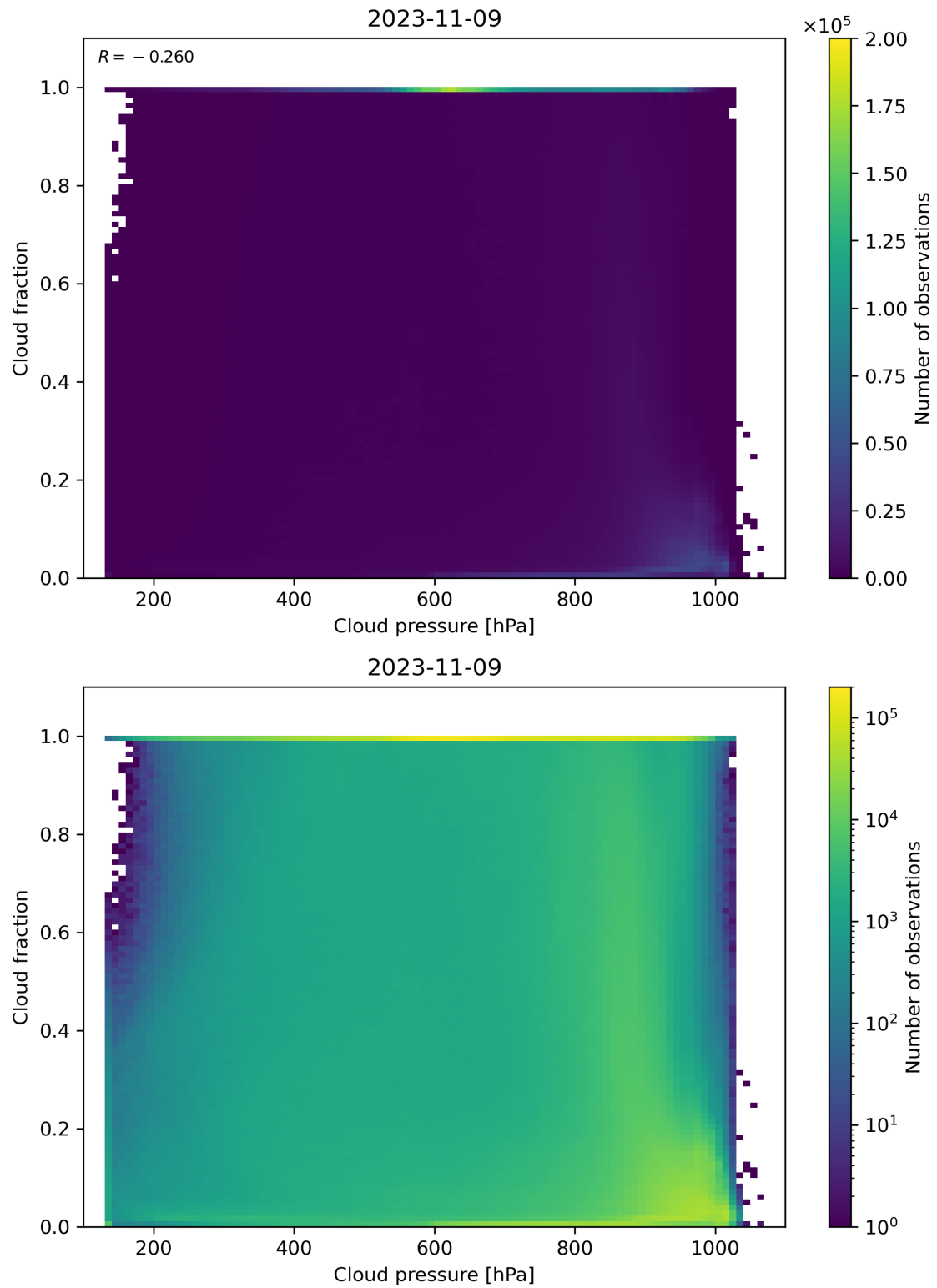
Figure 87: Scatter density plot of “Cloud pressure” against “Cloud fraction” for 2023-11-08 to 2023-11-10.
