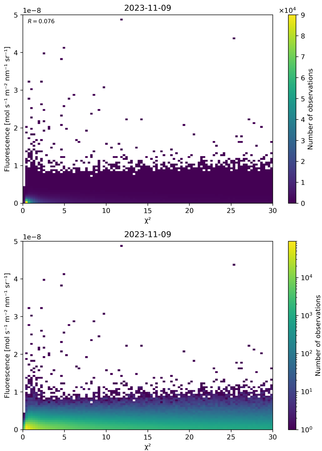
Figure 70: Scatter density plot of “ \chi^2 ” against “Fluorescence” for 2023-11-08 to 2023-11-10.
