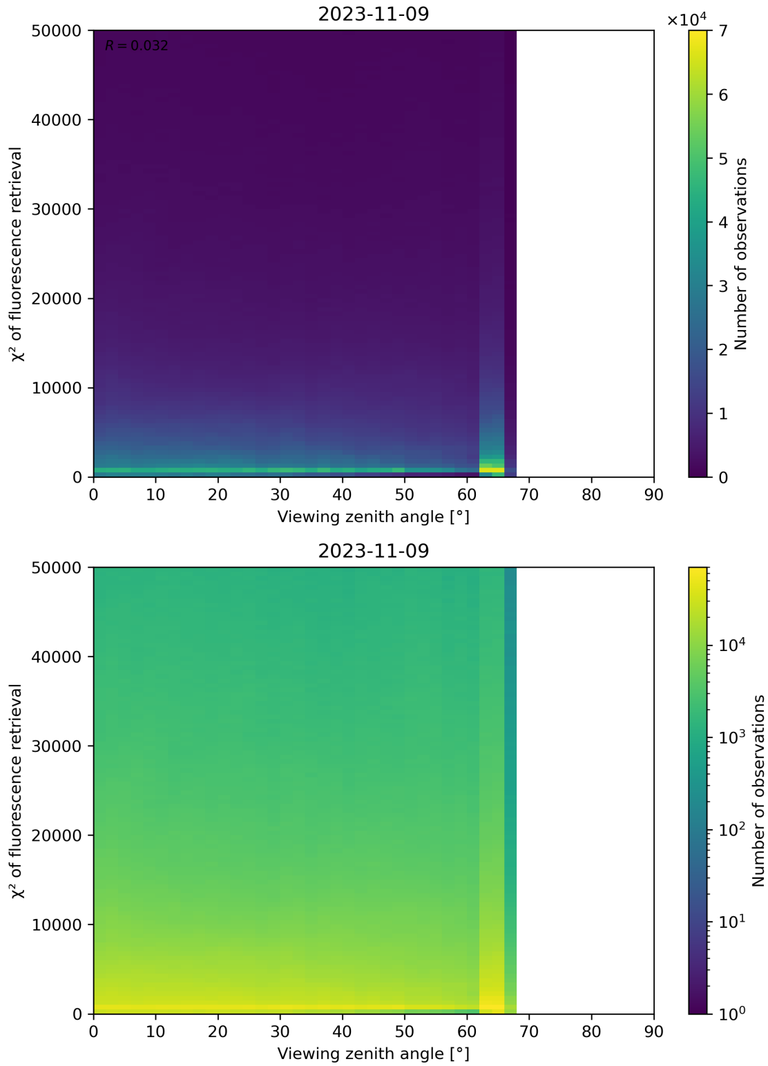
Figure 131: Scatter density plot of “Viewing zenith angle” against “ \chi^2 of fluorescence retrieval” for 2023-11-08 to 2023-11-10.
