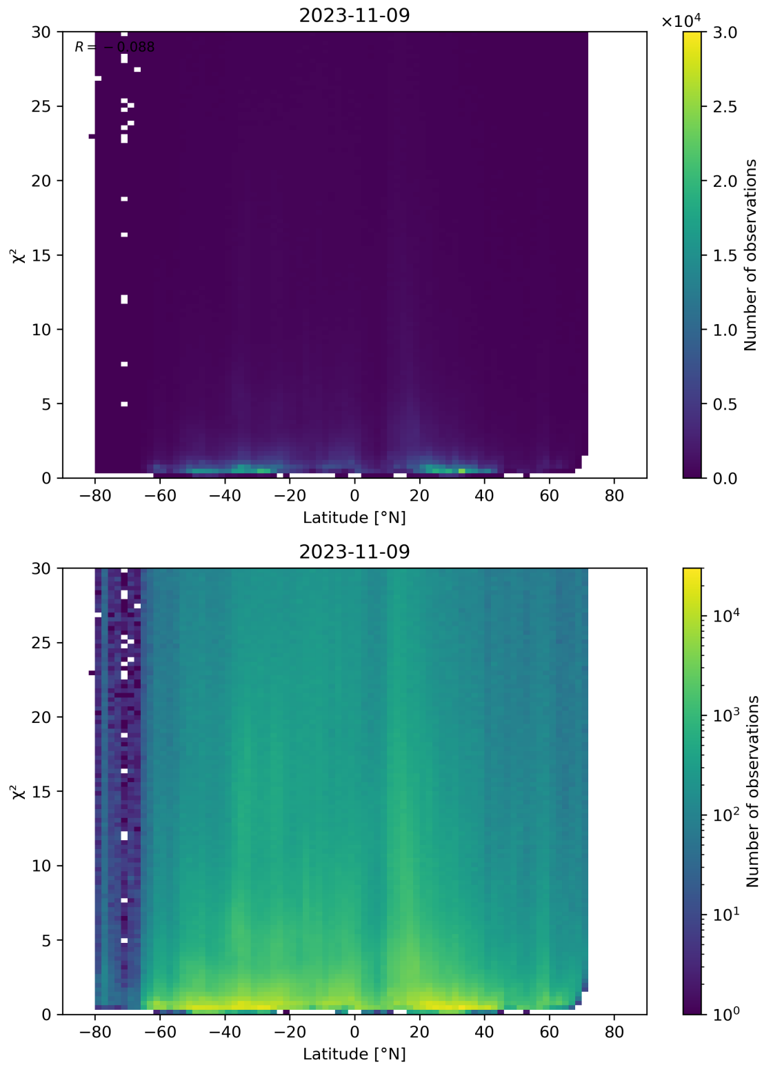
Figure 97: Scatter density plot of “Latitude” against “ \chi^2 ” for 2023-11-08 to 2023-11-10.
