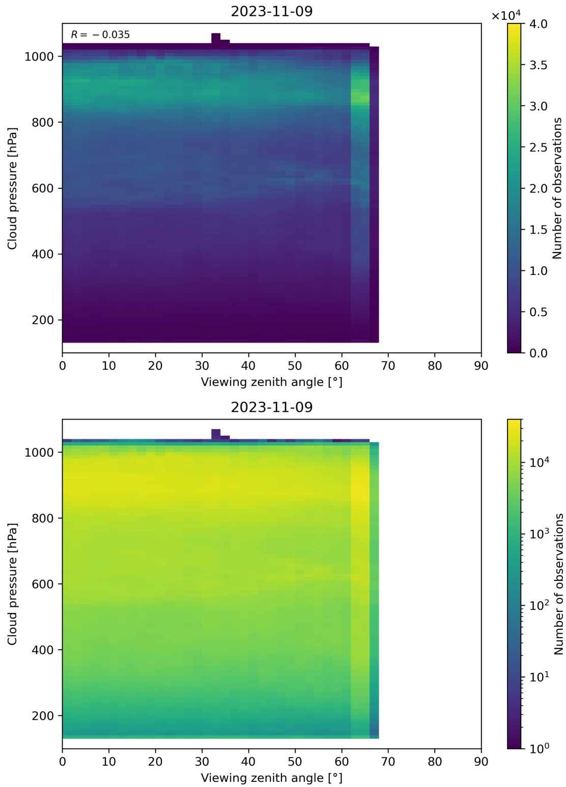
Figure 133: Scatter density plot of “Viewing zenith angle” against “Cloud pressure” for 2023-11-08 to 2023-11-10.
