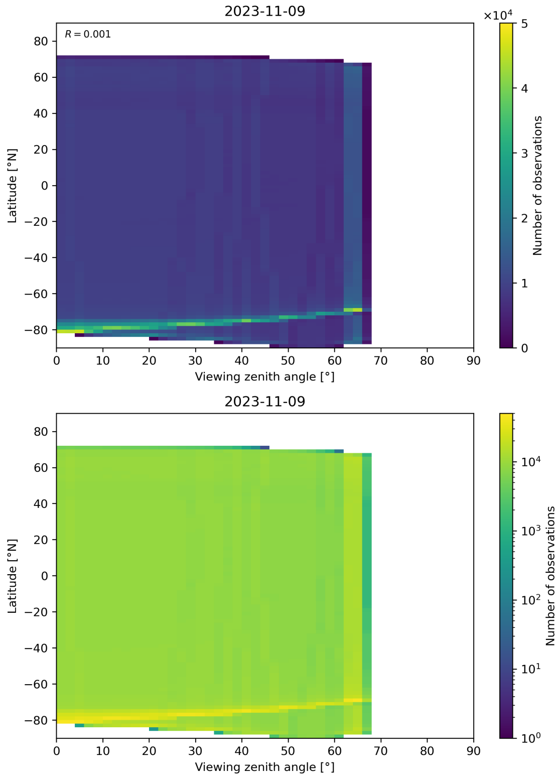
Figure 135: Scatter density plot of “Viewing zenith angle” against “Latitude” for 2023-11-08 to 2023-11-10.
