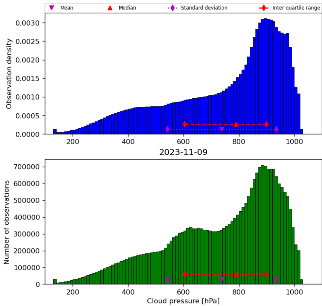
Figure 30: Histogram of “Cloud pressure” for 2023-11-08 to 2023-11-10
