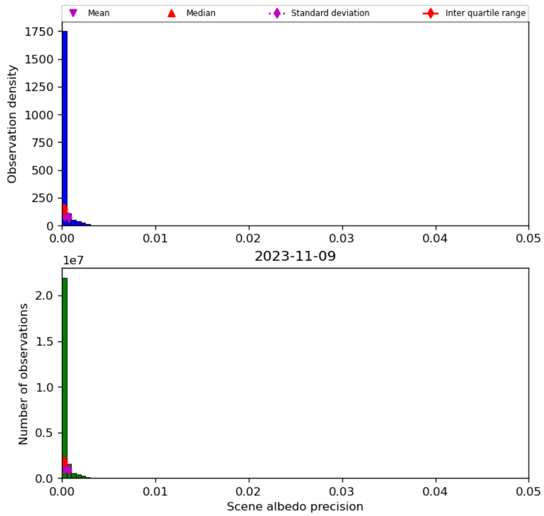
Figure 35: Histogram of “Scene albedo precision” for 2023-11-08 to 2023-11-10
