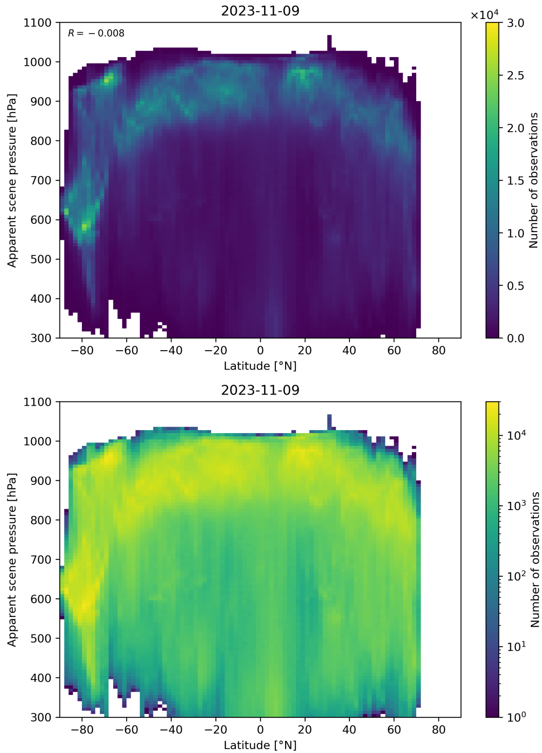
Figure 96: Scatter density plot of “Latitude” against “Apparent scene pressure” for 2023-11-08 to 2023-11-10.
