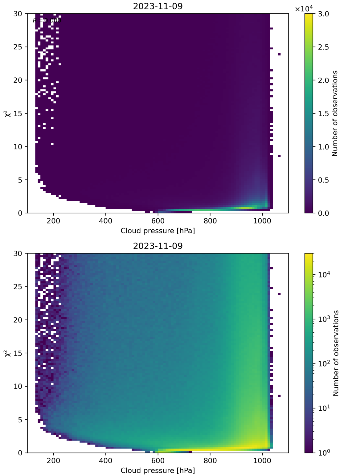
Figure 85: Scatter density plot of “Cloud pressure” against “ \chi^2 ” for 2023-11-08 to 2023-11-10.
