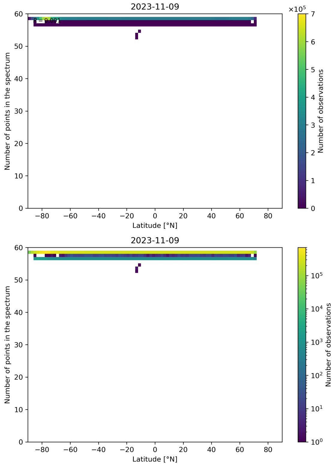
Figure 103: Scatter density plot of “Latitude” against “Number of points in the spectrum” for 2023-11-08 to 2023-11-10.
