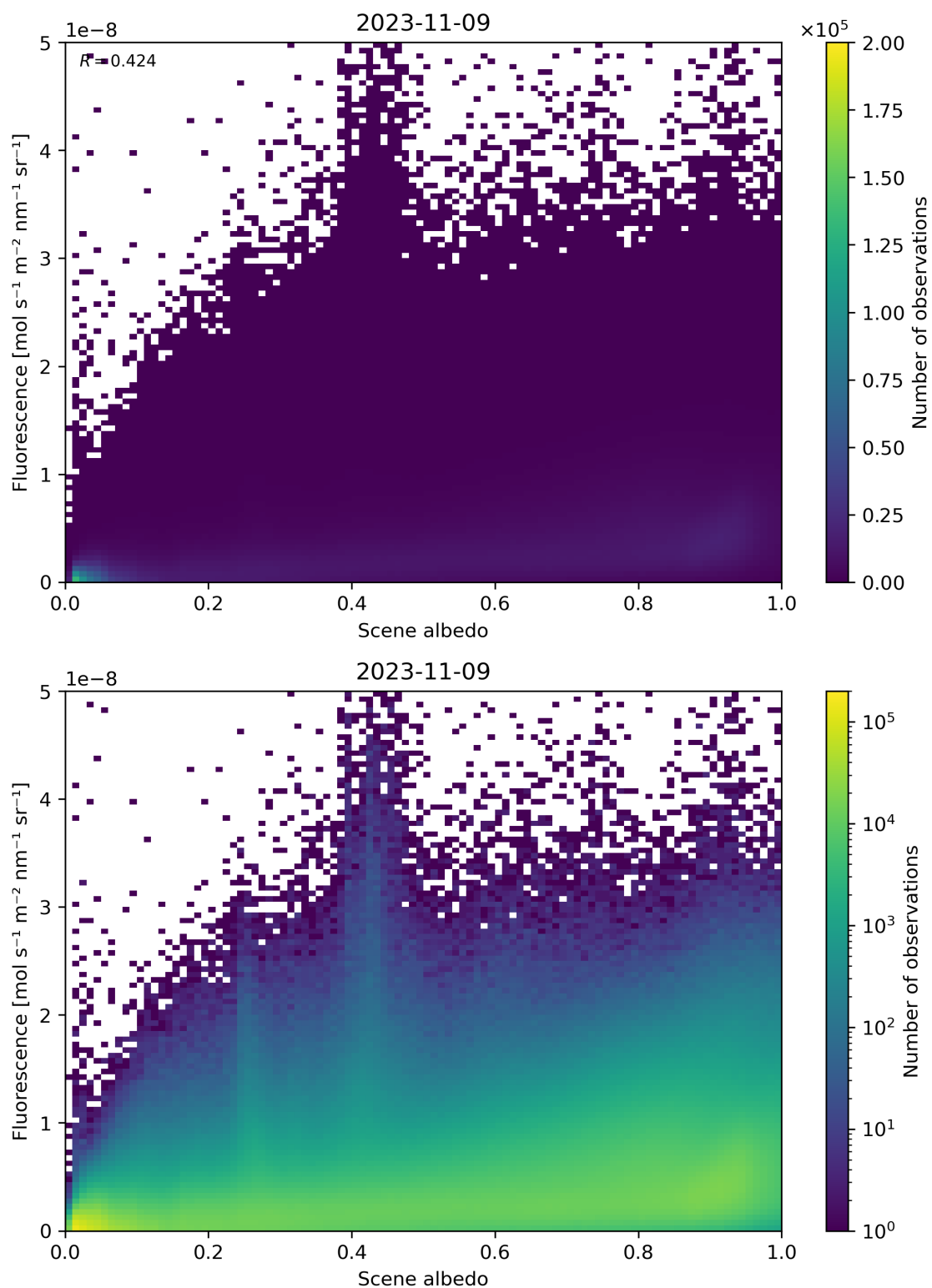
Figure 114: Scatter density plot of “Scene albedo” against “Fluorescence” for 2023-11-08 to 2023-11-10.
