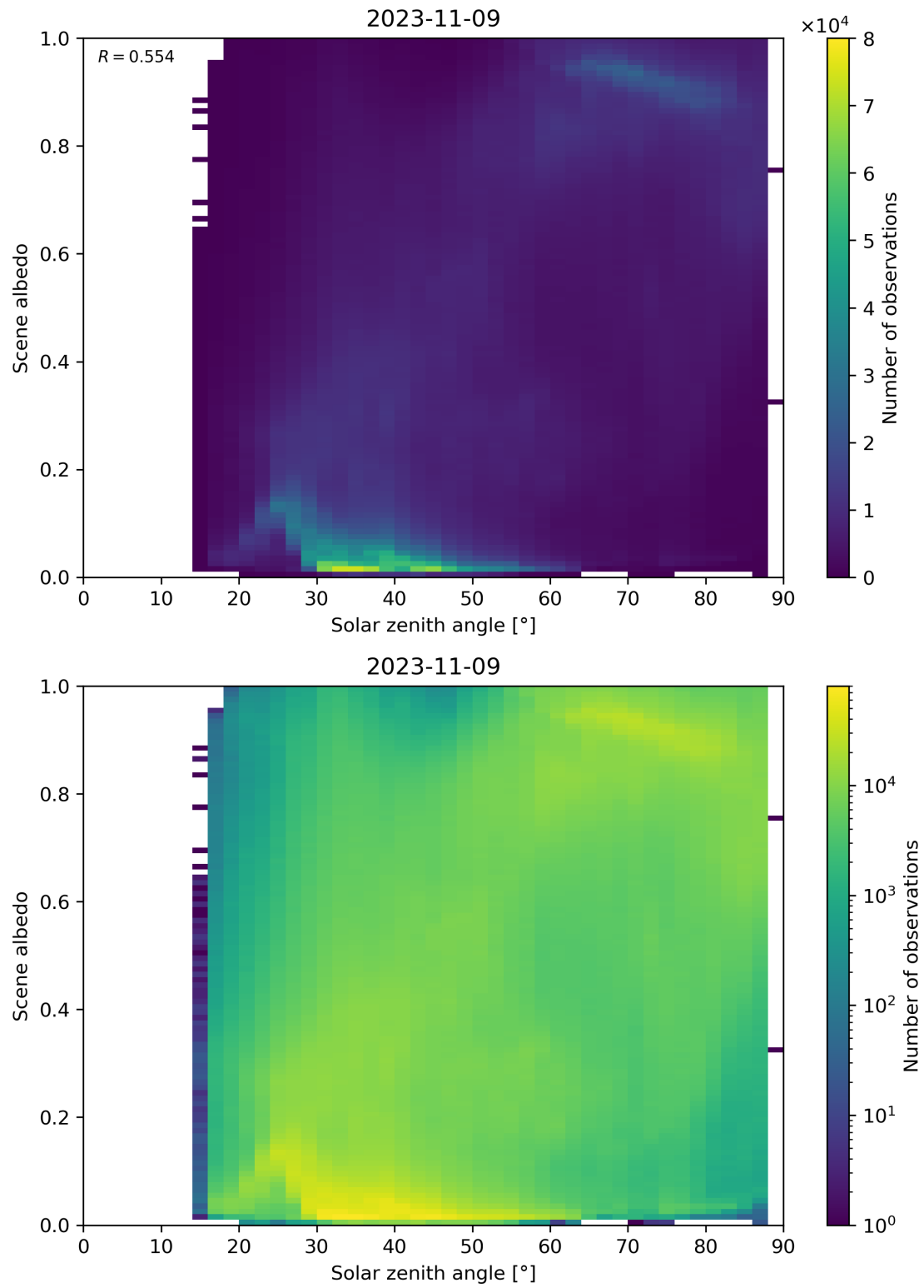
Figure 127: Scatter density plot of “Solar zenith angle” against “Scene albedo” for 2023-11-08 to 2023-11-10.
