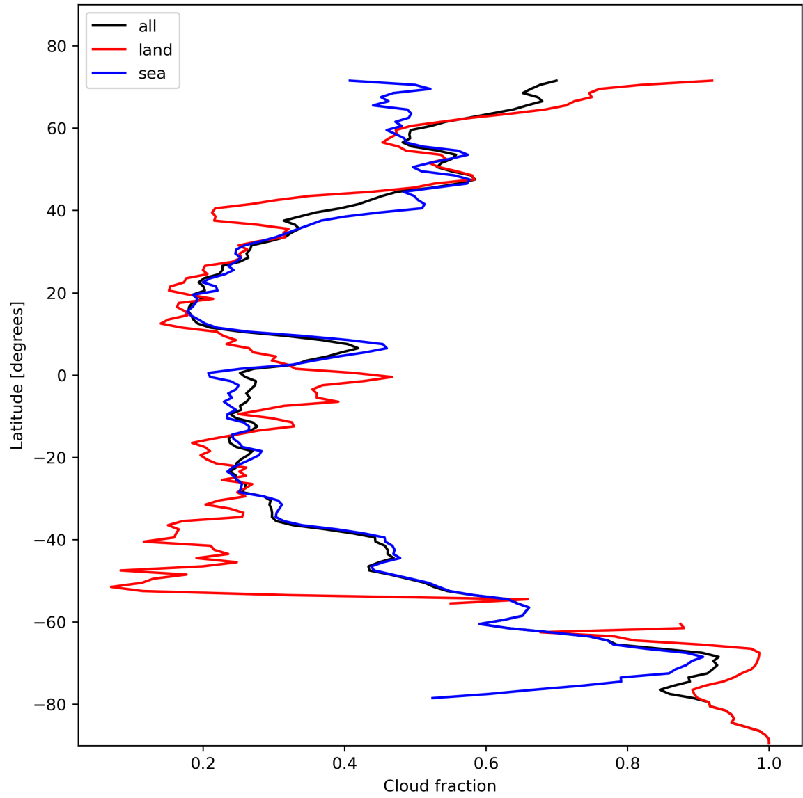
Figure 15: Zonal average of “Cloud fraction” for 2023-11-08 to 2023-11-10.
