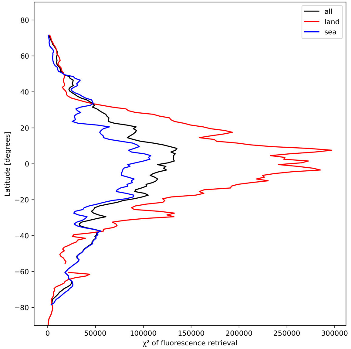
Figure 25: Zonal average of “ \chi^2 of fluorescence retrieval” for 2023-11-08 to 2023-11-10.
