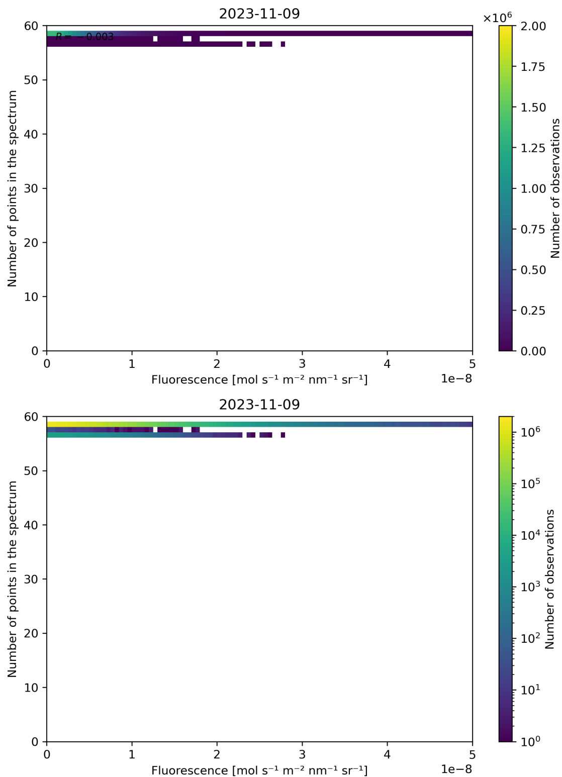
Figure 94: Scatter density plot of “Fluorescence” against “Number of points in the spectrum” for 2023-11-08 to 2023-11-10.
