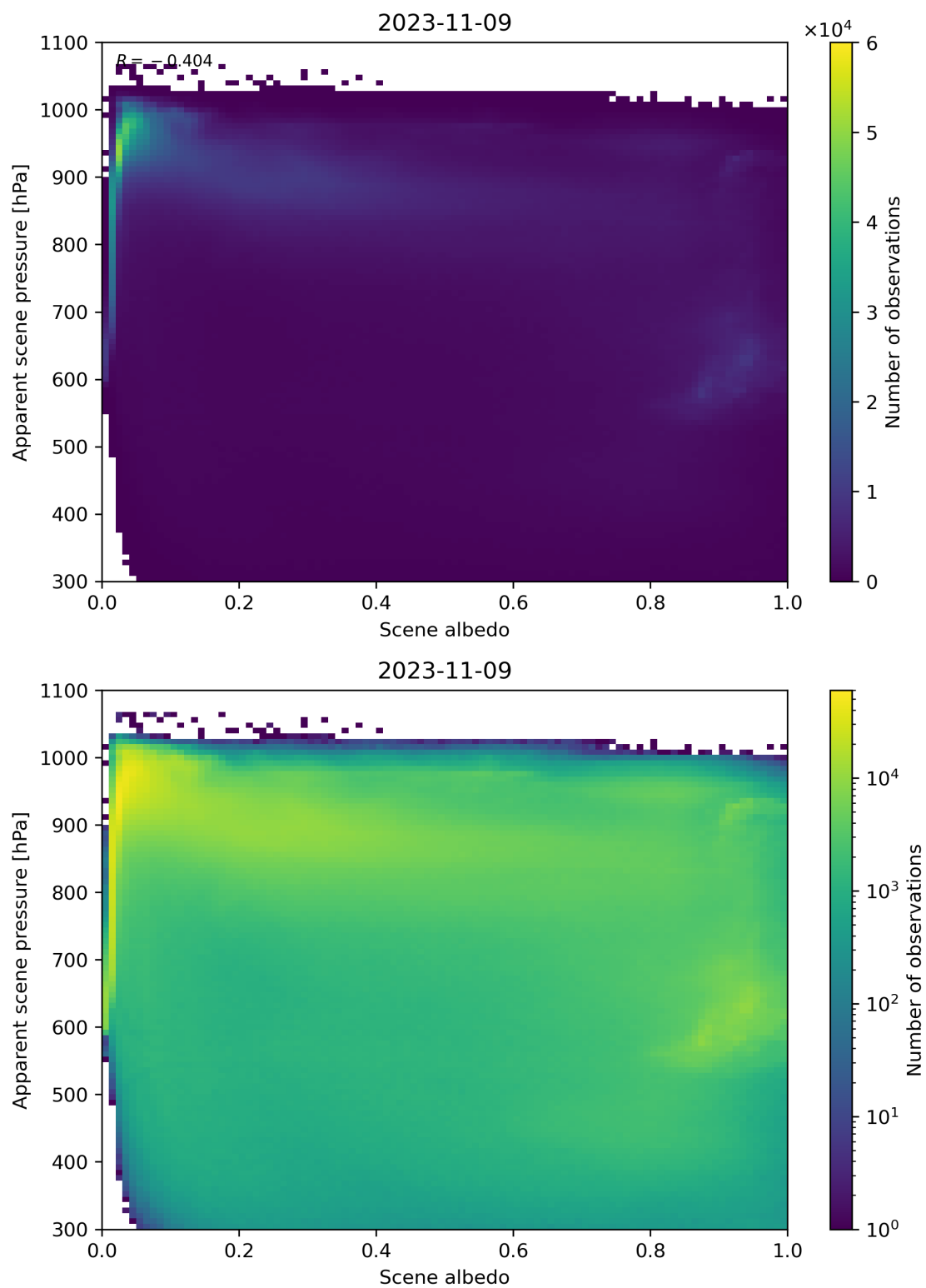
Figure 111: Scatter density plot of “Scene albedo” against “Apparent scene pressure” for 2023-11-08 to 2023-11-10.
