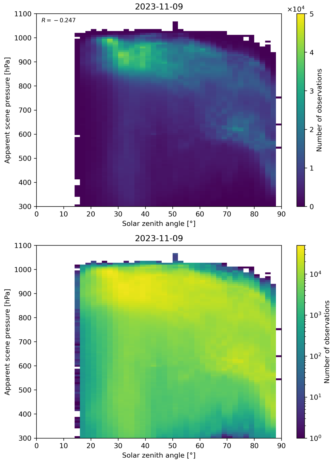
Figure 118: Scatter density plot of “Solar zenith angle” against “Apparent scene pressure” for 2023-11-08 to 2023-11-10.
