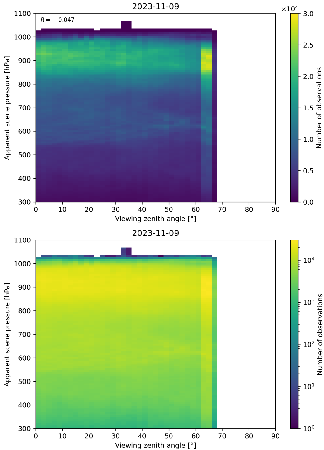
Figure 129: Scatter density plot of “Viewing zenith angle” against “Apparent scene pressure” for 2023-11-08 to 2023-11-10.
