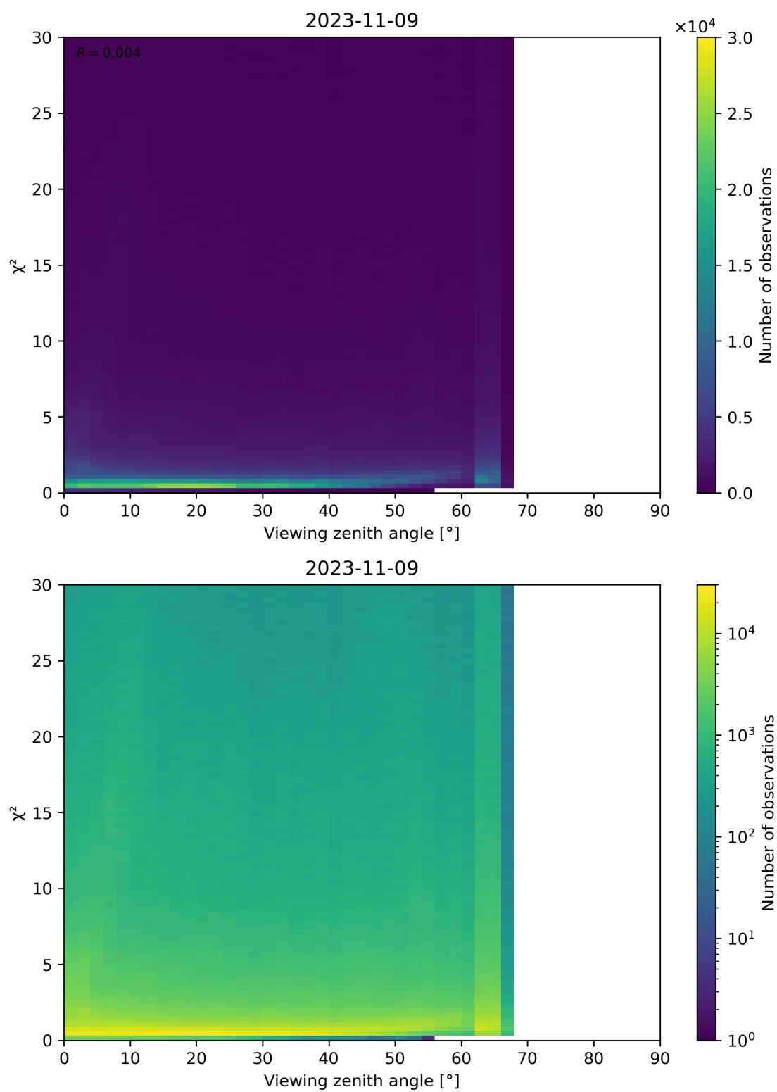
Figure 130: Scatter density plot of “Viewing zenith angle” against “ \chi^2 ” for 2023-11-08 to 2023-11-10.
