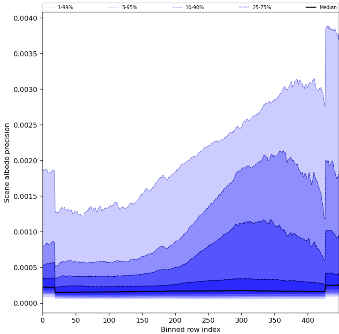
Figure 52: Along track statistics of “Scene albedo precision” for 2023-11-08 to 2023-11-10
