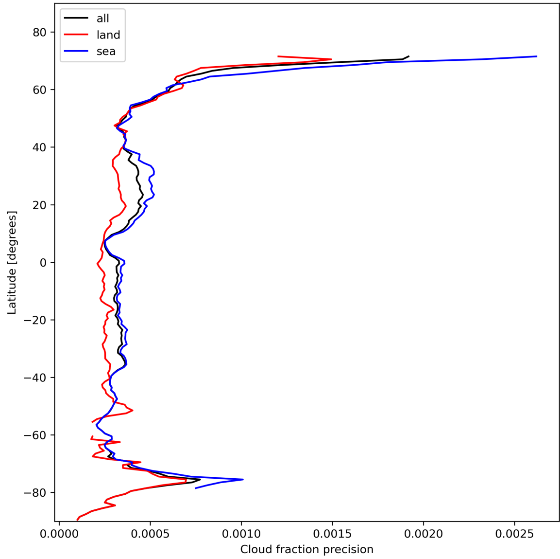
Figure 16: Zonal average of “Cloud fraction precision” for 2023-11-08 to 2023-11-10.
