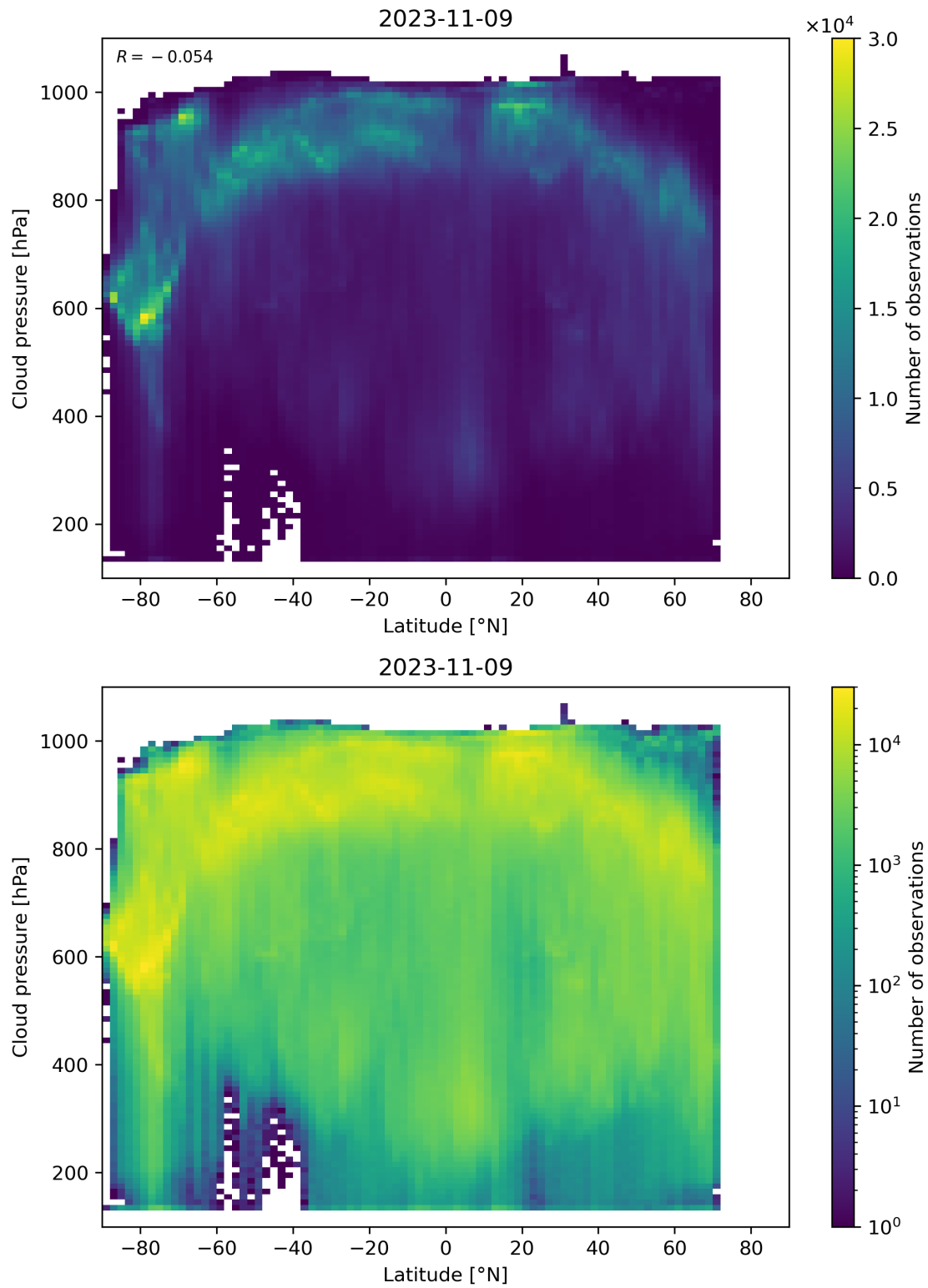
Figure 100: Scatter density plot of “Latitude” against “Cloud pressure” for 2023-11-08 to 2023-11-10.
