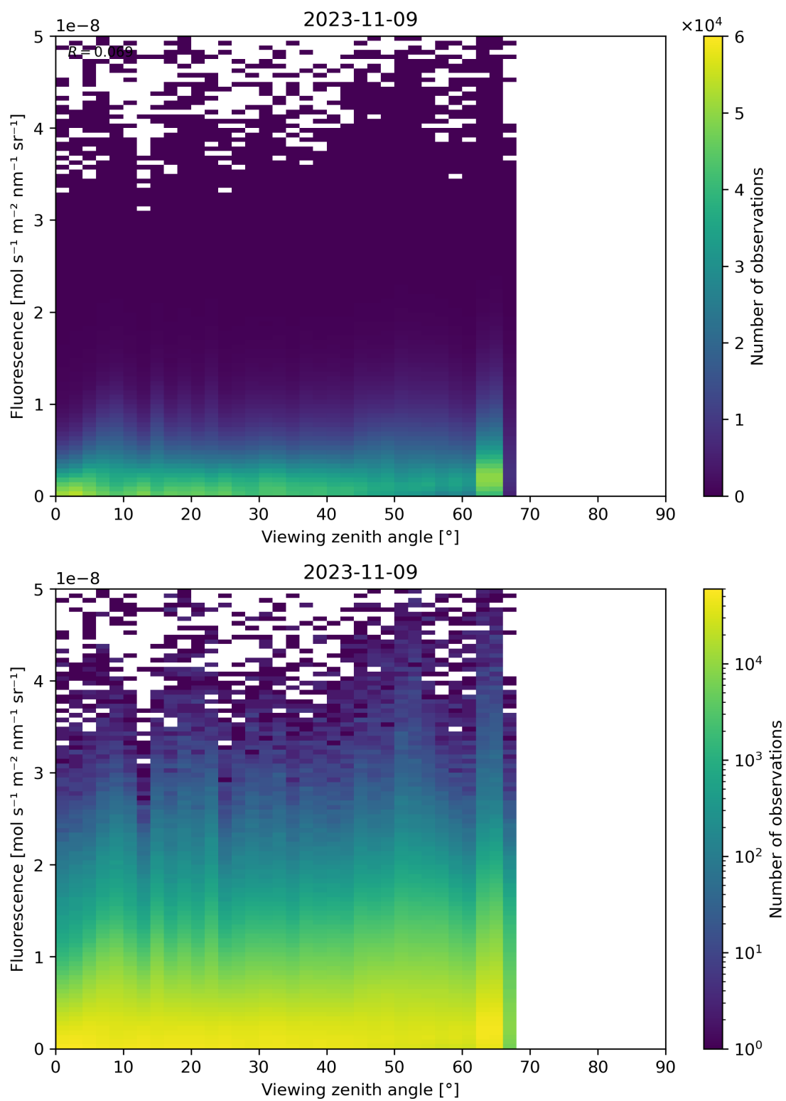
Figure 134: Scatter density plot of “Viewing zenith angle” against “Fluorescence” for 2023-11-08 to 2023-11-10.
