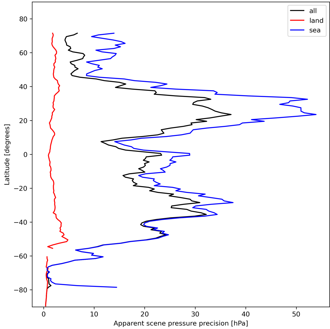
Figure 20: Zonal average of “Apparent scene pressure precision” for 2023-11-08 to 2023-11-10.
