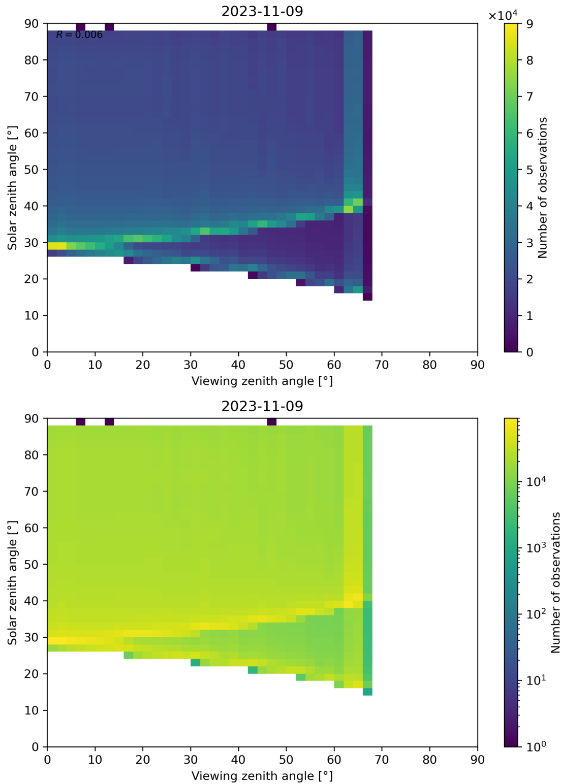
Figure 139: Scatter density plot of “Viewing zenith angle” against “Solar zenith angle” for 2023-11-08 to 2023-11-10.
