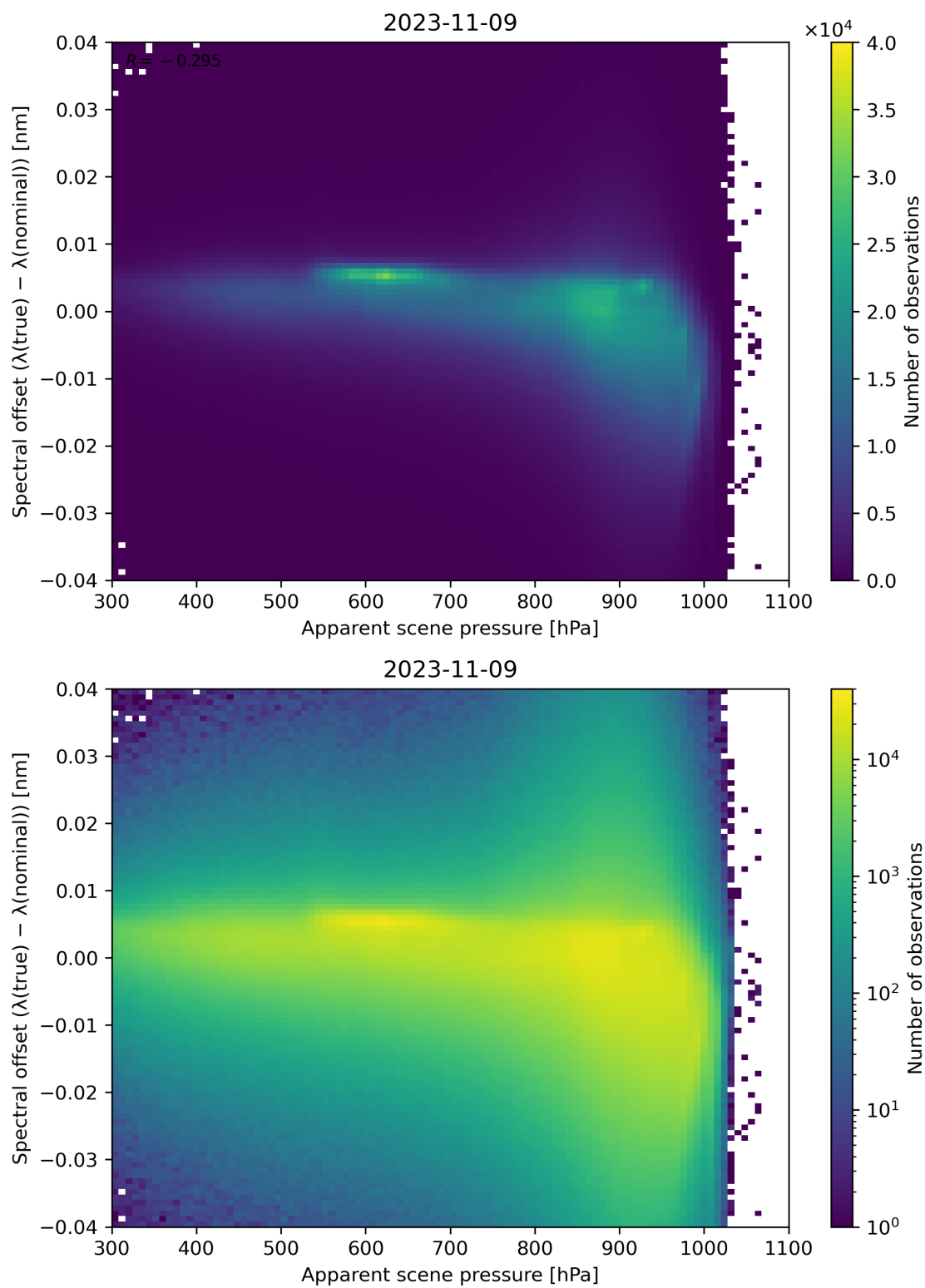
Figure 68: Scatter density plot of “Apparent scene pressure” against “Spectral offset ( \lambda(\text{true}) - \lambda(\text{nominal}) )” for 2023-11-08 to 2023-11-10.
