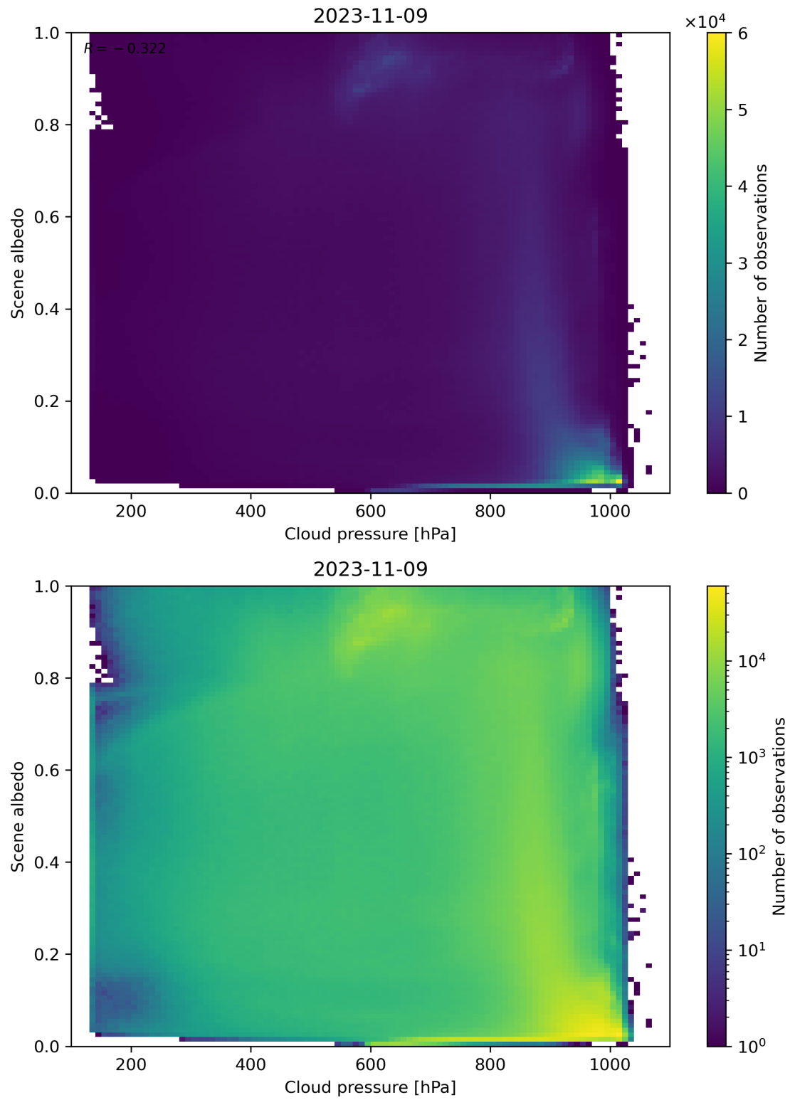
Figure 91: Scatter density plot of “Cloud pressure” against “Scene albedo” for 2023-11-08 to 2023-11-10.
