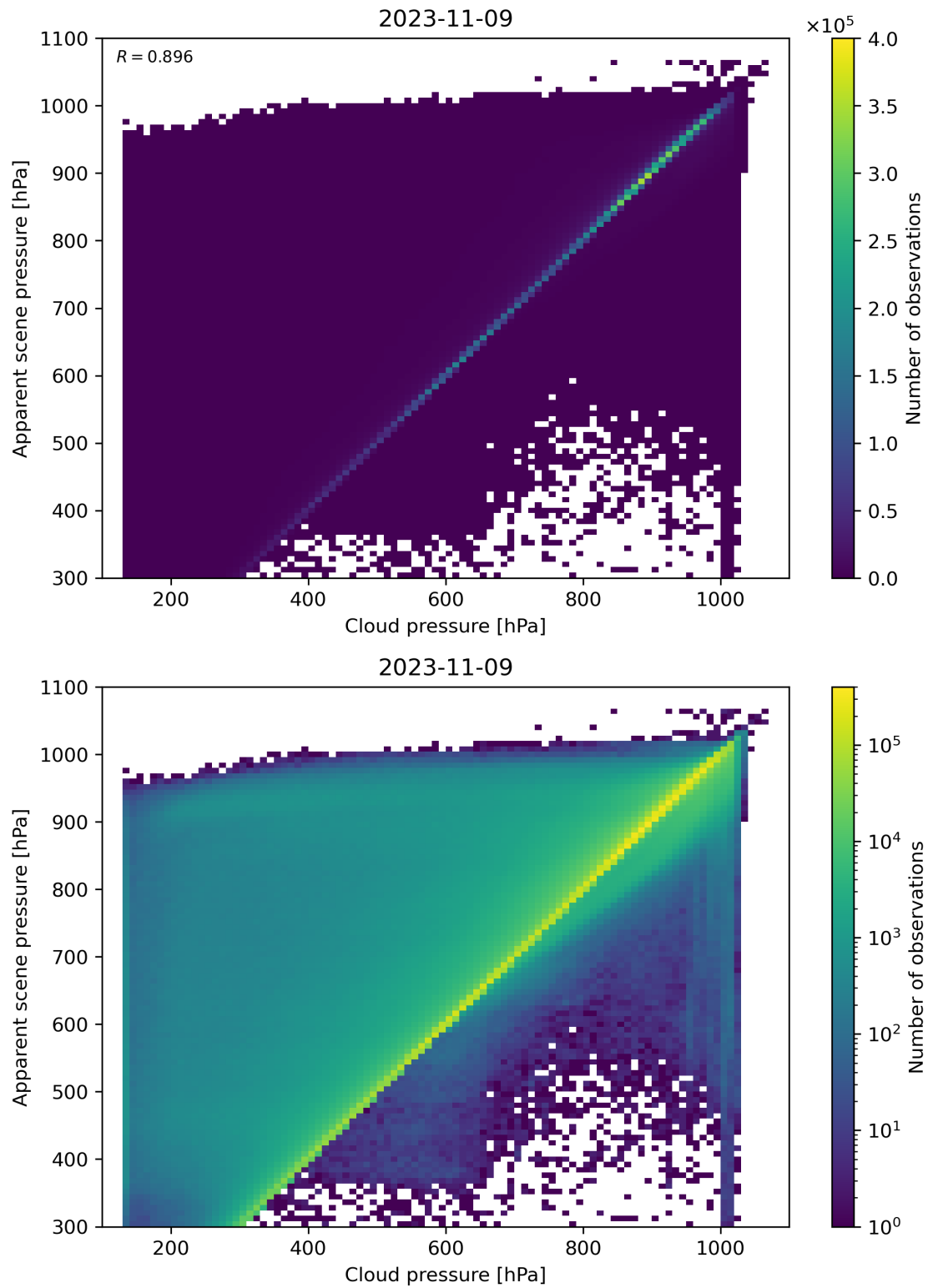
Figure 84: Scatter density plot of “Cloud pressure” against “Apparent scene pressure” for 2023-11-08 to 2023-11-10.
