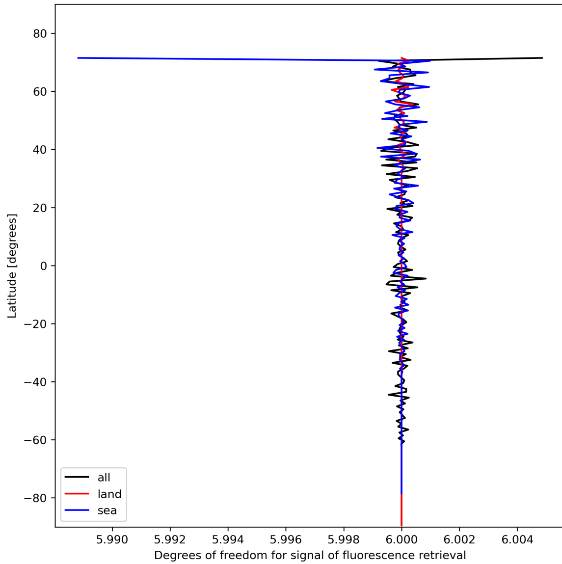
Figure 26: Zonal average of “Degrees of freedom for signal of fluorescence retrieval” for 2023-11-08 to 2023-11-10.
