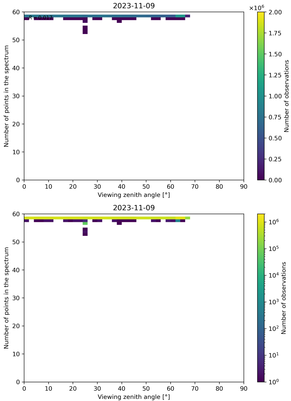
Figure 137: Scatter density plot of “Viewing zenith angle” against “Number of points in the spectrum” for 2023-11-08 to 2023-11-10.
