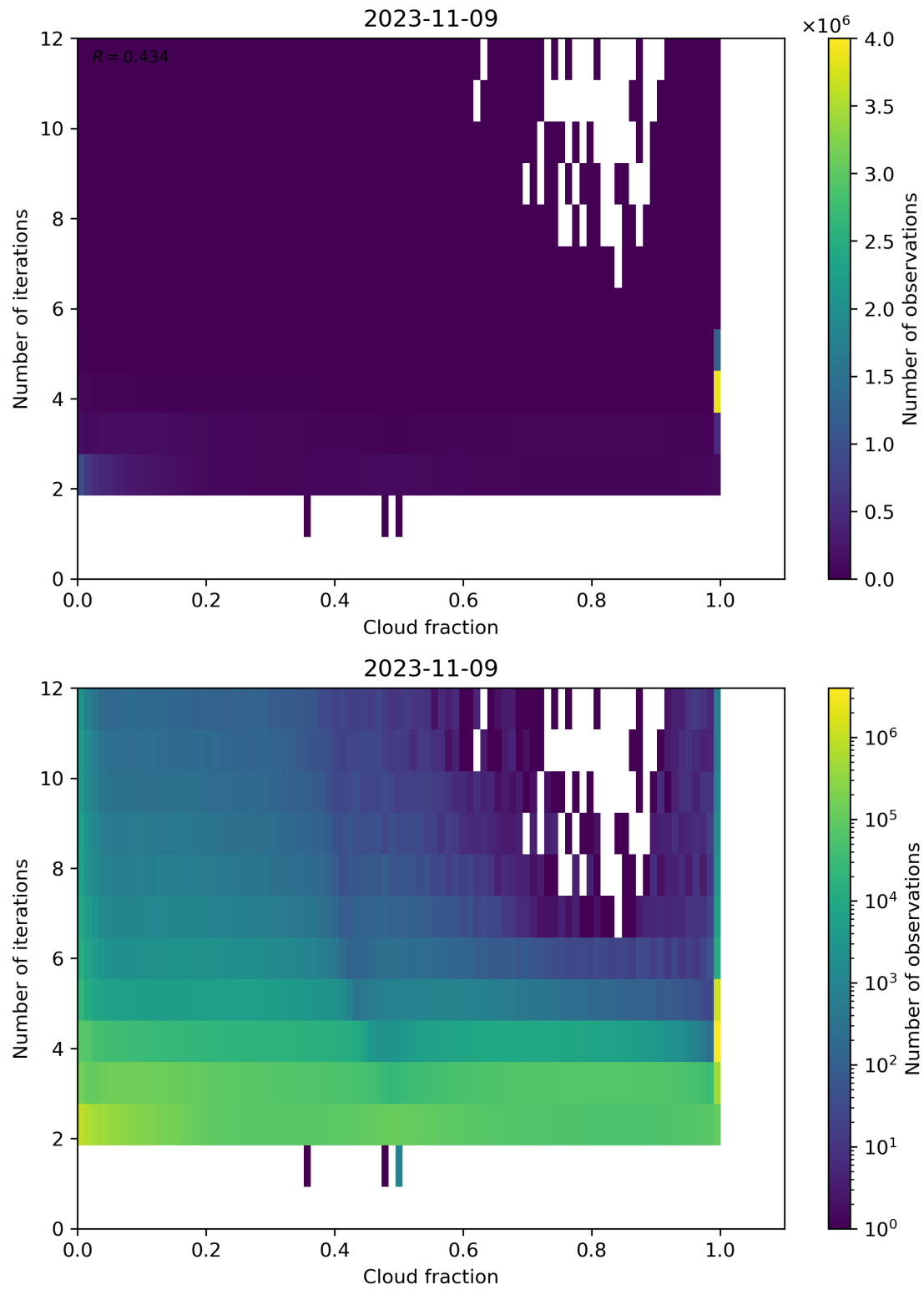
Figure 80: Scatter density plot of “Cloud fraction” against “Number of iterations” for 2023-11-08 to 2023-11-10.
