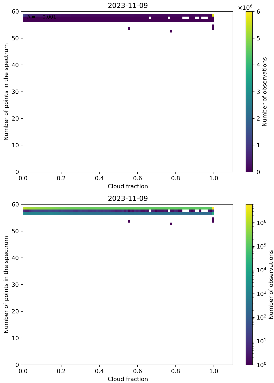
Figure 81: Scatter density plot of “Cloud fraction” against “Number of points in the spectrum” for 2023-11-08 to 2023-11-10.
