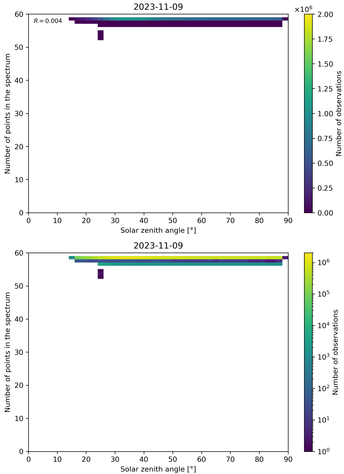
Figure 126: Scatter density plot of “Solar zenith angle” against “Number of points in the spectrum” for 2023-11-08 to 2023-11-10.
