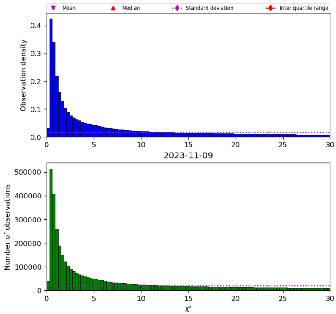
Figure 38: Histogram of “ \chi^2 ” for 2023-11-08 to 2023-11-10
