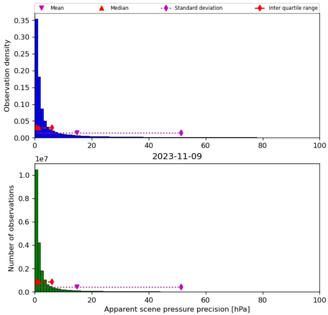
Figure 37: Histogram of “Apparent scene pressure precision” for 2023-11-08 to 2023-11-10
