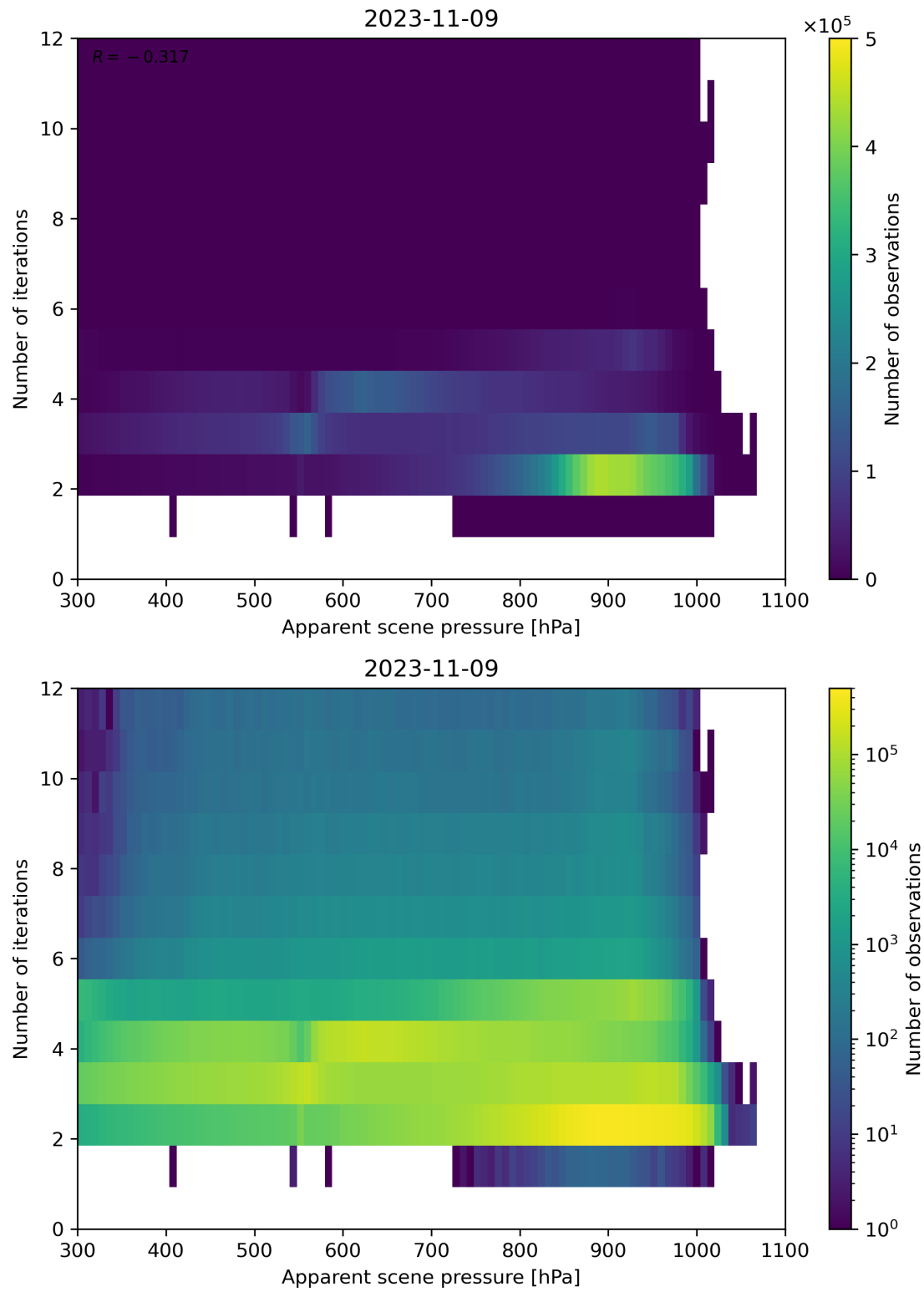
Figure 66: Scatter density plot of “Apparent scene pressure” against “Number of iterations” for 2023-11-08 to 2023-11-10.
