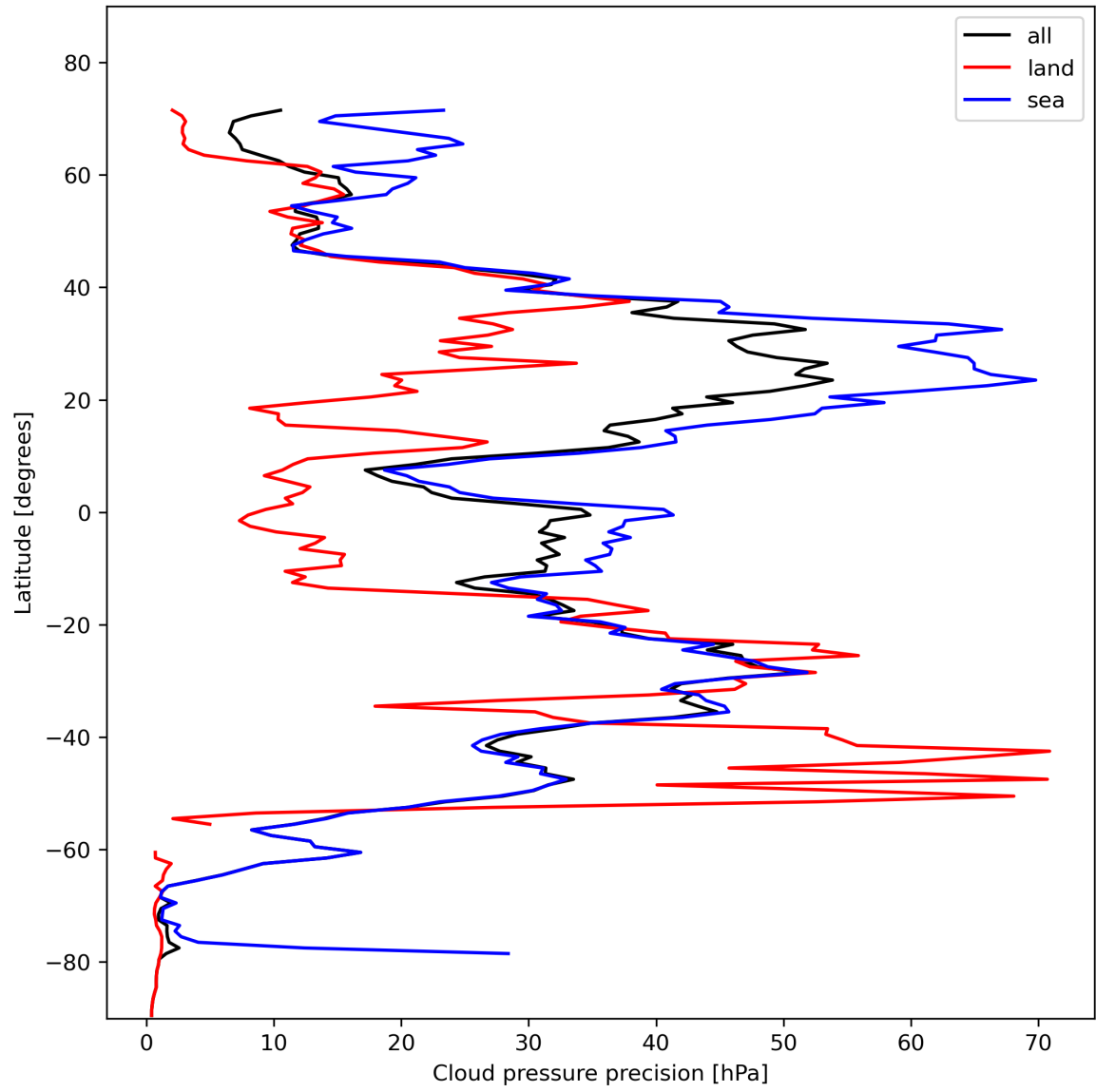
Figure 14: Zonal average of “Cloud pressure precision” for 2023-11-08 to 2023-11-10.
