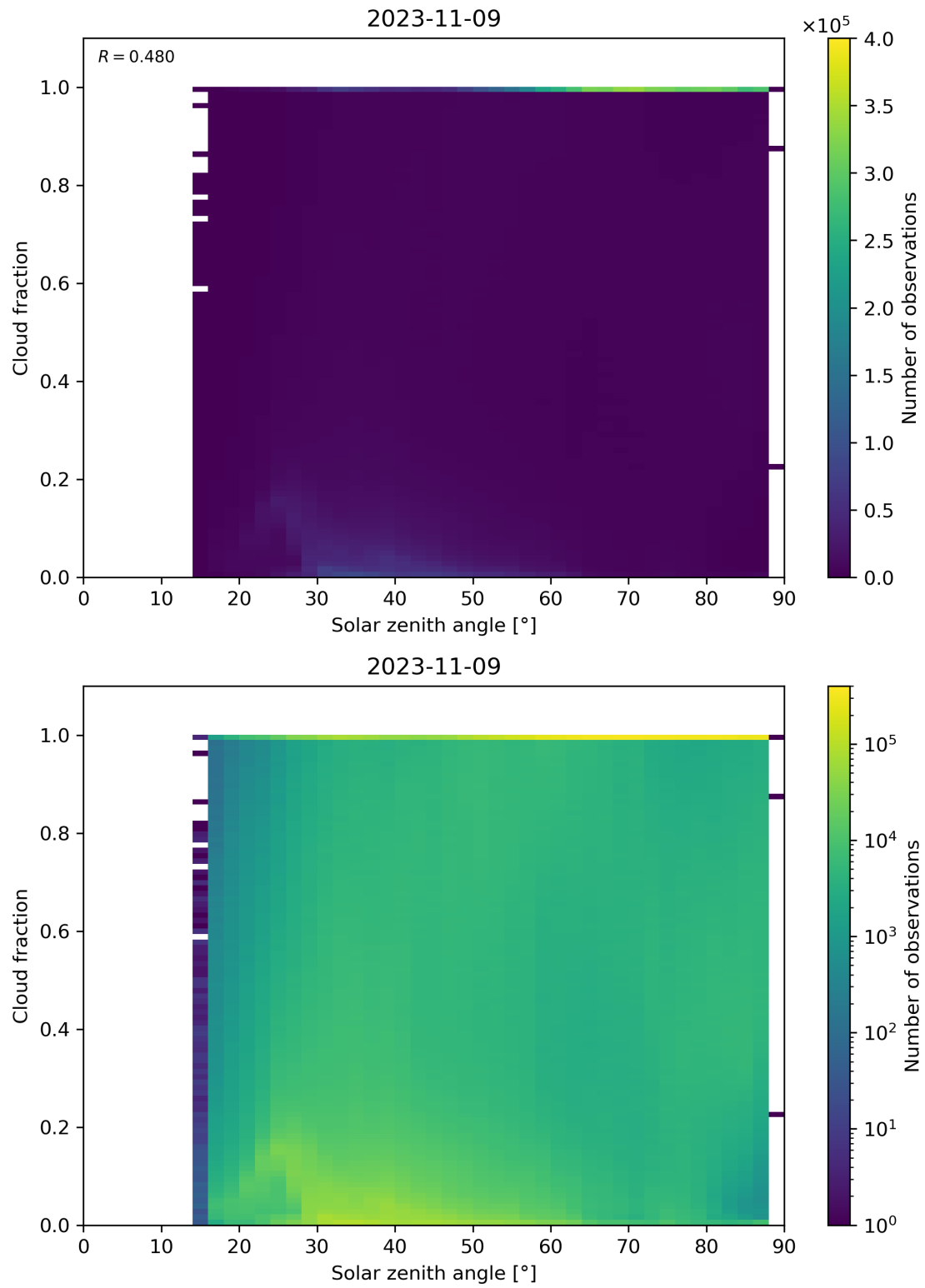
Figure 121: Scatter density plot of “Solar zenith angle” against “Cloud fraction” for 2023-11-08 to 2023-11-10.
