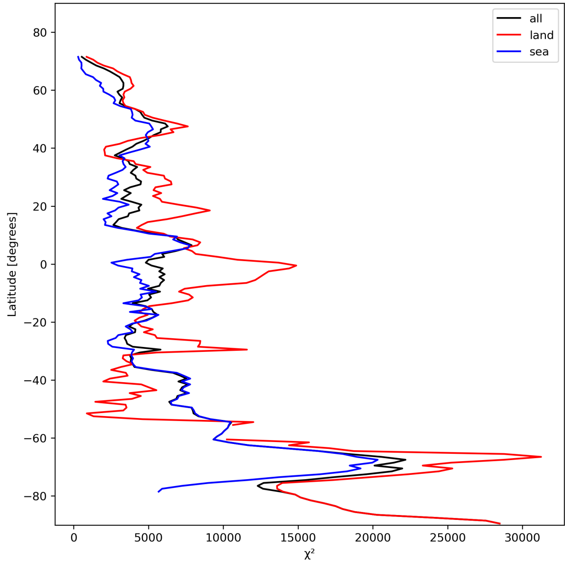
Figure 21: Zonal average of “ \chi^2 ” for 2023-11-08 to 2023-11-10.
