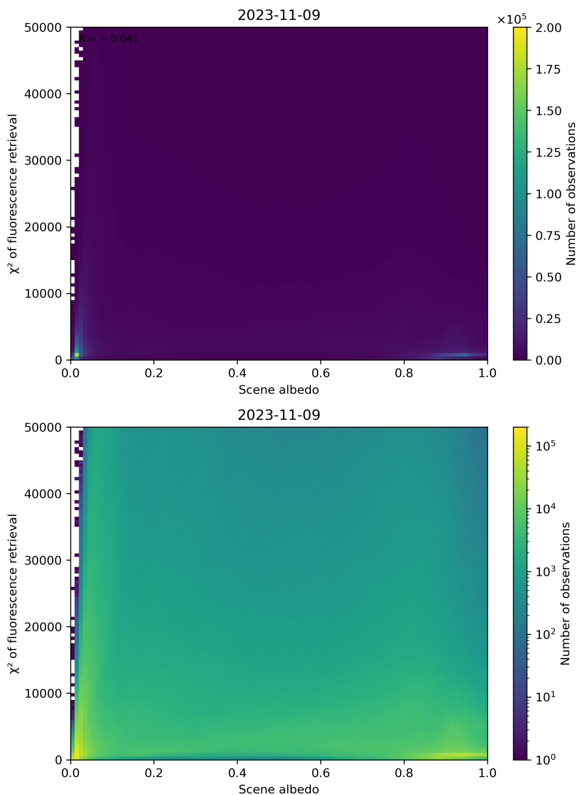
Figure 113: Scatter density plot of “Scene albedo” against “ \chi^2 of fluorescence retrieval” for 2023-11-08 to 2023-11-10.
