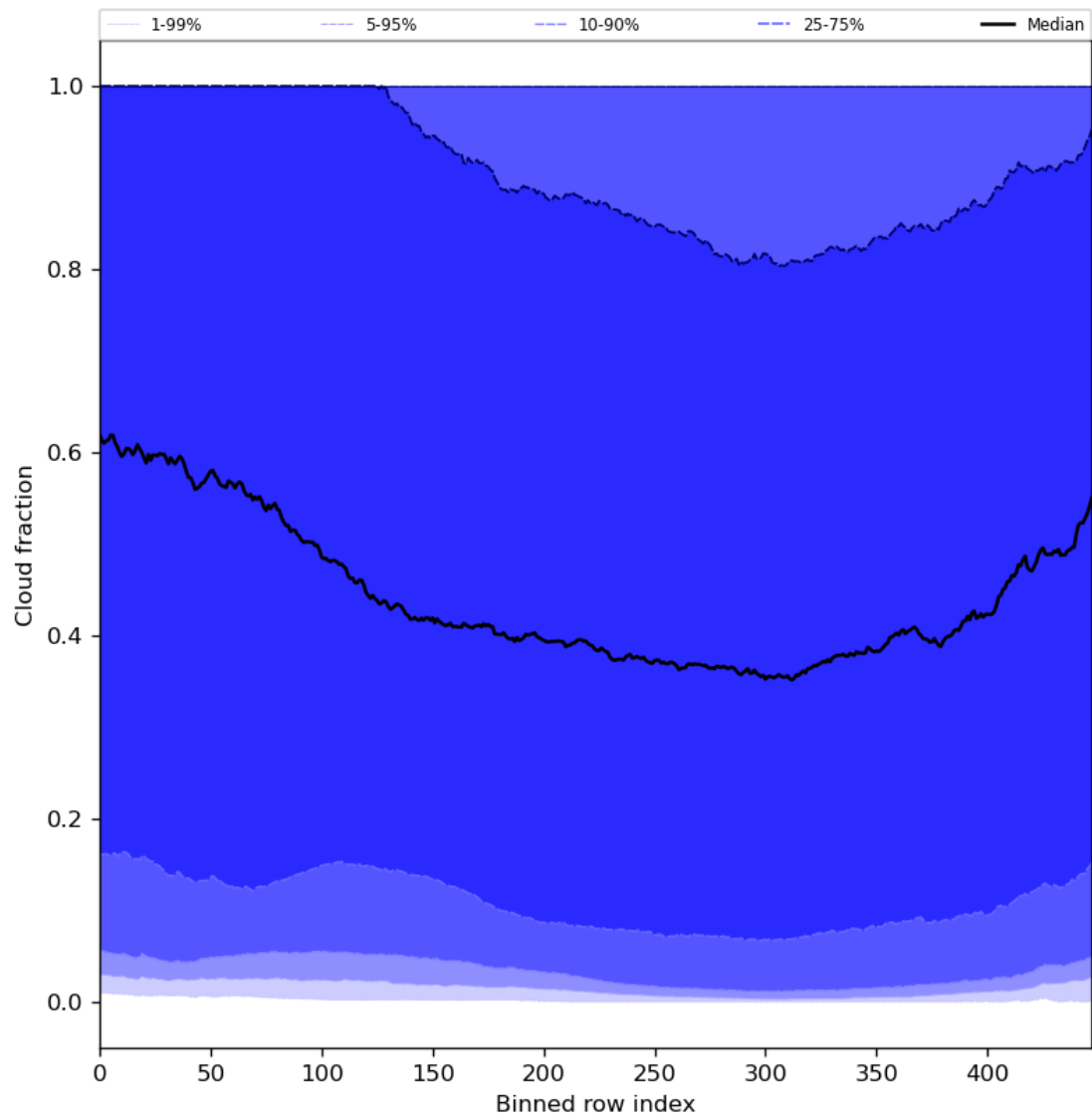
Figure 49: Along track statistics of “Cloud fraction” for 2023-11-08 to 2023-11-10
