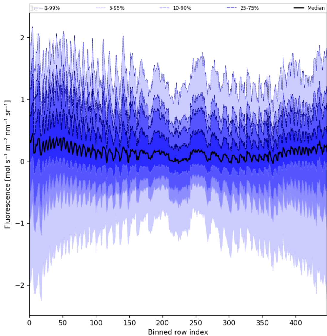
Figure 57: Along track statistics of “Fluorescence” for 2023-11-08 to 2023-11-10
