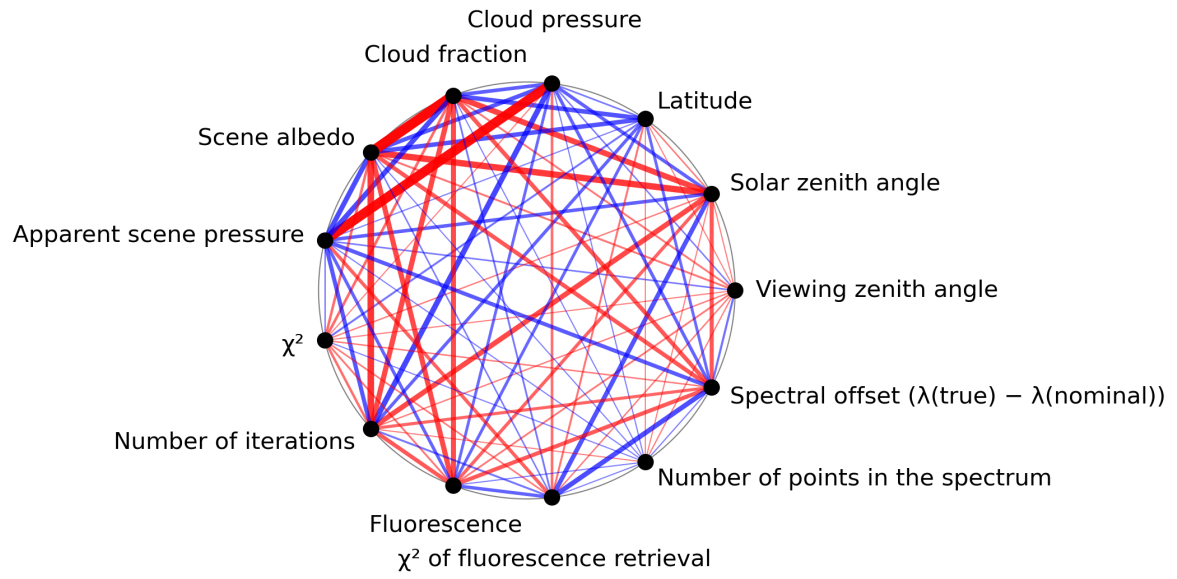
Figure 1: Map of correlation graph for 2023-11-08 to 2023-11-10.
