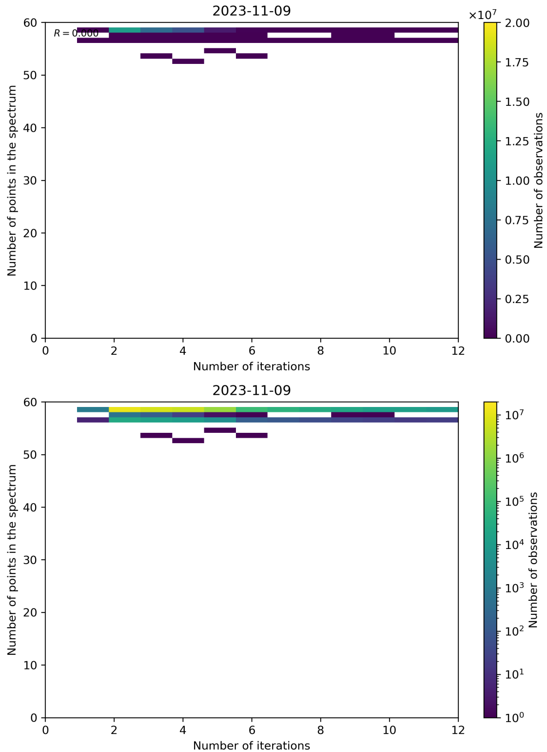
Figure 108: Scatter density plot of “Number of iterations” against “Number of points in the spectrum” for 2023-11-08 to 2023-11-10.
