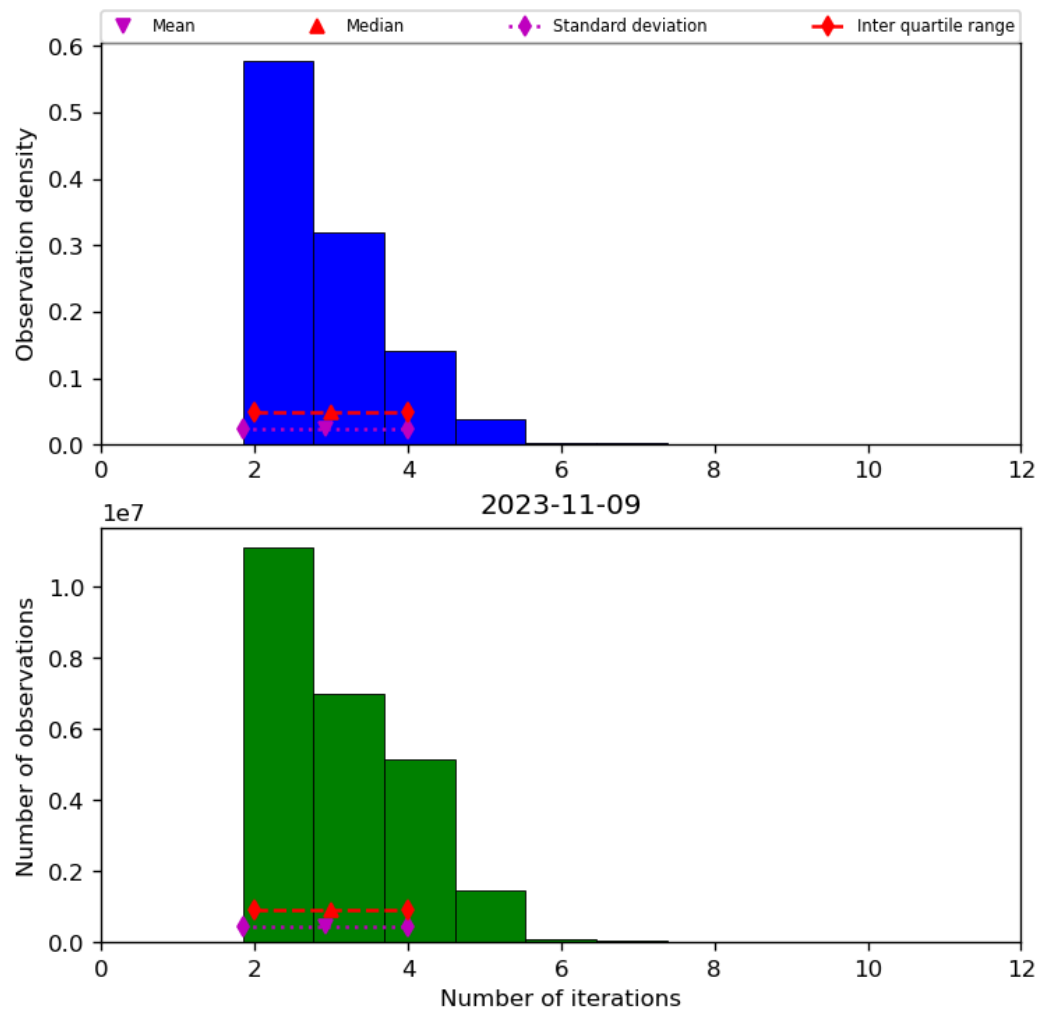
Figure 39: Histogram of “Number of iterations” for 2023-11-08 to 2023-11-10
