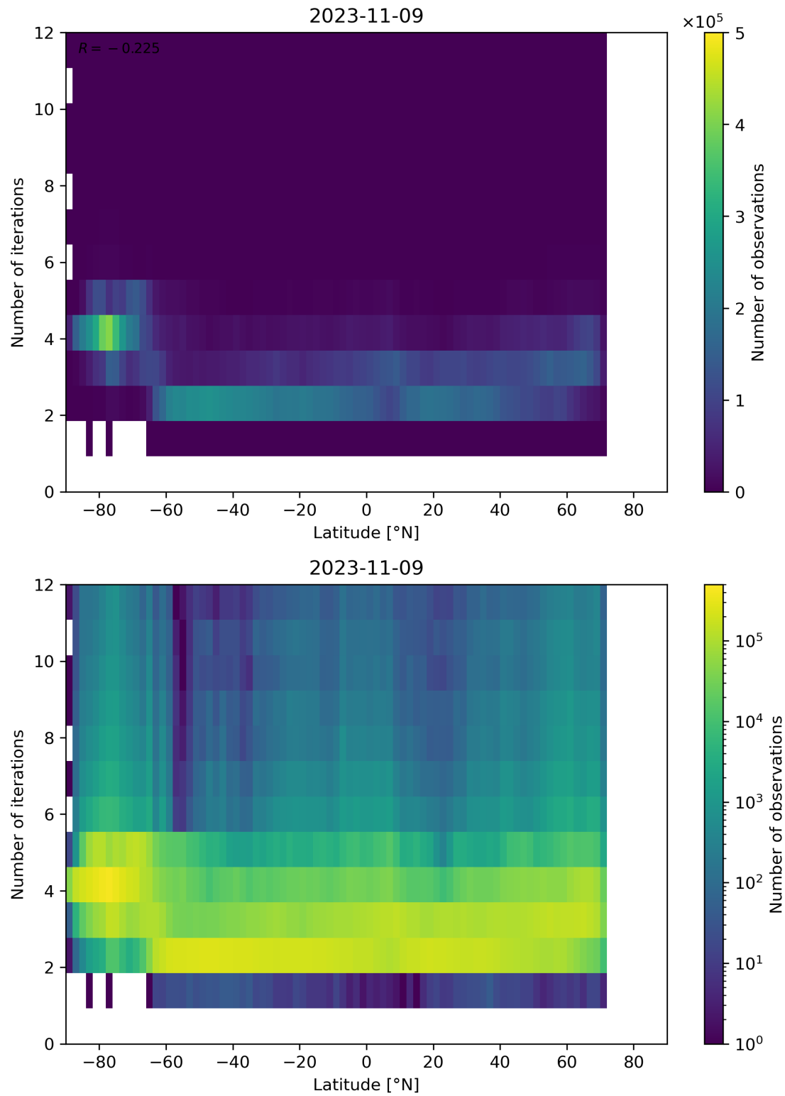
Figure 102: Scatter density plot of “Latitude” against “Number of iterations” for 2023-11-08 to 2023-11-10.
