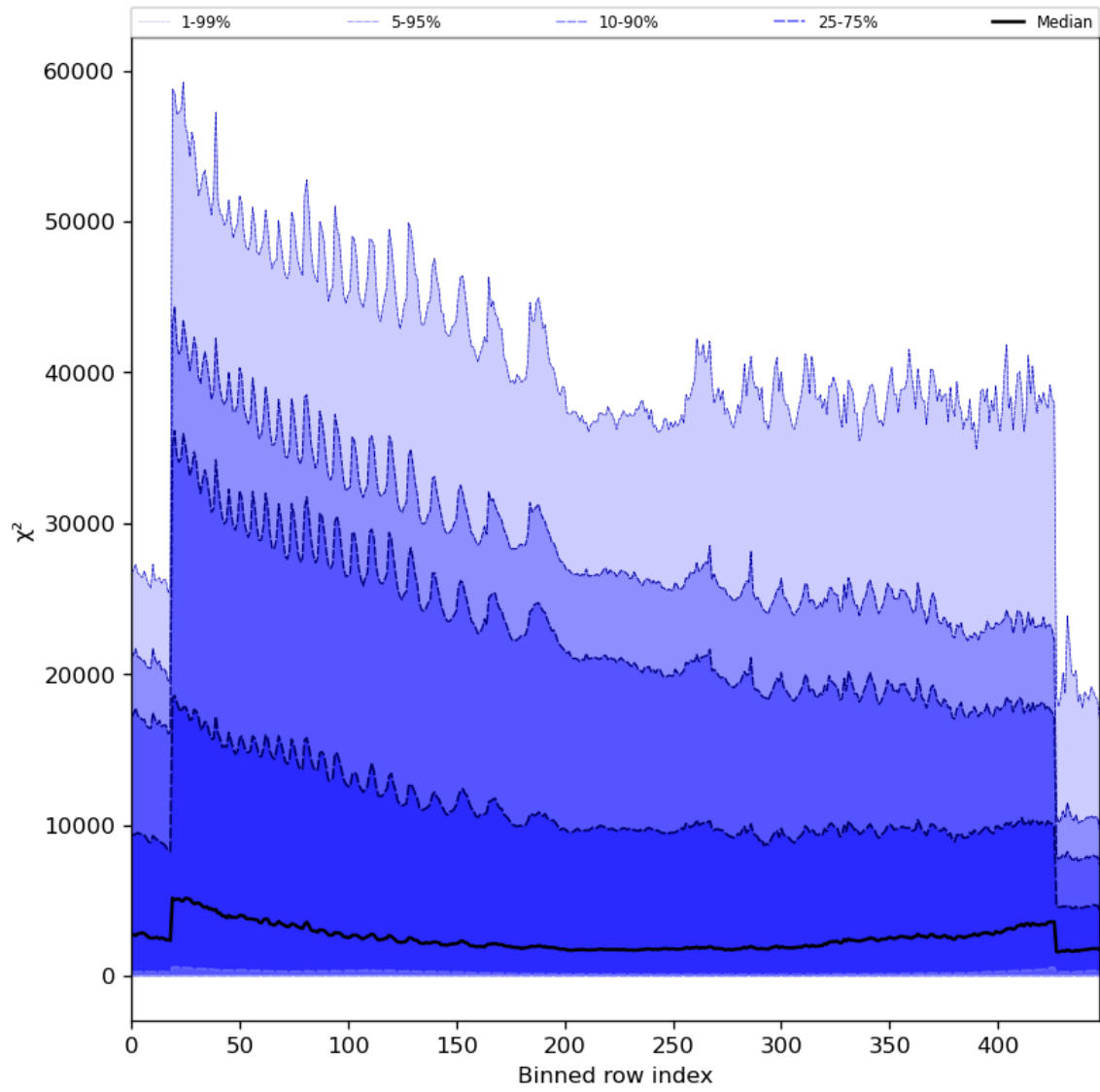
Figure 55: Along track statistics of “ \chi^2 ” for 2023-11-08 to 2023-11-10
