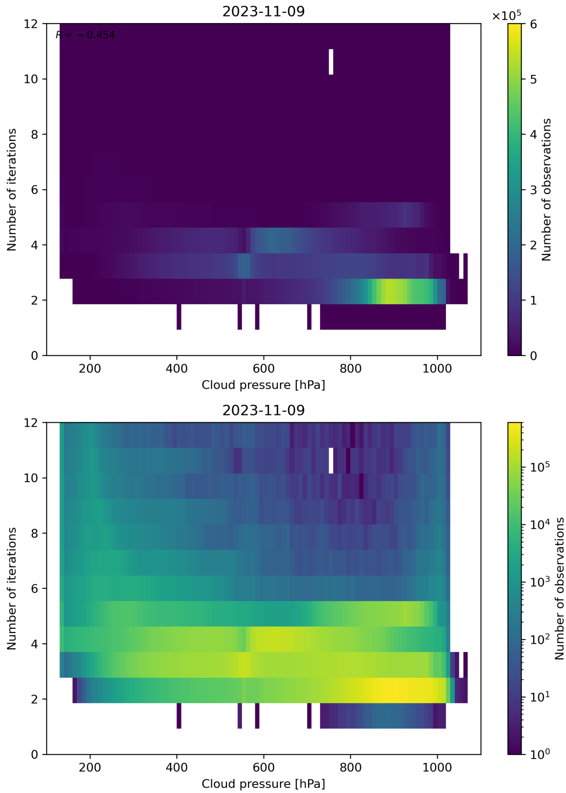
Figure 89: Scatter density plot of “Cloud pressure” against “Number of iterations” for 2023-11-08 to 2023-11-10.
