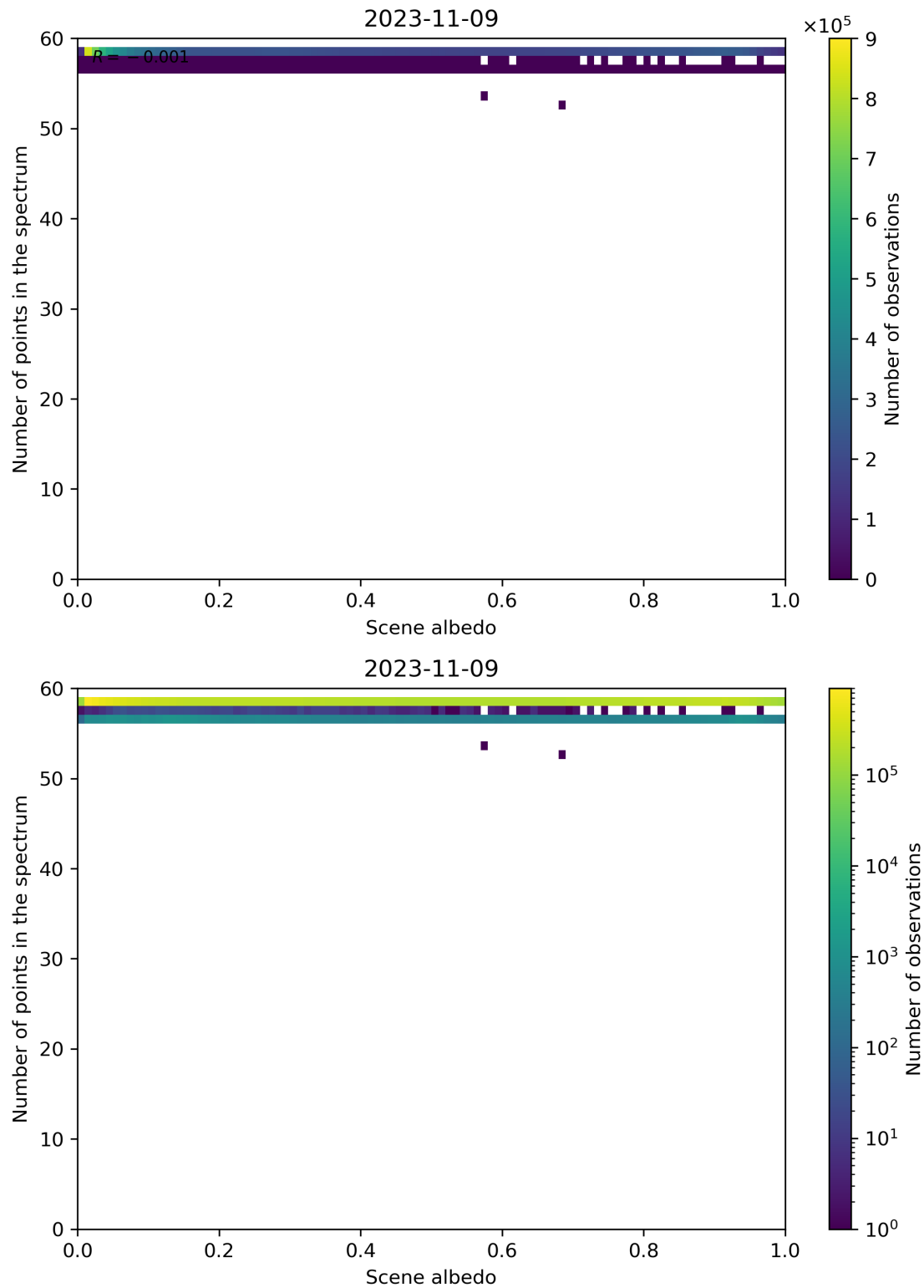
Figure 116: Scatter density plot of “Scene albedo” against “Number of points in the spectrum” for 2023-11-08 to 2023-11-10.
