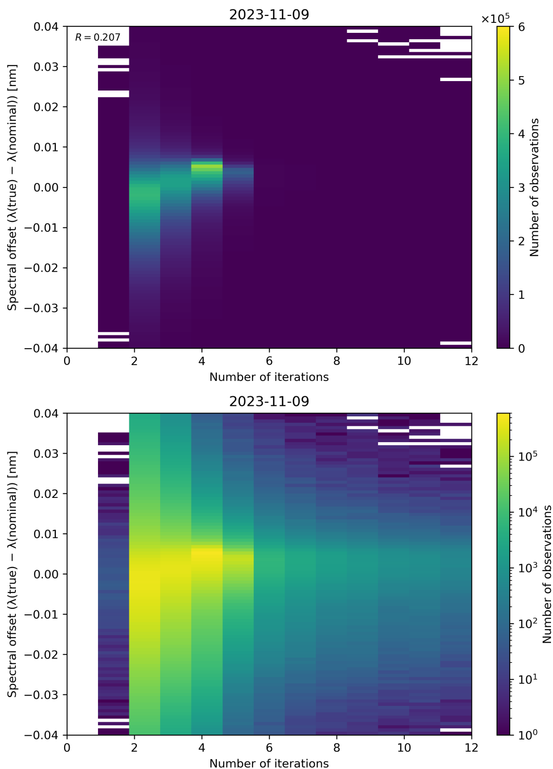
Figure 109: Scatter density plot of “Number of iterations” against “Spectral offset ( \lambda(\text{true}) - \lambda(\text{nominal}) )” for 2023-11-08 to 2023-11-10.
