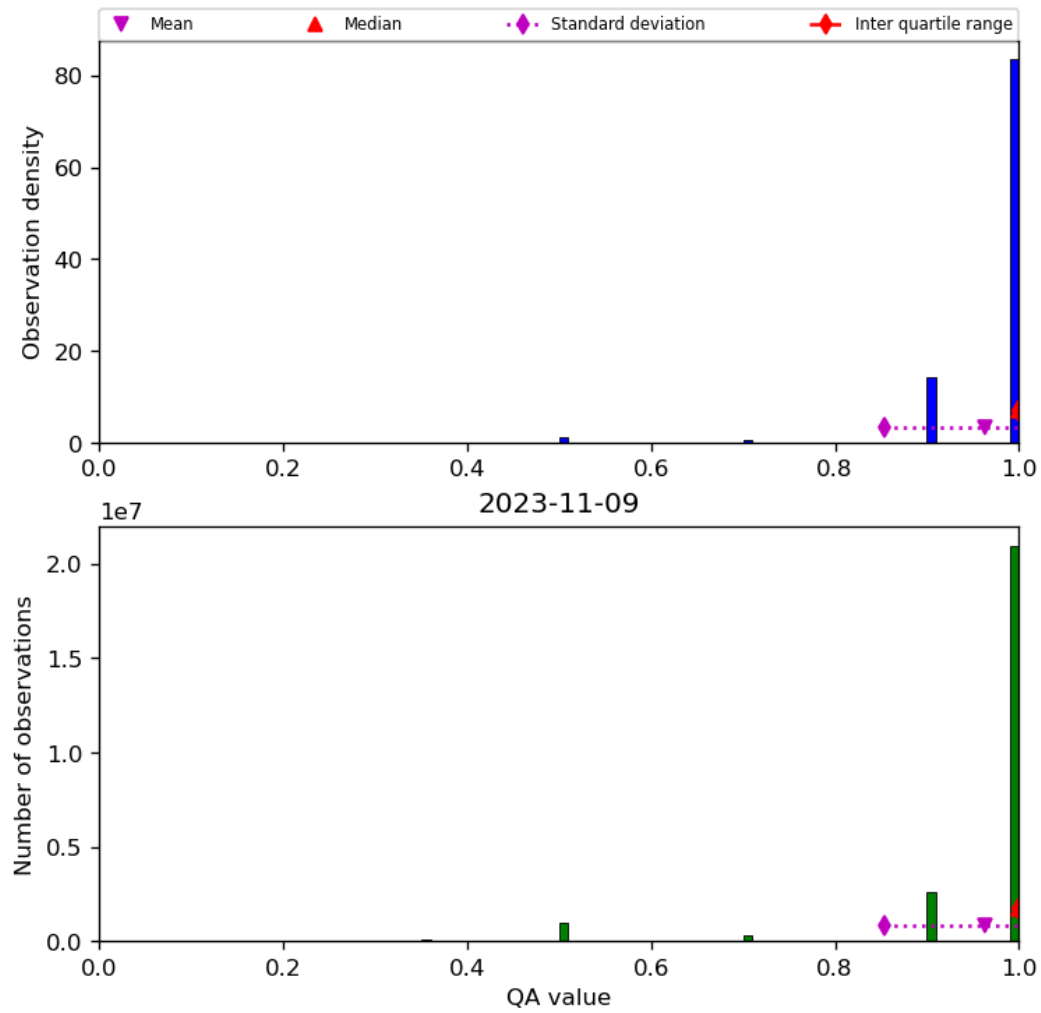
Figure 29: Histogram of “QA value” for 2023-11-08 to 2023-11-10
