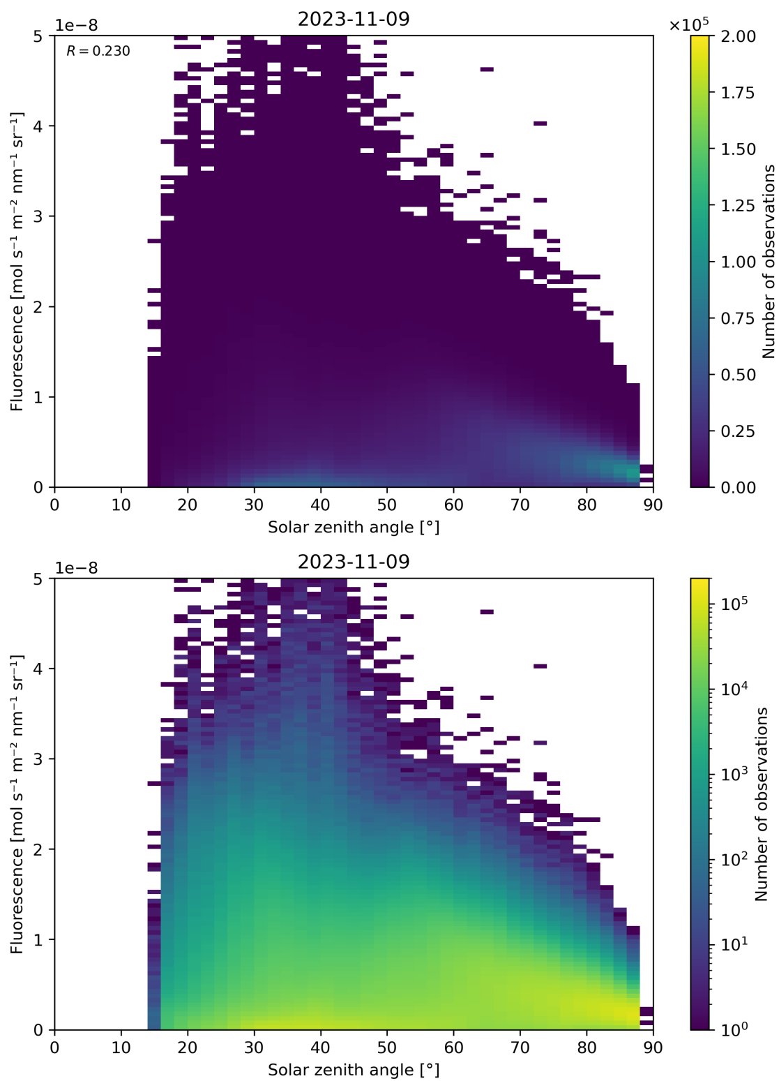
Figure 123: Scatter density plot of “Solar zenith angle” against “Fluorescence” for 2023-11-08 to 2023-11-10.
