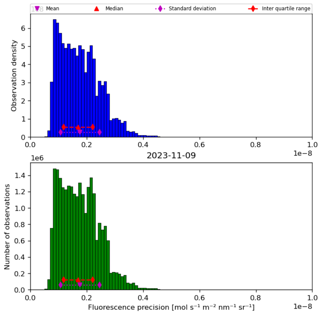
Figure 41: Histogram of “Fluorescence precision” for 2023-11-08 to 2023-11-10
