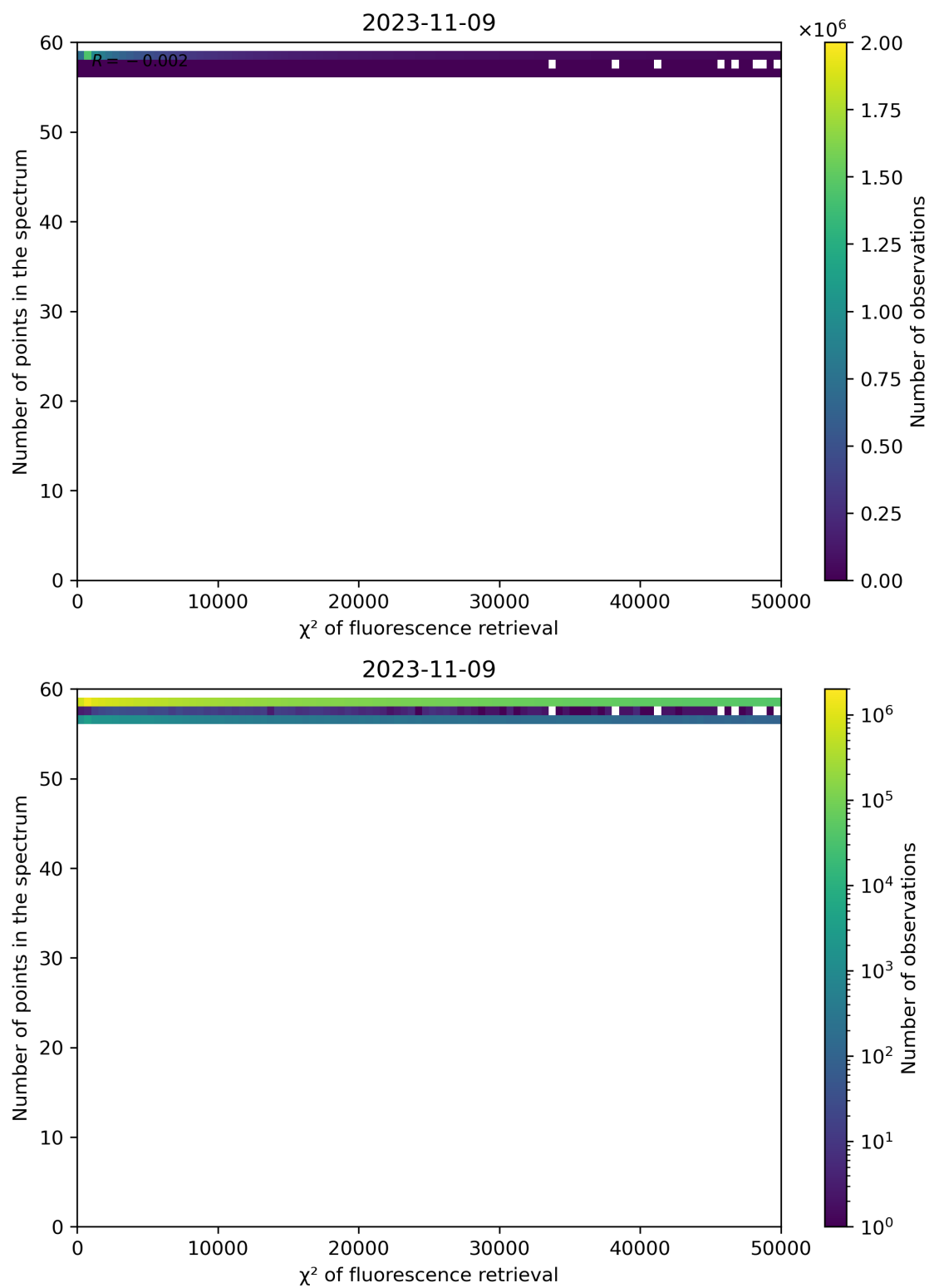
Figure 71: Scatter density plot of " \chi^2 of fluorescence retrieval" against "Number of points in the spectrum" for 2023-11-08 to 2023-11-10.
