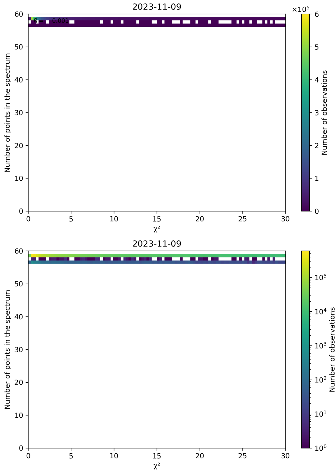
Figure 74: Scatter density plot of " \chi^2 " against "Number of points in the spectrum" for 2023-11-08 to 2023-11-10.
