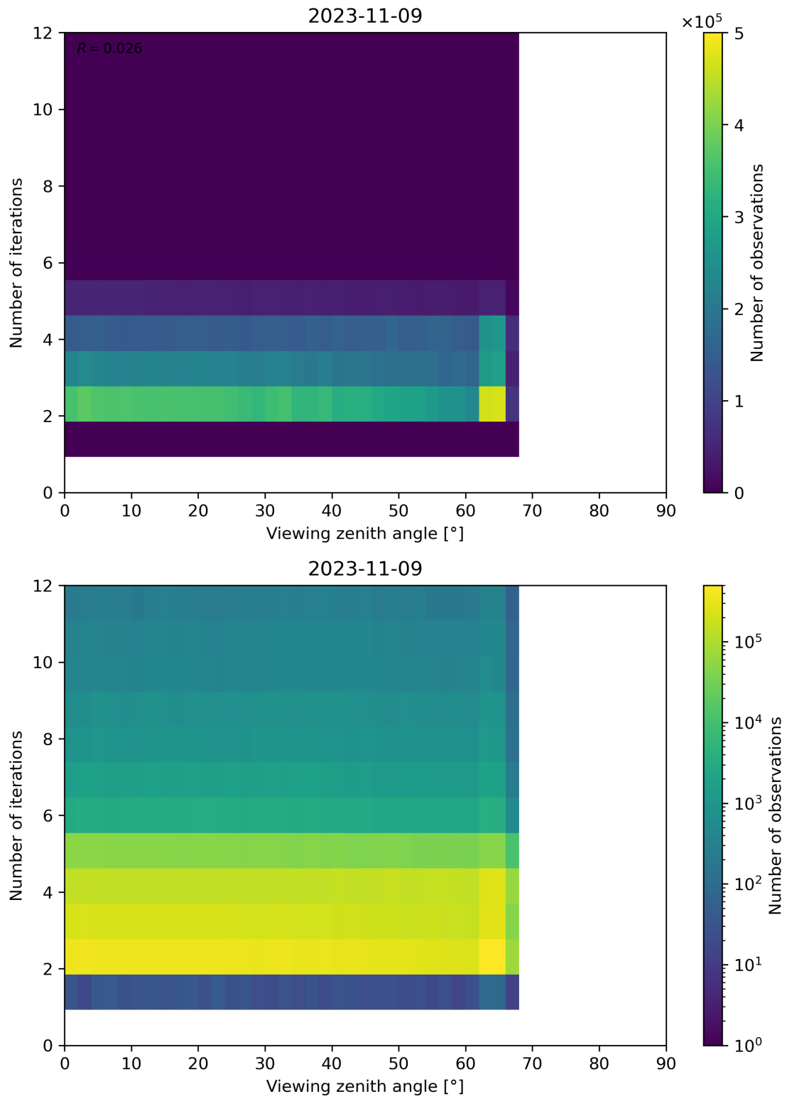
Figure 136: Scatter density plot of “Viewing zenith angle” against “Number of iterations” for 2023-11-08 to 2023-11-10.
