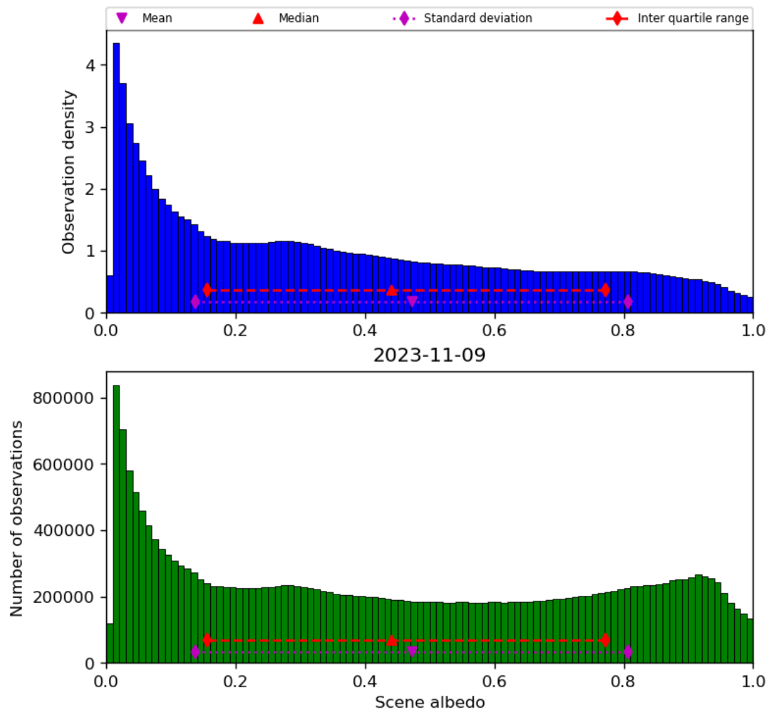
Figure 34: Histogram of “Scene albedo” for 2023-11-08 to 2023-11-10
