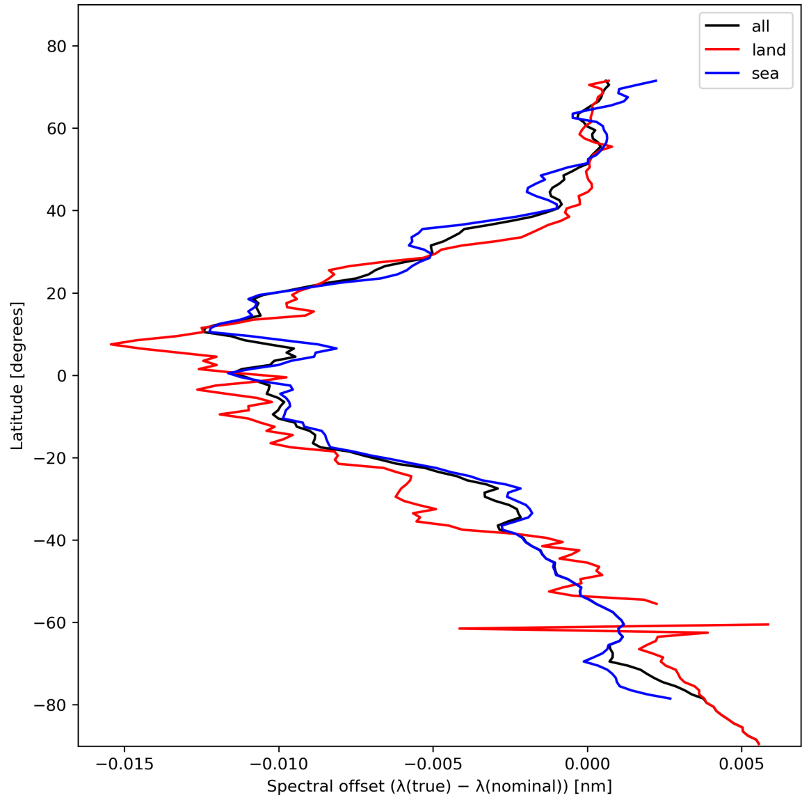
Figure 28: Zonal average of “Spectral offset ( \lambda(\text{true}) - \lambda(\text{nominal}) )” for 2023-11-08 to 2023-11-10.
