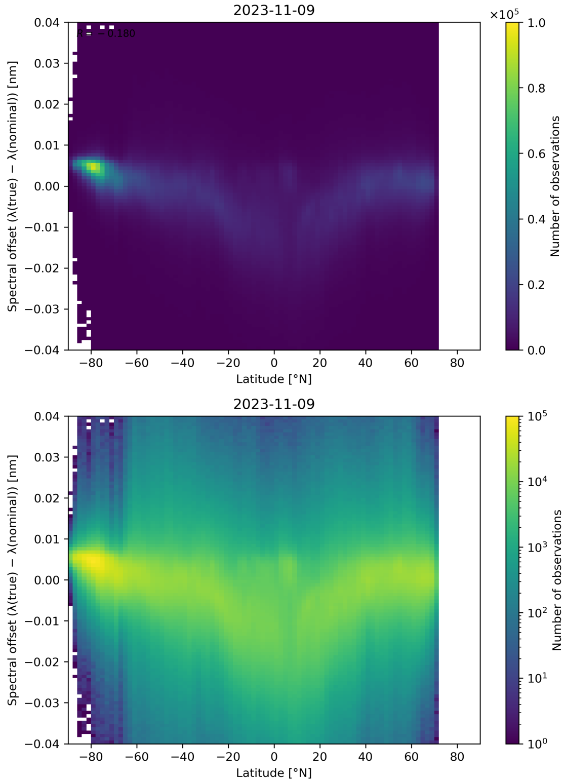
Figure 105: Scatter density plot of “Latitude” against “Spectral offset ( \lambda(\text{true}) - \lambda(\text{nominal}) )” for 2023-11-08 to 2023-11-10.
