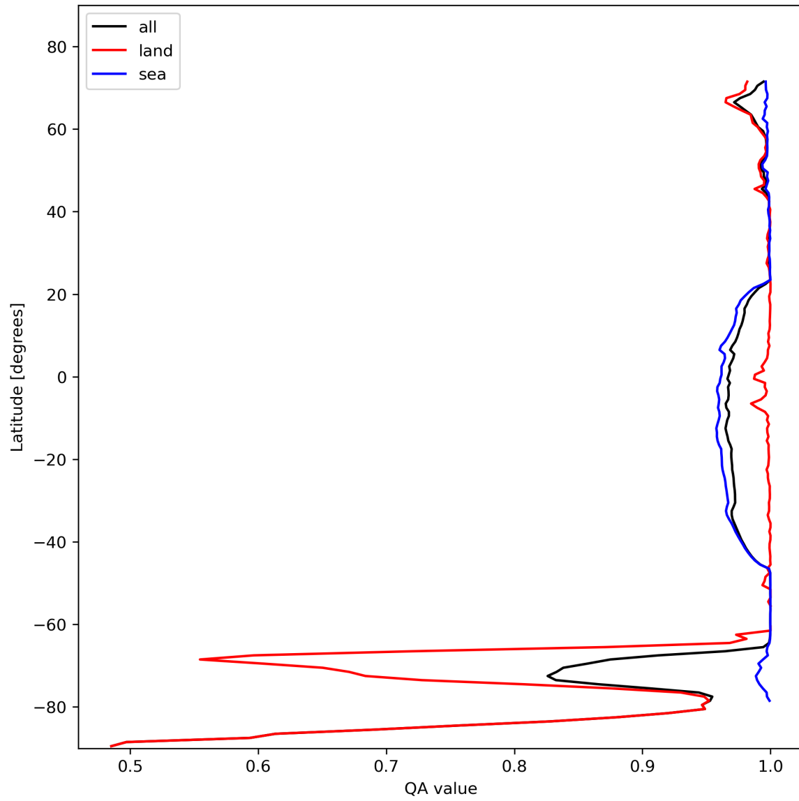
Figure 12: Zonal average of “QA value” for 2023-11-08 to 2023-11-10.
