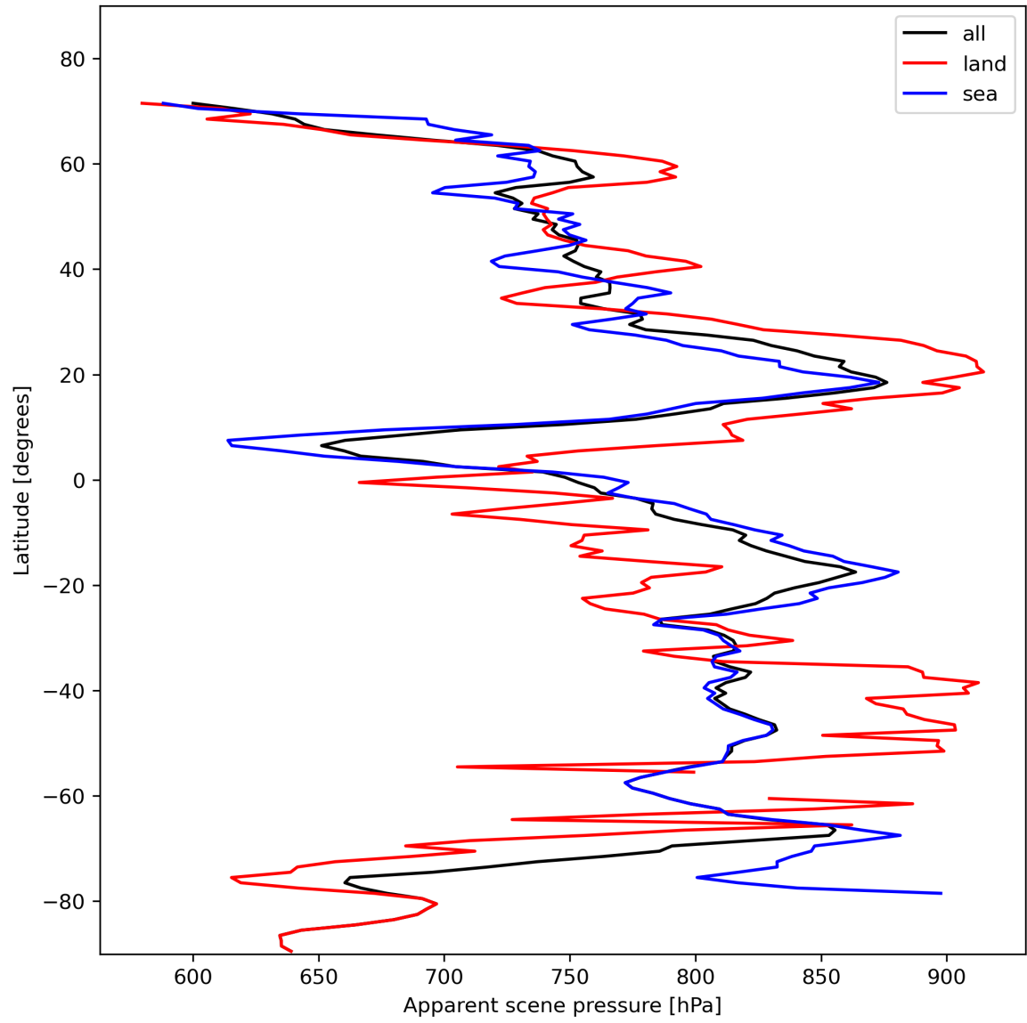
Figure 19: Zonal average of “Apparent scene pressure” for 2023-11-08 to 2023-11-10.
