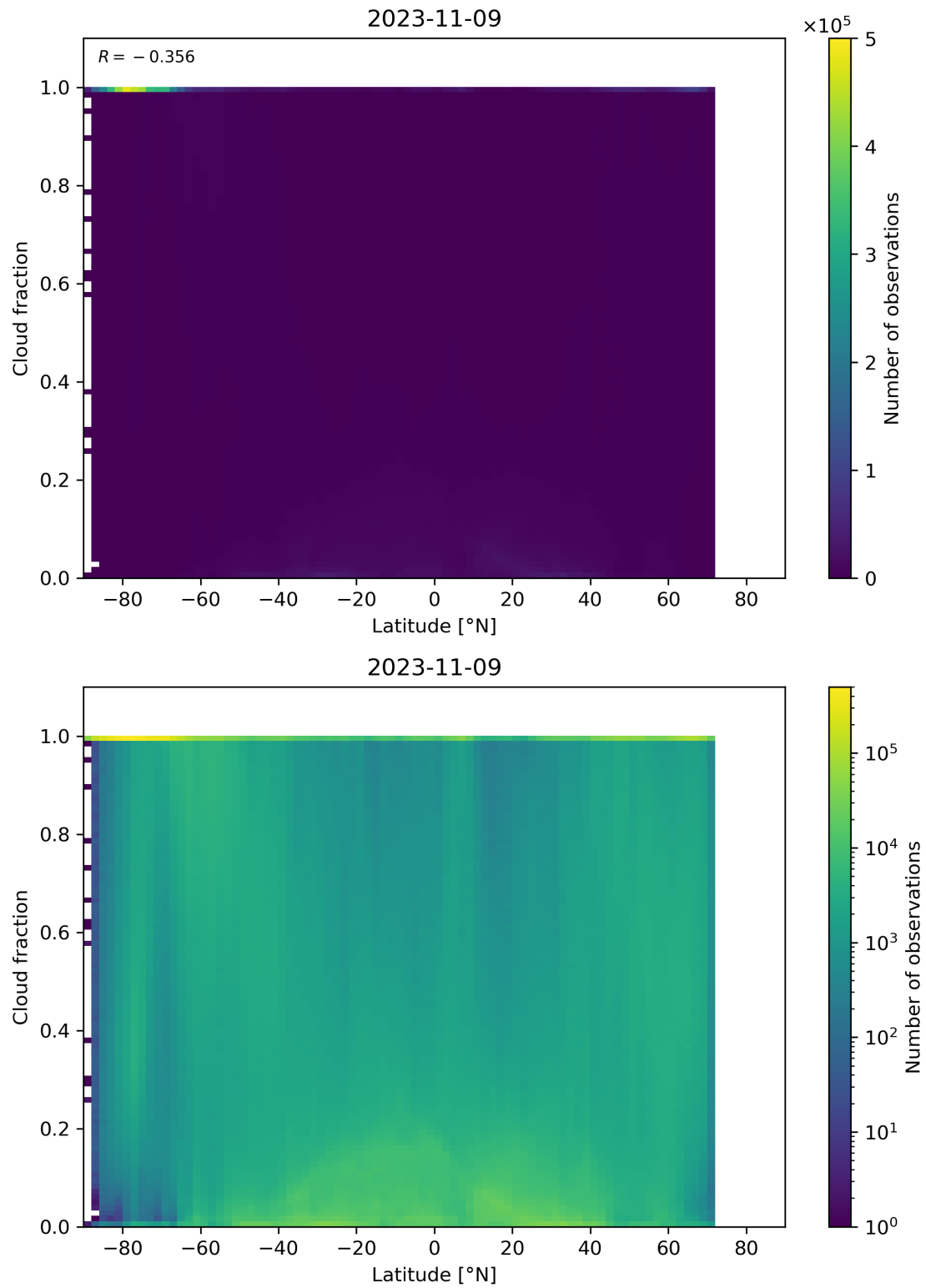
Figure 99: Scatter density plot of “Latitude” against “Cloud fraction” for 2023-11-08 to 2023-11-10.
