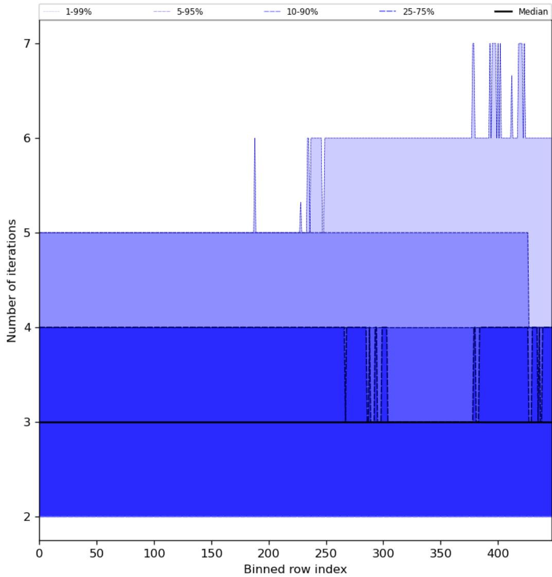
Figure 56: Along track statistics of “Number of iterations” for 2023-11-08 to 2023-11-10
