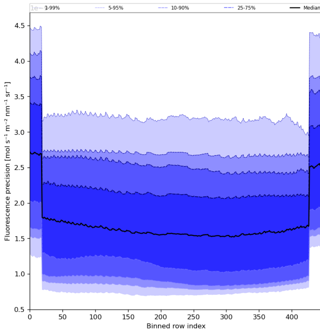
Figure 58: Along track statistics of “Fluorescence precision” for 2023-11-08 to 2023-11-10
