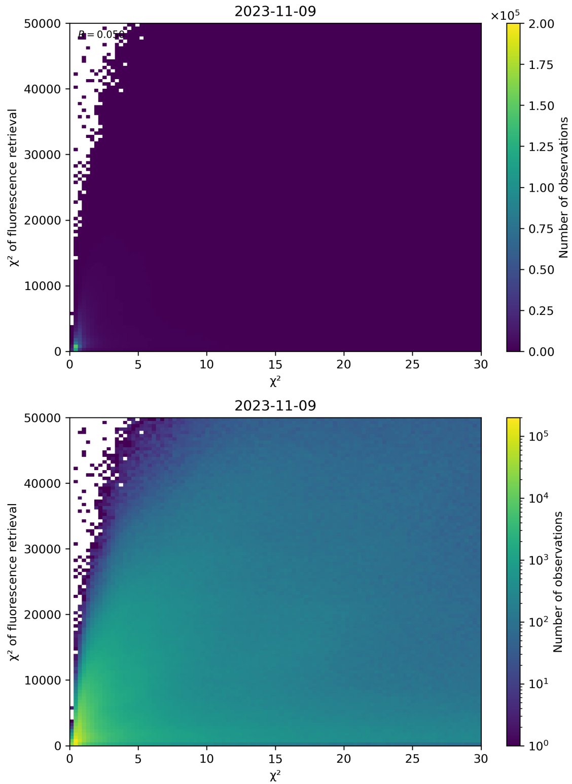
Figure 69: Scatter density plot of “ \chi^2 ” against “ \chi^2 of fluorescence retrieval” for 2023-11-08 to 2023-11-10.
