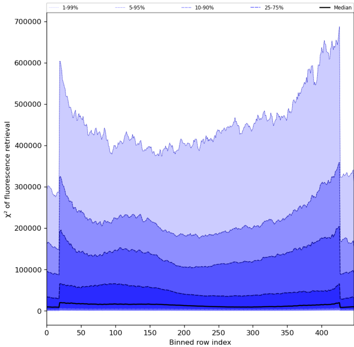
Figure 59: Along track statistics of “ \chi^2 of fluorescence retrieval” for 2023-11-08 to 2023-11-10
