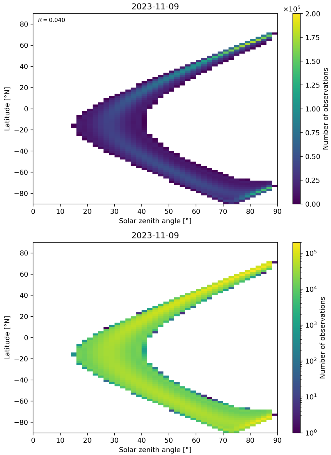
Figure 124: Scatter density plot of “Solar zenith angle” against “Latitude” for 2023-11-08 to 2023-11-10.
