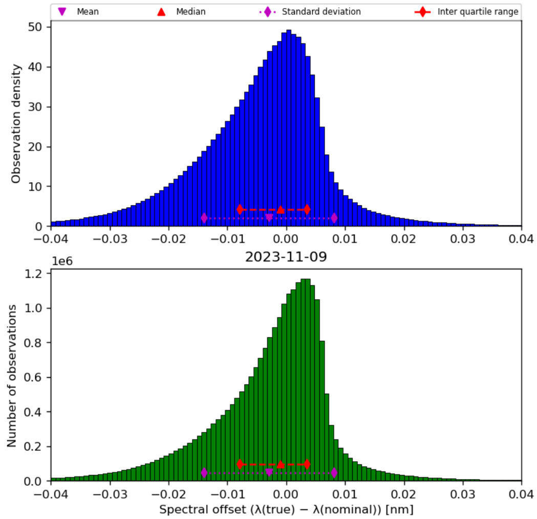
Figure 45: Histogram of “Spectral offset ( \lambda(\text{true}) - \lambda(\text{nominal}) )” for 2023-11-08 to 2023-11-10
