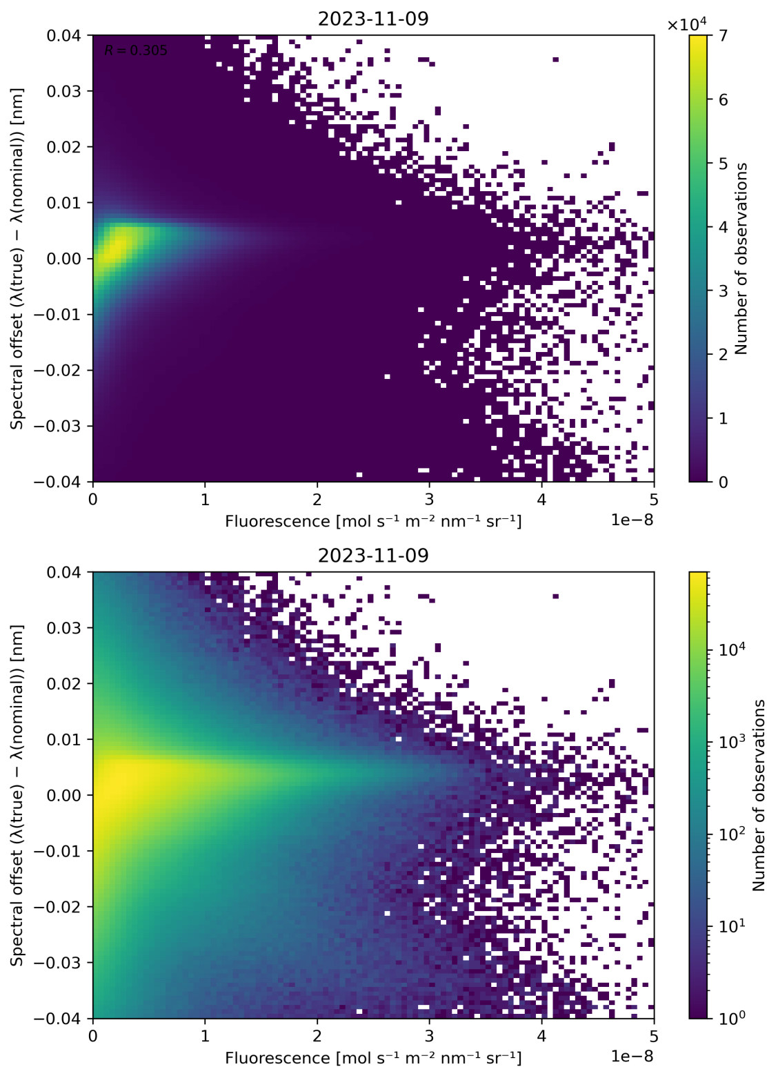
Figure 95: Scatter density plot of “Fluorescence” against “Spectral offset ( \lambda(\text{true}) - \lambda(\text{nominal}) )” for 2023-11-08 to 2023-11-10.
