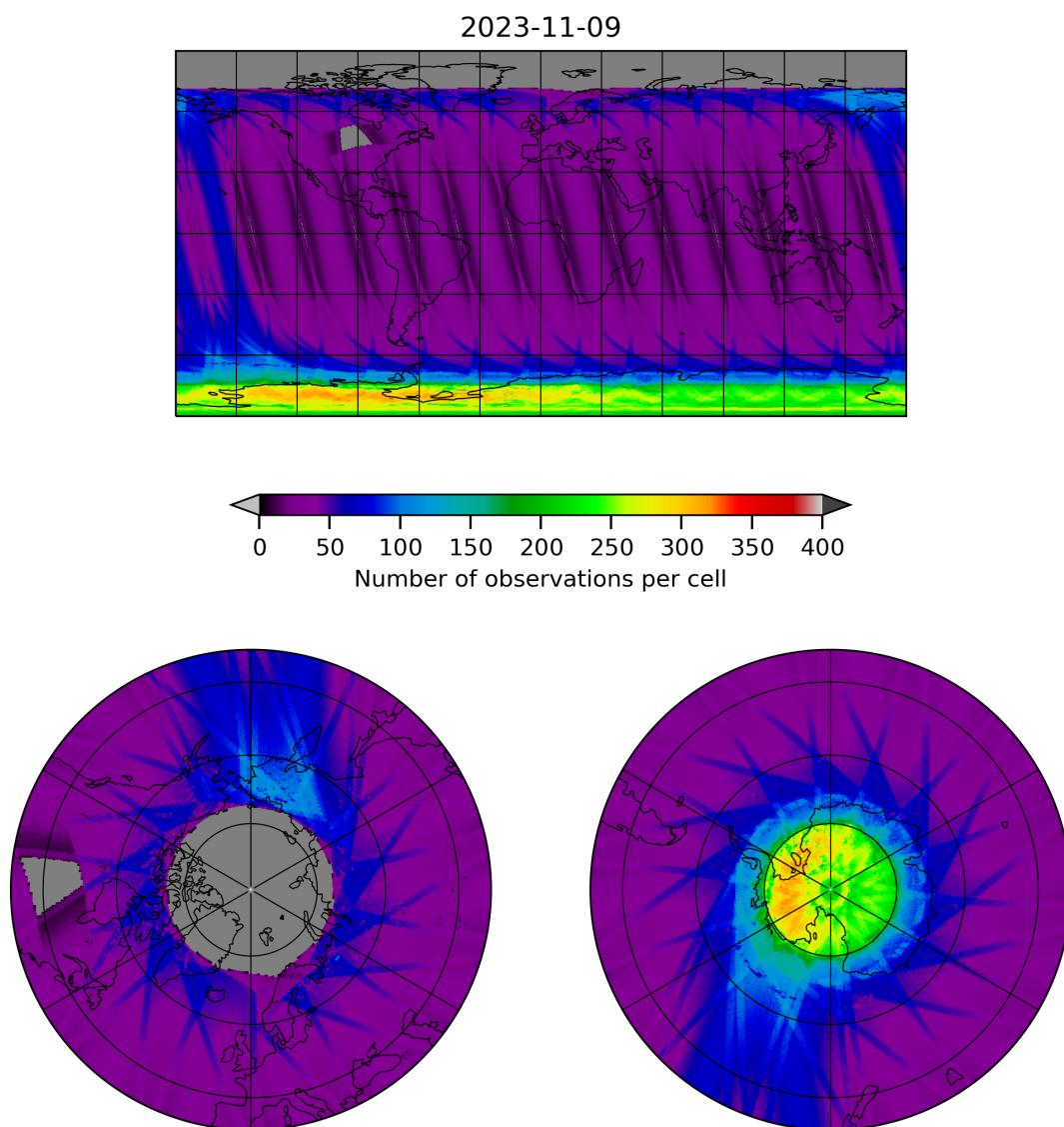
Figure 11: Map of the number of observations for 2023-11-08 to 2023-11-10
