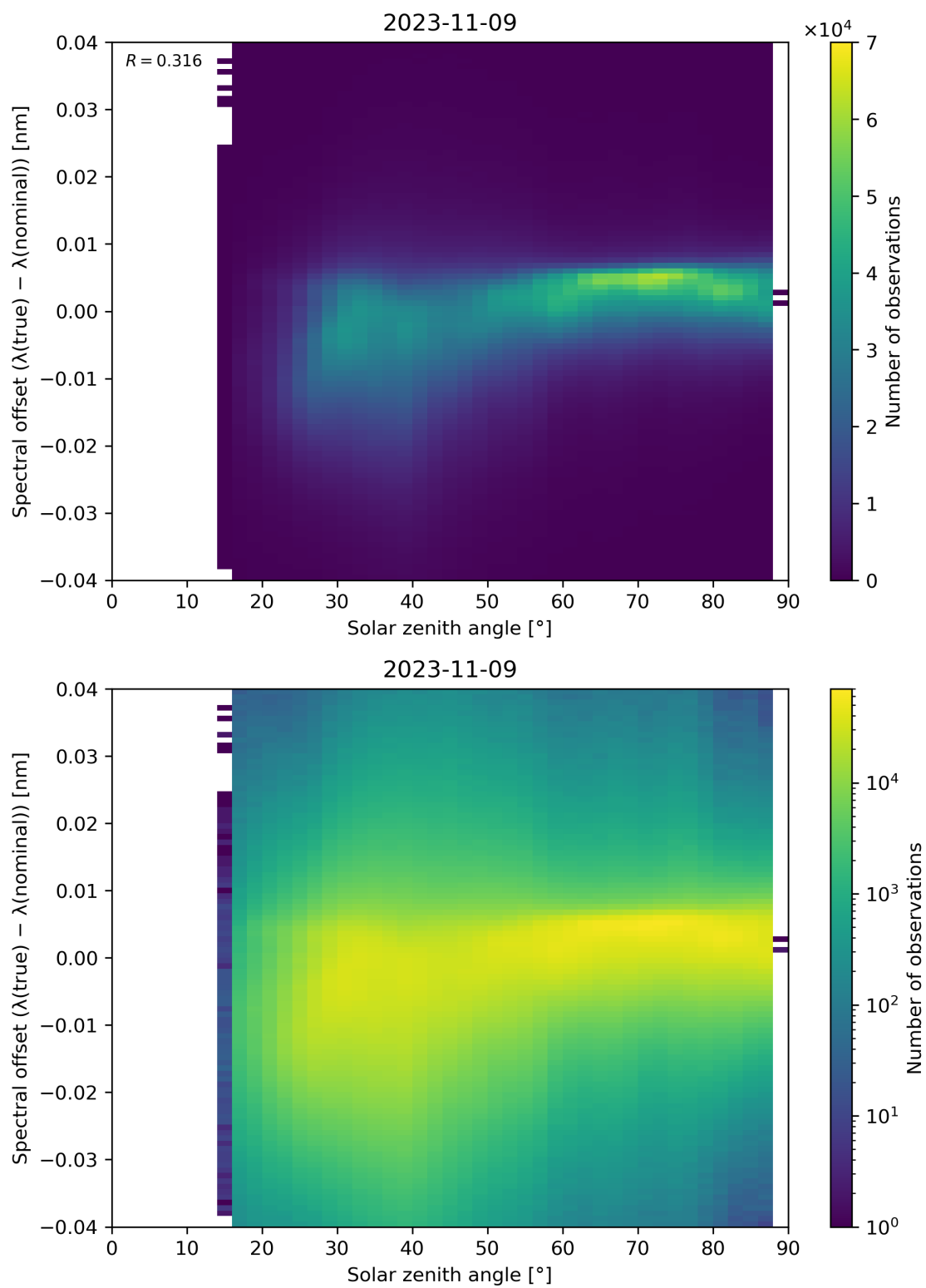
Figure 128: Scatter density plot of “Solar zenith angle” against “Spectral offset ( \lambda(\text{true}) - \lambda(\text{nominal}) )” for 2023-11-08 to 2023-11-10.
