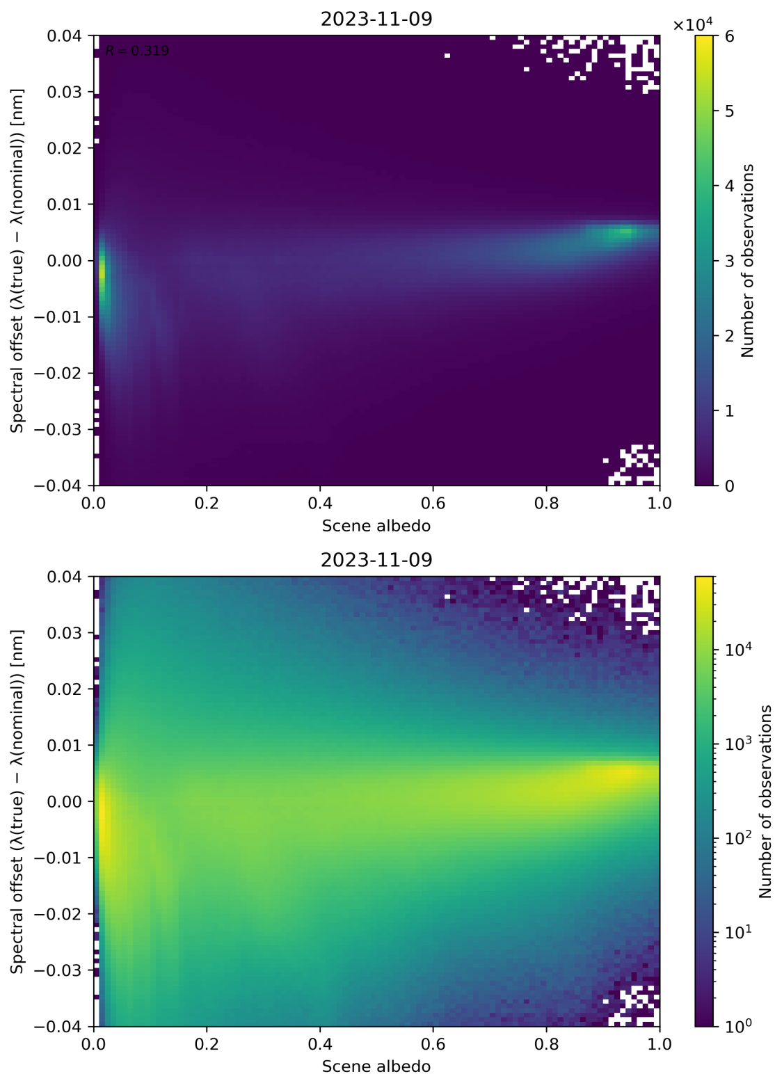
Figure 117: Scatter density plot of “Scene albedo” against “Spectral offset ( \lambda(\text{true}) - \lambda(\text{nominal}) )” for 2023-11-08 to 2023-11-10.
