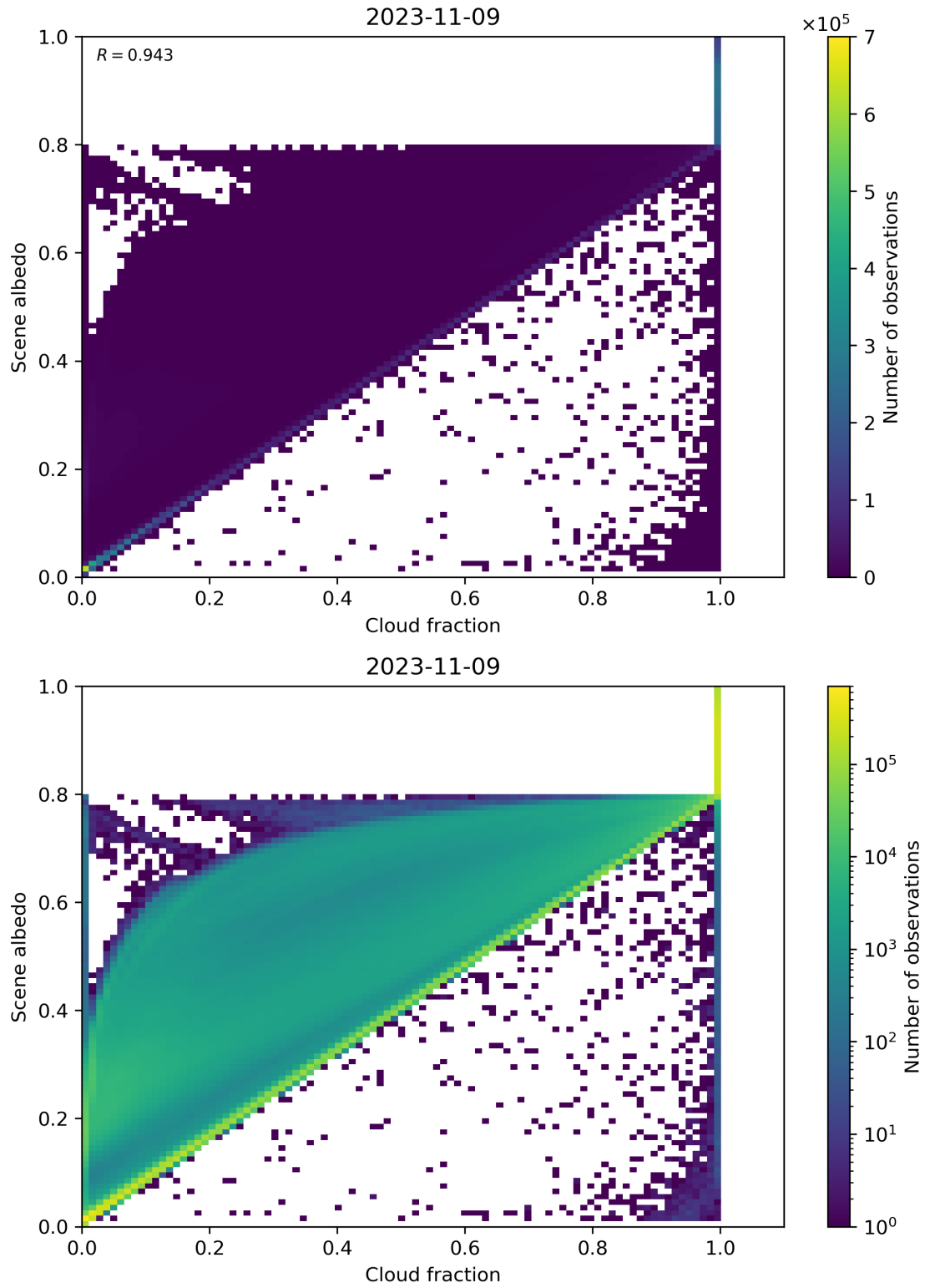
Figure 82: Scatter density plot of “Cloud fraction” against “Scene albedo” for 2023-11-08 to 2023-11-10.
