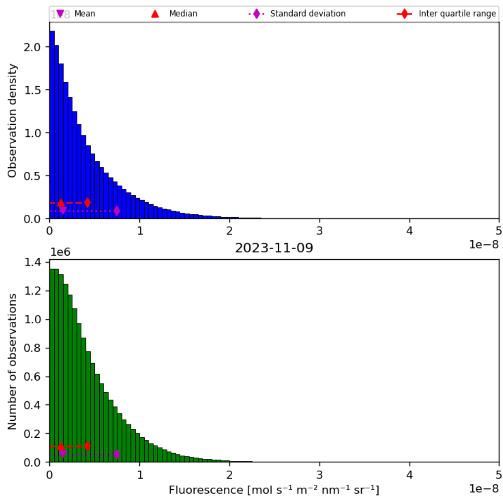
Figure 40: Histogram of “Fluorescence” for 2023-11-08 to 2023-11-10
