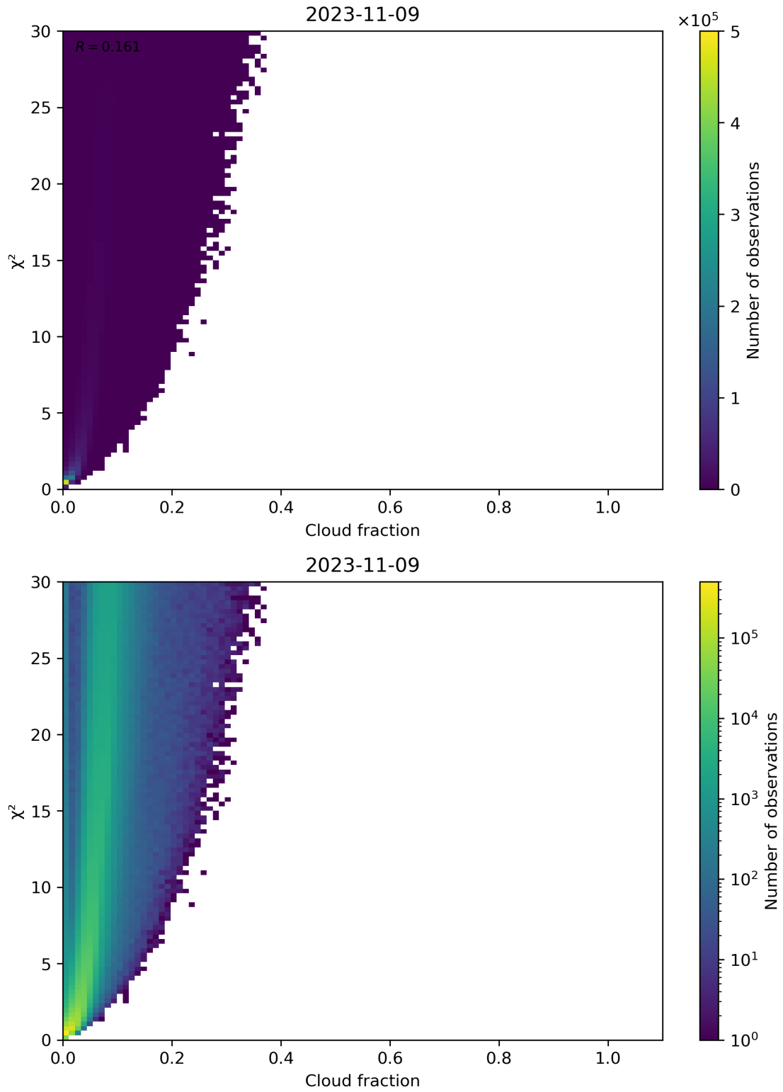
Figure 77: Scatter density plot of “Cloud fraction” against “ \chi^2 ” for 2023-11-08 to 2023-11-10.
