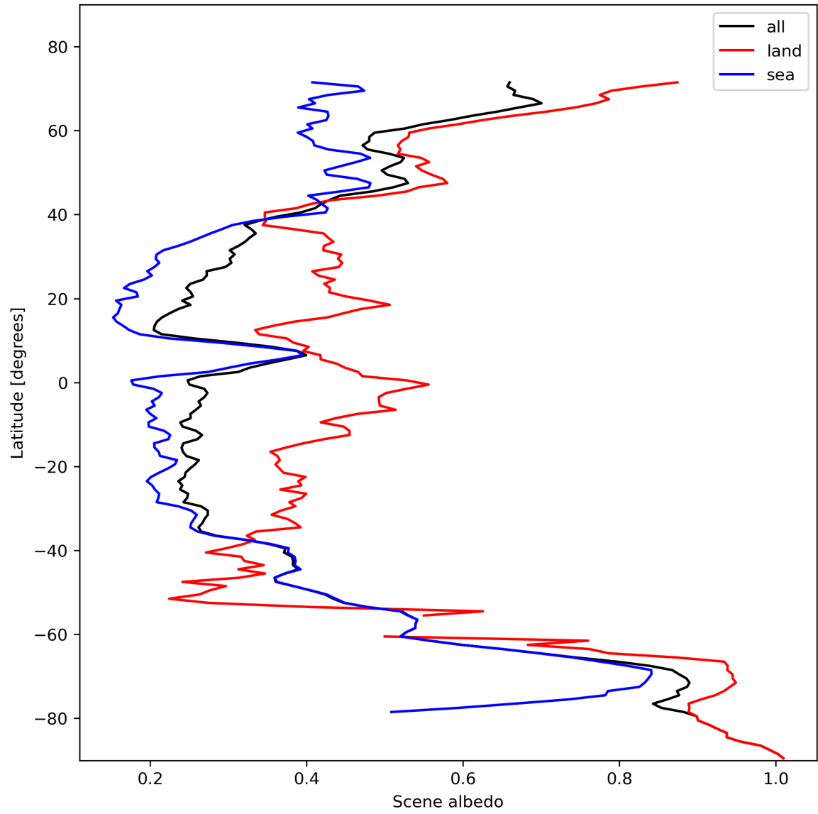
Figure 17: Zonal average of “Scene albedo” for 2023-11-08 to 2023-11-10.
