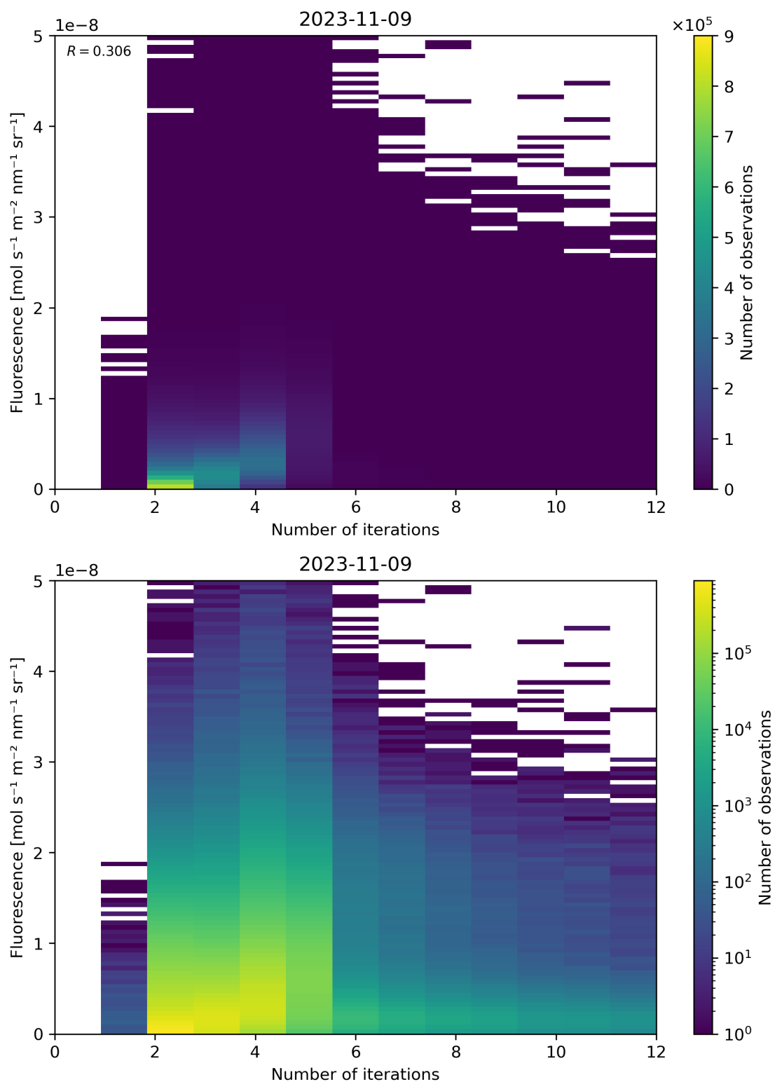
Figure 107: Scatter density plot of “Number of iterations” against “Fluorescence” for 2023-11-08 to 2023-11-10.
