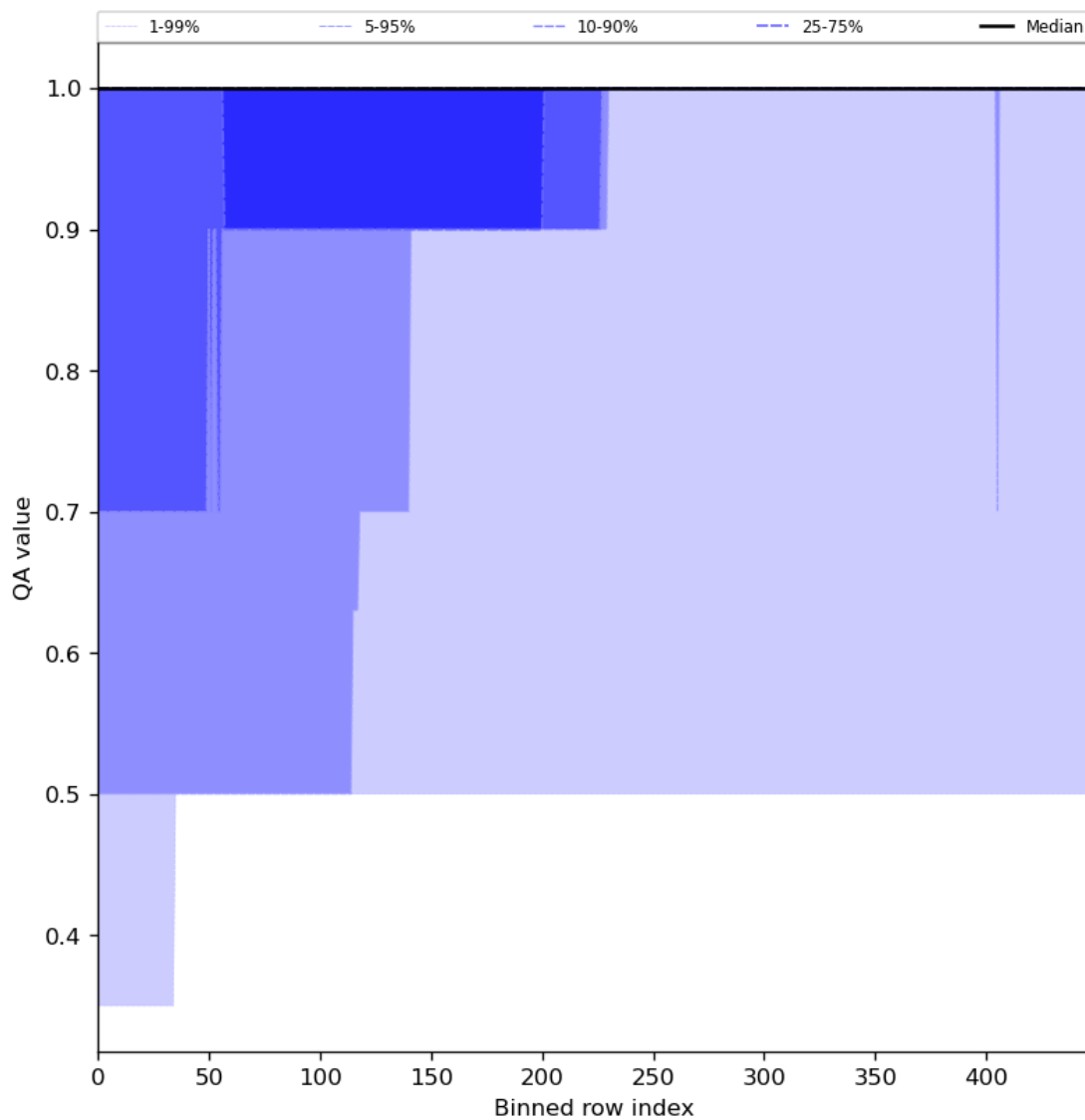
Figure 46: Along track statistics of “QA value” for 2023-11-08 to 2023-11-10
