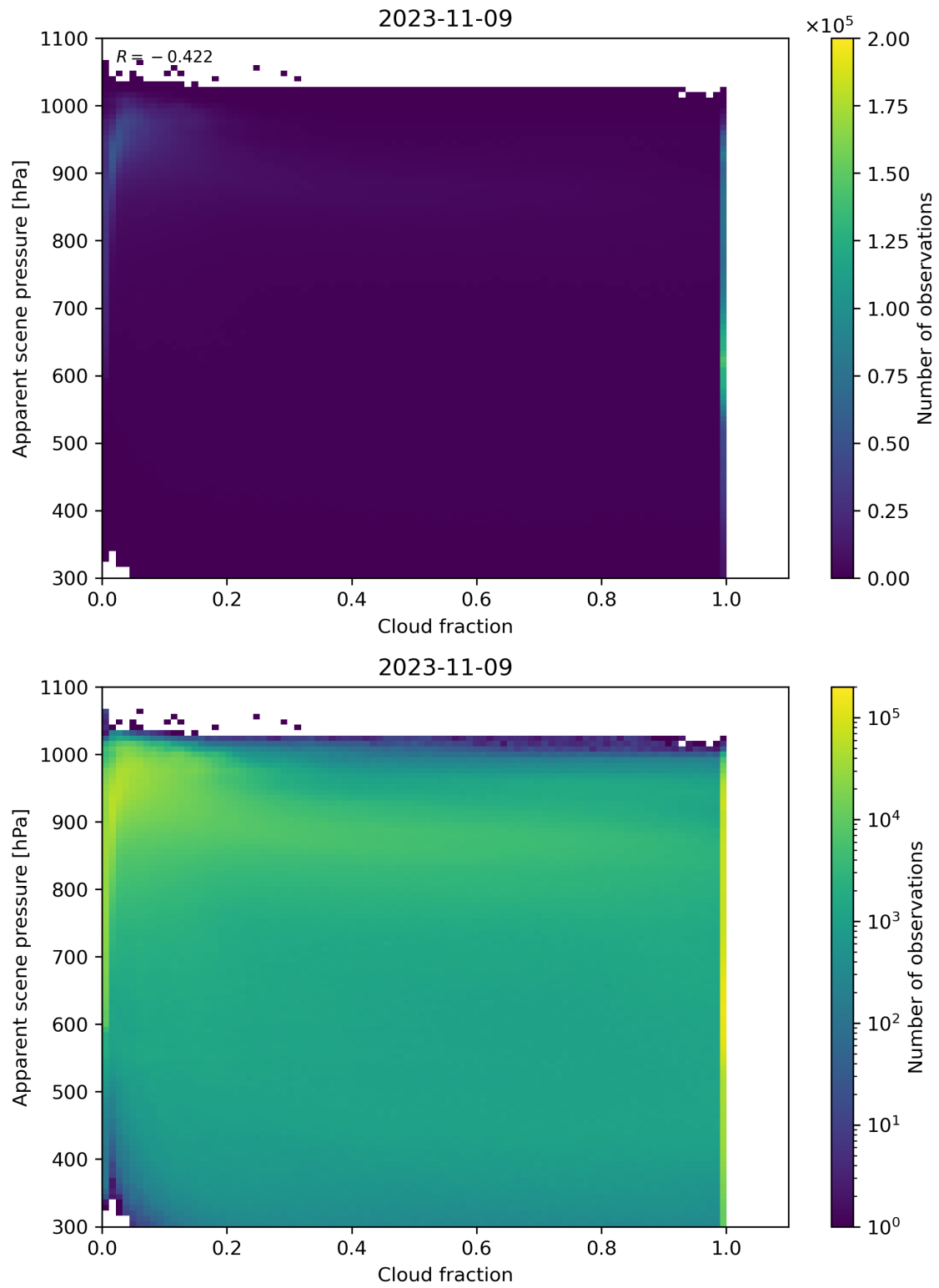
Figure 76: Scatter density plot of “Cloud fraction” against “Apparent scene pressure” for 2023-11-08 to 2023-11-10.
