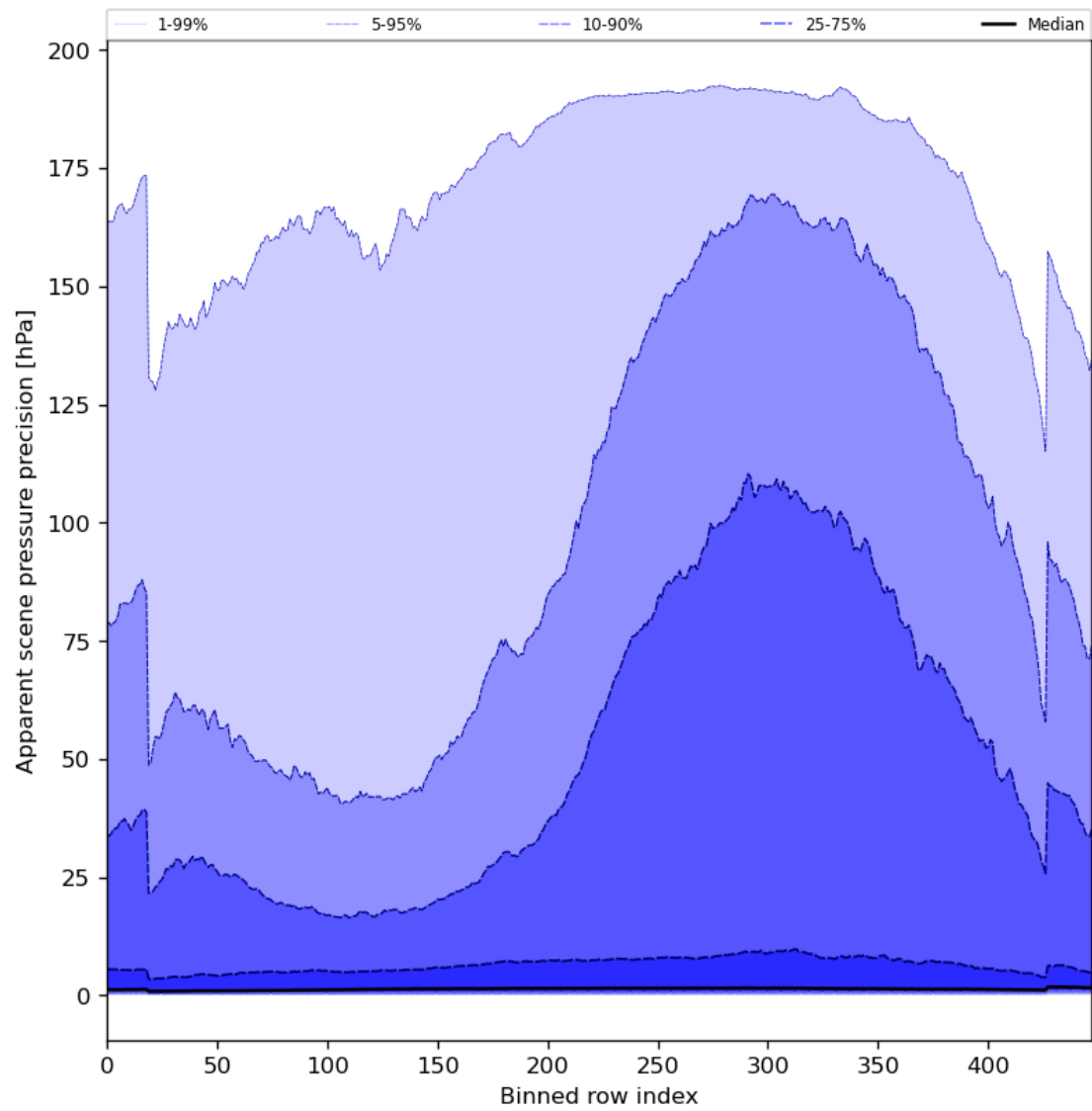
Figure 54: Along track statistics of “Apparent scene pressure precision” for 2023-11-08 to 2023-11-10
