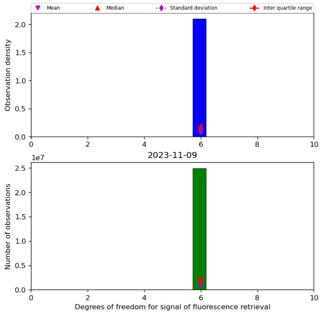
Figure 43: Histogram of “Degrees of freedom for signal of fluorescence retrieval” for 2023-11-08 to 2023-11-10
