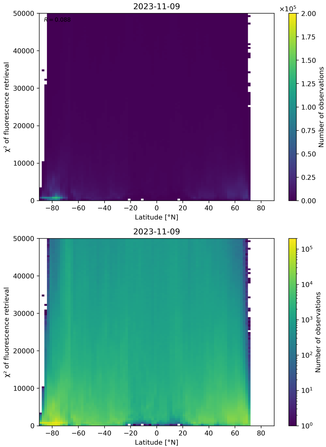
Figure 98: Scatter density plot of “Latitude” against “ \chi^2 of fluorescence retrieval” for 2023-11-08 to 2023-11-10.
