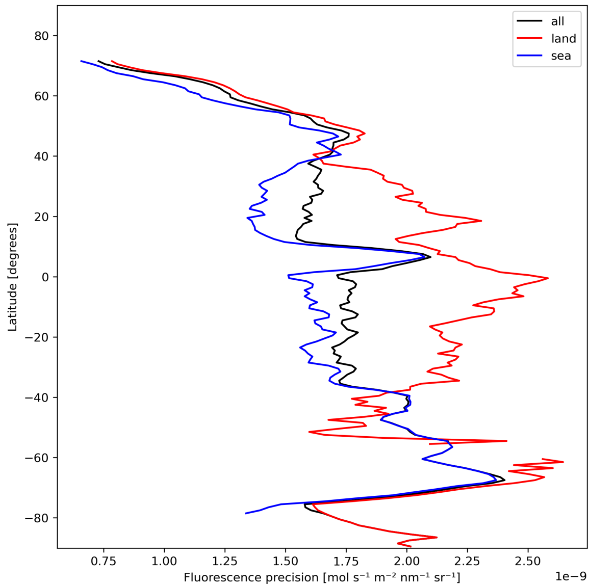
Figure 24: Zonal average of “Fluorescence precision” for 2023-11-08 to 2023-11-10.
