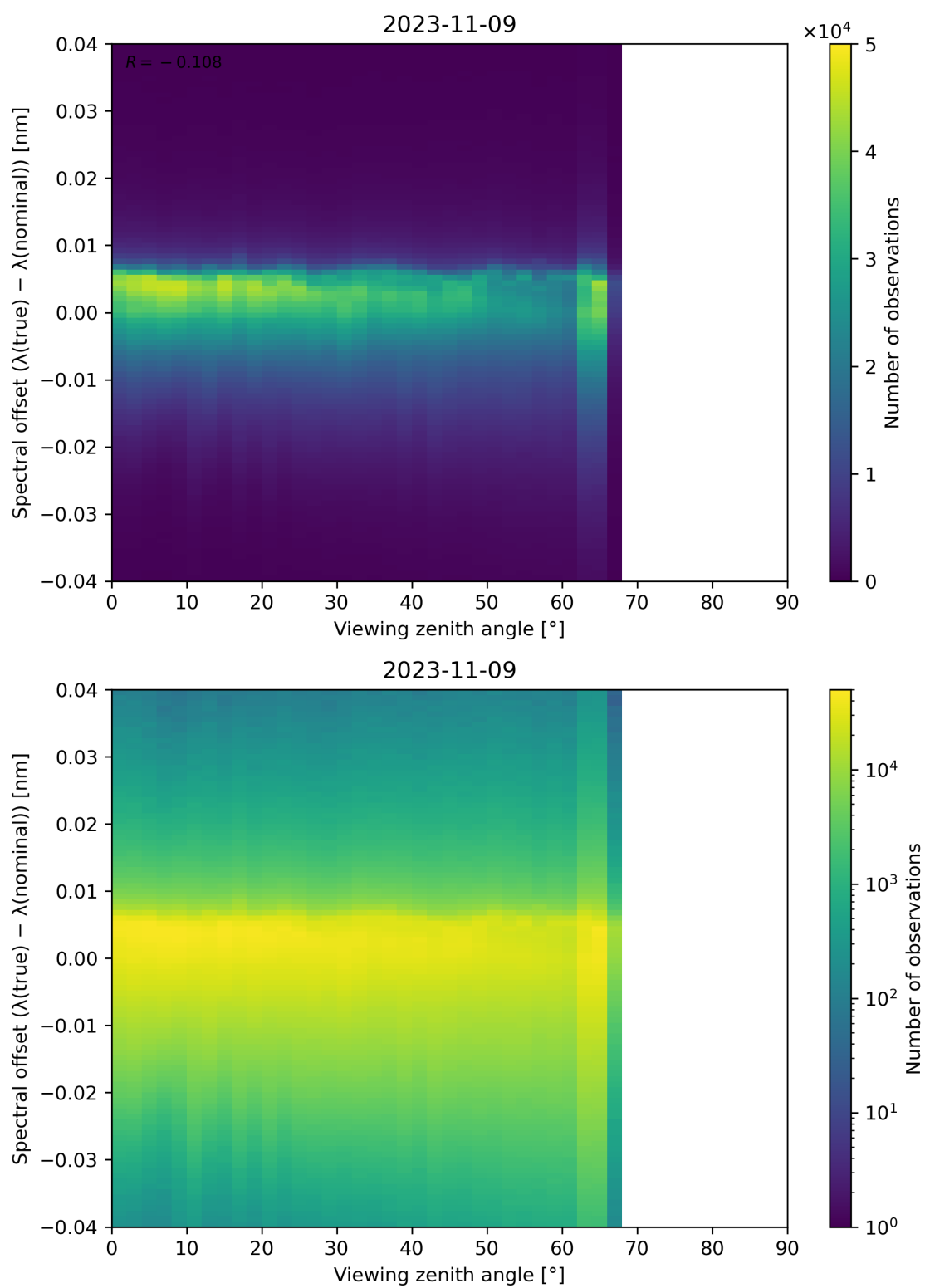
Figure 140: Scatter density plot of “Viewing zenith angle” against “Spectral offset ( \lambda(\text{true}) - \lambda(\text{nominal}) )” for 2023-11-08 to 2023-11-10.
