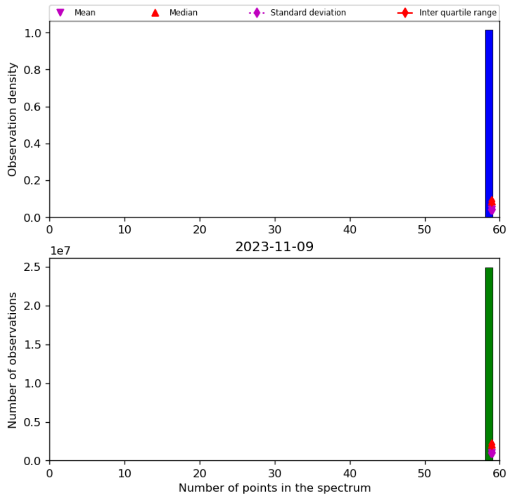
Figure 44: Histogram of “Number of points in the spectrum” for 2023-11-08 to 2023-11-10
