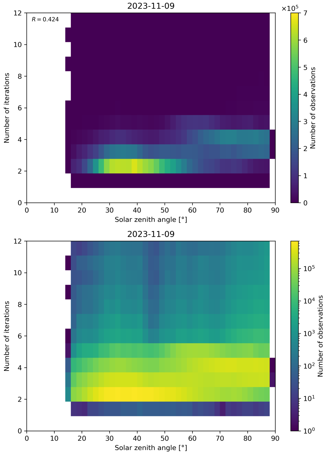
Figure 125: Scatter density plot of “Solar zenith angle” against “Number of iterations” for 2023-11-08 to 2023-11-10.
