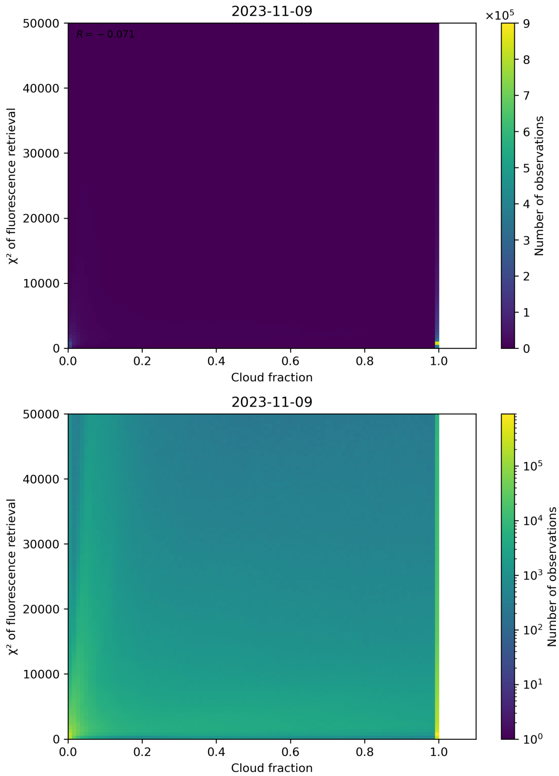
Figure 78: Scatter density plot of “Cloud fraction” against “ \chi^2 of fluorescence retrieval” for 2023-11-08 to 2023-11-10.
