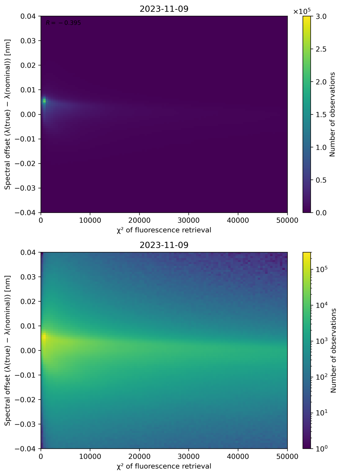
Figure 72: Scatter density plot of " \chi^2 of fluorescence retrieval" against "Spectral offset ( \lambda(\text{true}) - \lambda(\text{nominal})) " for 2023-11-08 to 2023-11-10.
