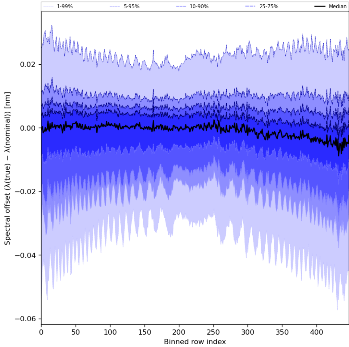
Figure 62: Along track statistics of “Spectral offset ( \lambda(\text{true}) - \lambda(\text{nominal}) )” for 2023-11-08 to 2023-11-10
