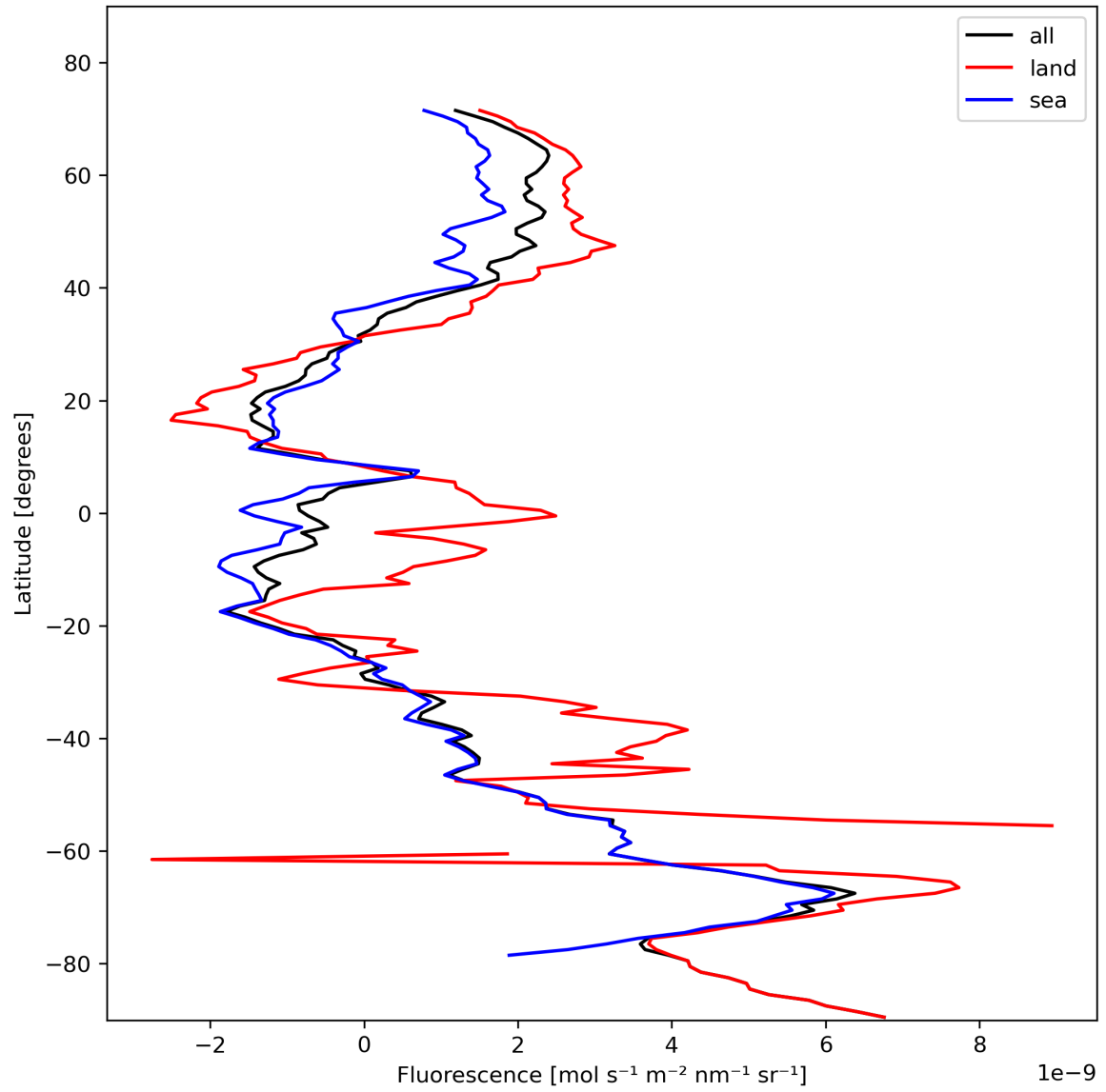
Figure 23: Zonal average of “Fluorescence” for 2023-11-08 to 2023-11-10.
