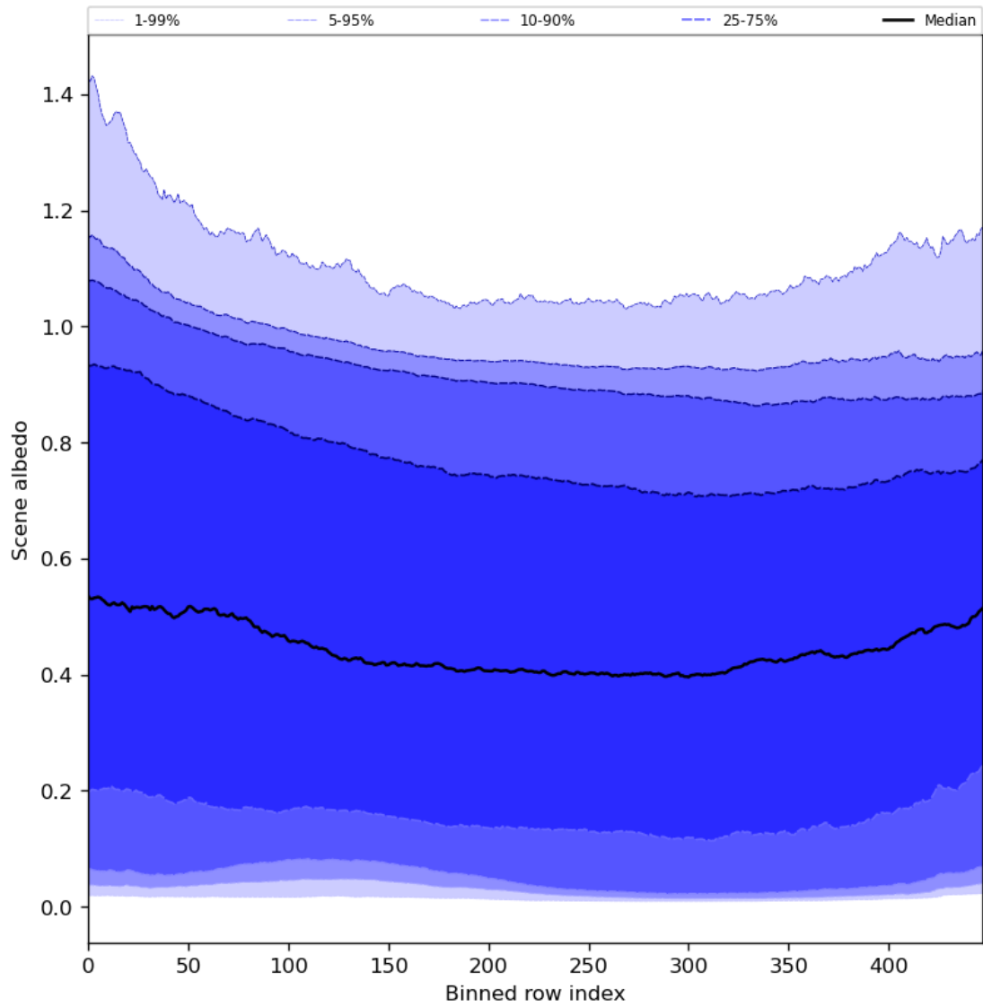
Figure 51: Along track statistics of “Scene albedo” for 2023-11-08 to 2023-11-10
