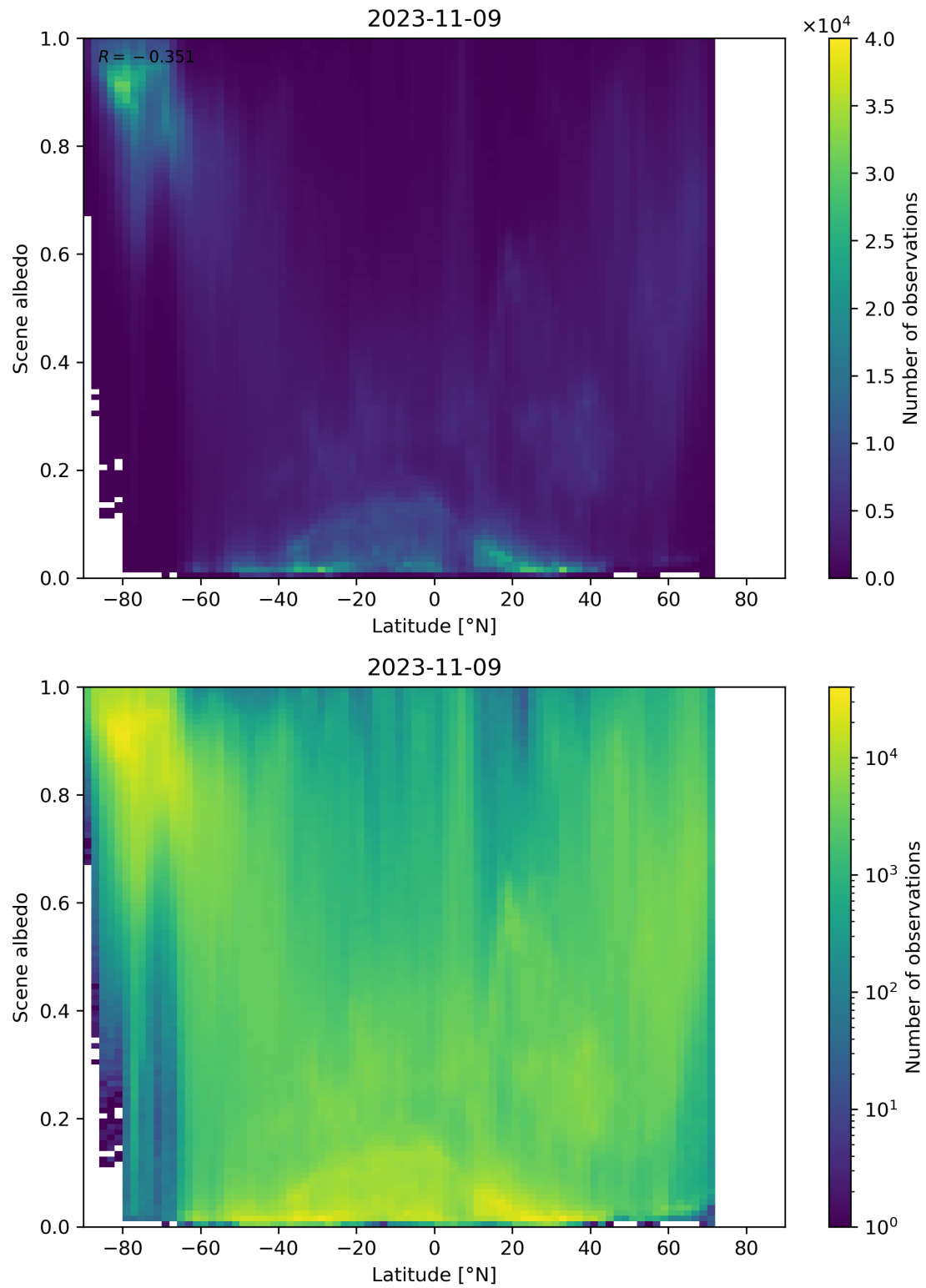
Figure 104: Scatter density plot of “Latitude” against “Scene albedo” for 2023-11-08 to 2023-11-10.
