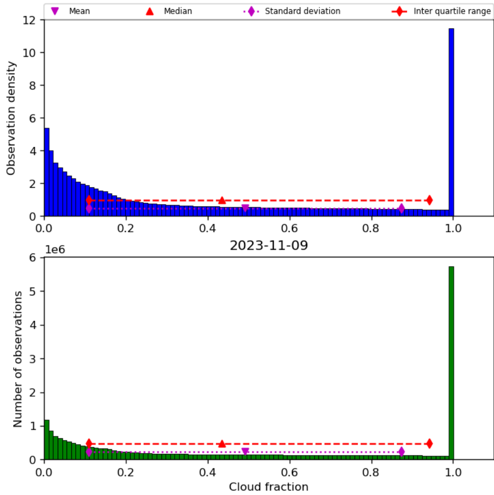
Figure 32: Histogram of “Cloud fraction” for 2023-11-08 to 2023-11-10
