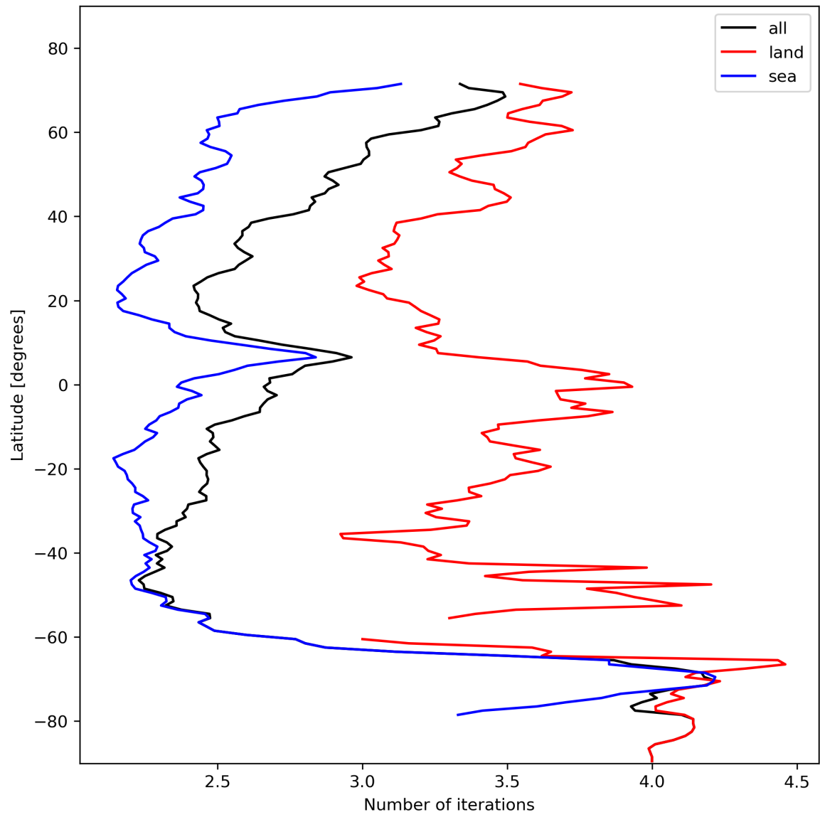
Figure 22: Zonal average of “Number of iterations” for 2023-11-08 to 2023-11-10.
