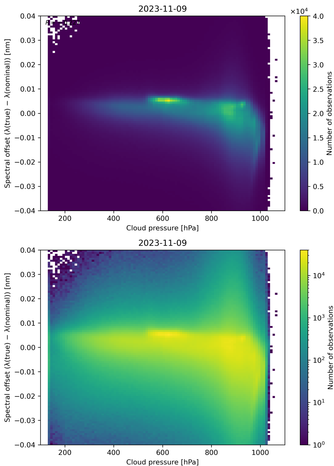
Figure 92: Scatter density plot of “Cloud pressure” against “Spectral offset ( \lambda(\text{true}) - \lambda(\text{nominal}) )” for 2023-11-08 to 2023-11-10.
