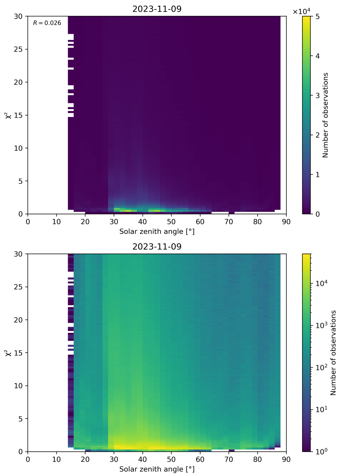
Figure 119: Scatter density plot of “Solar zenith angle” against “ \chi^2 ” for 2023-11-08 to 2023-11-10.
