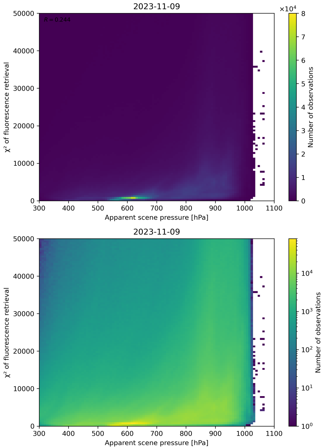
Figure 64: Scatter density plot of “Apparent scene pressure” against “ \chi^2 of fluorescence retrieval” for 2023-11-08 to 2023-11-10.
