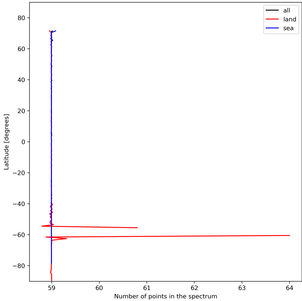
Figure 27: Zonal average of “Number of points in the spectrum” for 2023-11-08 to 2023-11-10.
