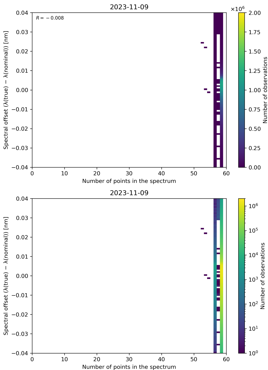
Figure 110: Scatter density plot of “Number of points in the spectrum” against “Spectral offset ( \lambda(\text{true}) - \lambda(\text{nominal}) )” for 2023-11-08 to 2023-11-10.
