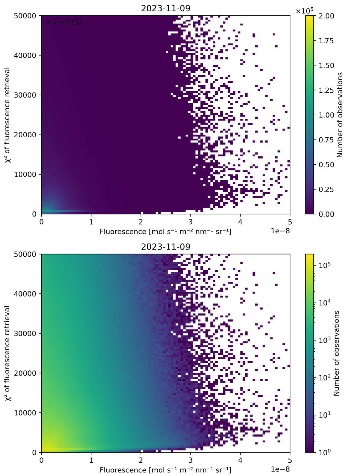
Figure 93: Scatter density plot of “Fluorescence” against “ \chi^2 of fluorescence retrieval” for 2023-11-08 to 2023-11-10.
