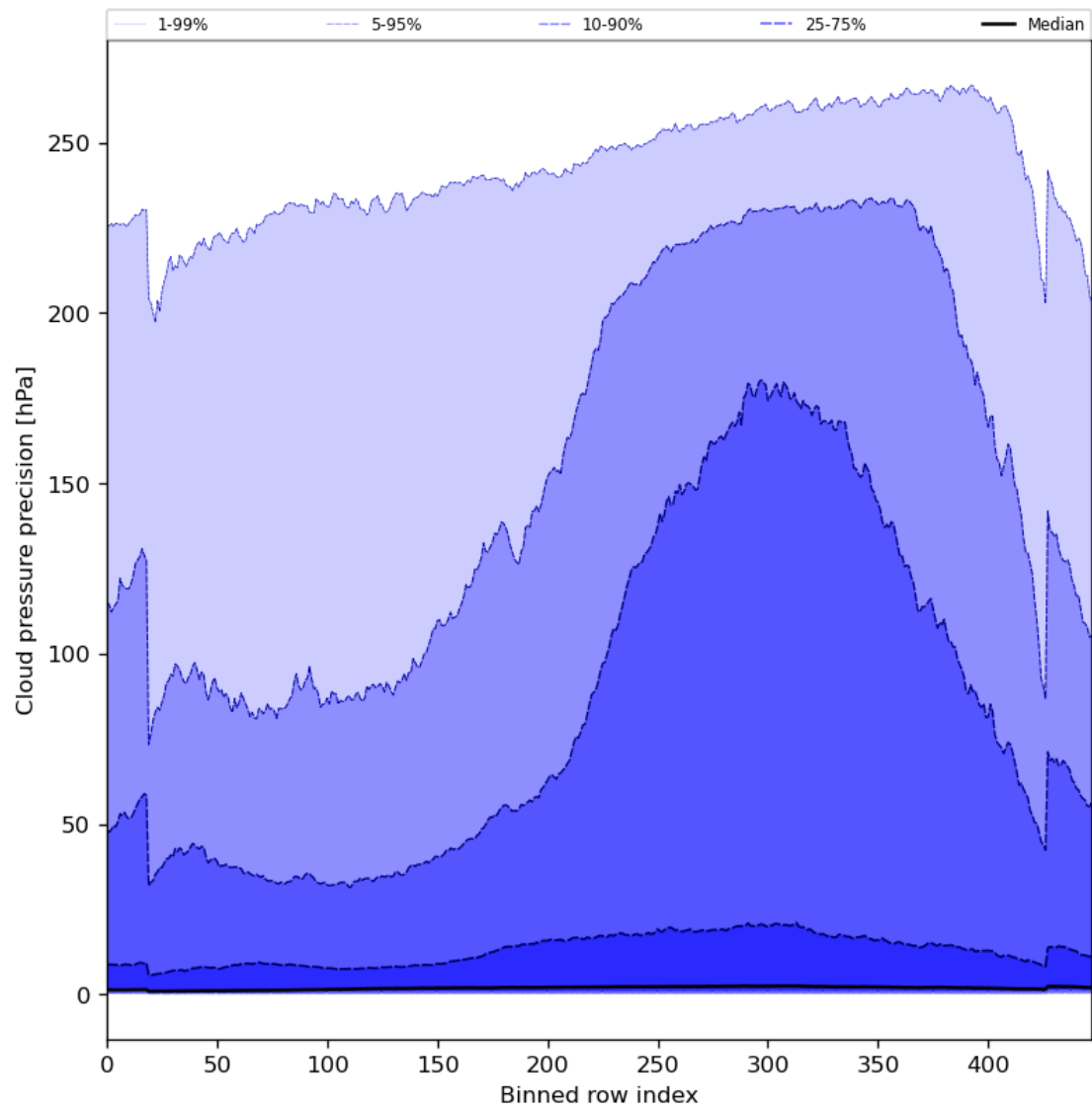
Figure 48: Along track statistics of “Cloud pressure precision” for 2023-11-08 to 2023-11-10
