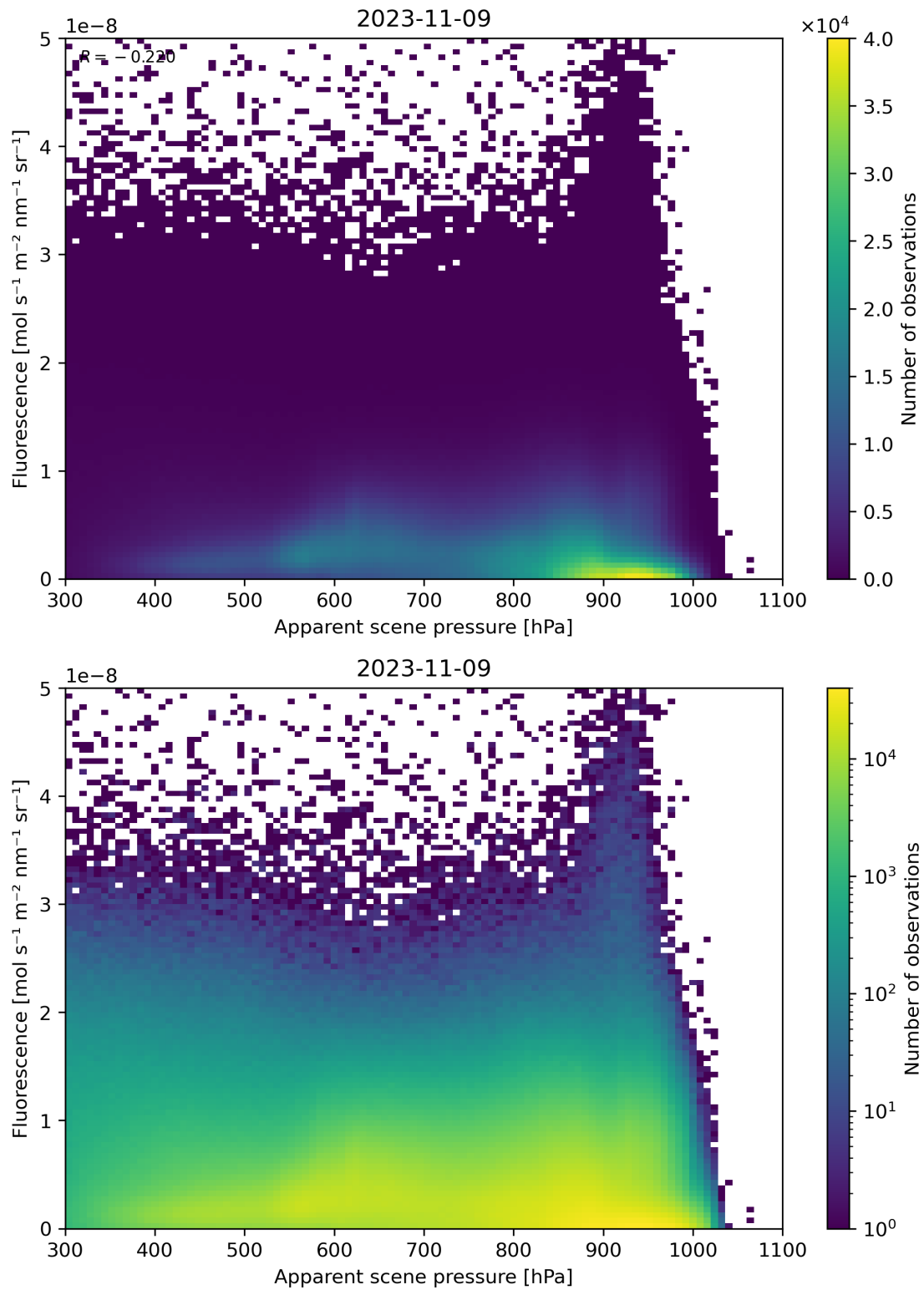
Figure 65: Scatter density plot of “Apparent scene pressure” against “Fluorescence” for 2023-11-08 to 2023-11-10.
