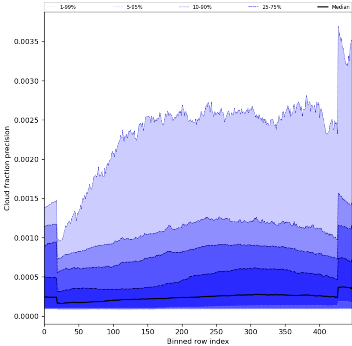
Figure 50: Along track statistics of “Cloud fraction precision” for 2023-11-08 to 2023-11-10
