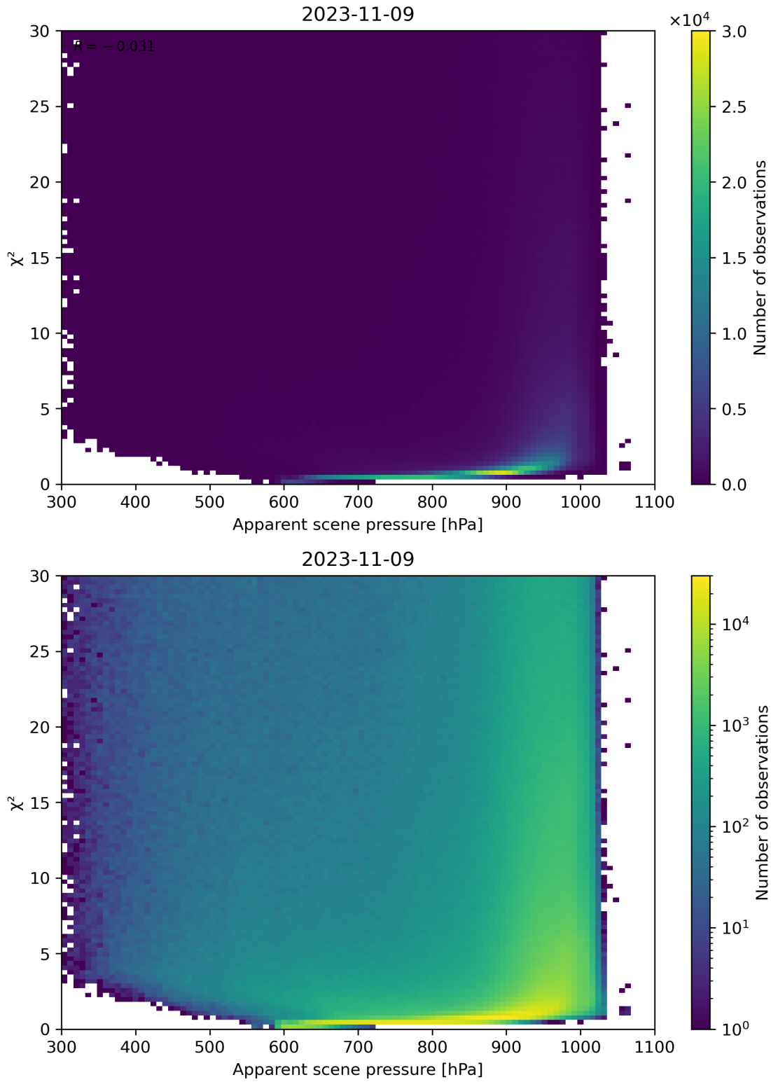
Figure 63: Scatter density plot of “Apparent scene pressure” against “ \chi^2 ” for 2023-11-08 to 2023-11-10.
