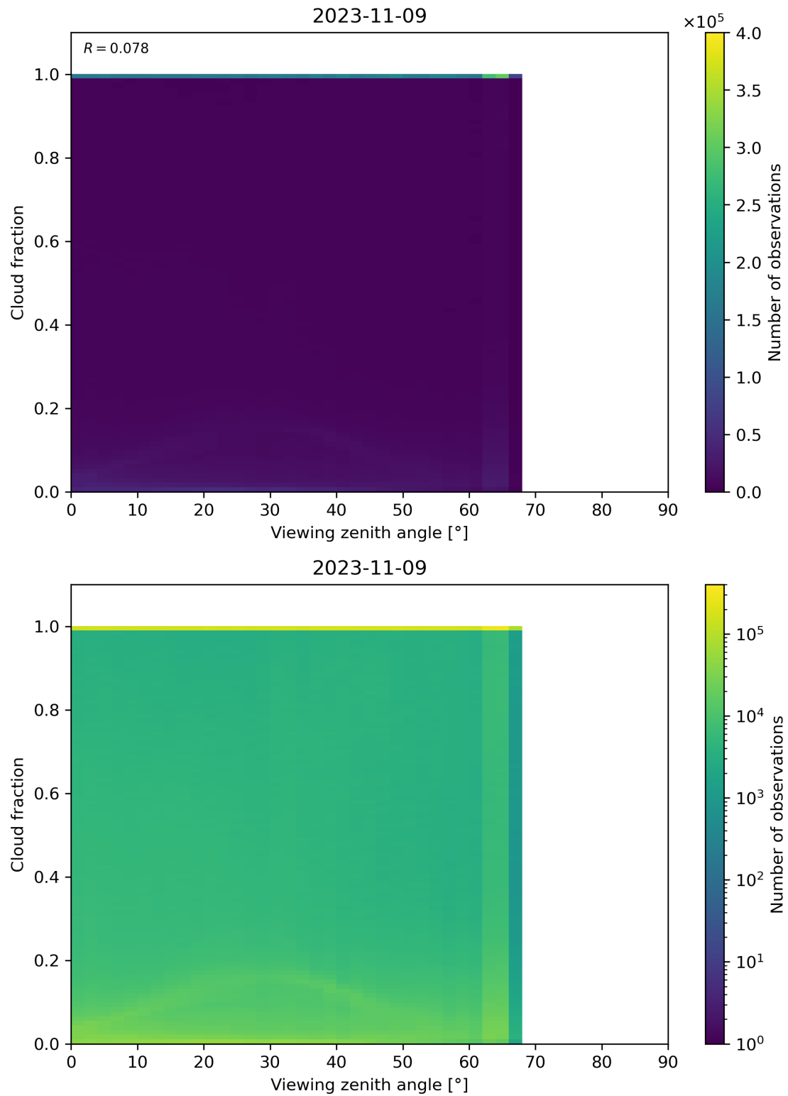
Figure 132: Scatter density plot of “Viewing zenith angle” against “Cloud fraction” for 2023-11-08 to 2023-11-10.
