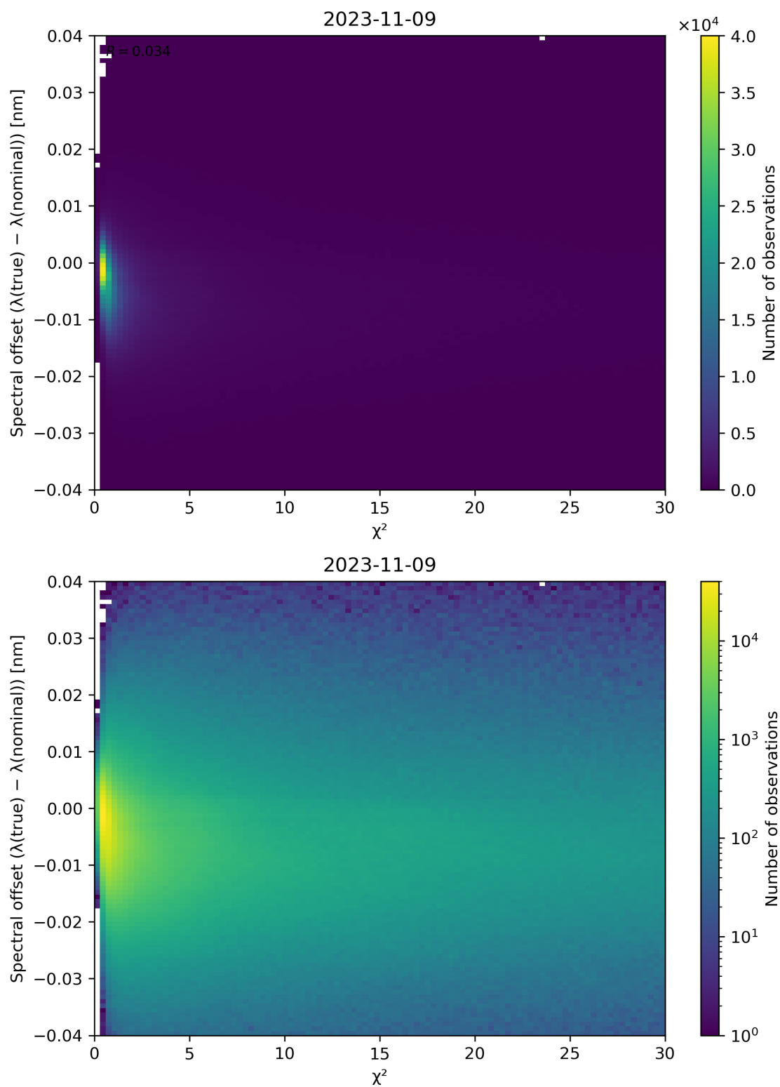
Figure 75: Scatter density plot of “ \chi^2 ” against “Spectral offset ( \lambda(\text{true}) - \lambda(\text{nominal}) )” for 2023-11-08 to 2023-11-10.
