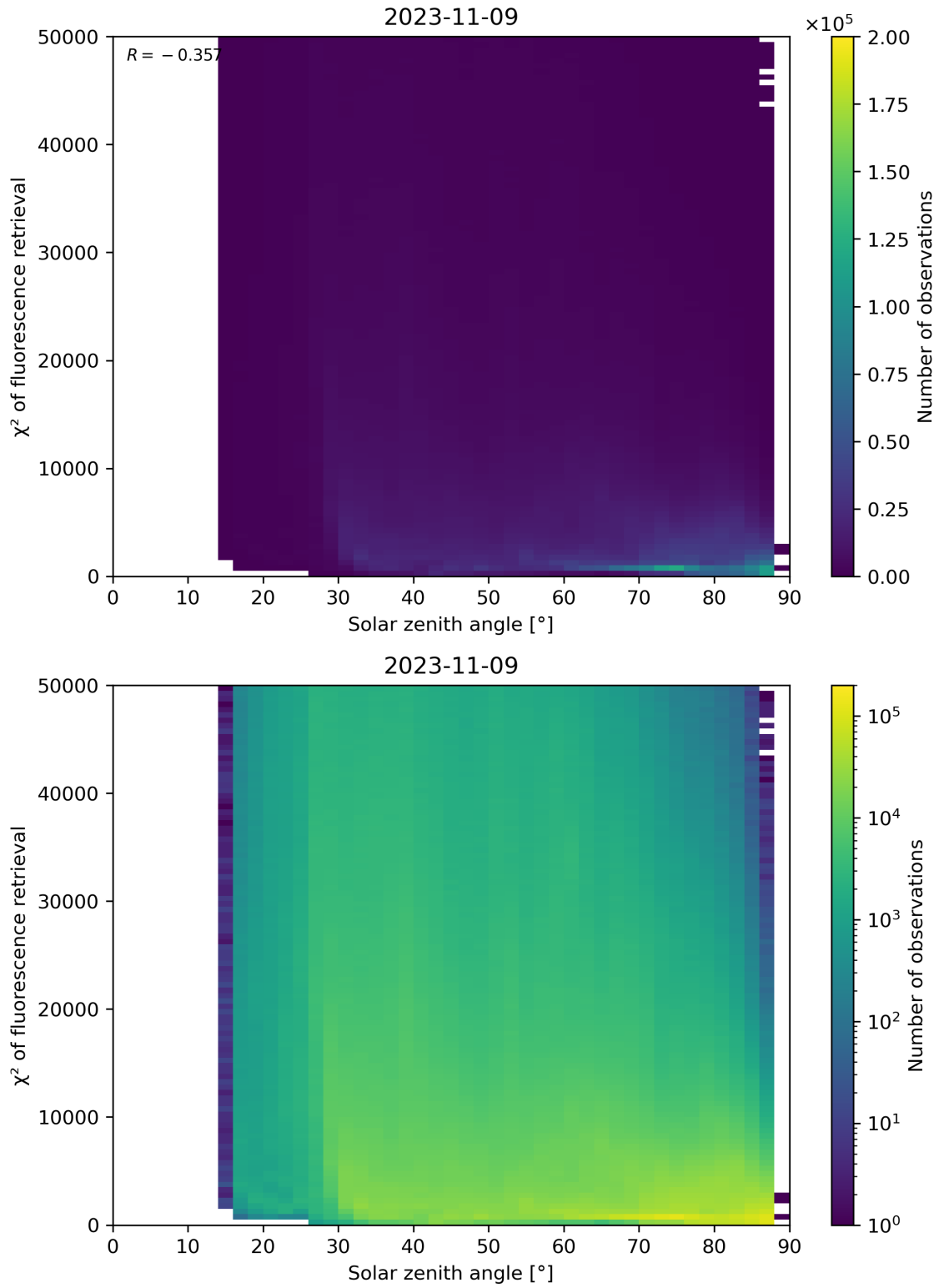
Figure 120: Scatter density plot of “Solar zenith angle” against “ \chi^2 of fluorescence retrieval” for 2023-11-08 to 2023-11-10.
