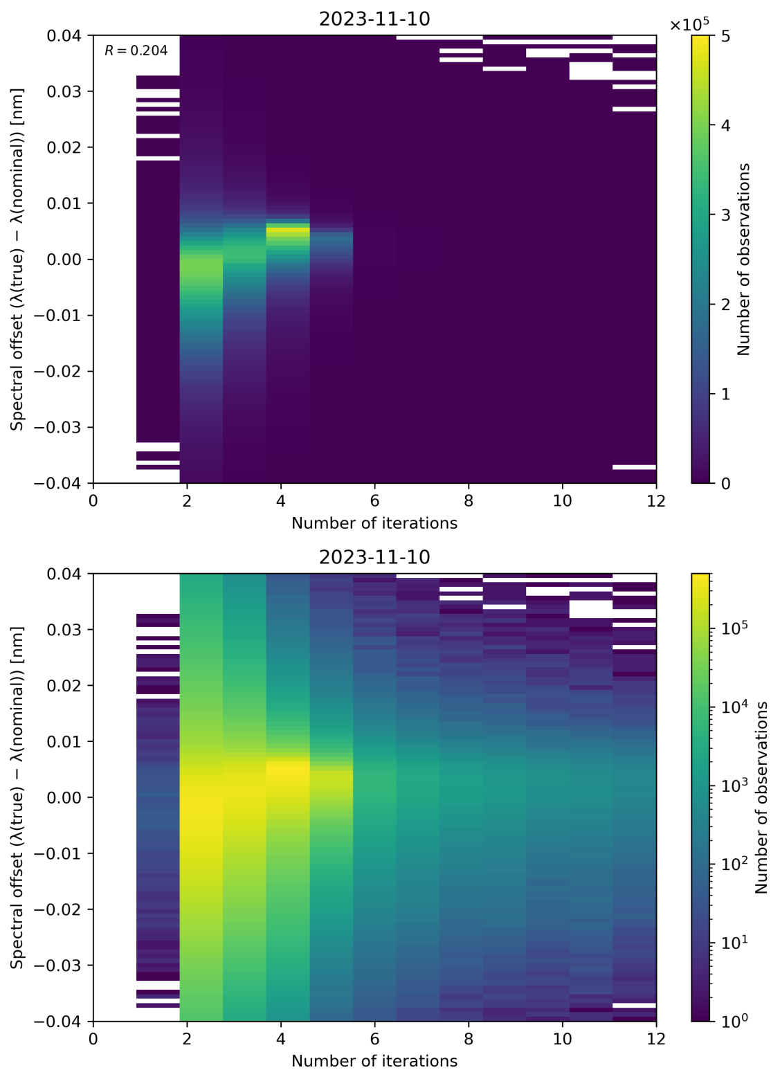
Figure 109: Scatter density plot of “Number of iterations” against “Spectral offset ( \lambda(\text{true}) - \lambda(\text{nominal}) )” for 2023-11-09 to 2023-11-11.
