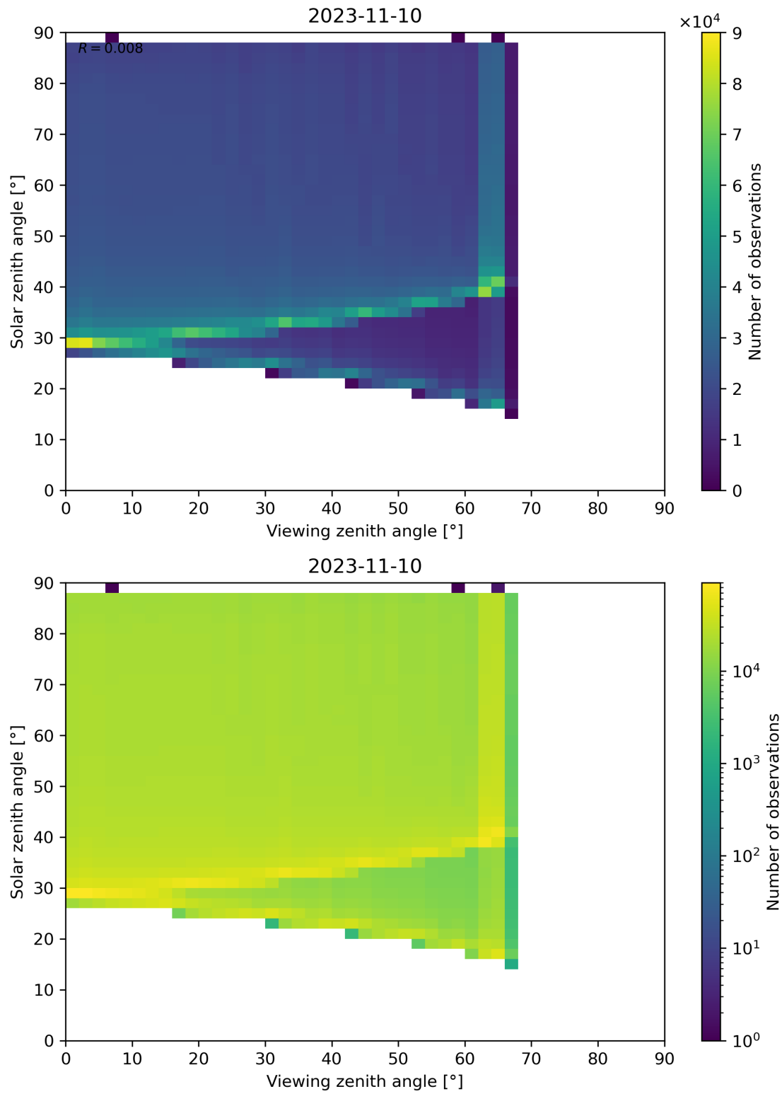
Figure 139: Scatter density plot of “Viewing zenith angle” against “Solar zenith angle” for 2023-11-09 to 2023-11-11.
