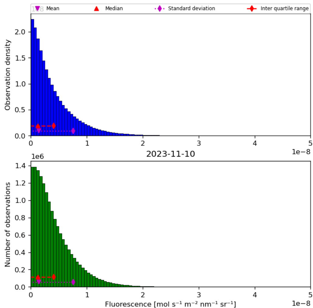
Figure 40: Histogram of “Fluorescence” for 2023-11-09 to 2023-11-11
