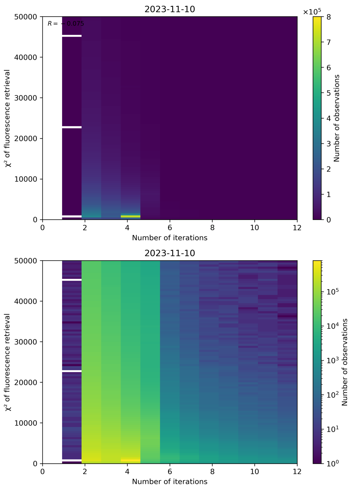
Figure 106: Scatter density plot of “Number of iterations” against “ \chi^2 of fluorescence retrieval” for 2023-11-09 to 2023-11-11.
