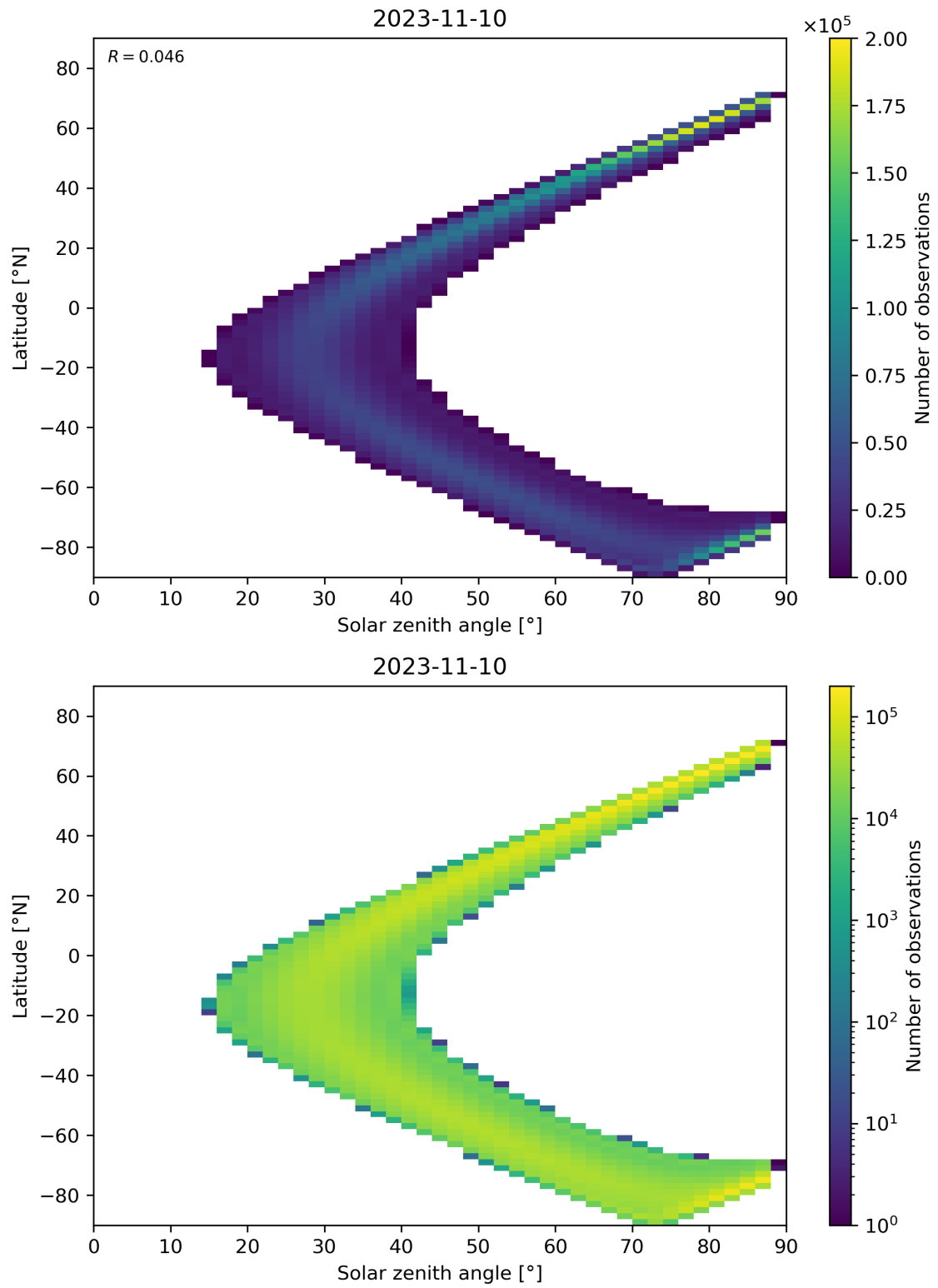
Figure 124: Scatter density plot of “Solar zenith angle” against “Latitude” for 2023-11-09 to 2023-11-11.
