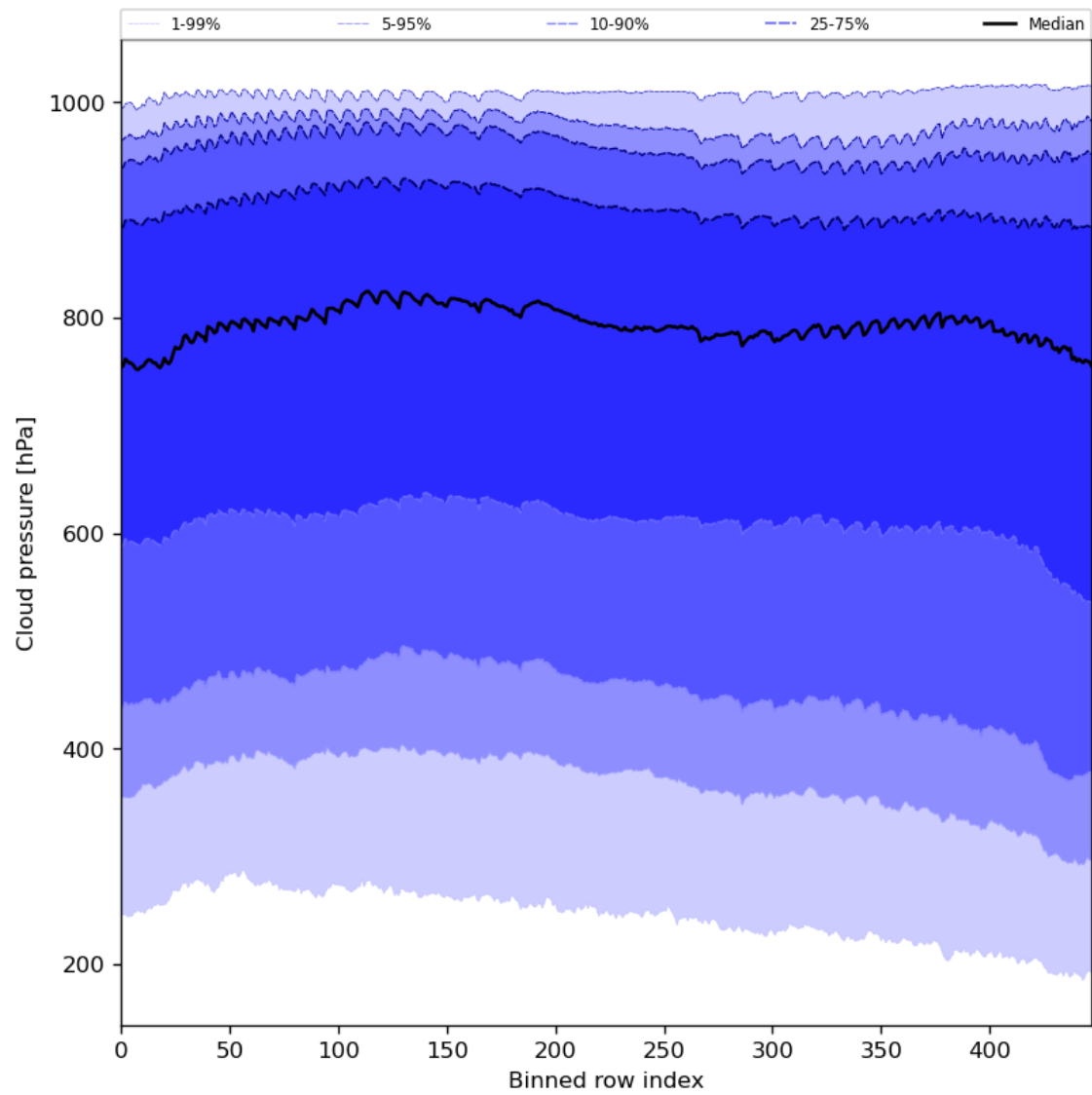
Figure 47: Along track statistics of “Cloud pressure” for 2023-11-09 to 2023-11-11
