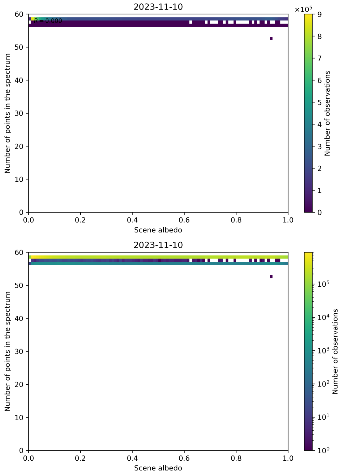
Figure 116: Scatter density plot of “Scene albedo” against “Number of points in the spectrum” for 2023-11-09 to 2023-11-11.
