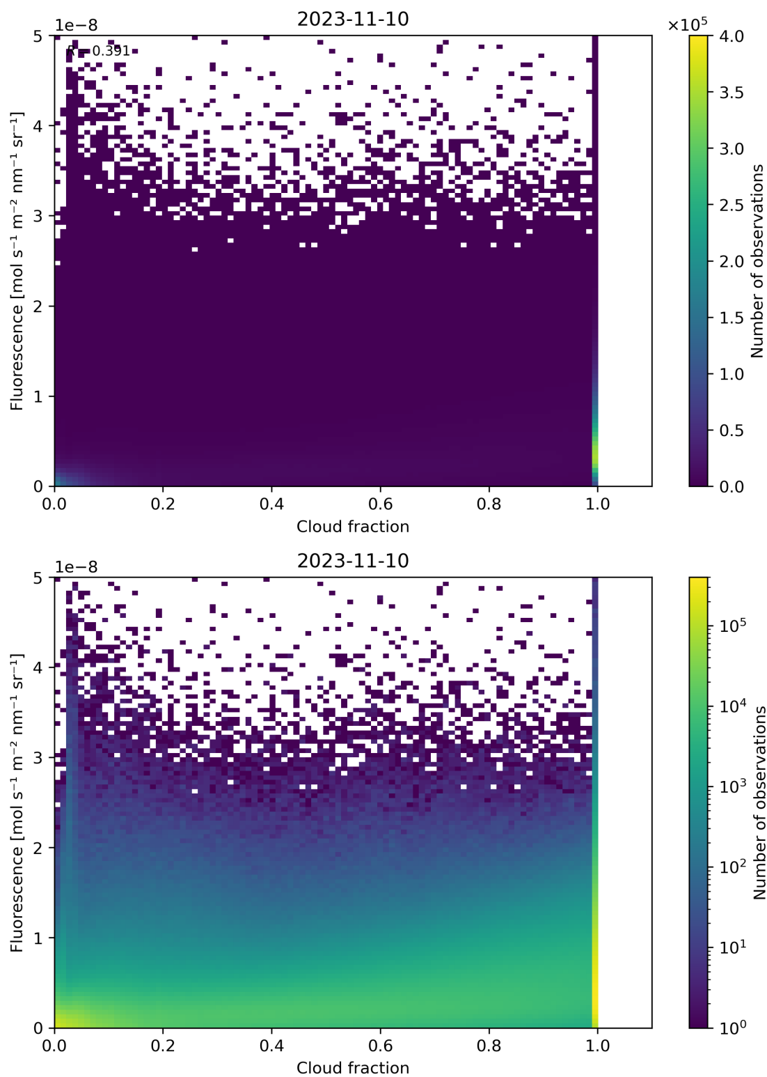
Figure 79: Scatter density plot of “Cloud fraction” against “Fluorescence” for 2023-11-09 to 2023-11-11.
