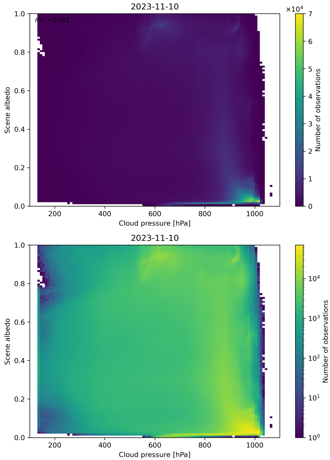
Figure 91: Scatter density plot of “Cloud pressure” against “Scene albedo” for 2023-11-09 to 2023-11-11.
