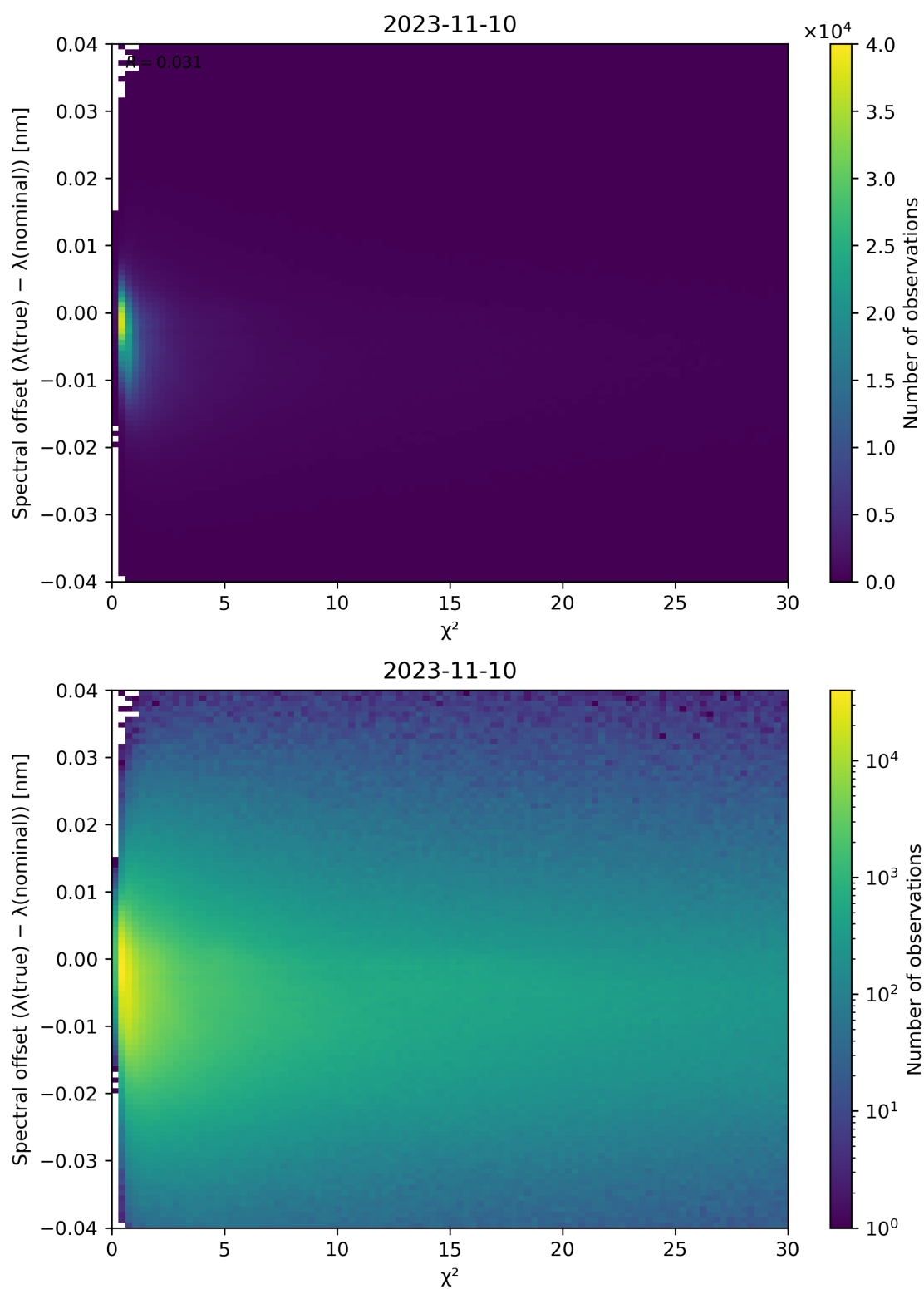
Figure 75: Scatter density plot of " \chi^2 " against "Spectral offset ( \lambda(\text{true}) - \lambda(\text{nominal}) )" for 2023-11-09 to 2023-11-11.
