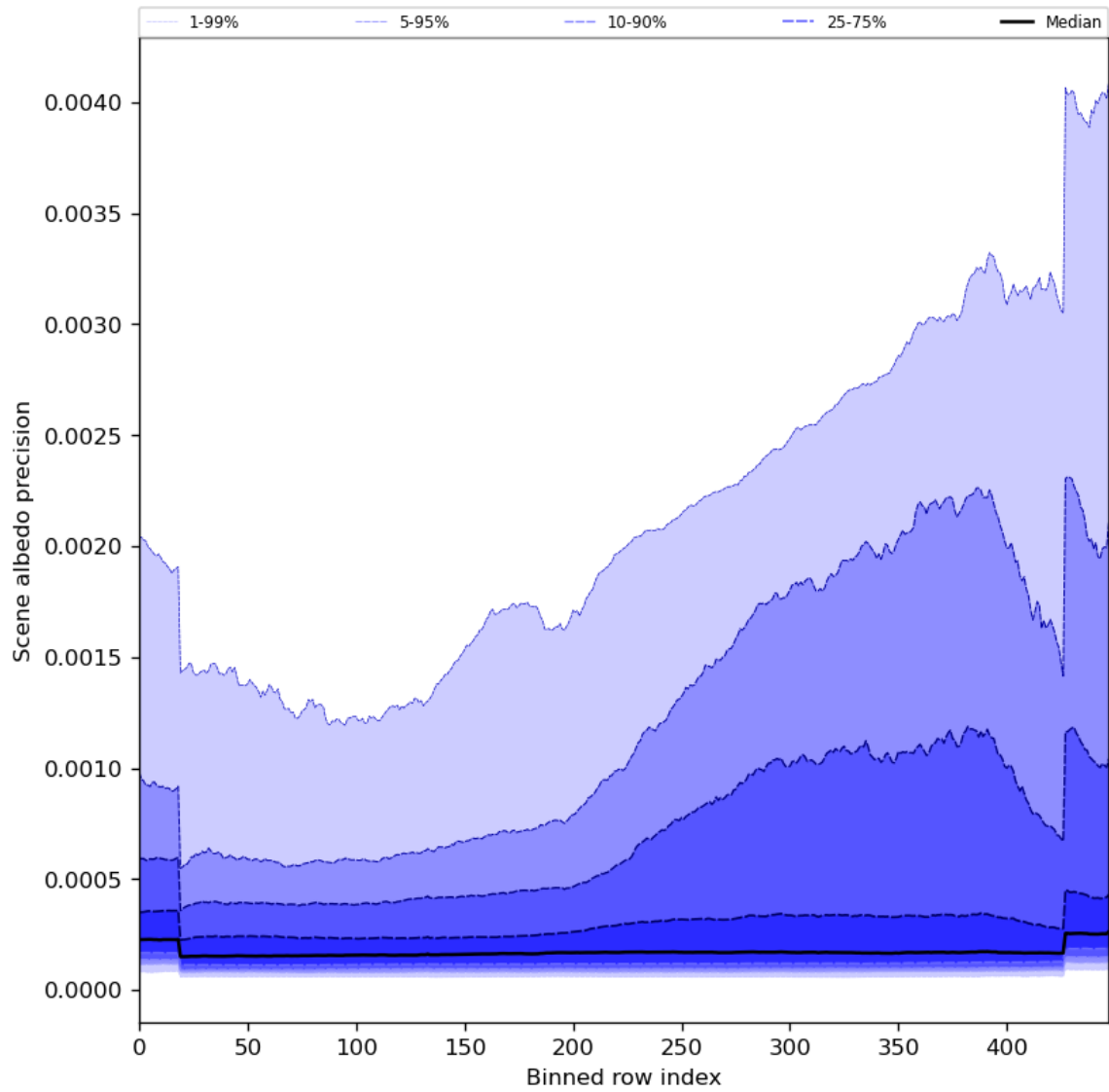
Figure 52: Along track statistics of “Scene albedo precision” for 2023-11-09 to 2023-11-11
