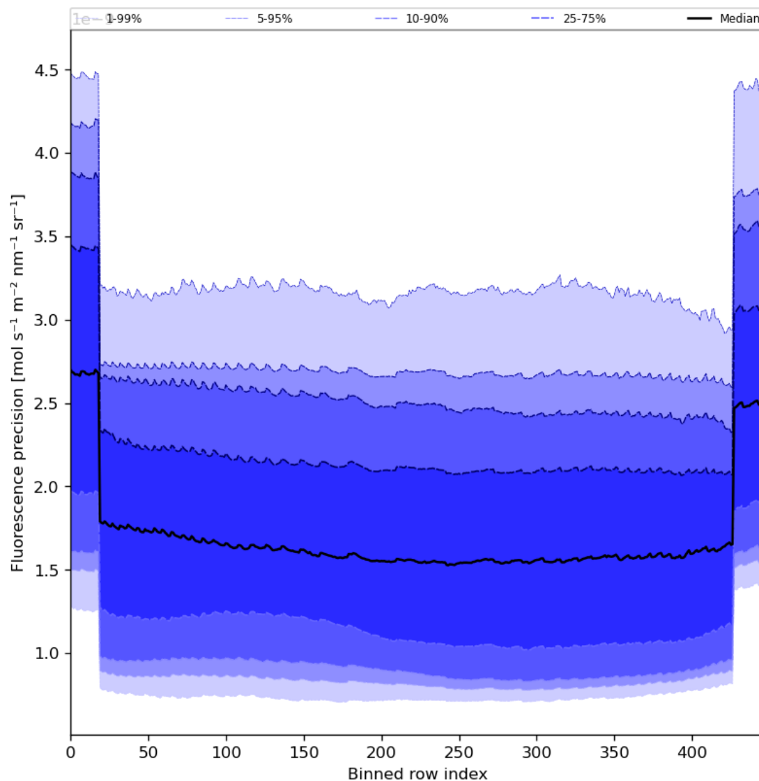
Figure 58: Along track statistics of “Fluorescence precision” for 2023-11-09 to 2023-11-11
