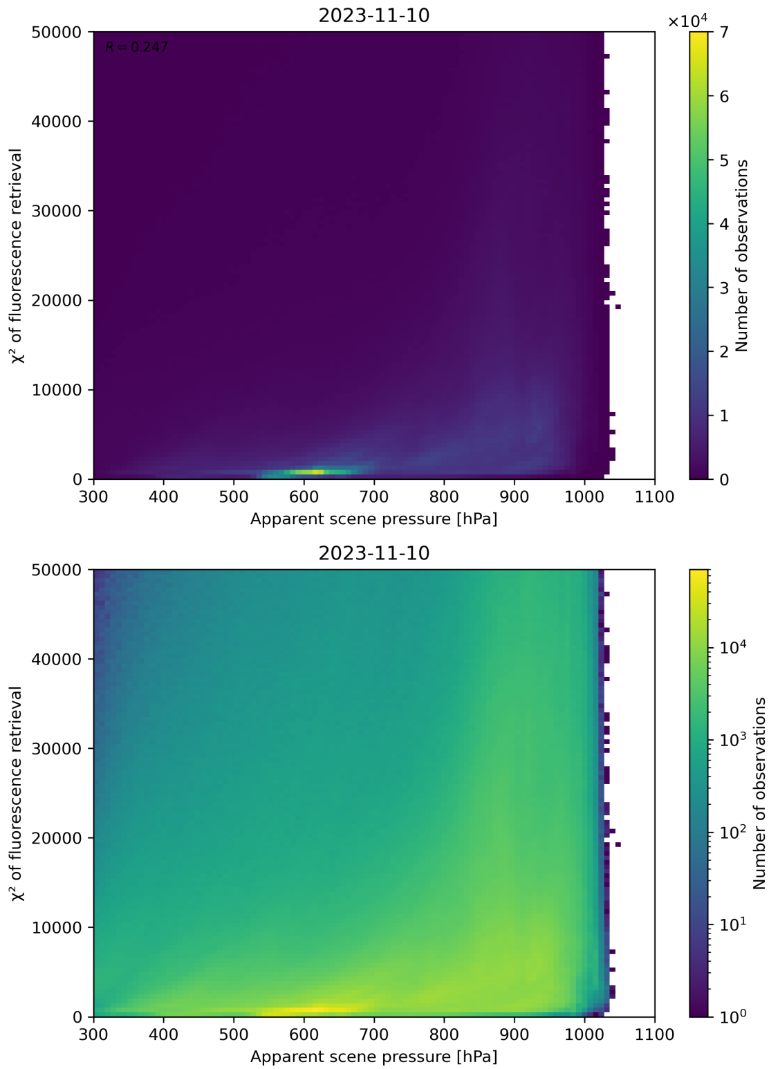
Figure 64: Scatter density plot of “Apparent scene pressure” against “ \chi^2 of fluorescence retrieval” for 2023-11-09 to 2023-11-11.
