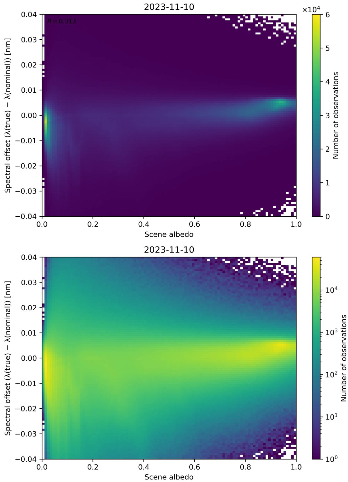
Figure 117: Scatter density plot of “Scene albedo” against “Spectral offset ( \lambda(\text{true}) - \lambda(\text{nominal}) )” for 2023-11-09 to 2023-11-11.
