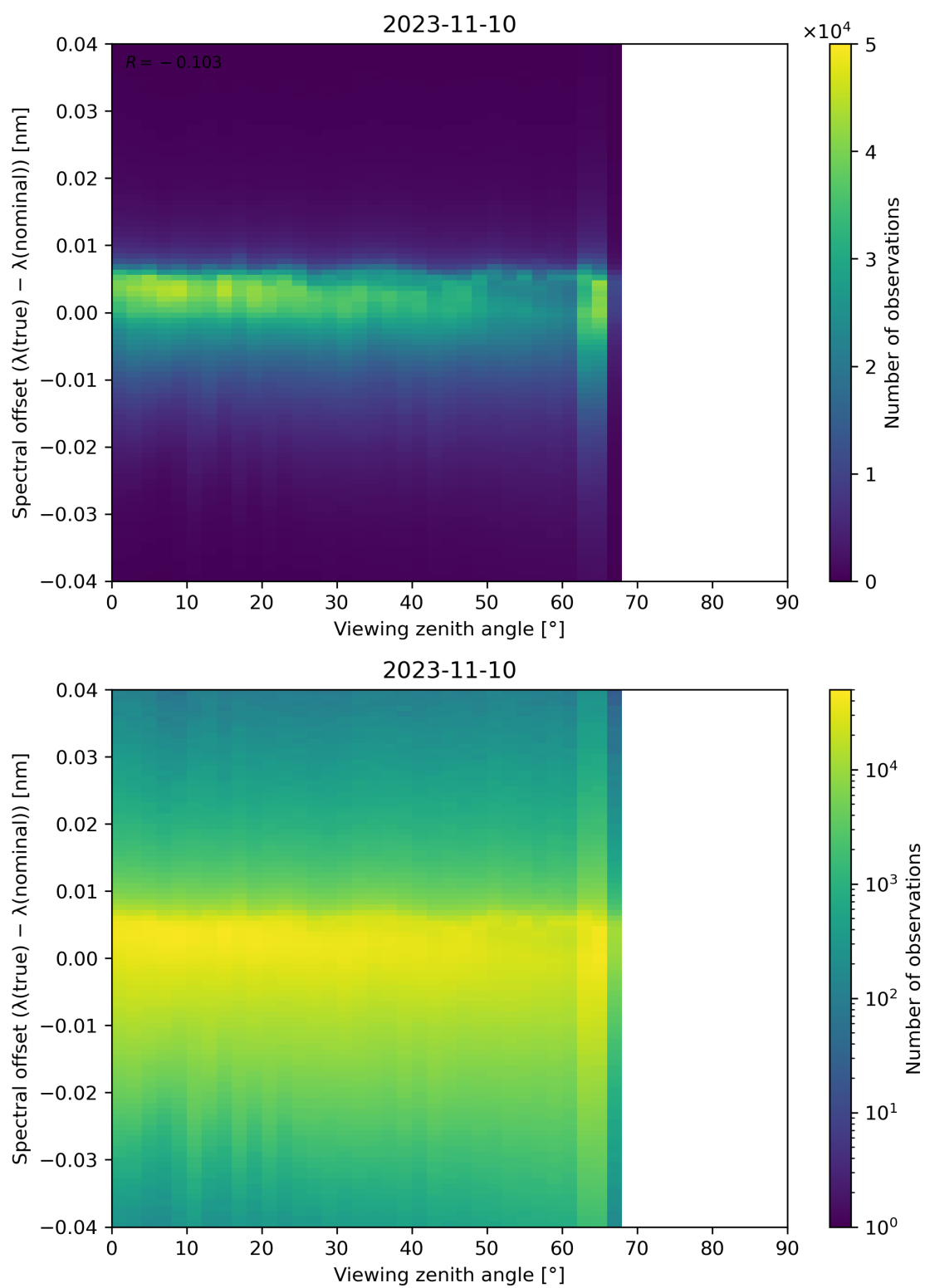
Figure 140: Scatter density plot of “Viewing zenith angle” against “Spectral offset ( \lambda(\text{true}) - \lambda(\text{nominal}) )” for 2023-11-09 to 2023-11-11.
