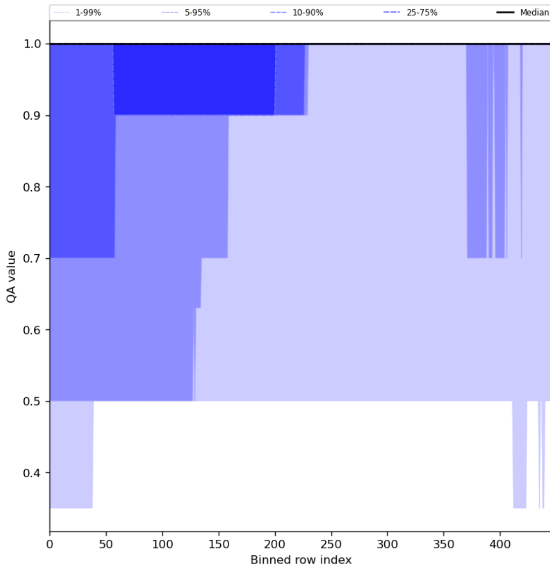
Figure 46: Along track statistics of “QA value” for 2023-11-09 to 2023-11-11
