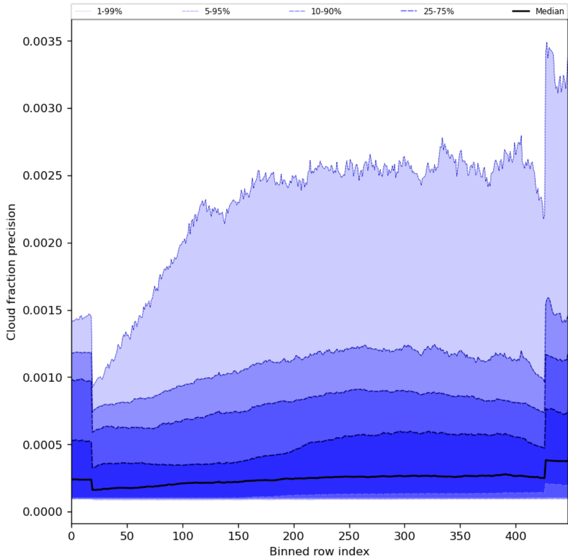
Figure 50: Along track statistics of “Cloud fraction precision” for 2023-11-09 to 2023-11-11
