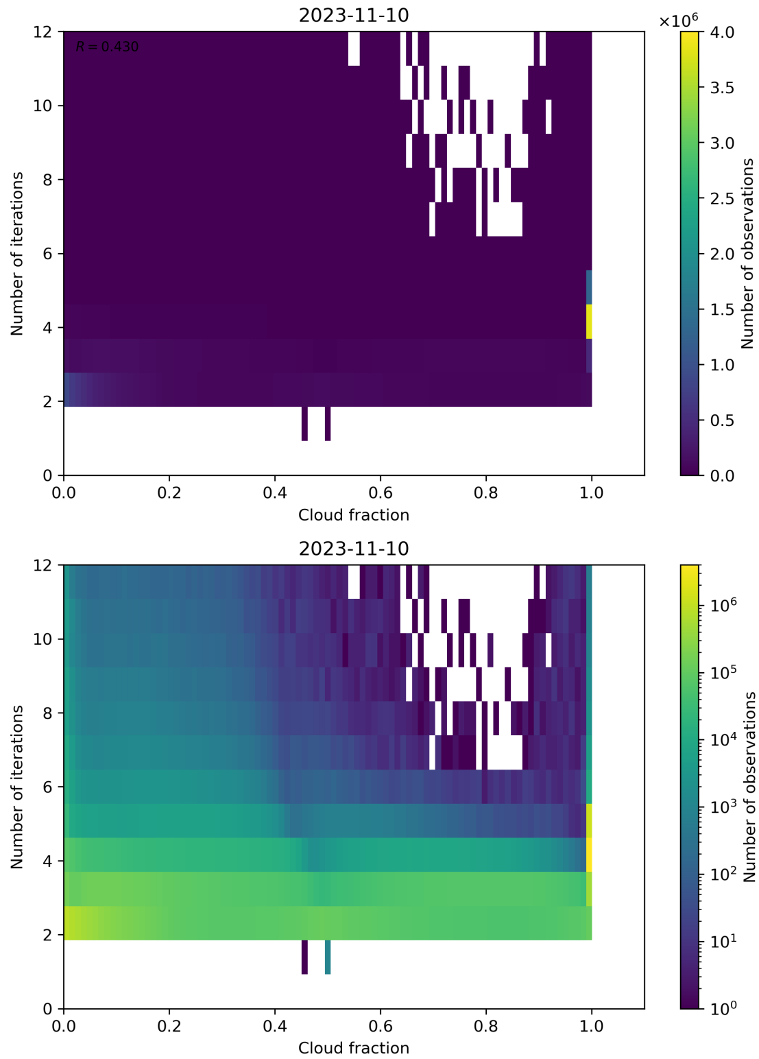
Figure 80: Scatter density plot of “Cloud fraction” against “Number of iterations” for 2023-11-09 to 2023-11-11.
