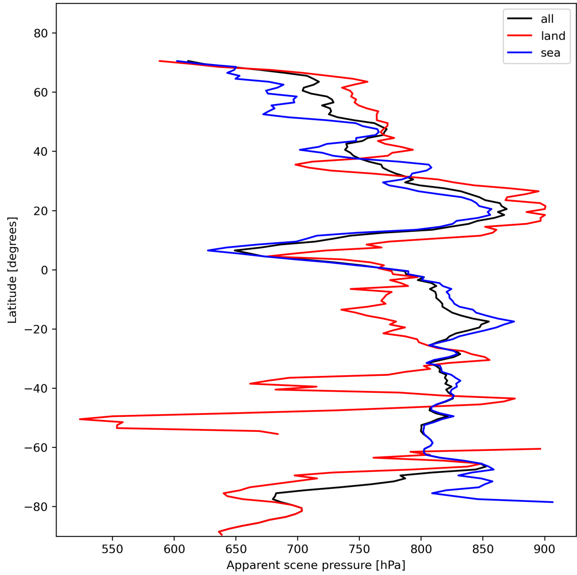
Figure 19: Zonal average of “Apparent scene pressure” for 2023-11-09 to 2023-11-11.
