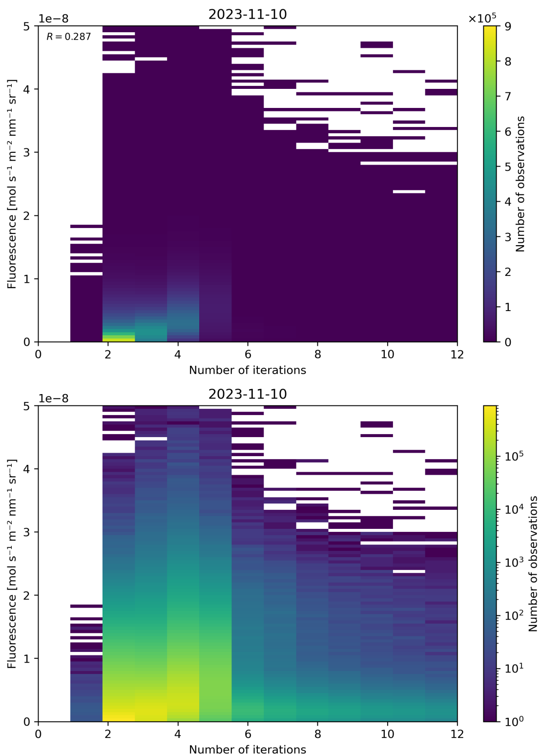
Figure 107: Scatter density plot of “Number of iterations” against “Fluorescence” for 2023-11-09 to 2023-11-11.
