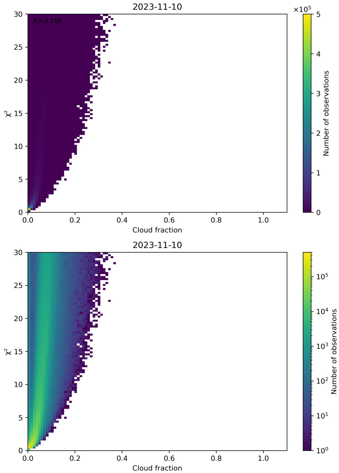
Figure 77: Scatter density plot of “Cloud fraction” against “ \chi^2 ” for 2023-11-09 to 2023-11-11.
