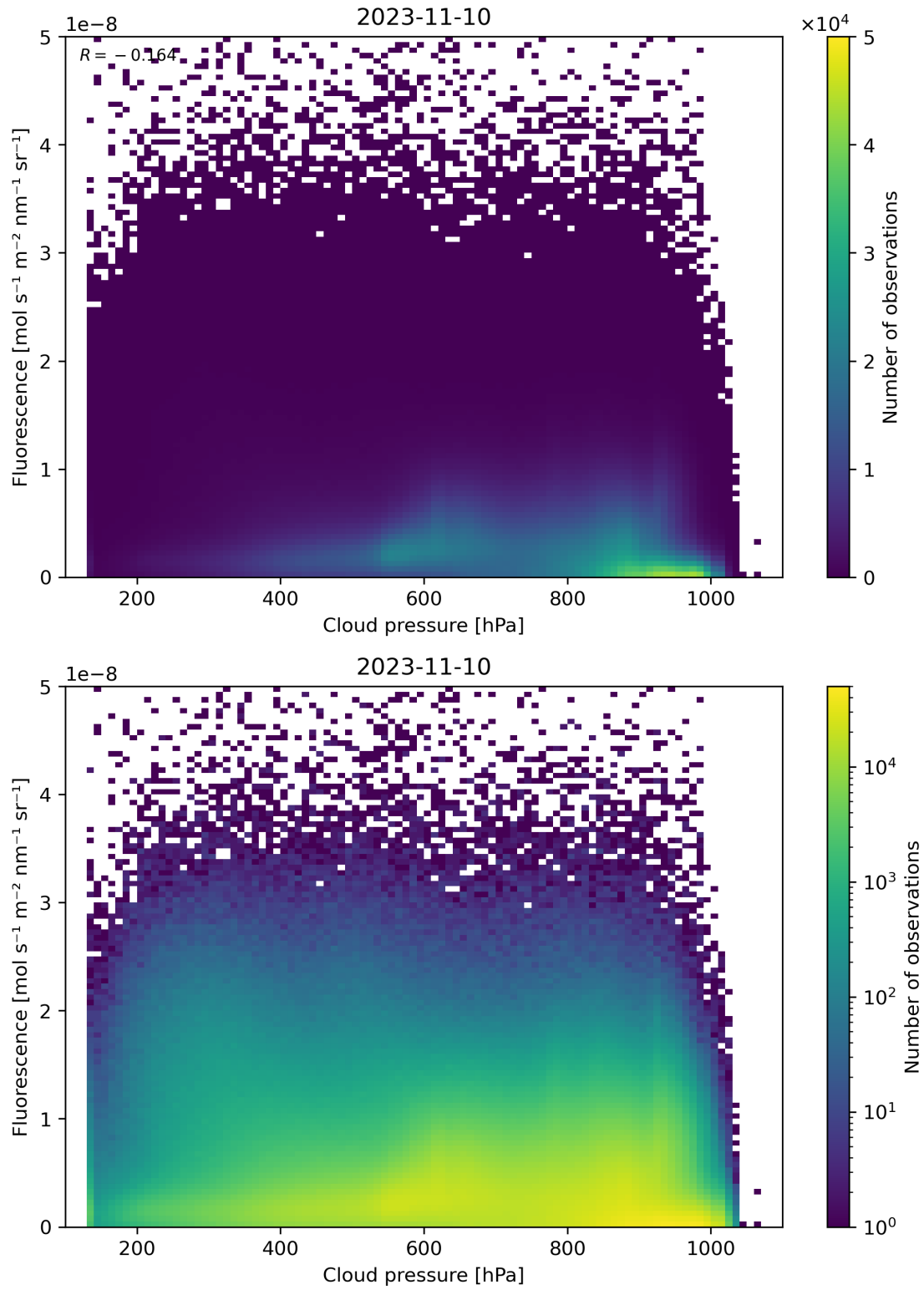
Figure 88: Scatter density plot of “Cloud pressure” against “Fluorescence” for 2023-11-09 to 2023-11-11.
