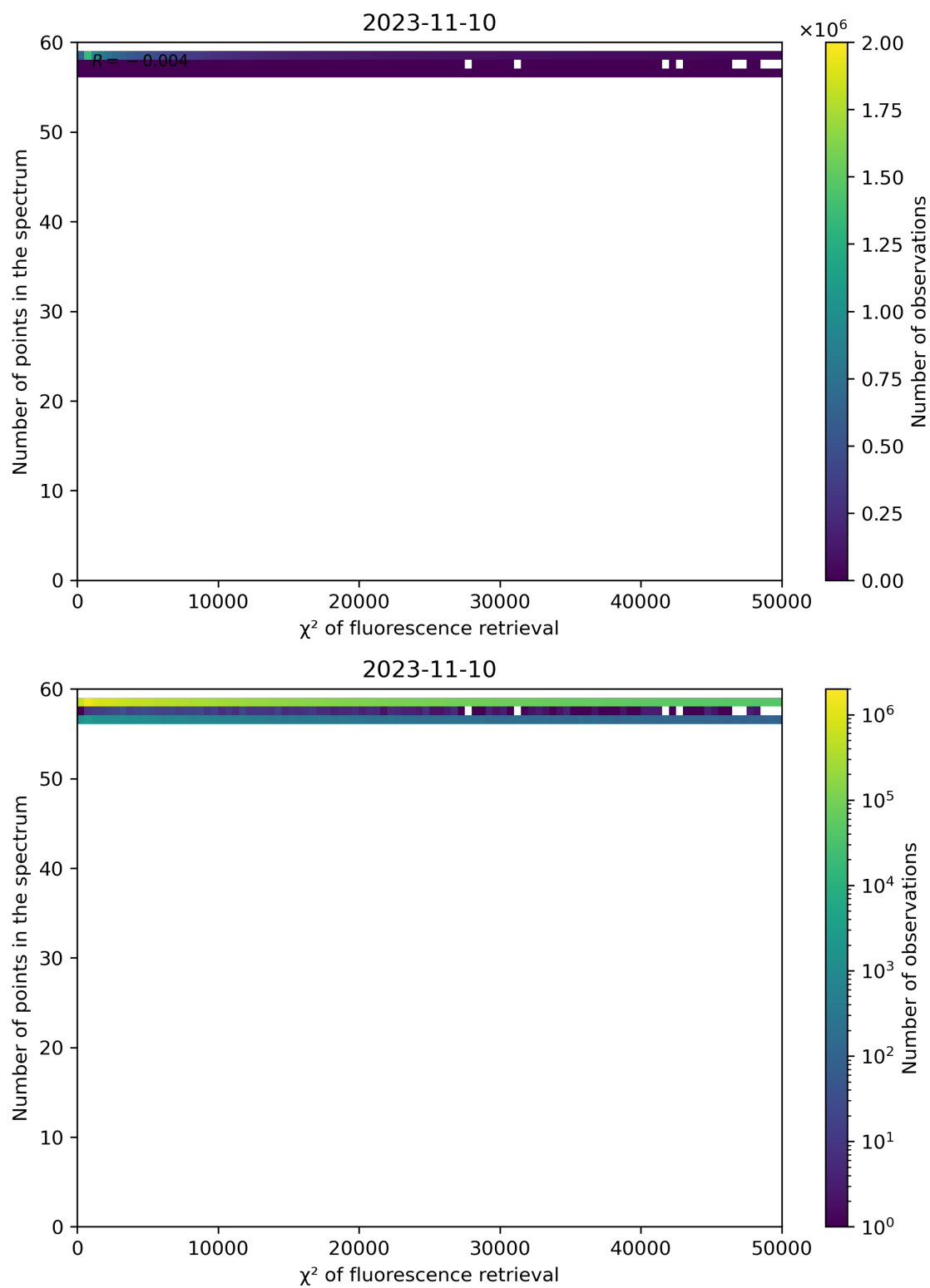
Figure 71: Scatter density plot of “ \chi^2 of fluorescence retrieval” against “Number of points in the spectrum” for 2023-11-09 to 2023-11-11.
