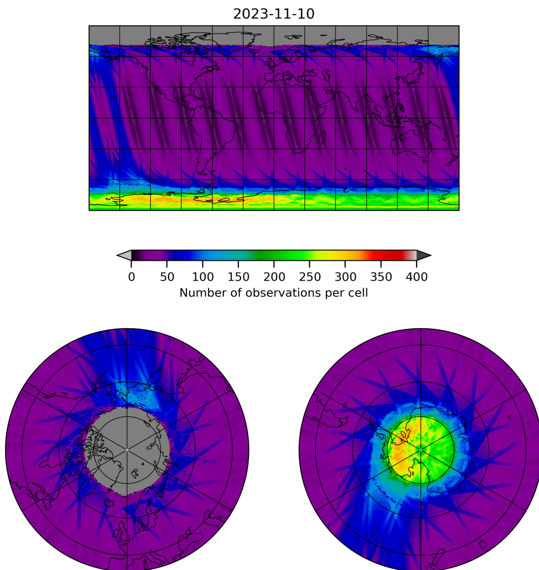
Figure 11: Map of the number of observations for 2023-11-09 to 2023-11-11
