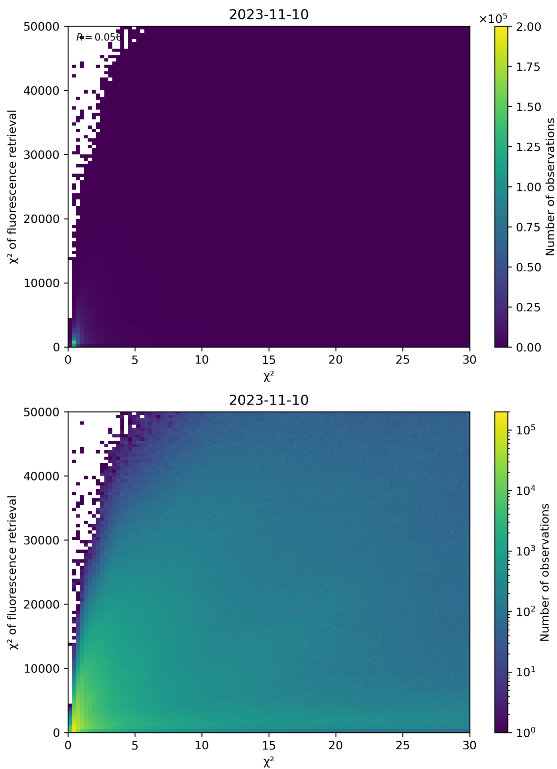
Figure 69: Scatter density plot of “ \chi^2 ” against “ \chi^2 of fluorescence retrieval” for 2023-11-09 to 2023-11-11.
