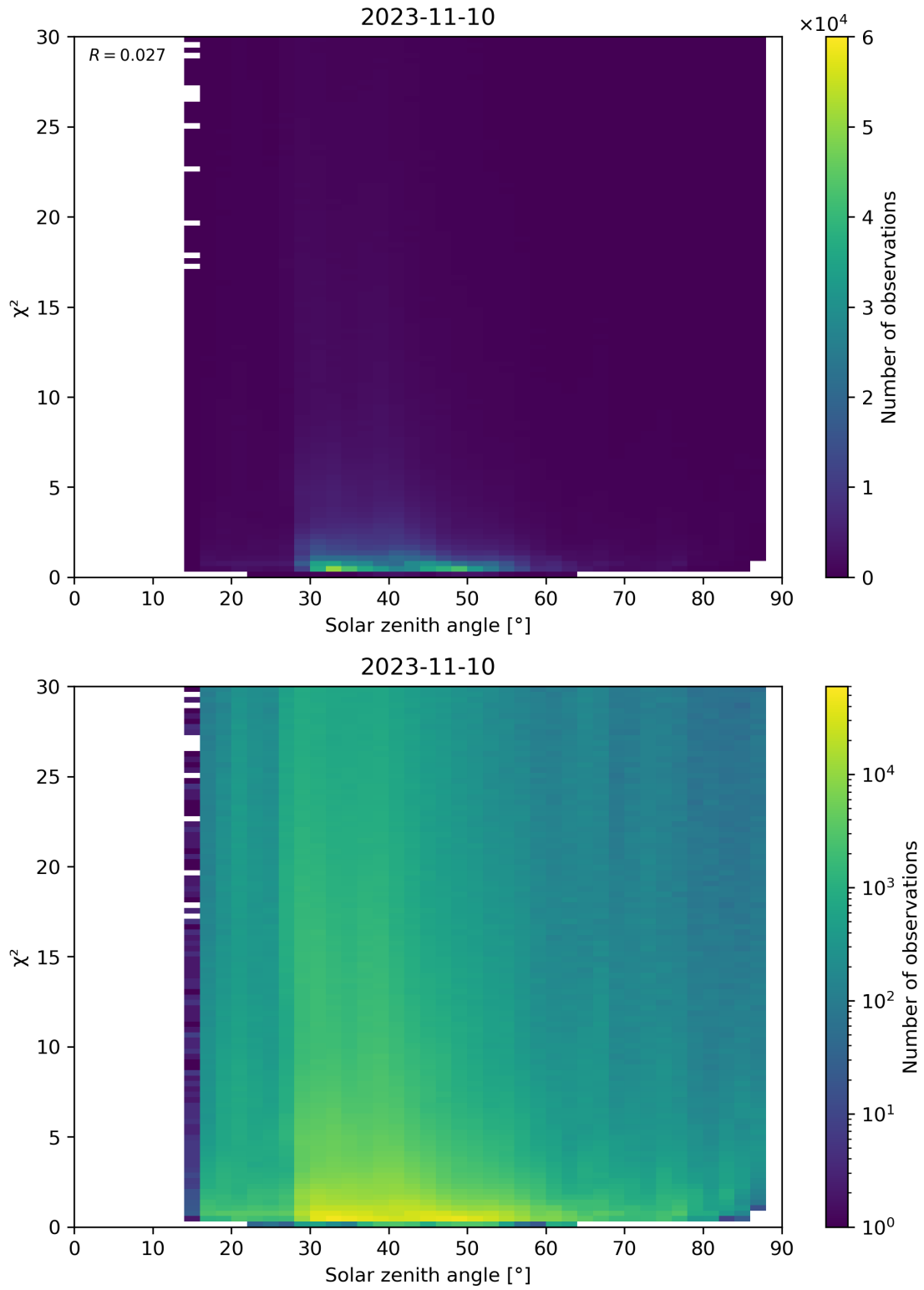
Figure 119: Scatter density plot of “Solar zenith angle” against “ \chi^2 ” for 2023-11-09 to 2023-11-11.
