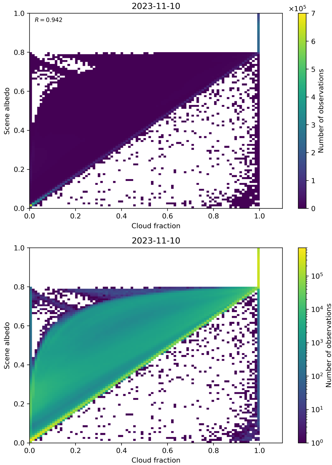
Figure 82: Scatter density plot of “Cloud fraction” against “Scene albedo” for 2023-11-09 to 2023-11-11.
