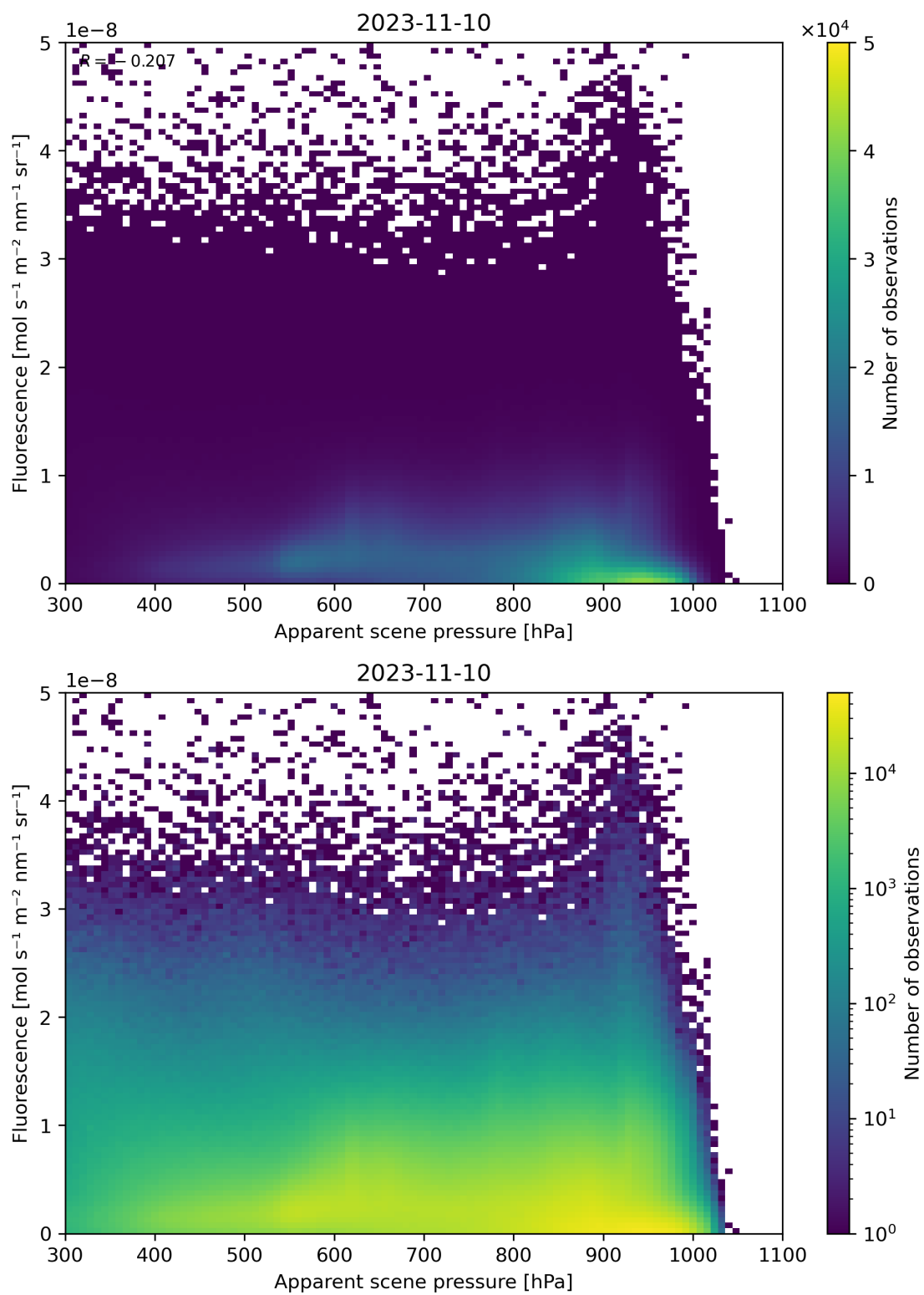
Figure 65: Scatter density plot of “Apparent scene pressure” against “Fluorescence” for 2023-11-09 to 2023-11-11.
