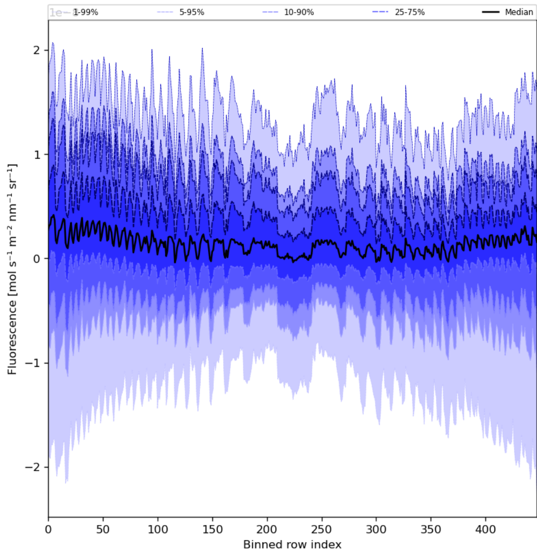
Figure 57: Along track statistics of “Fluorescence” for 2023-11-09 to 2023-11-11
