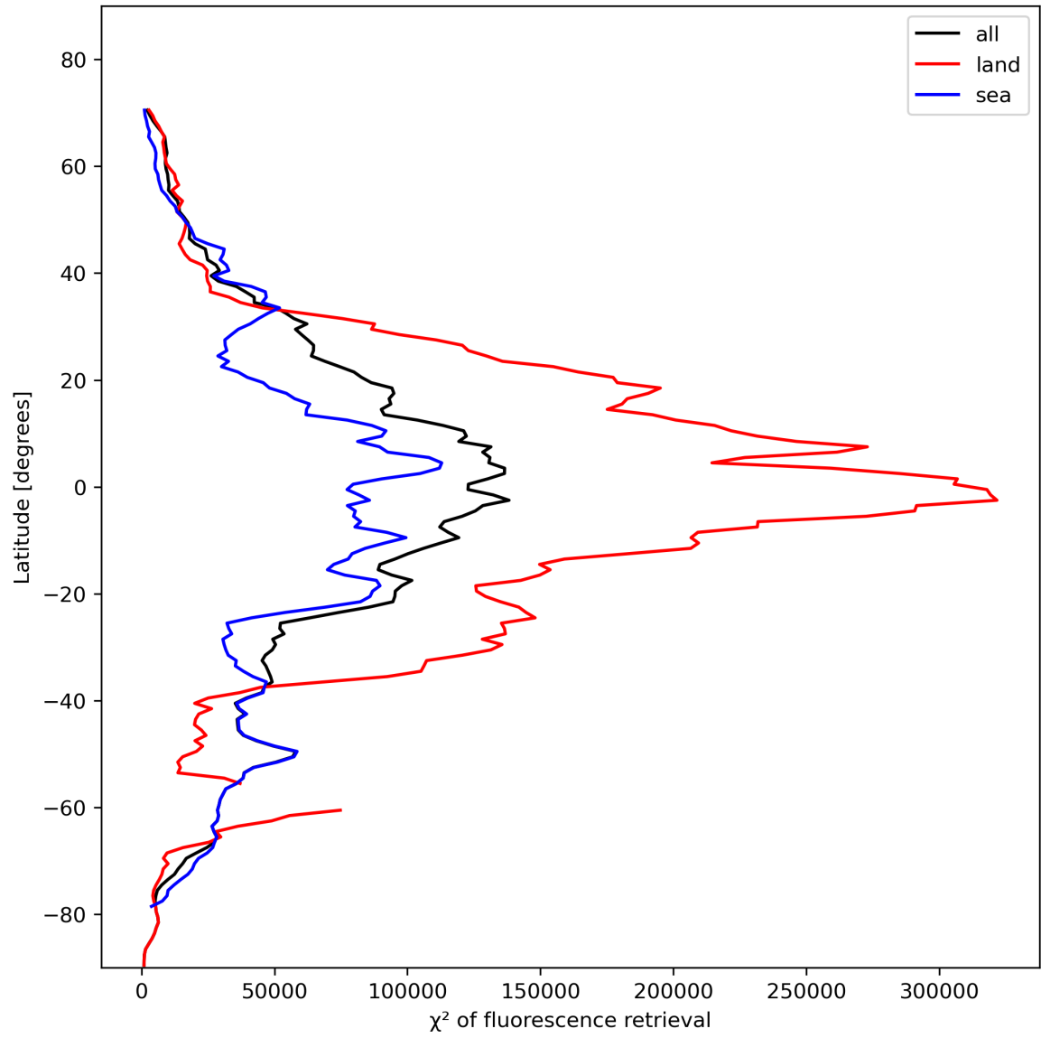
Figure 25: Zonal average of “ \chi^2 of fluorescence retrieval” for 2023-11-09 to 2023-11-11.
