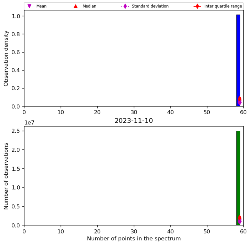
Figure 44: Histogram of “Number of points in the spectrum” for 2023-11-09 to 2023-11-11
