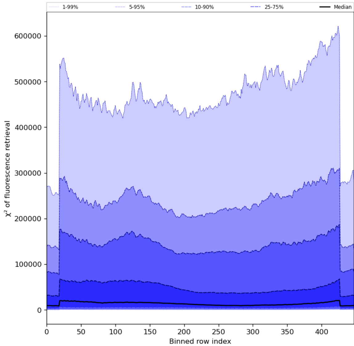
Figure 59: Along track statistics of “ \chi^2 of fluorescence retrieval” for 2023-11-09 to 2023-11-11
