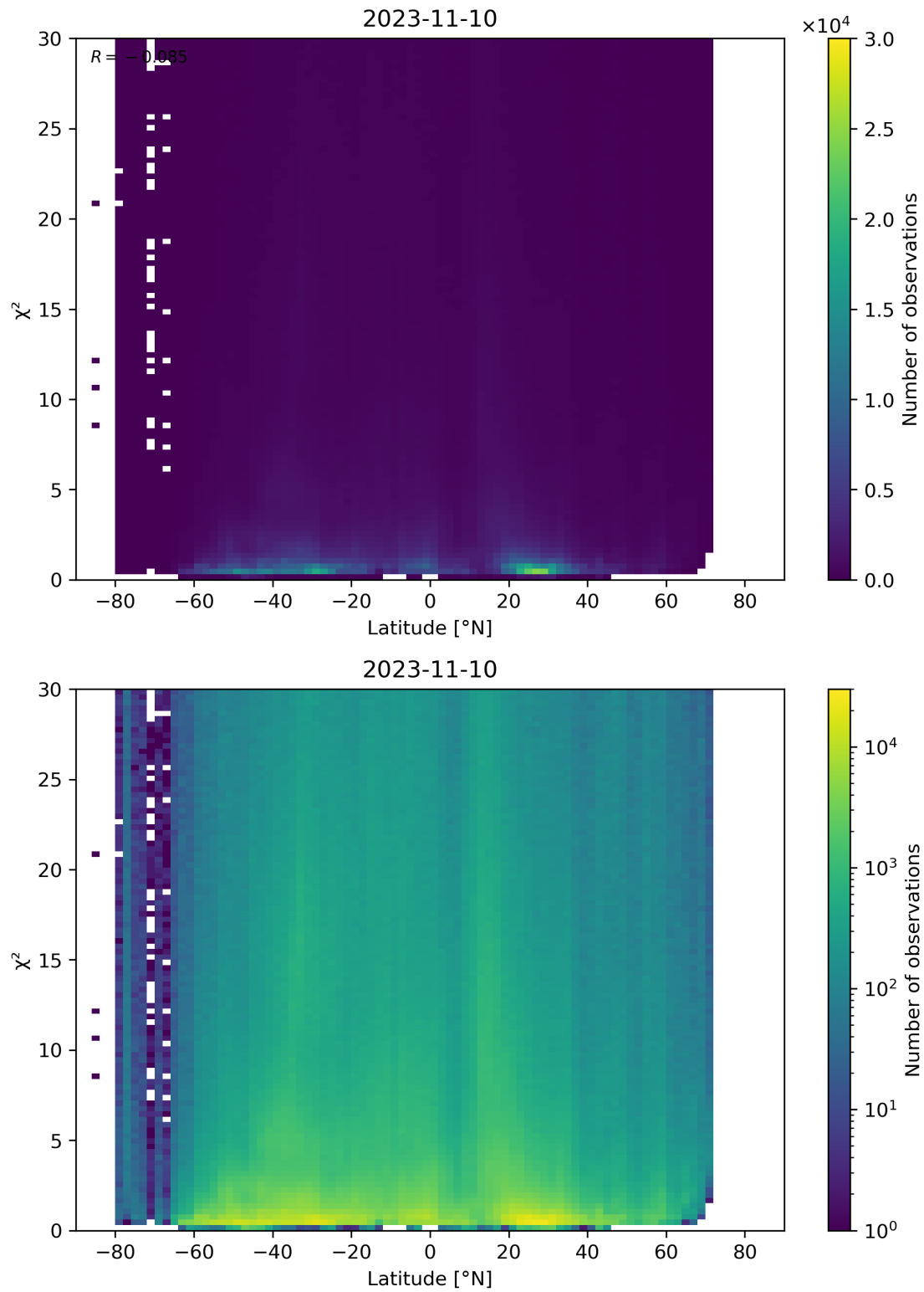
Figure 97: Scatter density plot of “Latitude” against “ \chi^2 ” for 2023-11-09 to 2023-11-11.
