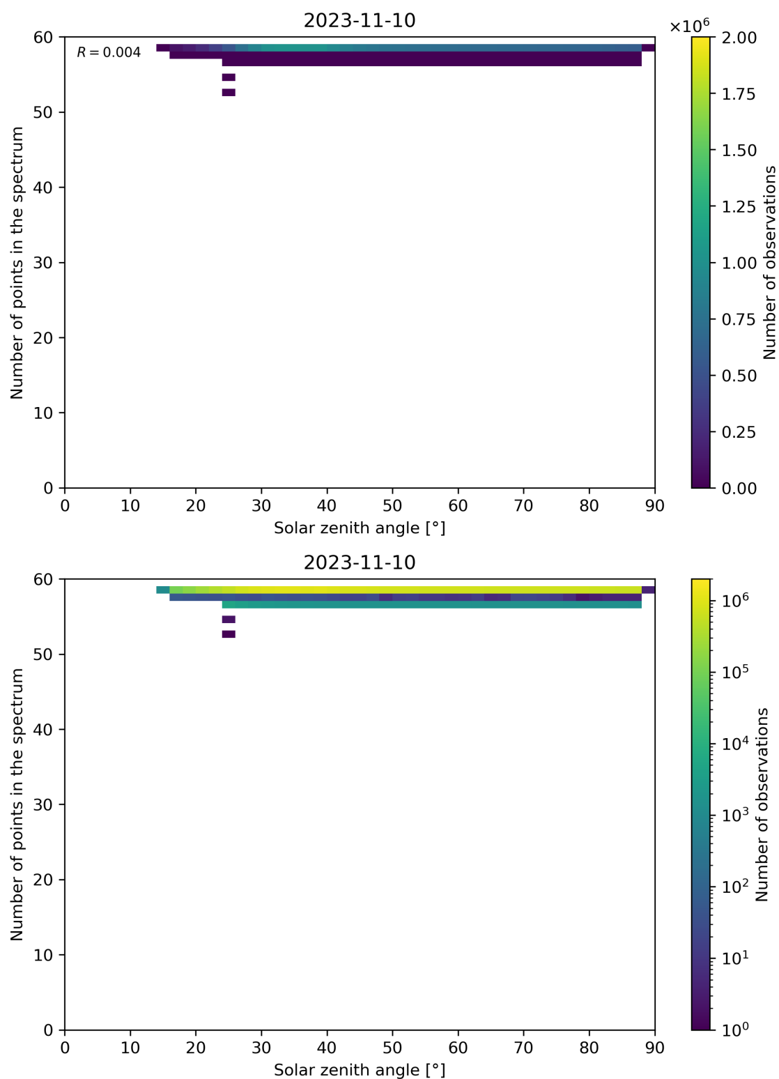
Figure 126: Scatter density plot of “Solar zenith angle” against “Number of points in the spectrum” for 2023-11-09 to 2023-11-11.
