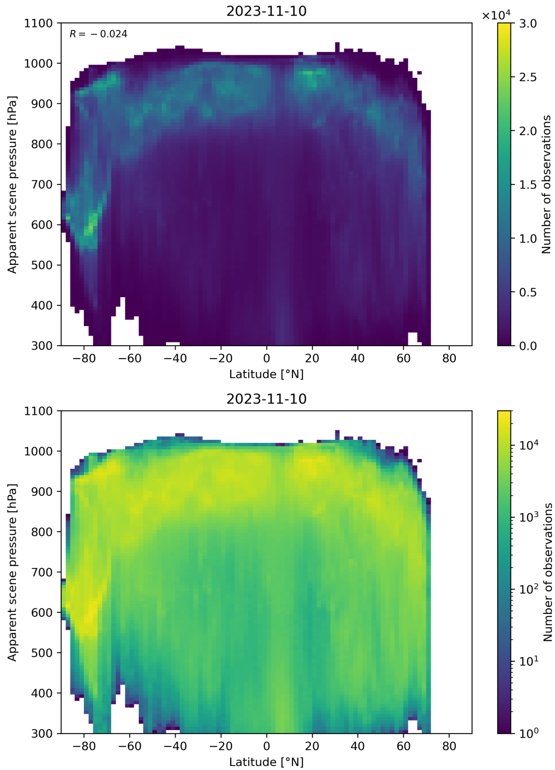
Figure 96: Scatter density plot of “Latitude” against “Apparent scene pressure” for 2023-11-09 to 2023-11-11.
