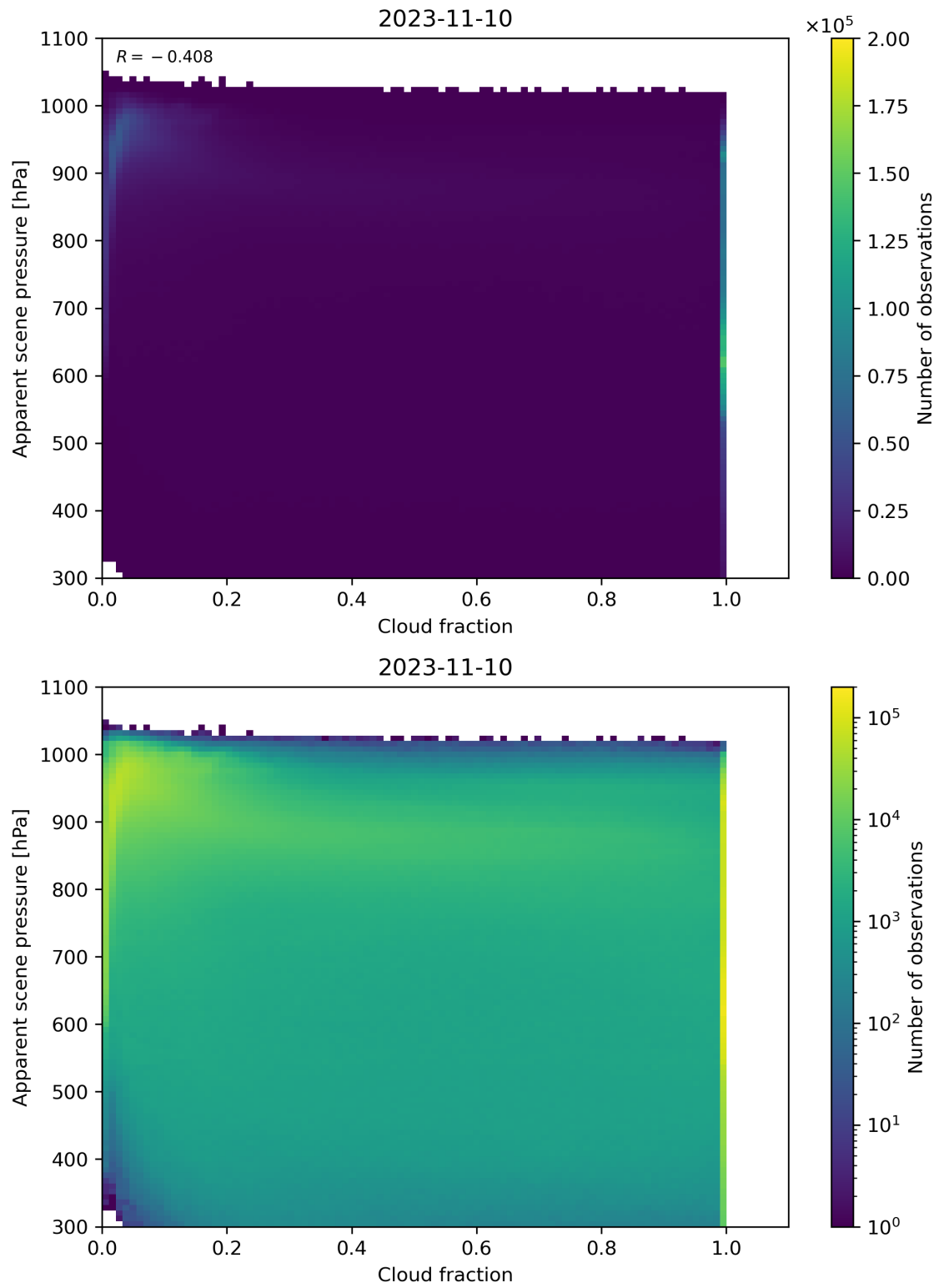
Figure 76: Scatter density plot of “Cloud fraction” against “Apparent scene pressure” for 2023-11-09 to 2023-11-11.
