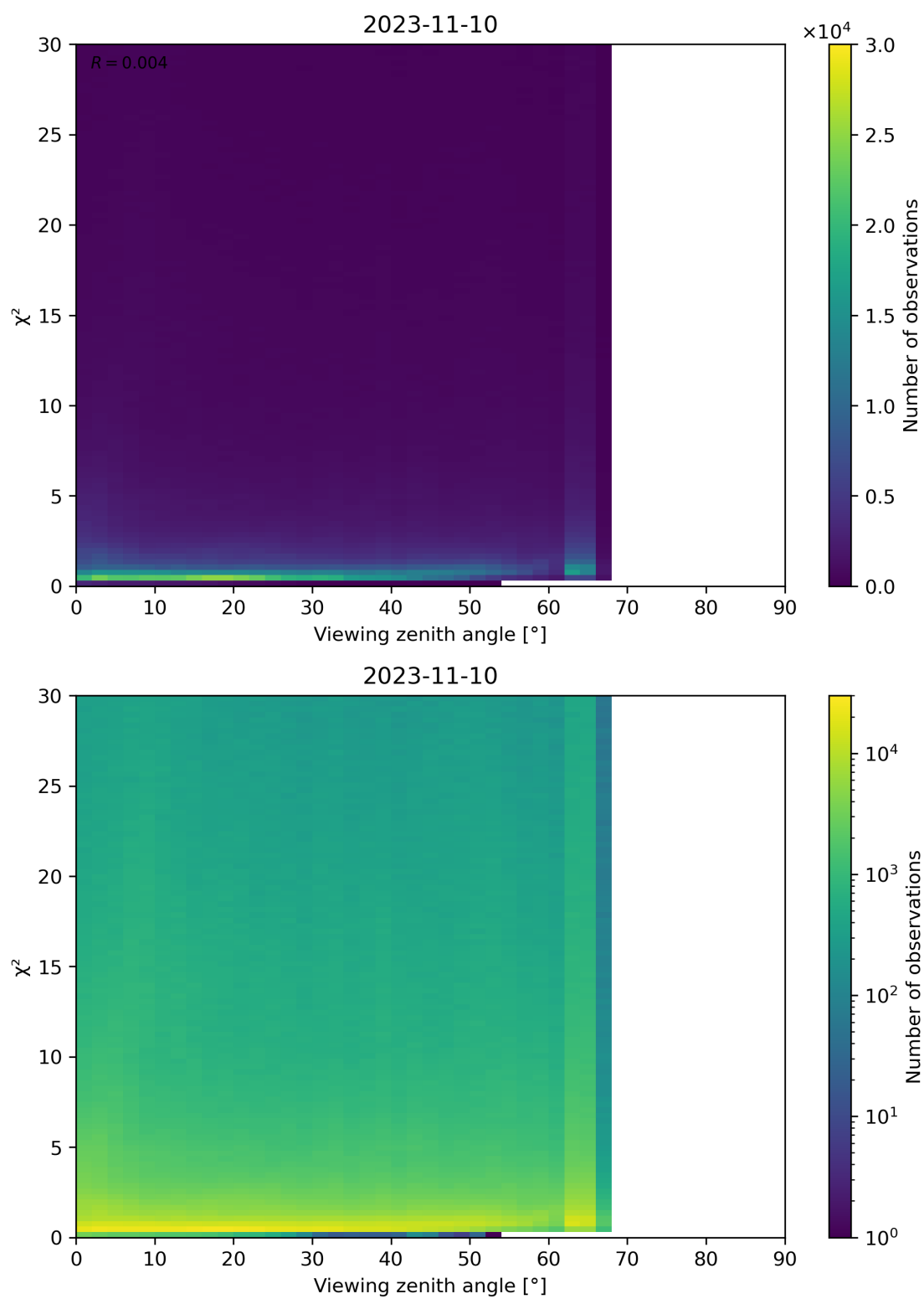
Figure 130: Scatter density plot of “Viewing zenith angle” against “ \chi^2 ” for 2023-11-09 to 2023-11-11.
