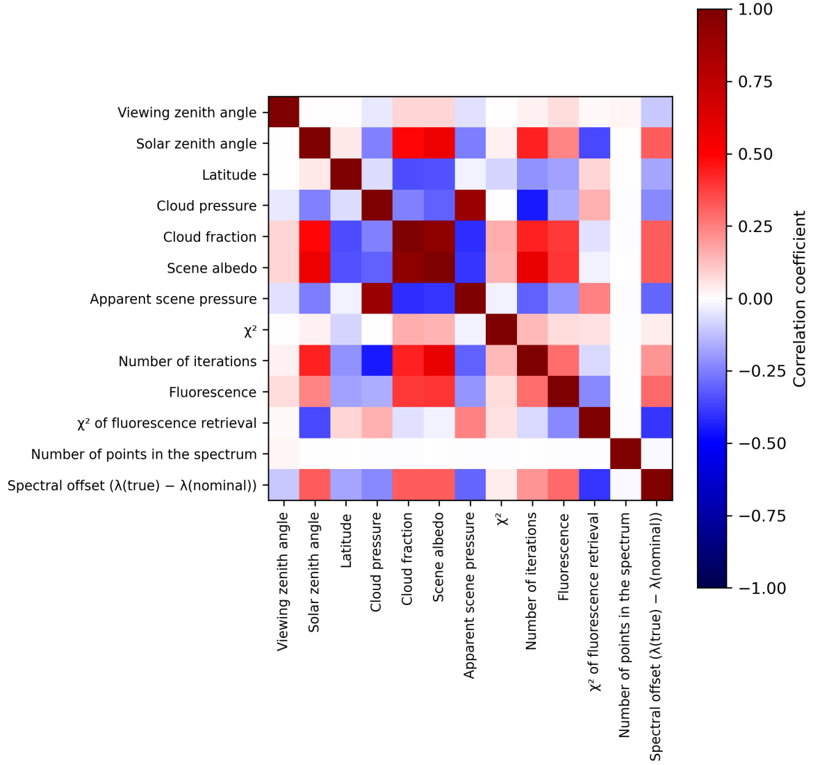
Figure 2: Map of correlation matrix for 2023-11-09 to 2023-11-11.
