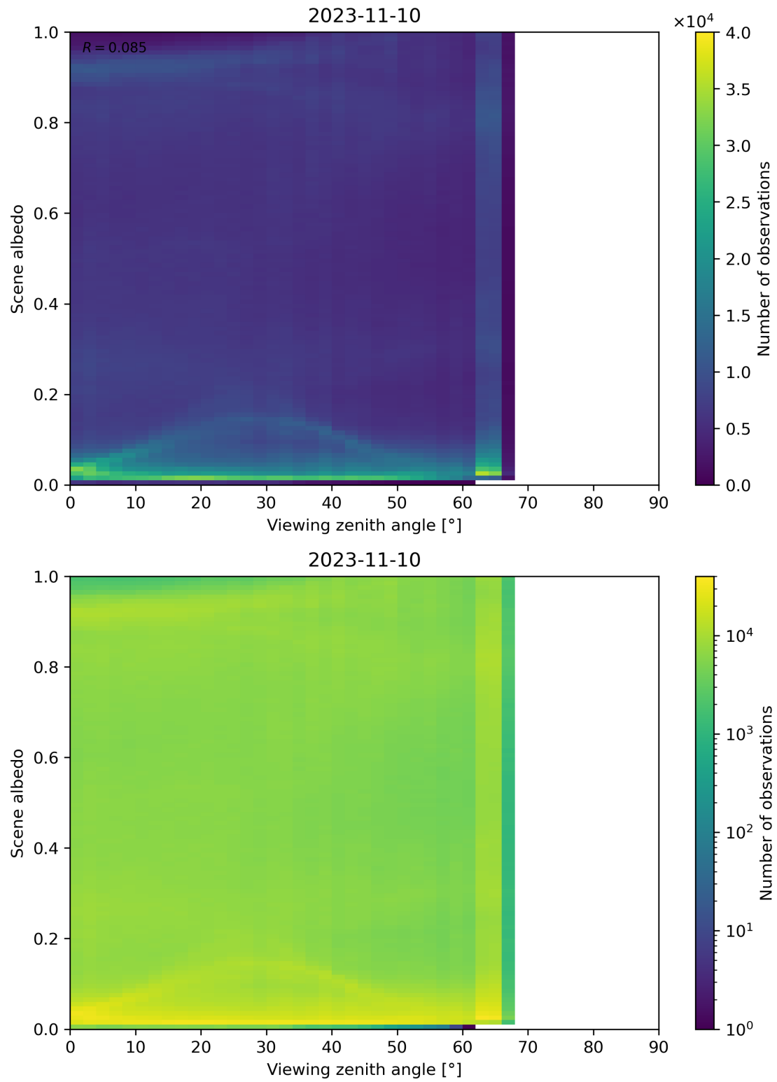
Figure 138: Scatter density plot of “Viewing zenith angle” against “Scene albedo” for 2023-11-09 to 2023-11-11.
