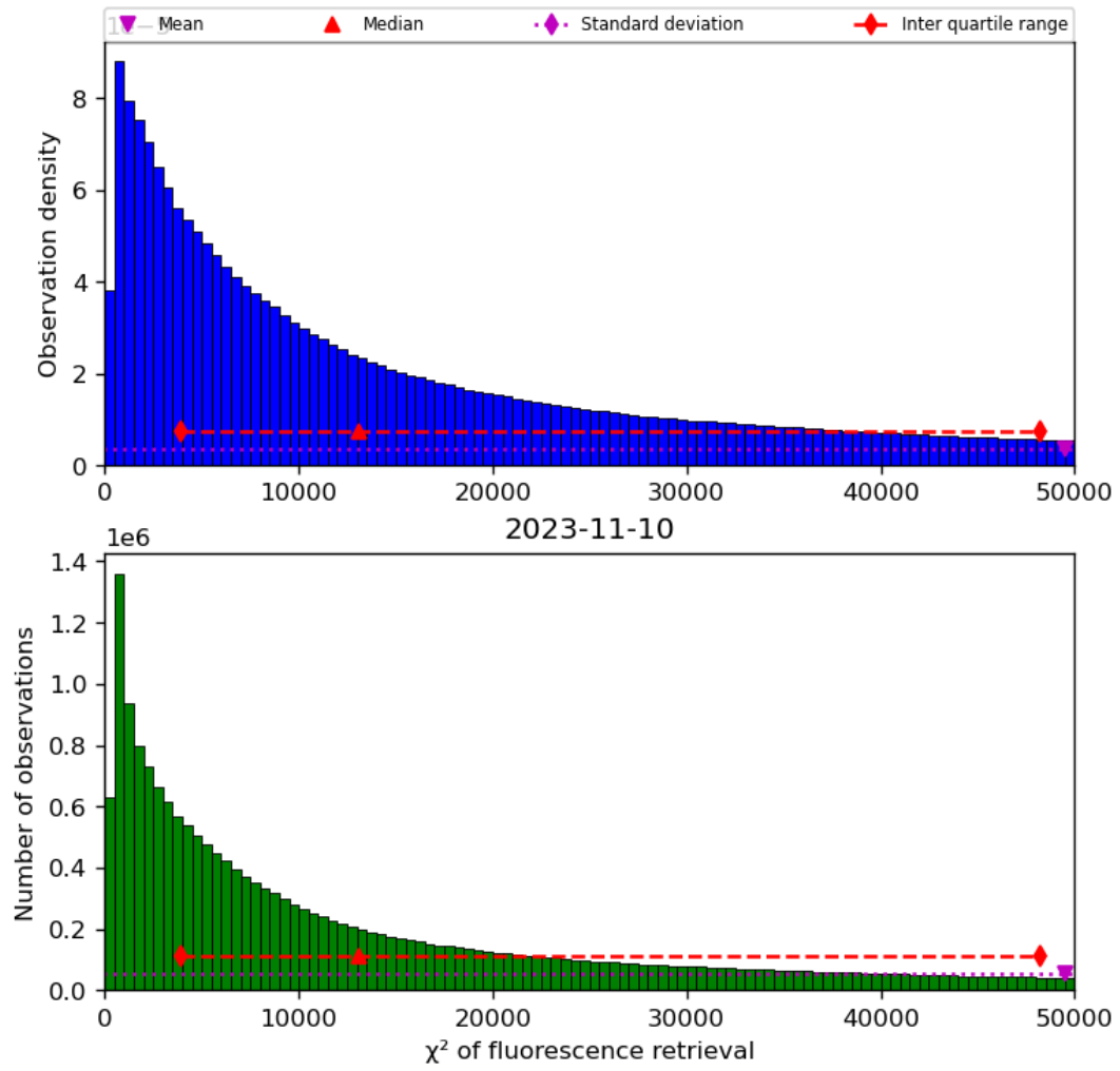
Figure 42: Histogram of “ \chi^2 of fluorescence retrieval” for 2023-11-09 to 2023-11-11
