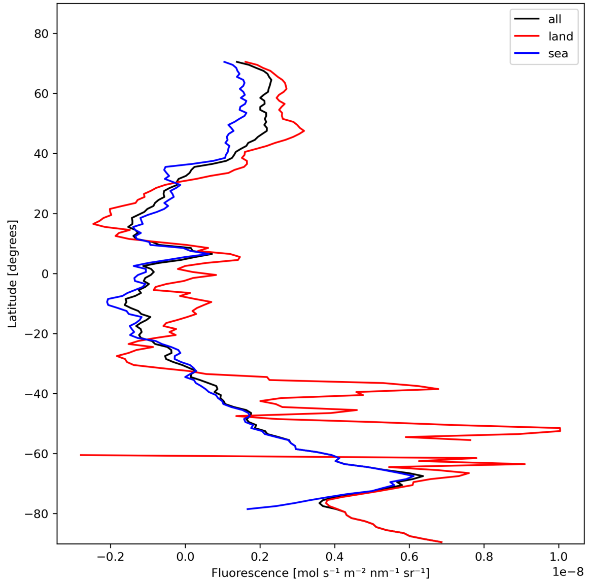
Figure 23: Zonal average of “Fluorescence” for 2023-11-09 to 2023-11-11.
