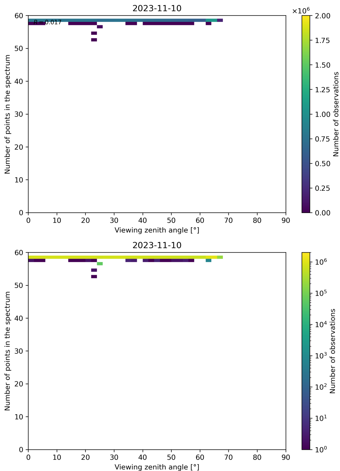
Figure 137: Scatter density plot of “Viewing zenith angle” against “Number of points in the spectrum” for 2023-11-09 to 2023-11-11.
