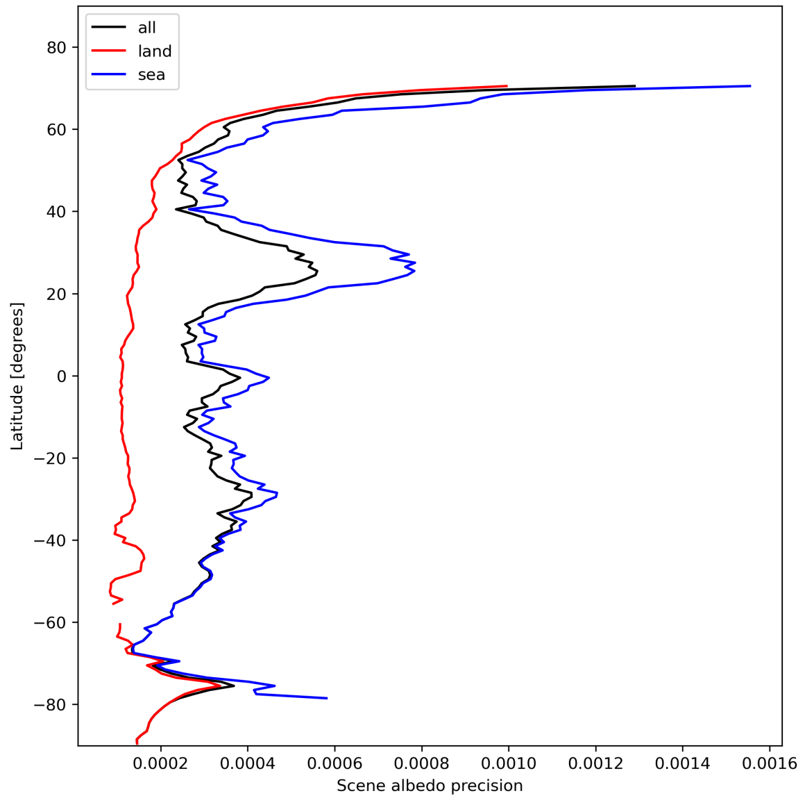
Figure 18: Zonal average of “Scene albedo precision” for 2023-11-09 to 2023-11-11.
