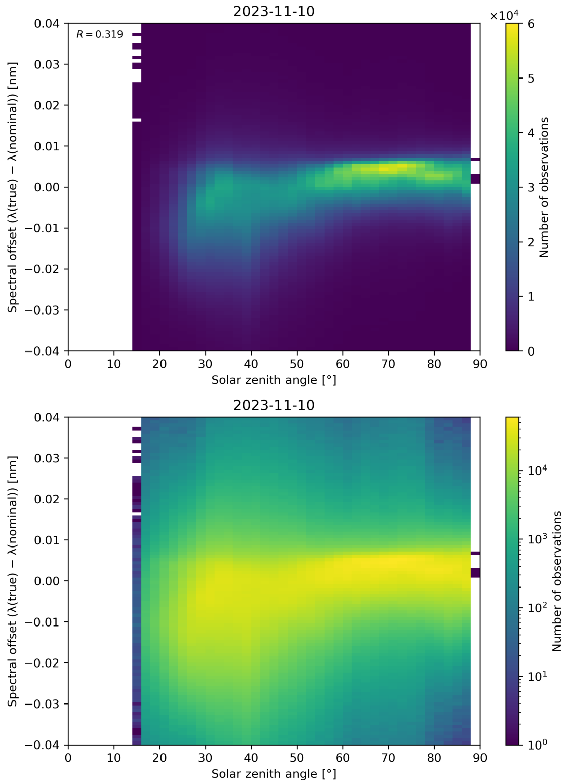
Figure 128: Scatter density plot of “Solar zenith angle” against “Spectral offset ( \lambda(\text{true}) - \lambda(\text{nominal}) )” for 2023-11-09 to 2023-11-11.
