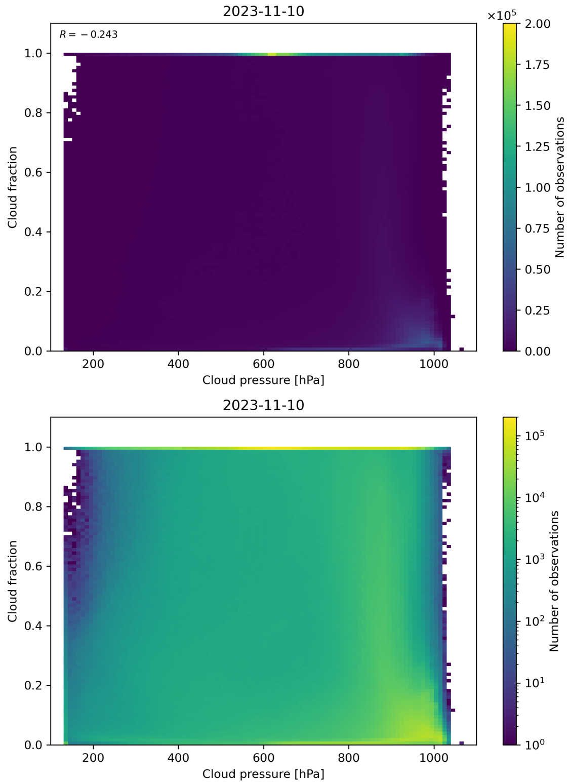
Figure 87: Scatter density plot of “Cloud pressure” against “Cloud fraction” for 2023-11-09 to 2023-11-11.
