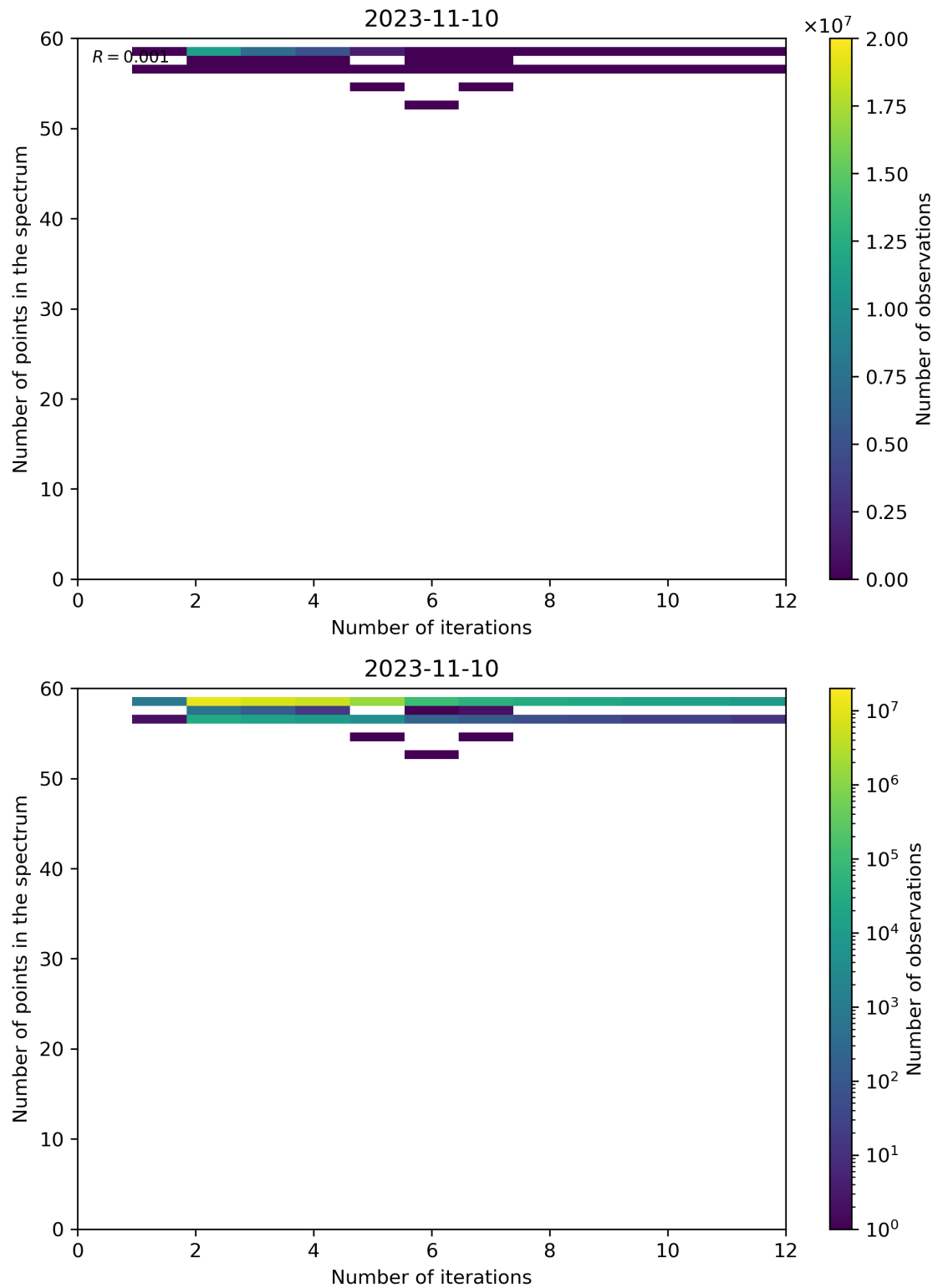
Figure 108: Scatter density plot of “Number of iterations” against “Number of points in the spectrum” for 2023-11-09 to 2023-11-11.
