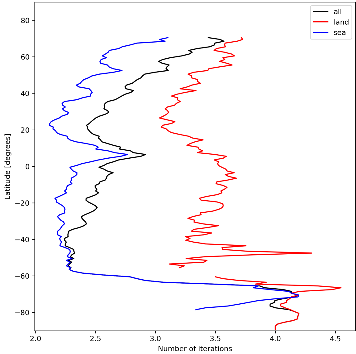
Figure 22: Zonal average of “Number of iterations” for 2023-11-09 to 2023-11-11.
