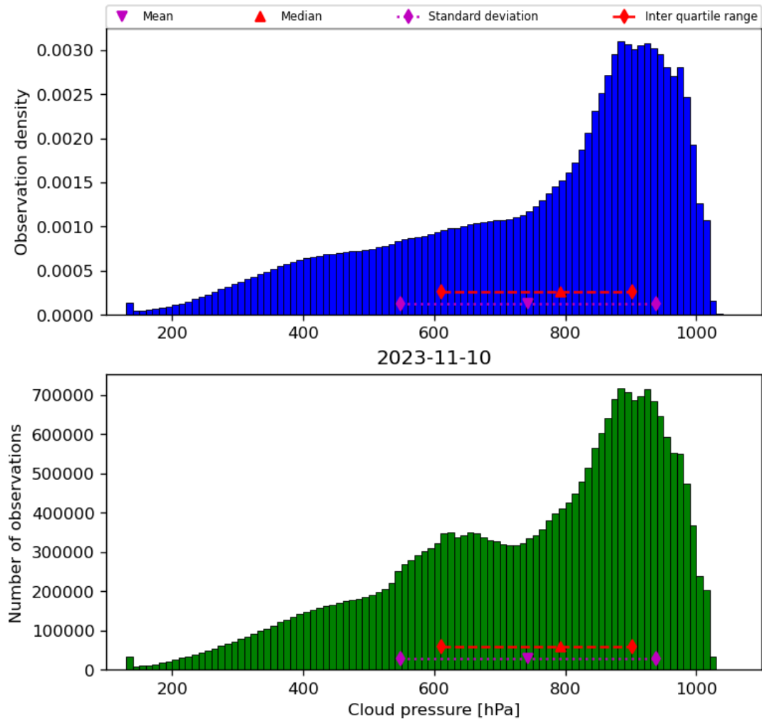
Figure 30: Histogram of “Cloud pressure” for 2023-11-09 to 2023-11-11
