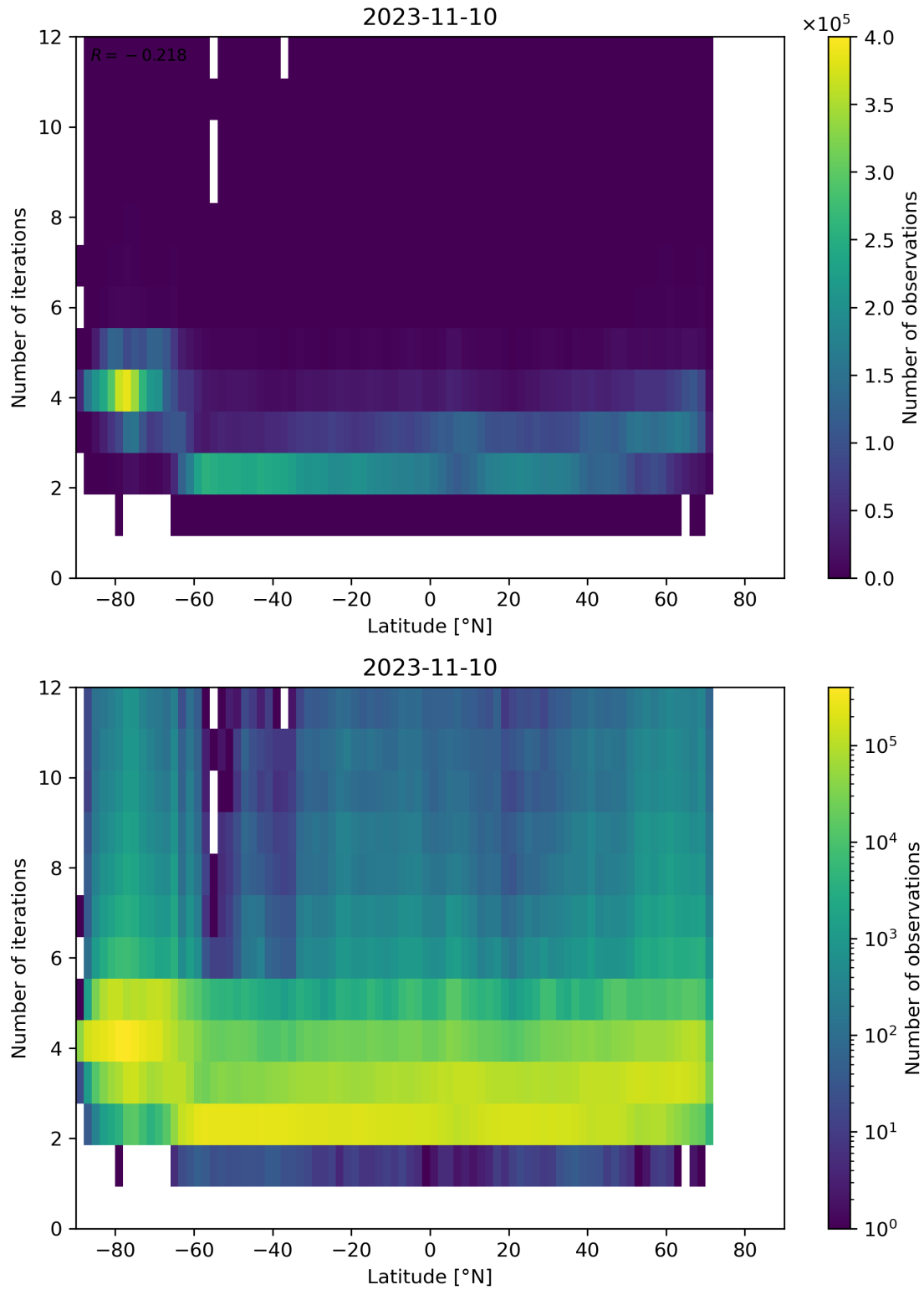
Figure 102: Scatter density plot of “Latitude” against “Number of iterations” for 2023-11-09 to 2023-11-11.
