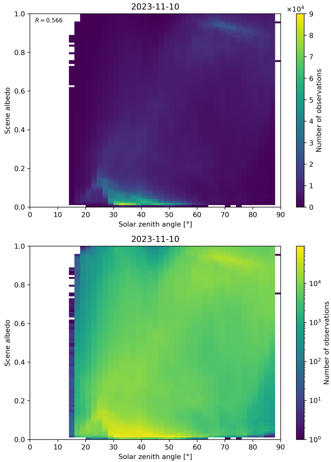
Figure 127: Scatter density plot of “Solar zenith angle” against “Scene albedo” for 2023-11-09 to 2023-11-11.
