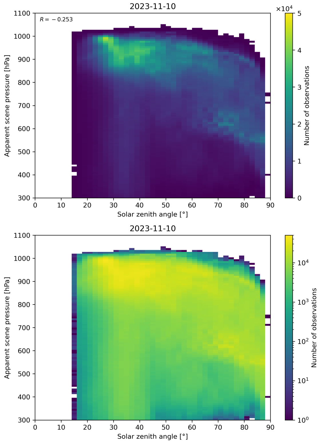
Figure 118: Scatter density plot of “Solar zenith angle” against “Apparent scene pressure” for 2023-11-09 to 2023-11-11.
