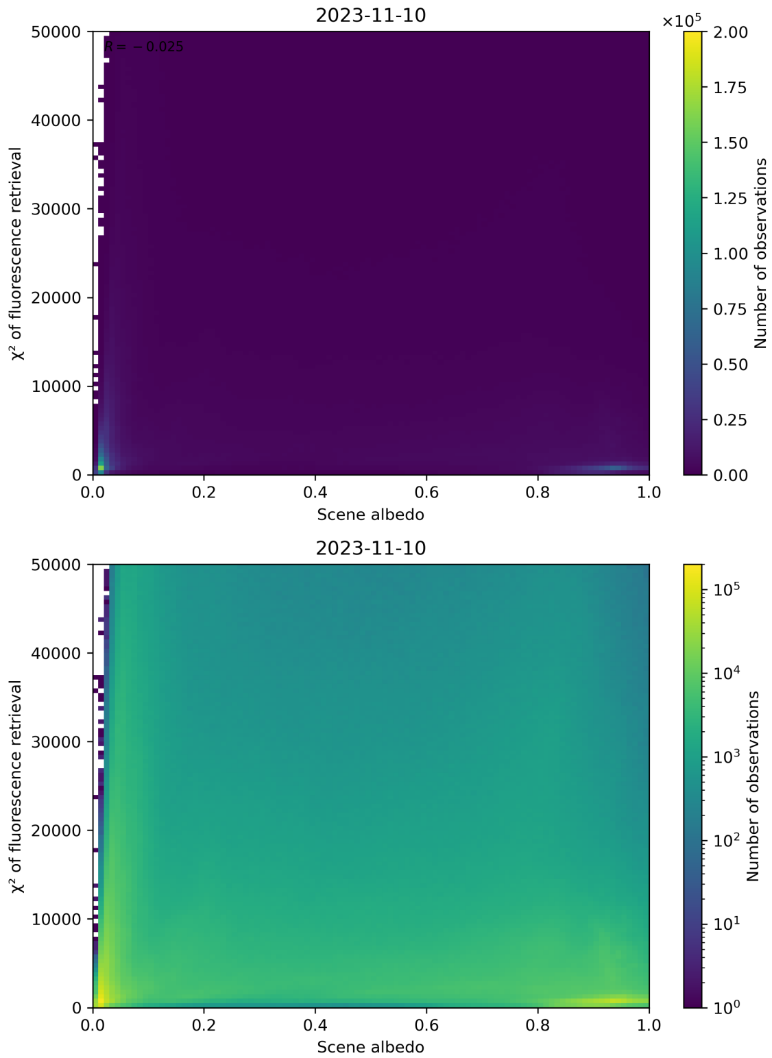
Figure 113: Scatter density plot of “Scene albedo” against “ \chi^2 of fluorescence retrieval” for 2023-11-09 to 2023-11-11.
