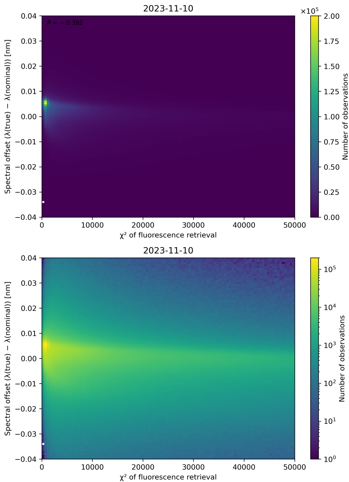
Figure 72: Scatter density plot of " \chi^2 of fluorescence retrieval" against "Spectral offset ( \lambda(\text{true}) - \lambda(\text{nominal}) )" for 2023-11-09 to 2023-11-11.
