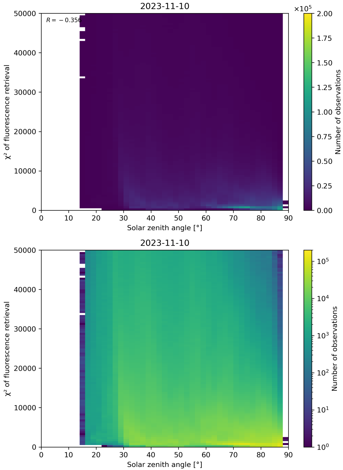
Figure 120: Scatter density plot of “Solar zenith angle” against “ \chi^2 of fluorescence retrieval” for 2023-11-09 to 2023-11-11.
