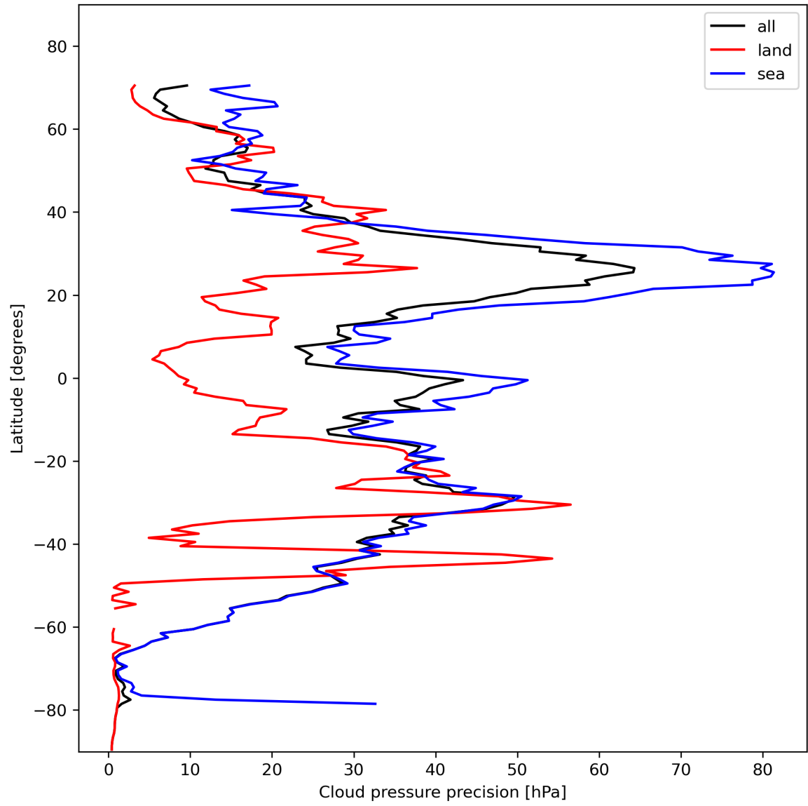
Figure 14: Zonal average of “Cloud pressure precision” for 2023-11-09 to 2023-11-11.
