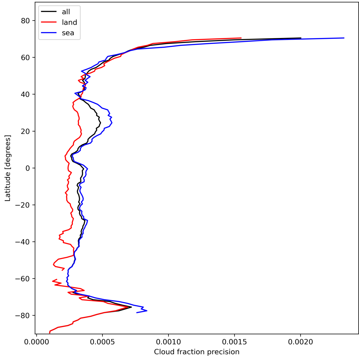
Figure 16: Zonal average of “Cloud fraction precision” for 2023-11-09 to 2023-11-11.
