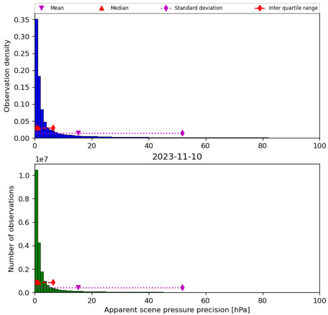
Figure 37: Histogram of “Apparent scene pressure precision” for 2023-11-09 to 2023-11-11
