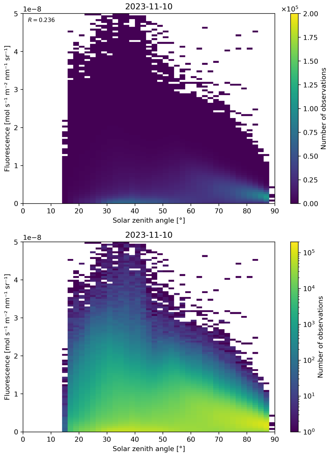
Figure 123: Scatter density plot of “Solar zenith angle” against “Fluorescence” for 2023-11-09 to 2023-11-11.
