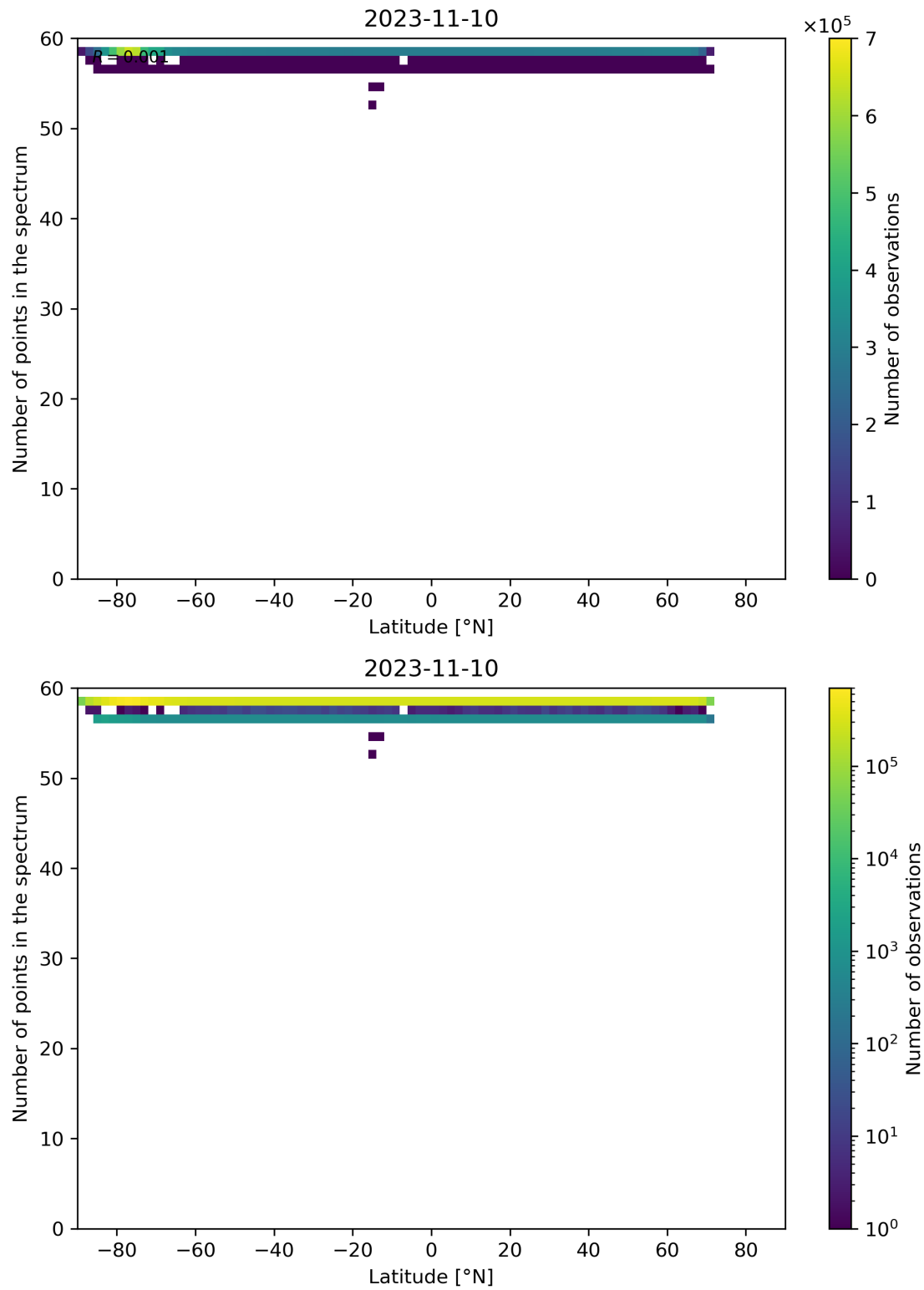
Figure 103: Scatter density plot of “Latitude” against “Number of points in the spectrum” for 2023-11-09 to 2023-11-11.
