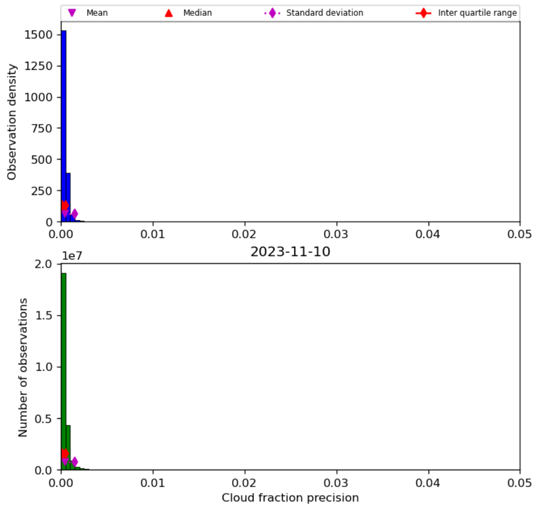
Figure 33: Histogram of “Cloud fraction precision” for 2023-11-09 to 2023-11-11
