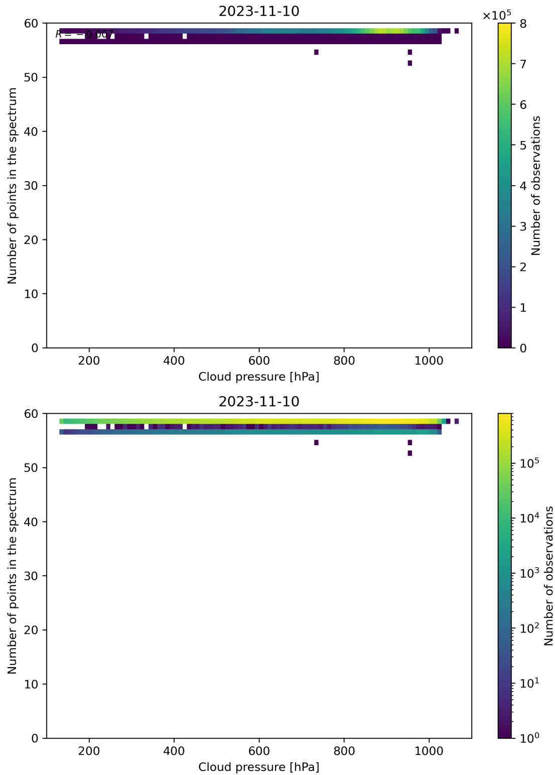
Figure 90: Scatter density plot of “Cloud pressure” against “Number of points in the spectrum” for 2023-11-09 to 2023-11-11.
