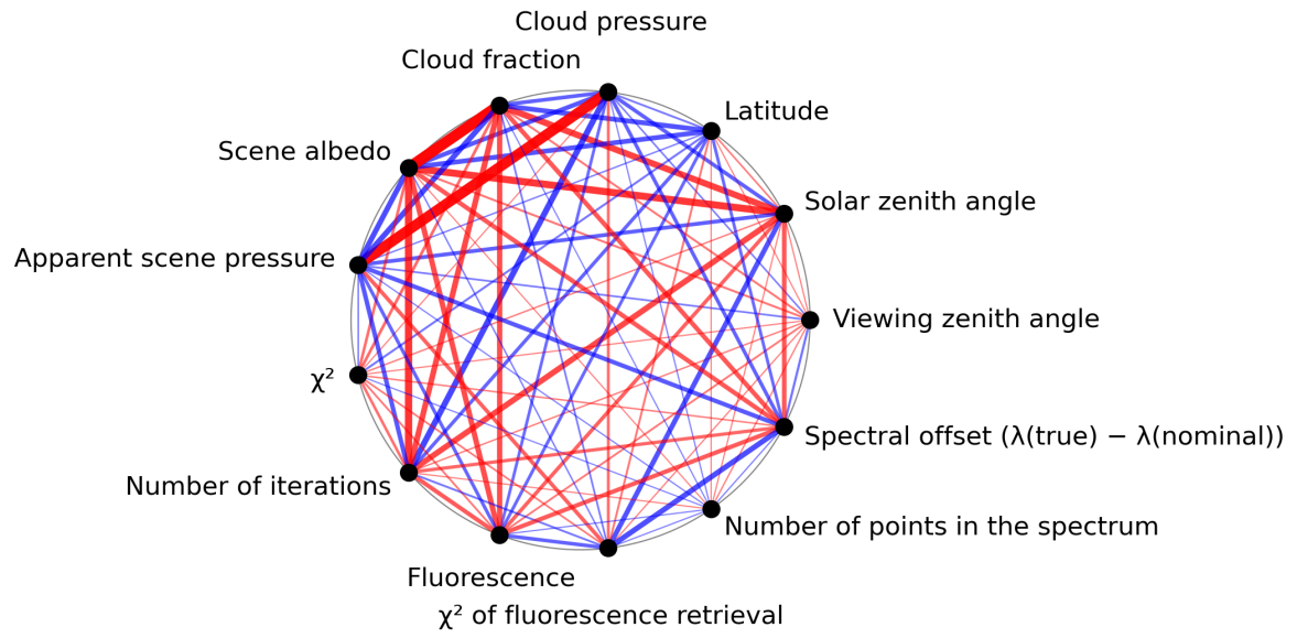
Figure 1: Map of correlation graph for 2023-11-09 to 2023-11-11.
