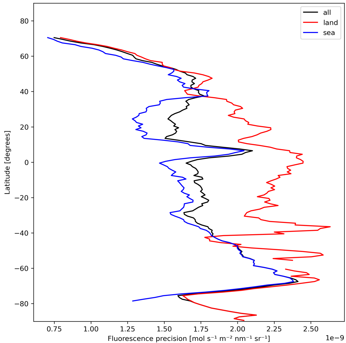
Figure 24: Zonal average of “Fluorescence precision” for 2023-11-09 to 2023-11-11.
