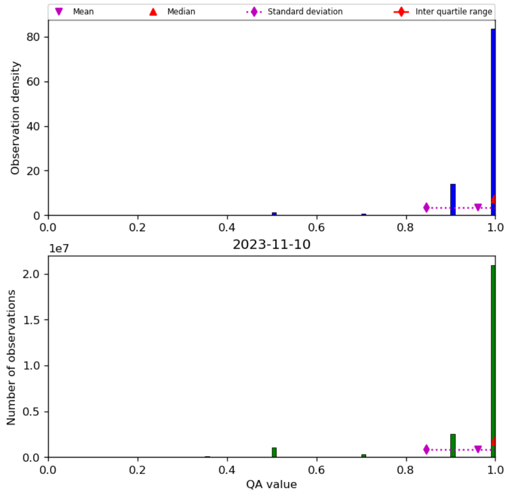
Figure 29: Histogram of “QA value” for 2023-11-09 to 2023-11-11
