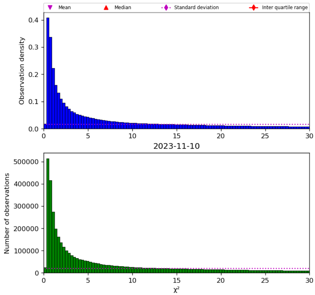
Figure 38: Histogram of “ \chi^2 ” for 2023-11-09 to 2023-11-11
