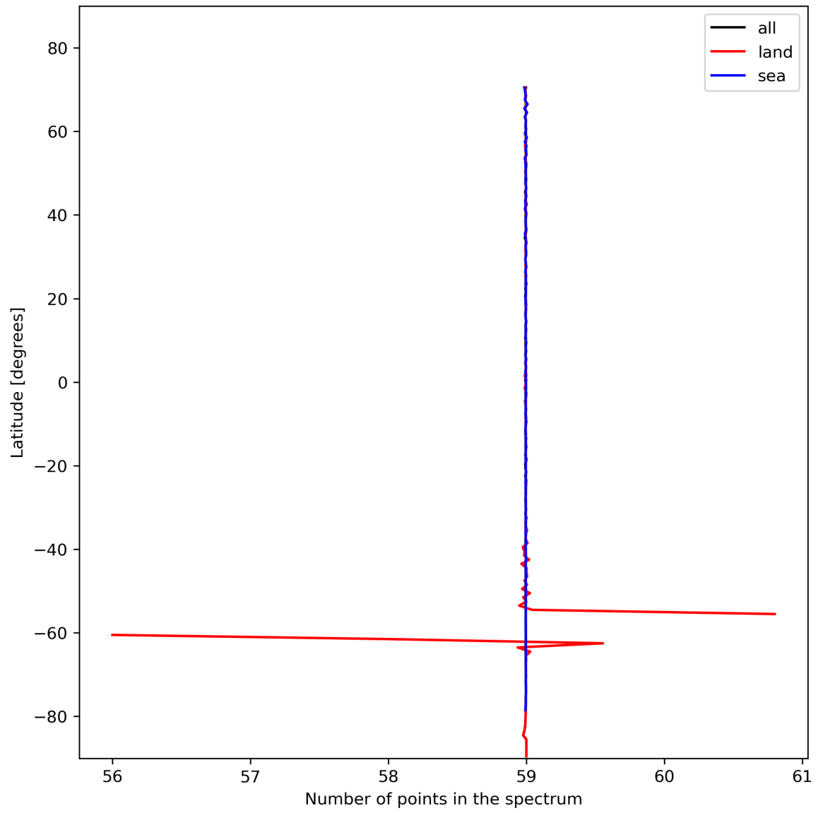
Figure 27: Zonal average of “Number of points in the spectrum” for 2023-11-09 to 2023-11-11.
