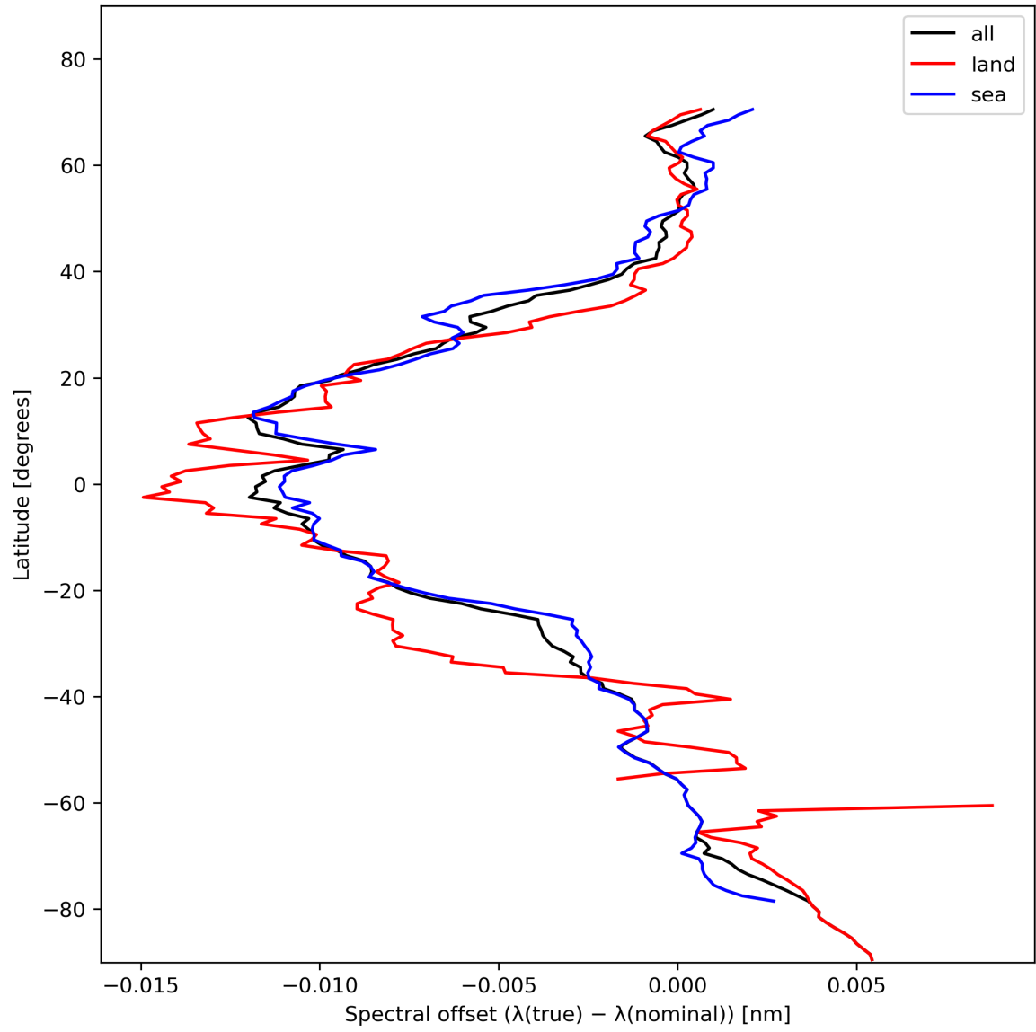
Figure 28: Zonal average of “Spectral offset ( \lambda(\text{true}) - \lambda(\text{nominal}) )” for 2023-11-09 to 2023-11-11.
