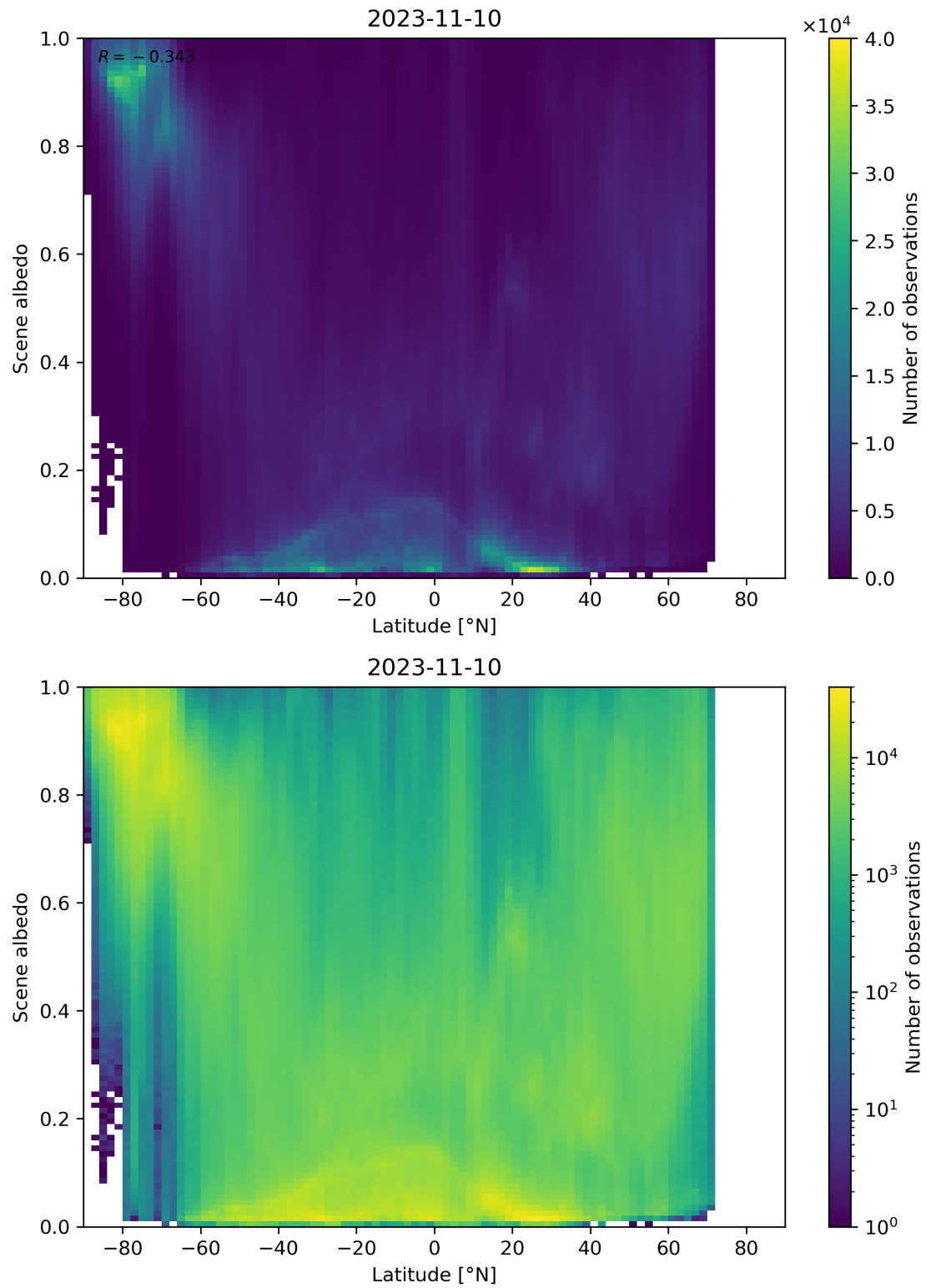
Figure 104: Scatter density plot of “Latitude” against “Scene albedo” for 2023-11-09 to 2023-11-11.
