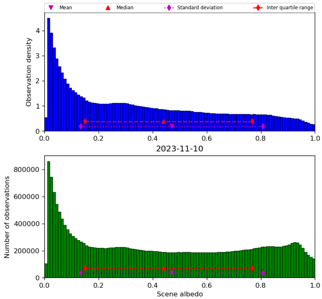
Figure 34: Histogram of “Scene albedo” for 2023-11-09 to 2023-11-11
