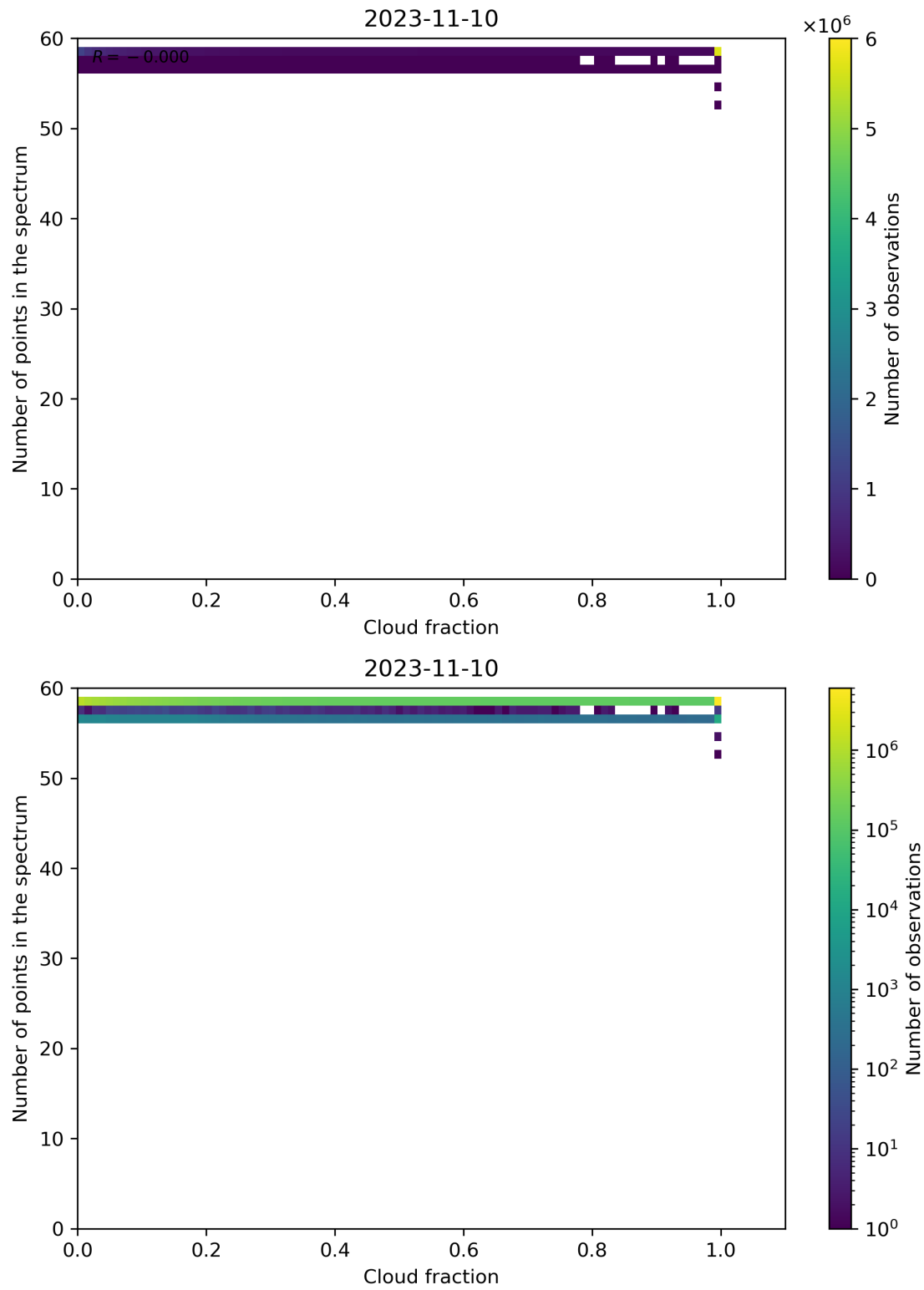
Figure 81: Scatter density plot of “Cloud fraction” against “Number of points in the spectrum” for 2023-11-09 to 2023-11-11.
