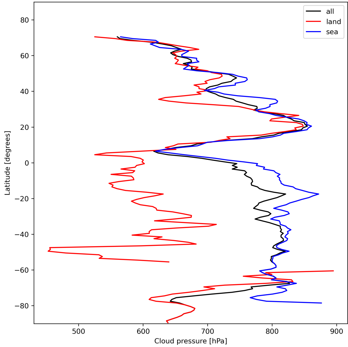
Figure 13: Zonal average of “Cloud pressure” for 2023-11-09 to 2023-11-11.
