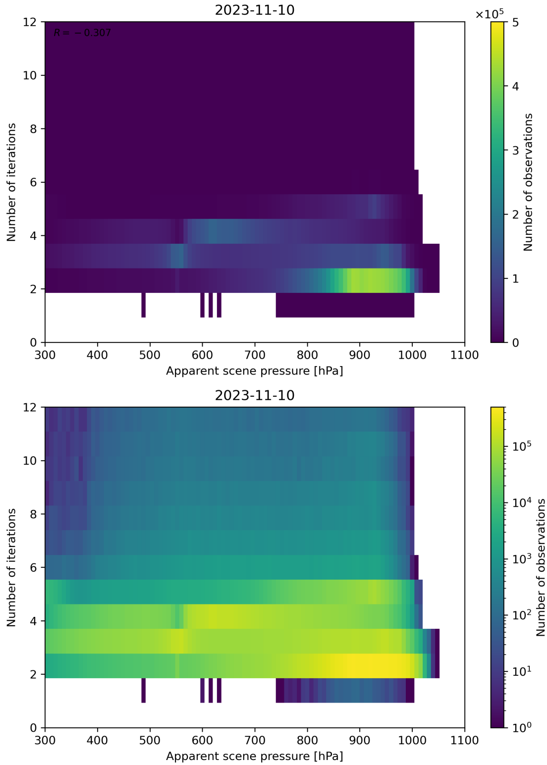
Figure 66: Scatter density plot of “Apparent scene pressure” against “Number of iterations” for 2023-11-09 to 2023-11-11.
