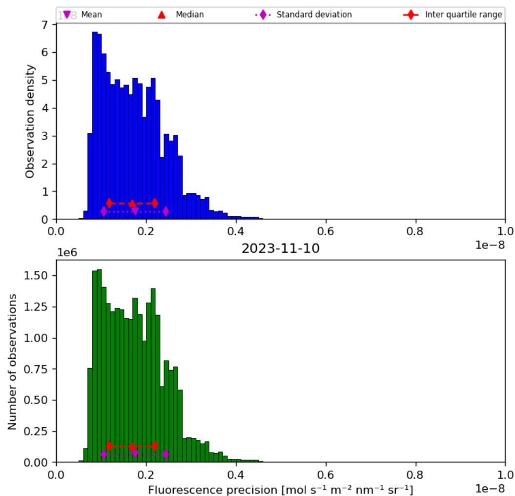
Figure 41: Histogram of “Fluorescence precision” for 2023-11-09 to 2023-11-11
