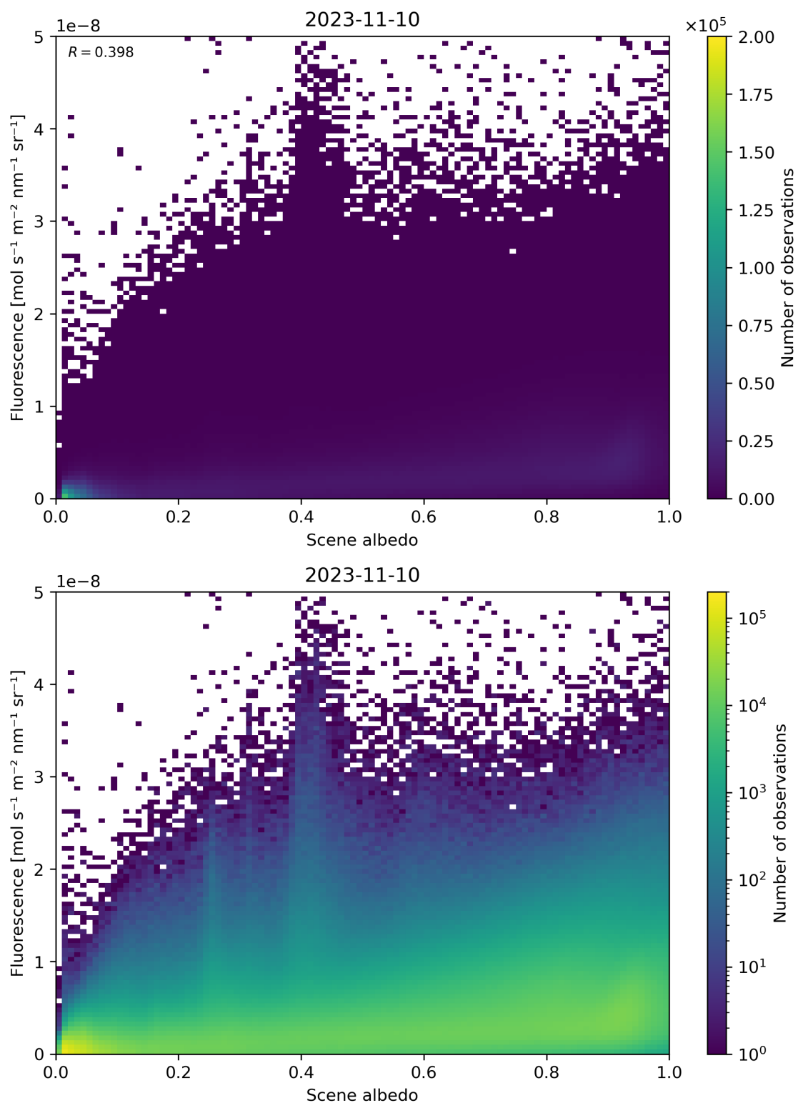
Figure 114: Scatter density plot of “Scene albedo” against “Fluorescence” for 2023-11-09 to 2023-11-11.
