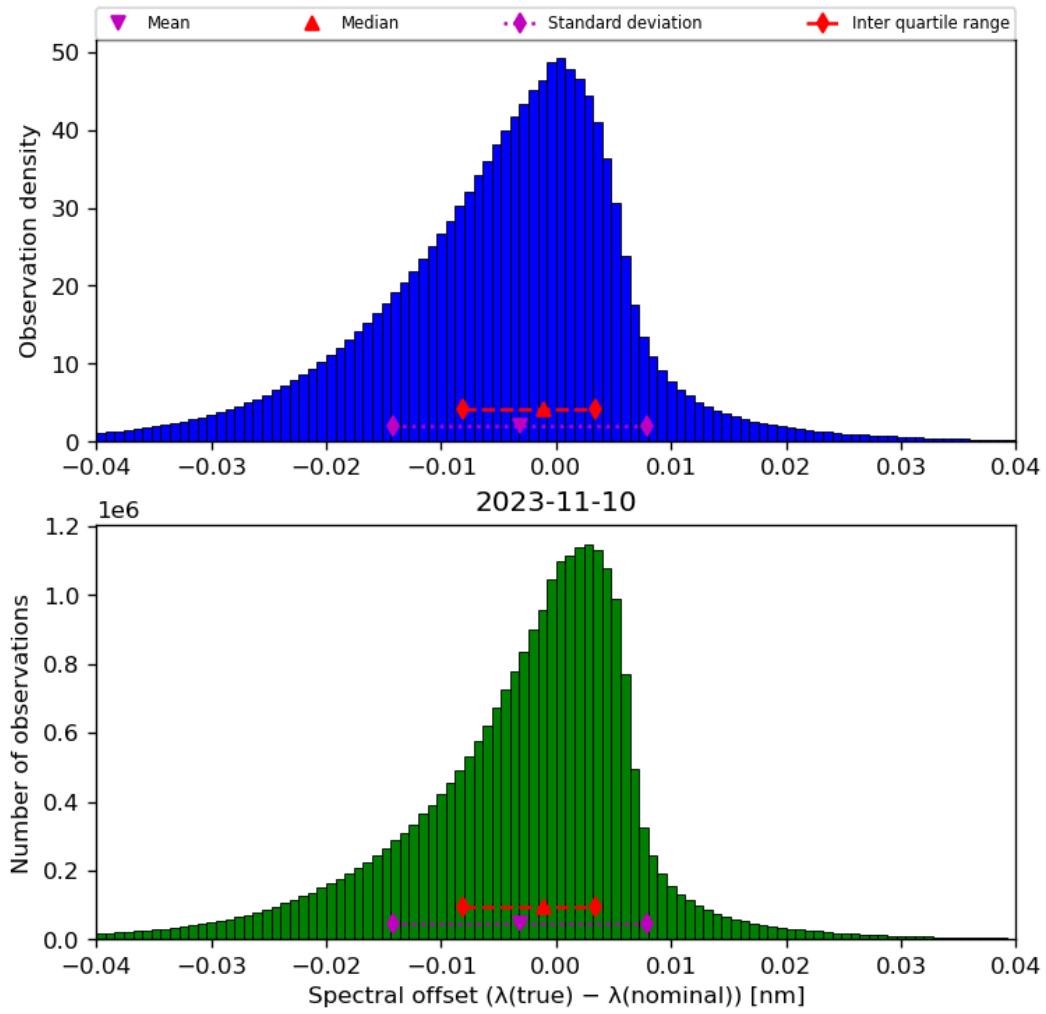
Figure 45: Histogram of “Spectral offset ( \lambda(\text{true}) - \lambda(\text{nominal}) )” for 2023-11-09 to 2023-11-11
