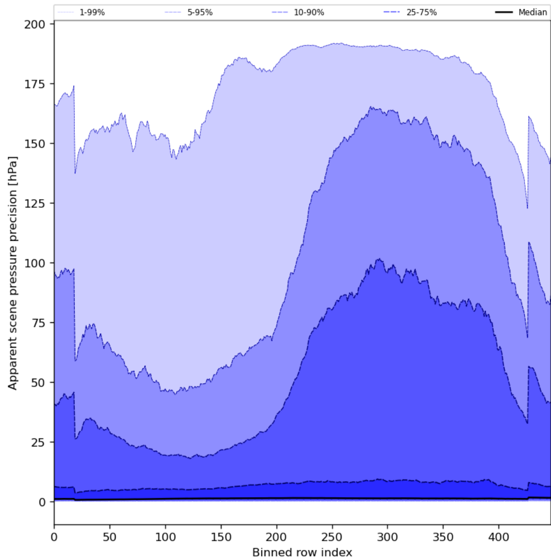
Figure 54: Along track statistics of “Apparent scene pressure precision” for 2023-11-09 to 2023-11-11
