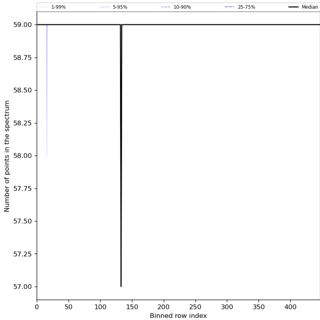
Figure 61: Along track statistics of “Number of points in the spectrum” for 2023-11-09 to 2023-11-11
