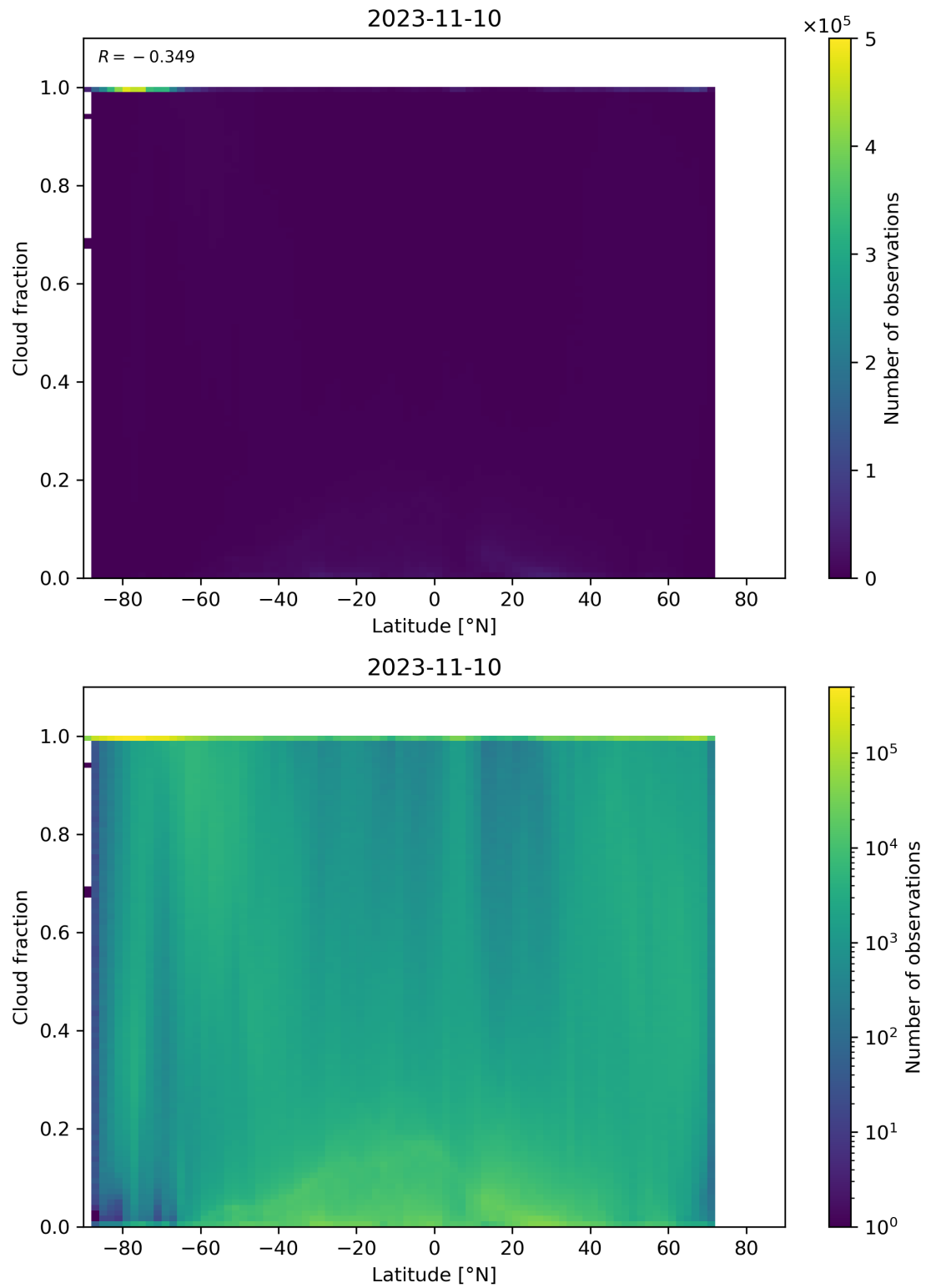
Figure 99: Scatter density plot of “Latitude” against “Cloud fraction” for 2023-11-09 to 2023-11-11.
