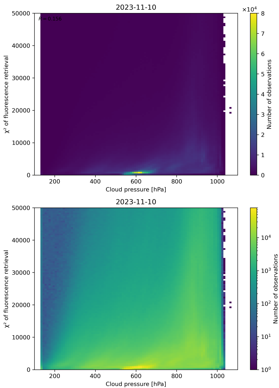
Figure 86: Scatter density plot of “Cloud pressure” against “ \chi^2 of fluorescence retrieval” for 2023-11-09 to 2023-11-11.
