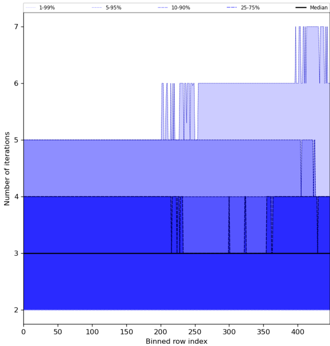
Figure 56: Along track statistics of “Number of iterations” for 2023-11-09 to 2023-11-11
