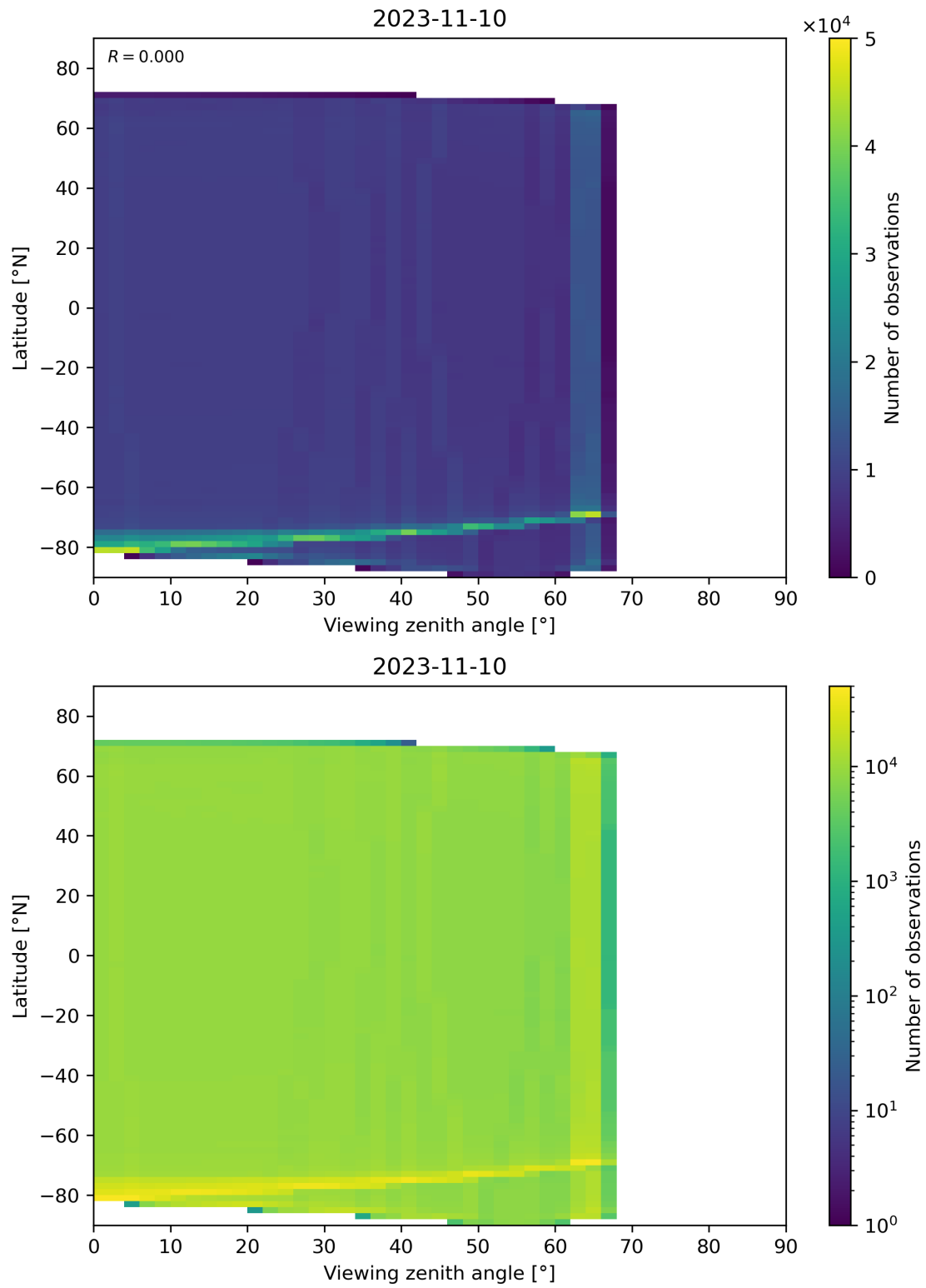
Figure 135: Scatter density plot of “Viewing zenith angle” against “Latitude” for 2023-11-09 to 2023-11-11.
