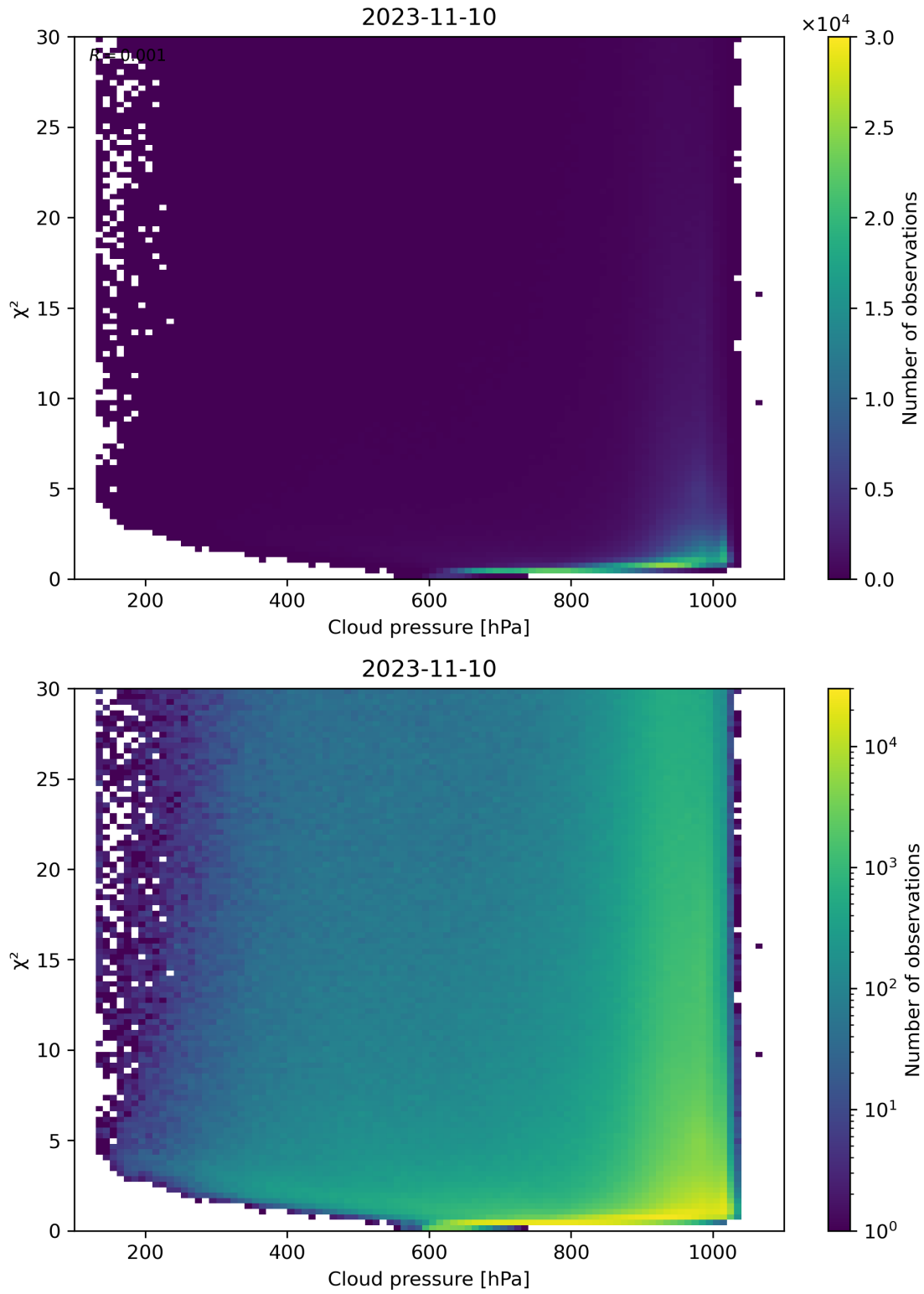
Figure 85: Scatter density plot of “Cloud pressure” against “ \chi^2 ” for 2023-11-09 to 2023-11-11.
