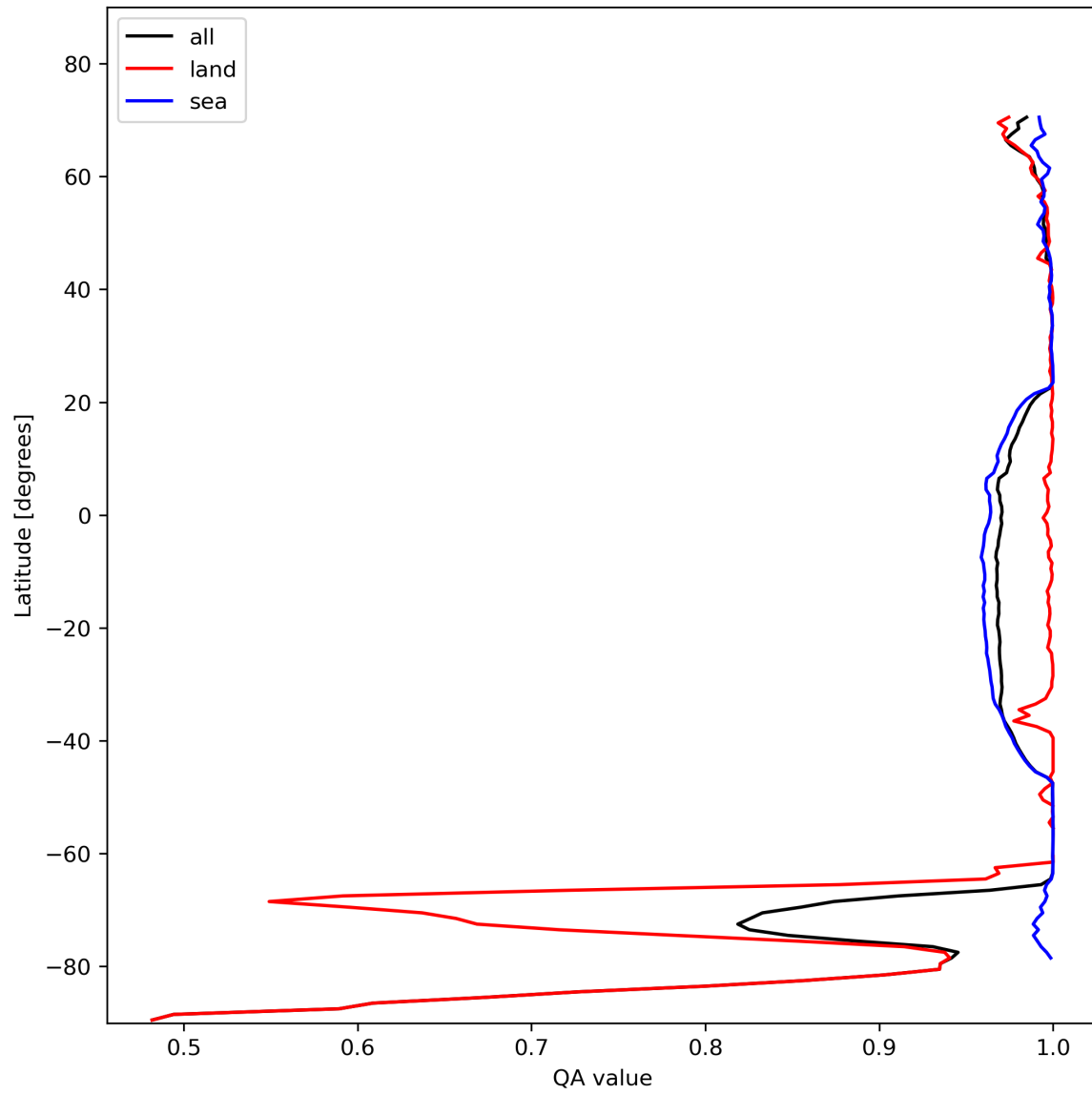
Figure 12: Zonal average of “QA value” for 2023-11-09 to 2023-11-11.
