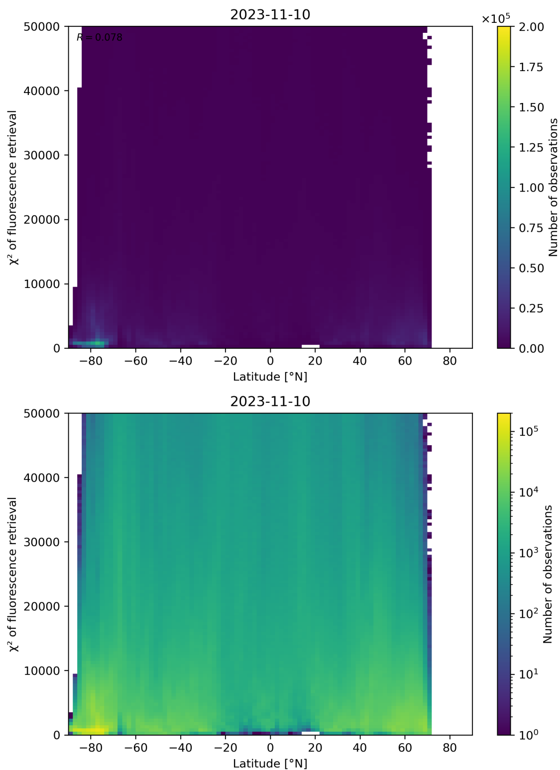
Figure 98: Scatter density plot of “Latitude” against “ \chi^2 of fluorescence retrieval” for 2023-11-09 to 2023-11-11.
