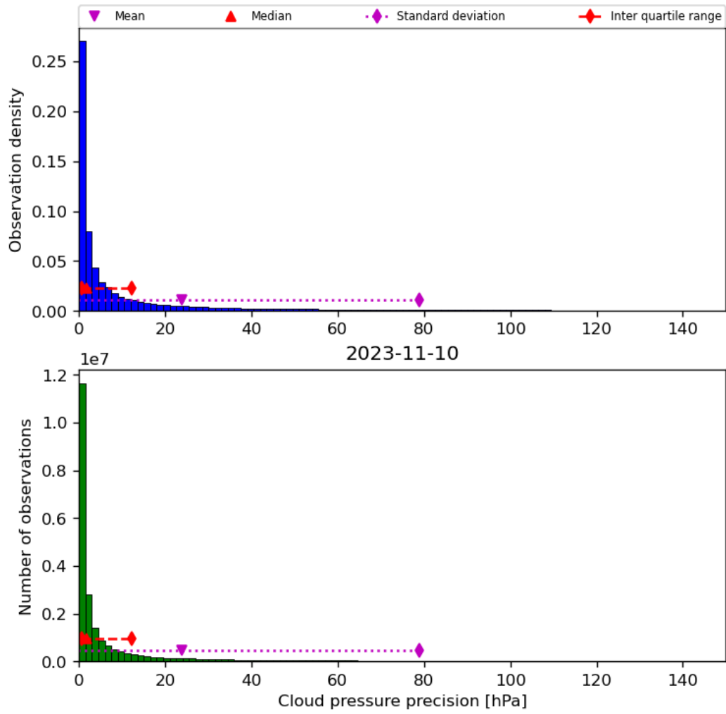
Figure 31: Histogram of “Cloud pressure precision” for 2023-11-09 to 2023-11-11
