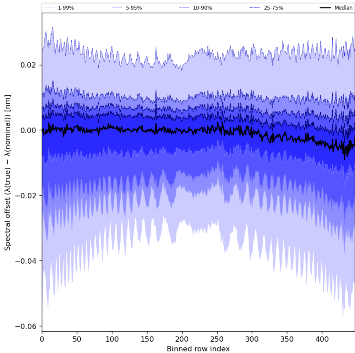
Figure 62: Along track statistics of “Spectral offset ( \lambda(\text{true}) - \lambda(\text{nominal}) )” for 2023-11-09 to 2023-11-11
