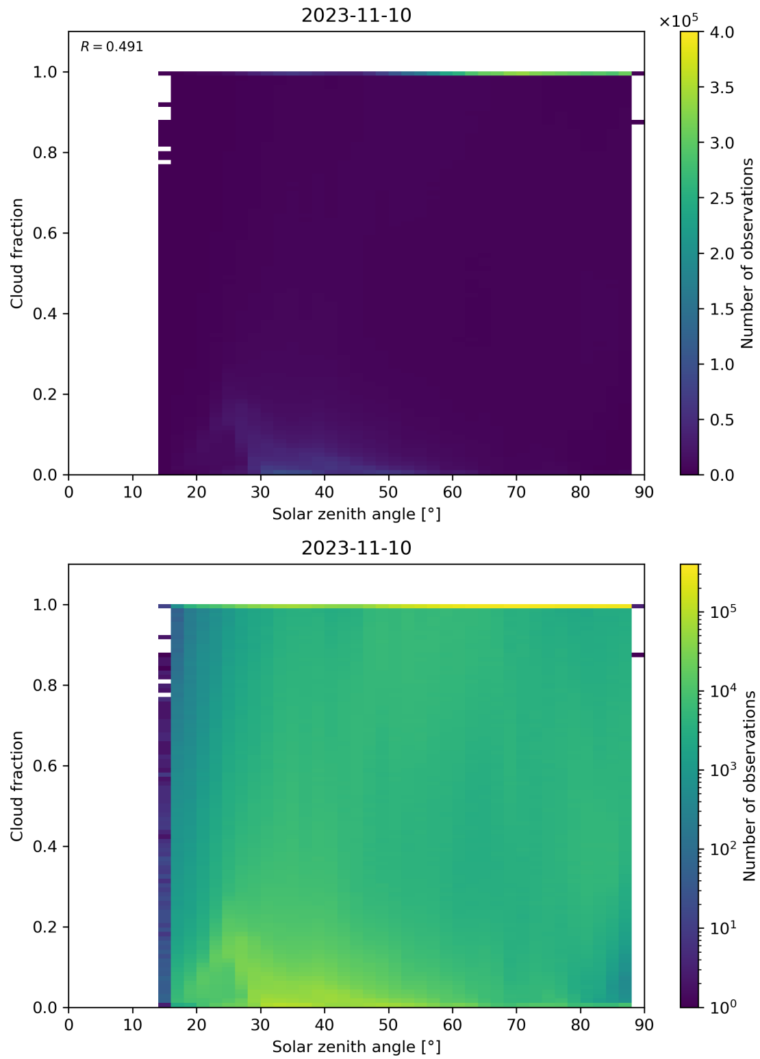
Figure 121: Scatter density plot of “Solar zenith angle” against “Cloud fraction” for 2023-11-09 to 2023-11-11.
