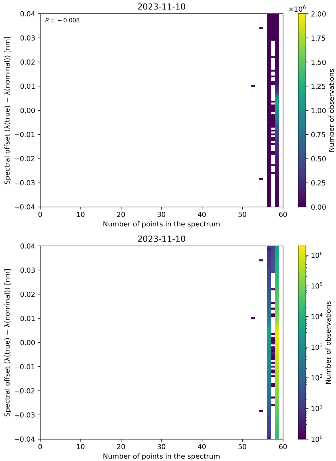
Figure 110: Scatter density plot of “Number of points in the spectrum” against “Spectral offset ( \lambda(\text{true}) - \lambda(\text{nominal}) )” for 2023-11-09 to 2023-11-11.
