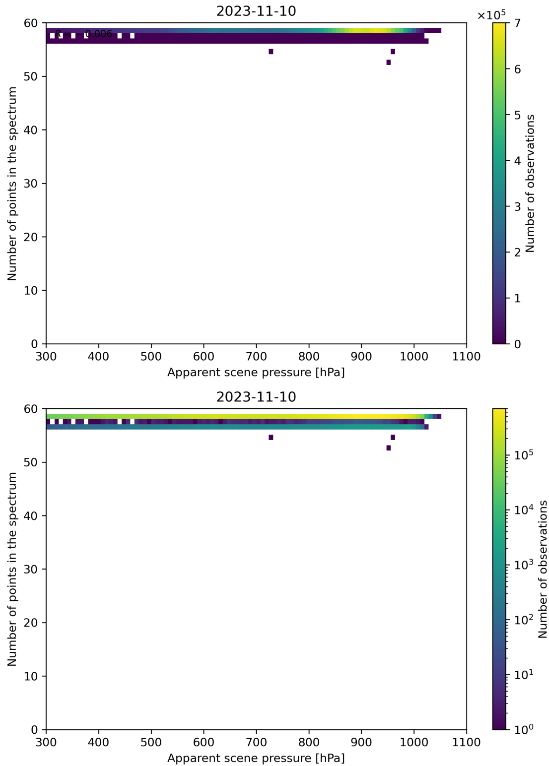
Figure 67: Scatter density plot of “Apparent scene pressure” against “Number of points in the spectrum” for 2023-11-09 to 2023-11-11.
