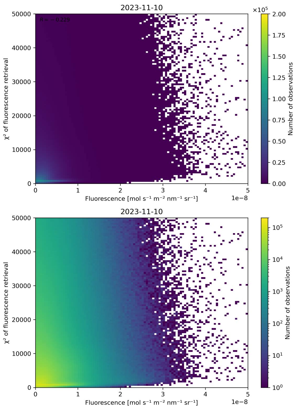
Figure 93: Scatter density plot of “Fluorescence” against “ \chi^2 of fluorescence retrieval” for 2023-11-09 to 2023-11-11.
