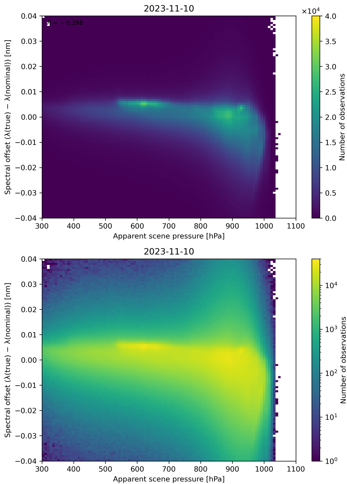
Figure 68: Scatter density plot of “Apparent scene pressure” against “Spectral offset ( \lambda(\text{true}) - \lambda(\text{nominal}) )” for 2023-11-09 to 2023-11-11.
