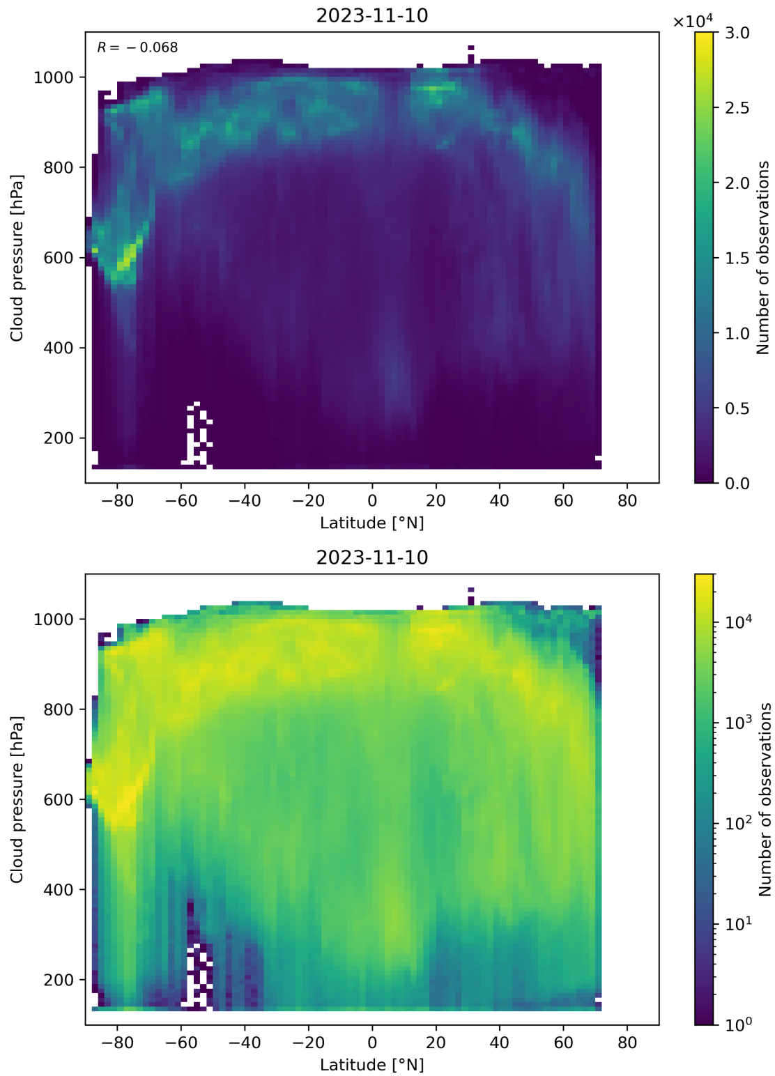
Figure 100: Scatter density plot of “Latitude” against “Cloud pressure” for 2023-11-09 to 2023-11-11.
