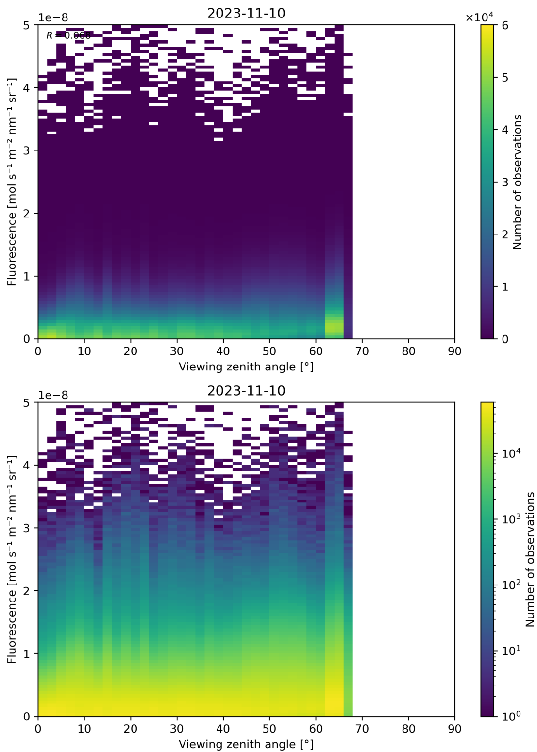
Figure 134: Scatter density plot of “Viewing zenith angle” against “Fluorescence” for 2023-11-09 to 2023-11-11.
