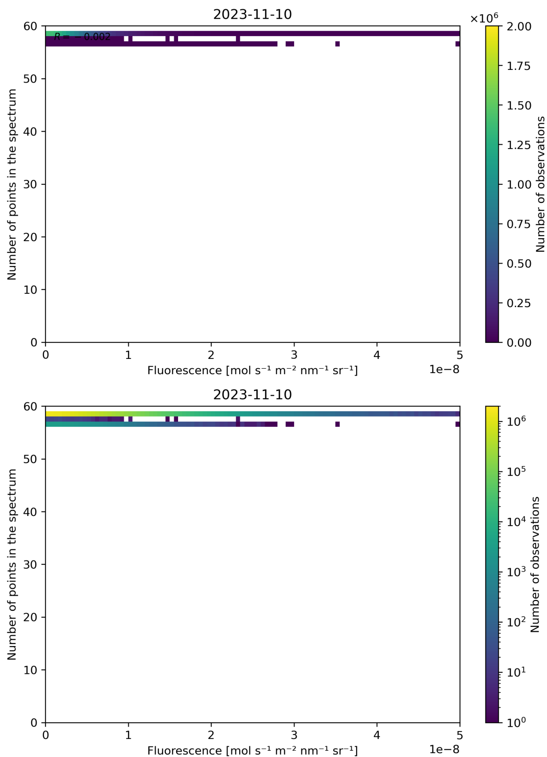
Figure 94: Scatter density plot of “Fluorescence” against “Number of points in the spectrum” for 2023-11-09 to 2023-11-11.
