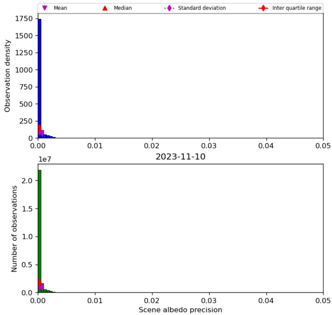
Figure 35: Histogram of “Scene albedo precision” for 2023-11-09 to 2023-11-11
