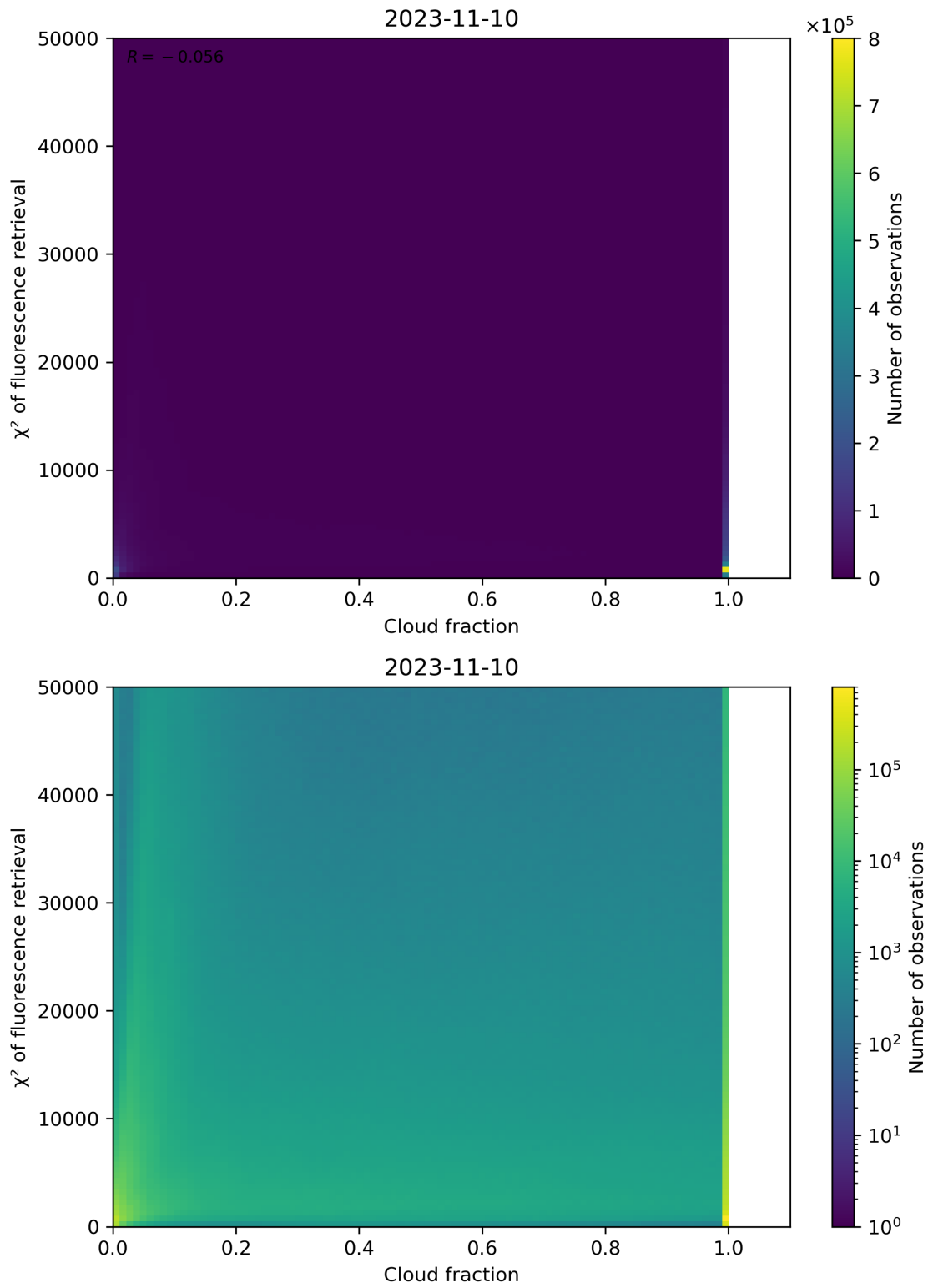
Figure 78: Scatter density plot of “Cloud fraction” against “ \chi^2 of fluorescence retrieval” for 2023-11-09 to 2023-11-11.
