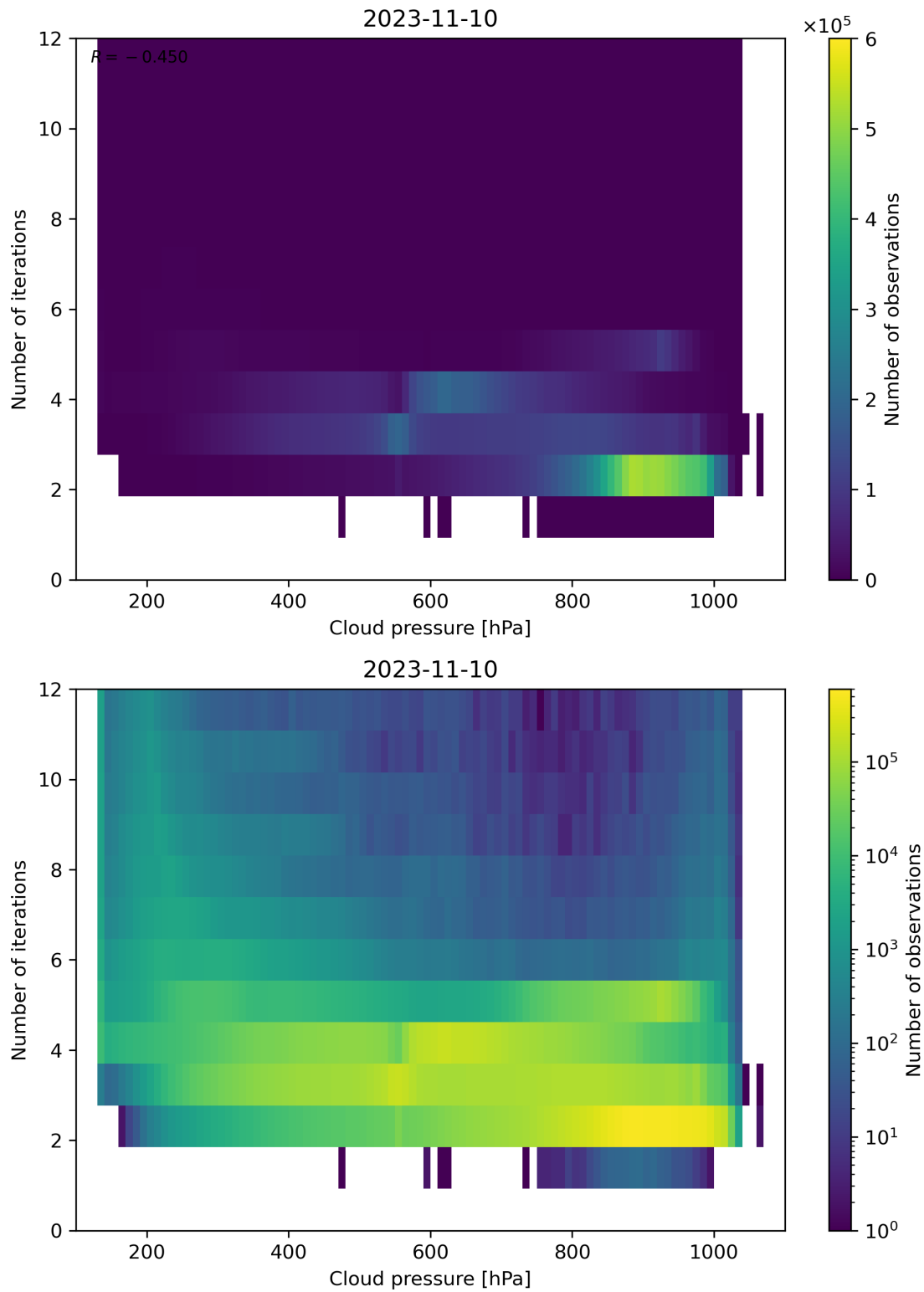
Figure 89: Scatter density plot of “Cloud pressure” against “Number of iterations” for 2023-11-09 to 2023-11-11.
