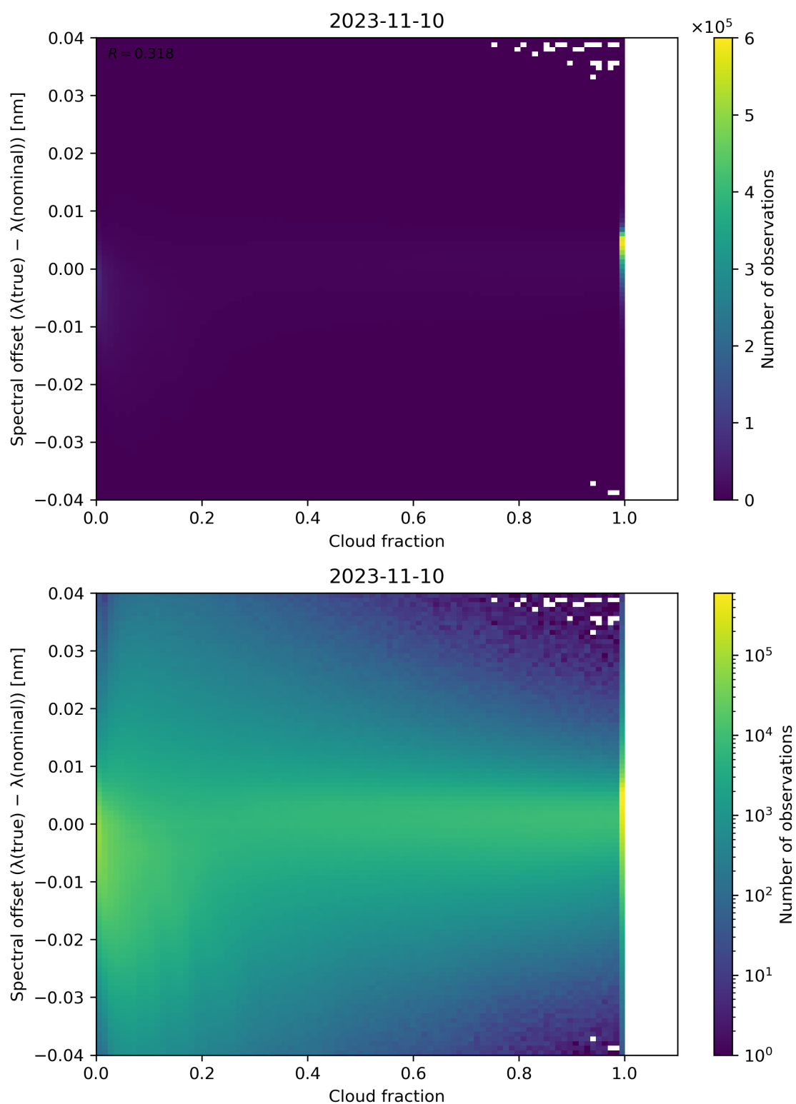
Figure 83: Scatter density plot of “Cloud fraction” against “Spectral offset ( \lambda(\text{true}) - \lambda(\text{nominal}) )” for 2023-11-09 to 2023-11-11.
