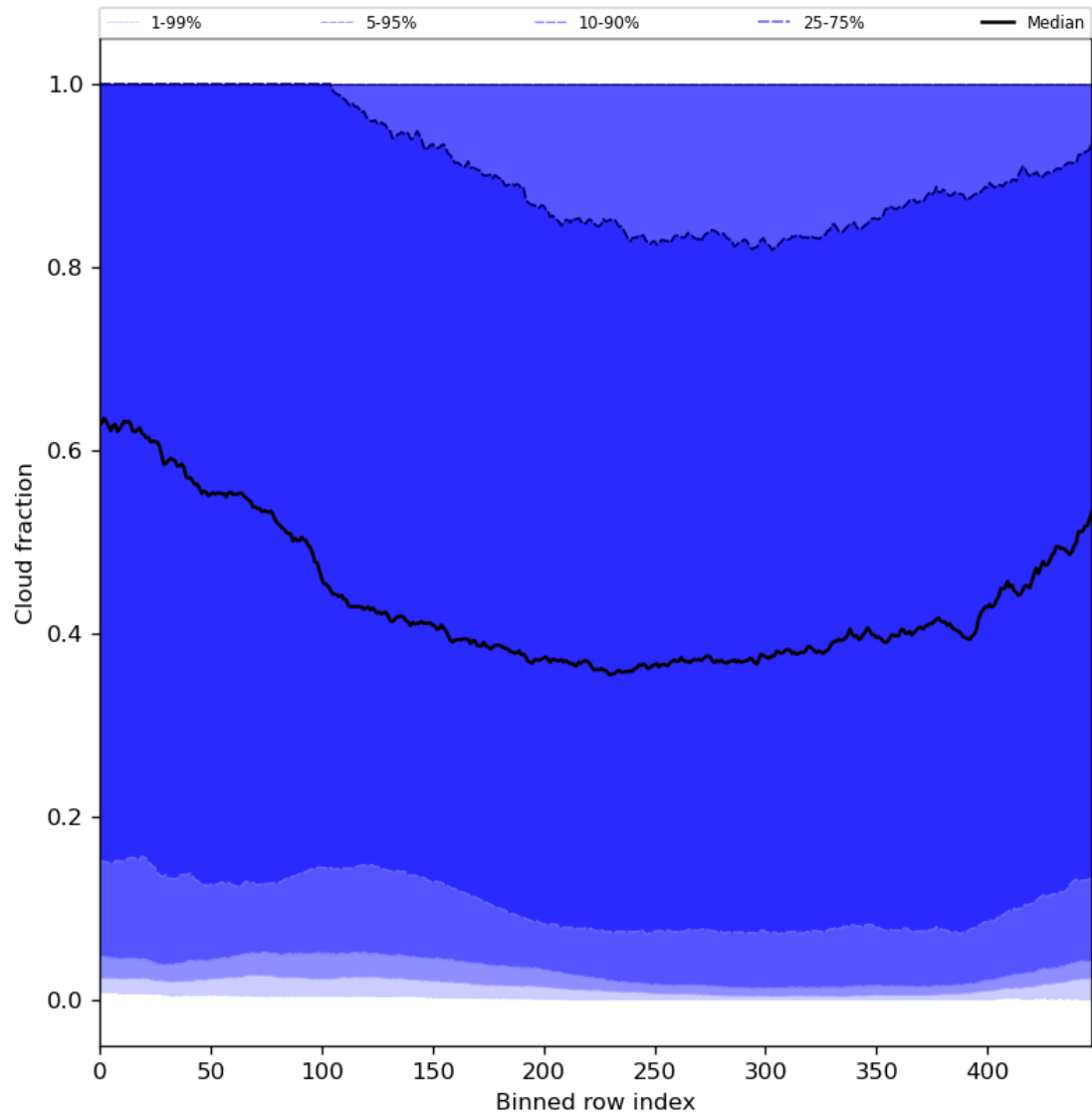
Figure 49: Along track statistics of “Cloud fraction” for 2023-11-09 to 2023-11-11
