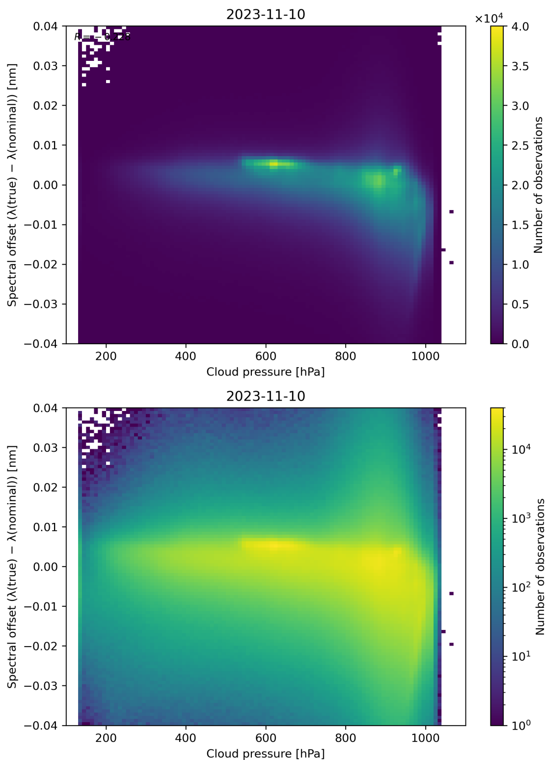
Figure 92: Scatter density plot of “Cloud pressure” against “Spectral offset ( \lambda(\text{true}) - \lambda(\text{nominal}) )” for 2023-11-09 to 2023-11-11.
