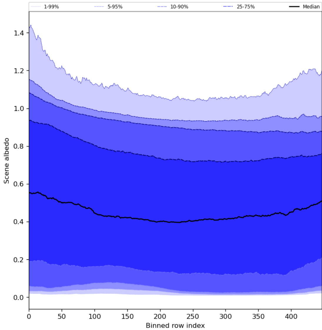
Figure 51: Along track statistics of “Scene albedo” for 2023-11-09 to 2023-11-11
