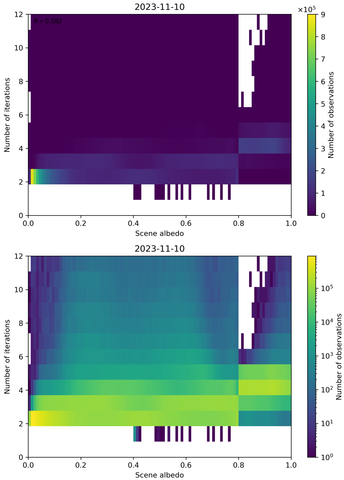
Figure 115: Scatter density plot of “Scene albedo” against “Number of iterations” for 2023-11-09 to 2023-11-11.
