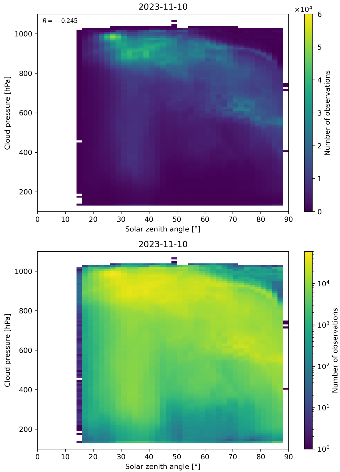
Figure 122: Scatter density plot of “Solar zenith angle” against “Cloud pressure” for 2023-11-09 to 2023-11-11.
