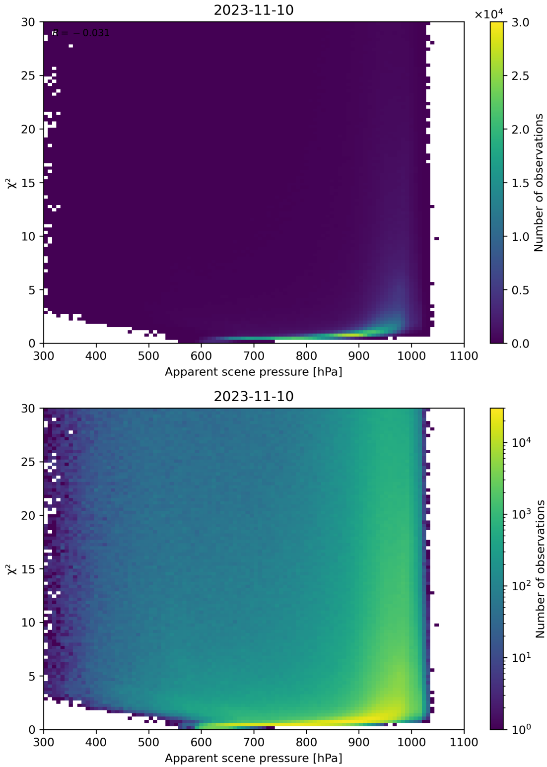
Figure 63: Scatter density plot of “Apparent scene pressure” against “ \chi^2 ” for 2023-11-09 to 2023-11-11.
