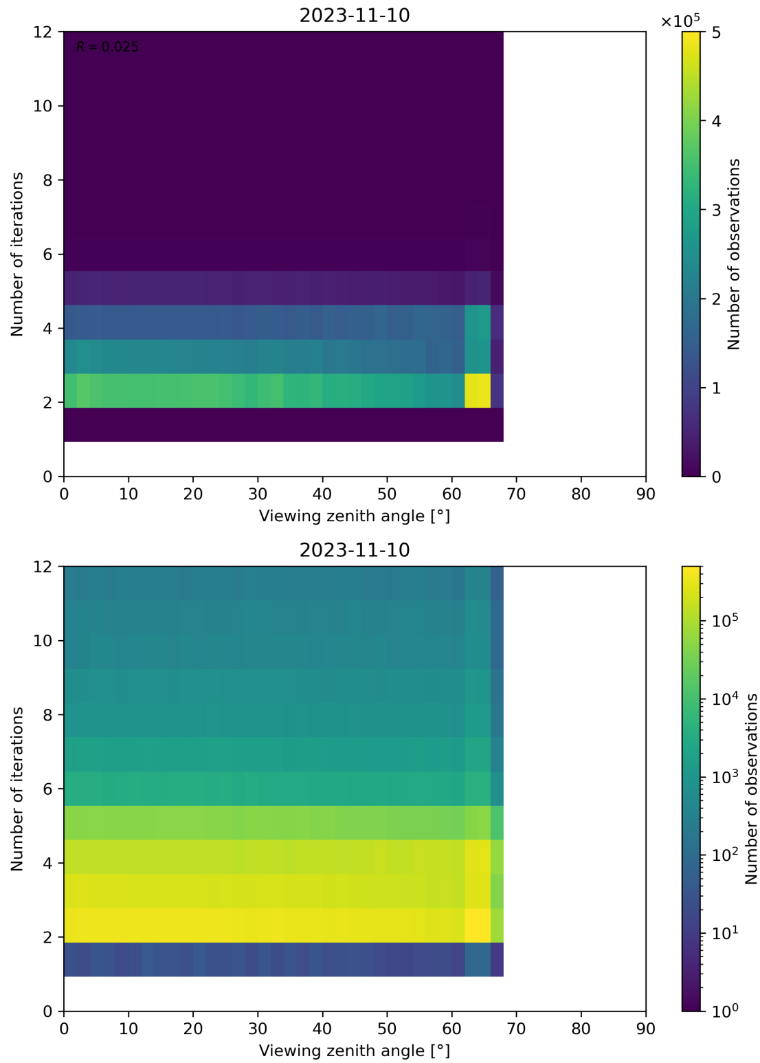
Figure 136: Scatter density plot of “Viewing zenith angle” against “Number of iterations” for 2023-11-09 to 2023-11-11.
