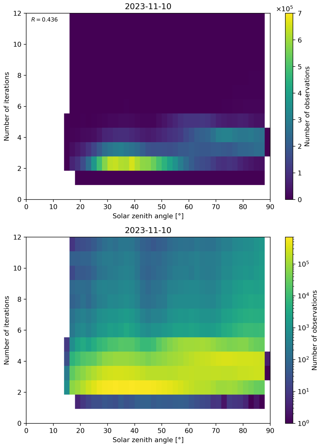
Figure 125: Scatter density plot of “Solar zenith angle” against “Number of iterations” for 2023-11-09 to 2023-11-11.
