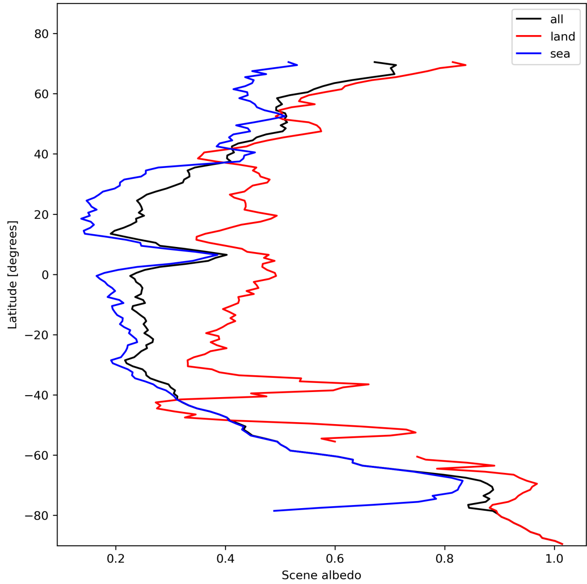
Figure 17: Zonal average of “Scene albedo” for 2023-11-09 to 2023-11-11.
