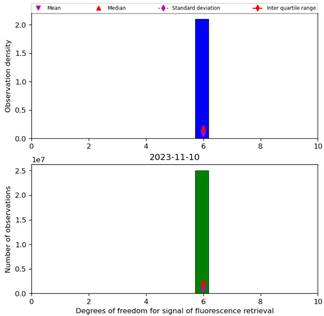
Figure 43: Histogram of “Degrees of freedom for signal of fluorescence retrieval” for 2023-11-09 to 2023-11-11
