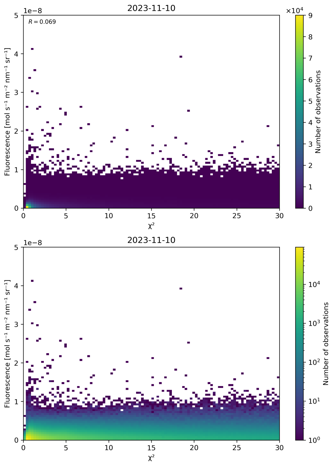
Figure 70: Scatter density plot of “ \chi^2 ” against “Fluorescence” for 2023-11-09 to 2023-11-11.
