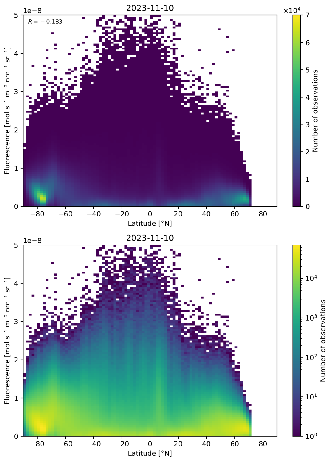
Figure 101: Scatter density plot of “Latitude” against “Fluorescence” for 2023-11-09 to 2023-11-11.
