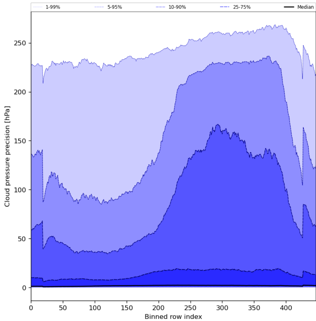
Figure 48: Along track statistics of “Cloud pressure precision” for 2023-11-09 to 2023-11-11
