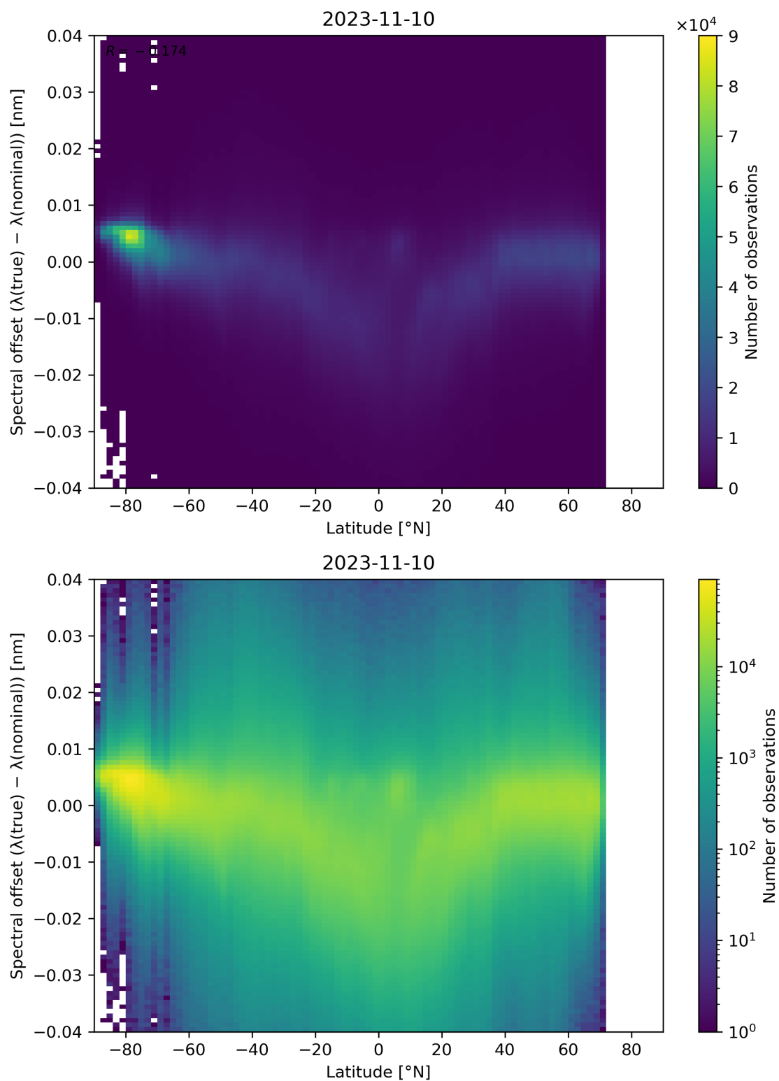
Figure 105: Scatter density plot of “Latitude” against “Spectral offset ( \lambda(\text{true}) - \lambda(\text{nominal}) )” for 2023-11-09 to 2023-11-11.
