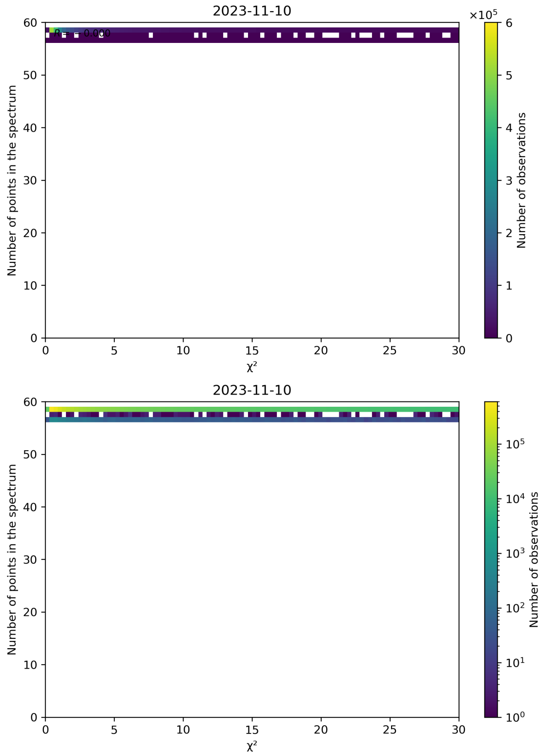
Figure 74: Scatter density plot of “ \chi^2 ” against “Number of points in the spectrum” for 2023-11-09 to 2023-11-11.
