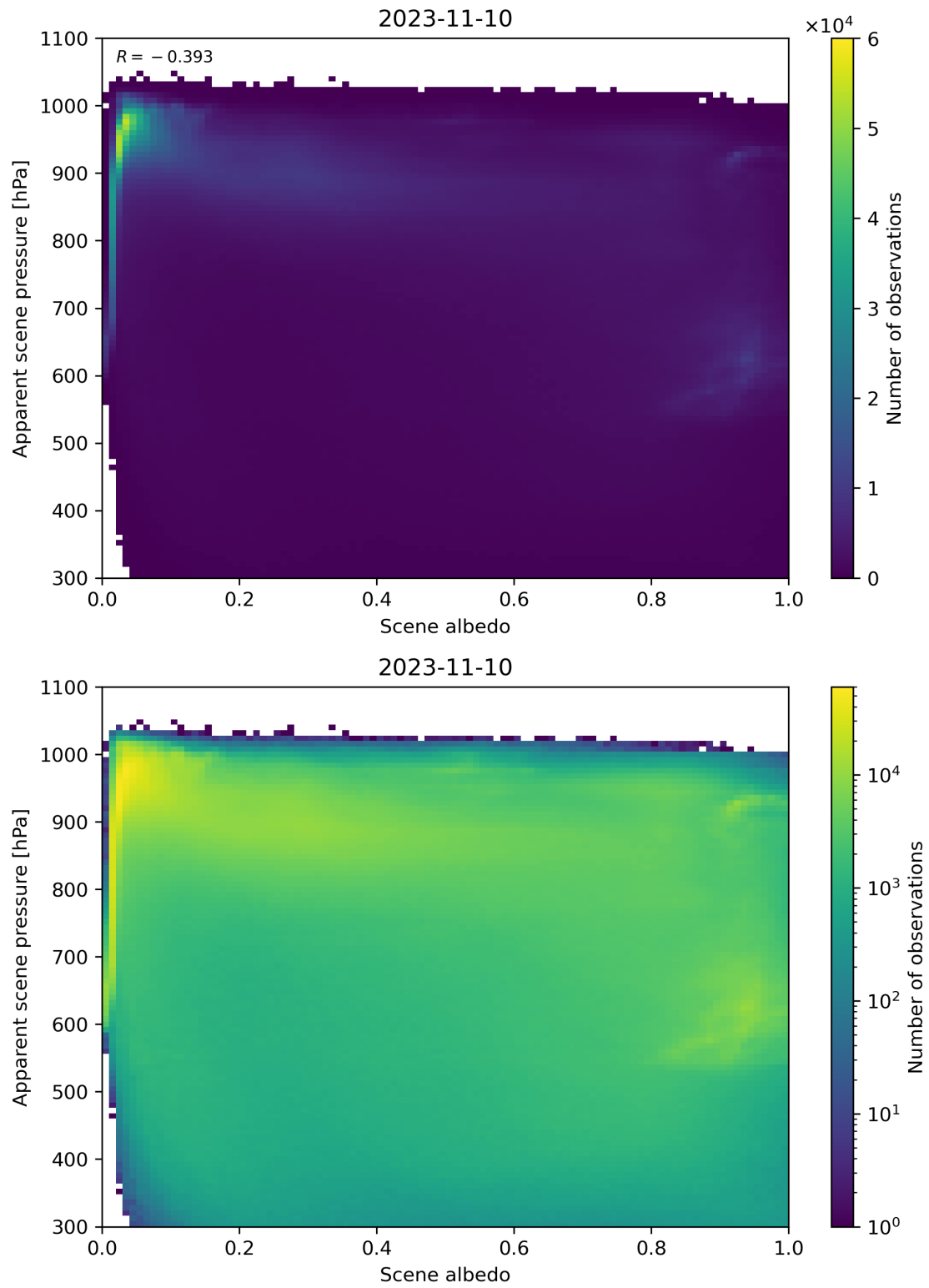
Figure 111: Scatter density plot of “Scene albedo” against “Apparent scene pressure” for 2023-11-09 to 2023-11-11.
