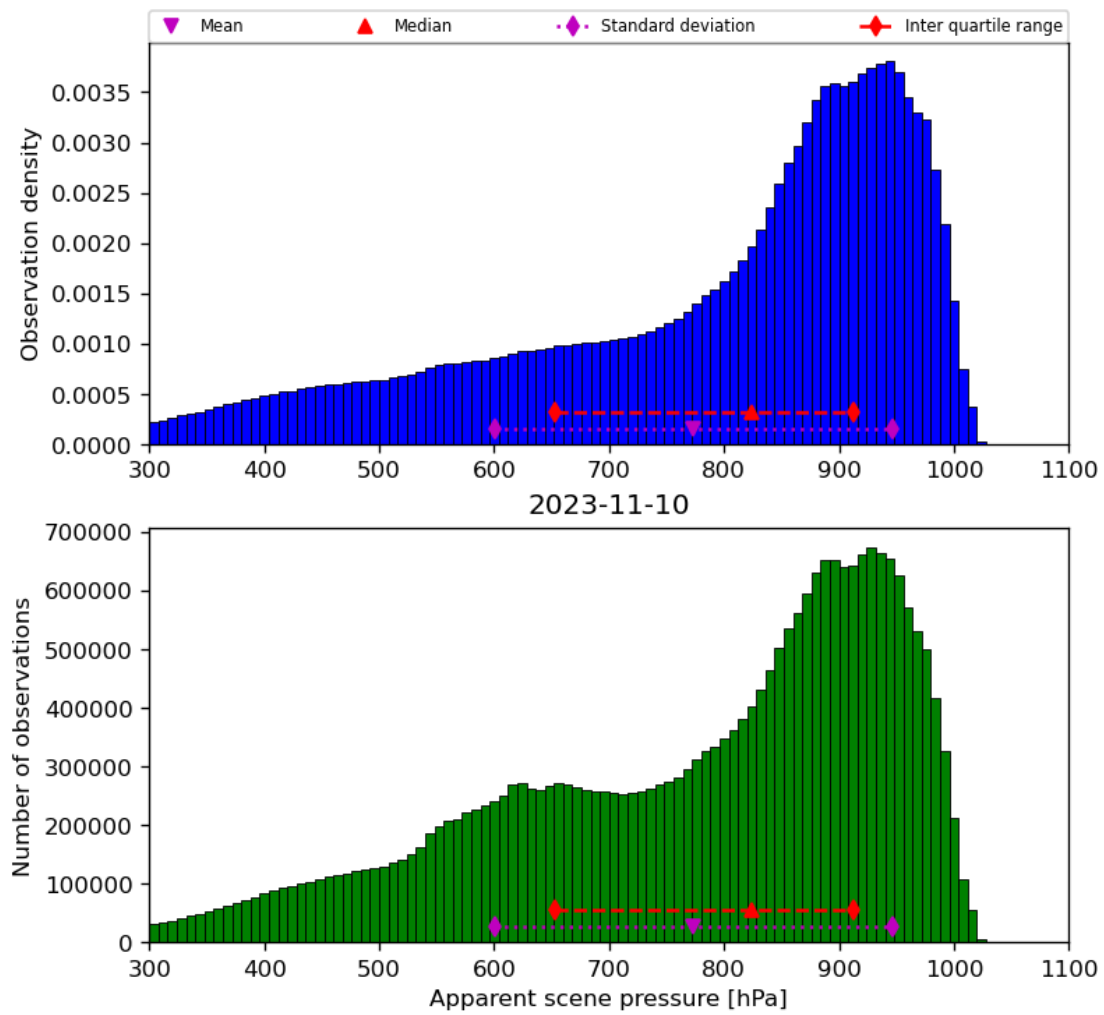
Figure 36: Histogram of “Apparent scene pressure” for 2023-11-09 to 2023-11-11
