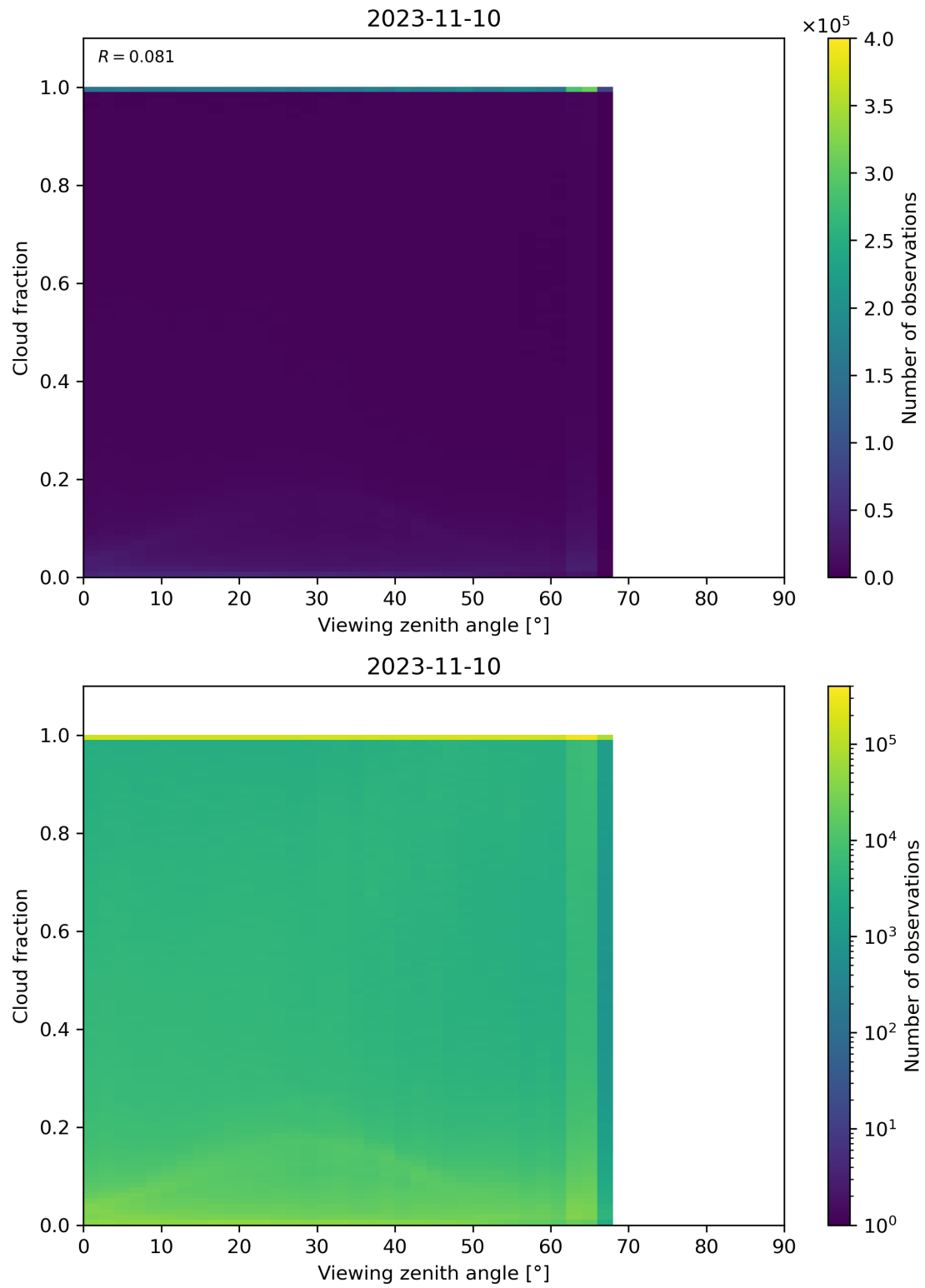
Figure 132: Scatter density plot of “Viewing zenith angle” against “Cloud fraction” for 2023-11-09 to 2023-11-11.
