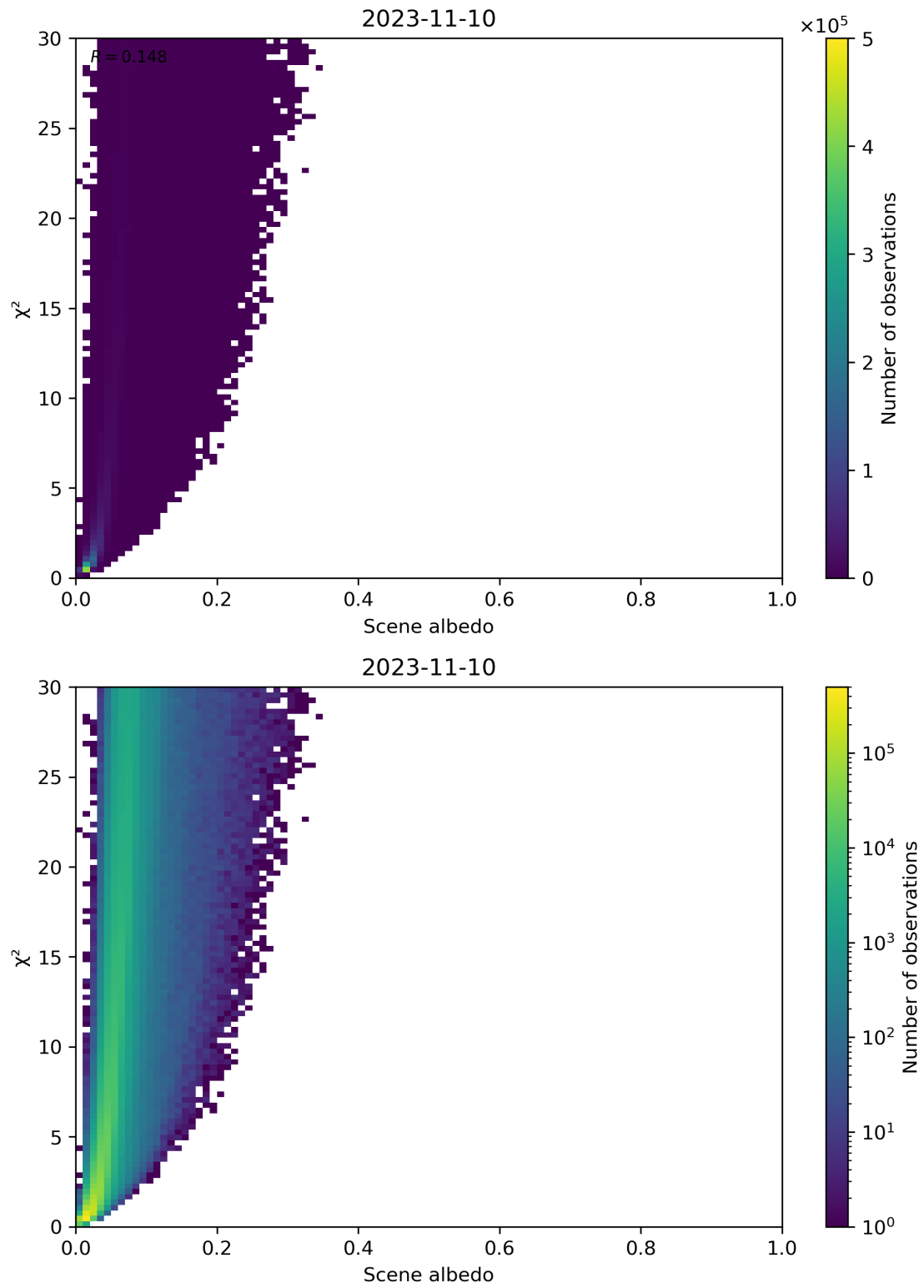
Figure 112: Scatter density plot of “Scene albedo” against “ \chi^2 ” for 2023-11-09 to 2023-11-11.
