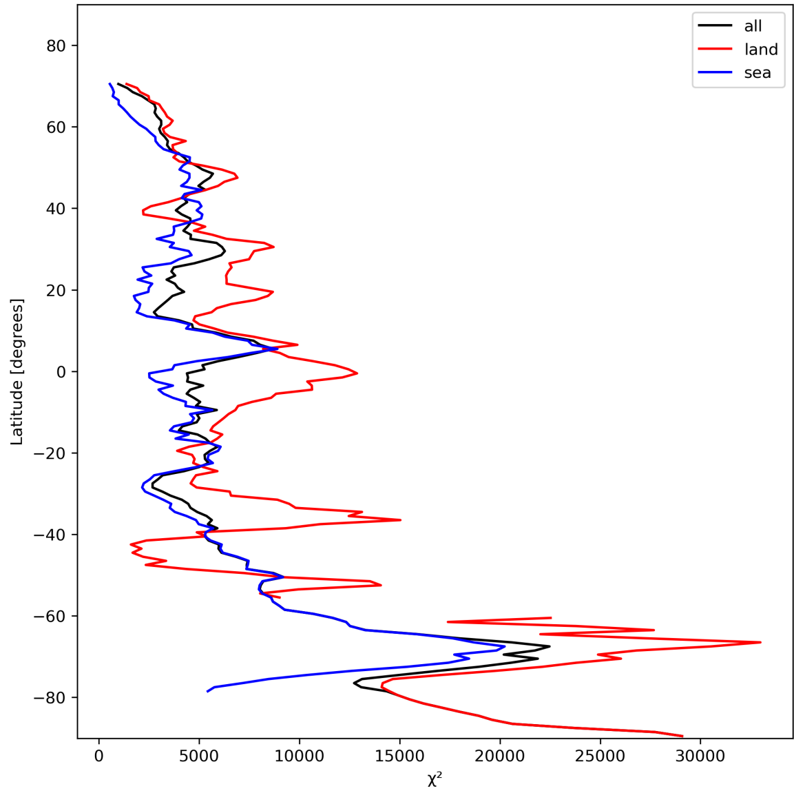
Figure 21: Zonal average of “ \chi^2 ” for 2023-11-09 to 2023-11-11.
