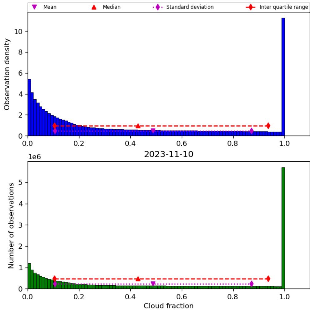
Figure 32: Histogram of “Cloud fraction” for 2023-11-09 to 2023-11-11
