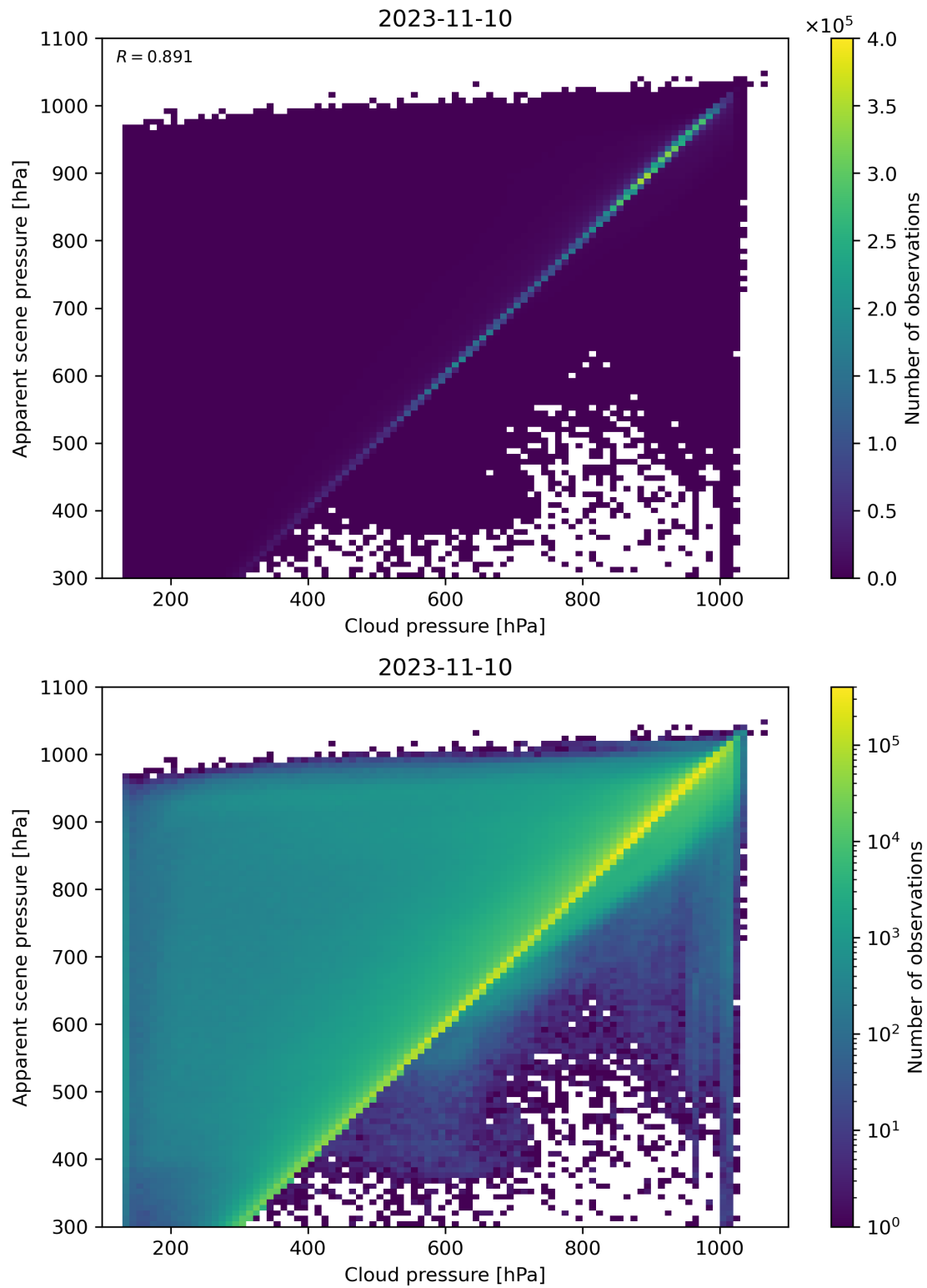
Figure 84: Scatter density plot of “Cloud pressure” against “Apparent scene pressure” for 2023-11-09 to 2023-11-11.
