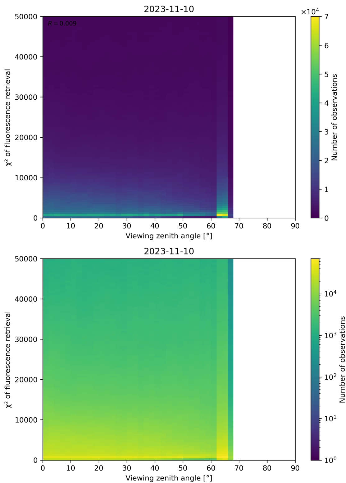
Figure 131: Scatter density plot of “Viewing zenith angle” against “ \chi^2 of fluorescence retrieval” for 2023-11-09 to 2023-11-11.
