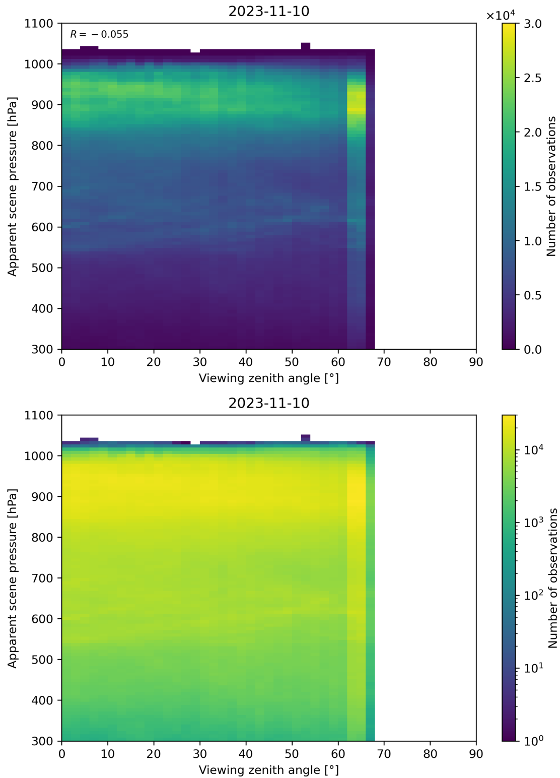
Figure 129: Scatter density plot of “Viewing zenith angle” against “Apparent scene pressure” for 2023-11-09 to 2023-11-11.
