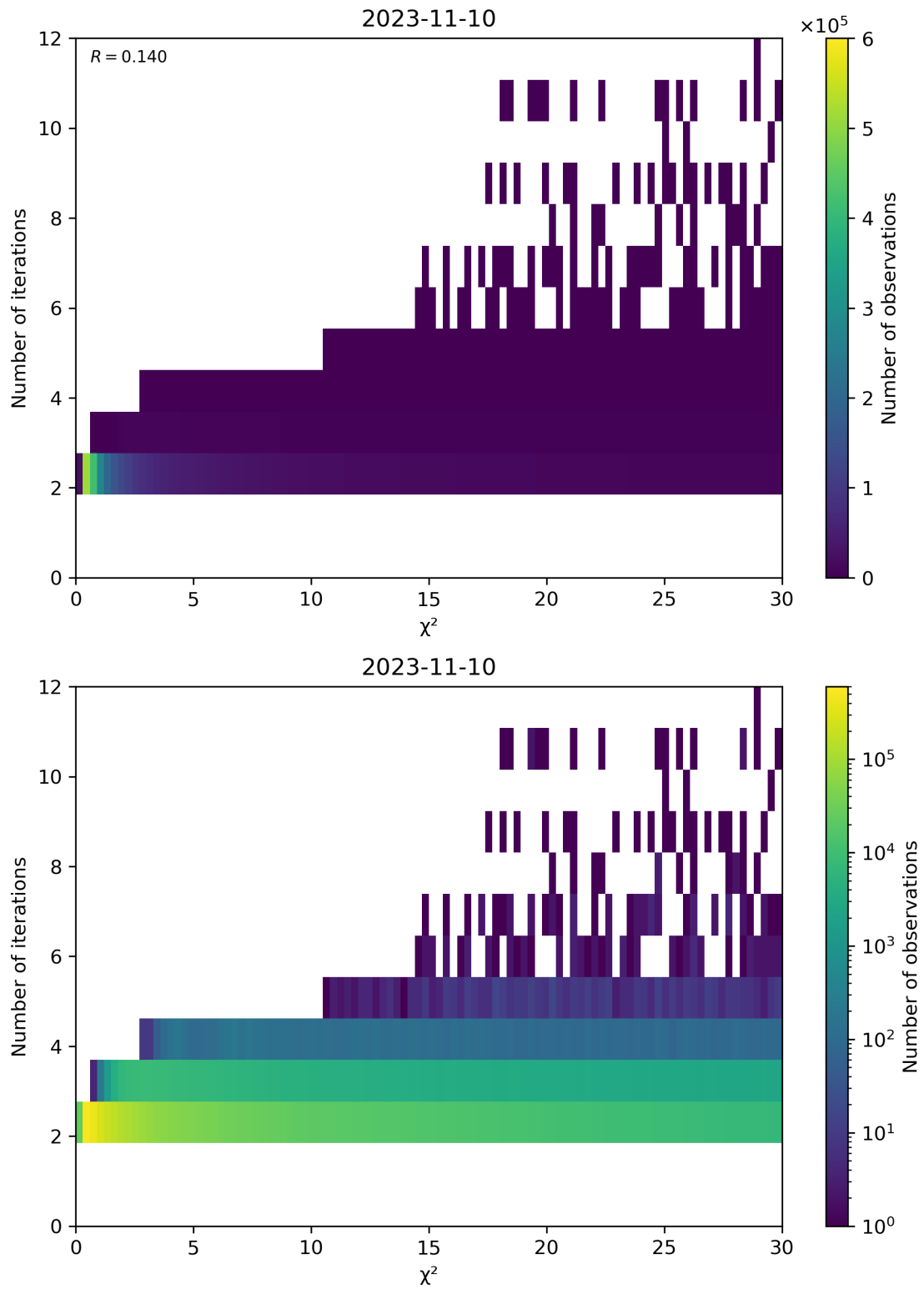
Figure 73: Scatter density plot of “ \chi^2 ” against “Number of iterations” for 2023-11-09 to 2023-11-11.
