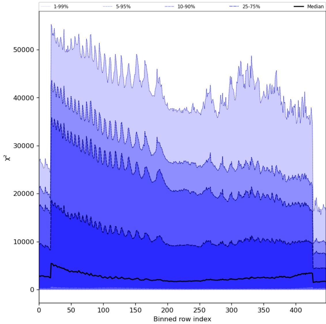
Figure 55: Along track statistics of “ \chi^2 ” for 2023-11-09 to 2023-11-11
