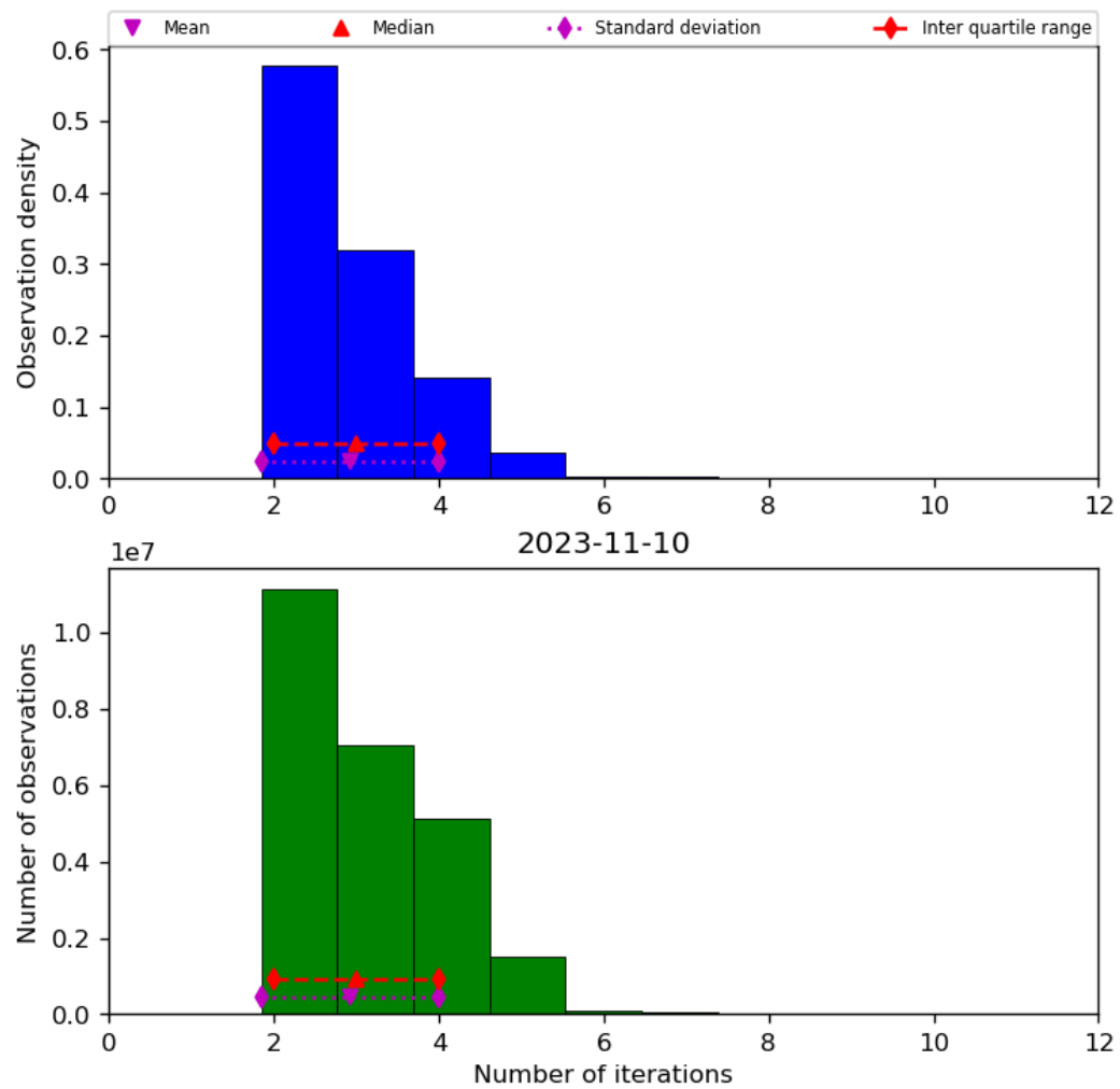
Figure 39: Histogram of “Number of iterations” for 2023-11-09 to 2023-11-11
