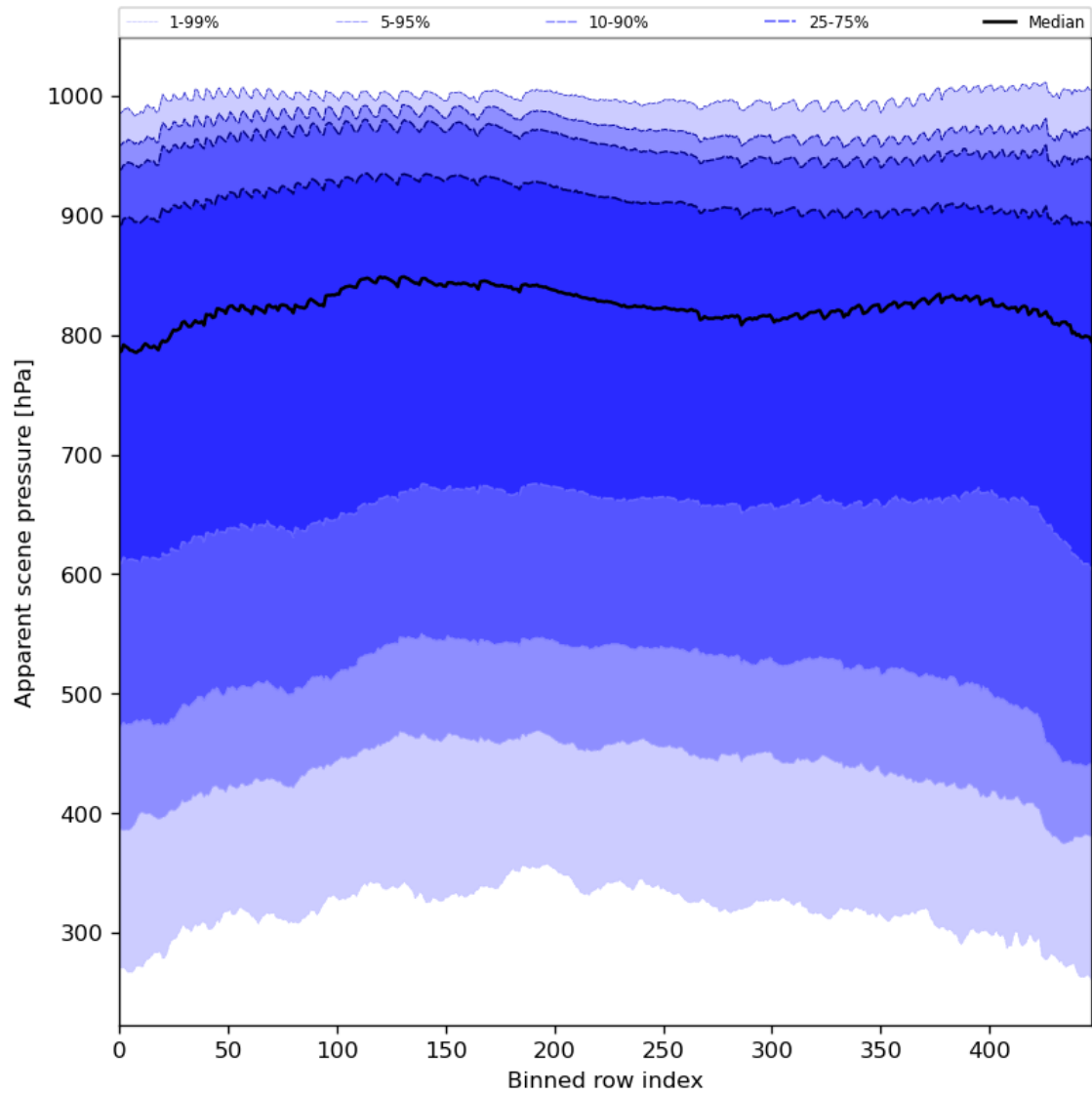
Figure 53: Along track statistics of “Apparent scene pressure” for 2023-11-09 to 2023-11-11
