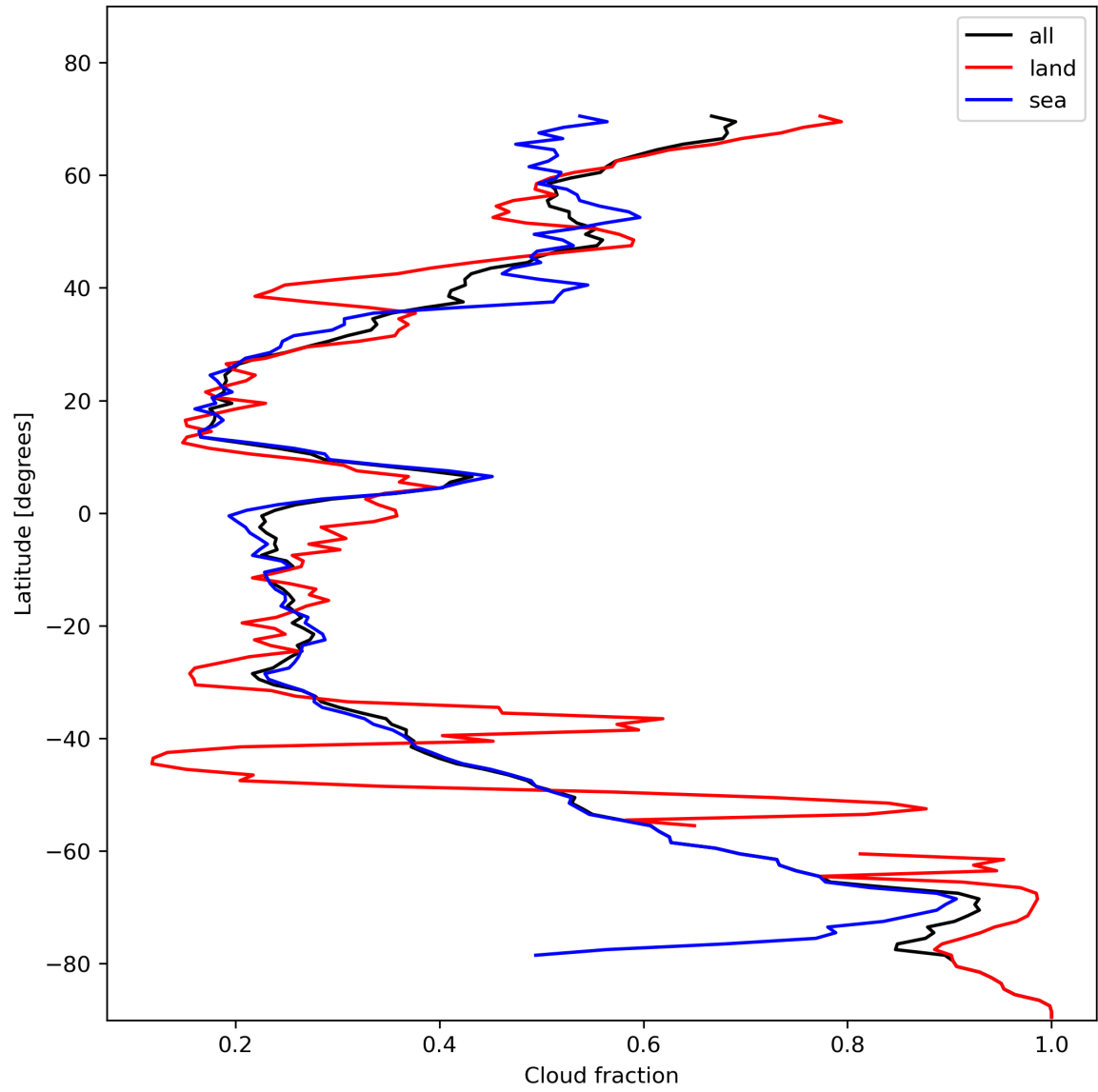
Figure 15: Zonal average of “Cloud fraction” for 2023-11-09 to 2023-11-11.
