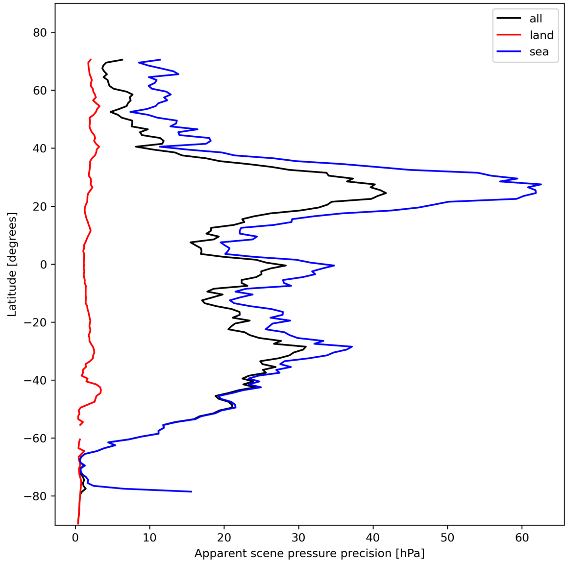
Figure 20: Zonal average of “Apparent scene pressure precision” for 2023-11-09 to 2023-11-11.
