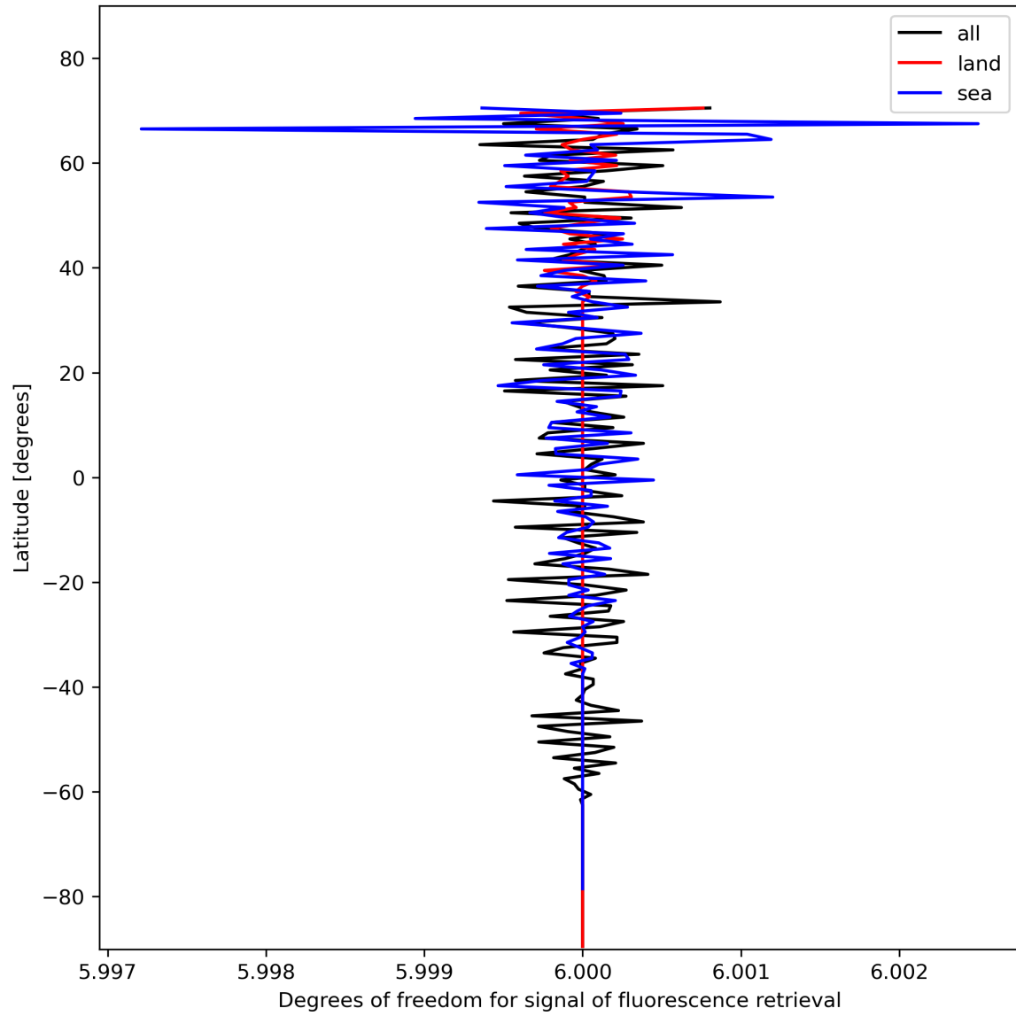
Figure 26: Zonal average of “Degrees of freedom for signal of fluorescence retrieval” for 2023-11-09 to 2023-11-11.
