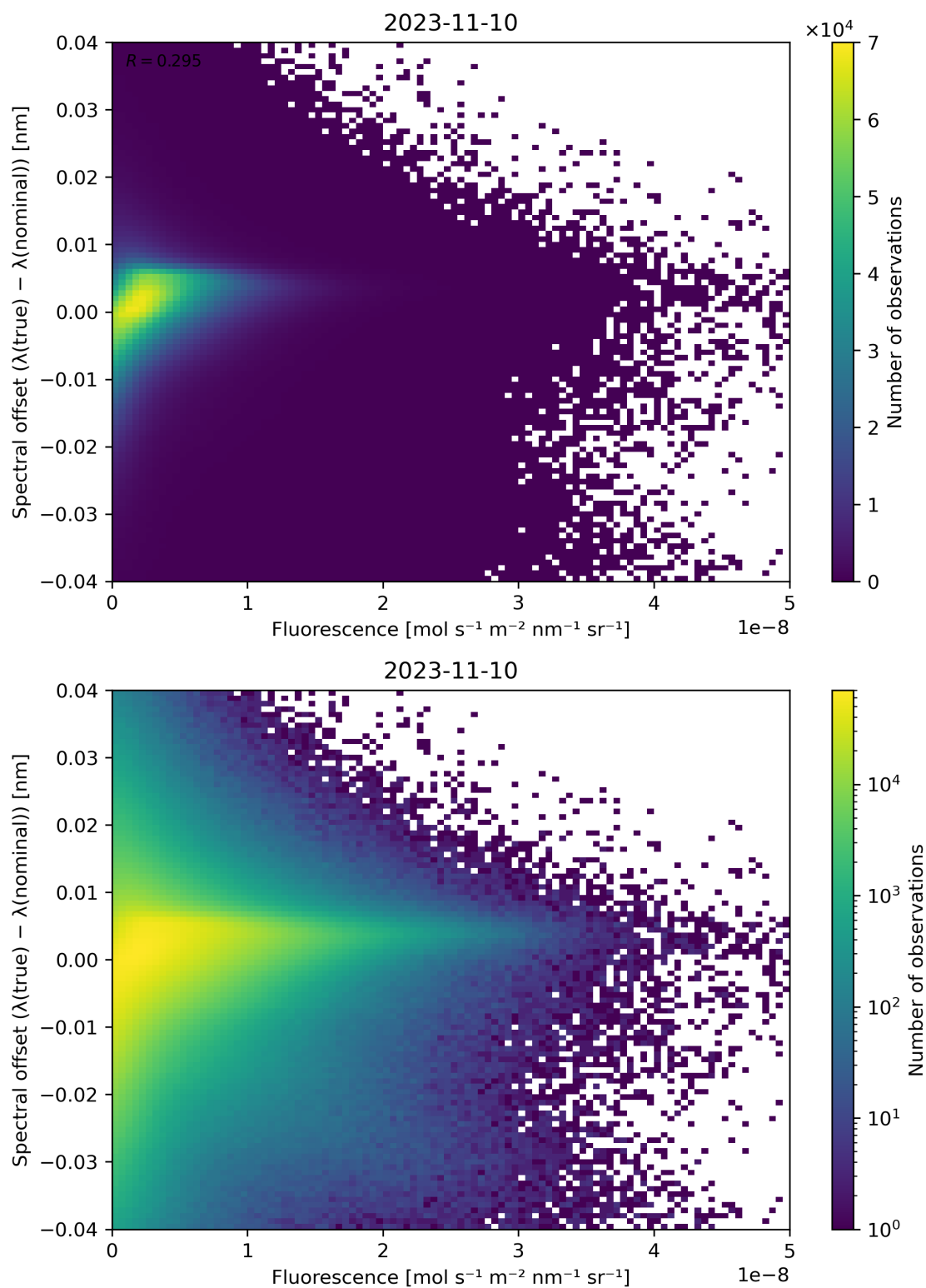
Figure 95: Scatter density plot of “Fluorescence” against “Spectral offset ( \lambda(\text{true}) - \lambda(\text{nominal}) )” for 2023-11-09 to 2023-11-11.
