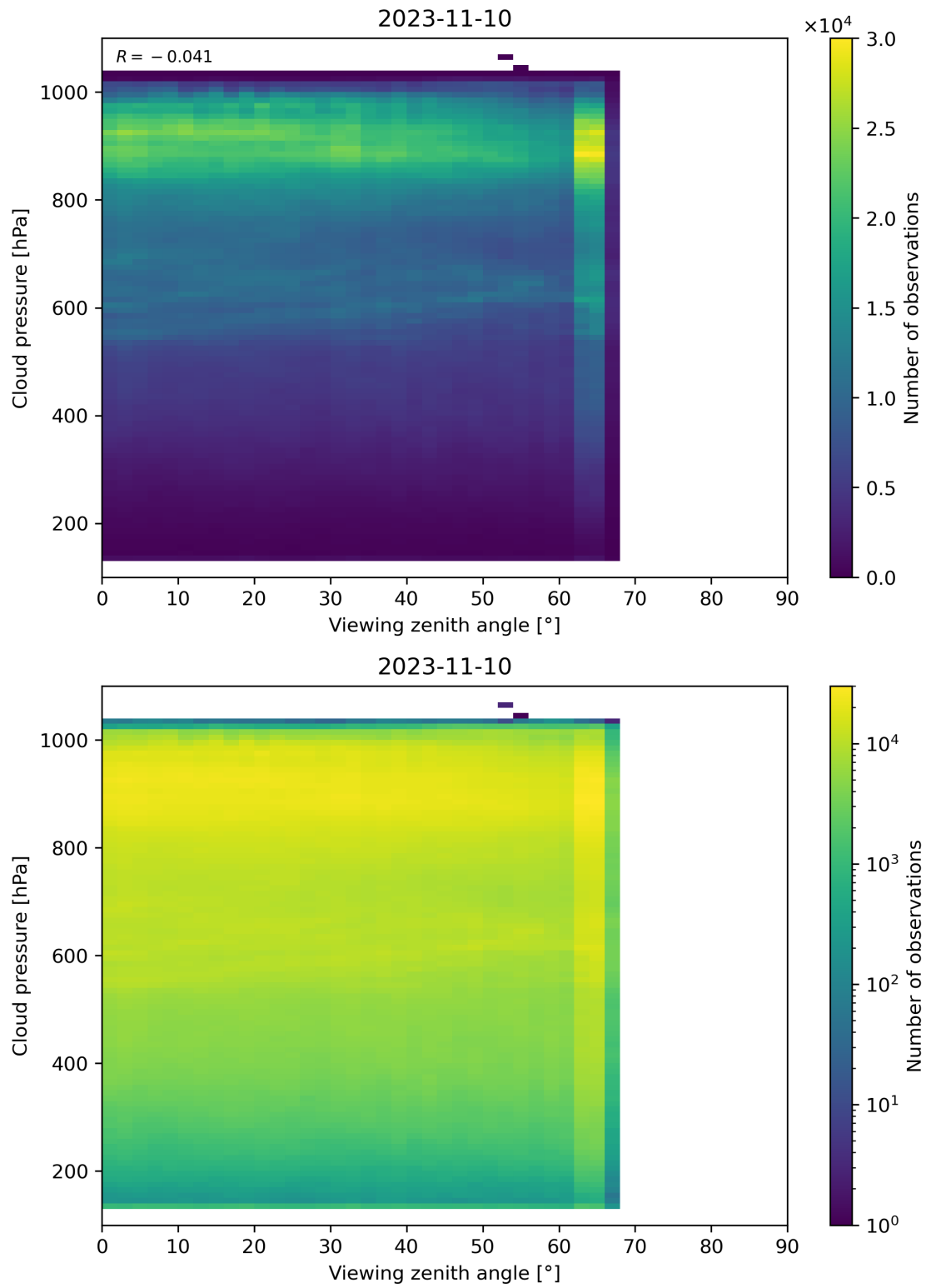
Figure 133: Scatter density plot of “Viewing zenith angle” against “Cloud pressure” for 2023-11-09 to 2023-11-11.
