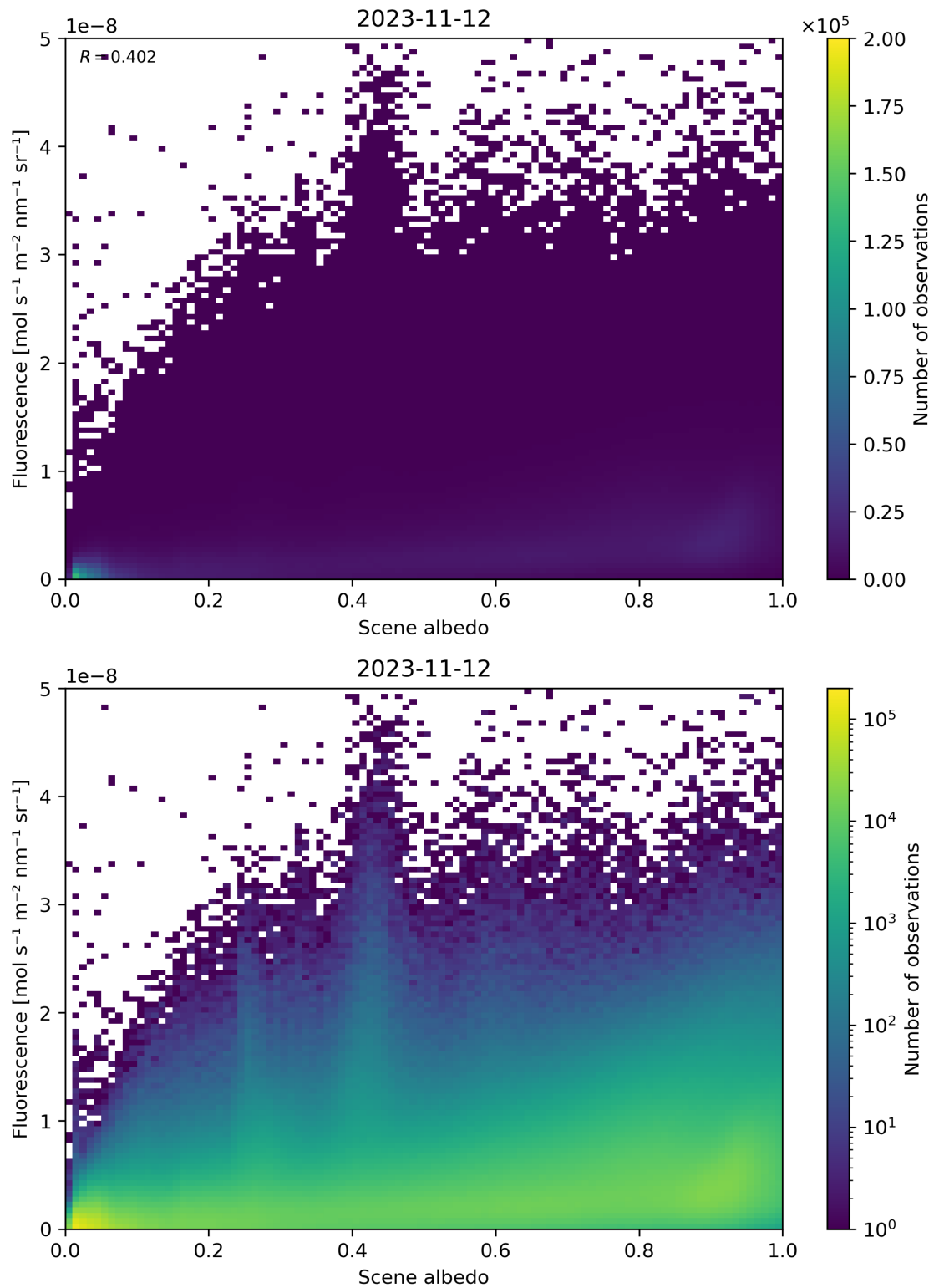
Figure 114: Scatter density plot of “Scene albedo” against “Fluorescence” for 2023-11-12 to 2023-11-13.
