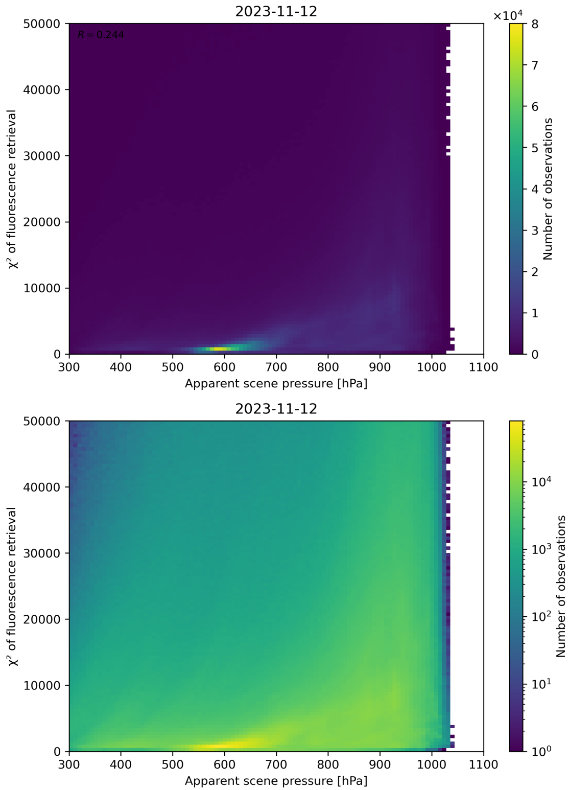
Figure 64: Scatter density plot of “Apparent scene pressure” against “ \chi^2 of fluorescence retrieval” for 2023-11-12 to 2023-11-13.
