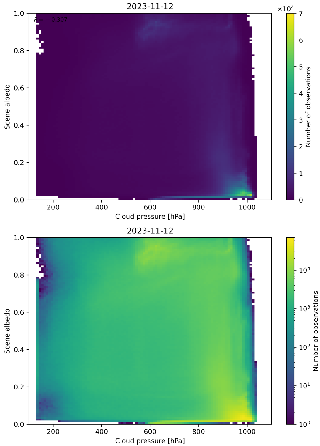
Figure 91: Scatter density plot of “Cloud pressure” against “Scene albedo” for 2023-11-12 to 2023-11-13.
