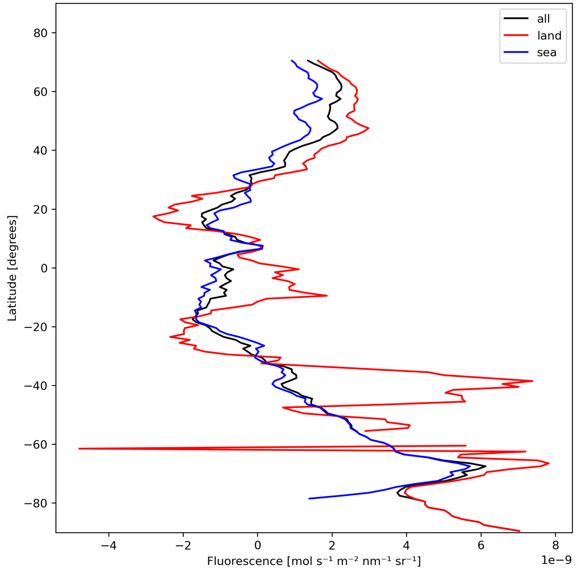
Figure 23: Zonal average of “Fluorescence” for 2023-11-12 to 2023-11-13.
