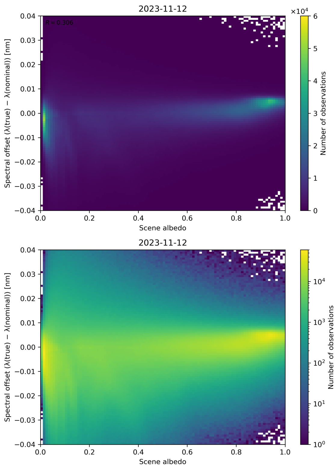
Figure 117: Scatter density plot of “Scene albedo” against “Spectral offset ( \lambda(\text{true}) - \lambda(\text{nominal}) )” for 2023-11-12 to 2023-11-13.
