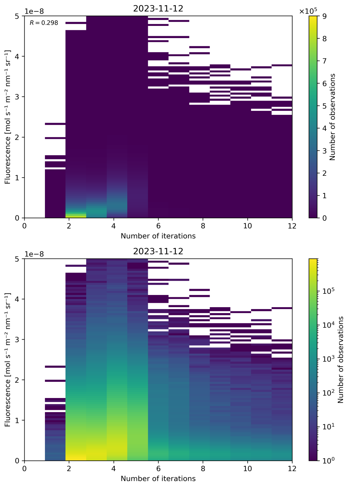
Figure 107: Scatter density plot of “Number of iterations” against “Fluorescence” for 2023-11-12 to 2023-11-13.
