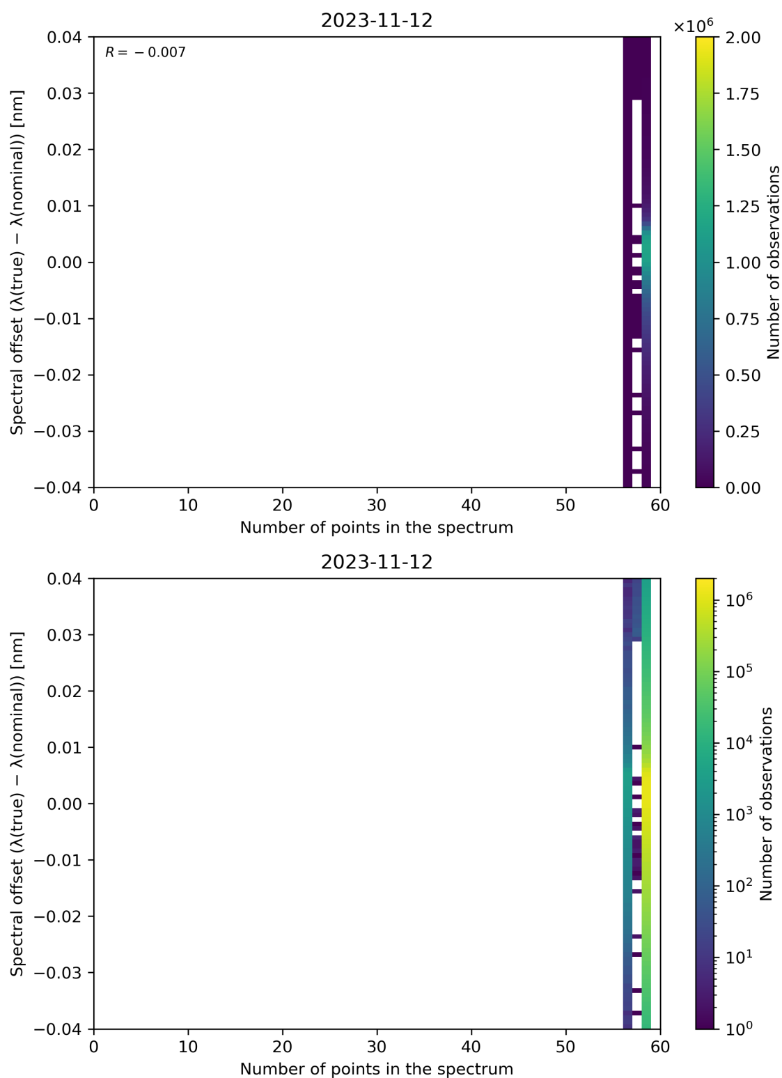
Figure 110: Scatter density plot of “Number of points in the spectrum” against “Spectral offset ( \lambda(\text{true}) - \lambda(\text{nominal}) )” for 2023-11-12 to 2023-11-13.
