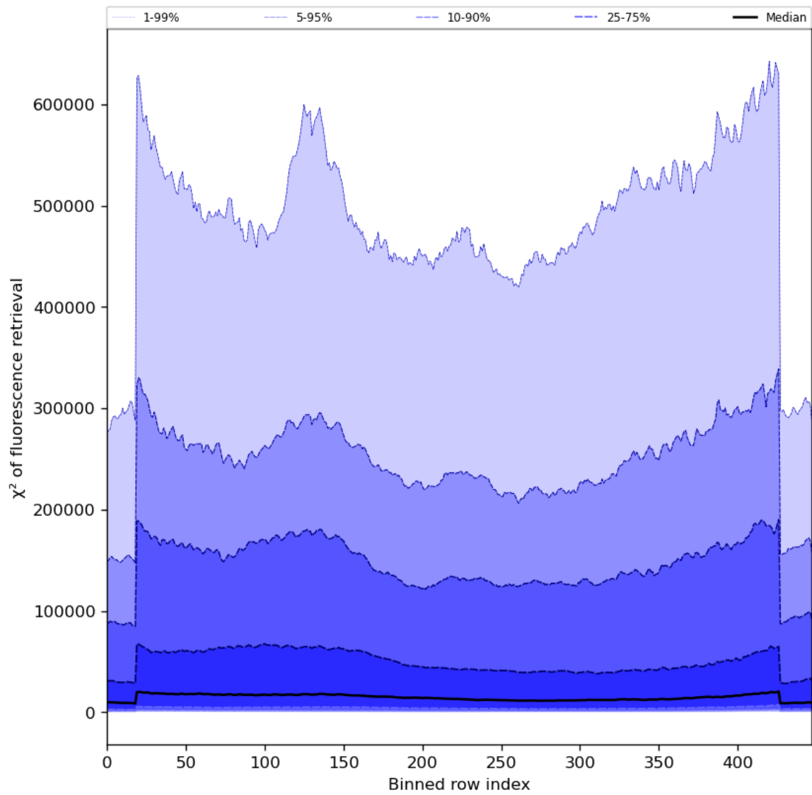
Figure 59: Along track statistics of “ \chi^2 of fluorescence retrieval” for 2023-11-12 to 2023-11-13
