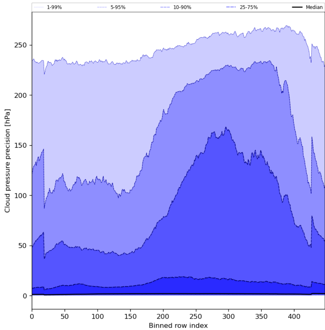
Figure 48: Along track statistics of “Cloud pressure precision” for 2023-11-12 to 2023-11-13
