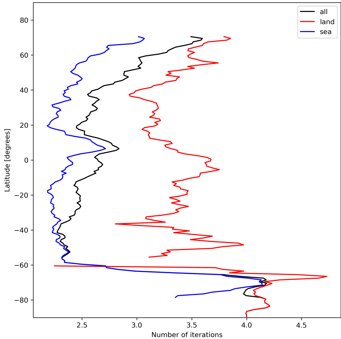
Figure 22: Zonal average of “Number of iterations” for 2023-11-12 to 2023-11-13.
