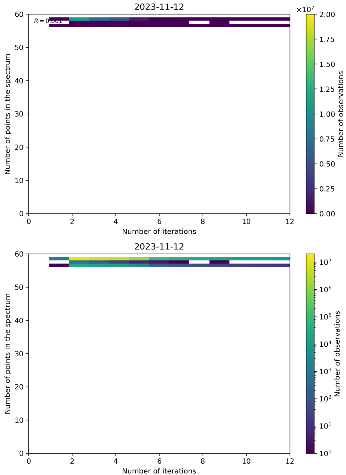
Figure 108: Scatter density plot of “Number of iterations” against “Number of points in the spectrum” for 2023-11-12 to 2023-11-13.
