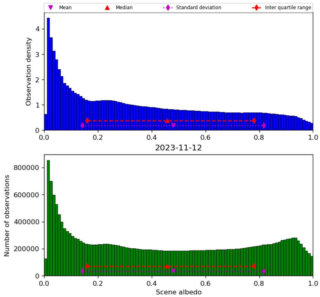
Figure 34: Histogram of “Scene albedo” for 2023-11-12 to 2023-11-13
