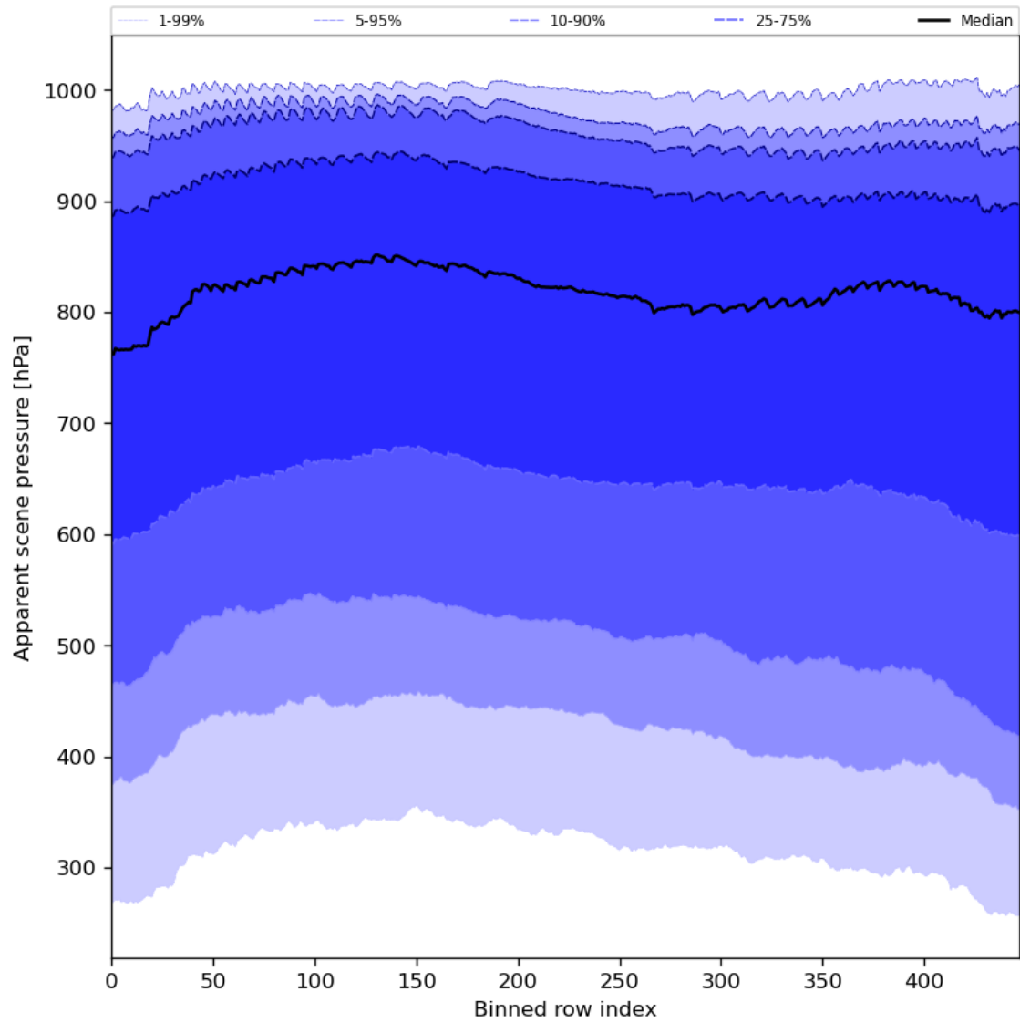
Figure 53: Along track statistics of “Apparent scene pressure” for 2023-11-12 to 2023-11-13
