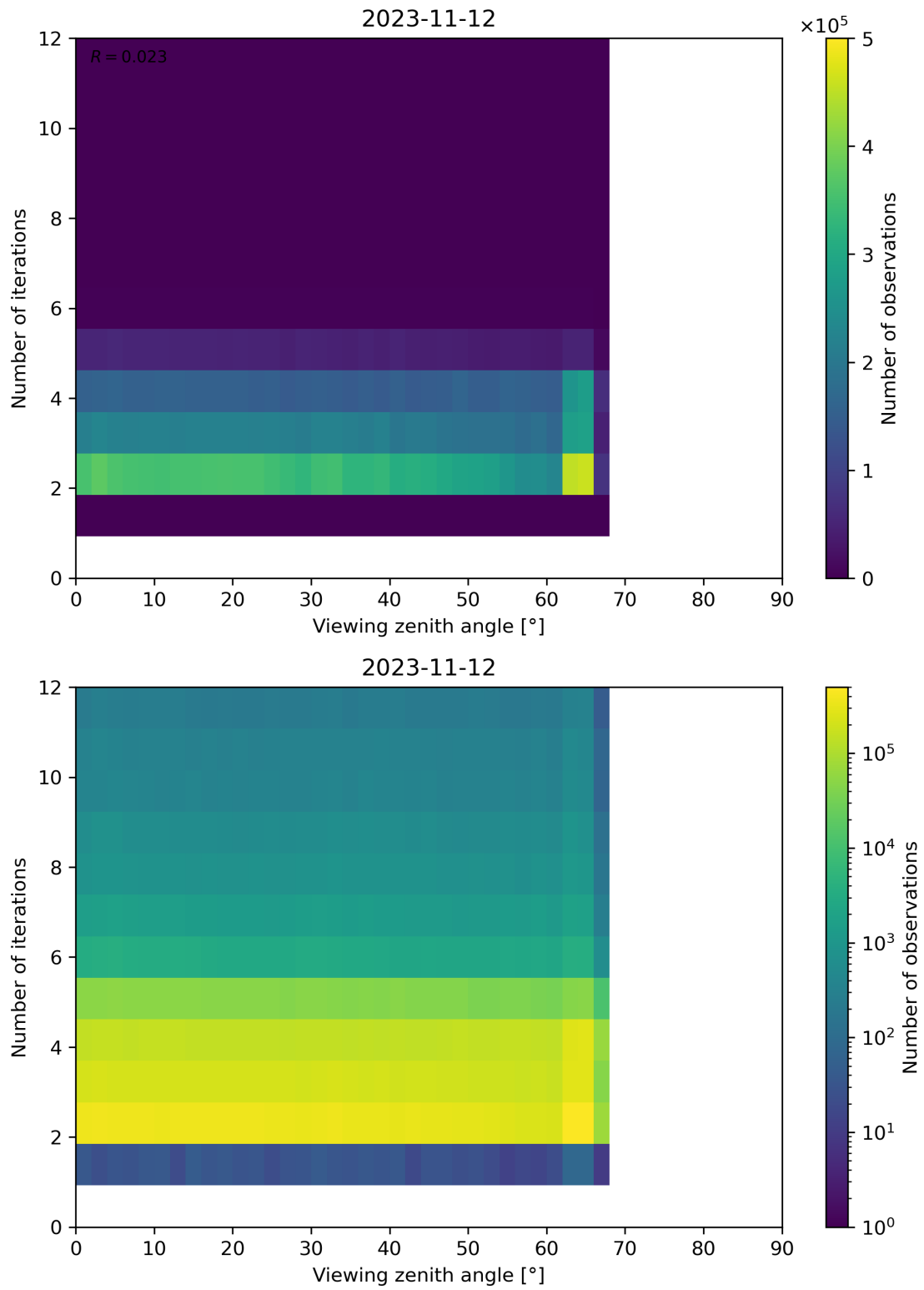
Figure 136: Scatter density plot of “Viewing zenith angle” against “Number of iterations” for 2023-11-12 to 2023-11-13.
