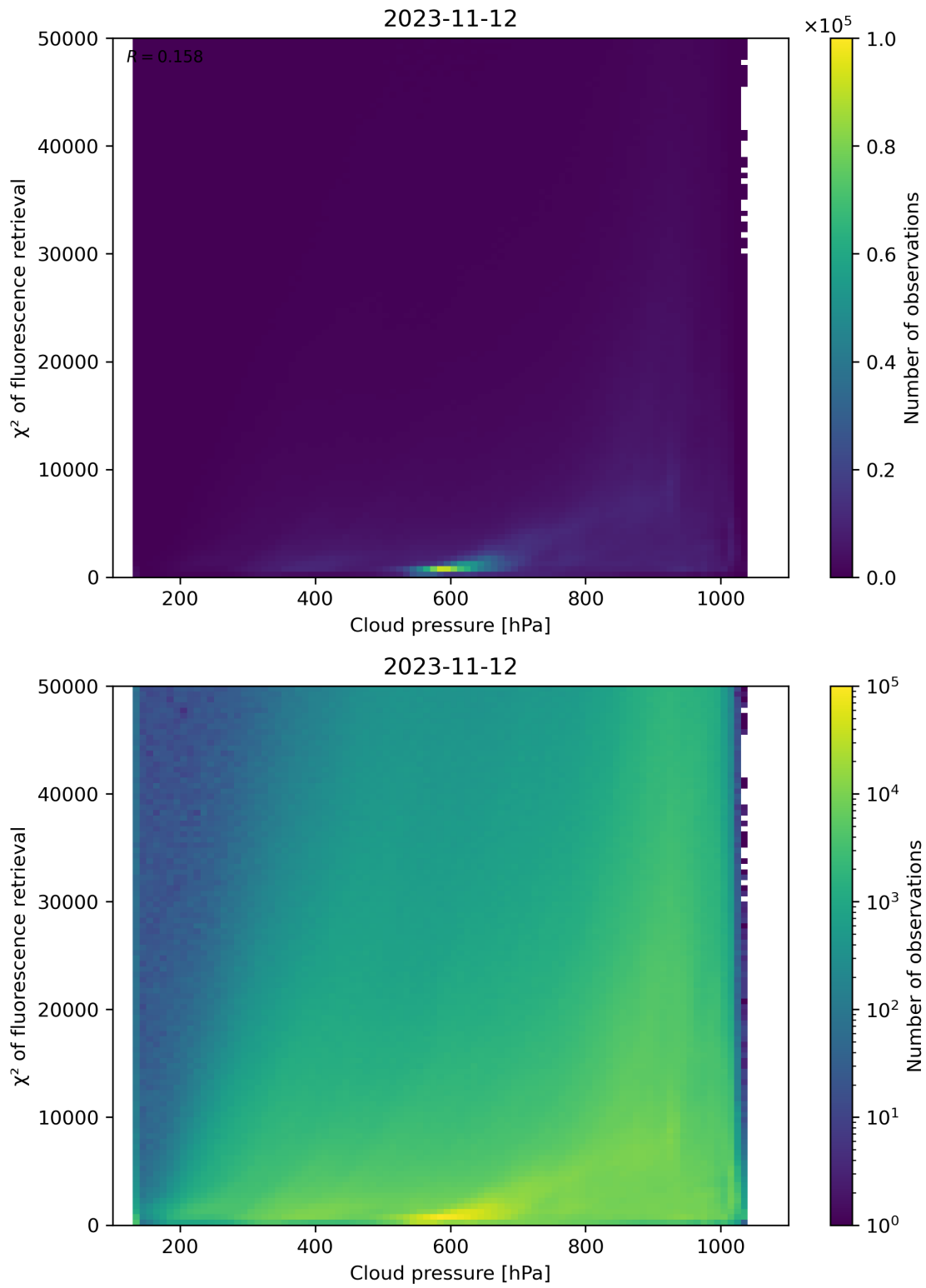
Figure 86: Scatter density plot of “Cloud pressure” against “ \chi^2 of fluorescence retrieval” for 2023-11-12 to 2023-11-13.
