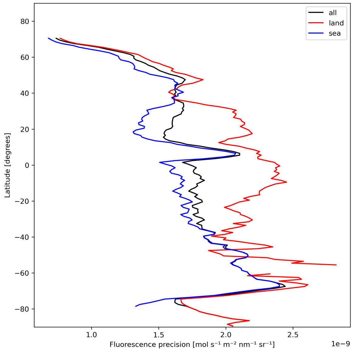
Figure 24: Zonal average of “Fluorescence precision” for 2023-11-12 to 2023-11-13.
