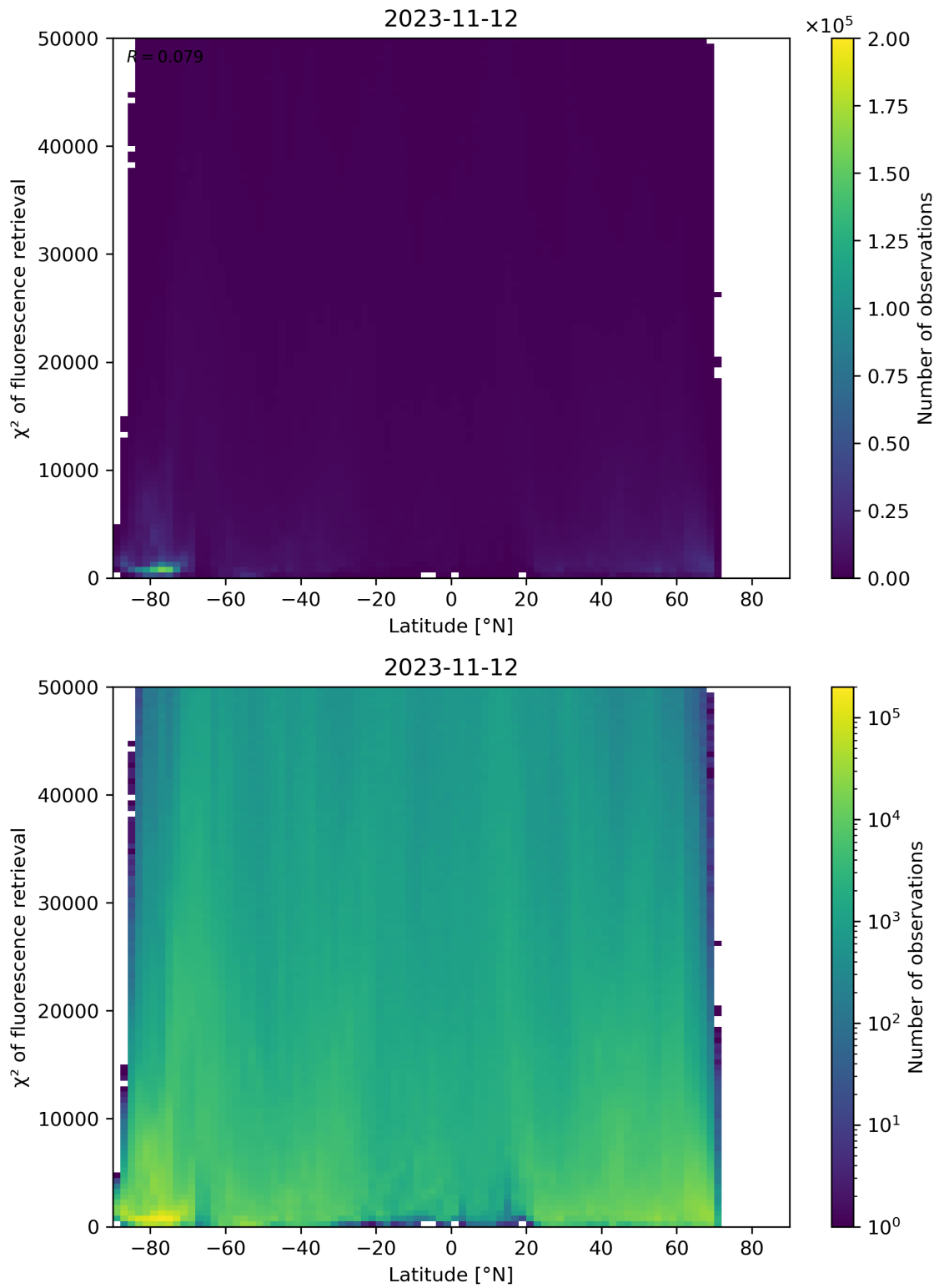
Figure 98: Scatter density plot of “Latitude” against “ \chi^2 of fluorescence retrieval” for 2023-11-12 to 2023-11-13.
