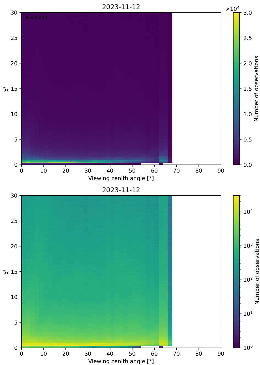
Figure 130: Scatter density plot of “Viewing zenith angle” against “ \chi^2 ” for 2023-11-12 to 2023-11-13.
