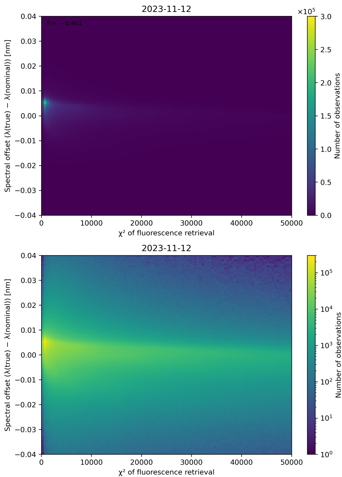
Figure 72: Scatter density plot of " \chi^2 of fluorescence retrieval" against "Spectral offset ( \lambda(\text{true}) - \lambda(\text{nominal}) )" for 2023-11-12 to 2023-11-13.
