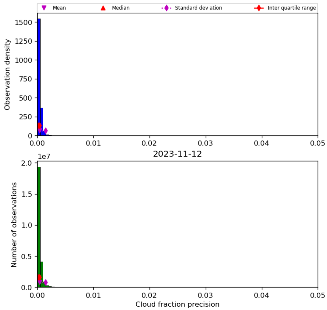
Figure 33: Histogram of “Cloud fraction precision” for 2023-11-12 to 2023-11-13
