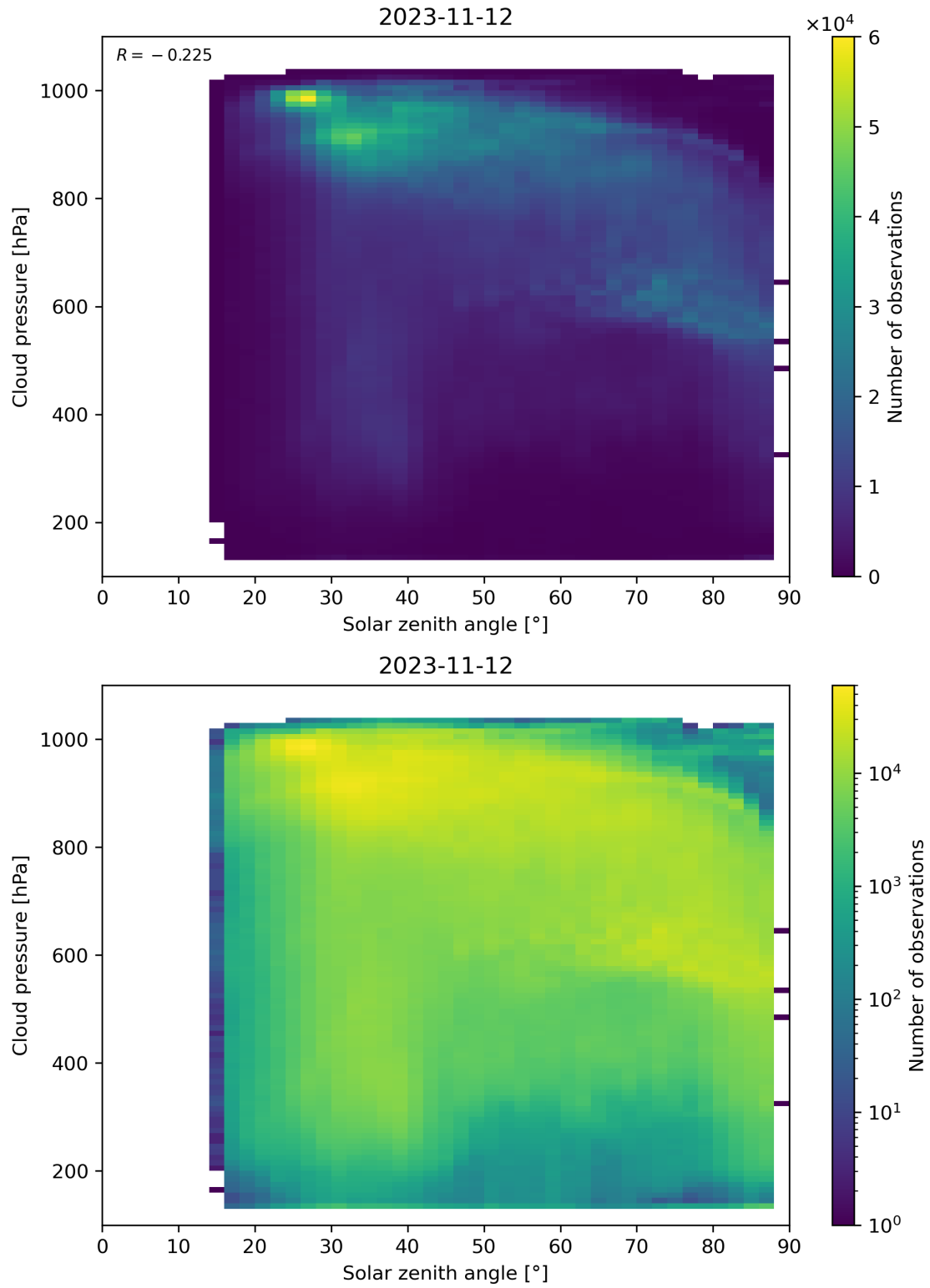
Figure 122: Scatter density plot of “Solar zenith angle” against “Cloud pressure” for 2023-11-12 to 2023-11-13.
