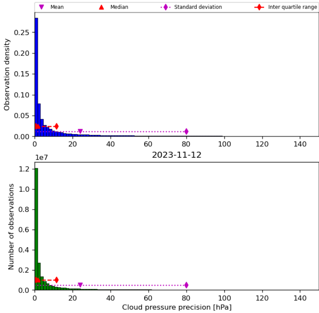
Figure 31: Histogram of “Cloud pressure precision” for 2023-11-12 to 2023-11-13
