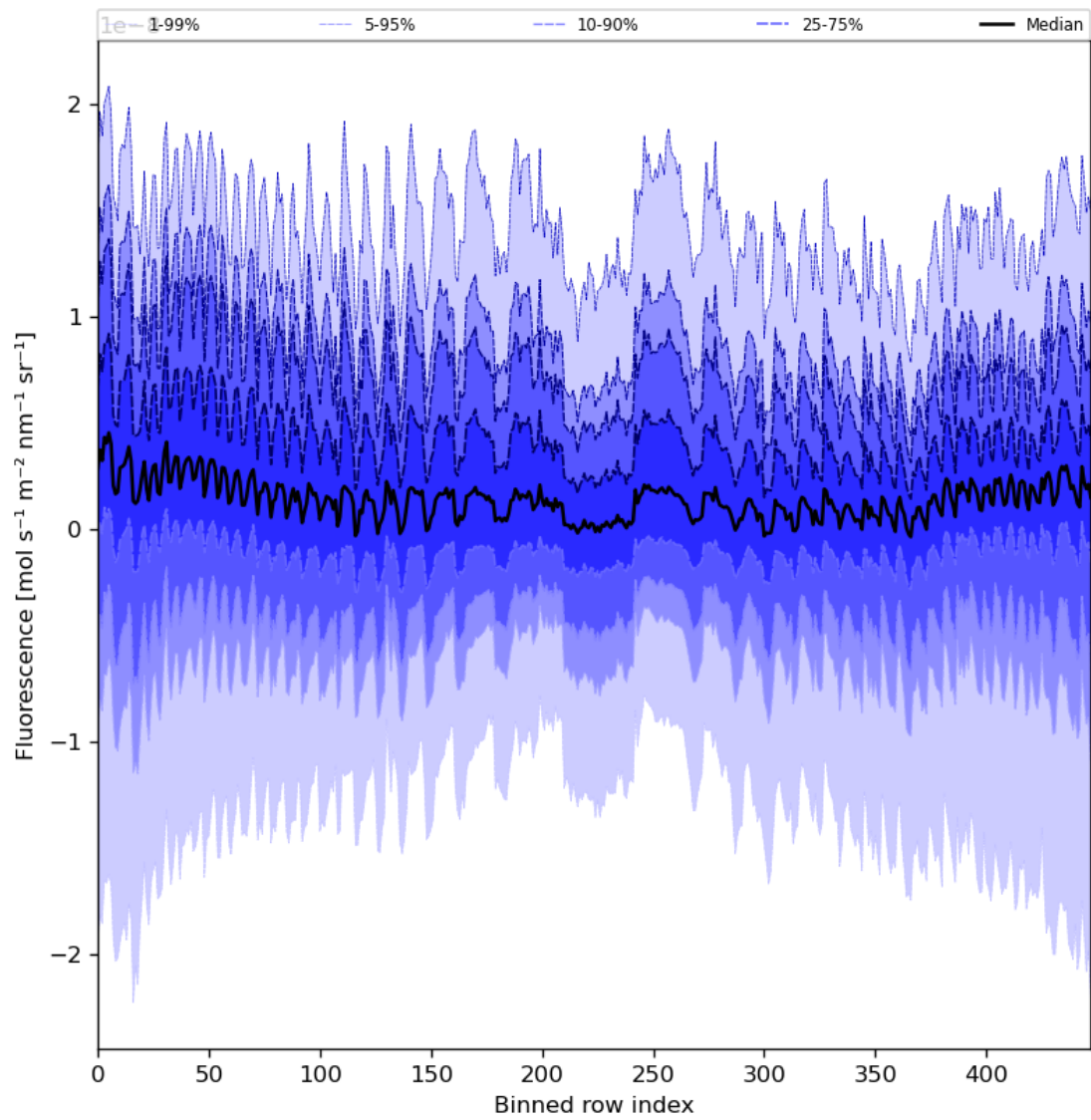
Figure 57: Along track statistics of “Fluorescence” for 2023-11-12 to 2023-11-13
