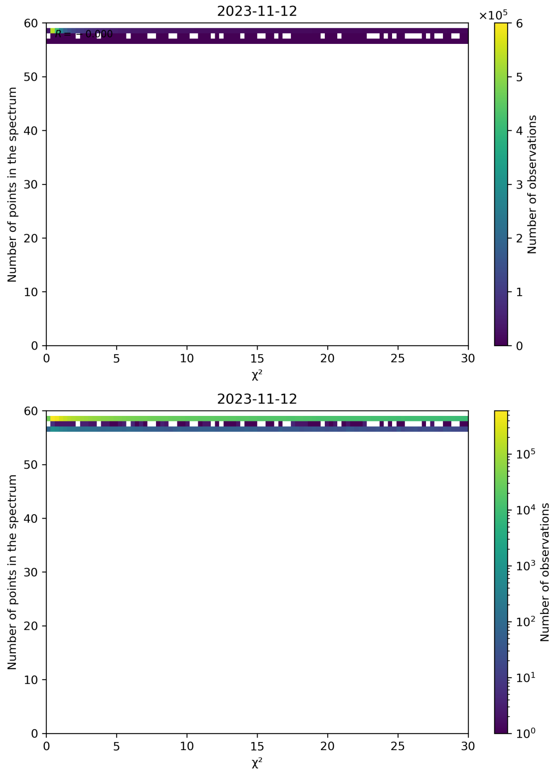
Figure 74: Scatter density plot of “ \chi^2 ” against “Number of points in the spectrum” for 2023-11-12 to 2023-11-13.
