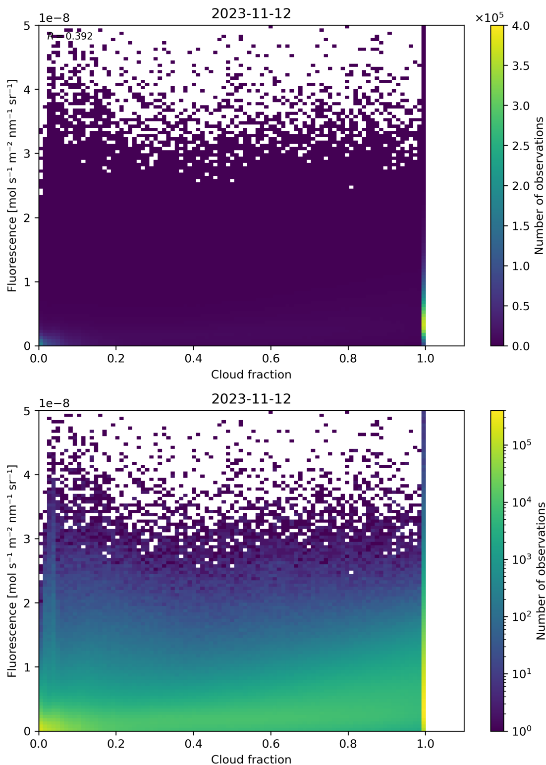
Figure 79: Scatter density plot of “Cloud fraction” against “Fluorescence” for 2023-11-12 to 2023-11-13.
