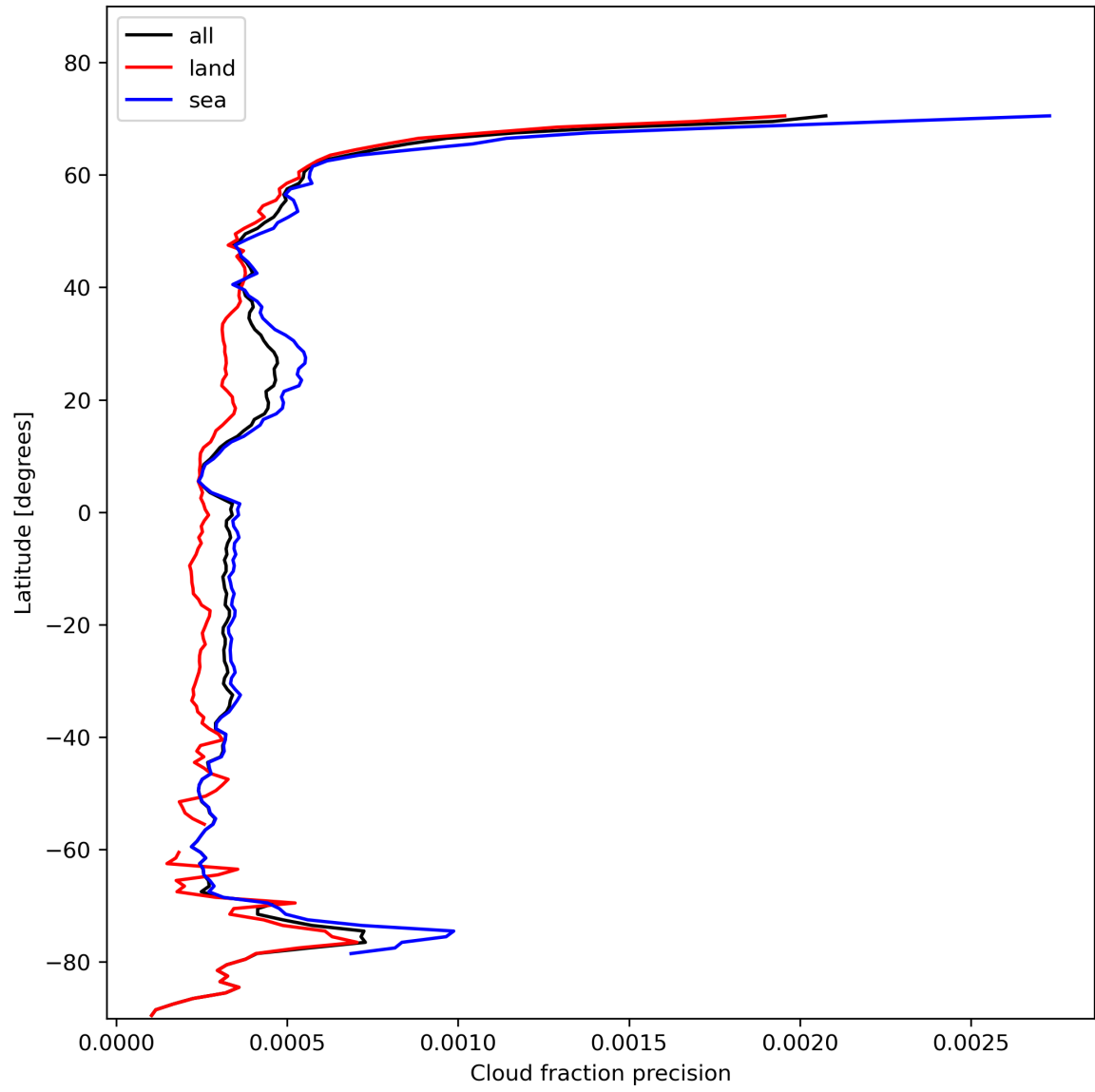
Figure 16: Zonal average of “Cloud fraction precision” for 2023-11-12 to 2023-11-13.
