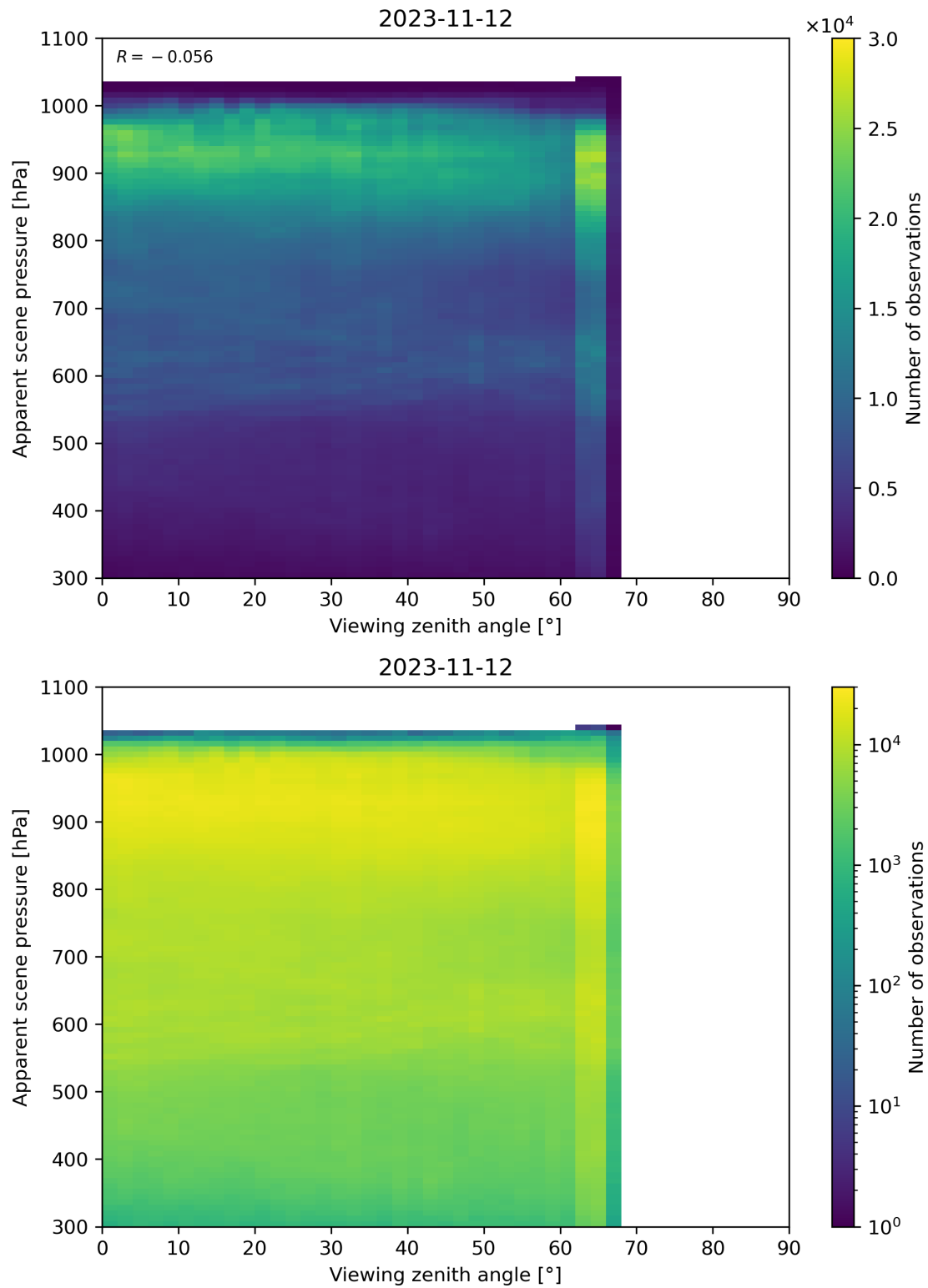
Figure 129: Scatter density plot of “Viewing zenith angle” against “Apparent scene pressure” for 2023-11-12 to 2023-11-13.
