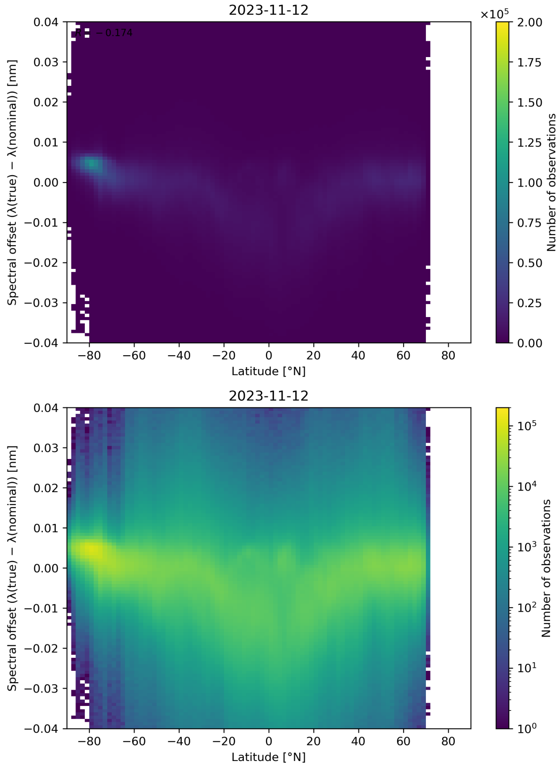
Figure 105: Scatter density plot of “Latitude” against “Spectral offset ( \lambda(\text{true}) - \lambda(\text{nominal}) )” for 2023-11-12 to 2023-11-13.
