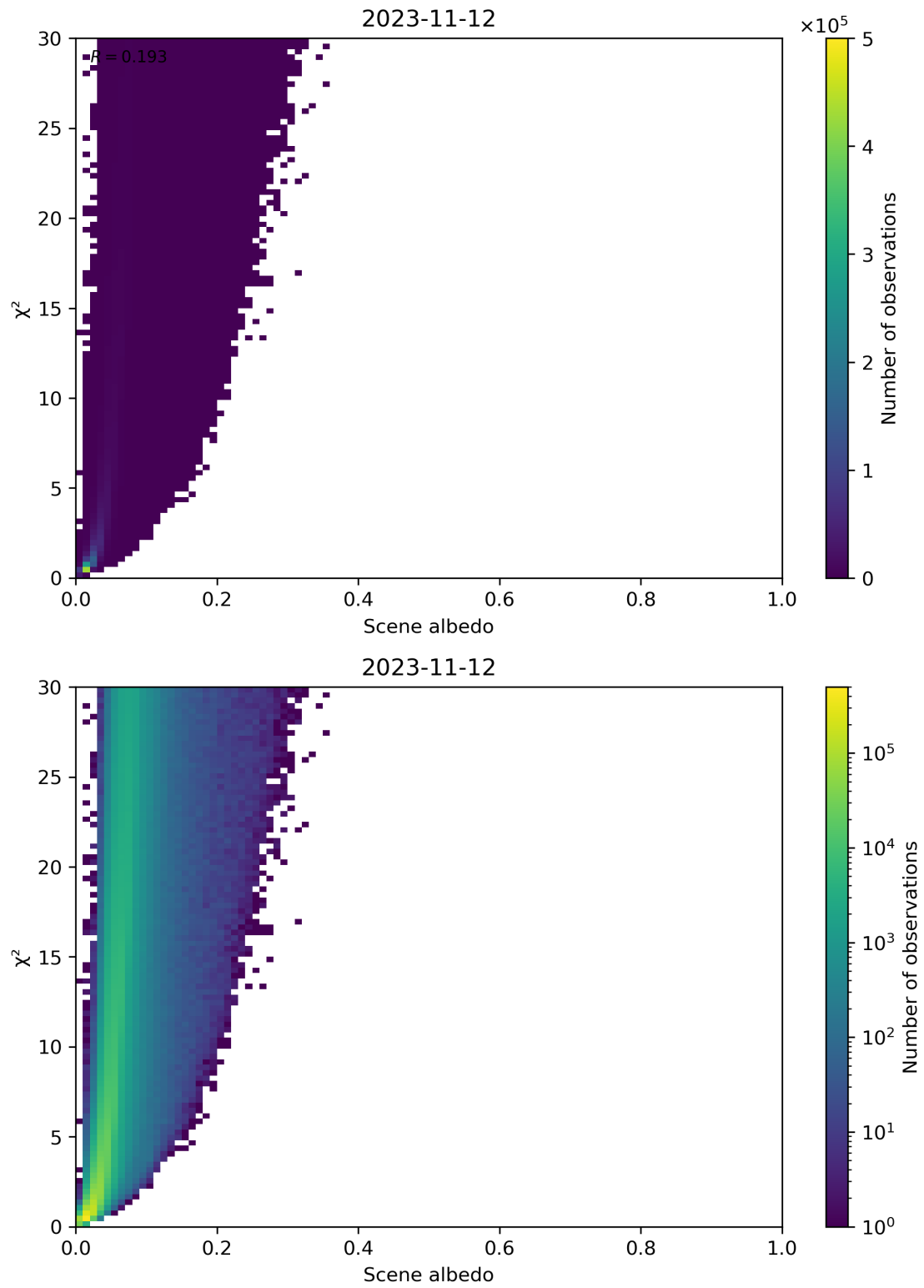
Figure 112: Scatter density plot of “Scene albedo” against “ \chi^2 ” for 2023-11-12 to 2023-11-13.
