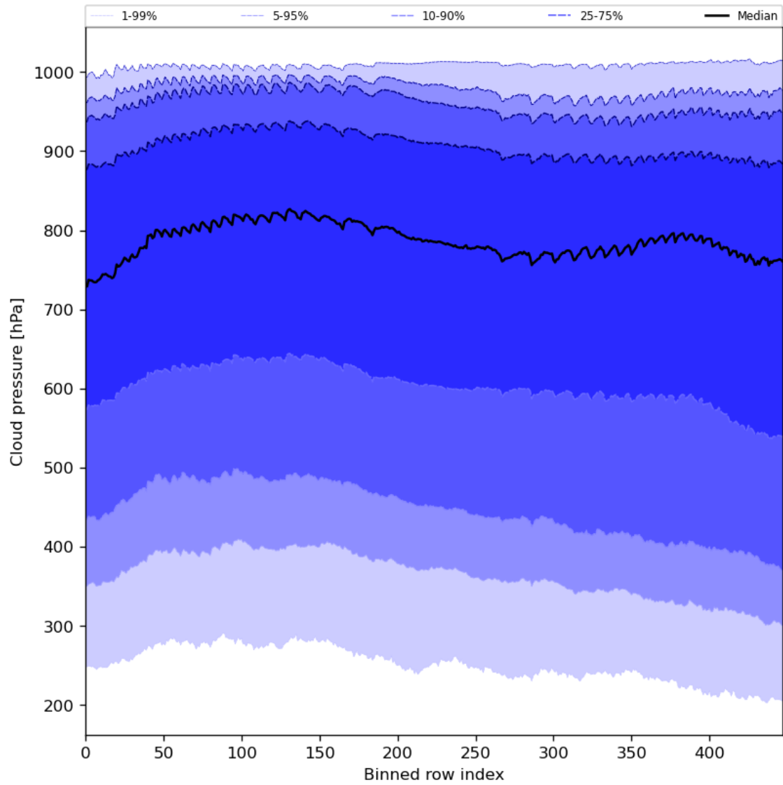
Figure 47: Along track statistics of "Cloud pressure" for 2023-11-12 to 2023-11-13
