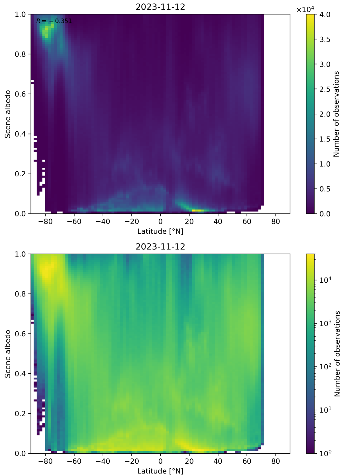
Figure 104: Scatter density plot of “Latitude” against “Scene albedo” for 2023-11-12 to 2023-11-13.
