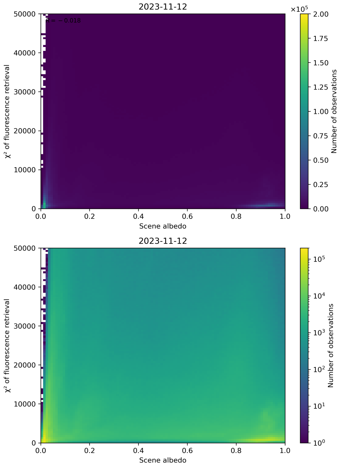
Figure 113: Scatter density plot of “Scene albedo” against “ \chi^2 of fluorescence retrieval” for 2023-11-12 to 2023-11-13.
