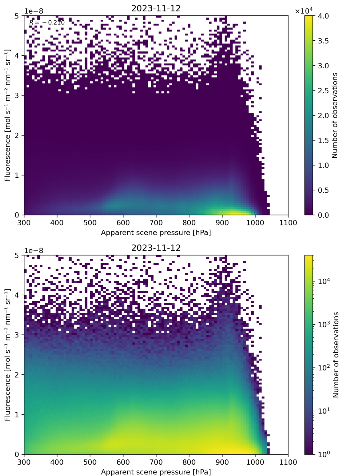
Figure 65: Scatter density plot of “Apparent scene pressure” against “Fluorescence” for 2023-11-12 to 2023-11-13.
