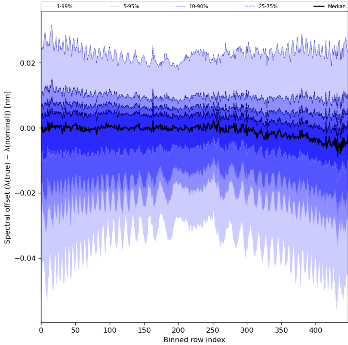
Figure 62: Along track statistics of “Spectral offset ( \lambda(\text{true}) - \lambda(\text{nominal}) )” for 2023-11-12 to 2023-11-13
