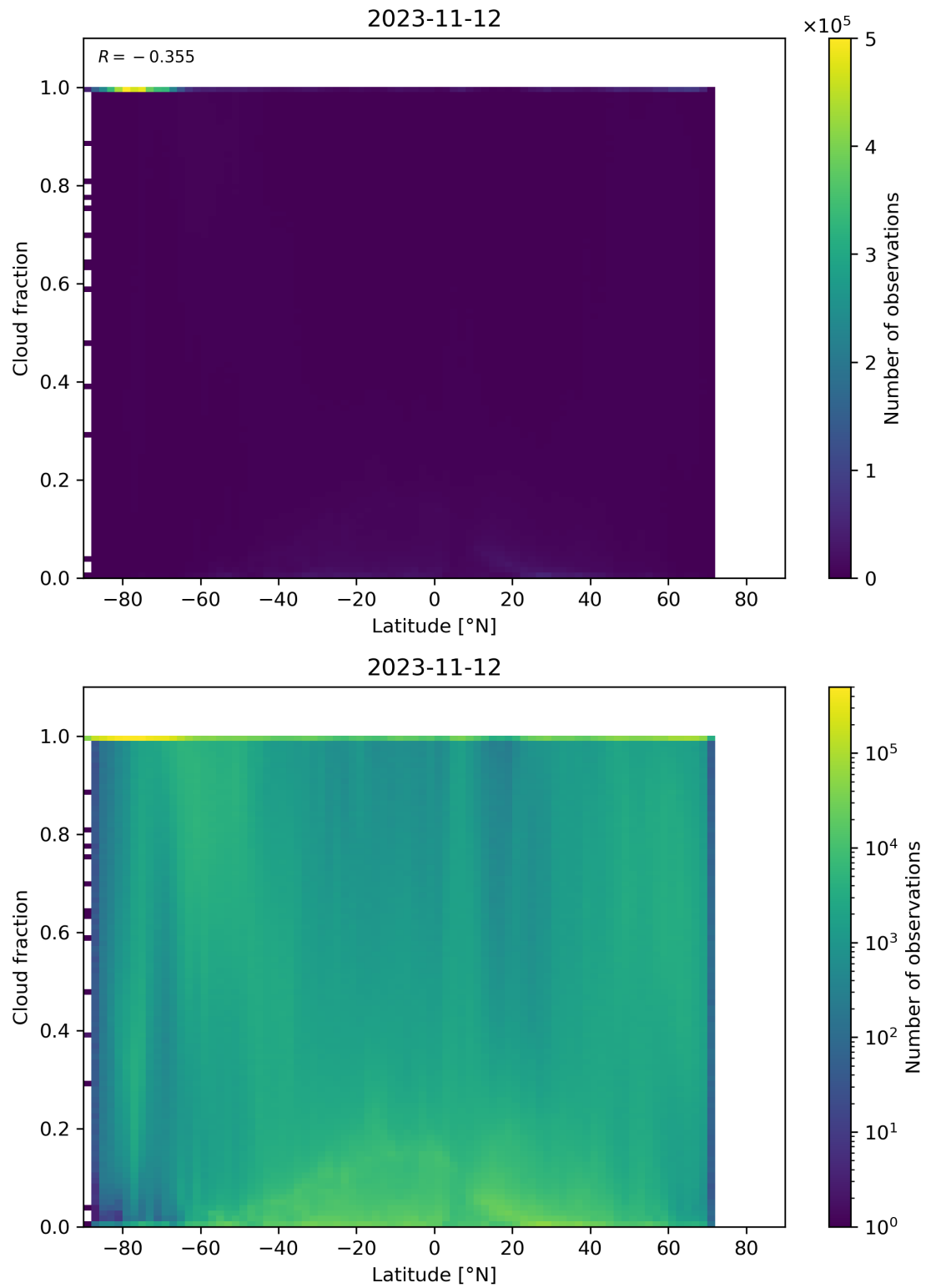
Figure 99: Scatter density plot of “Latitude” against “Cloud fraction” for 2023-11-12 to 2023-11-13.
