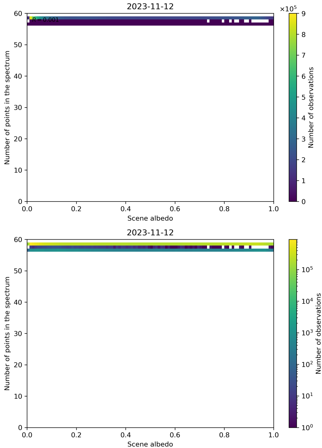
Figure 116: Scatter density plot of “Scene albedo” against “Number of points in the spectrum” for 2023-11-12 to 2023-11-13.
