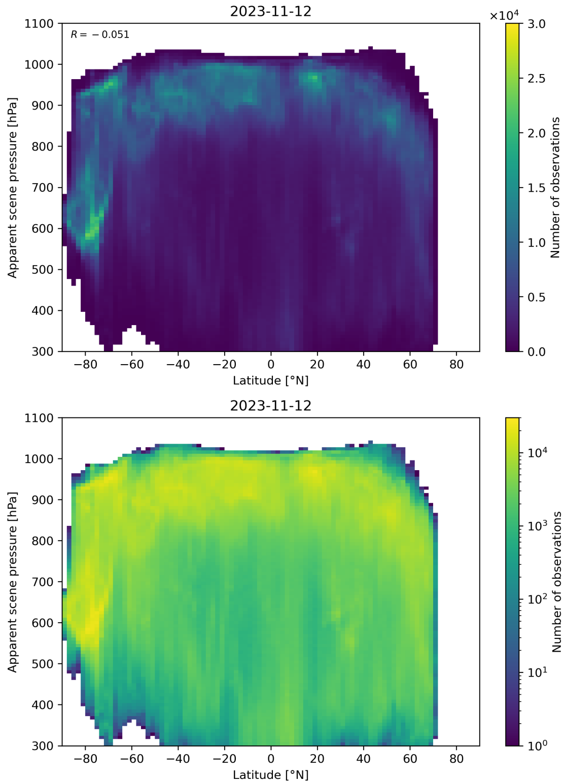
Figure 96: Scatter density plot of “Latitude” against “Apparent scene pressure” for 2023-11-12 to 2023-11-13.
