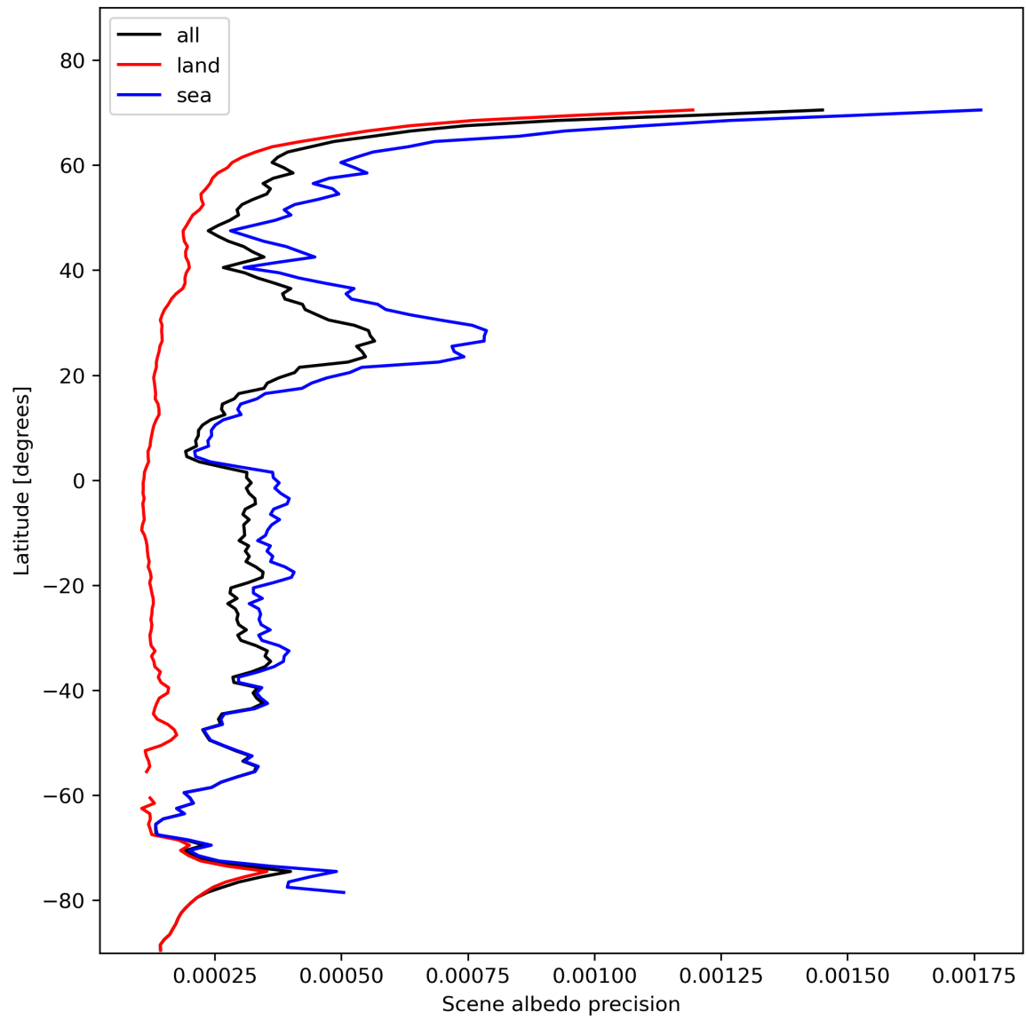
Figure 18: Zonal average of “Scene albedo precision” for 2023-11-12 to 2023-11-13.
