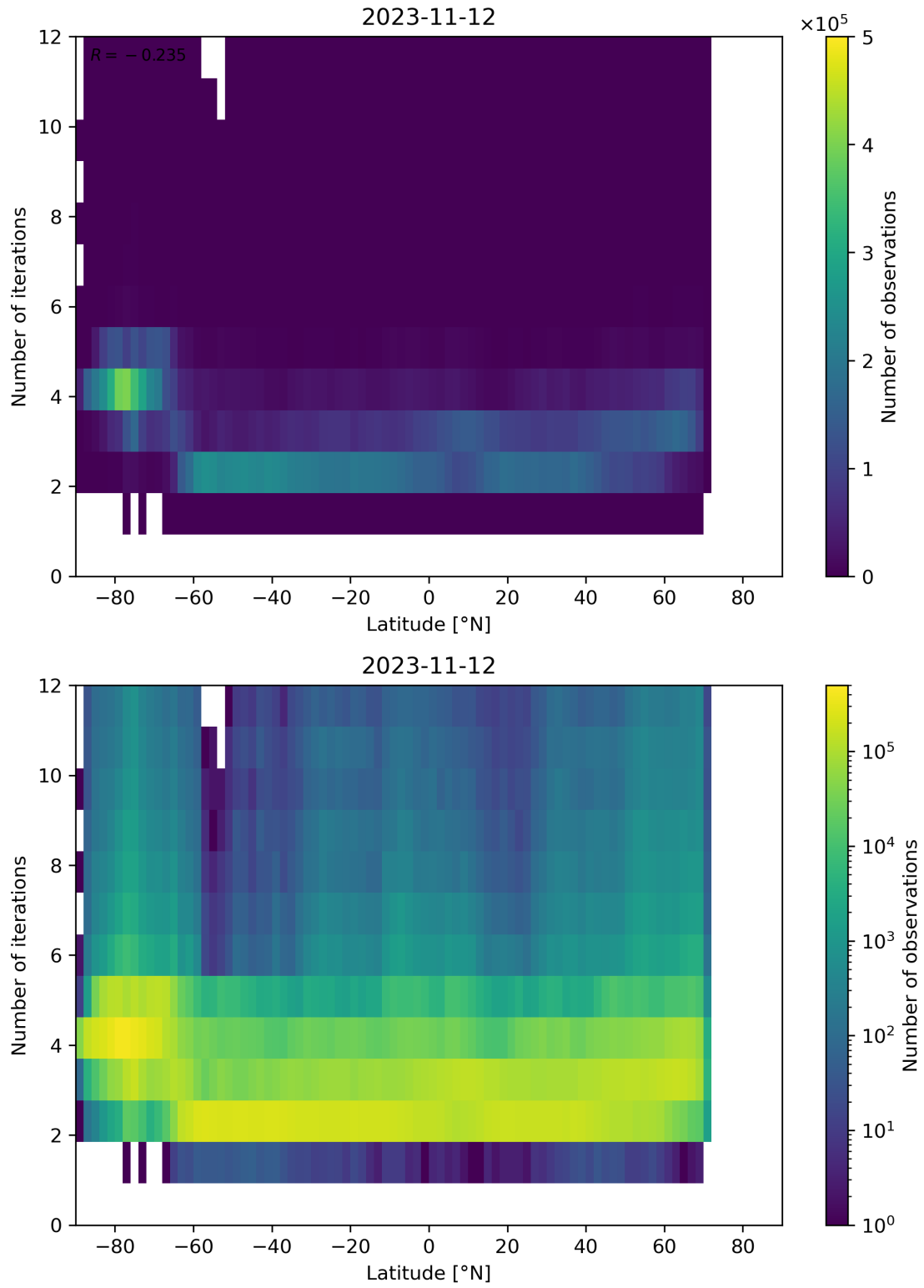
Figure 102: Scatter density plot of “Latitude” against “Number of iterations” for 2023-11-12 to 2023-11-13.
