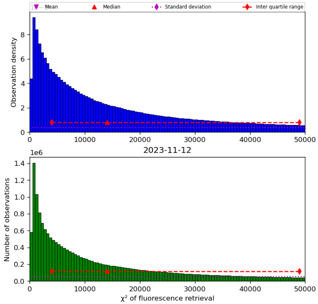
Figure 42: Histogram of “ \chi^2 of fluorescence retrieval” for 2023-11-12 to 2023-11-13
