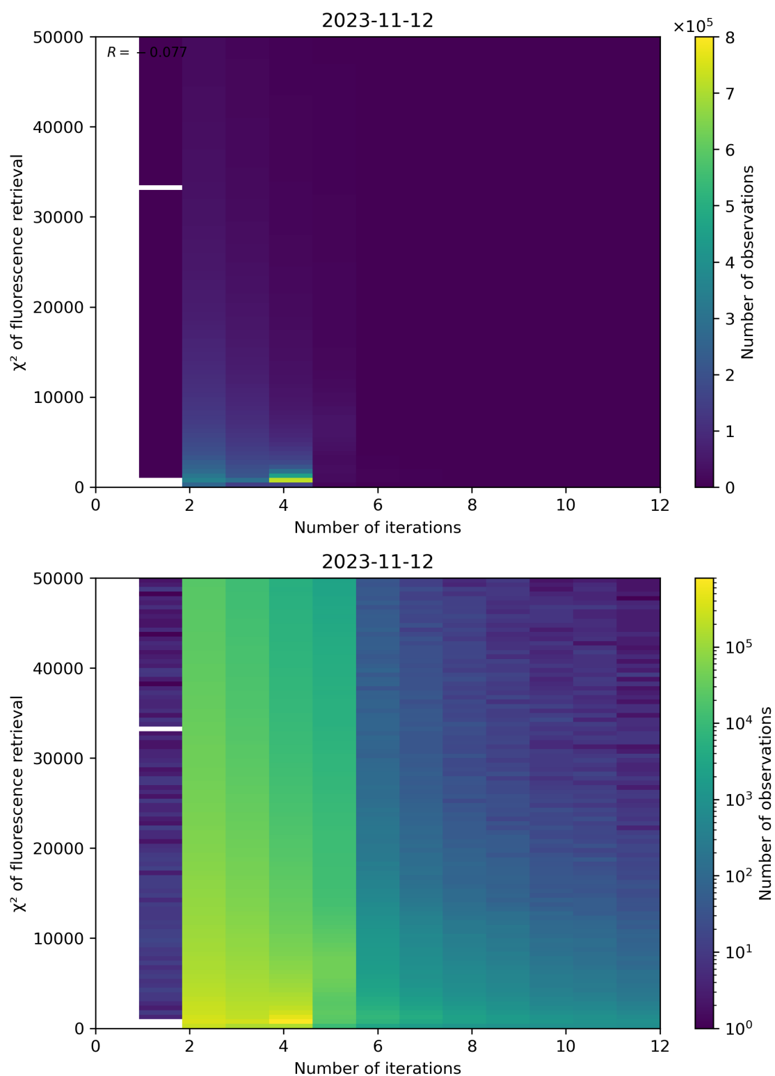
Figure 106: Scatter density plot of “Number of iterations” against “ \chi^2 of fluorescence retrieval” for 2023-11-12 to 2023-11-13.
