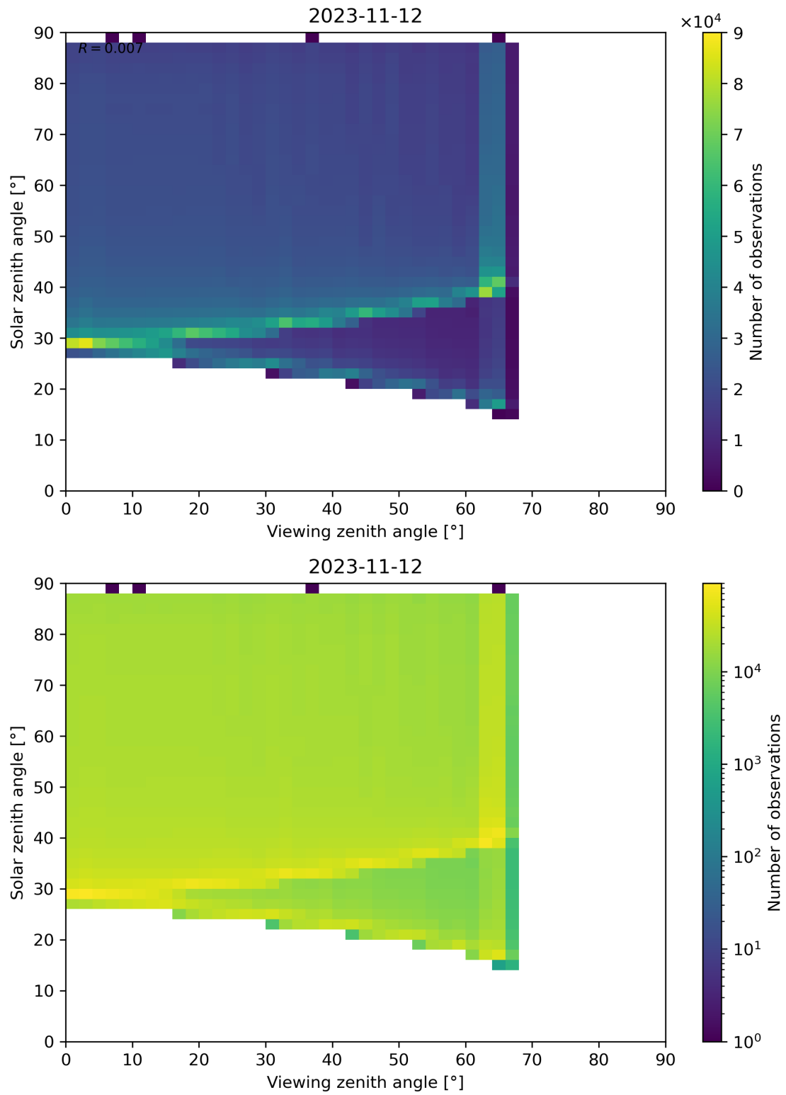
Figure 139: Scatter density plot of “Viewing zenith angle” against “Solar zenith angle” for 2023-11-12 to 2023-11-13.
