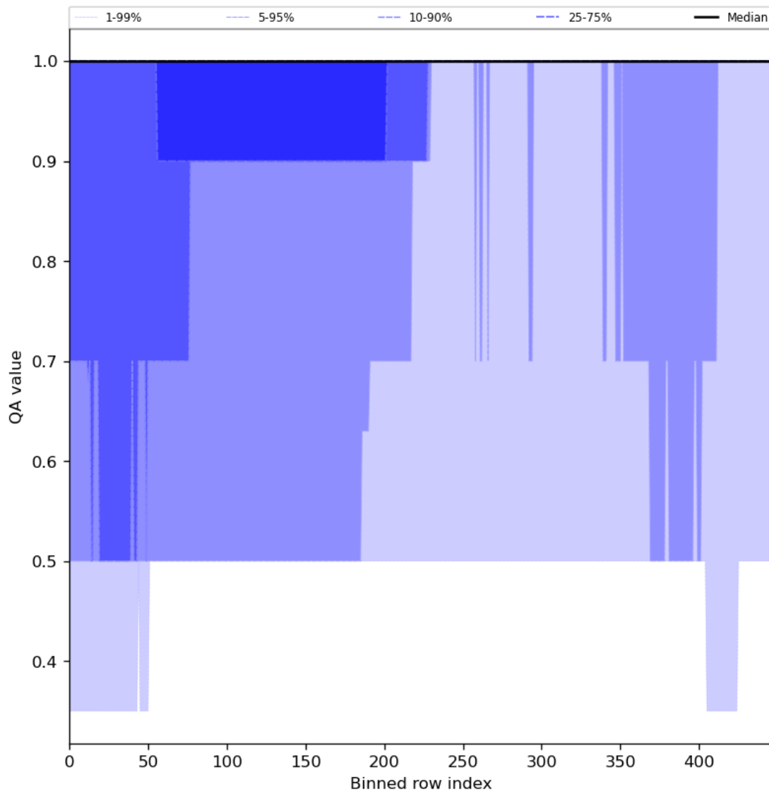
Figure 46: Along track statistics of “QA value” for 2023-11-12 to 2023-11-13
