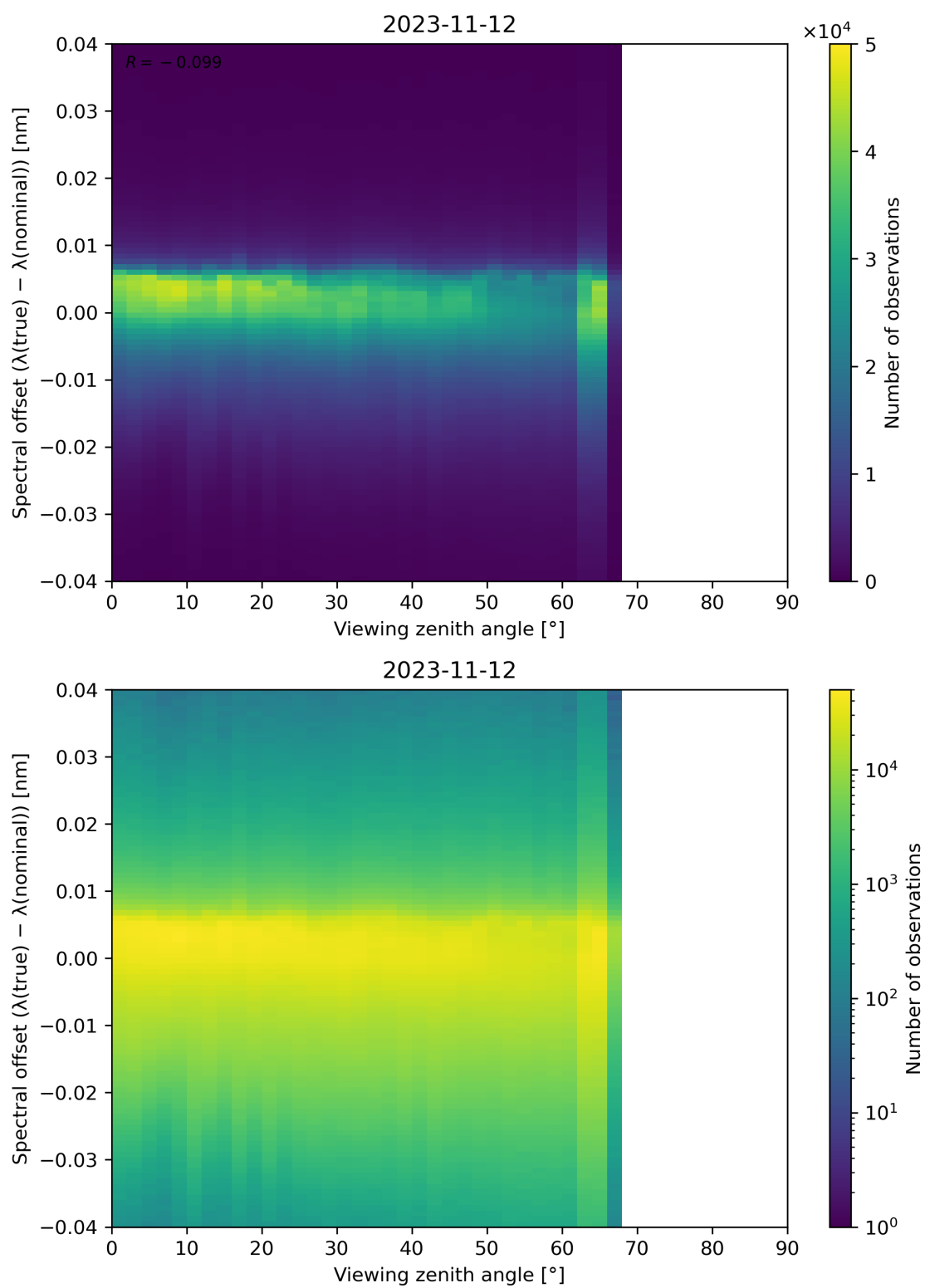
Figure 140: Scatter density plot of “Viewing zenith angle” against “Spectral offset ( \lambda(\text{true}) - \lambda(\text{nominal}) )” for 2023-11-12 to 2023-11-13.
