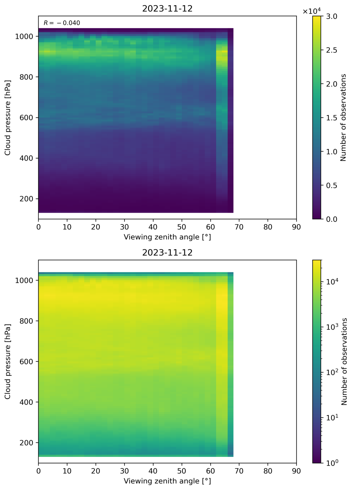
Figure 133: Scatter density plot of “Viewing zenith angle” against “Cloud pressure” for 2023-11-12 to 2023-11-13.
