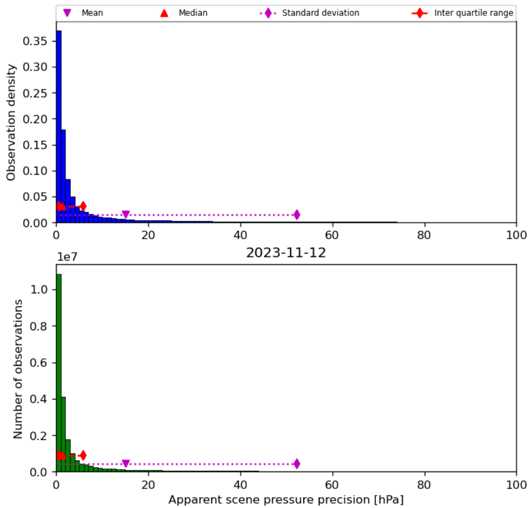
Figure 37: Histogram of “Apparent scene pressure precision” for 2023-11-12 to 2023-11-13
