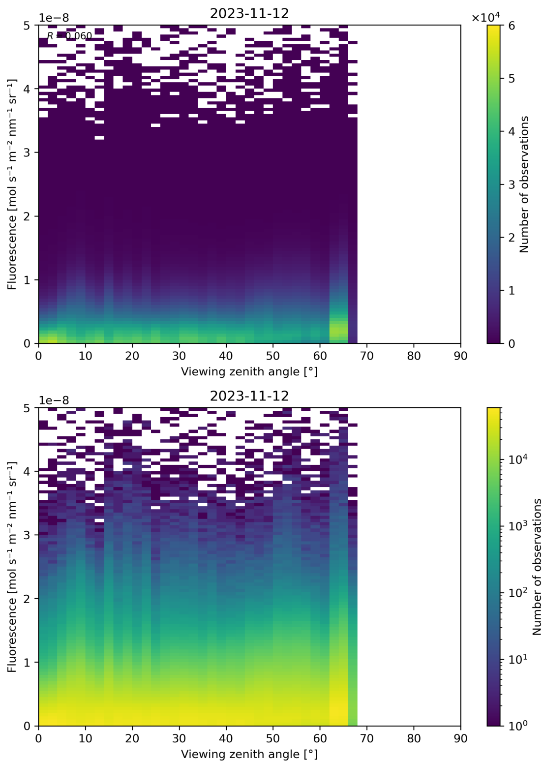
Figure 134: Scatter density plot of “Viewing zenith angle” against “Fluorescence” for 2023-11-12 to 2023-11-13.
