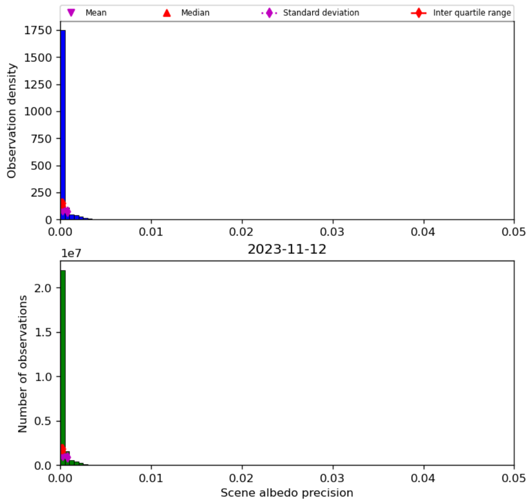
Figure 35: Histogram of “Scene albedo precision” for 2023-11-12 to 2023-11-13
