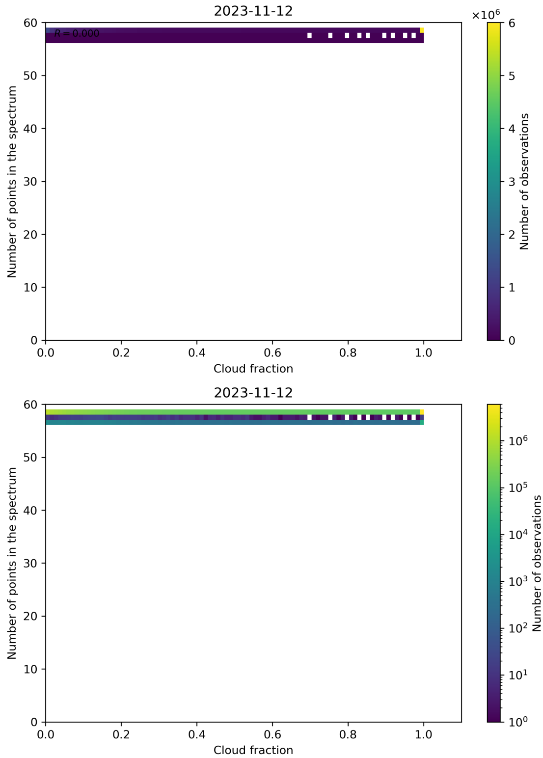
Figure 81: Scatter density plot of “Cloud fraction” against “Number of points in the spectrum” for 2023-11-12 to 2023-11-13.
