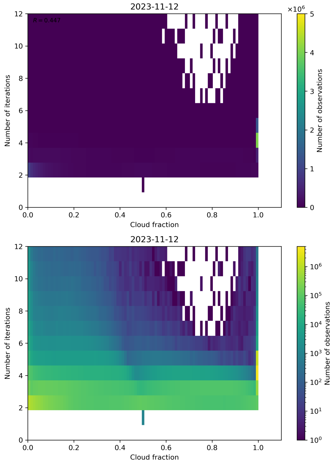
Figure 80: Scatter density plot of “Cloud fraction” against “Number of iterations” for 2023-11-12 to 2023-11-13.
