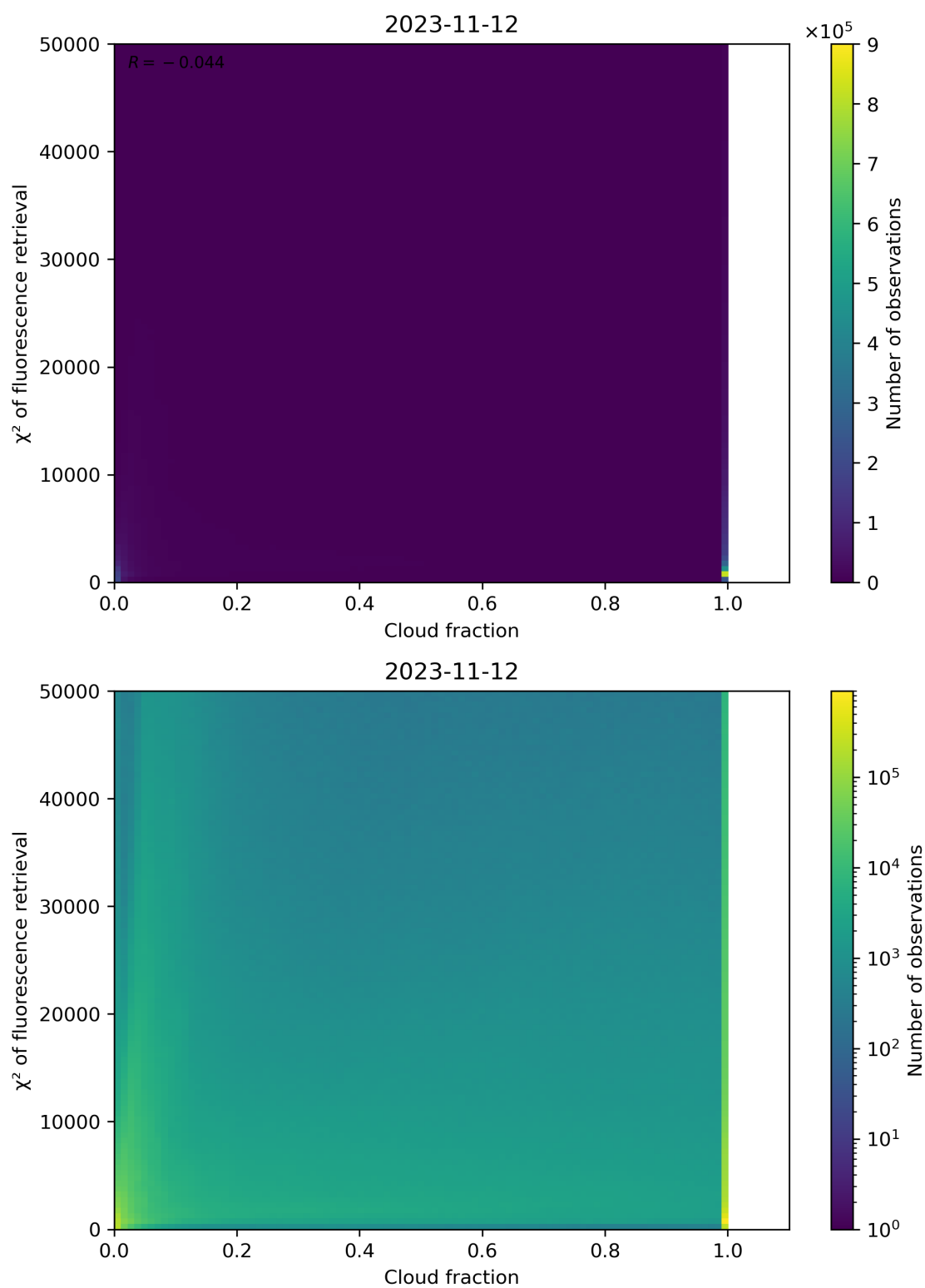
Figure 78: Scatter density plot of “Cloud fraction” against “ \chi^2 of fluorescence retrieval” for 2023-11-12 to 2023-11-13.
