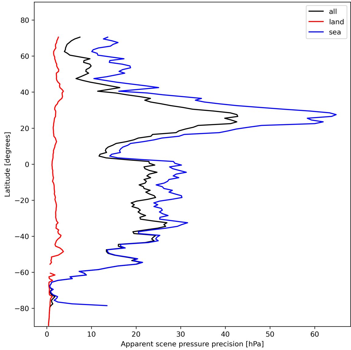
Figure 20: Zonal average of “Apparent scene pressure precision” for 2023-11-12 to 2023-11-13.
