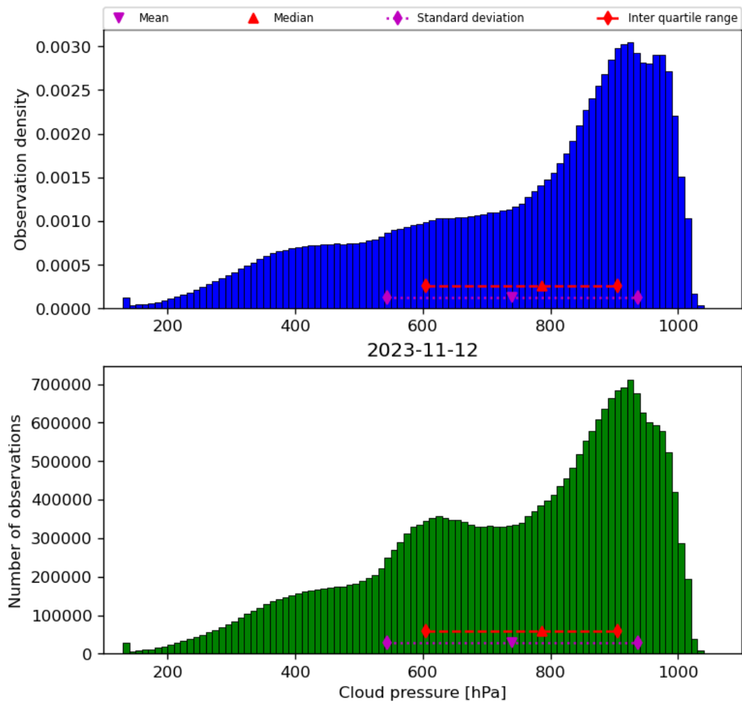
Figure 30: Histogram of “Cloud pressure” for 2023-11-12 to 2023-11-13
