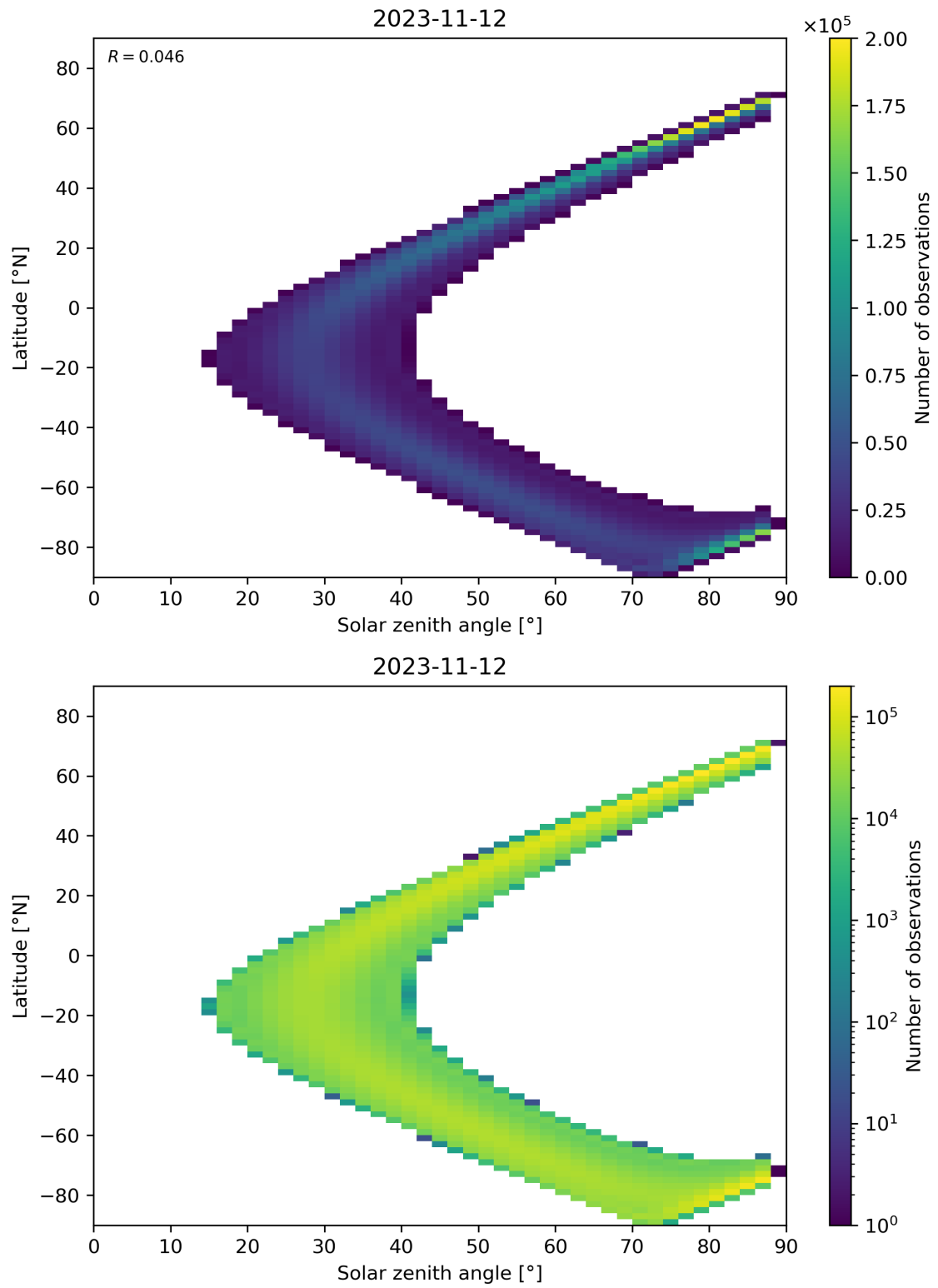
Figure 124: Scatter density plot of “Solar zenith angle” against “Latitude” for 2023-11-12 to 2023-11-13.
