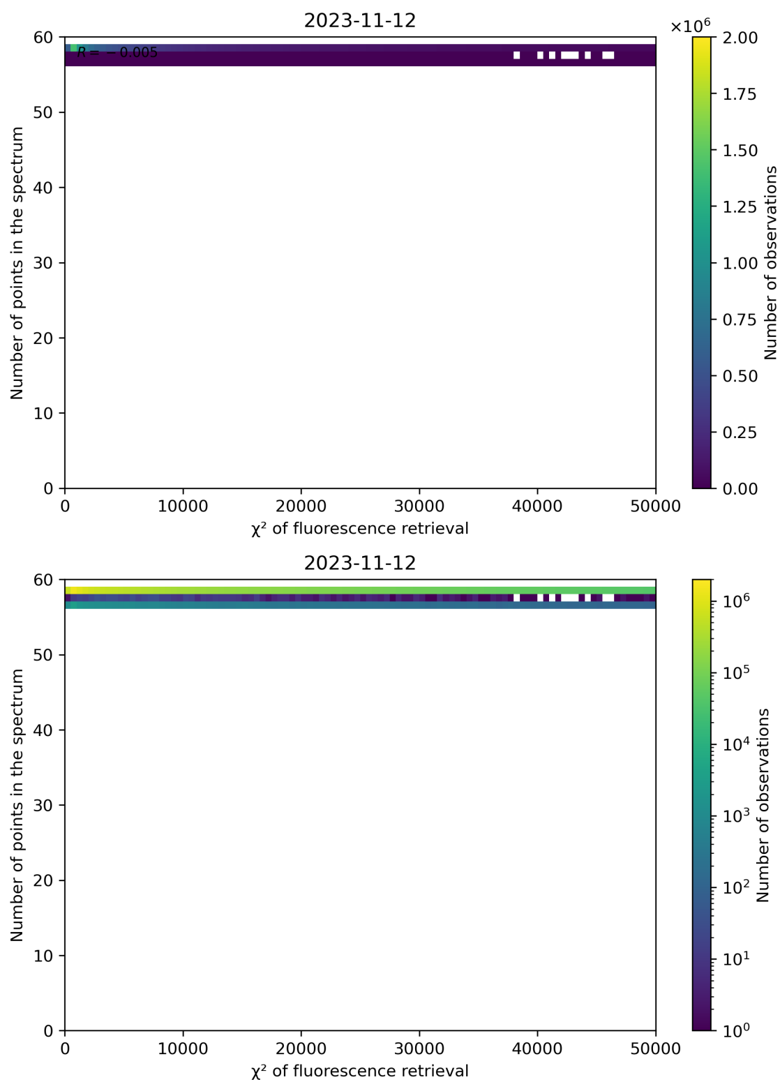
Figure 71: Scatter density plot of " \chi^2 of fluorescence retrieval" against "Number of points in the spectrum" for 2023-11-12 to 2023-11-13.
