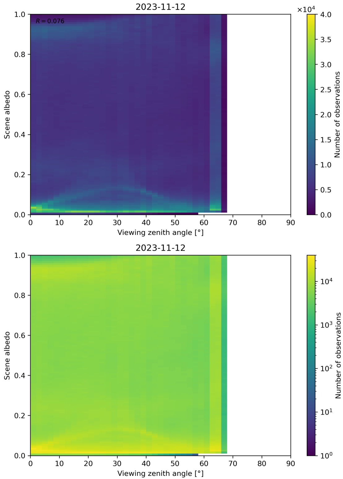
Figure 138: Scatter density plot of “Viewing zenith angle” against “Scene albedo” for 2023-11-12 to 2023-11-13.
