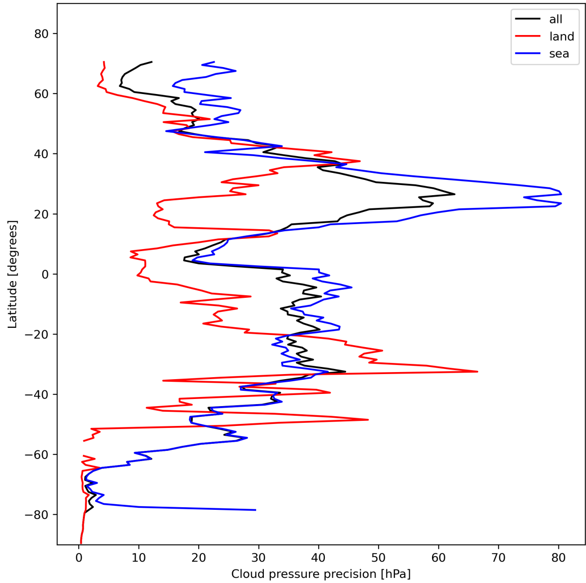
Figure 14: Zonal average of “Cloud pressure precision” for 2023-11-12 to 2023-11-13.
