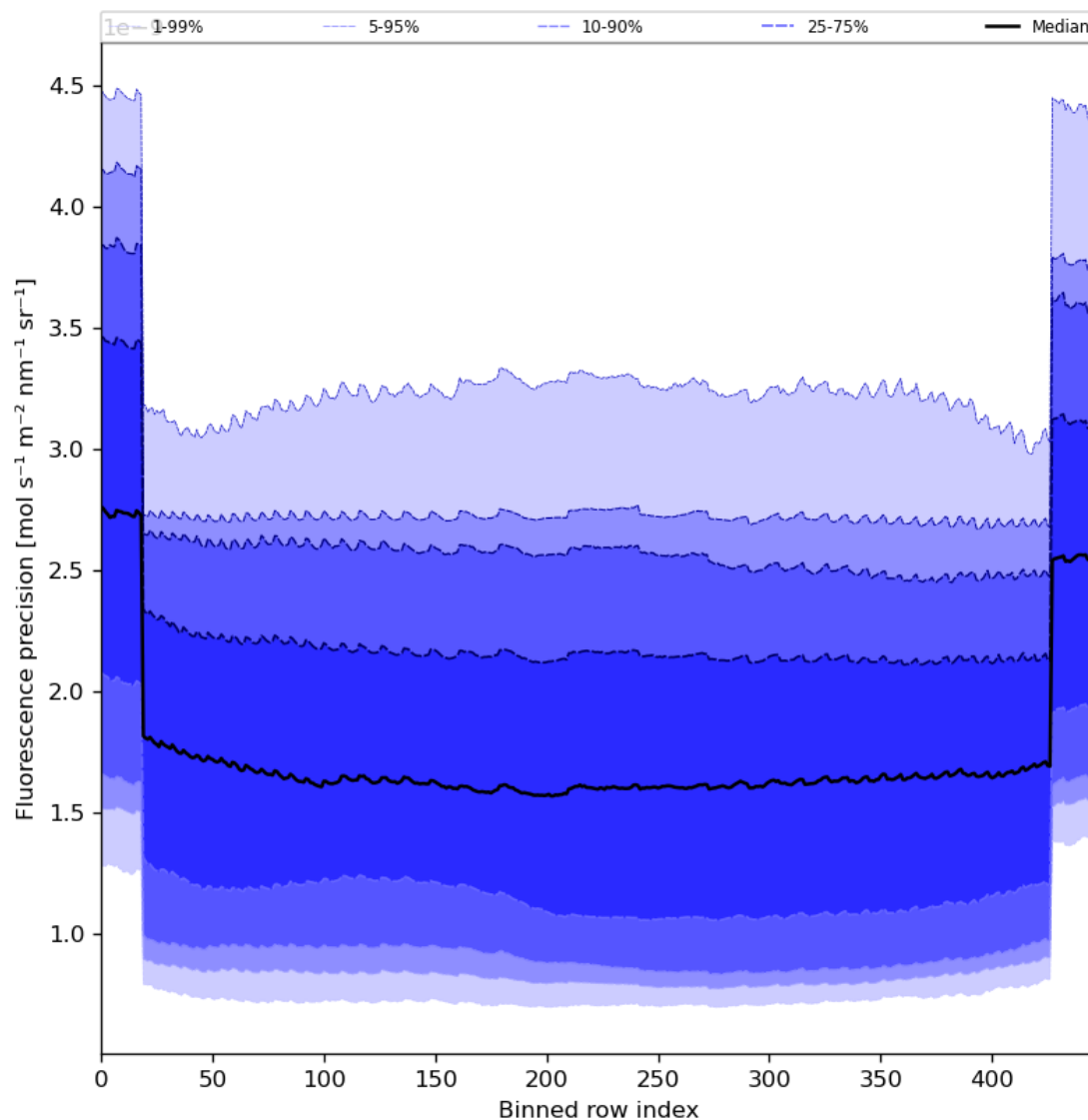
Figure 58: Along track statistics of “Fluorescence precision” for 2023-11-12 to 2023-11-13
