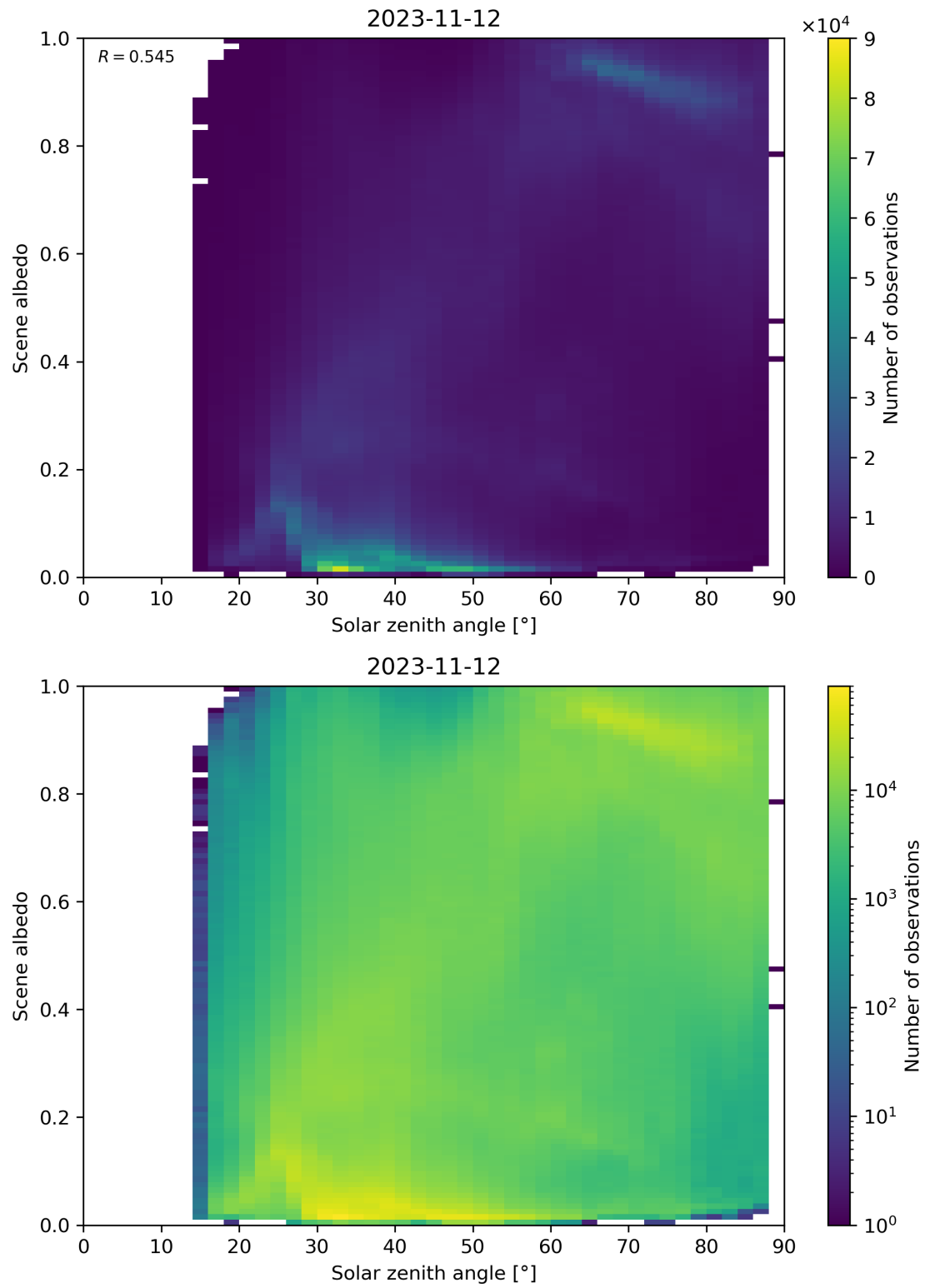
Figure 127: Scatter density plot of “Solar zenith angle” against “Scene albedo” for 2023-11-12 to 2023-11-13.
