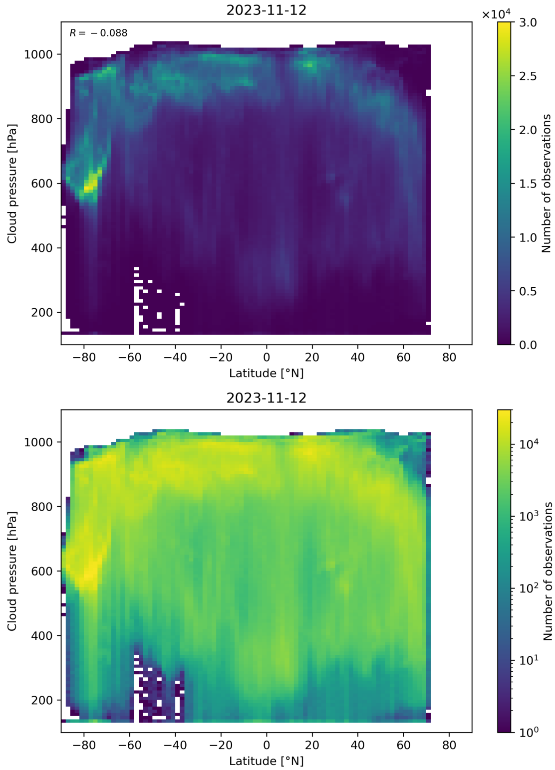
Figure 100: Scatter density plot of “Latitude” against “Cloud pressure” for 2023-11-12 to 2023-11-13.
