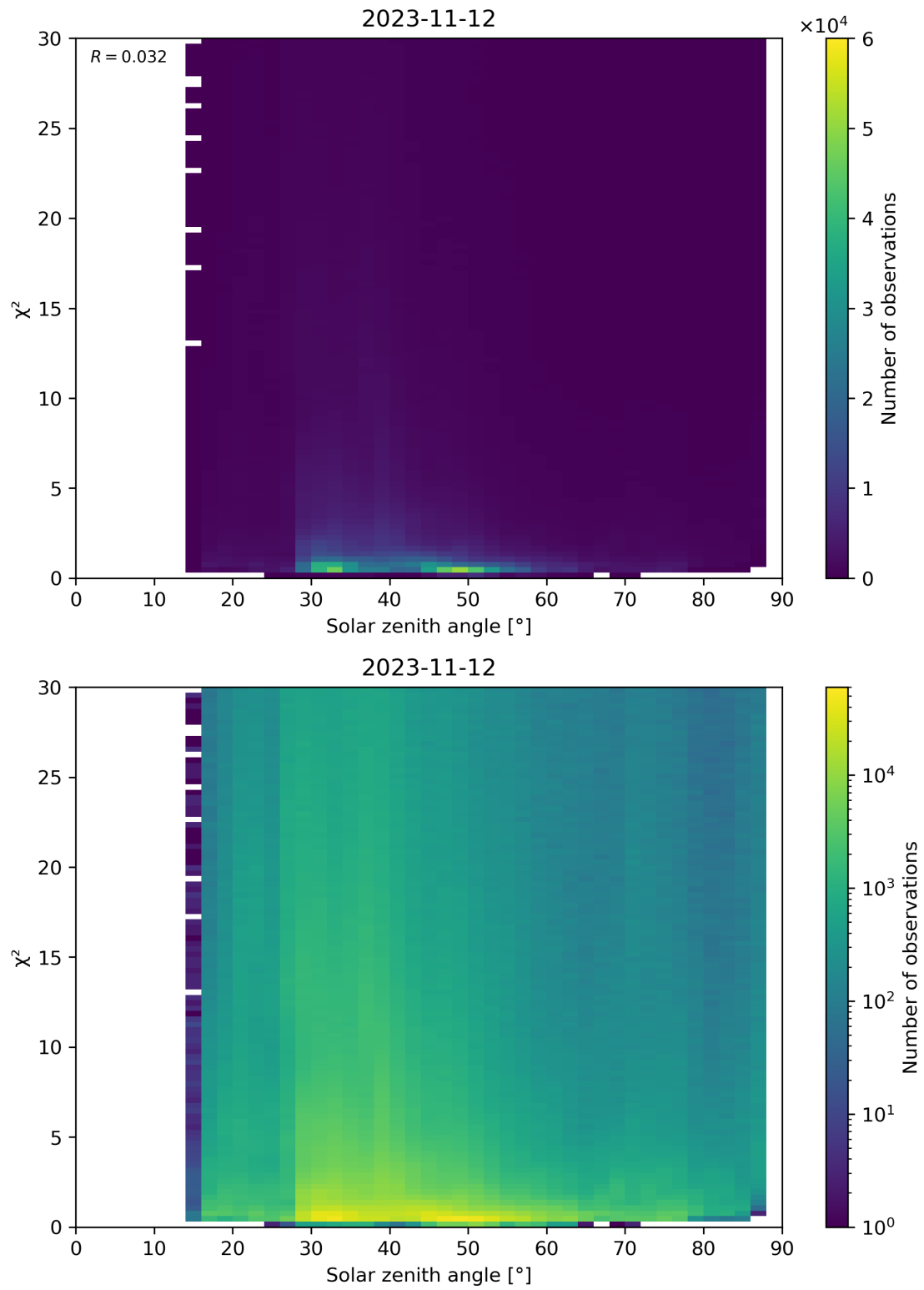
Figure 119: Scatter density plot of “Solar zenith angle” against “ \chi^2 ” for 2023-11-12 to 2023-11-13.
