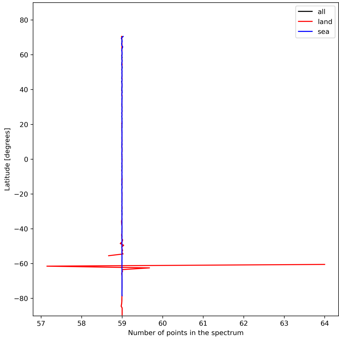
Figure 27: Zonal average of “Number of points in the spectrum” for 2023-11-12 to 2023-11-13.
