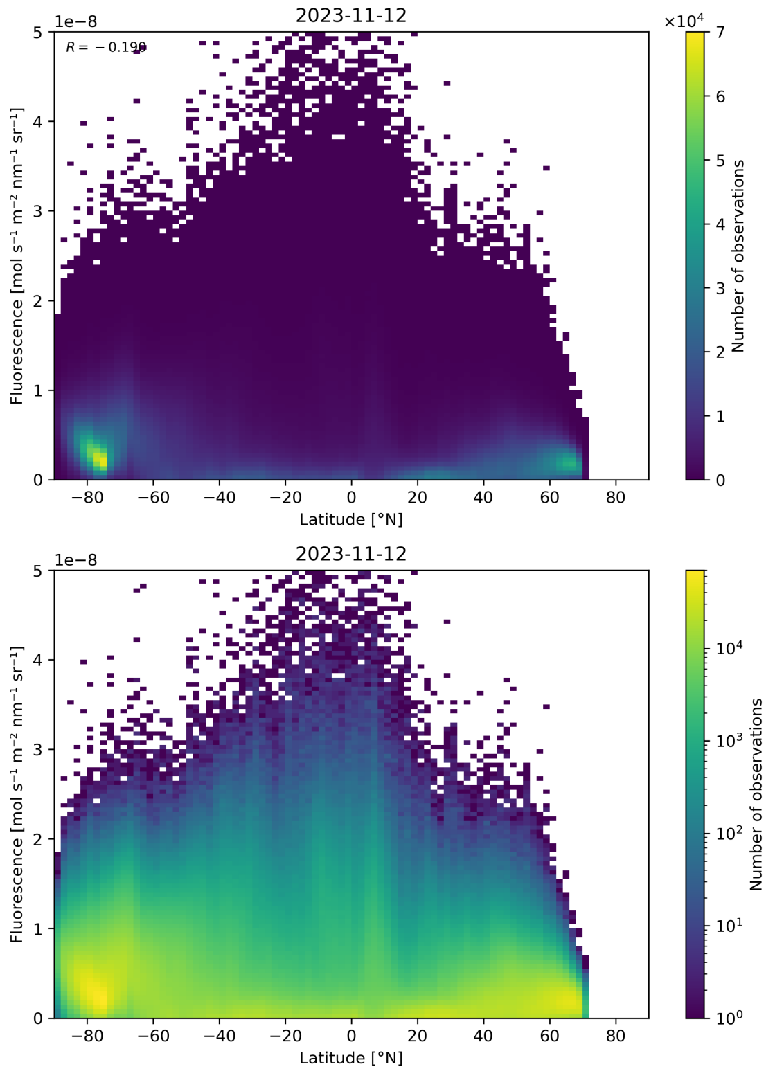
Figure 101: Scatter density plot of “Latitude” against “Fluorescence” for 2023-11-12 to 2023-11-13.
