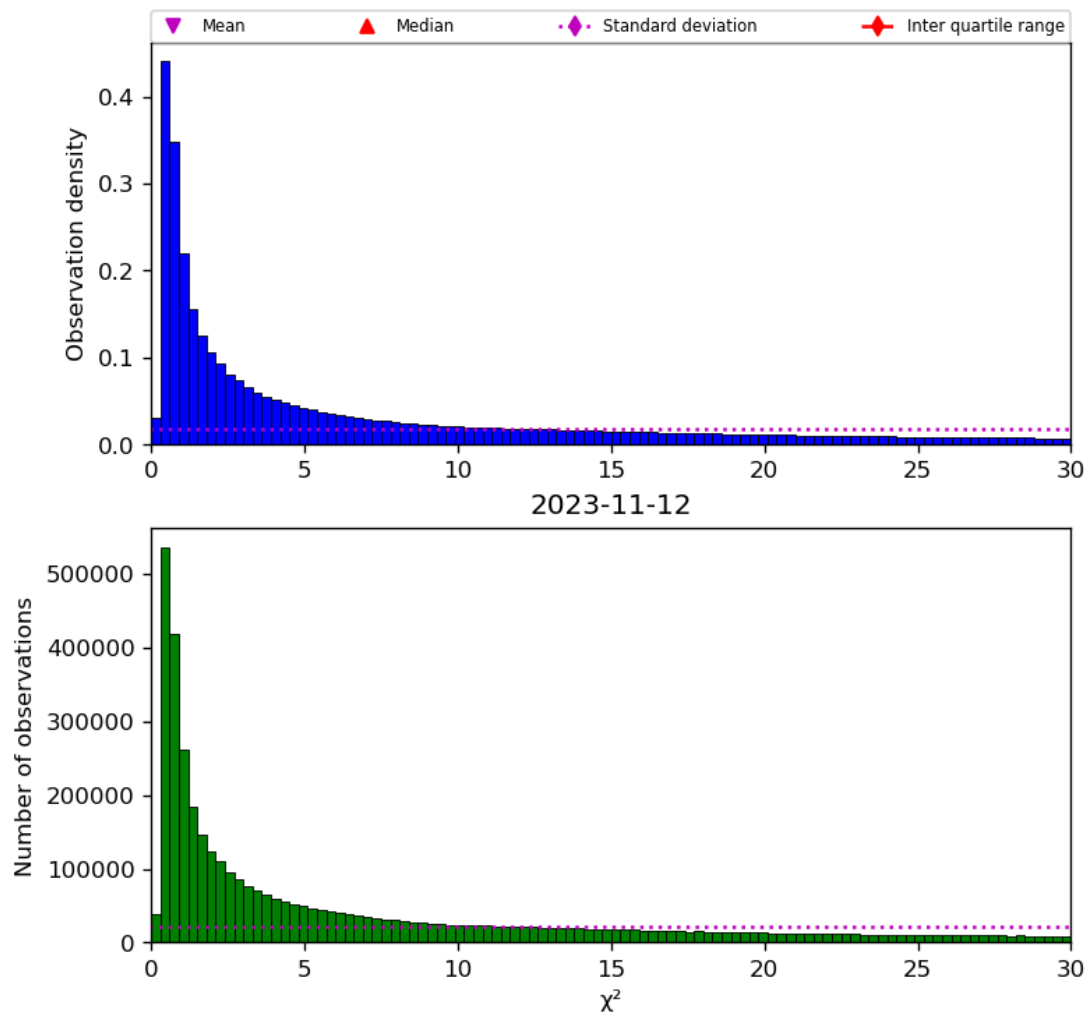
Figure 38: Histogram of “ \chi^2 ” for 2023-11-12 to 2023-11-13
