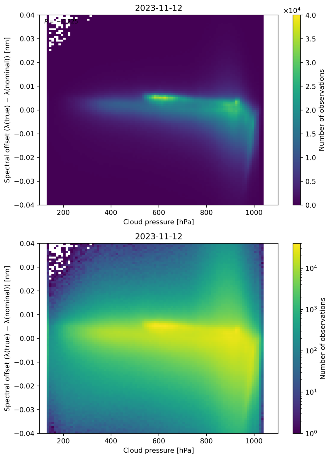
Figure 92: Scatter density plot of “Cloud pressure” against “Spectral offset ( \lambda(\text{true}) - \lambda(\text{nominal}) )” for 2023-11-12 to 2023-11-13.
