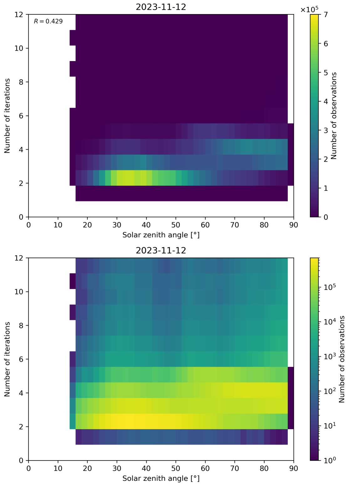
Figure 125: Scatter density plot of “Solar zenith angle” against “Number of iterations” for 2023-11-12 to 2023-11-13.
