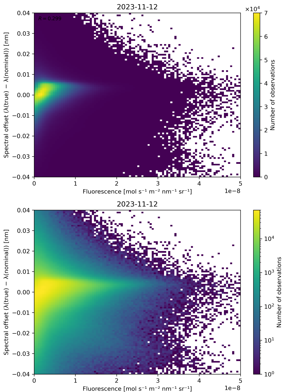
Figure 95: Scatter density plot of “Fluorescence” against “Spectral offset ( \lambda(\text{true}) - \lambda(\text{nominal}) )” for 2023-11-12 to 2023-11-13.
