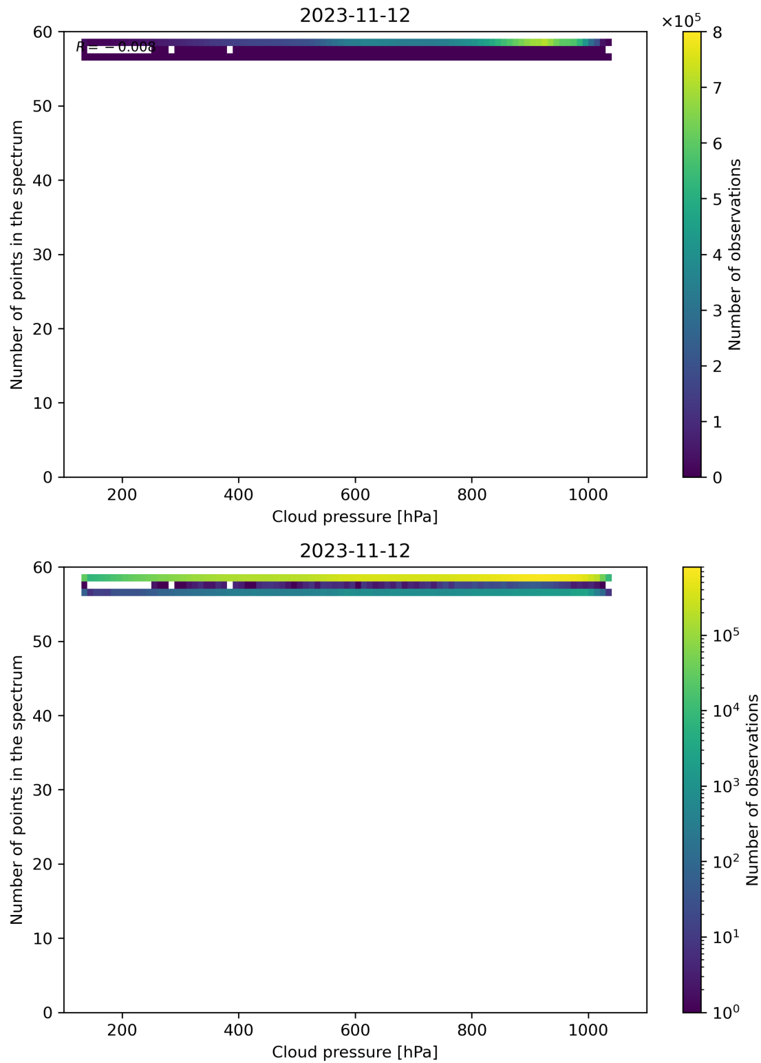
Figure 90: Scatter density plot of “Cloud pressure” against “Number of points in the spectrum” for 2023-11-12 to 2023-11-13.
