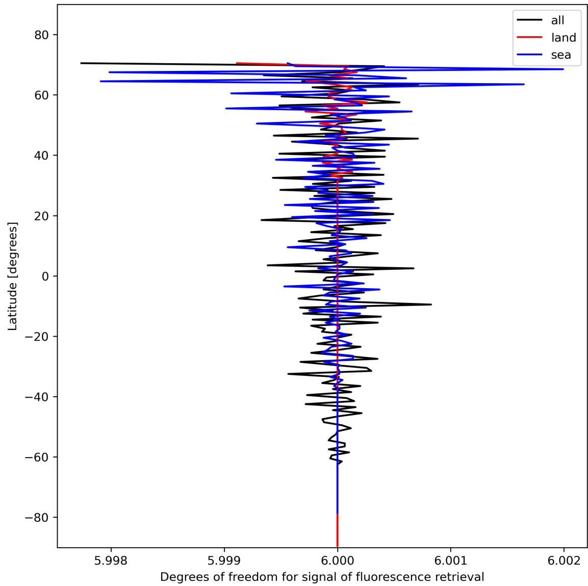
Figure 26: Zonal average of “Degrees of freedom for signal of fluorescence retrieval” for 2023-11-12 to 2023-11-13.
