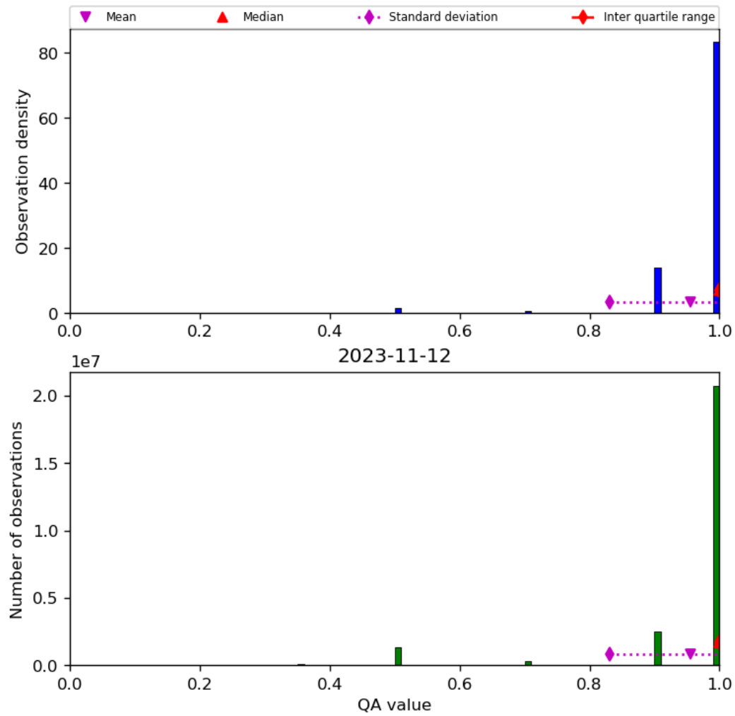
Figure 29: Histogram of “QA value” for 2023-11-12 to 2023-11-13
