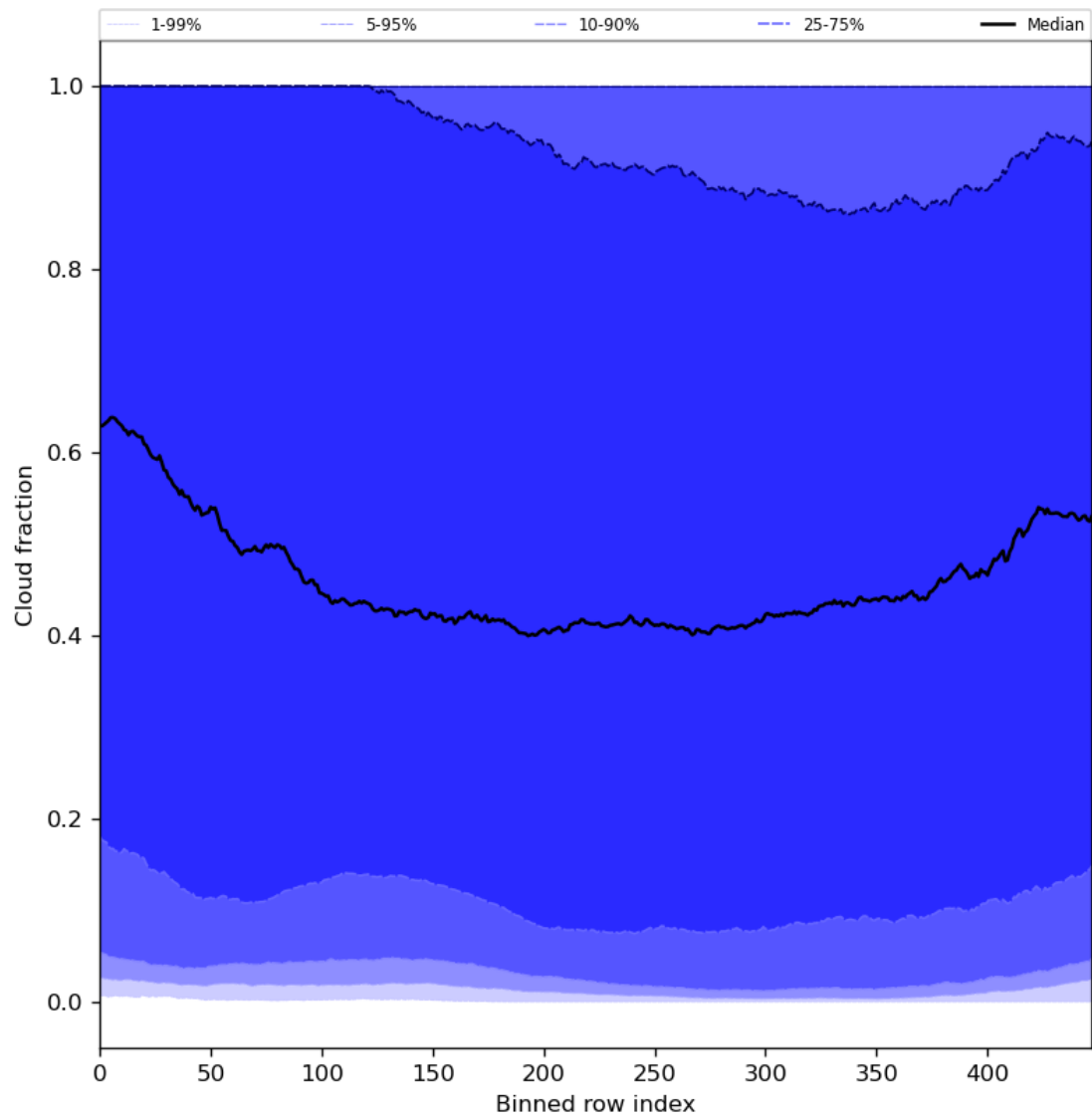
Figure 49: Along track statistics of “Cloud fraction” for 2023-11-12 to 2023-11-13
