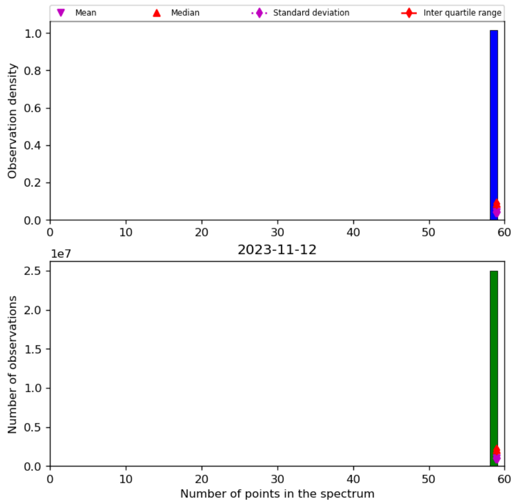
Figure 44: Histogram of “Number of points in the spectrum” for 2023-11-12 to 2023-11-13
