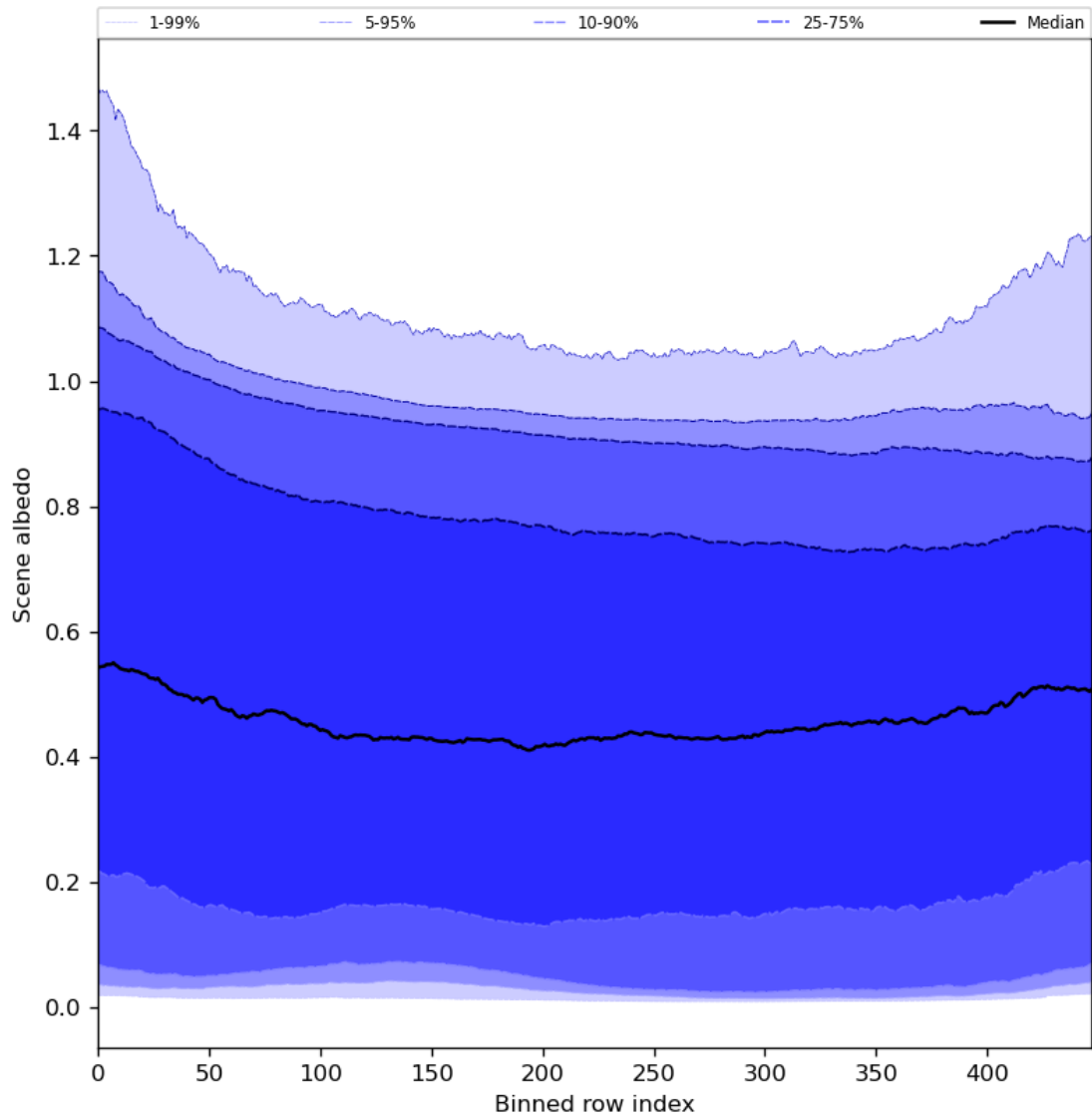
Figure 51: Along track statistics of “Scene albedo” for 2023-11-12 to 2023-11-13
