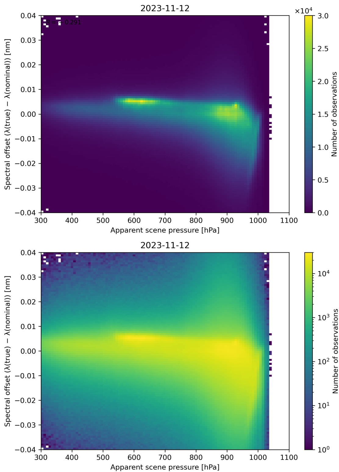
Figure 68: Scatter density plot of “Apparent scene pressure” against “Spectral offset ( \lambda(\text{true}) - \lambda(\text{nominal}) )” for 2023-11-12 to 2023-11-13.
