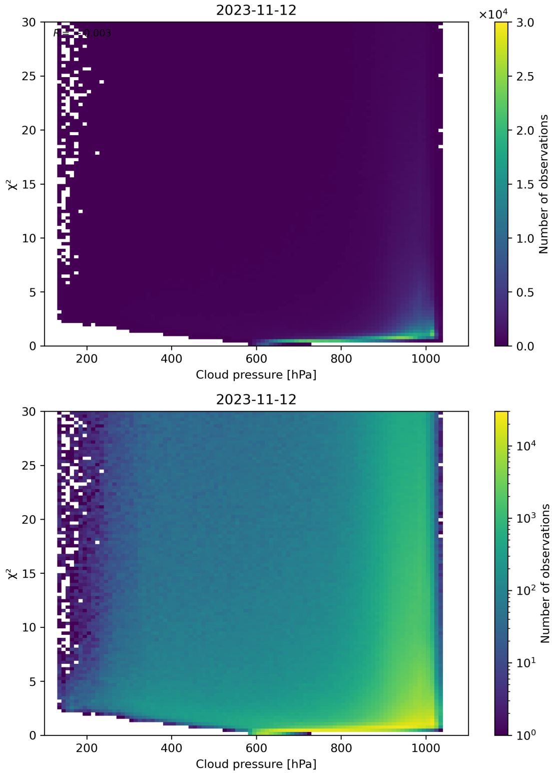
Figure 85: Scatter density plot of “Cloud pressure” against “ \chi^2 ” for 2023-11-12 to 2023-11-13.
