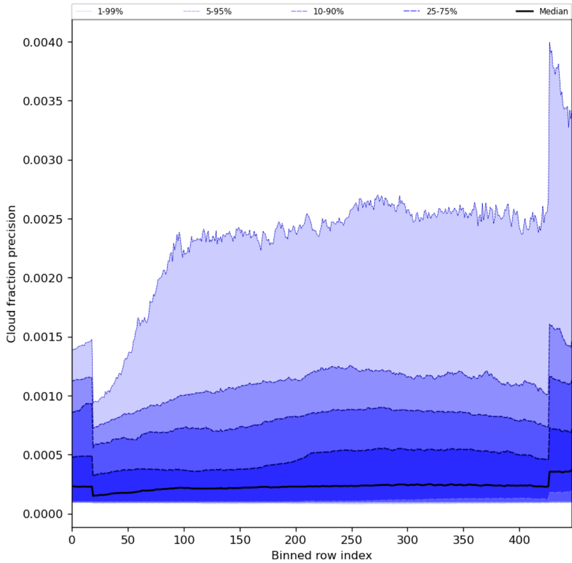
Figure 50: Along track statistics of “Cloud fraction precision” for 2023-11-12 to 2023-11-13
