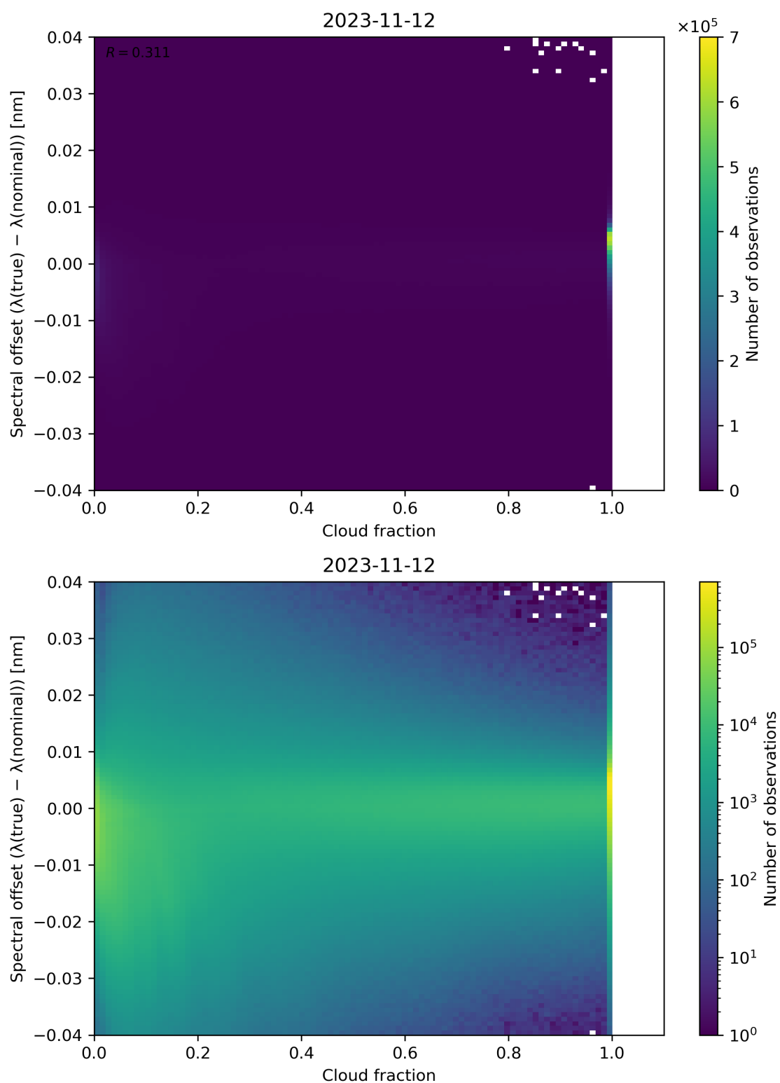
Figure 83: Scatter density plot of “Cloud fraction” against “Spectral offset ( \lambda(\text{true}) - \lambda(\text{nominal}) )” for 2023-11-12 to 2023-11-13.
