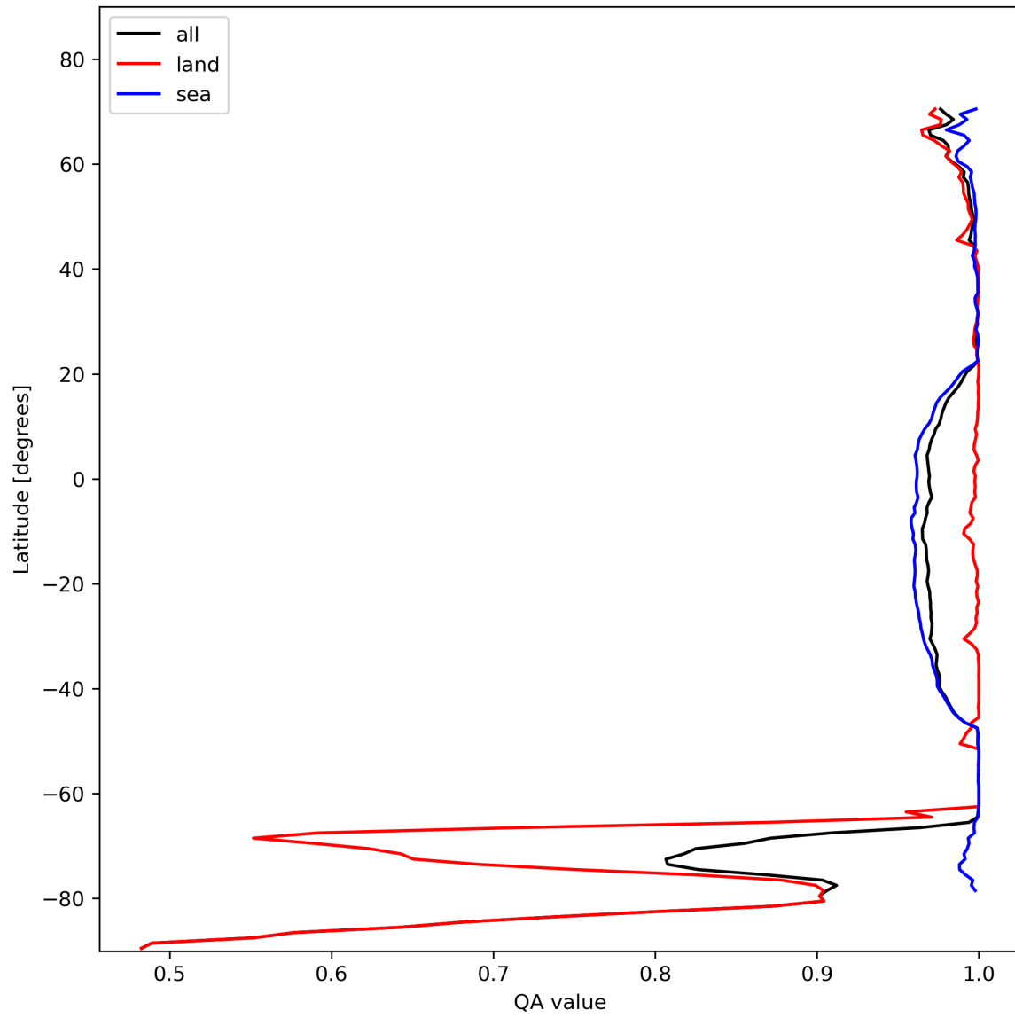
Figure 12: Zonal average of “QA value” for 2023-11-12 to 2023-11-13.
