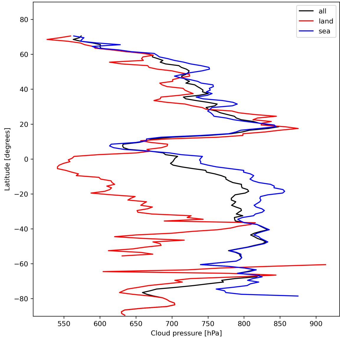
Figure 13: Zonal average of “Cloud pressure” for 2023-11-12 to 2023-11-13.
