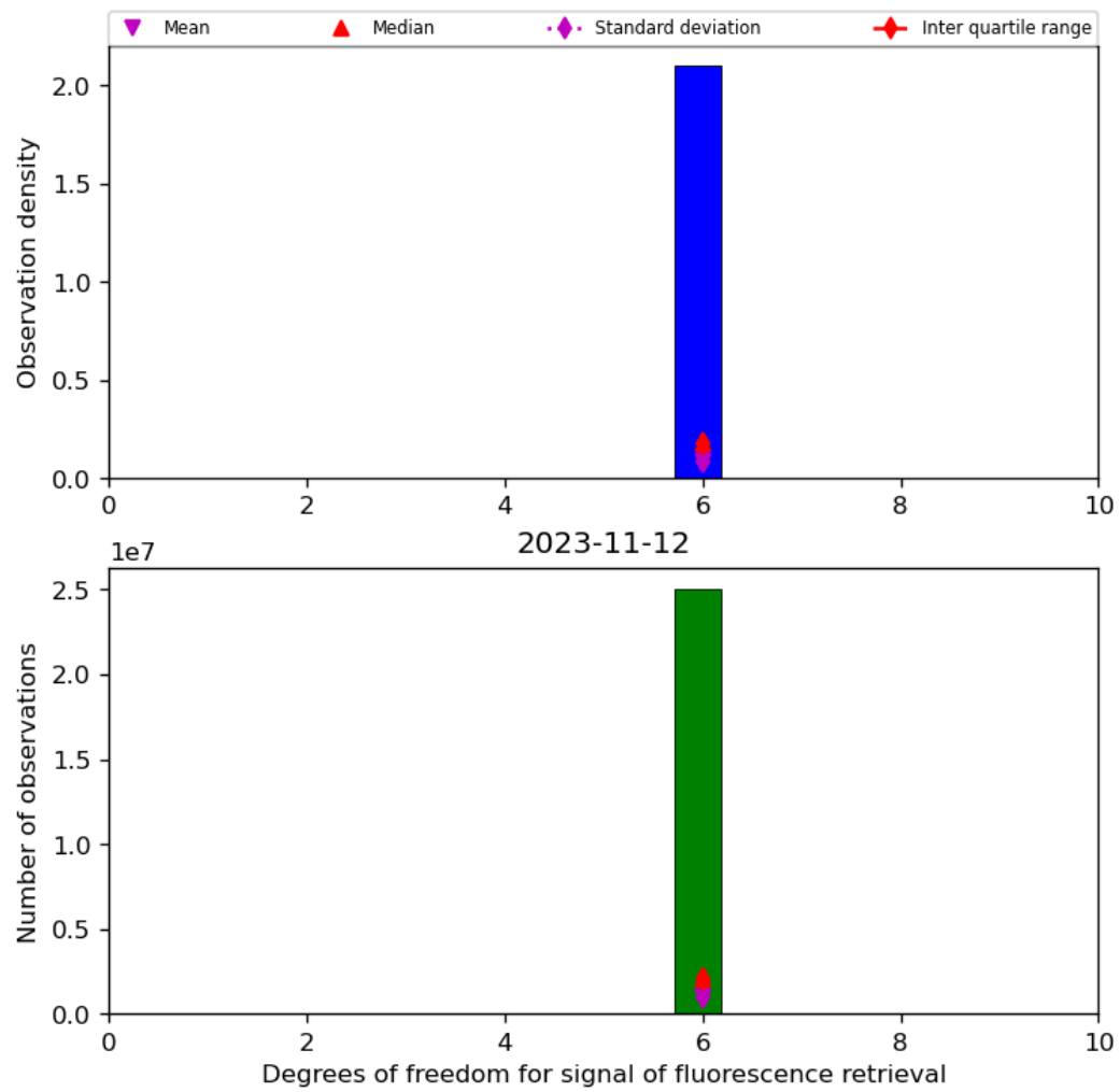
Figure 43: Histogram of “Degrees of freedom for signal of fluorescence retrieval” for 2023-11-12 to 2023-11-13
