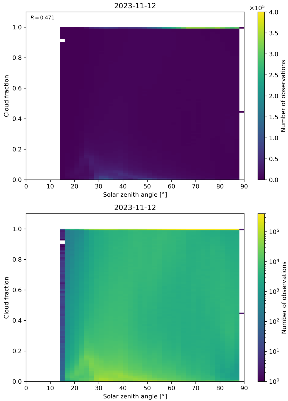
Figure 121: Scatter density plot of “Solar zenith angle” against “Cloud fraction” for 2023-11-12 to 2023-11-13.
