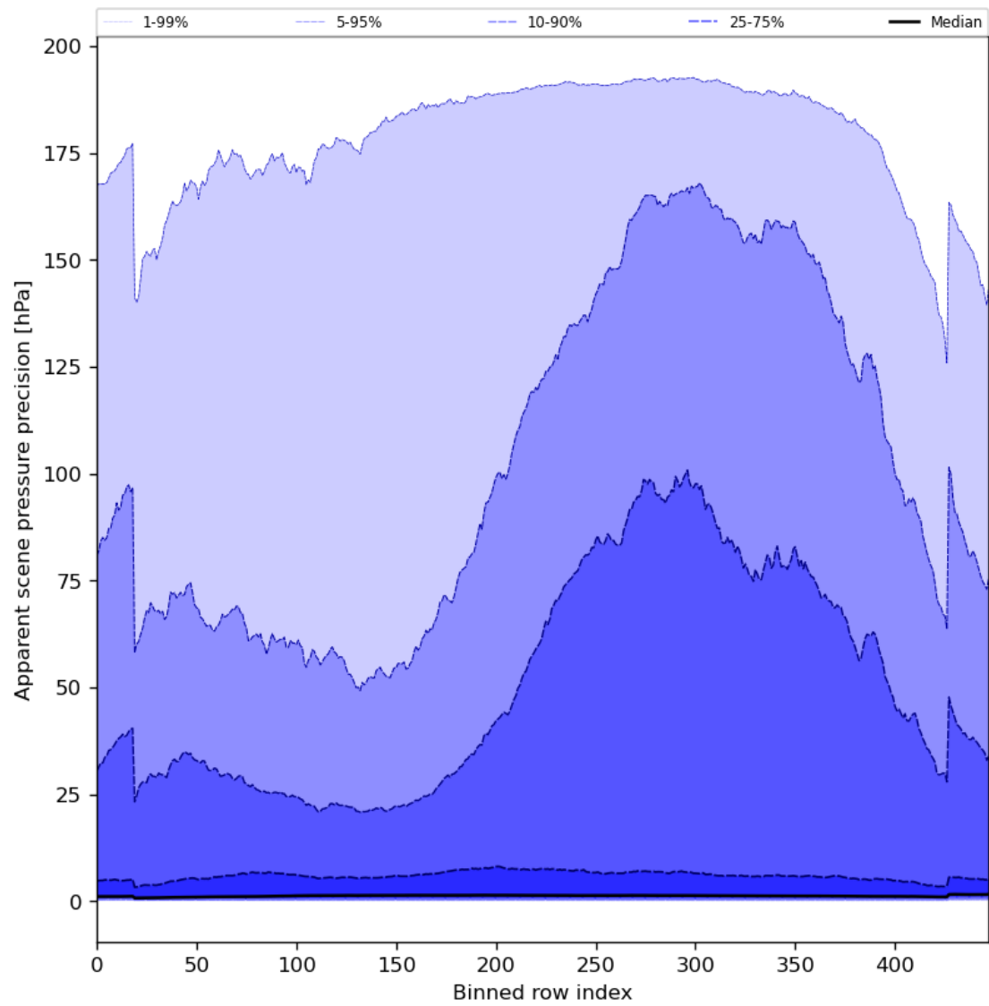
Figure 54: Along track statistics of “Apparent scene pressure precision” for 2023-11-12 to 2023-11-13
