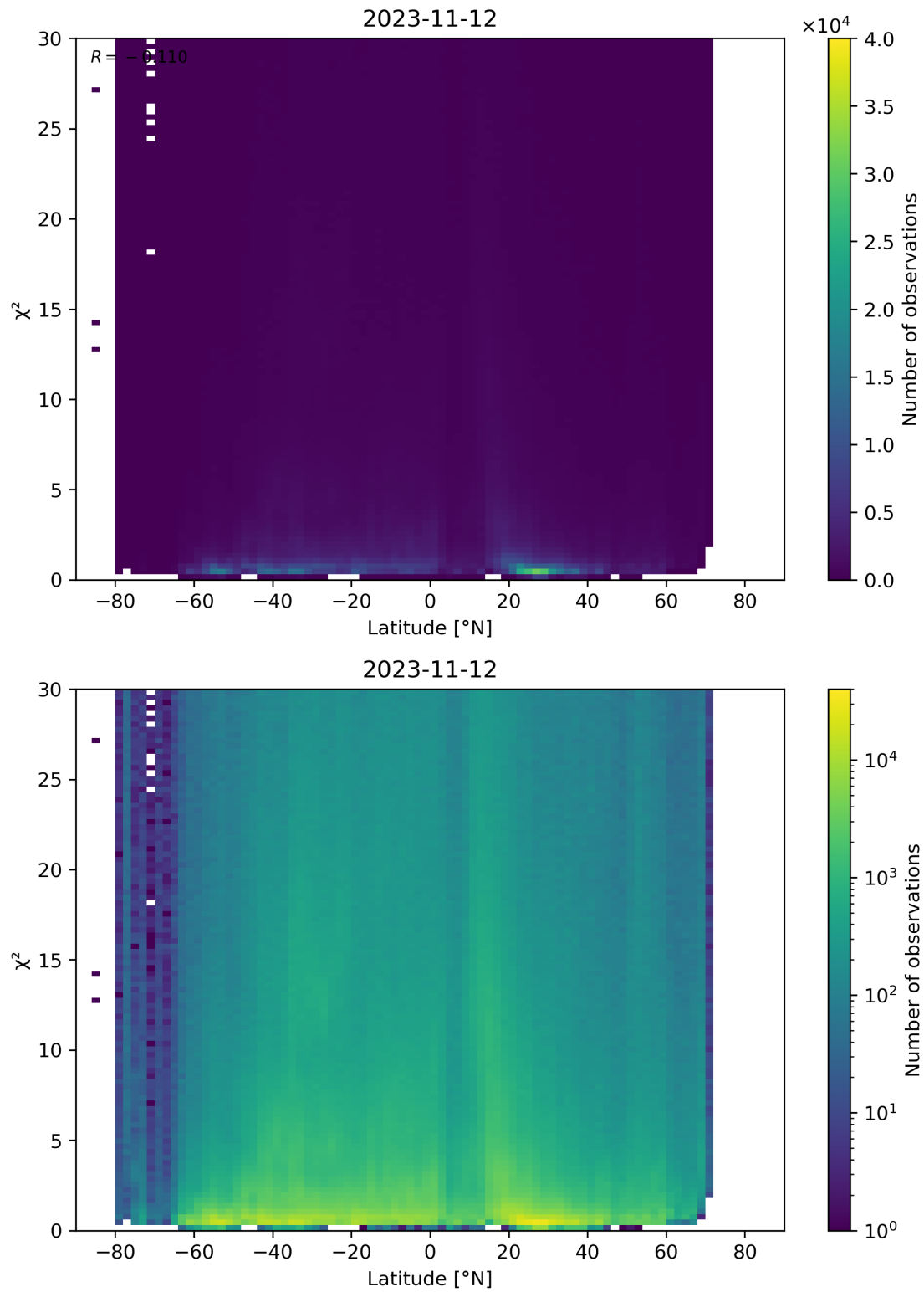
Figure 97: Scatter density plot of “Latitude” against “ \chi^2 ” for 2023-11-12 to 2023-11-13.
