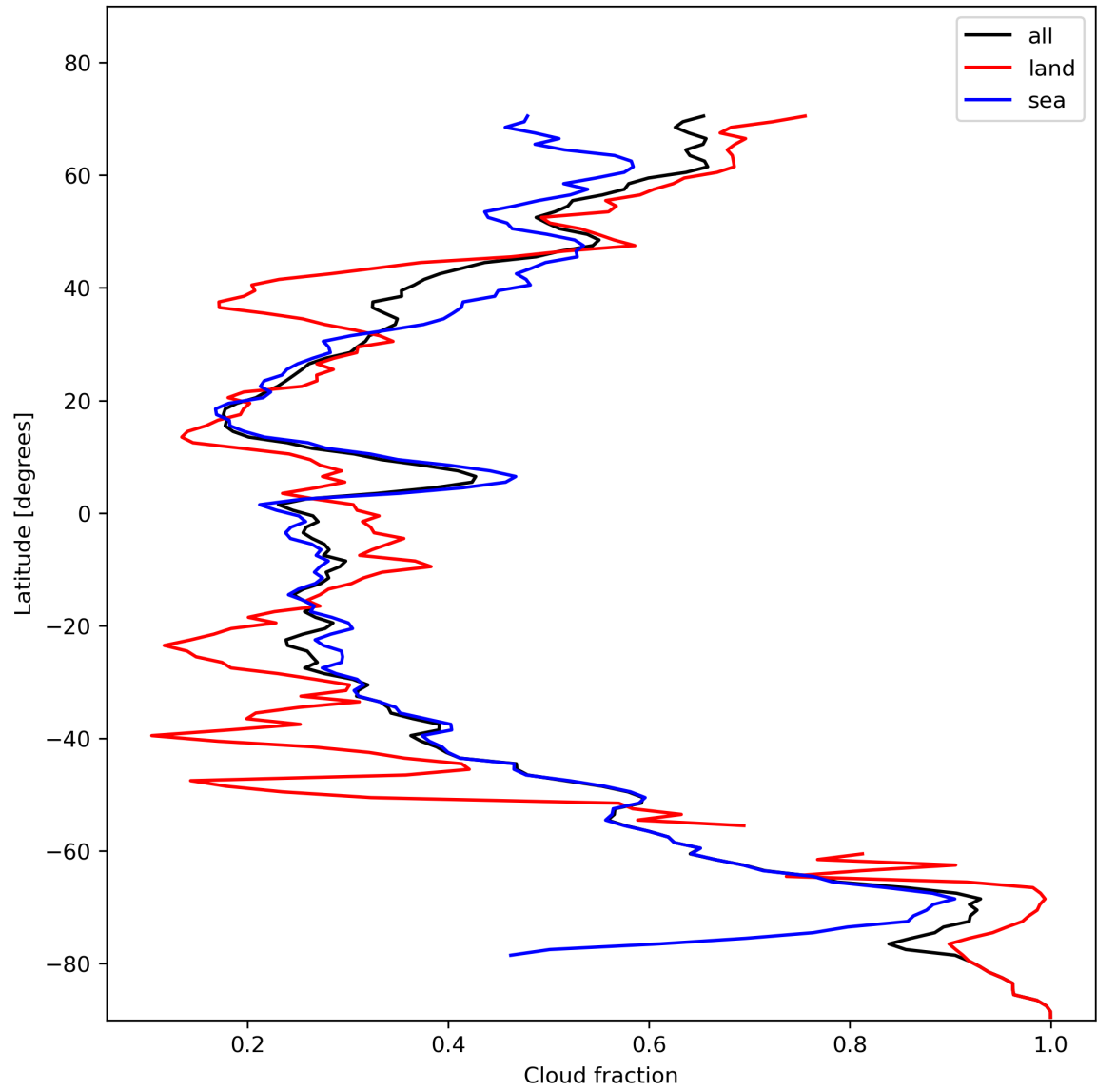
Figure 15: Zonal average of “Cloud fraction” for 2023-11-12 to 2023-11-13.
