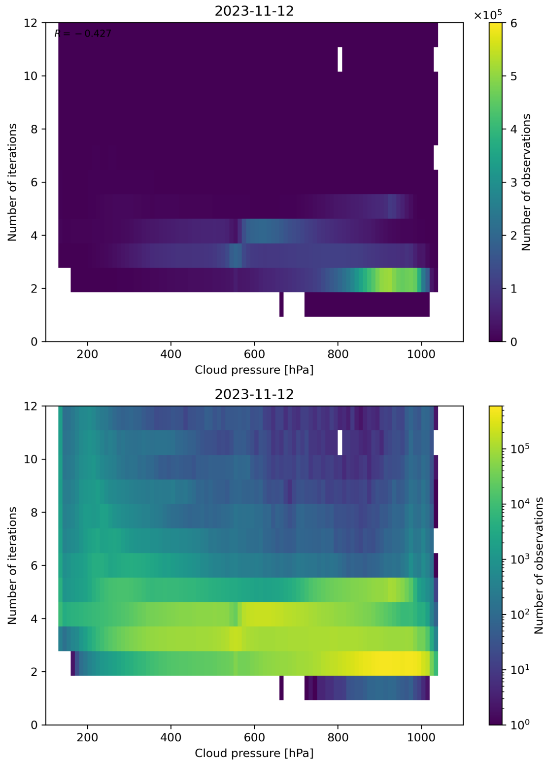
Figure 89: Scatter density plot of “Cloud pressure” against “Number of iterations” for 2023-11-12 to 2023-11-13.
