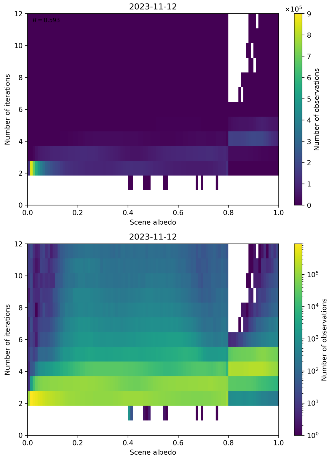
Figure 115: Scatter density plot of “Scene albedo” against “Number of iterations” for 2023-11-12 to 2023-11-13.
