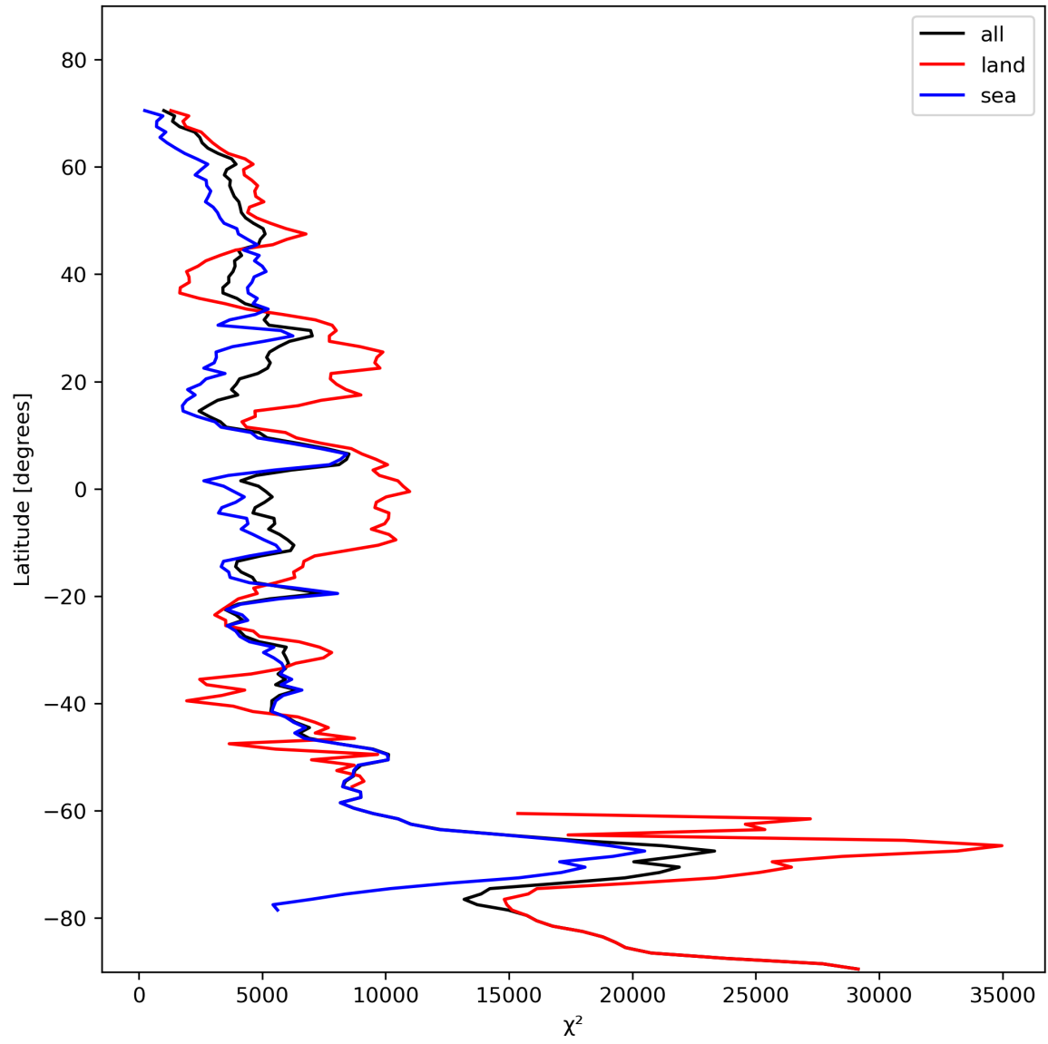
Figure 21: Zonal average of “ \chi^2 ” for 2023-11-12 to 2023-11-13.
