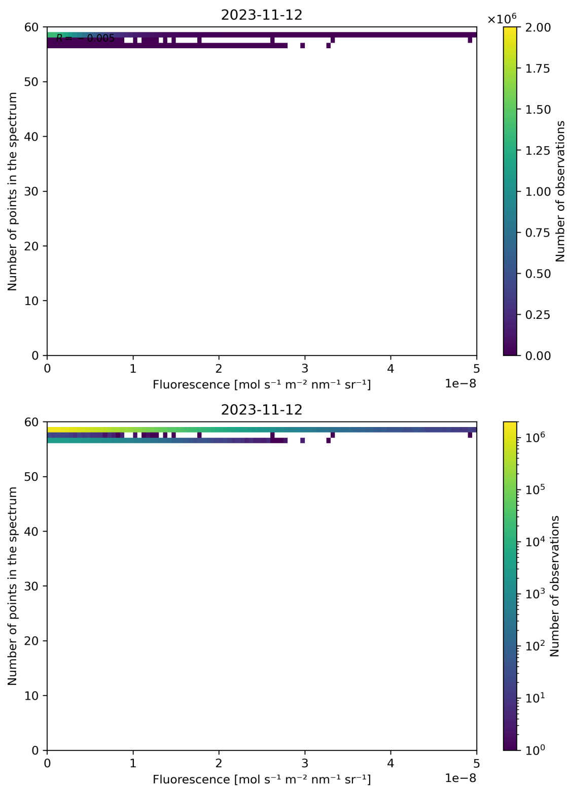
Figure 94: Scatter density plot of “Fluorescence” against “Number of points in the spectrum” for 2023-11-12 to 2023-11-13.
