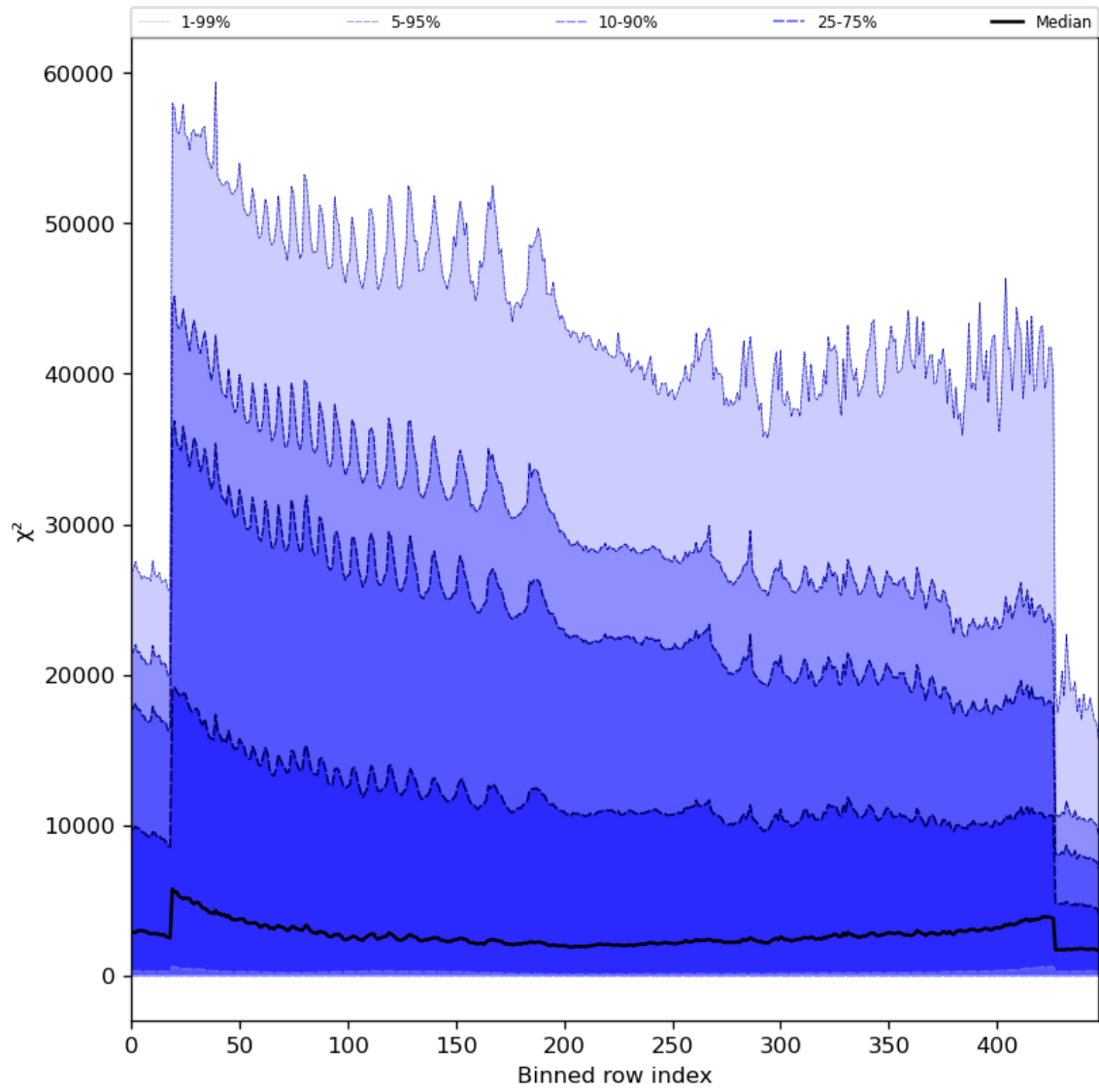
Figure 55: Along track statistics of “ \chi^2 ” for 2023-11-12 to 2023-11-13
