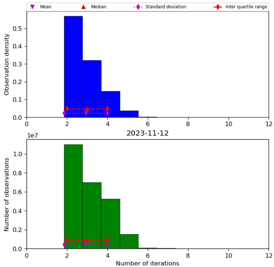
Figure 39: Histogram of “Number of iterations” for 2023-11-12 to 2023-11-13
