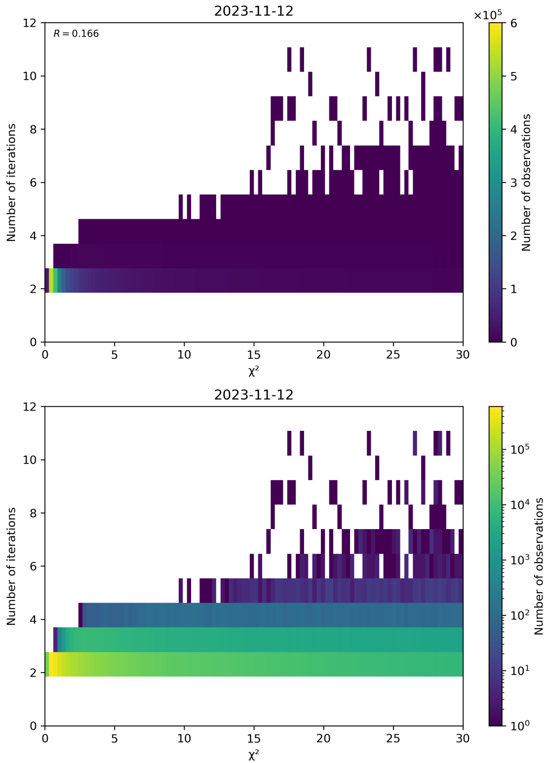
Figure 73: Scatter density plot of “ \chi^2 ” against “Number of iterations” for 2023-11-12 to 2023-11-13.
