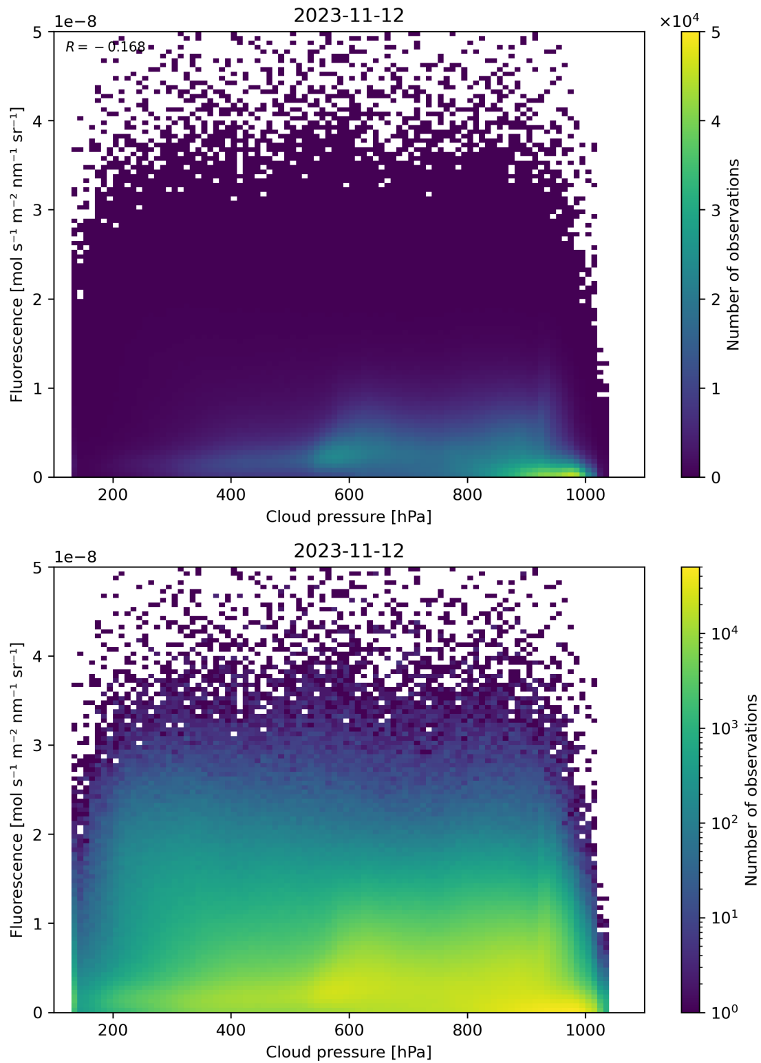
Figure 88: Scatter density plot of “Cloud pressure” against “Fluorescence” for 2023-11-12 to 2023-11-13.
