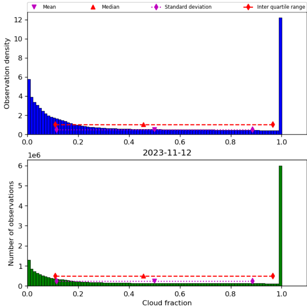
Figure 32: Histogram of “Cloud fraction” for 2023-11-12 to 2023-11-13
