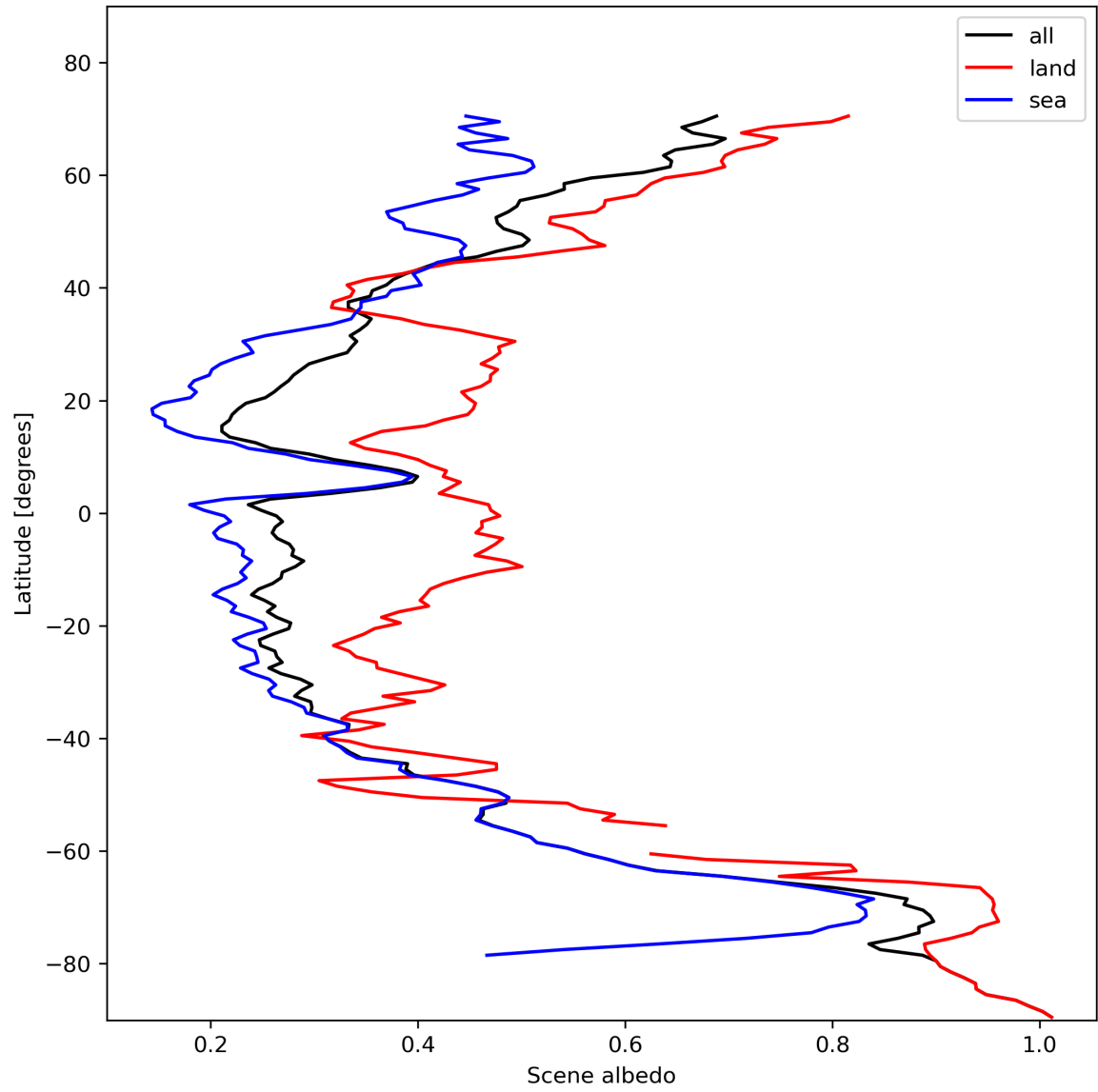
Figure 17: Zonal average of “Scene albedo” for 2023-11-12 to 2023-11-13.
