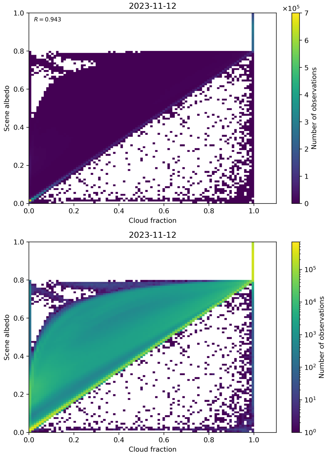
Figure 82: Scatter density plot of “Cloud fraction” against “Scene albedo” for 2023-11-12 to 2023-11-13.
