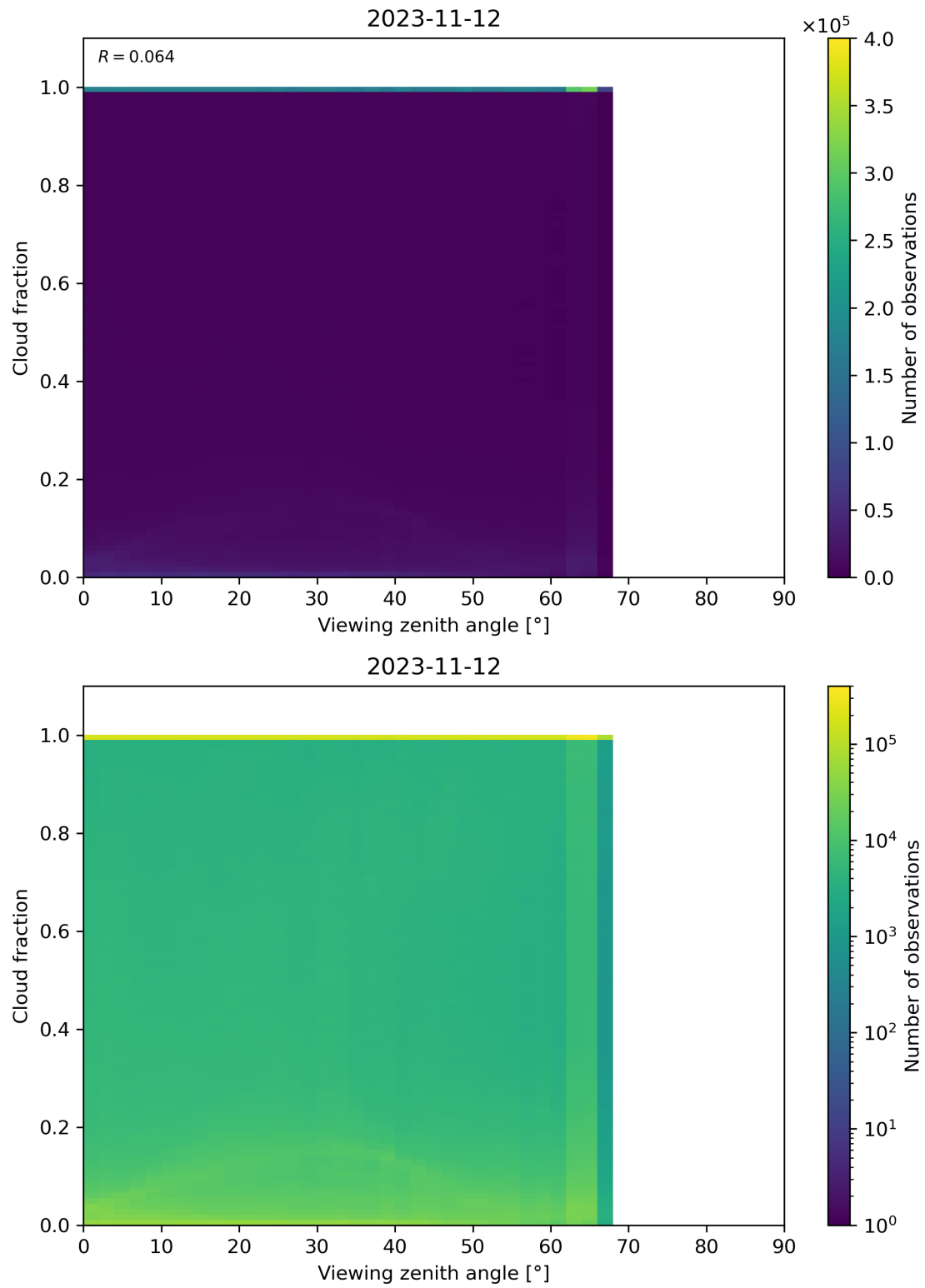
Figure 132: Scatter density plot of “Viewing zenith angle” against “Cloud fraction” for 2023-11-12 to 2023-11-13.
