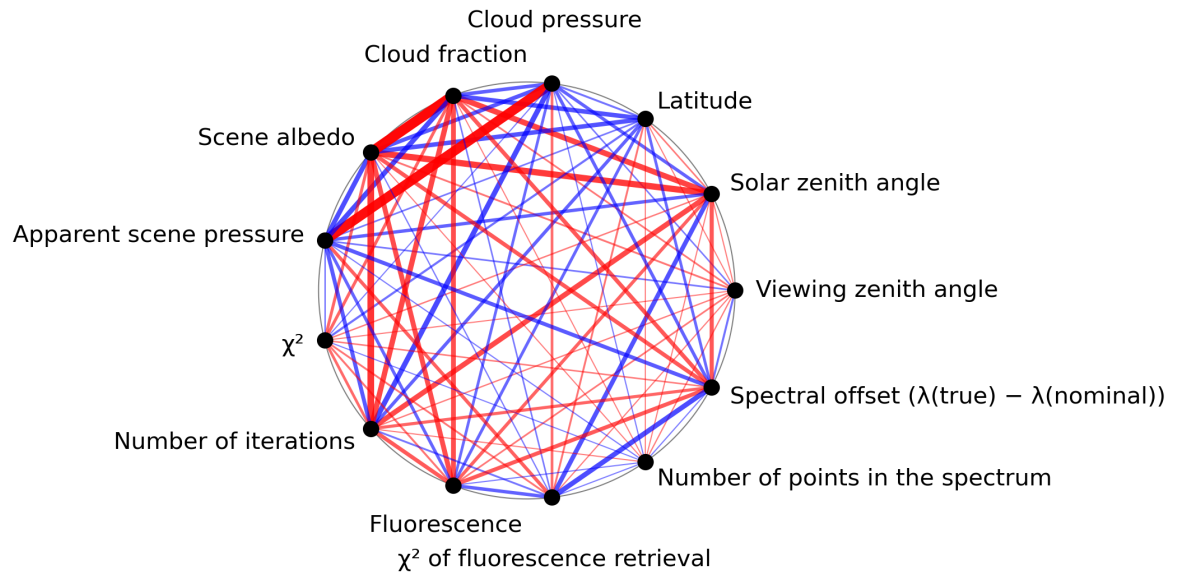
Figure 1: Map of correlation graph for 2023-11-12 to 2023-11-13.
