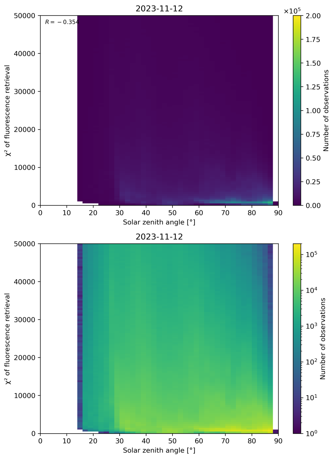
Figure 120: Scatter density plot of “Solar zenith angle” against “ \chi^2 of fluorescence retrieval” for 2023-11-12 to 2023-11-13.
