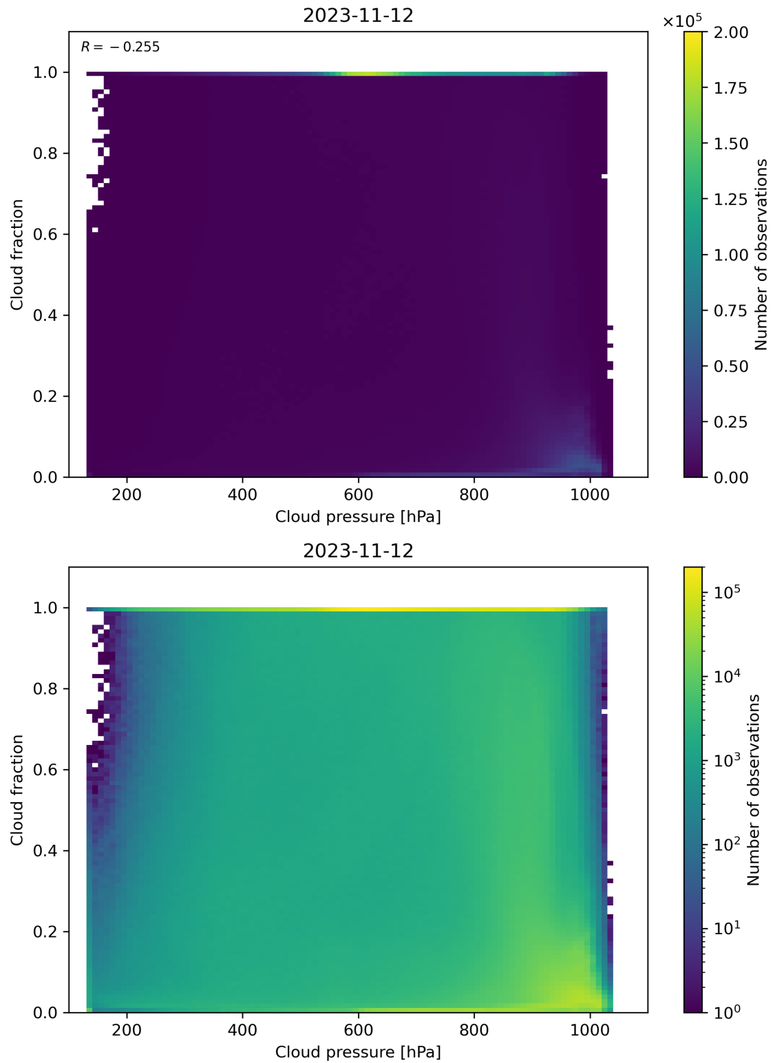
Figure 87: Scatter density plot of “Cloud pressure” against “Cloud fraction” for 2023-11-12 to 2023-11-13.
