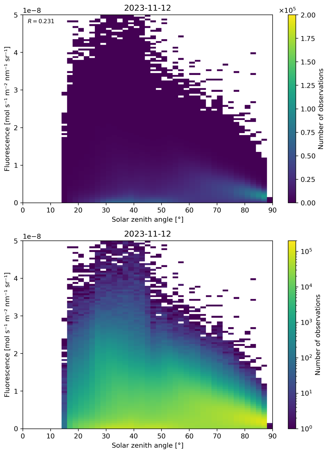
Figure 123: Scatter density plot of “Solar zenith angle” against “Fluorescence” for 2023-11-12 to 2023-11-13.
