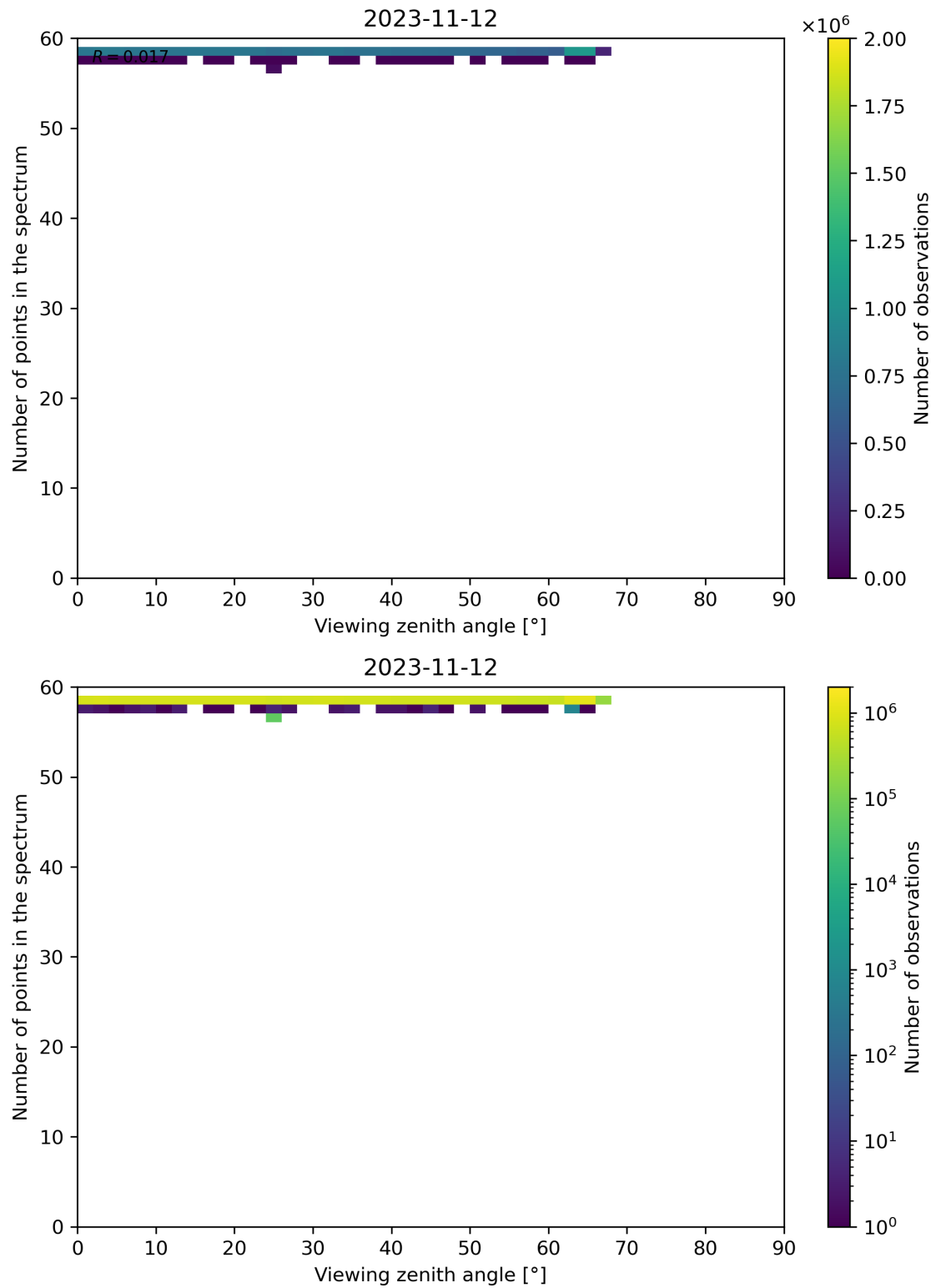
Figure 137: Scatter density plot of “Viewing zenith angle” against “Number of points in the spectrum” for 2023-11-12 to 2023-11-13.
