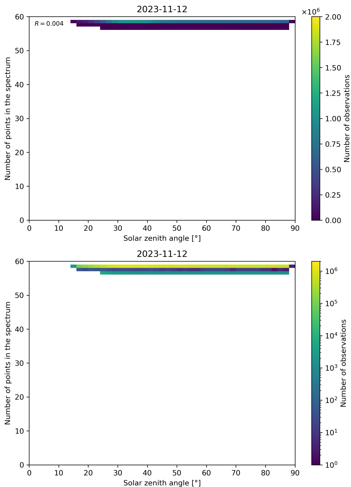
Figure 126: Scatter density plot of “Solar zenith angle” against “Number of points in the spectrum” for 2023-11-12 to 2023-11-13.
