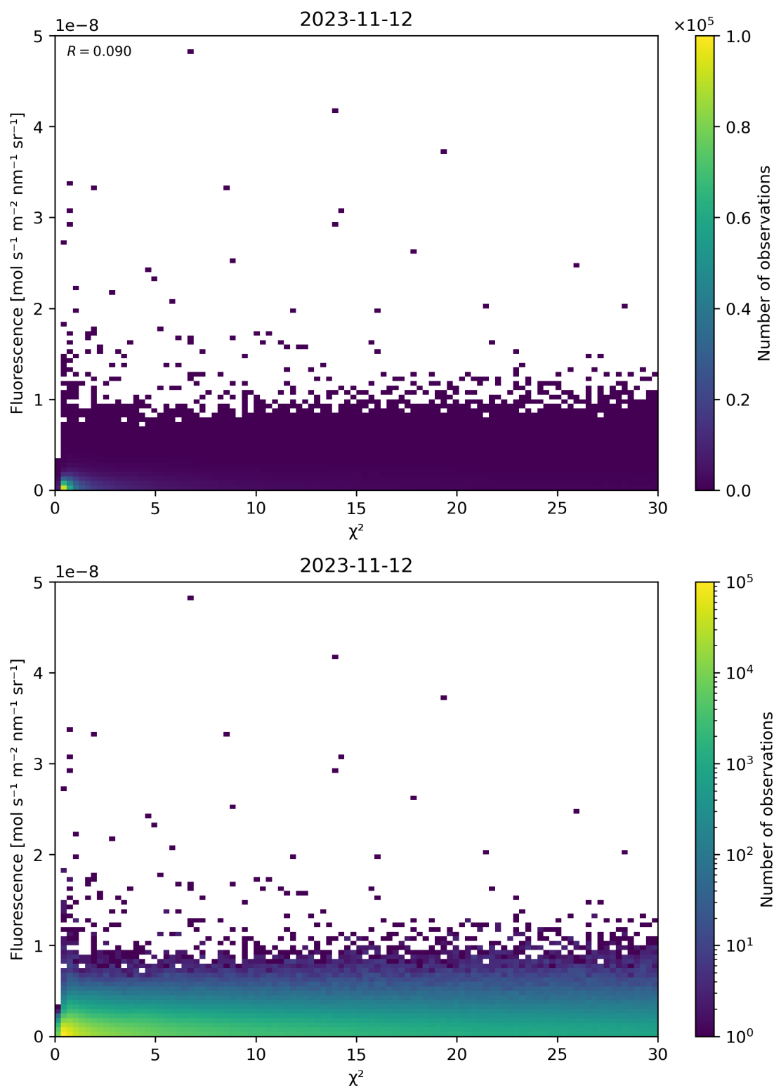
Figure 70: Scatter density plot of “ \chi^2 ” against “Fluorescence” for 2023-11-12 to 2023-11-13.
