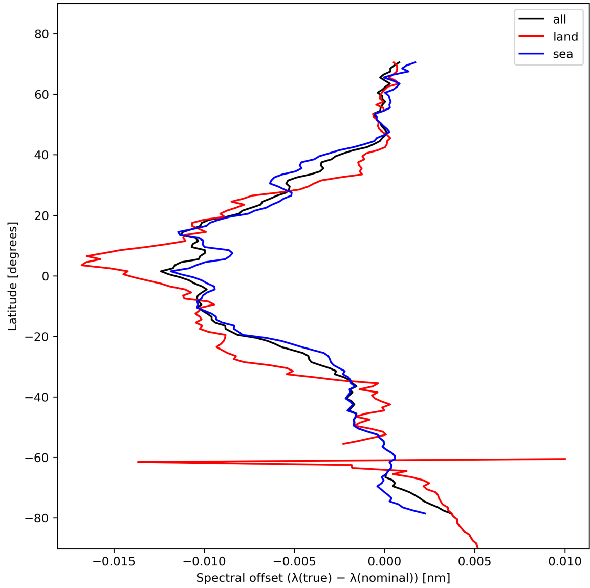
Figure 28: Zonal average of “Spectral offset ( \lambda(\text{true}) - \lambda(\text{nominal}) )” for 2023-11-12 to 2023-11-13.
