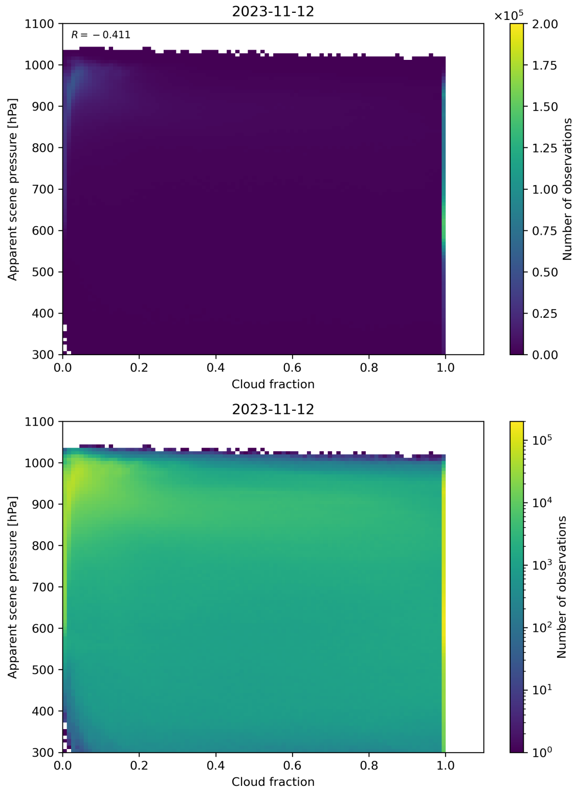
Figure 76: Scatter density plot of “Cloud fraction” against “Apparent scene pressure” for 2023-11-12 to 2023-11-13.
