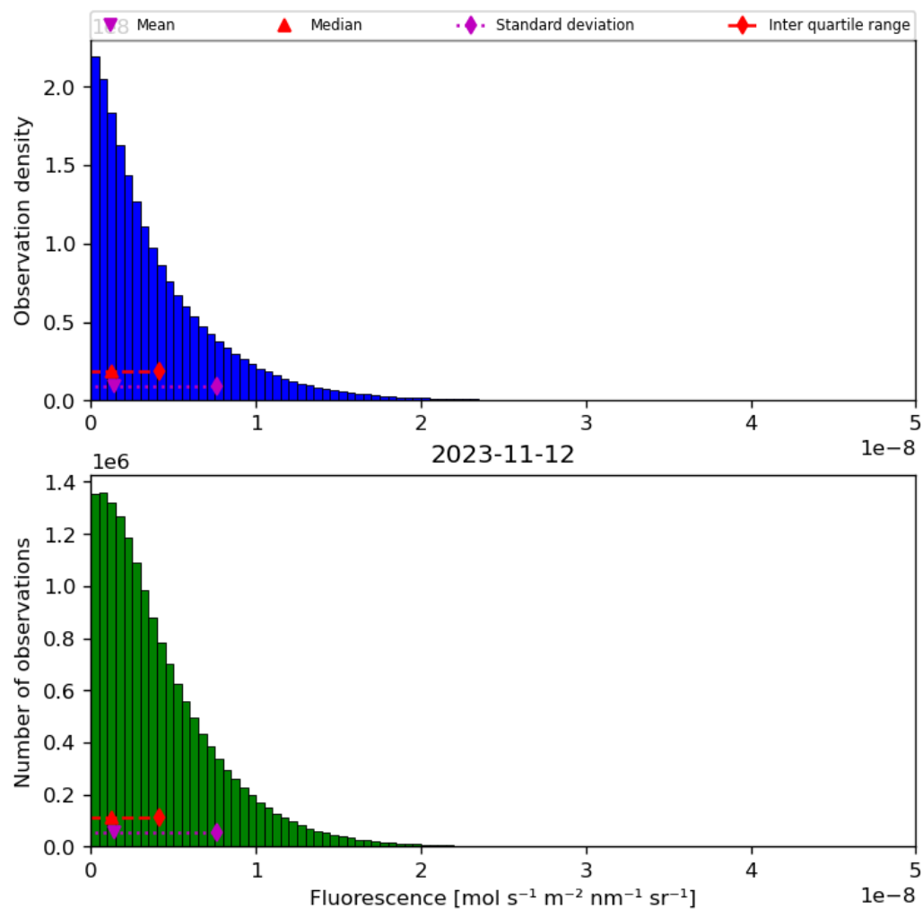
Figure 40: Histogram of “Fluorescence” for 2023-11-12 to 2023-11-13
