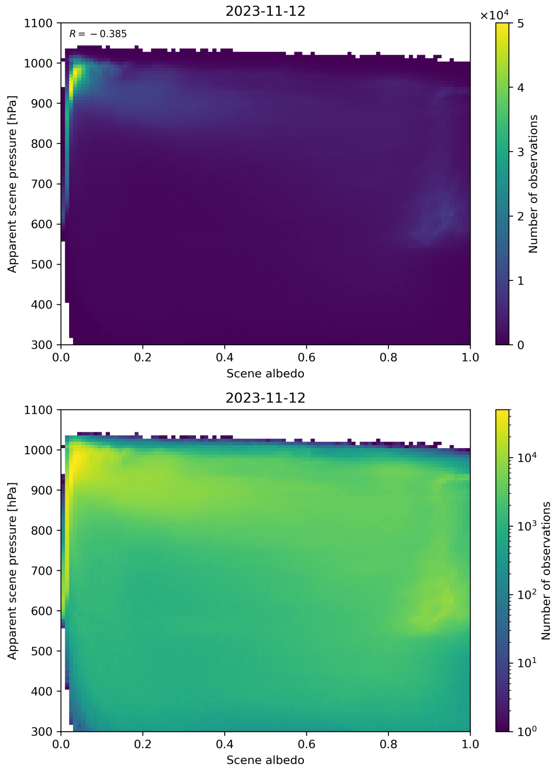
Figure 111: Scatter density plot of “Scene albedo” against “Apparent scene pressure” for 2023-11-12 to 2023-11-13.
