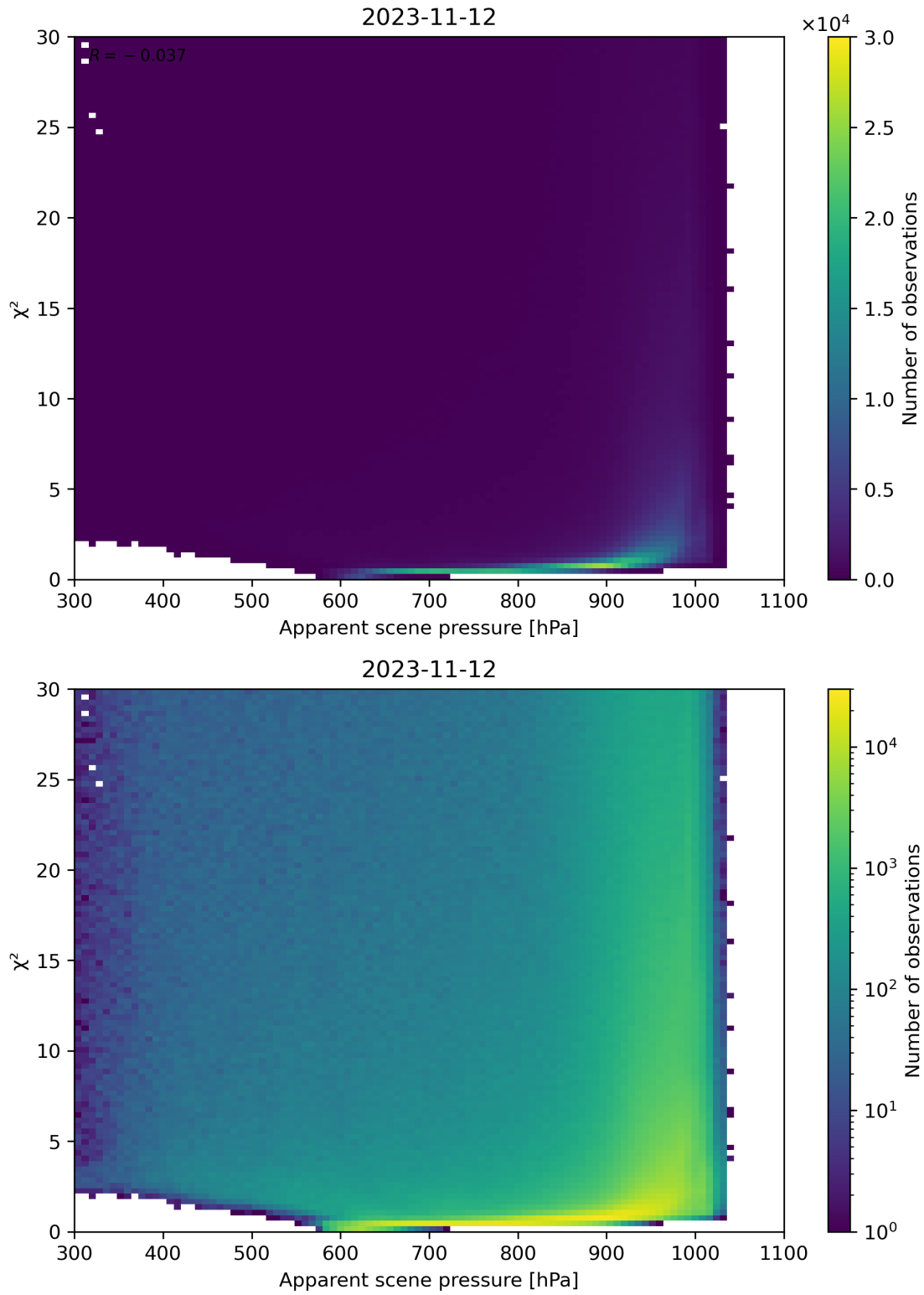
Figure 63: Scatter density plot of “Apparent scene pressure” against “ \chi^2 ” for 2023-11-12 to 2023-11-13.
