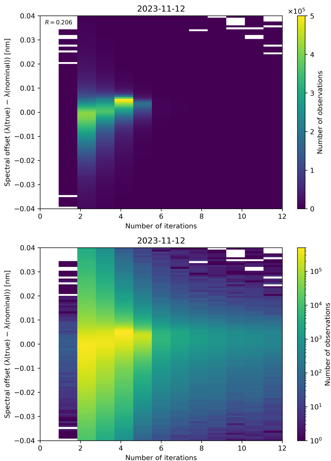
Figure 109: Scatter density plot of “Number of iterations” against “Spectral offset ( \lambda(\text{true}) - \lambda(\text{nominal}) )” for 2023-11-12 to 2023-11-13.
