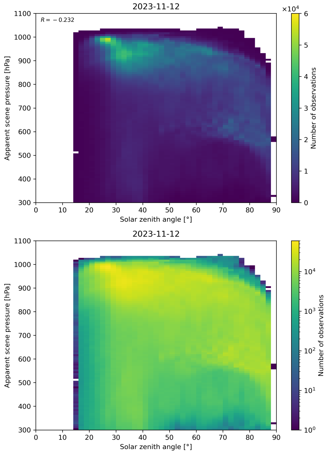
Figure 118: Scatter density plot of “Solar zenith angle” against “Apparent scene pressure” for 2023-11-12 to 2023-11-13.
