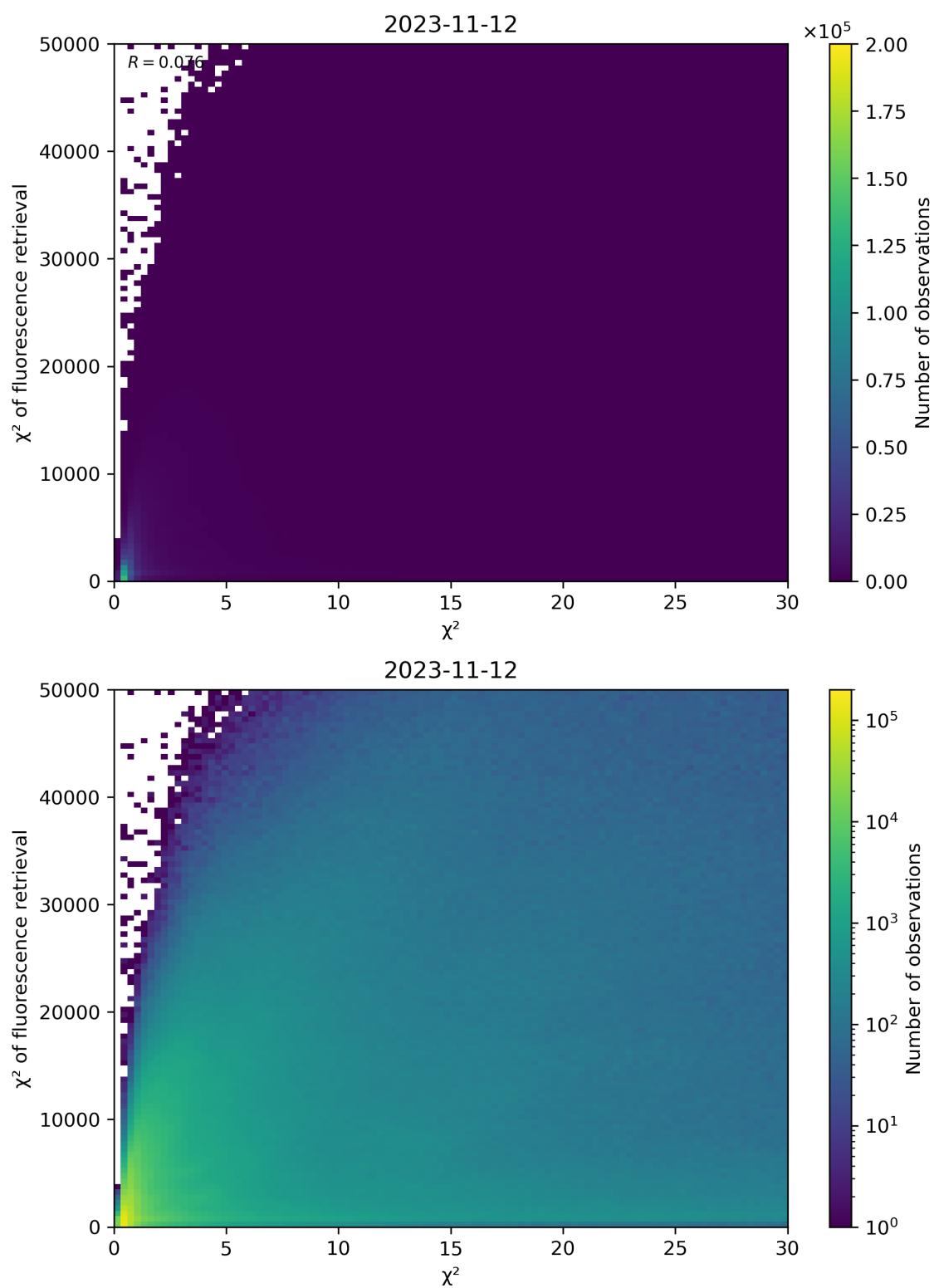
Figure 69: Scatter density plot of “ \chi^2 ” against “ \chi^2 of fluorescence retrieval” for 2023-11-12 to 2023-11-13.
