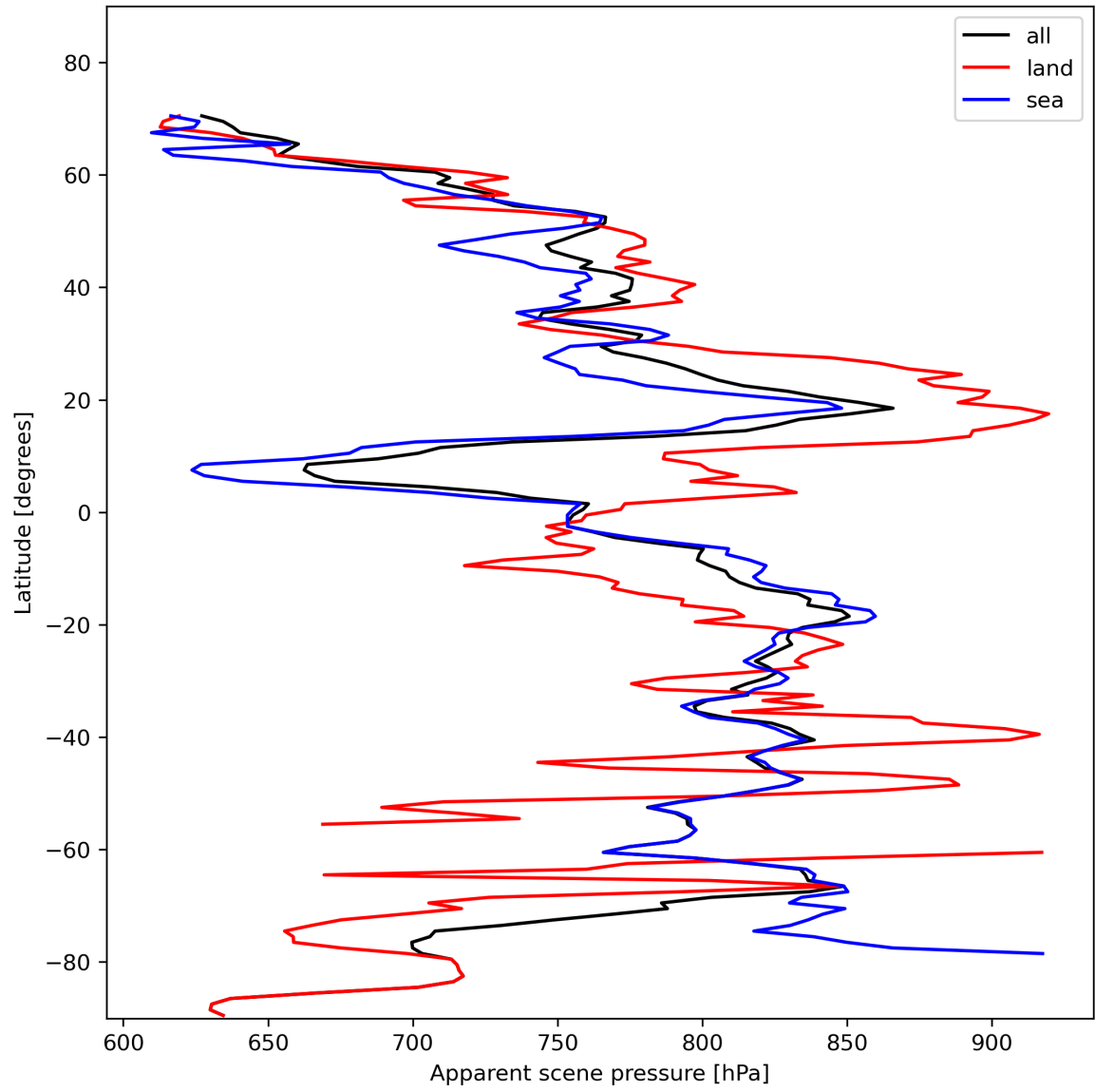
Figure 19: Zonal average of “Apparent scene pressure” for 2023-11-12 to 2023-11-13.
