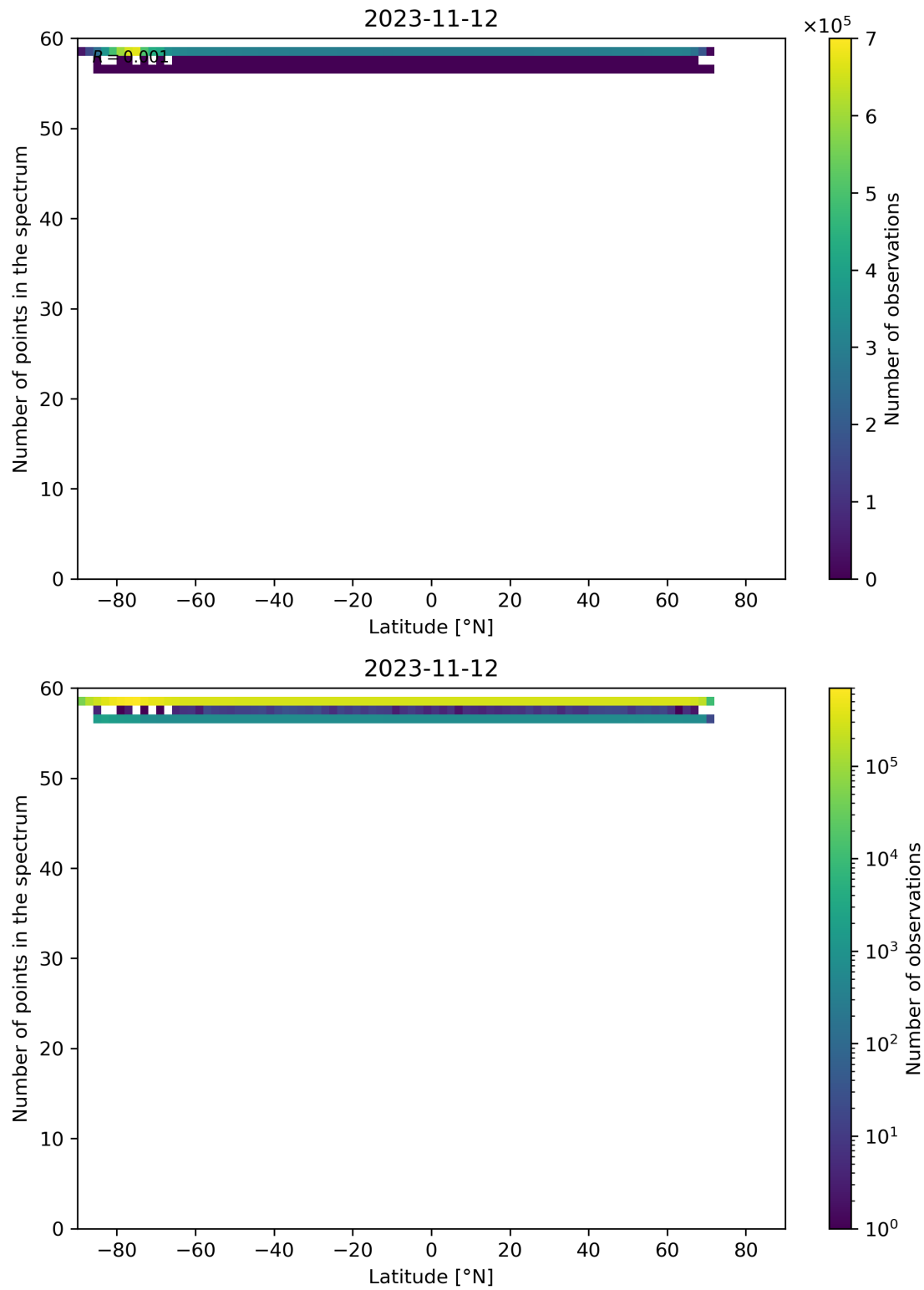
Figure 103: Scatter density plot of “Latitude” against “Number of points in the spectrum” for 2023-11-12 to 2023-11-13.
