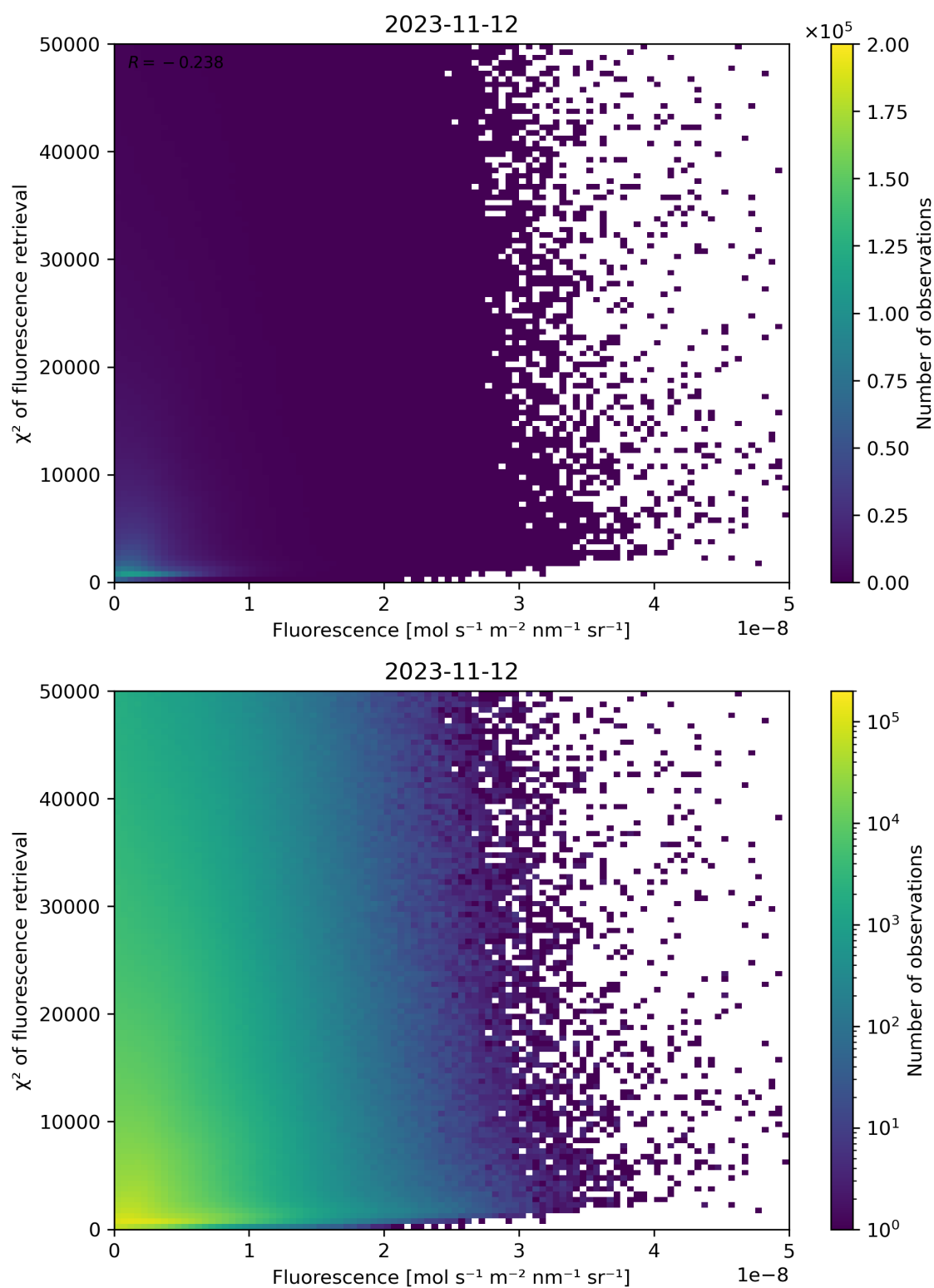
Figure 93: Scatter density plot of “Fluorescence” against “ \chi^2 of fluorescence retrieval” for 2023-11-12 to 2023-11-13.
