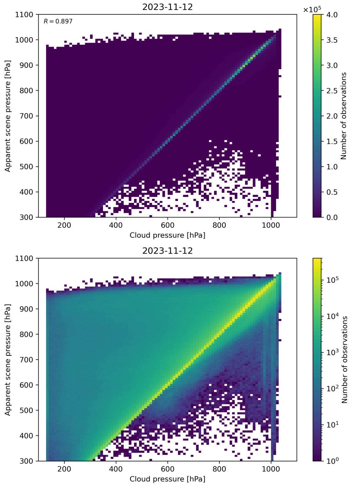
Figure 84: Scatter density plot of “Cloud pressure” against “Apparent scene pressure” for 2023-11-12 to 2023-11-13.
