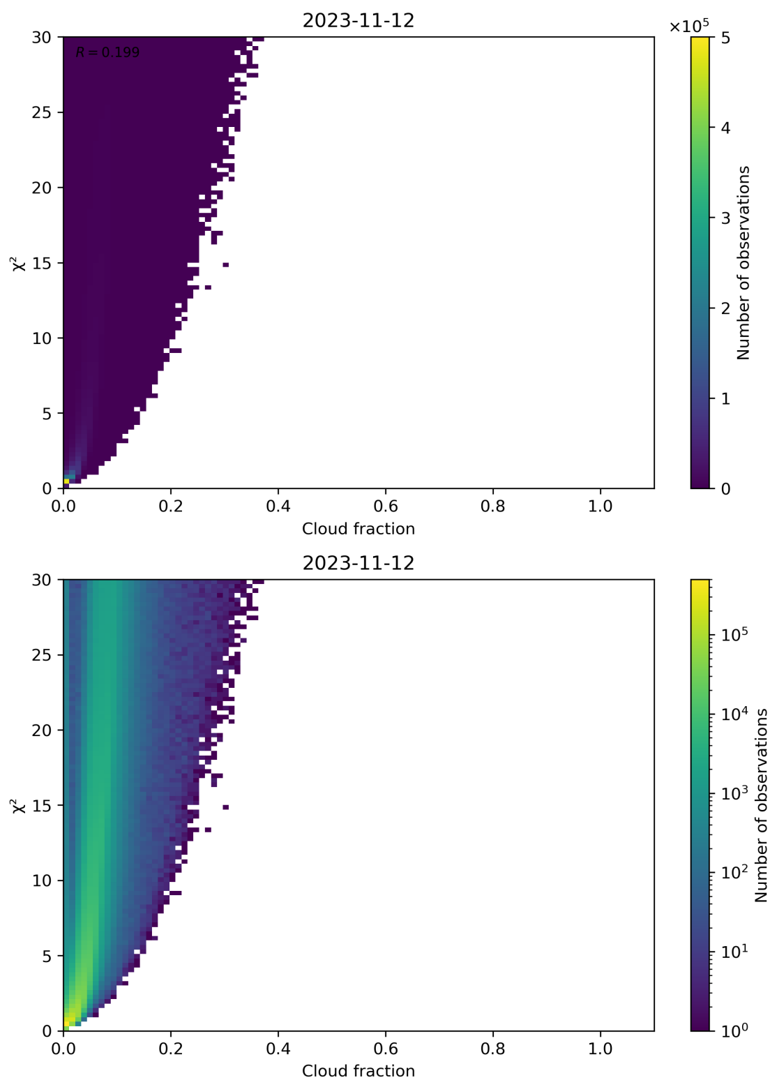
Figure 77: Scatter density plot of “Cloud fraction” against “ \chi^2 ” for 2023-11-12 to 2023-11-13.
