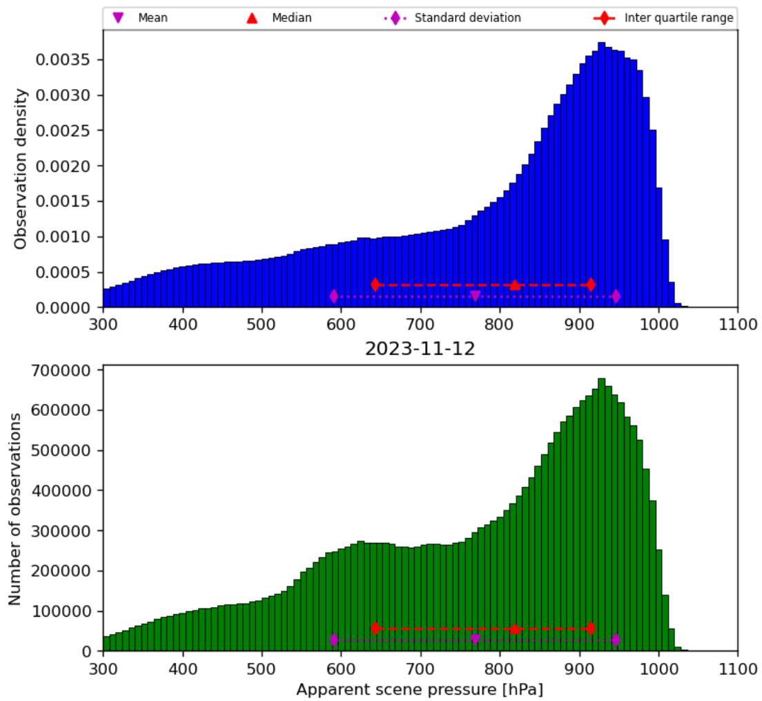
Figure 36: Histogram of “Apparent scene pressure” for 2023-11-12 to 2023-11-13
