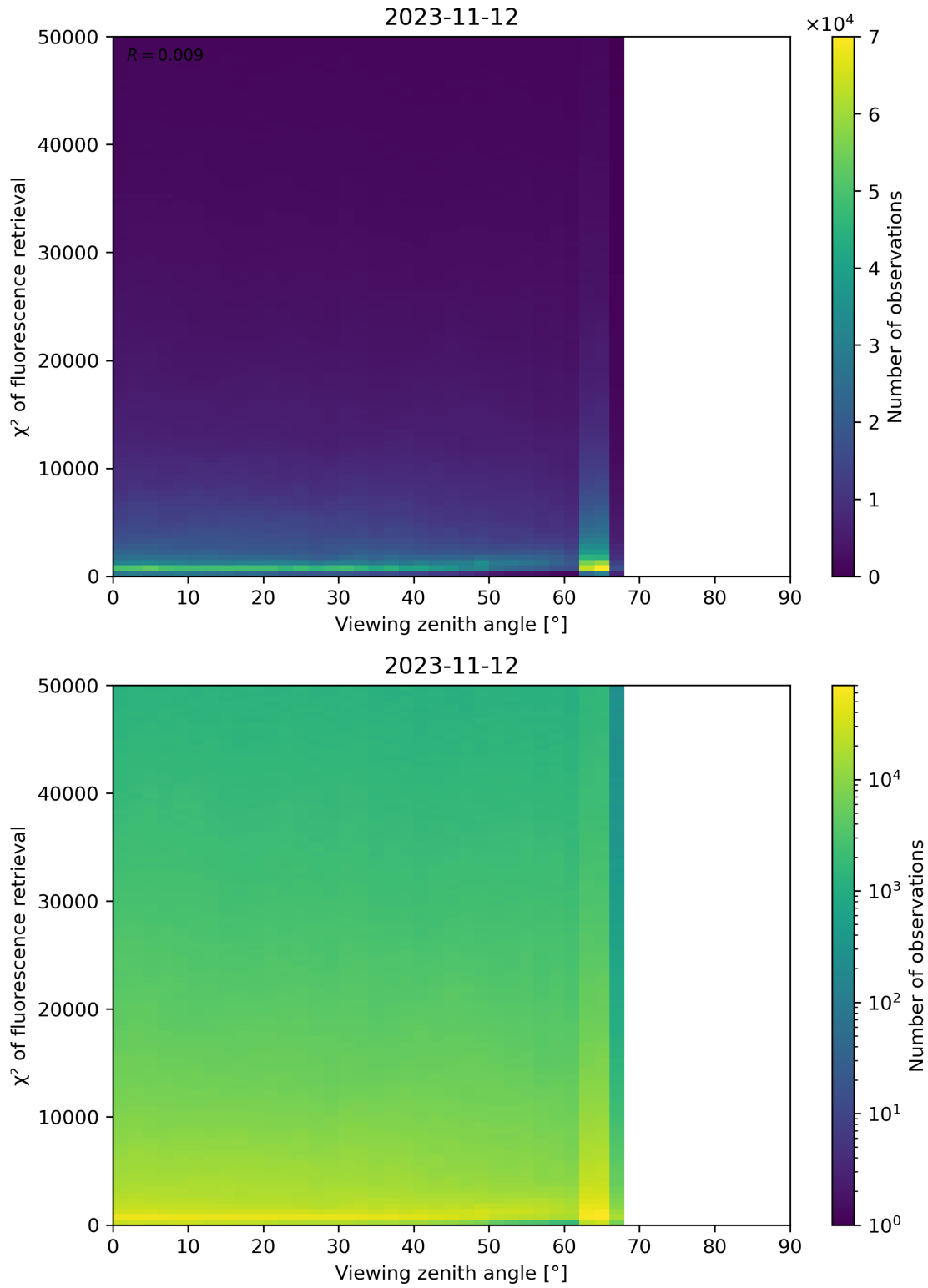
Figure 131: Scatter density plot of “Viewing zenith angle” against “ \chi^2 of fluorescence retrieval” for 2023-11-12 to 2023-11-13.
