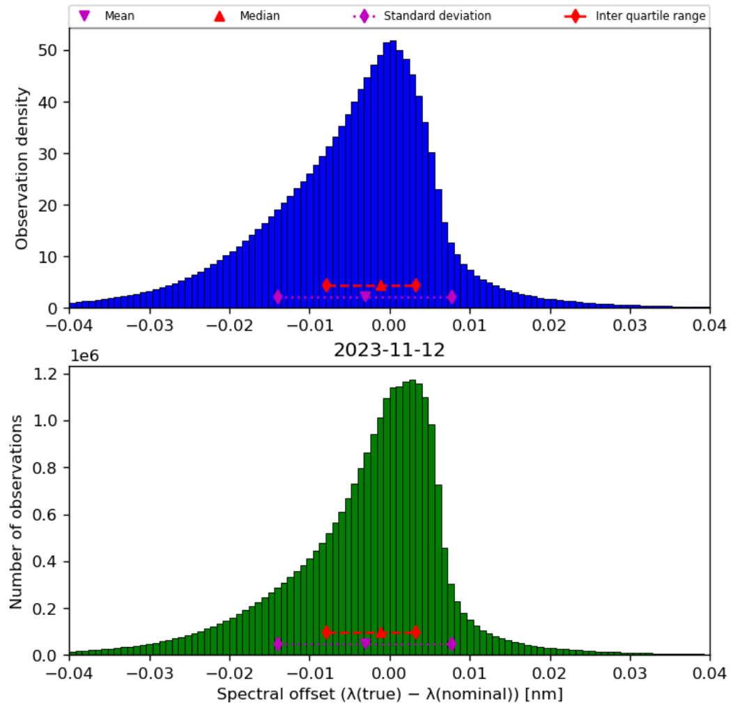
Figure 45: Histogram of “Spectral offset ( \lambda(\text{true}) - \lambda(\text{nominal}) )” for 2023-11-12 to 2023-11-13
