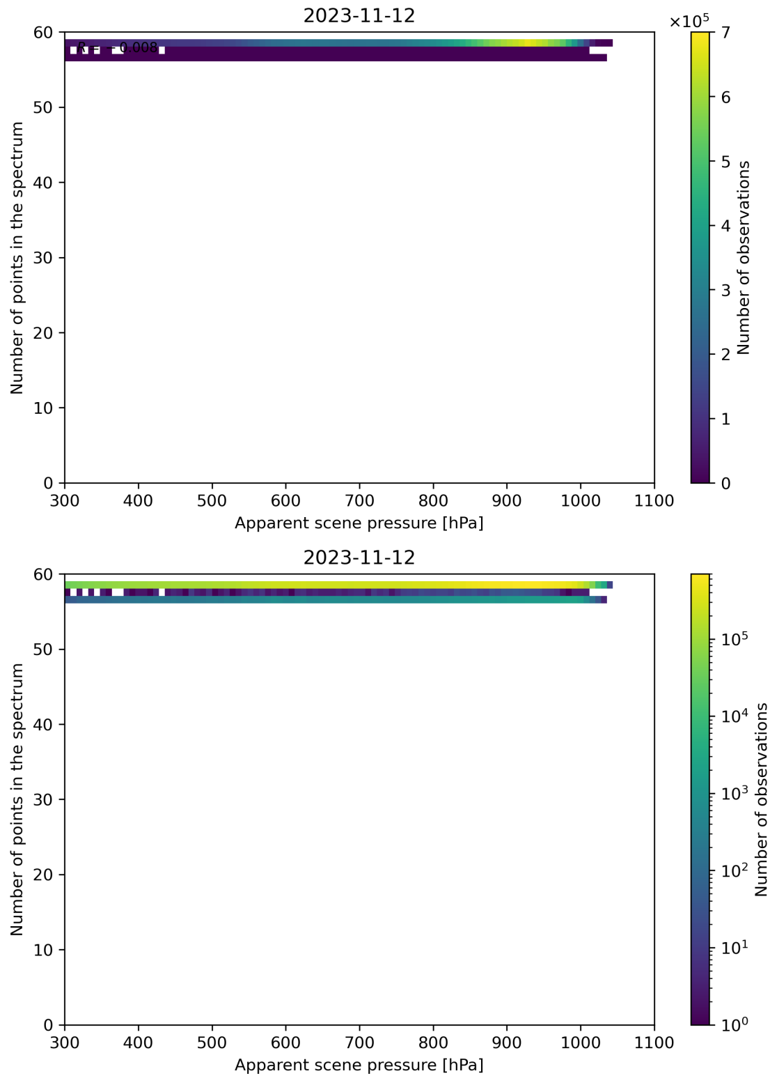
Figure 67: Scatter density plot of “Apparent scene pressure” against “Number of points in the spectrum” for 2023-11-12 to 2023-11-13.
