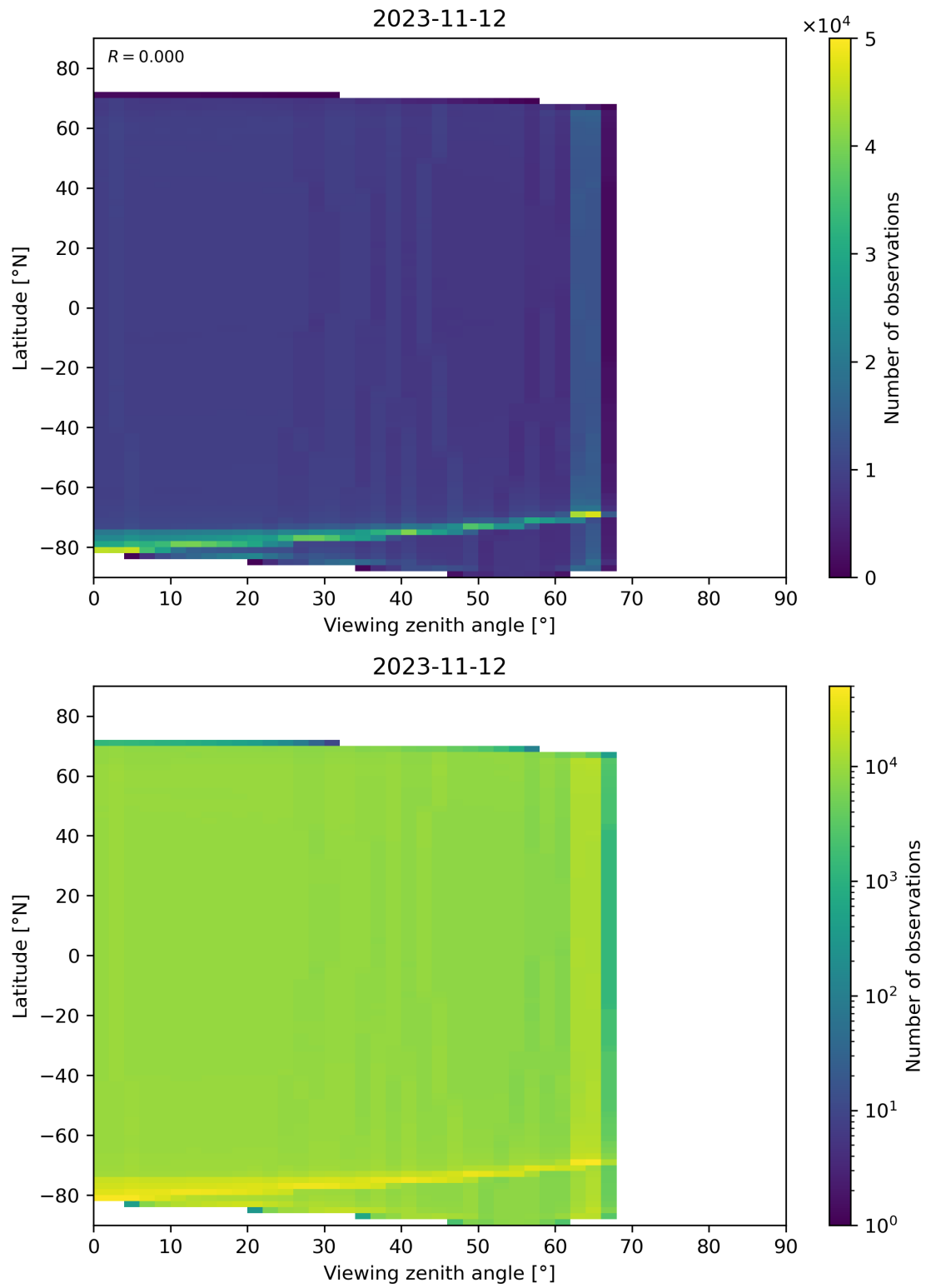
Figure 135: Scatter density plot of “Viewing zenith angle” against “Latitude” for 2023-11-12 to 2023-11-13.
