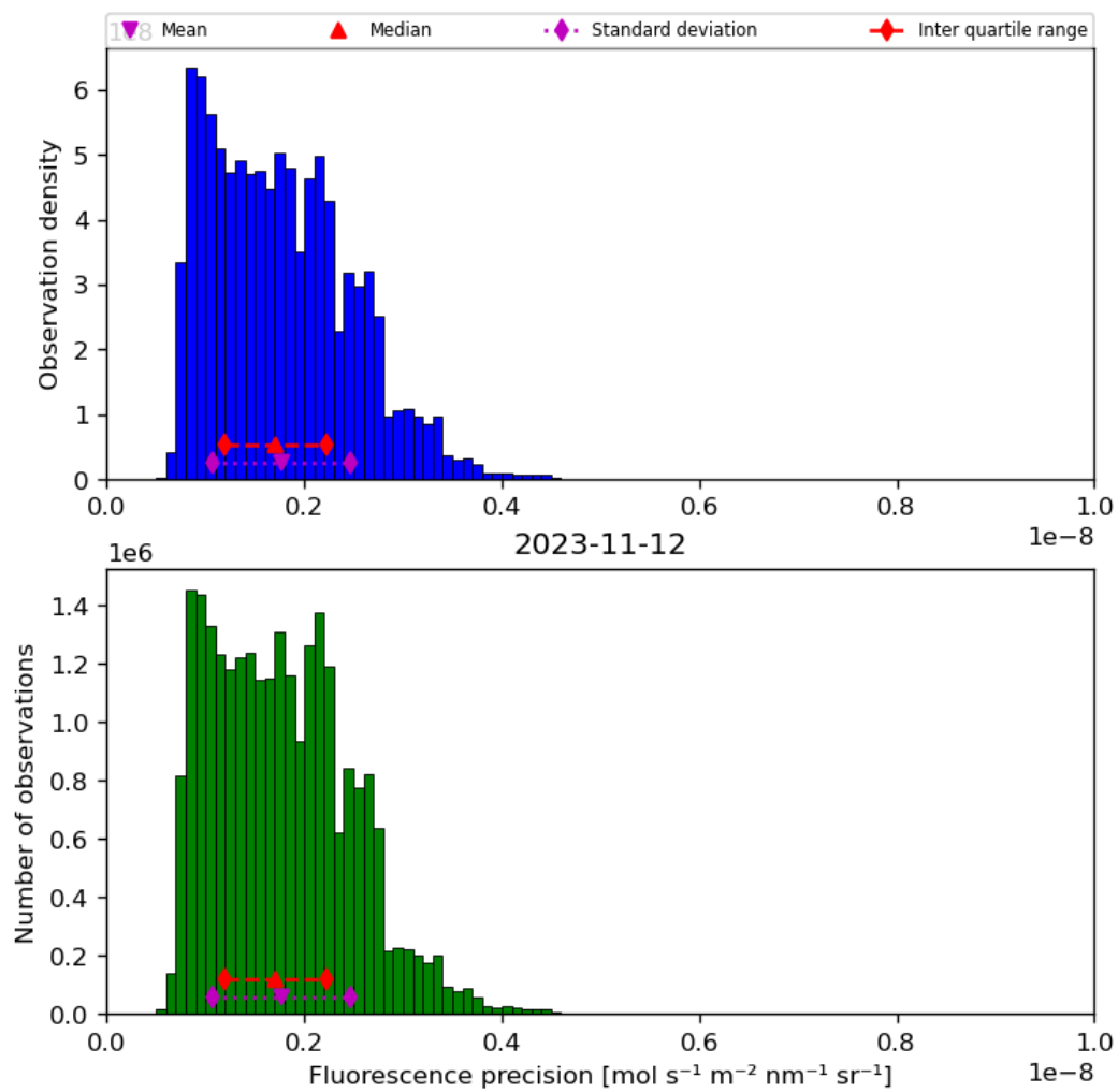
Figure 41: Histogram of “Fluorescence precision” for 2023-11-12 to 2023-11-13
