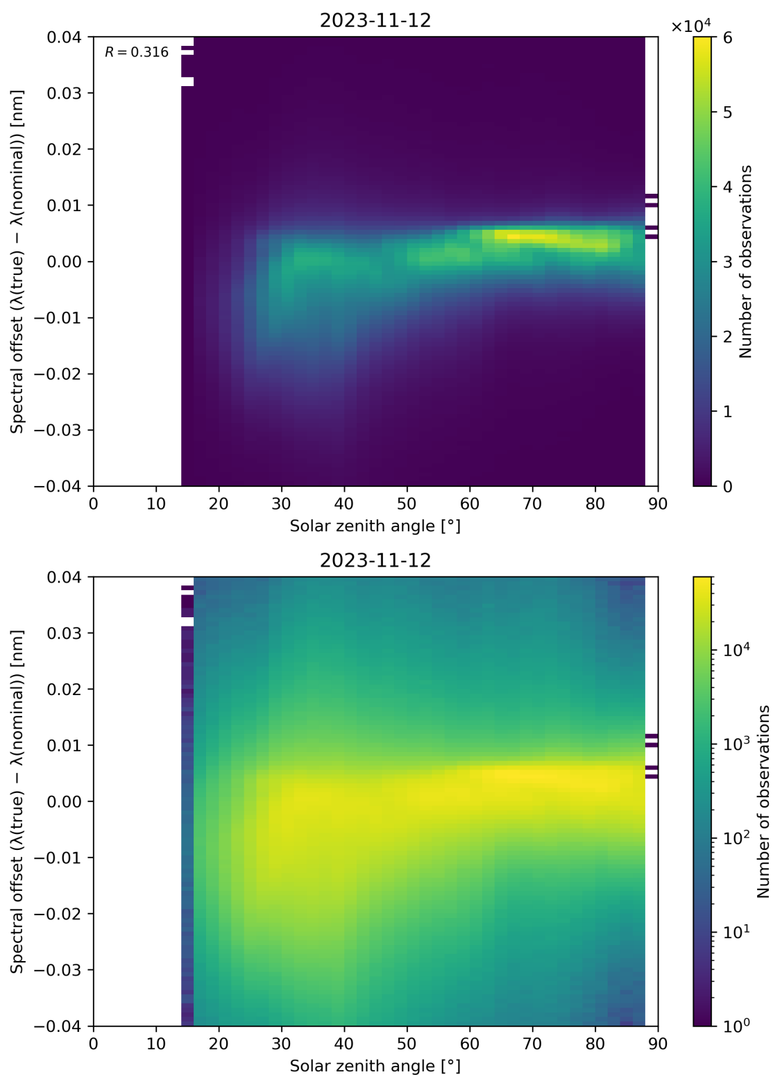
Figure 128: Scatter density plot of “Solar zenith angle” against “Spectral offset ( \lambda(\text{true}) - \lambda(\text{nominal}) )” for 2023-11-12 to 2023-11-13.
