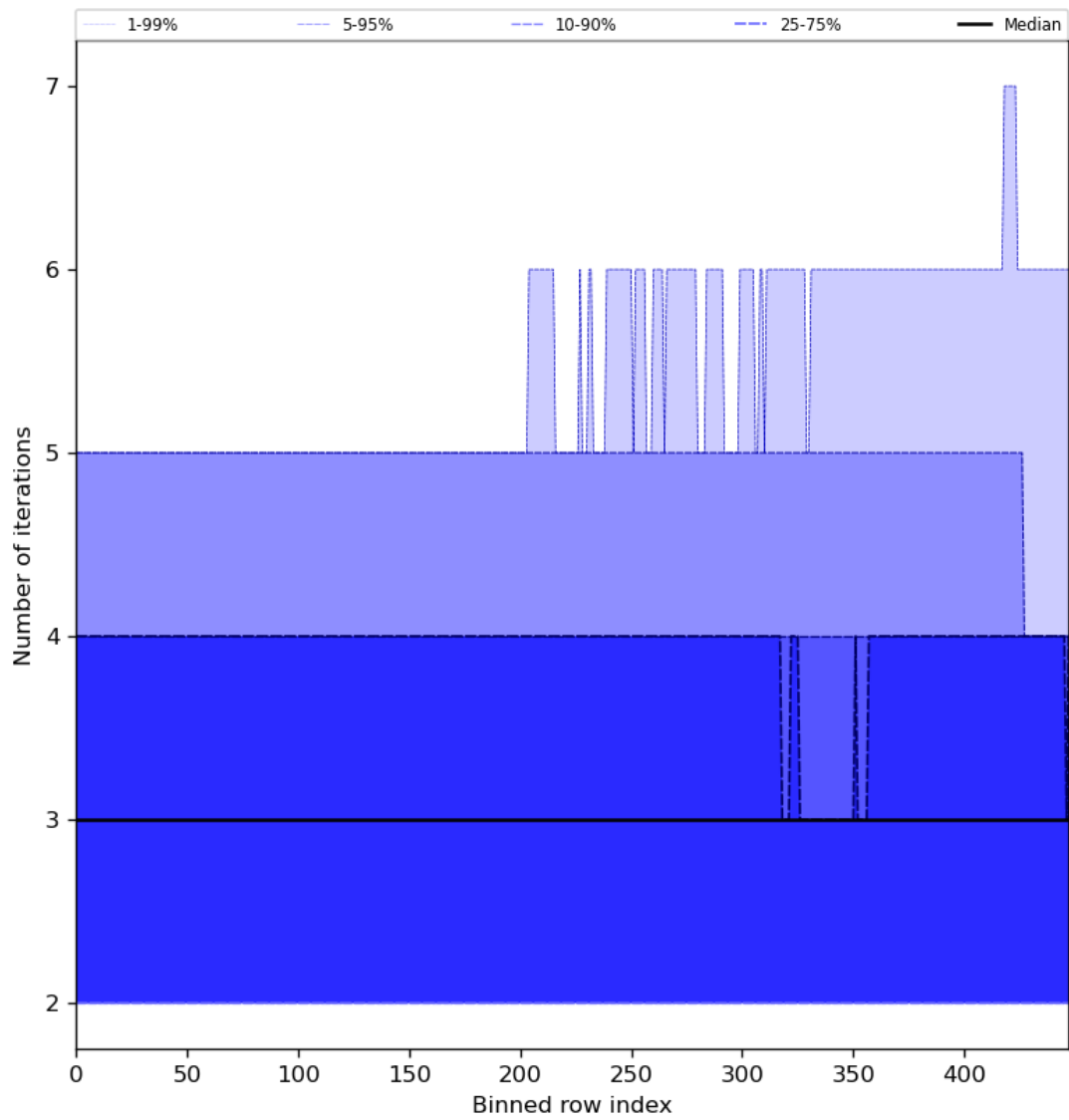
Figure 56: Along track statistics of “Number of iterations” for 2023-11-12 to 2023-11-13
