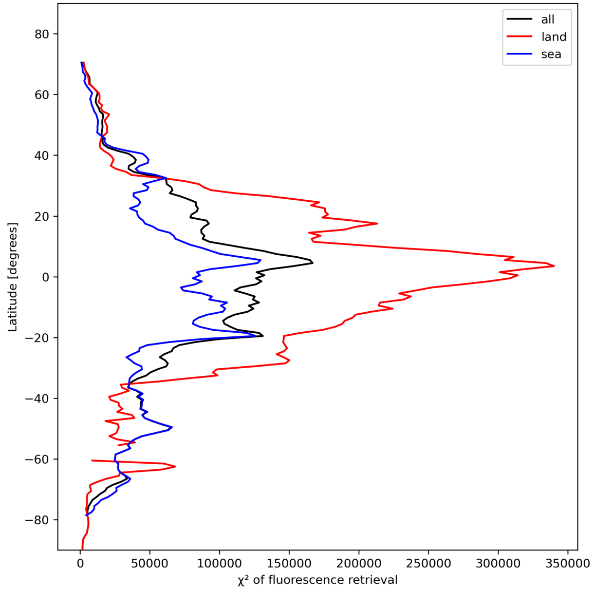
Figure 25: Zonal average of “ \chi^2 of fluorescence retrieval” for 2023-11-12 to 2023-11-13.
