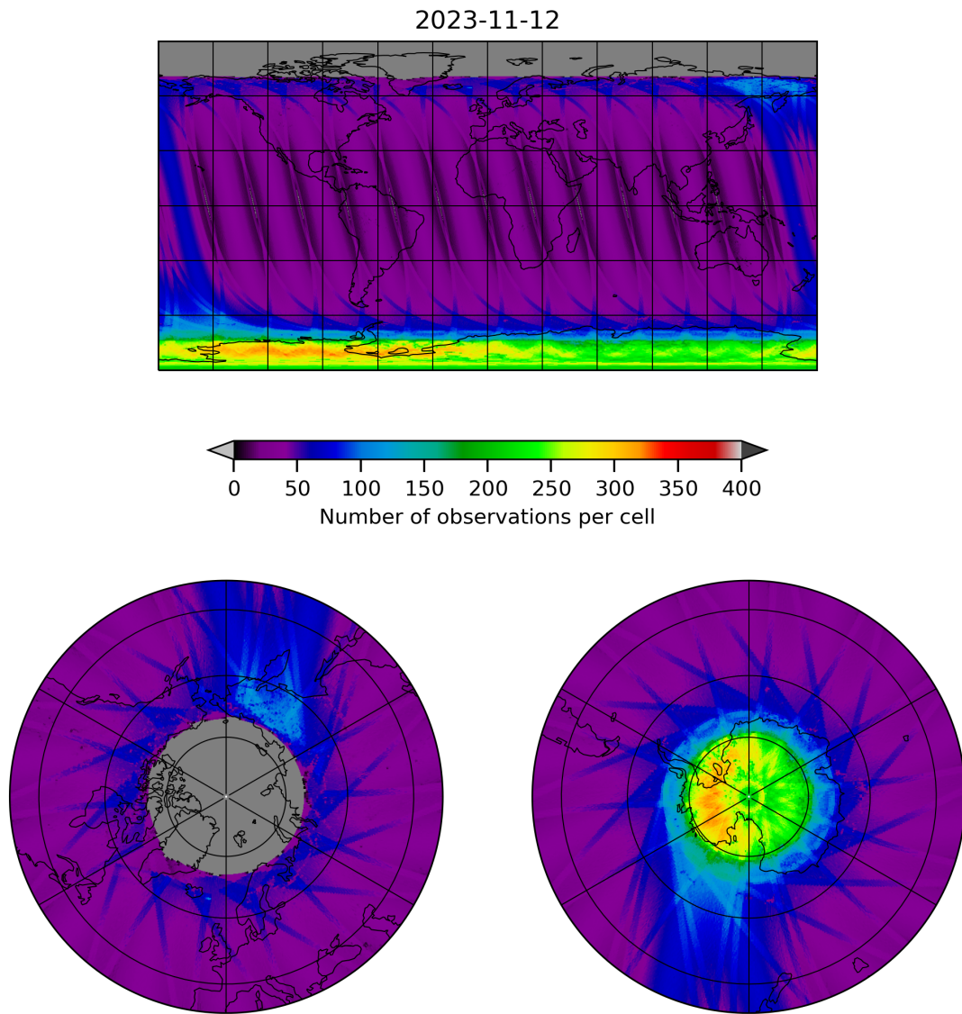
Figure 11: Map of the number of observations for 2023-11-12 to 2023-11-13
