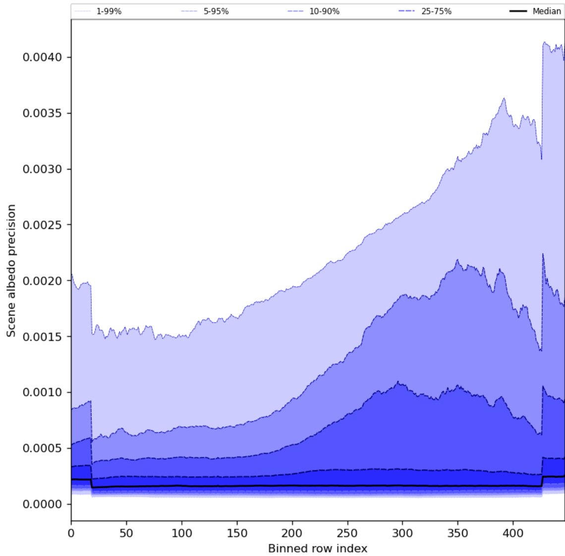
Figure 52: Along track statistics of “Scene albedo precision” for 2023-11-12 to 2023-11-13
