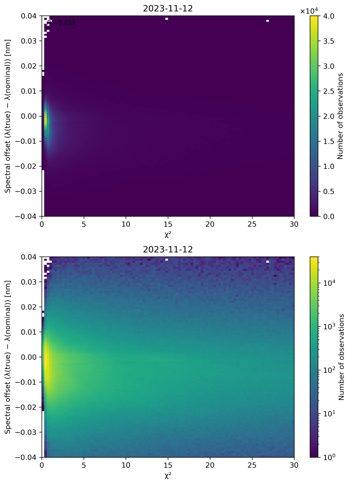
Figure 75: Scatter density plot of " \chi^2 " against "Spectral offset ( \lambda(\text{true}) - \lambda(\text{nominal}) )" for 2023-11-12 to 2023-11-13.
