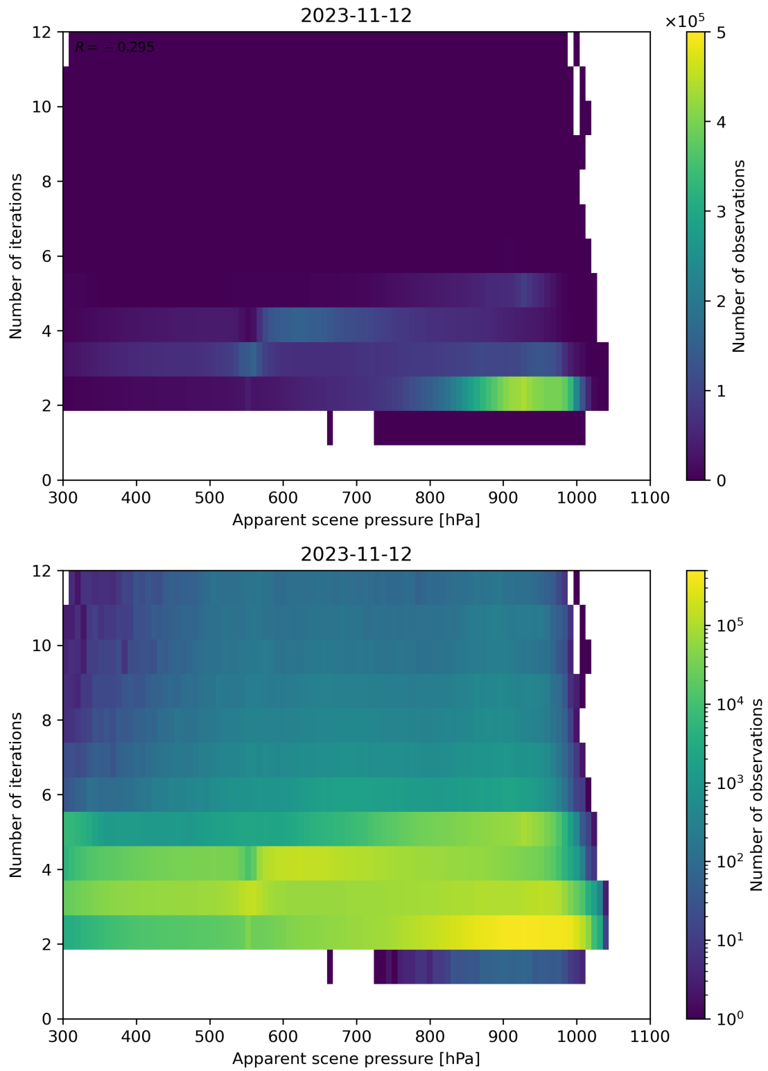
Figure 66: Scatter density plot of “Apparent scene pressure” against “Number of iterations” for 2023-11-12 to 2023-11-13.
