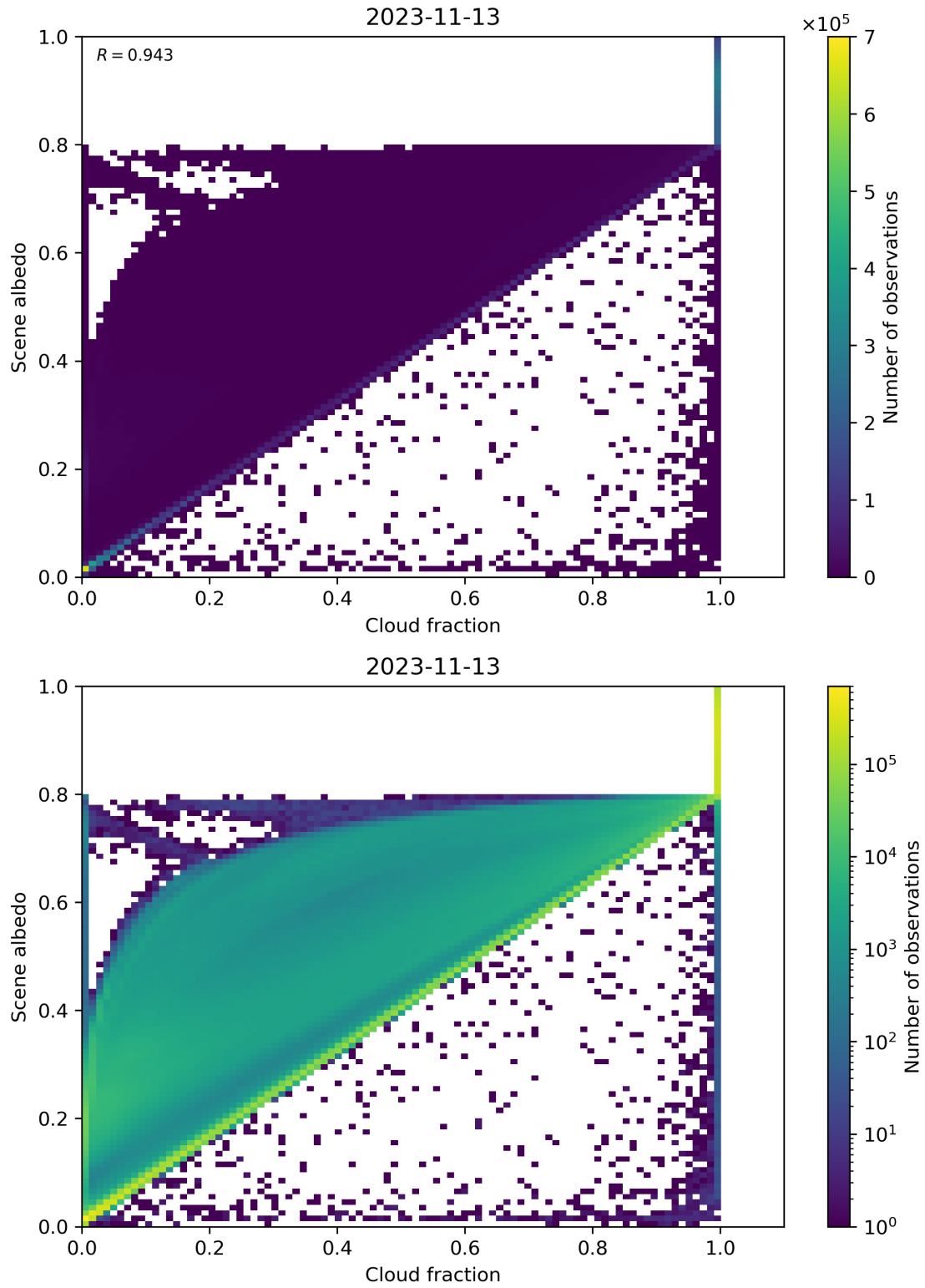
Figure 82: Scatter density plot of “Cloud fraction” against “Scene albedo” for 2023-11-13 to 2023-11-14.
