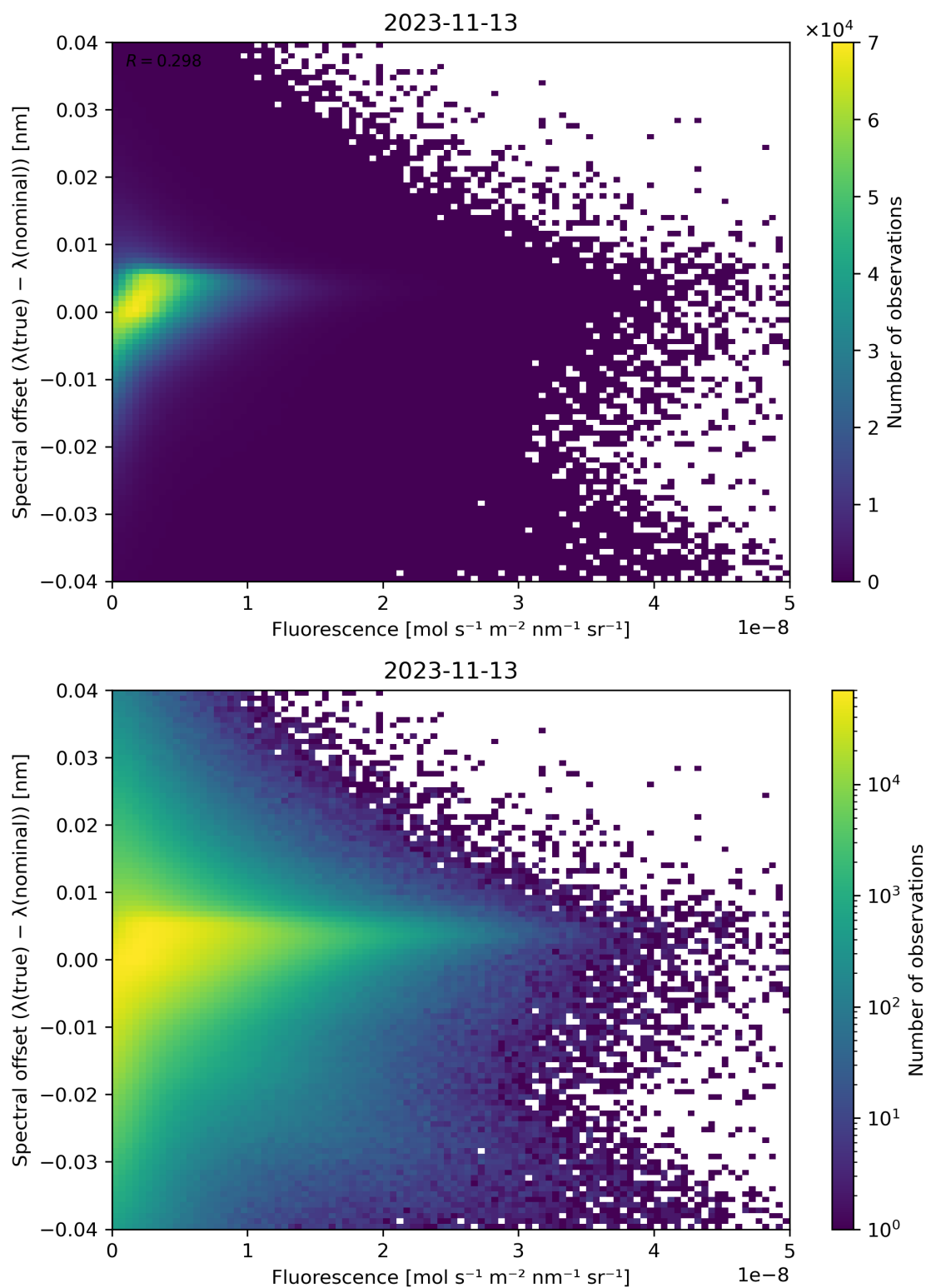
Figure 95: Scatter density plot of “Fluorescence” against “Spectral offset ( \lambda(\text{true}) - \lambda(\text{nominal}) )” for 2023-11-13 to 2023-11-14.
