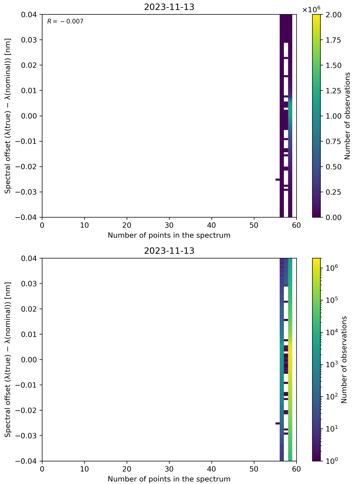
Figure 110: Scatter density plot of “Number of points in the spectrum” against “Spectral offset ( \lambda(\text{true}) - \lambda(\text{nominal}) )” for 2023-11-13 to 2023-11-14.
