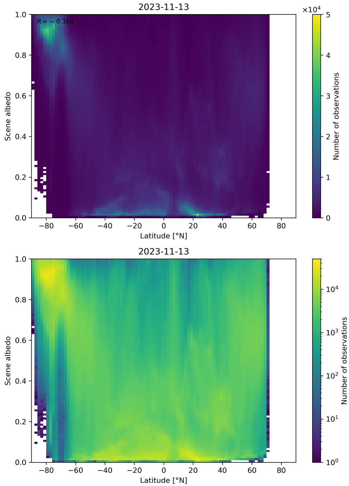
Figure 104: Scatter density plot of “Latitude” against “Scene albedo” for 2023-11-13 to 2023-11-14.
