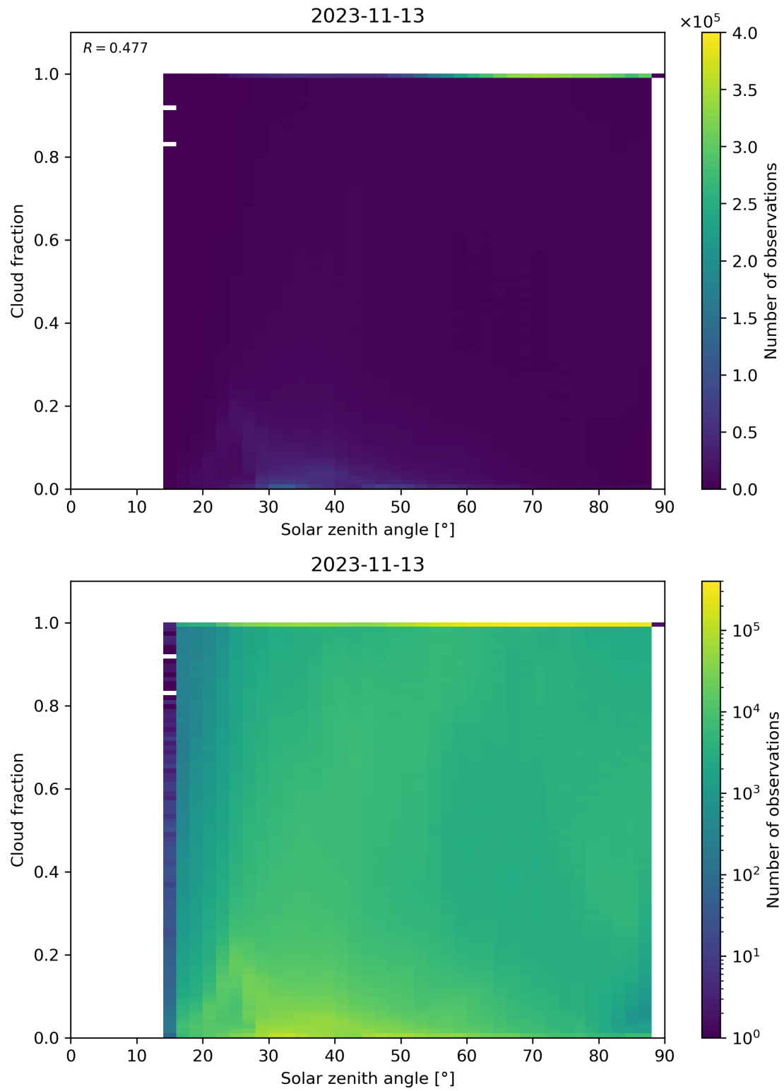
Figure 121: Scatter density plot of “Solar zenith angle” against “Cloud fraction” for 2023-11-13 to 2023-11-14.
