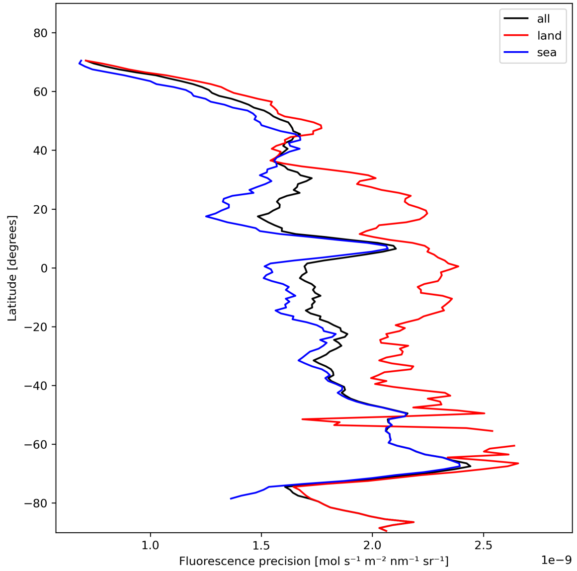
Figure 24: Zonal average of “Fluorescence precision” for 2023-11-13 to 2023-11-14.
