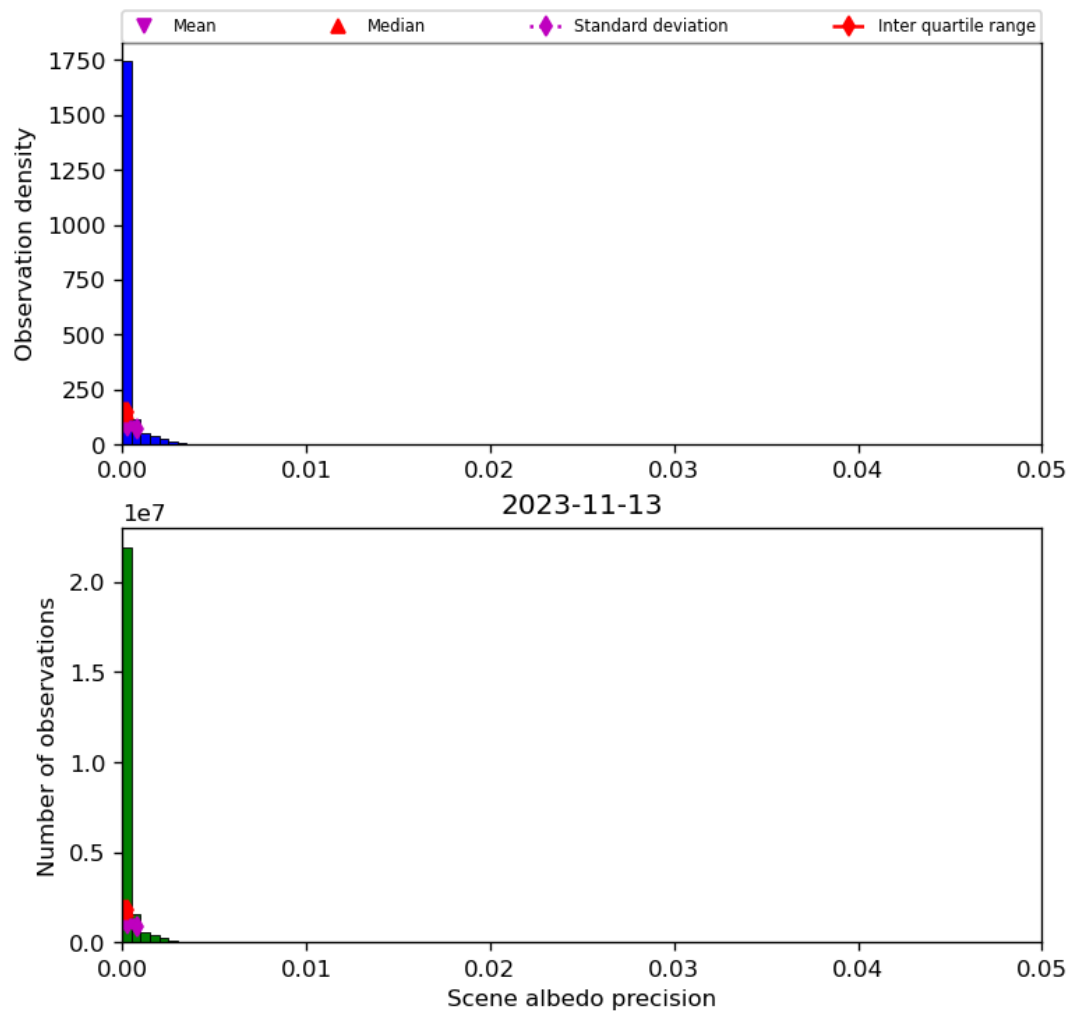
Figure 35: Histogram of “Scene albedo precision” for 2023-11-13 to 2023-11-14
