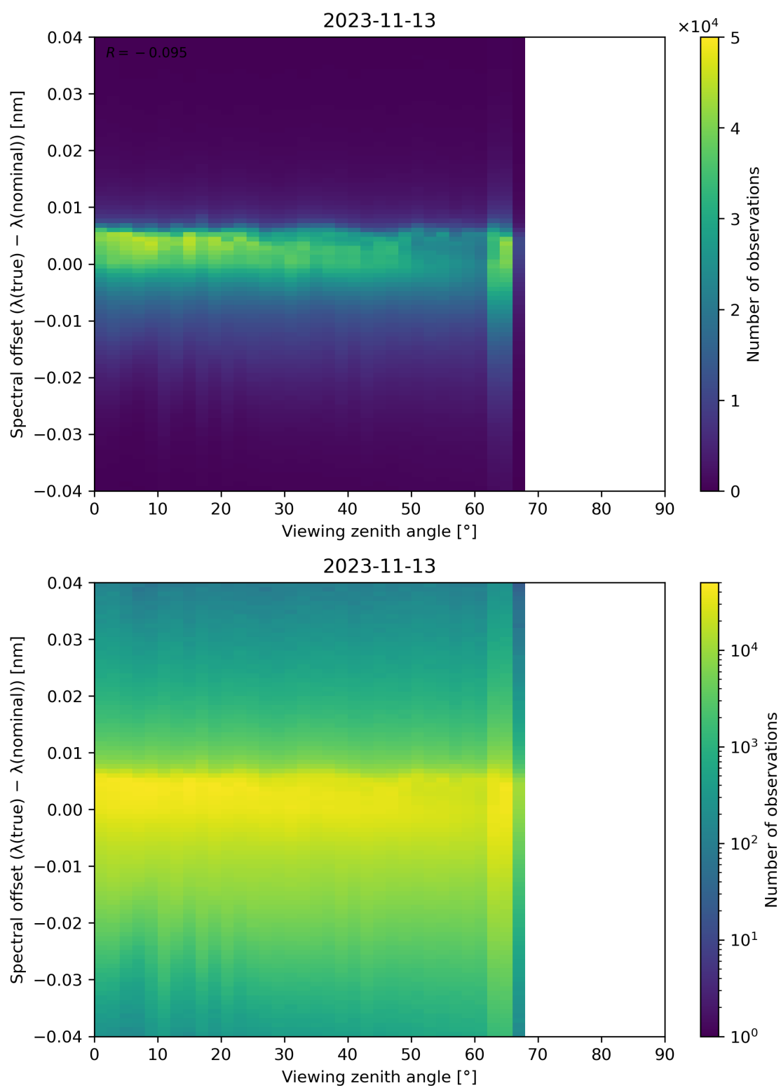
Figure 140: Scatter density plot of “Viewing zenith angle” against “Spectral offset ( \lambda(\text{true}) - \lambda(\text{nominal}) )” for 2023-11-13 to 2023-11-14.
