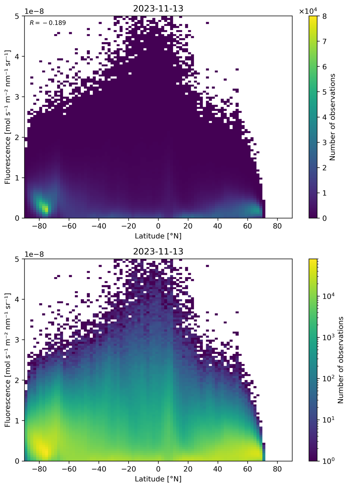
Figure 101: Scatter density plot of “Latitude” against “Fluorescence” for 2023-11-13 to 2023-11-14.
