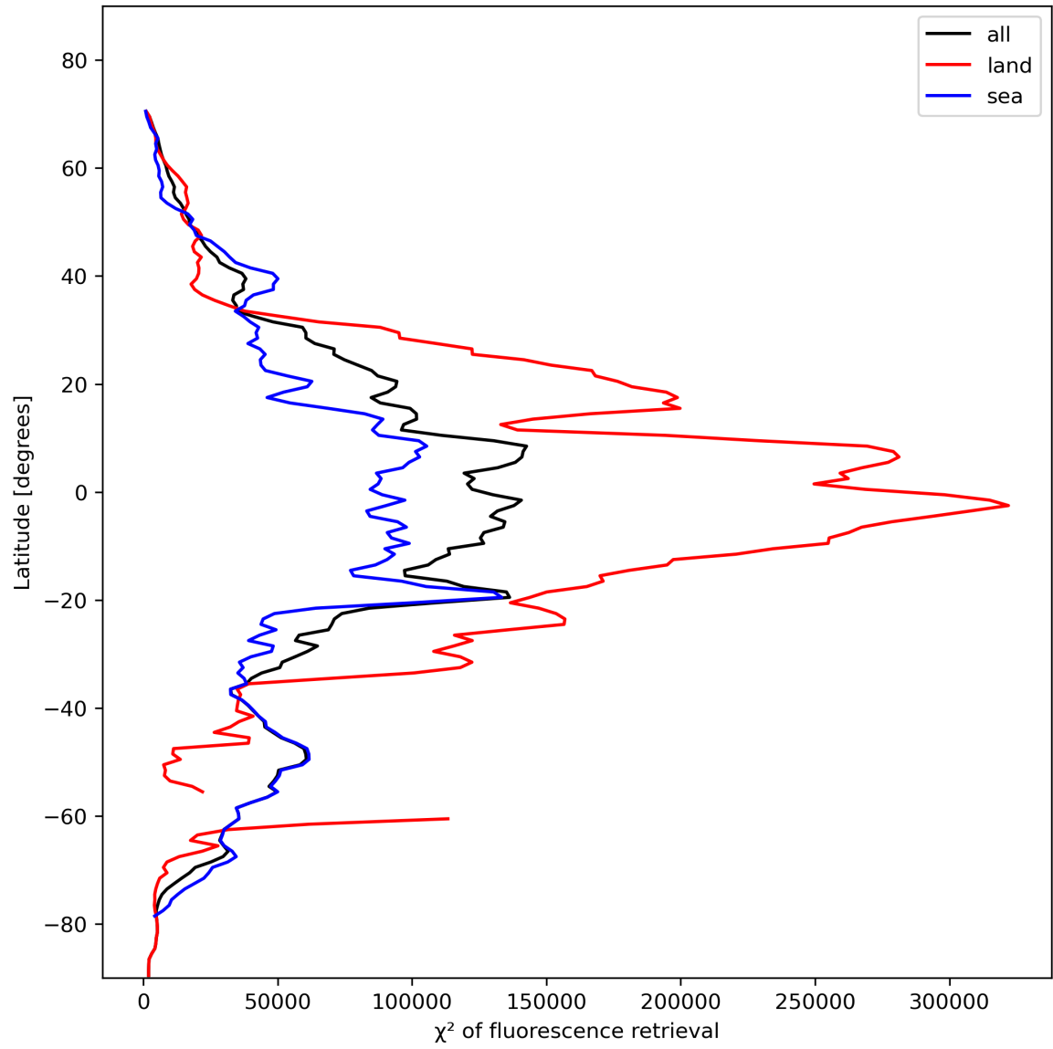
Figure 25: Zonal average of “ \chi^2 of fluorescence retrieval” for 2023-11-13 to 2023-11-14.
