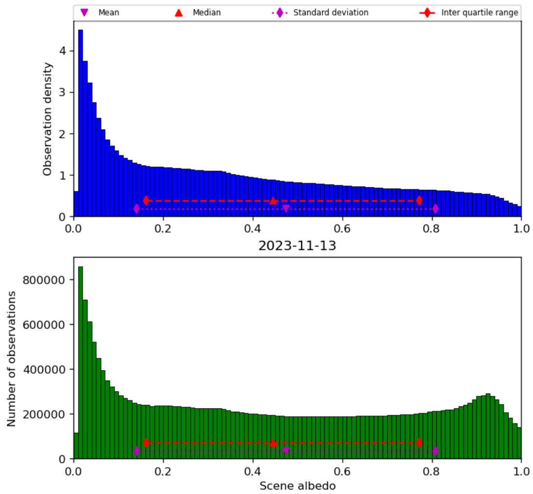
Figure 34: Histogram of “Scene albedo” for 2023-11-13 to 2023-11-14
