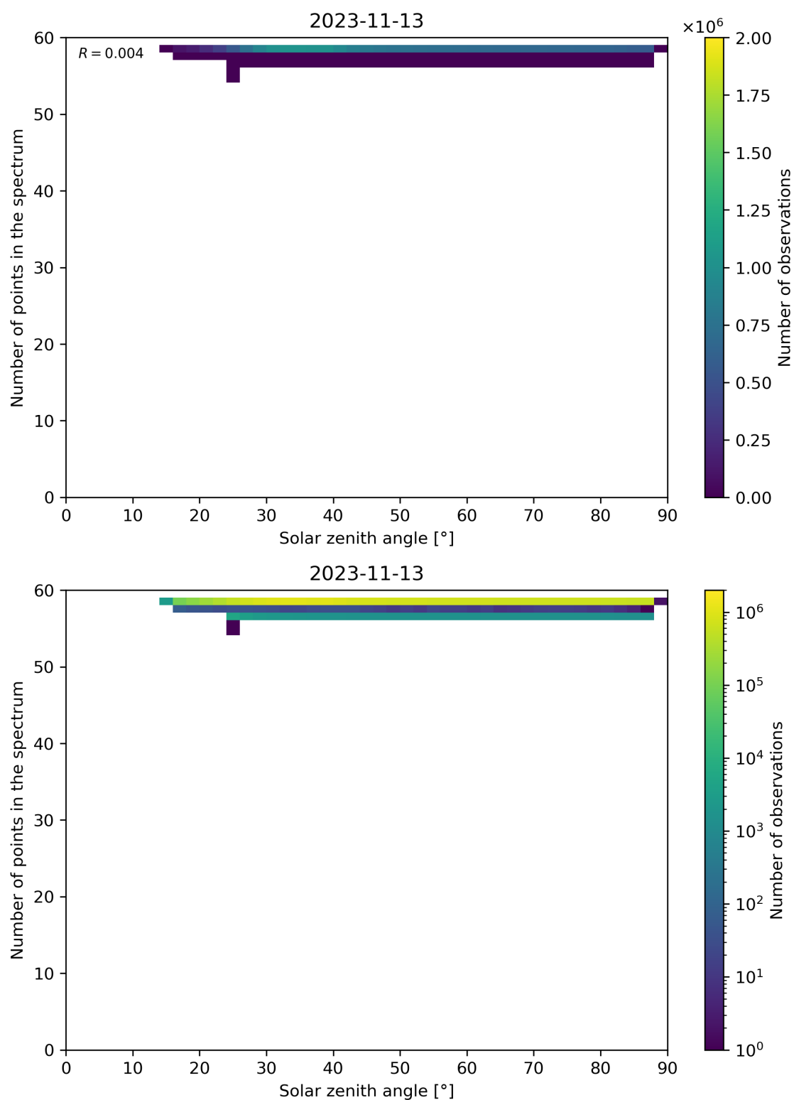
Figure 126: Scatter density plot of “Solar zenith angle” against “Number of points in the spectrum” for 2023-11-13 to 2023-11-14.
