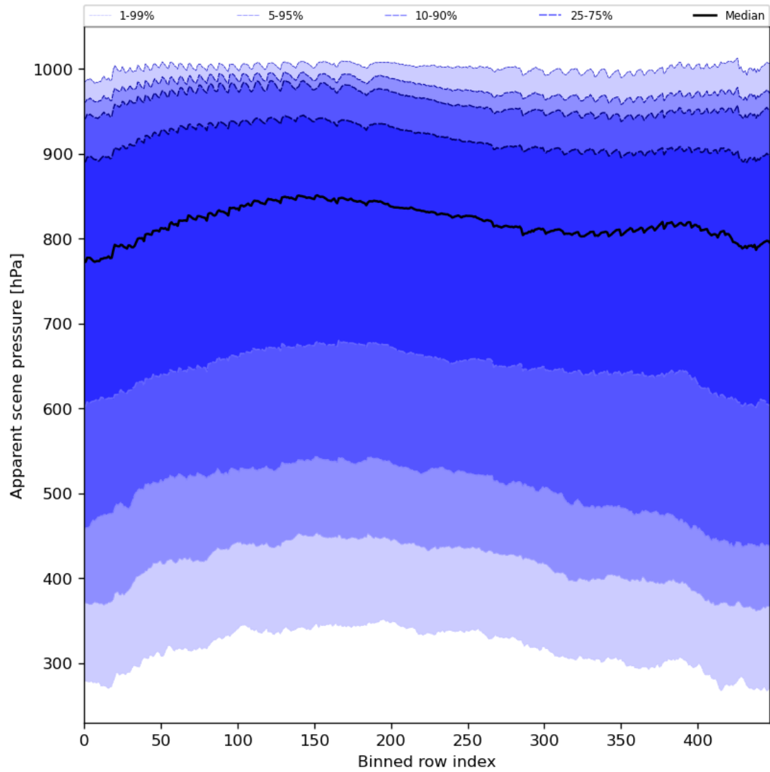
Figure 53: Along track statistics of “Apparent scene pressure” for 2023-11-13 to 2023-11-14
