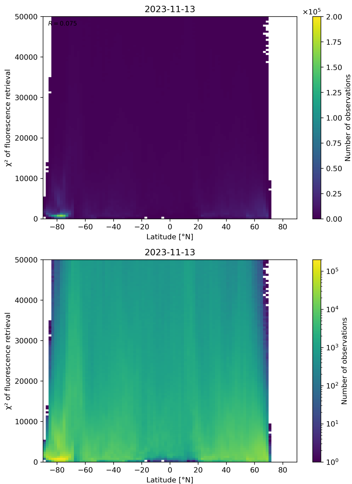
Figure 98: Scatter density plot of “Latitude” against “ \chi^2 of fluorescence retrieval” for 2023-11-13 to 2023-11-14.
