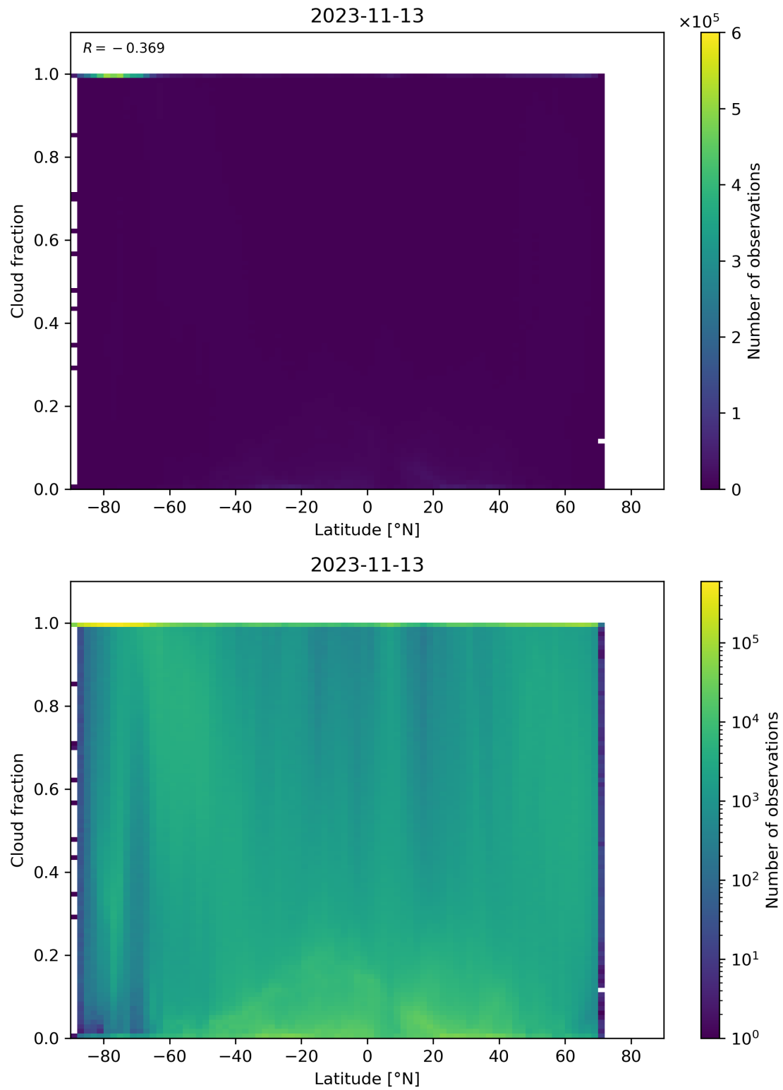
Figure 99: Scatter density plot of “Latitude” against “Cloud fraction” for 2023-11-13 to 2023-11-14.
