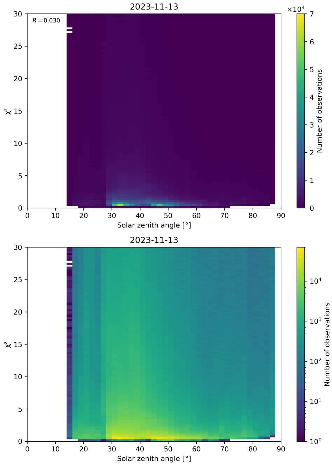
Figure 119: Scatter density plot of “Solar zenith angle” against “ \chi^2 ” for 2023-11-13 to 2023-11-14.
