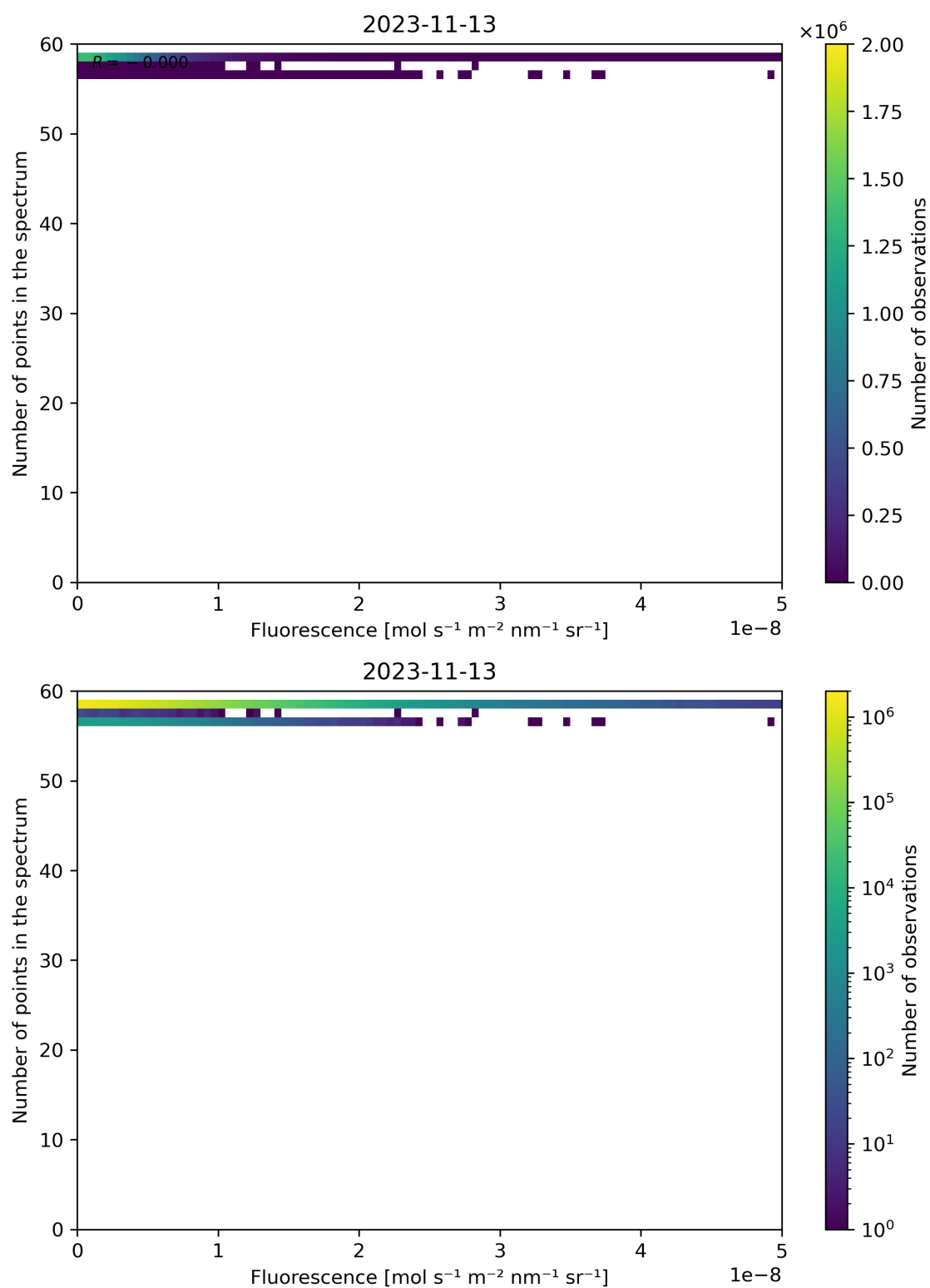
Figure 94: Scatter density plot of “Fluorescence” against “Number of points in the spectrum” for 2023-11-13 to 2023-11-14.
