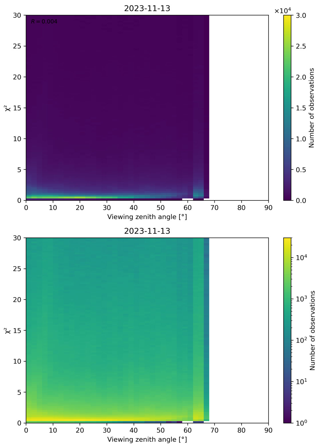
Figure 130: Scatter density plot of “Viewing zenith angle” against “ \chi^2 ” for 2023-11-13 to 2023-11-14.
