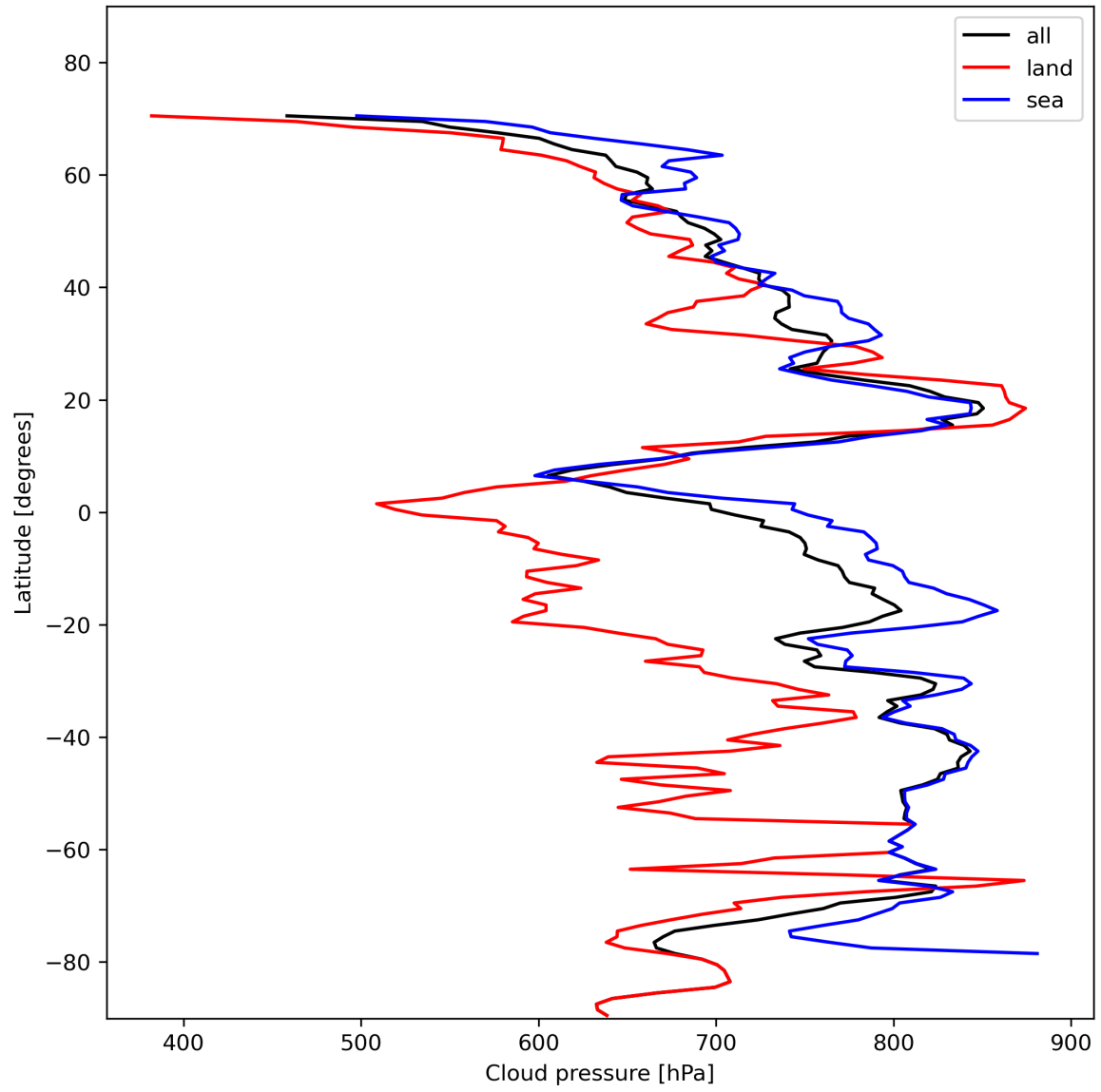
Figure 13: Zonal average of “Cloud pressure” for 2023-11-13 to 2023-11-14.
