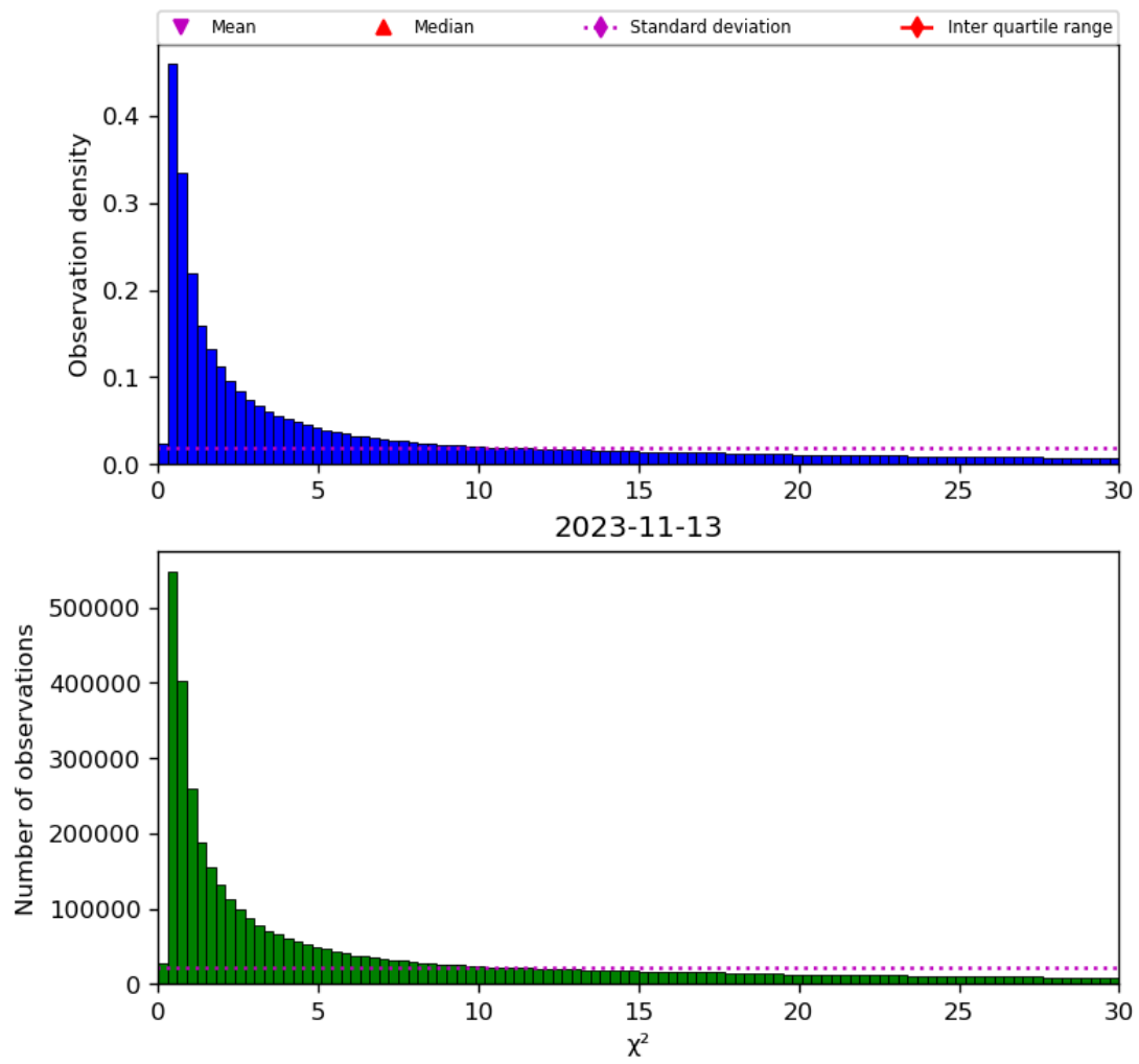
Figure 38: Histogram of “ \chi^2 ” for 2023-11-13 to 2023-11-14
