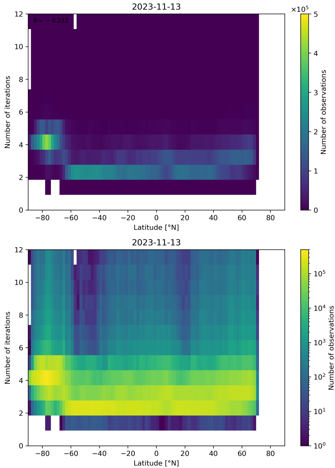
Figure 102: Scatter density plot of “Latitude” against “Number of iterations” for 2023-11-13 to 2023-11-14.
