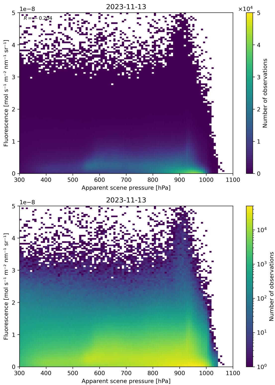
Figure 65: Scatter density plot of “Apparent scene pressure” against “Fluorescence” for 2023-11-13 to 2023-11-14.
