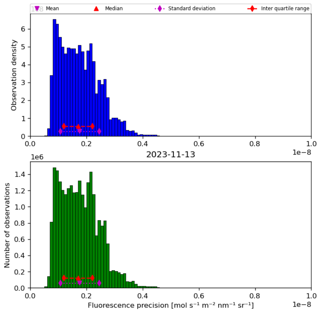
Figure 41: Histogram of “Fluorescence precision” for 2023-11-13 to 2023-11-14
