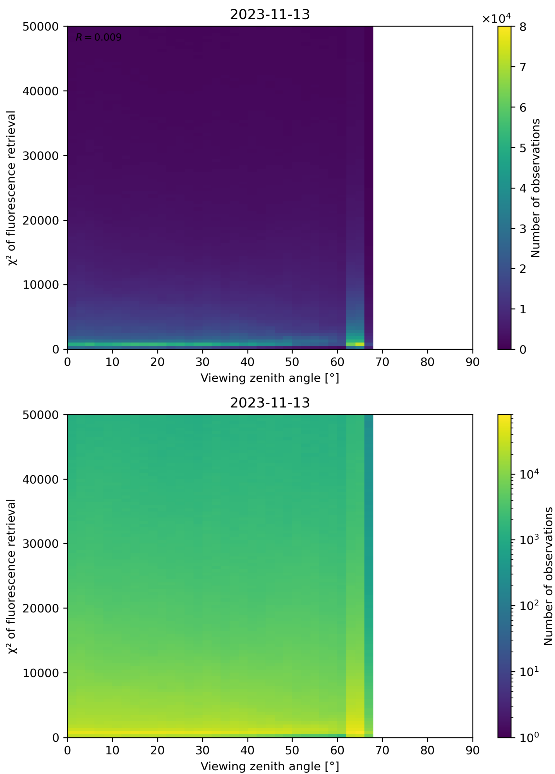
Figure 131: Scatter density plot of “Viewing zenith angle” against “ \chi^2 of fluorescence retrieval” for 2023-11-13 to 2023-11-14.
