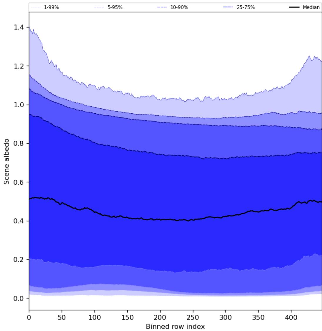
Figure 51: Along track statistics of “Scene albedo” for 2023-11-13 to 2023-11-14
