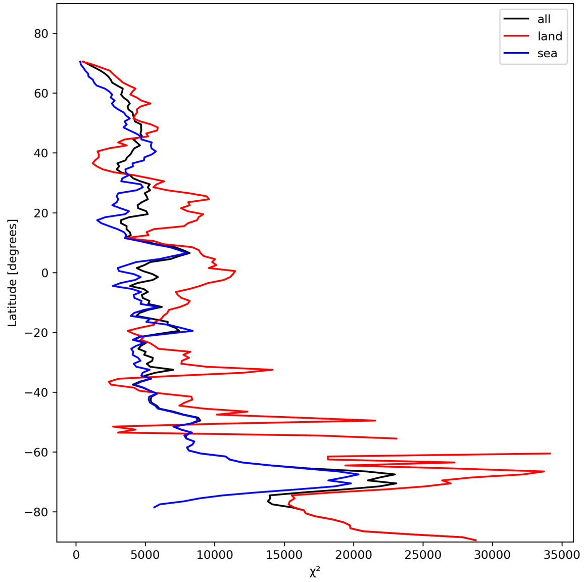
Figure 21: Zonal average of “ \chi^2 ” for 2023-11-13 to 2023-11-14.
