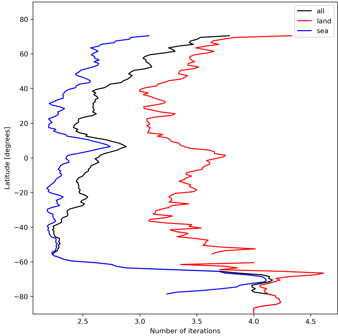
Figure 22: Zonal average of “Number of iterations” for 2023-11-13 to 2023-11-14.
