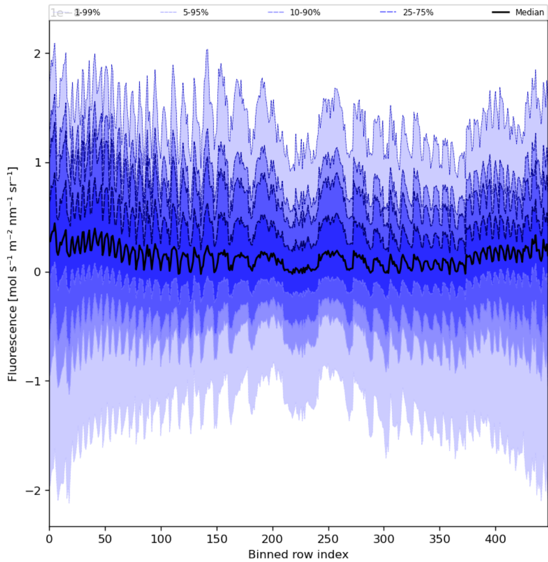
Figure 57: Along track statistics of “Fluorescence” for 2023-11-13 to 2023-11-14
