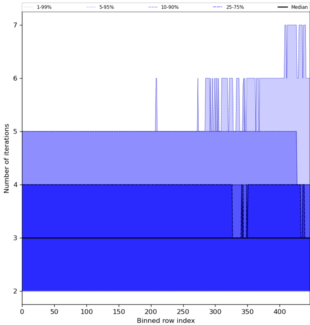
Figure 56: Along track statistics of “Number of iterations” for 2023-11-13 to 2023-11-14
