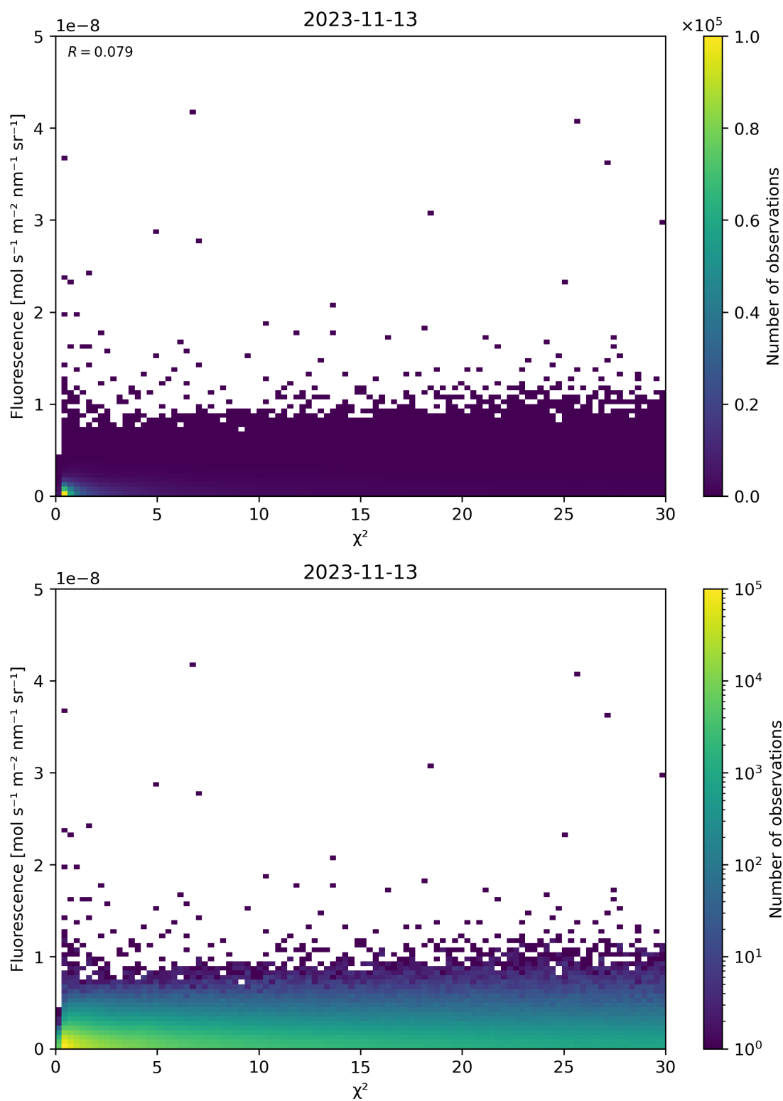
Figure 70: Scatter density plot of “ \chi^2 ” against “Fluorescence” for 2023-11-13 to 2023-11-14.
