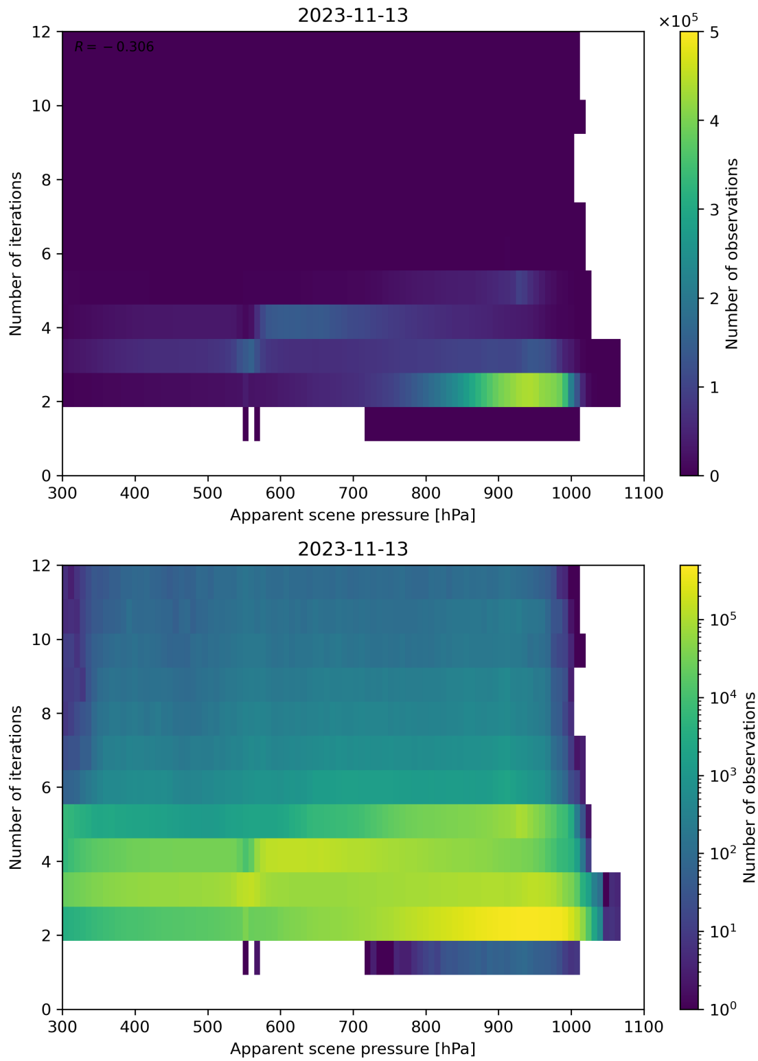
Figure 66: Scatter density plot of “Apparent scene pressure” against “Number of iterations” for 2023-11-13 to 2023-11-14.
