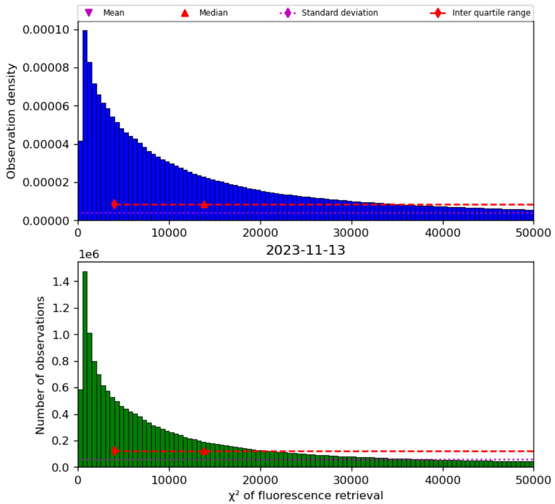
Figure 42: Histogram of “ \chi^2 of fluorescence retrieval” for 2023-11-13 to 2023-11-14
