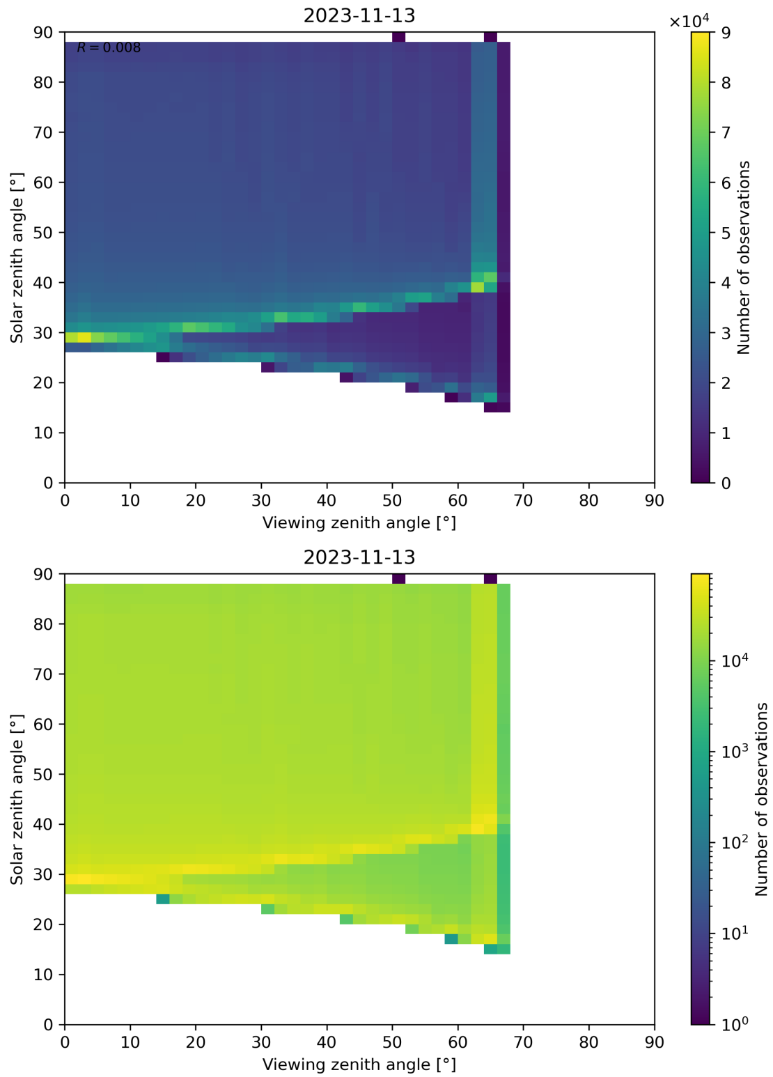
Figure 139: Scatter density plot of “Viewing zenith angle” against “Solar zenith angle” for 2023-11-13 to 2023-11-14.
