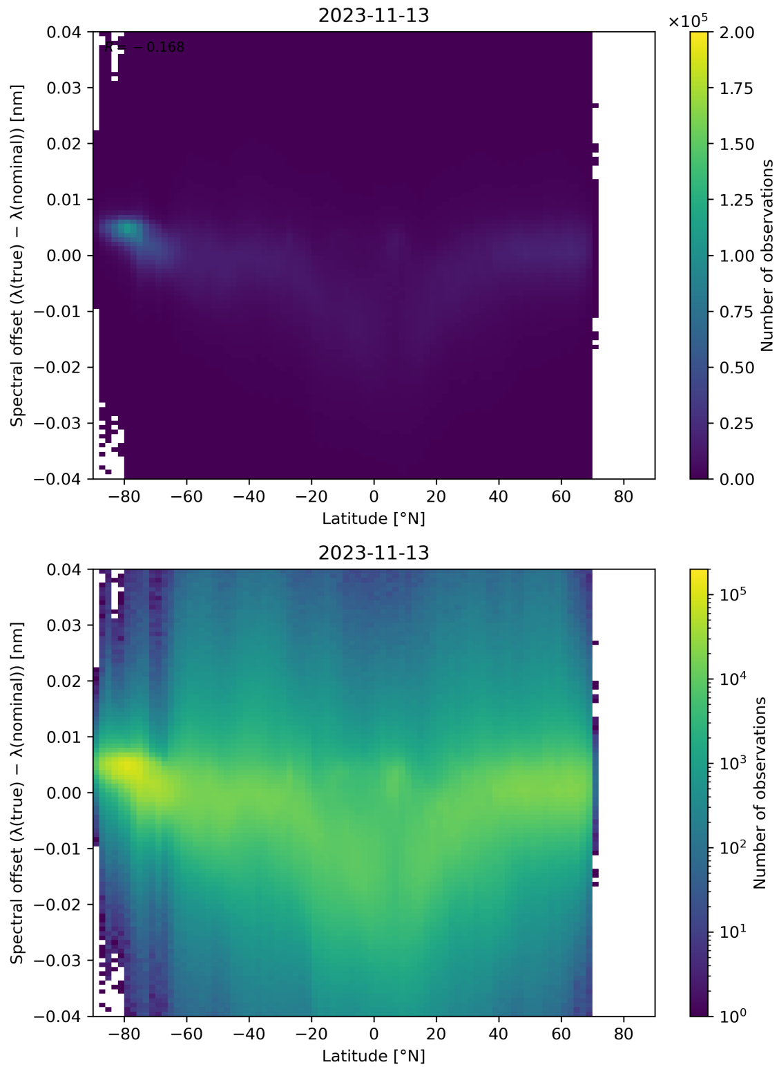
Figure 105: Scatter density plot of “Latitude” against “Spectral offset ( \lambda(\text{true}) - \lambda(\text{nominal}) )” for 2023-11-13 to 2023-11-14.
