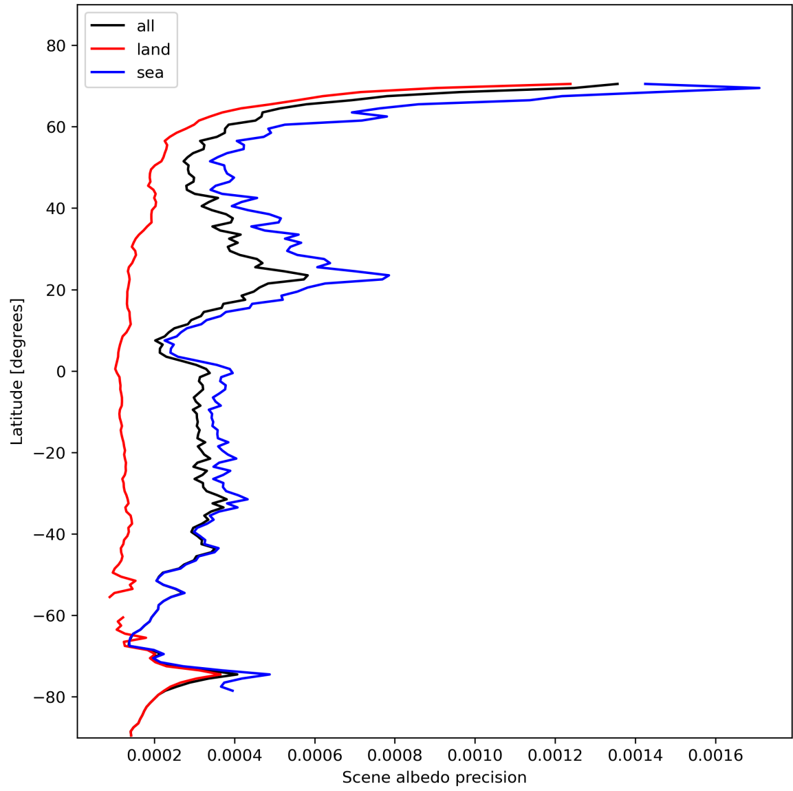
Figure 18: Zonal average of "Scene albedo precision" for 2023-11-13 to 2023-11-14.
