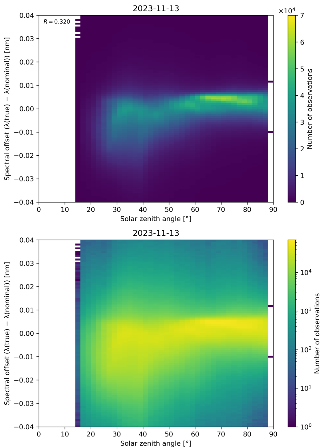
Figure 128: Scatter density plot of “Solar zenith angle” against “Spectral offset ( \lambda(\text{true}) - \lambda(\text{nominal}) )” for 2023-11-13 to 2023-11-14.
