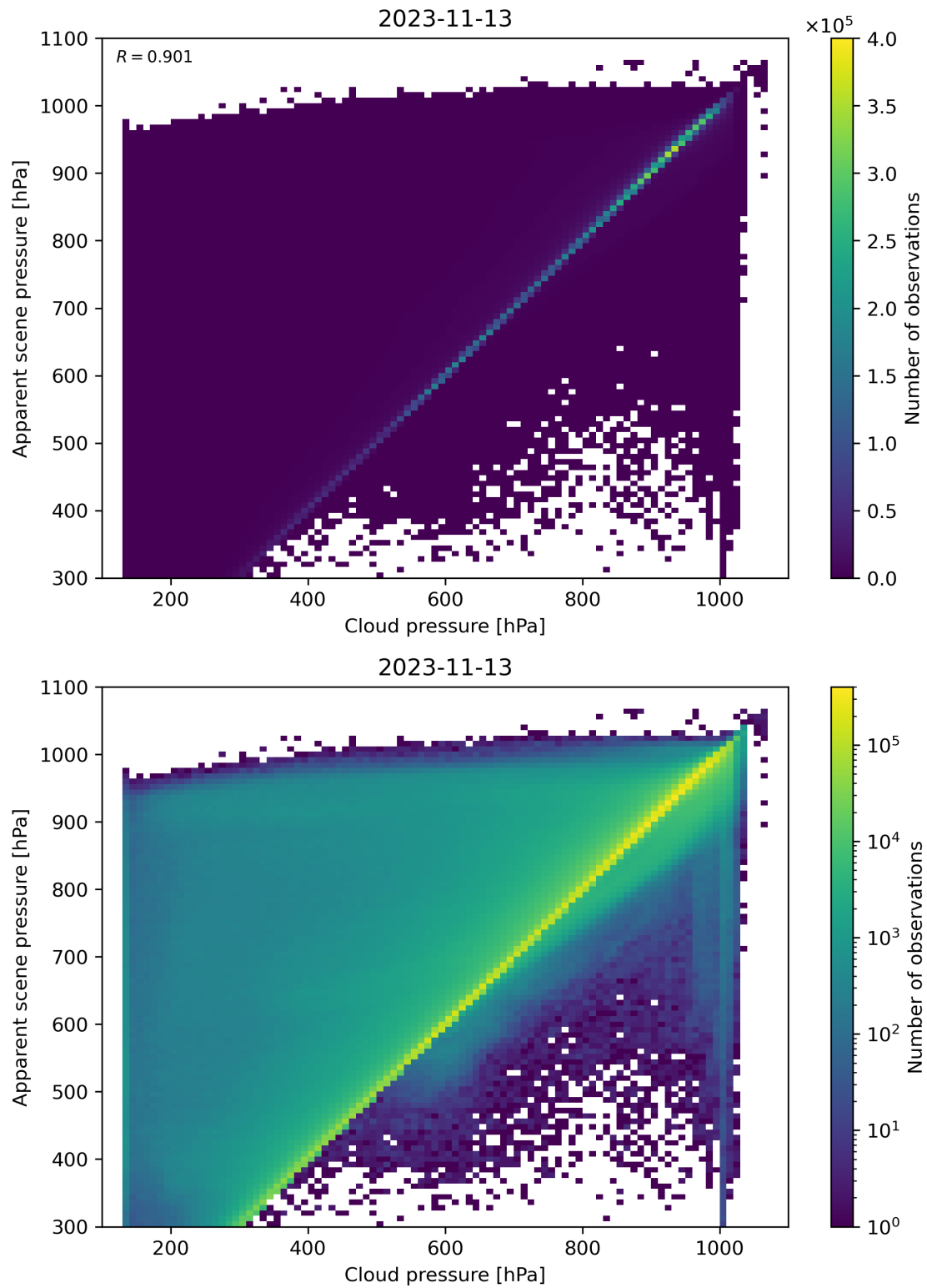
Figure 84: Scatter density plot of “Cloud pressure” against “Apparent scene pressure” for 2023-11-13 to 2023-11-14.
