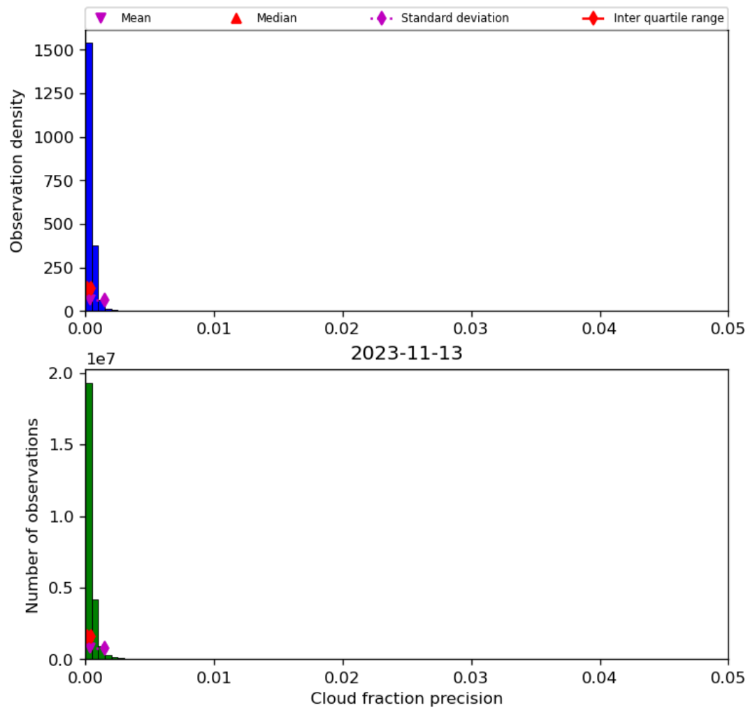
Figure 33: Histogram of “Cloud fraction precision” for 2023-11-13 to 2023-11-14
