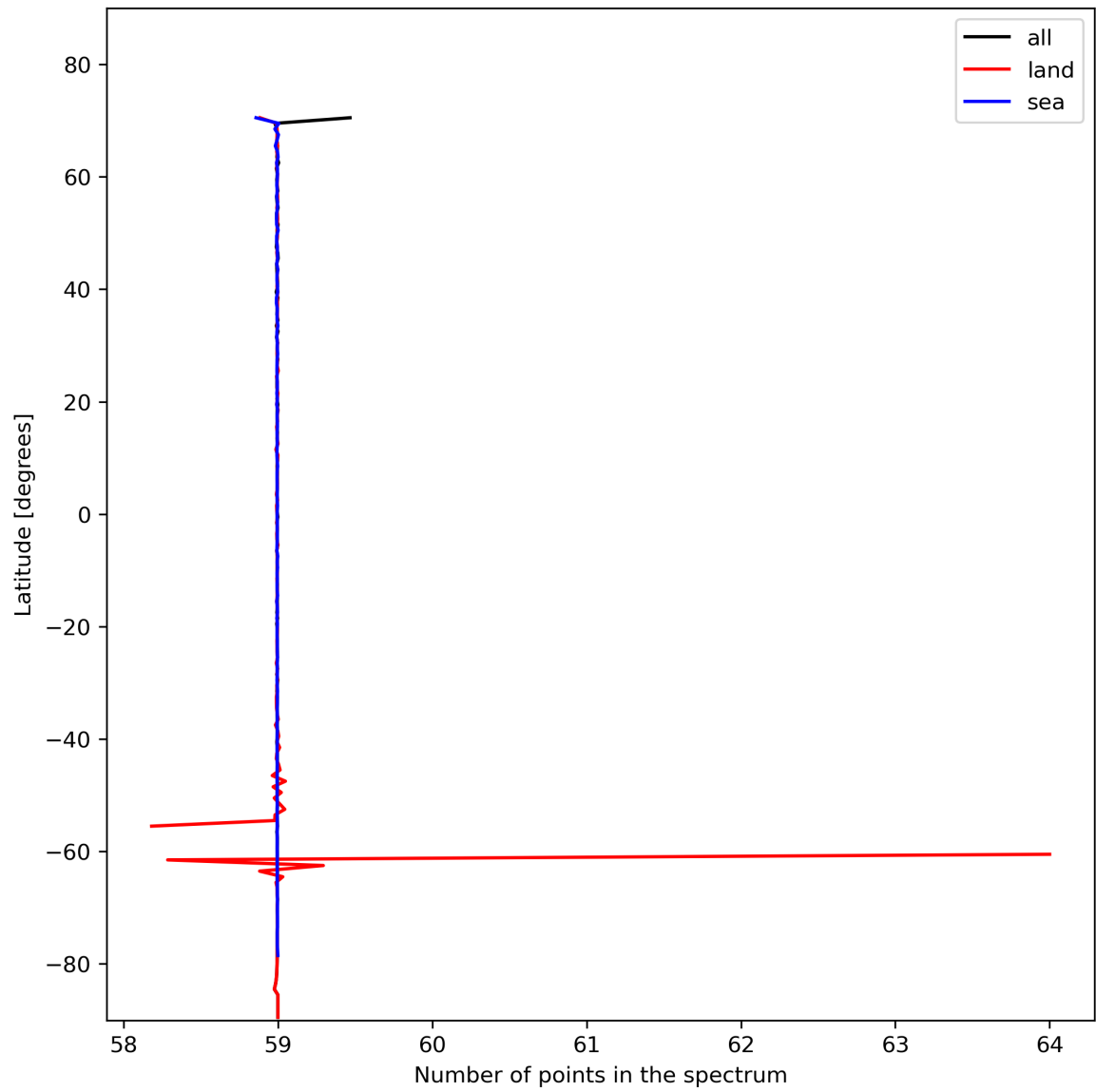
Figure 27: Zonal average of “Number of points in the spectrum” for 2023-11-13 to 2023-11-14.
