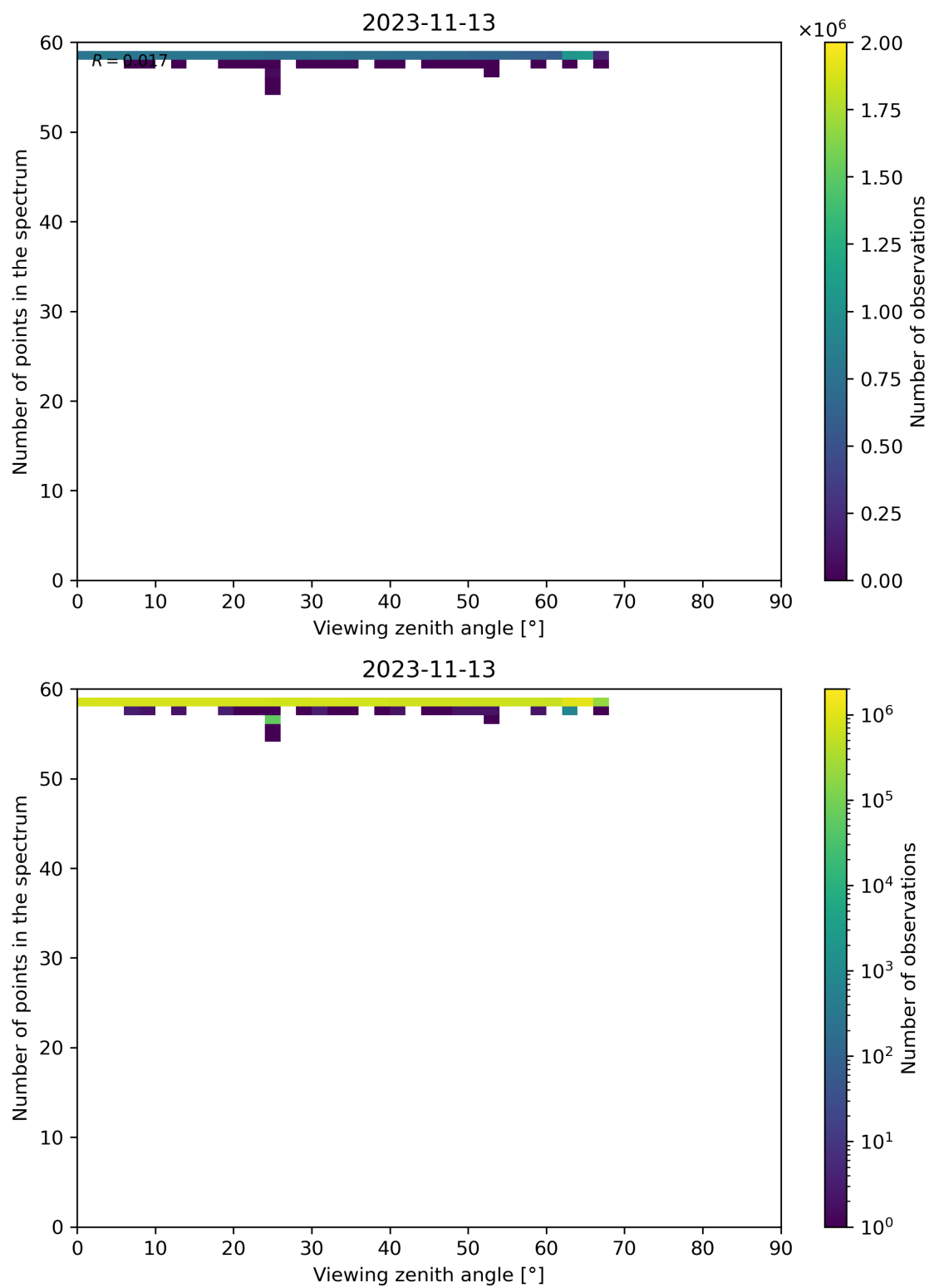
Figure 137: Scatter density plot of “Viewing zenith angle” against “Number of points in the spectrum” for 2023-11-13 to 2023-11-14.
