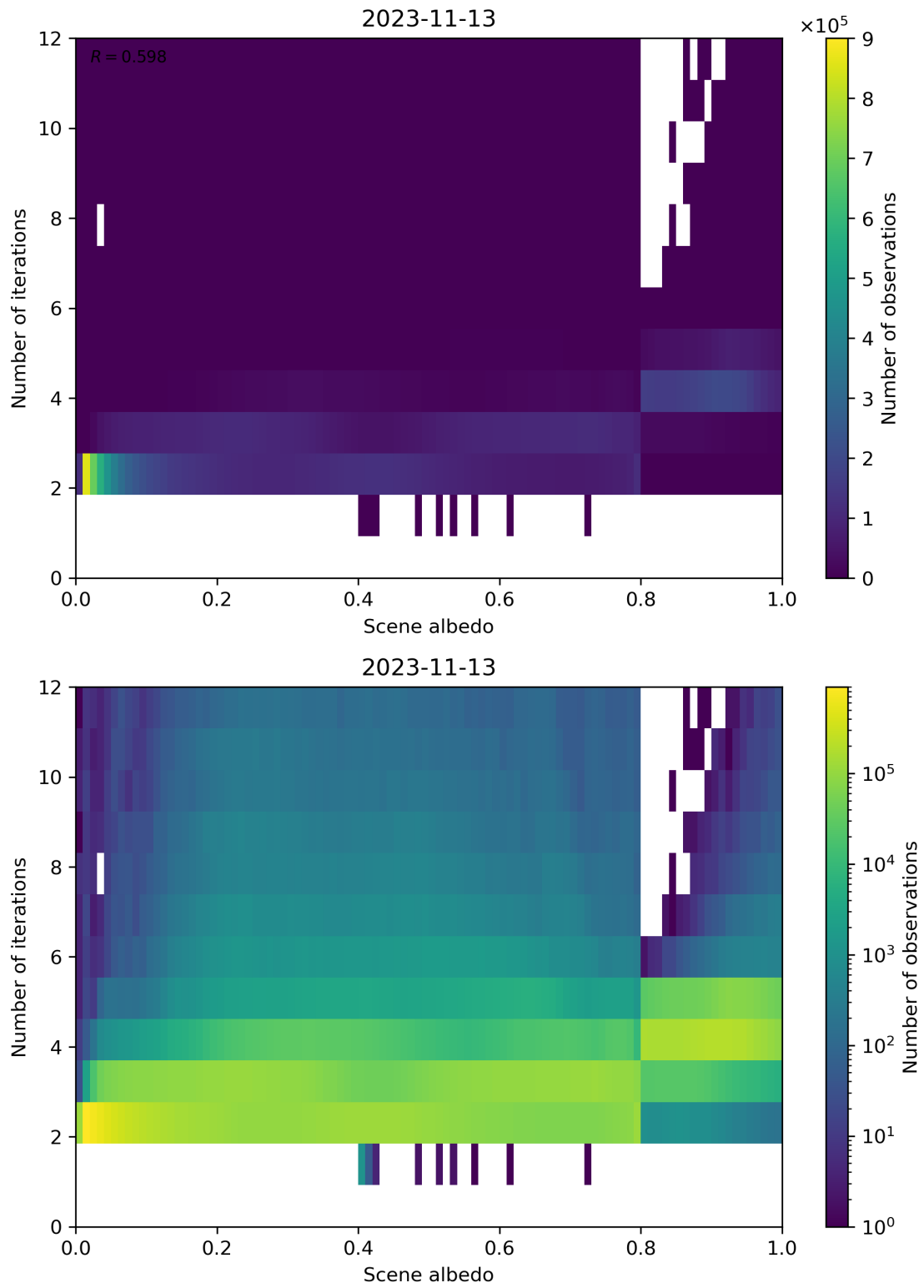
Figure 115: Scatter density plot of “Scene albedo” against “Number of iterations” for 2023-11-13 to 2023-11-14.
