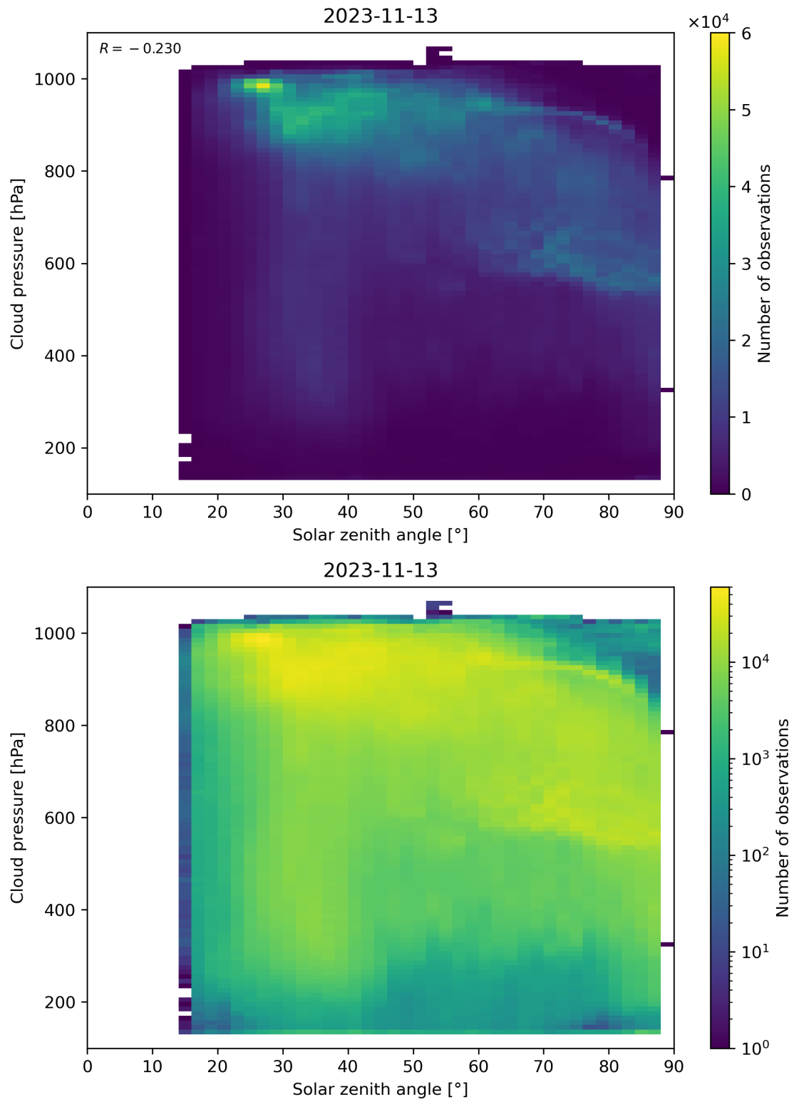
Figure 122: Scatter density plot of “Solar zenith angle” against “Cloud pressure” for 2023-11-13 to 2023-11-14.
