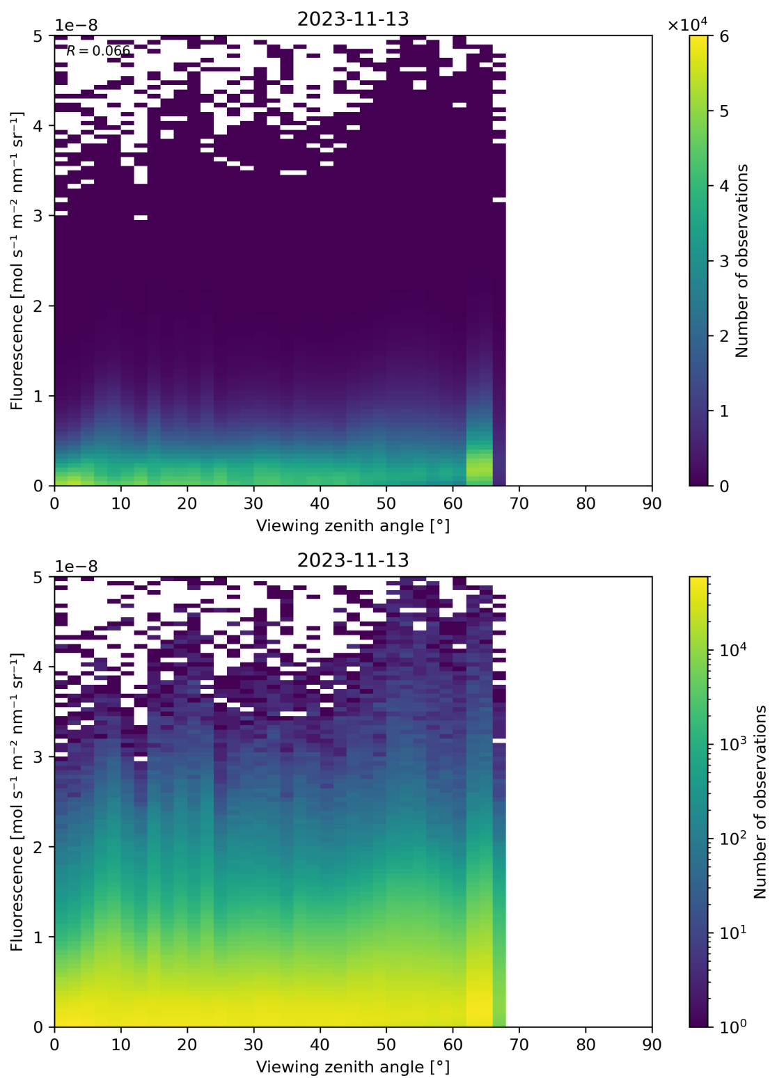
Figure 134: Scatter density plot of “Viewing zenith angle” against “Fluorescence” for 2023-11-13 to 2023-11-14.
