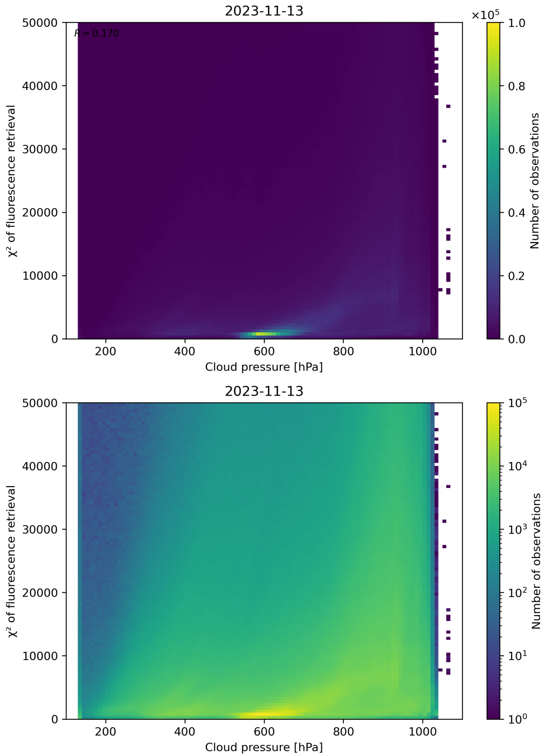
Figure 86: Scatter density plot of “Cloud pressure” against “ \chi^2 of fluorescence retrieval” for 2023-11-13 to 2023-11-14.
