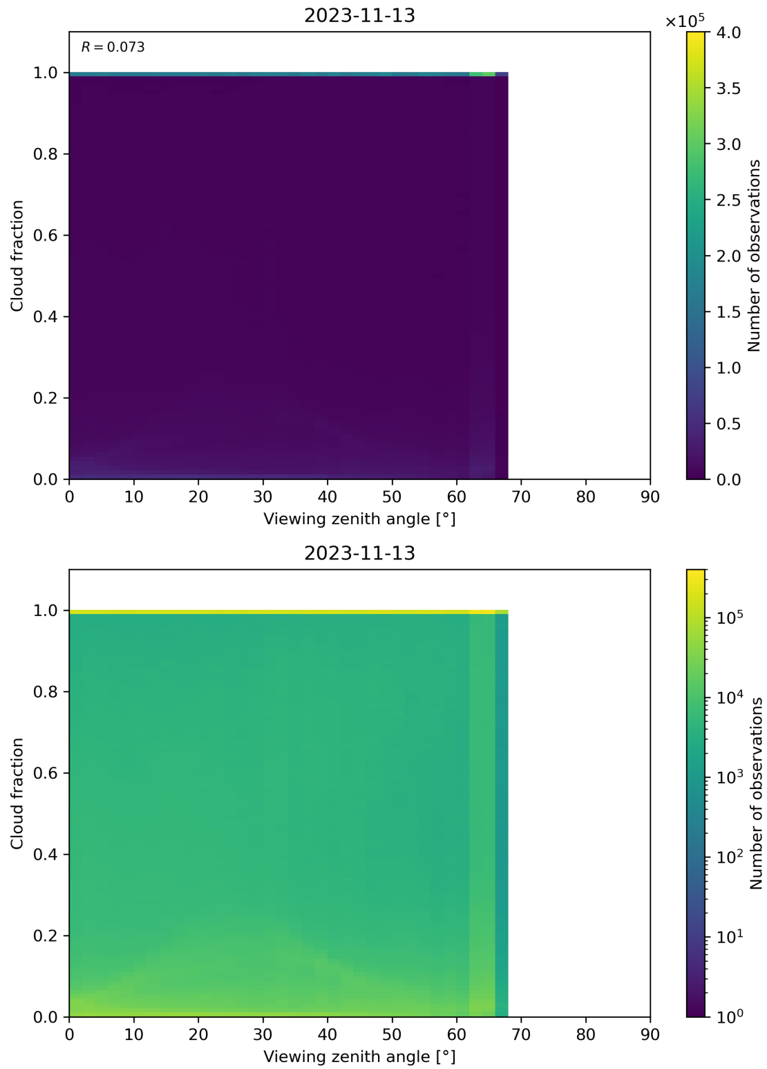
Figure 132: Scatter density plot of “Viewing zenith angle” against “Cloud fraction” for 2023-11-13 to 2023-11-14.
