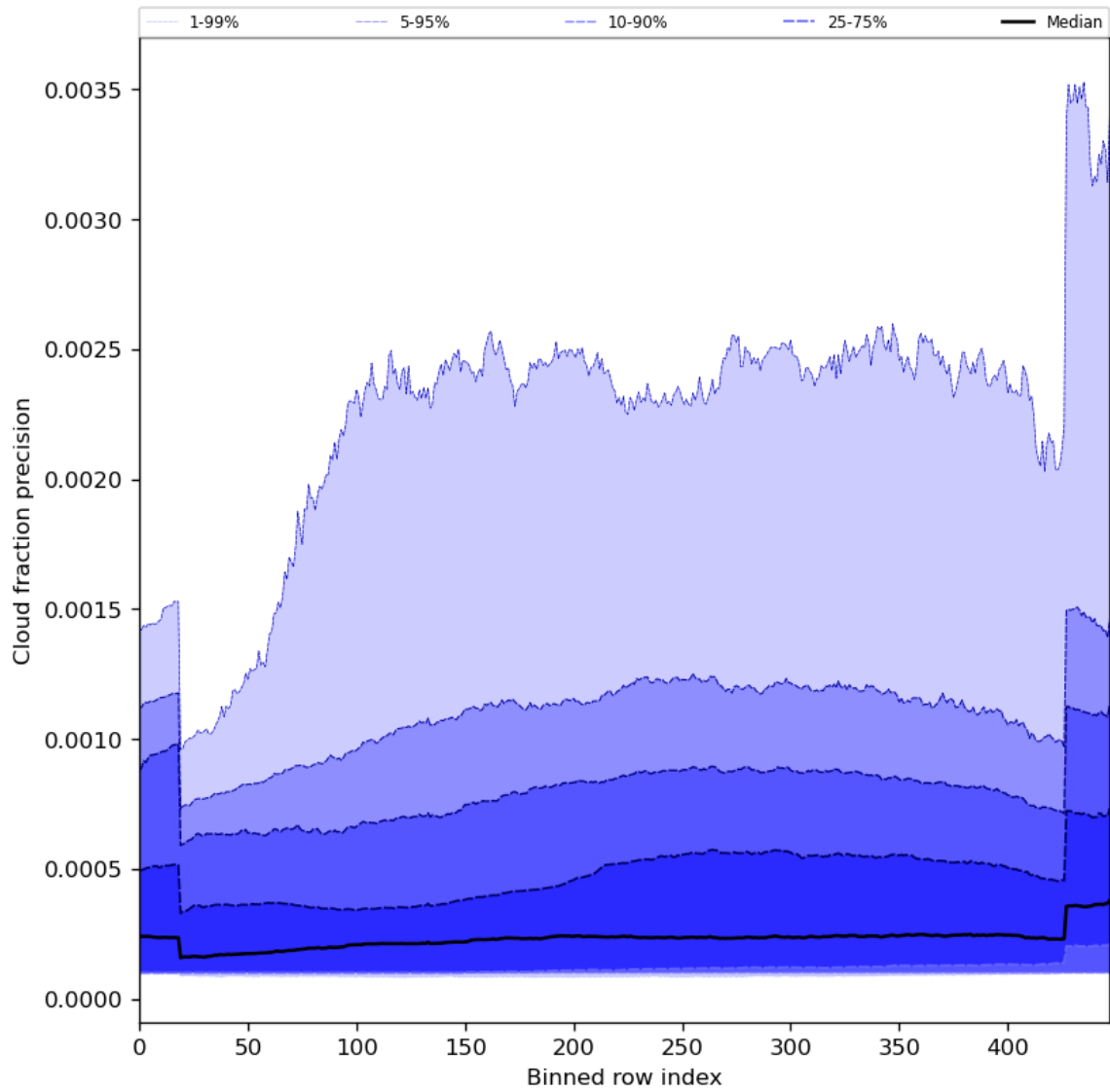
Figure 50: Along track statistics of “Cloud fraction precision” for 2023-11-13 to 2023-11-14
