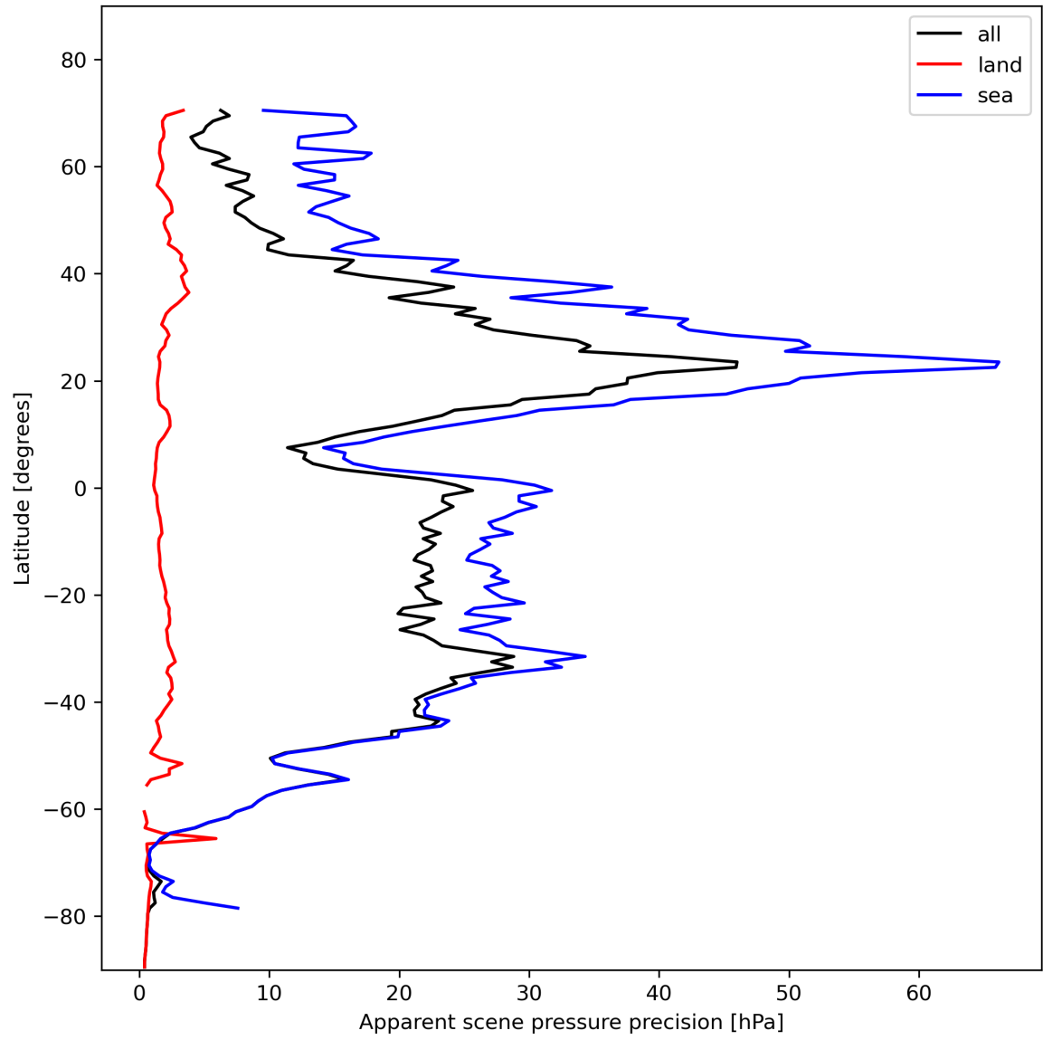
Figure 20: Zonal average of “Apparent scene pressure precision” for 2023-11-13 to 2023-11-14.
