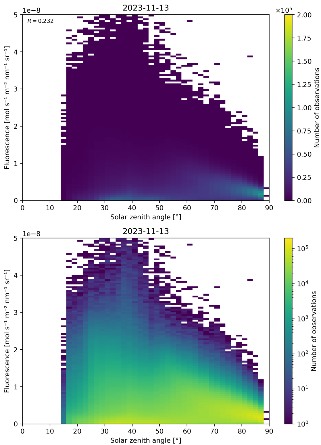
Figure 123: Scatter density plot of “Solar zenith angle” against “Fluorescence” for 2023-11-13 to 2023-11-14.
