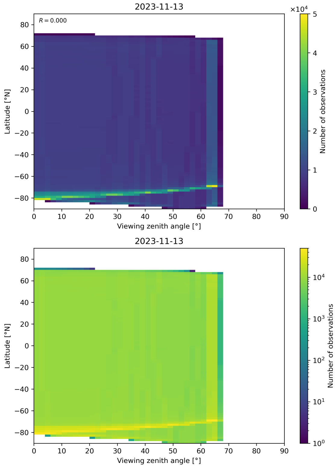
Figure 135: Scatter density plot of “Viewing zenith angle” against “Latitude” for 2023-11-13 to 2023-11-14.
