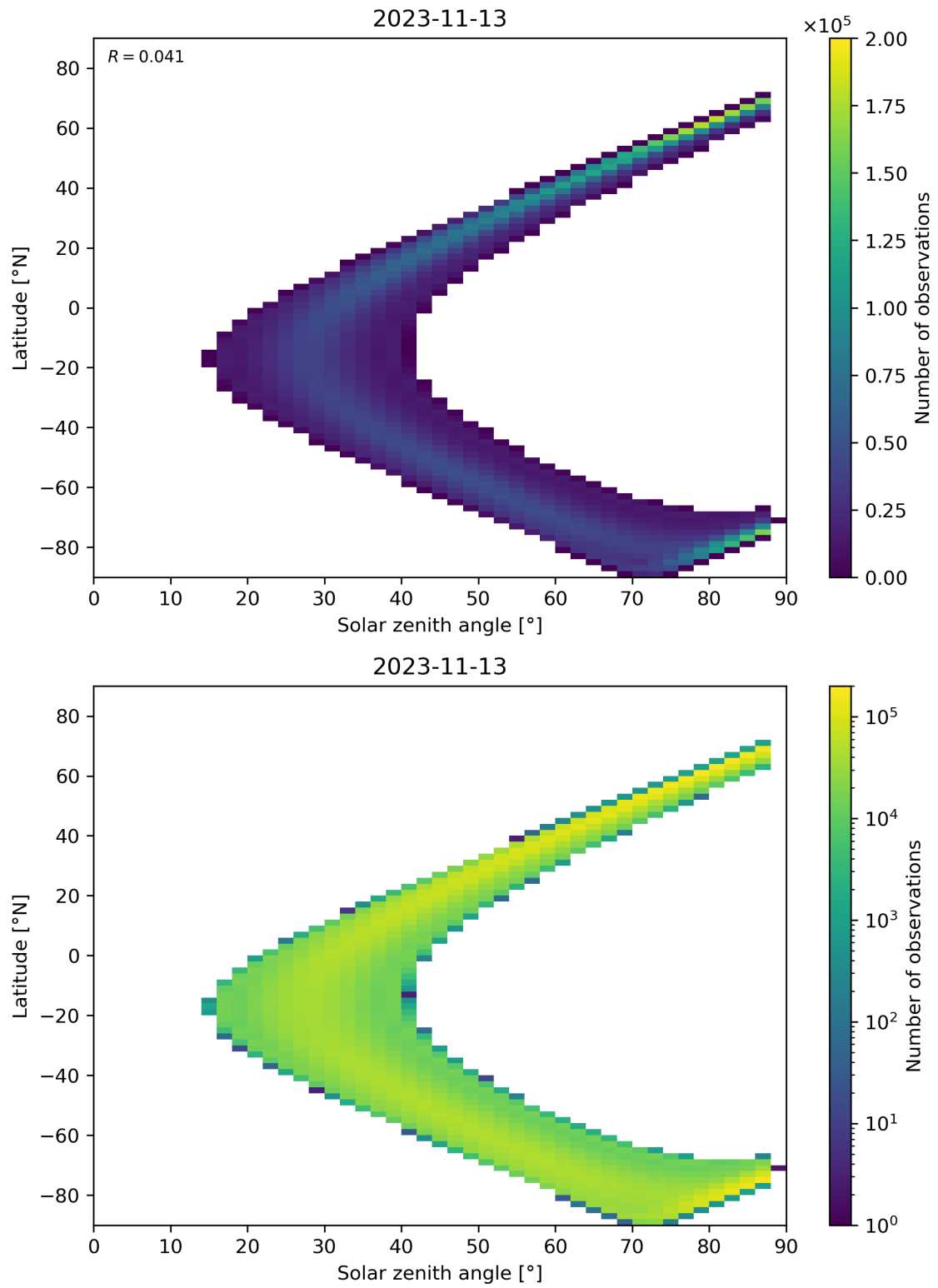
Figure 124: Scatter density plot of “Solar zenith angle” against “Latitude” for 2023-11-13 to 2023-11-14.
