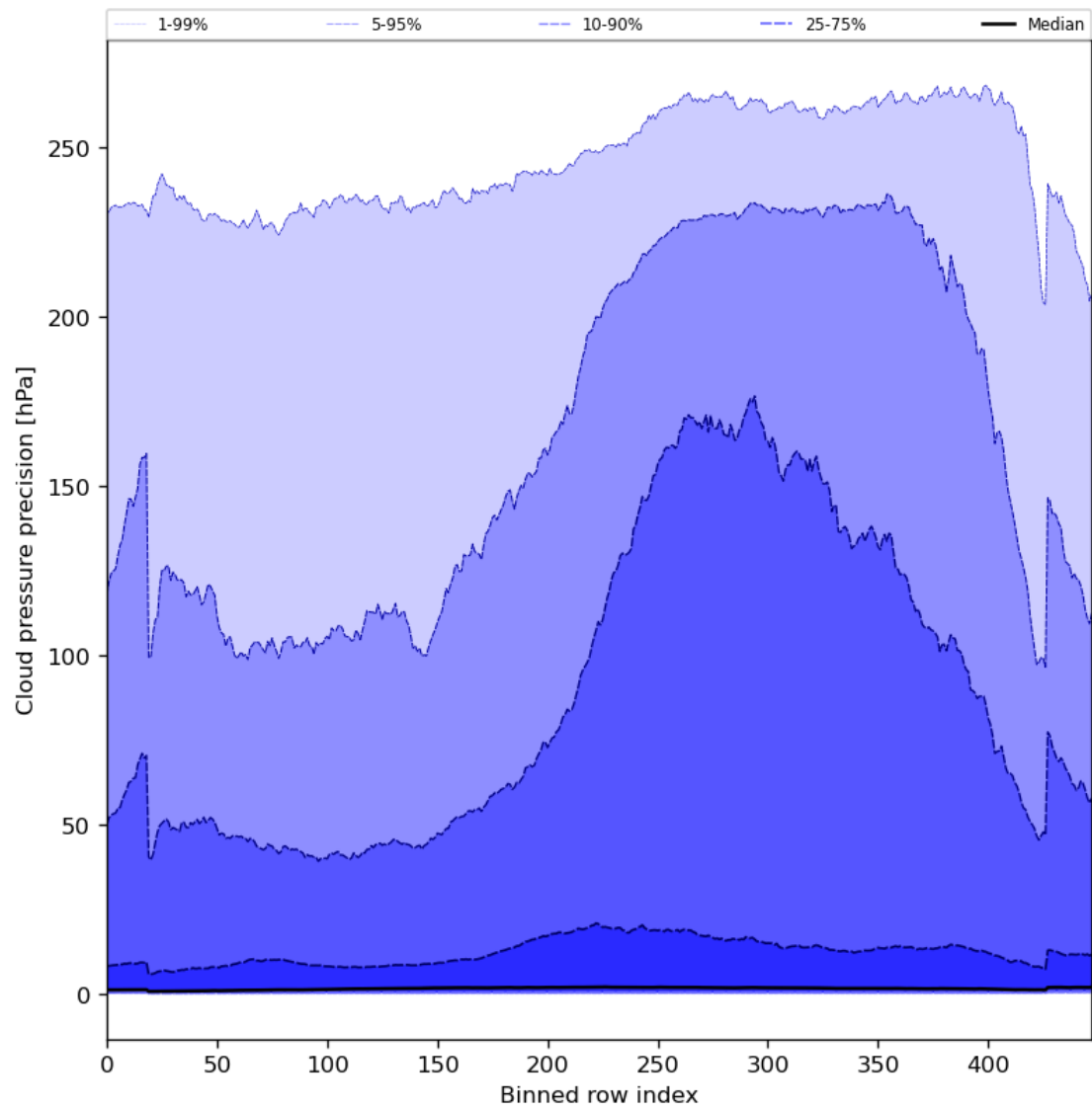
Figure 48: Along track statistics of “Cloud pressure precision” for 2023-11-13 to 2023-11-14
