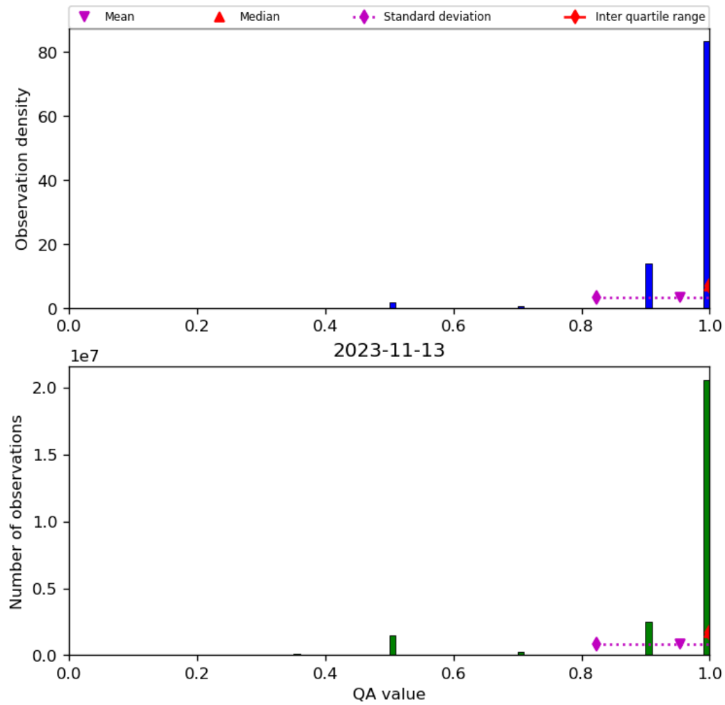
Figure 29: Histogram of “QA value” for 2023-11-13 to 2023-11-14
