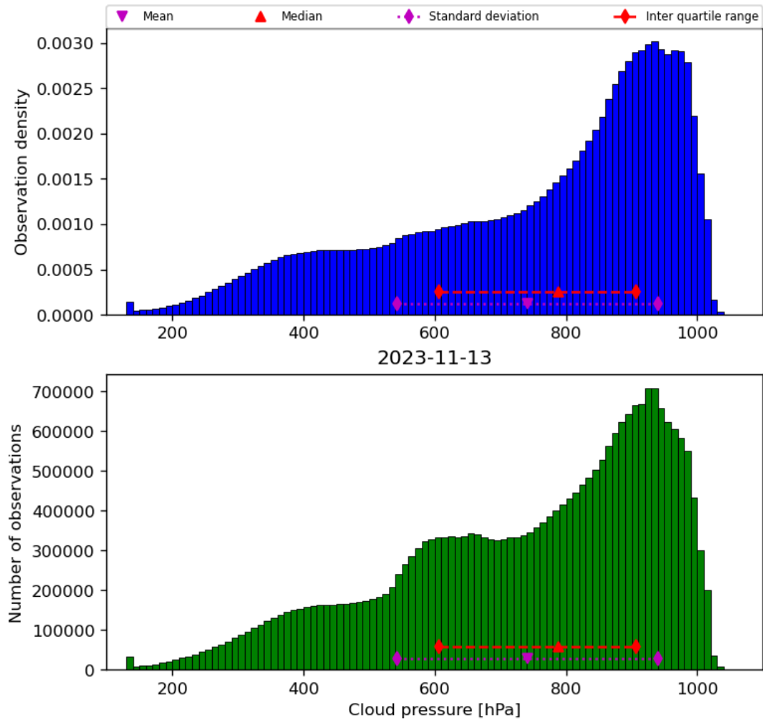
Figure 30: Histogram of “Cloud pressure” for 2023-11-13 to 2023-11-14
