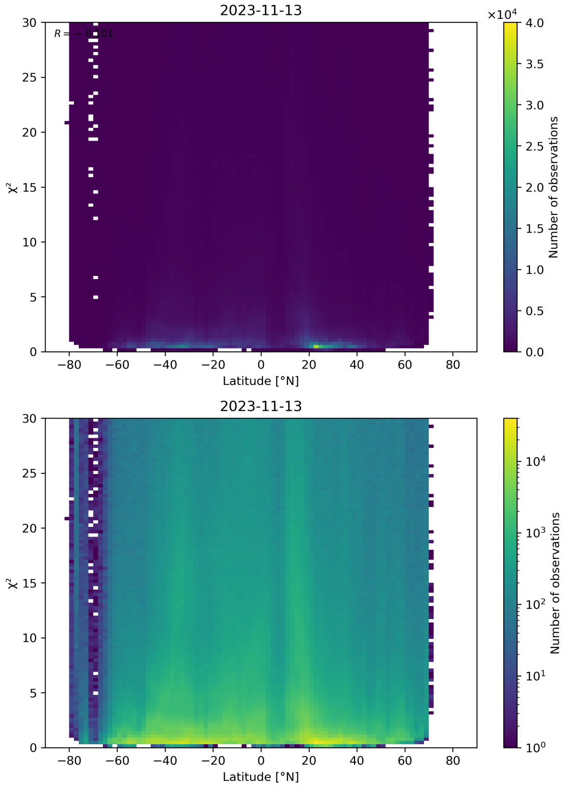
Figure 97: Scatter density plot of “Latitude” against “ \chi^2 ” for 2023-11-13 to 2023-11-14.
