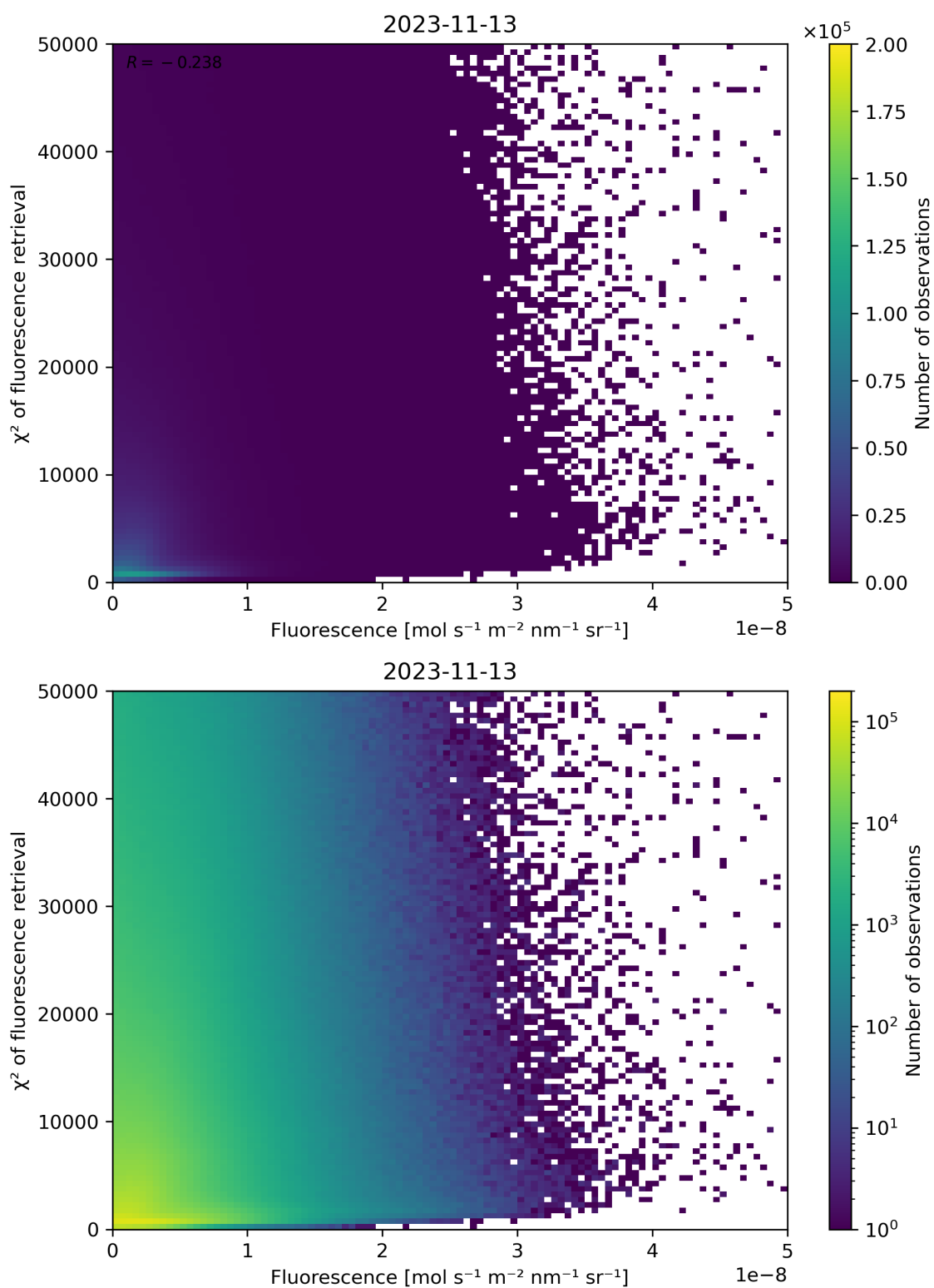
Figure 93: Scatter density plot of “Fluorescence” against “ \chi^2 of fluorescence retrieval” for 2023-11-13 to 2023-11-14.
