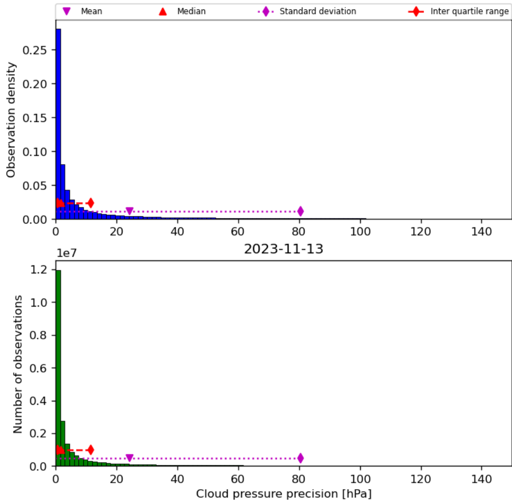
Figure 31: Histogram of “Cloud pressure precision” for 2023-11-13 to 2023-11-14
