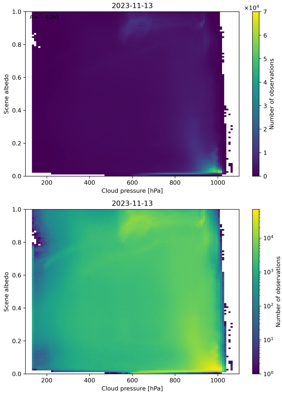
Figure 91: Scatter density plot of “Cloud pressure” against “Scene albedo” for 2023-11-13 to 2023-11-14.
