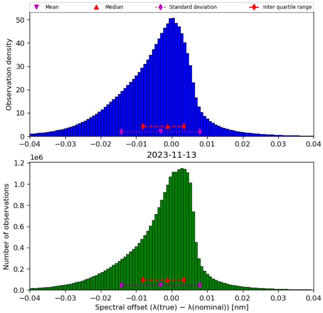
Figure 45: Histogram of “Spectral offset ( \lambda(\text{true}) - \lambda(\text{nominal}) )” for 2023-11-13 to 2023-11-14
