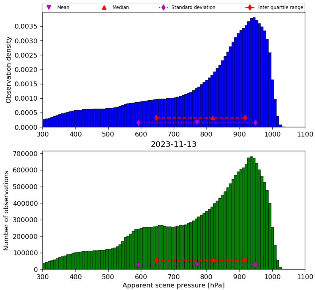
Figure 36: Histogram of “Apparent scene pressure” for 2023-11-13 to 2023-11-14
