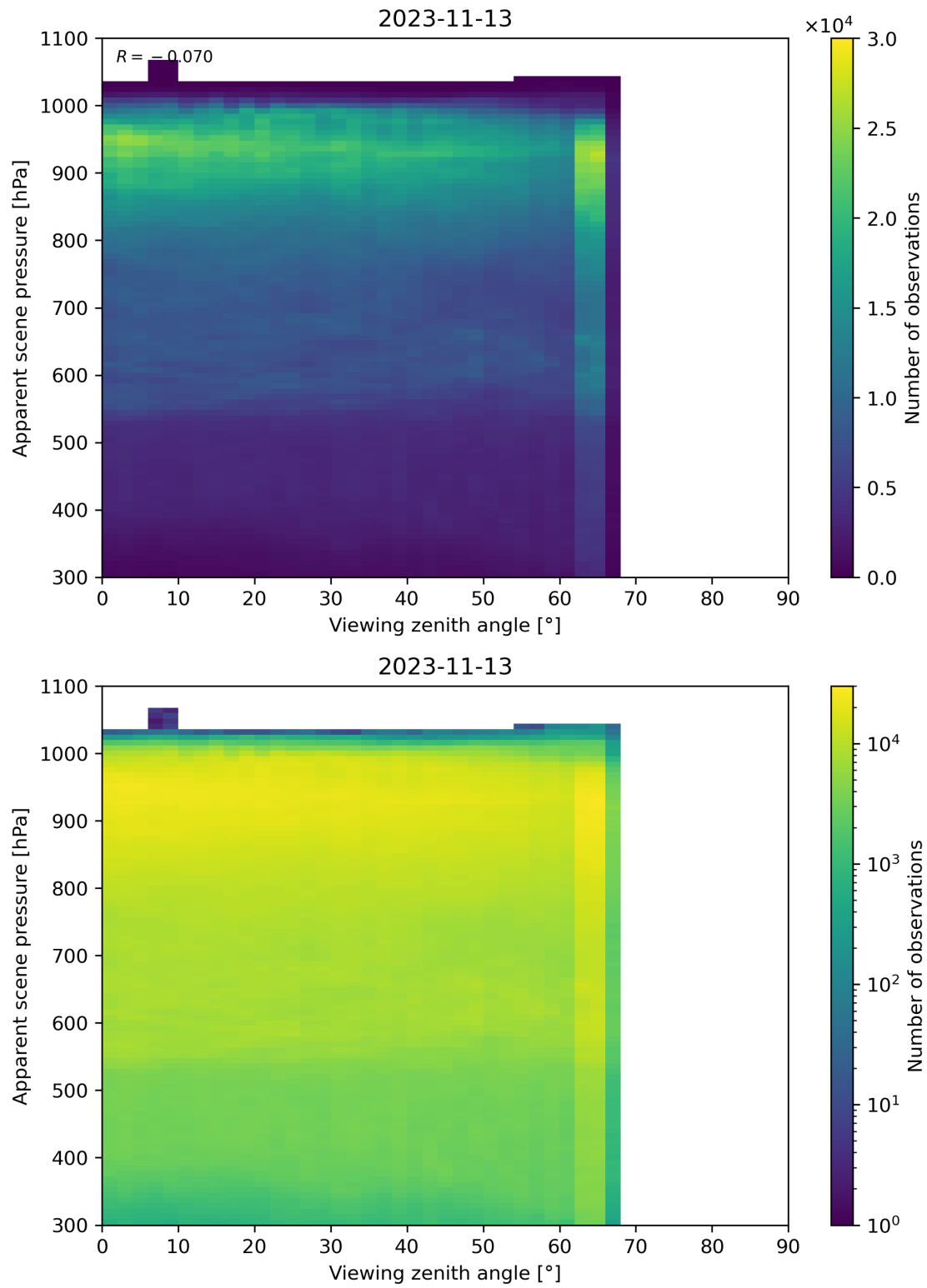
Figure 129: Scatter density plot of “Viewing zenith angle” against “Apparent scene pressure” for 2023-11-13 to 2023-11-14.
