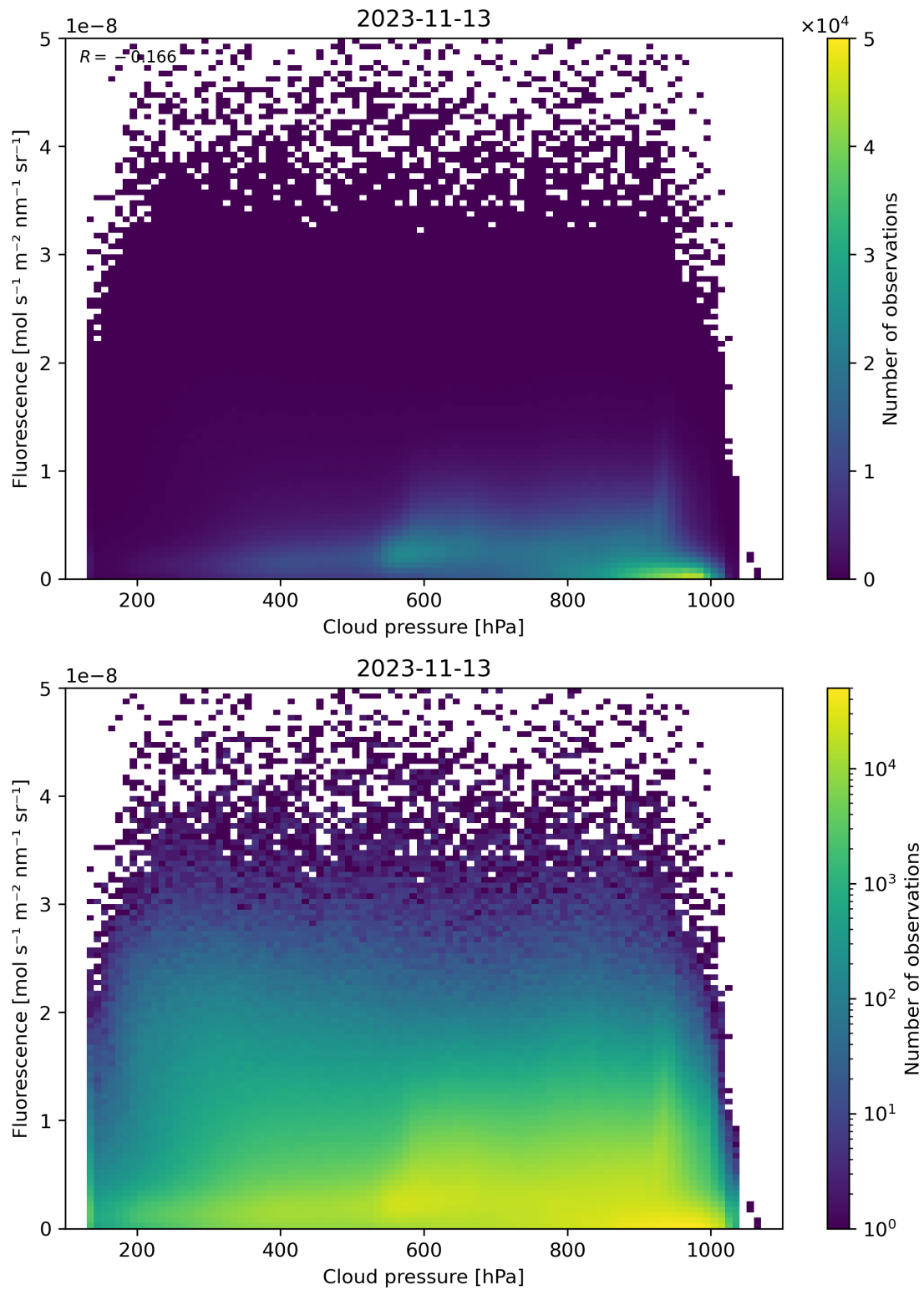
Figure 88: Scatter density plot of “Cloud pressure” against “Fluorescence” for 2023-11-13 to 2023-11-14.
