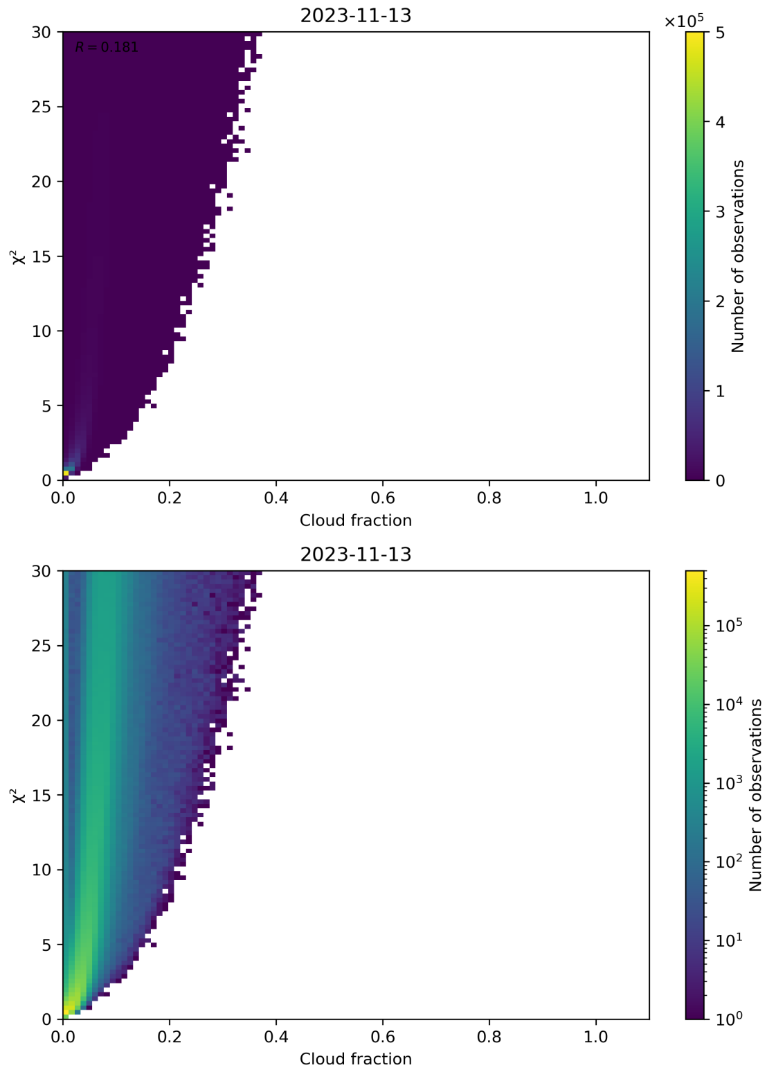
Figure 77: Scatter density plot of “Cloud fraction” against “ \chi^2 ” for 2023-11-13 to 2023-11-14.
