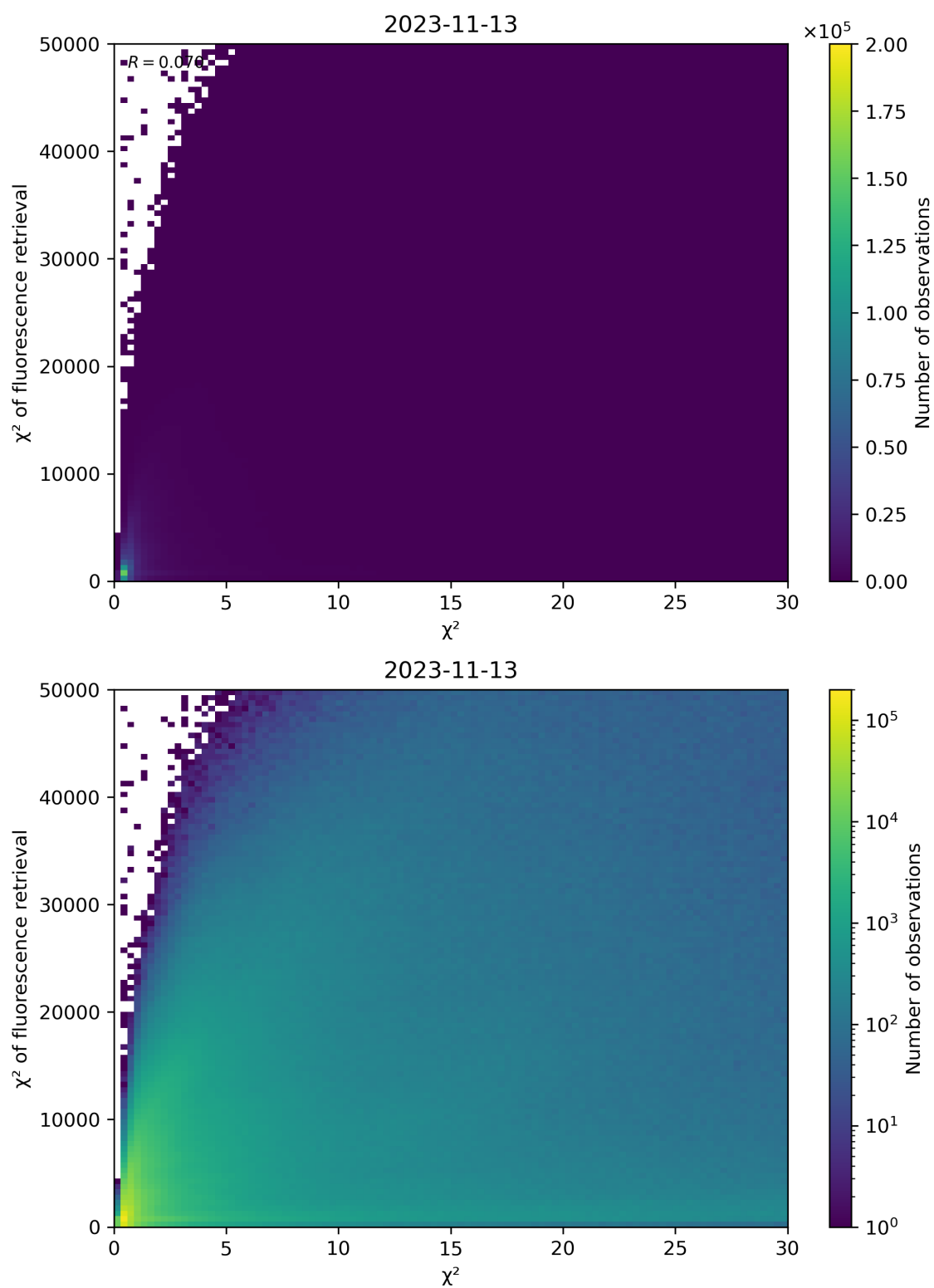
Figure 69: Scatter density plot of “ \chi^2 ” against “ \chi^2 of fluorescence retrieval” for 2023-11-13 to 2023-11-14.
