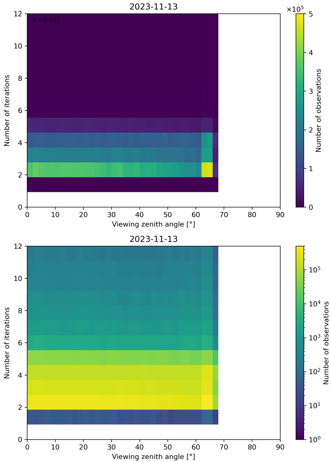
Figure 136: Scatter density plot of “Viewing zenith angle” against “Number of iterations” for 2023-11-13 to 2023-11-14.
