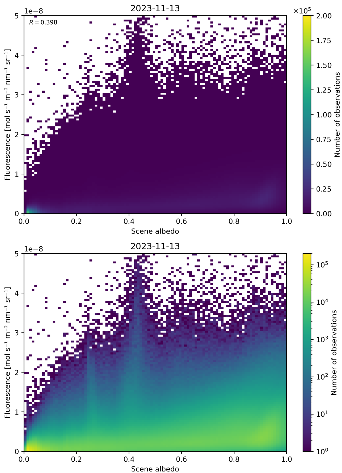
Figure 114: Scatter density plot of “Scene albedo” against “Fluorescence” for 2023-11-13 to 2023-11-14.
