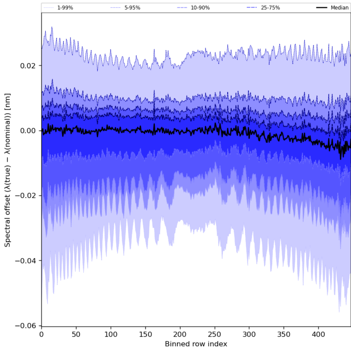
Figure 62: Along track statistics of “Spectral offset ( \lambda(\text{true}) - \lambda(\text{nominal}) )” for 2023-11-13 to 2023-11-14
