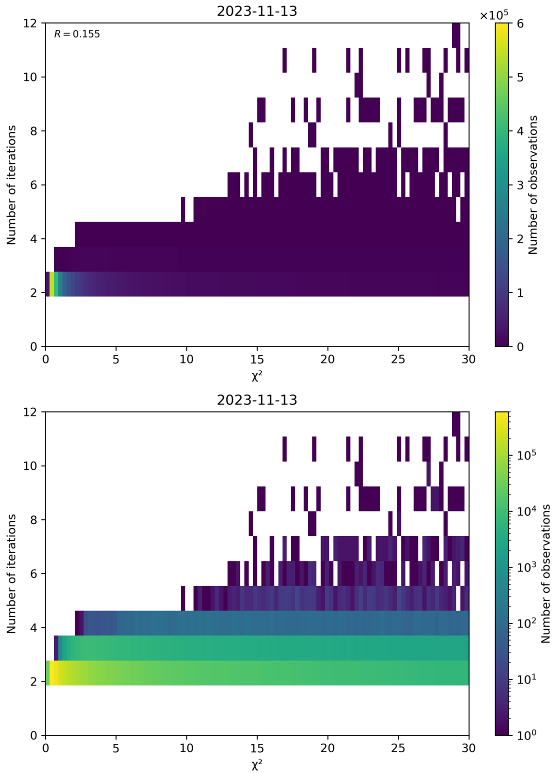
Figure 73: Scatter density plot of “ \chi^2 ” against “Number of iterations” for 2023-11-13 to 2023-11-14.
