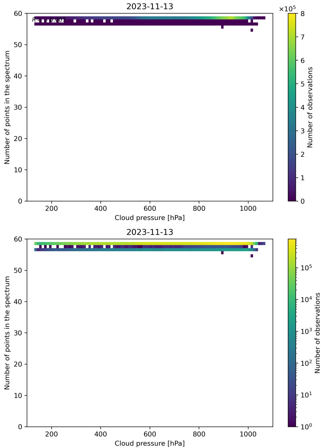
Figure 90: Scatter density plot of “Cloud pressure” against “Number of points in the spectrum” for 2023-11-13 to 2023-11-14.
