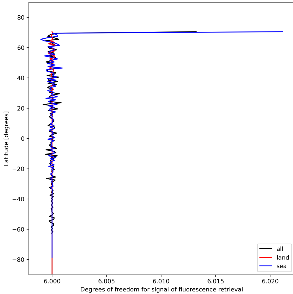
Figure 26: Zonal average of “Degrees of freedom for signal of fluorescence retrieval” for 2023-11-13 to 2023-11-14.
