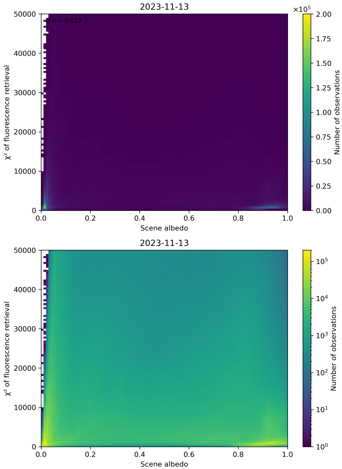
Figure 113: Scatter density plot of “Scene albedo” against “ \chi^2 of fluorescence retrieval” for 2023-11-13 to 2023-11-14.
