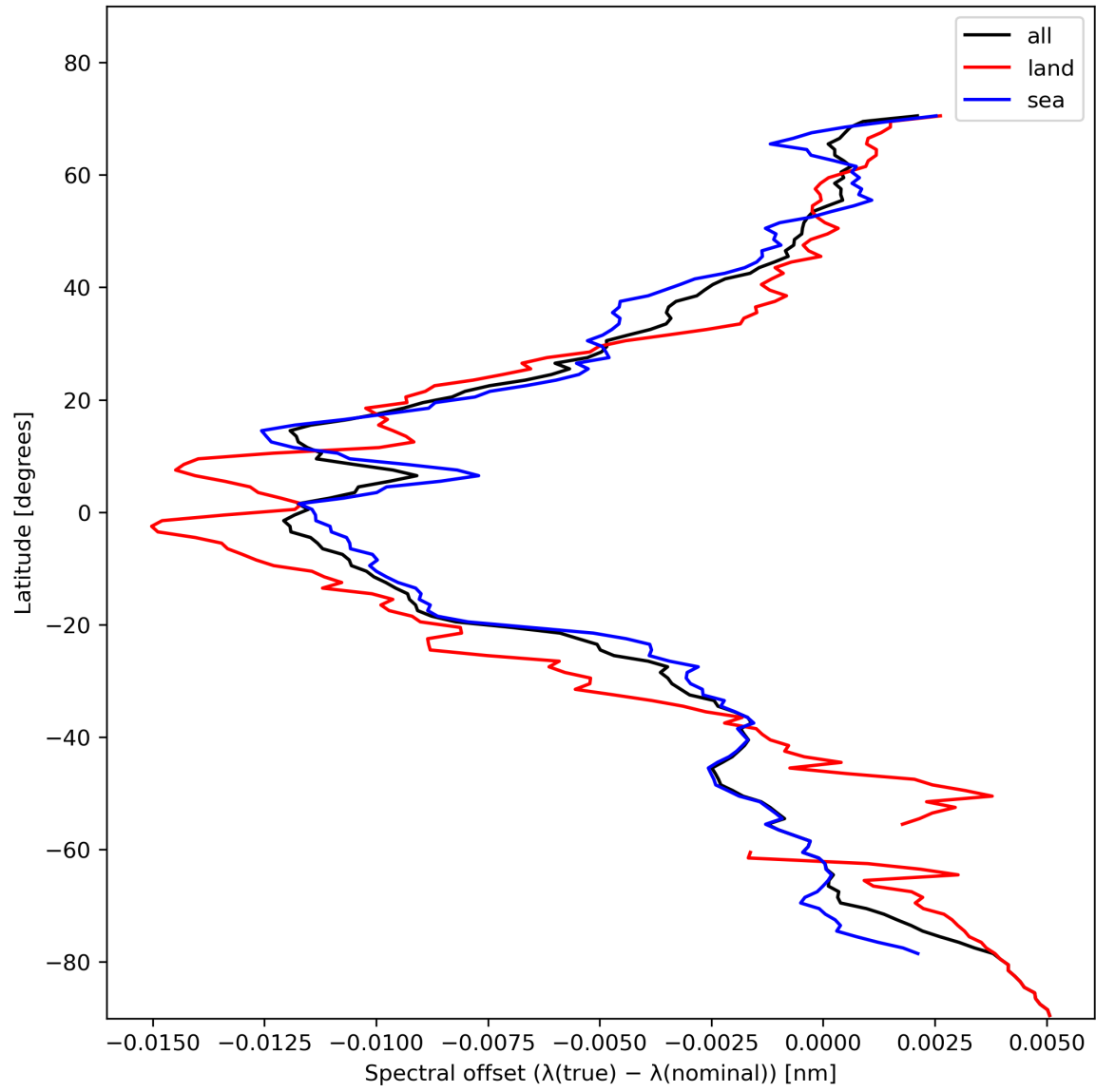
Figure 28: Zonal average of “Spectral offset ( \lambda(\text{true}) - \lambda(\text{nominal}) )” for 2023-11-13 to 2023-11-14.
