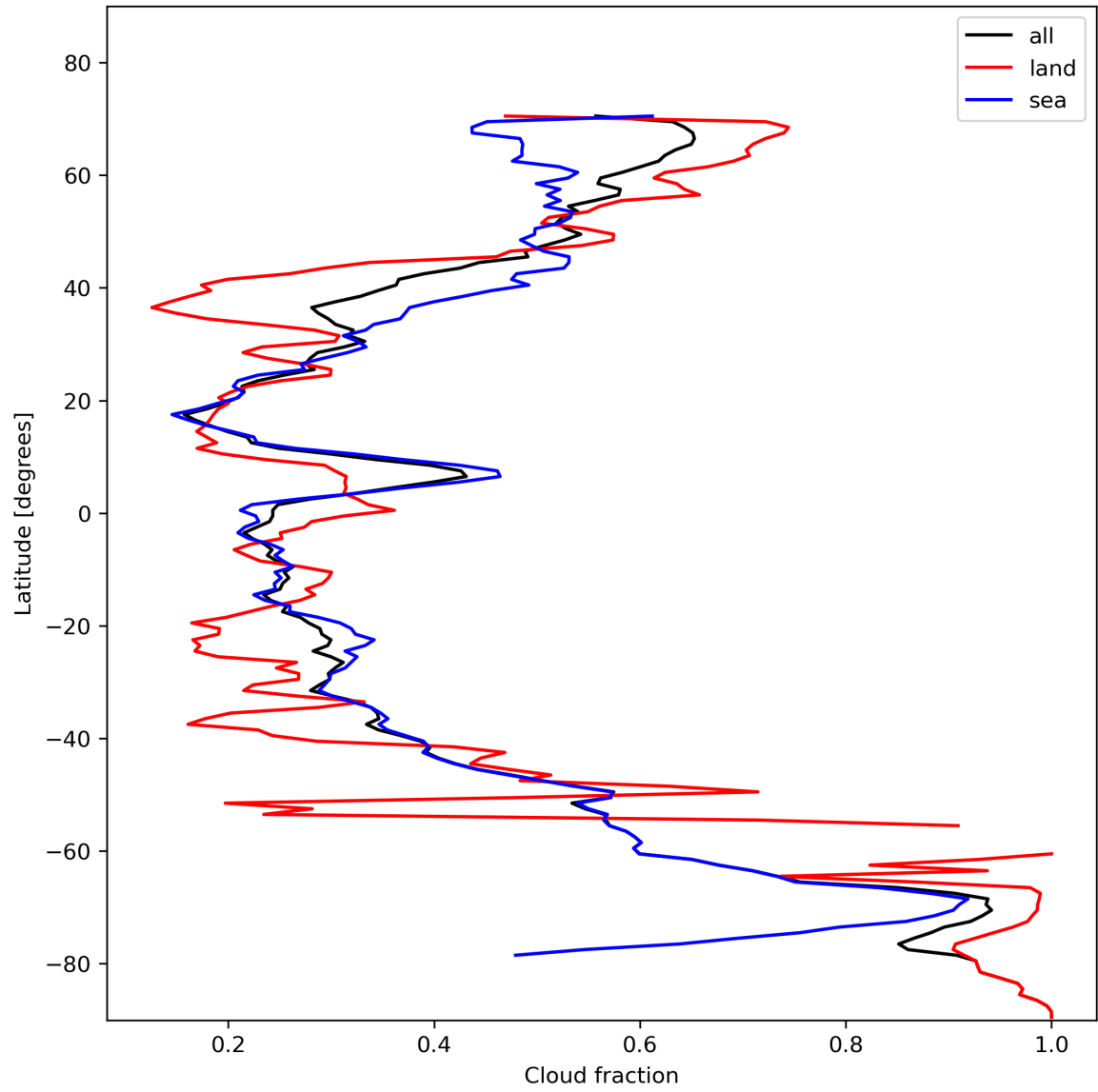
Figure 15: Zonal average of “Cloud fraction” for 2023-11-13 to 2023-11-14.
