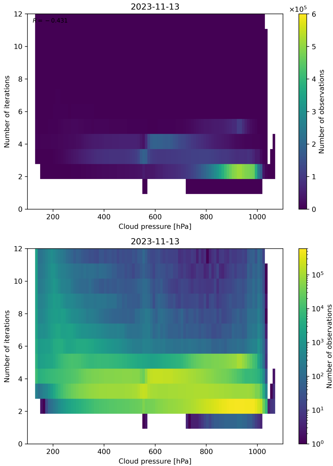
Figure 89: Scatter density plot of “Cloud pressure” against “Number of iterations” for 2023-11-13 to 2023-11-14.
