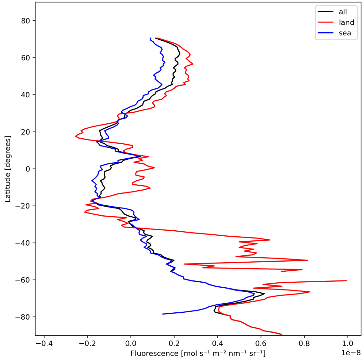
Figure 23: Zonal average of “Fluorescence” for 2023-11-13 to 2023-11-14.
