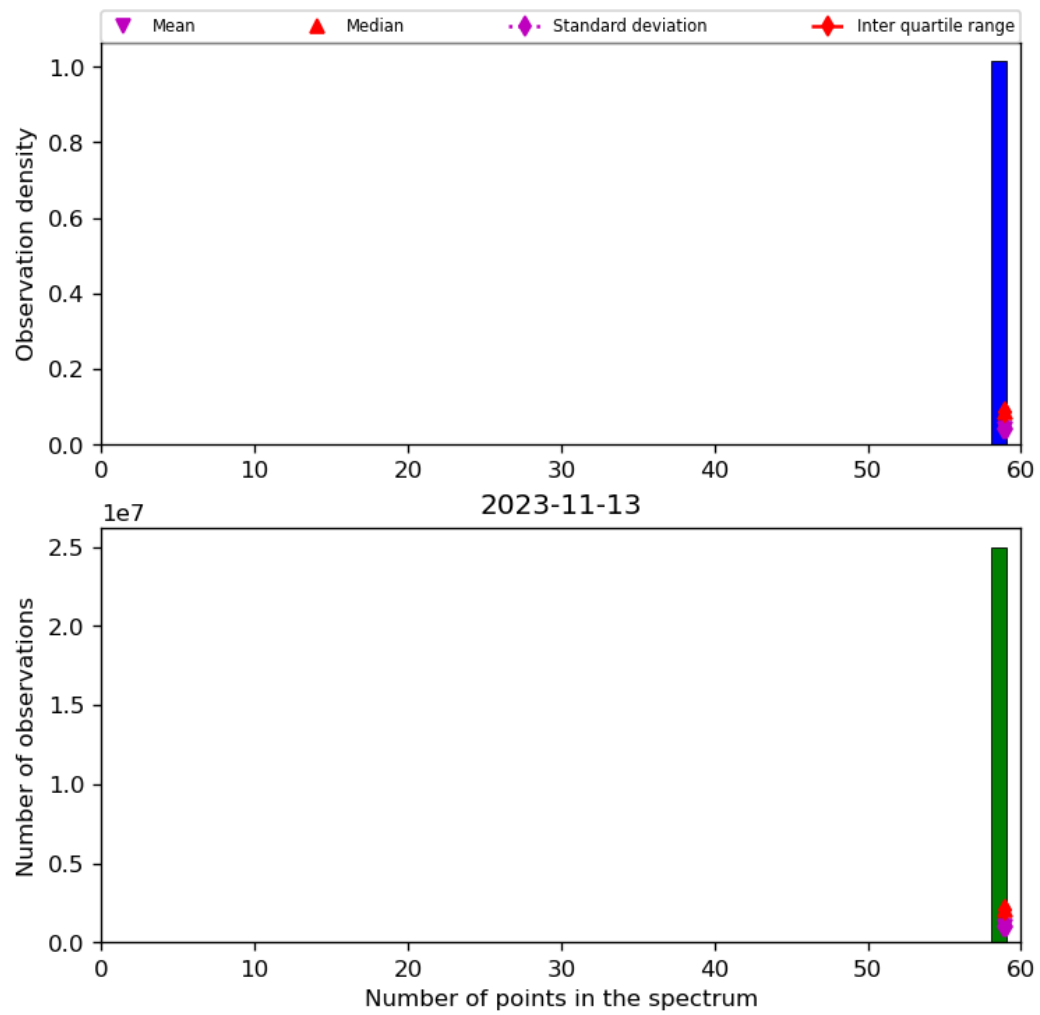
Figure 44: Histogram of “Number of points in the spectrum” for 2023-11-13 to 2023-11-14
