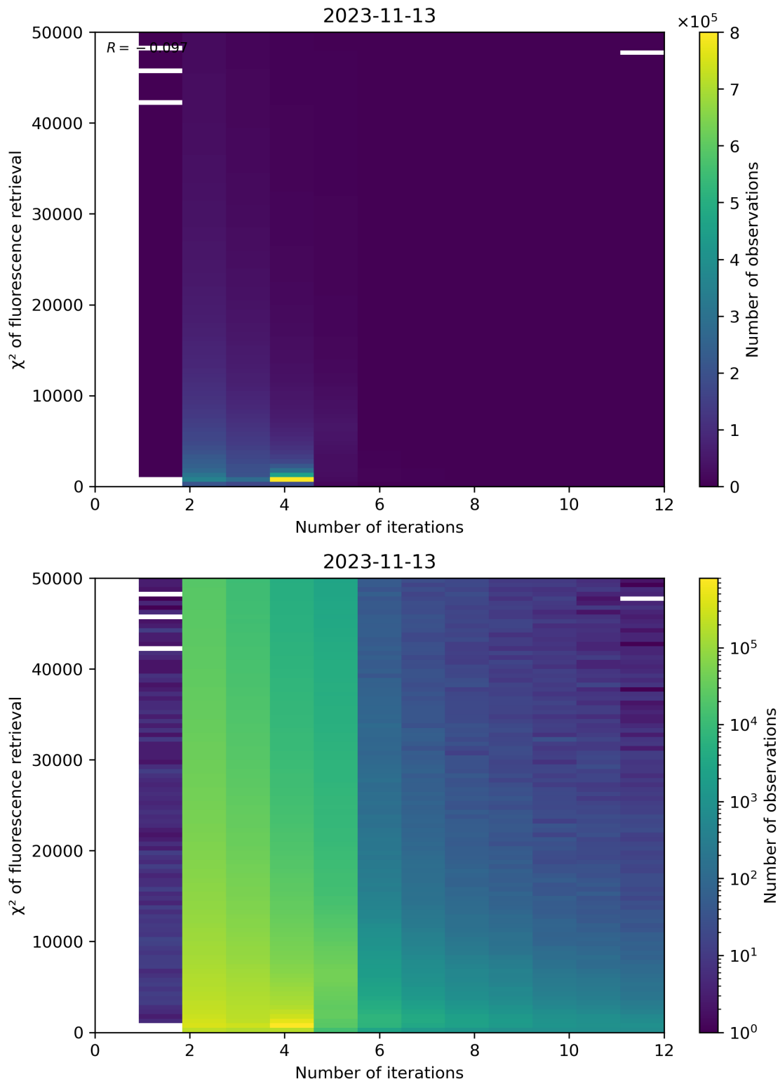
Figure 106: Scatter density plot of “Number of iterations” against “ \chi^2 of fluorescence retrieval” for 2023-11-13 to 2023-11-14.
