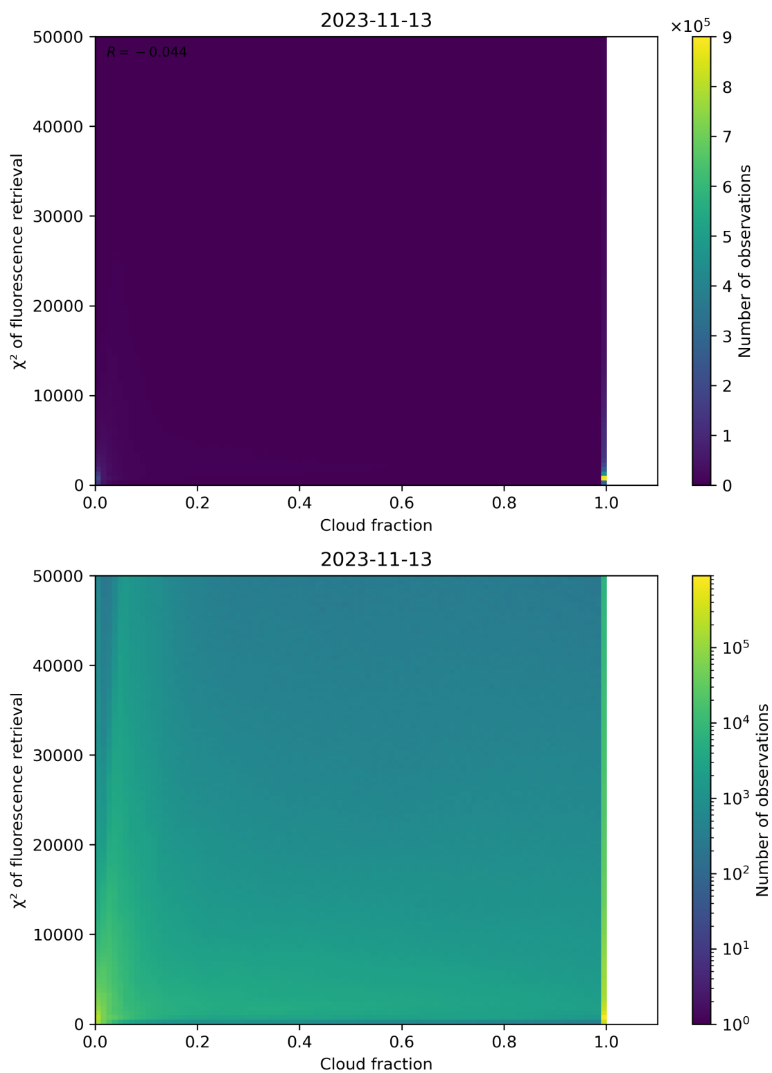
Figure 78: Scatter density plot of “Cloud fraction” against “ \chi^2 of fluorescence retrieval” for 2023-11-13 to 2023-11-14.
