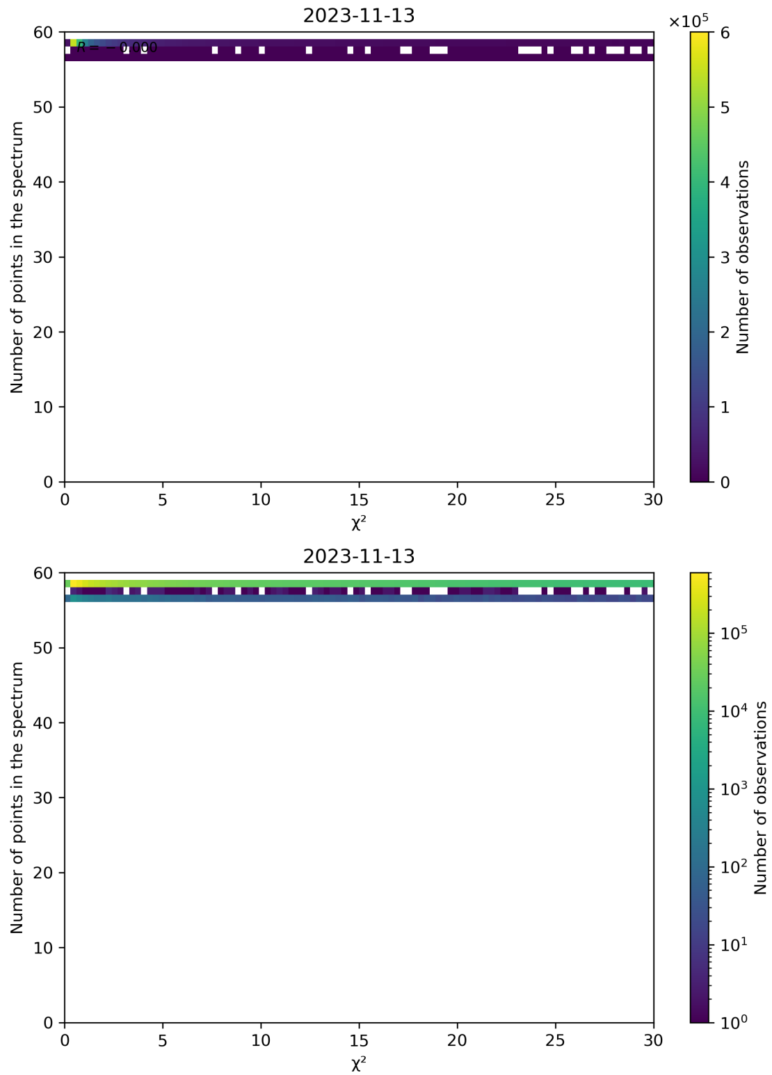
Figure 74: Scatter density plot of " \chi^2 " against "Number of points in the spectrum" for 2023-11-13 to 2023-11-14.
