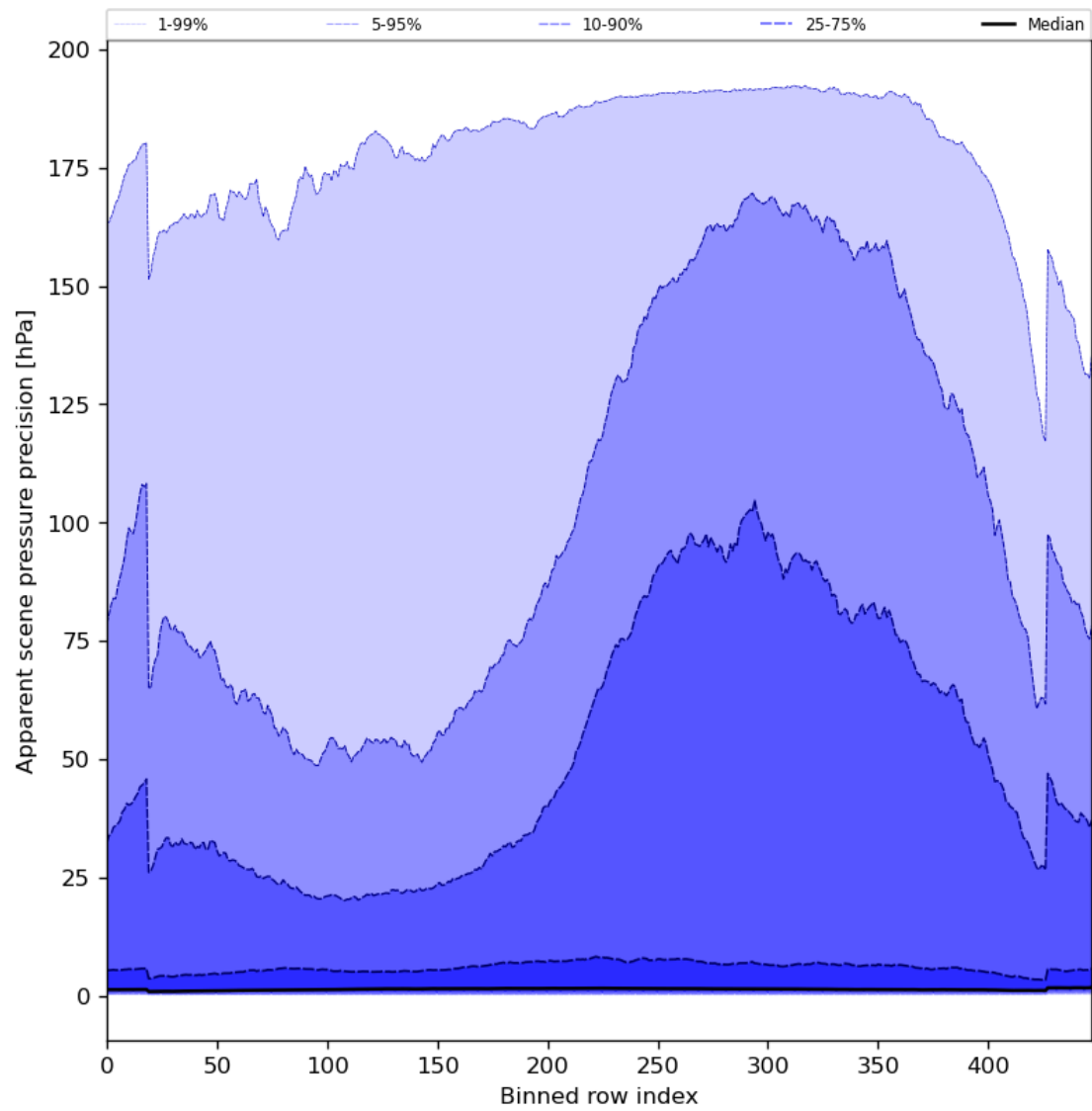
Figure 54: Along track statistics of “Apparent scene pressure precision” for 2023-11-13 to 2023-11-14
