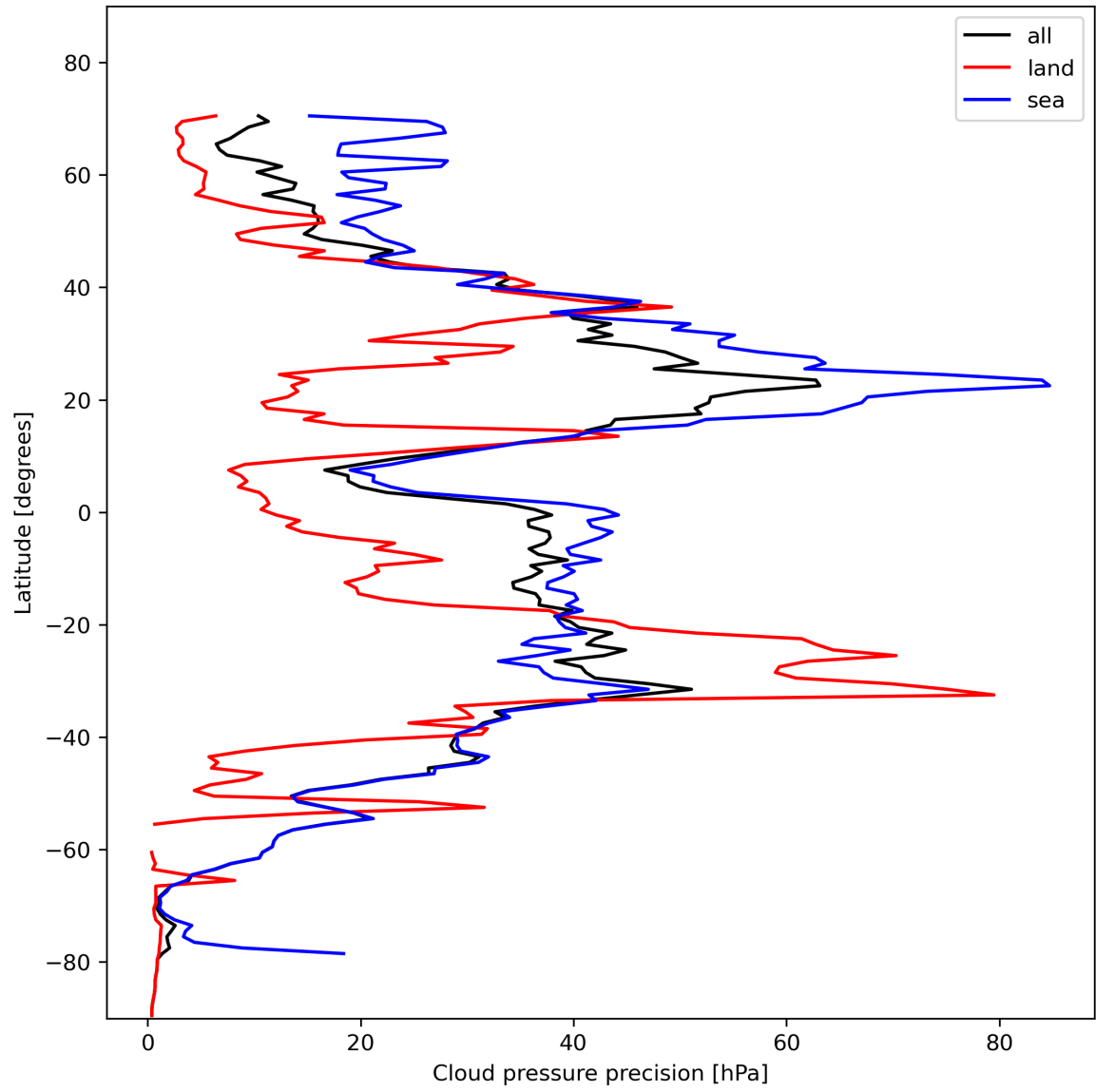
Figure 14: Zonal average of “Cloud pressure precision” for 2023-11-13 to 2023-11-14.
