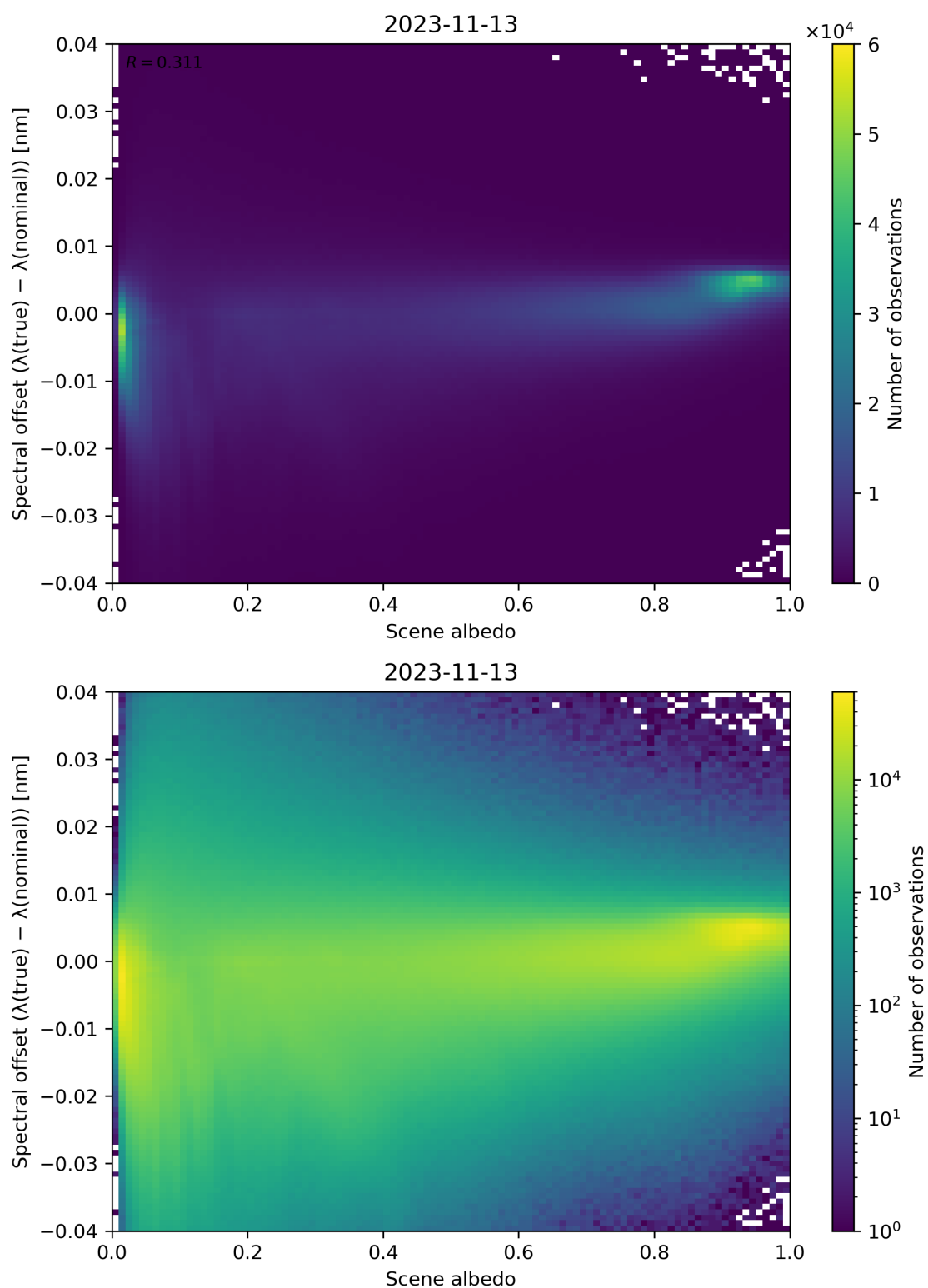
Figure 117: Scatter density plot of “Scene albedo” against “Spectral offset ( \lambda(\text{true}) - \lambda(\text{nominal}) )” for 2023-11-13 to 2023-11-14.
