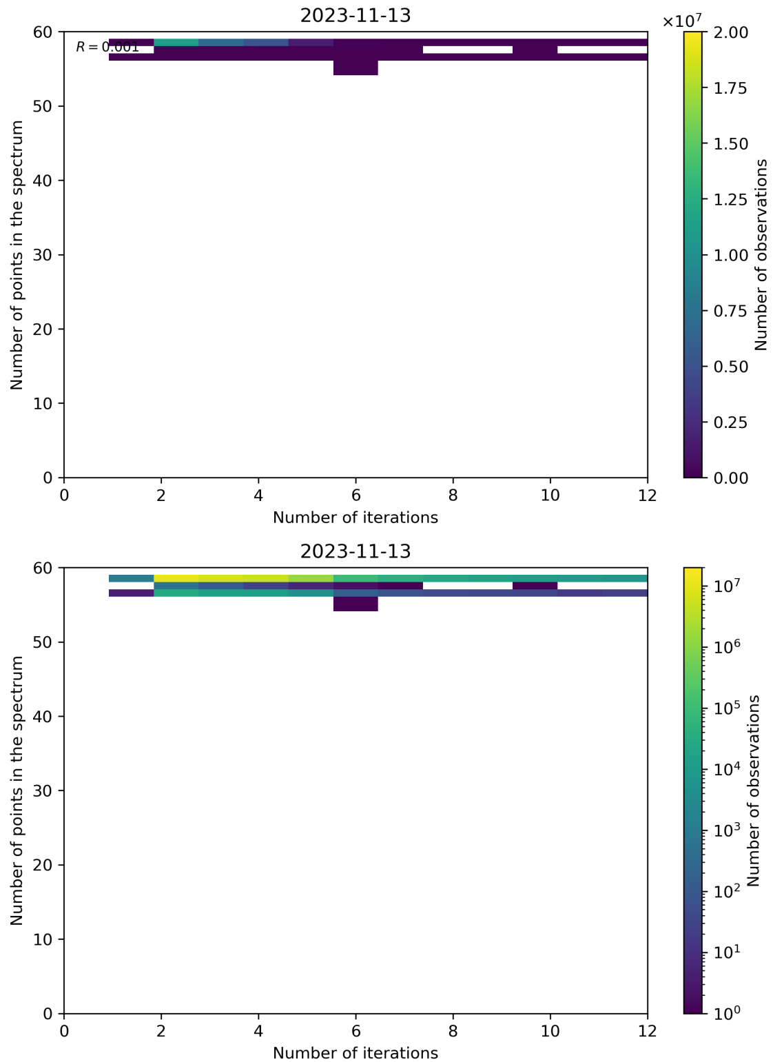
Figure 108: Scatter density plot of “Number of iterations” against “Number of points in the spectrum” for 2023-11-13 to 2023-11-14.
