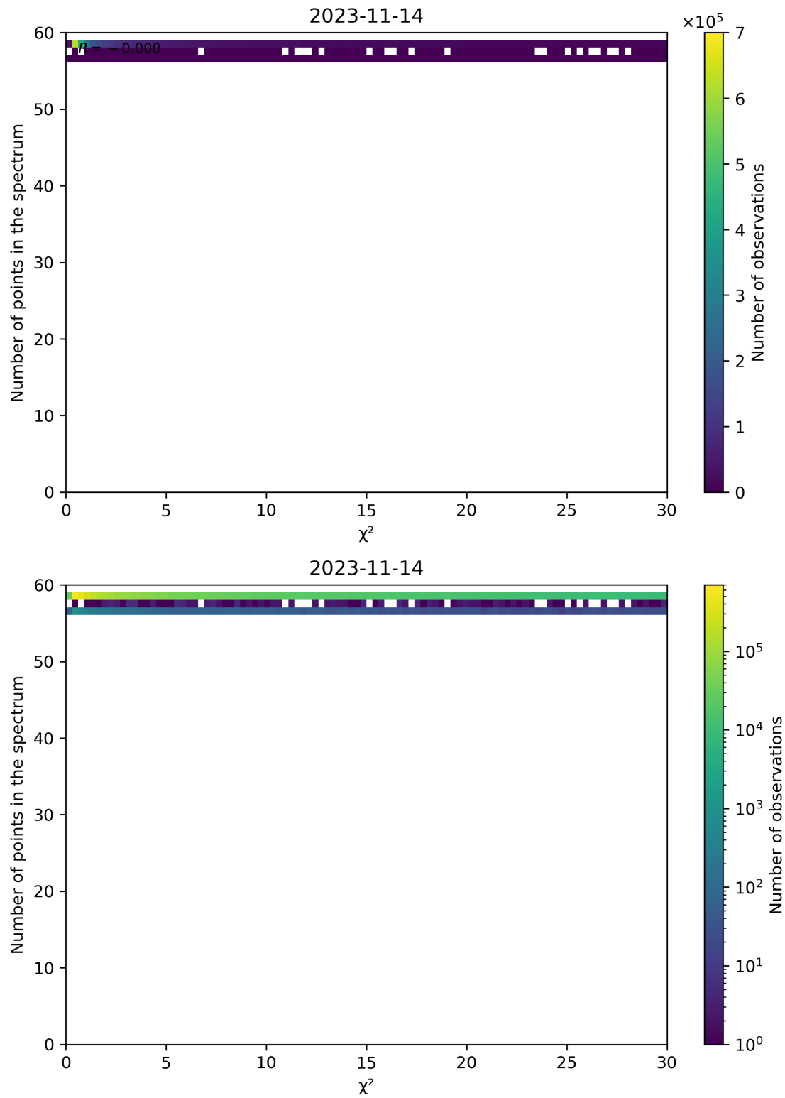
Figure 74: Scatter density plot of " \chi^2 " against "Number of points in the spectrum" for 2023-11-13 to 2023-11-15.
