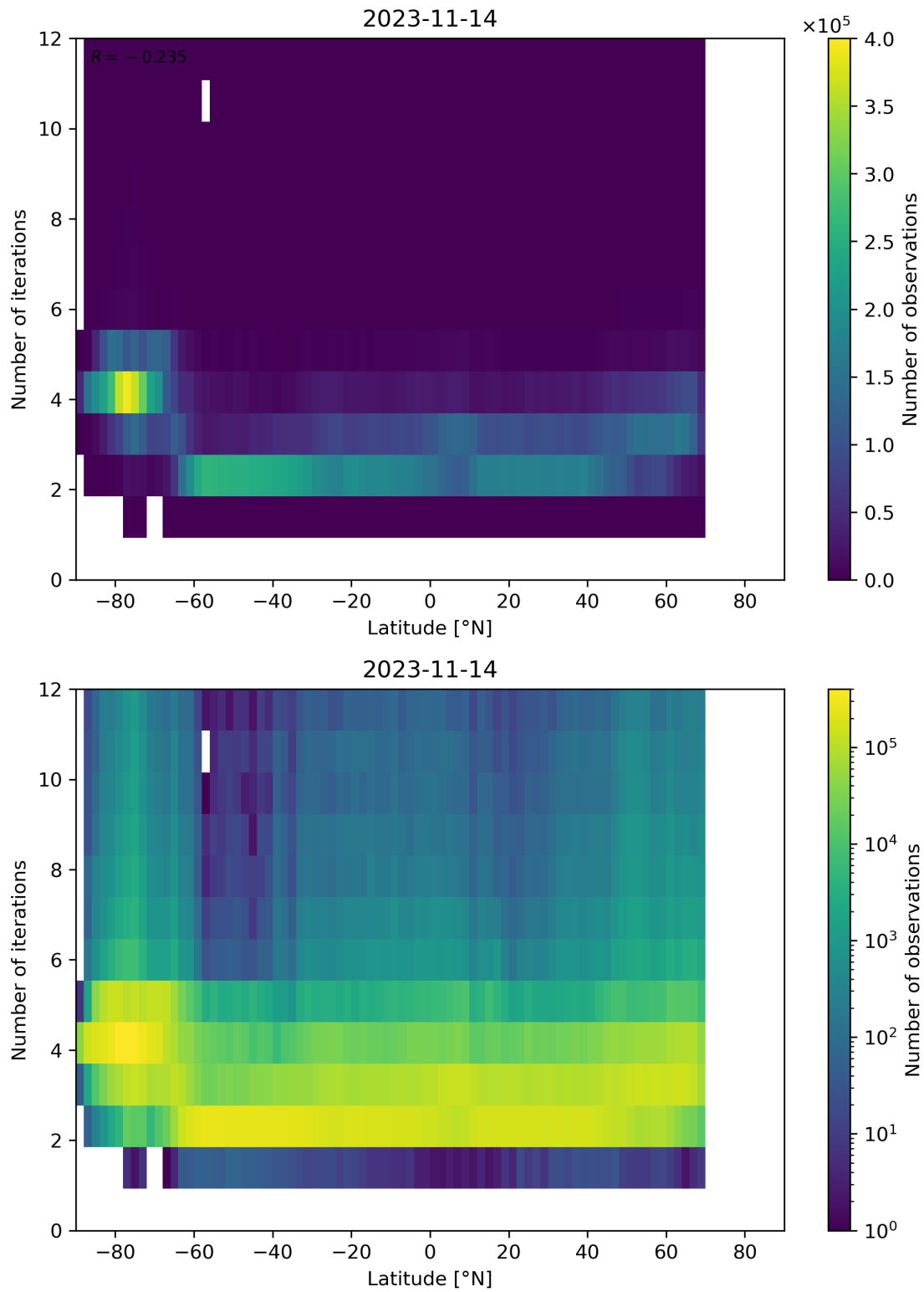
Figure 102: Scatter density plot of “Latitude” against “Number of iterations” for 2023-11-13 to 2023-11-15.
