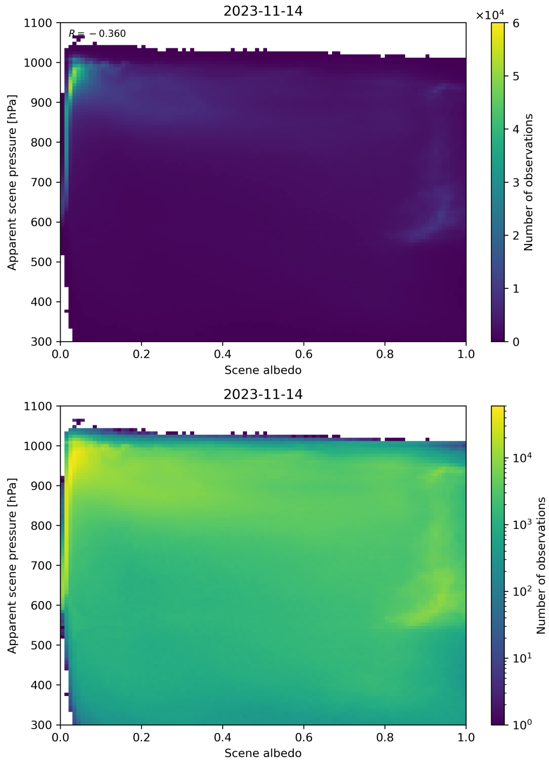
Figure 111: Scatter density plot of “Scene albedo” against “Apparent scene pressure” for 2023-11-13 to 2023-11-15.
