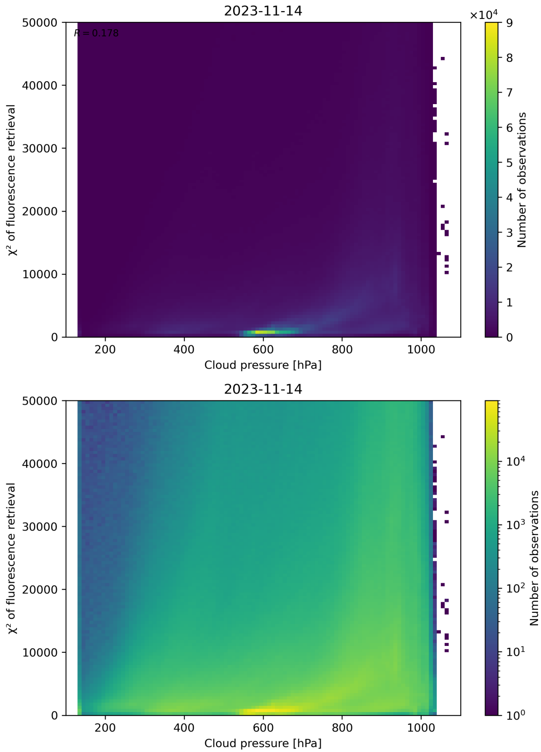
Figure 86: Scatter density plot of “Cloud pressure” against “ \chi^2 of fluorescence retrieval” for 2023-11-13 to 2023-11-15.
