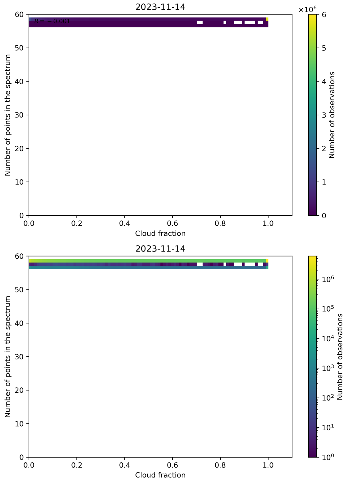
Figure 81: Scatter density plot of “Cloud fraction” against “Number of points in the spectrum” for 2023-11-13 to 2023-11-15.
