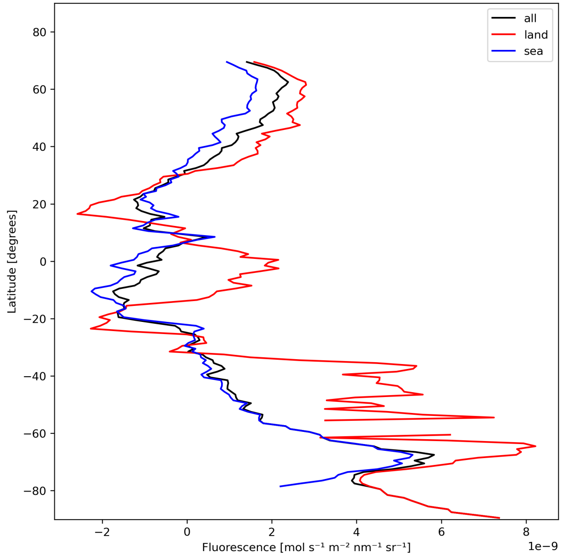
Figure 23: Zonal average of “Fluorescence” for 2023-11-13 to 2023-11-15.
