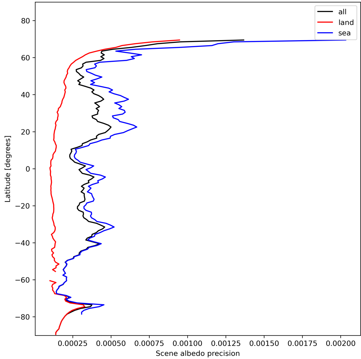
Figure 18: Zonal average of “Scene albedo precision” for 2023-11-13 to 2023-11-15.
