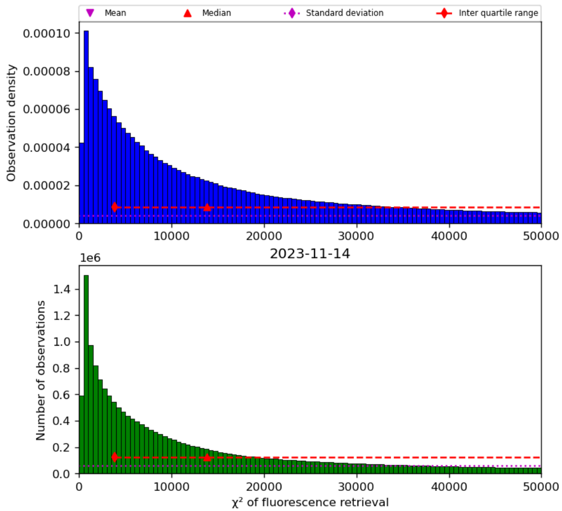
Figure 42: Histogram of “ \chi^2 of fluorescence retrieval” for 2023-11-13 to 2023-11-15
