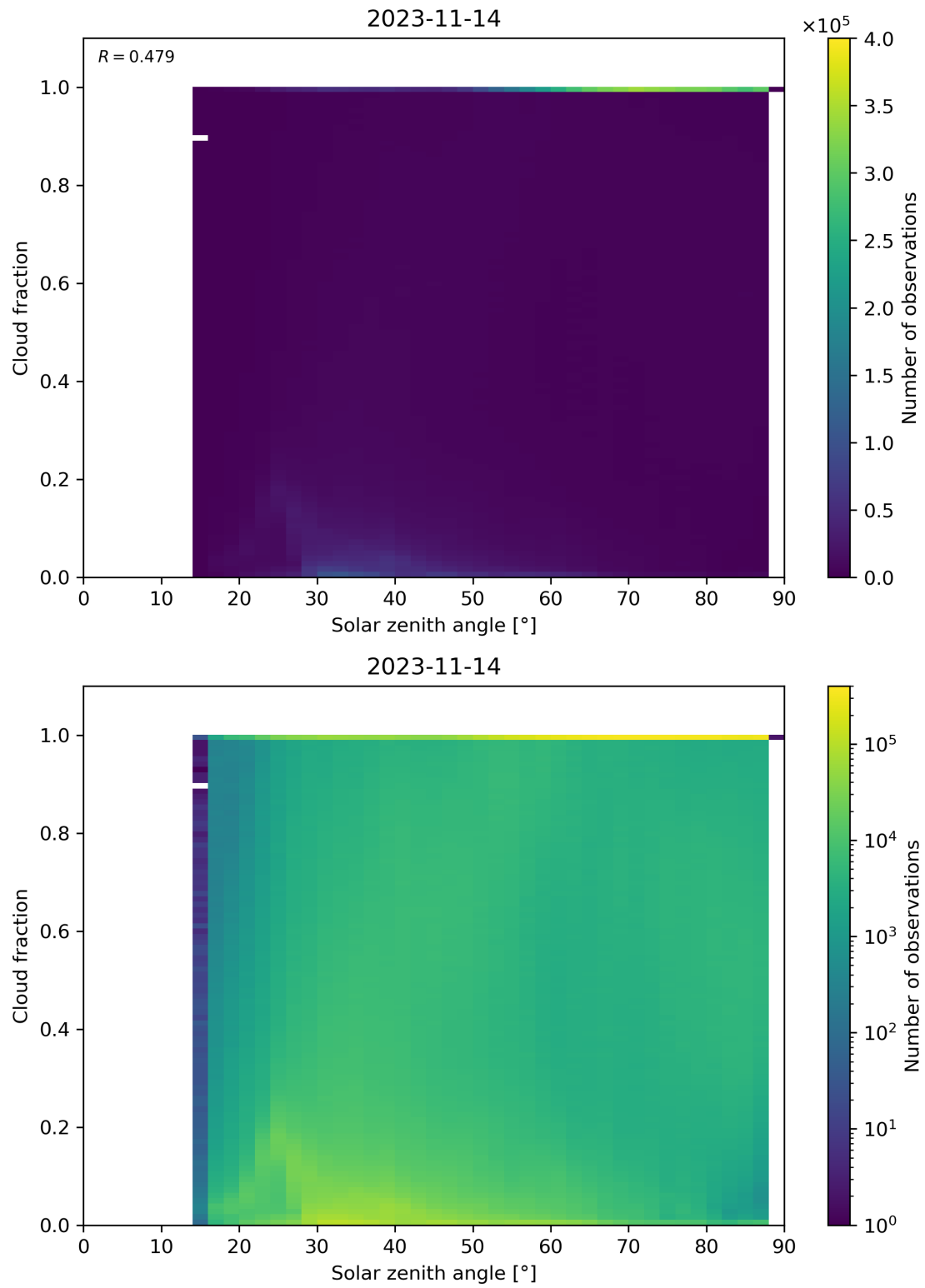
Figure 121: Scatter density plot of “Solar zenith angle” against “Cloud fraction” for 2023-11-13 to 2023-11-15.
