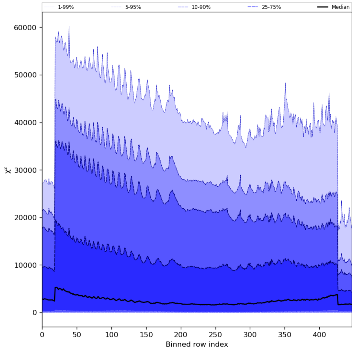
Figure 55: Along track statistics of “ \chi^2 ” for 2023-11-13 to 2023-11-15
