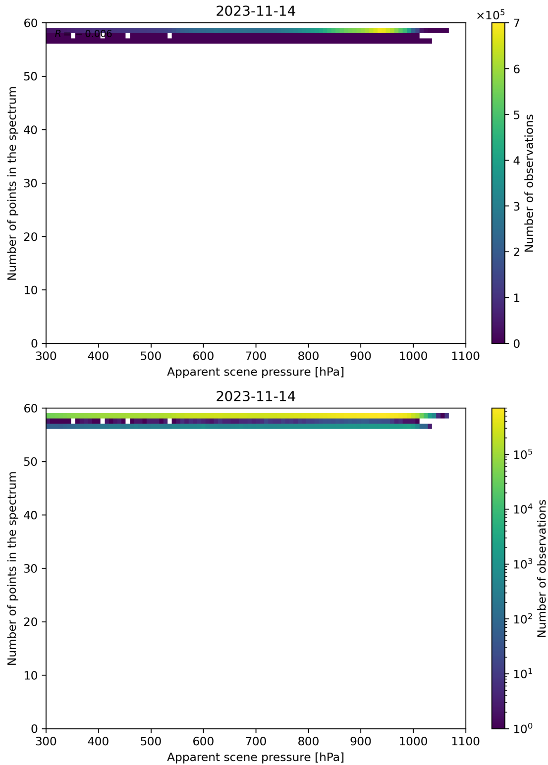
Figure 67: Scatter density plot of “Apparent scene pressure” against “Number of points in the spectrum” for 2023-11-13 to 2023-11-15.
