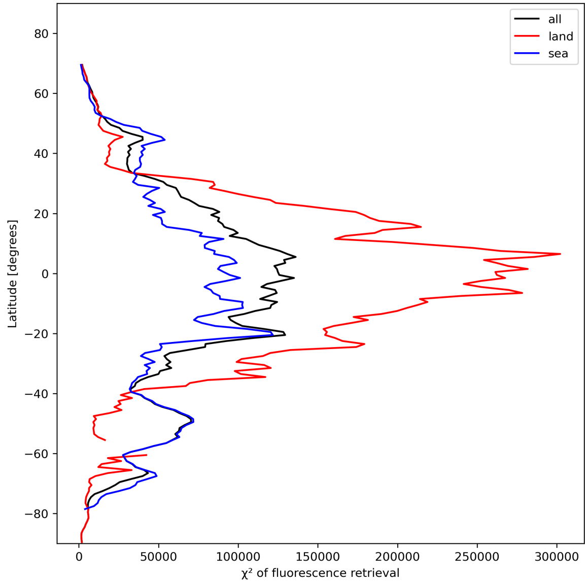
Figure 25: Zonal average of “ \chi^2 of fluorescence retrieval” for 2023-11-13 to 2023-11-15.
