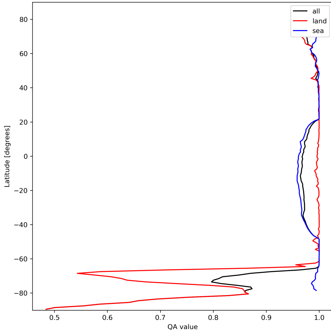
Figure 12: Zonal average of “QA value” for 2023-11-13 to 2023-11-15.
