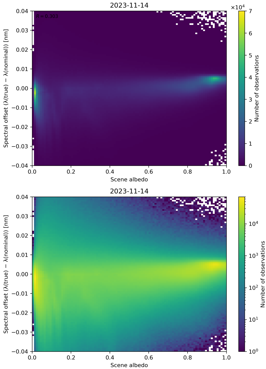
Figure 117: Scatter density plot of “Scene albedo” against “Spectral offset ( \lambda(\text{true}) - \lambda(\text{nominal}) )” for 2023-11-13 to 2023-11-15.
