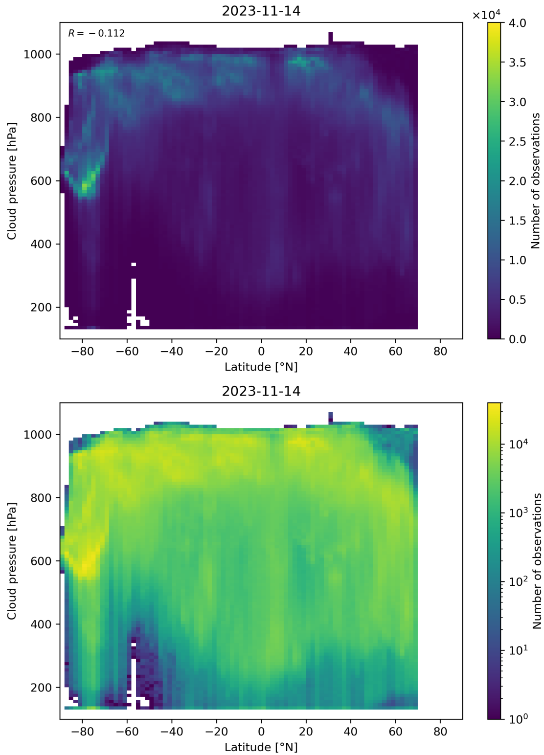
Figure 100: Scatter density plot of “Latitude” against “Cloud pressure” for 2023-11-13 to 2023-11-15.
