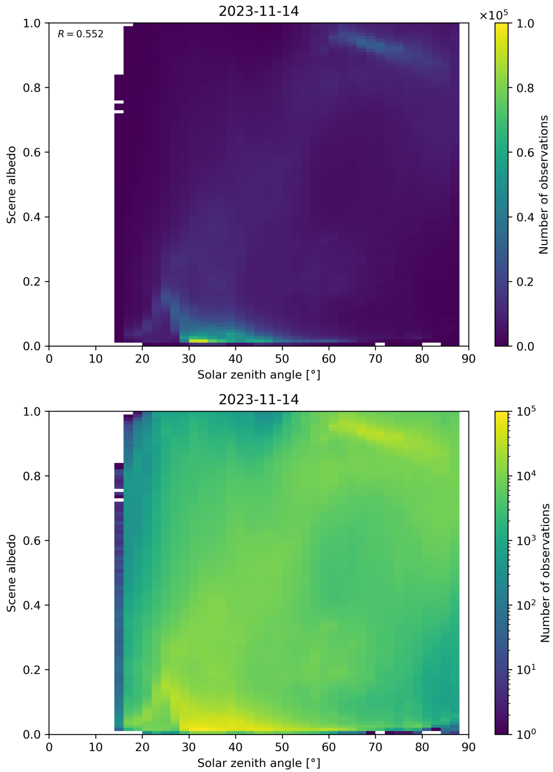
Figure 127: Scatter density plot of “Solar zenith angle” against “Scene albedo” for 2023-11-13 to 2023-11-15.
