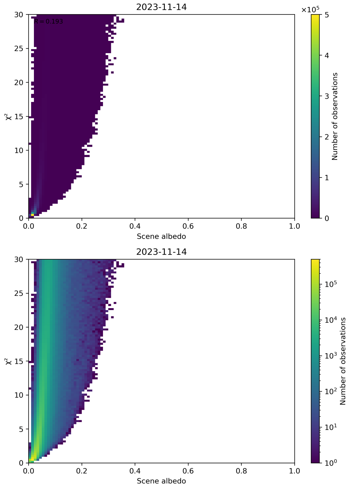
Figure 112: Scatter density plot of “Scene albedo” against “ \chi^2 ” for 2023-11-13 to 2023-11-15.
