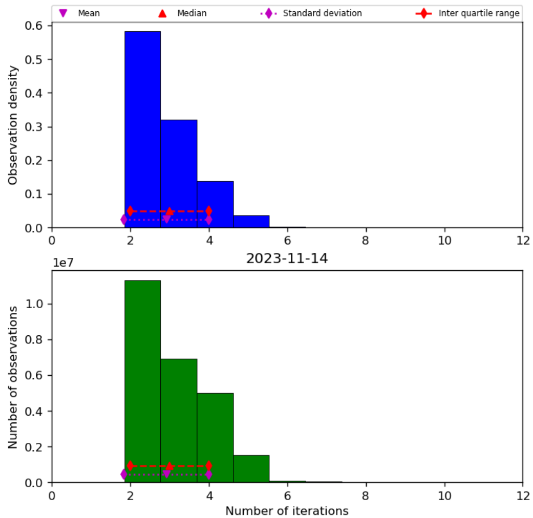
Figure 39: Histogram of “Number of iterations” for 2023-11-13 to 2023-11-15
