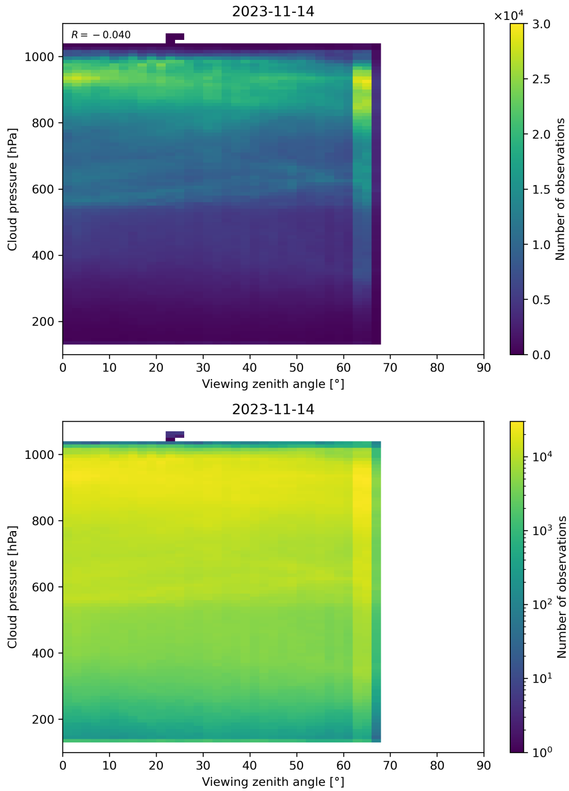
Figure 133: Scatter density plot of “Viewing zenith angle” against “Cloud pressure” for 2023-11-13 to 2023-11-15.
