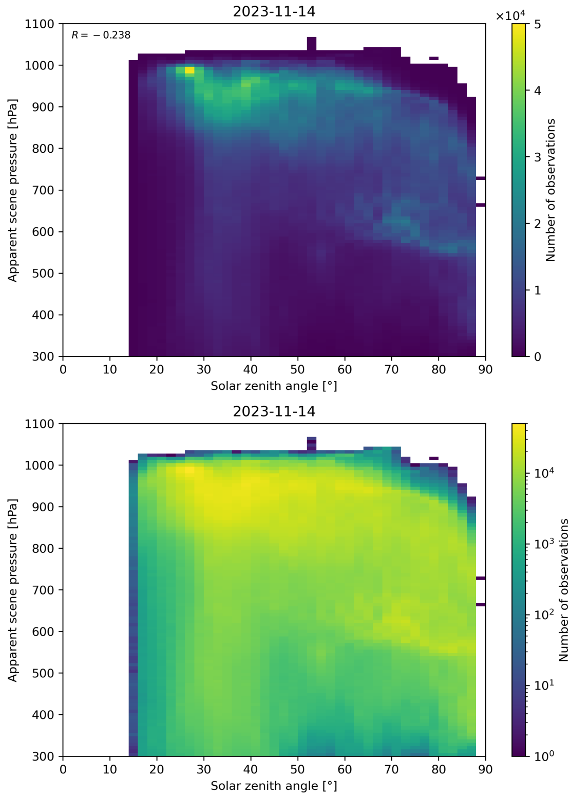
Figure 118: Scatter density plot of “Solar zenith angle” against “Apparent scene pressure” for 2023-11-13 to 2023-11-15.
