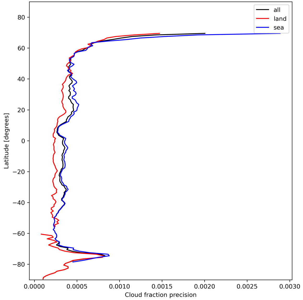
Figure 16: Zonal average of “Cloud fraction precision” for 2023-11-13 to 2023-11-15.
