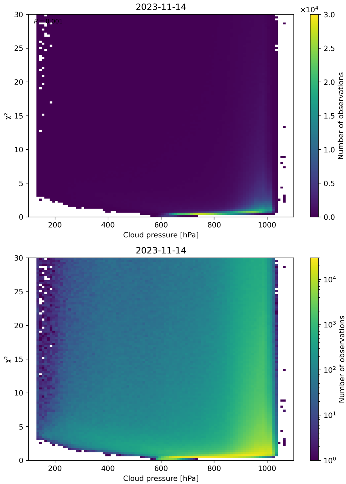
Figure 85: Scatter density plot of “Cloud pressure” against “ \chi^2 ” for 2023-11-13 to 2023-11-15.
