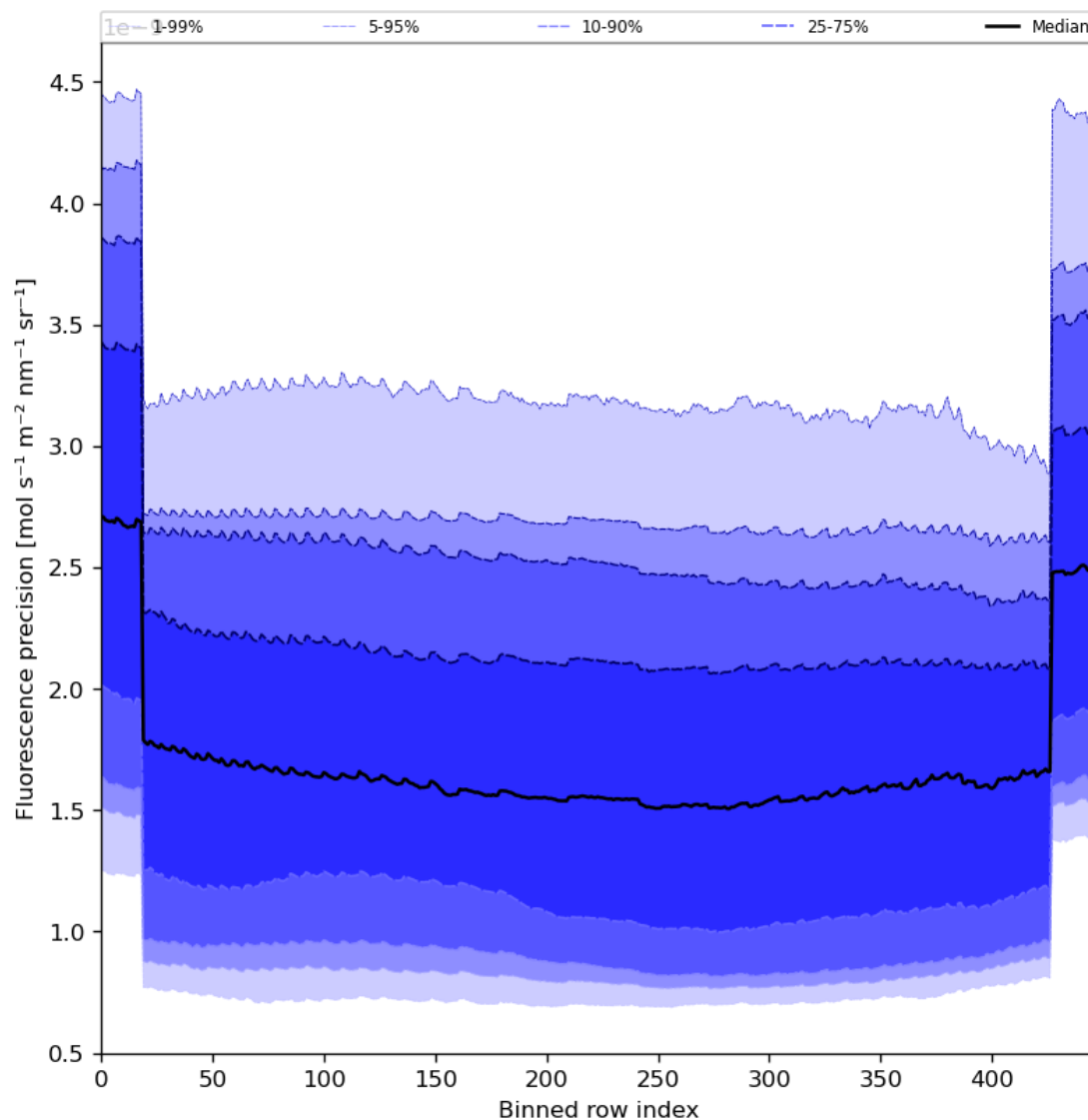
Figure 58: Along track statistics of “Fluorescence precision” for 2023-11-13 to 2023-11-15
