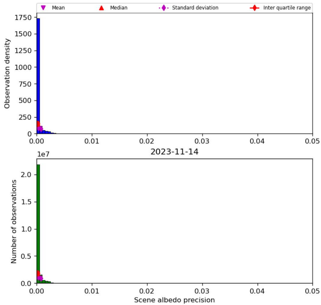
Figure 35: Histogram of “Scene albedo precision” for 2023-11-13 to 2023-11-15
