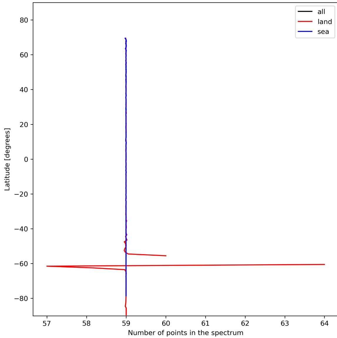
Figure 27: Zonal average of “Number of points in the spectrum” for 2023-11-13 to 2023-11-15.
