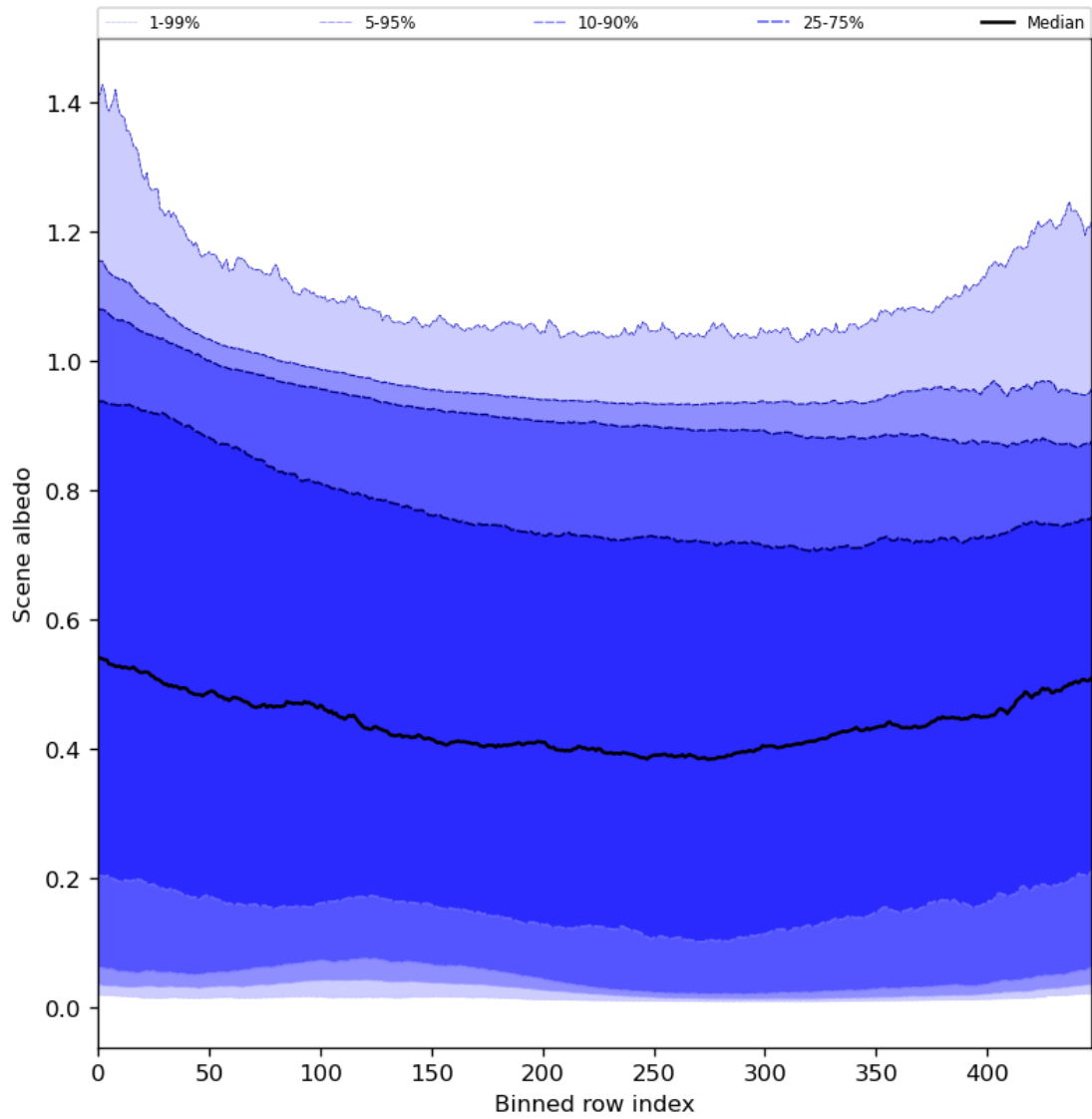
Figure 51: Along track statistics of “Scene albedo” for 2023-11-13 to 2023-11-15
