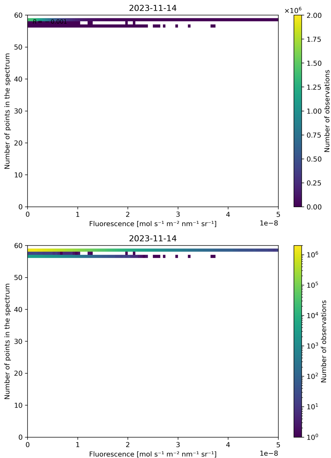
Figure 94: Scatter density plot of “Fluorescence” against “Number of points in the spectrum” for 2023-11-13 to 2023-11-15.
