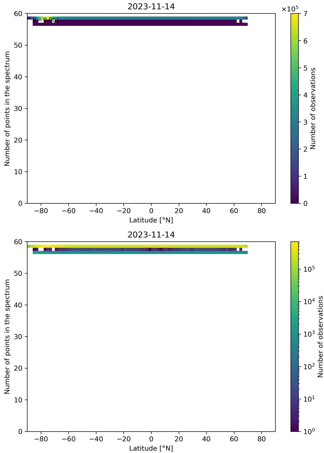
Figure 103: Scatter density plot of “Latitude” against “Number of points in the spectrum” for 2023-11-13 to 2023-11-15.
