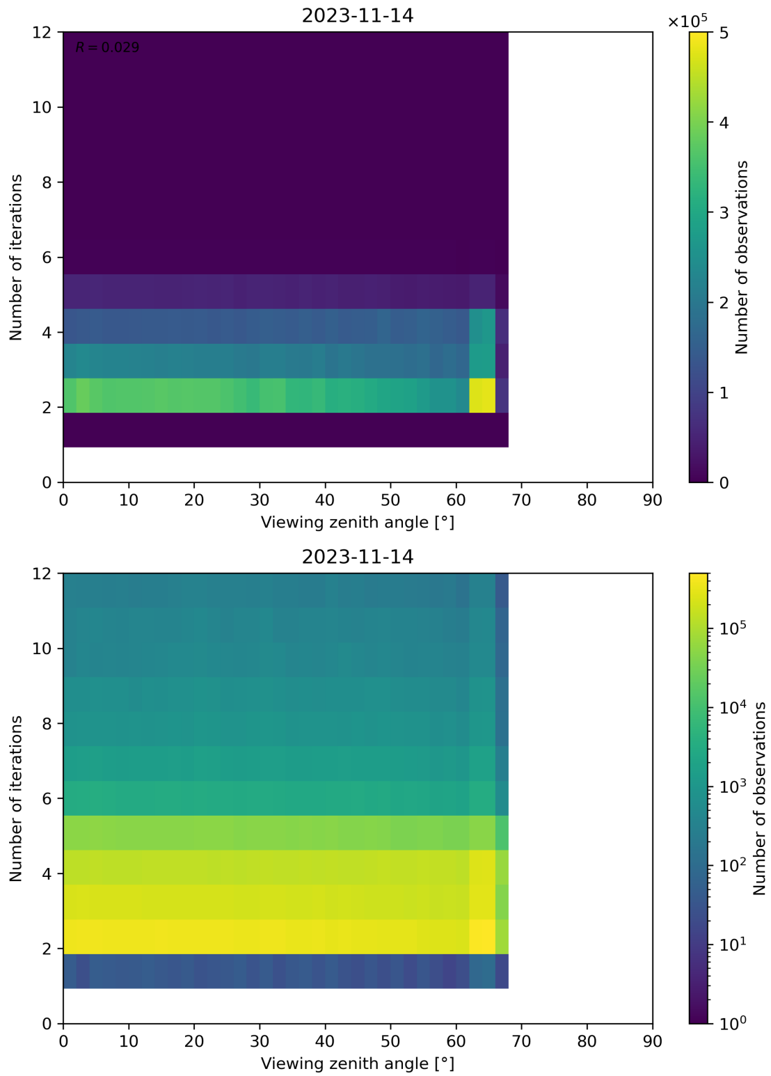
Figure 136: Scatter density plot of “Viewing zenith angle” against “Number of iterations” for 2023-11-13 to 2023-11-15.
