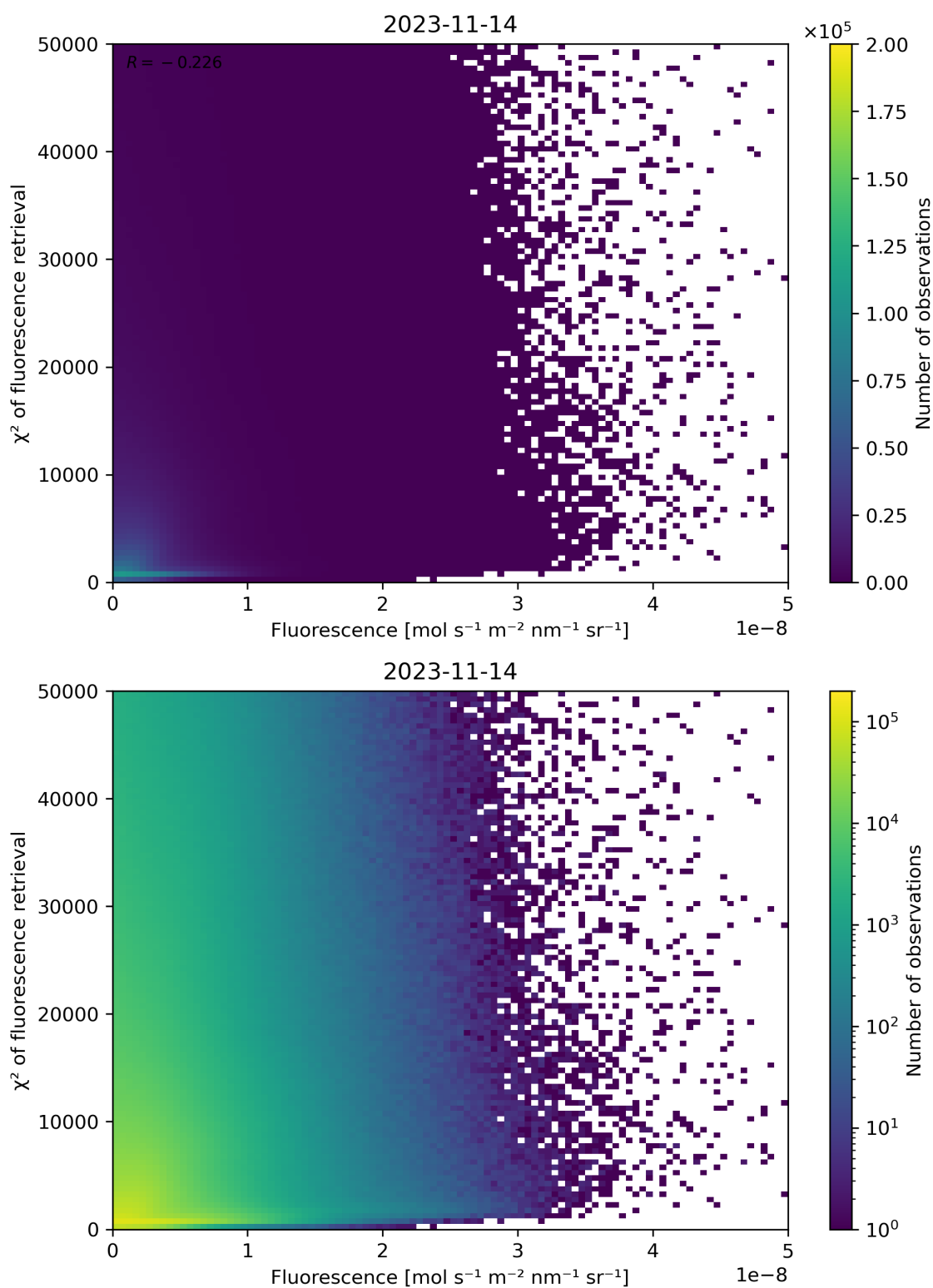
Figure 93: Scatter density plot of “Fluorescence” against “ \chi^2 of fluorescence retrieval” for 2023-11-13 to 2023-11-15.
