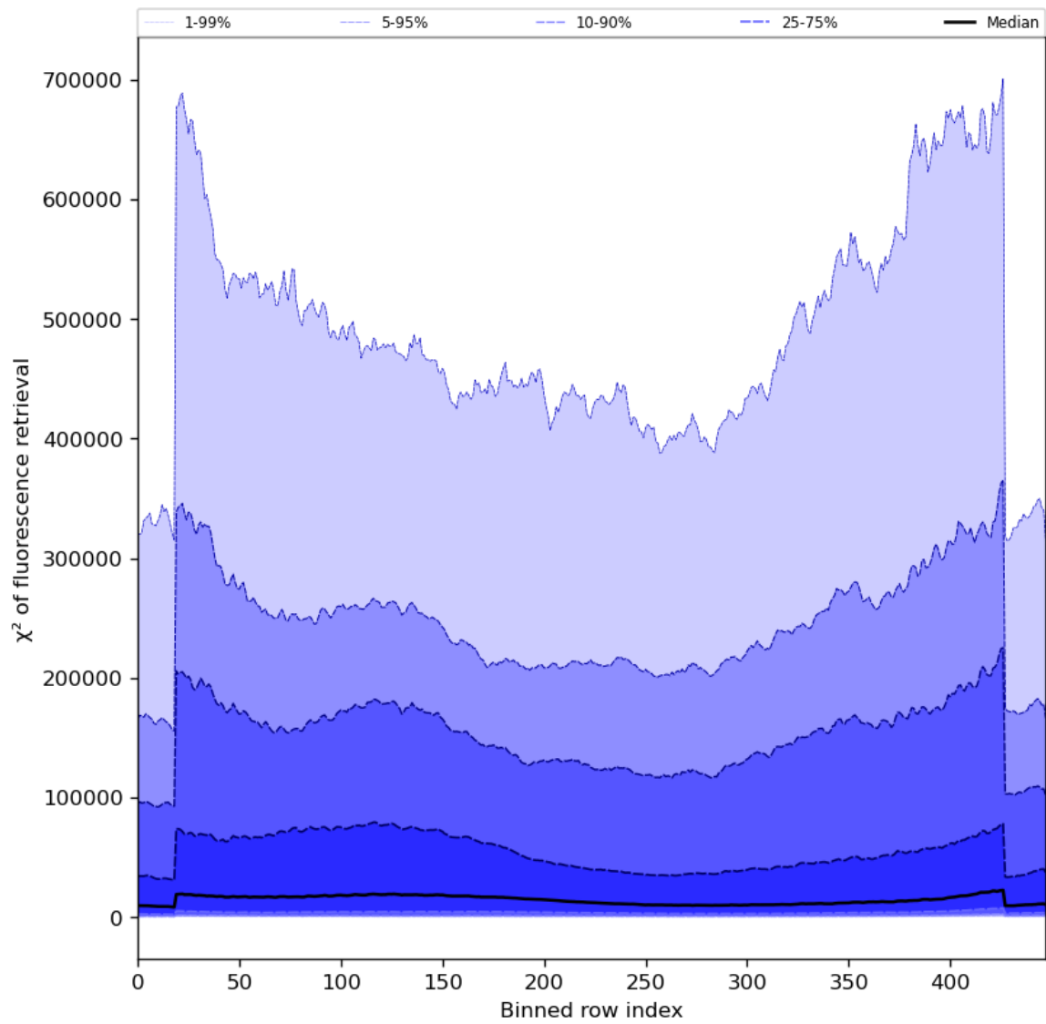
Figure 59: Along track statistics of “ \chi^2 of fluorescence retrieval” for 2023-11-13 to 2023-11-15
