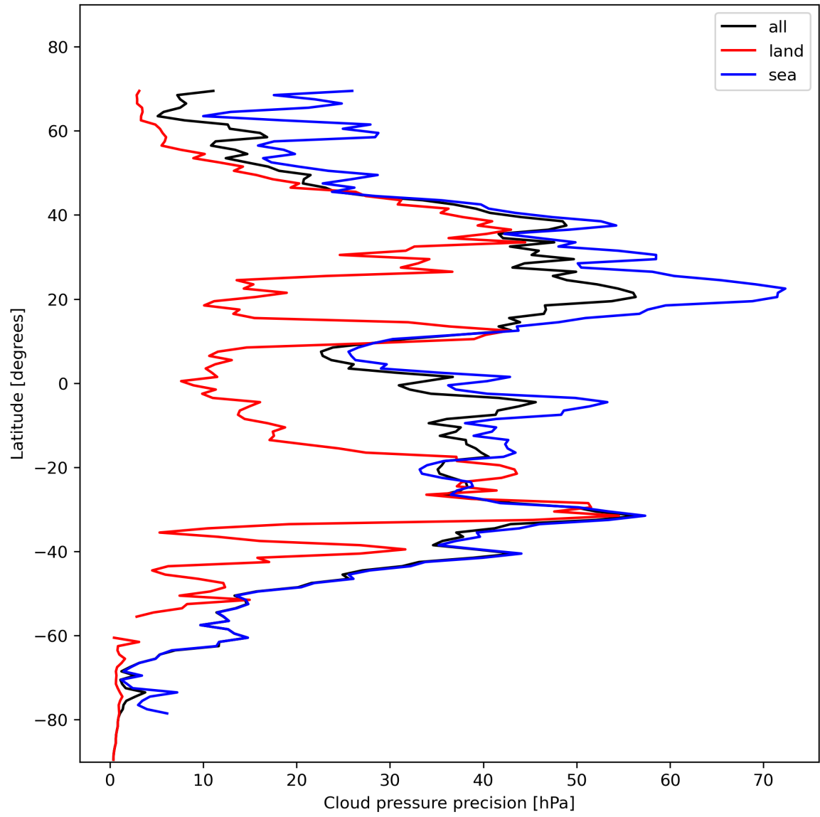
Figure 14: Zonal average of “Cloud pressure precision” for 2023-11-13 to 2023-11-15.
