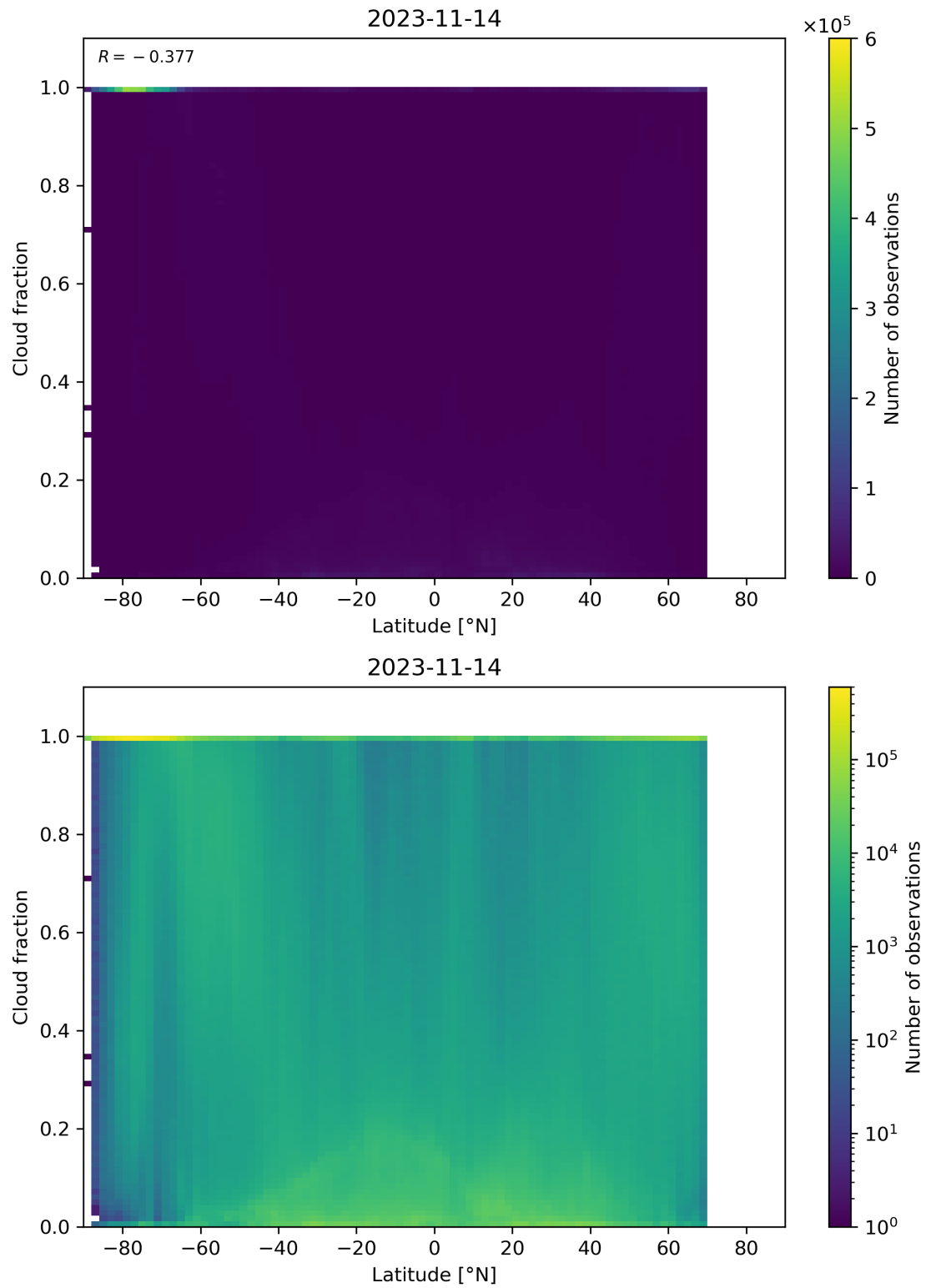
Figure 99: Scatter density plot of “Latitude” against “Cloud fraction” for 2023-11-13 to 2023-11-15.
