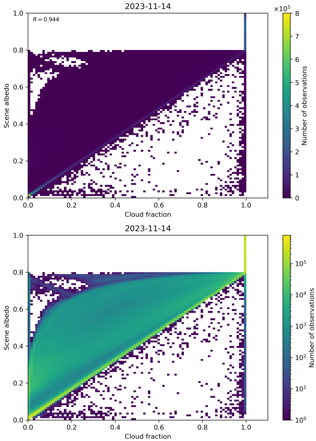
Figure 82: Scatter density plot of “Cloud fraction” against “Scene albedo” for 2023-11-13 to 2023-11-15.
