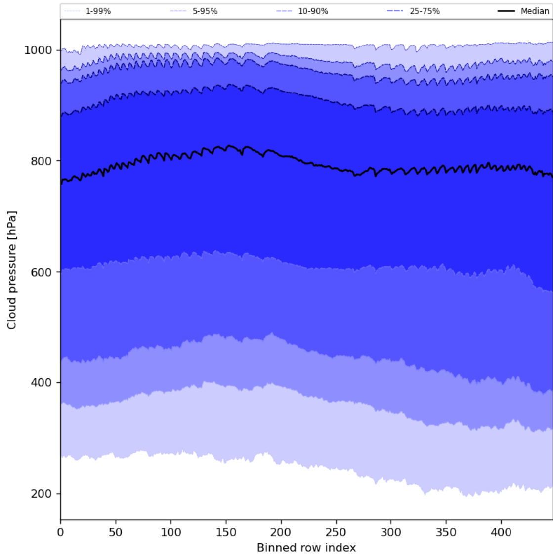
Figure 47: Along track statistics of “Cloud pressure” for 2023-11-13 to 2023-11-15
