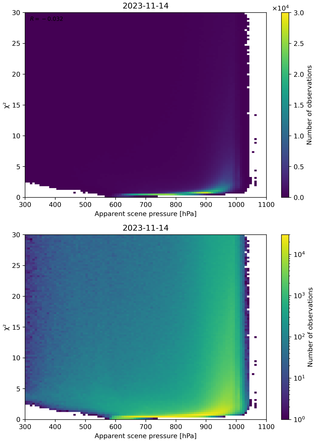
Figure 63: Scatter density plot of “Apparent scene pressure” against “ \chi^2 ” for 2023-11-13 to 2023-11-15.
