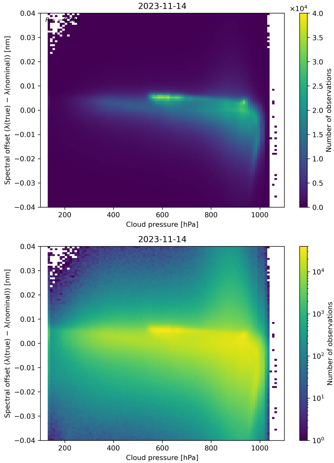
Figure 92: Scatter density plot of “Cloud pressure” against “Spectral offset ( \lambda(\text{true}) - \lambda(\text{nominal}) )” for 2023-11-13 to 2023-11-15.
