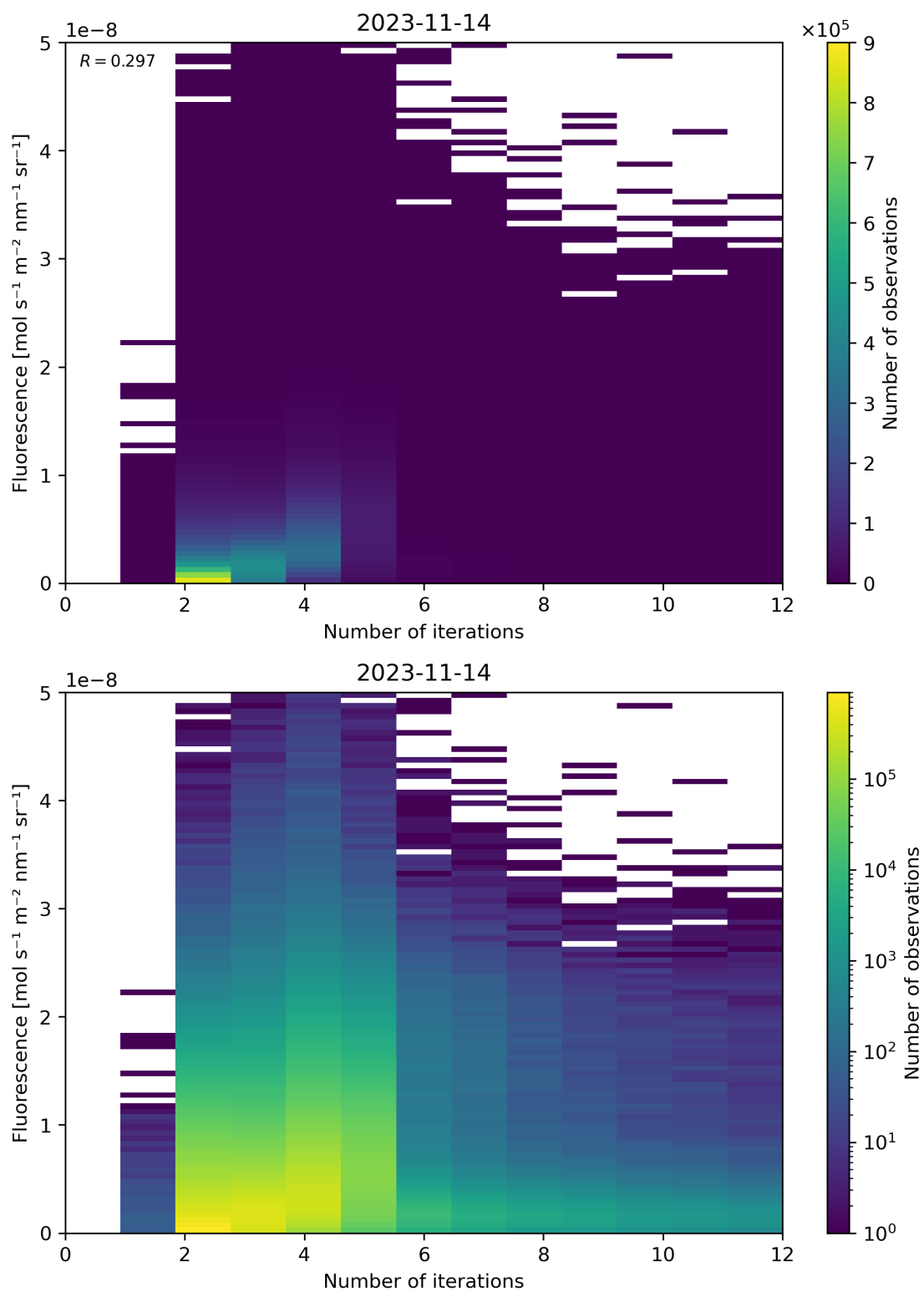
Figure 107: Scatter density plot of “Number of iterations” against “Fluorescence” for 2023-11-13 to 2023-11-15.
