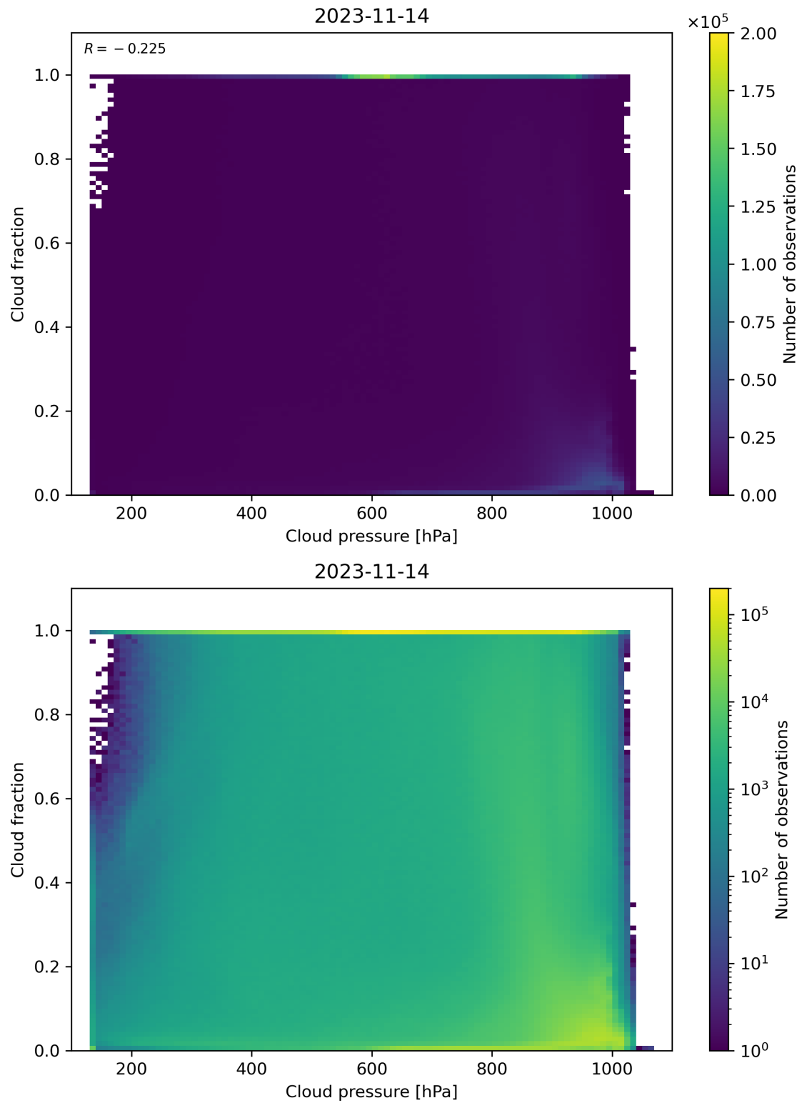
Figure 87: Scatter density plot of “Cloud pressure” against “Cloud fraction” for 2023-11-13 to 2023-11-15.
