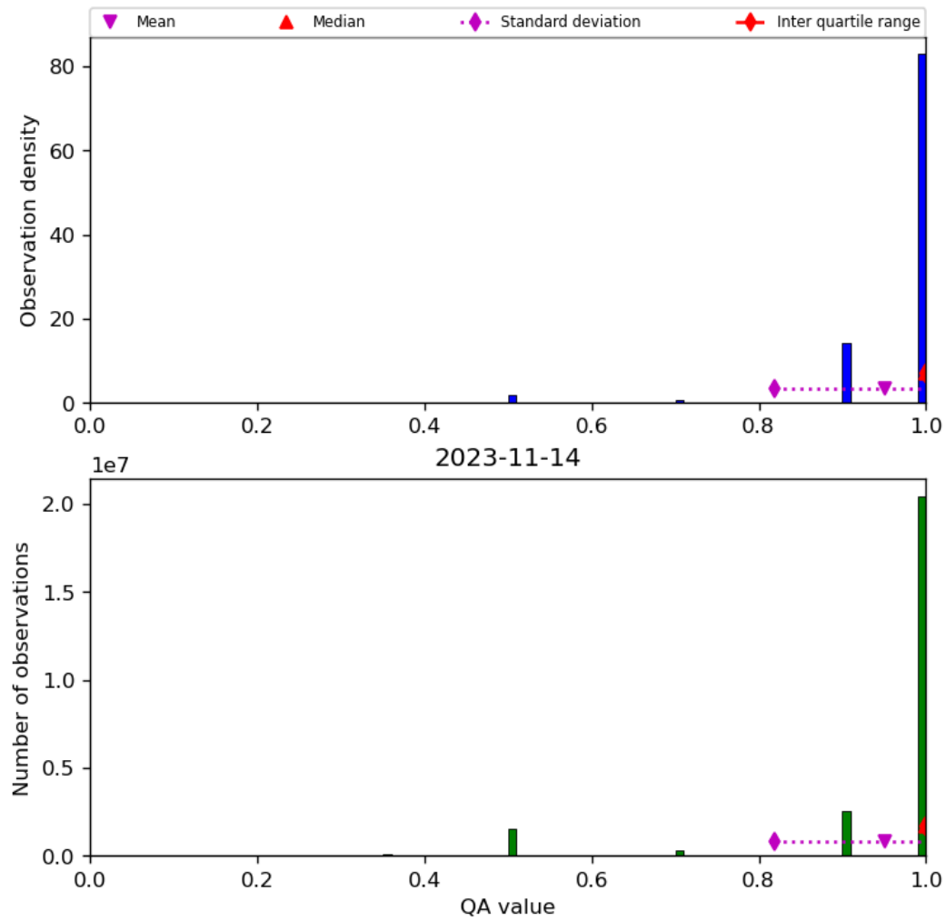
Figure 29: Histogram of “QA value” for 2023-11-13 to 2023-11-15
