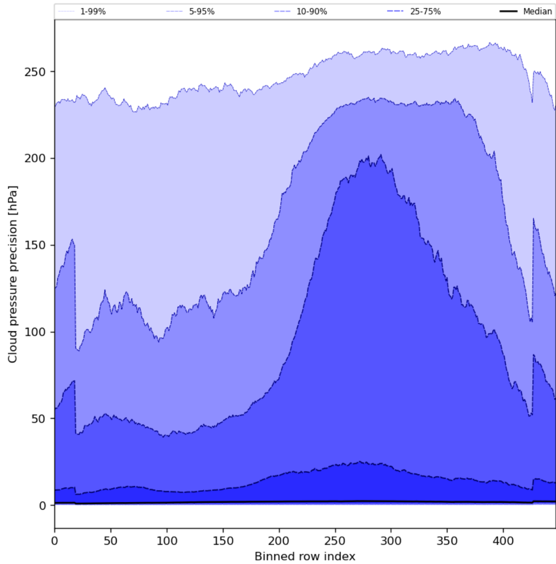
Figure 48: Along track statistics of “Cloud pressure precision” for 2023-11-13 to 2023-11-15
