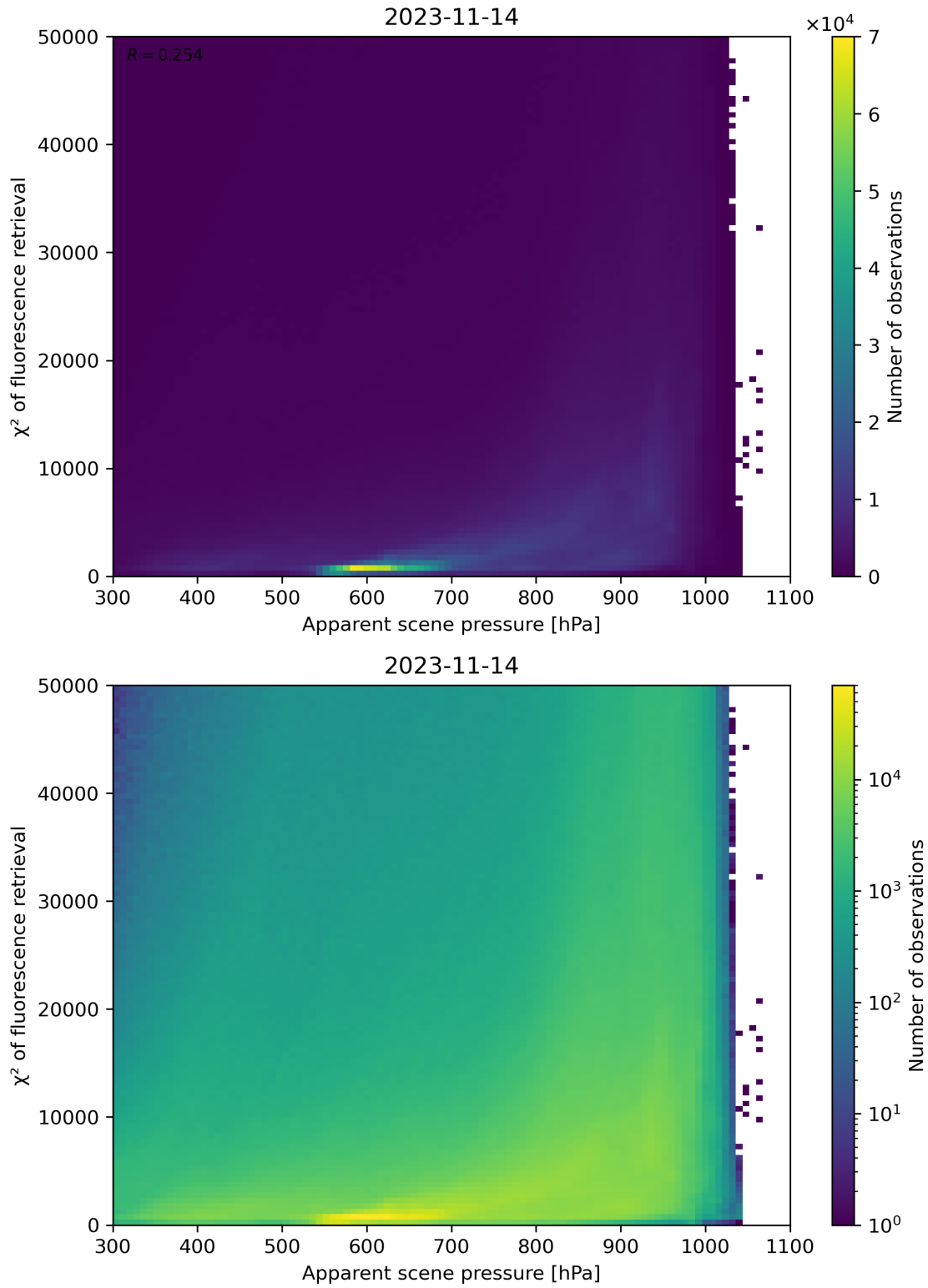
Figure 64: Scatter density plot of “Apparent scene pressure” against “ \chi^2 of fluorescence retrieval” for 2023-11-13 to 2023-11-15.
