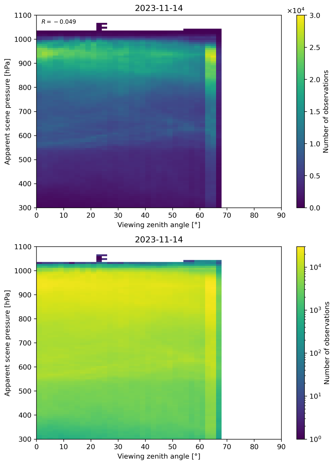
Figure 129: Scatter density plot of “Viewing zenith angle” against “Apparent scene pressure” for 2023-11-13 to 2023-11-15.
