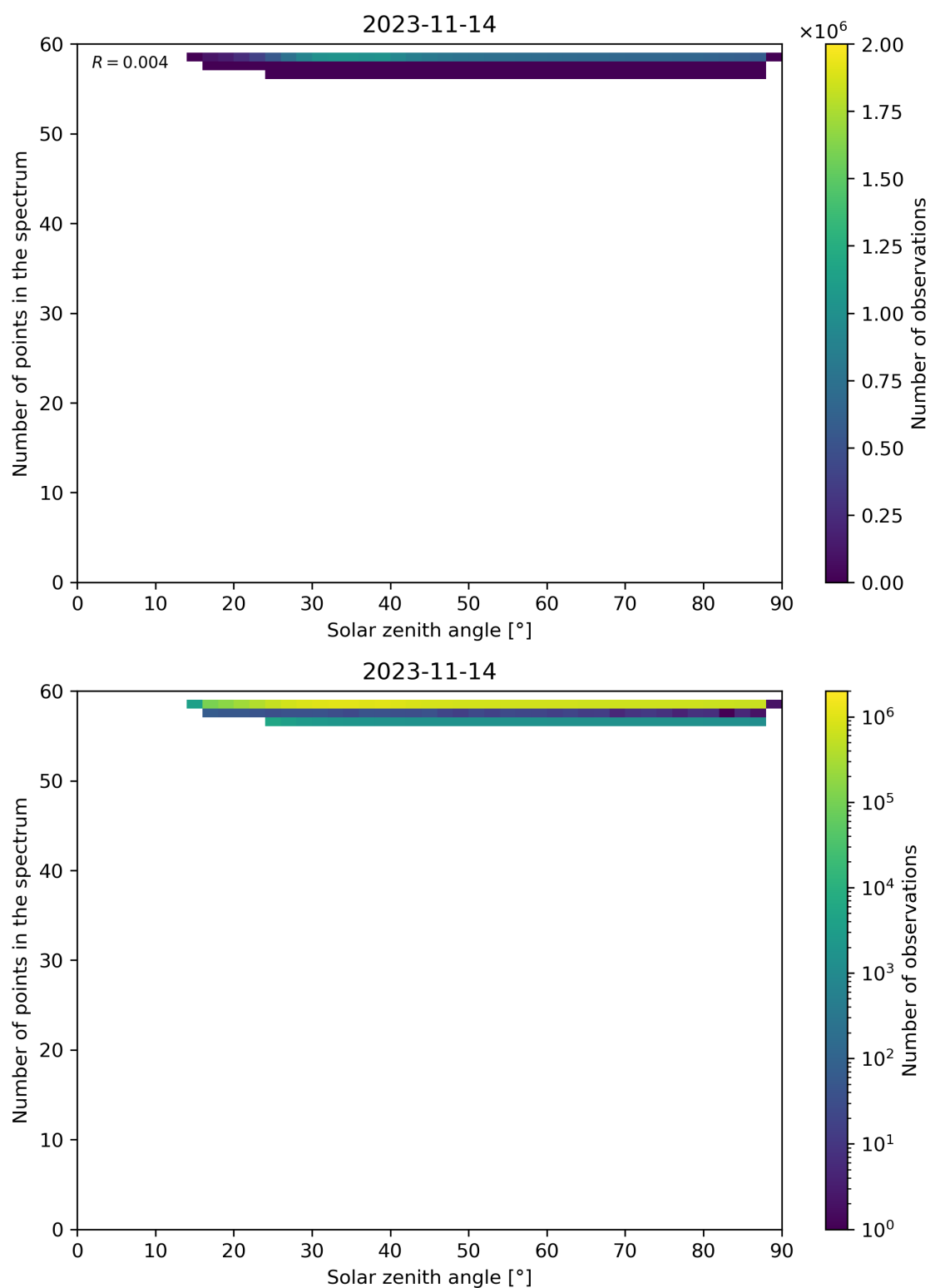
Figure 126: Scatter density plot of “Solar zenith angle” against “Number of points in the spectrum” for 2023-11-13 to 2023-11-15.
