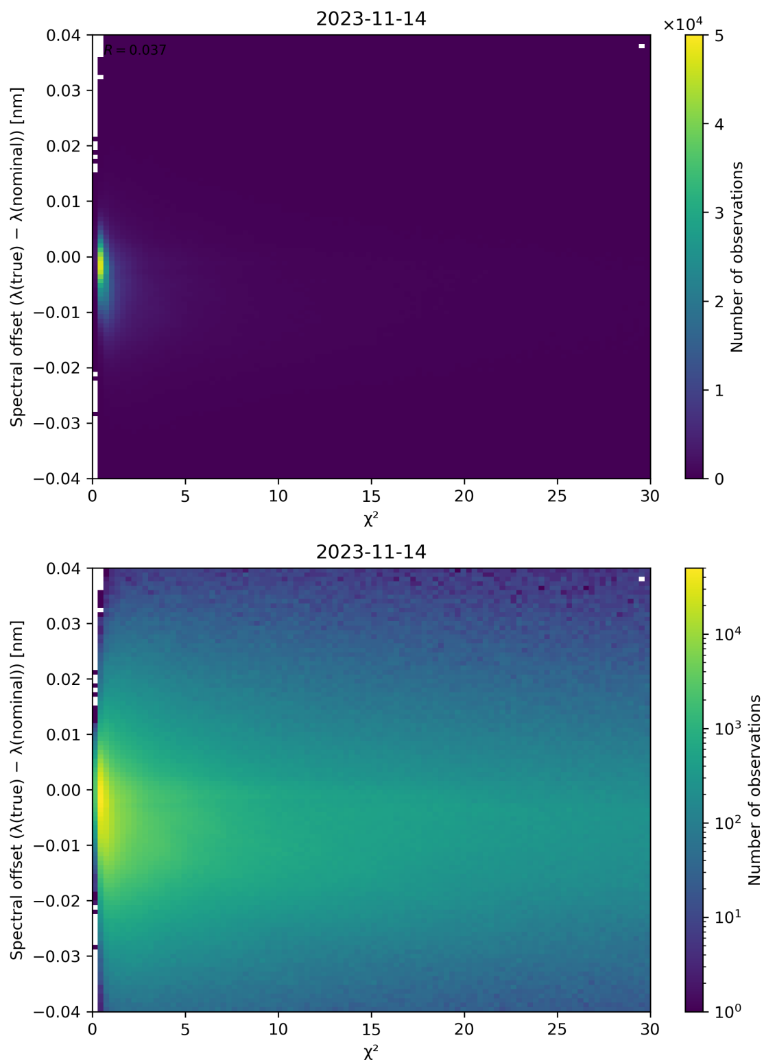
Figure 75: Scatter density plot of " \chi^2 " against "Spectral offset ( \lambda(\text{true}) - \lambda(\text{nominal})) " for 2023-11-13 to 2023-11-15.
