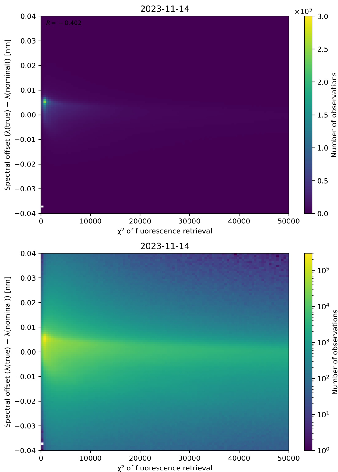
Figure 72: Scatter density plot of “ \chi^2 of fluorescence retrieval” against “Spectral offset ( \lambda(\text{true}) - \lambda(\text{nominal}) )” for 2023-11-13 to 2023-11-15.
