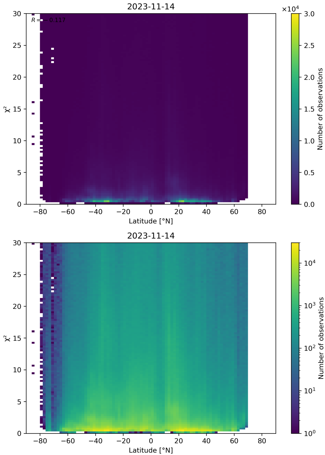
Figure 97: Scatter density plot of “Latitude” against “ \chi^2 ” for 2023-11-13 to 2023-11-15.
