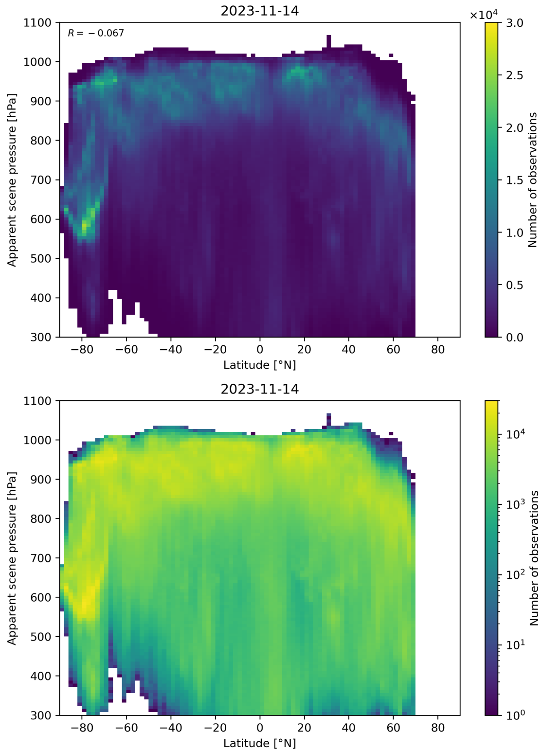
Figure 96: Scatter density plot of “Latitude” against “Apparent scene pressure” for 2023-11-13 to 2023-11-15.
