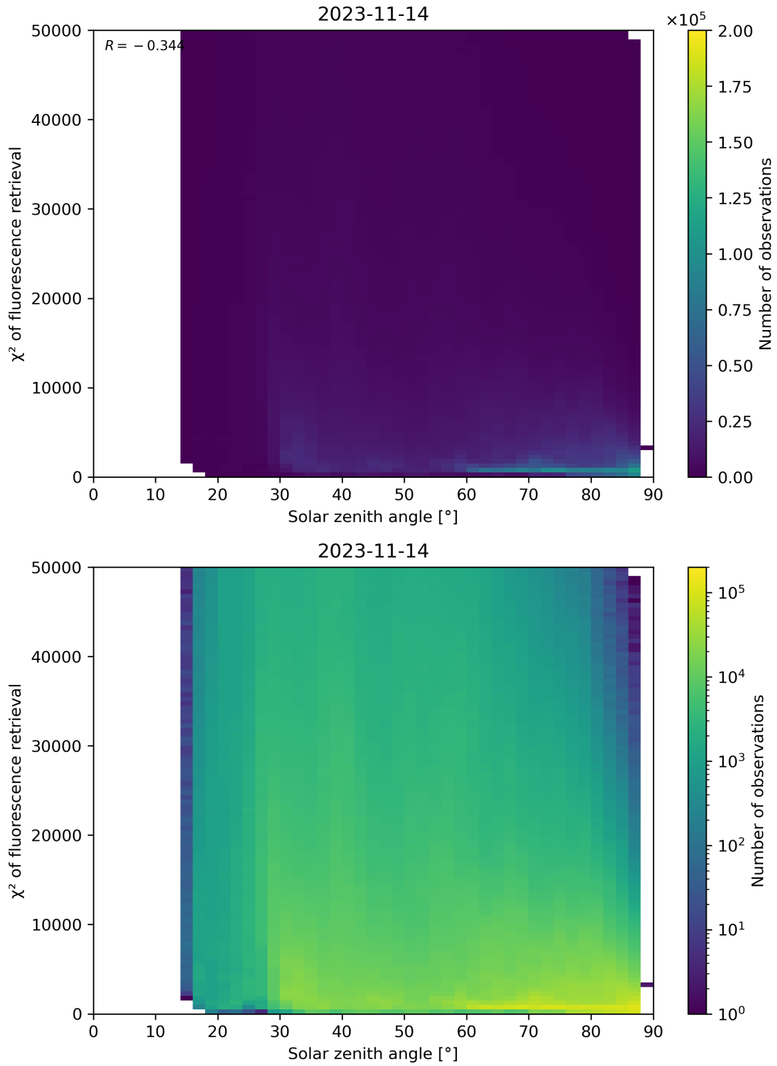
Figure 120: Scatter density plot of “Solar zenith angle” against “ \chi^2 of fluorescence retrieval” for 2023-11-13 to 2023-11-15.
