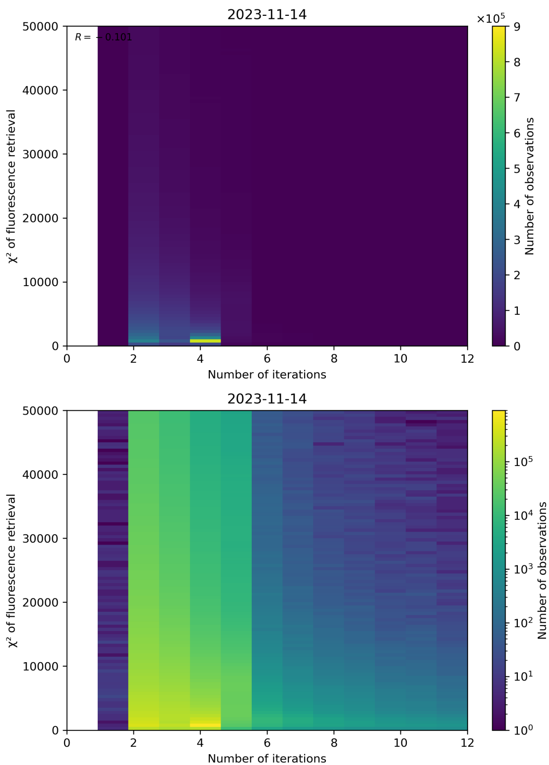
Figure 106: Scatter density plot of “Number of iterations” against “ \chi^2 of fluorescence retrieval” for 2023-11-13 to 2023-11-15.
