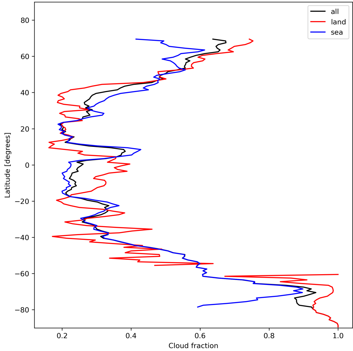
Figure 15: Zonal average of “Cloud fraction” for 2023-11-13 to 2023-11-15.
