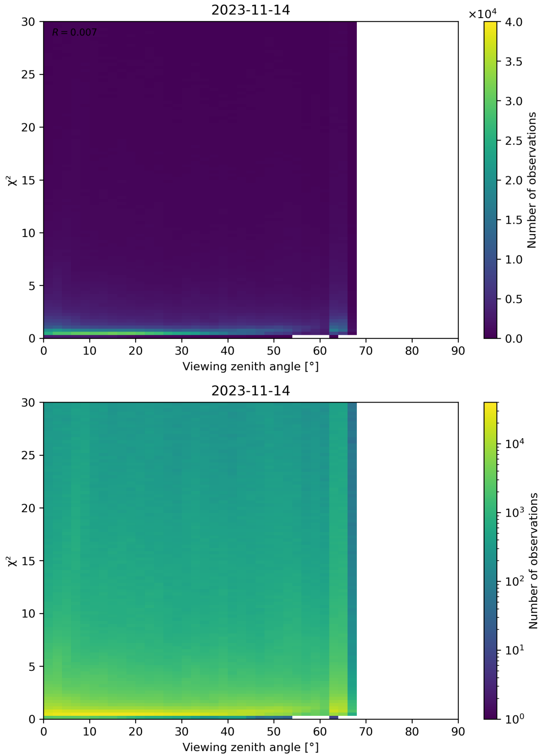
Figure 130: Scatter density plot of “Viewing zenith angle” against “ \chi^2 ” for 2023-11-13 to 2023-11-15.
