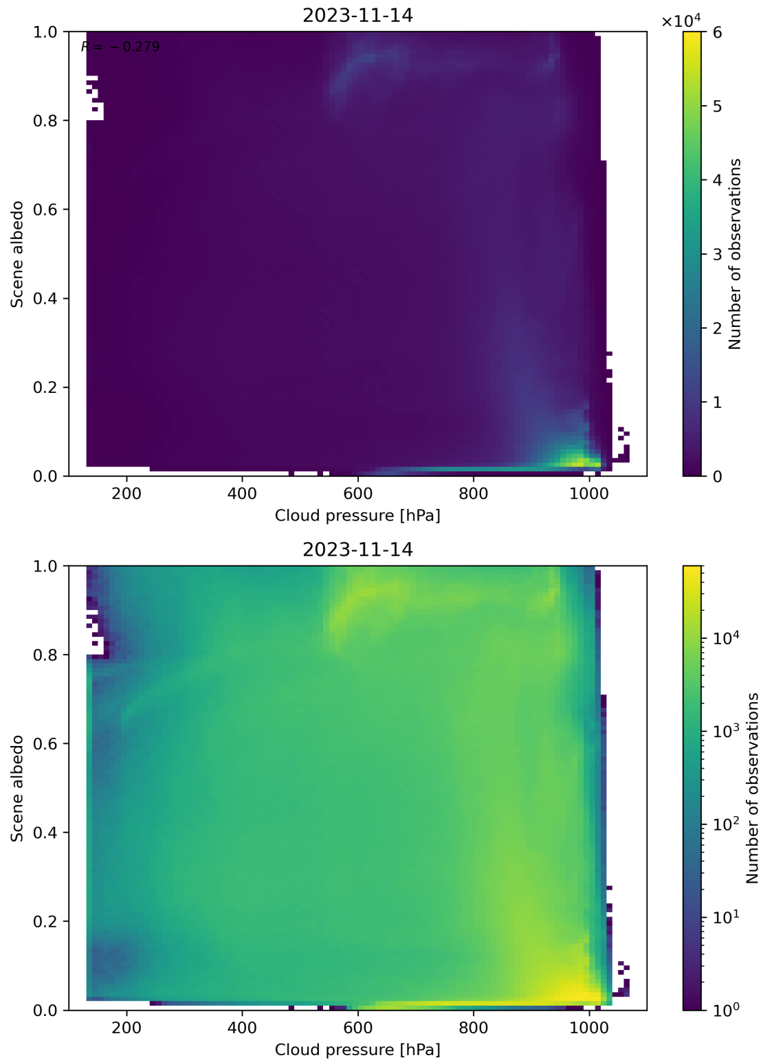
Figure 91: Scatter density plot of “Cloud pressure” against “Scene albedo” for 2023-11-13 to 2023-11-15.
