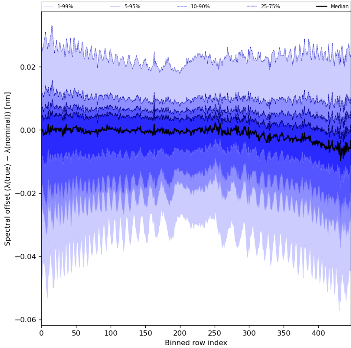
Figure 62: Along track statistics of “Spectral offset ( \lambda(\text{true}) - \lambda(\text{nominal}) )” for 2023-11-13 to 2023-11-15
