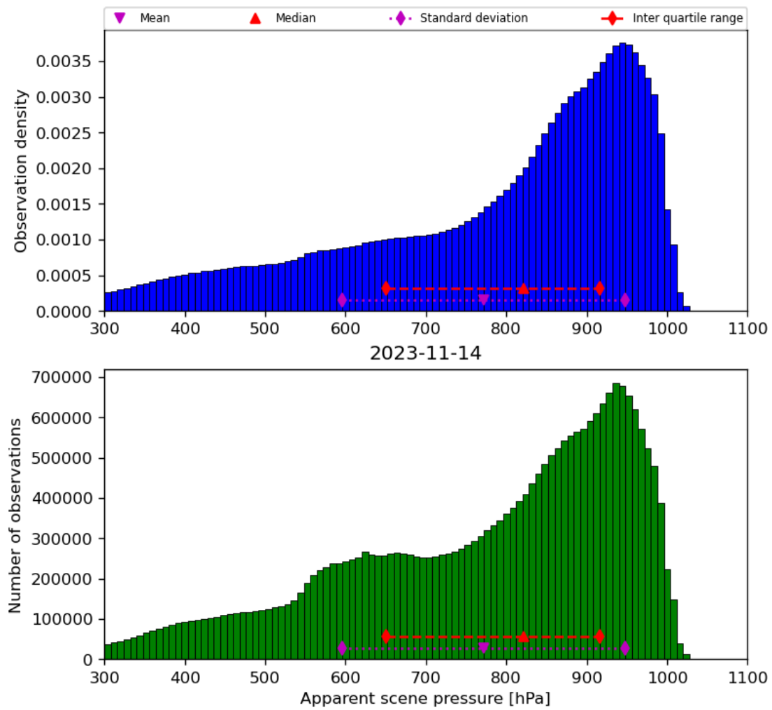
Figure 36: Histogram of “Apparent scene pressure” for 2023-11-13 to 2023-11-15
