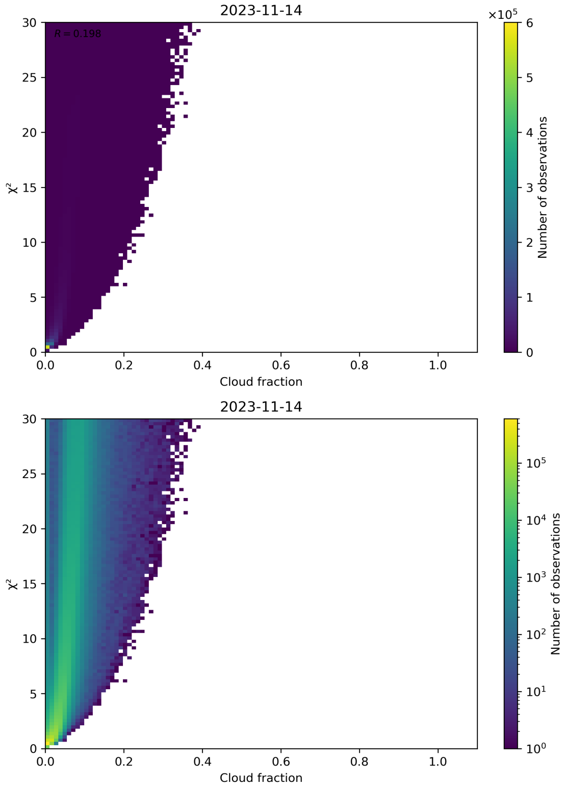
Figure 77: Scatter density plot of “Cloud fraction” against “ \chi^2 ” for 2023-11-13 to 2023-11-15.
