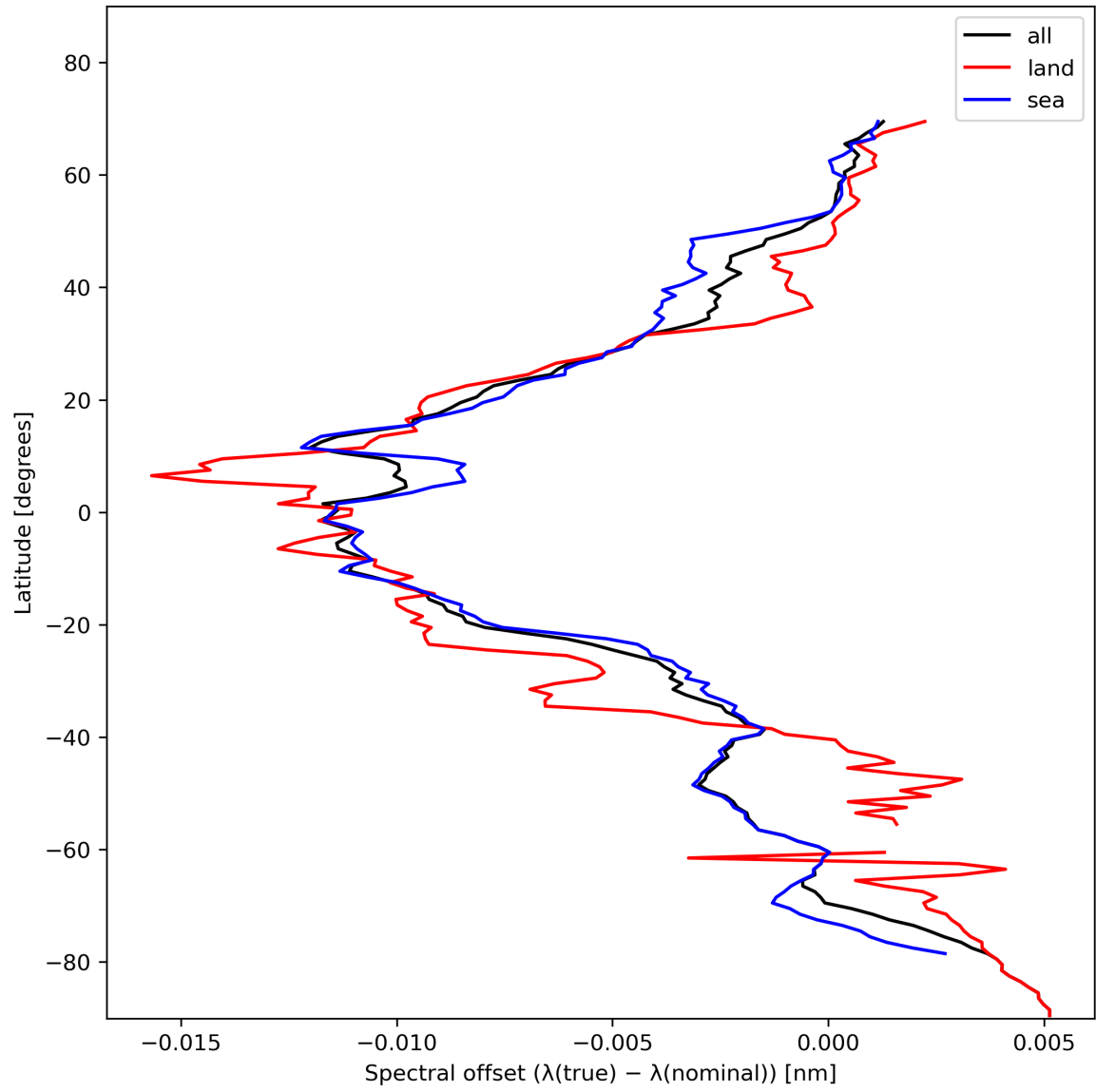
Figure 28: Zonal average of “Spectral offset ( \lambda(\text{true}) - \lambda(\text{nominal}) )” for 2023-11-13 to 2023-11-15.
