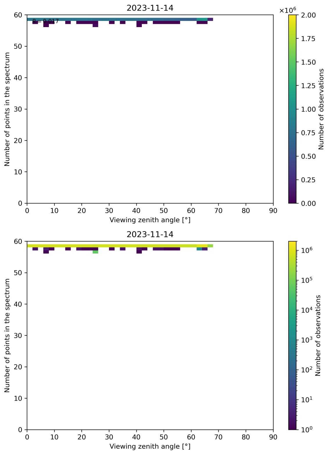
Figure 137: Scatter density plot of “Viewing zenith angle” against “Number of points in the spectrum” for 2023-11-13 to 2023-11-15.
