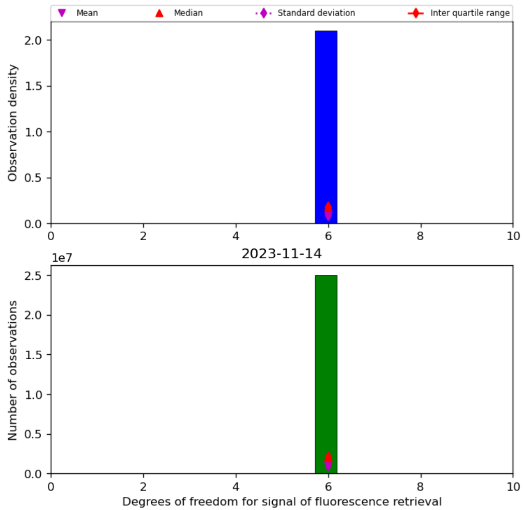
Figure 43: Histogram of “Degrees of freedom for signal of fluorescence retrieval” for 2023-11-13 to 2023-11-15
