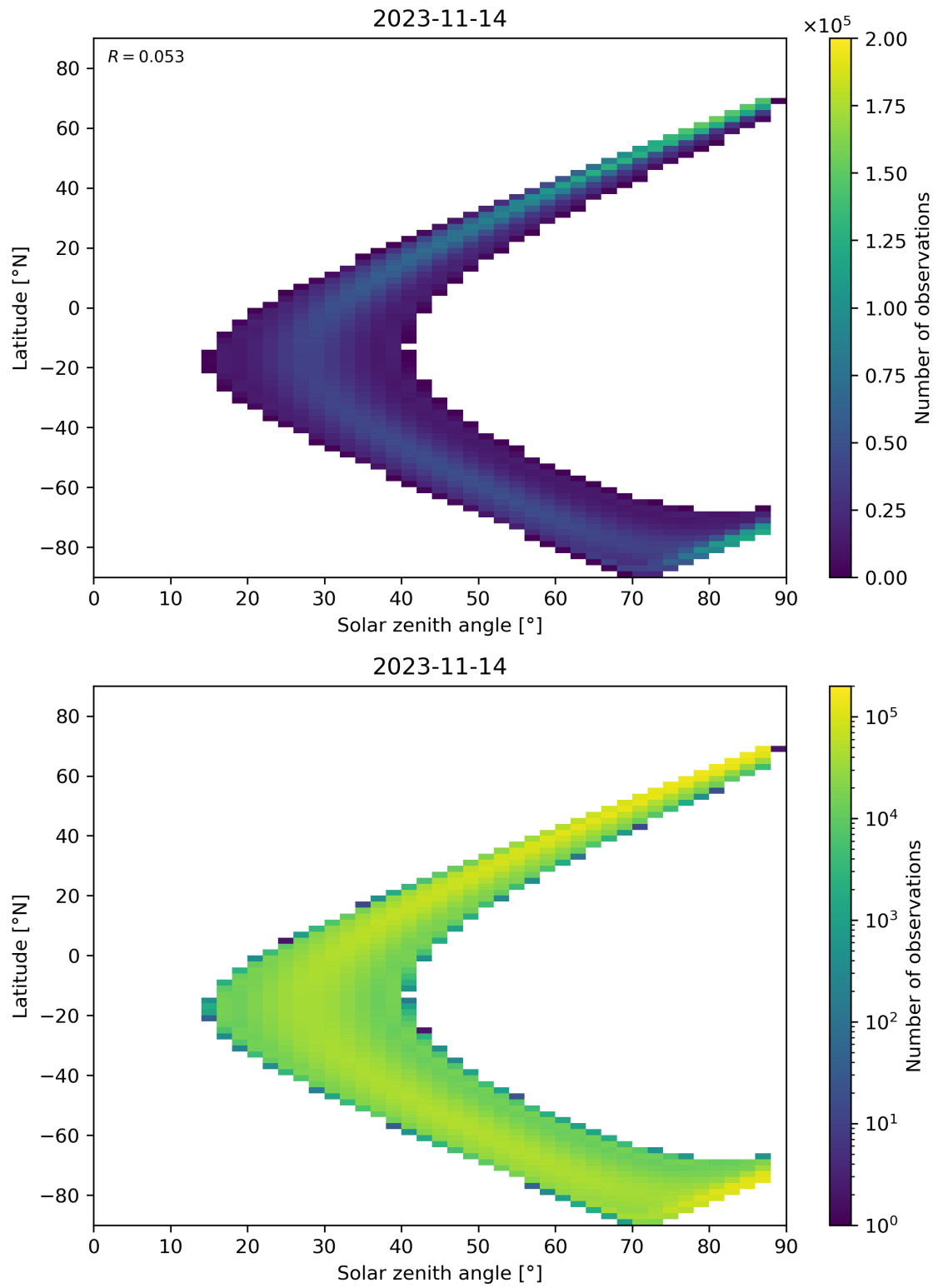
Figure 124: Scatter density plot of “Solar zenith angle” against “Latitude” for 2023-11-13 to 2023-11-15.
