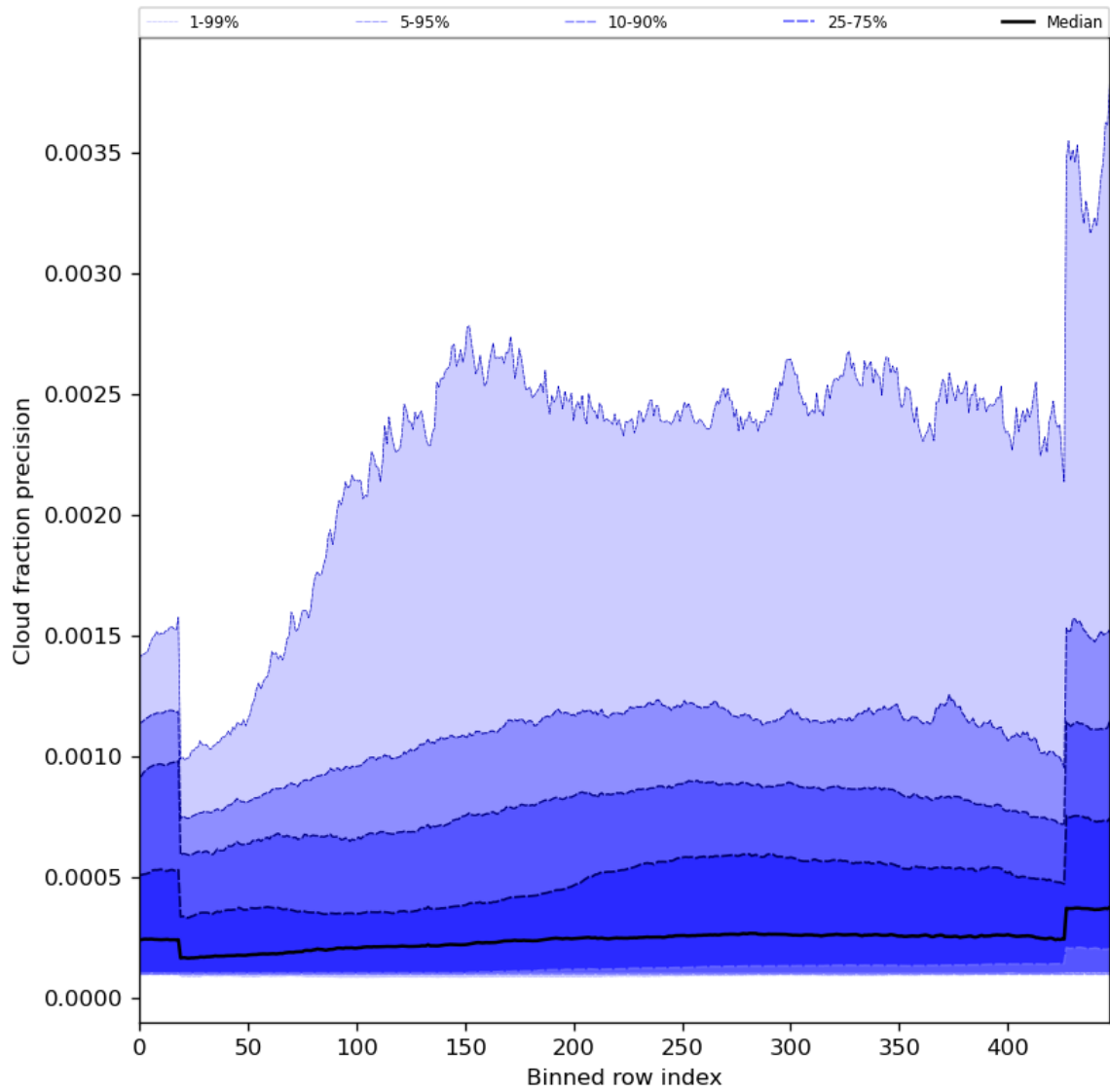
Figure 50: Along track statistics of “Cloud fraction precision” for 2023-11-13 to 2023-11-15
