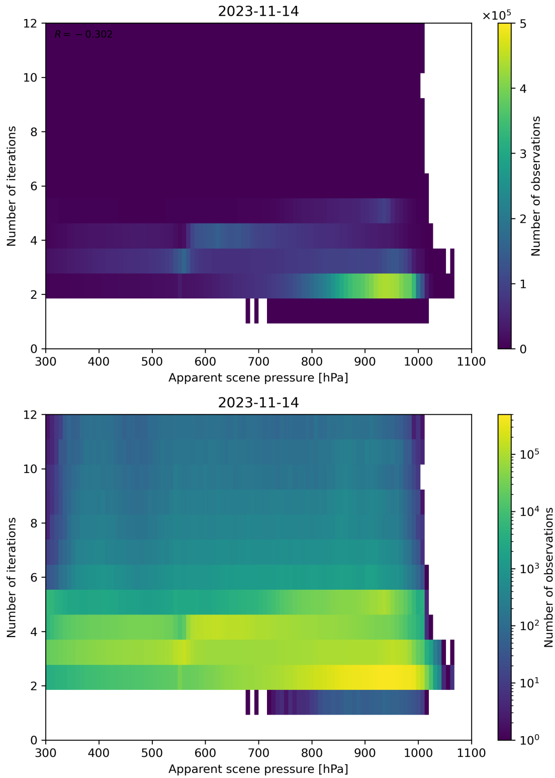
Figure 66: Scatter density plot of “Apparent scene pressure” against “Number of iterations” for 2023-11-13 to 2023-11-15.
