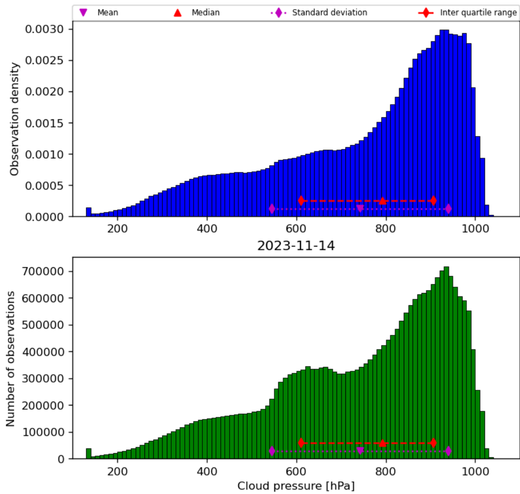
Figure 30: Histogram of “Cloud pressure” for 2023-11-13 to 2023-11-15
