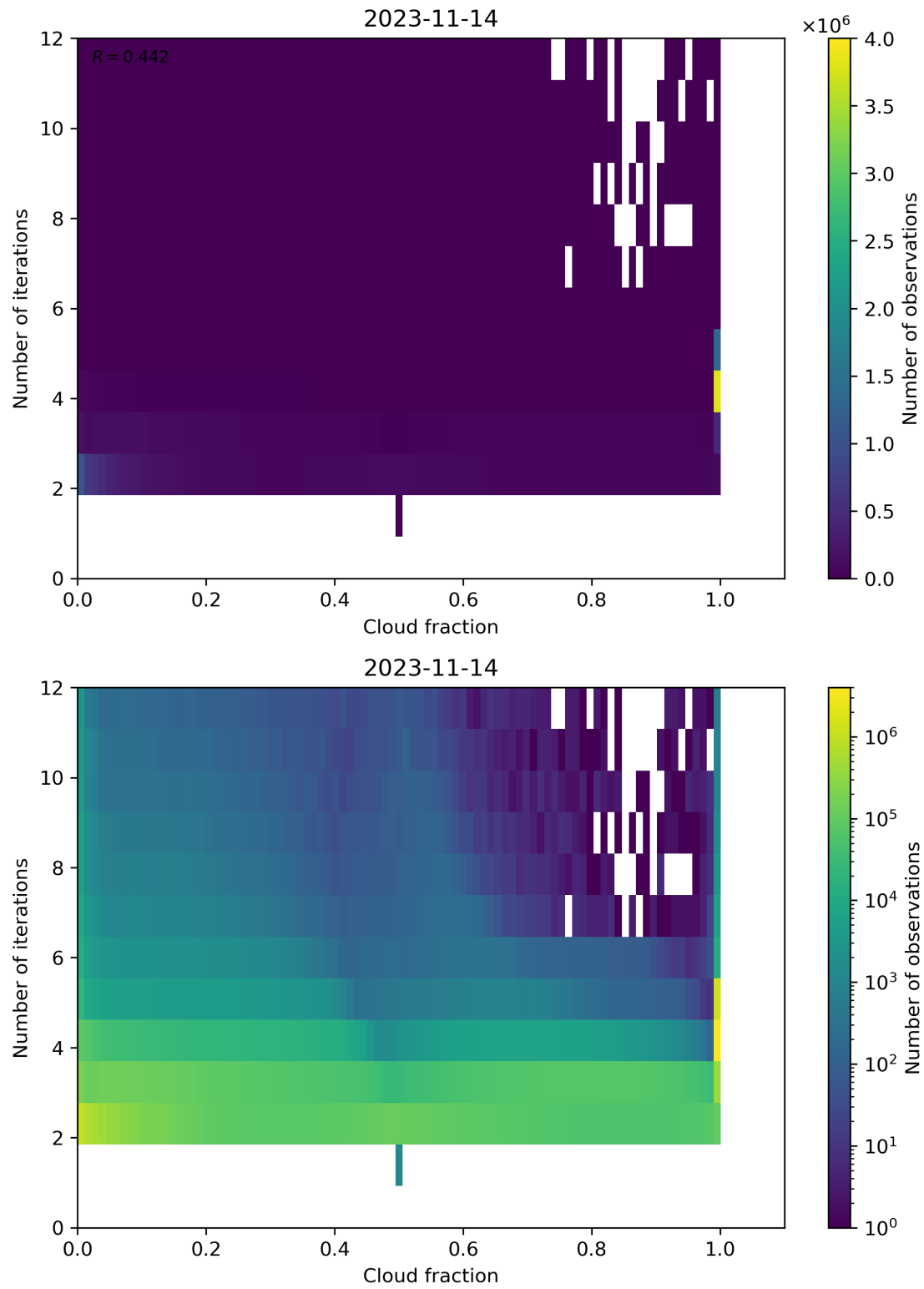
Figure 80: Scatter density plot of “Cloud fraction” against “Number of iterations” for 2023-11-13 to 2023-11-15.
