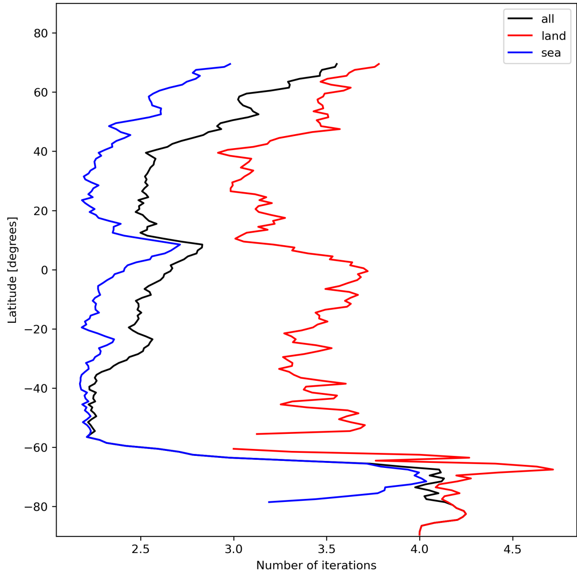
Figure 22: Zonal average of “Number of iterations” for 2023-11-13 to 2023-11-15.
