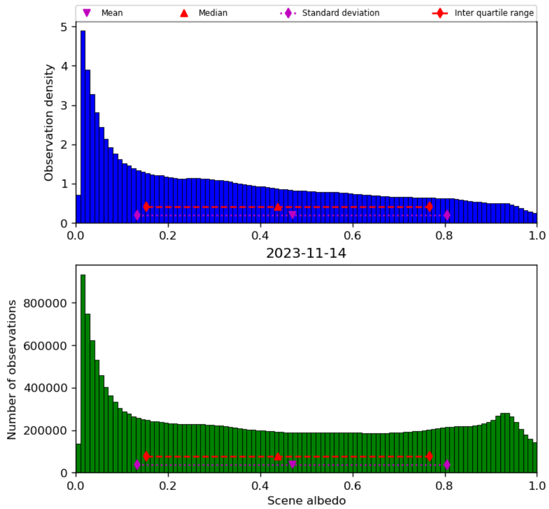
Figure 34: Histogram of “Scene albedo” for 2023-11-13 to 2023-11-15
