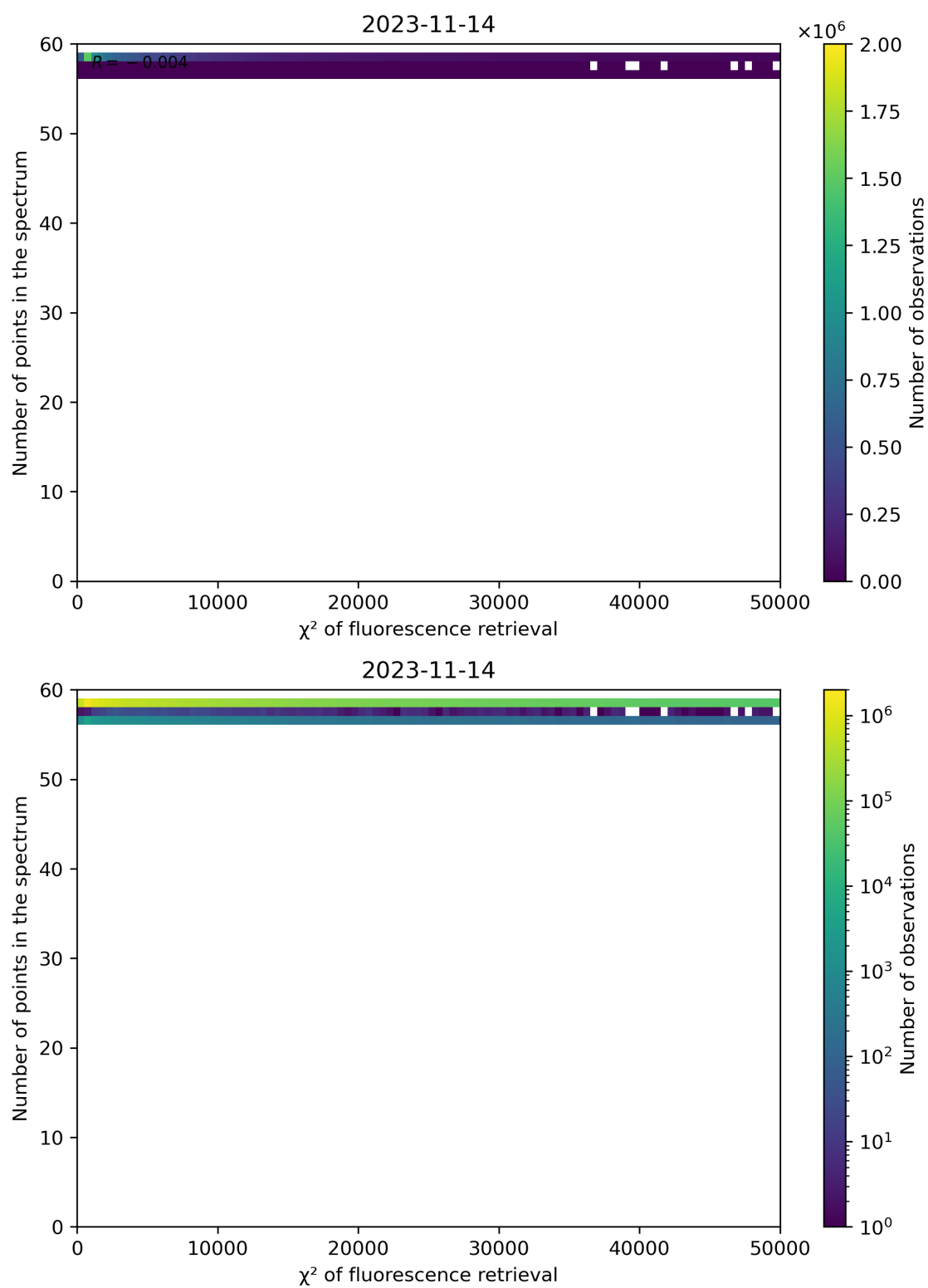
Figure 71: Scatter density plot of " \chi^2 of fluorescence retrieval" against "Number of points in the spectrum" for 2023-11-13 to 2023-11-15.
