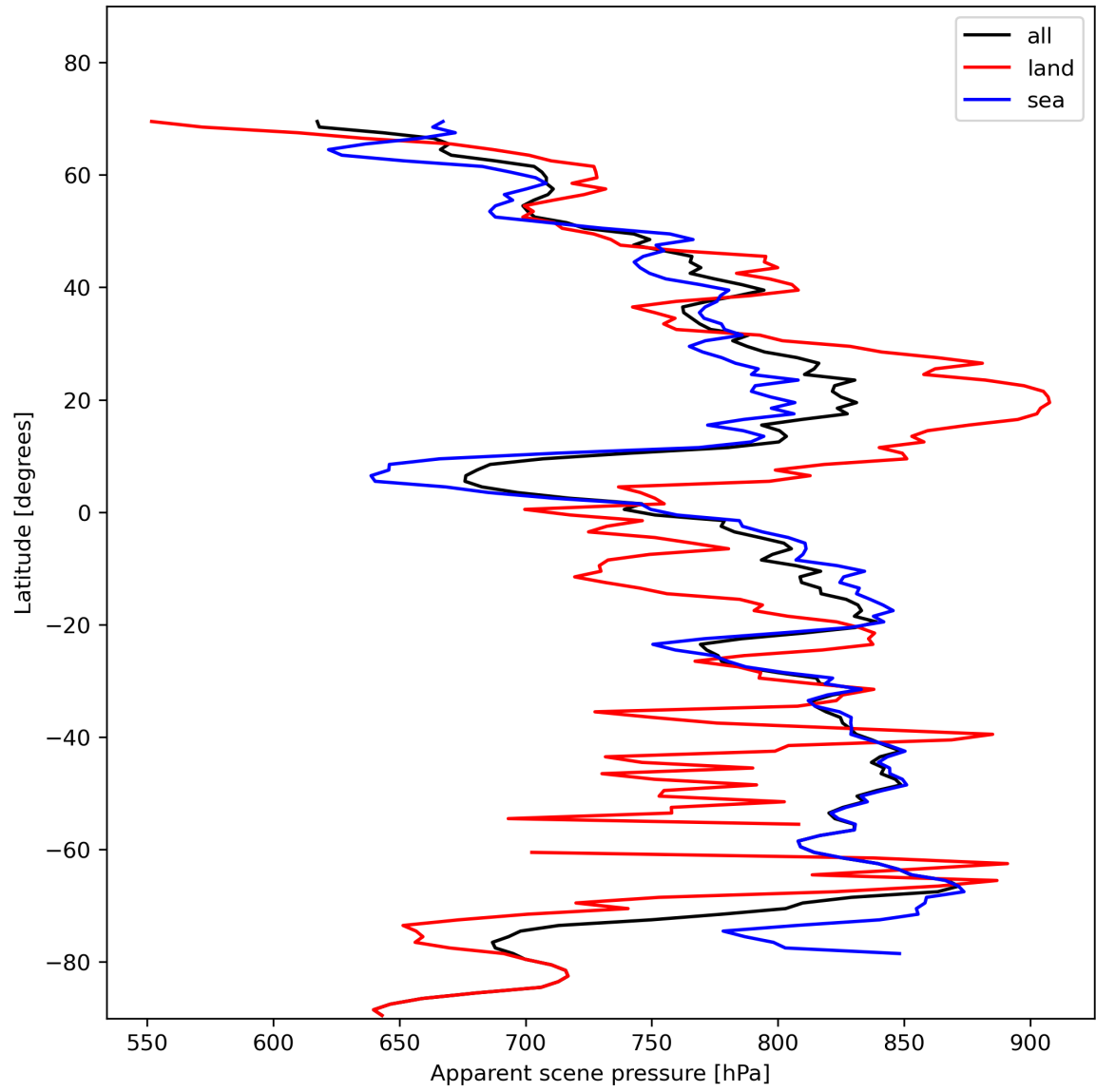
Figure 19: Zonal average of “Apparent scene pressure” for 2023-11-13 to 2023-11-15.
