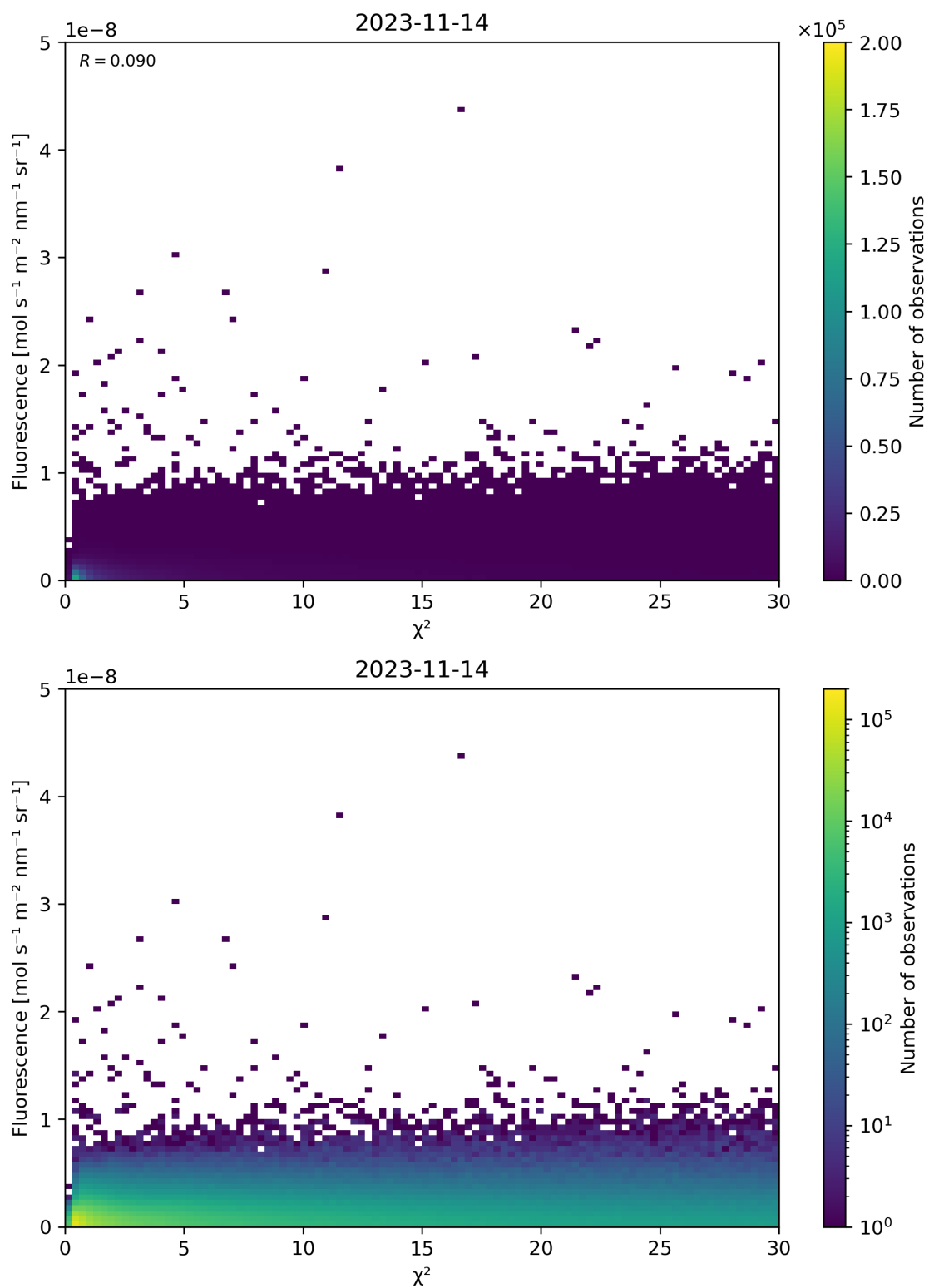
Figure 70: Scatter density plot of “ \chi^2 ” against “Fluorescence” for 2023-11-13 to 2023-11-15.
