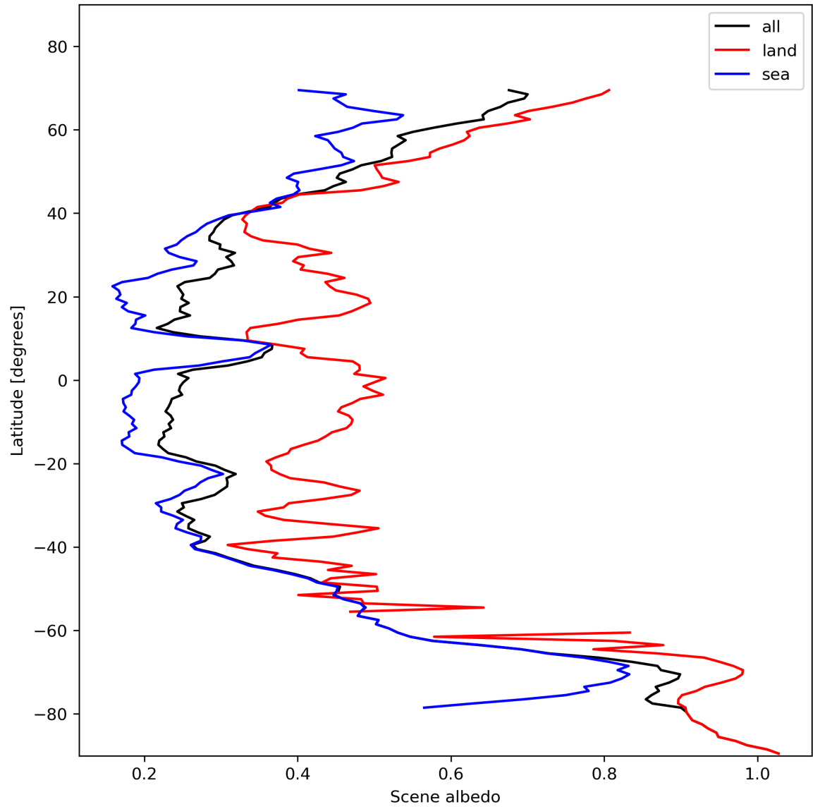
Figure 17: Zonal average of “Scene albedo” for 2023-11-13 to 2023-11-15.
