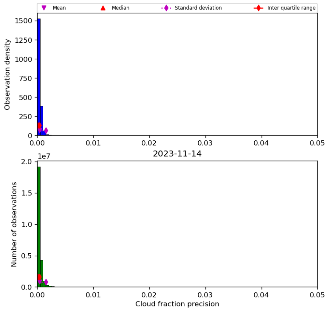
Figure 33: Histogram of “Cloud fraction precision” for 2023-11-13 to 2023-11-15
