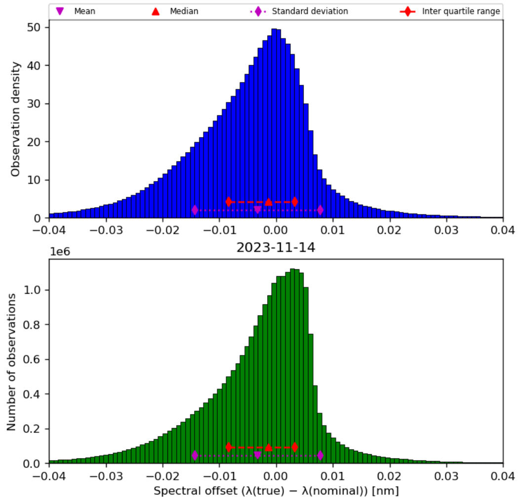
Figure 45: Histogram of “Spectral offset ( \lambda(\text{true}) - \lambda(\text{nominal}) )” for 2023-11-13 to 2023-11-15
