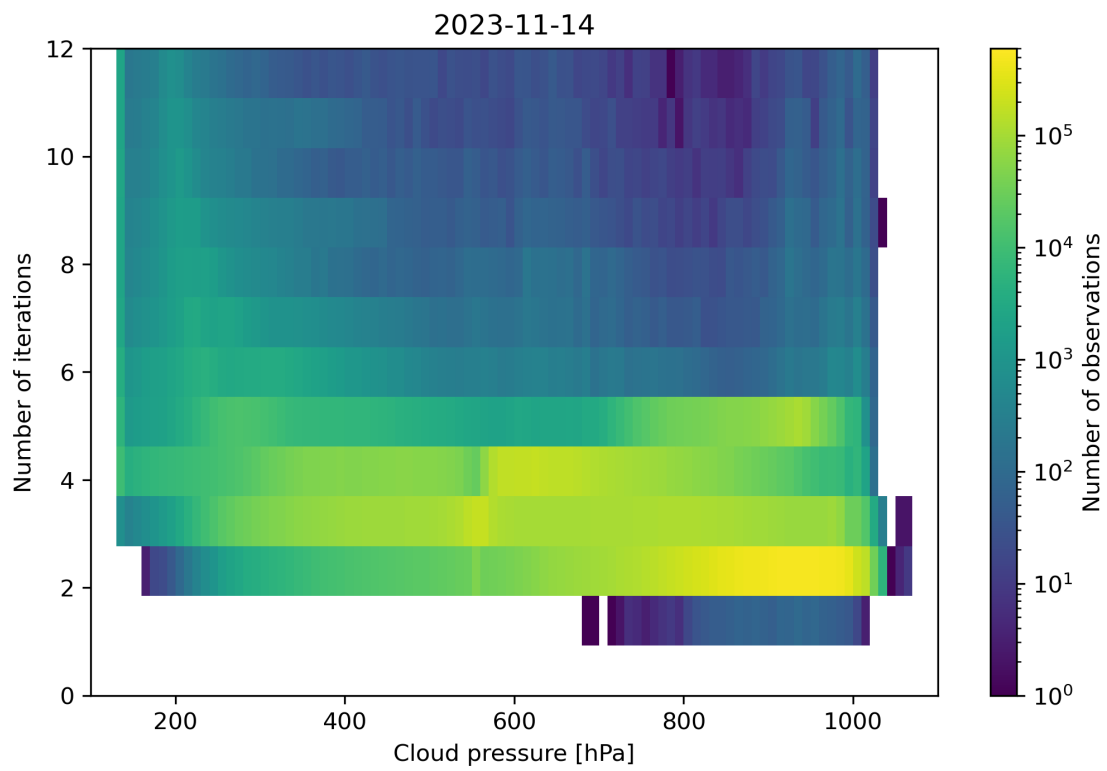
Figure 89: Scatter density plot of “Cloud pressure” against “Number of iterations” for 2023-11-13 to 2023-11-15.
