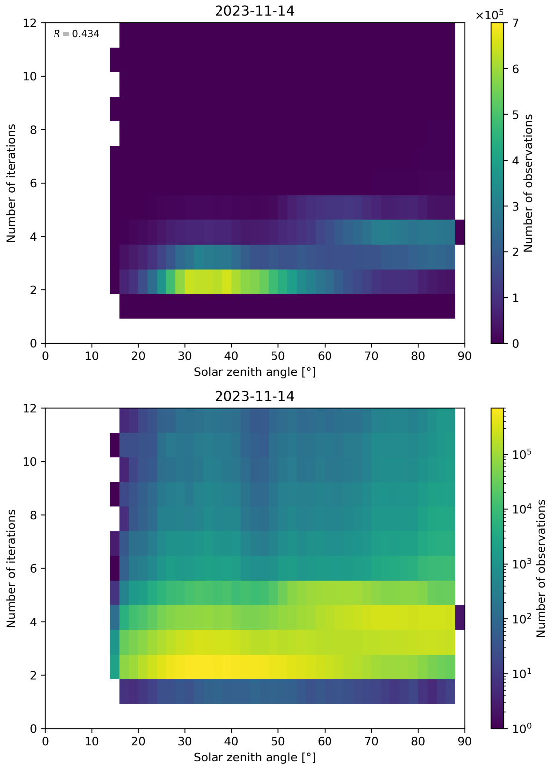
Figure 125: Scatter density plot of “Solar zenith angle” against “Number of iterations” for 2023-11-13 to 2023-11-15.
