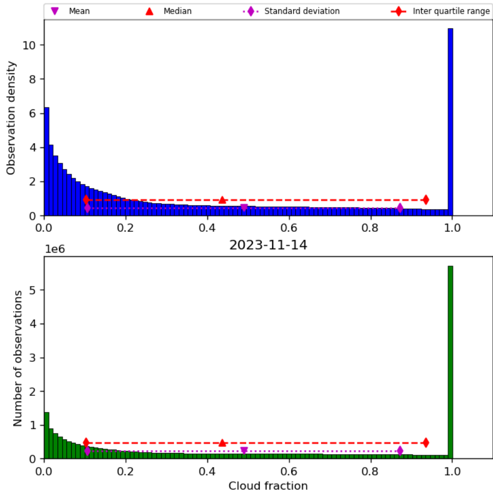
Figure 32: Histogram of “Cloud fraction” for 2023-11-13 to 2023-11-15
