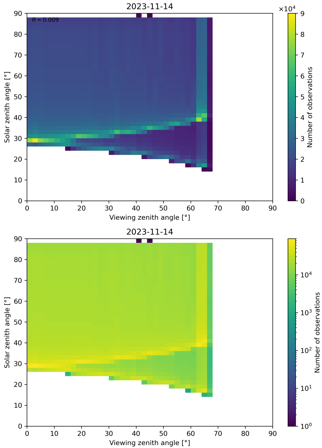
Figure 139: Scatter density plot of “Viewing zenith angle” against “Solar zenith angle” for 2023-11-13 to 2023-11-15.
