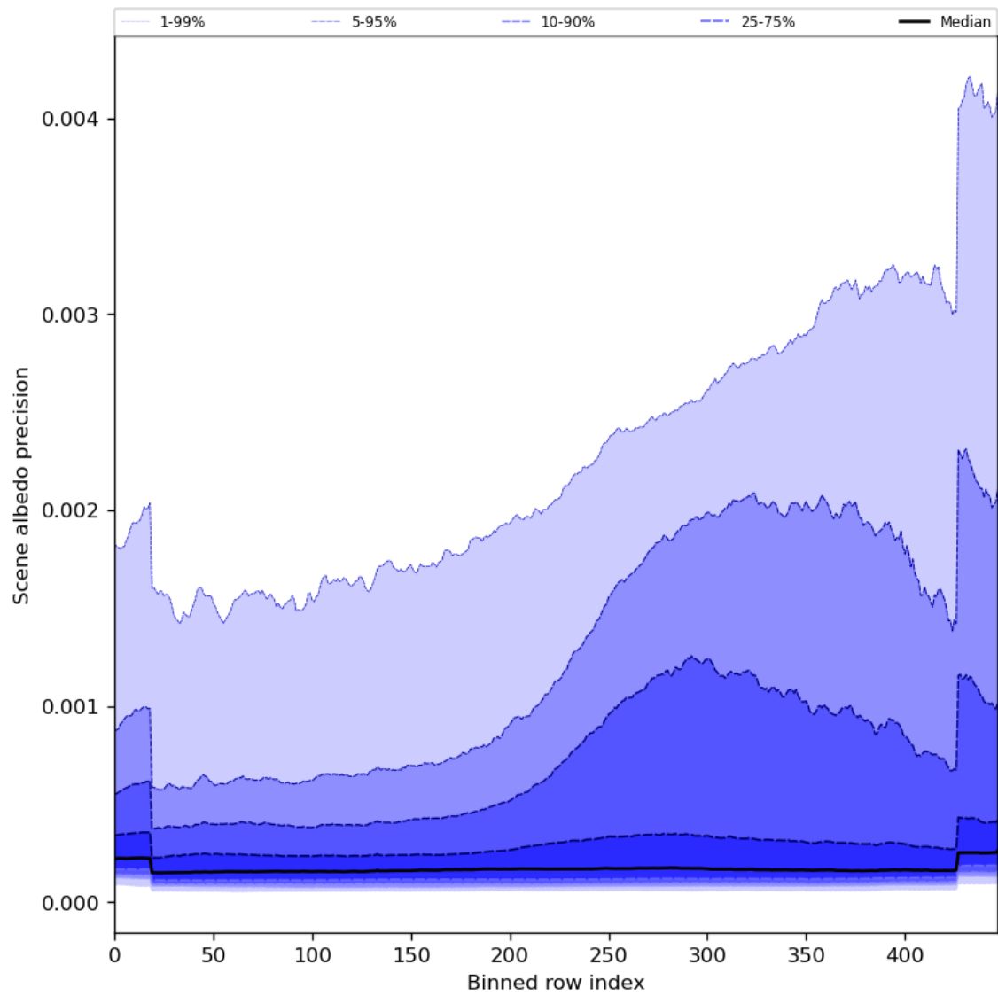
Figure 52: Along track statistics of “Scene albedo precision” for 2023-11-13 to 2023-11-15
