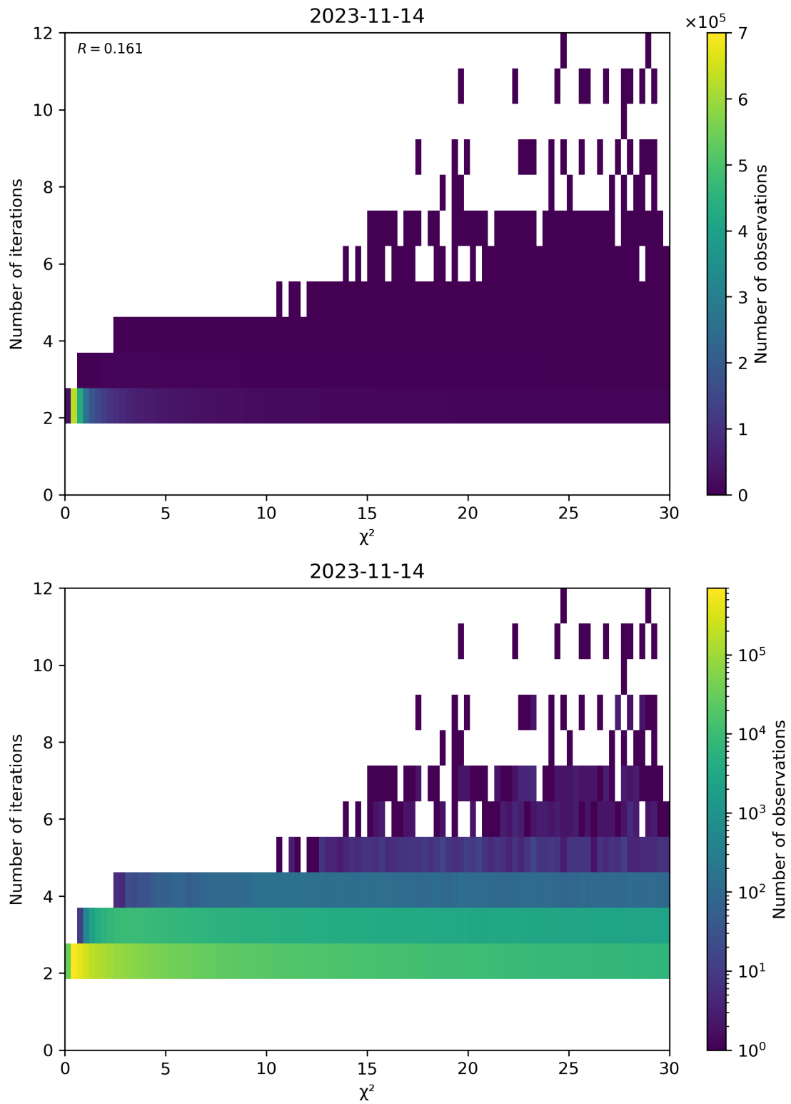
Figure 73: Scatter density plot of “ \chi^2 ” against “Number of iterations” for 2023-11-13 to 2023-11-15.
