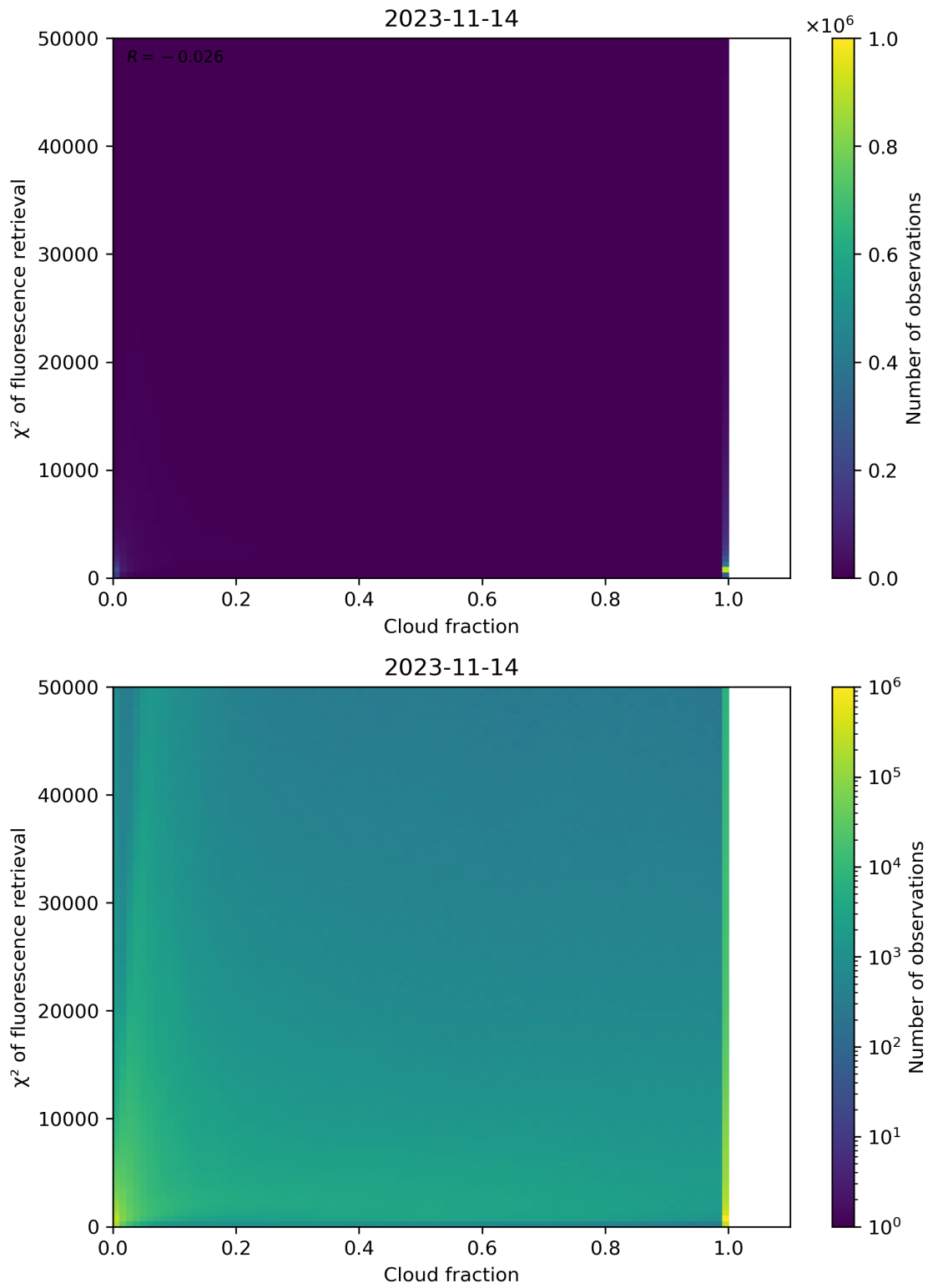
Figure 78: Scatter density plot of “Cloud fraction” against “ \chi^2 of fluorescence retrieval” for 2023-11-13 to 2023-11-15.
