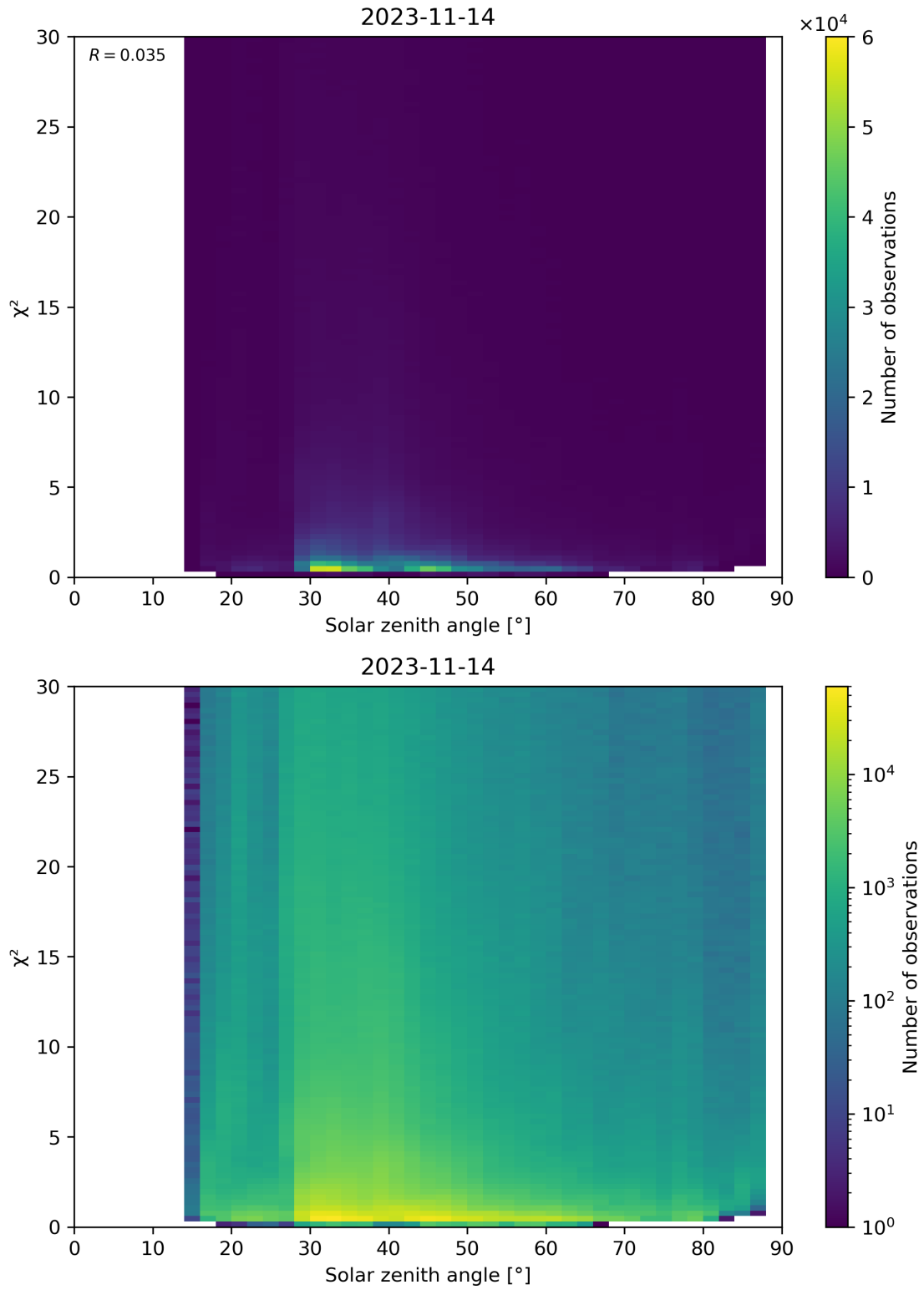
Figure 119: Scatter density plot of “Solar zenith angle” against “ \chi^2 ” for 2023-11-13 to 2023-11-15.
