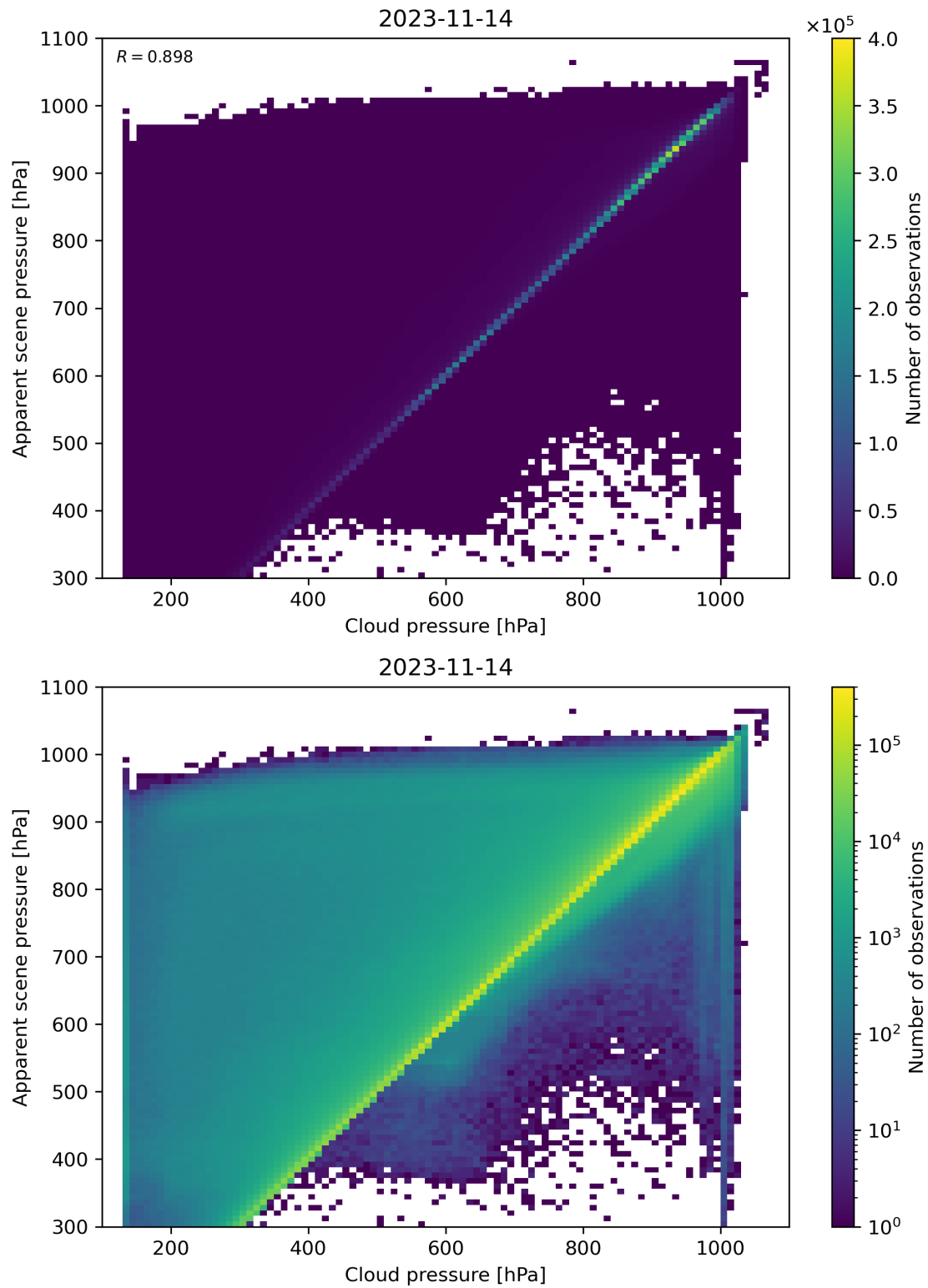
Figure 84: Scatter density plot of “Cloud pressure” against “Apparent scene pressure” for 2023-11-13 to 2023-11-15.
