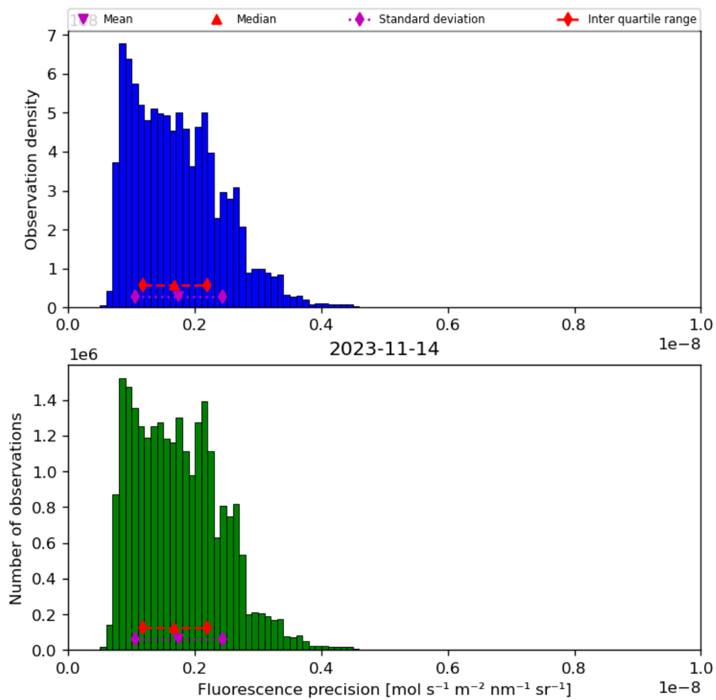
Figure 41: Histogram of “Fluorescence precision” for 2023-11-13 to 2023-11-15
