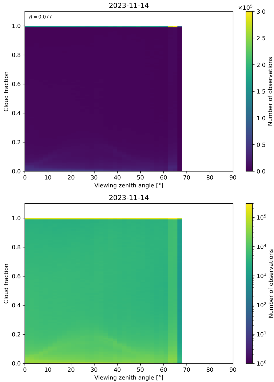
Figure 132: Scatter density plot of “Viewing zenith angle” against “Cloud fraction” for 2023-11-13 to 2023-11-15.
