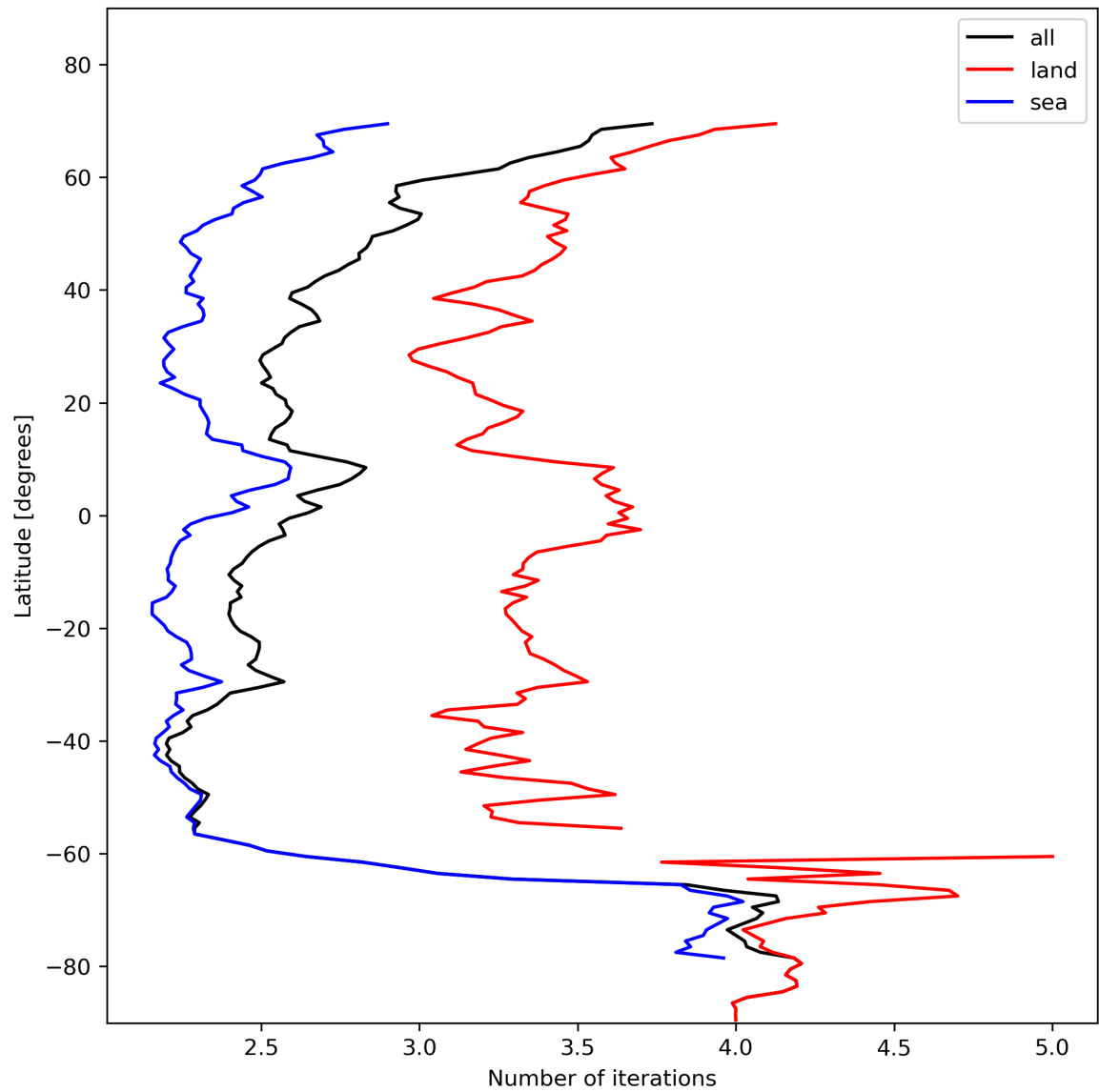
Figure 22: Zonal average of “Number of iterations” for 2023-11-14 to 2023-11-16.
