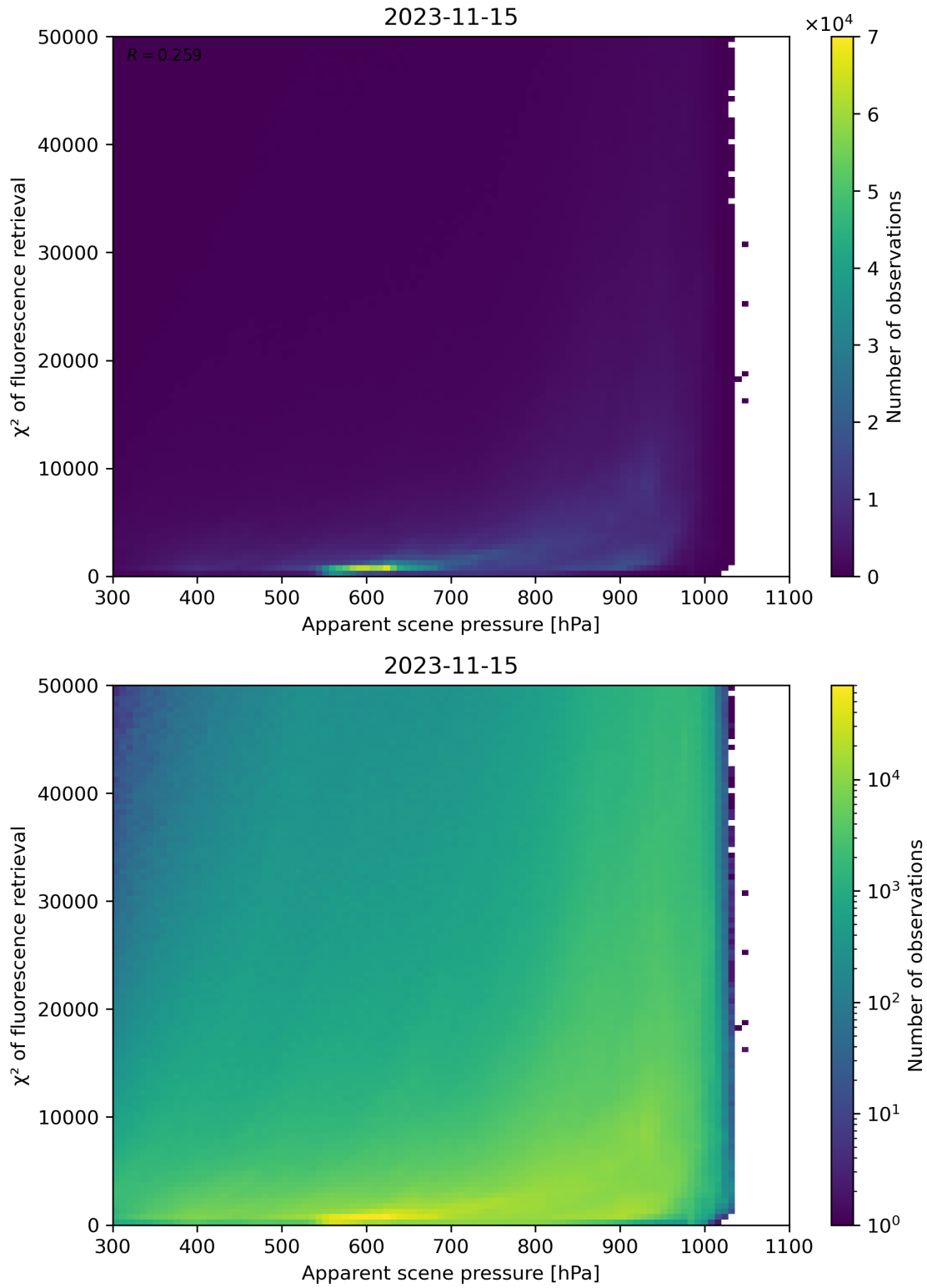
Figure 64: Scatter density plot of “Apparent scene pressure” against “ \chi^2 of fluorescence retrieval” for 2023-11-14 to 2023-11-16.
