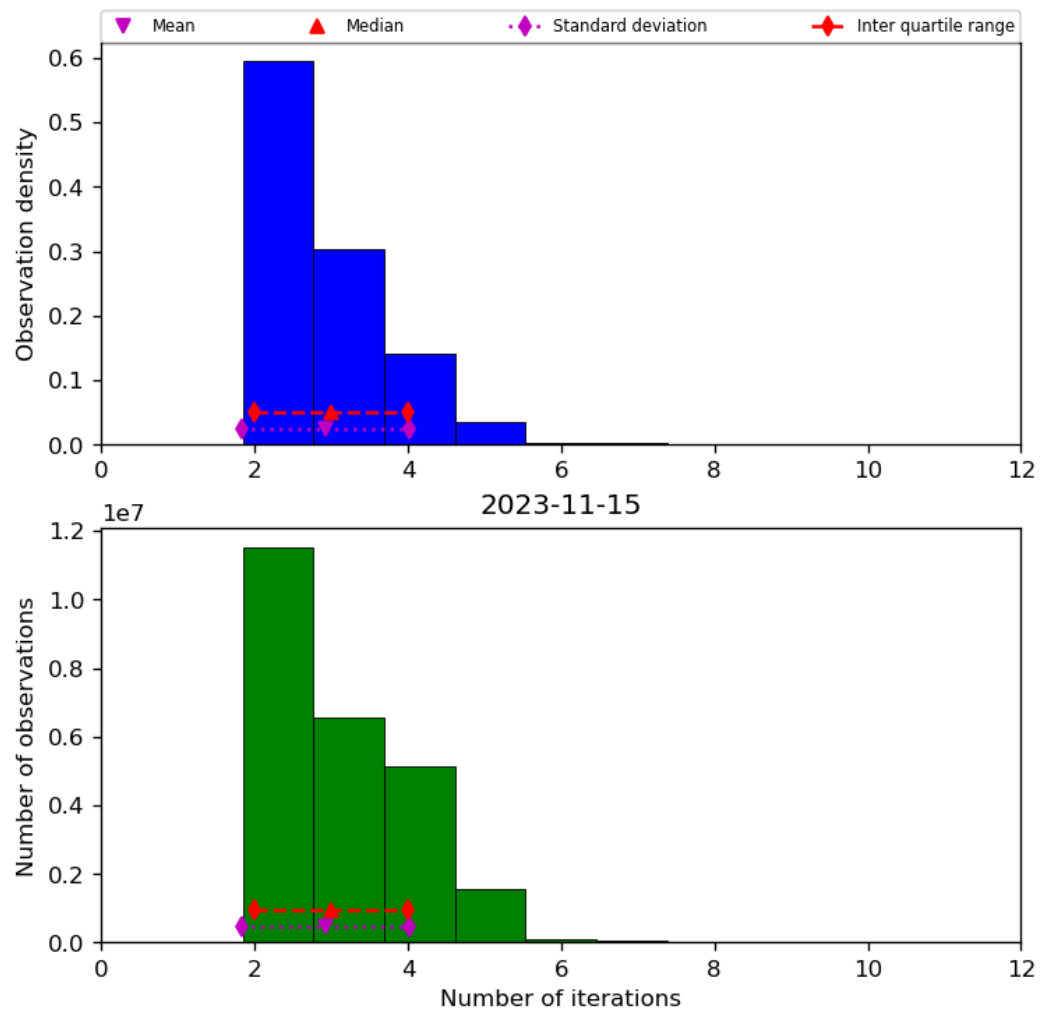
Figure 39: Histogram of “Number of iterations” for 2023-11-14 to 2023-11-16
