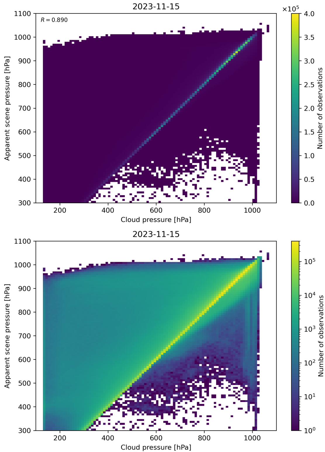
Figure 84: Scatter density plot of “Cloud pressure” against “Apparent scene pressure” for 2023-11-14 to 2023-11-16.
