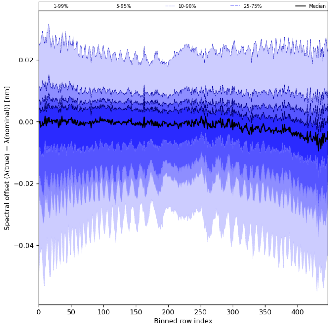
Figure 62: Along track statistics of “Spectral offset ( \lambda(\text{true}) - \lambda(\text{nominal}) )” for 2023-11-14 to 2023-11-16
