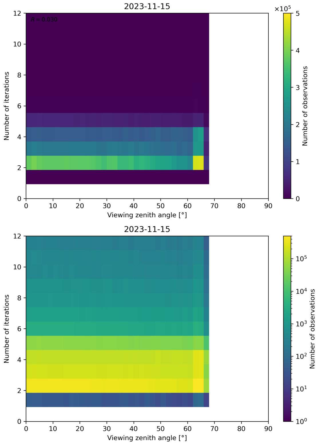
Figure 136: Scatter density plot of “Viewing zenith angle” against “Number of iterations” for 2023-11-14 to 2023-11-16.
