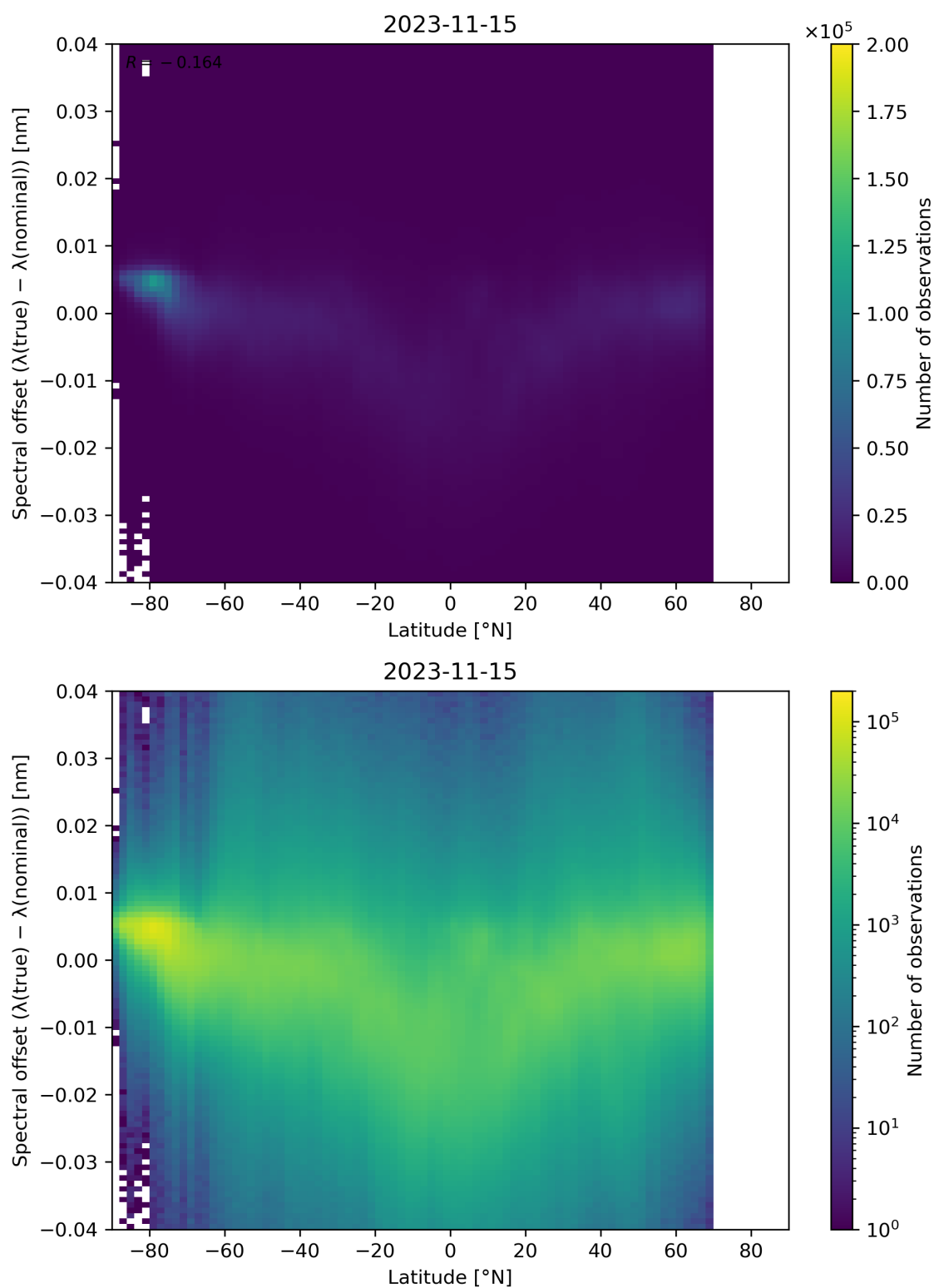
Figure 105: Scatter density plot of “Latitude” against “Spectral offset ( \lambda(\text{true}) - \lambda(\text{nominal}) )” for 2023-11-14 to 2023-11-16.
