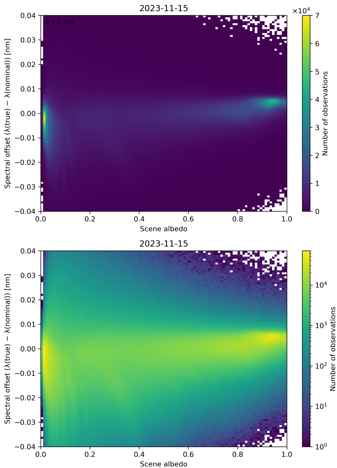
Figure 117: Scatter density plot of “Scene albedo” against “Spectral offset ( \lambda(\text{true}) - \lambda(\text{nominal}) )” for 2023-11-14 to 2023-11-16.
