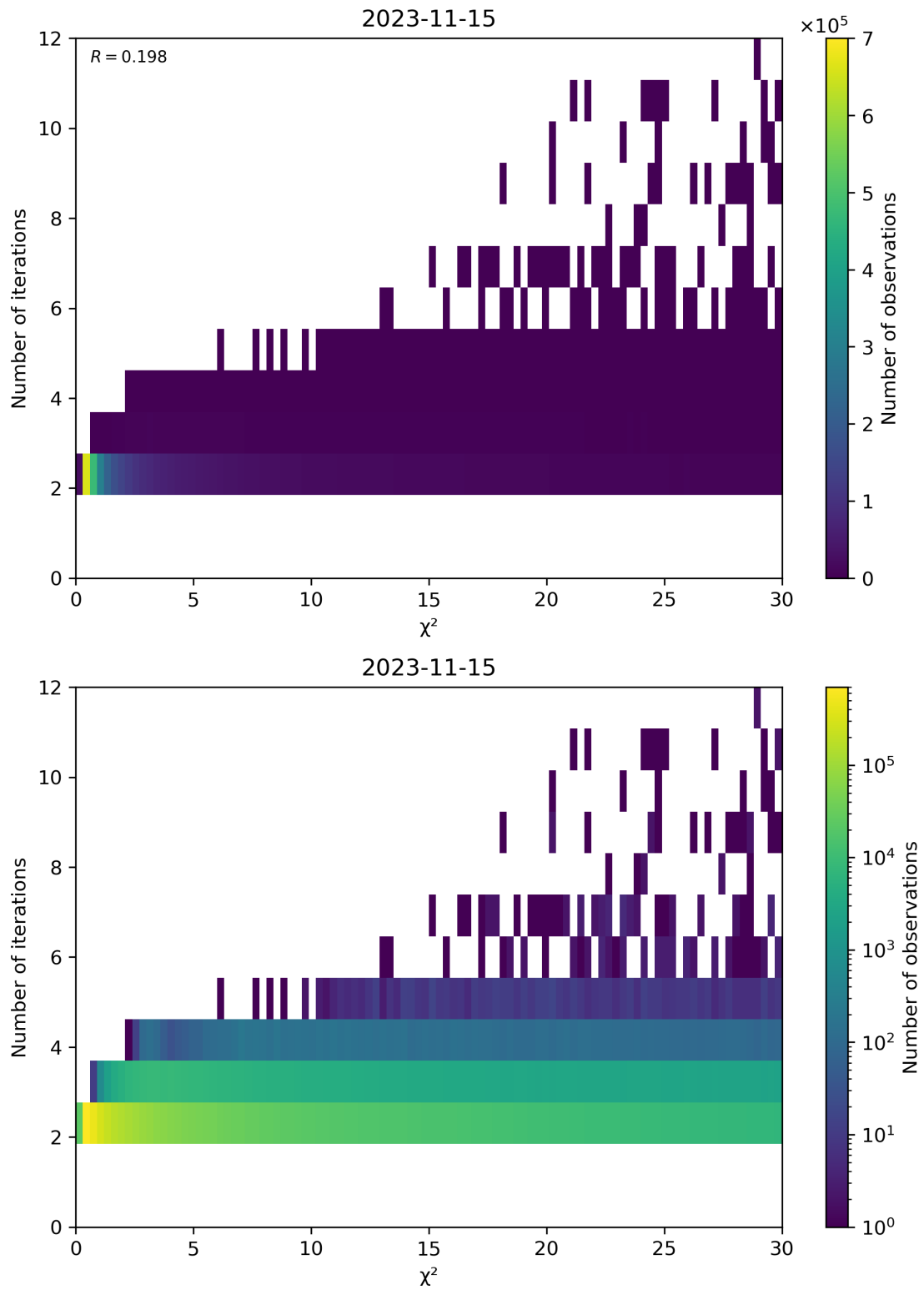
Figure 73: Scatter density plot of “ \chi^2 ” against “Number of iterations” for 2023-11-14 to 2023-11-16.
