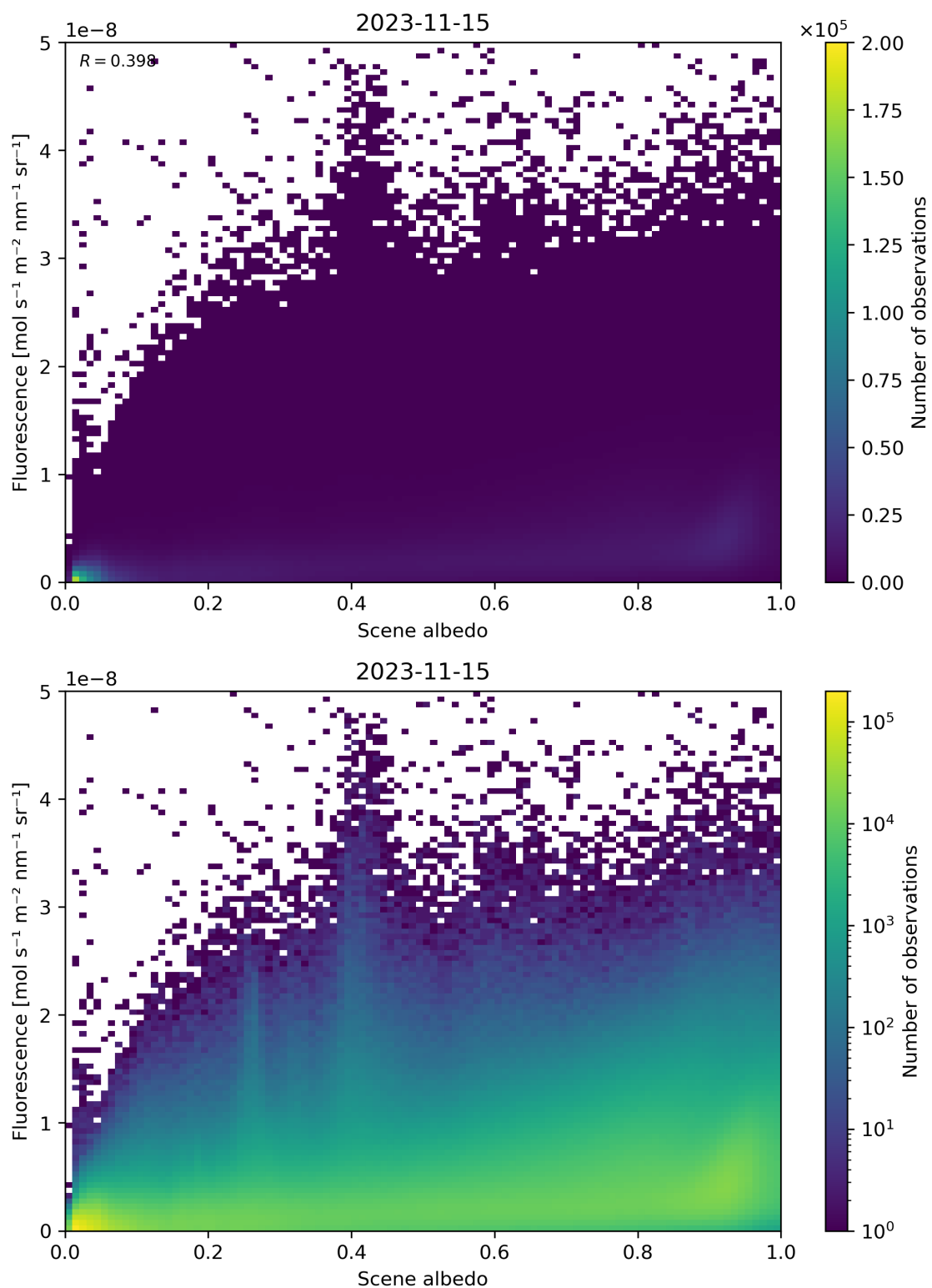
Figure 114: Scatter density plot of “Scene albedo” against “Fluorescence” for 2023-11-14 to 2023-11-16.
