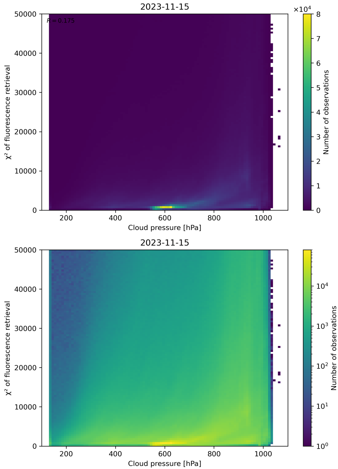
Figure 86: Scatter density plot of “Cloud pressure” against “ \chi^2 of fluorescence retrieval” for 2023-11-14 to 2023-11-16.
