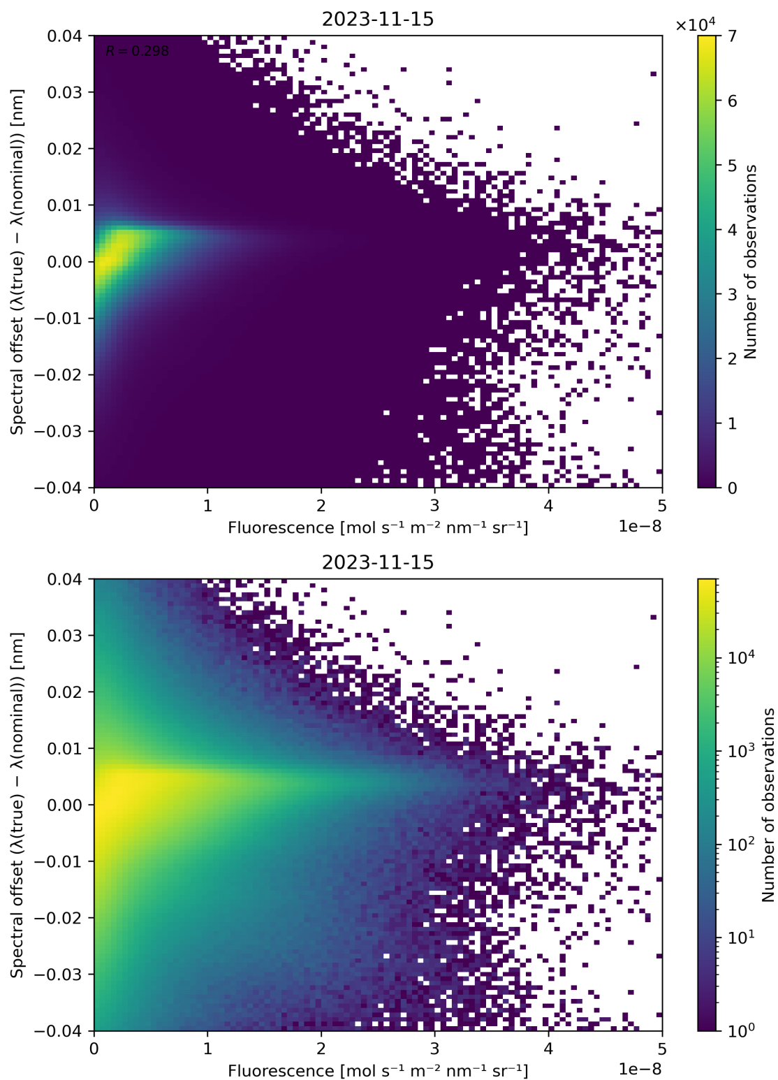
Figure 95: Scatter density plot of “Fluorescence” against “Spectral offset ( \lambda(\text{true}) - \lambda(\text{nominal}) )” for 2023-11-14 to 2023-11-16.
