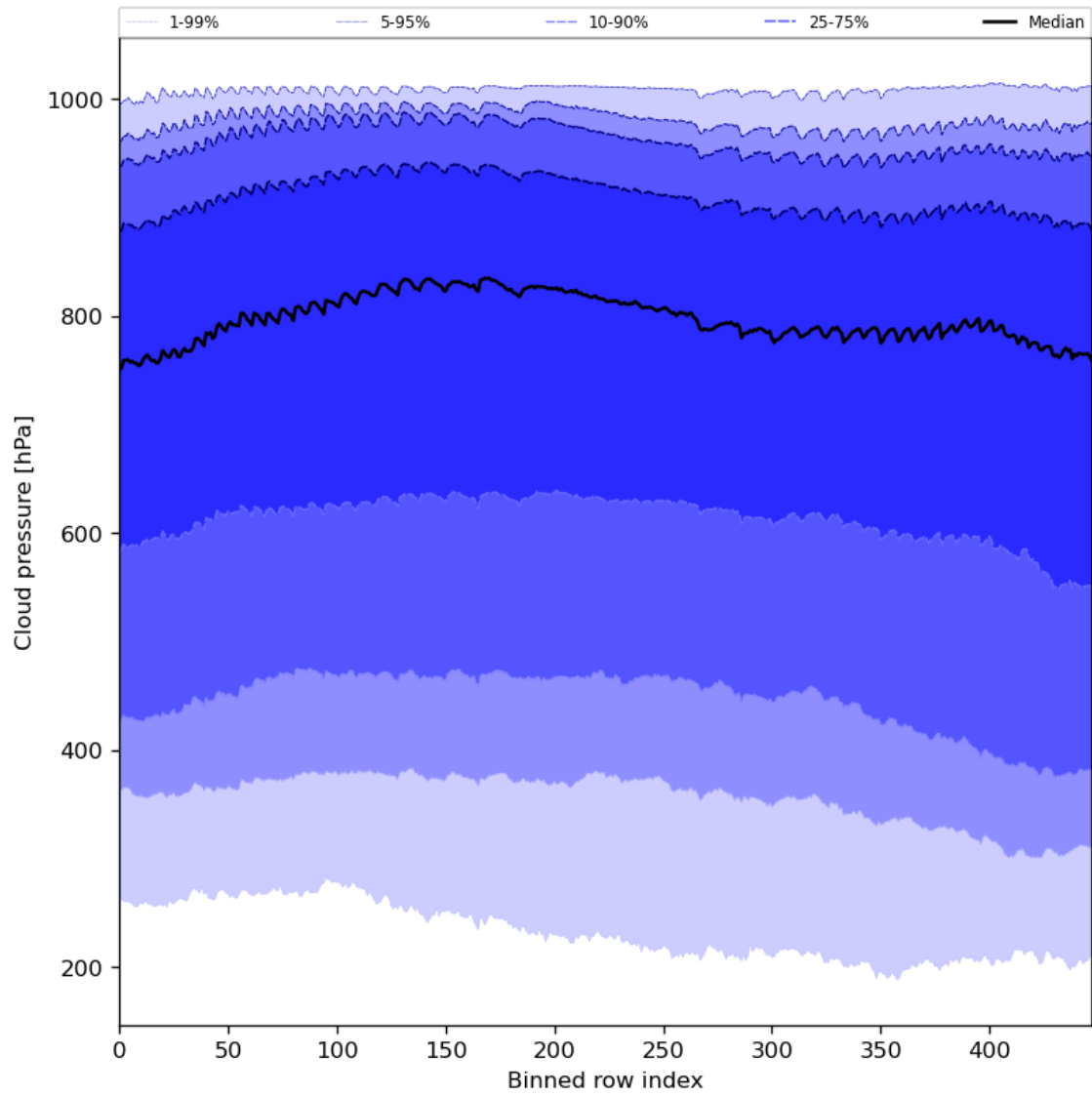
Figure 47: Along track statistics of “Cloud pressure” for 2023-11-14 to 2023-11-16
