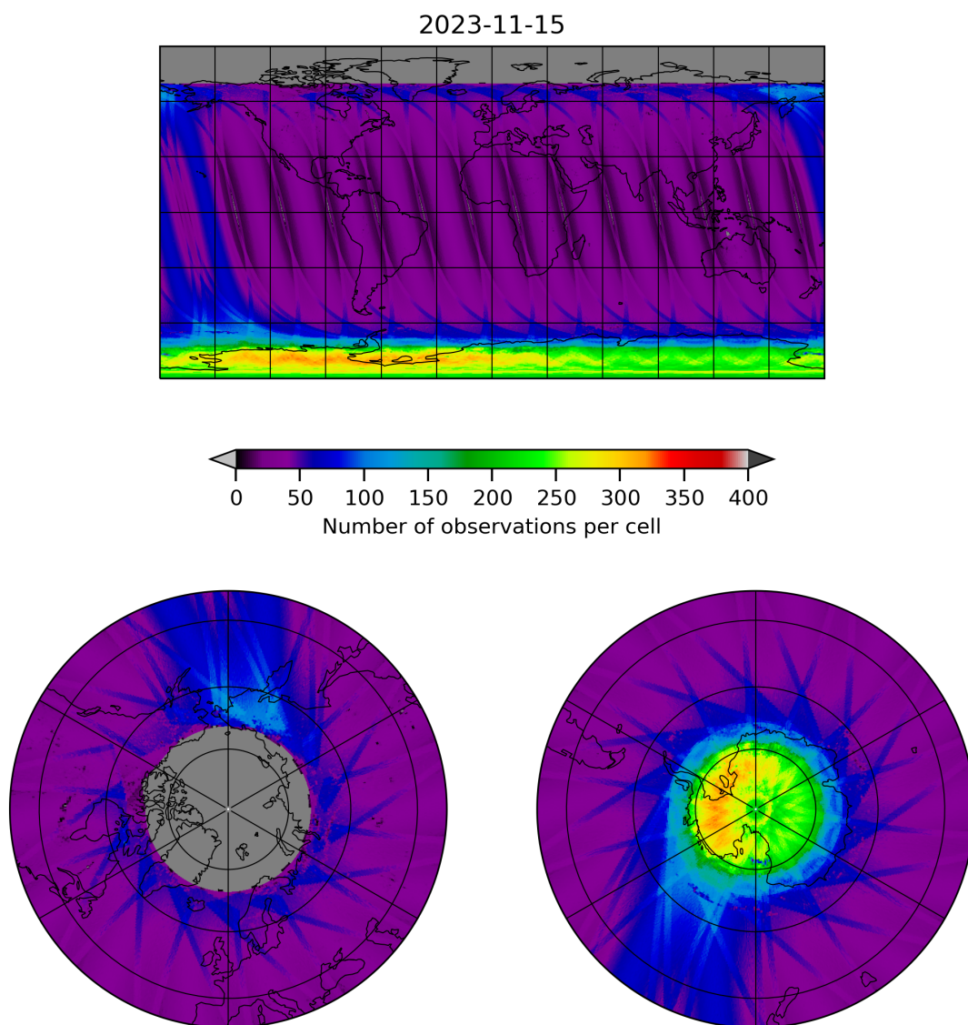
Figure 11: Map of the number of observations for 2023-11-14 to 2023-11-16
