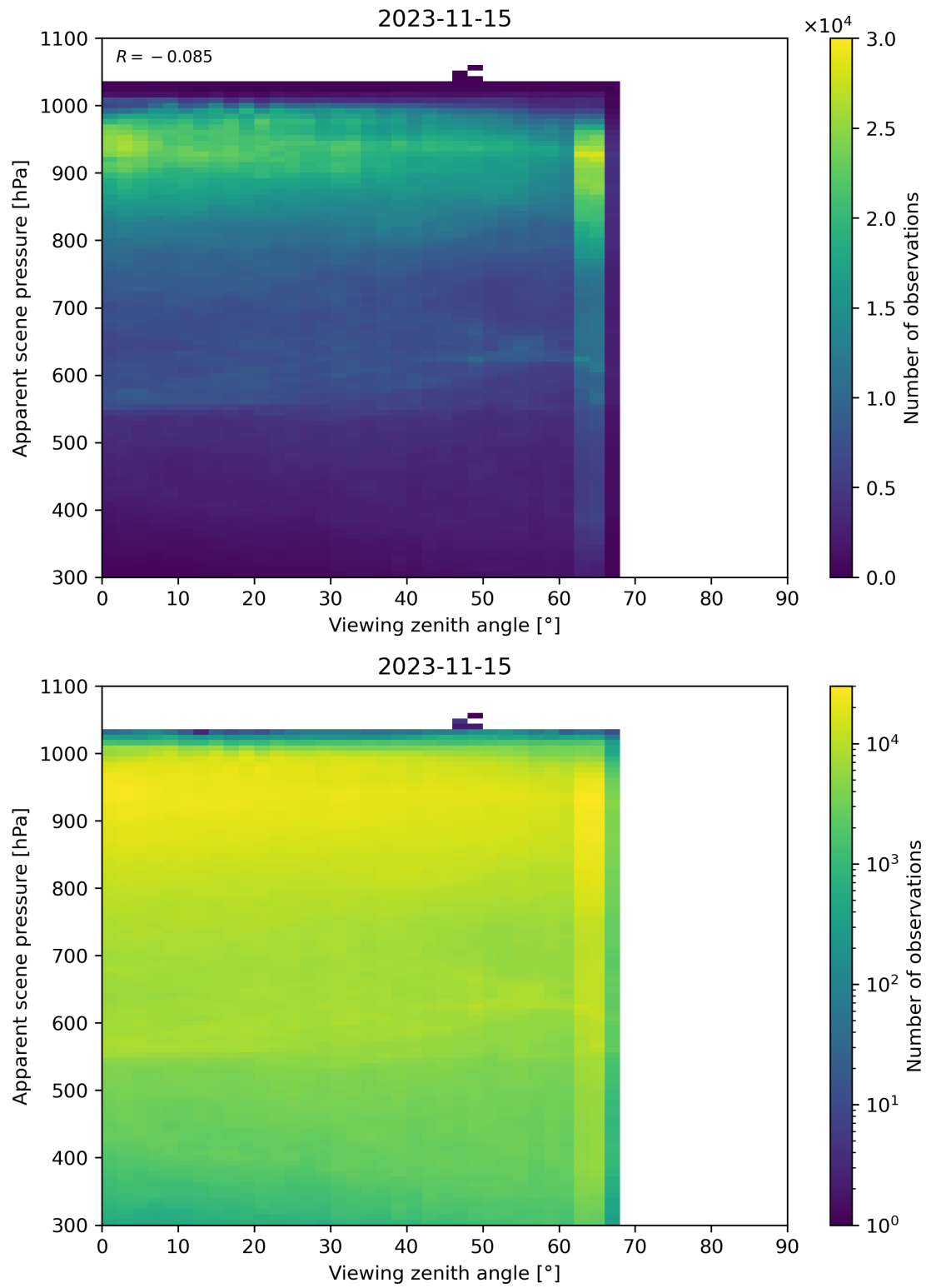
Figure 129: Scatter density plot of “Viewing zenith angle” against “Apparent scene pressure” for 2023-11-14 to 2023-11-16.
