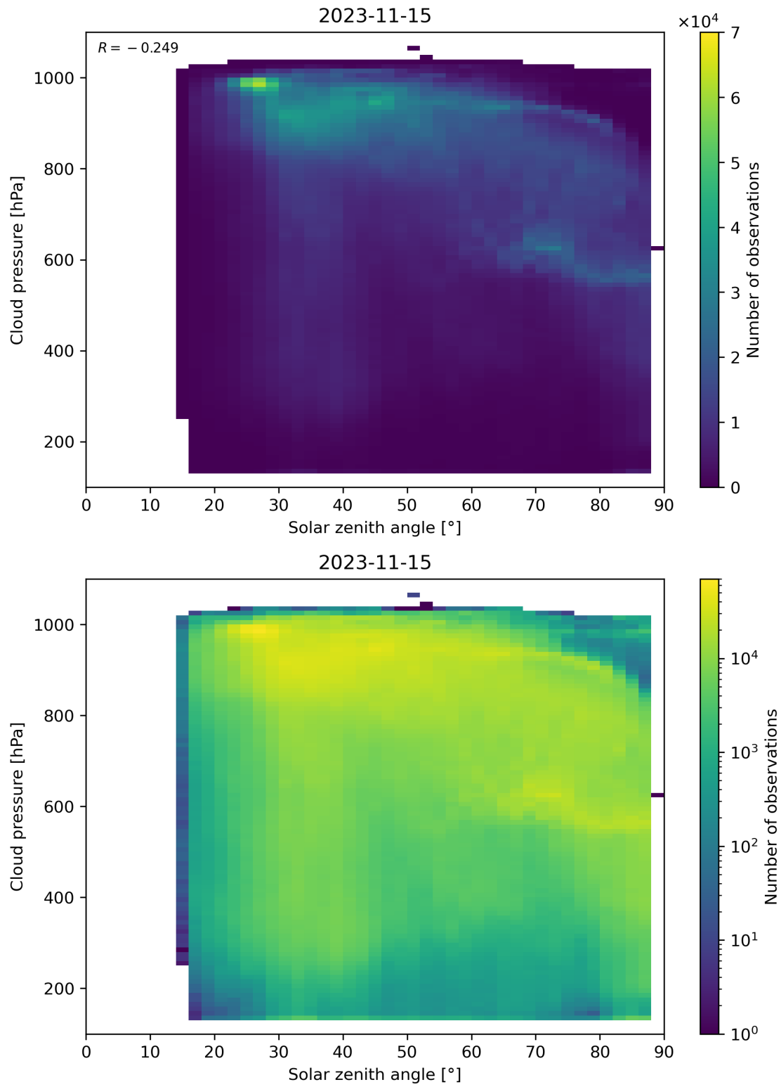
Figure 122: Scatter density plot of “Solar zenith angle” against “Cloud pressure” for 2023-11-14 to 2023-11-16.
