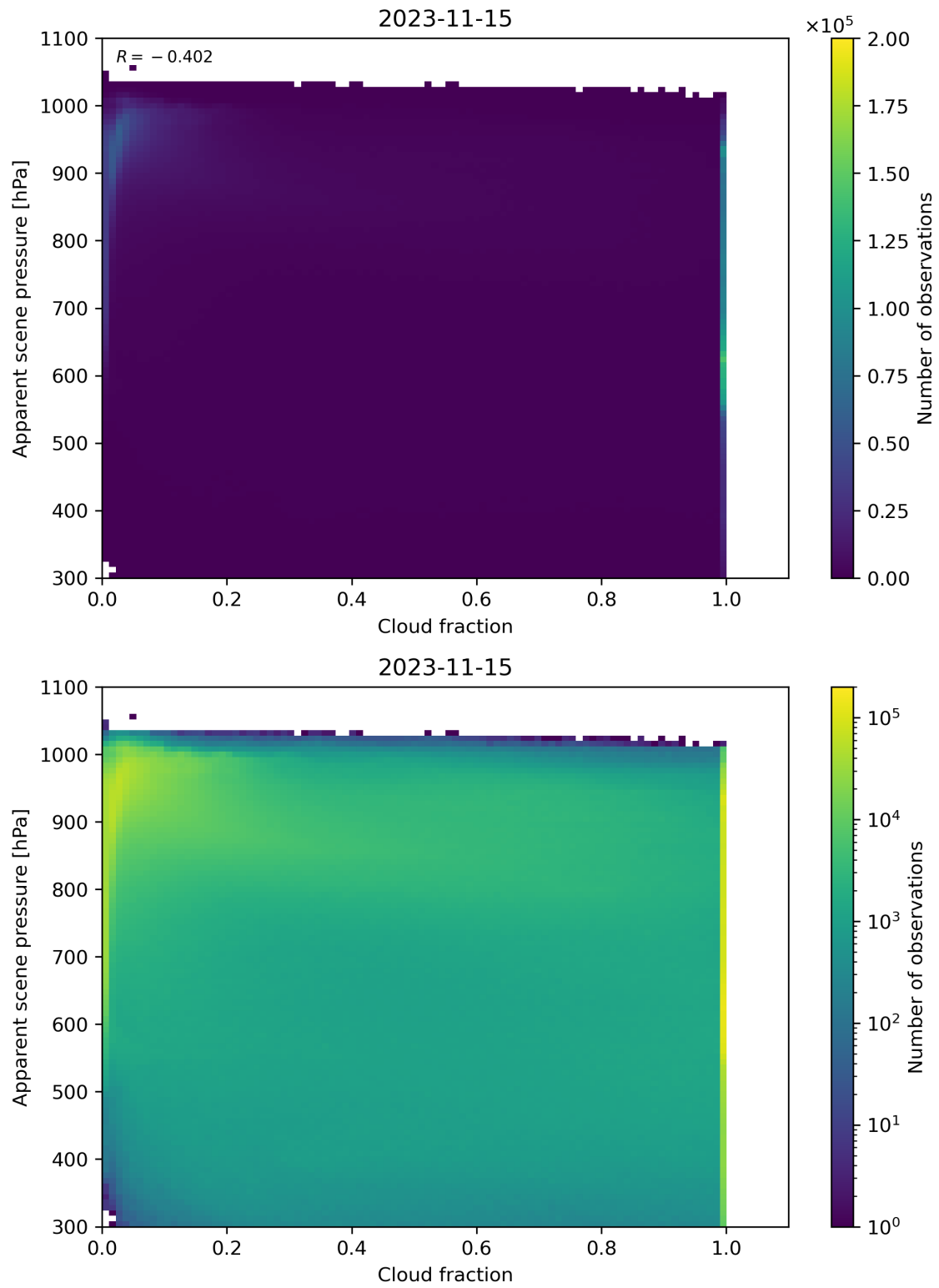
Figure 76: Scatter density plot of “Cloud fraction” against “Apparent scene pressure” for 2023-11-14 to 2023-11-16.
