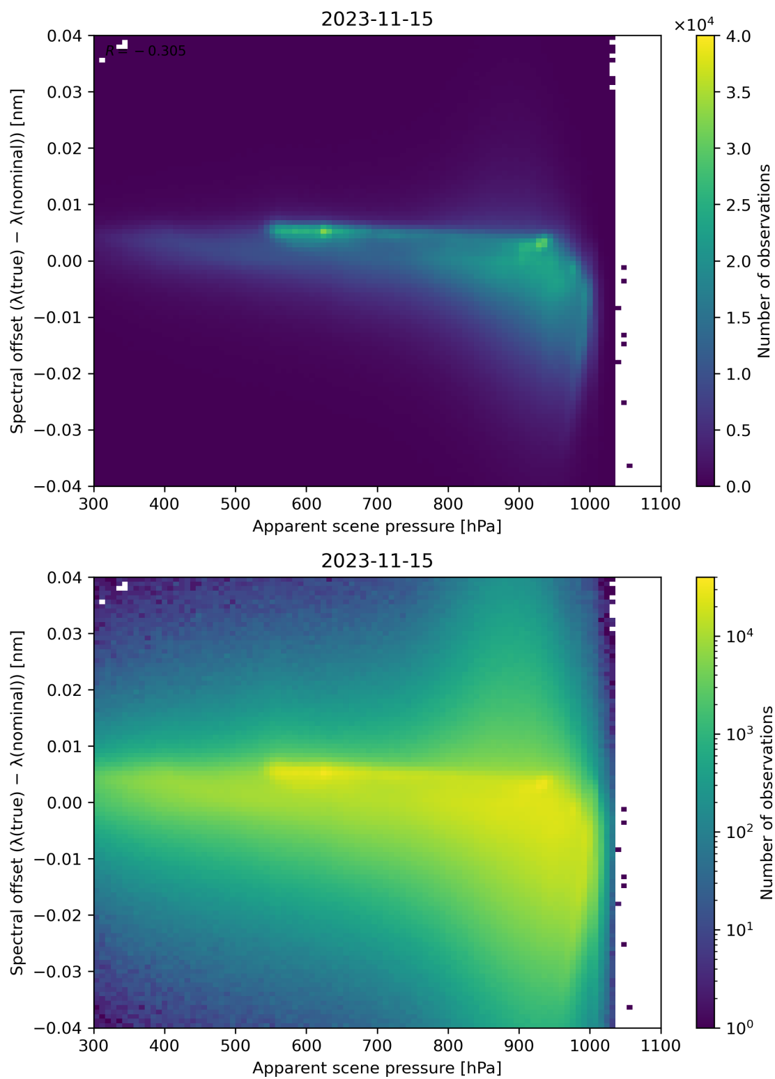
Figure 68: Scatter density plot of “Apparent scene pressure” against “Spectral offset ( \lambda(\text{true}) - \lambda(\text{nominal}) )” for 2023-11-14 to 2023-11-16.
