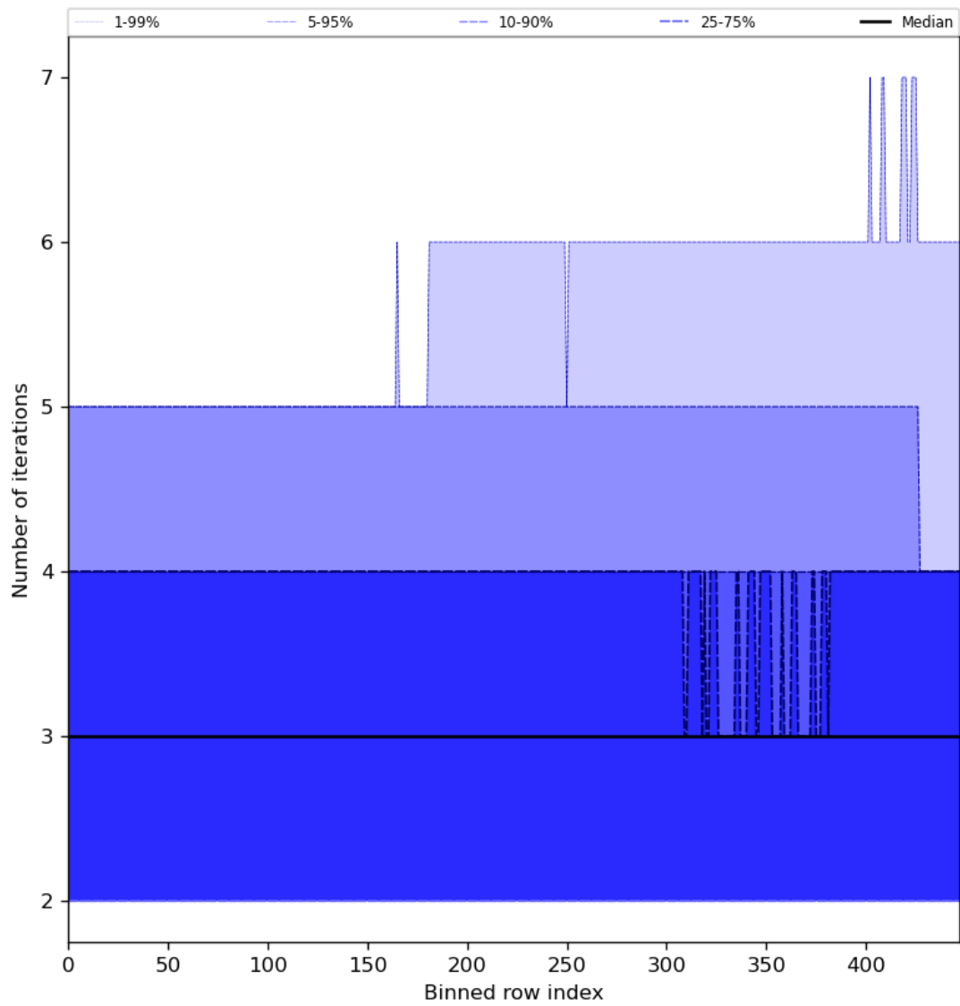
Figure 56: Along track statistics of “Number of iterations” for 2023-11-14 to 2023-11-16
