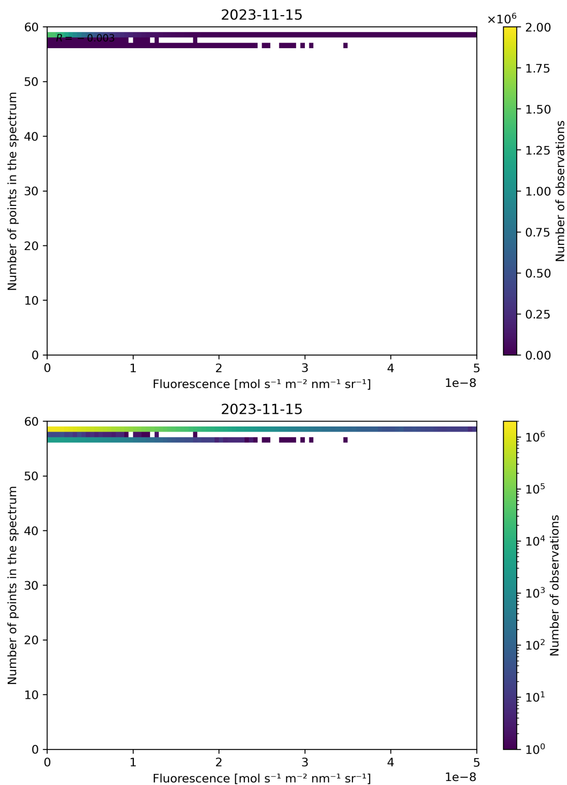
Figure 94: Scatter density plot of “Fluorescence” against “Number of points in the spectrum” for 2023-11-14 to 2023-11-16.
