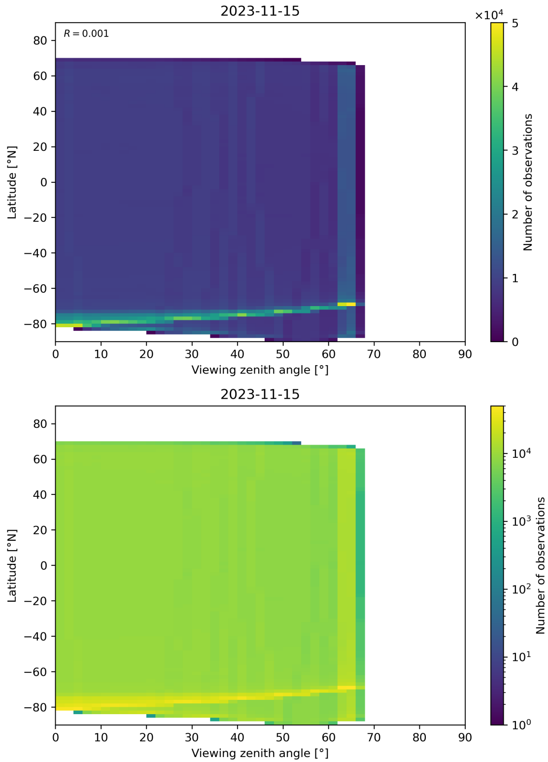
Figure 135: Scatter density plot of “Viewing zenith angle” against “Latitude” for 2023-11-14 to 2023-11-16.
