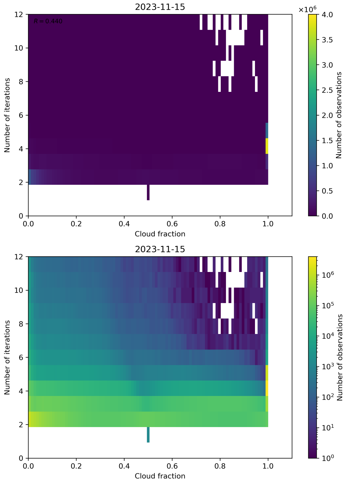
Figure 80: Scatter density plot of “Cloud fraction” against “Number of iterations” for 2023-11-14 to 2023-11-16.
