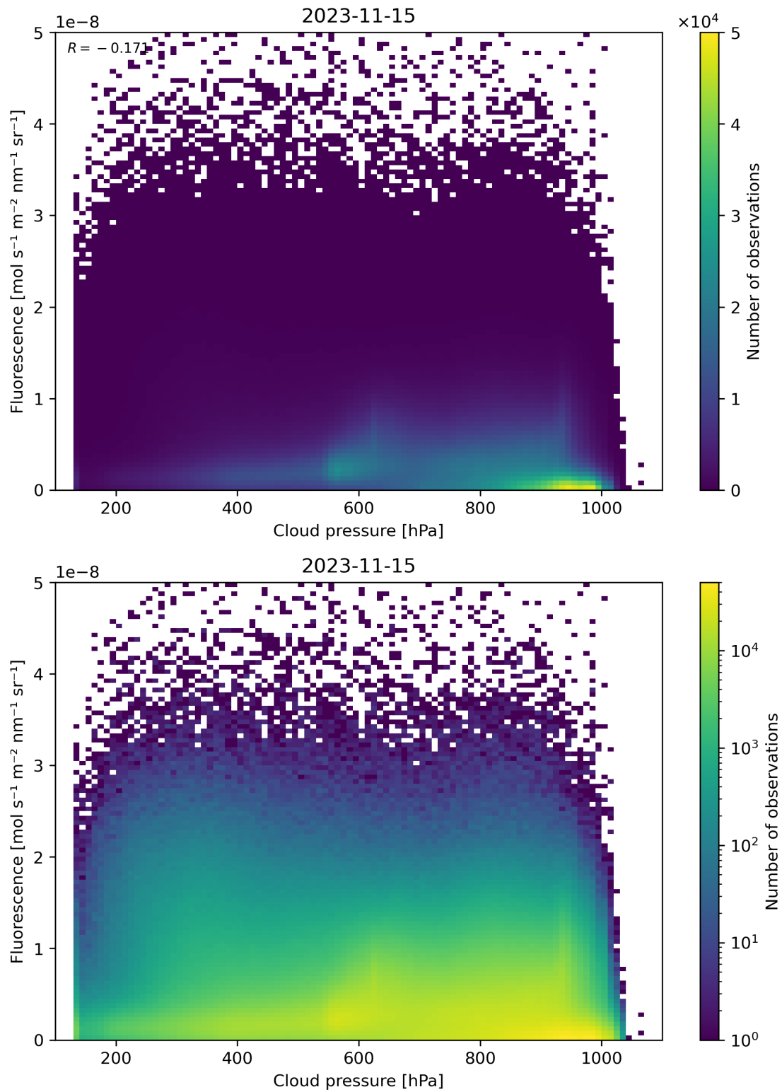
Figure 88: Scatter density plot of “Cloud pressure” against “Fluorescence” for 2023-11-14 to 2023-11-16.
