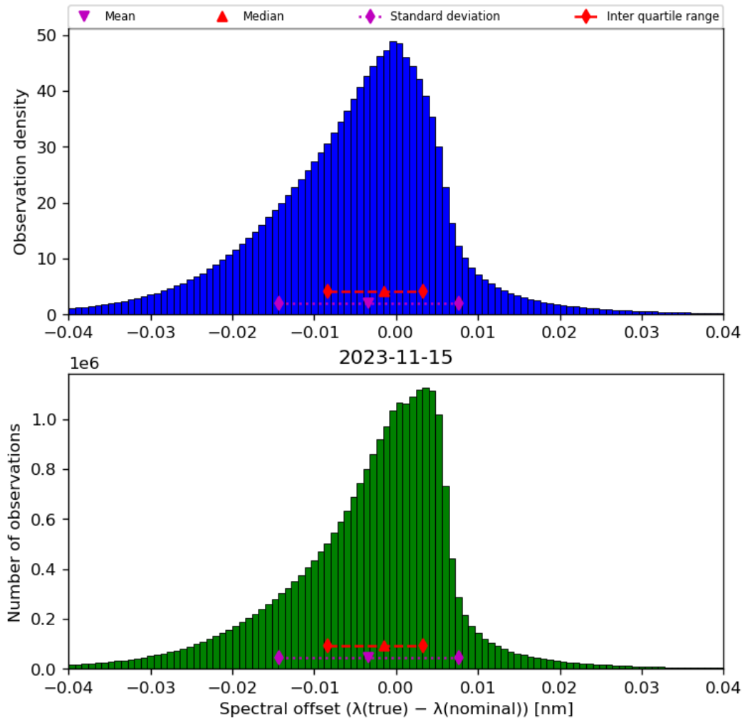
Figure 45: Histogram of “Spectral offset ( \lambda(\text{true}) - \lambda(\text{nominal}) )” for 2023-11-14 to 2023-11-16
