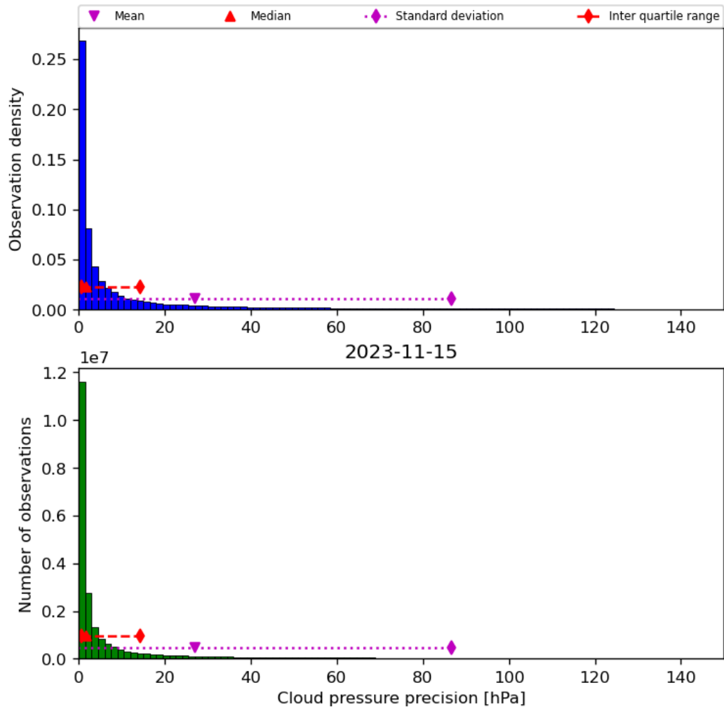
Figure 31: Histogram of “Cloud pressure precision” for 2023-11-14 to 2023-11-16
