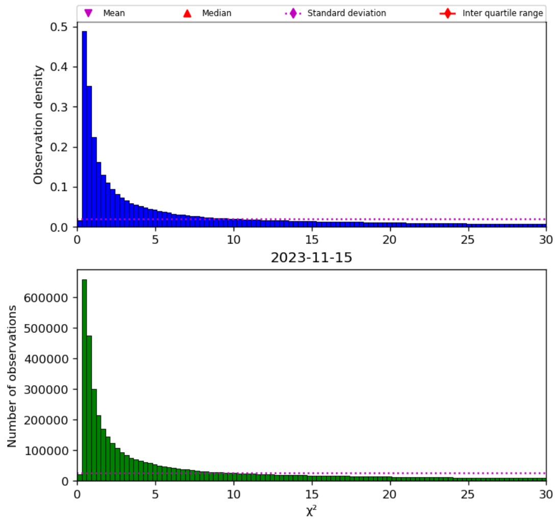
Figure 38: Histogram of “ \chi^2 ” for 2023-11-14 to 2023-11-16
