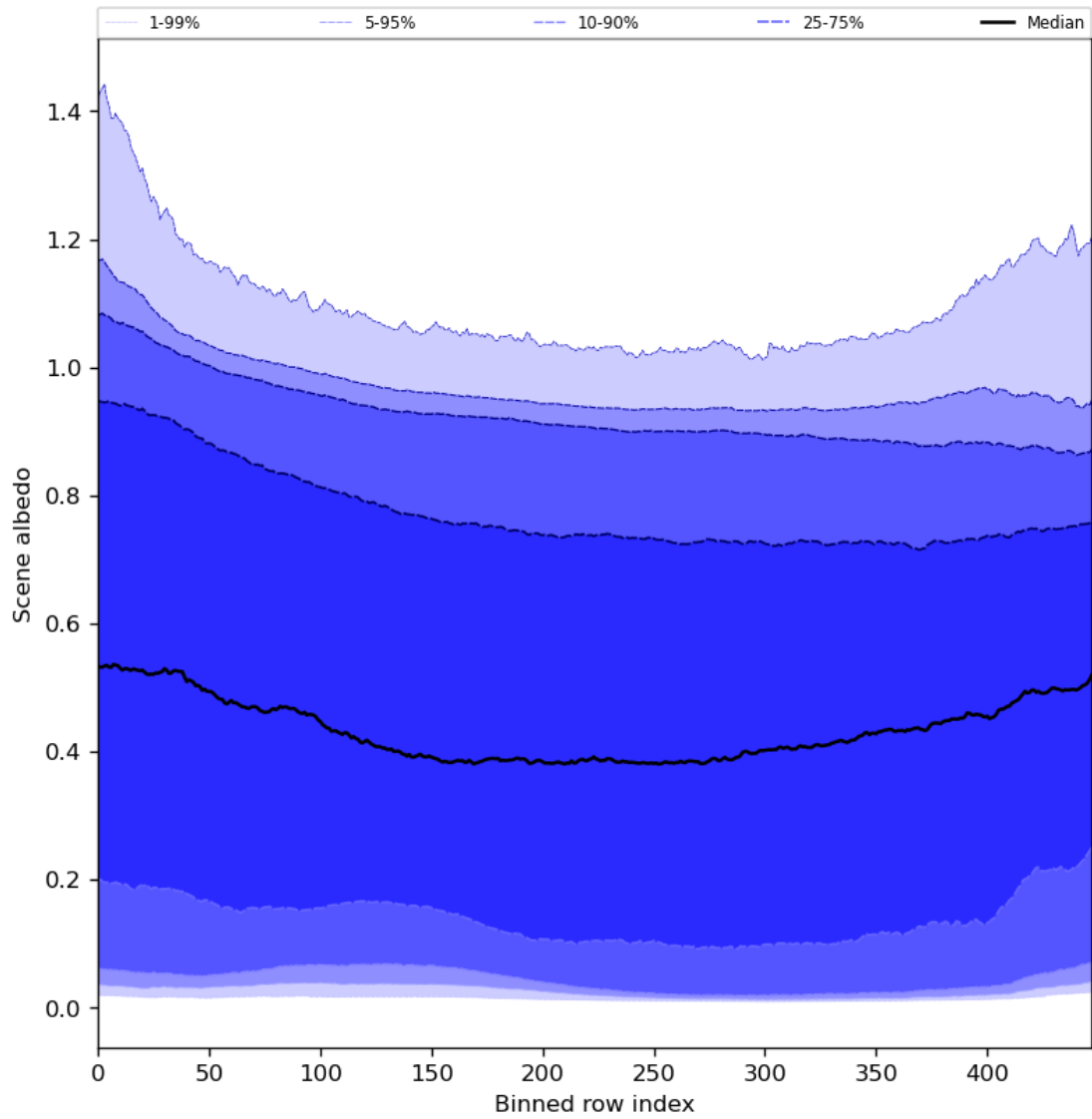
Figure 51: Along track statistics of “Scene albedo” for 2023-11-14 to 2023-11-16
