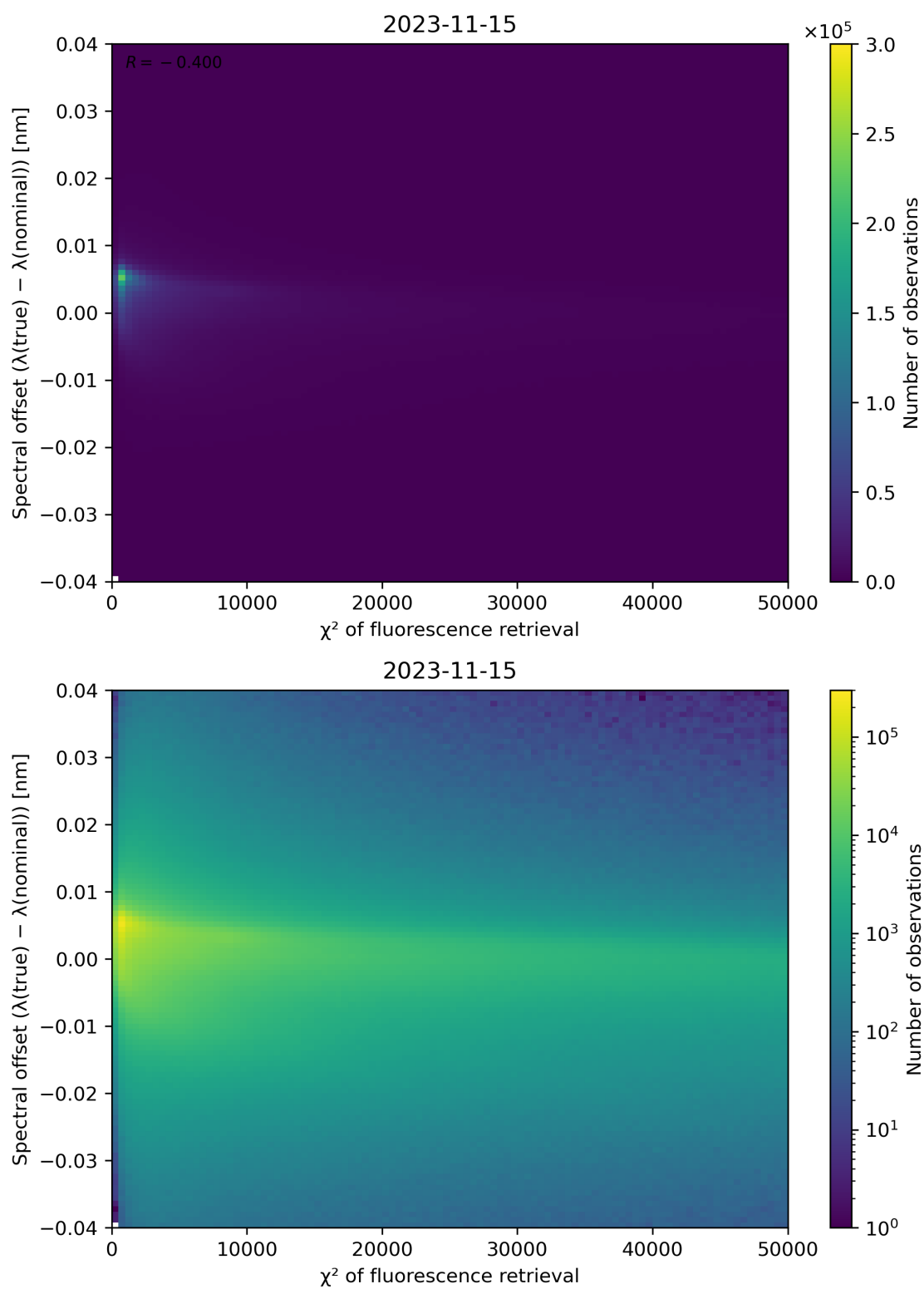
Figure 72: Scatter density plot of “ \chi^2 of fluorescence retrieval” against “Spectral offset ( \lambda(\text{true}) - \lambda(\text{nominal}) )” for 2023-11-14 to 2023-11-16.
