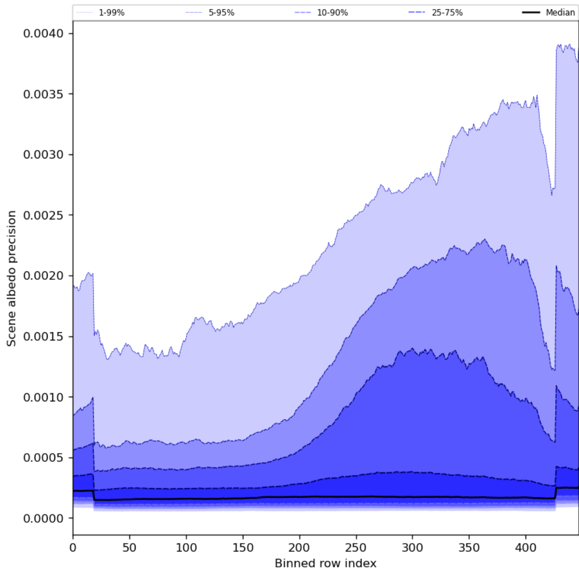
Figure 52: Along track statistics of “Scene albedo precision” for 2023-11-14 to 2023-11-16
