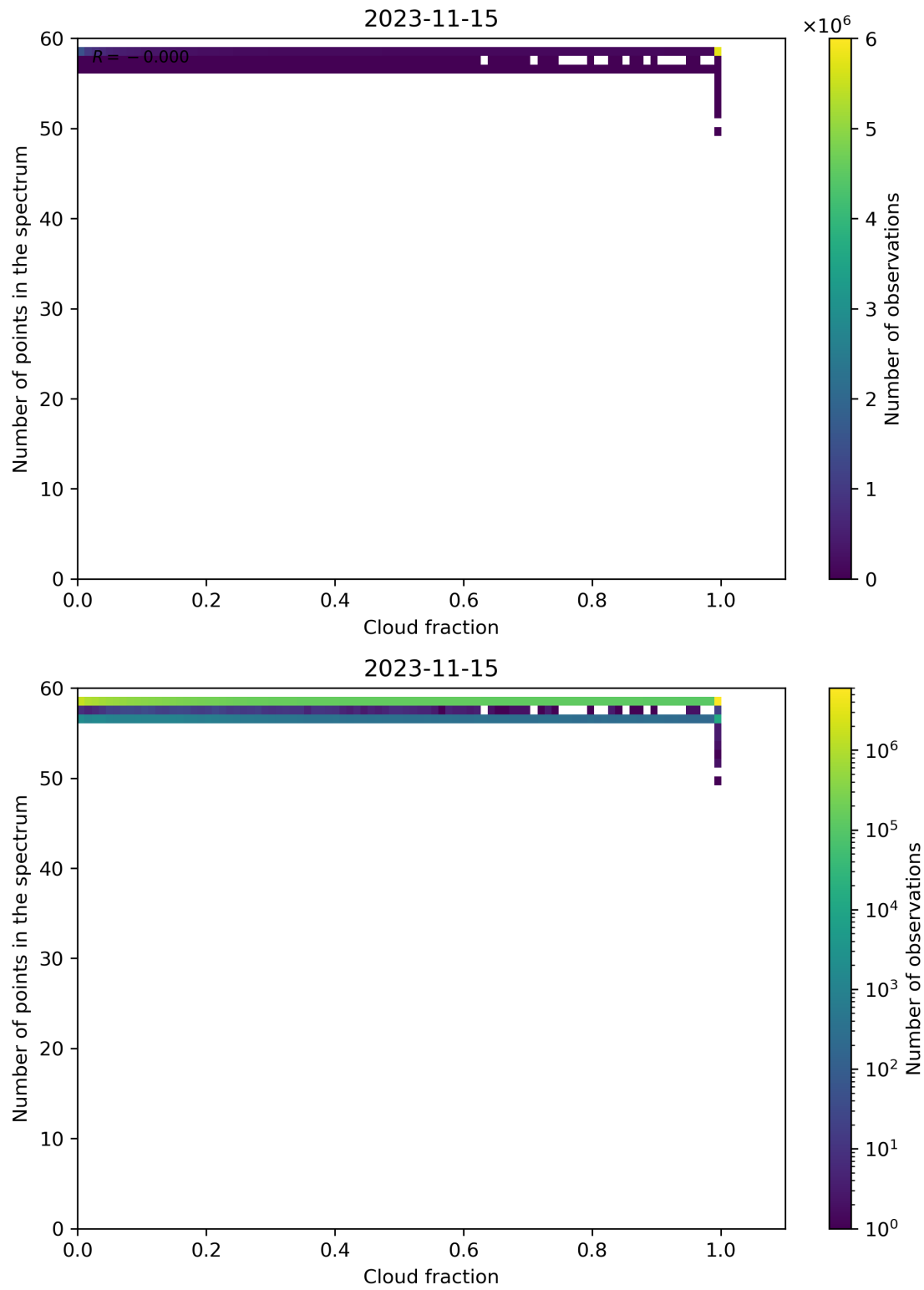
Figure 81: Scatter density plot of “Cloud fraction” against “Number of points in the spectrum” for 2023-11-14 to 2023-11-16.
