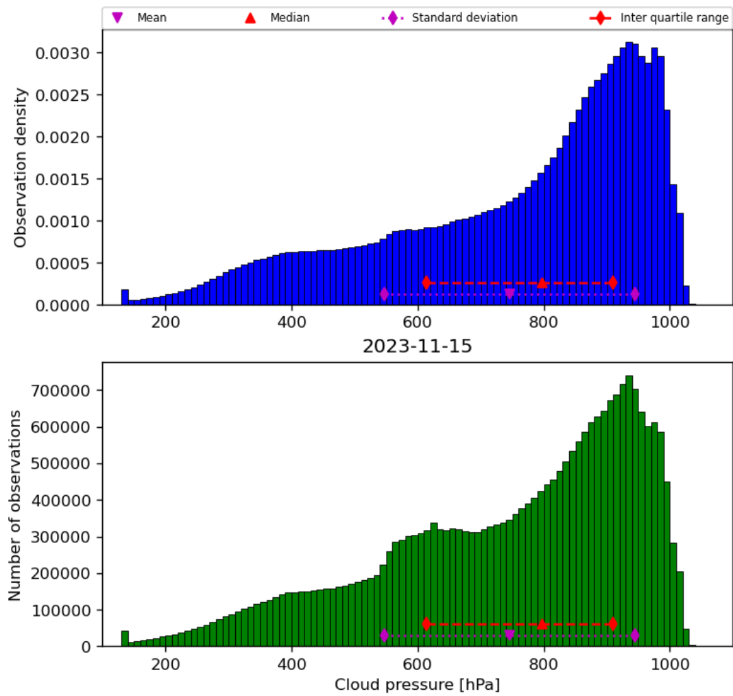
Figure 30: Histogram of “Cloud pressure” for 2023-11-14 to 2023-11-16
