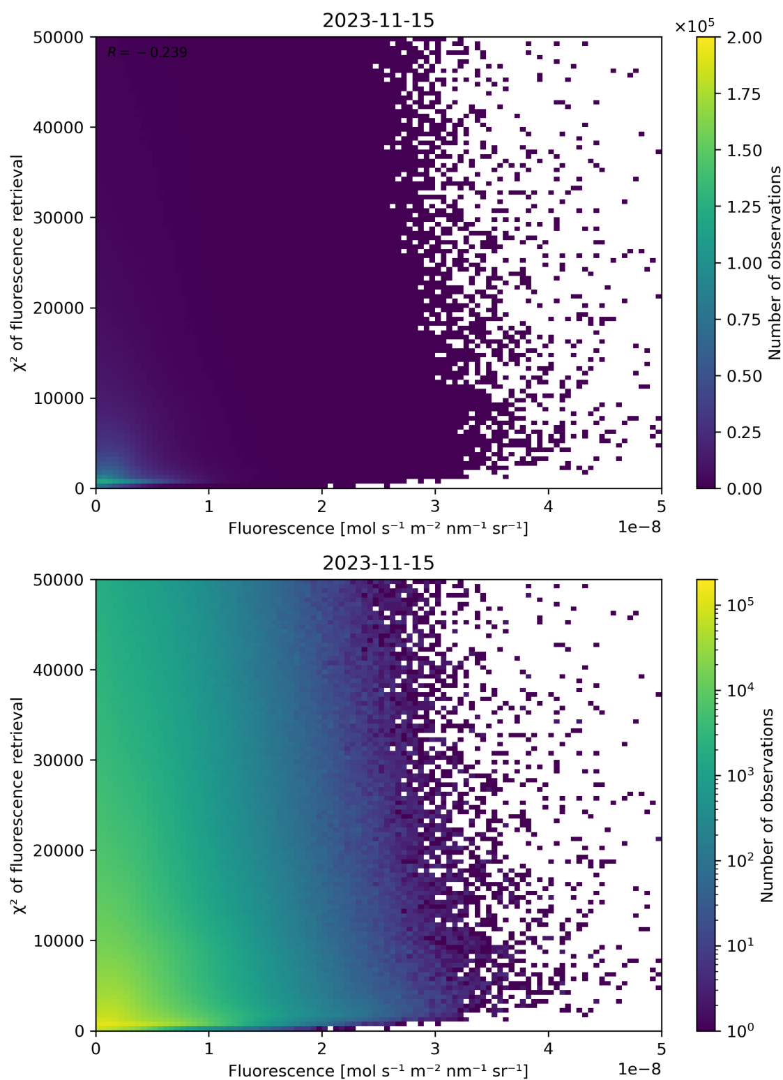
Figure 93: Scatter density plot of “Fluorescence” against “ \chi^2 of fluorescence retrieval” for 2023-11-14 to 2023-11-16.
