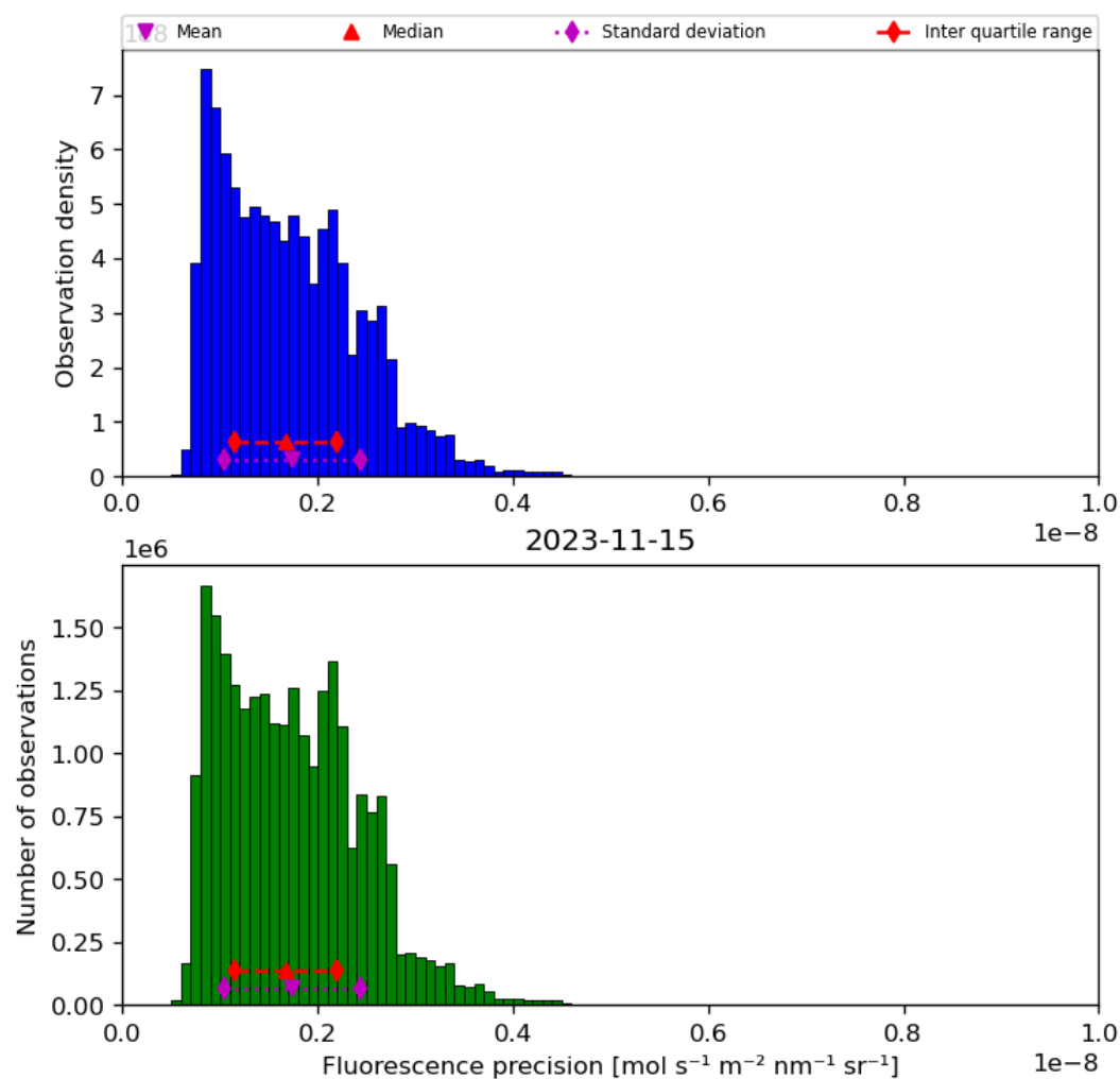
Figure 41: Histogram of “Fluorescence precision” for 2023-11-14 to 2023-11-16
