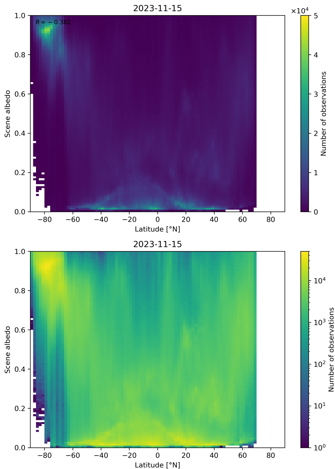
Figure 104: Scatter density plot of “Latitude” against “Scene albedo” for 2023-11-14 to 2023-11-16.
