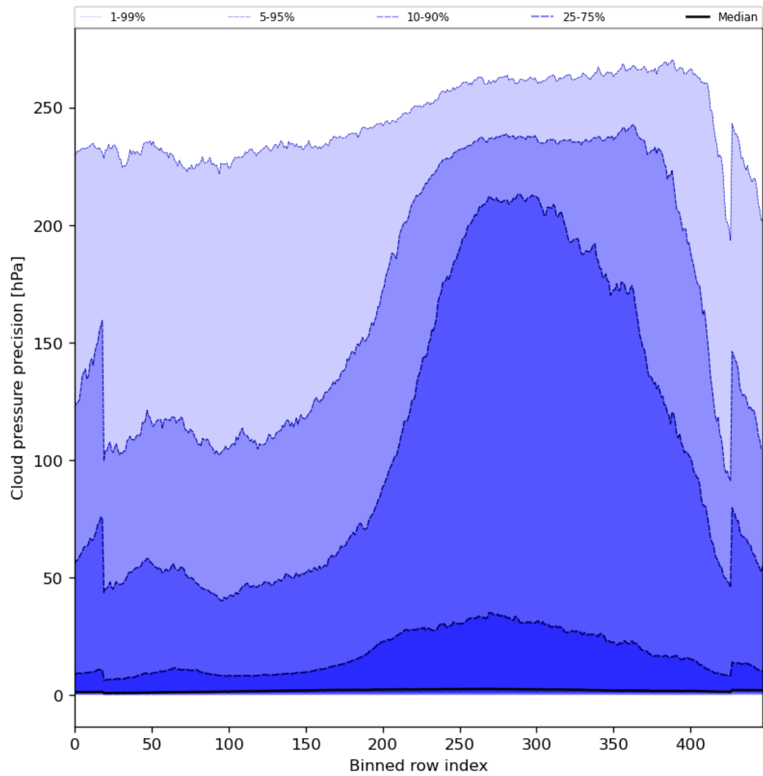
Figure 48: Along track statistics of “Cloud pressure precision” for 2023-11-14 to 2023-11-16
