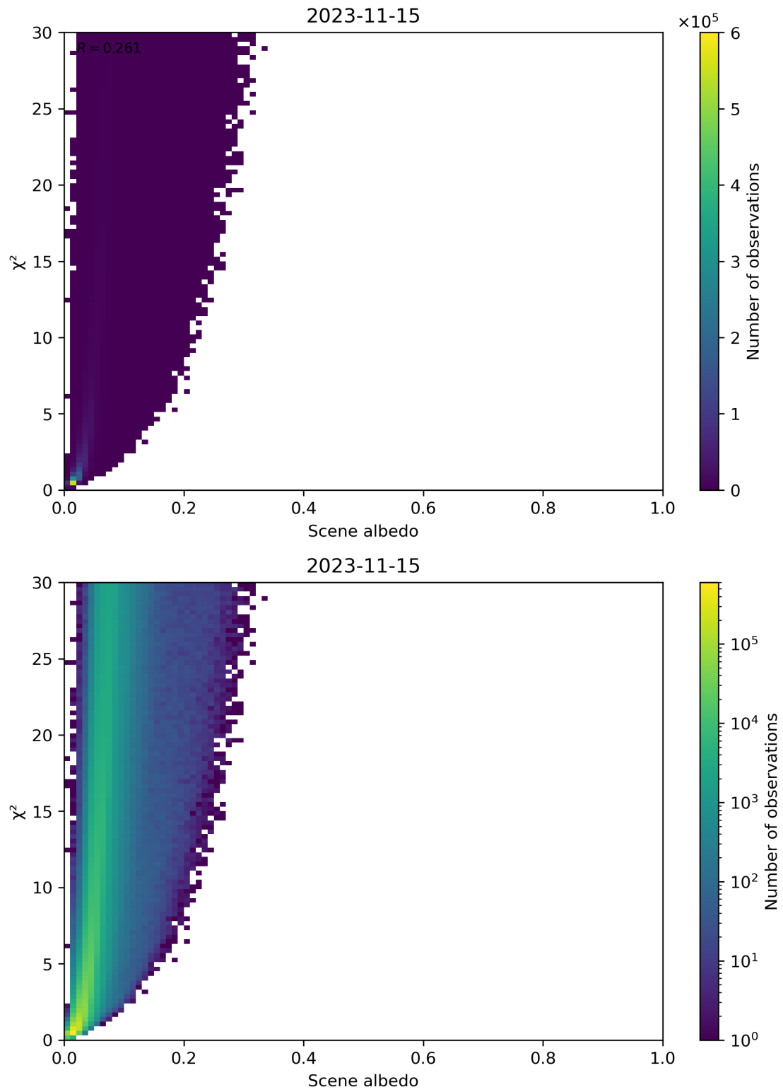
Figure 112: Scatter density plot of “Scene albedo” against “ \chi^2 ” for 2023-11-14 to 2023-11-16.
