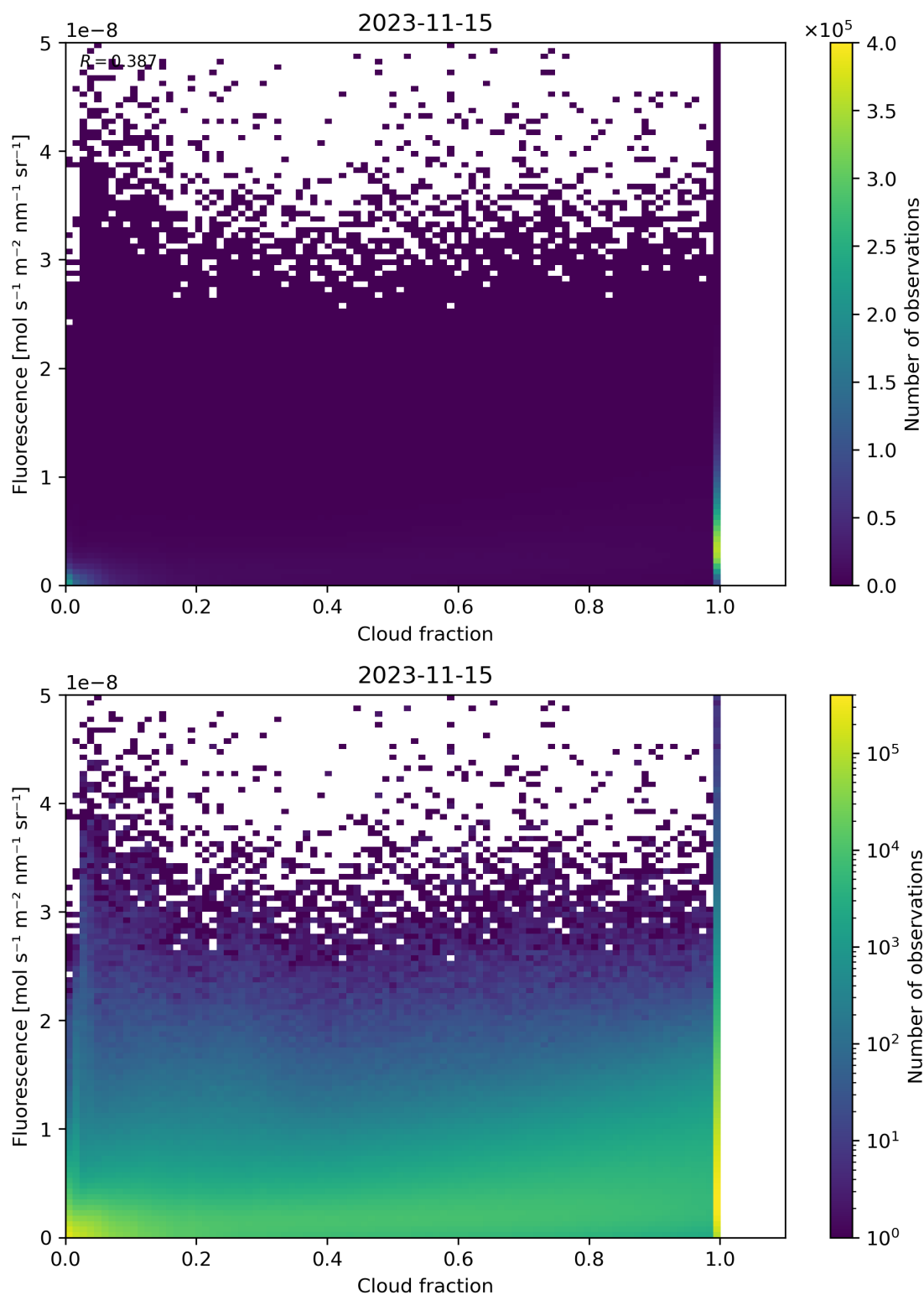
Figure 79: Scatter density plot of “Cloud fraction” against “Fluorescence” for 2023-11-14 to 2023-11-16.
