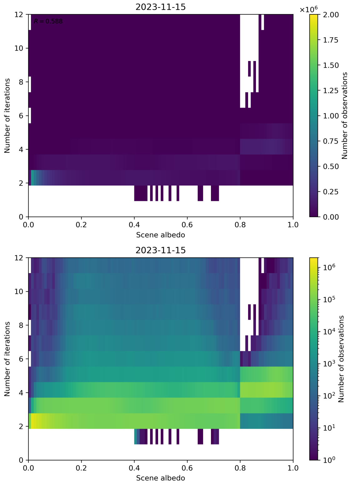
Figure 115: Scatter density plot of “Scene albedo” against “Number of iterations” for 2023-11-14 to 2023-11-16.
