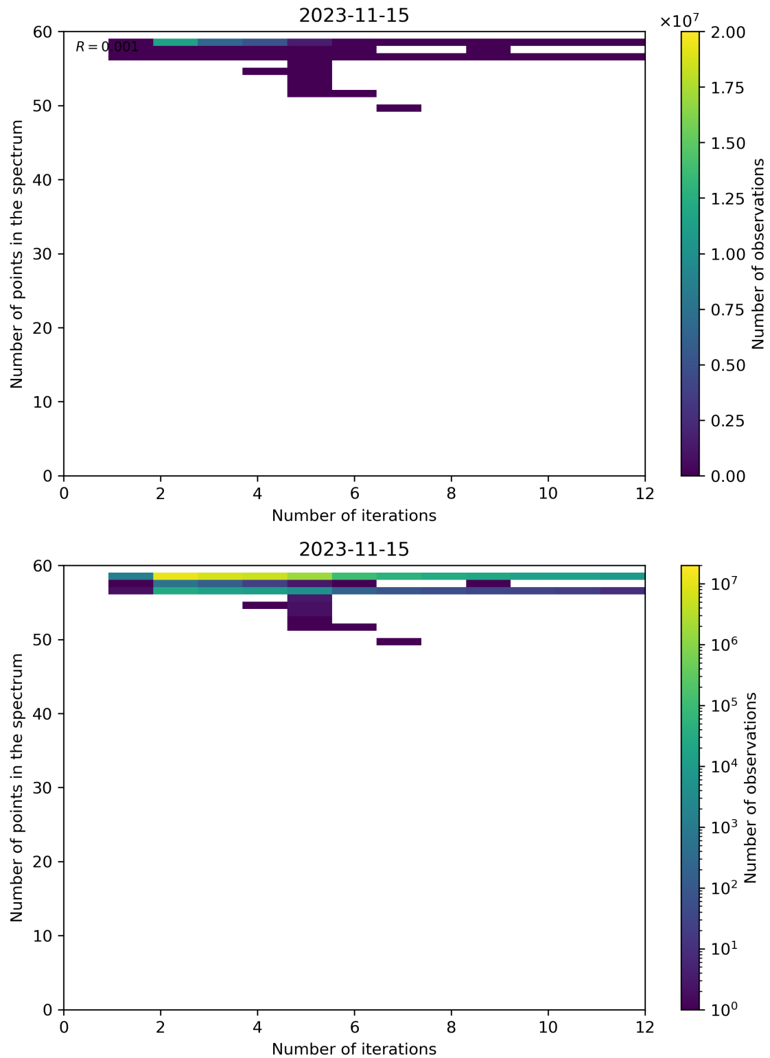
Figure 108: Scatter density plot of “Number of iterations” against “Number of points in the spectrum” for 2023-11-14 to 2023-11-16.
