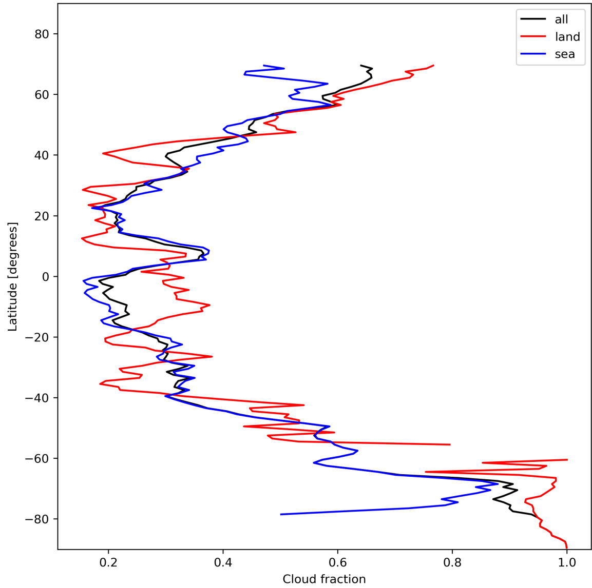
Figure 15: Zonal average of “Cloud fraction” for 2023-11-14 to 2023-11-16.
