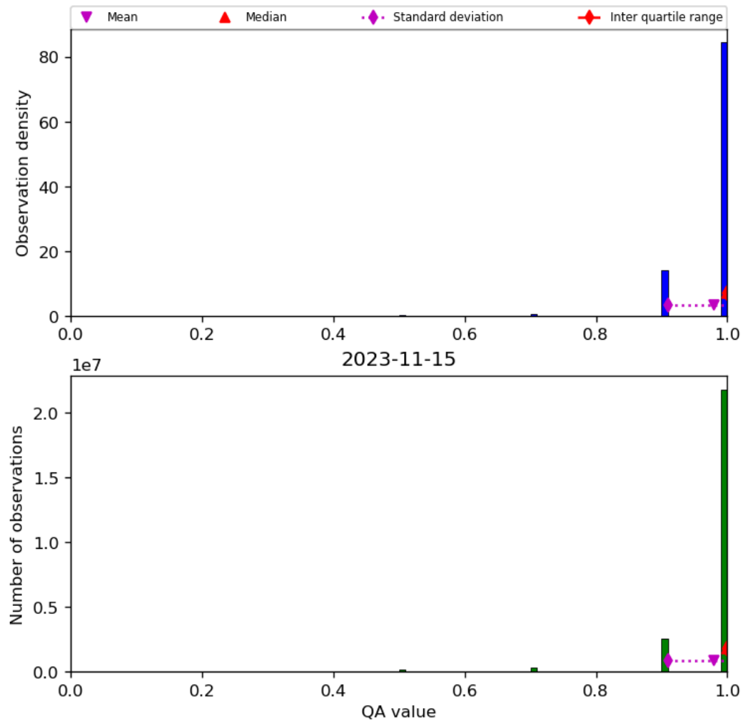
Figure 29: Histogram of “QA value” for 2023-11-14 to 2023-11-16
