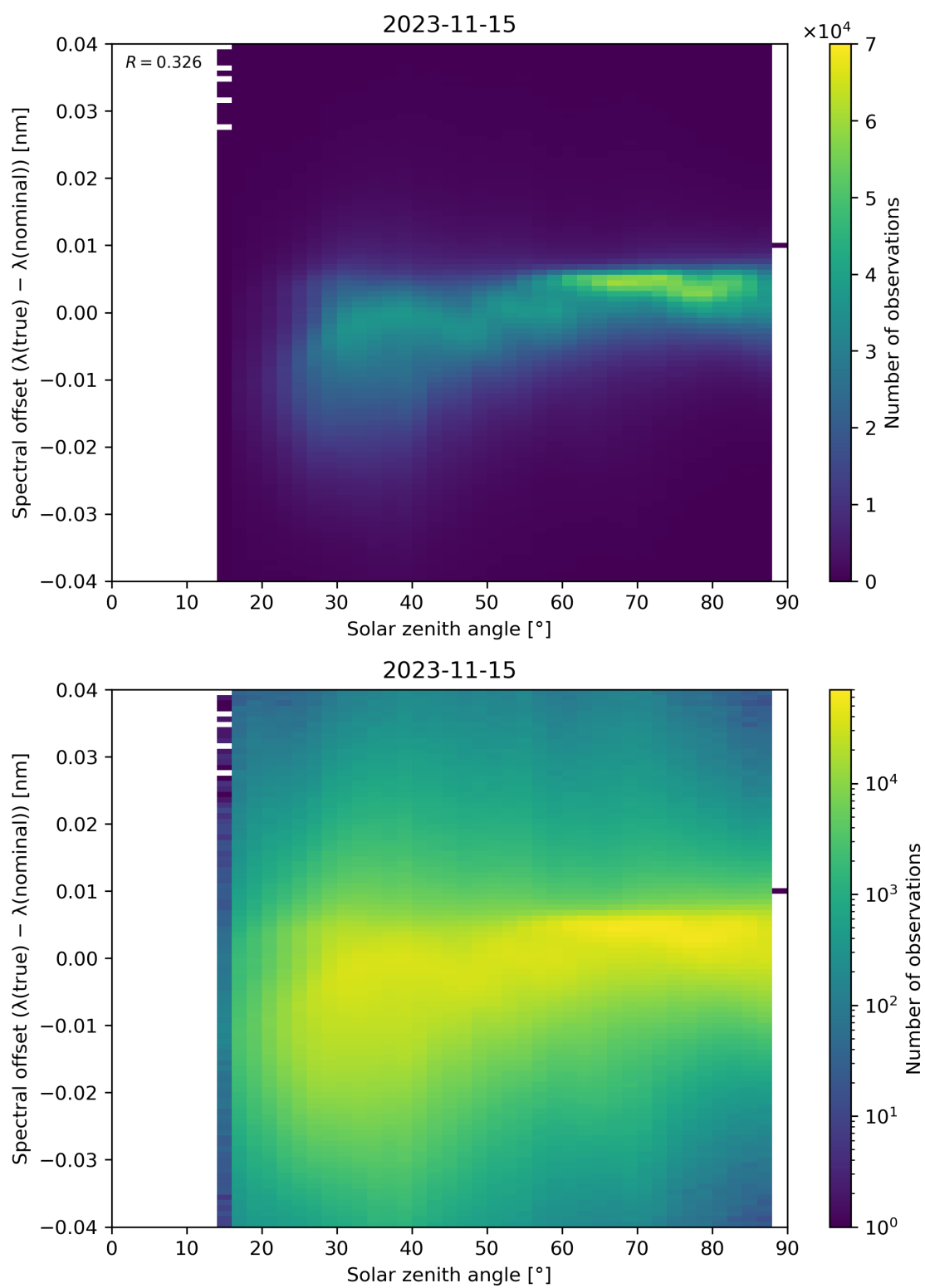
Figure 128: Scatter density plot of “Solar zenith angle” against “Spectral offset ( \lambda(\text{true}) - \lambda(\text{nominal}) )” for 2023-11-14 to 2023-11-16.
