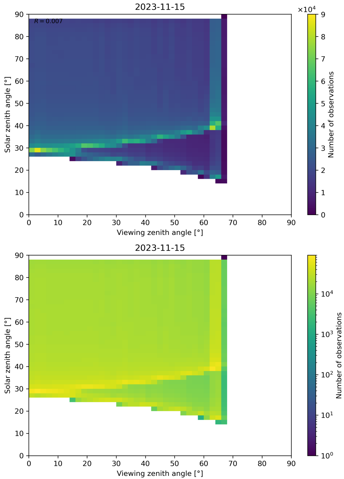
Figure 139: Scatter density plot of “Viewing zenith angle” against “Solar zenith angle” for 2023-11-14 to 2023-11-16.
