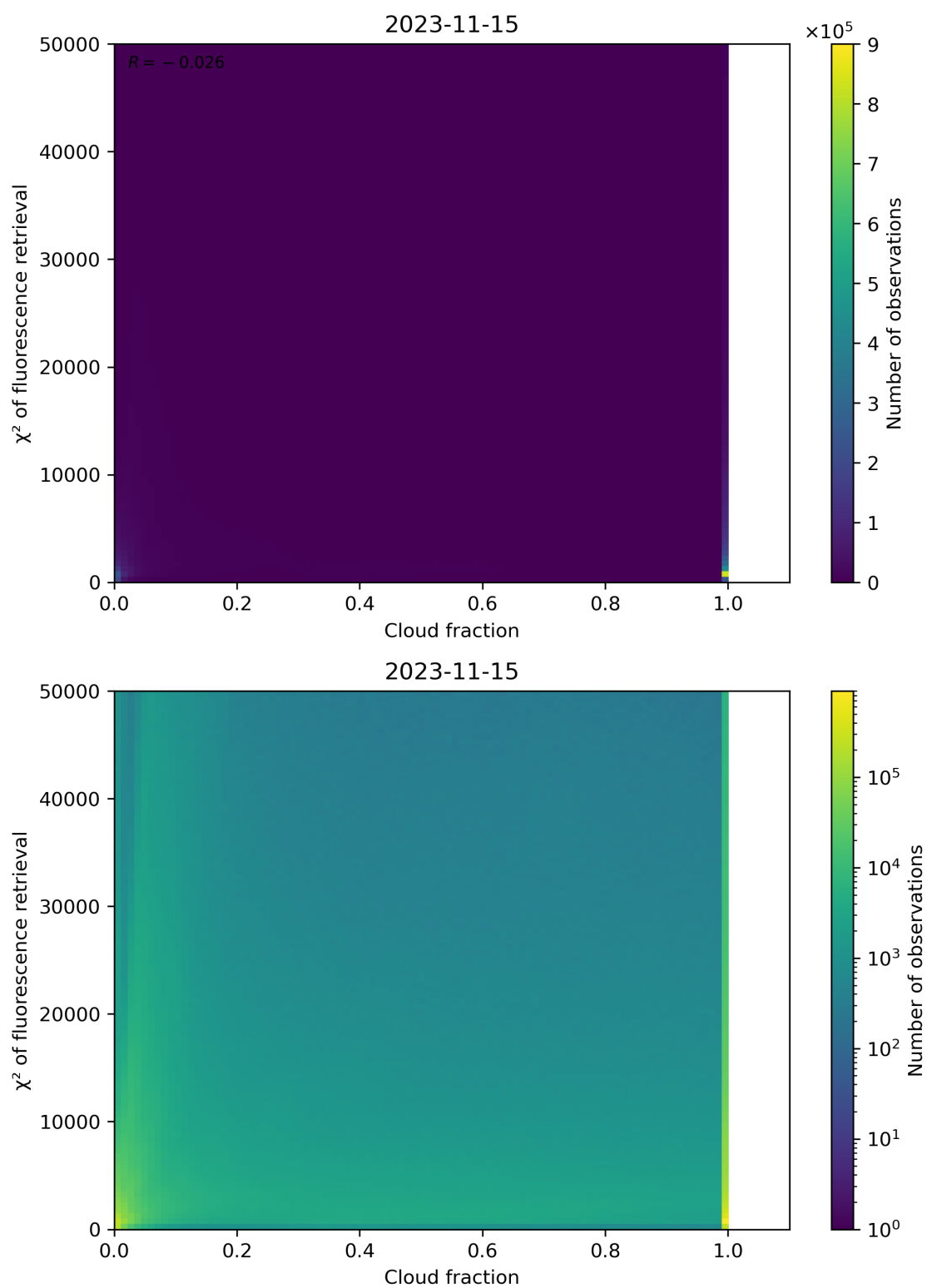
Figure 78: Scatter density plot of “Cloud fraction” against “ \chi^2 of fluorescence retrieval” for 2023-11-14 to 2023-11-16.
