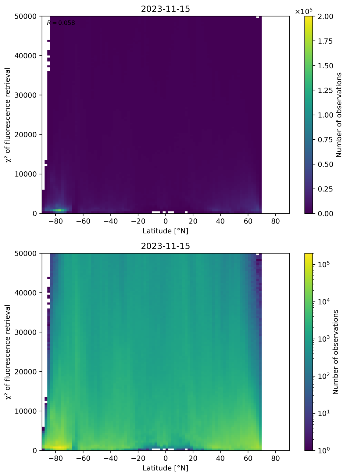
Figure 98: Scatter density plot of “Latitude” against “ \chi^2 of fluorescence retrieval” for 2023-11-14 to 2023-11-16.
