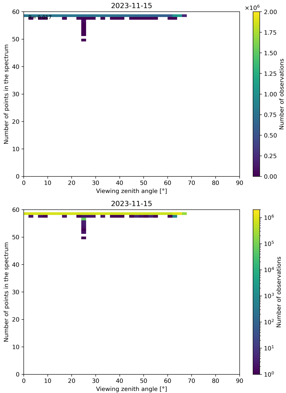
Figure 137: Scatter density plot of “Viewing zenith angle” against “Number of points in the spectrum” for 2023-11-14 to 2023-11-16.
