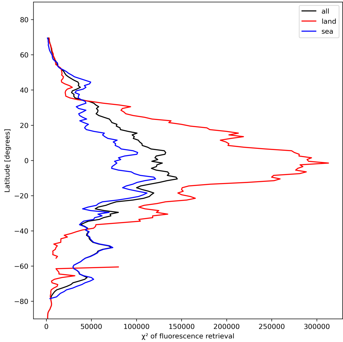
Figure 25: Zonal average of “ \chi^2 of fluorescence retrieval” for 2023-11-14 to 2023-11-16.
