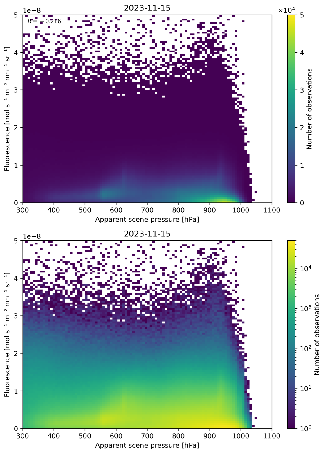
Figure 65: Scatter density plot of “Apparent scene pressure” against “Fluorescence” for 2023-11-14 to 2023-11-16.
