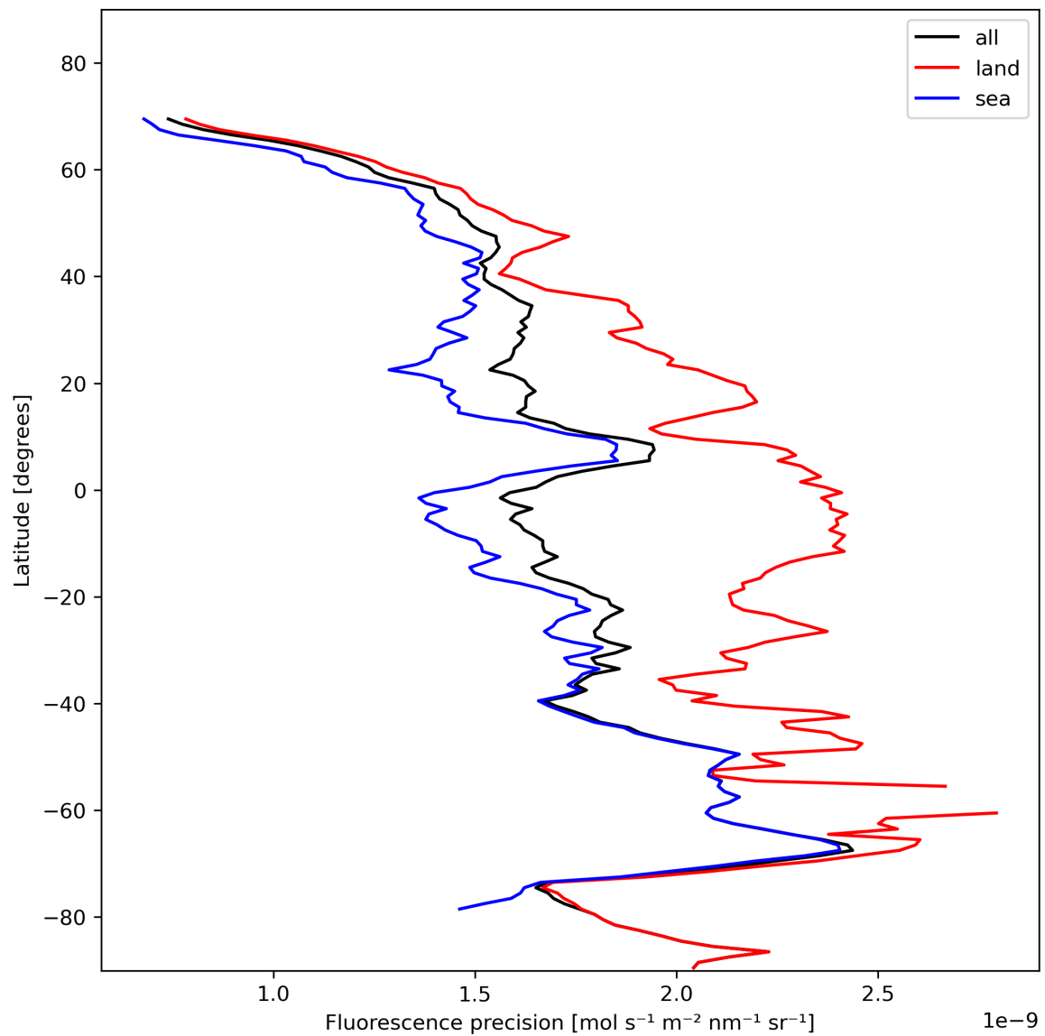
Figure 24: Zonal average of “Fluorescence precision” for 2023-11-14 to 2023-11-16.
