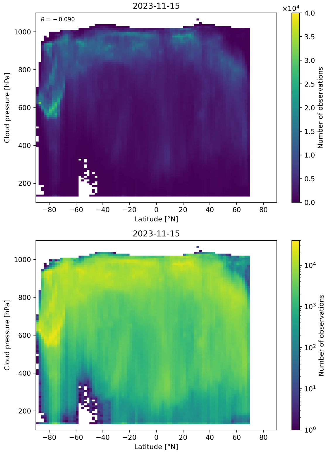
Figure 100: Scatter density plot of “Latitude” against “Cloud pressure” for 2023-11-14 to 2023-11-16.
