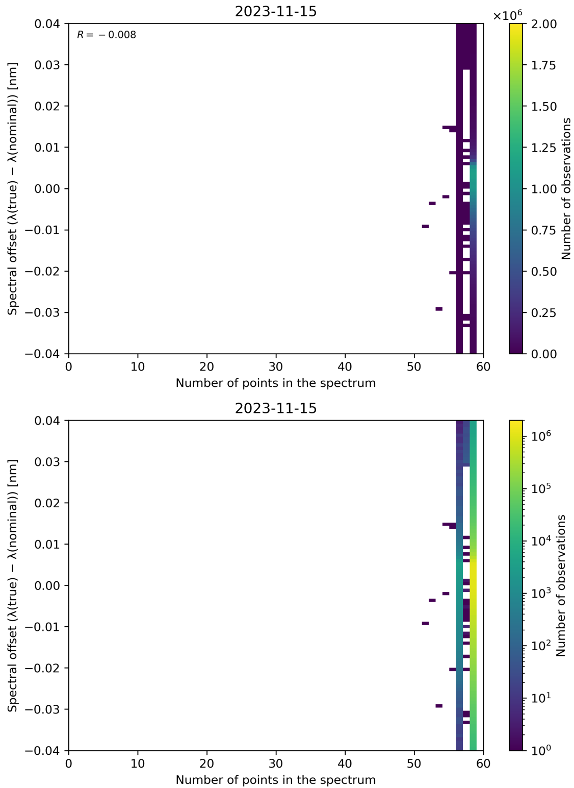
Figure 110: Scatter density plot of “Number of points in the spectrum” against “Spectral offset ( \lambda(\text{true}) - \lambda(\text{nominal}) )” for 2023-11-14 to 2023-11-16.
