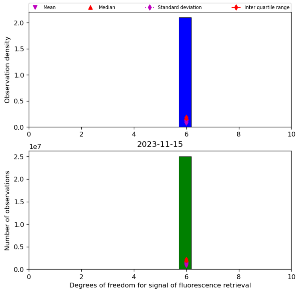
Figure 43: Histogram of “Degrees of freedom for signal of fluorescence retrieval” for 2023-11-14 to 2023-11-16
