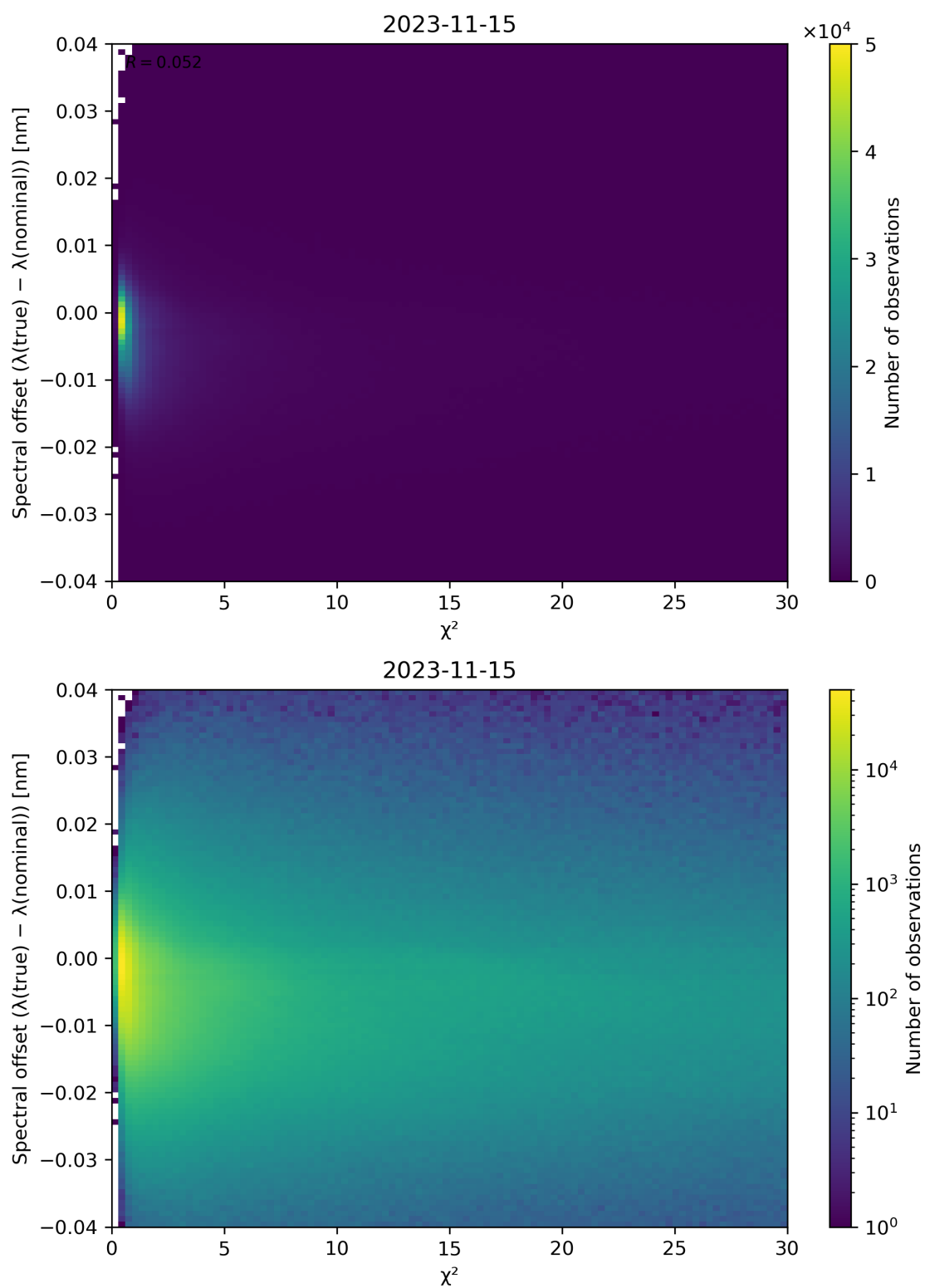
Figure 75: Scatter density plot of “ \chi^2 ” against “Spectral offset ( \lambda(\text{true}) - \lambda(\text{nominal}) )” for 2023-11-14 to 2023-11-16.
