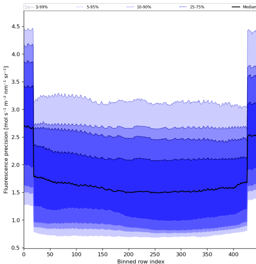
Figure 58: Along track statistics of “Fluorescence precision” for 2023-11-14 to 2023-11-16
