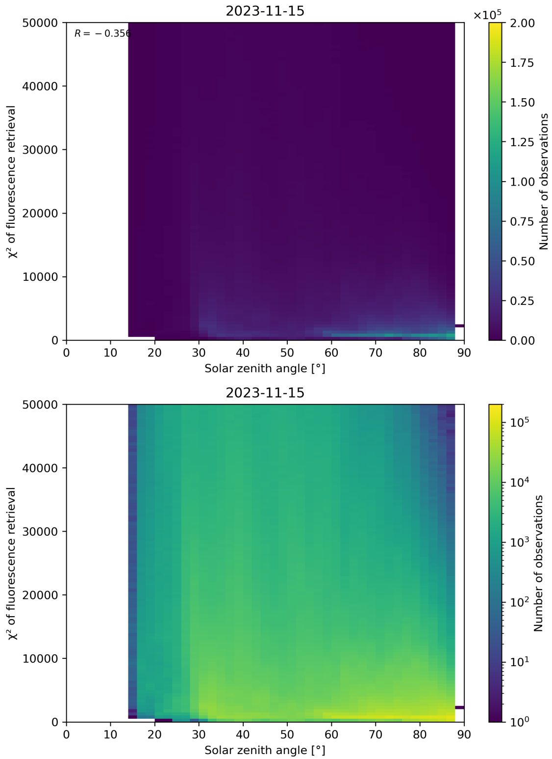
Figure 120: Scatter density plot of “Solar zenith angle” against “ \chi^2 of fluorescence retrieval” for 2023-11-14 to 2023-11-16.
