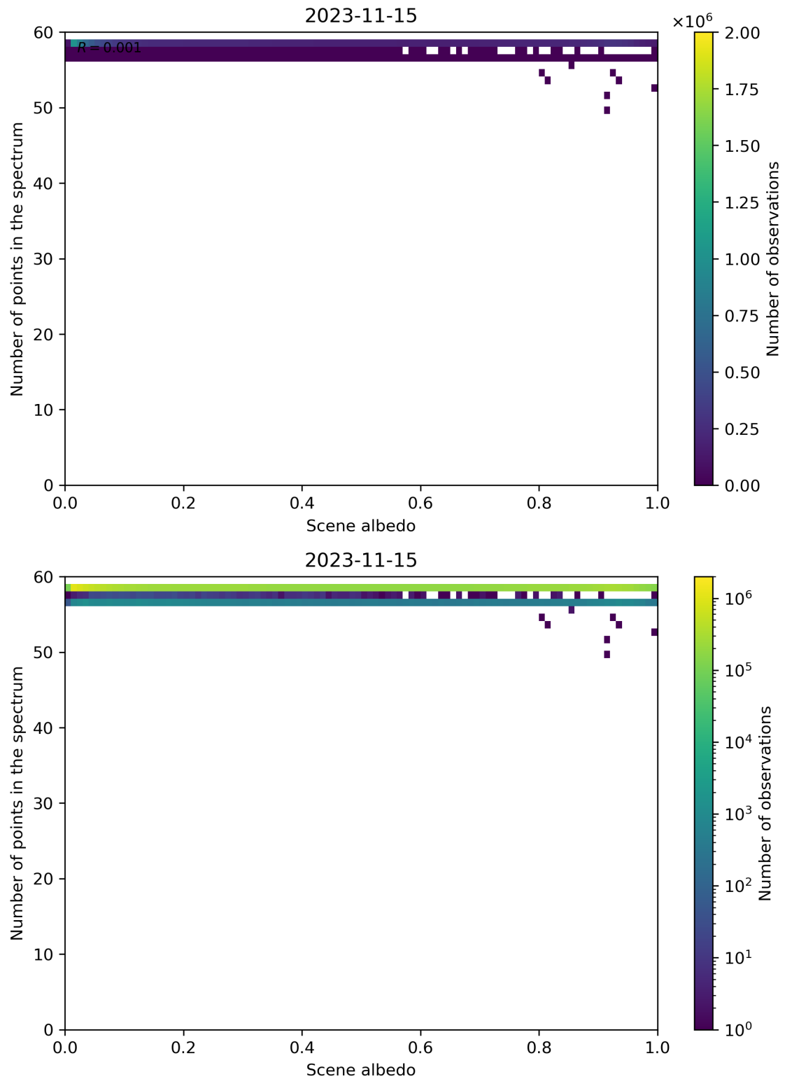
Figure 116: Scatter density plot of “Scene albedo” against “Number of points in the spectrum” for 2023-11-14 to 2023-11-16.
