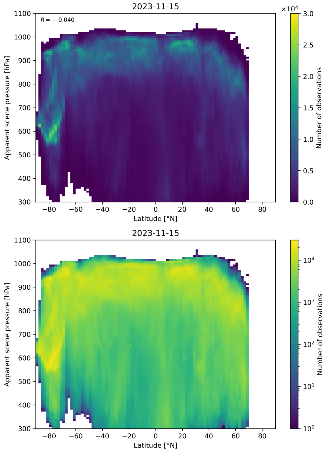
Figure 96: Scatter density plot of “Latitude” against “Apparent scene pressure” for 2023-11-14 to 2023-11-16.
