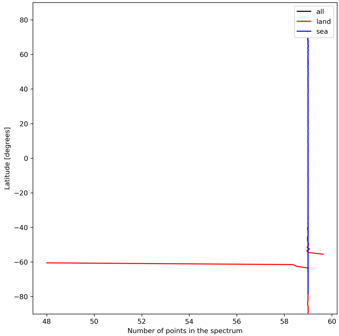
Figure 27: Zonal average of “Number of points in the spectrum” for 2023-11-14 to 2023-11-16.
