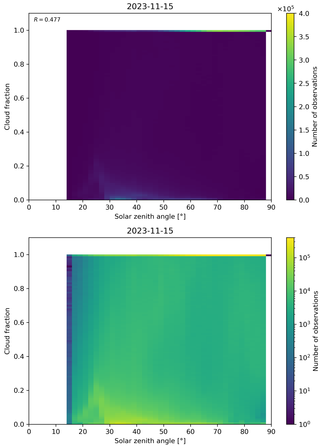
Figure 121: Scatter density plot of “Solar zenith angle” against “Cloud fraction” for 2023-11-14 to 2023-11-16.
