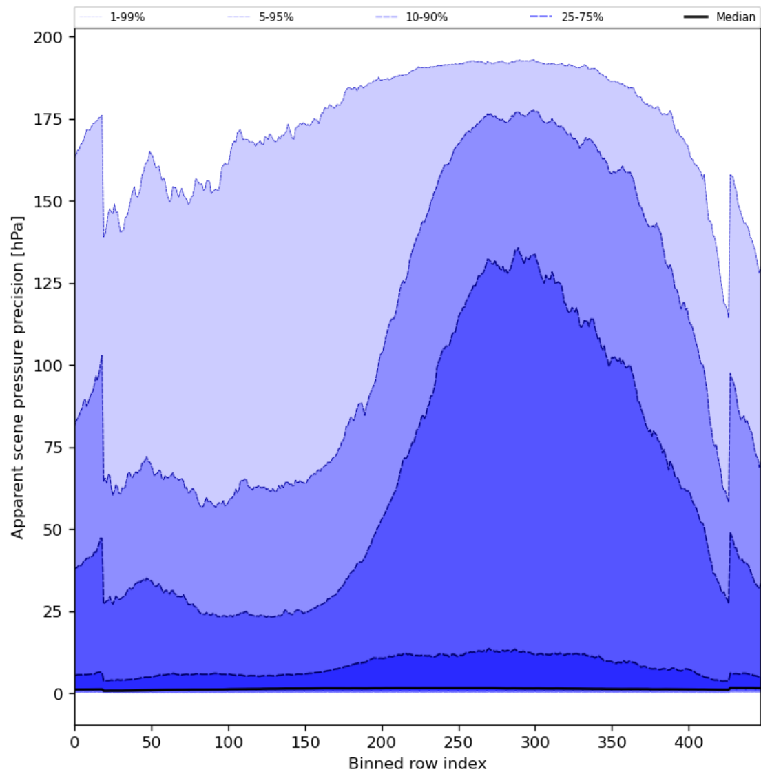
Figure 54: Along track statistics of “Apparent scene pressure precision” for 2023-11-14 to 2023-11-16
