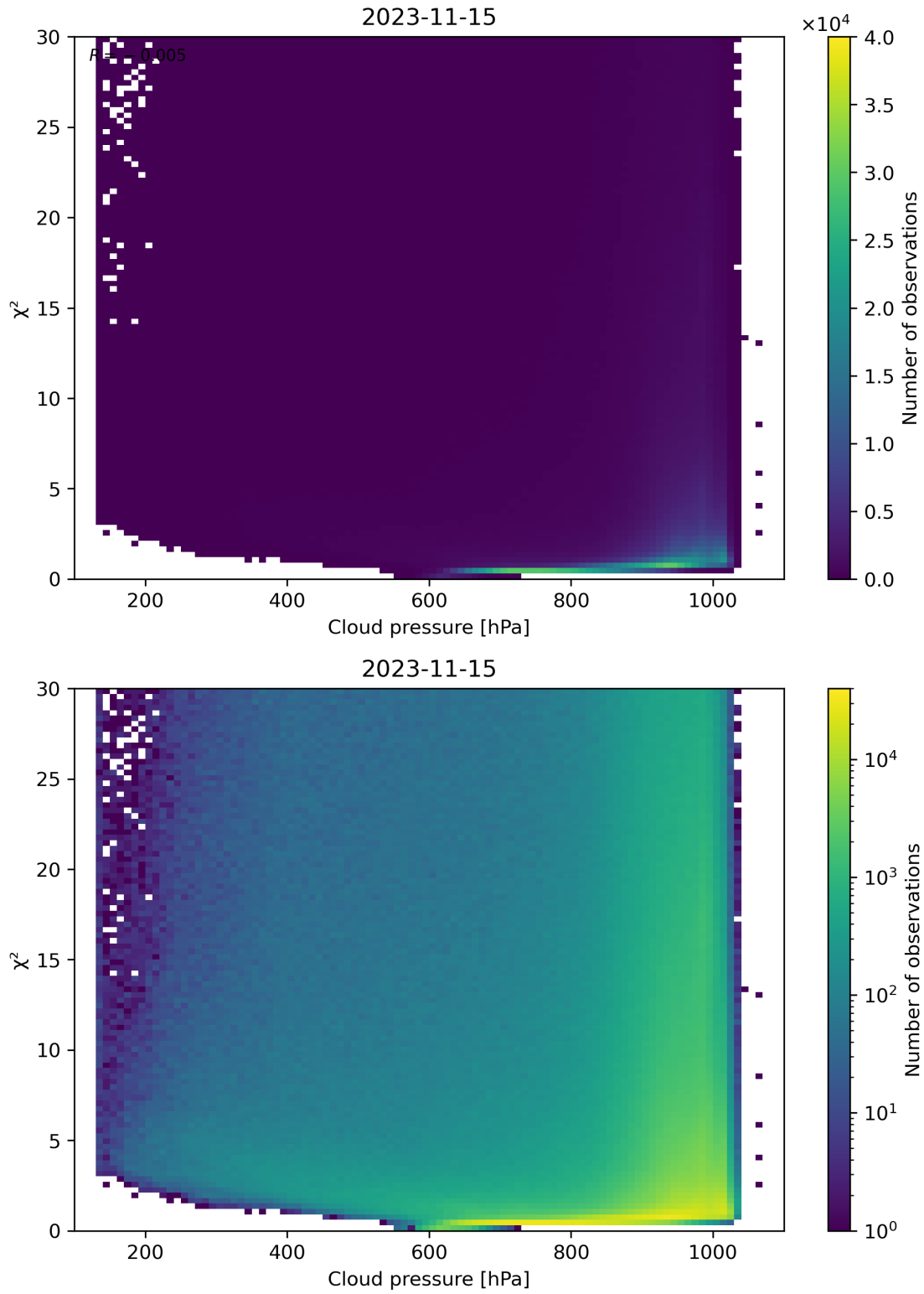
Figure 85: Scatter density plot of “Cloud pressure” against “ \chi^2 ” for 2023-11-14 to 2023-11-16.
