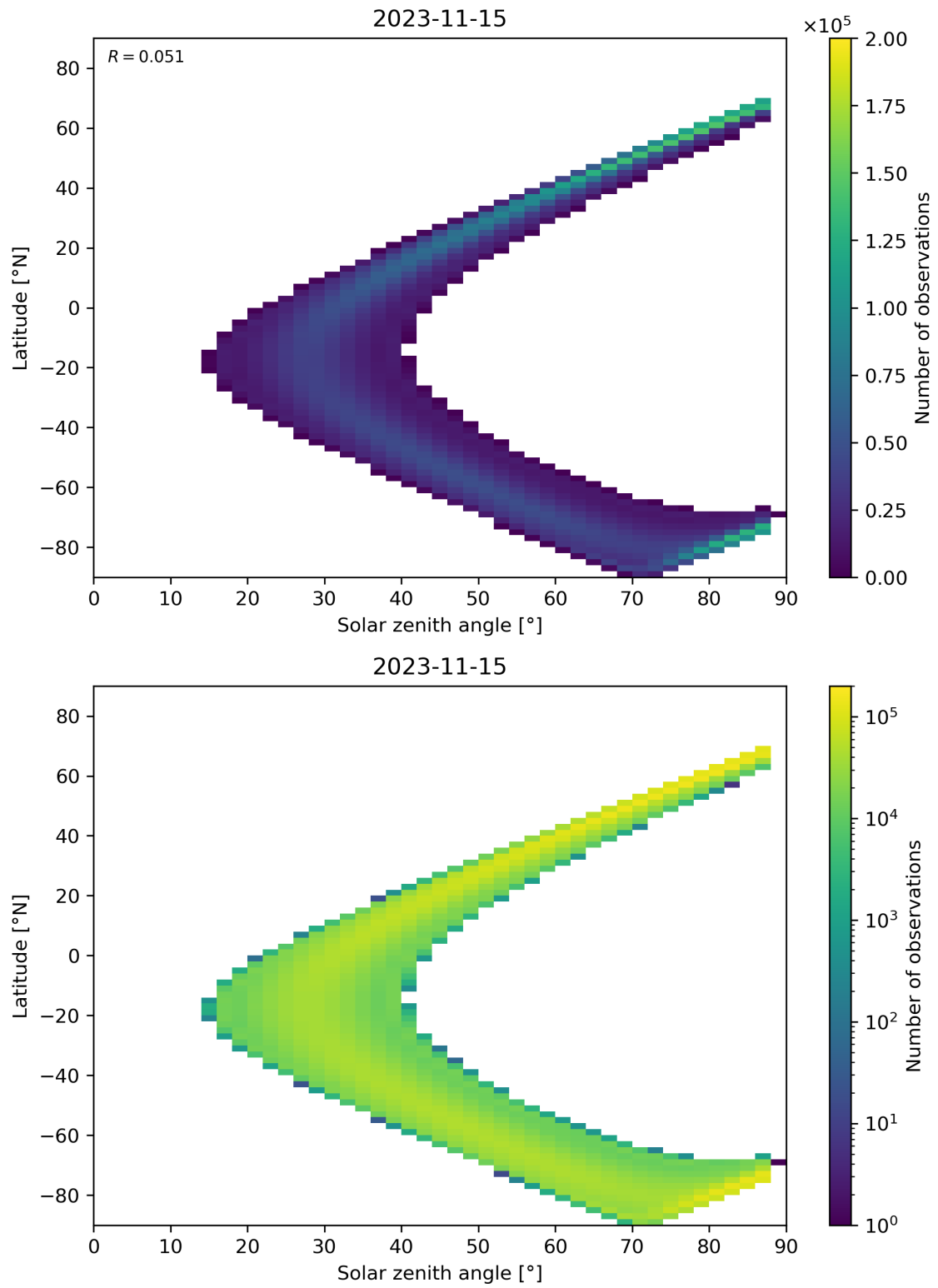
Figure 124: Scatter density plot of “Solar zenith angle” against “Latitude” for 2023-11-14 to 2023-11-16.
