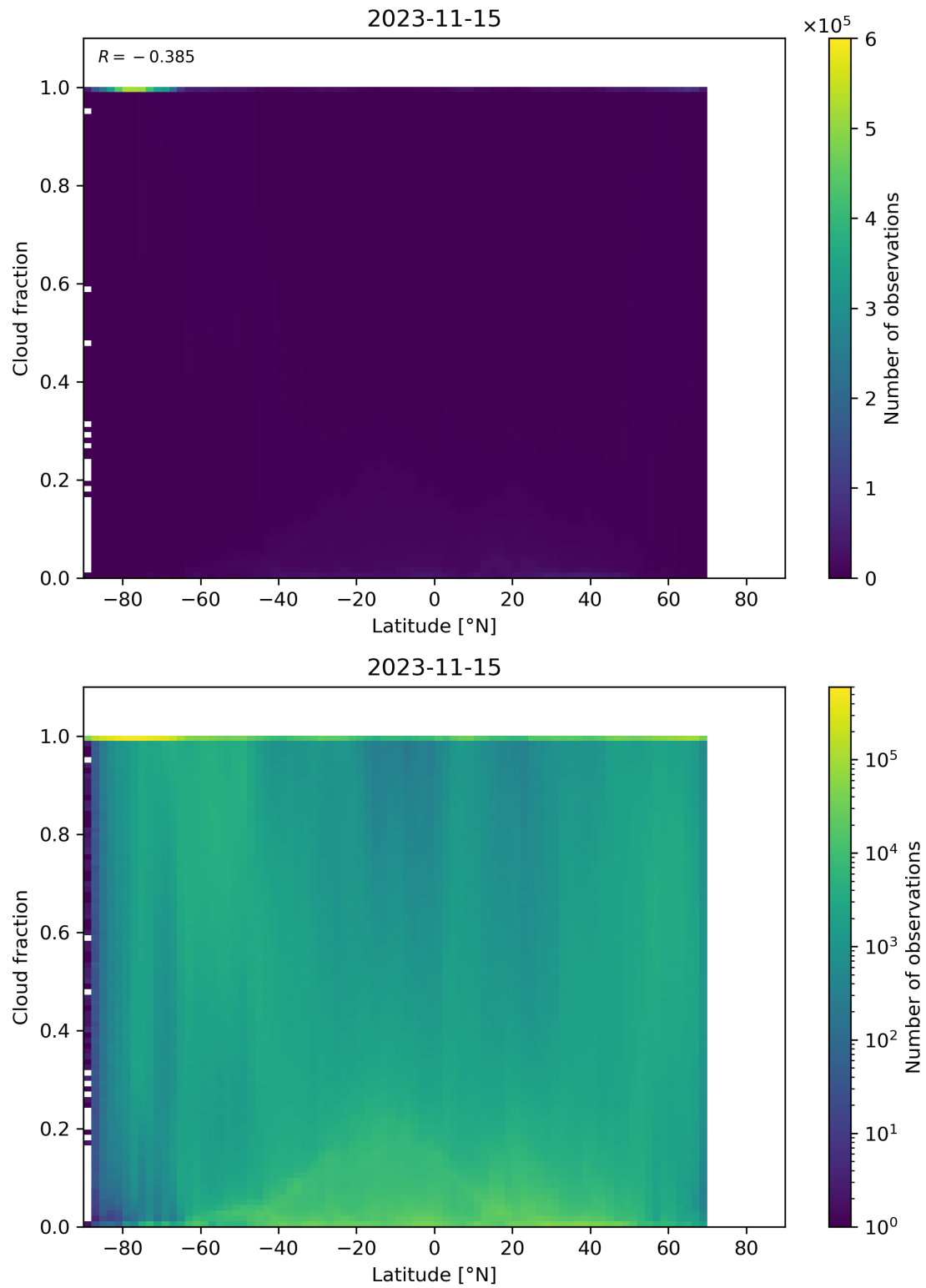
Figure 99: Scatter density plot of “Latitude” against “Cloud fraction” for 2023-11-14 to 2023-11-16.
