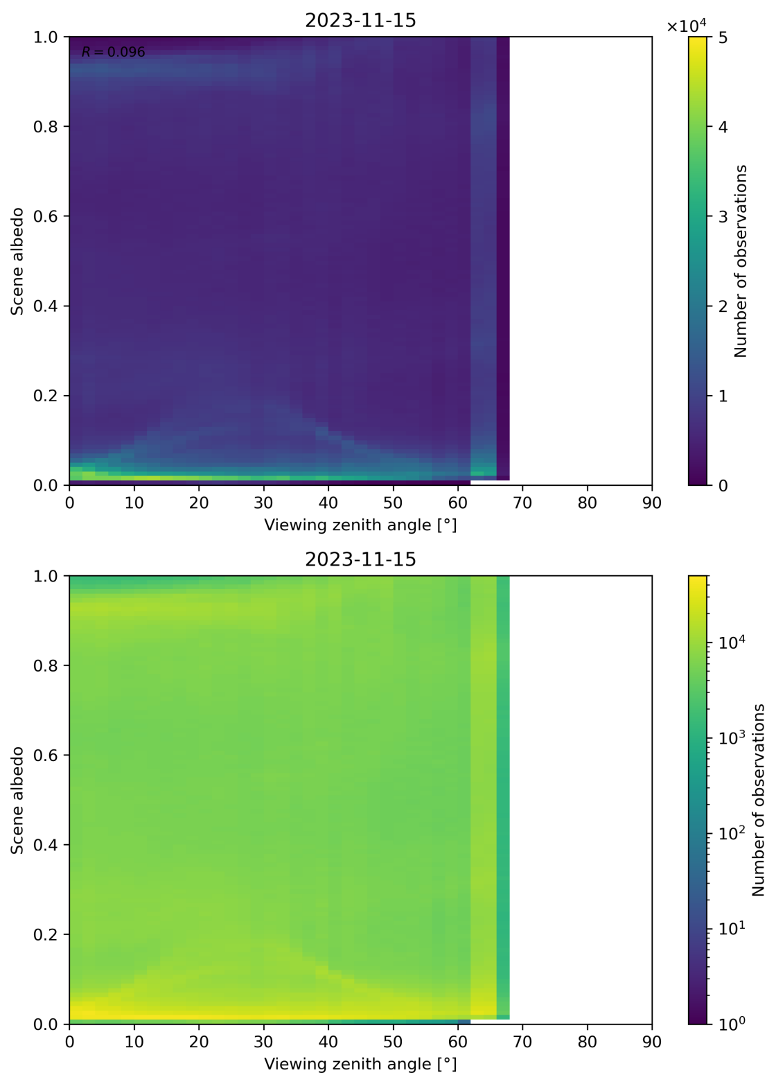
Figure 138: Scatter density plot of “Viewing zenith angle” against “Scene albedo” for 2023-11-14 to 2023-11-16.
