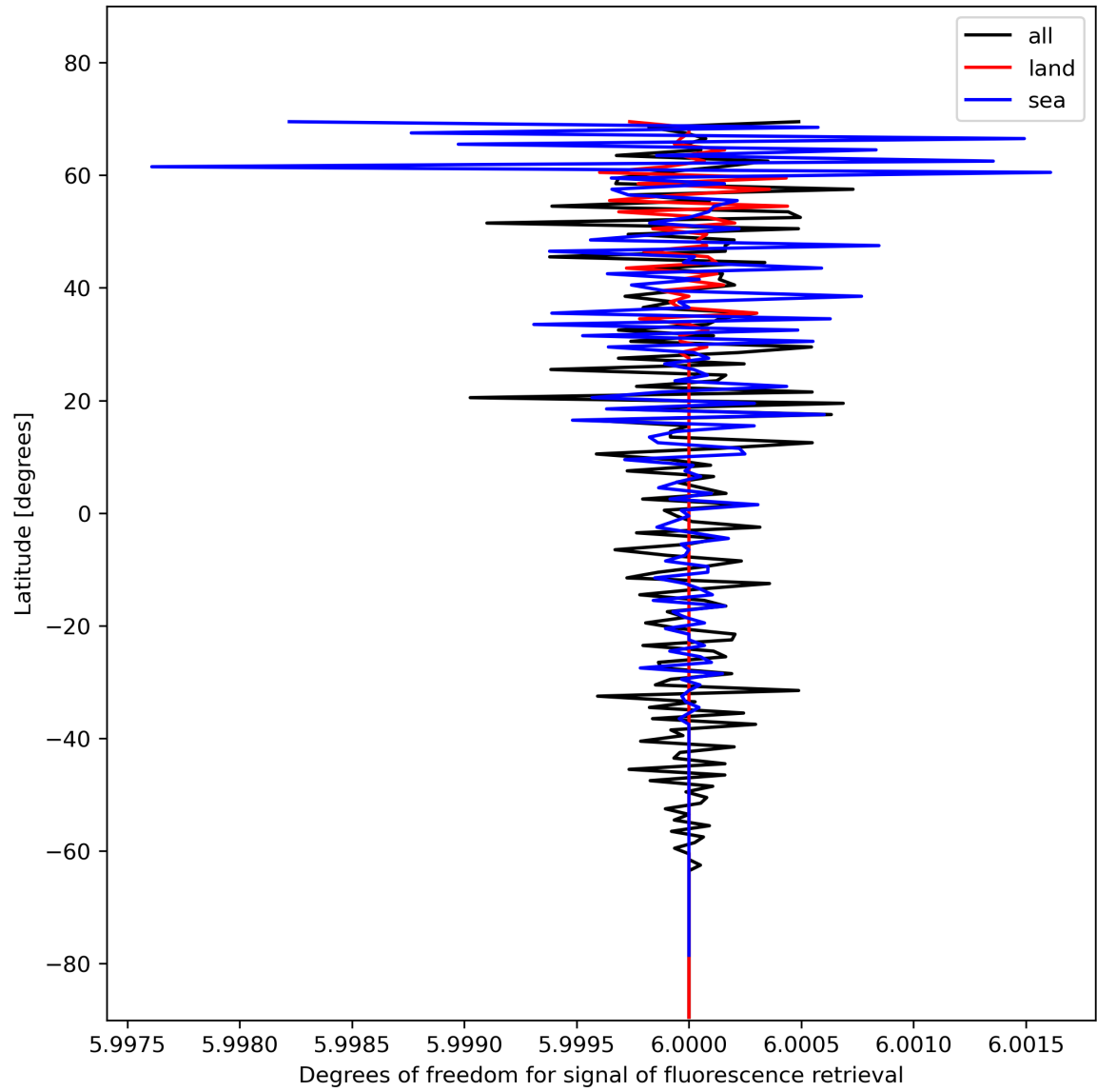
Figure 26: Zonal average of “Degrees of freedom for signal of fluorescence retrieval” for 2023-11-14 to 2023-11-16.
