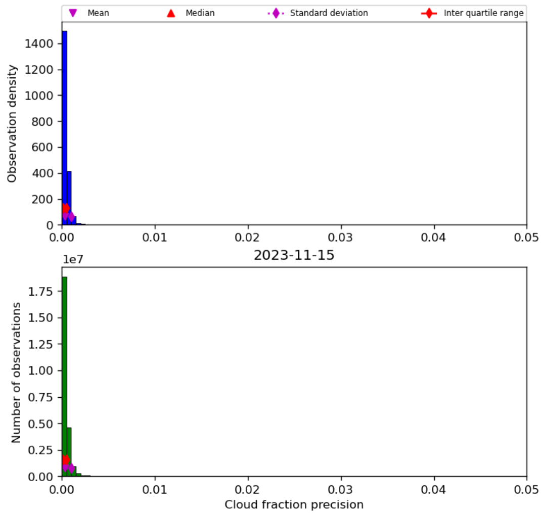
Figure 33: Histogram of “Cloud fraction precision” for 2023-11-14 to 2023-11-16
