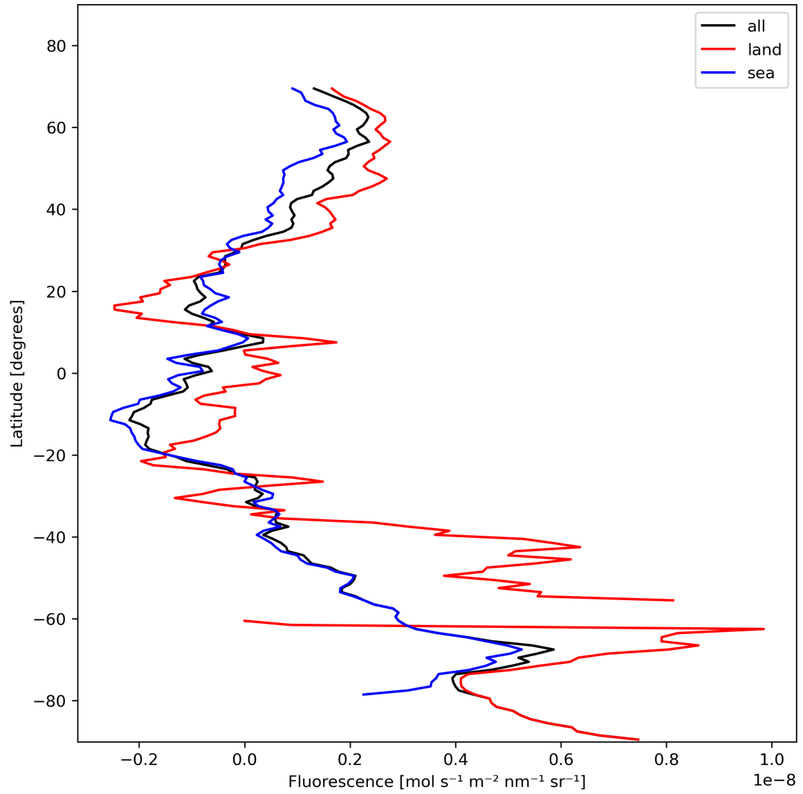
Figure 23: Zonal average of “Fluorescence” for 2023-11-14 to 2023-11-16.
