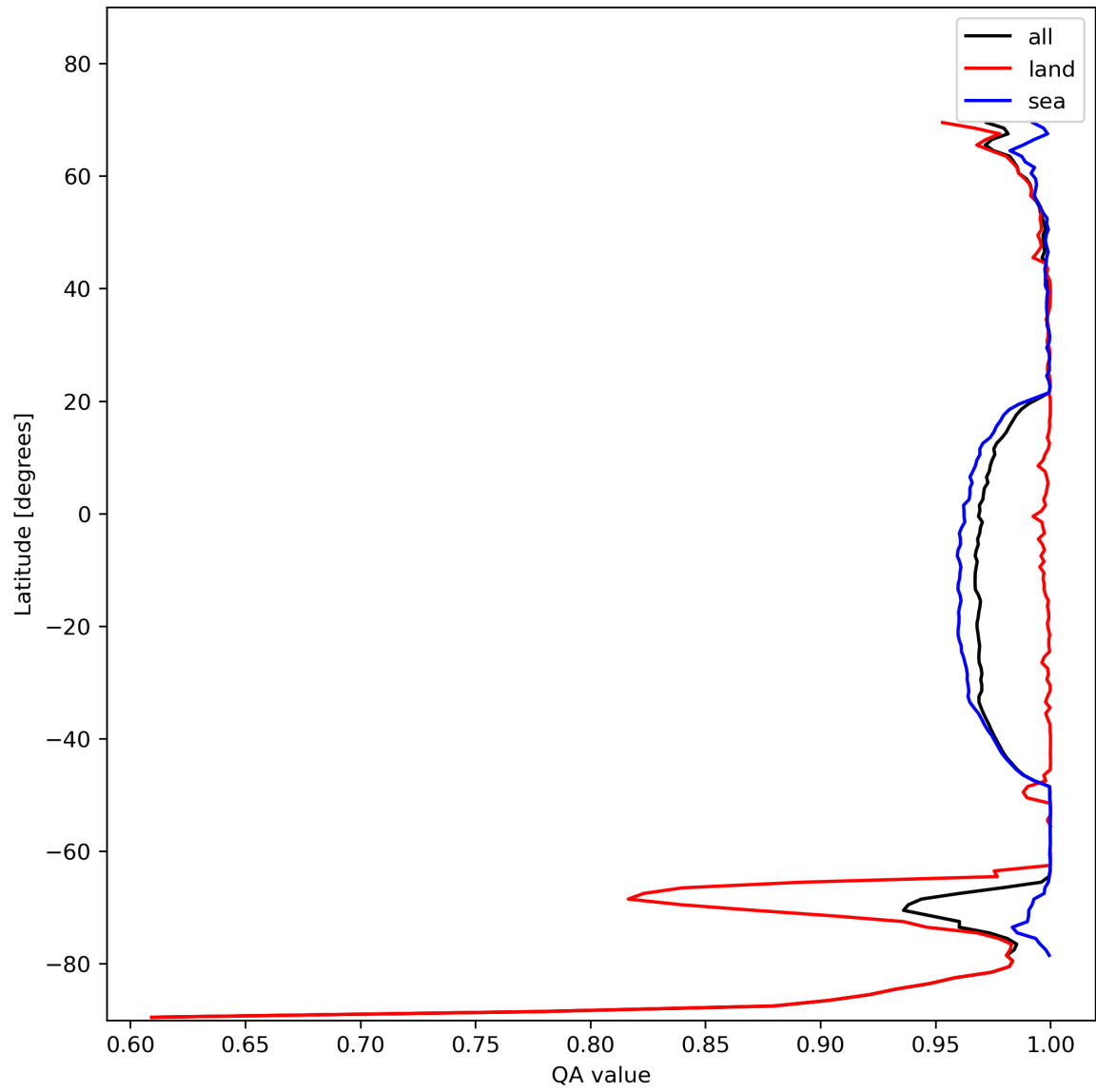
Figure 12: Zonal average of “QA value” for 2023-11-14 to 2023-11-16.
