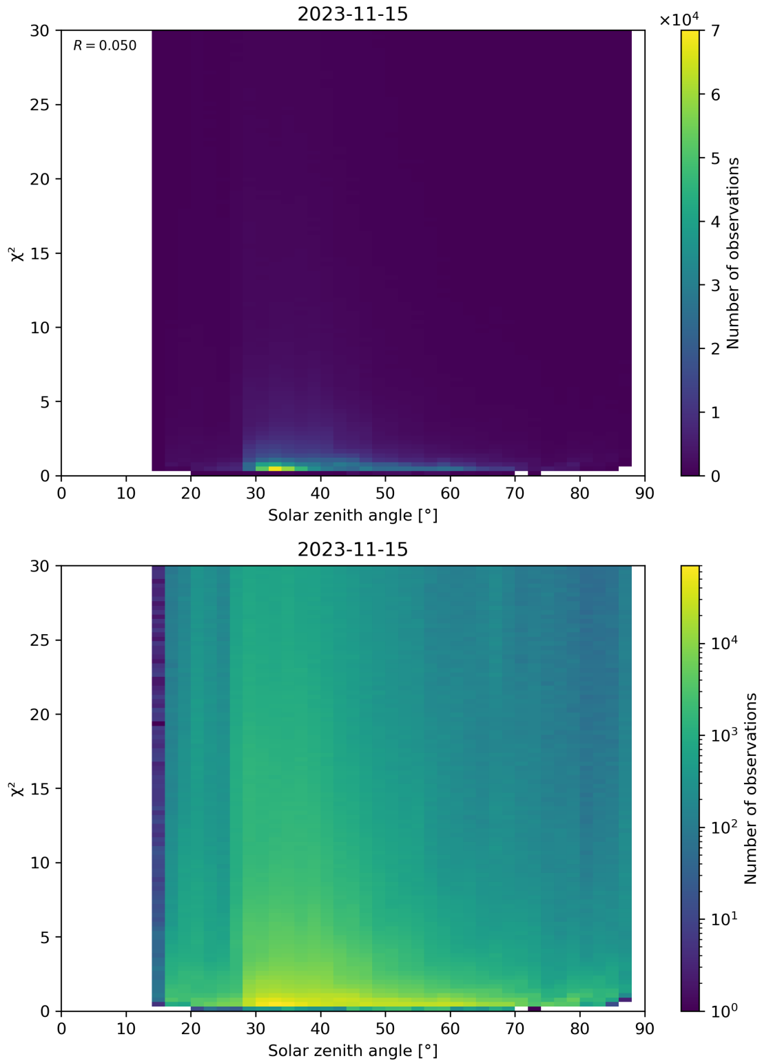
Figure 119: Scatter density plot of “Solar zenith angle” against “ \chi^2 ” for 2023-11-14 to 2023-11-16.
