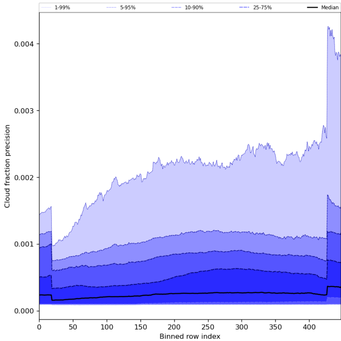
Figure 50: Along track statistics of “Cloud fraction precision” for 2023-11-14 to 2023-11-16
