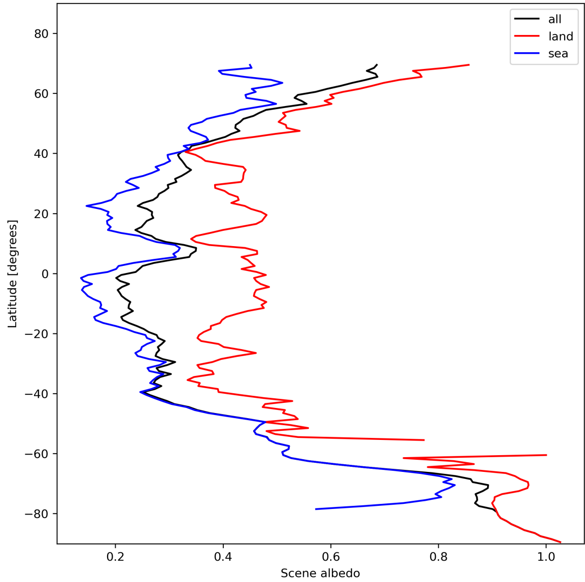
Figure 17: Zonal average of “Scene albedo” for 2023-11-14 to 2023-11-16.
