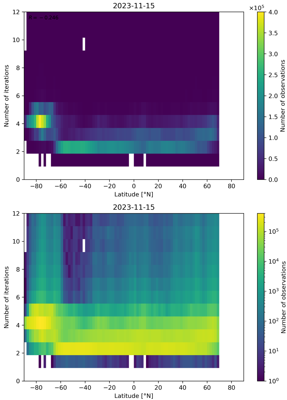
Figure 102: Scatter density plot of “Latitude” against “Number of iterations” for 2023-11-14 to 2023-11-16.
