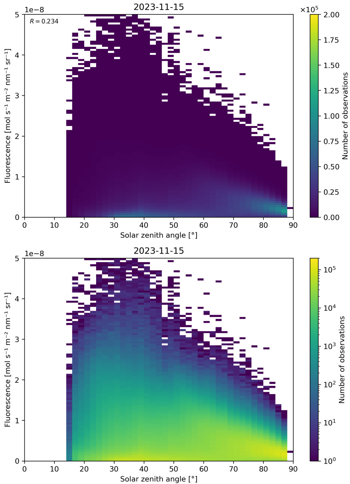
Figure 123: Scatter density plot of “Solar zenith angle” against “Fluorescence” for 2023-11-14 to 2023-11-16.
