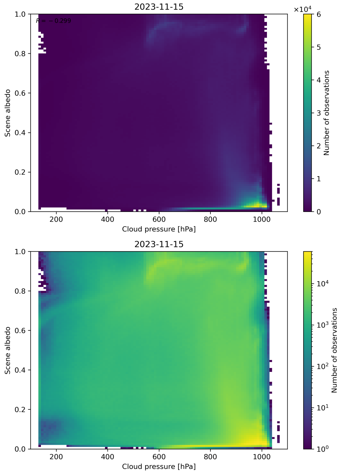
Figure 91: Scatter density plot of “Cloud pressure” against “Scene albedo” for 2023-11-14 to 2023-11-16.
