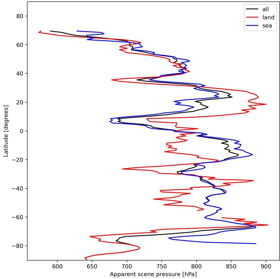
Figure 19: Zonal average of “Apparent scene pressure” for 2023-11-14 to 2023-11-16.
