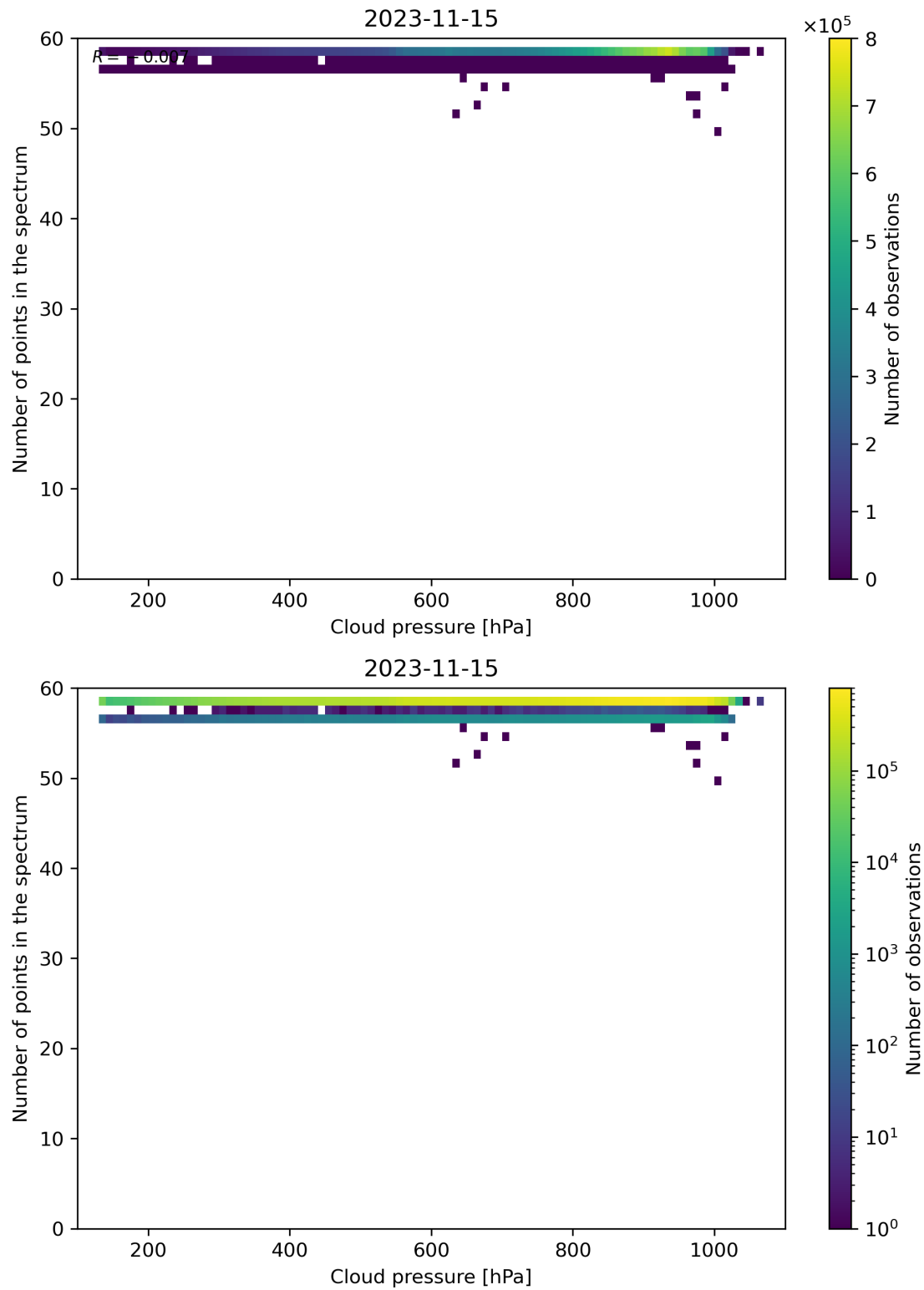
Figure 90: Scatter density plot of “Cloud pressure” against “Number of points in the spectrum” for 2023-11-14 to 2023-11-16.
