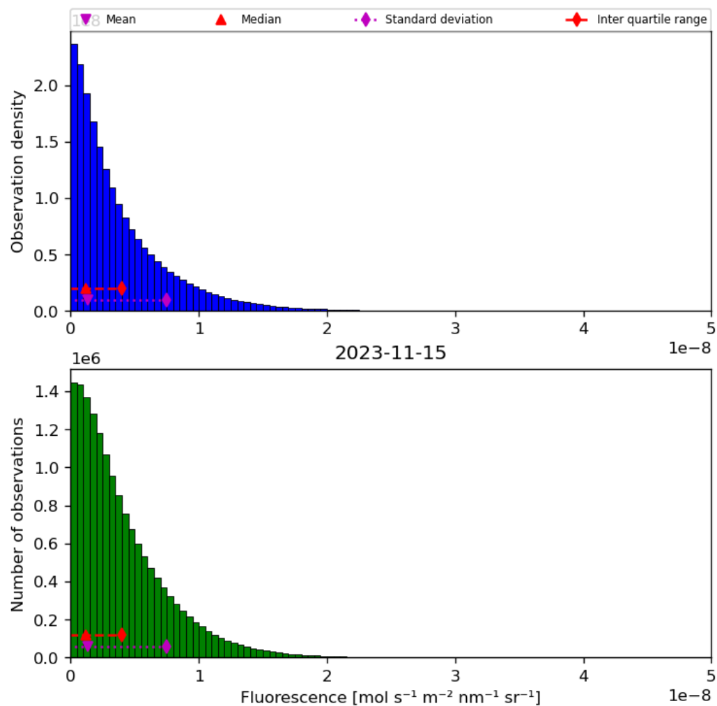
Figure 40: Histogram of “Fluorescence” for 2023-11-14 to 2023-11-16
