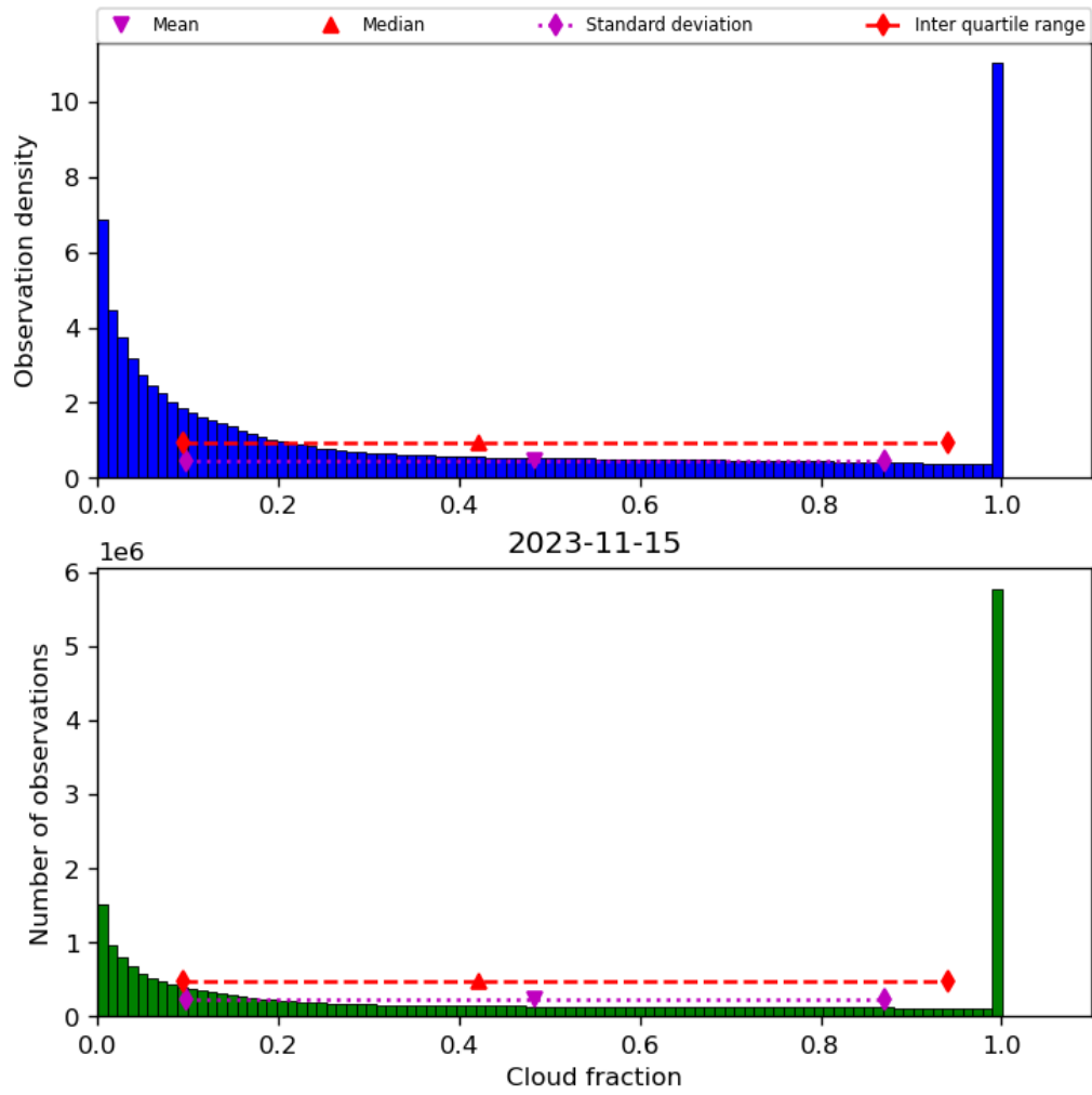
Figure 32: Histogram of “Cloud fraction” for 2023-11-14 to 2023-11-16
