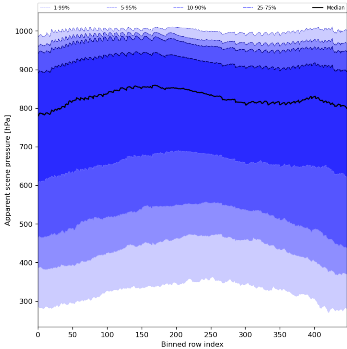
Figure 53: Along track statistics of “Apparent scene pressure” for 2023-11-14 to 2023-11-16
