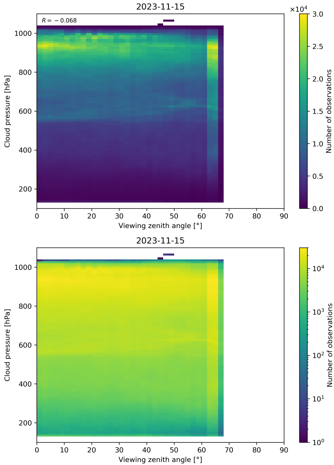
Figure 133: Scatter density plot of “Viewing zenith angle” against “Cloud pressure” for 2023-11-14 to 2023-11-16.
