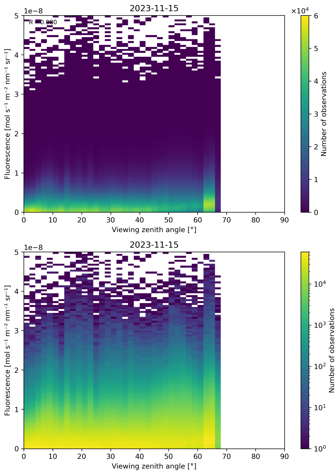
Figure 134: Scatter density plot of “Viewing zenith angle” against “Fluorescence” for 2023-11-14 to 2023-11-16.
