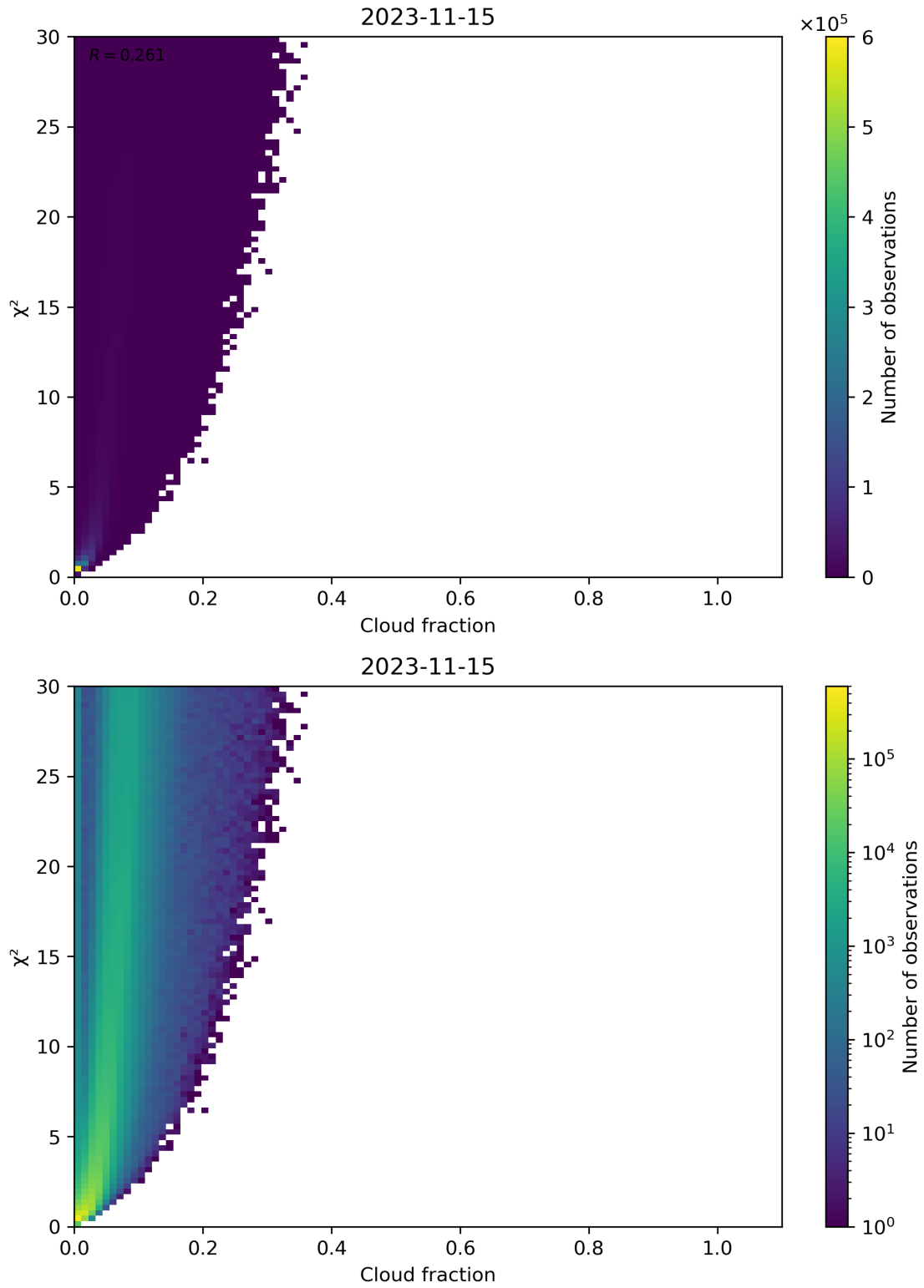
Figure 77: Scatter density plot of “Cloud fraction” against “ \chi^2 ” for 2023-11-14 to 2023-11-16.
