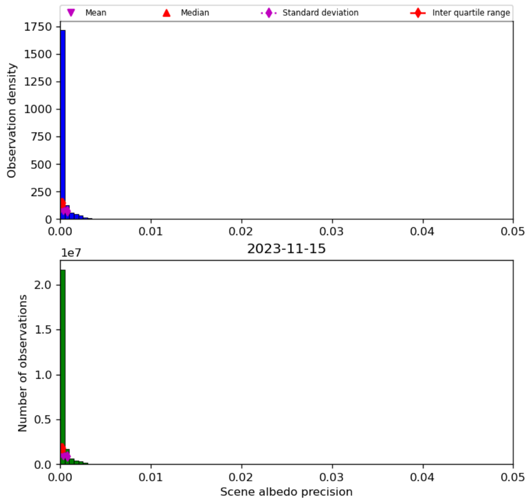
Figure 35: Histogram of “Scene albedo precision” for 2023-11-14 to 2023-11-16
