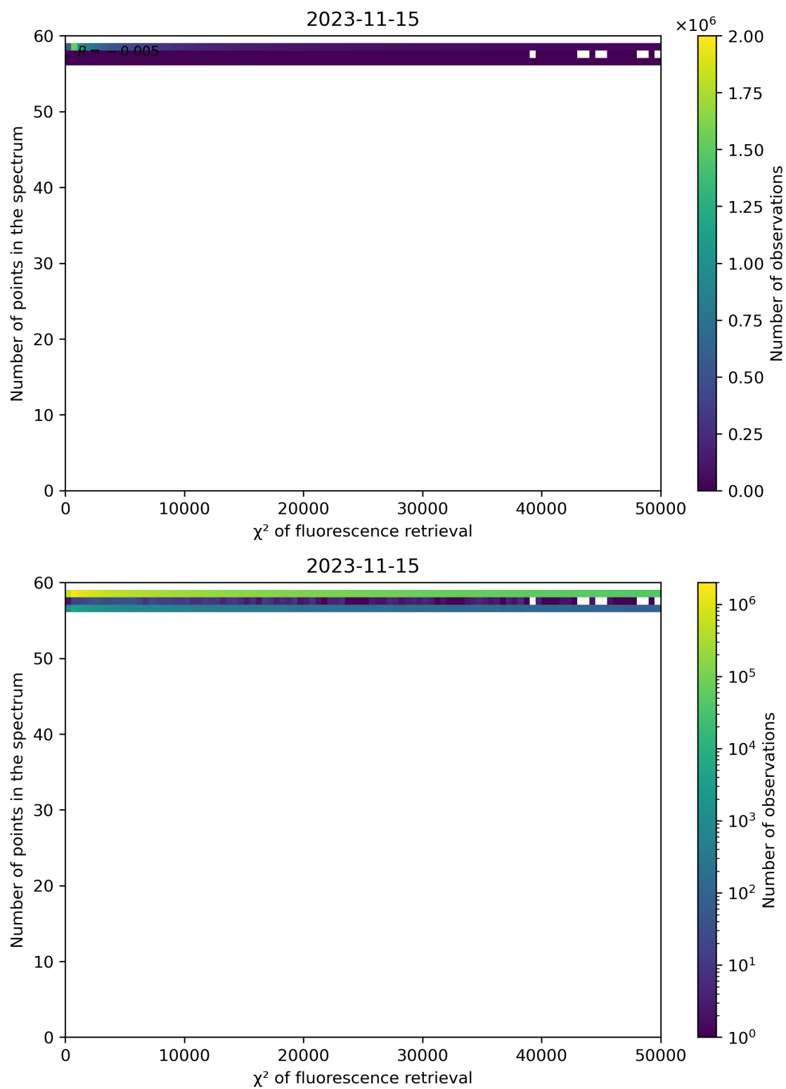
Figure 71: Scatter density plot of " \chi^2 of fluorescence retrieval" against "Number of points in the spectrum" for 2023-11-14 to 2023-11-16.
