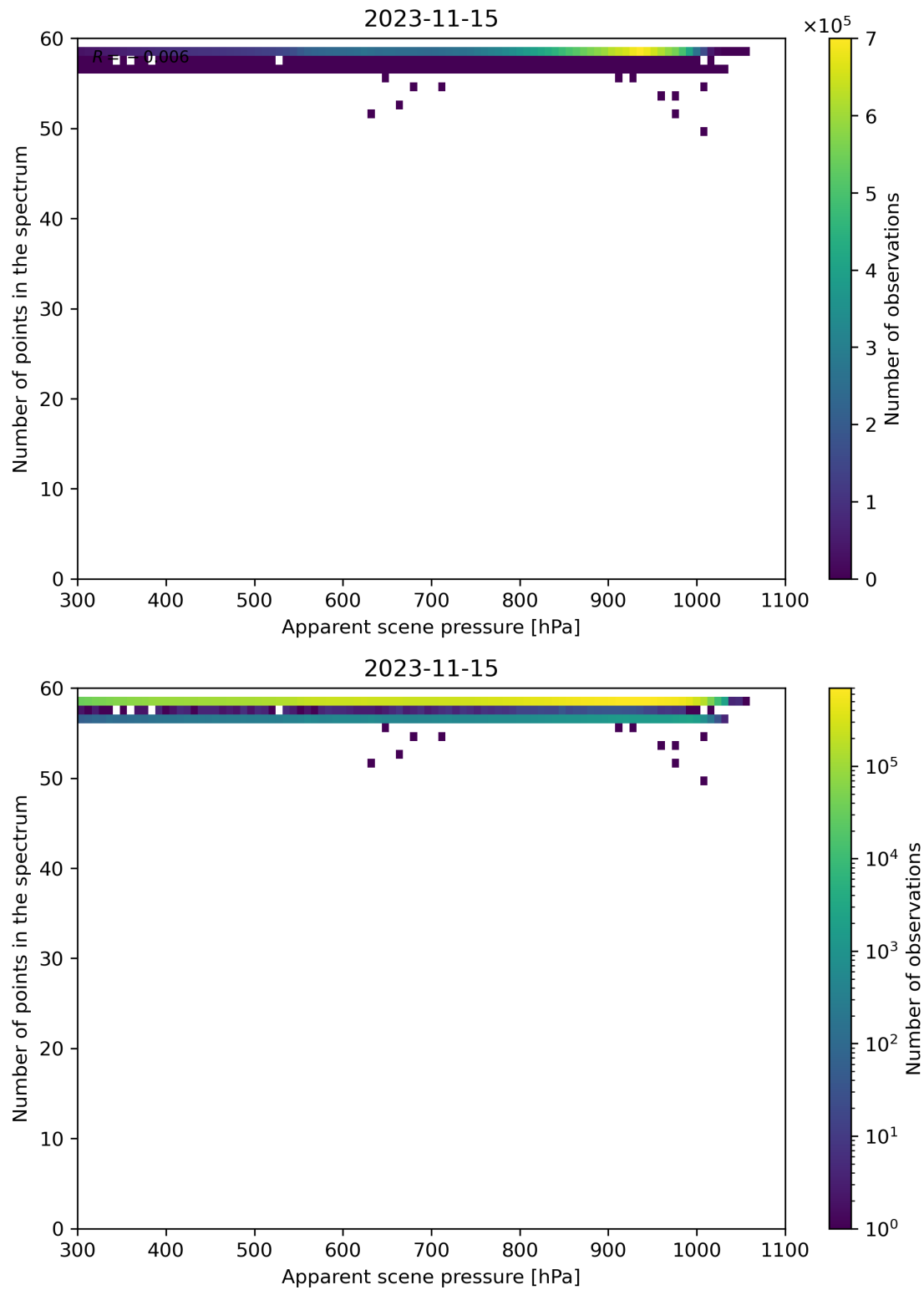
Figure 67: Scatter density plot of “Apparent scene pressure” against “Number of points in the spectrum” for 2023-11-14 to 2023-11-16.
