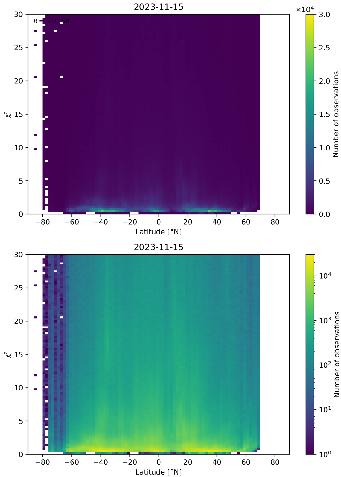
Figure 97: Scatter density plot of “Latitude” against “ \chi^2 ” for 2023-11-14 to 2023-11-16.
