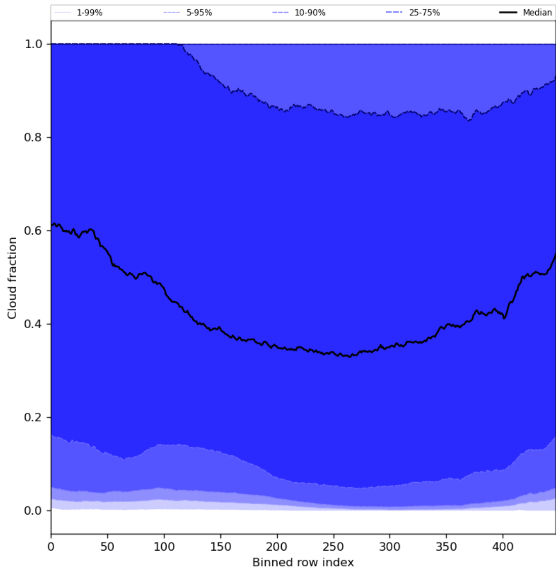
Figure 49: Along track statistics of “Cloud fraction” for 2023-11-14 to 2023-11-16
