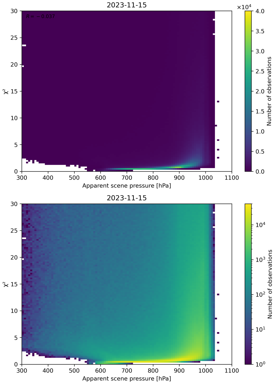
Figure 63: Scatter density plot of “Apparent scene pressure” against “ \chi^2 ” for 2023-11-14 to 2023-11-16.
