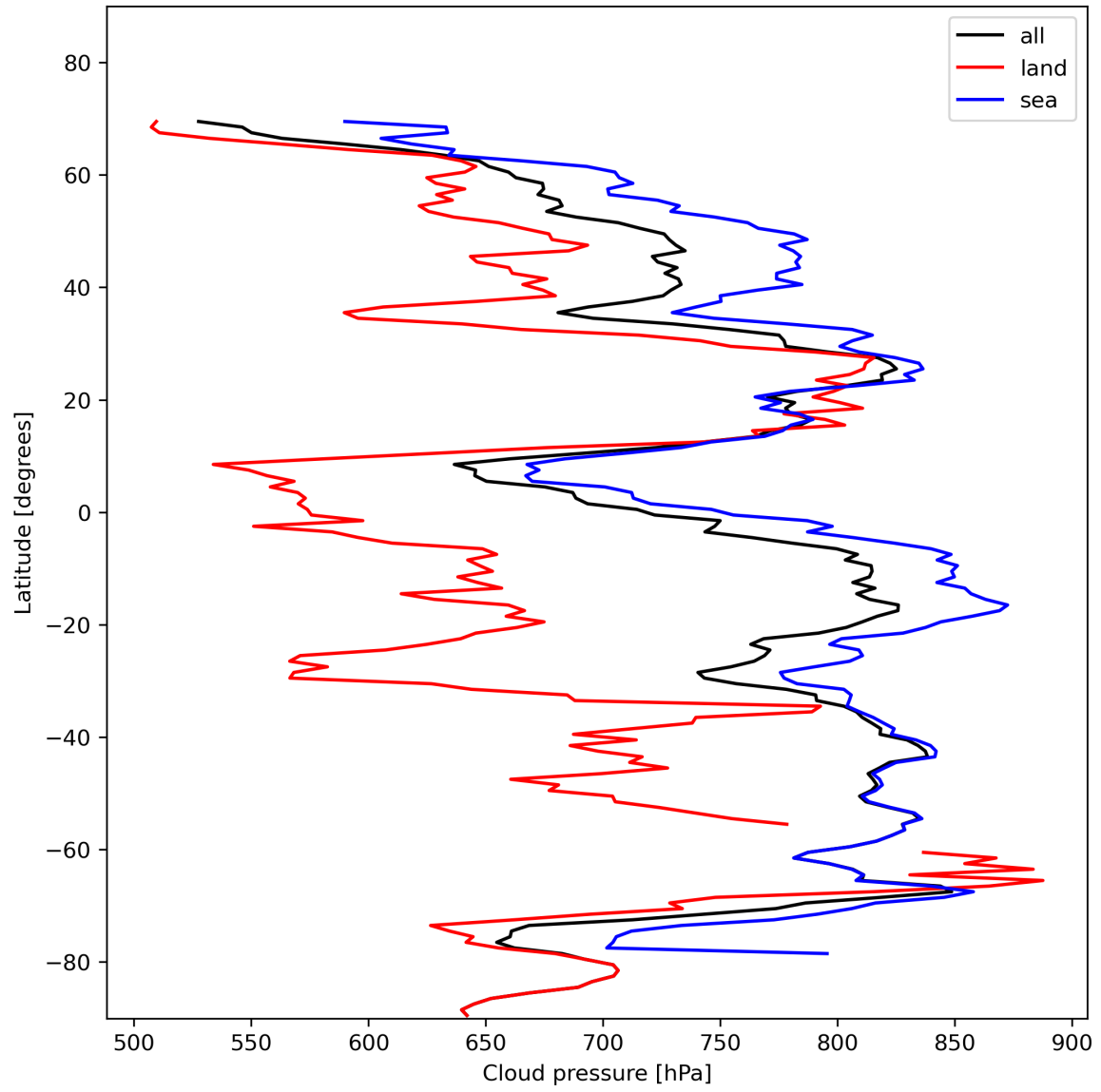
Figure 13: Zonal average of “Cloud pressure” for 2023-11-14 to 2023-11-16.
