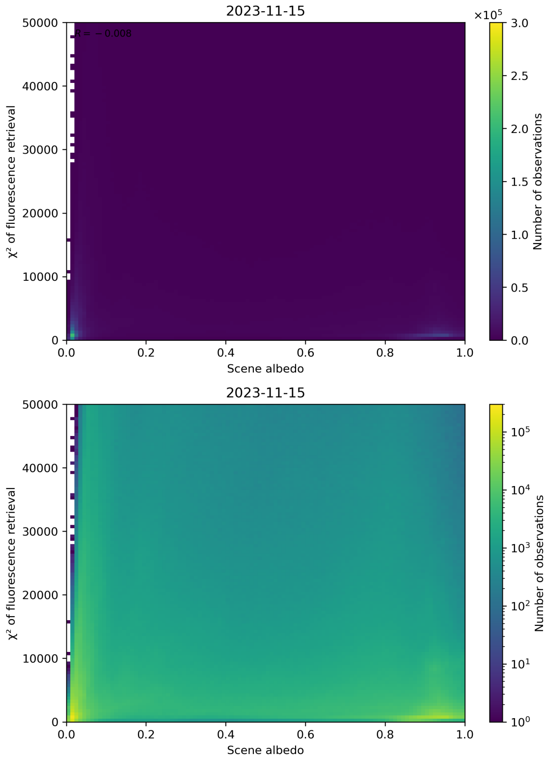
Figure 113: Scatter density plot of “Scene albedo” against “ \chi^2 of fluorescence retrieval” for 2023-11-14 to 2023-11-16.
