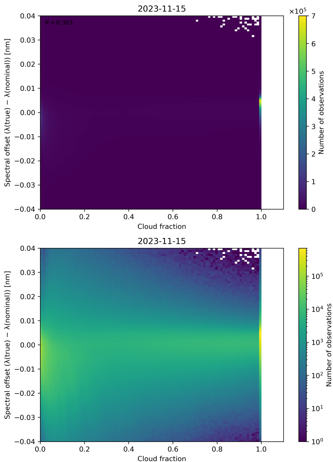
Figure 83: Scatter density plot of “Cloud fraction” against “Spectral offset ( \lambda(\text{true}) - \lambda(\text{nominal}) )” for 2023-11-14 to 2023-11-16.
