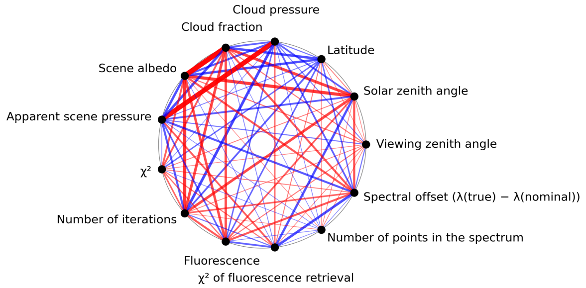
Figure 1: Map of correlation graph for 2023-11-14 to 2023-11-16.
