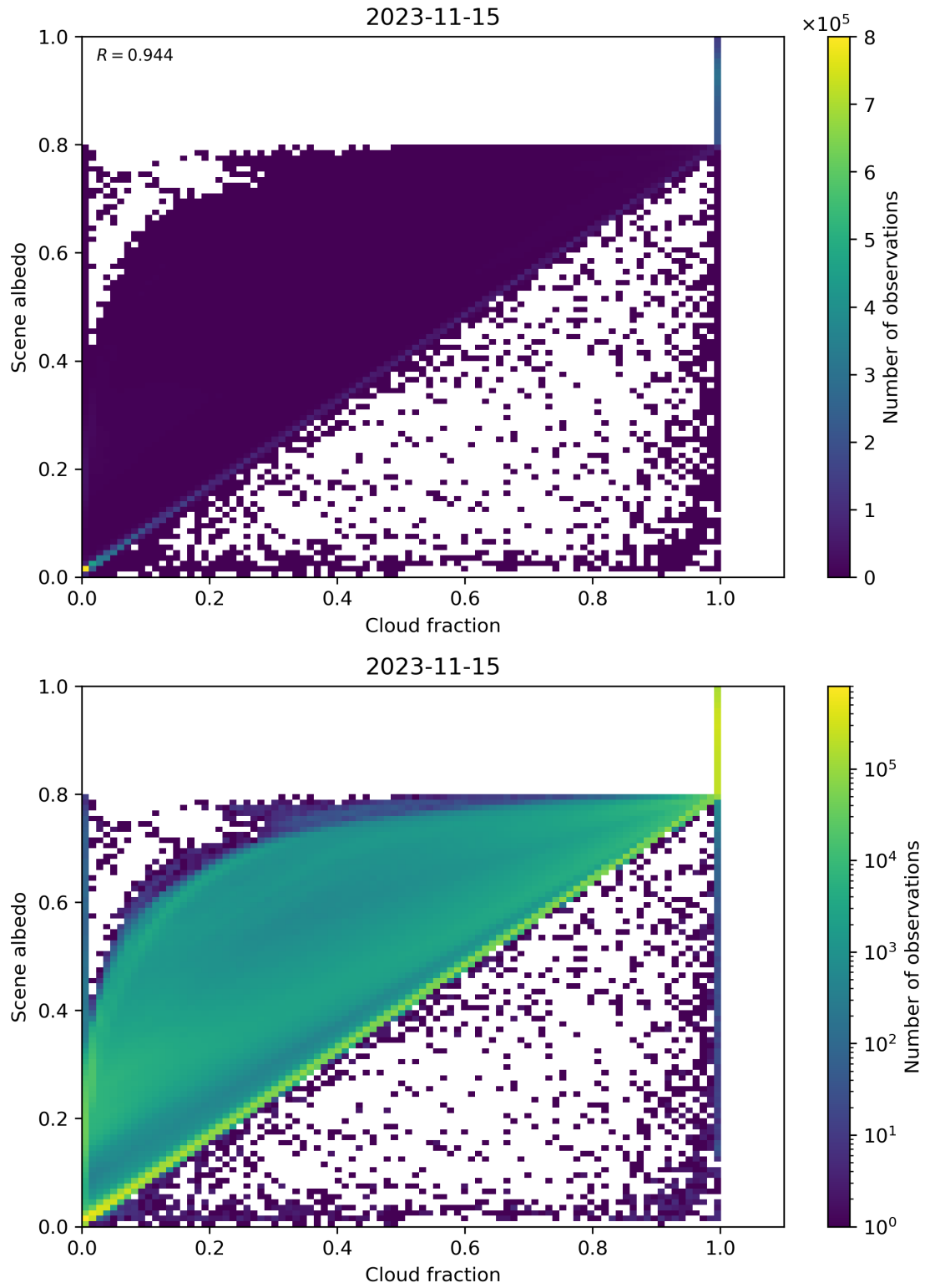
Figure 82: Scatter density plot of “Cloud fraction” against “Scene albedo” for 2023-11-14 to 2023-11-16.
