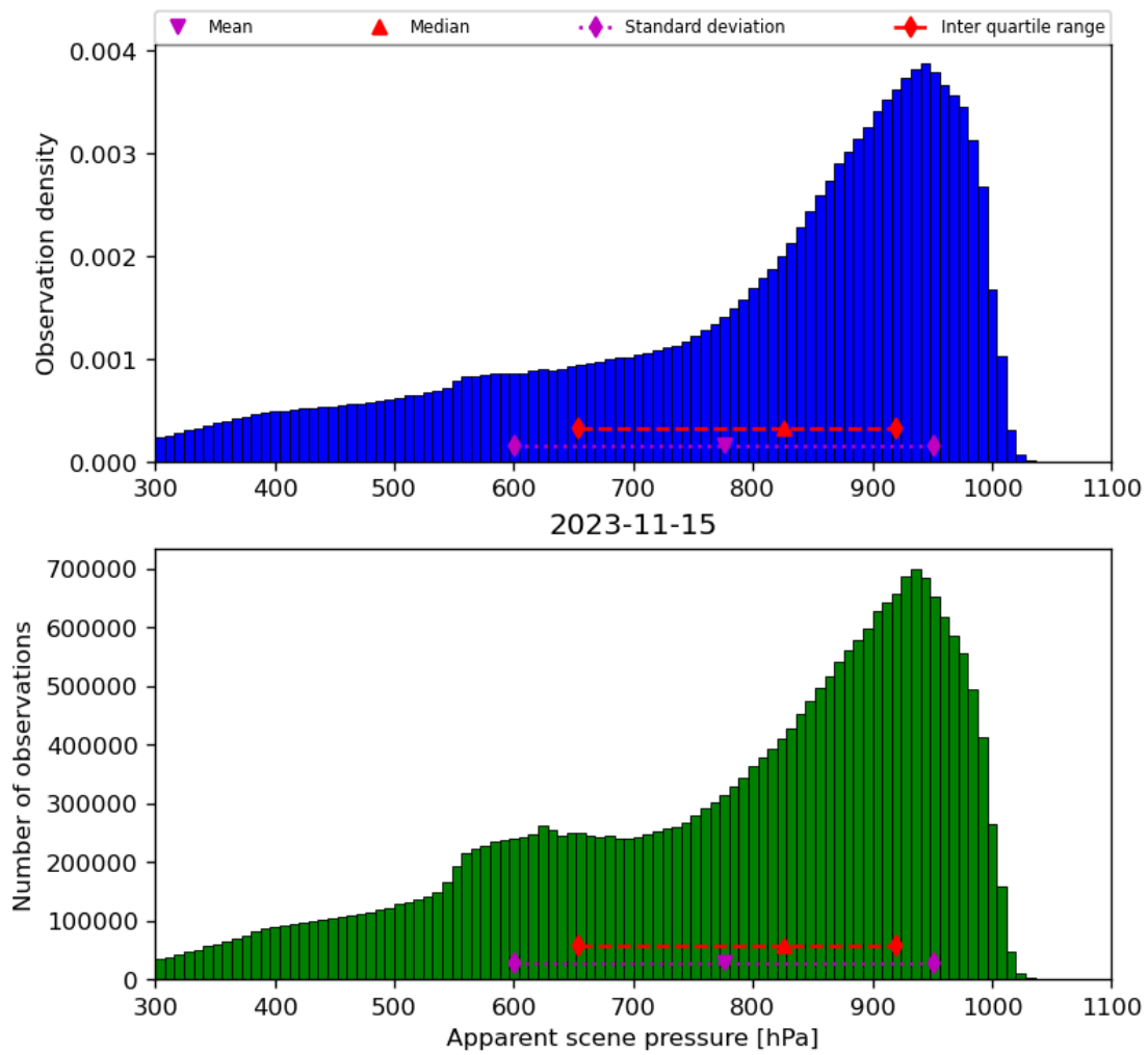
Figure 36: Histogram of “Apparent scene pressure” for 2023-11-14 to 2023-11-16
