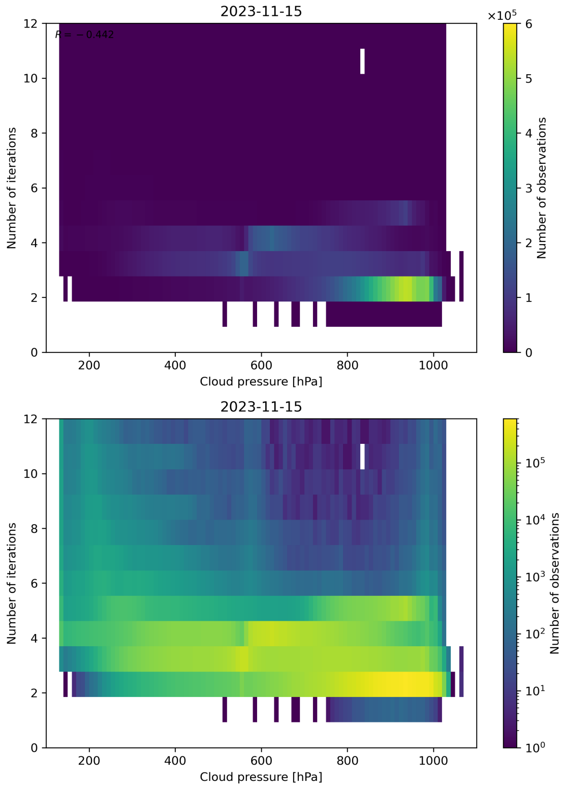
Figure 89: Scatter density plot of “Cloud pressure” against “Number of iterations” for 2023-11-14 to 2023-11-16.
