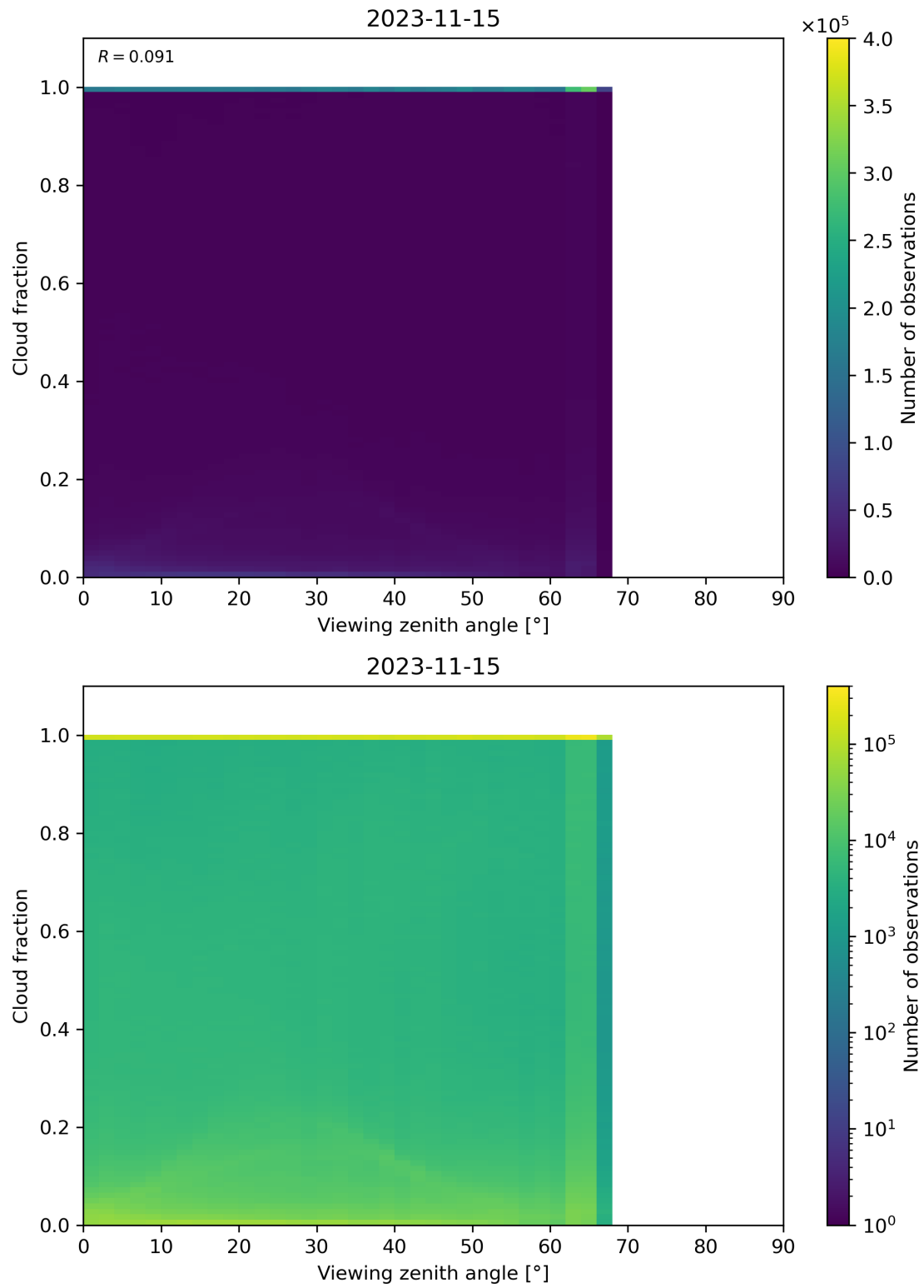
Figure 132: Scatter density plot of “Viewing zenith angle” against “Cloud fraction” for 2023-11-14 to 2023-11-16.
