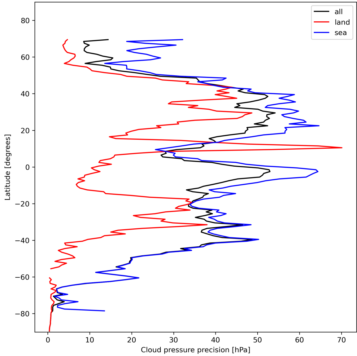
Figure 14: Zonal average of “Cloud pressure precision” for 2023-11-14 to 2023-11-16.
