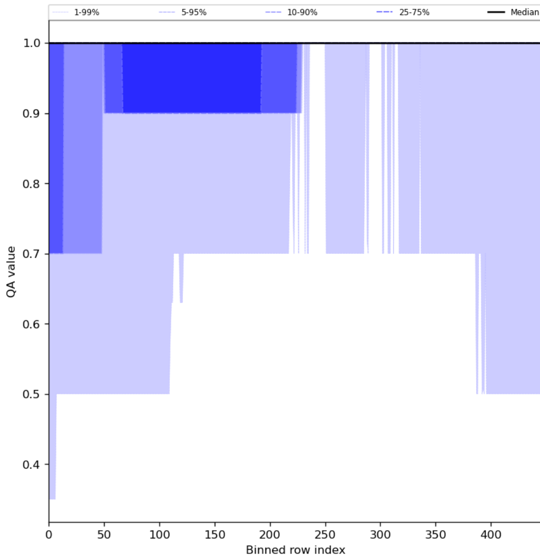
Figure 46: Along track statistics of “QA value” for 2023-11-14 to 2023-11-16
