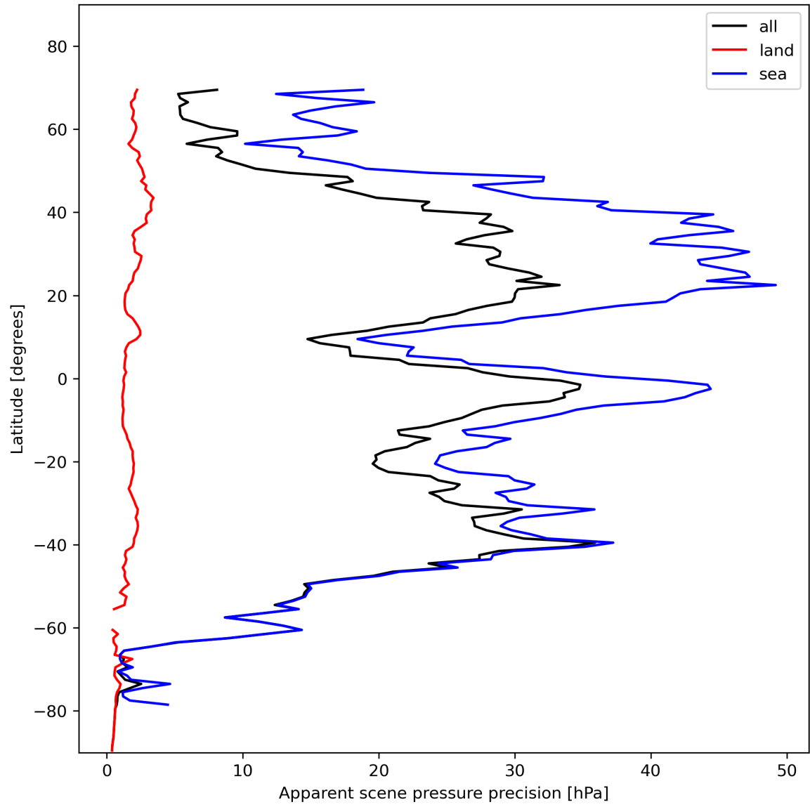
Figure 20: Zonal average of “Apparent scene pressure precision” for 2023-11-14 to 2023-11-16.
