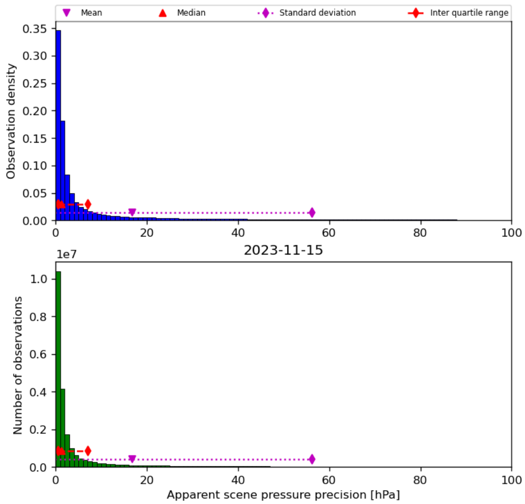
Figure 37: Histogram of “Apparent scene pressure precision” for 2023-11-14 to 2023-11-16
