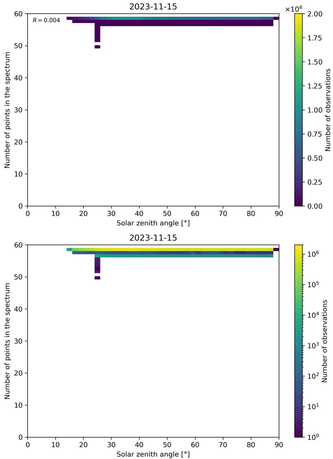
Figure 126: Scatter density plot of “Solar zenith angle” against “Number of points in the spectrum” for 2023-11-14 to 2023-11-16.
