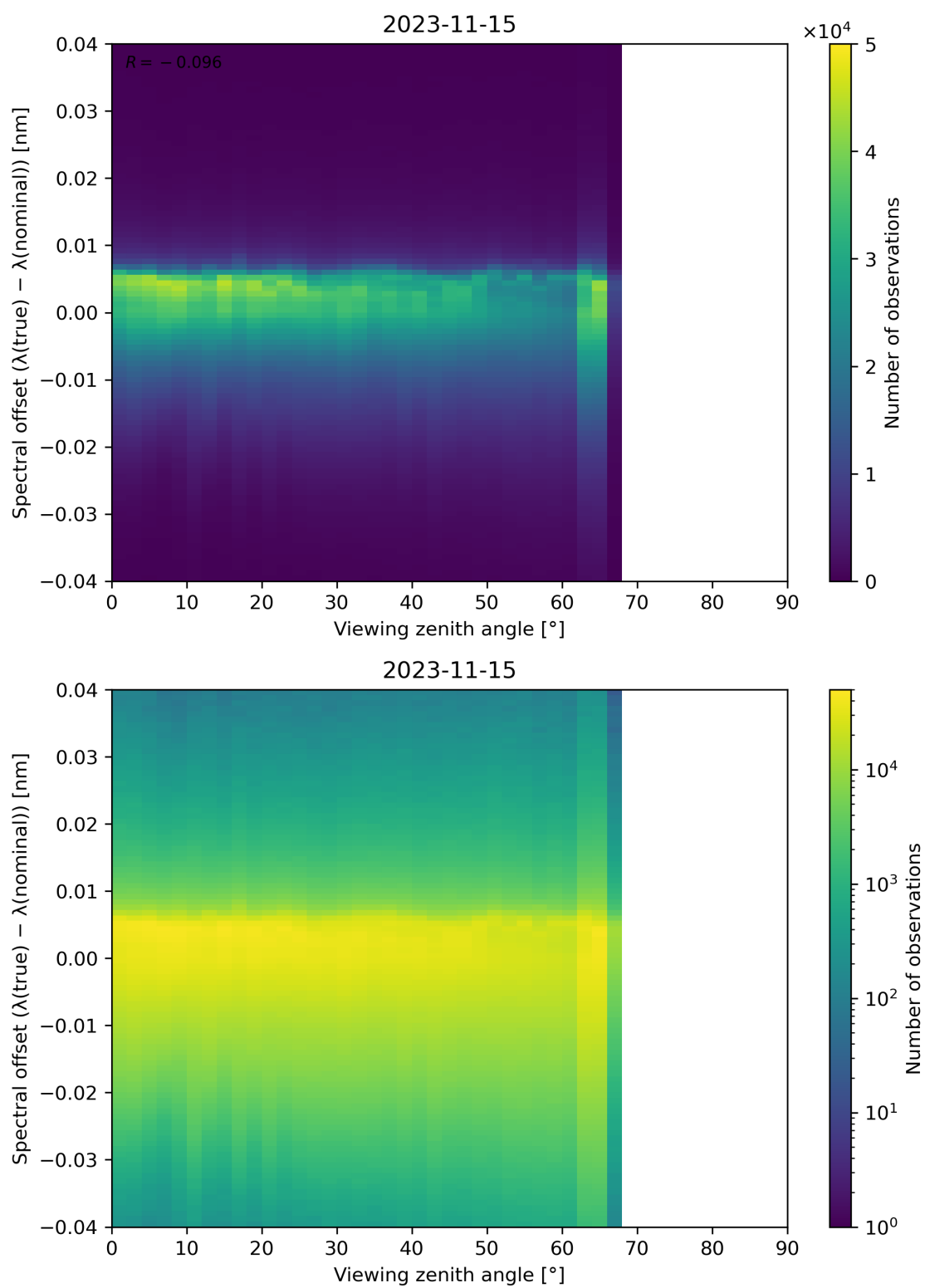
Figure 140: Scatter density plot of “Viewing zenith angle” against “Spectral offset ( \lambda(\text{true}) - \lambda(\text{nominal}) )” for 2023-11-14 to 2023-11-16.
