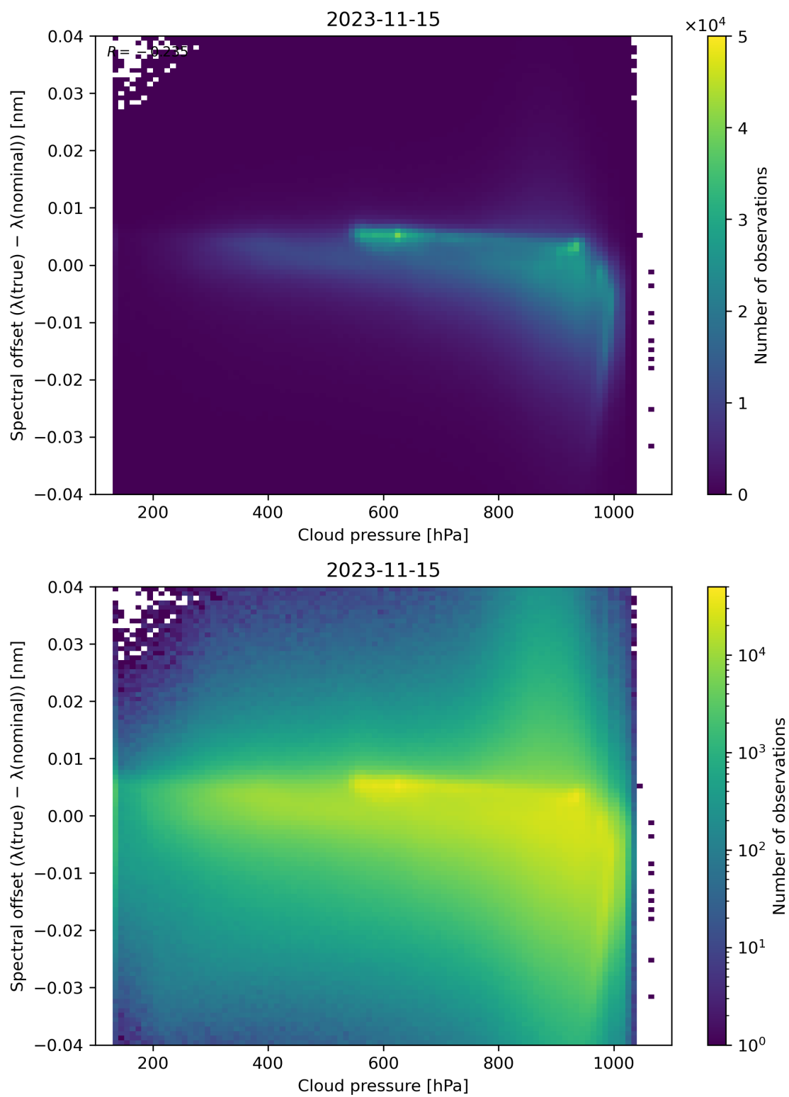
Figure 92: Scatter density plot of “Cloud pressure” against “Spectral offset ( \lambda(\text{true}) - \lambda(\text{nominal}) )” for 2023-11-14 to 2023-11-16.
