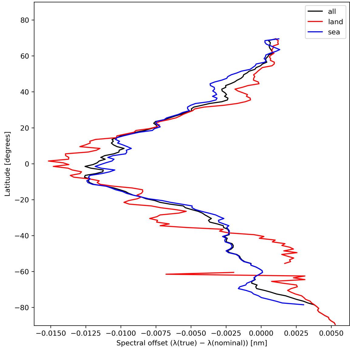
Figure 28: Zonal average of “Spectral offset ( \lambda(\text{true}) - \lambda(\text{nominal}) )” for 2023-11-14 to 2023-11-16.
