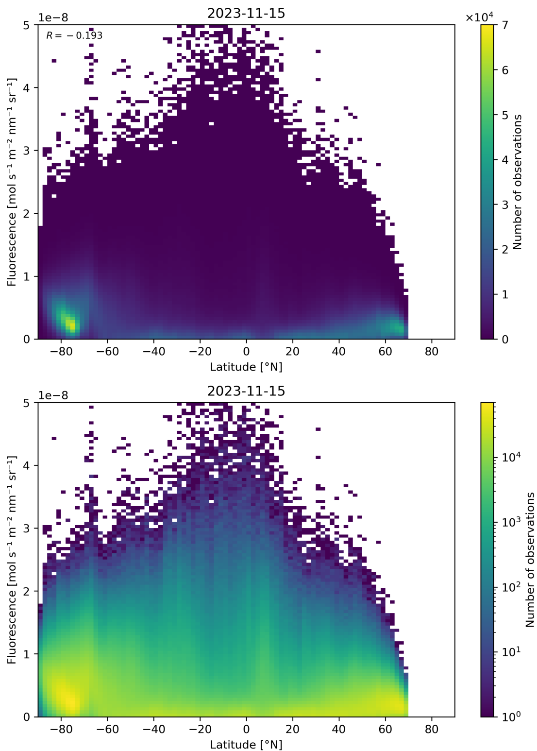
Figure 101: Scatter density plot of “Latitude” against “Fluorescence” for 2023-11-14 to 2023-11-16.
