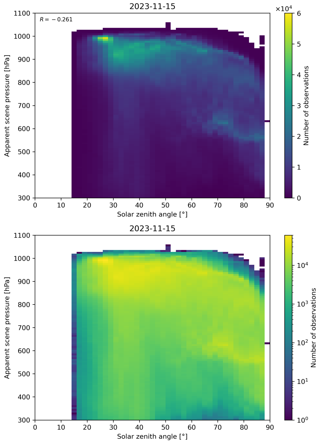
Figure 118: Scatter density plot of “Solar zenith angle” against “Apparent scene pressure” for 2023-11-14 to 2023-11-16.
