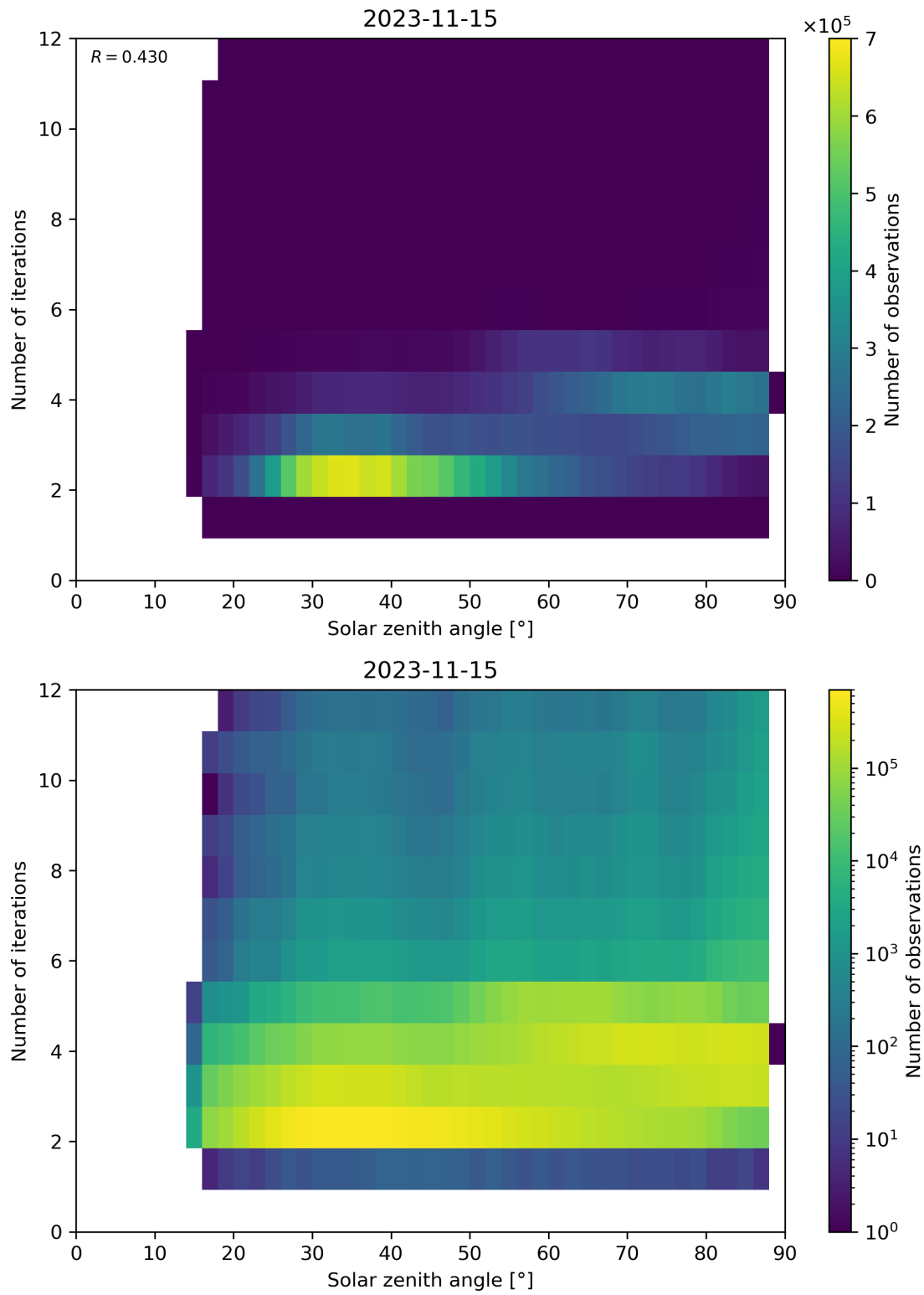
Figure 125: Scatter density plot of “Solar zenith angle” against “Number of iterations” for 2023-11-14 to 2023-11-16.
