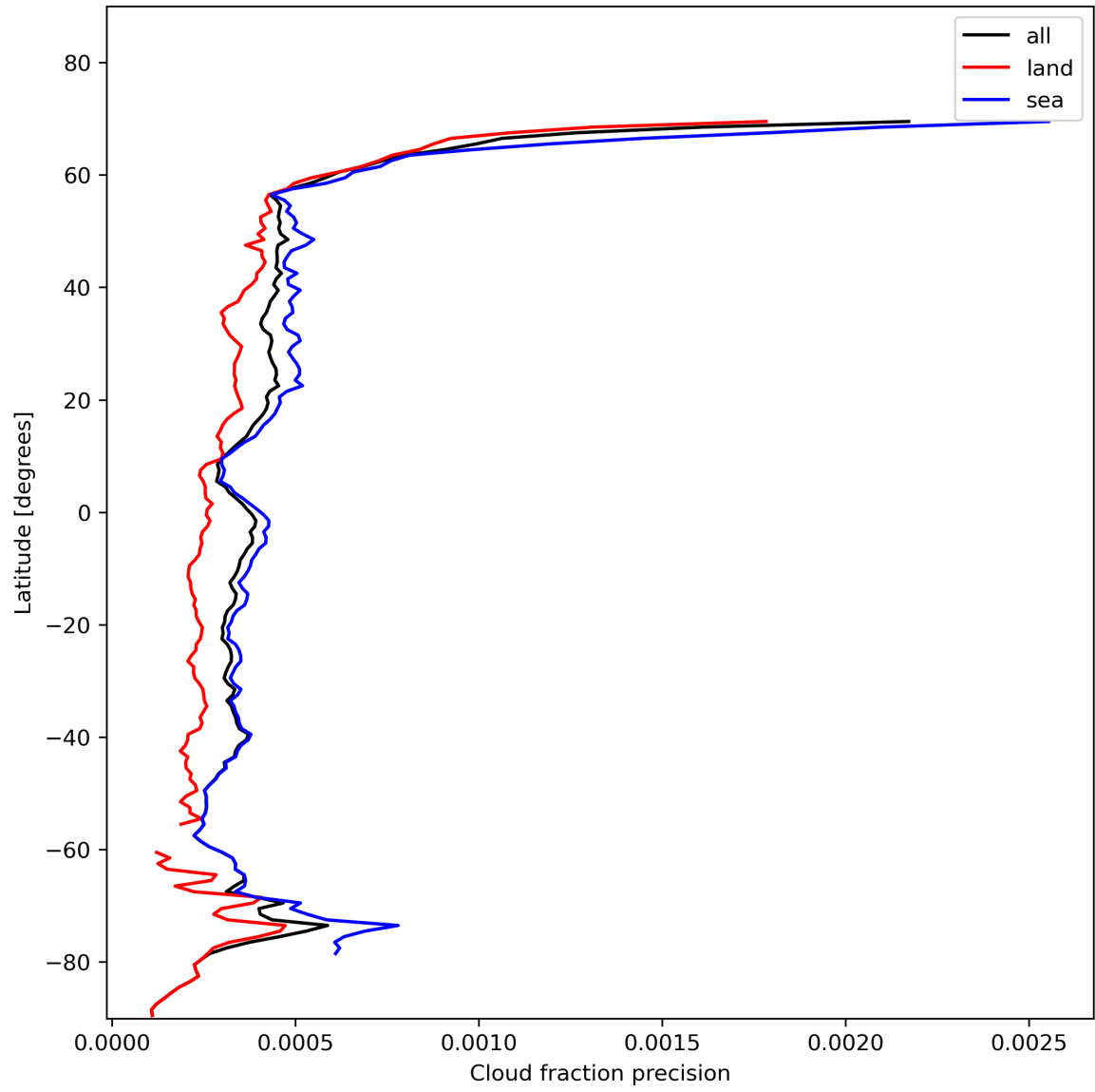
Figure 16: Zonal average of “Cloud fraction precision” for 2023-11-14 to 2023-11-16.
