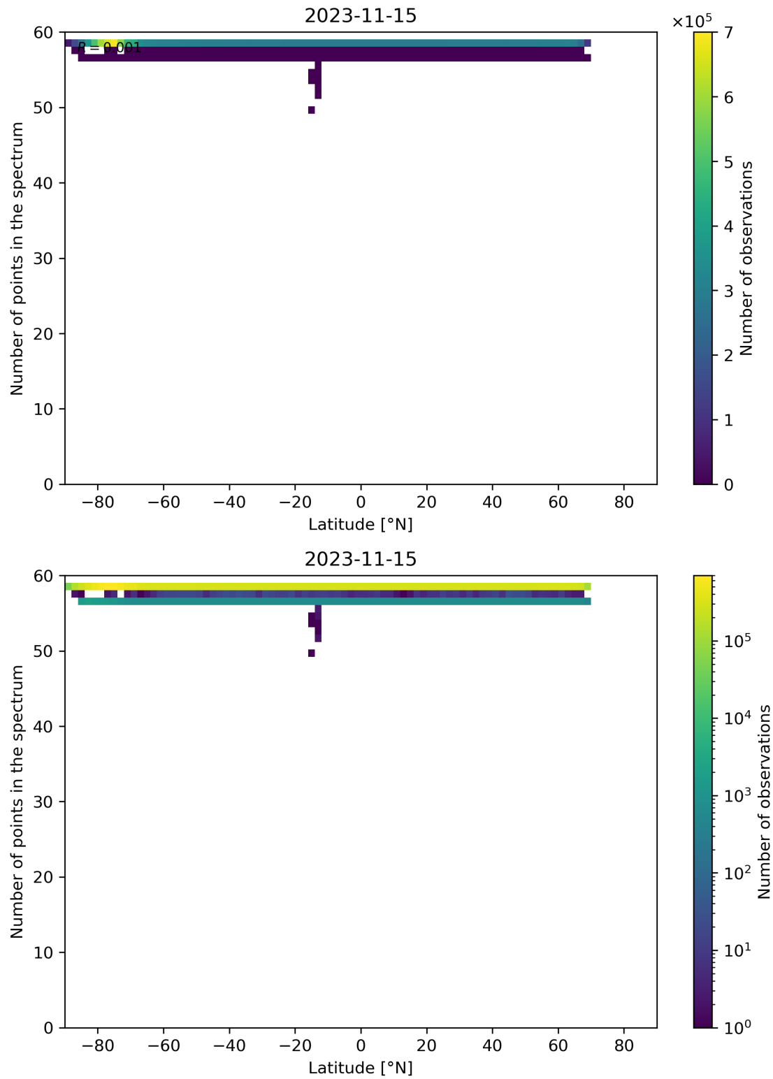
Figure 103: Scatter density plot of “Latitude” against “Number of points in the spectrum” for 2023-11-14 to 2023-11-16.
