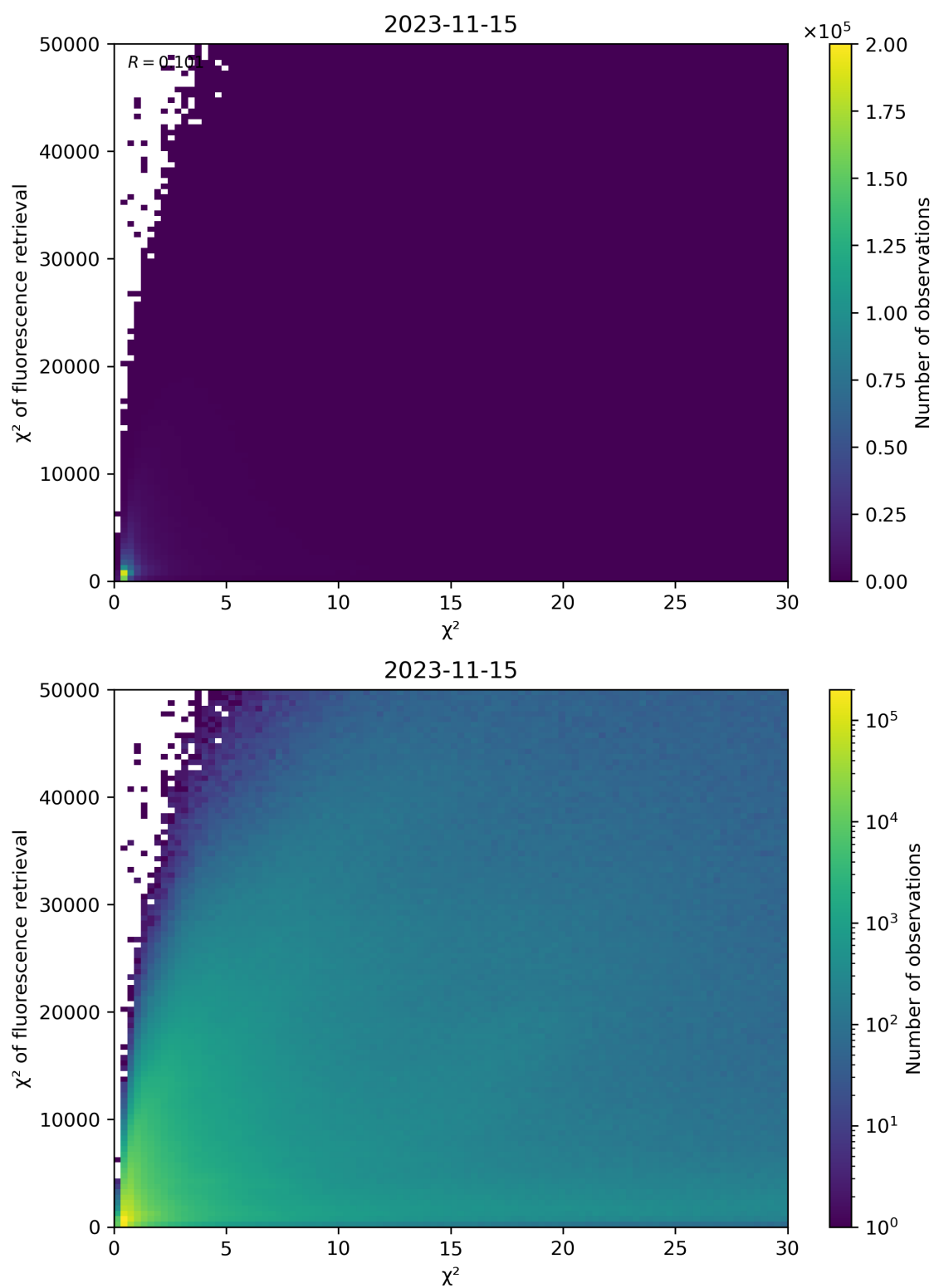
Figure 69: Scatter density plot of “ \chi^2 ” against “ \chi^2 of fluorescence retrieval” for 2023-11-14 to 2023-11-16.
