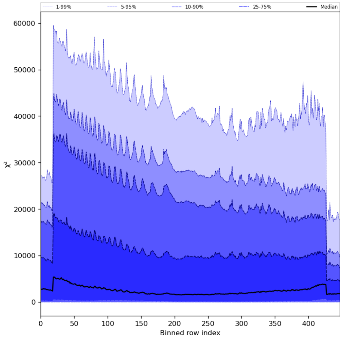
Figure 55: Along track statistics of “ \chi^2 ” for 2023-11-14 to 2023-11-16
