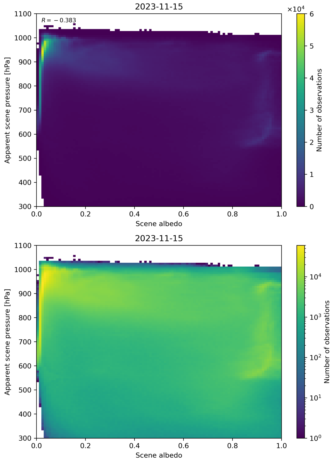
Figure 111: Scatter density plot of “Scene albedo” against “Apparent scene pressure” for 2023-11-14 to 2023-11-16.
