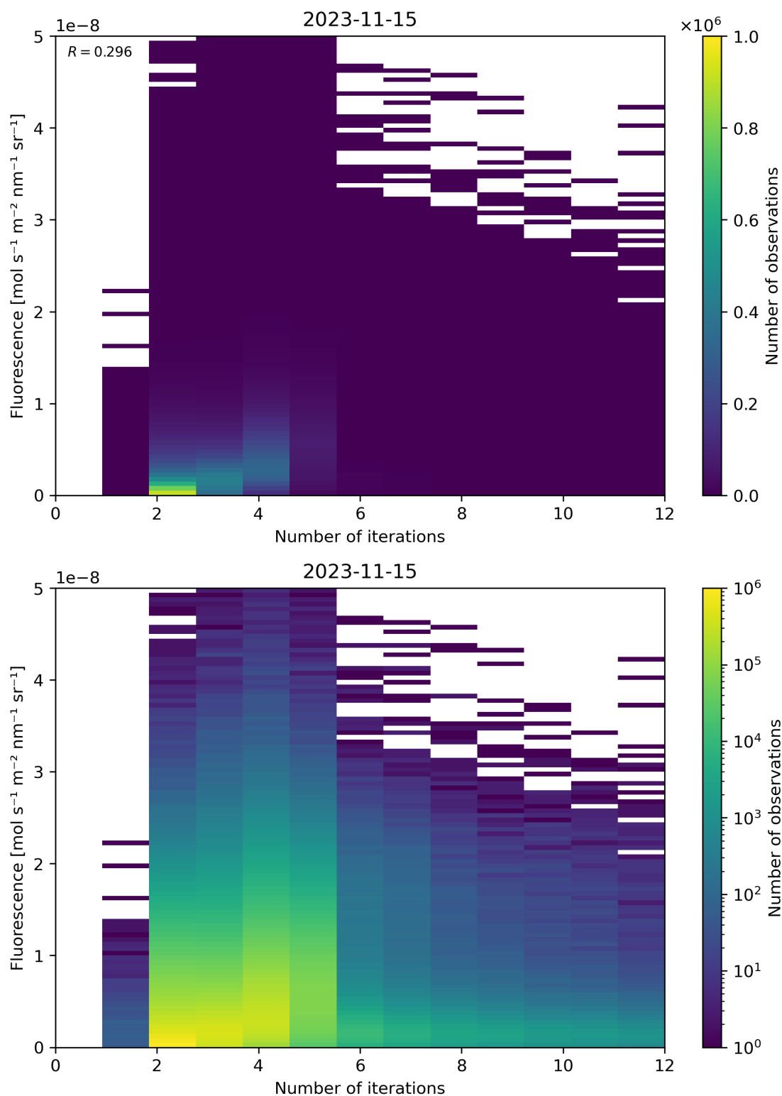
Figure 107: Scatter density plot of “Number of iterations” against “Fluorescence” for 2023-11-14 to 2023-11-16.
