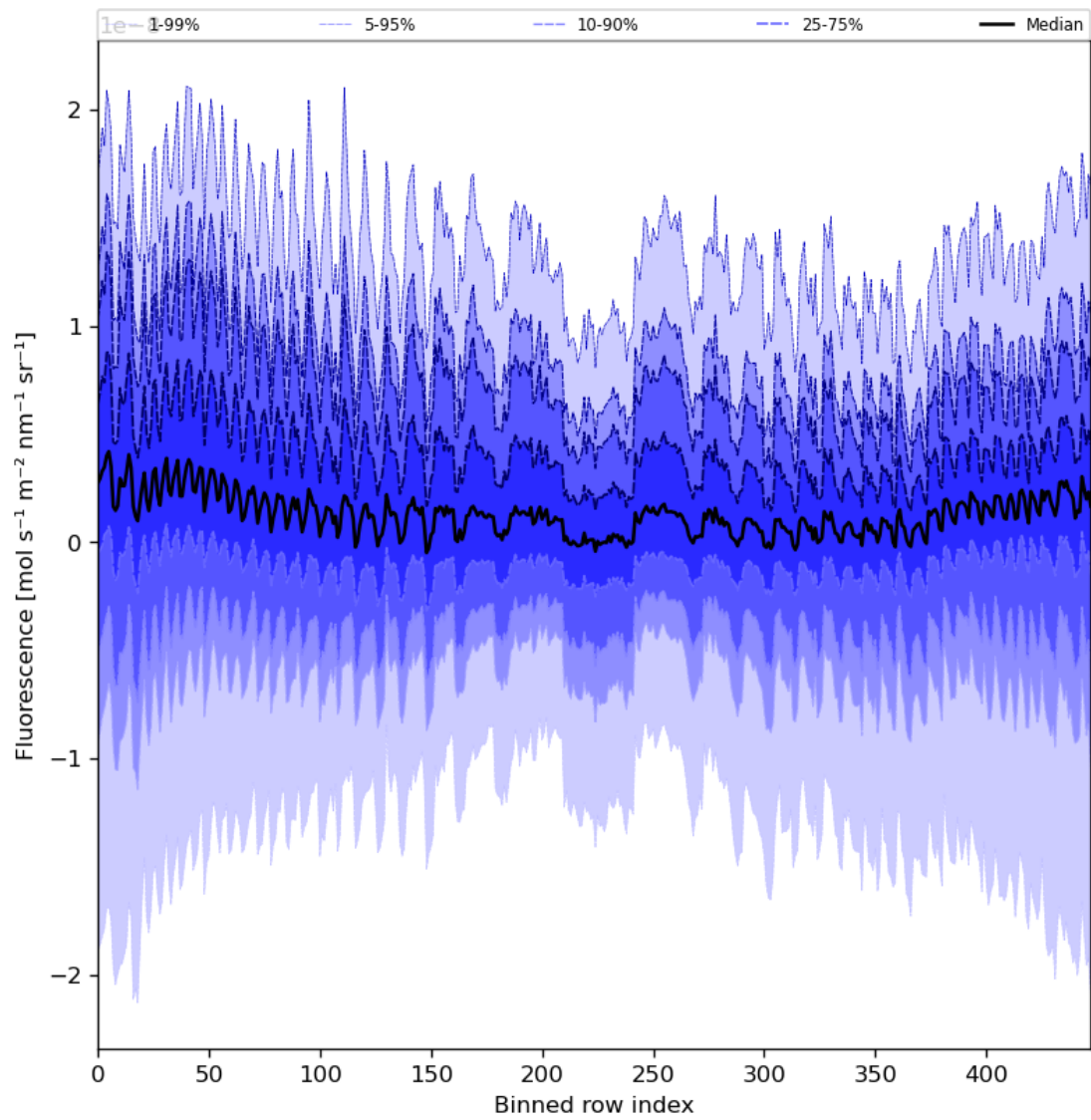
Figure 57: Along track statistics of “Fluorescence” for 2023-11-14 to 2023-11-16
