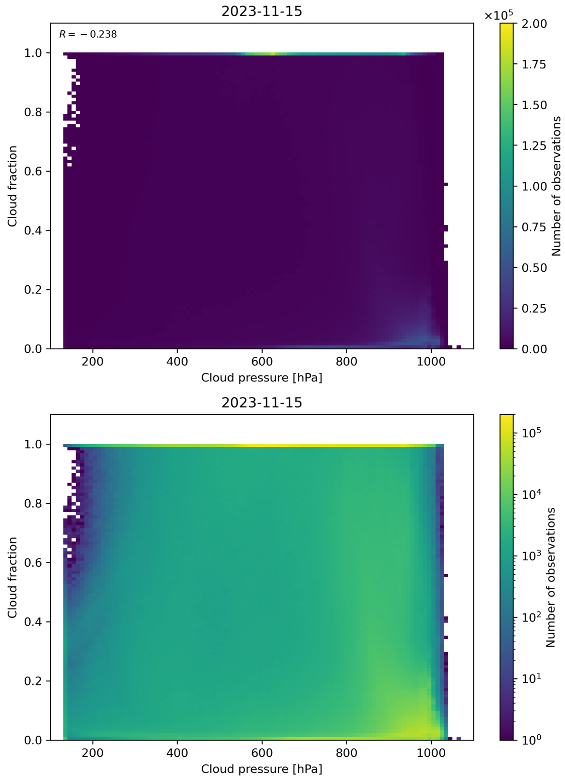
Figure 87: Scatter density plot of “Cloud pressure” against “Cloud fraction” for 2023-11-14 to 2023-11-16.
