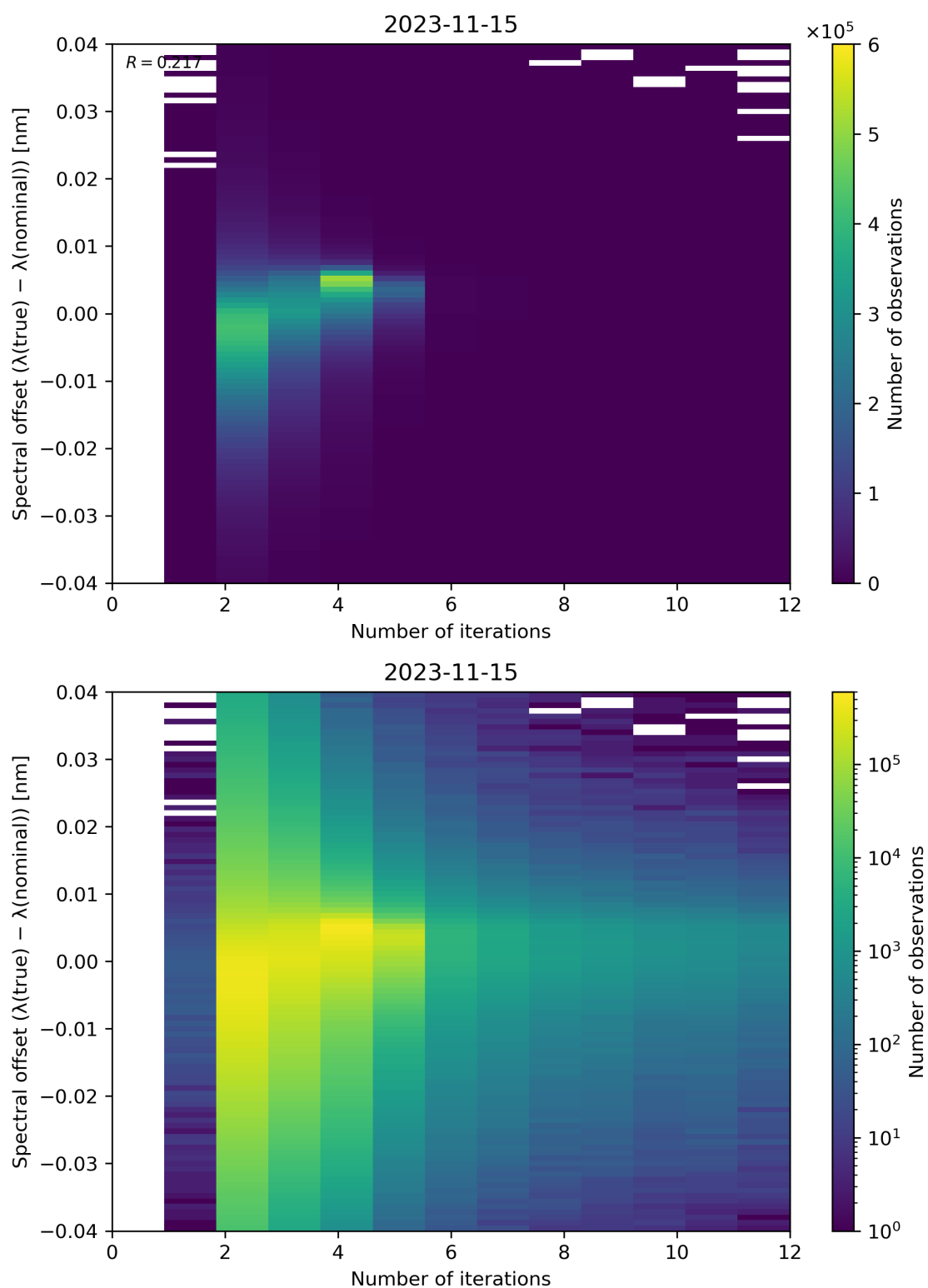
Figure 109: Scatter density plot of “Number of iterations” against “Spectral offset ( \lambda(\text{true}) - \lambda(\text{nominal}) )” for 2023-11-14 to 2023-11-16.
