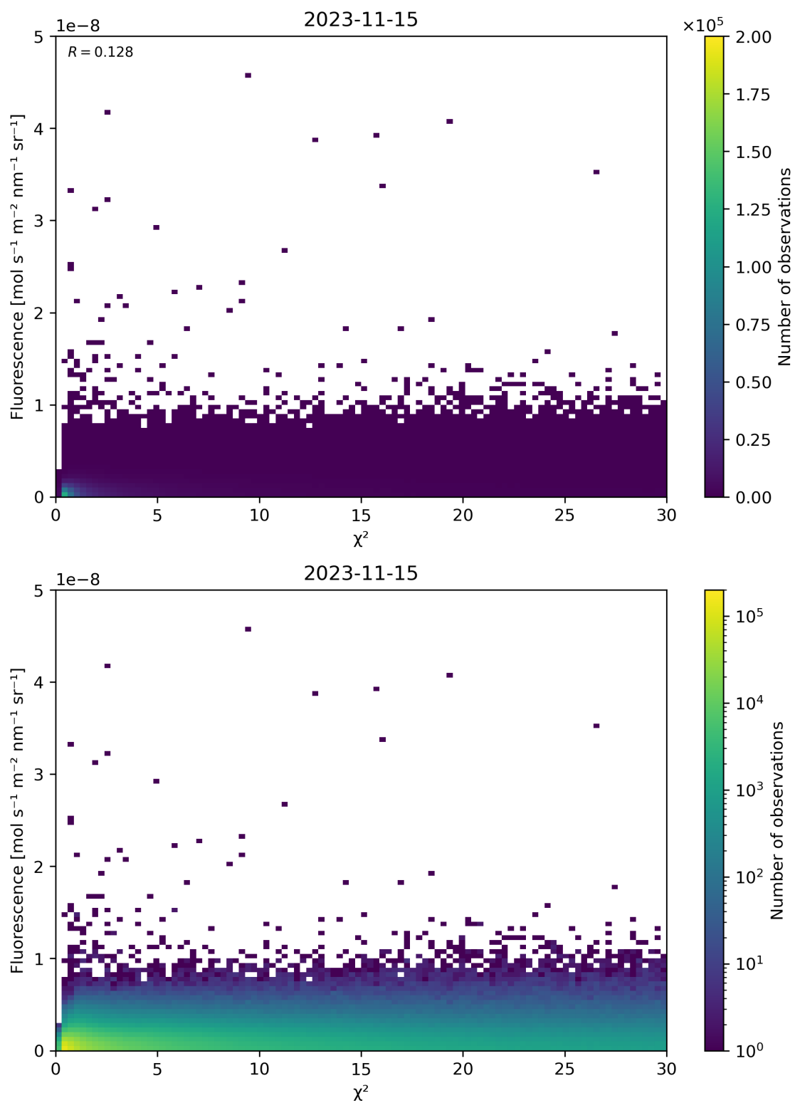
Figure 70: Scatter density plot of “ \chi^2 ” against “Fluorescence” for 2023-11-14 to 2023-11-16.
