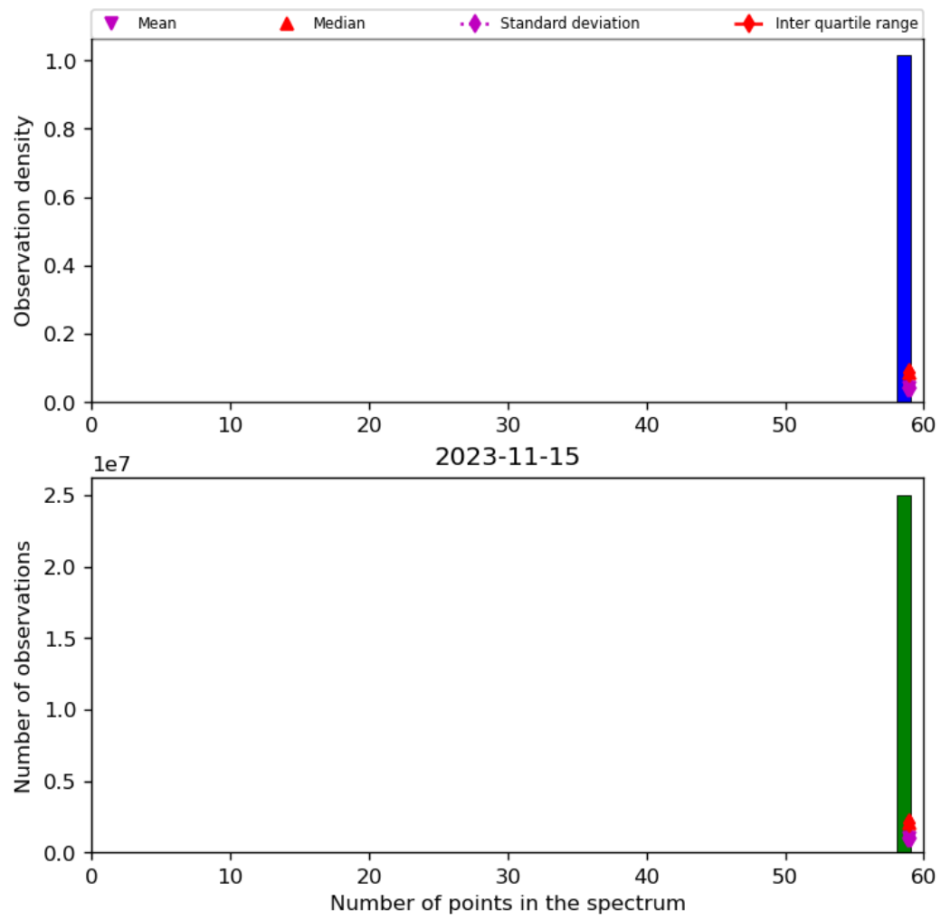
Figure 44: Histogram of “Number of points in the spectrum” for 2023-11-14 to 2023-11-16
