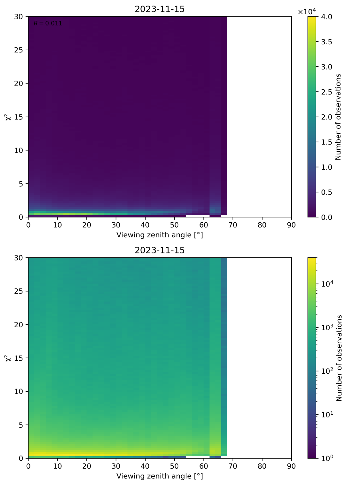
Figure 130: Scatter density plot of “Viewing zenith angle” against “ \chi^2 ” for 2023-11-14 to 2023-11-16.
