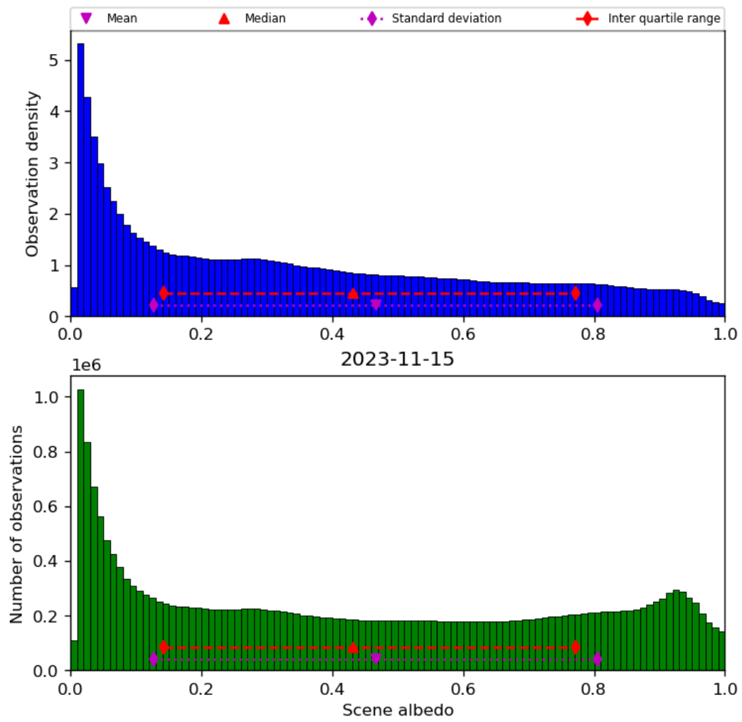
Figure 34: Histogram of “Scene albedo” for 2023-11-14 to 2023-11-16
