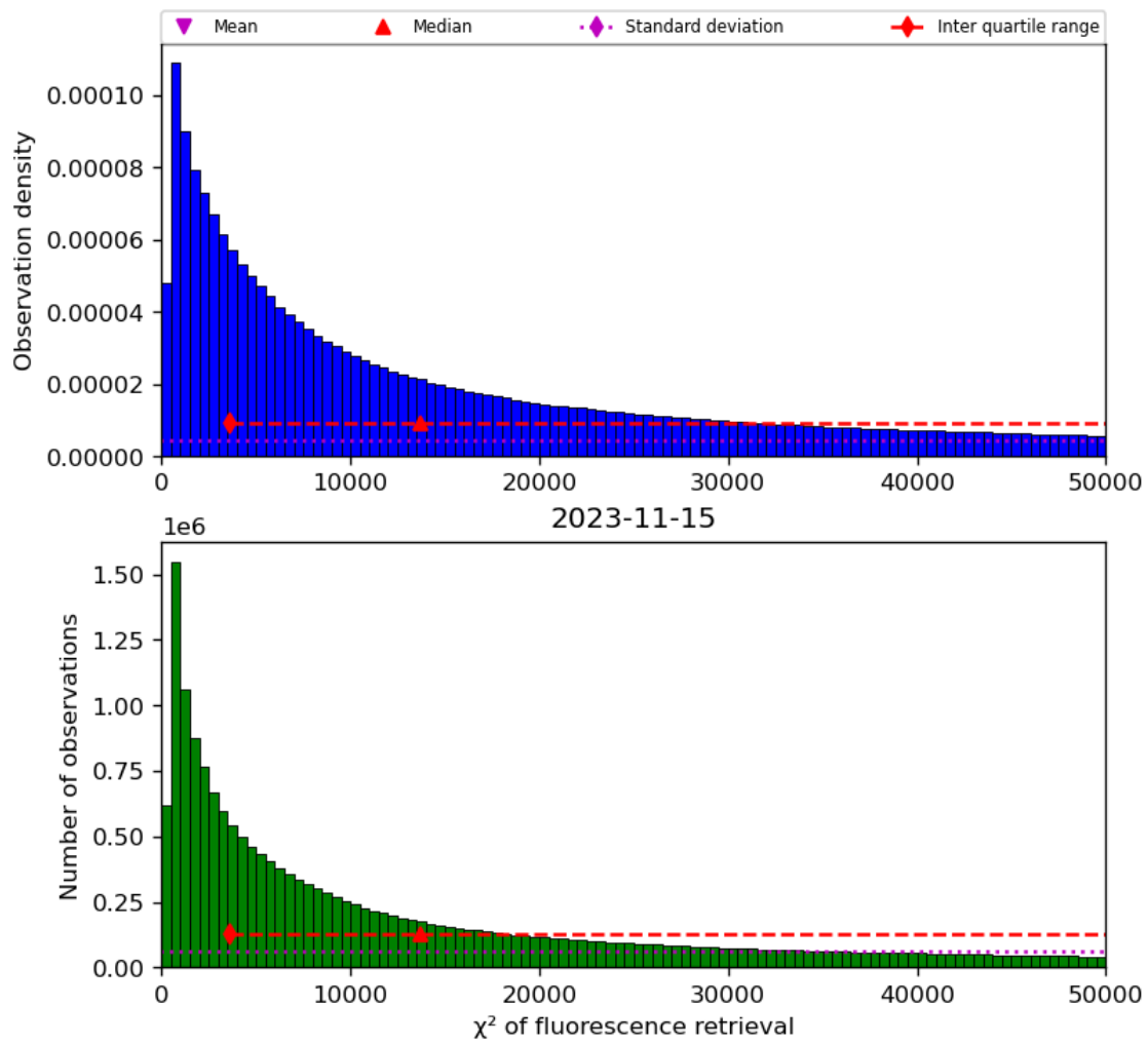
Figure 42: Histogram of “ \chi^2 of fluorescence retrieval” for 2023-11-14 to 2023-11-16
