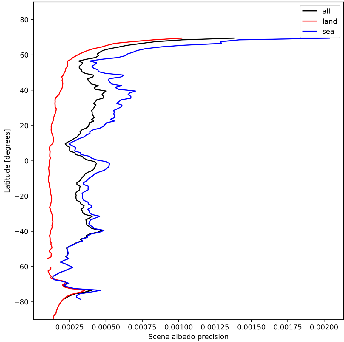
Figure 18: Zonal average of "Scene albedo precision" for 2023-11-14 to 2023-11-16.
