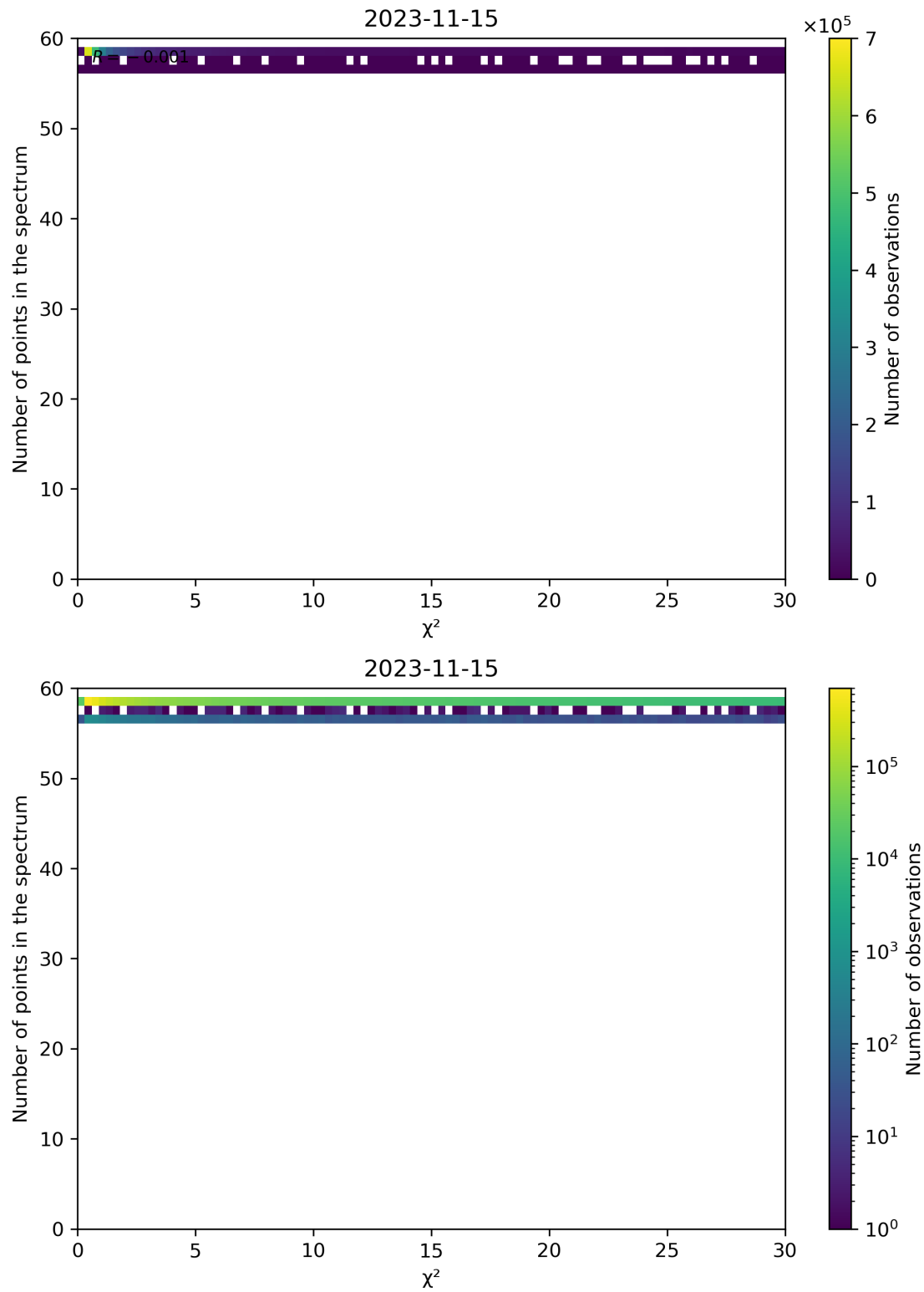
Figure 74: Scatter density plot of " \chi^2 " against "Number of points in the spectrum" for 2023-11-14 to 2023-11-16.
