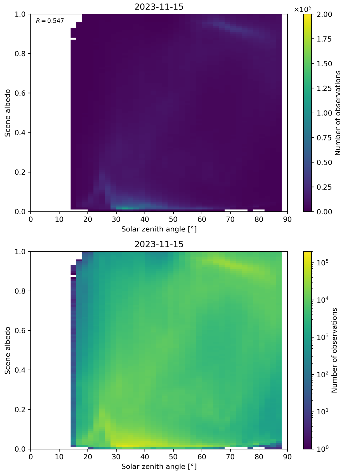
Figure 127: Scatter density plot of “Solar zenith angle” against “Scene albedo” for 2023-11-14 to 2023-11-16.
