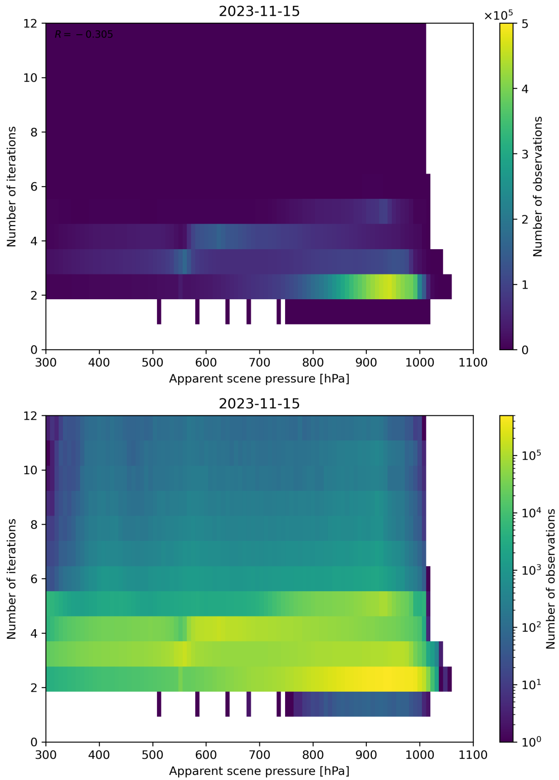
Figure 66: Scatter density plot of “Apparent scene pressure” against “Number of iterations” for 2023-11-14 to 2023-11-16.
