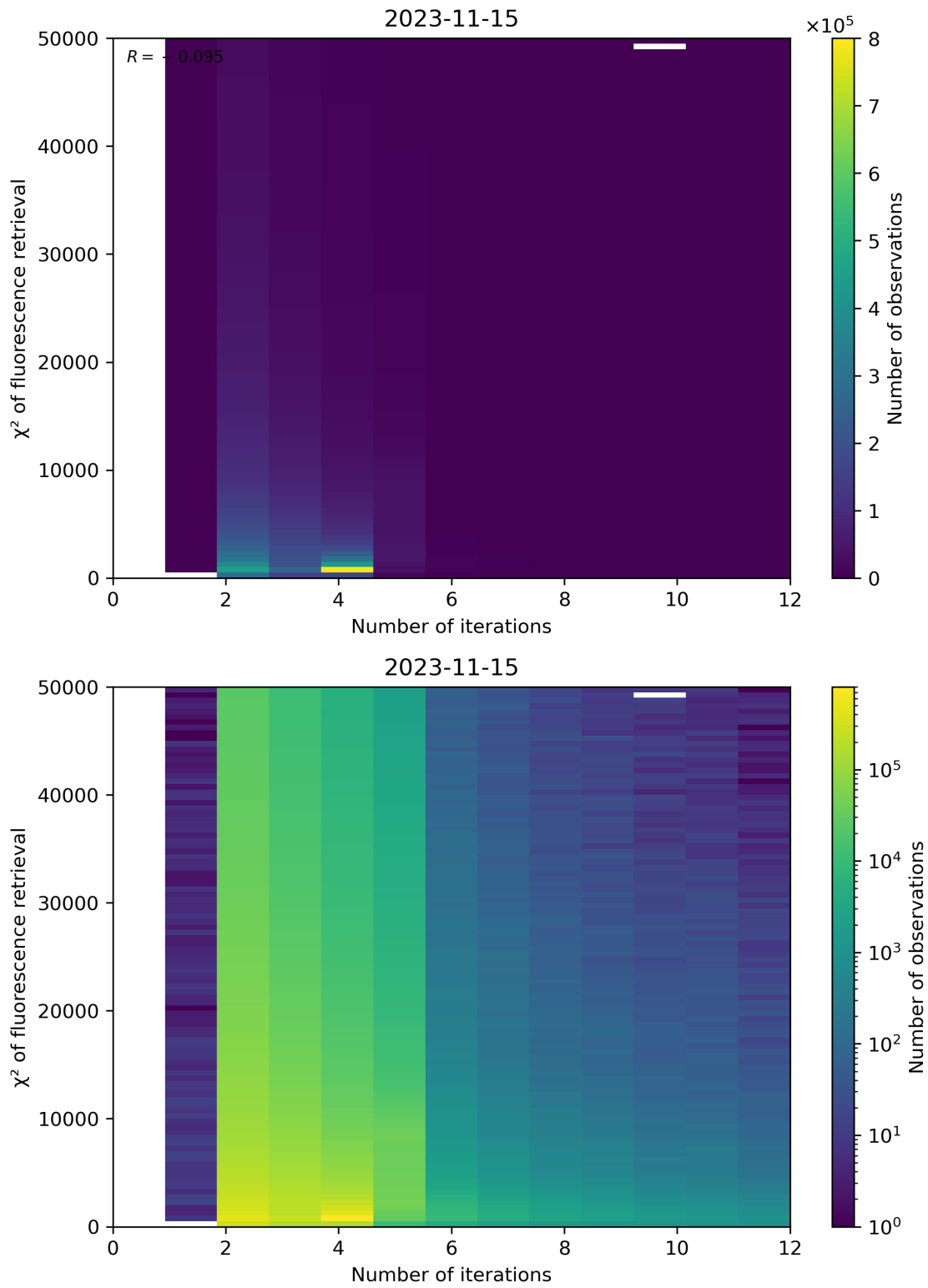
Figure 106: Scatter density plot of “Number of iterations” against “ \chi^2 of fluorescence retrieval” for 2023-11-14 to 2023-11-16.
