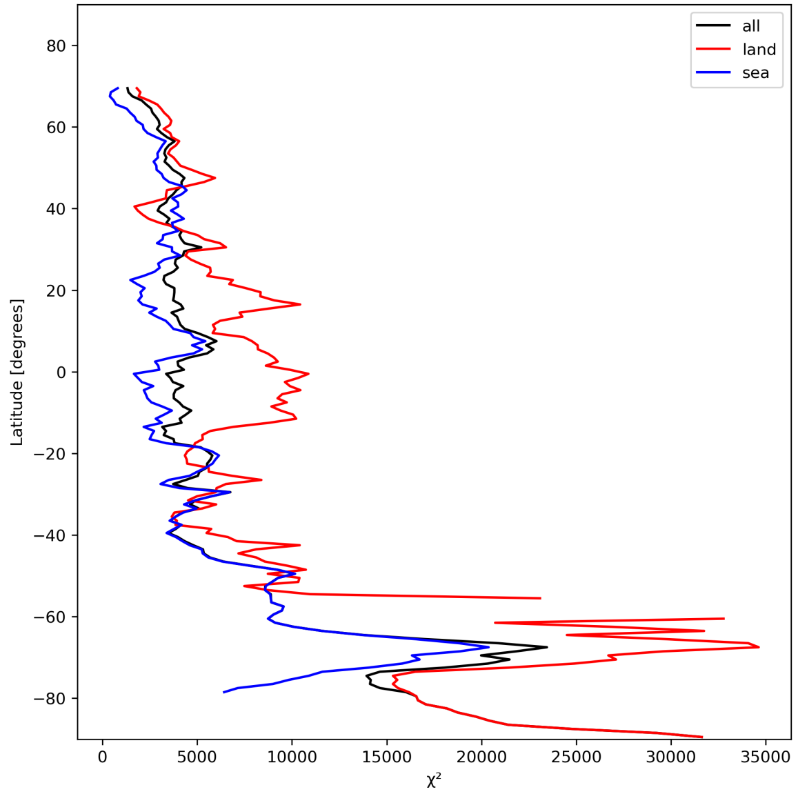
Figure 21: Zonal average of “ \chi^2 ” for 2023-11-14 to 2023-11-16.
