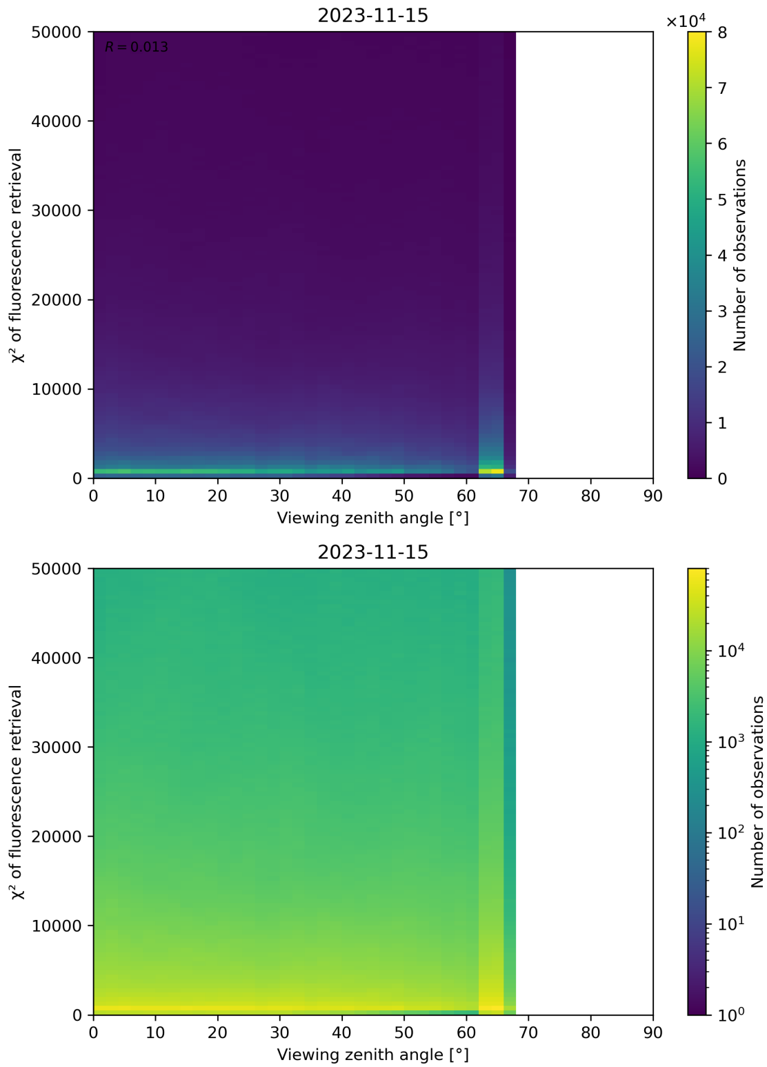
Figure 131: Scatter density plot of “Viewing zenith angle” against “ \chi^2 of fluorescence retrieval” for 2023-11-14 to 2023-11-16.
