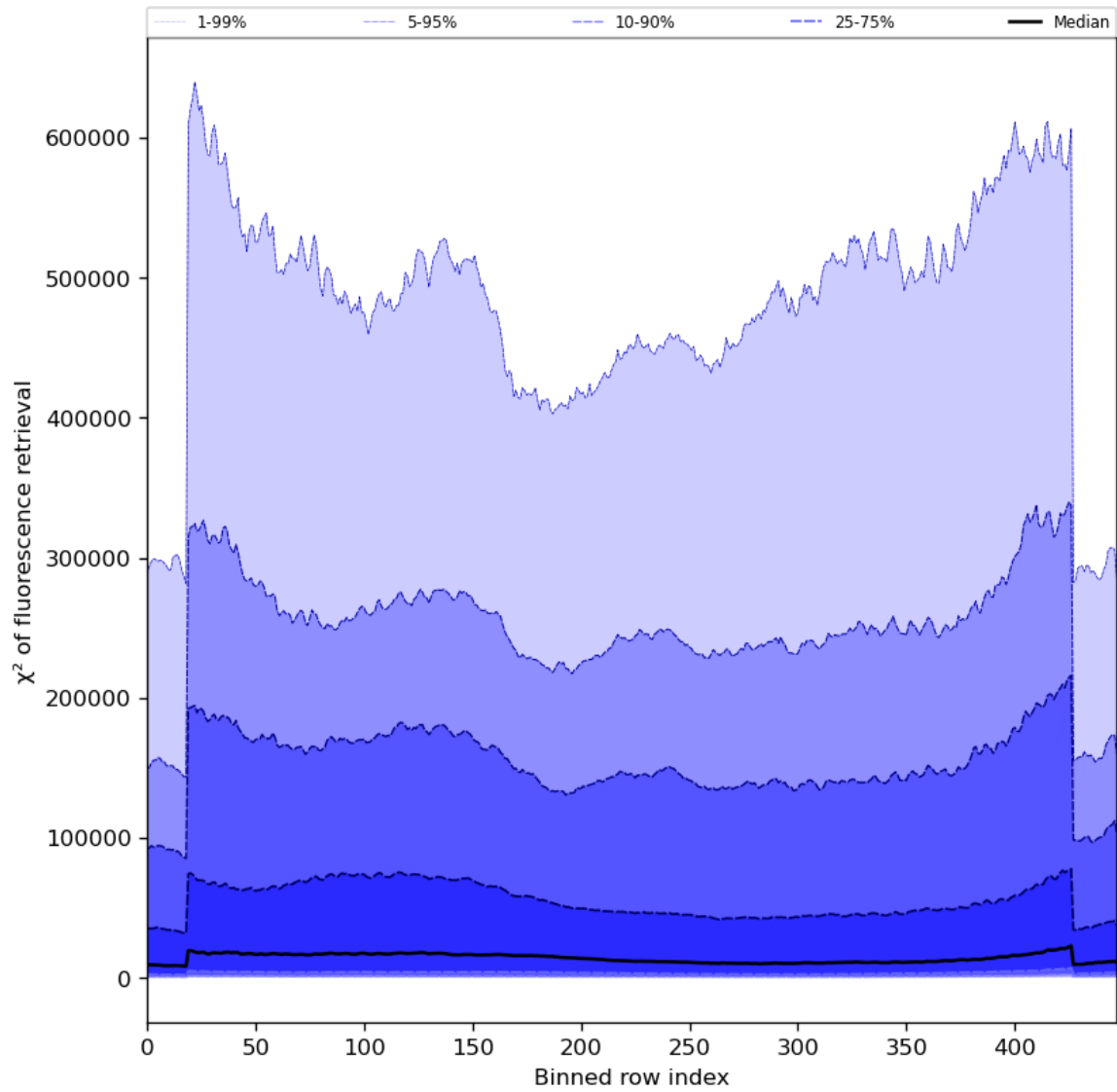
Figure 59: Along track statistics of “ \chi^2 of fluorescence retrieval” for 2023-11-14 to 2023-11-16
