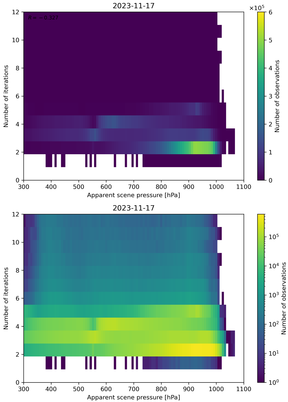
Figure 66: Scatter density plot of “Apparent scene pressure” against “Number of iterations” for 2023-11-16 to 2023-11-18.
