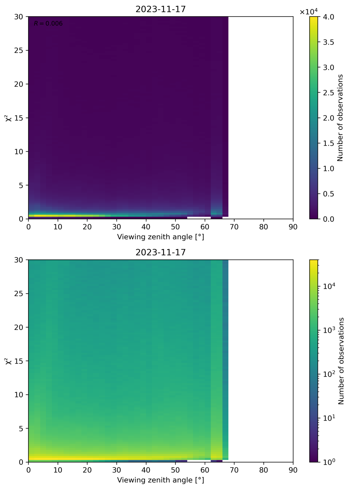
Figure 130: Scatter density plot of “Viewing zenith angle” against “ \chi^2 ” for 2023-11-16 to 2023-11-18.
