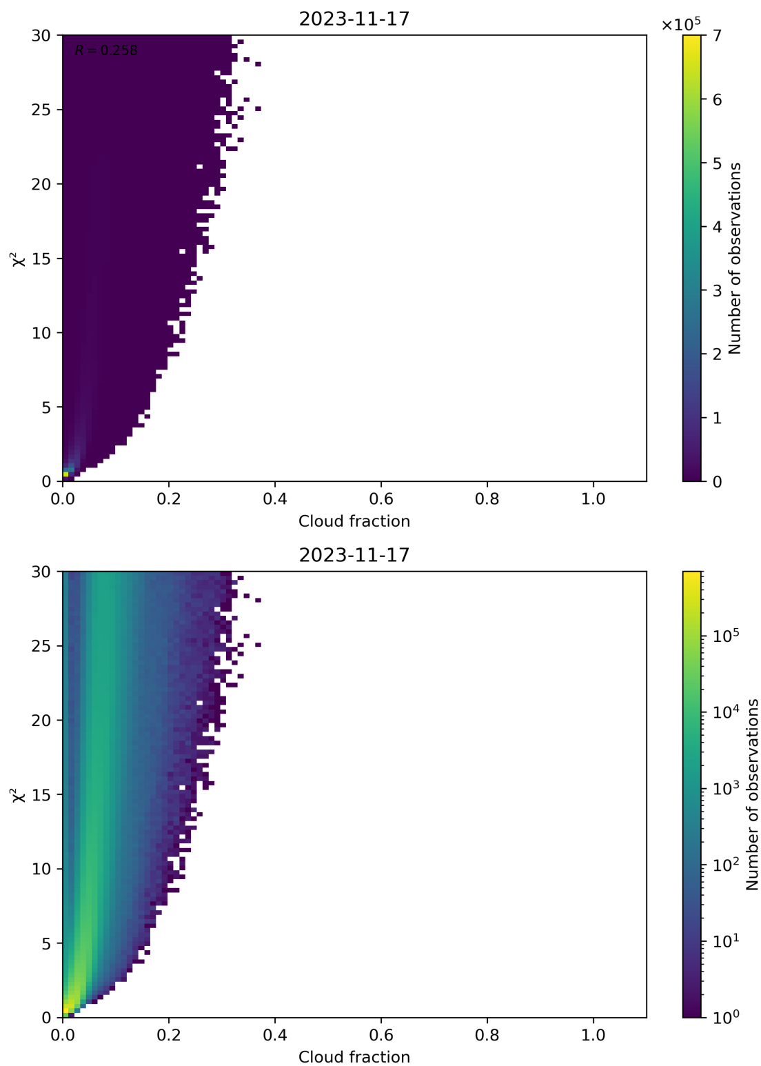
Figure 77: Scatter density plot of “Cloud fraction” against “ \chi^2 ” for 2023-11-16 to 2023-11-18.
