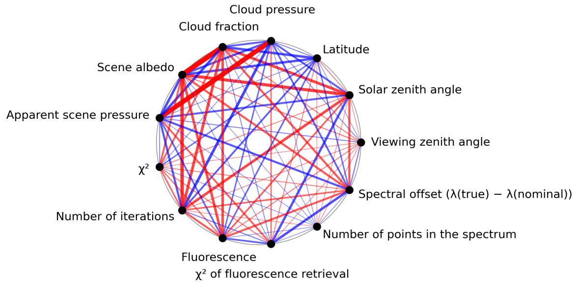
Figure 1: Map of correlation graph for 2023-11-16 to 2023-11-18.
