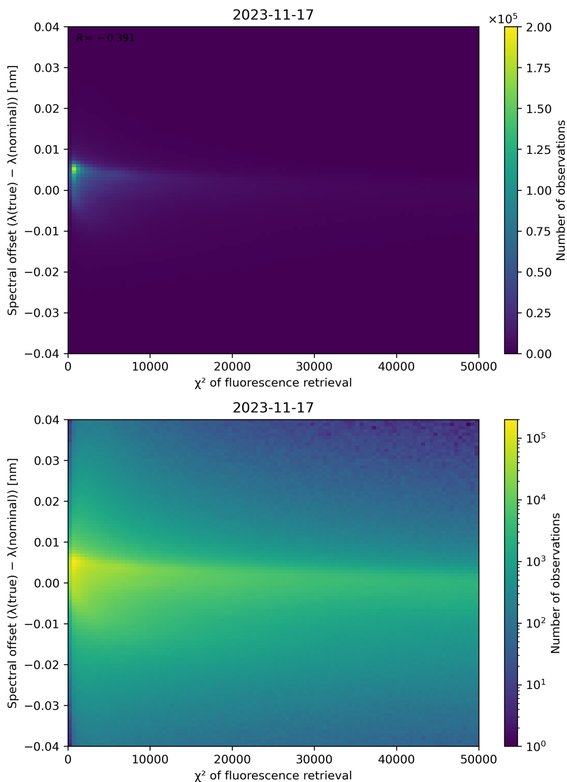
Figure 72: Scatter density plot of " \chi^2 of fluorescence retrieval" against "Spectral offset ( \lambda(\text{true}) - \lambda(\text{nominal}) )" for 2023-11-16 to 2023-11-18.
