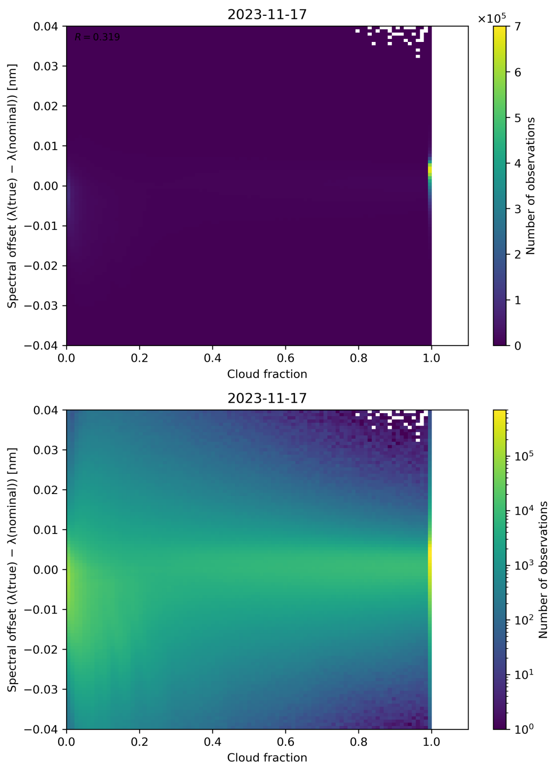
Figure 83: Scatter density plot of “Cloud fraction” against “Spectral offset ( \lambda(\text{true}) - \lambda(\text{nominal}) )” for 2023-11-16 to 2023-11-18.
