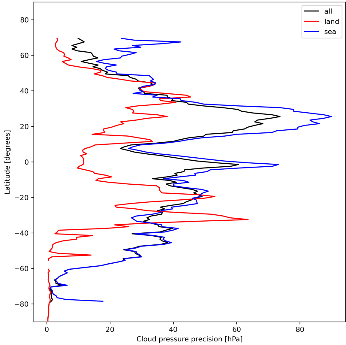
Figure 14: Zonal average of "Cloud pressure precision" for 2023-11-16 to 2023-11-18.
