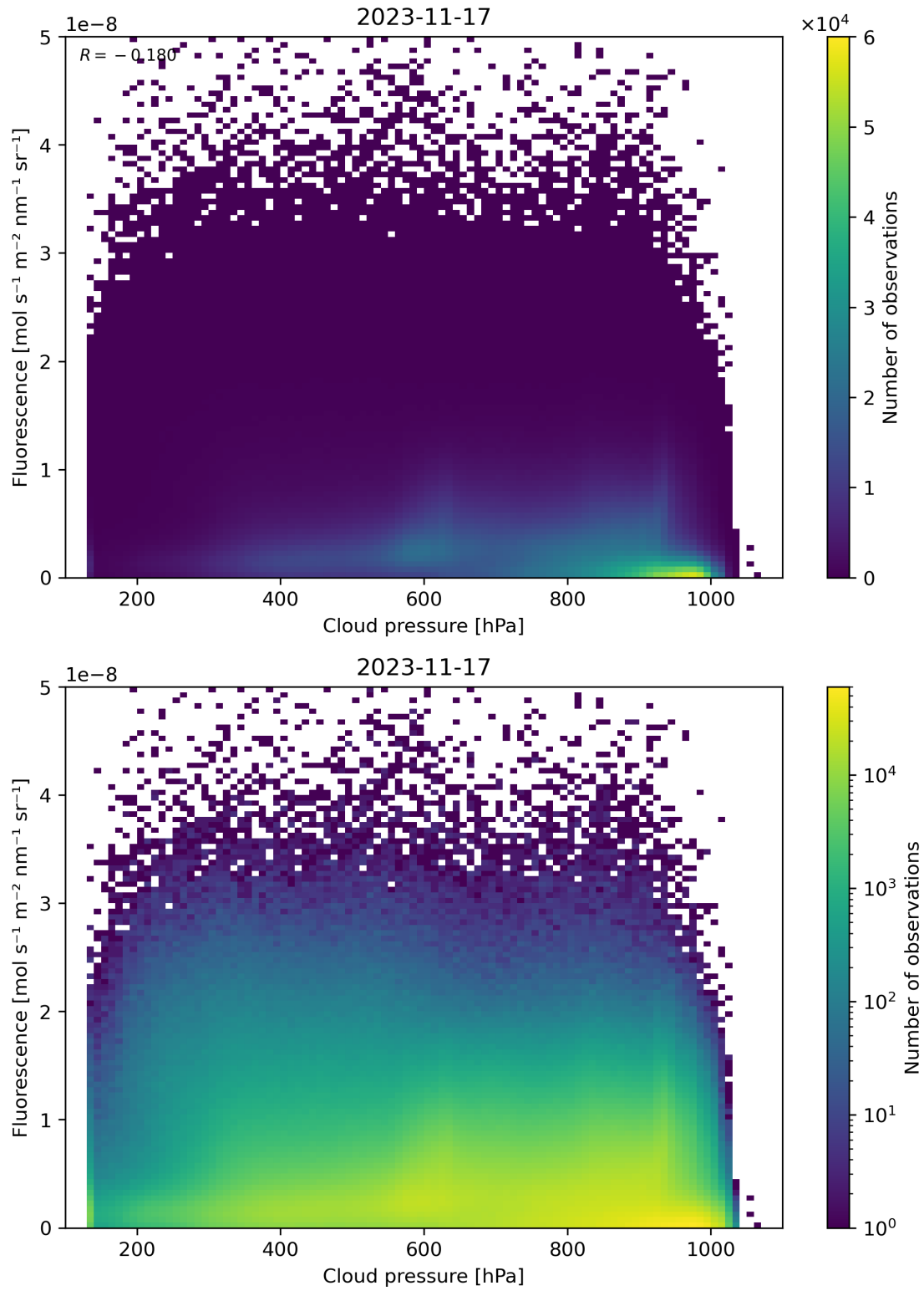
Figure 88: Scatter density plot of “Cloud pressure” against “Fluorescence” for 2023-11-16 to 2023-11-18.
