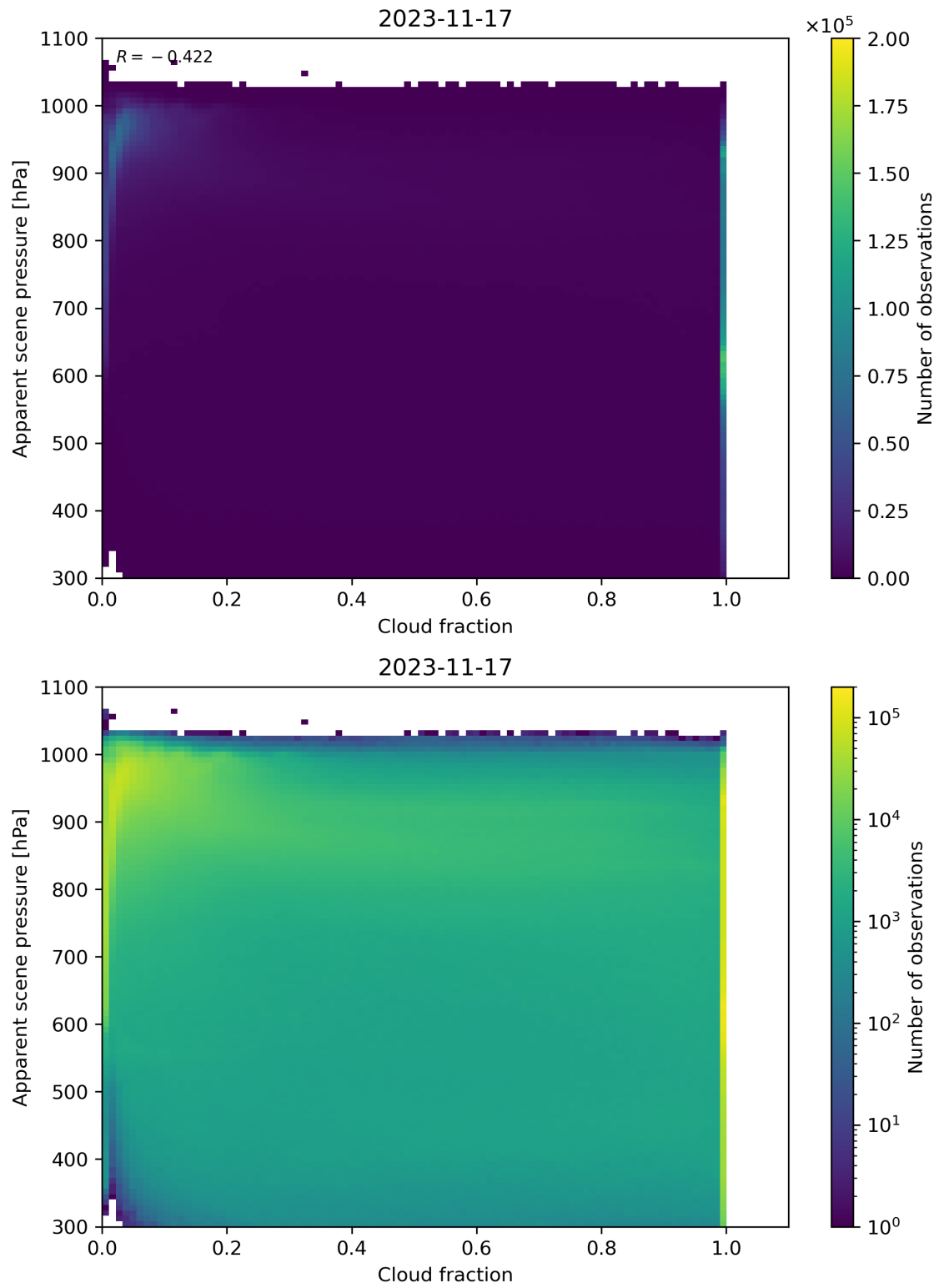
Figure 76: Scatter density plot of “Cloud fraction” against “Apparent scene pressure” for 2023-11-16 to 2023-11-18.
