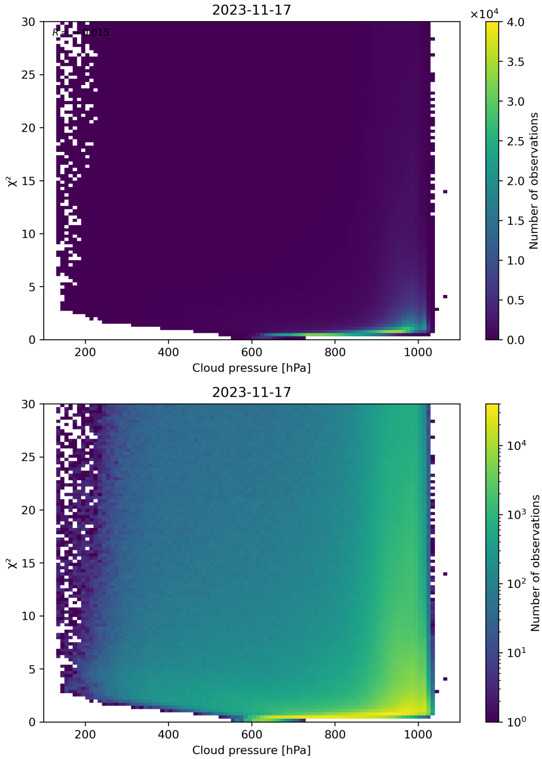
Figure 85: Scatter density plot of “Cloud pressure” against “ \chi^2 ” for 2023-11-16 to 2023-11-18.
