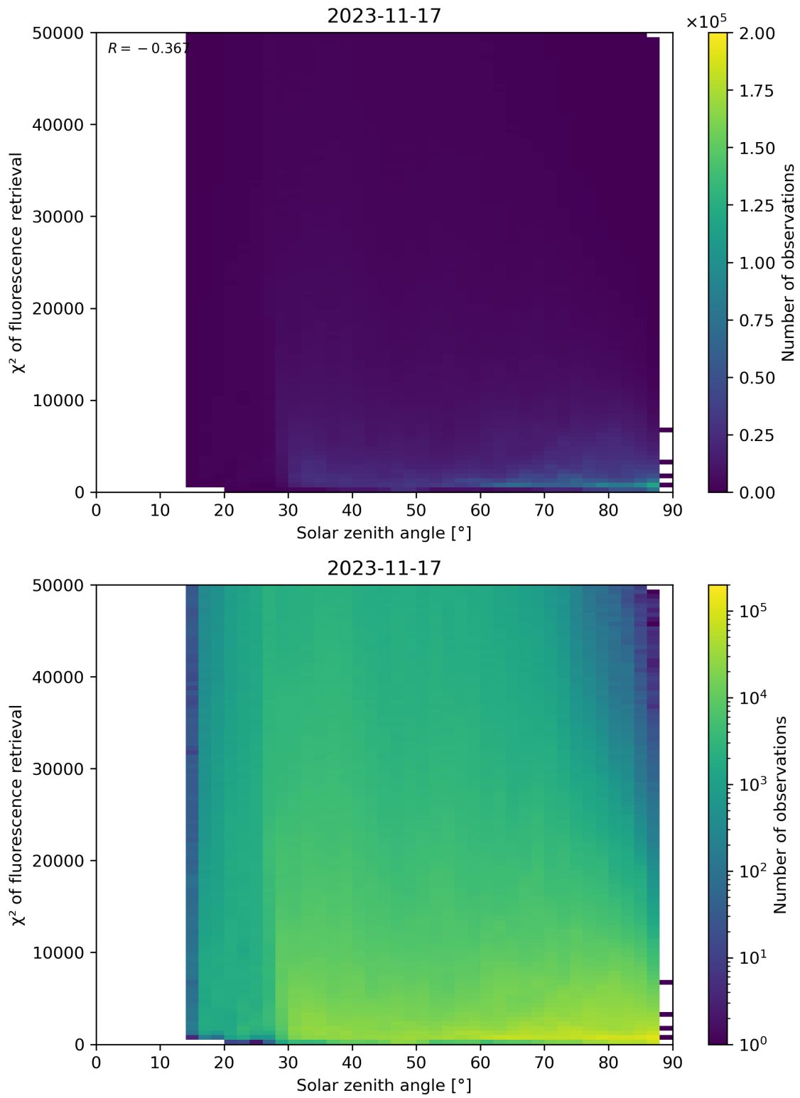
Figure 120: Scatter density plot of “Solar zenith angle” against “ \chi^2 of fluorescence retrieval” for 2023-11-16 to 2023-11-18.
