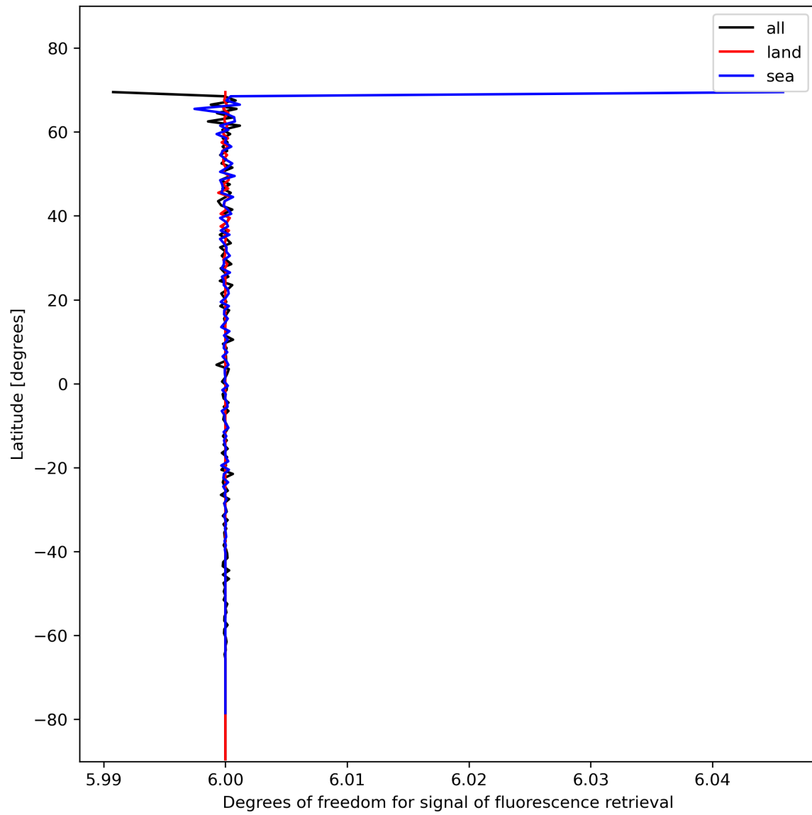
Figure 26: Zonal average of “Degrees of freedom for signal of fluorescence retrieval” for 2023-11-16 to 2023-11-18.
