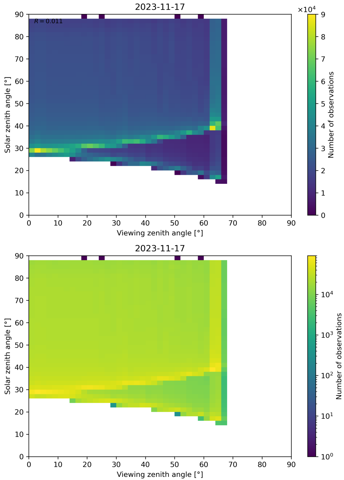
Figure 139: Scatter density plot of “Viewing zenith angle” against “Solar zenith angle” for 2023-11-16 to 2023-11-18.
