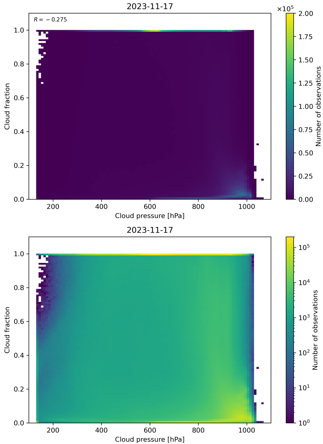
Figure 87: Scatter density plot of “Cloud pressure” against “Cloud fraction” for 2023-11-16 to 2023-11-18.
