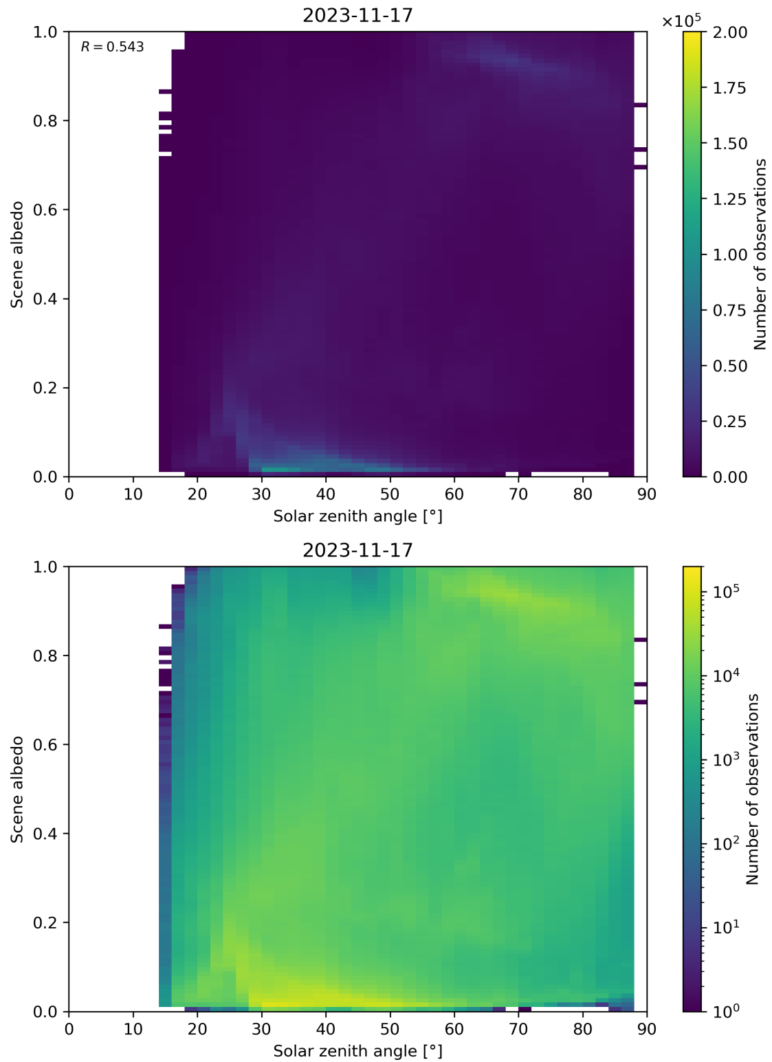
Figure 127: Scatter density plot of “Solar zenith angle” against “Scene albedo” for 2023-11-16 to 2023-11-18.
