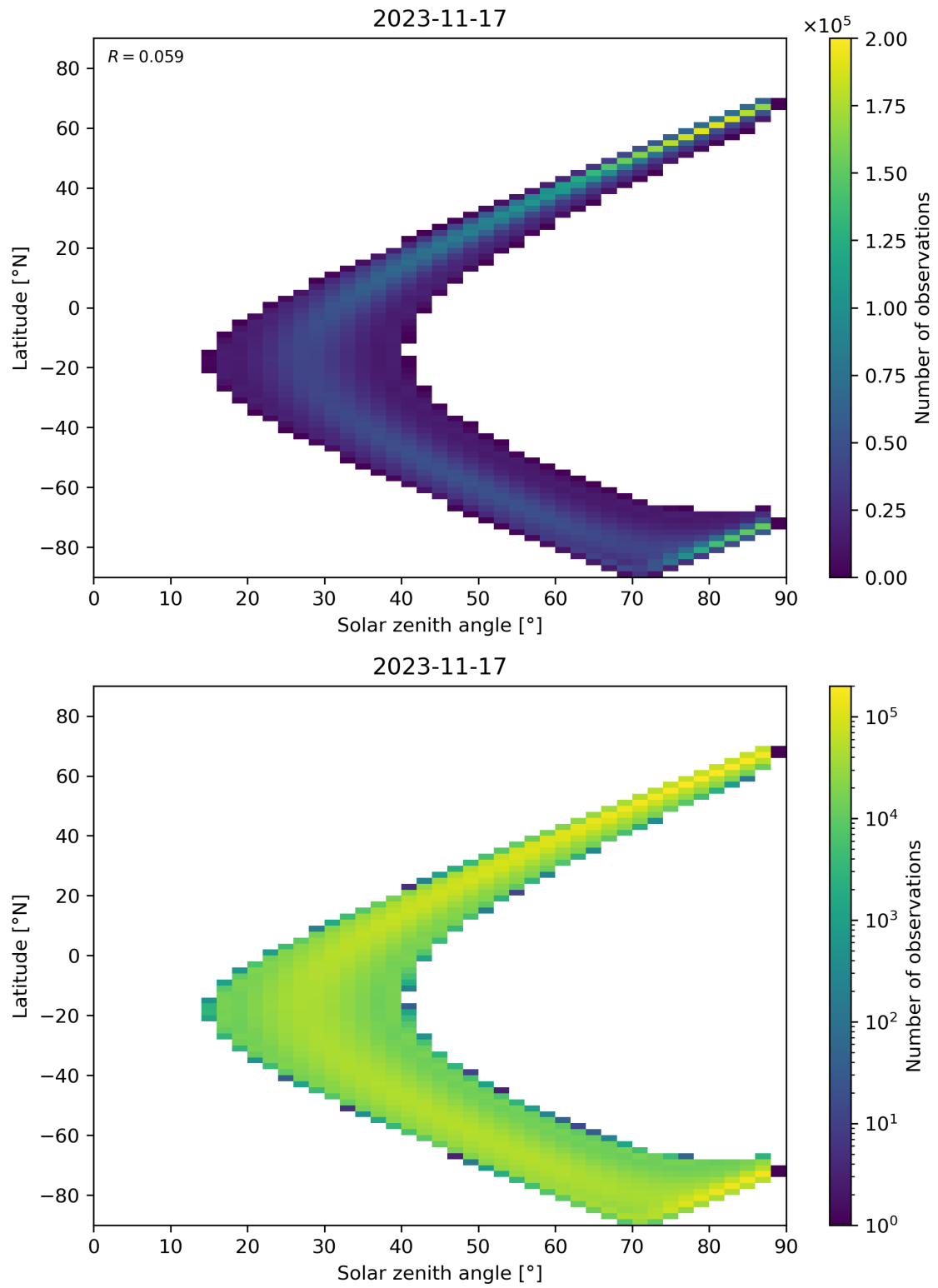
Figure 124: Scatter density plot of “Solar zenith angle” against “Latitude” for 2023-11-16 to 2023-11-18.
