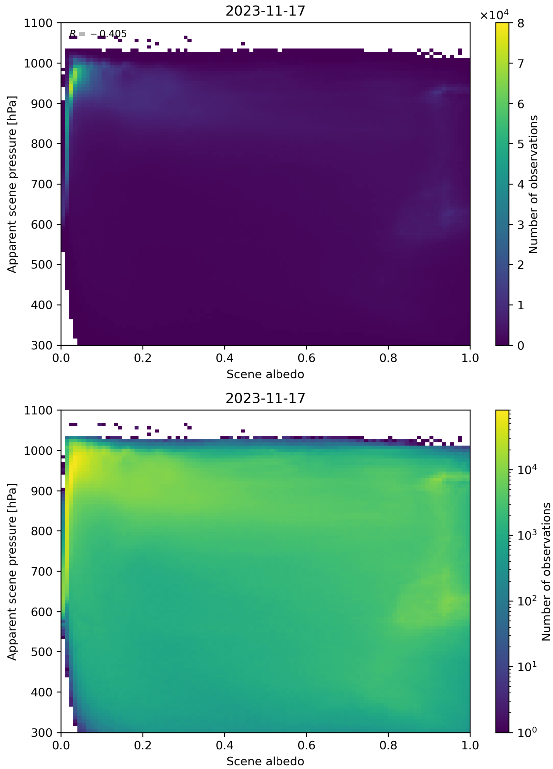
Figure 111: Scatter density plot of “Scene albedo” against “Apparent scene pressure” for 2023-11-16 to 2023-11-18.
