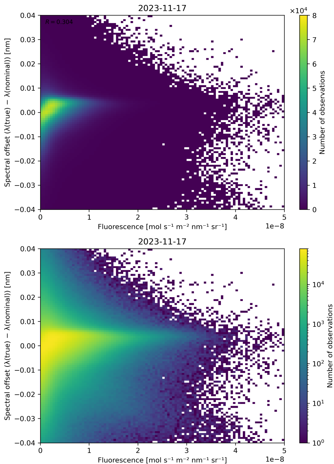
Figure 95: Scatter density plot of “Fluorescence” against “Spectral offset ( \lambda(\text{true}) - \lambda(\text{nominal}) )” for 2023-11-16 to 2023-11-18.
