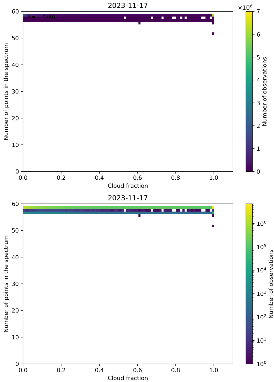
Figure 81: Scatter density plot of “Cloud fraction” against “Number of points in the spectrum” for 2023-11-16 to 2023-11-18.
