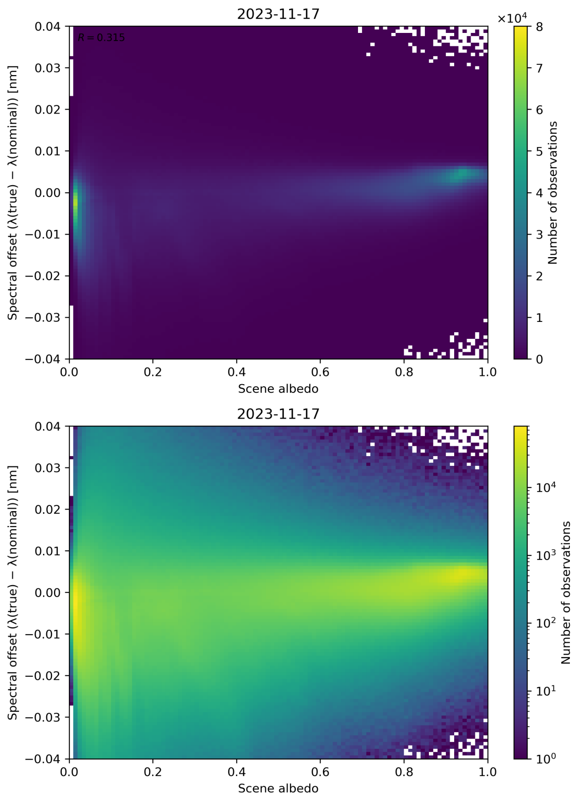
Figure 117: Scatter density plot of “Scene albedo” against “Spectral offset ( \lambda(\text{true}) - \lambda(\text{nominal}) )” for 2023-11-16 to 2023-11-18.
