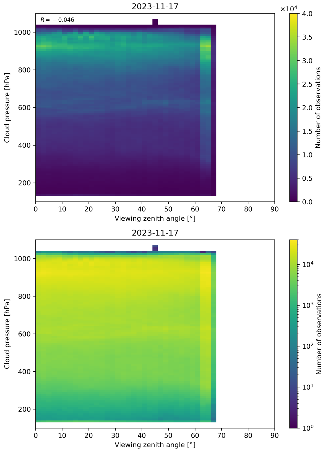
Figure 133: Scatter density plot of “Viewing zenith angle” against “Cloud pressure” for 2023-11-16 to 2023-11-18.
