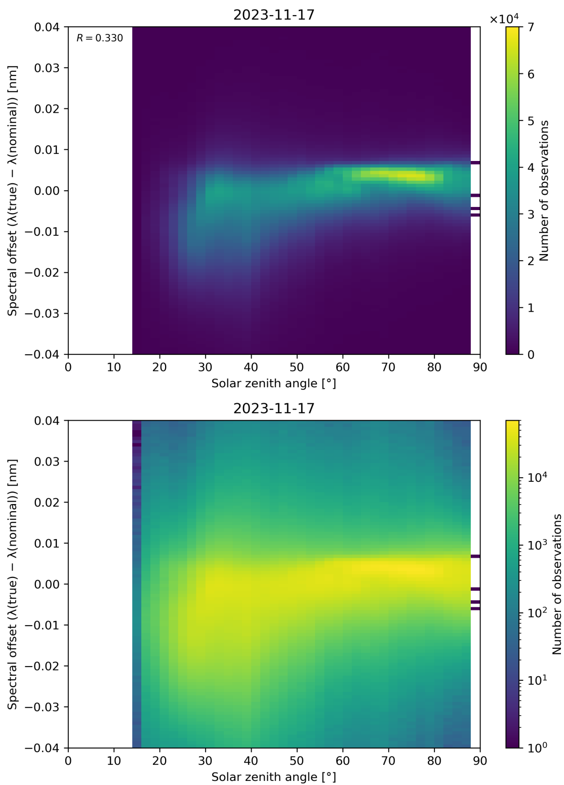
Figure 128: Scatter density plot of “Solar zenith angle” against “Spectral offset ( \lambda(\text{true}) - \lambda(\text{nominal}) )” for 2023-11-16 to 2023-11-18.
