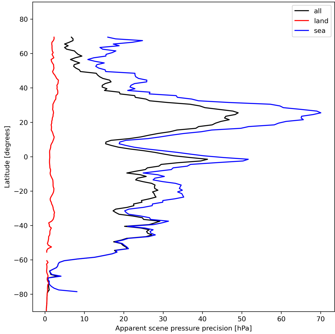
Figure 20: Zonal average of “Apparent scene pressure precision” for 2023-11-16 to 2023-11-18.
