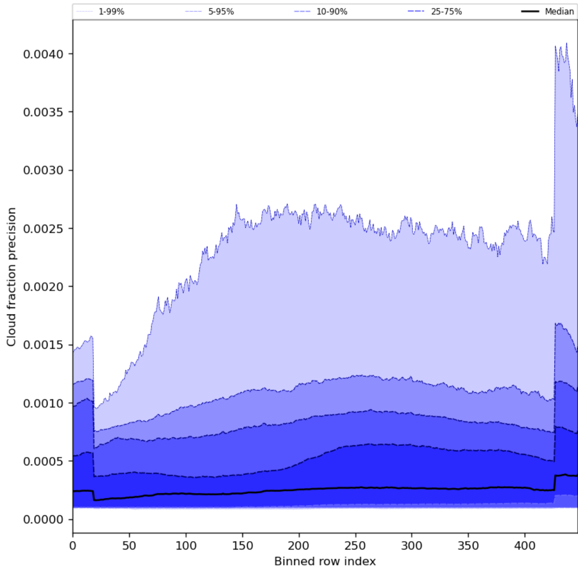
Figure 50: Along track statistics of “Cloud fraction precision” for 2023-11-16 to 2023-11-18
