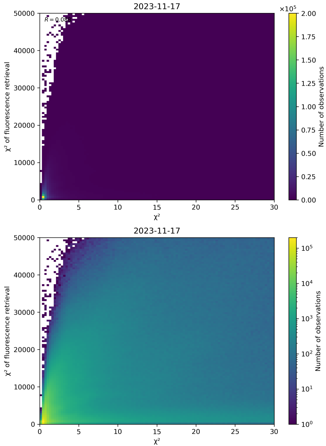
Figure 69: Scatter density plot of “ \chi^2 ” against “ \chi^2 of fluorescence retrieval” for 2023-11-16 to 2023-11-18.
