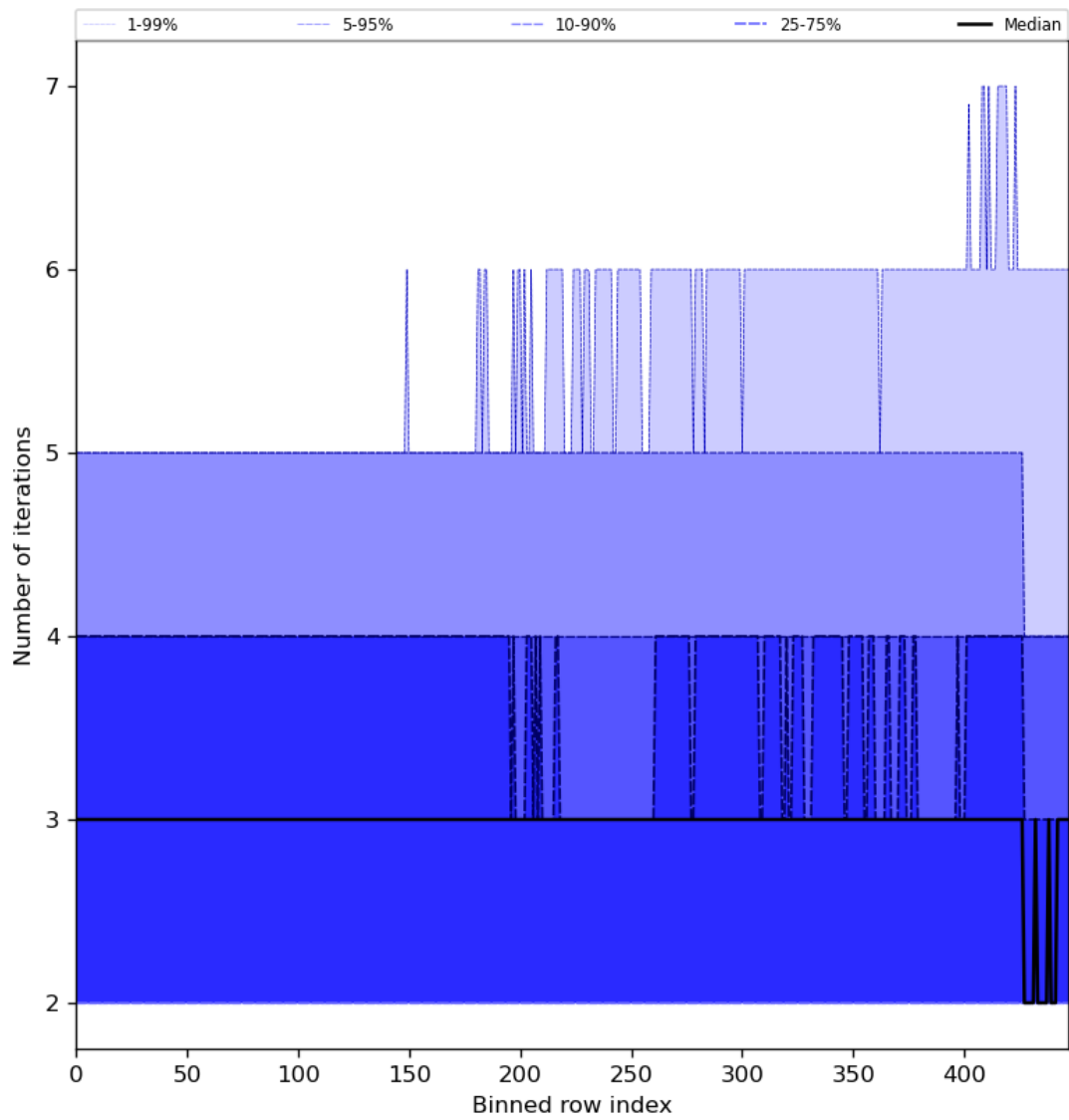
Figure 56: Along track statistics of “Number of iterations” for 2023-11-16 to 2023-11-18
