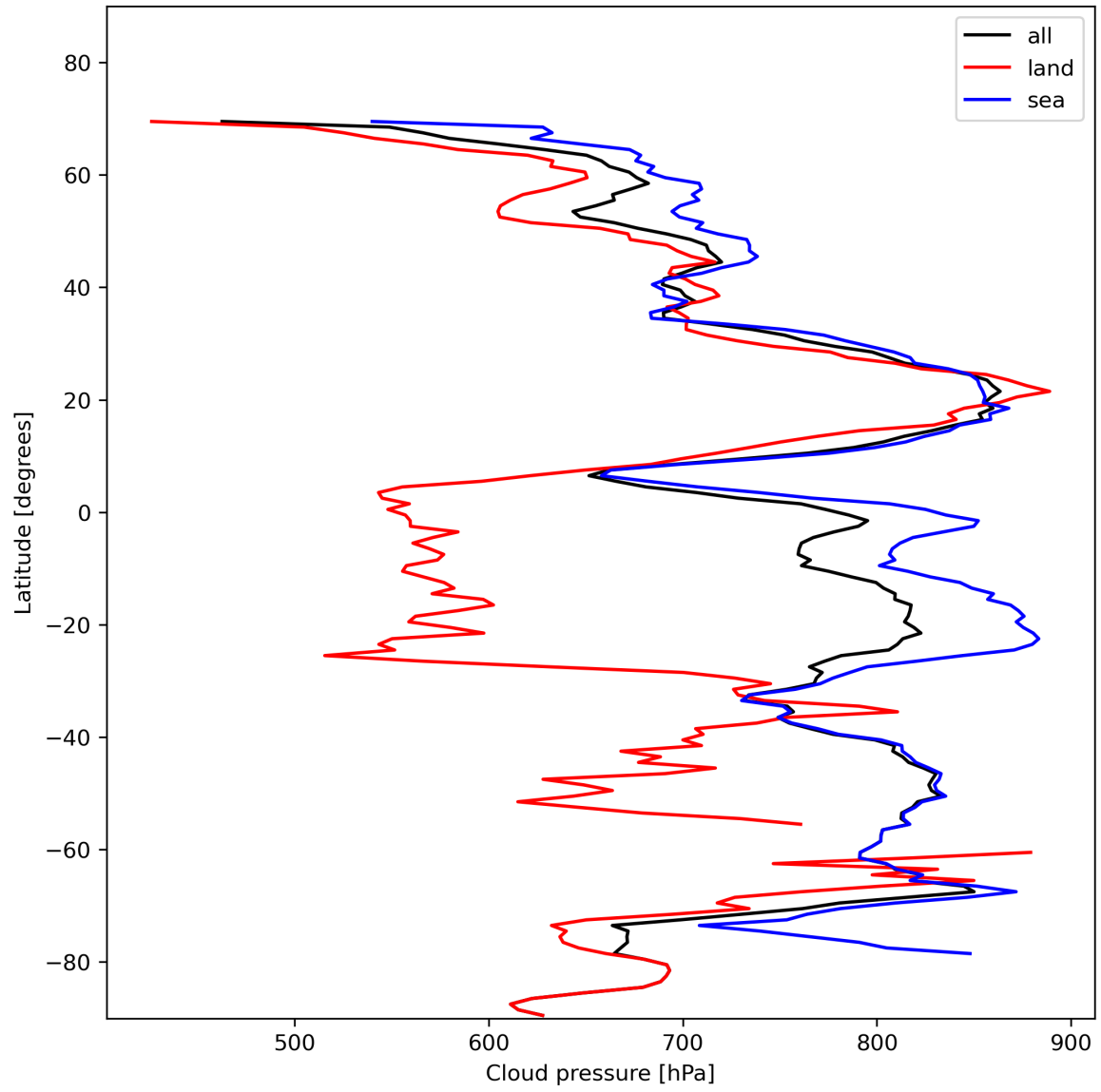
Figure 13: Zonal average of “Cloud pressure” for 2023-11-16 to 2023-11-18.
