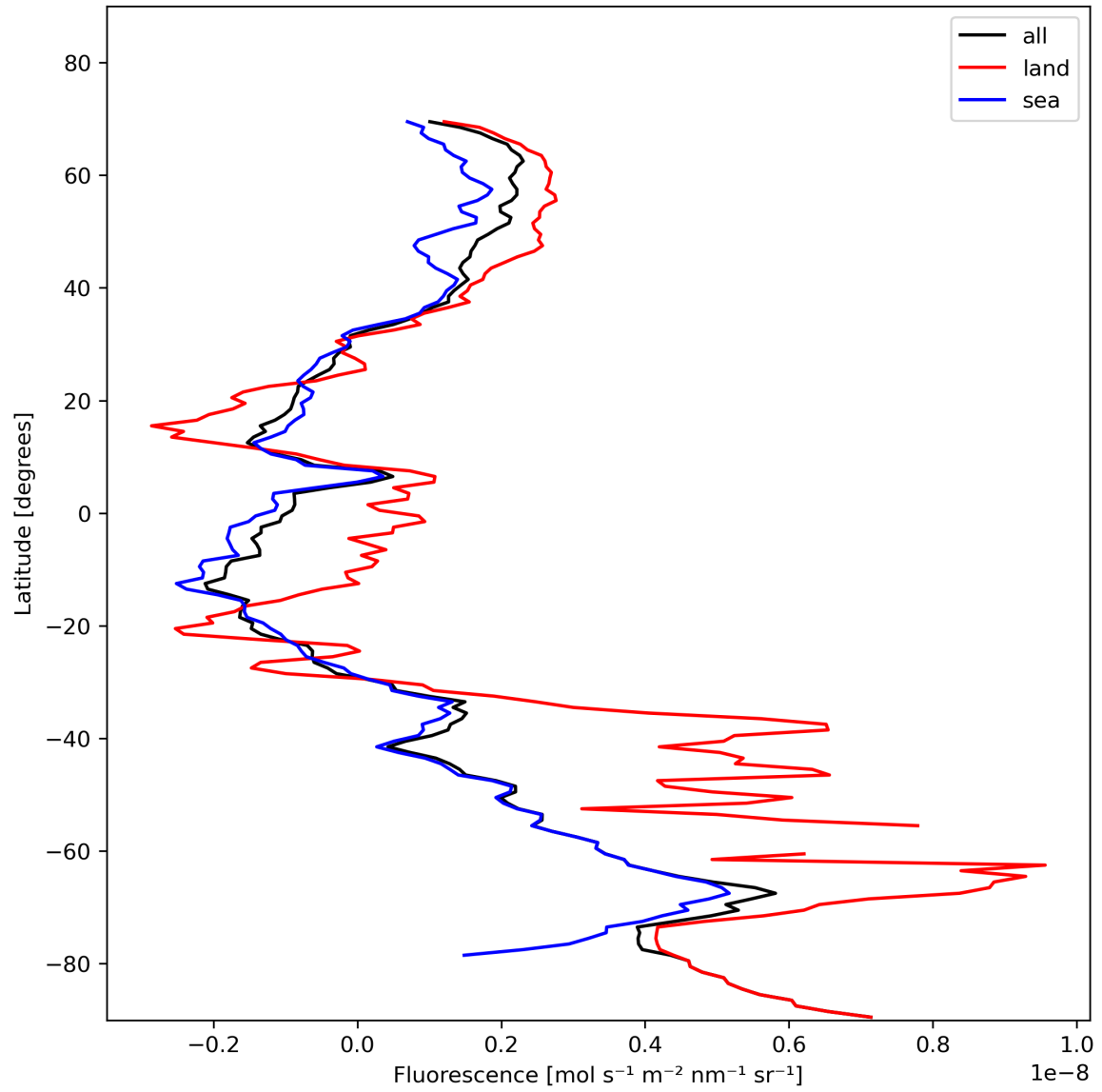
Figure 23: Zonal average of “Fluorescence” for 2023-11-16 to 2023-11-18.
