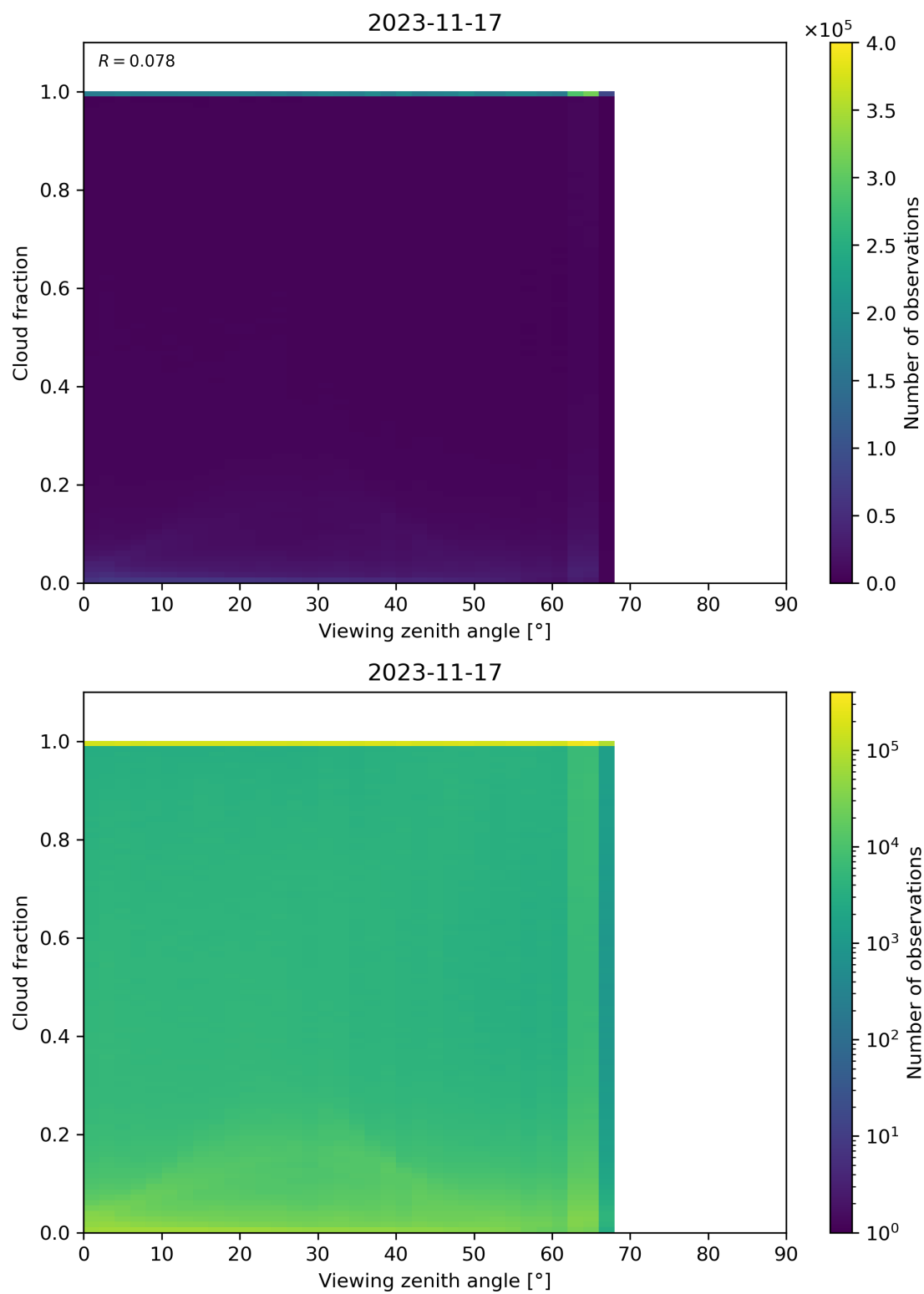
Figure 132: Scatter density plot of “Viewing zenith angle” against “Cloud fraction” for 2023-11-16 to 2023-11-18.
