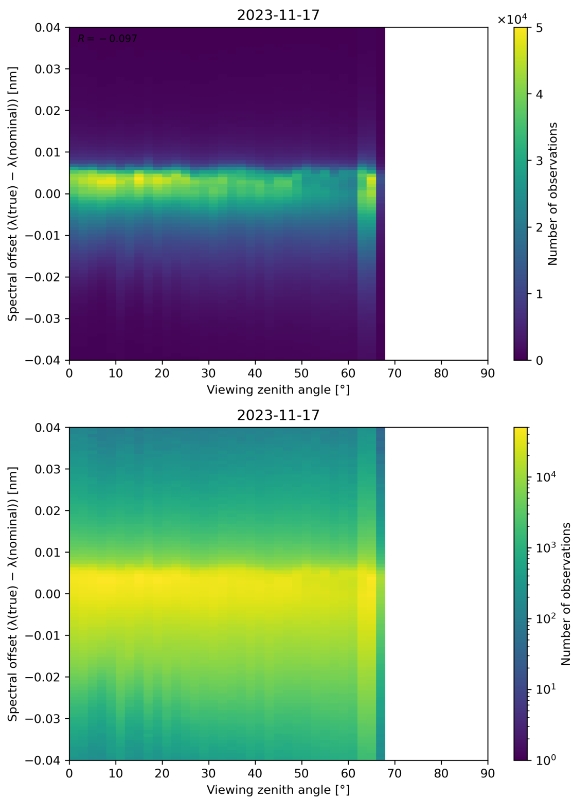
Figure 140: Scatter density plot of “Viewing zenith angle” against “Spectral offset ( \lambda(\text{true}) - \lambda(\text{nominal}) )” for 2023-11-16 to 2023-11-18.
