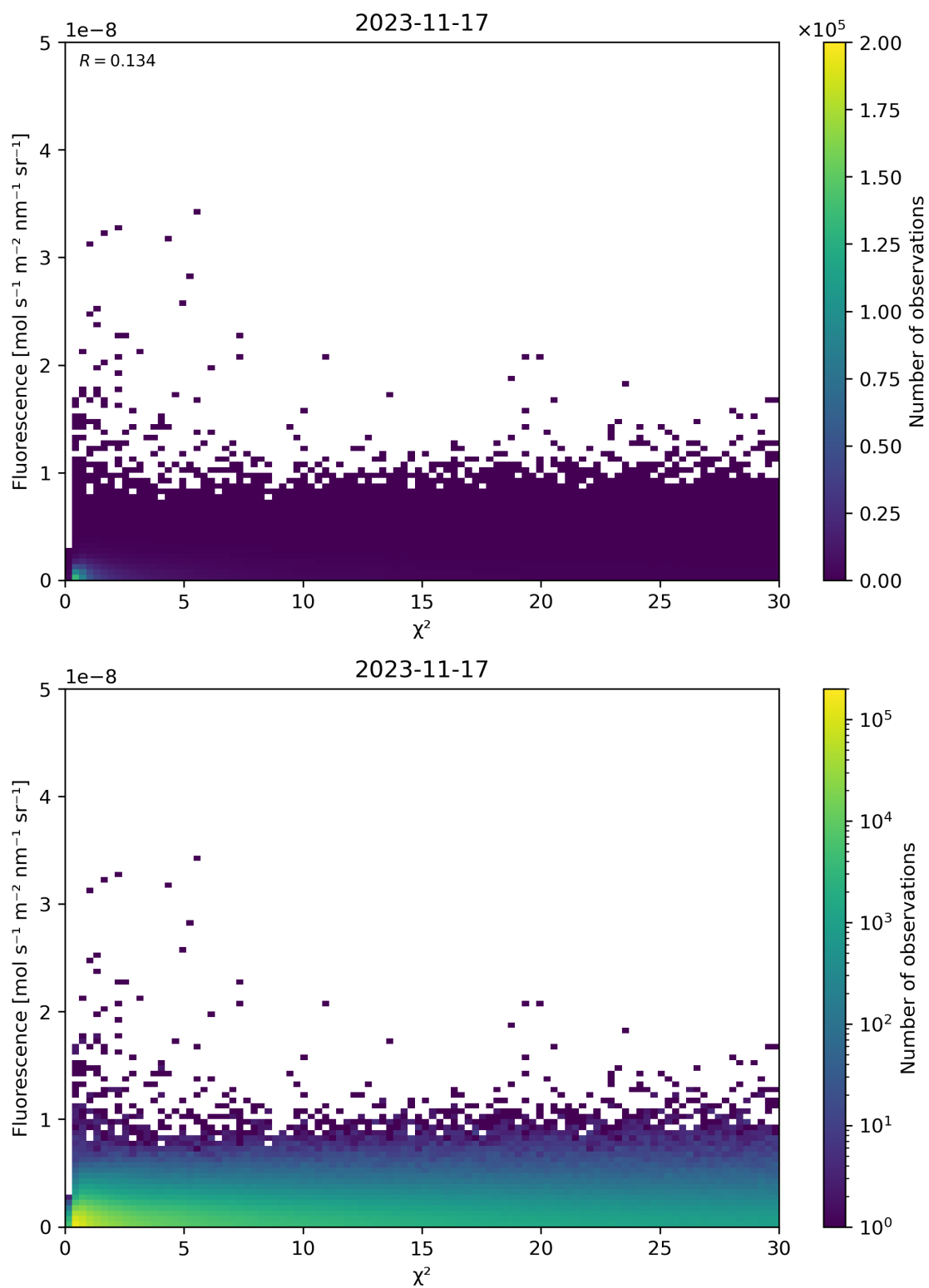
Figure 70: Scatter density plot of “ \chi^2 ” against “Fluorescence” for 2023-11-16 to 2023-11-18.
