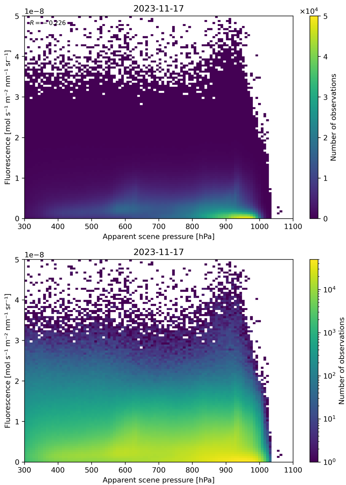
Figure 65: Scatter density plot of “Apparent scene pressure” against “Fluorescence” for 2023-11-16 to 2023-11-18.
