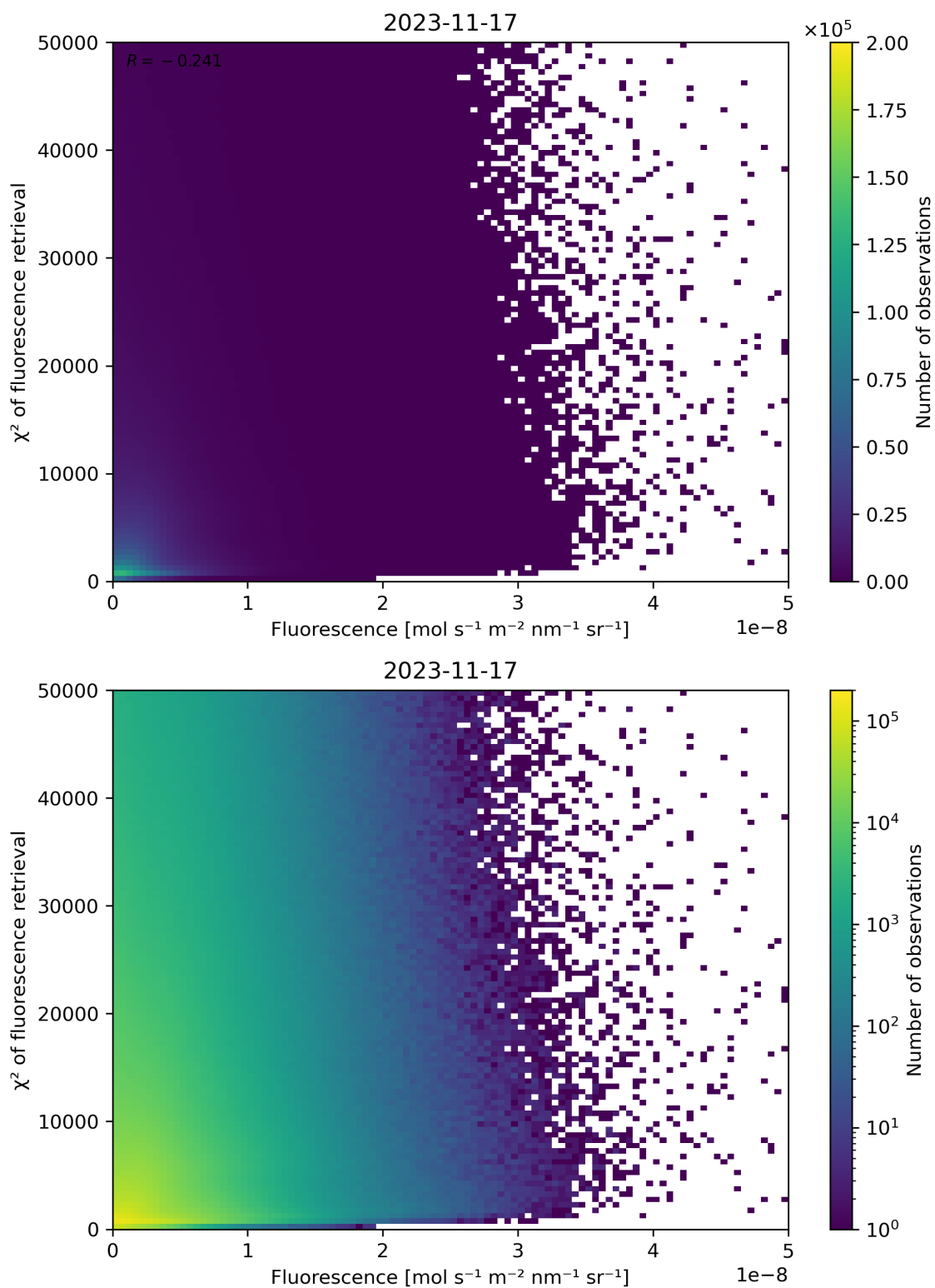
Figure 93: Scatter density plot of “Fluorescence” against “ \chi^2 of fluorescence retrieval” for 2023-11-16 to 2023-11-18.
