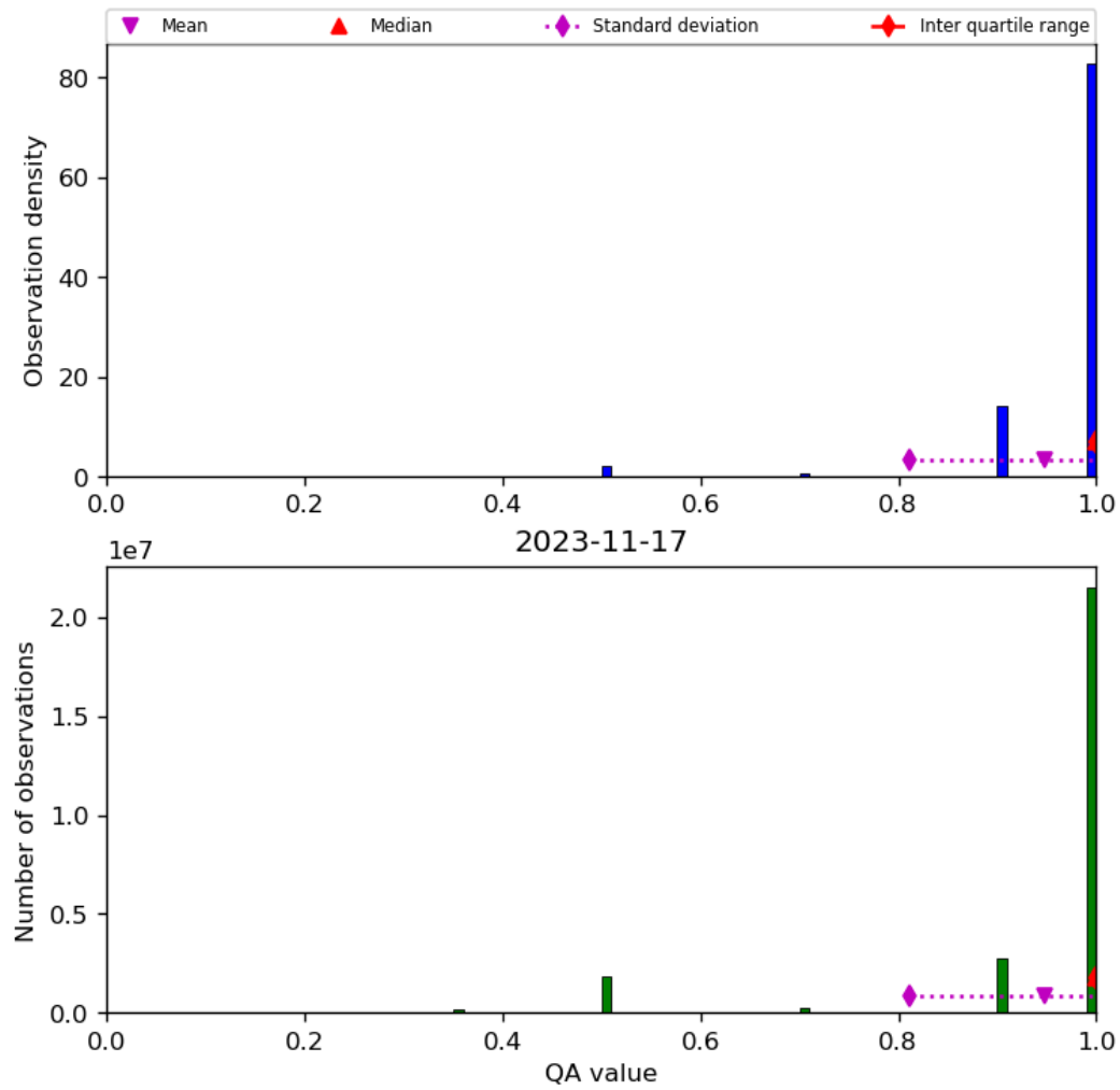
Figure 29: Histogram of “QA value” for 2023-11-16 to 2023-11-18
