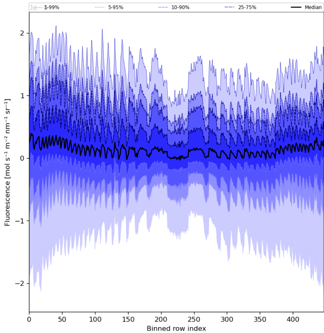
Figure 57: Along track statistics of “Fluorescence” for 2023-11-16 to 2023-11-18
