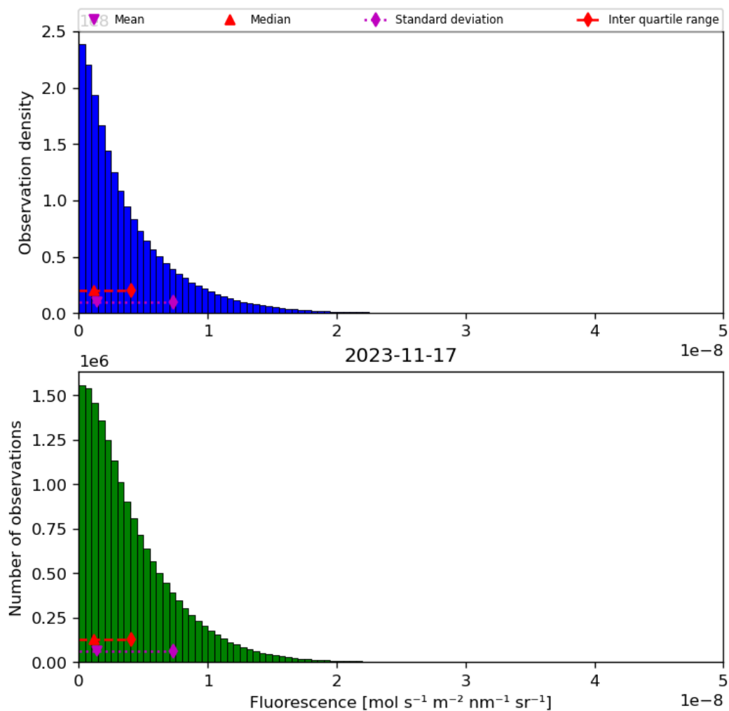
Figure 40: Histogram of “Fluorescence” for 2023-11-16 to 2023-11-18
