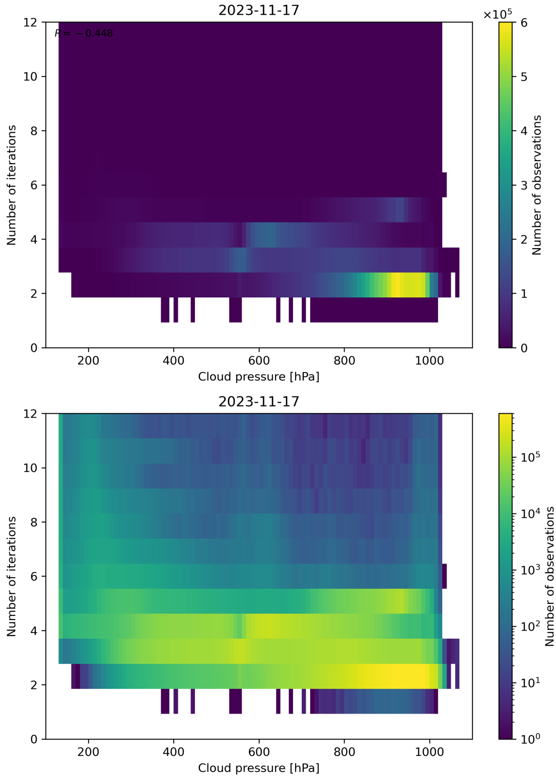
Figure 89: Scatter density plot of “Cloud pressure” against “Number of iterations” for 2023-11-16 to 2023-11-18.
