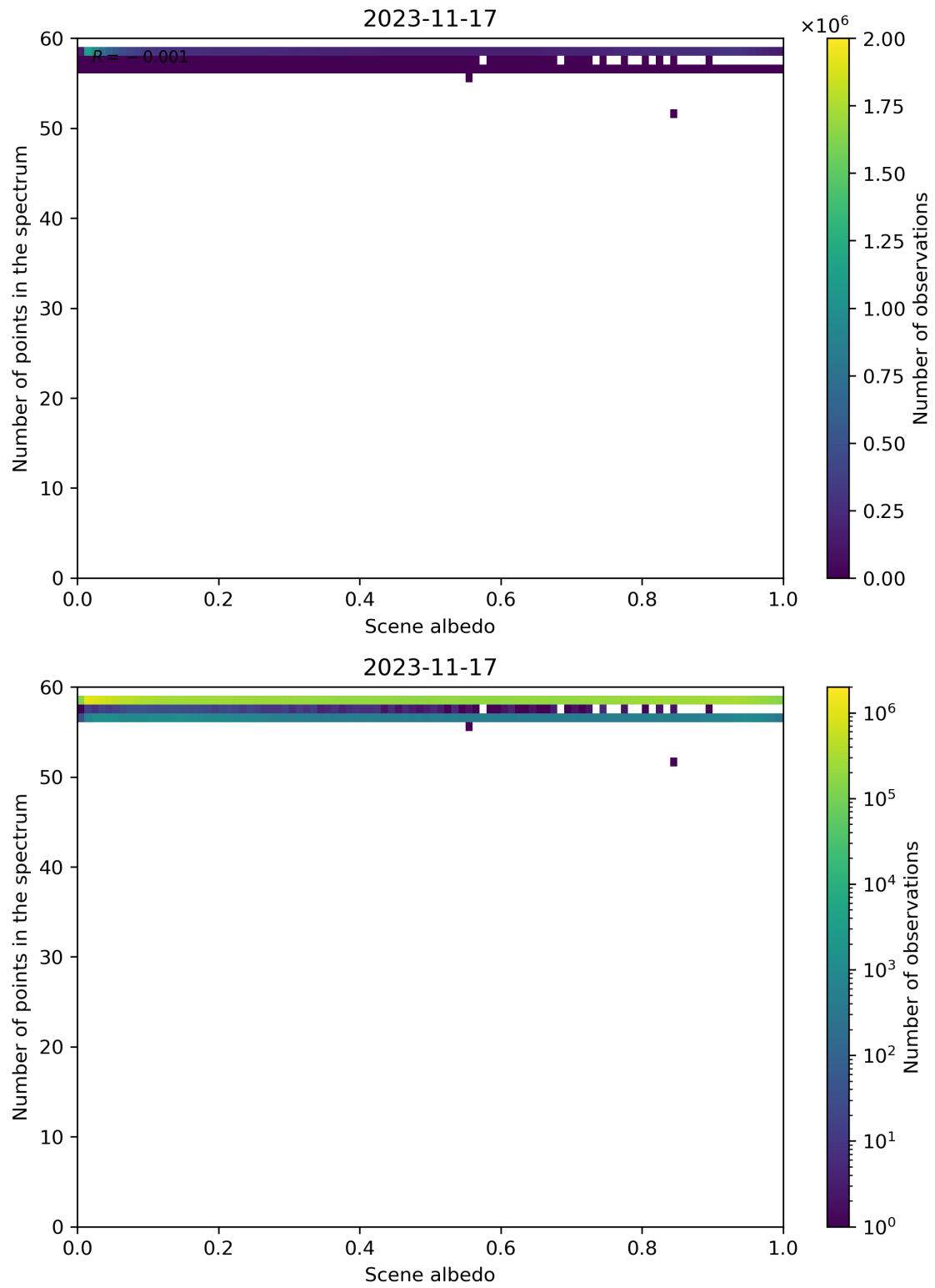
Figure 116: Scatter density plot of “Scene albedo” against “Number of points in the spectrum” for 2023-11-16 to 2023-11-18.
