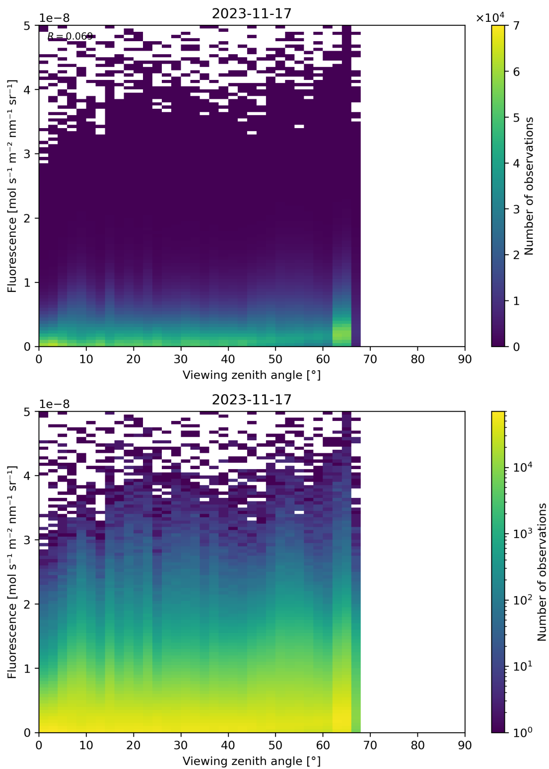
Figure 134: Scatter density plot of “Viewing zenith angle” against “Fluorescence” for 2023-11-16 to 2023-11-18.
