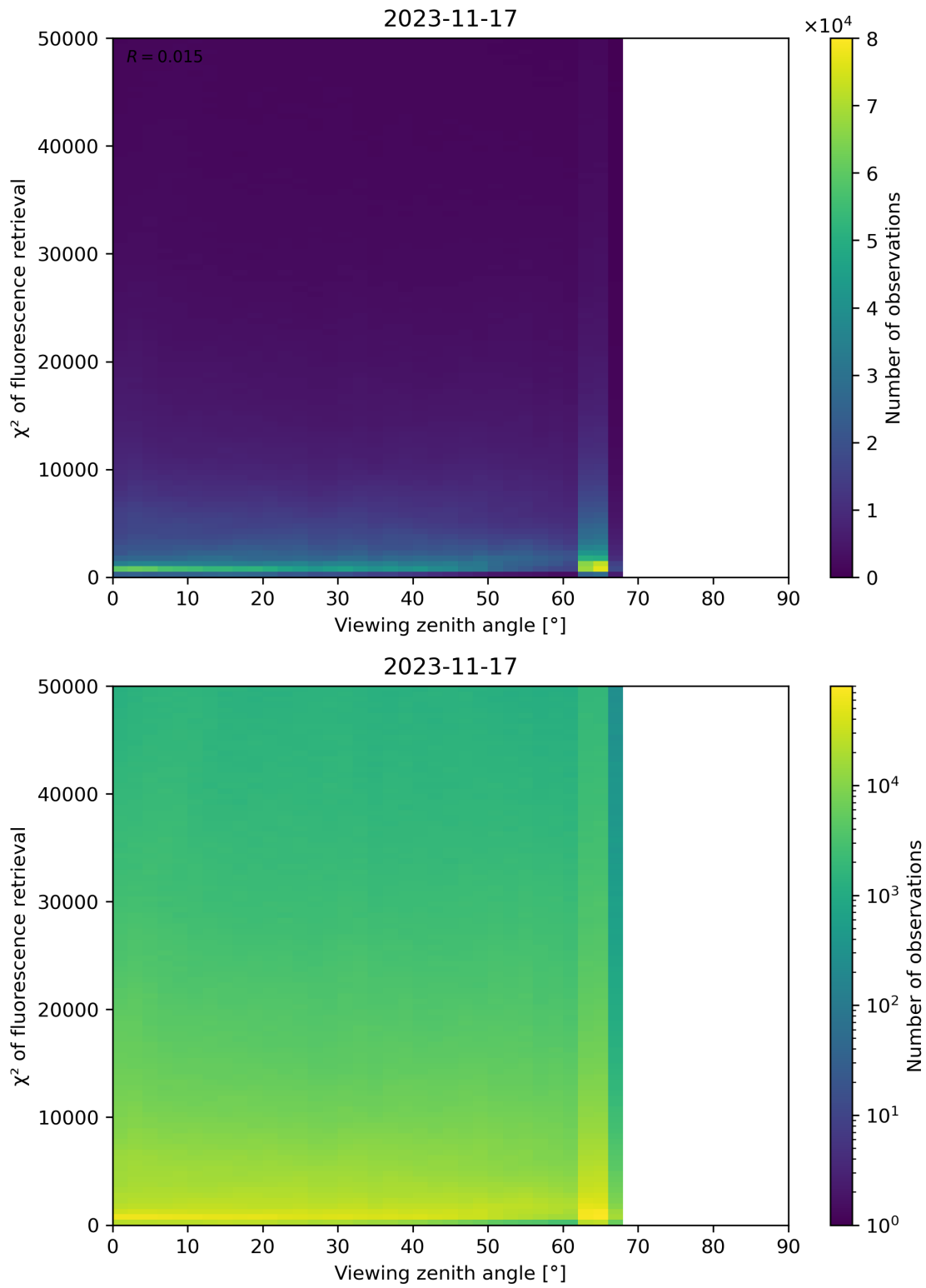
Figure 131: Scatter density plot of “Viewing zenith angle” against “ \chi^2 of fluorescence retrieval” for 2023-11-16 to 2023-11-18.
