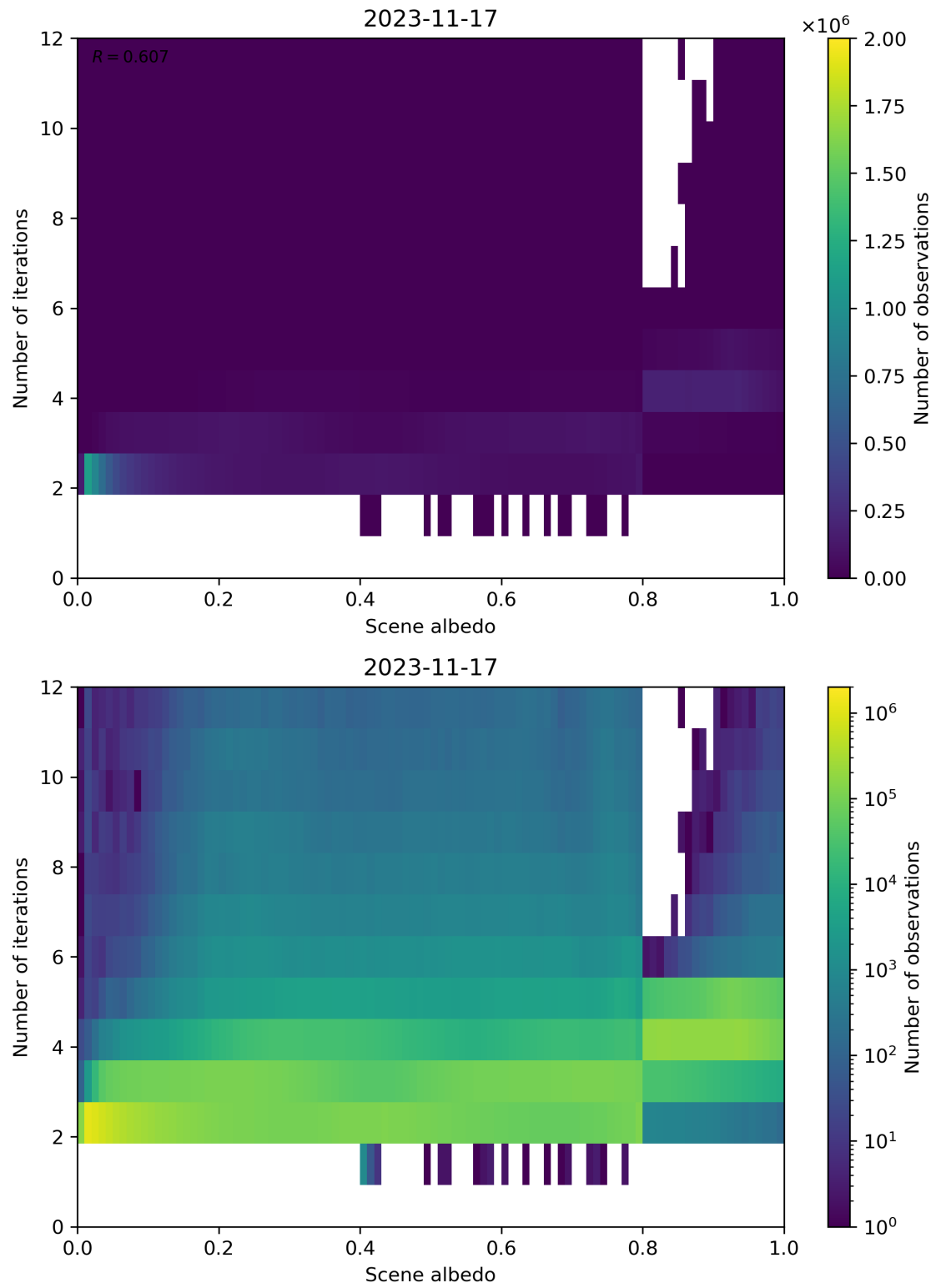
Figure 115: Scatter density plot of “Scene albedo” against “Number of iterations” for 2023-11-16 to 2023-11-18.
