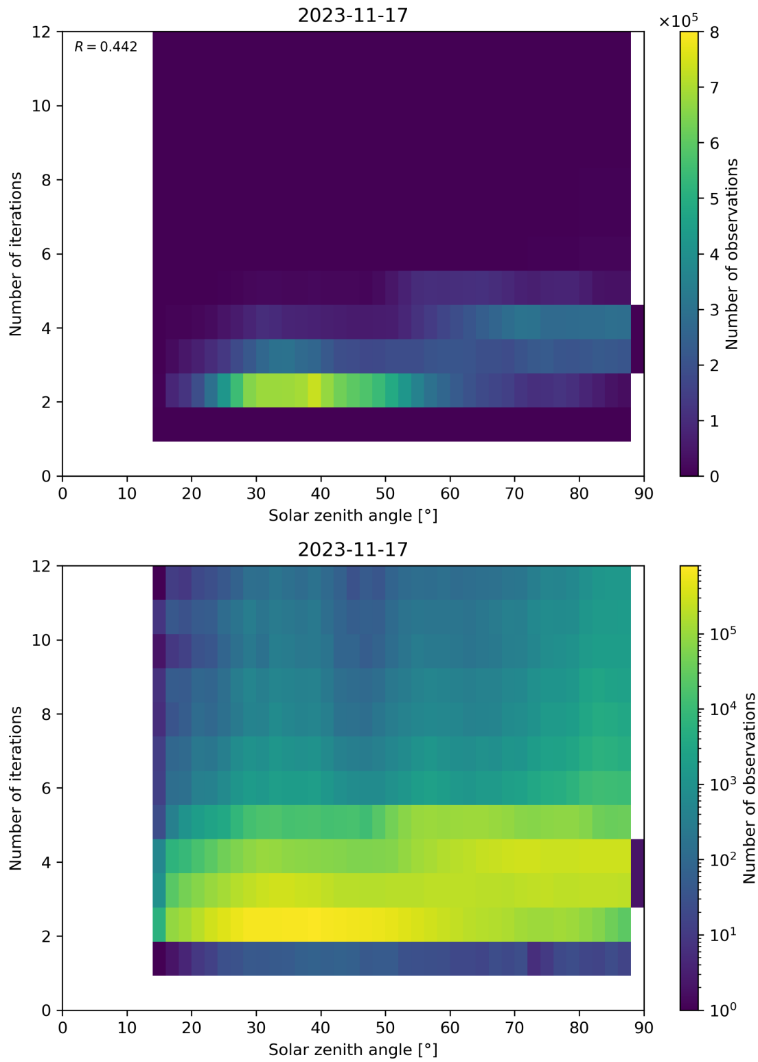
Figure 125: Scatter density plot of “Solar zenith angle” against “Number of iterations” for 2023-11-16 to 2023-11-18.
