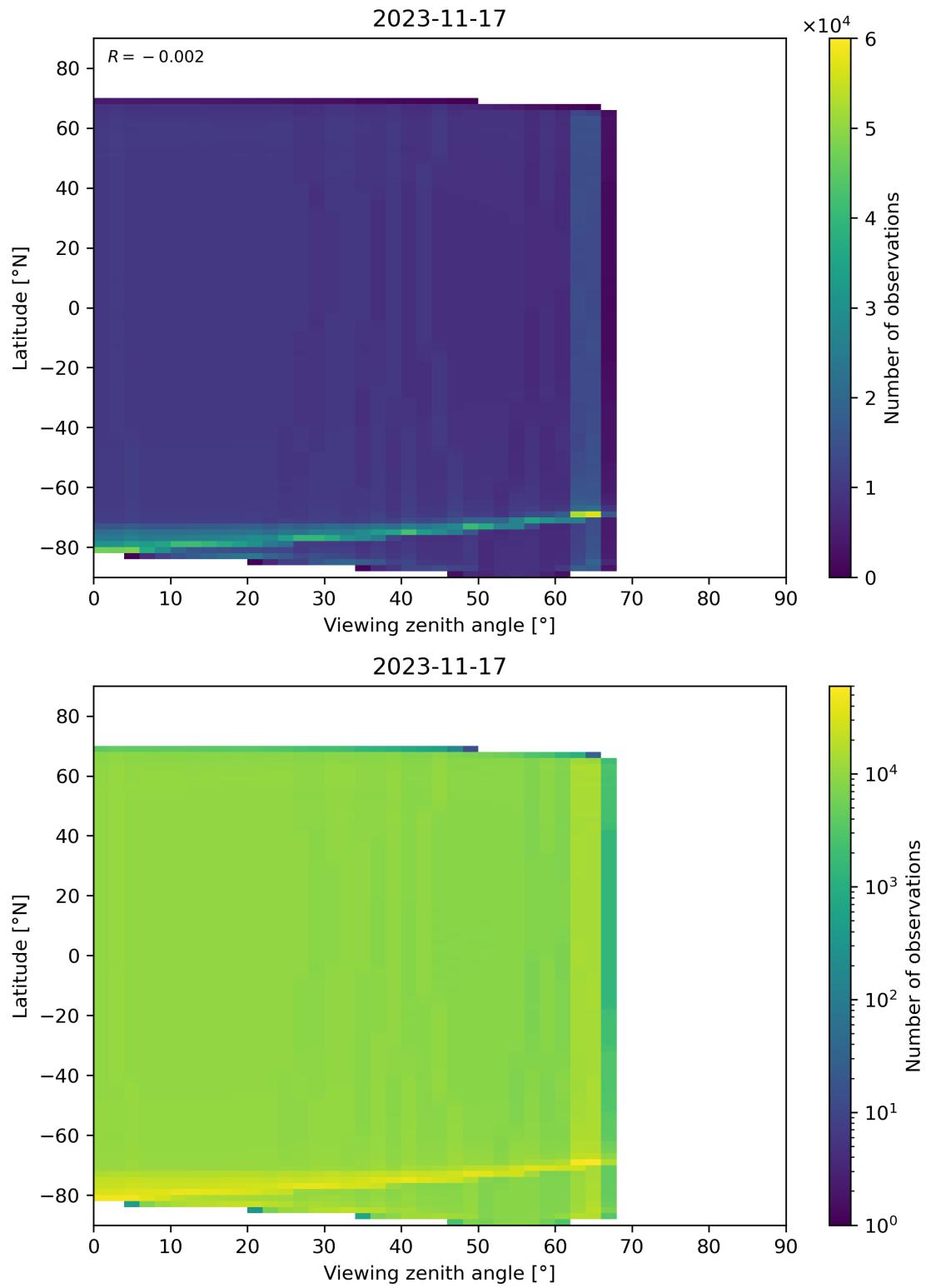
Figure 135: Scatter density plot of “Viewing zenith angle” against “Latitude” for 2023-11-16 to 2023-11-18.
