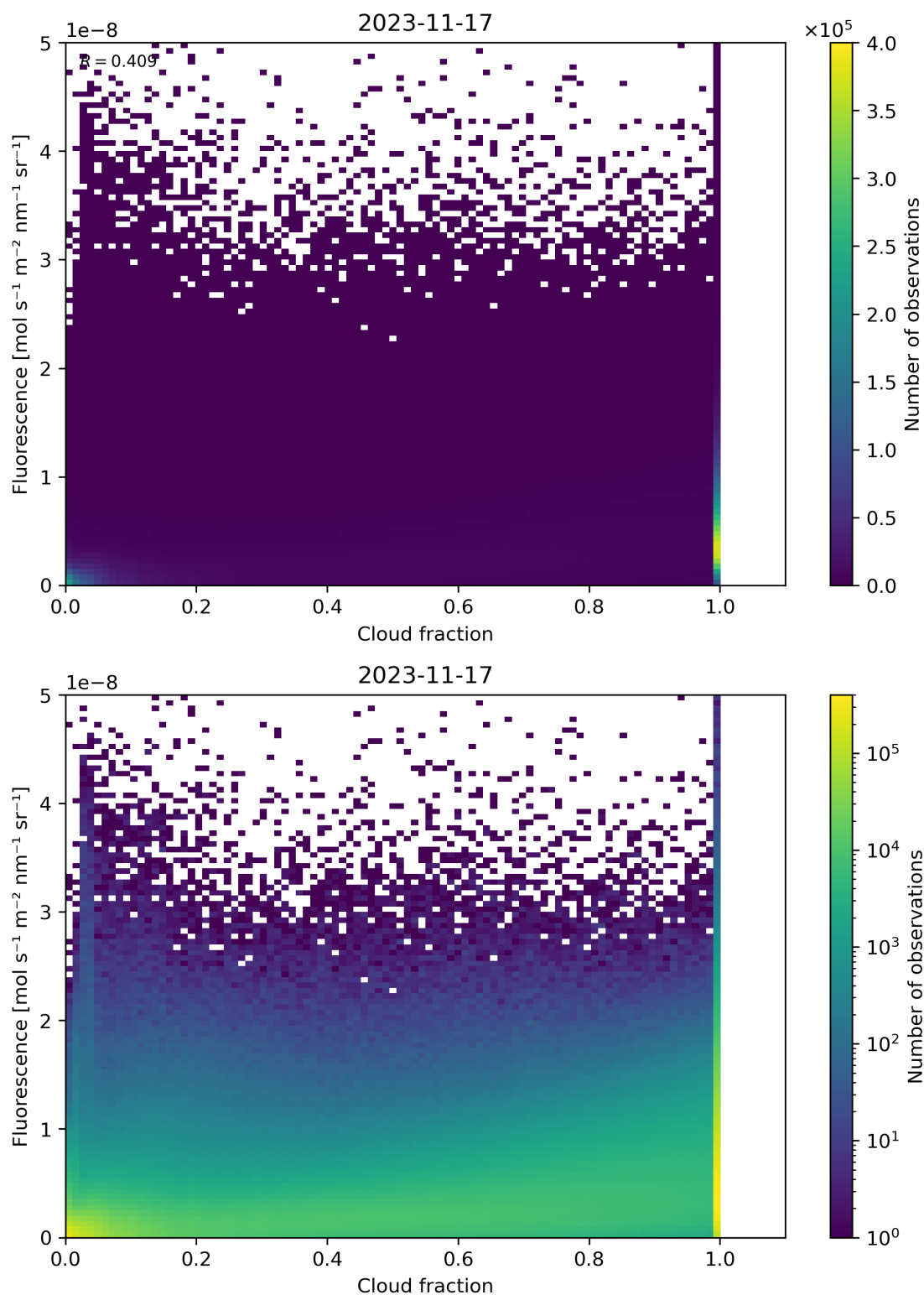
Figure 79: Scatter density plot of “Cloud fraction” against “Fluorescence” for 2023-11-16 to 2023-11-18.
