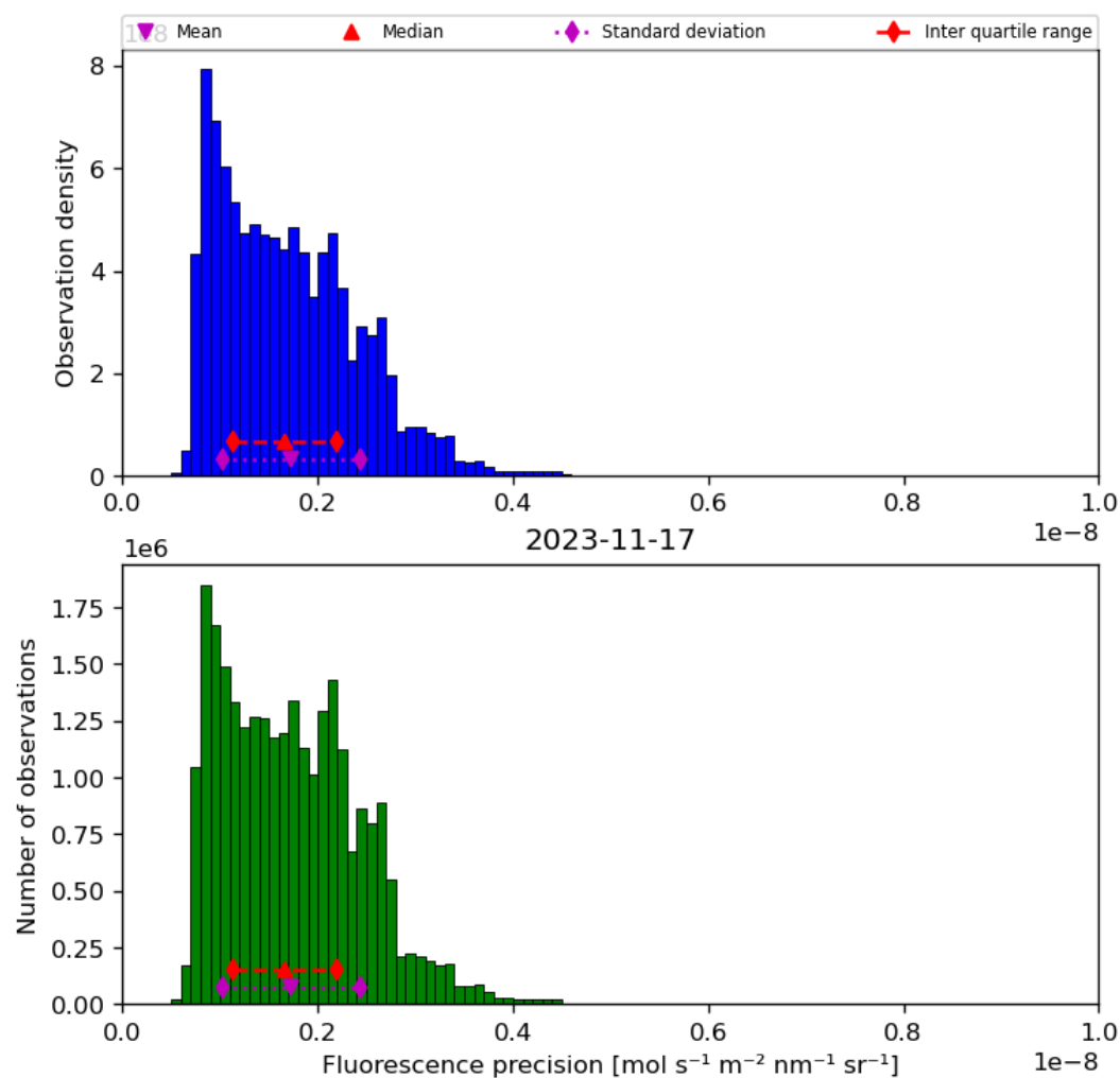
Figure 41: Histogram of “Fluorescence precision” for 2023-11-16 to 2023-11-18
