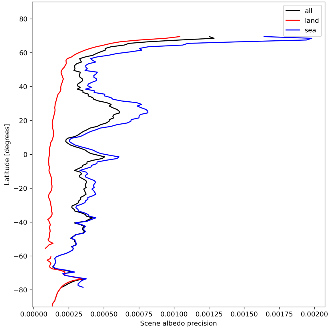
Figure 18: Zonal average of “Scene albedo precision” for 2023-11-16 to 2023-11-18.
