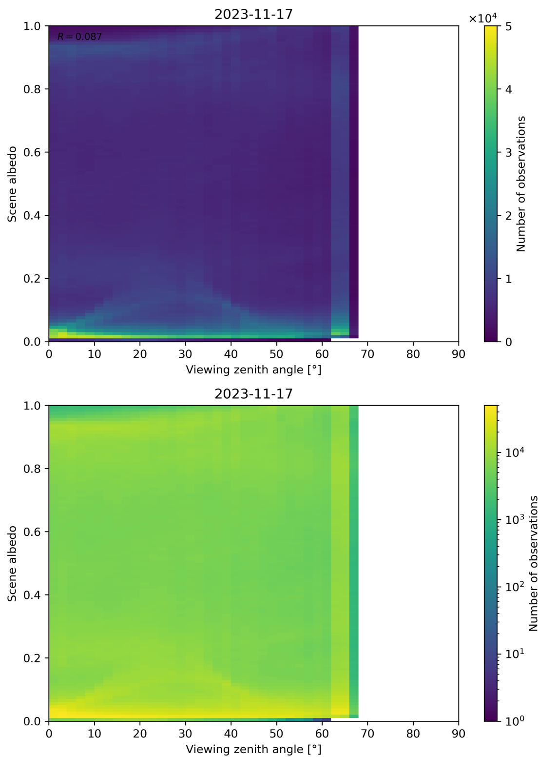
Figure 138: Scatter density plot of “Viewing zenith angle” against “Scene albedo” for 2023-11-16 to 2023-11-18.
