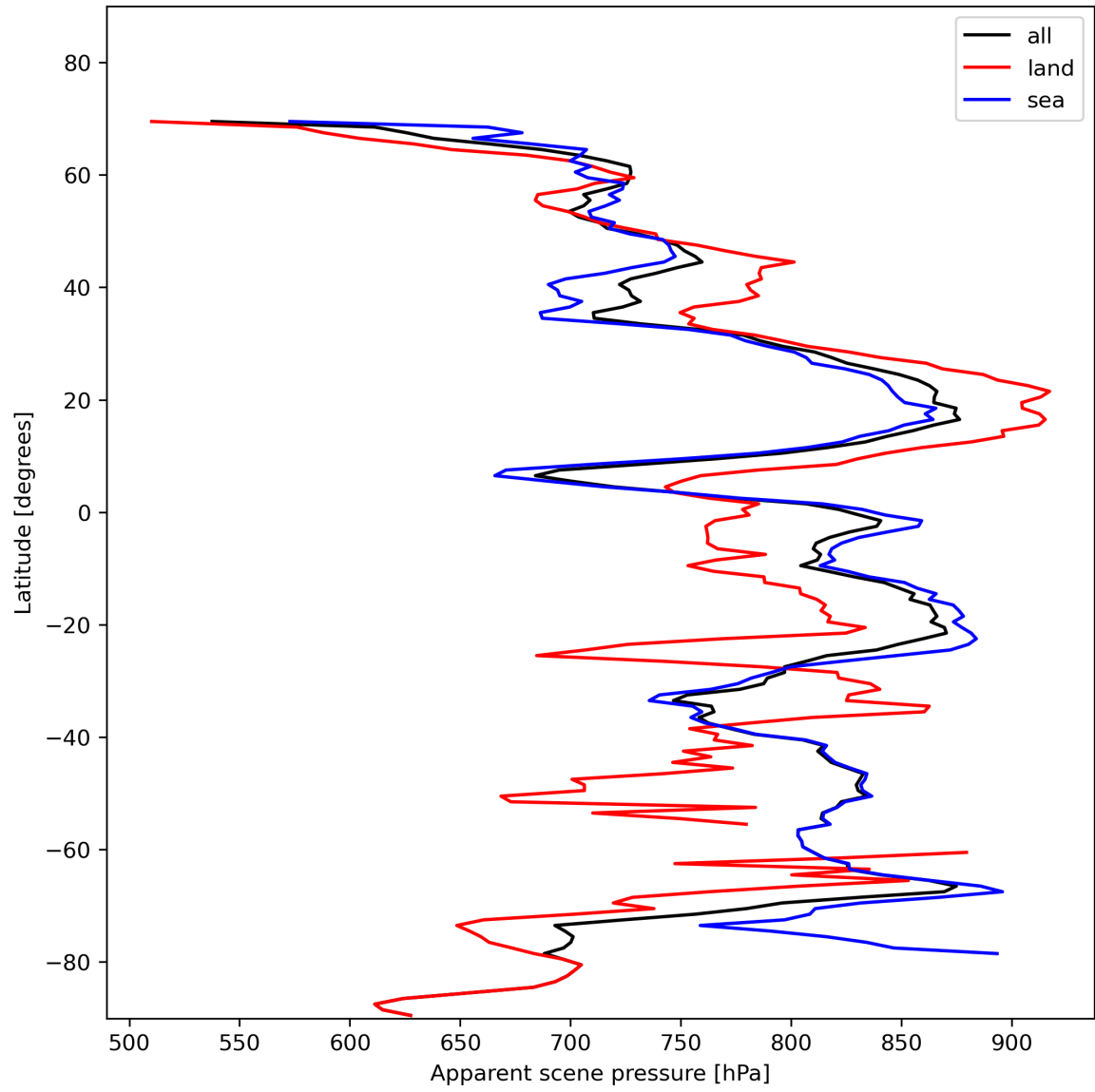
Figure 19: Zonal average of “Apparent scene pressure” for 2023-11-16 to 2023-11-18.
