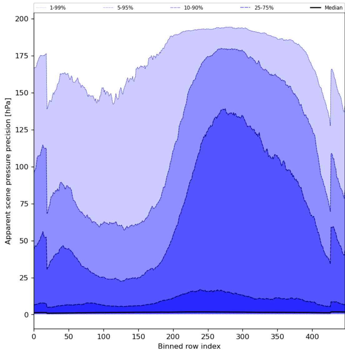
Figure 54: Along track statistics of “Apparent scene pressure precision” for 2023-11-16 to 2023-11-18
