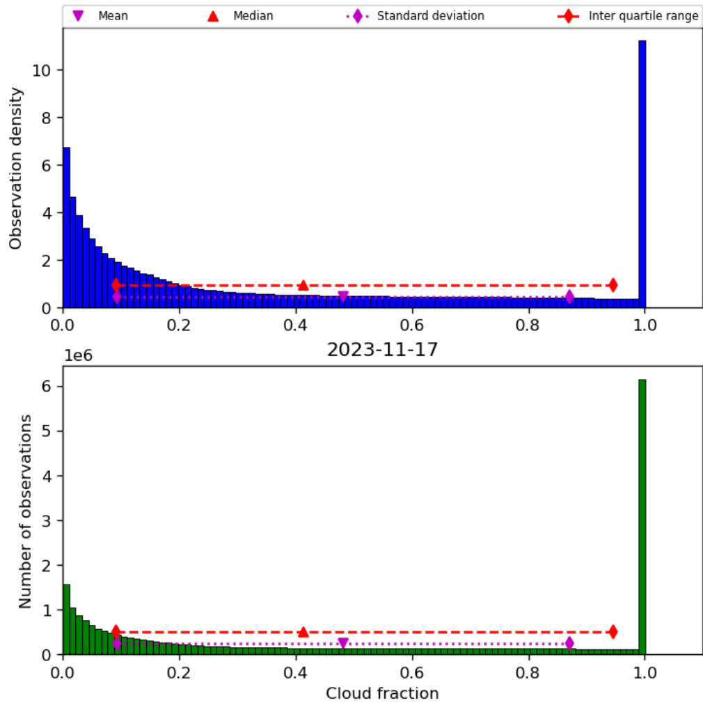
Figure 32: Histogram of “Cloud fraction” for 2023-11-16 to 2023-11-18
