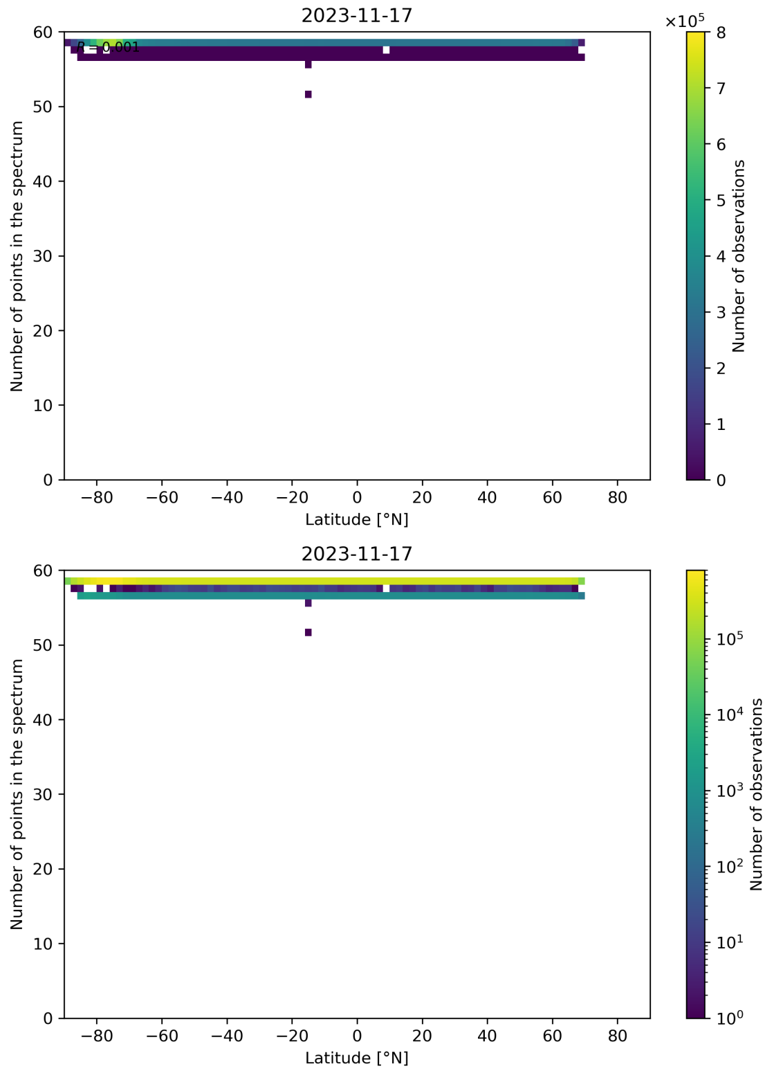
Figure 103: Scatter density plot of “Latitude” against “Number of points in the spectrum” for 2023-11-16 to 2023-11-18.
