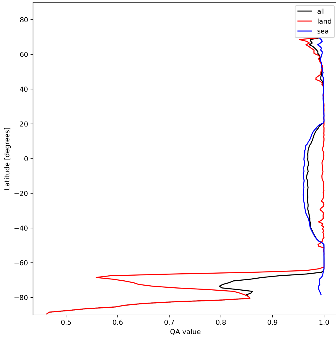
Figure 12: Zonal average of “QA value” for 2023-11-16 to 2023-11-18.
