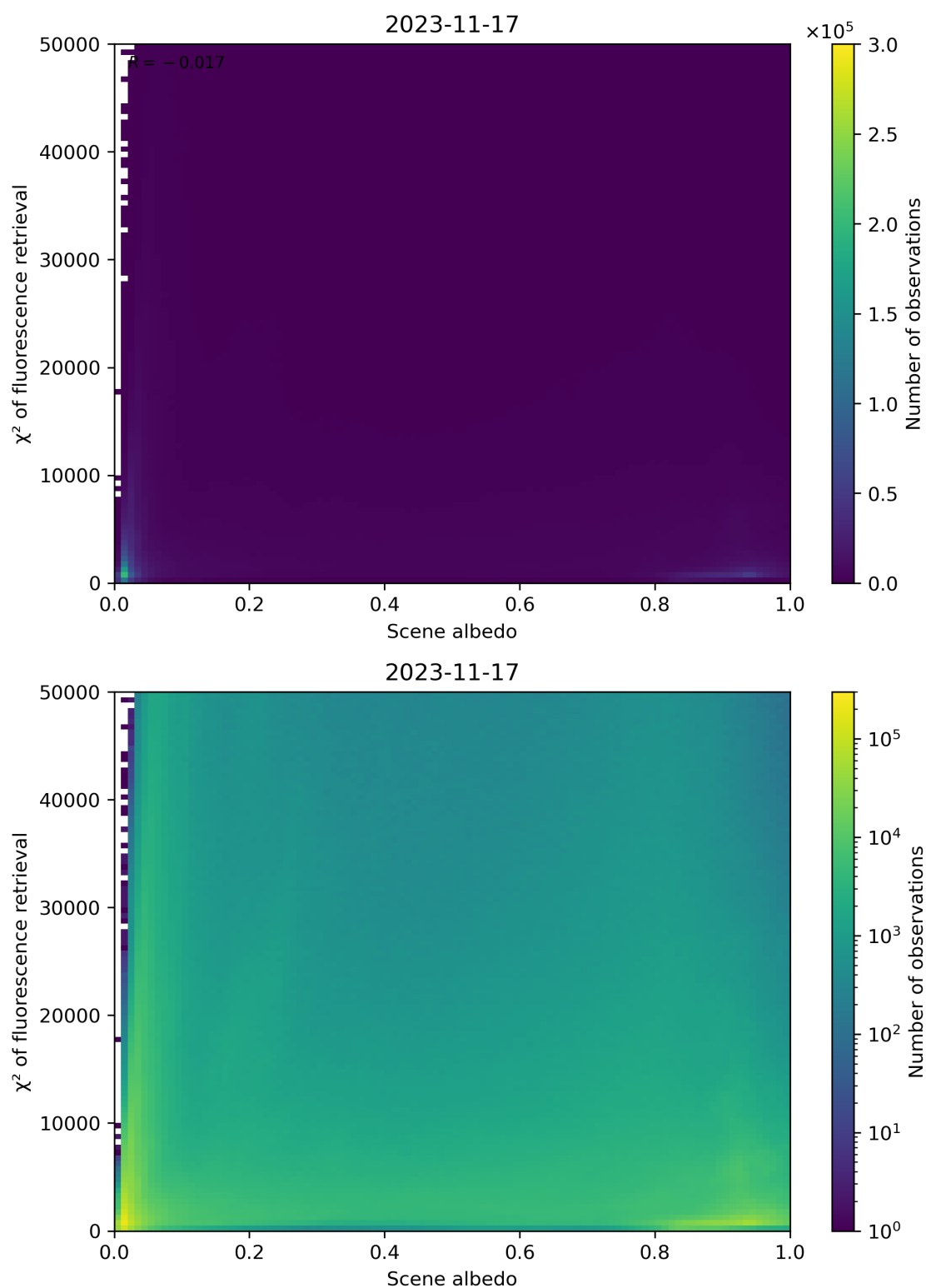
Figure 113: Scatter density plot of “Scene albedo” against “ \chi^2 of fluorescence retrieval” for 2023-11-16 to 2023-11-18.
