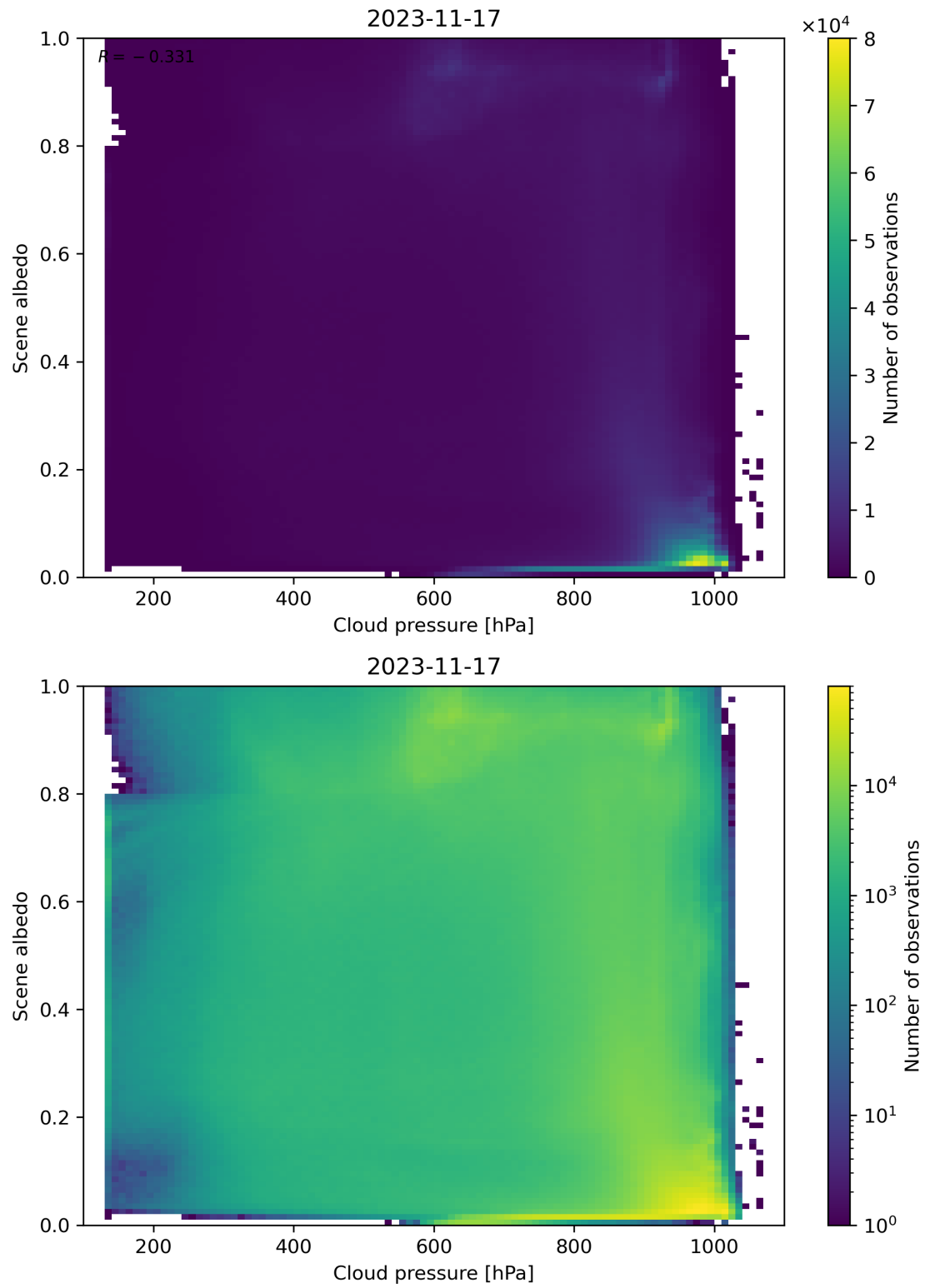
Figure 91: Scatter density plot of “Cloud pressure” against “Scene albedo” for 2023-11-16 to 2023-11-18.
