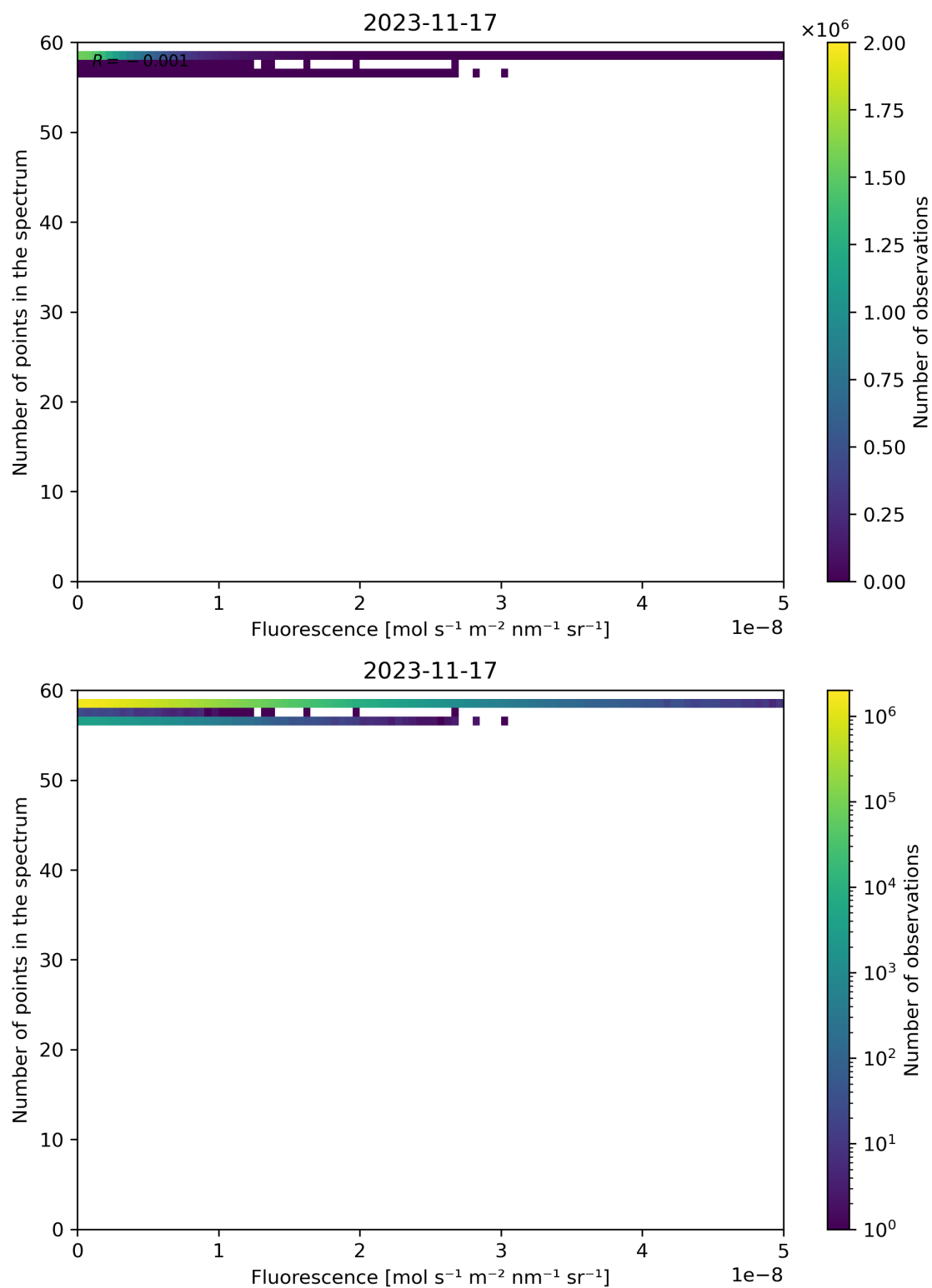
Figure 94: Scatter density plot of “Fluorescence” against “Number of points in the spectrum” for 2023-11-16 to 2023-11-18.
