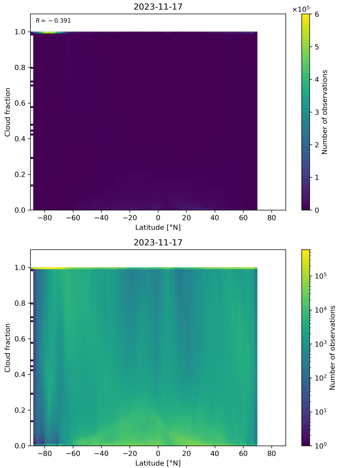
Figure 99: Scatter density plot of “Latitude” against “Cloud fraction” for 2023-11-16 to 2023-11-18.
