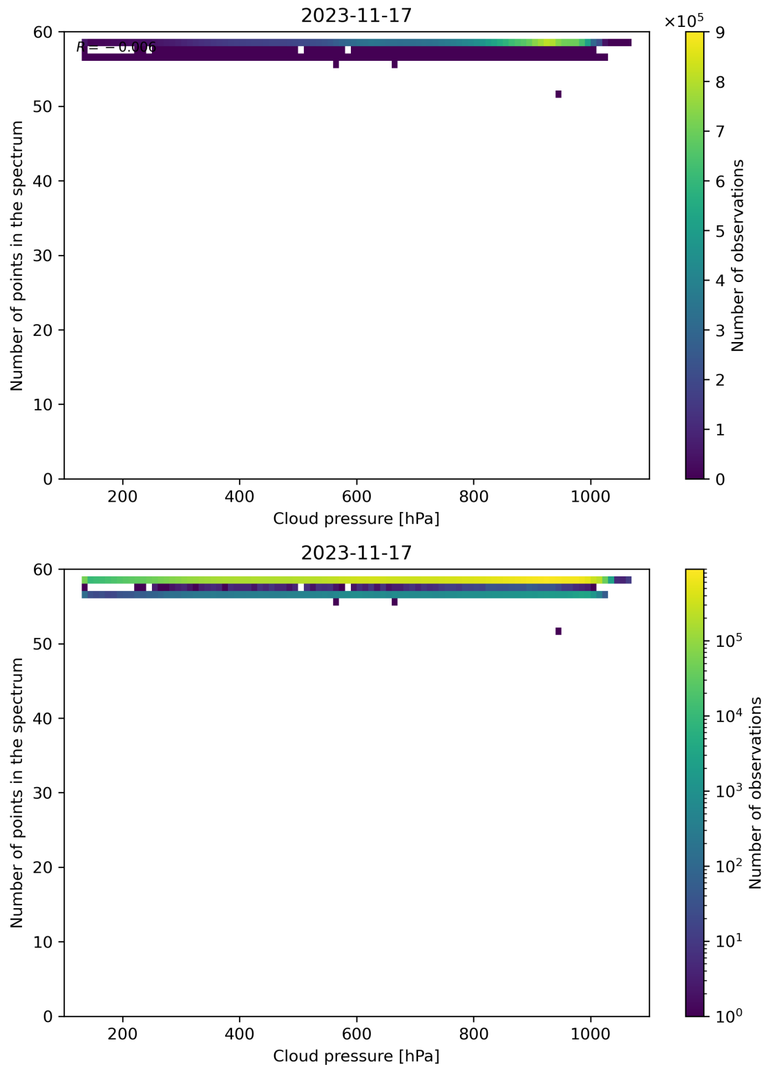
Figure 90: Scatter density plot of “Cloud pressure” against “Number of points in the spectrum” for 2023-11-16 to 2023-11-18.
