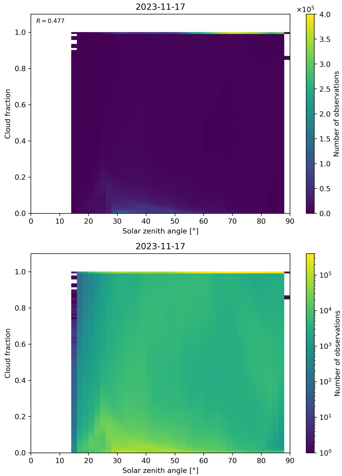
Figure 121: Scatter density plot of “Solar zenith angle” against “Cloud fraction” for 2023-11-16 to 2023-11-18.
