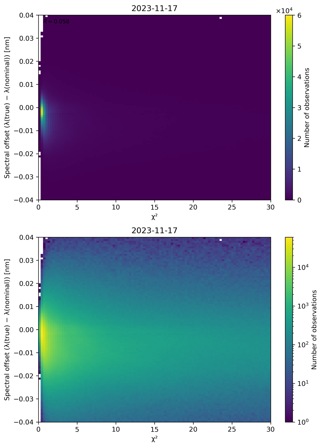
Figure 75: Scatter density plot of " \chi^2 " against "Spectral offset ( \lambda(\text{true}) - \lambda(\text{nominal}) )" for 2023-11-16 to 2023-11-18.
