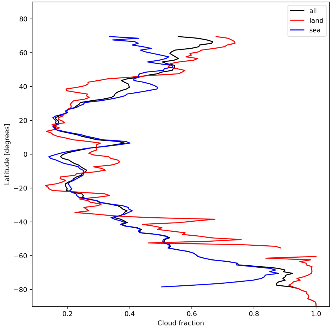
Figure 15: Zonal average of “Cloud fraction” for 2023-11-16 to 2023-11-18.
