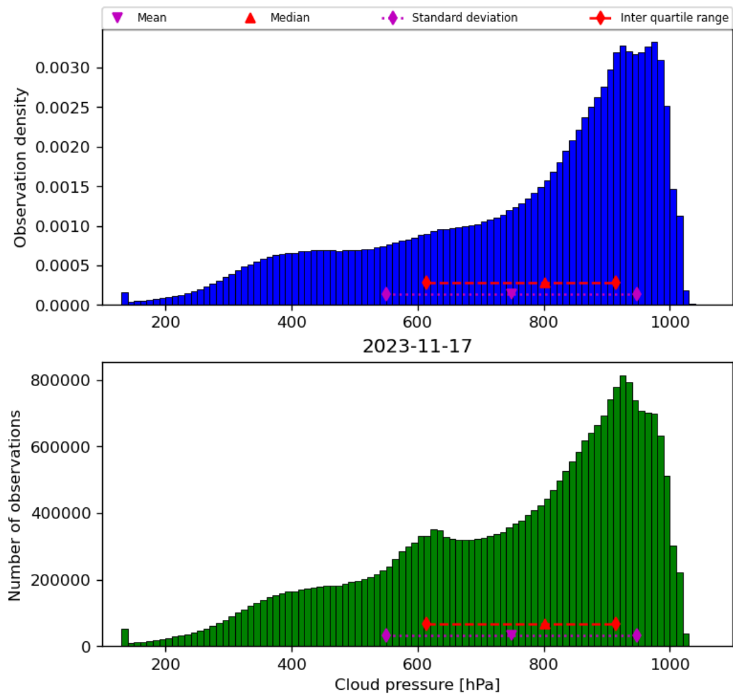
Figure 30: Histogram of “Cloud pressure” for 2023-11-16 to 2023-11-18
