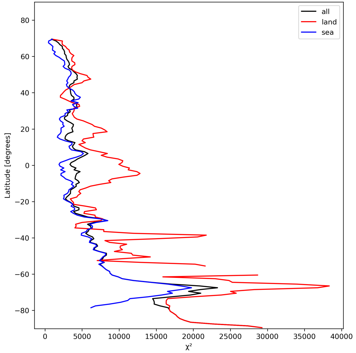
Figure 21: Zonal average of “ \chi^2 ” for 2023-11-16 to 2023-11-18.
