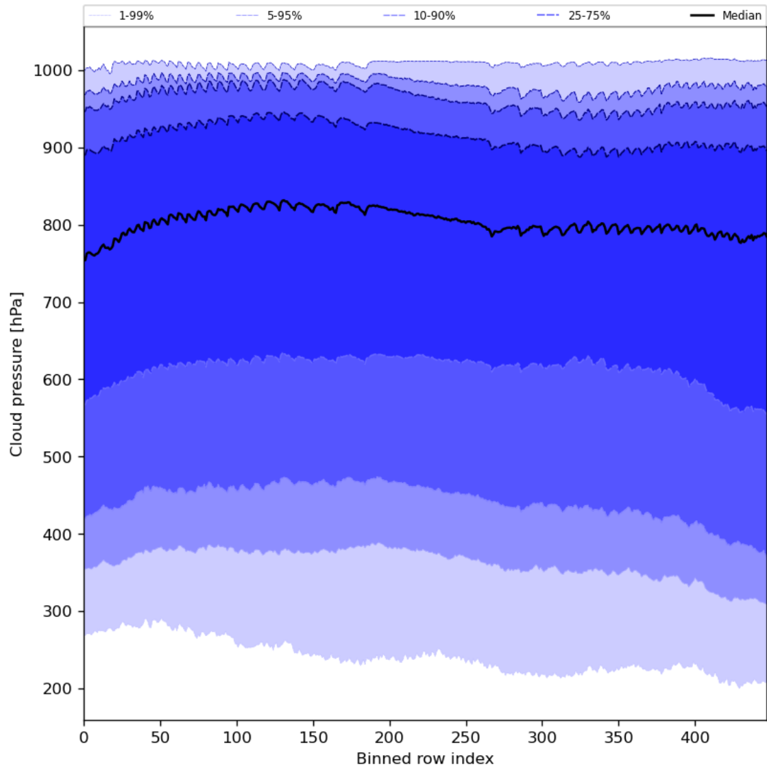
Figure 47: Along track statistics of “Cloud pressure” for 2023-11-16 to 2023-11-18
