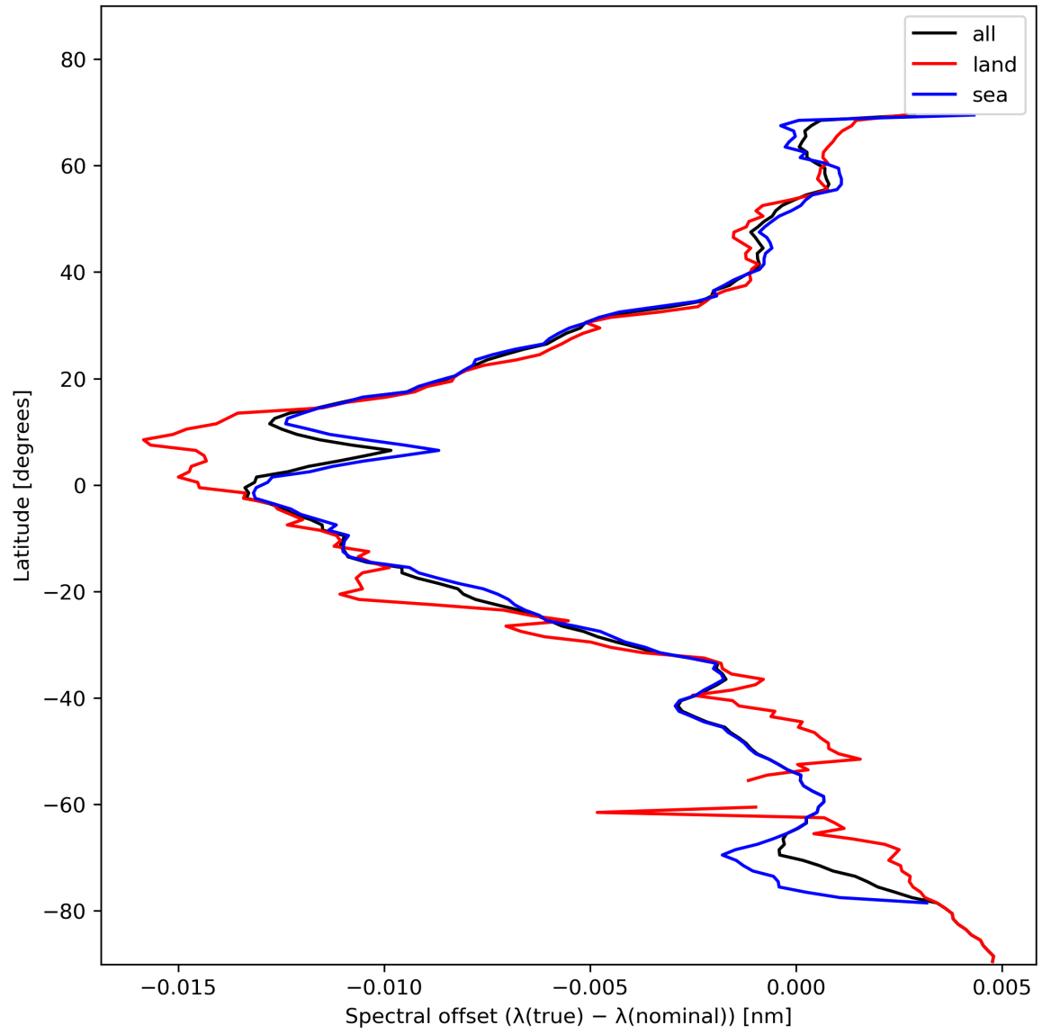
Figure 28: Zonal average of “Spectral offset ( \lambda(\text{true}) - \lambda(\text{nominal}) )” for 2023-11-16 to 2023-11-18.
