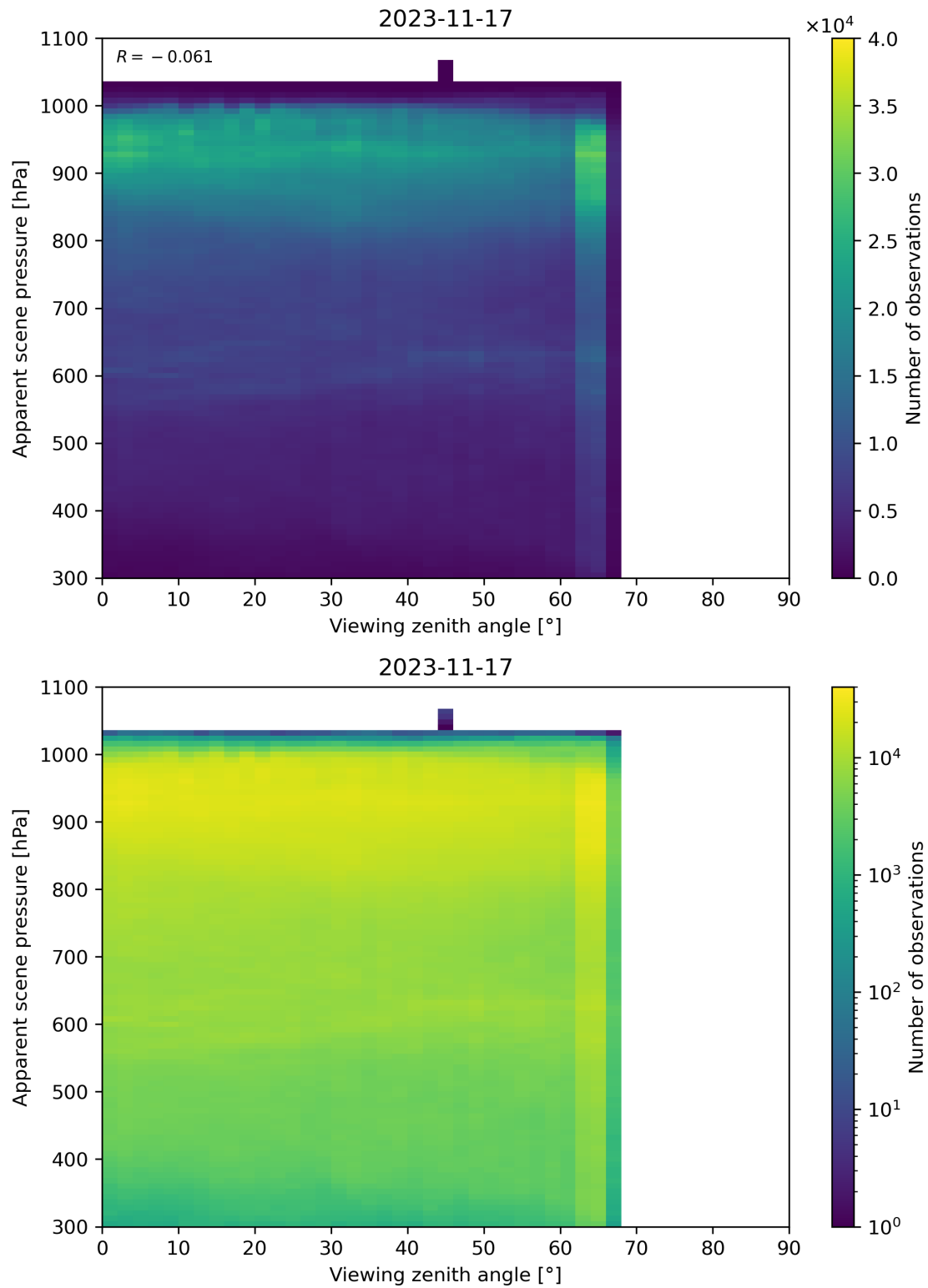
Figure 129: Scatter density plot of “Viewing zenith angle” against “Apparent scene pressure” for 2023-11-16 to 2023-11-18.
