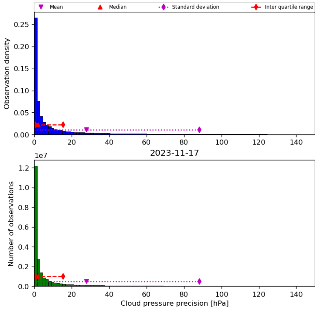
Figure 31: Histogram of “Cloud pressure precision” for 2023-11-16 to 2023-11-18
