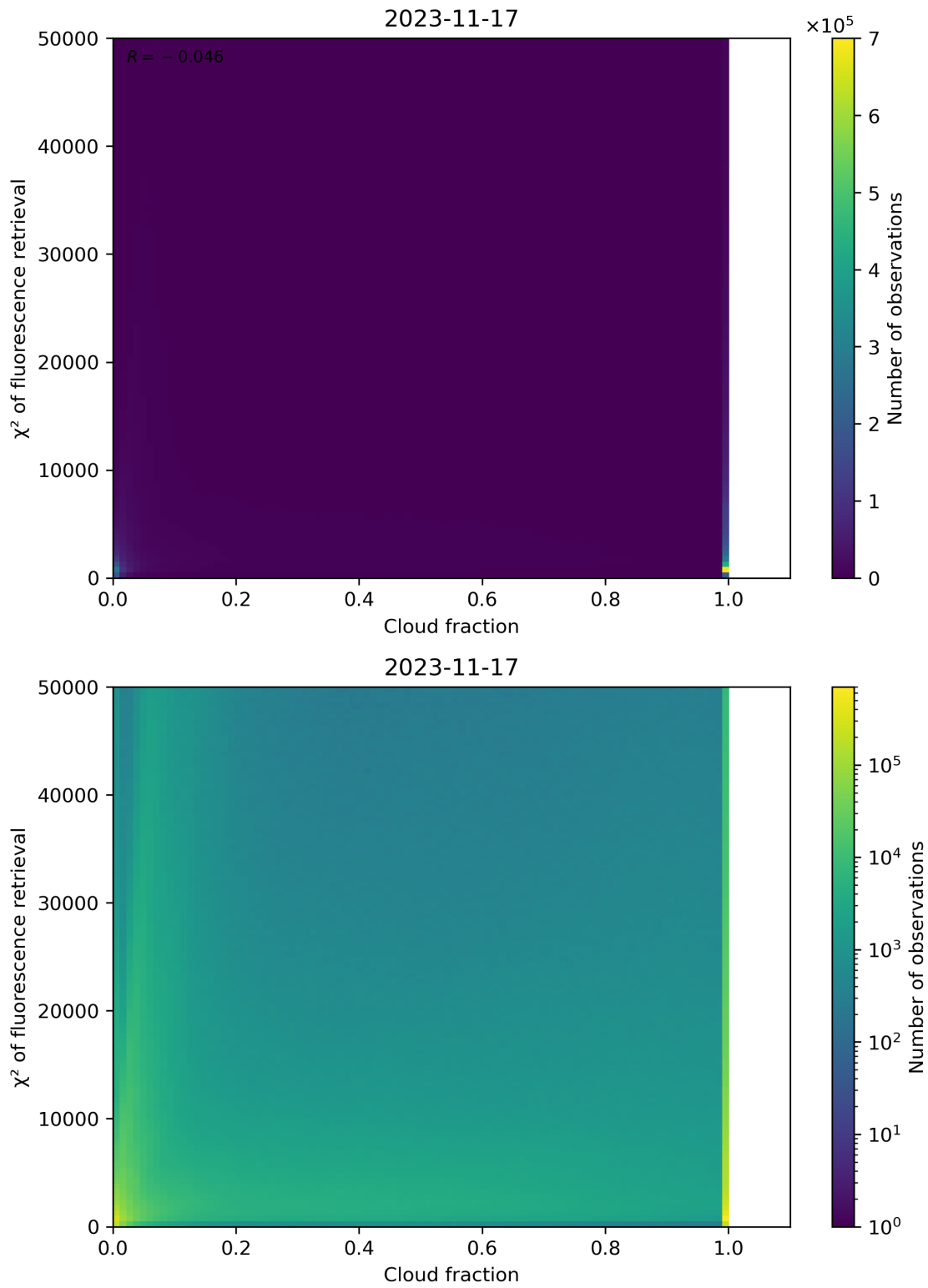
Figure 78: Scatter density plot of “Cloud fraction” against “ \chi^2 of fluorescence retrieval” for 2023-11-16 to 2023-11-18.
