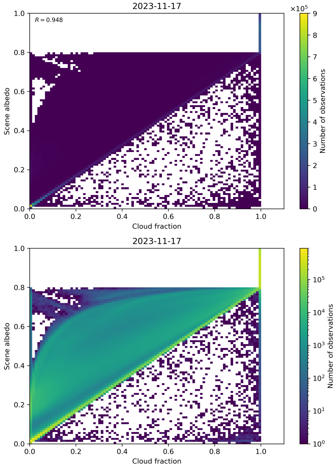
Figure 82: Scatter density plot of “Cloud fraction” against “Scene albedo” for 2023-11-16 to 2023-11-18.
