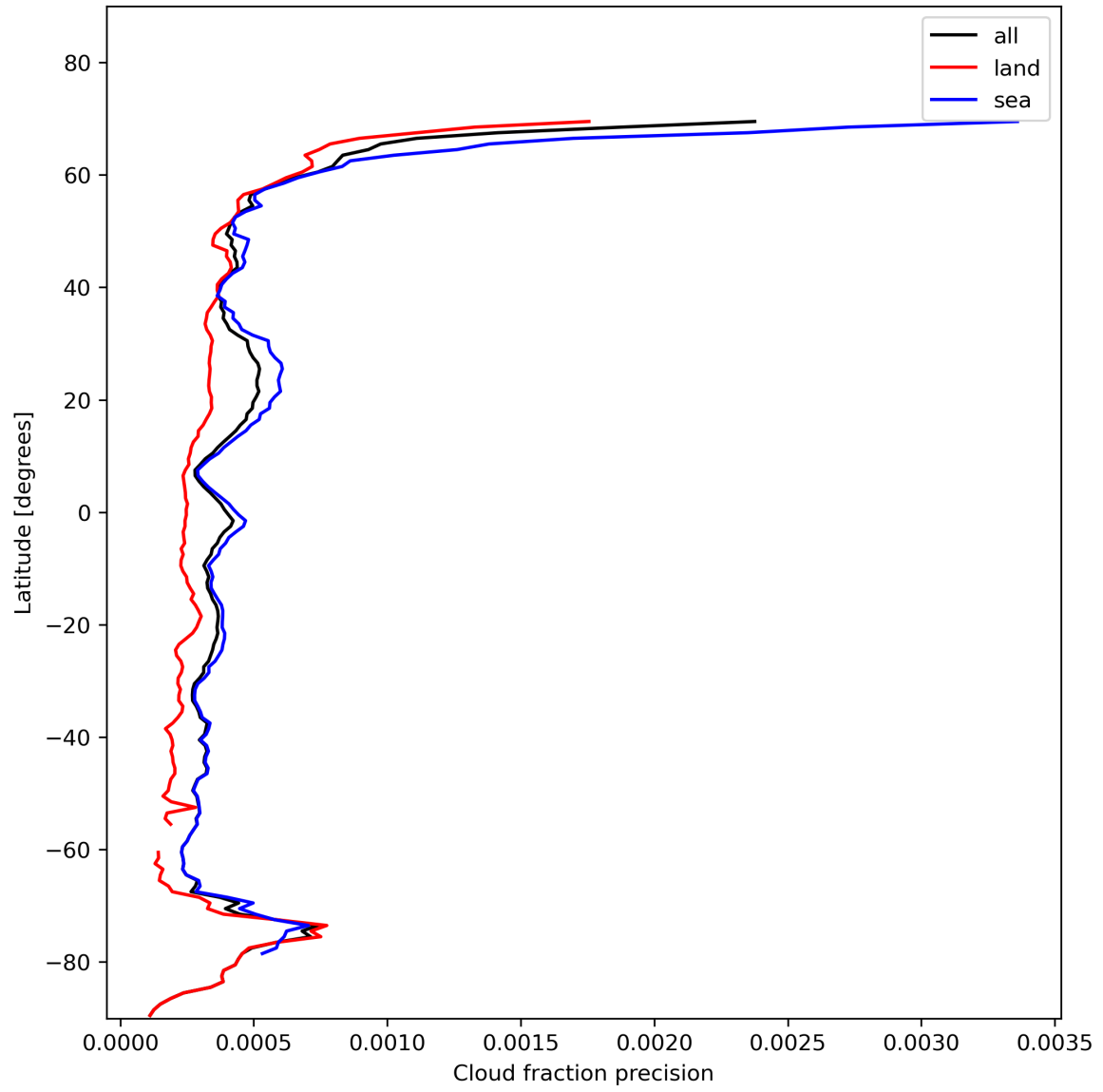
Figure 16: Zonal average of “Cloud fraction precision” for 2023-11-16 to 2023-11-18.
