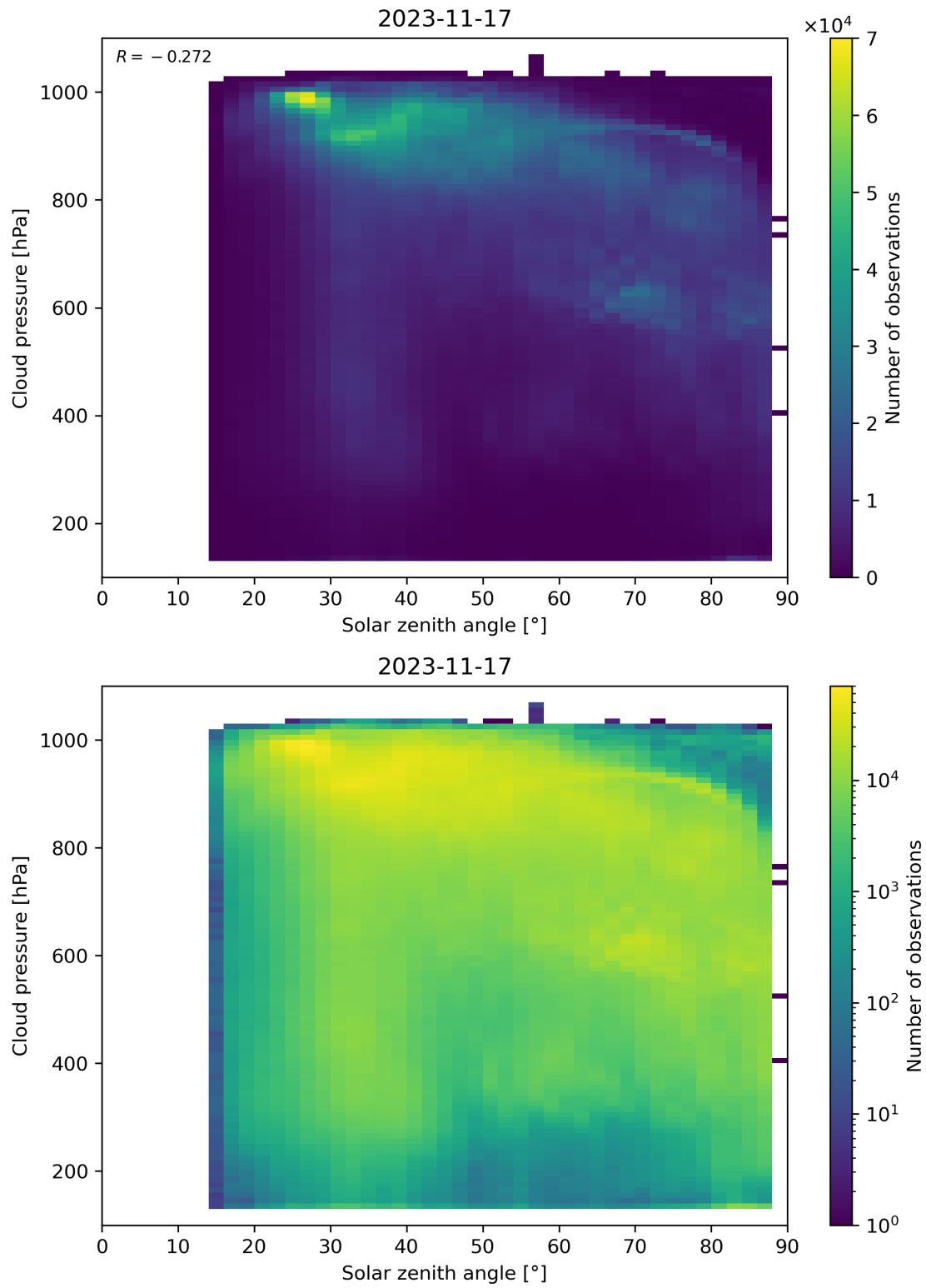
Figure 122: Scatter density plot of “Solar zenith angle” against “Cloud pressure” for 2023-11-16 to 2023-11-18.
