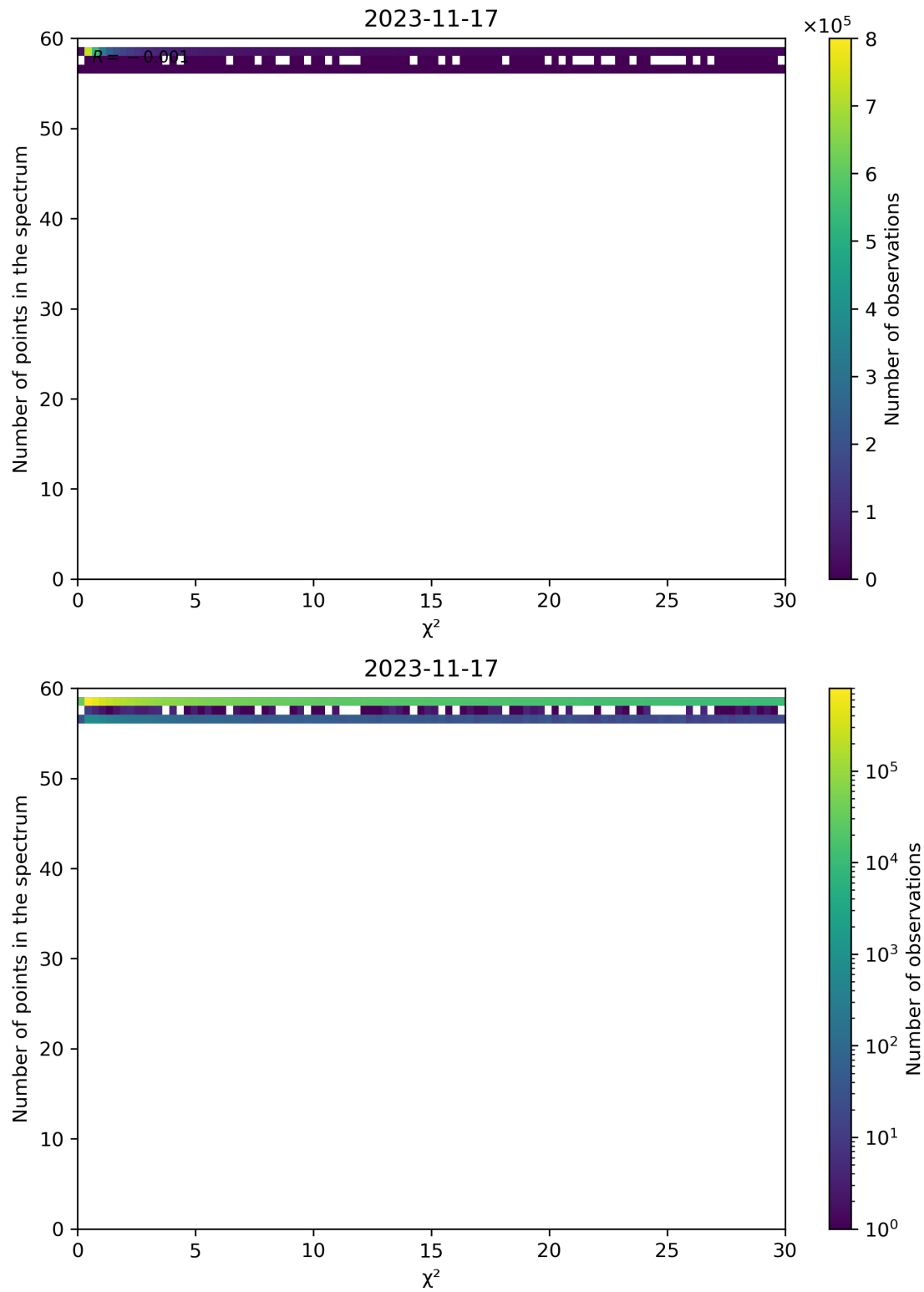
Figure 74: Scatter density plot of " \chi^2 " against "Number of points in the spectrum" for 2023-11-16 to 2023-11-18.
