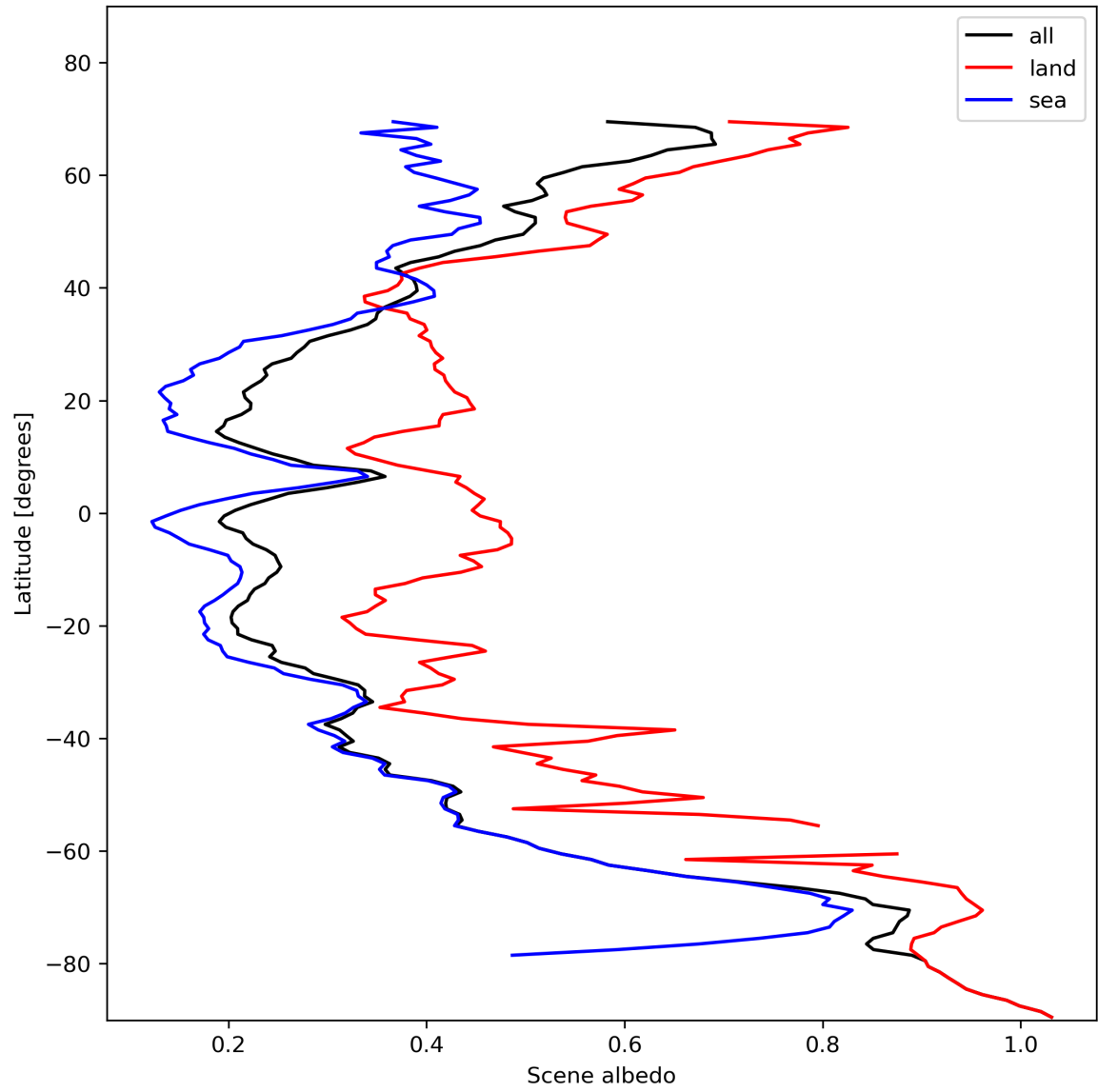
Figure 17: Zonal average of “Scene albedo” for 2023-11-16 to 2023-11-18.
