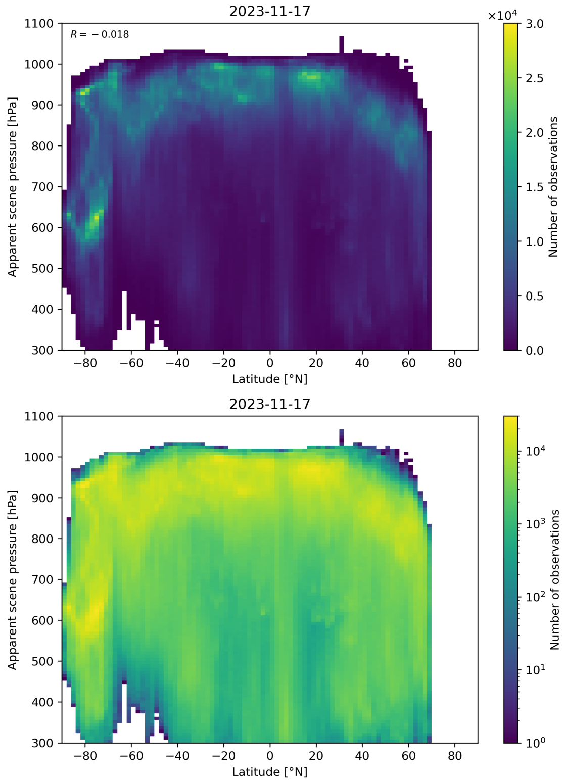
Figure 96: Scatter density plot of “Latitude” against “Apparent scene pressure” for 2023-11-16 to 2023-11-18.
