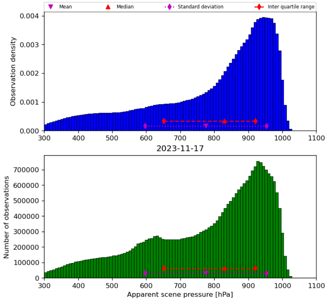
Figure 36: Histogram of “Apparent scene pressure” for 2023-11-16 to 2023-11-18
