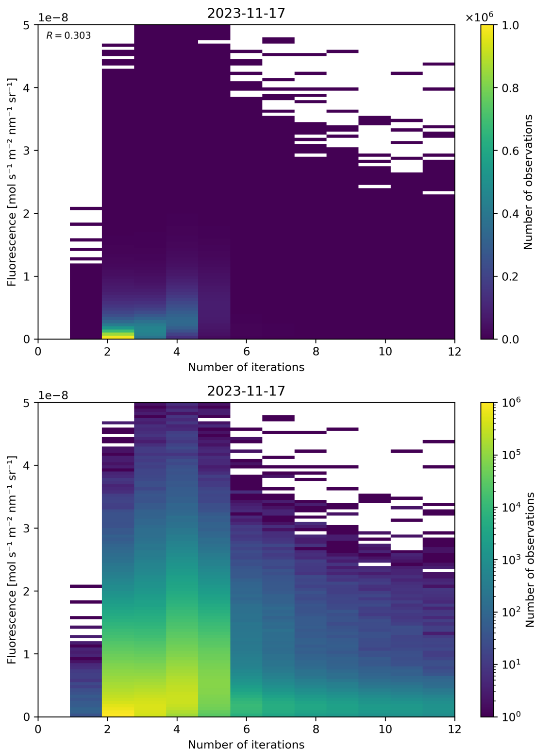
Figure 107: Scatter density plot of “Number of iterations” against “Fluorescence” for 2023-11-16 to 2023-11-18.
