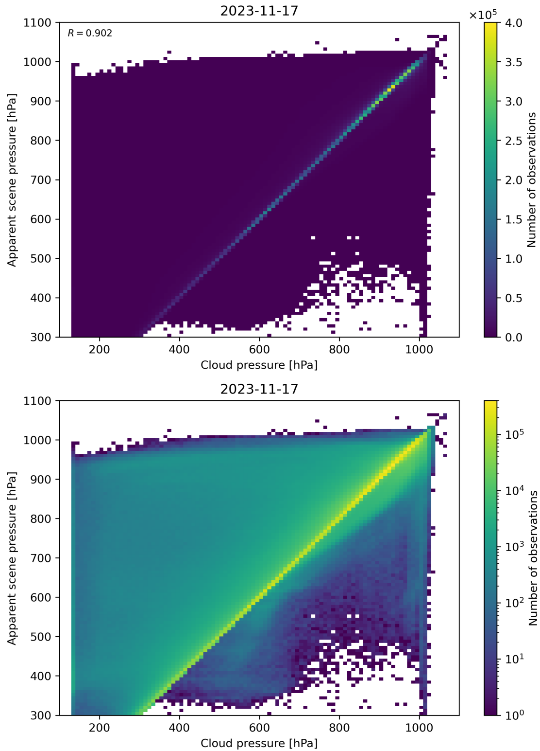
Figure 84: Scatter density plot of “Cloud pressure” against “Apparent scene pressure” for 2023-11-16 to 2023-11-18.
