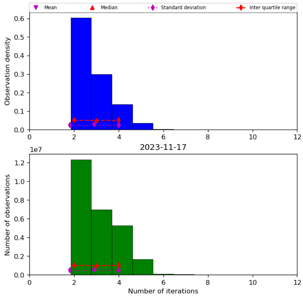
Figure 39: Histogram of “Number of iterations” for 2023-11-16 to 2023-11-18
