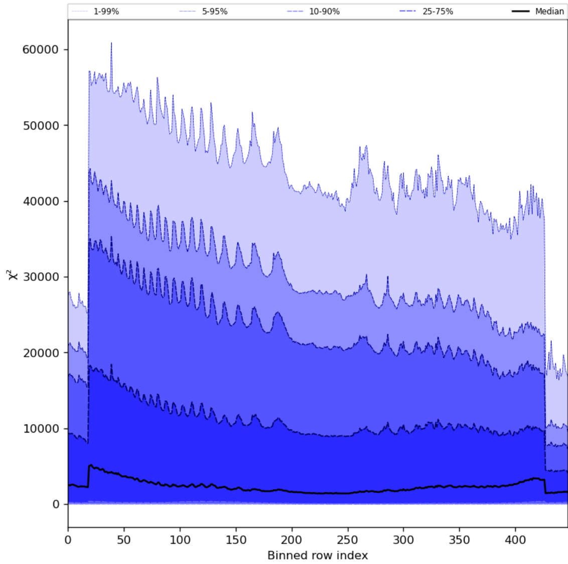
Figure 55: Along track statistics of “ \chi^2 ” for 2023-11-16 to 2023-11-18
