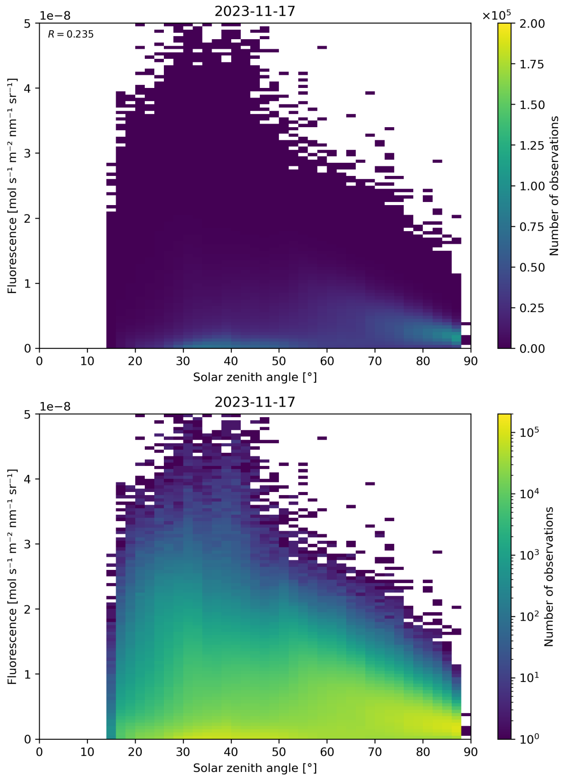
Figure 123: Scatter density plot of “Solar zenith angle” against “Fluorescence” for 2023-11-16 to 2023-11-18.
