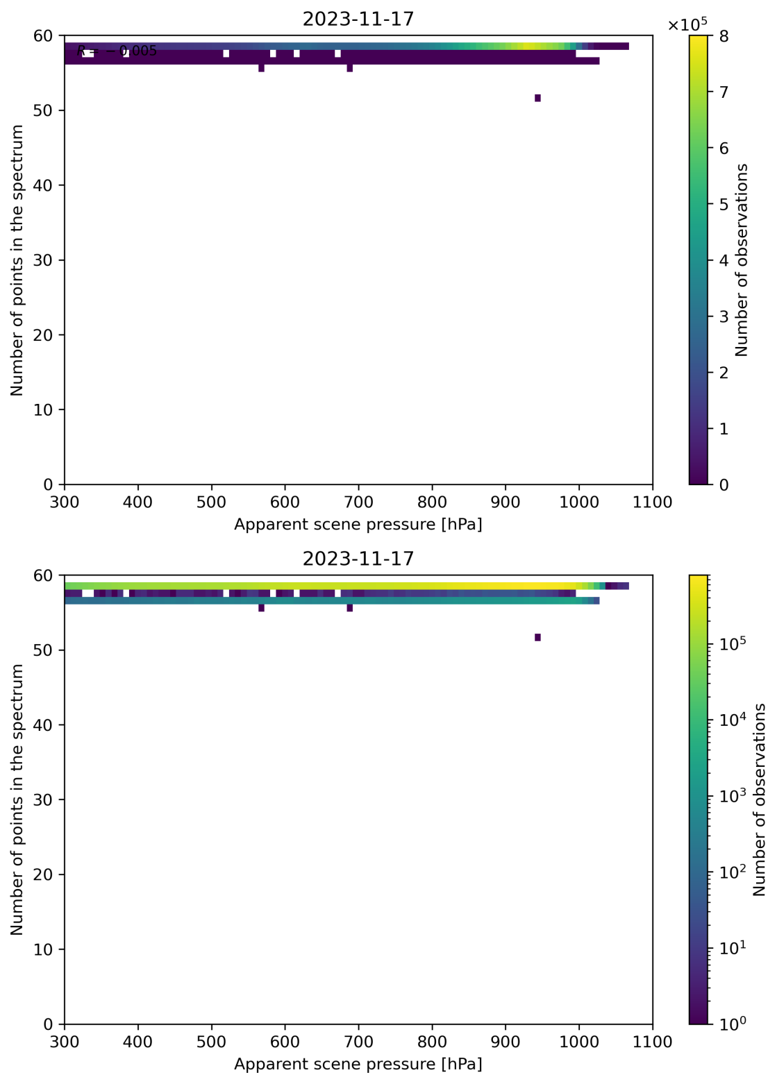
Figure 67: Scatter density plot of “Apparent scene pressure” against “Number of points in the spectrum” for 2023-11-16 to 2023-11-18.
