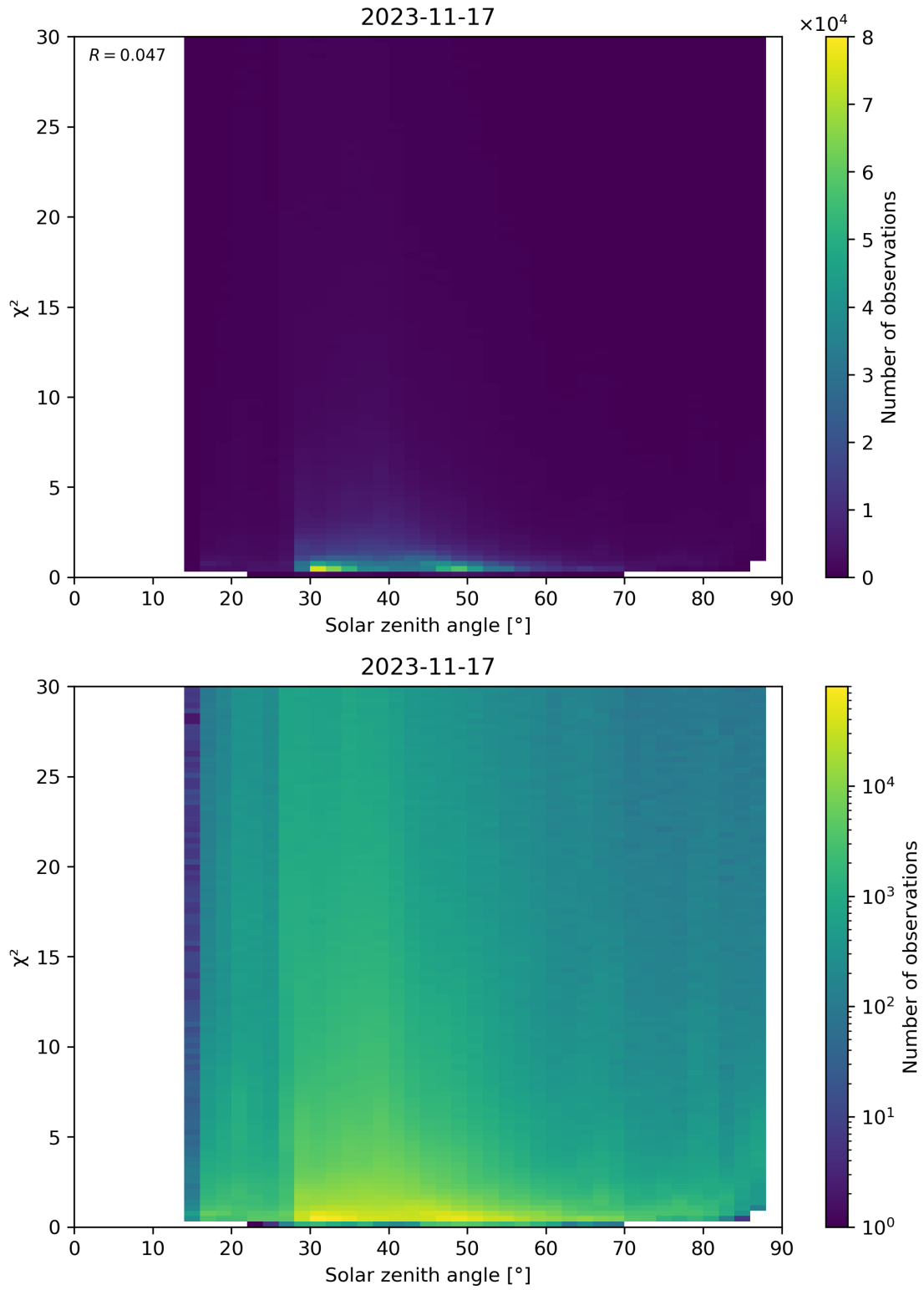
Figure 119: Scatter density plot of “Solar zenith angle” against “ \chi^2 ” for 2023-11-16 to 2023-11-18.
