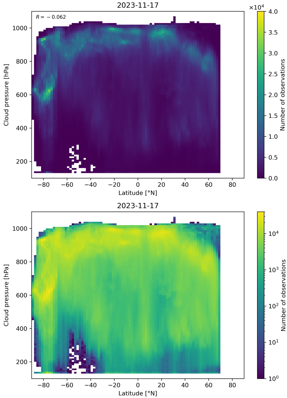
Figure 100: Scatter density plot of “Latitude” against “Cloud pressure” for 2023-11-16 to 2023-11-18.
