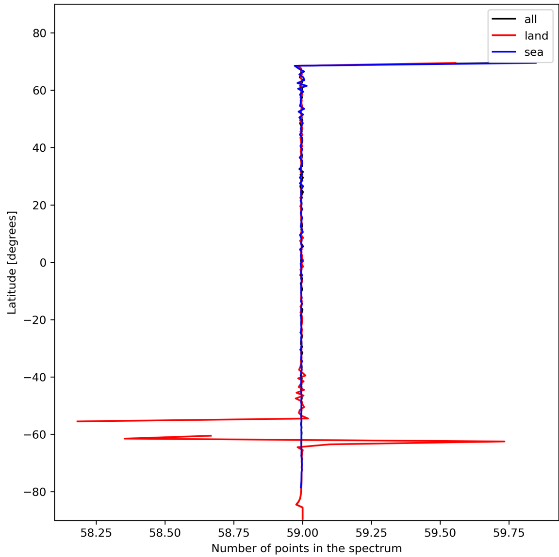
Figure 27: Zonal average of “Number of points in the spectrum” for 2023-11-16 to 2023-11-18.
