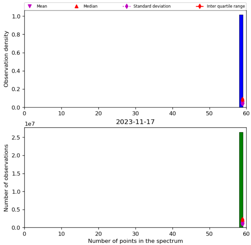
Figure 44: Histogram of “Number of points in the spectrum” for 2023-11-16 to 2023-11-18
