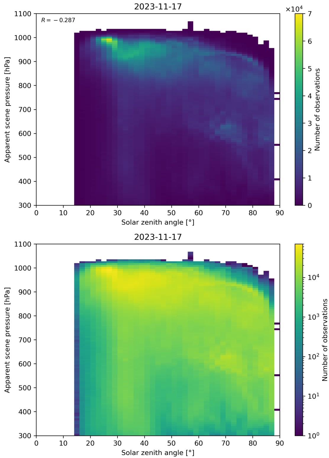
Figure 118: Scatter density plot of “Solar zenith angle” against “Apparent scene pressure” for 2023-11-16 to 2023-11-18.
