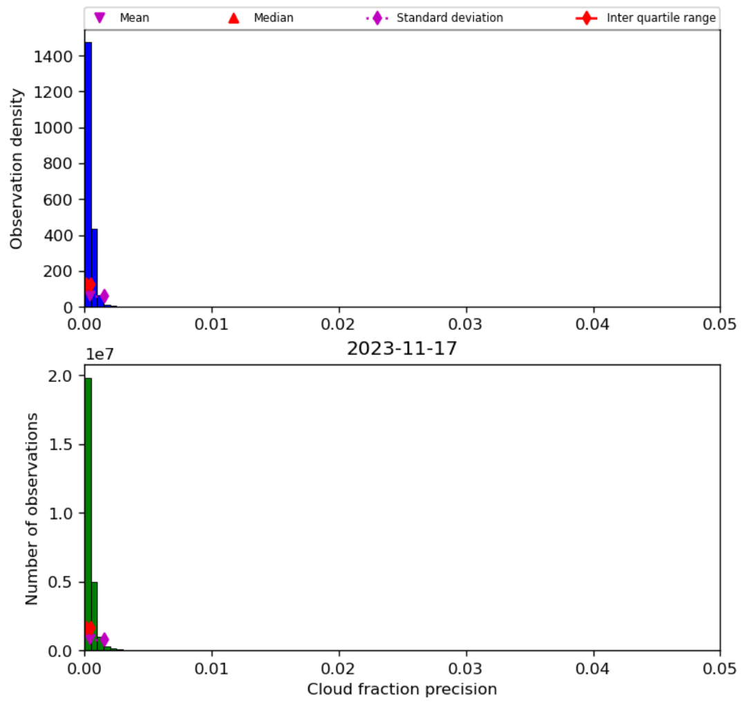
Figure 33: Histogram of “Cloud fraction precision” for 2023-11-16 to 2023-11-18
