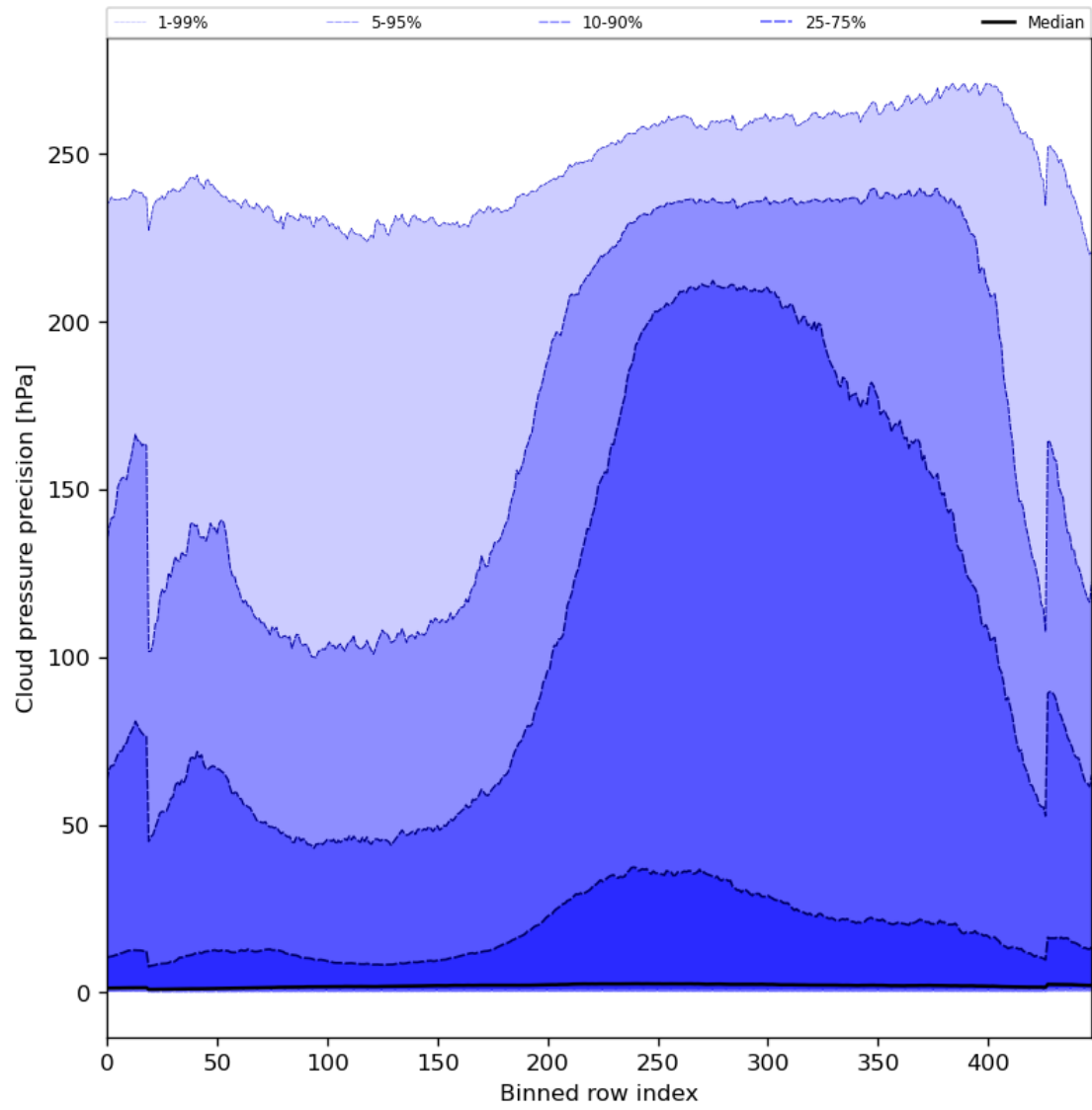
Figure 48: Along track statistics of “Cloud pressure precision” for 2023-11-16 to 2023-11-18
