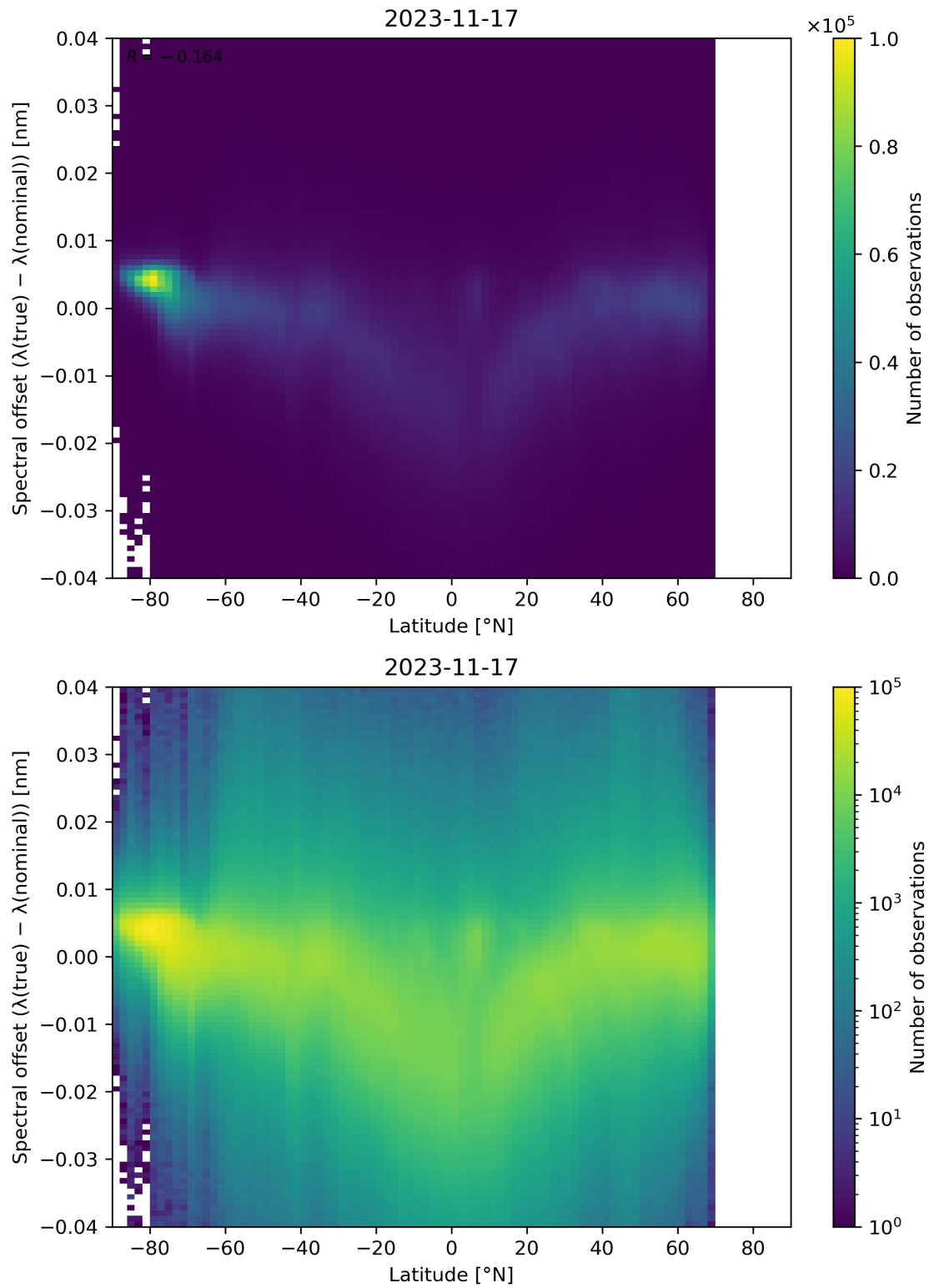
Figure 105: Scatter density plot of “Latitude” against “Spectral offset ( \lambda(\text{true}) - \lambda(\text{nominal}) )” for 2023-11-16 to 2023-11-18.
