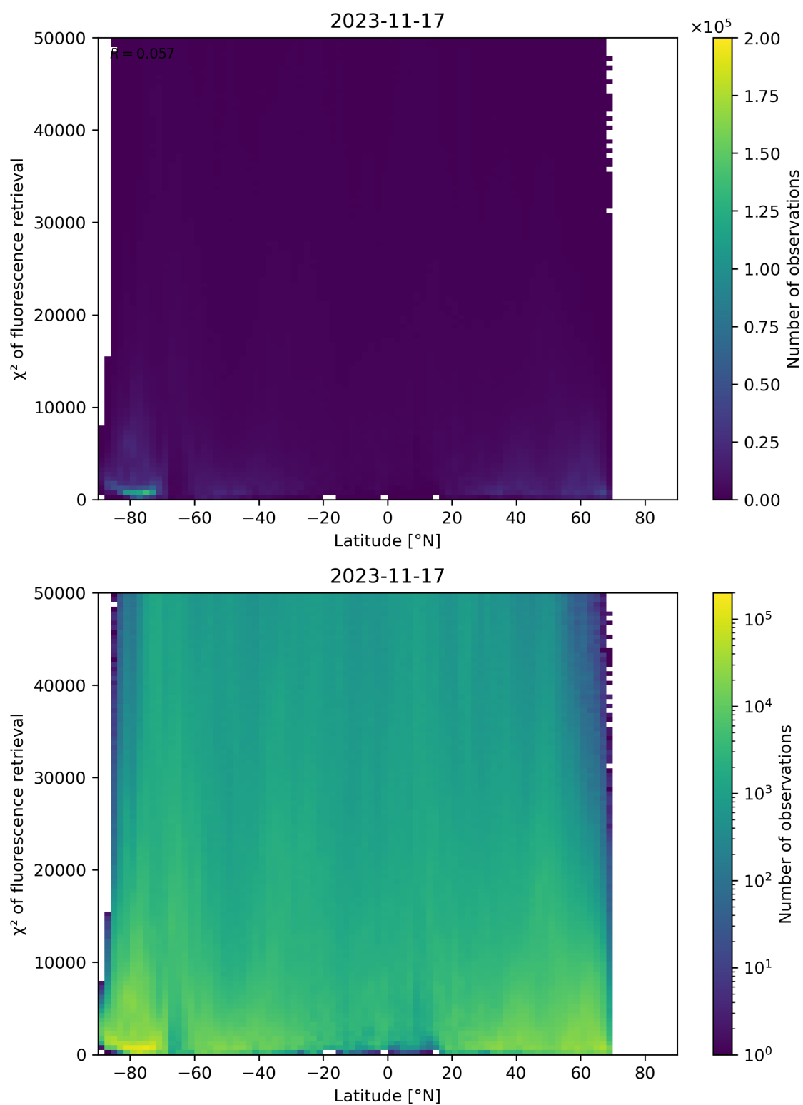
Figure 98: Scatter density plot of “Latitude” against “ \chi^2 of fluorescence retrieval” for 2023-11-16 to 2023-11-18.
