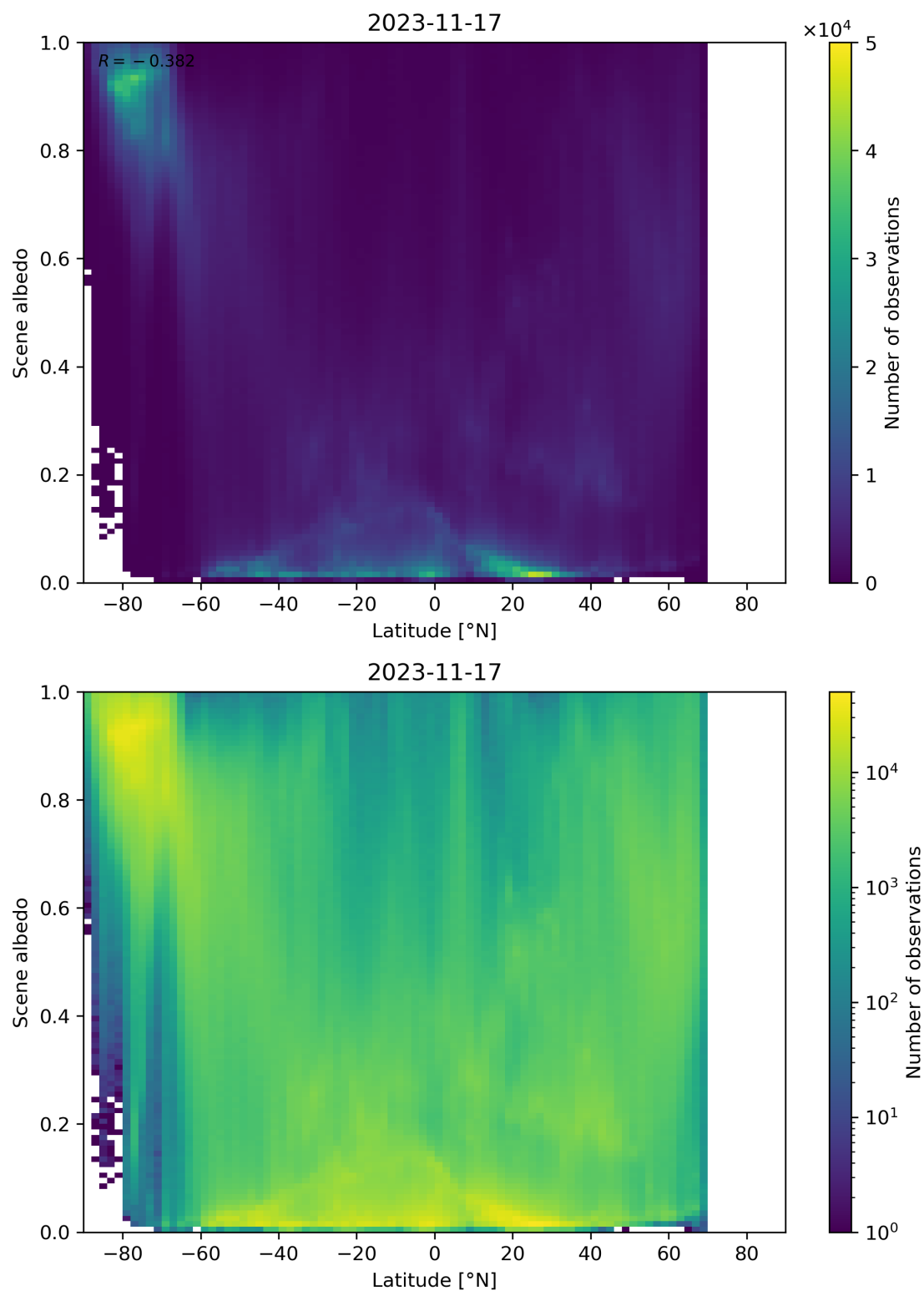
Figure 104: Scatter density plot of “Latitude” against “Scene albedo” for 2023-11-16 to 2023-11-18.
