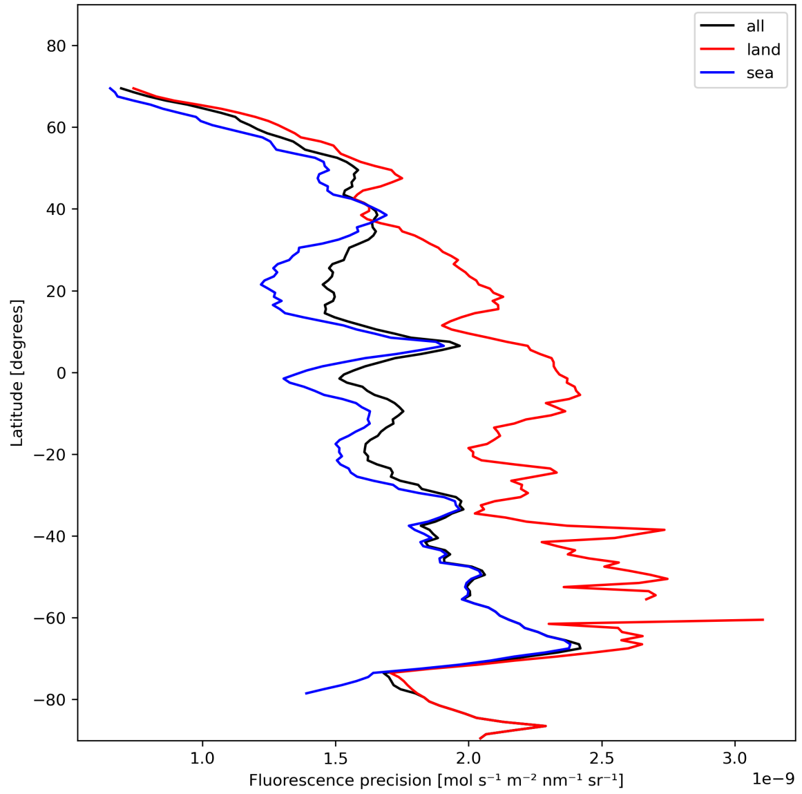
Figure 24: Zonal average of “Fluorescence precision” for 2023-11-16 to 2023-11-18.
