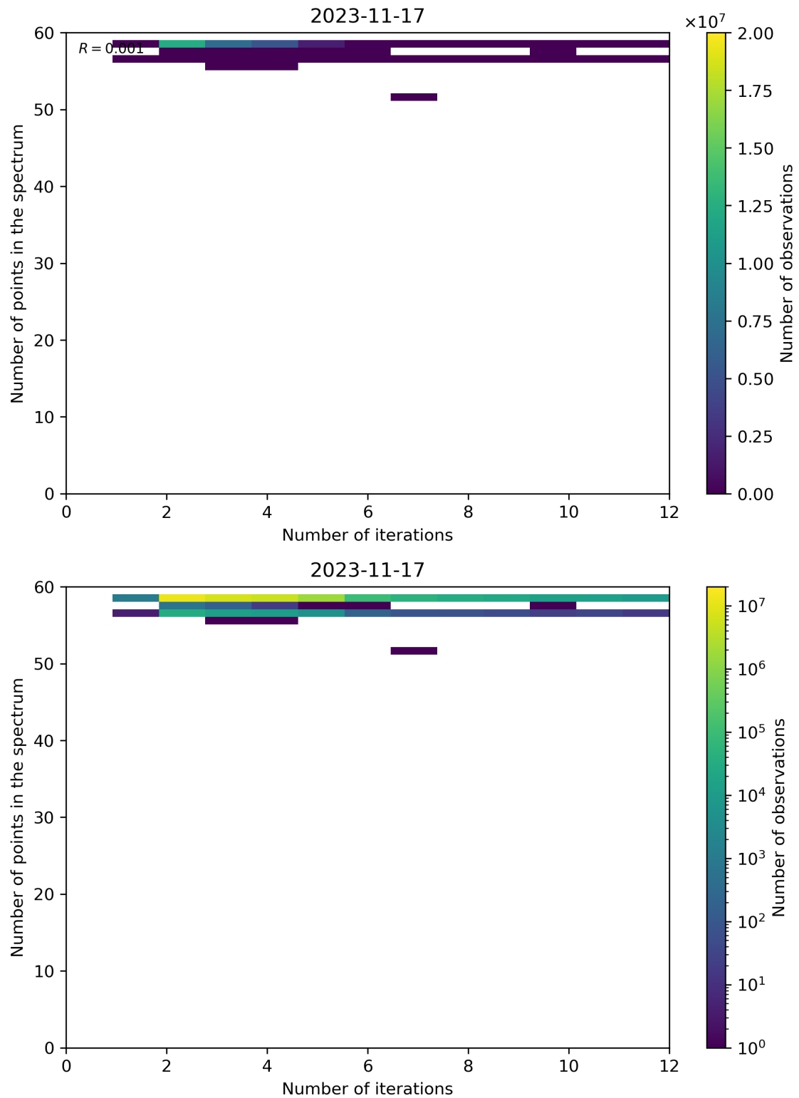
Figure 108: Scatter density plot of “Number of iterations” against “Number of points in the spectrum” for 2023-11-16 to 2023-11-18.
