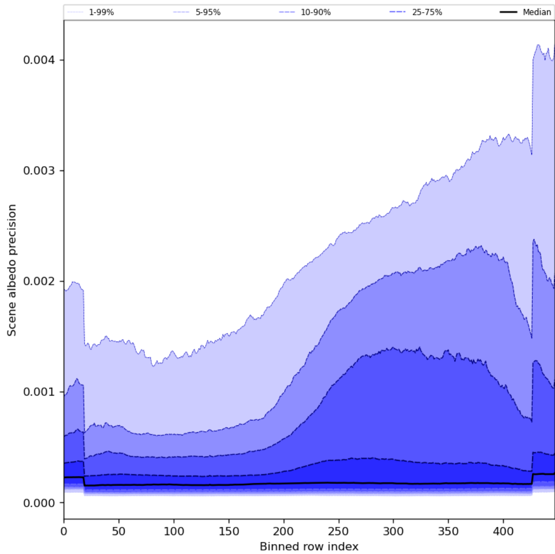
Figure 52: Along track statistics of “Scene albedo precision” for 2023-11-16 to 2023-11-18
