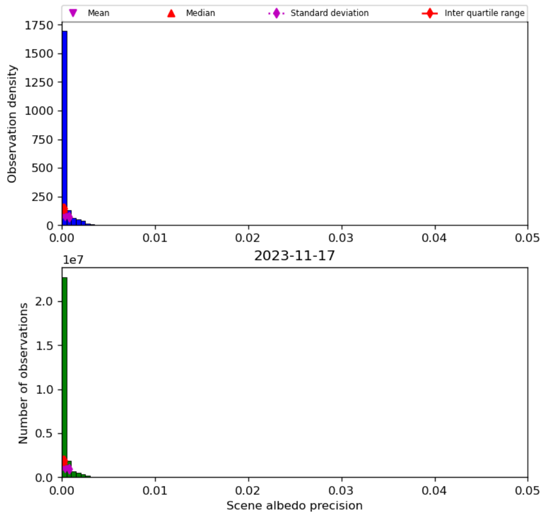
Figure 35: Histogram of “Scene albedo precision” for 2023-11-16 to 2023-11-18
