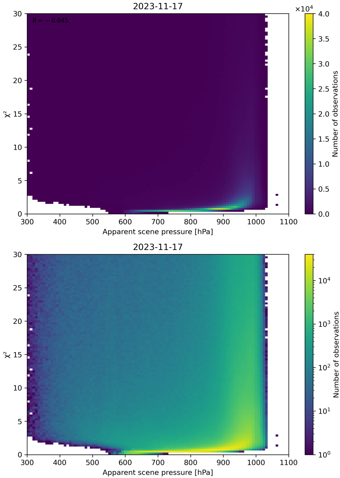
Figure 63: Scatter density plot of “Apparent scene pressure” against “ \chi^2 ” for 2023-11-16 to 2023-11-18.
