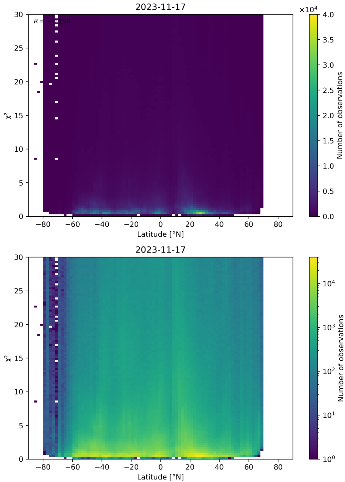
Figure 97: Scatter density plot of “Latitude” against “ \chi^2 ” for 2023-11-16 to 2023-11-18.
