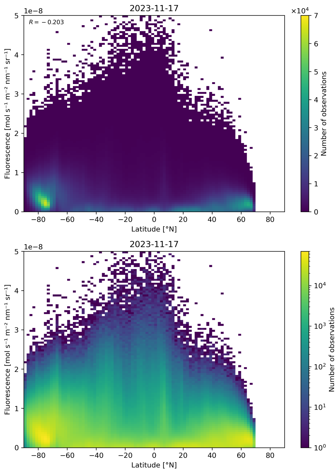
Figure 101: Scatter density plot of “Latitude” against “Fluorescence” for 2023-11-16 to 2023-11-18.
