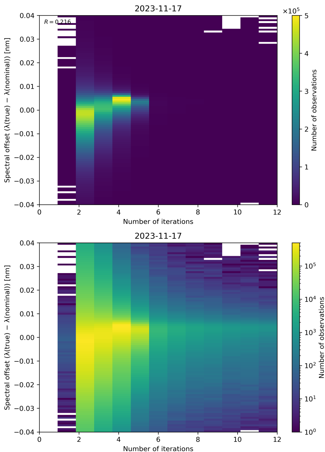
Figure 109: Scatter density plot of “Number of iterations” against “Spectral offset ( \lambda(\text{true}) - \lambda(\text{nominal}) )” for 2023-11-16 to 2023-11-18.
