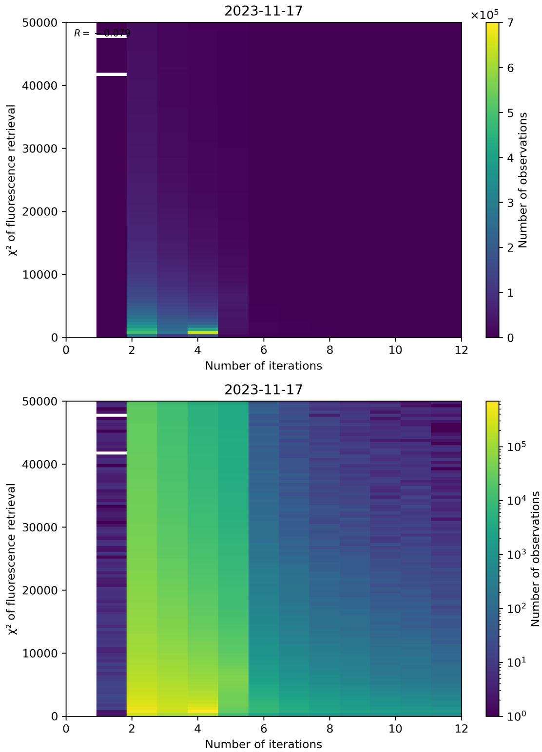
Figure 106: Scatter density plot of “Number of iterations” against “ \chi^2 of fluorescence retrieval” for 2023-11-16 to 2023-11-18.
