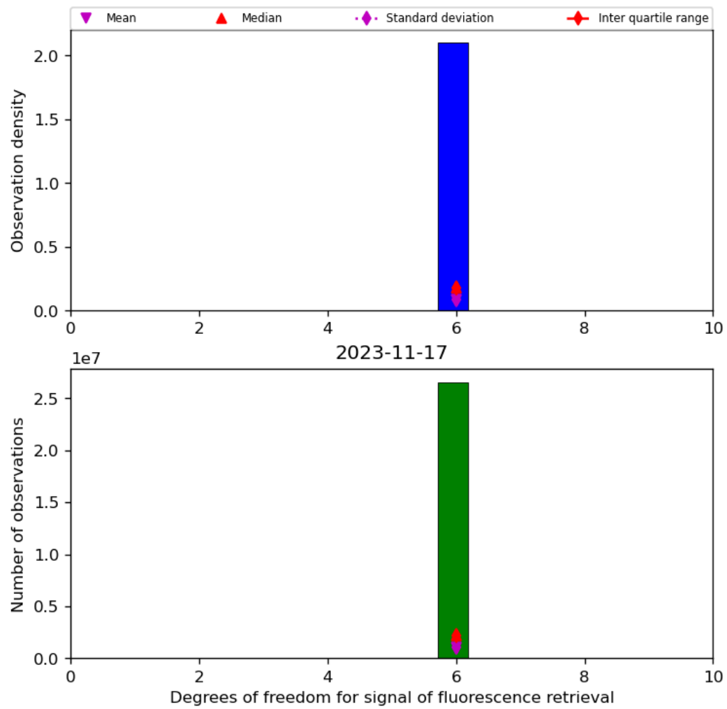
Figure 43: Histogram of “Degrees of freedom for signal of fluorescence retrieval” for 2023-11-16 to 2023-11-18
