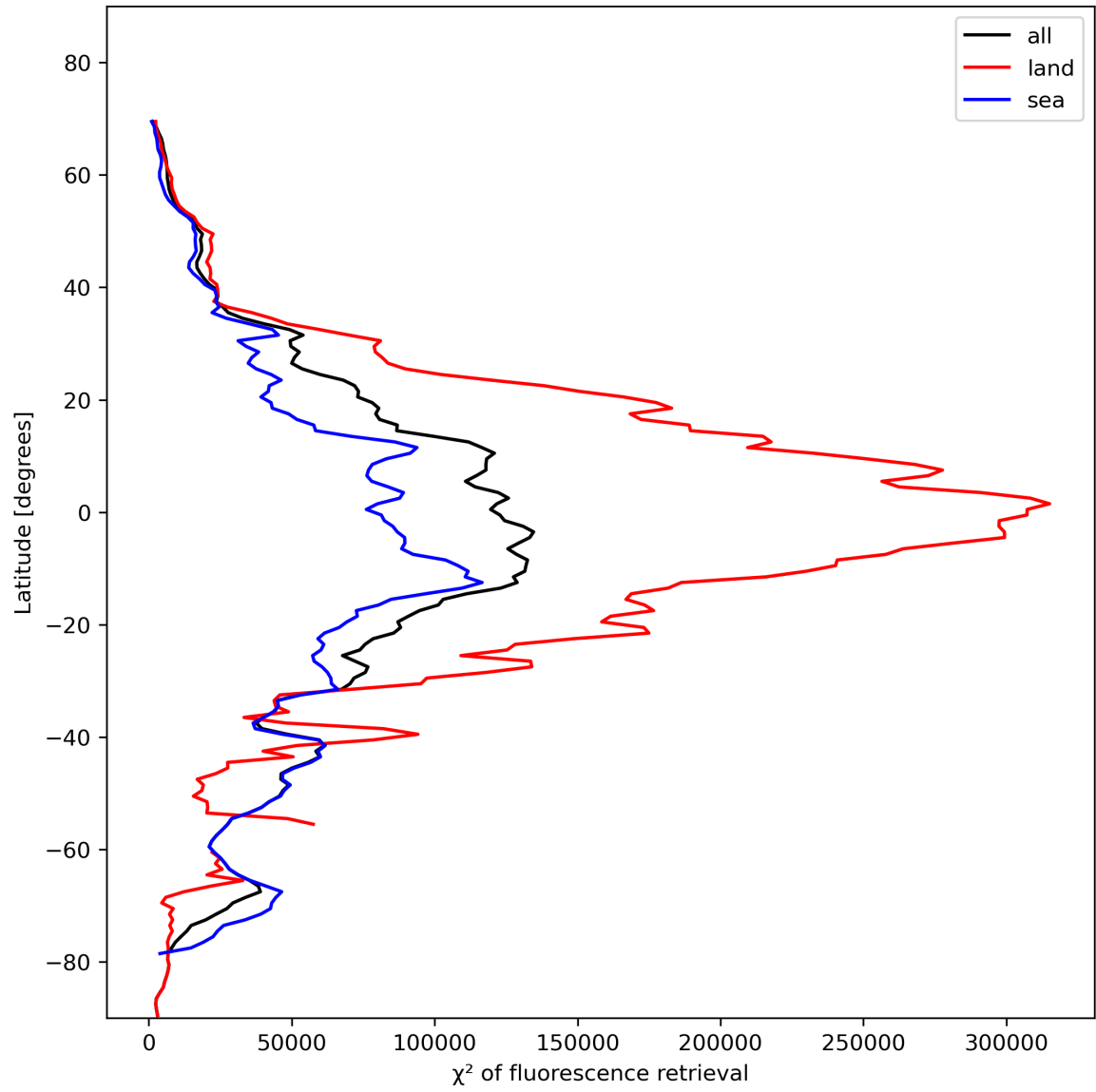
Figure 25: Zonal average of “ \chi^2 of fluorescence retrieval” for 2023-11-16 to 2023-11-18.
