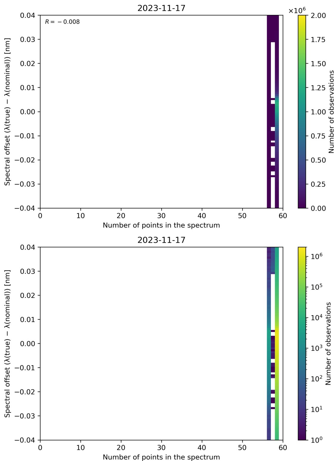
Figure 110: Scatter density plot of “Number of points in the spectrum” against “Spectral offset ( \lambda(\text{true}) - \lambda(\text{nominal}) )” for 2023-11-16 to 2023-11-18.
