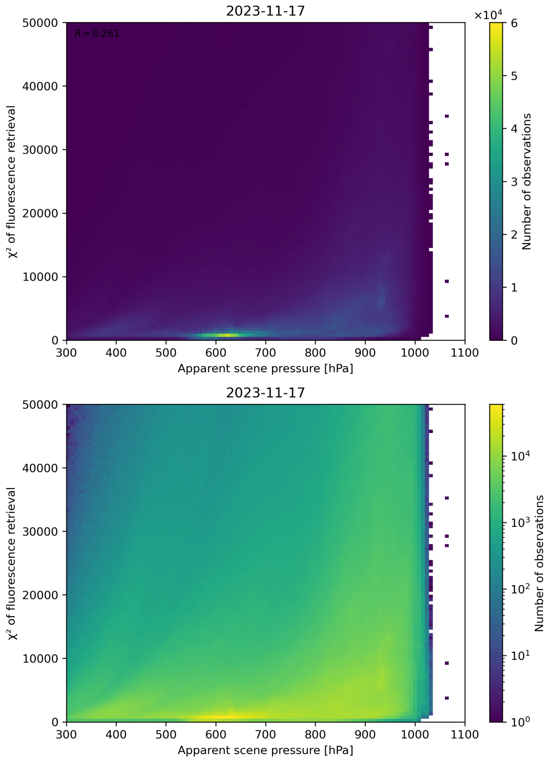
Figure 64: Scatter density plot of “Apparent scene pressure” against “ \chi^2 of fluorescence retrieval” for 2023-11-16 to 2023-11-18.
