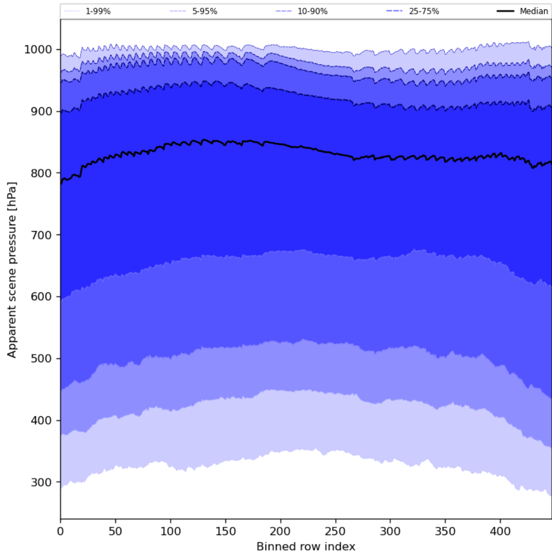
Figure 53: Along track statistics of “Apparent scene pressure” for 2023-11-16 to 2023-11-18
