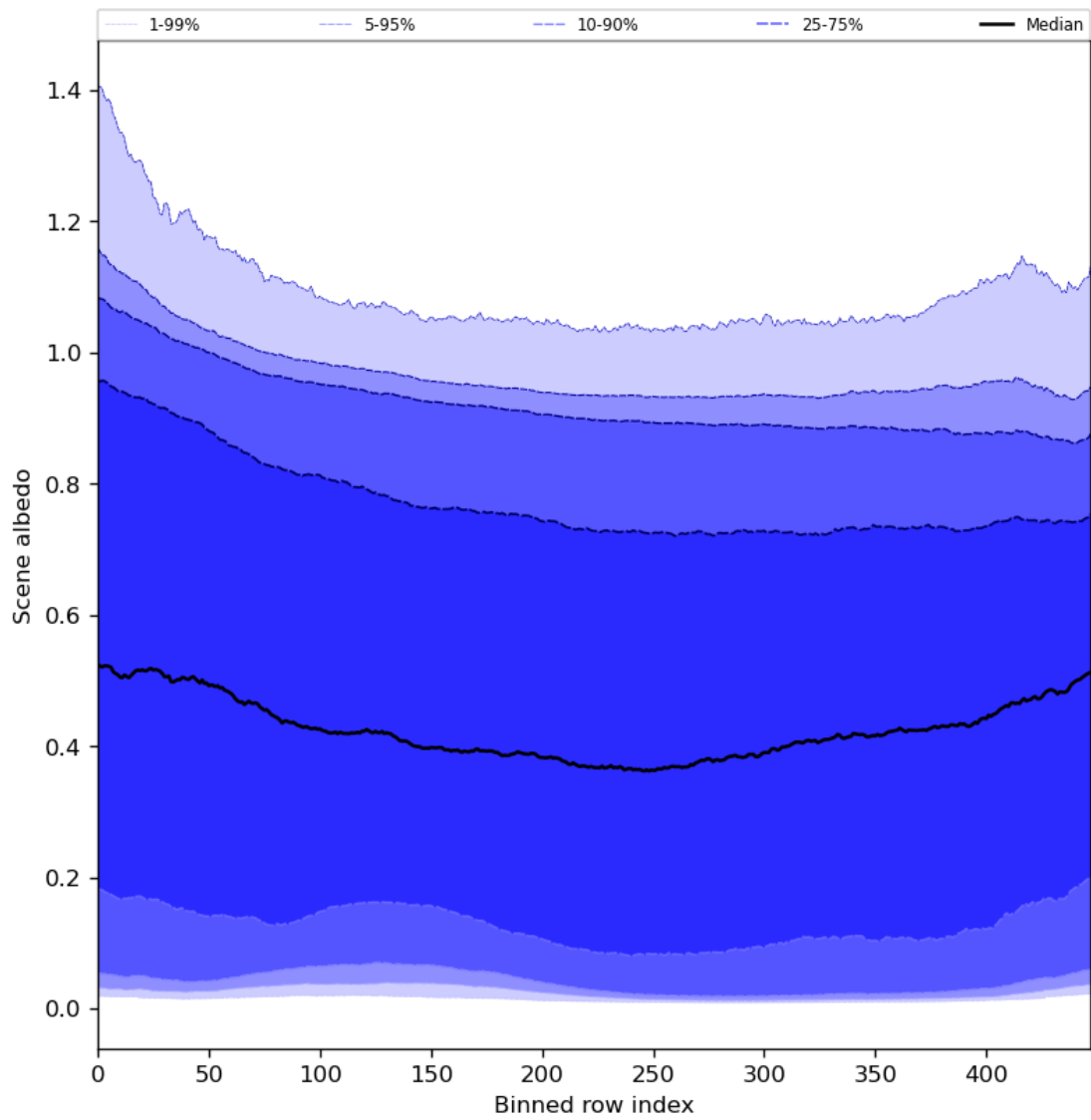
Figure 51: Along track statistics of “Scene albedo” for 2023-11-16 to 2023-11-18
