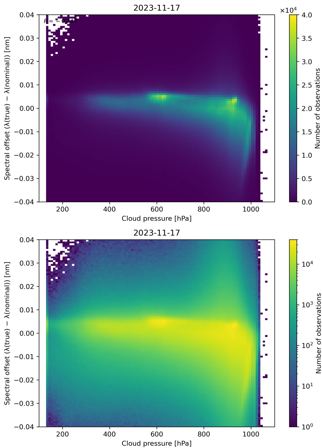
Figure 92: Scatter density plot of “Cloud pressure” against “Spectral offset ( \lambda(\text{true}) - \lambda(\text{nominal}) )” for 2023-11-16 to 2023-11-18.
