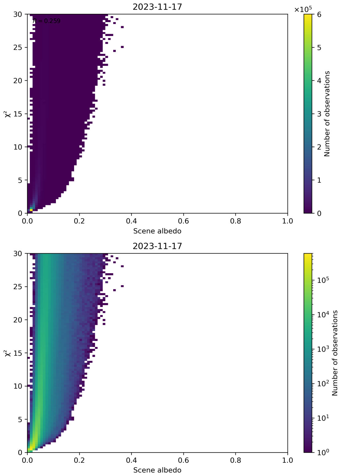
Figure 112: Scatter density plot of “Scene albedo” against “ \chi^2 ” for 2023-11-16 to 2023-11-18.
