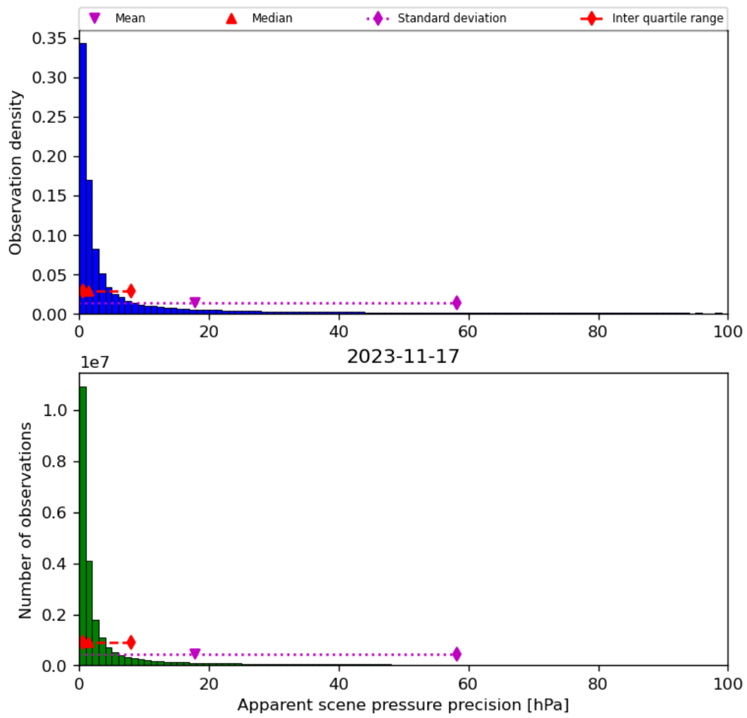
Figure 37: Histogram of “Apparent scene pressure precision” for 2023-11-16 to 2023-11-18
