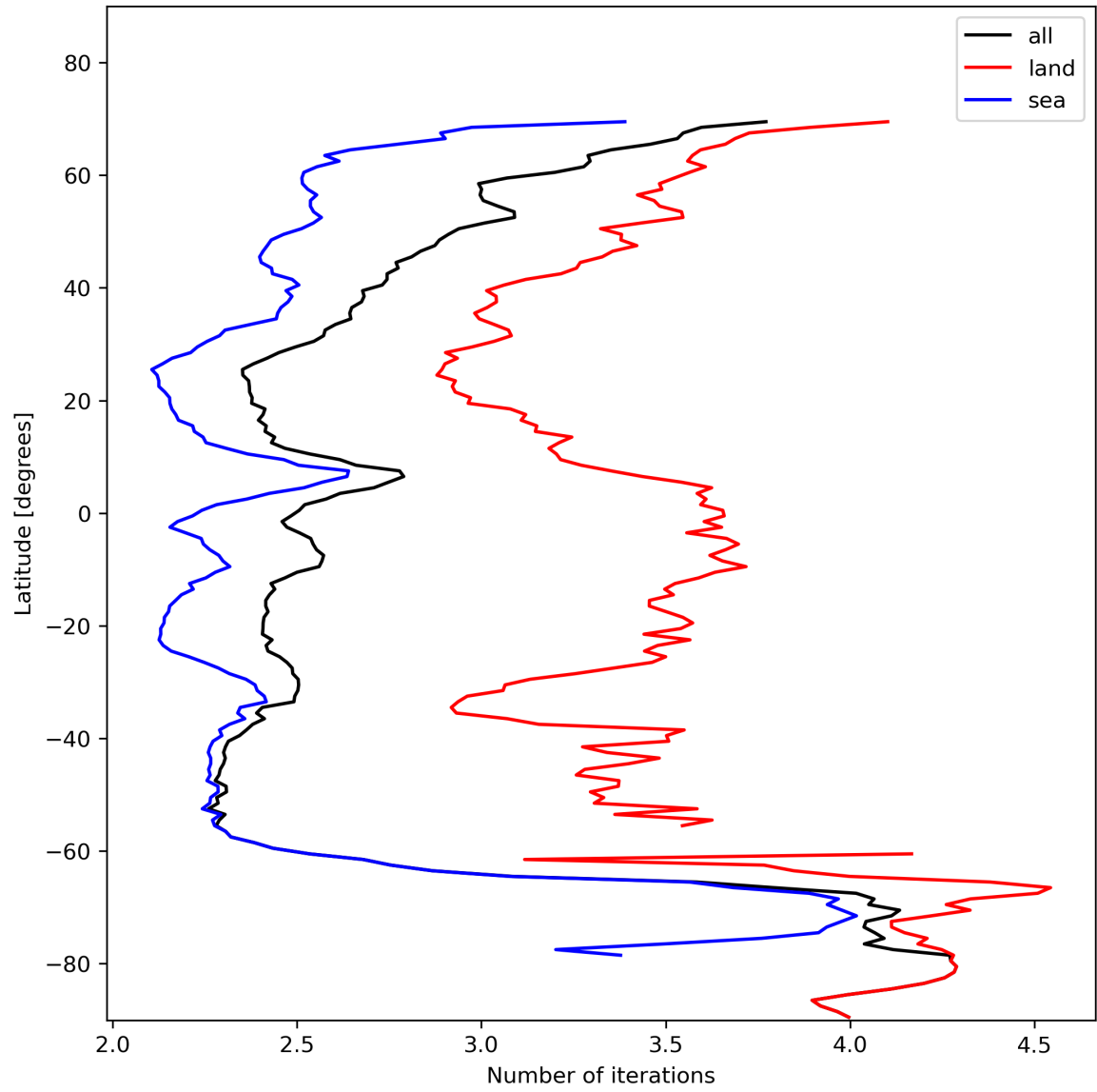
Figure 22: Zonal average of “Number of iterations” for 2023-11-16 to 2023-11-18.
