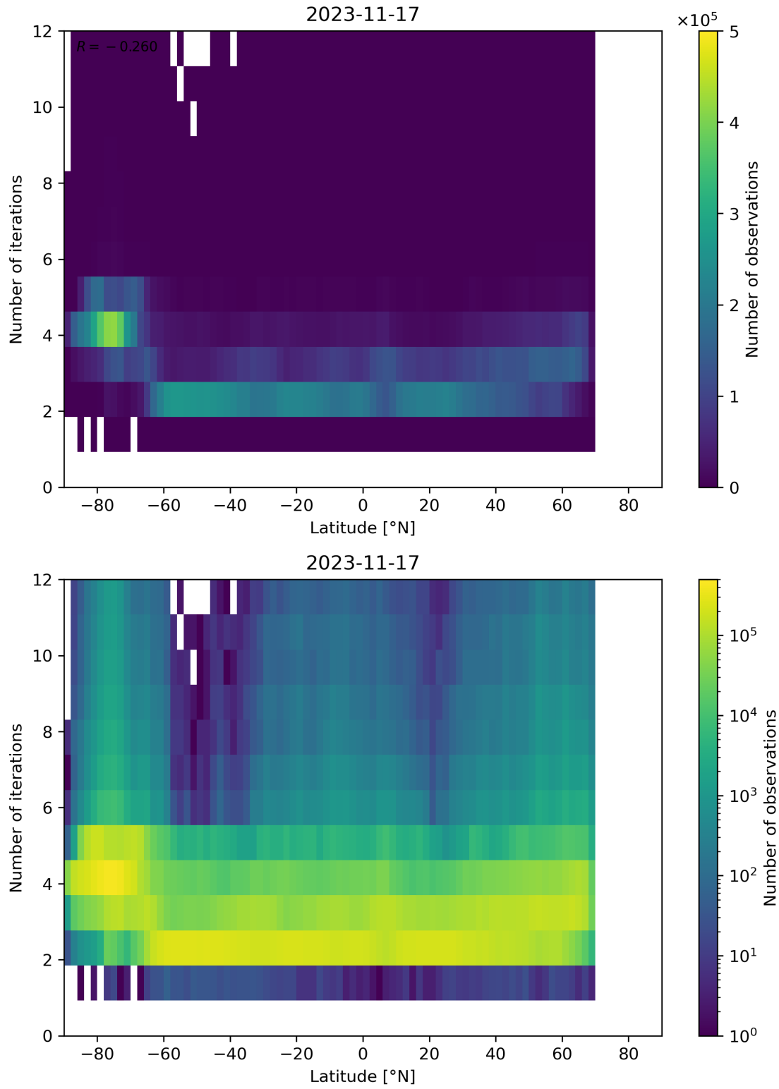
Figure 102: Scatter density plot of “Latitude” against “Number of iterations” for 2023-11-16 to 2023-11-18.
