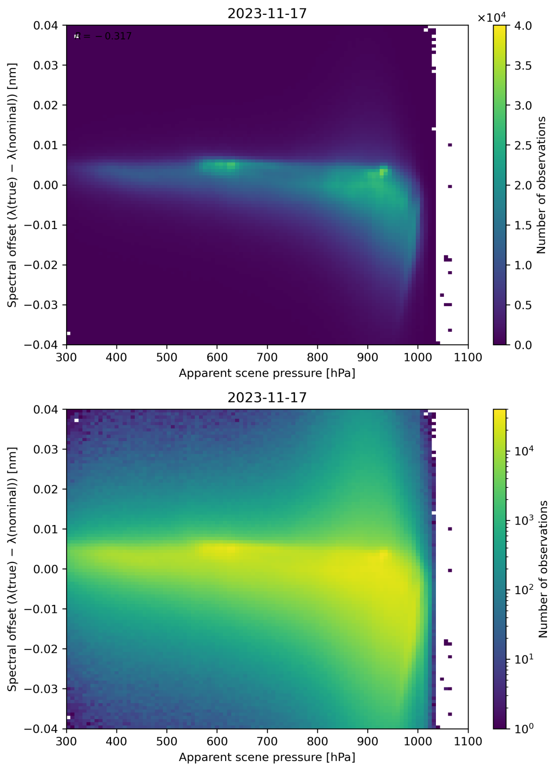
Figure 68: Scatter density plot of “Apparent scene pressure” against “Spectral offset ( \lambda(\text{true}) - \lambda(\text{nominal}) )” for 2023-11-16 to 2023-11-18.
