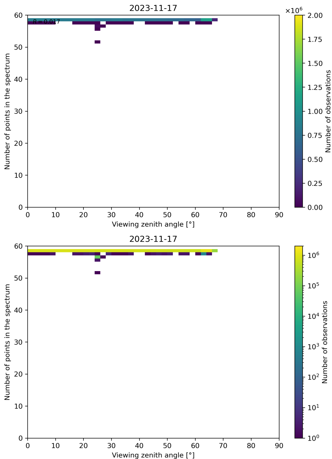
Figure 137: Scatter density plot of “Viewing zenith angle” against “Number of points in the spectrum” for 2023-11-16 to 2023-11-18.
