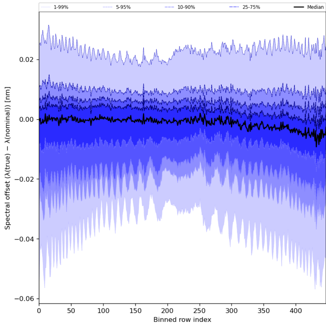
Figure 62: Along track statistics of “Spectral offset ( \lambda(\text{true}) - \lambda(\text{nominal}) )” for 2023-11-16 to 2023-11-18
