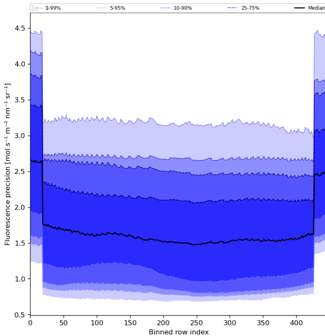
Figure 58: Along track statistics of “Fluorescence precision” for 2023-11-16 to 2023-11-18
