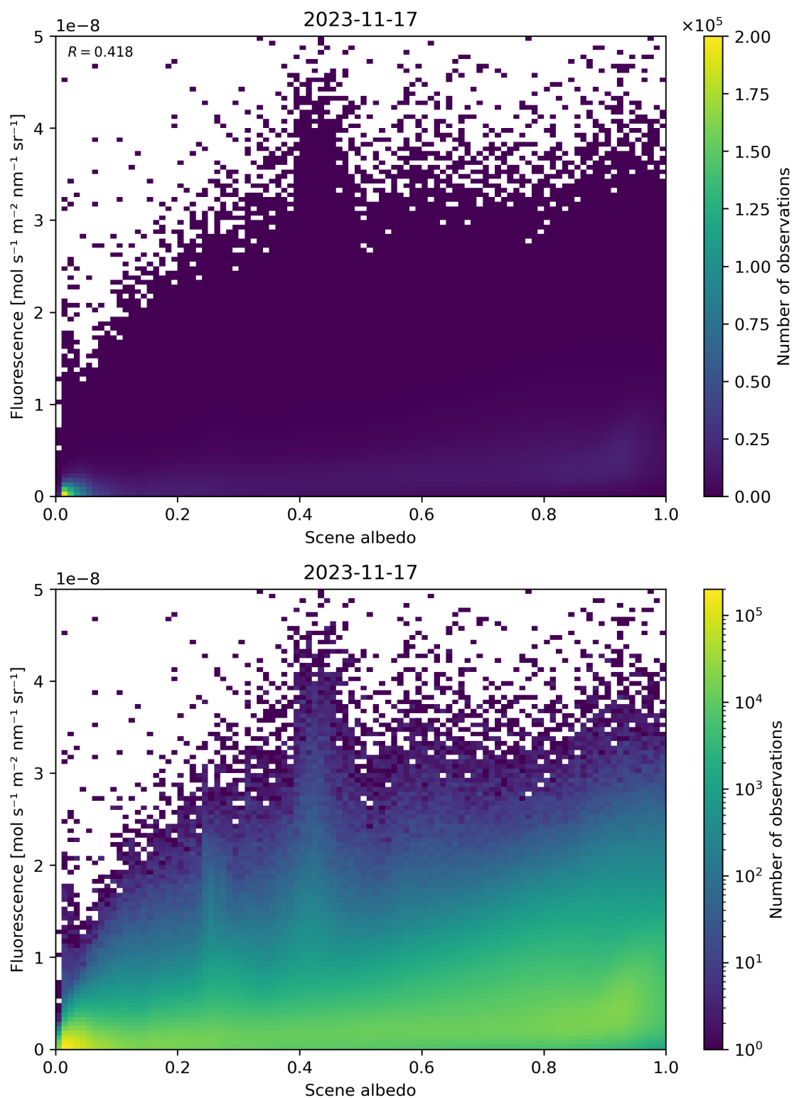
Figure 114: Scatter density plot of “Scene albedo” against “Fluorescence” for 2023-11-16 to 2023-11-18.
