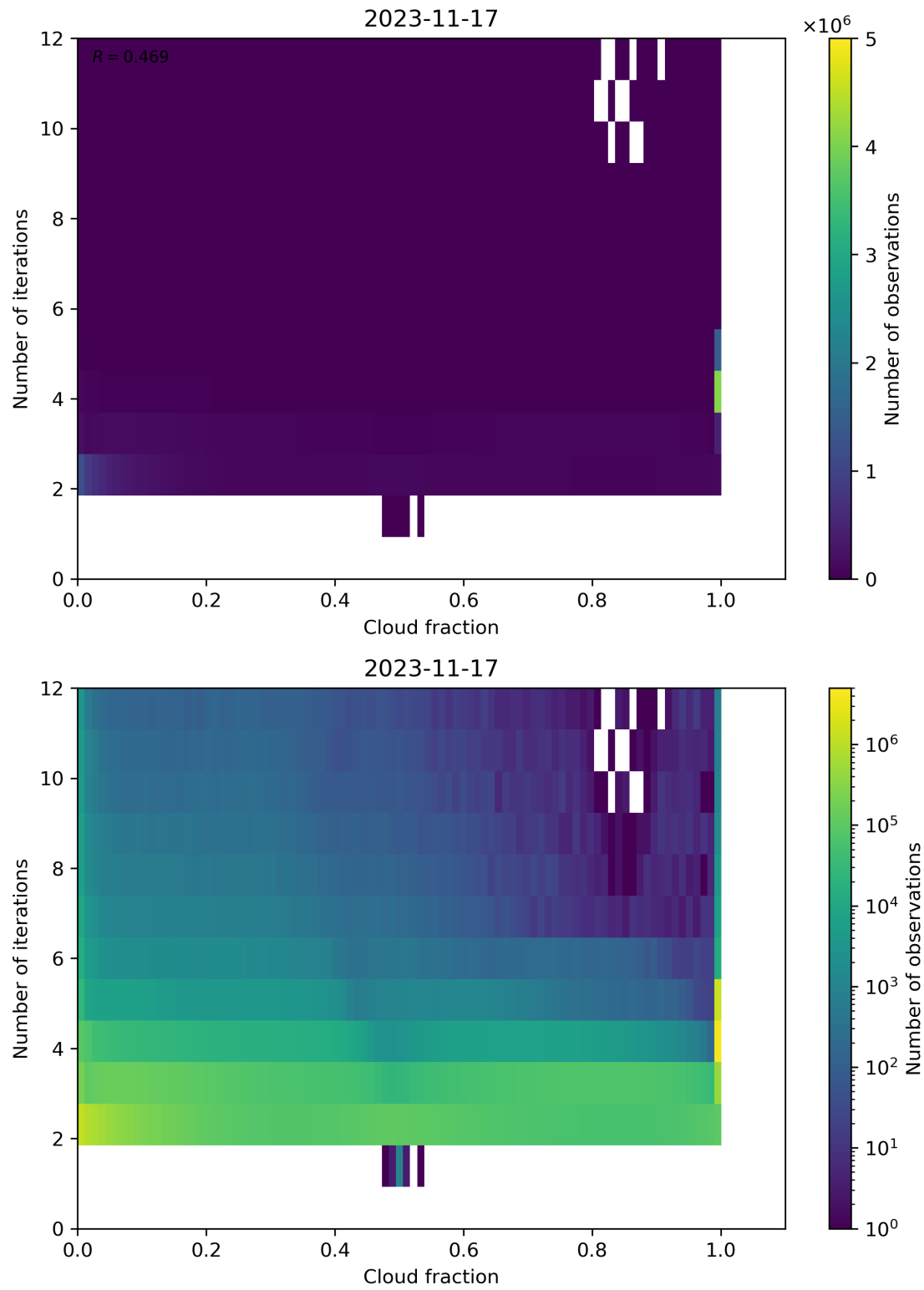
Figure 80: Scatter density plot of “Cloud fraction” against “Number of iterations” for 2023-11-16 to 2023-11-18.
