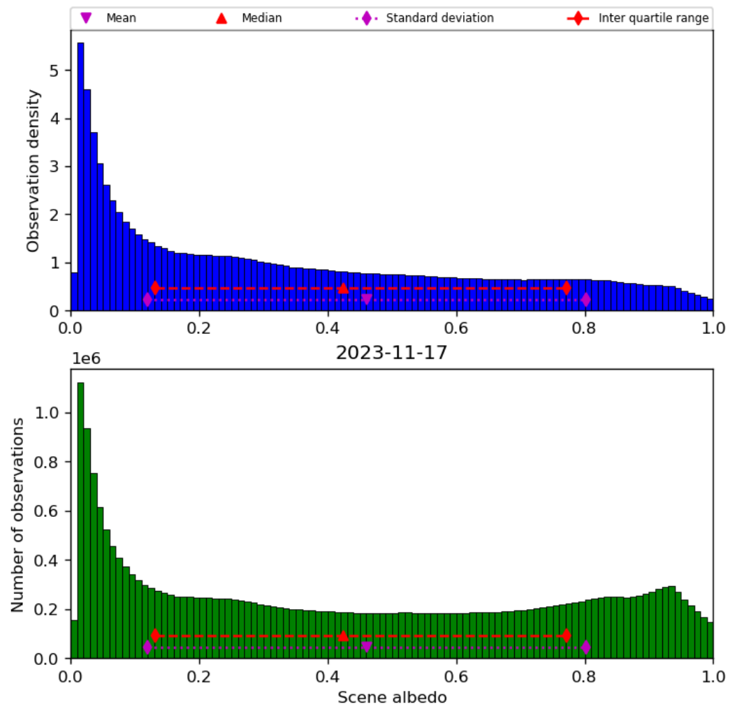
Figure 34: Histogram of “Scene albedo” for 2023-11-16 to 2023-11-18
