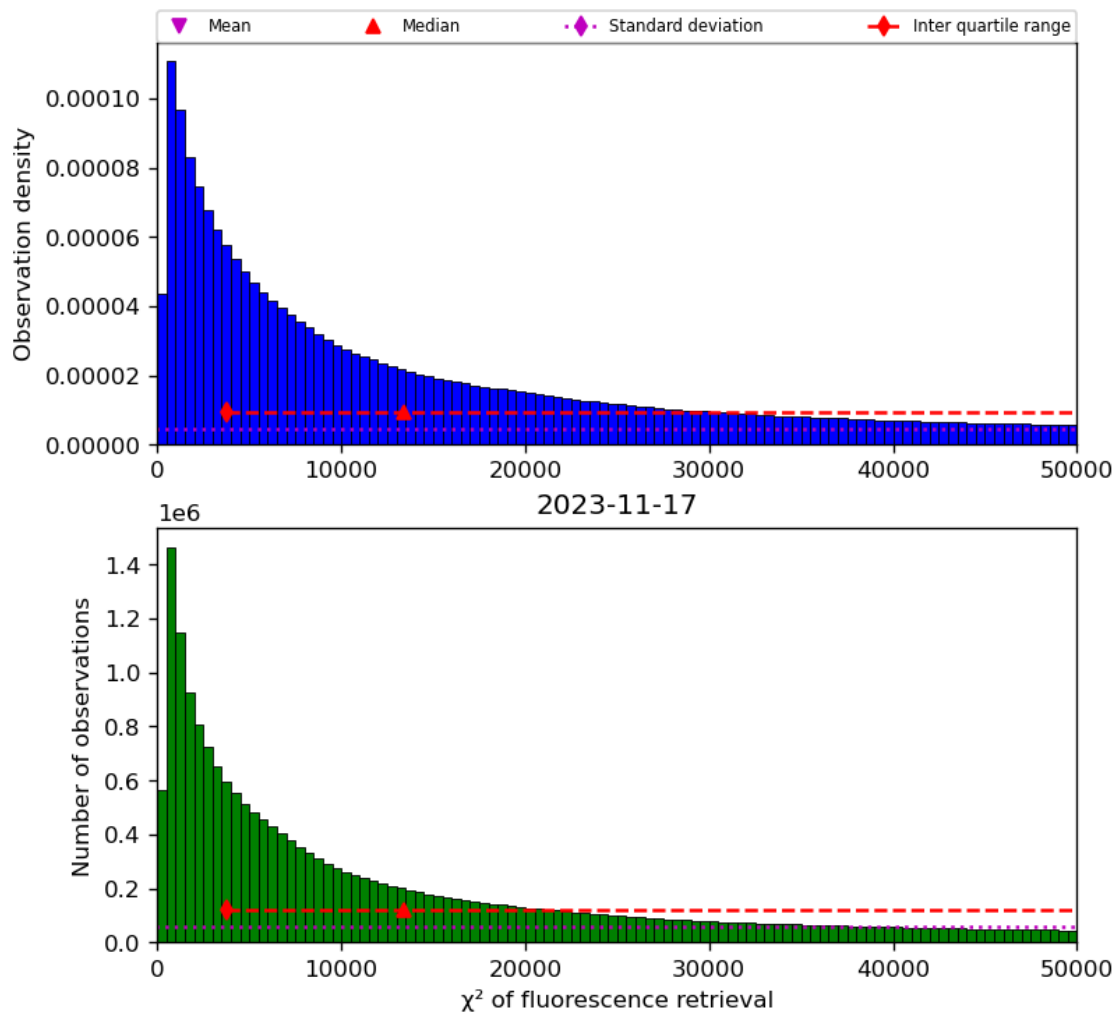
Figure 42: Histogram of “ \chi^2 of fluorescence retrieval” for 2023-11-16 to 2023-11-18
