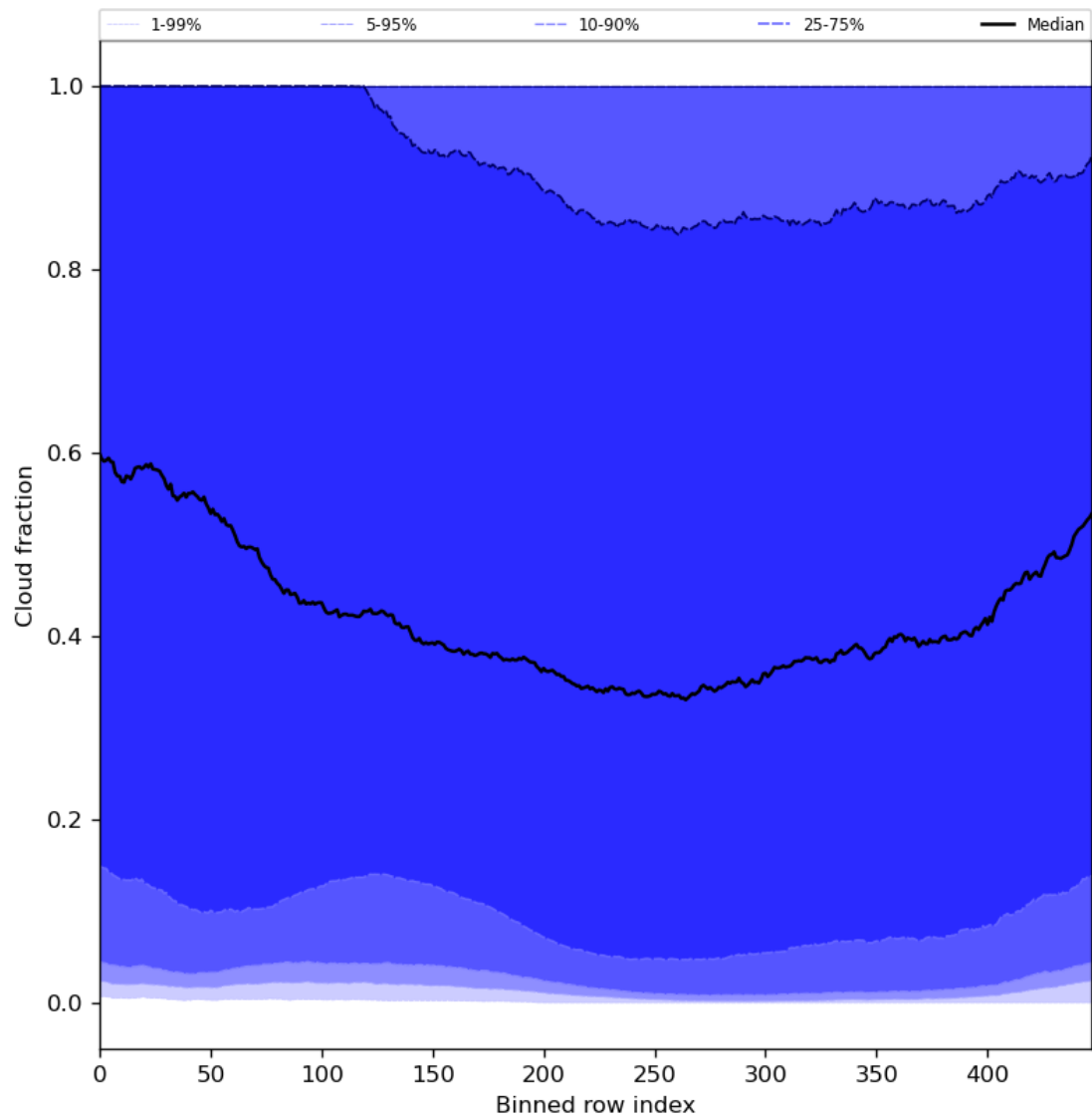
Figure 49: Along track statistics of “Cloud fraction” for 2023-11-16 to 2023-11-18
