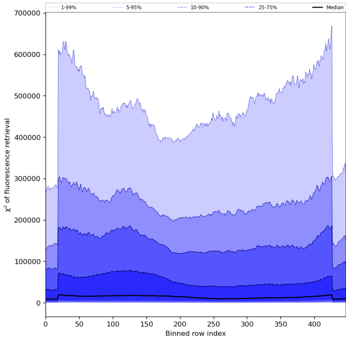
Figure 59: Along track statistics of “ \chi^2 of fluorescence retrieval” for 2023-11-16 to 2023-11-18
