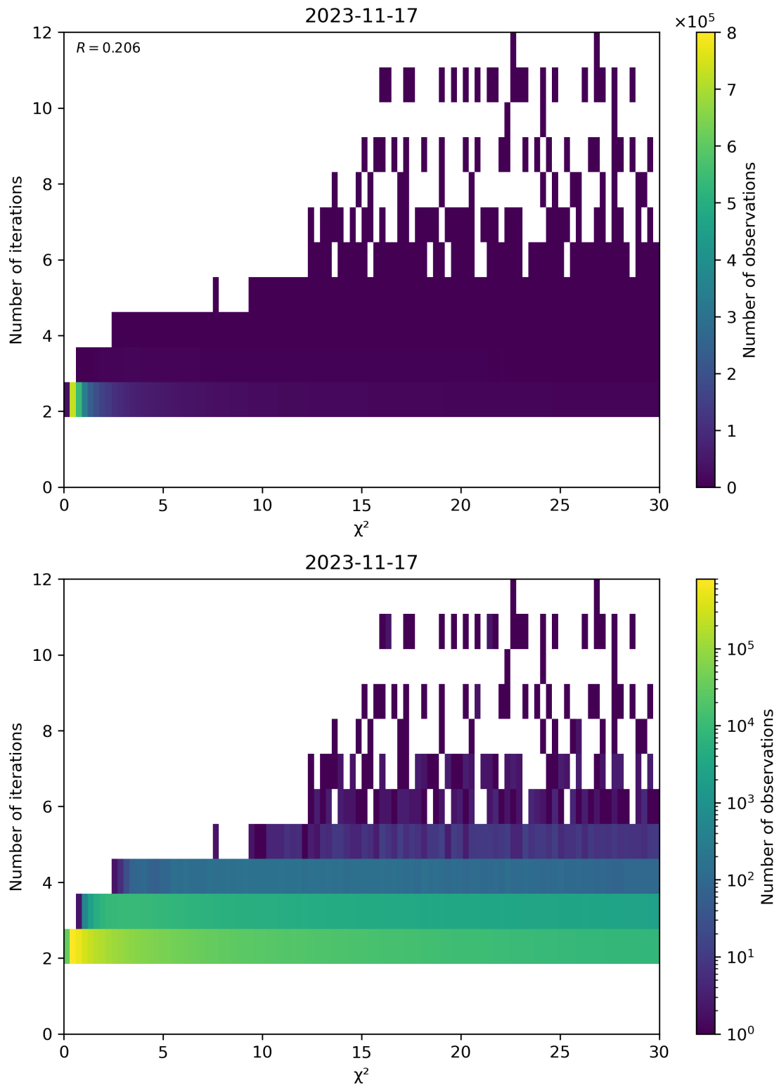
Figure 73: Scatter density plot of “ \chi^2 ” against “Number of iterations” for 2023-11-16 to 2023-11-18.
