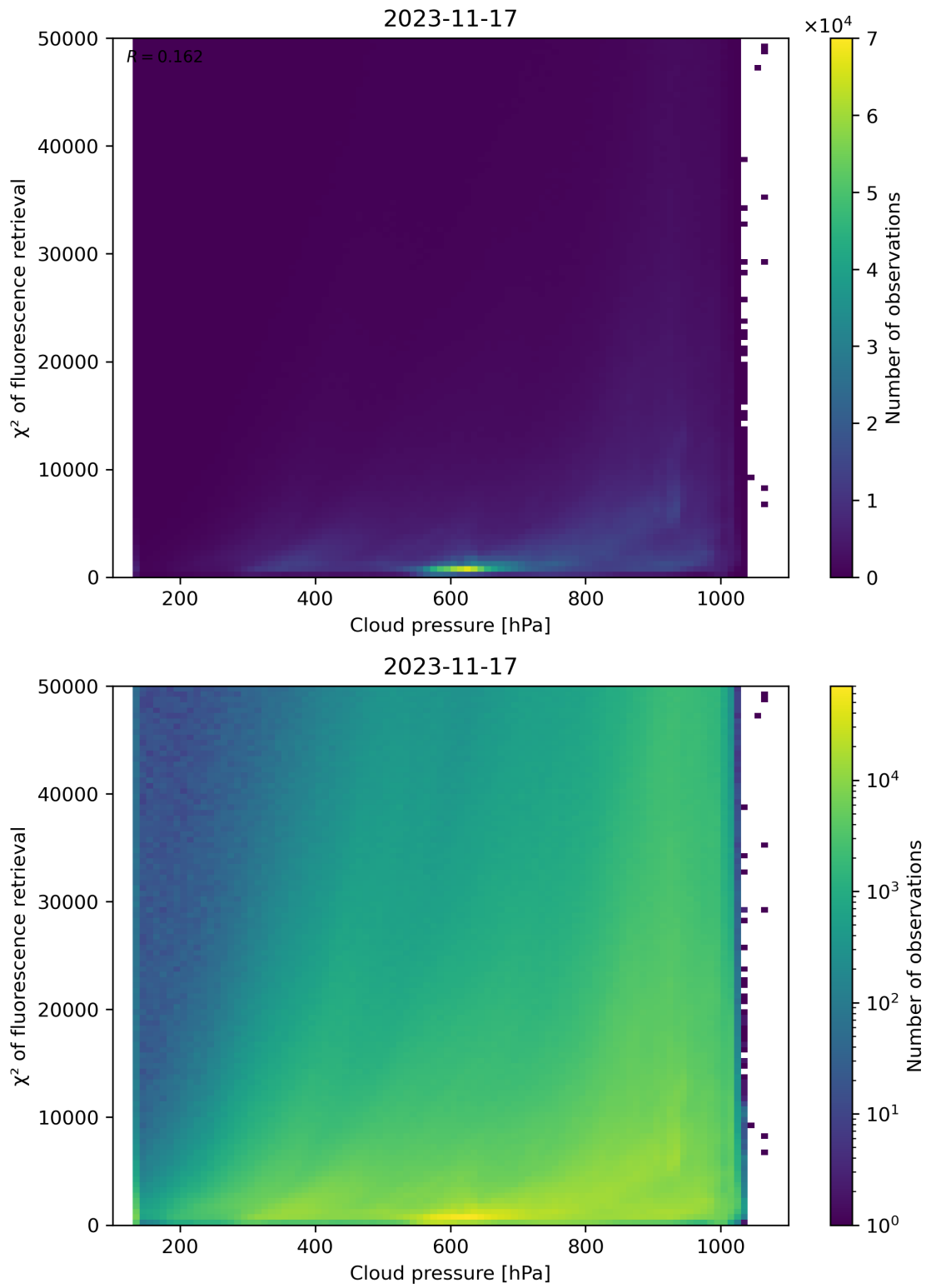
Figure 86: Scatter density plot of “Cloud pressure” against “ \chi^2 of fluorescence retrieval” for 2023-11-16 to 2023-11-18.
