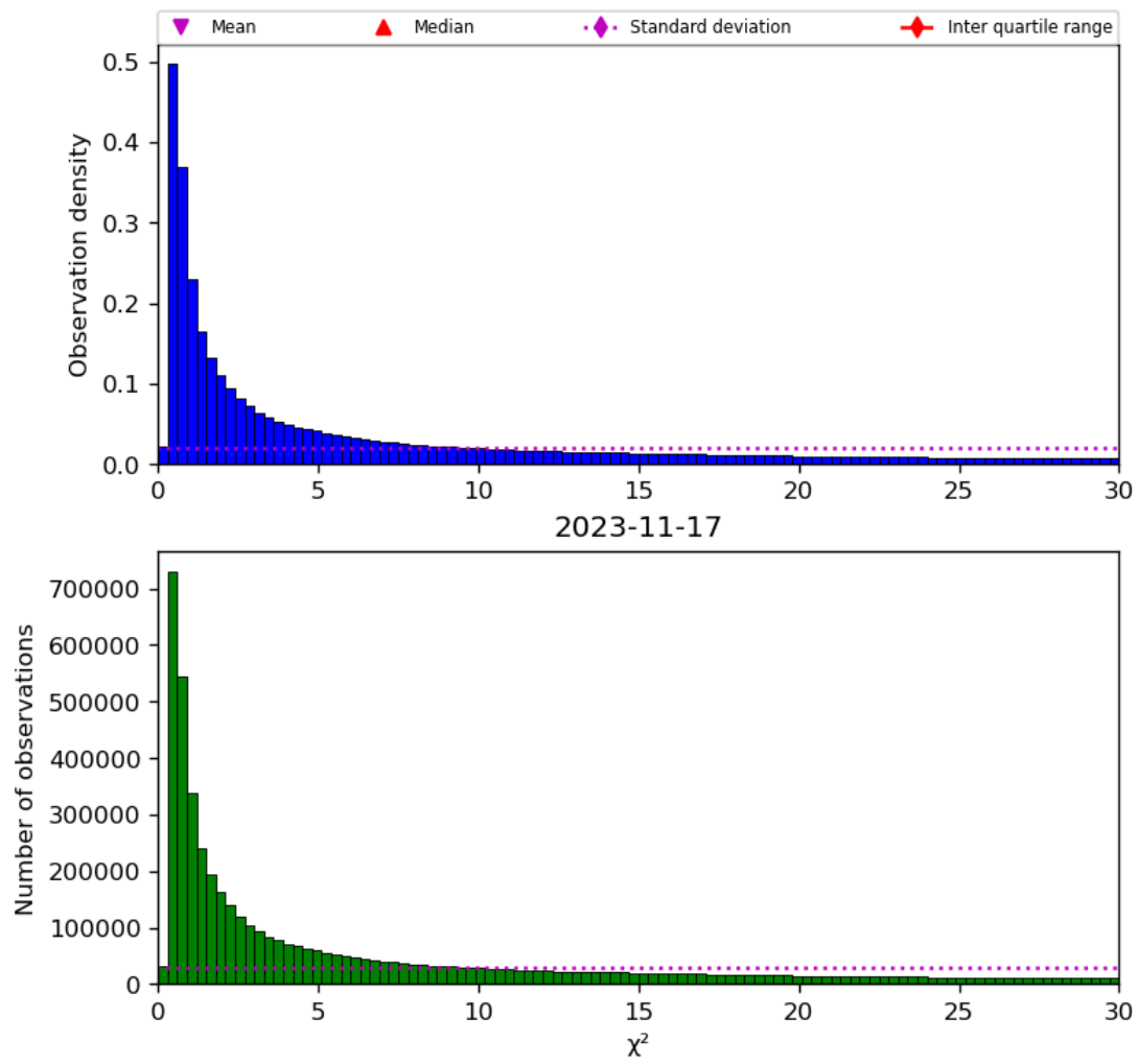
Figure 38: Histogram of “ \chi^2 ” for 2023-11-16 to 2023-11-18
