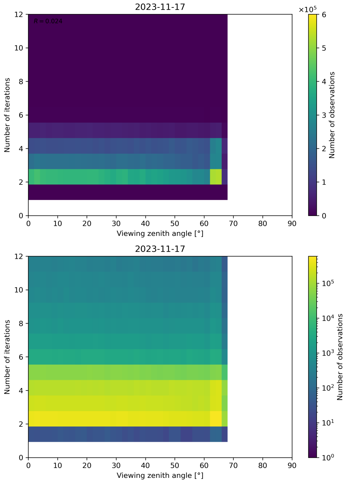
Figure 136: Scatter density plot of “Viewing zenith angle” against “Number of iterations” for 2023-11-16 to 2023-11-18.
