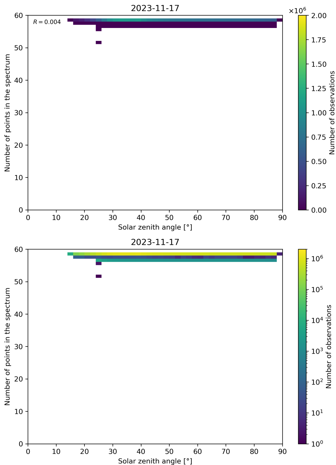
Figure 126: Scatter density plot of “Solar zenith angle” against “Number of points in the spectrum” for 2023-11-16 to 2023-11-18.
