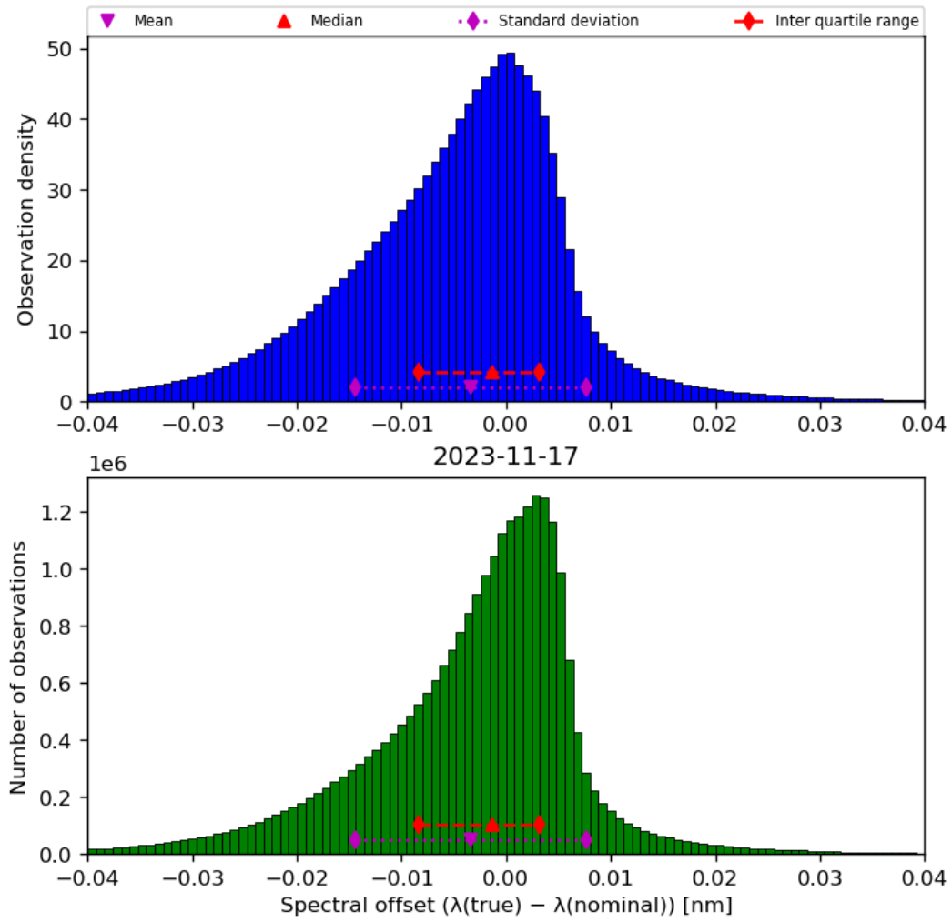
Figure 45: Histogram of “Spectral offset ( \lambda(\text{true}) - \lambda(\text{nominal}) )” for 2023-11-16 to 2023-11-18
