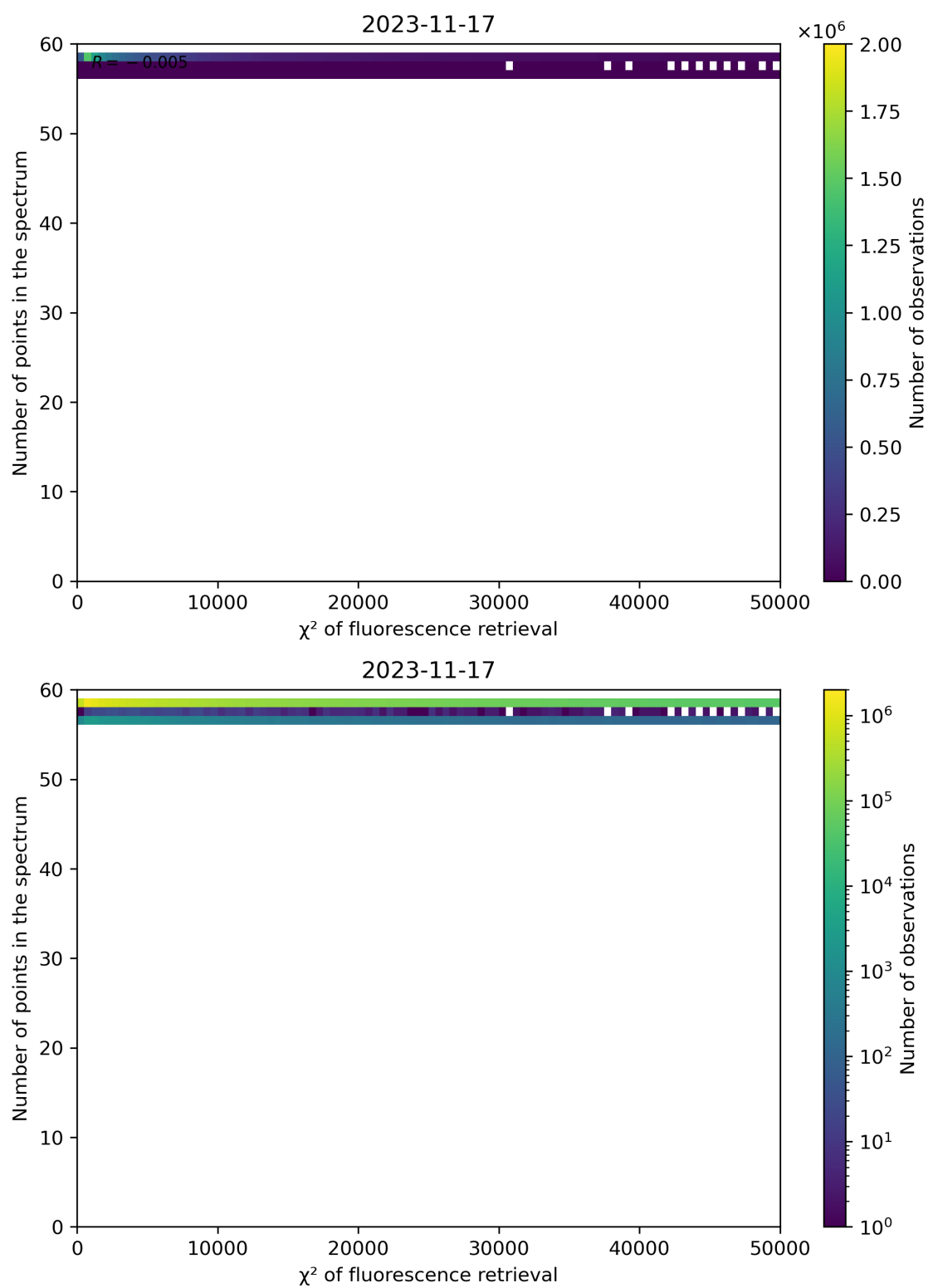
Figure 71: Scatter density plot of " \chi^2 of fluorescence retrieval" against "Number of points in the spectrum" for 2023-11-16 to 2023-11-18.
