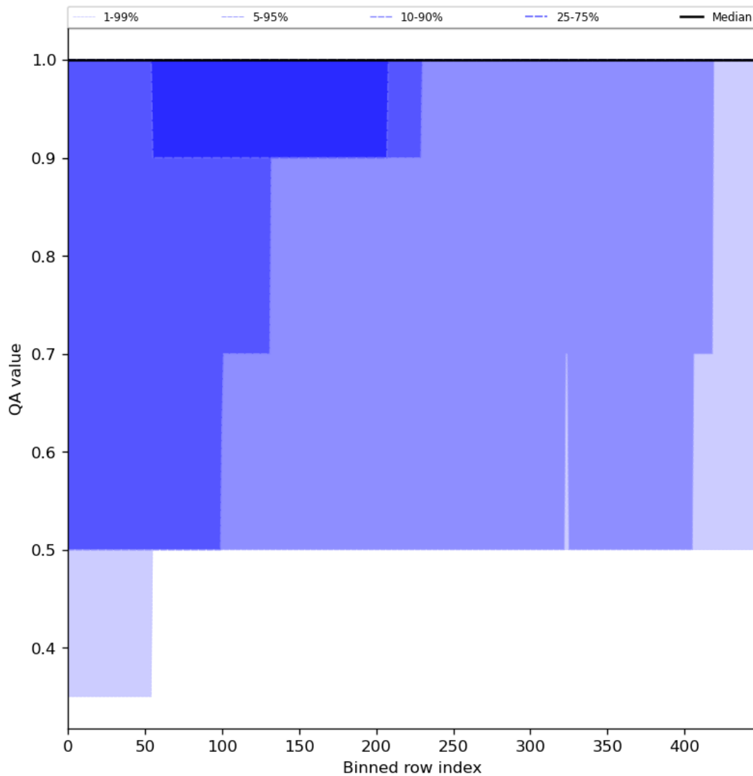
Figure 46: Along track statistics of “QA value” for 2023-11-16 to 2023-11-18
