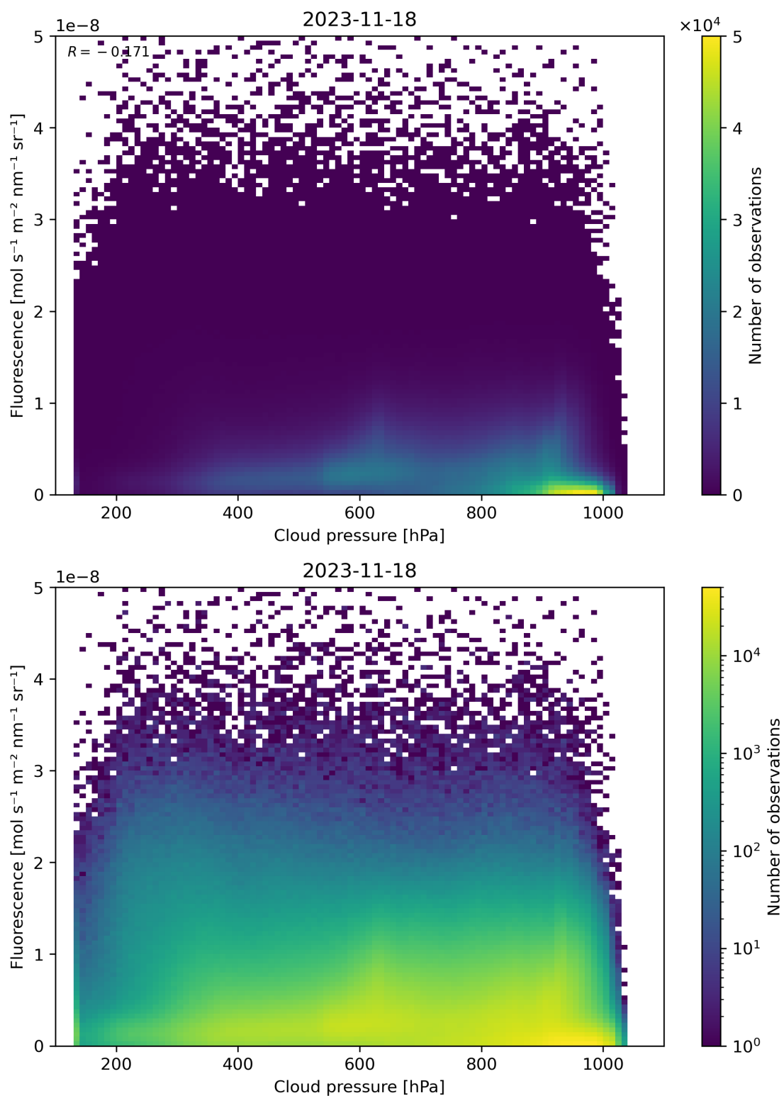
Figure 88: Scatter density plot of “Cloud pressure” against “Fluorescence” for 2023-11-18 to 2023-11-19.
