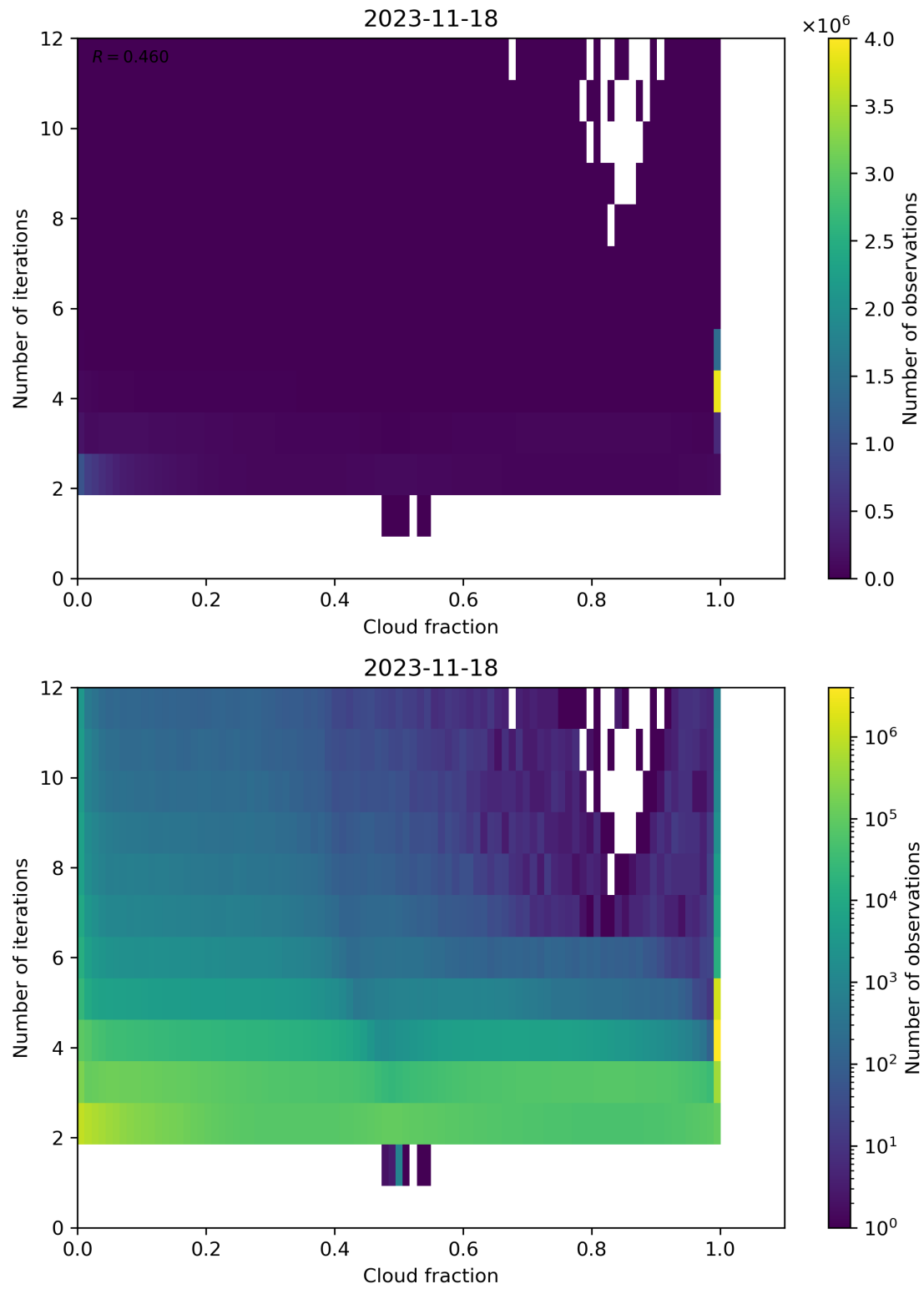
Figure 80: Scatter density plot of “Cloud fraction” against “Number of iterations” for 2023-11-18 to 2023-11-19.
