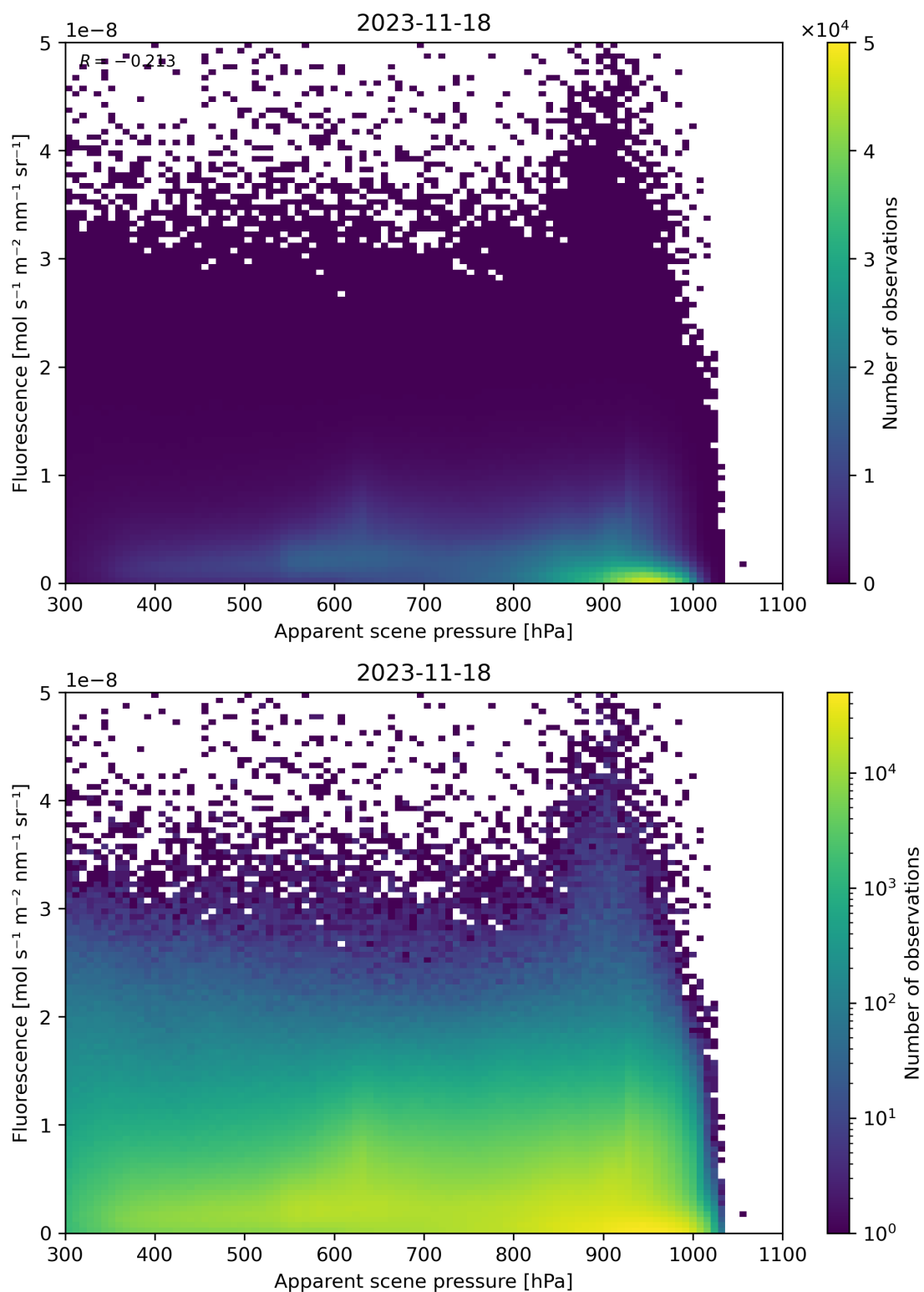
Figure 65: Scatter density plot of “Apparent scene pressure” against “Fluorescence” for 2023-11-18 to 2023-11-19.
