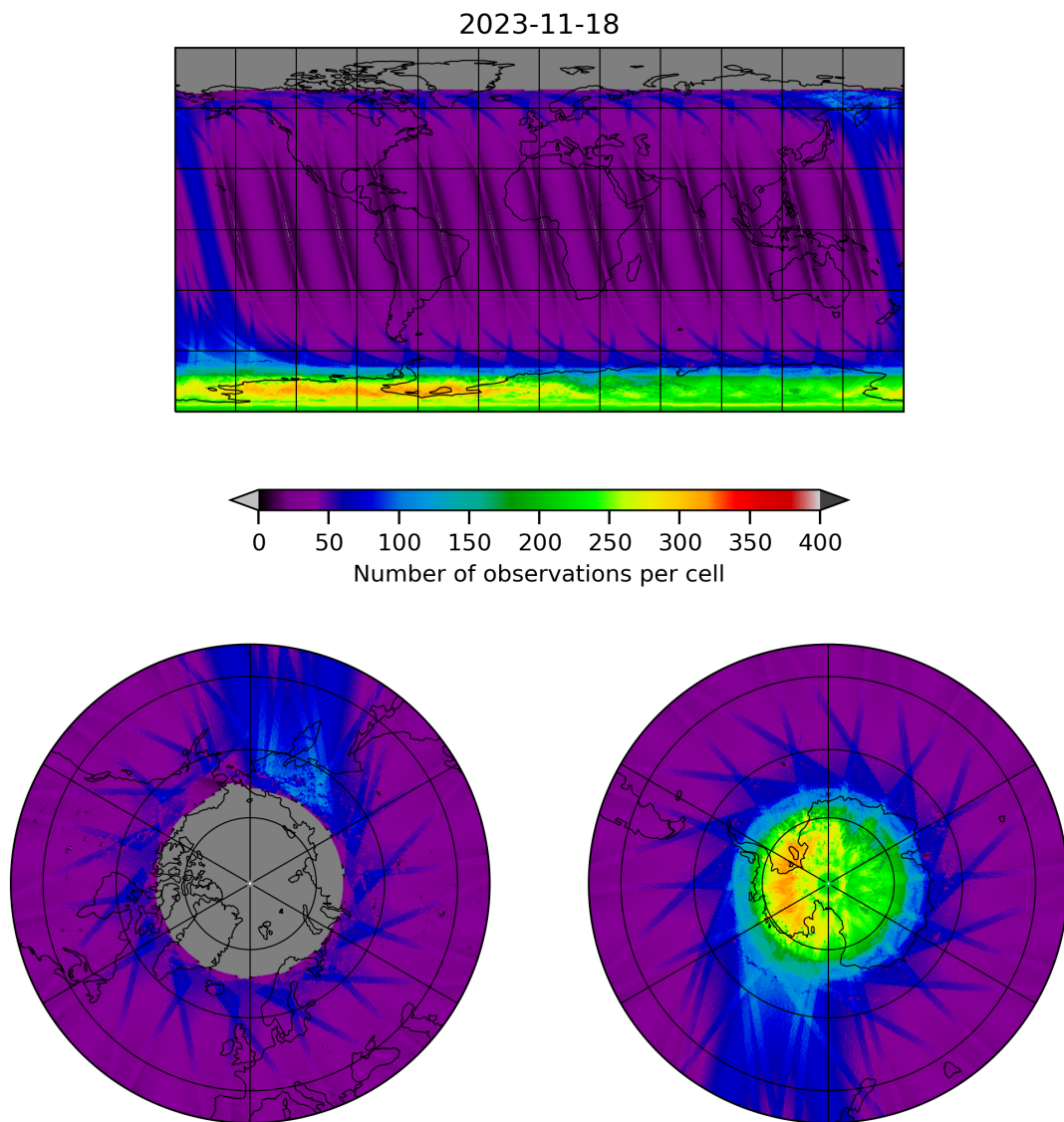
Figure 11: Map of the number of observations for 2023-11-18 to 2023-11-19
