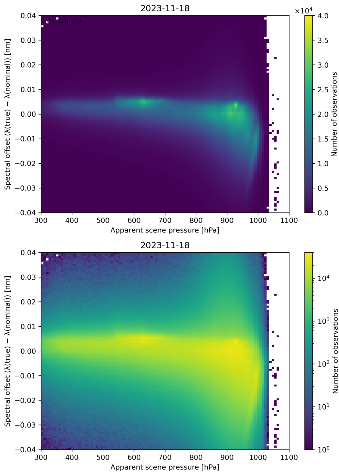
Figure 68: Scatter density plot of “Apparent scene pressure” against “Spectral offset ( \lambda(\text{true}) - \lambda(\text{nominal}) )” for 2023-11-18 to 2023-11-19.
