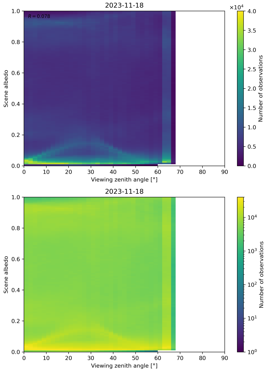
Figure 138: Scatter density plot of “Viewing zenith angle” against “Scene albedo” for 2023-11-18 to 2023-11-19.
