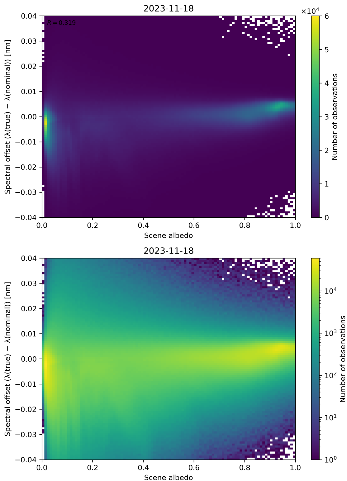
Figure 117: Scatter density plot of “Scene albedo” against “Spectral offset ( \lambda(\text{true}) - \lambda(\text{nominal}) )” for 2023-11-18 to 2023-11-19.
