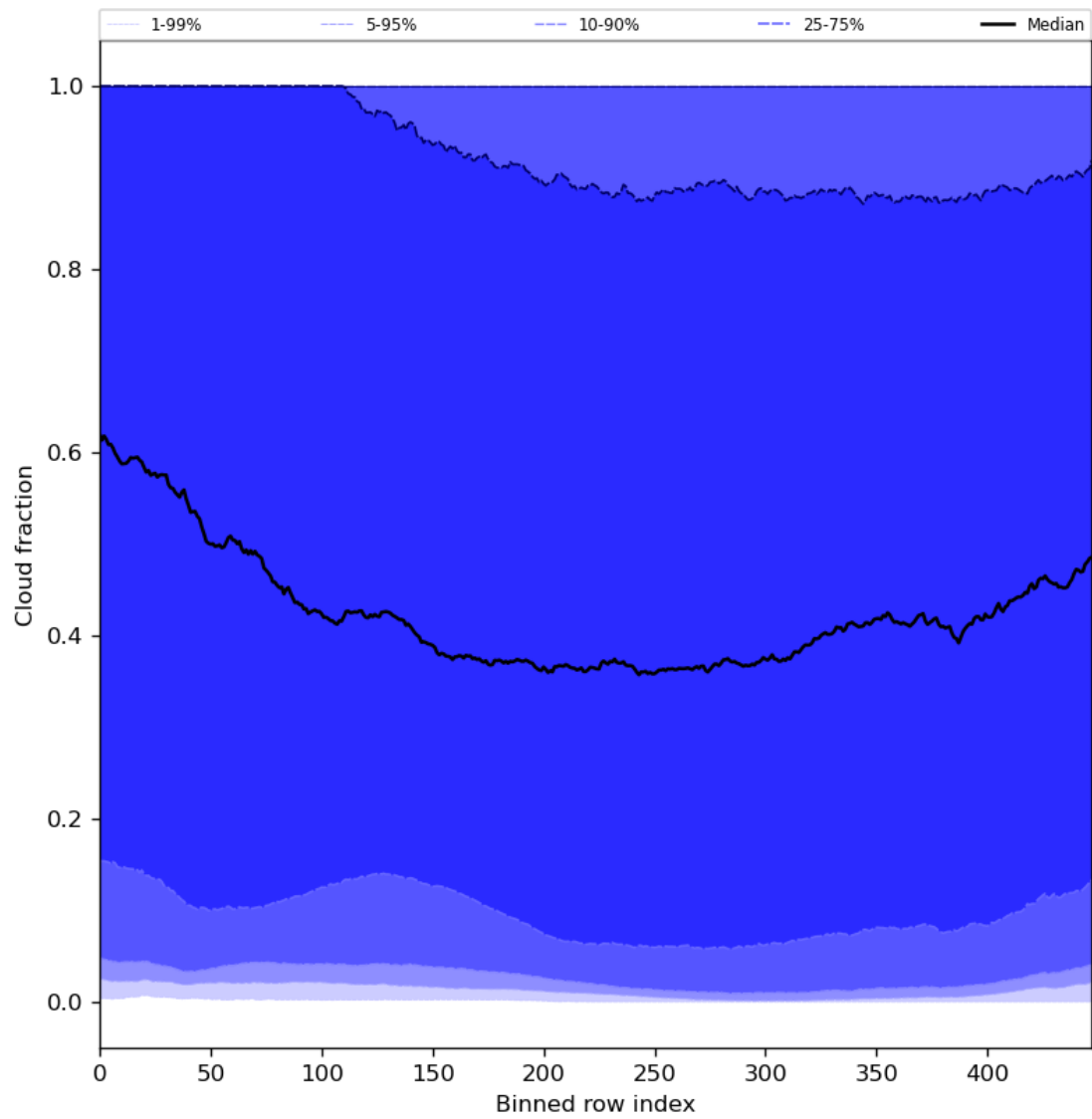
Figure 49: Along track statistics of “Cloud fraction” for 2023-11-18 to 2023-11-19
