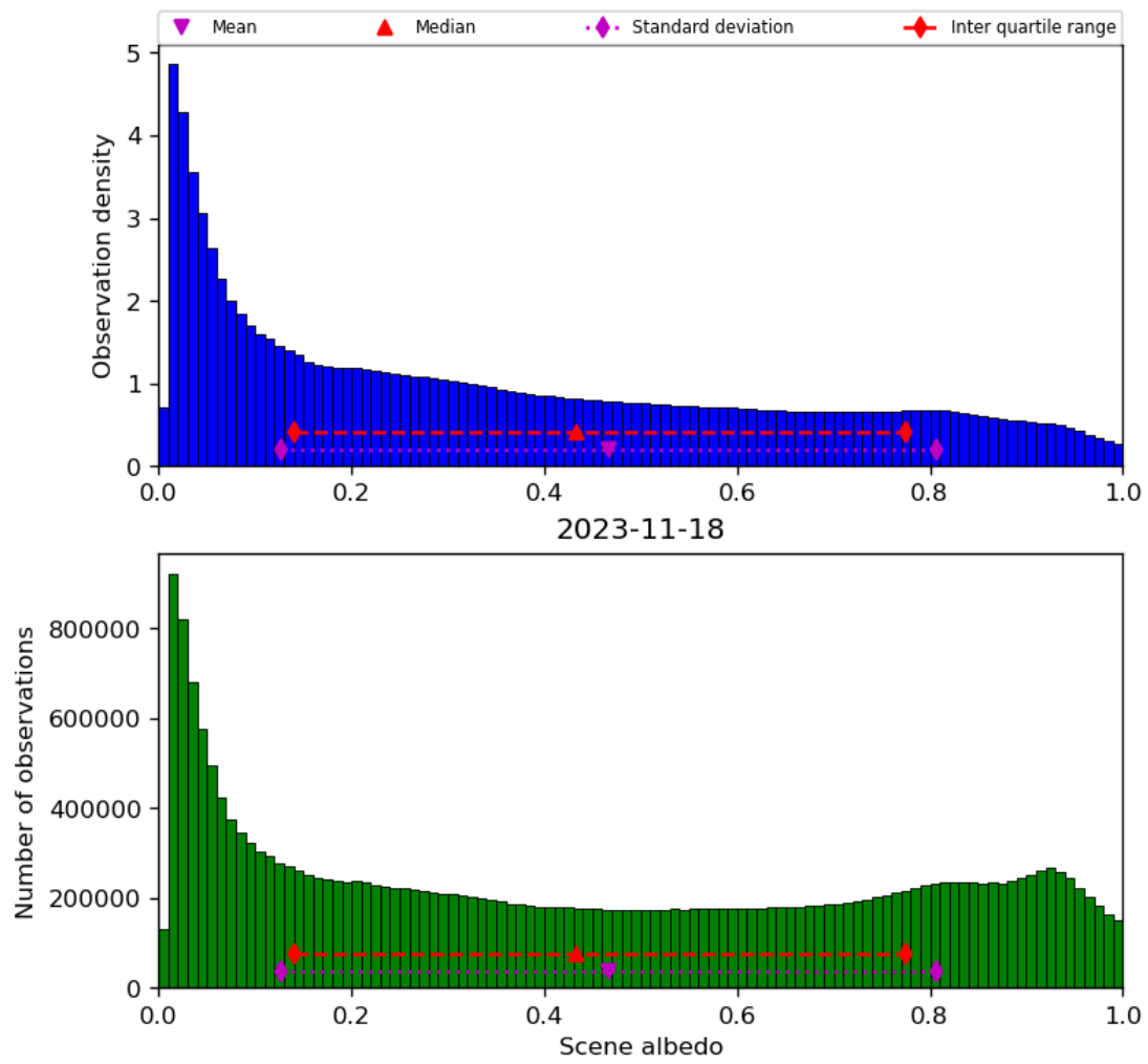
Figure 34: Histogram of “Scene albedo” for 2023-11-18 to 2023-11-19
