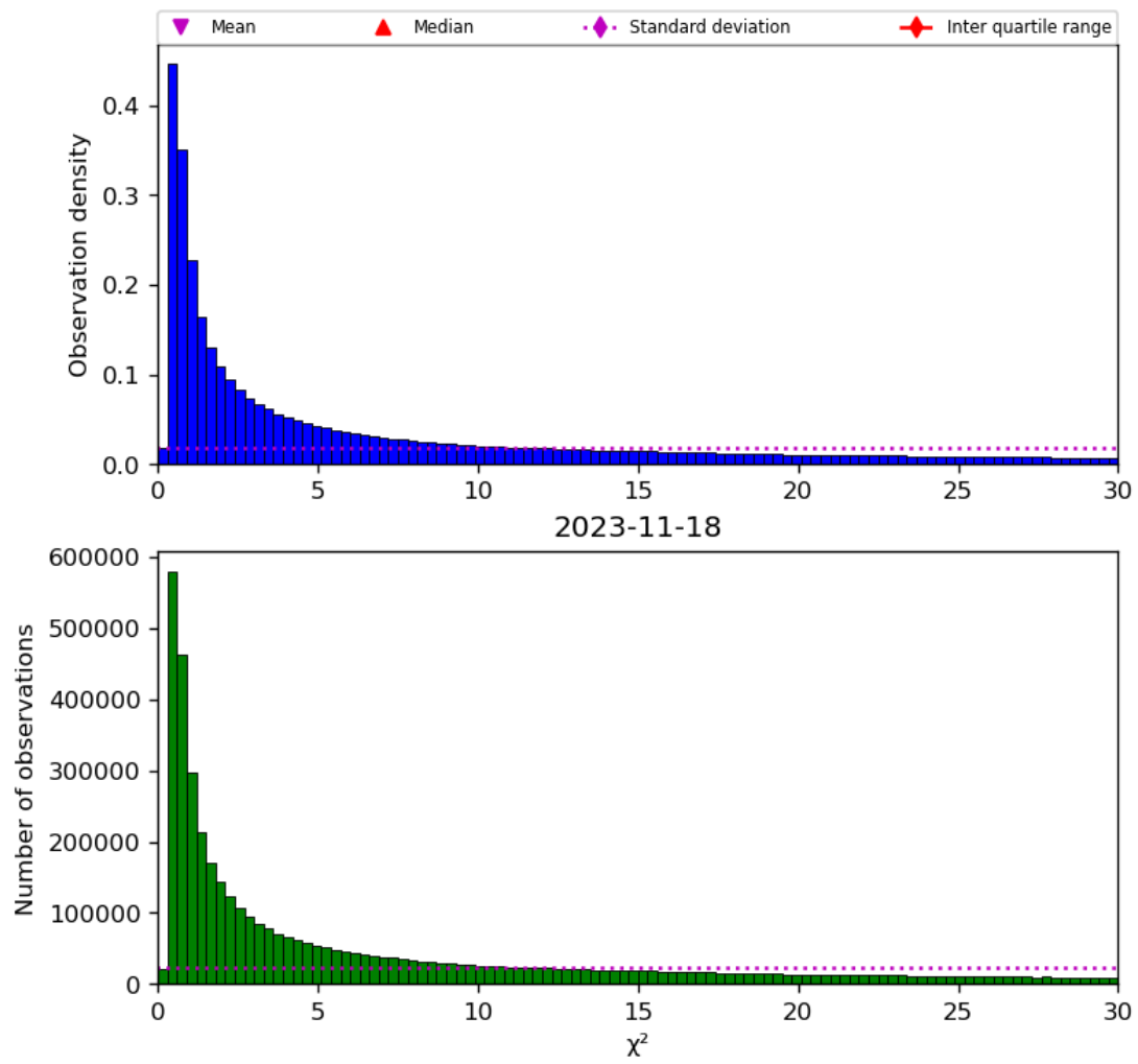
Figure 38: Histogram of “ \chi^2 ” for 2023-11-18 to 2023-11-19
