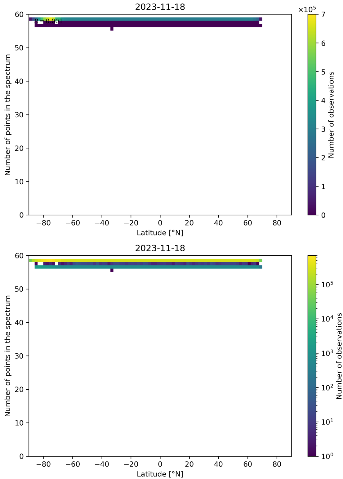
Figure 103: Scatter density plot of “Latitude” against “Number of points in the spectrum” for 2023-11-18 to 2023-11-19.
