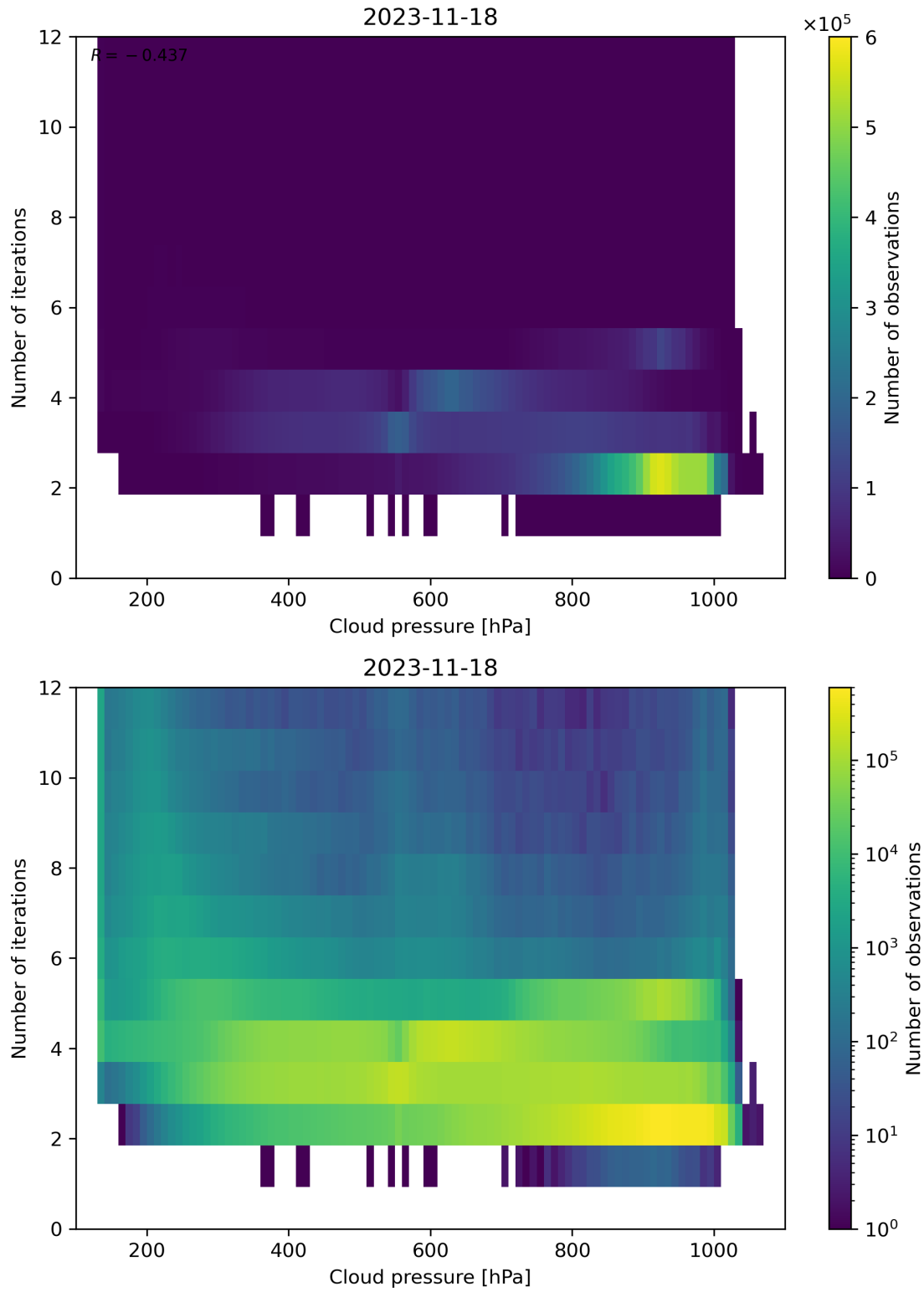
Figure 89: Scatter density plot of “Cloud pressure” against “Number of iterations” for 2023-11-18 to 2023-11-19.
