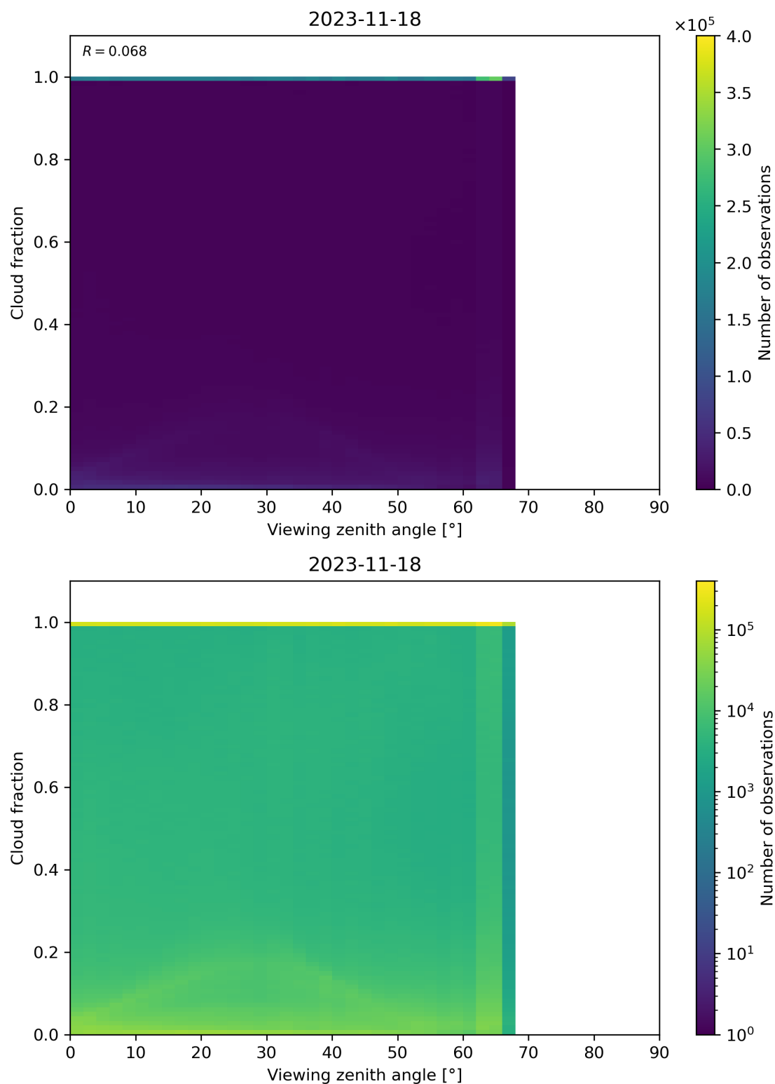
Figure 132: Scatter density plot of “Viewing zenith angle” against “Cloud fraction” for 2023-11-18 to 2023-11-19.
