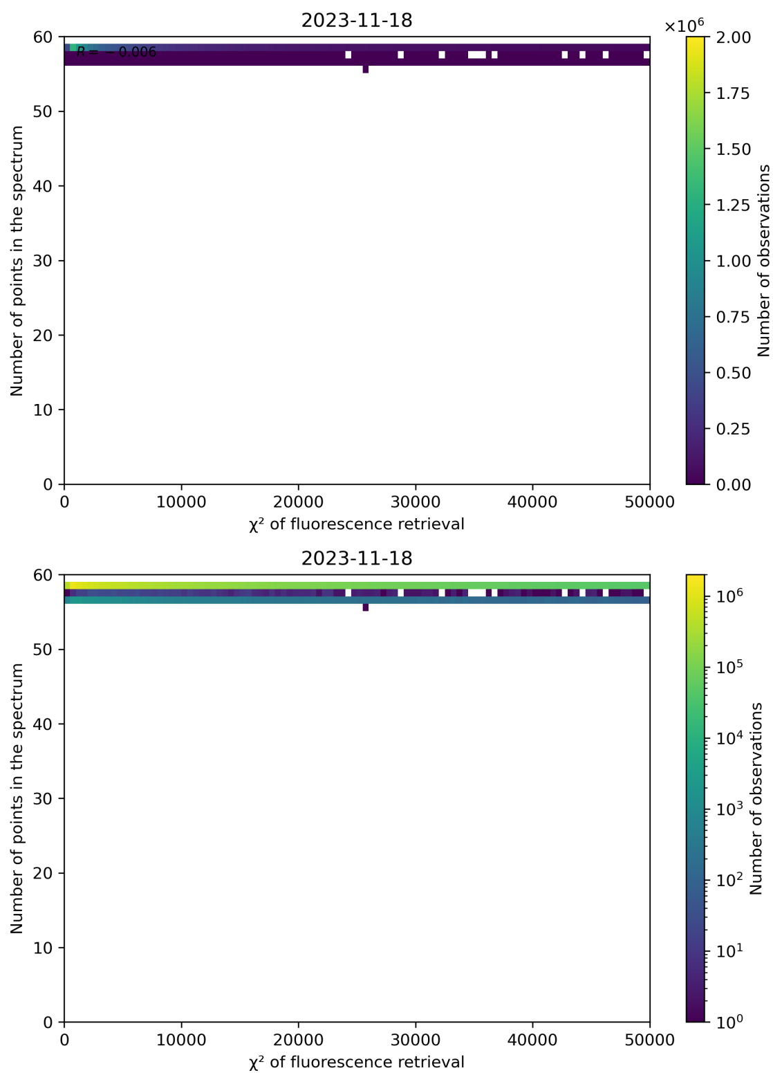
Figure 71: Scatter density plot of " \chi^2 of fluorescence retrieval" against "Number of points in the spectrum" for 2023-11-18 to 2023-11-19.
