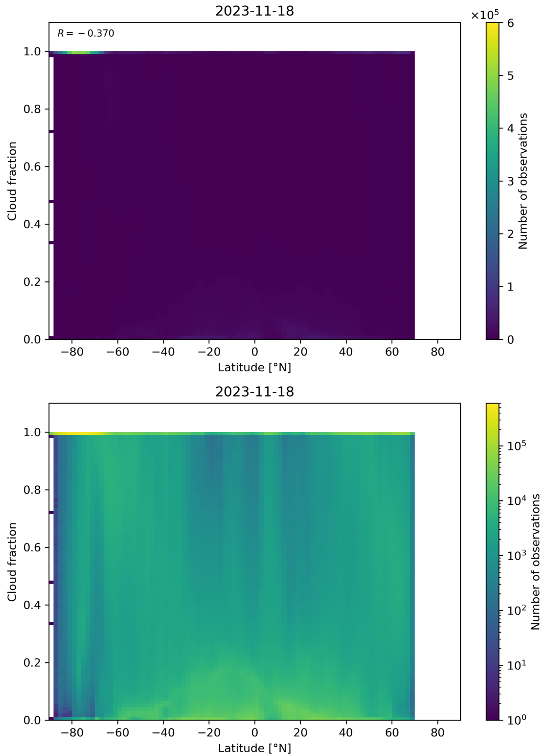
Figure 99: Scatter density plot of “Latitude” against “Cloud fraction” for 2023-11-18 to 2023-11-19.
