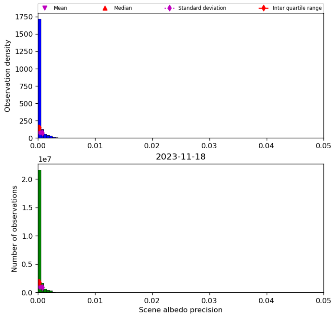
Figure 35: Histogram of “Scene albedo precision” for 2023-11-18 to 2023-11-19
