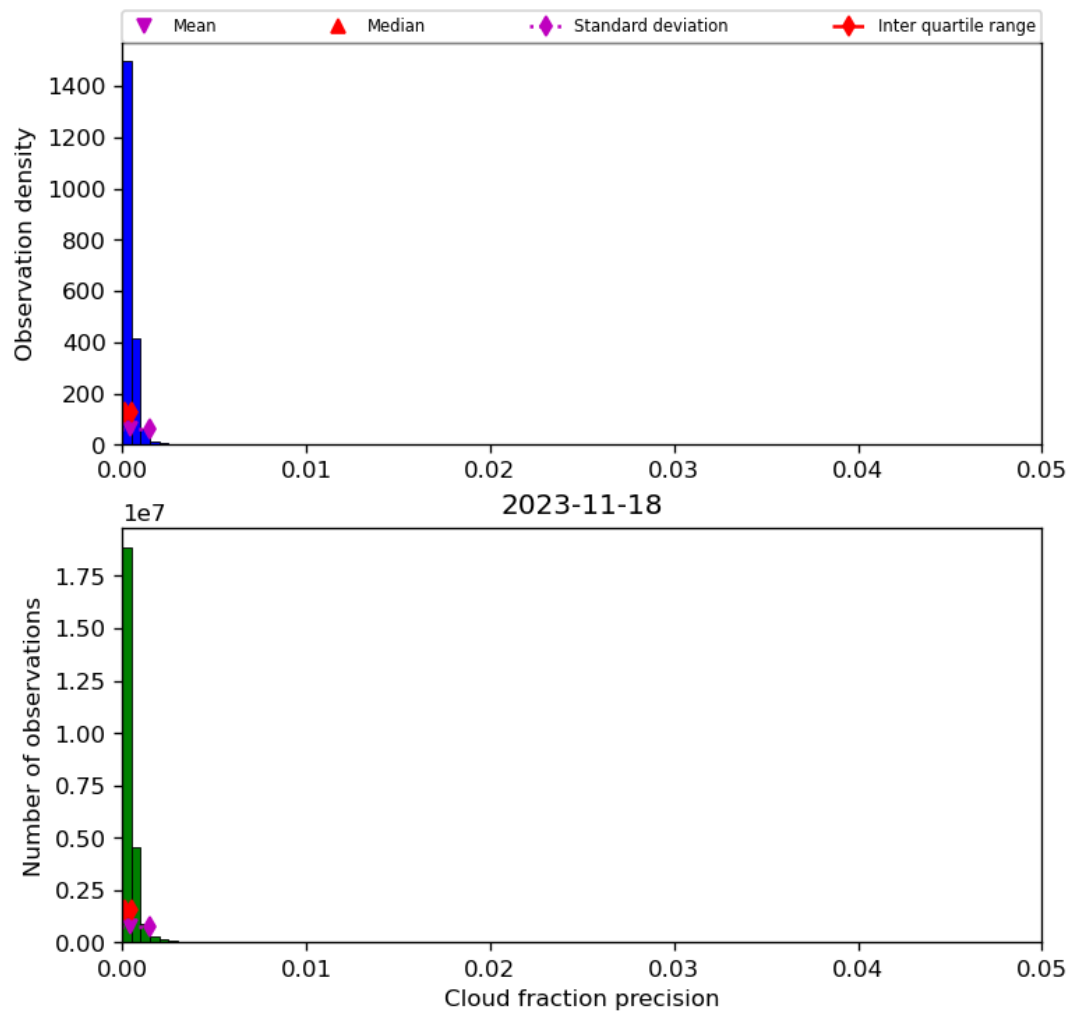
Figure 33: Histogram of “Cloud fraction precision” for 2023-11-18 to 2023-11-19
