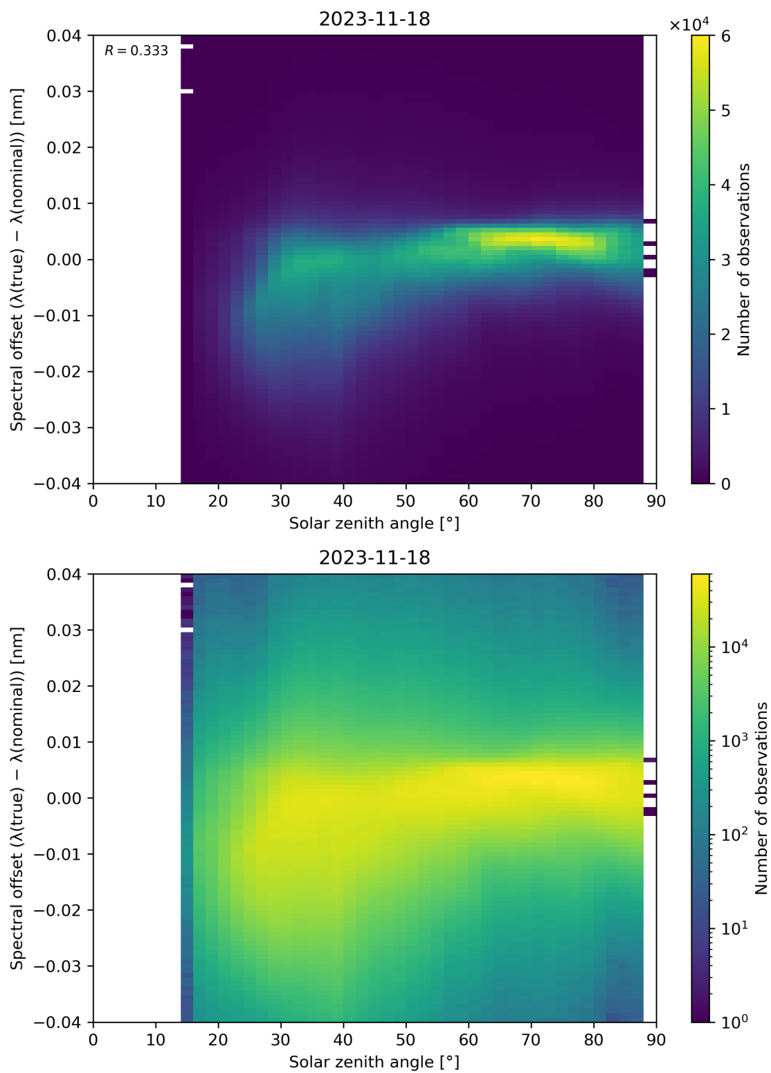
Figure 128: Scatter density plot of “Solar zenith angle” against “Spectral offset ( \lambda(\text{true}) - \lambda(\text{nominal}) )” for 2023-11-18 to 2023-11-19.
