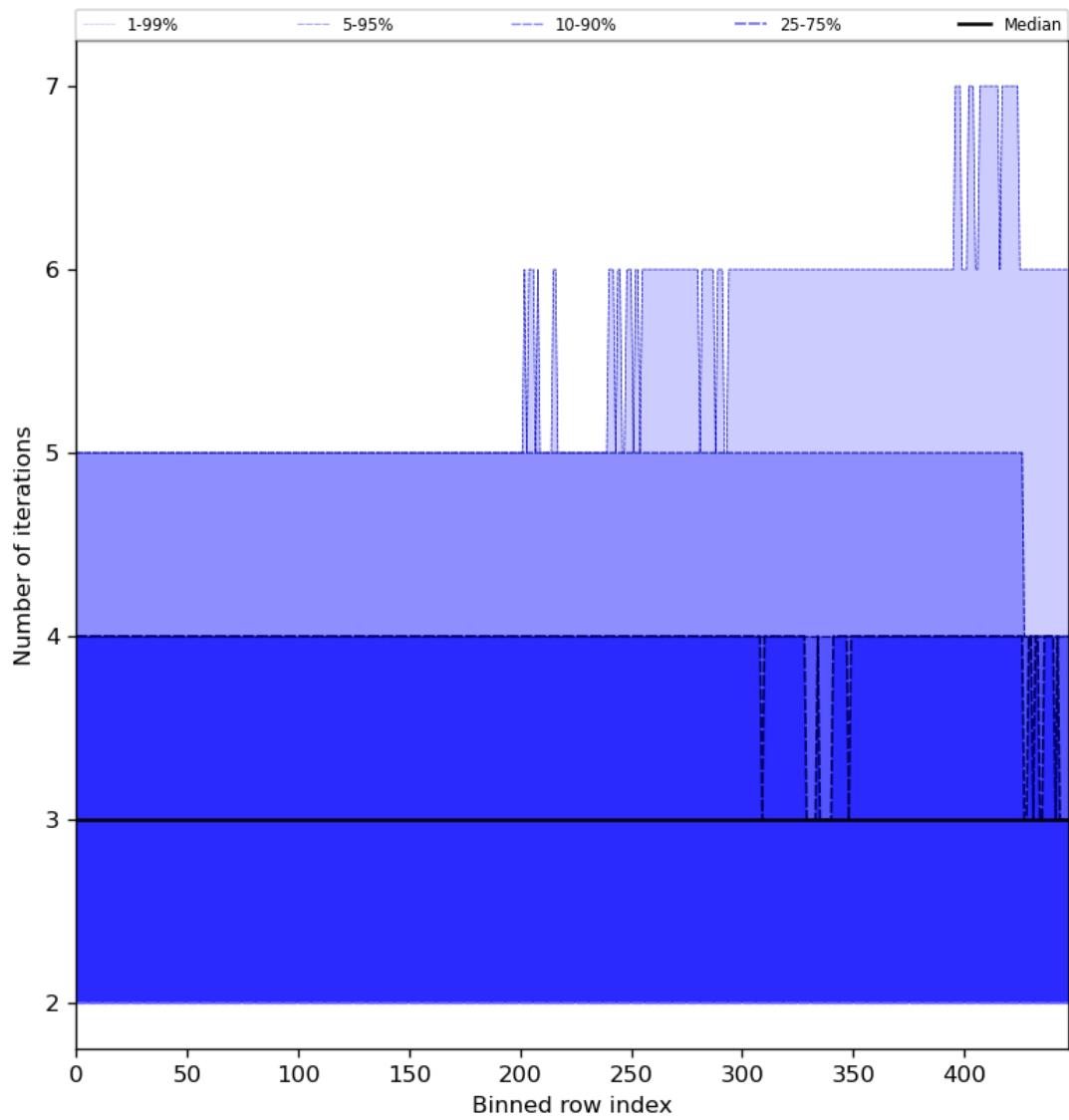
Figure 56: Along track statistics of “Number of iterations” for 2023-11-18 to 2023-11-19
