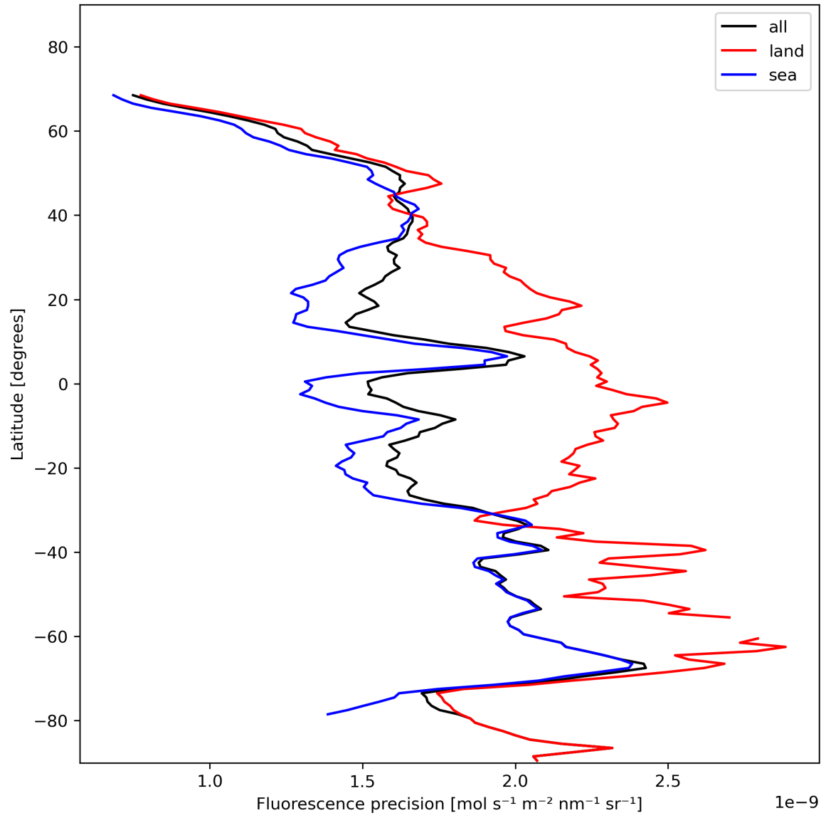
Figure 24: Zonal average of “Fluorescence precision” for 2023-11-18 to 2023-11-19.
