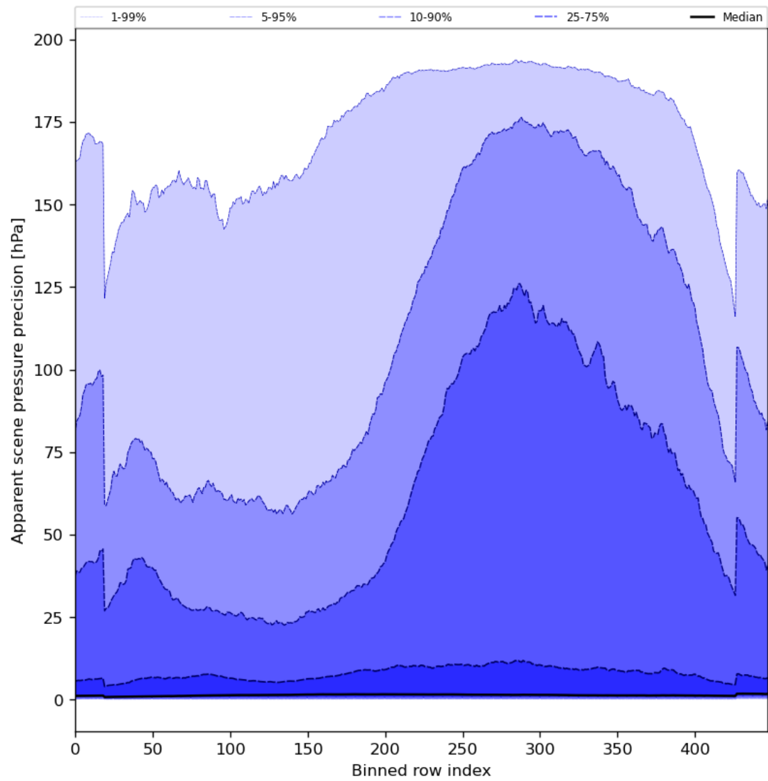
Figure 54: Along track statistics of “Apparent scene pressure precision” for 2023-11-18 to 2023-11-19
