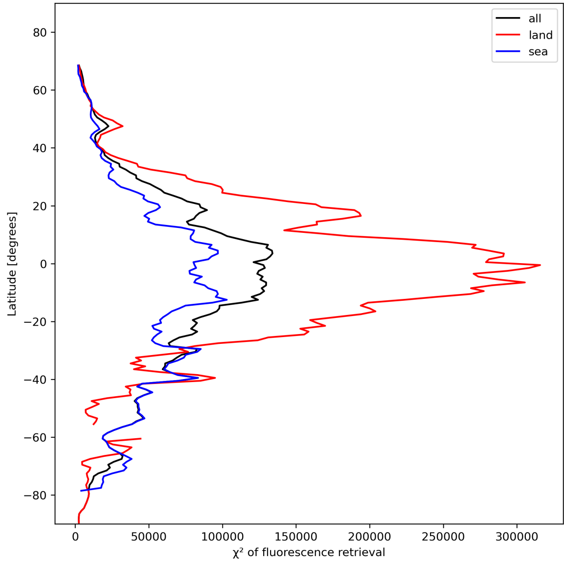
Figure 25: Zonal average of “ \chi^2 of fluorescence retrieval” for 2023-11-18 to 2023-11-19.
