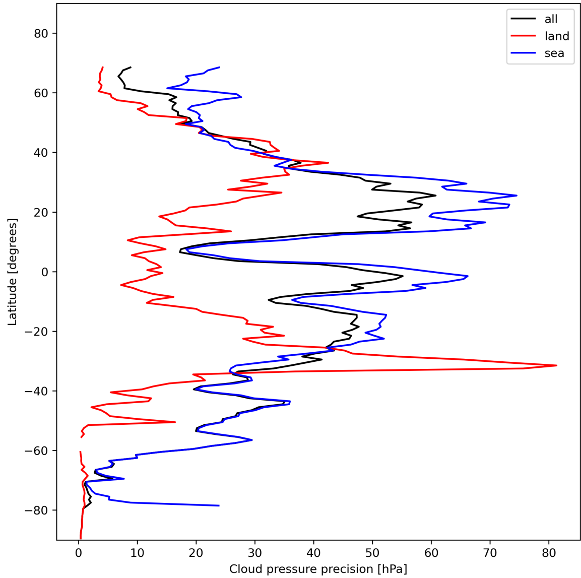
Figure 14: Zonal average of “Cloud pressure precision” for 2023-11-18 to 2023-11-19.
