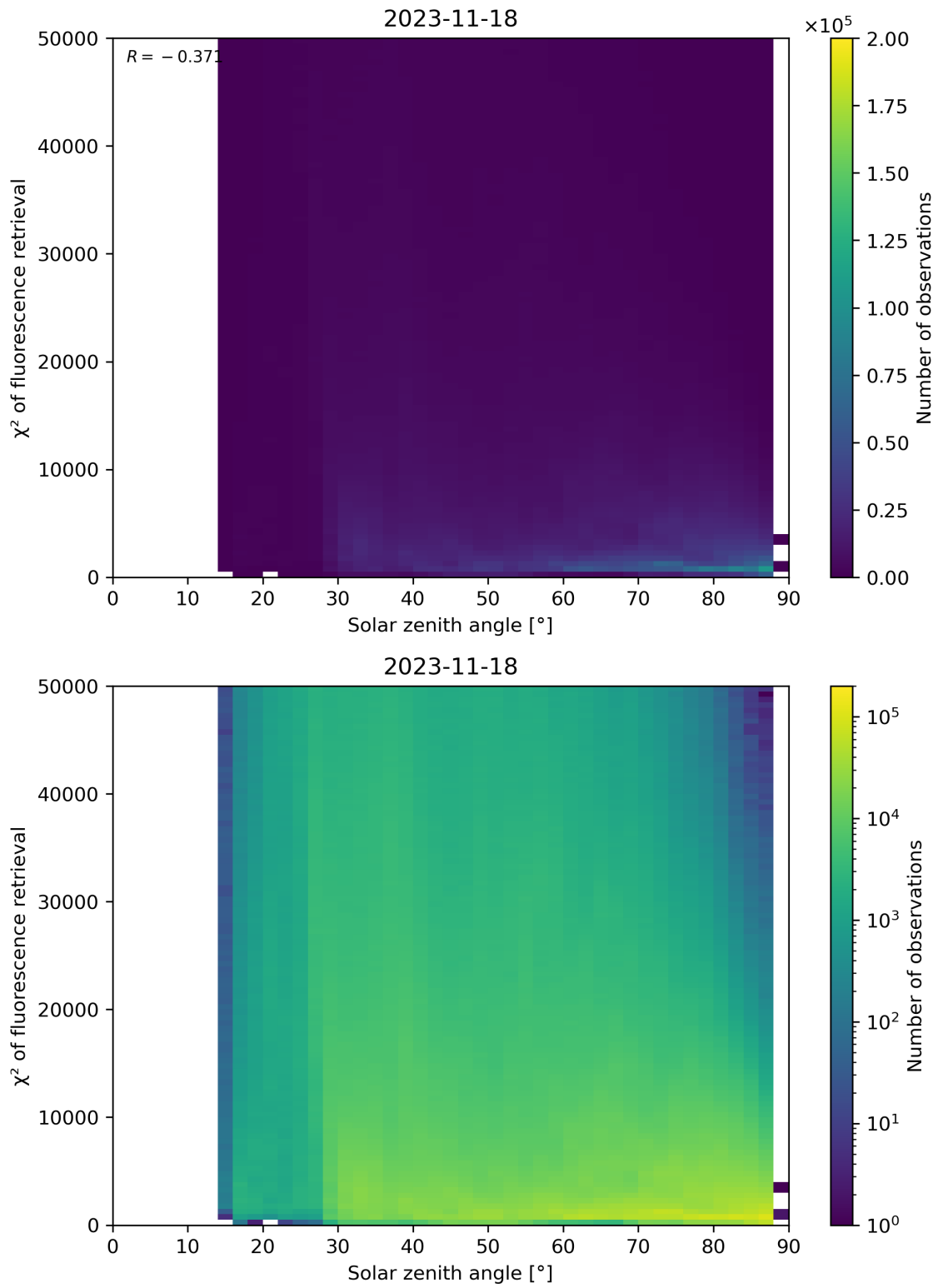
Figure 120: Scatter density plot of “Solar zenith angle” against “ \chi^2 of fluorescence retrieval” for 2023-11-18 to 2023-11-19.
