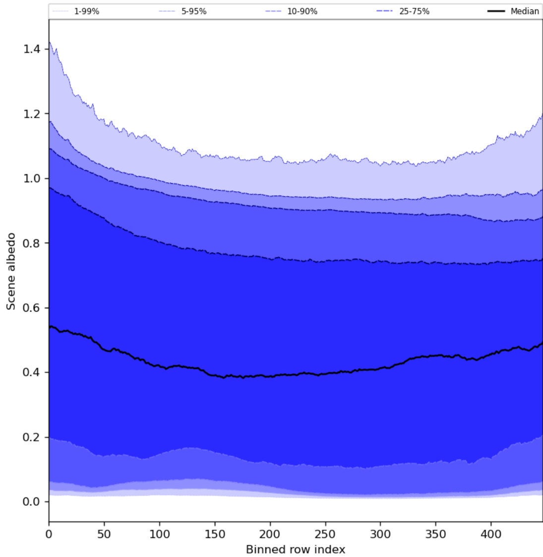
Figure 51: Along track statistics of “Scene albedo” for 2023-11-18 to 2023-11-19
