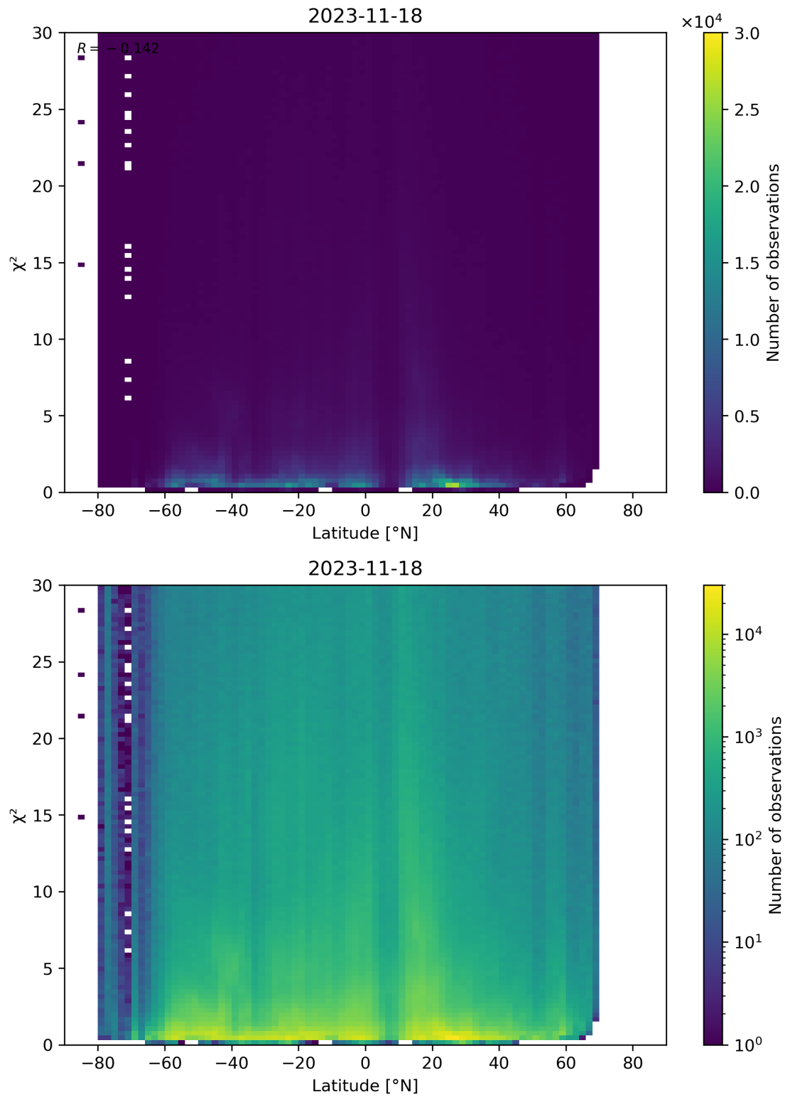
Figure 97: Scatter density plot of “Latitude” against “ \chi^2 ” for 2023-11-18 to 2023-11-19.
