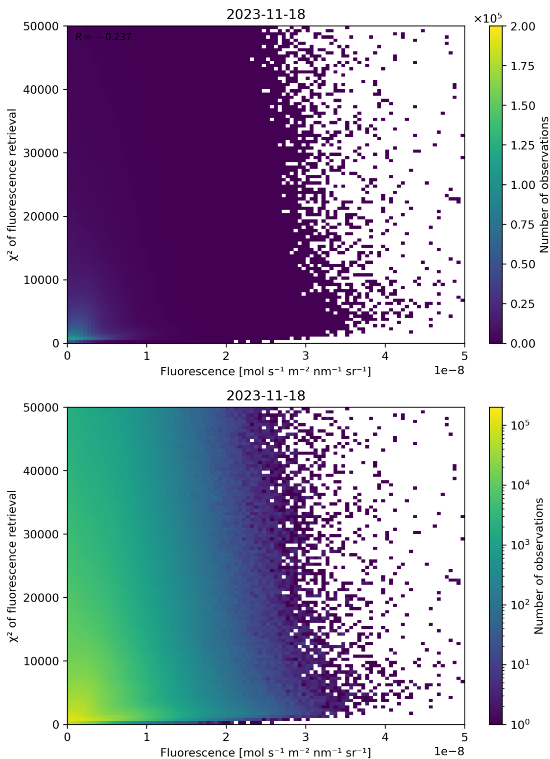
Figure 93: Scatter density plot of “Fluorescence” against “ \chi^2 of fluorescence retrieval” for 2023-11-18 to 2023-11-19.
