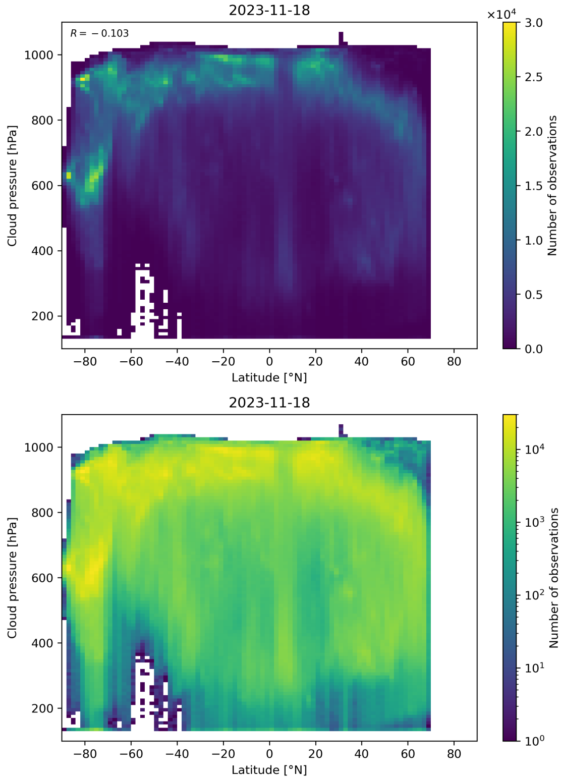
Figure 100: Scatter density plot of “Latitude” against “Cloud pressure” for 2023-11-18 to 2023-11-19.
