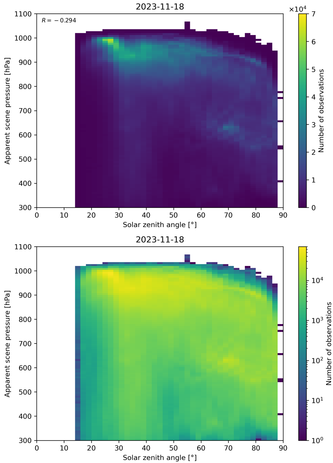
Figure 118: Scatter density plot of “Solar zenith angle” against “Apparent scene pressure” for 2023-11-18 to 2023-11-19.
