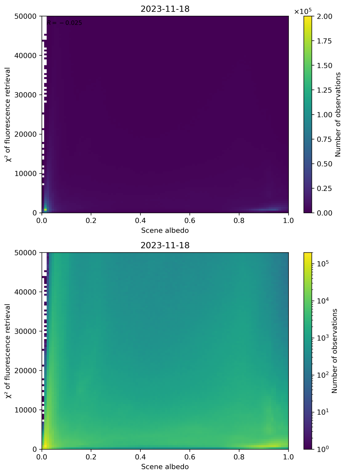
Figure 113: Scatter density plot of “Scene albedo” against “ \chi^2 of fluorescence retrieval” for 2023-11-18 to 2023-11-19.
