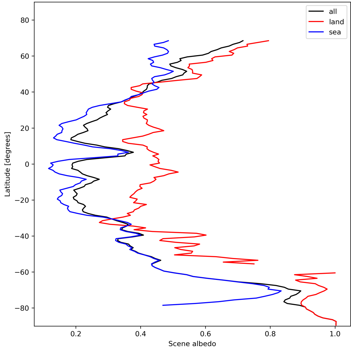
Figure 17: Zonal average of “Scene albedo” for 2023-11-18 to 2023-11-19.
