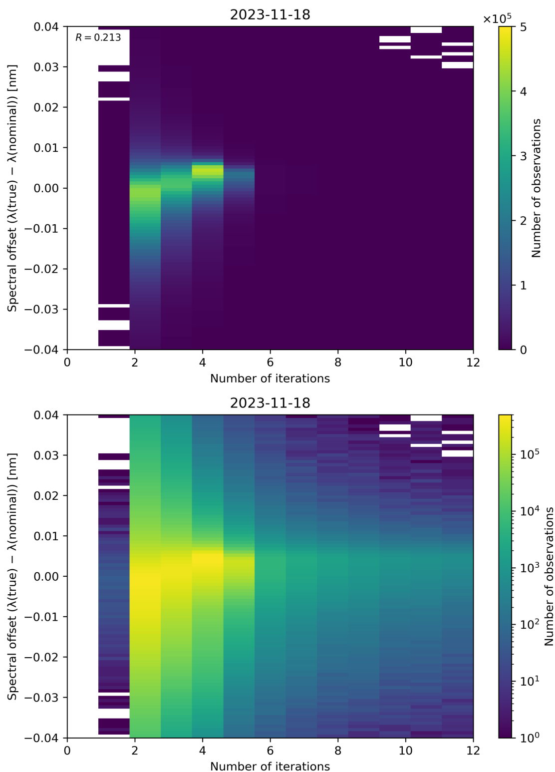
Figure 109: Scatter density plot of “Number of iterations” against “Spectral offset ( \lambda(\text{true}) - \lambda(\text{nominal}) )” for 2023-11-18 to 2023-11-19.
