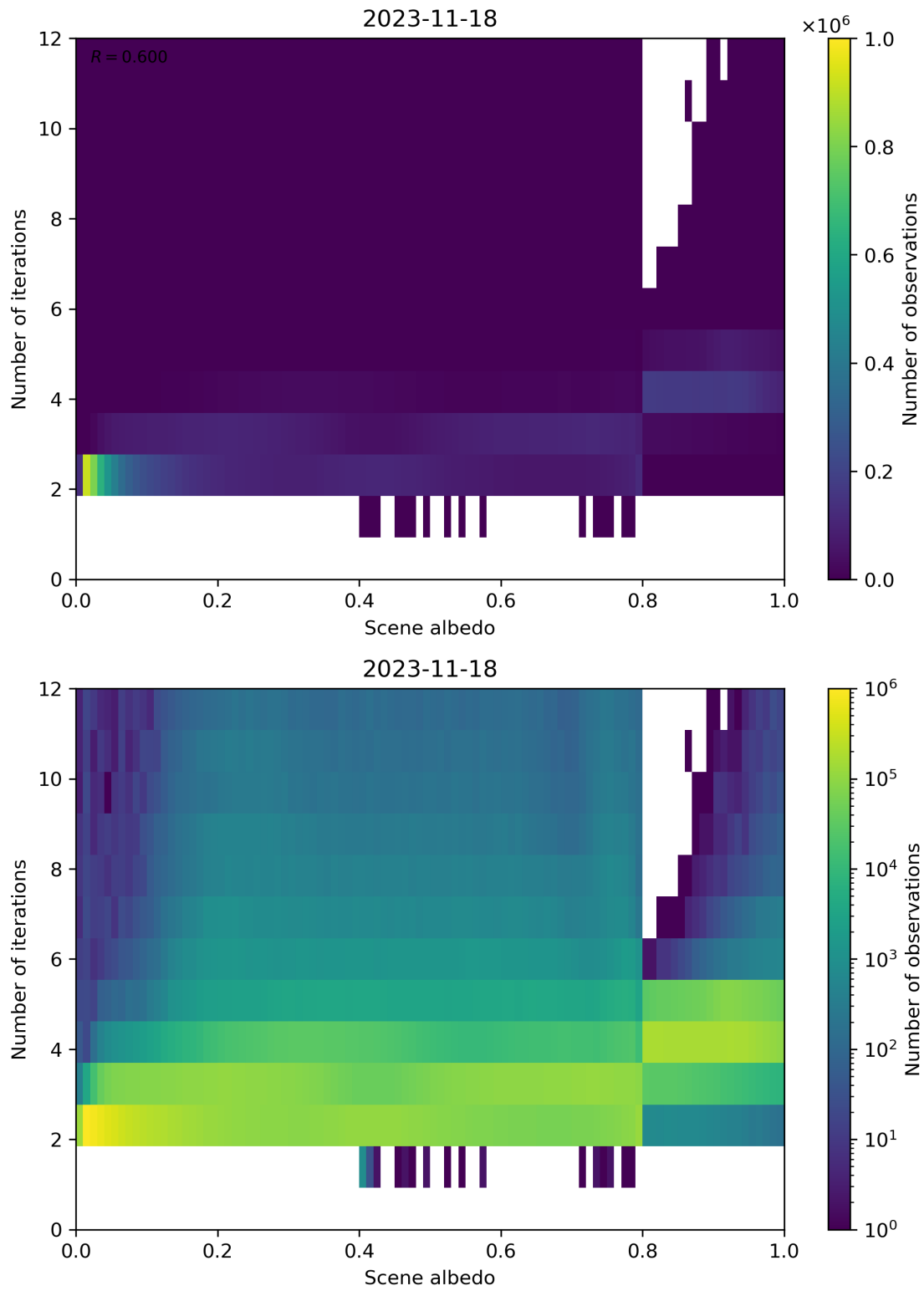
Figure 115: Scatter density plot of “Scene albedo” against “Number of iterations” for 2023-11-18 to 2023-11-19.
