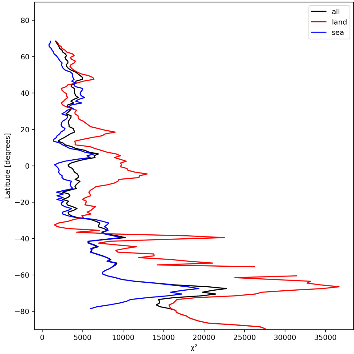
Figure 21: Zonal average of “ \chi^2 ” for 2023-11-18 to 2023-11-19.
