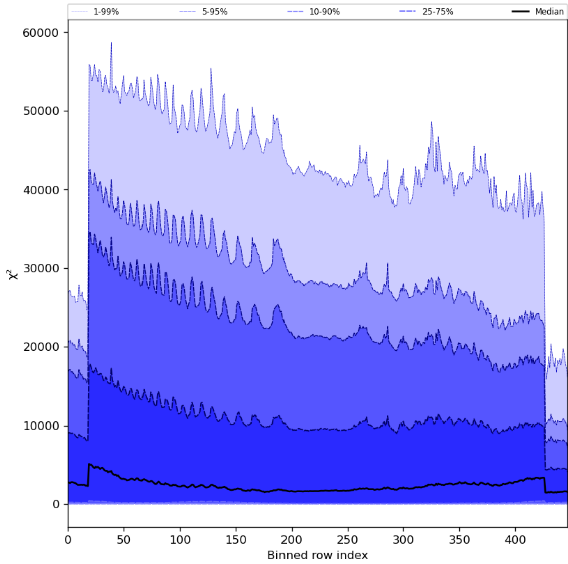
Figure 55: Along track statistics of “ \chi^2 ” for 2023-11-18 to 2023-11-19
