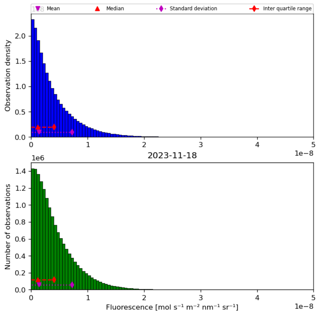
Figure 40: Histogram of “Fluorescence” for 2023-11-18 to 2023-11-19
