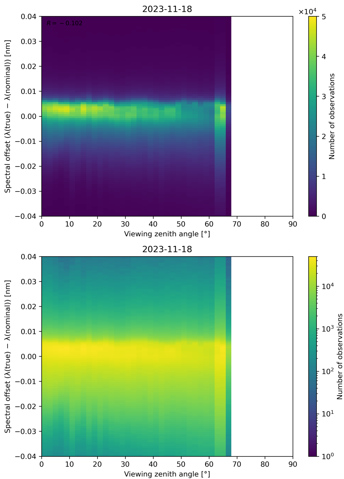
Figure 140: Scatter density plot of “Viewing zenith angle” against “Spectral offset ( \lambda(\text{true}) - \lambda(\text{nominal}) )” for 2023-11-18 to 2023-11-19.
