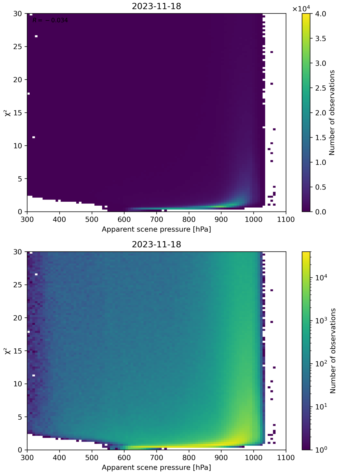
Figure 63: Scatter density plot of “Apparent scene pressure” against “ \chi^2 ” for 2023-11-18 to 2023-11-19.
