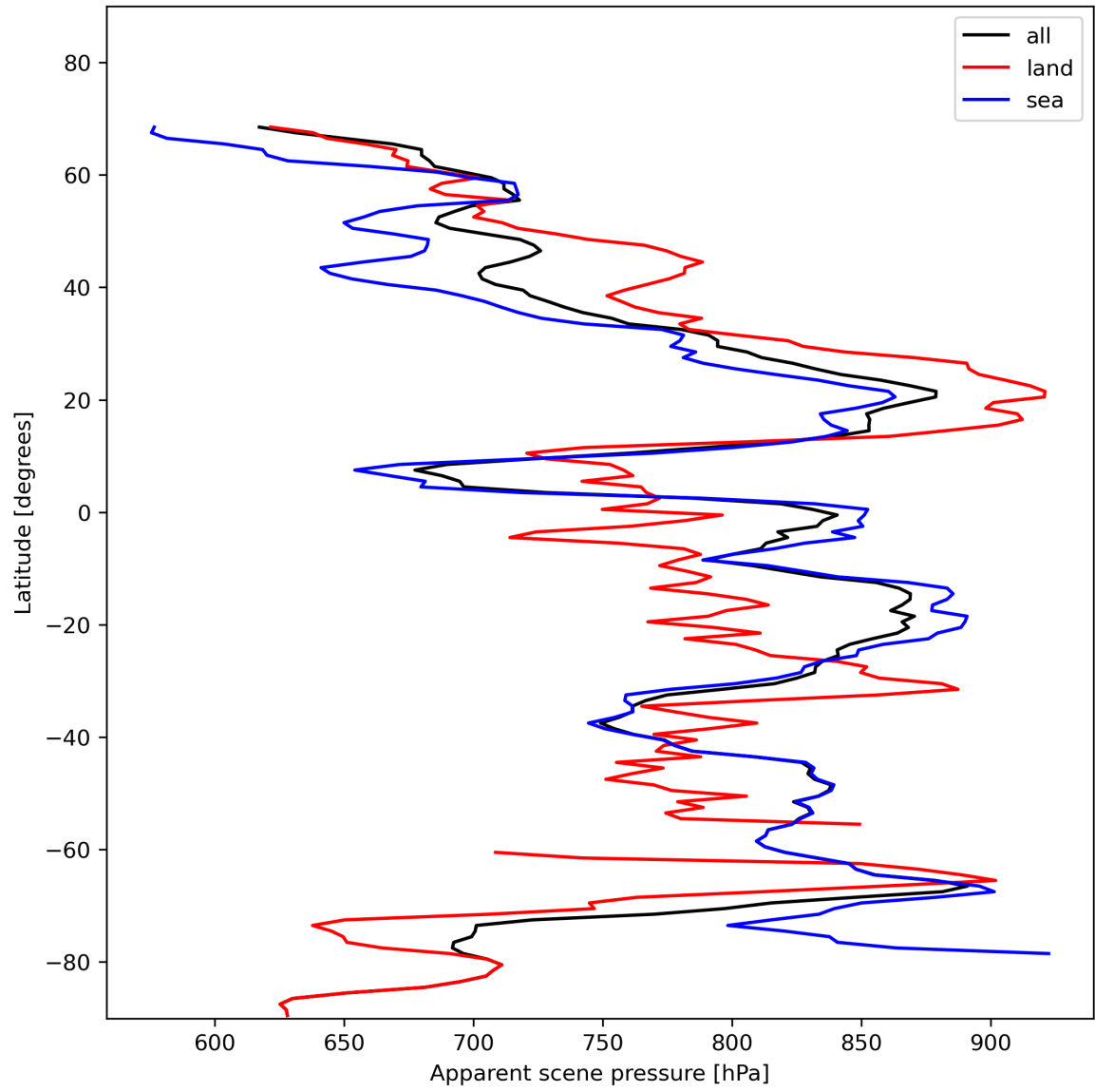
Figure 19: Zonal average of “Apparent scene pressure” for 2023-11-18 to 2023-11-19.
