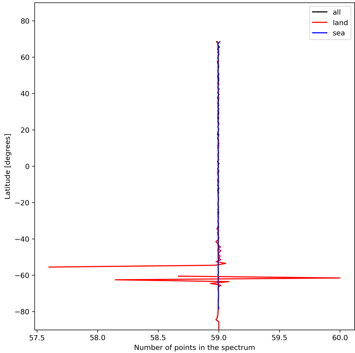
Figure 27: Zonal average of “Number of points in the spectrum” for 2023-11-18 to 2023-11-19.
