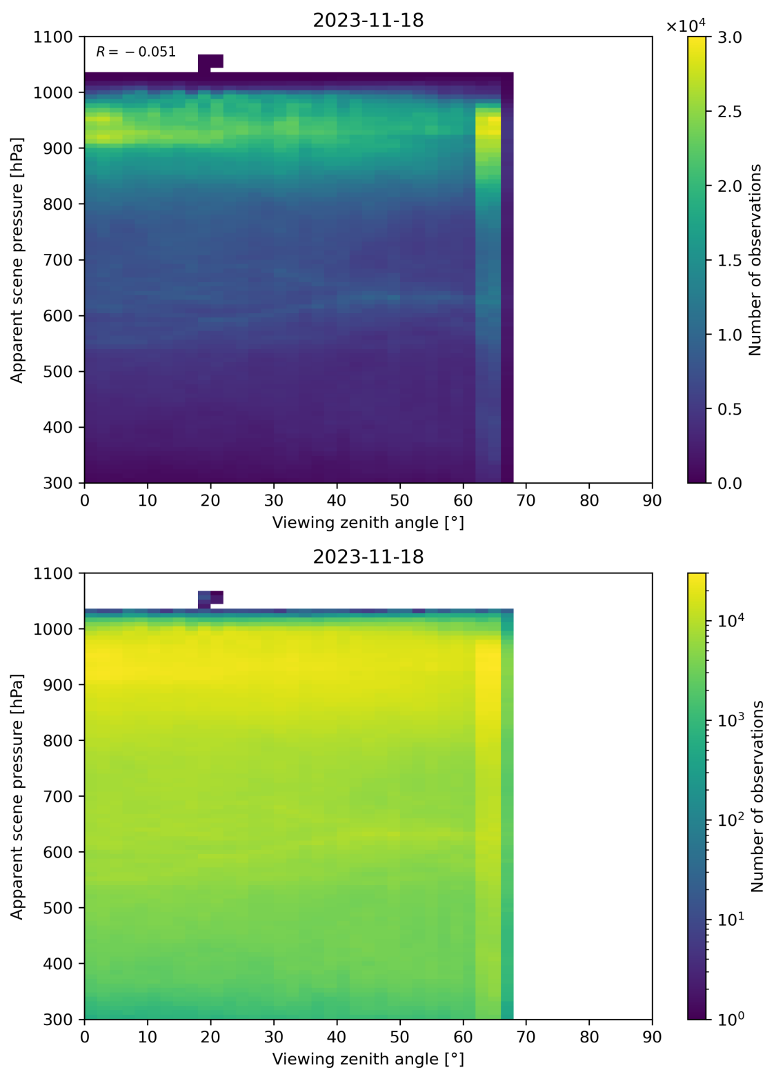
Figure 129: Scatter density plot of “Viewing zenith angle” against “Apparent scene pressure” for 2023-11-18 to 2023-11-19.
