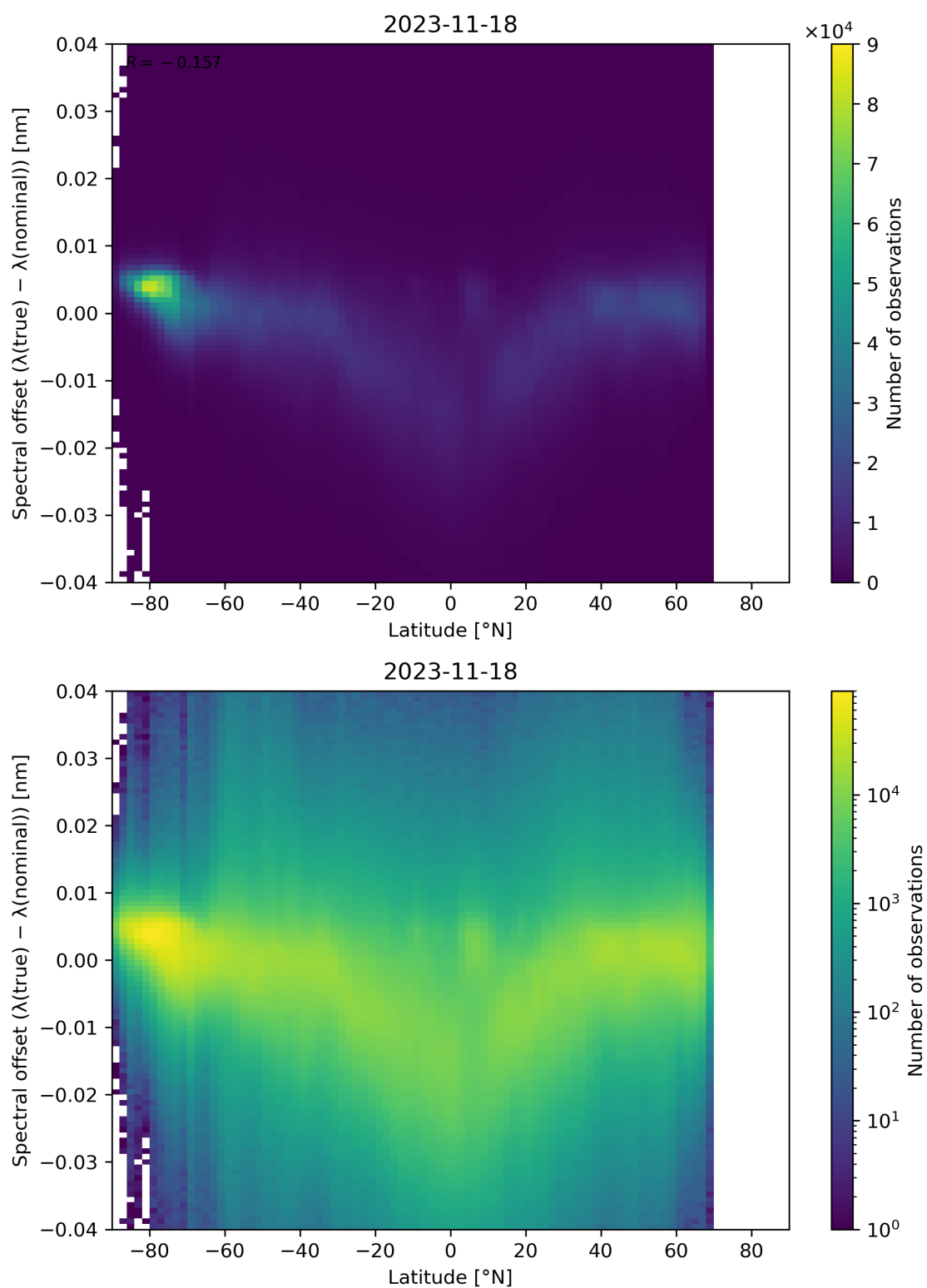
Figure 105: Scatter density plot of “Latitude” against “Spectral offset ( \lambda(\text{true}) - \lambda(\text{nominal}) )” for 2023-11-18 to 2023-11-19.
