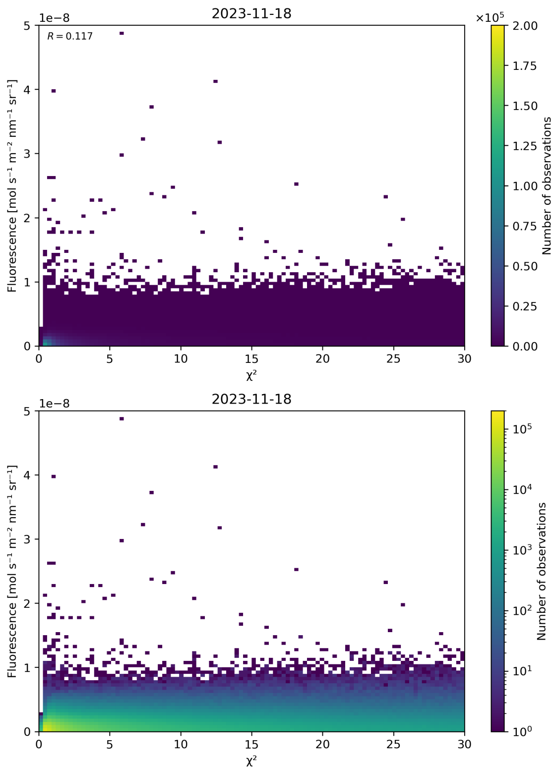
Figure 70: Scatter density plot of “ \chi^2 ” against “Fluorescence” for 2023-11-18 to 2023-11-19.
