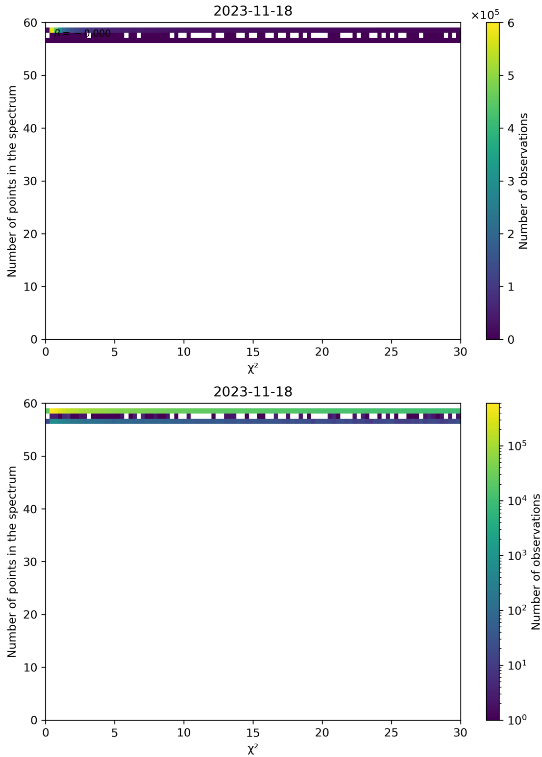
Figure 74: Scatter density plot of " \chi^2 " against "Number of points in the spectrum" for 2023-11-18 to 2023-11-19.
