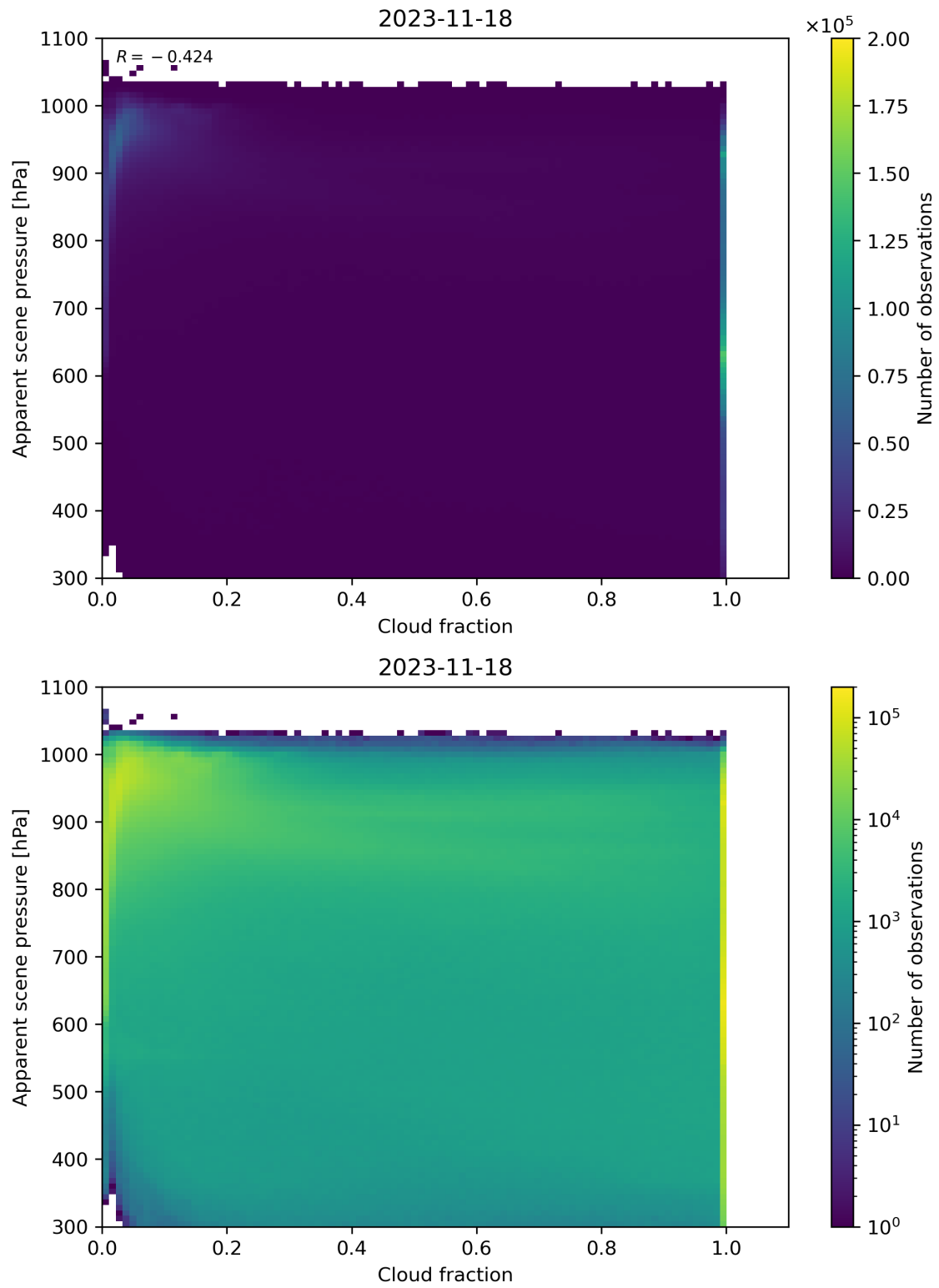
Figure 76: Scatter density plot of “Cloud fraction” against “Apparent scene pressure” for 2023-11-18 to 2023-11-19.
