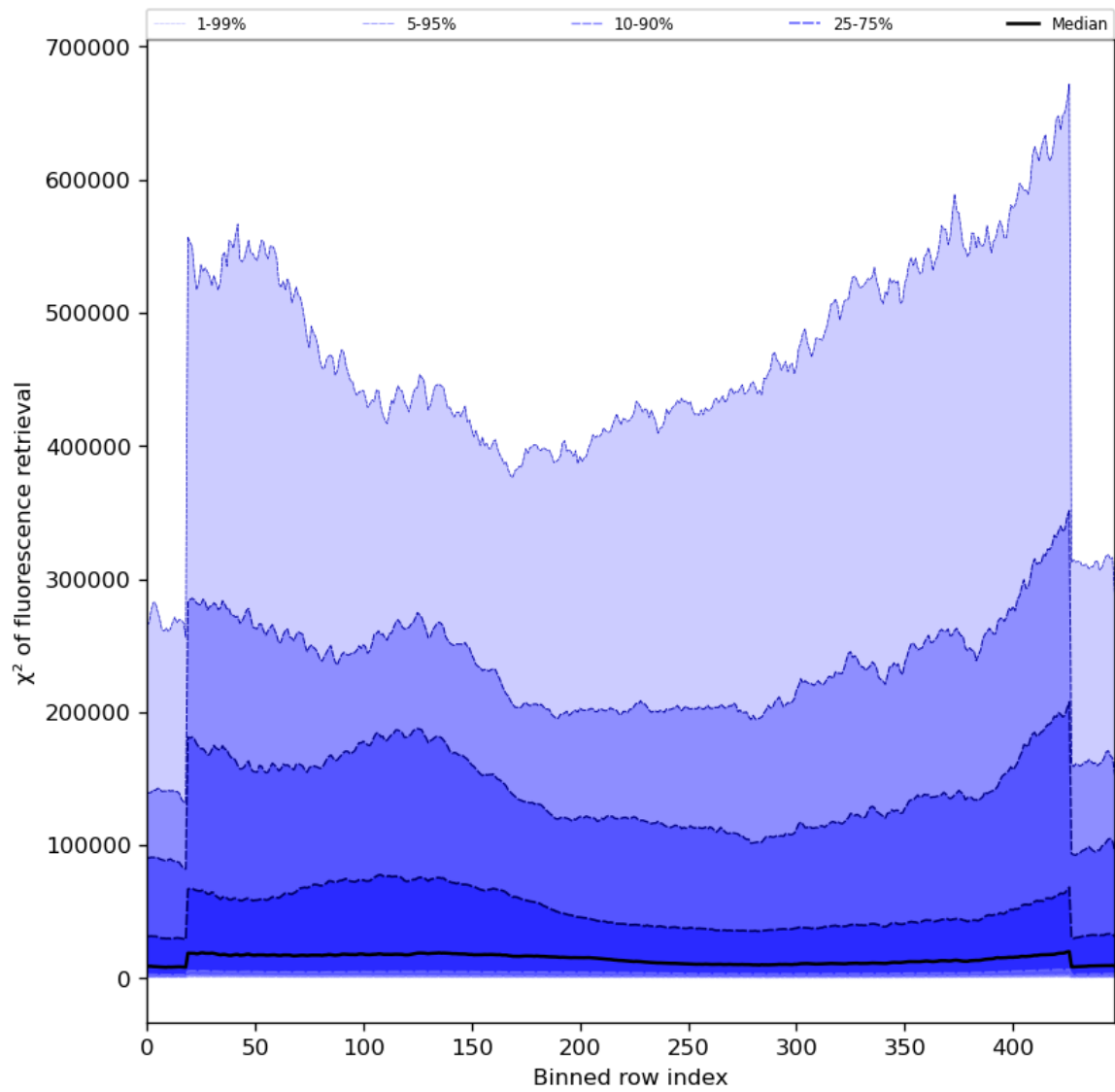
Figure 59: Along track statistics of “ \chi^2 of fluorescence retrieval” for 2023-11-18 to 2023-11-19
