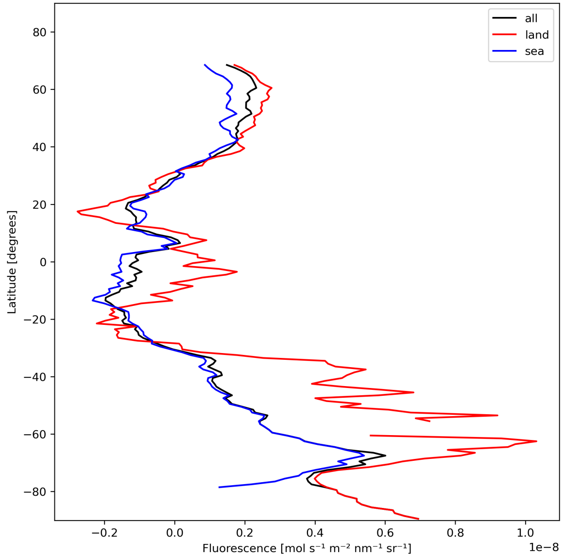
Figure 23: Zonal average of “Fluorescence” for 2023-11-18 to 2023-11-19.
