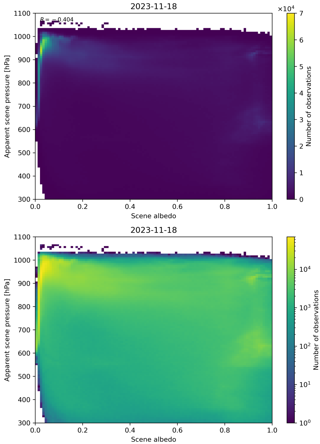
Figure 111: Scatter density plot of “Scene albedo” against “Apparent scene pressure” for 2023-11-18 to 2023-11-19.
