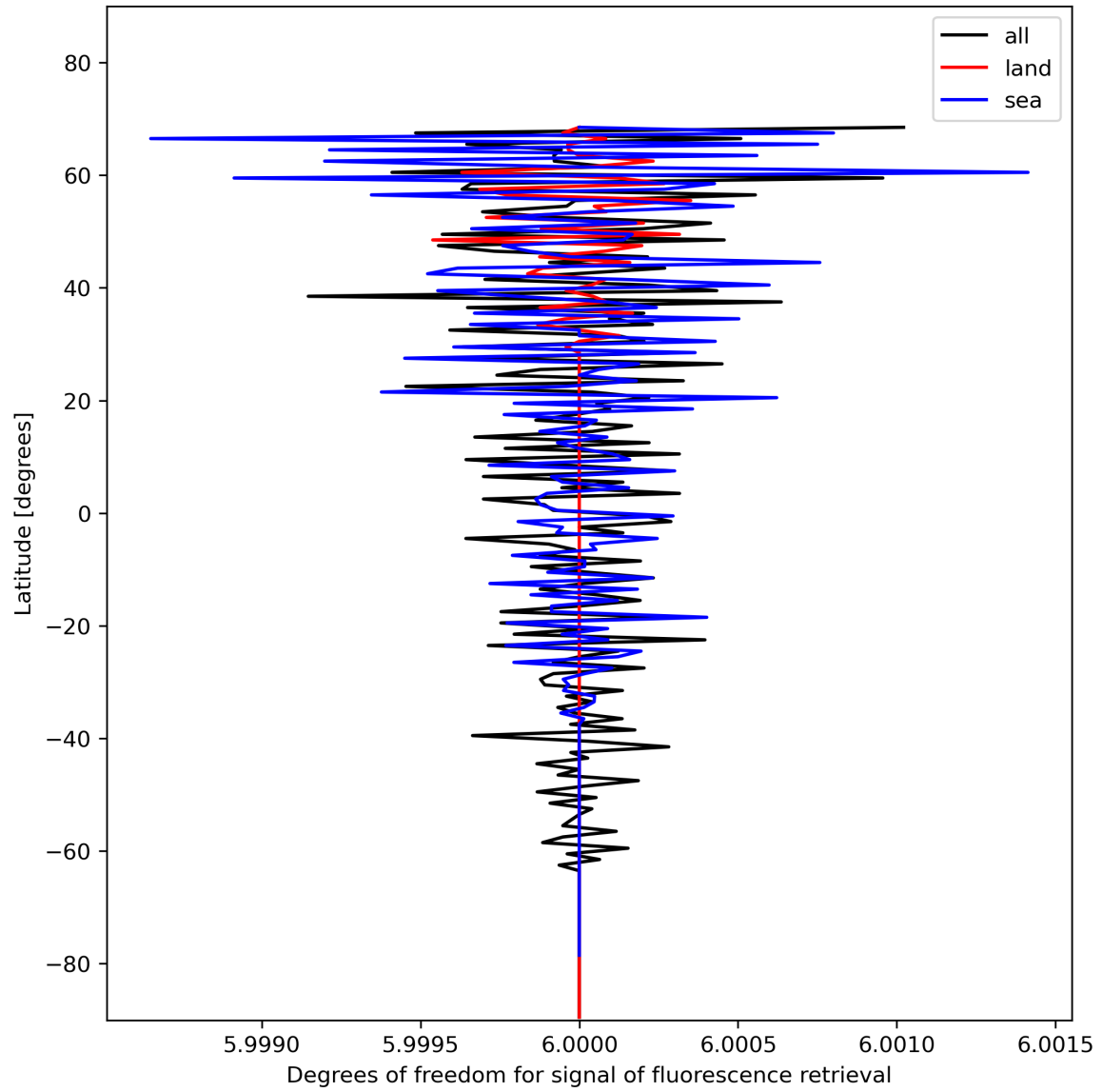
Figure 26: Zonal average of “Degrees of freedom for signal of fluorescence retrieval” for 2023-11-18 to 2023-11-19.
