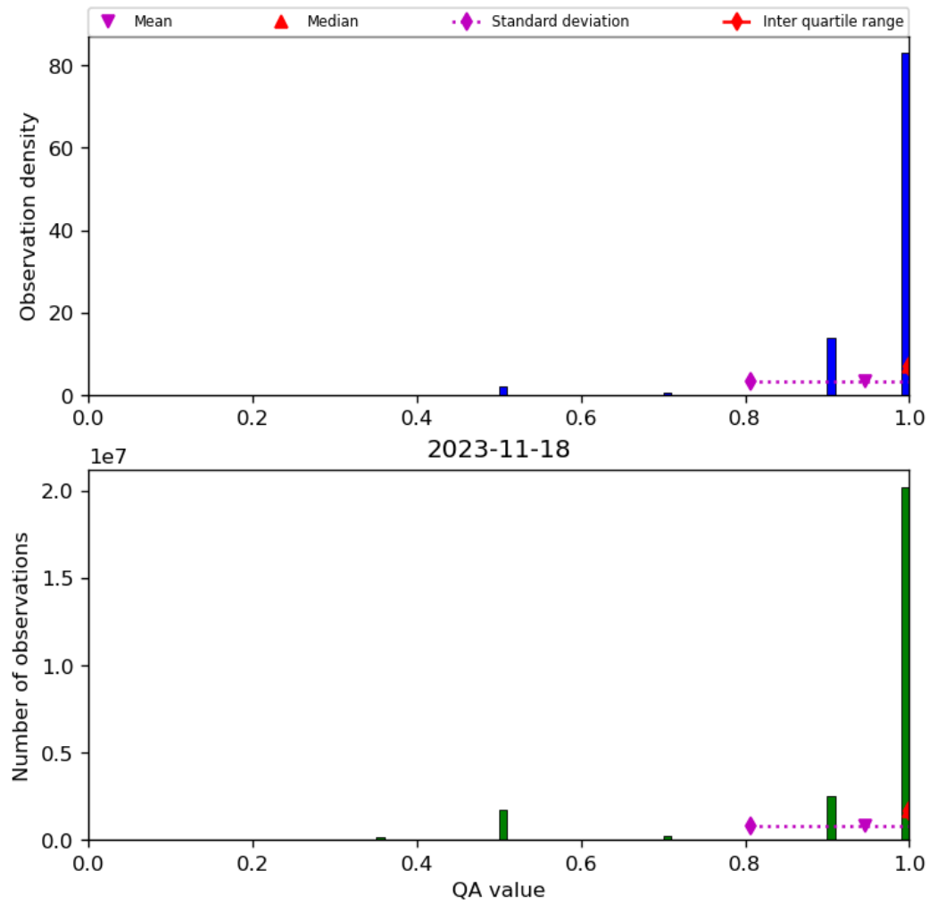
Figure 29: Histogram of “QA value” for 2023-11-18 to 2023-11-19
