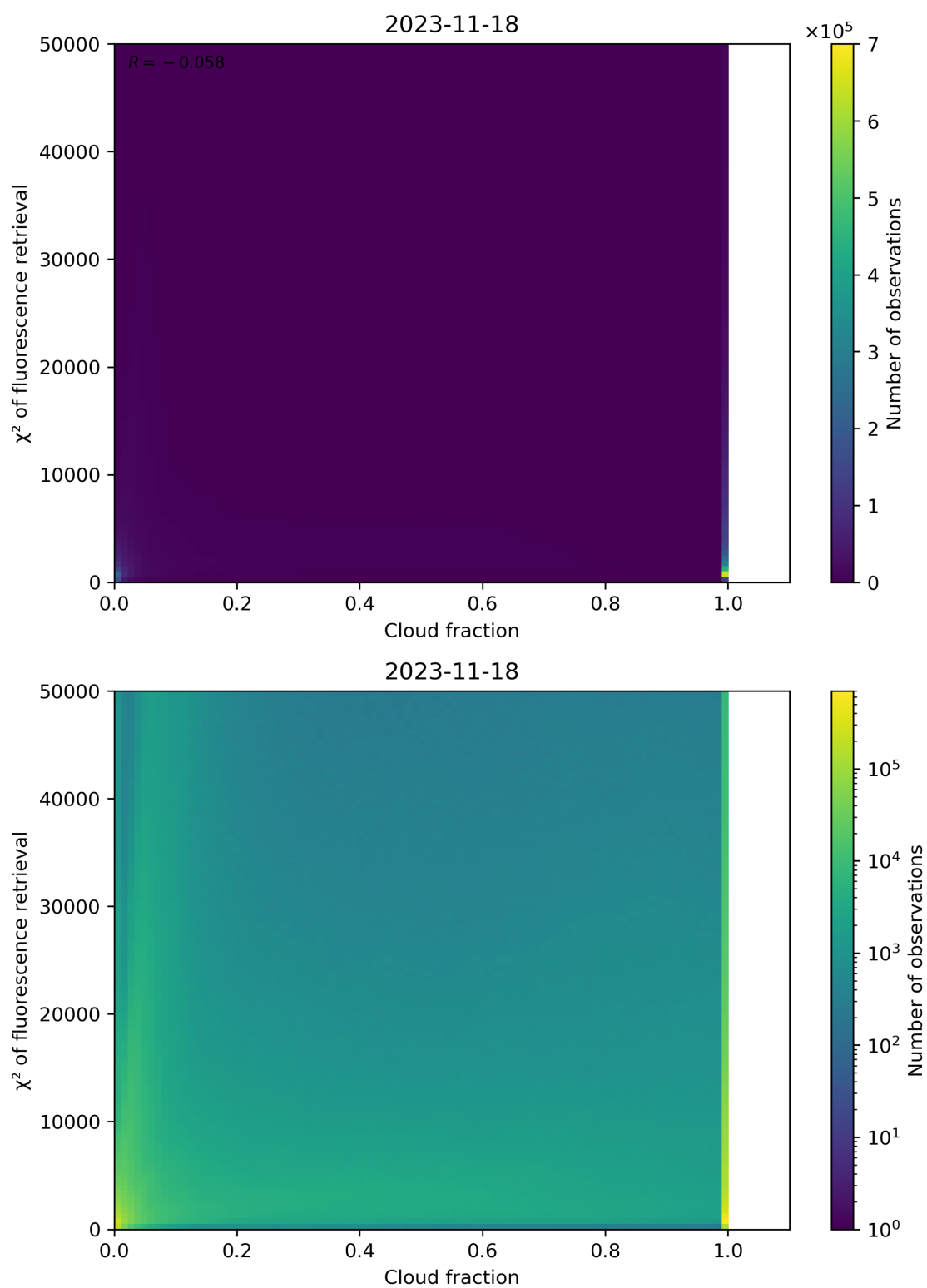
Figure 78: Scatter density plot of “Cloud fraction” against “ \chi^2 of fluorescence retrieval” for 2023-11-18 to 2023-11-19.
