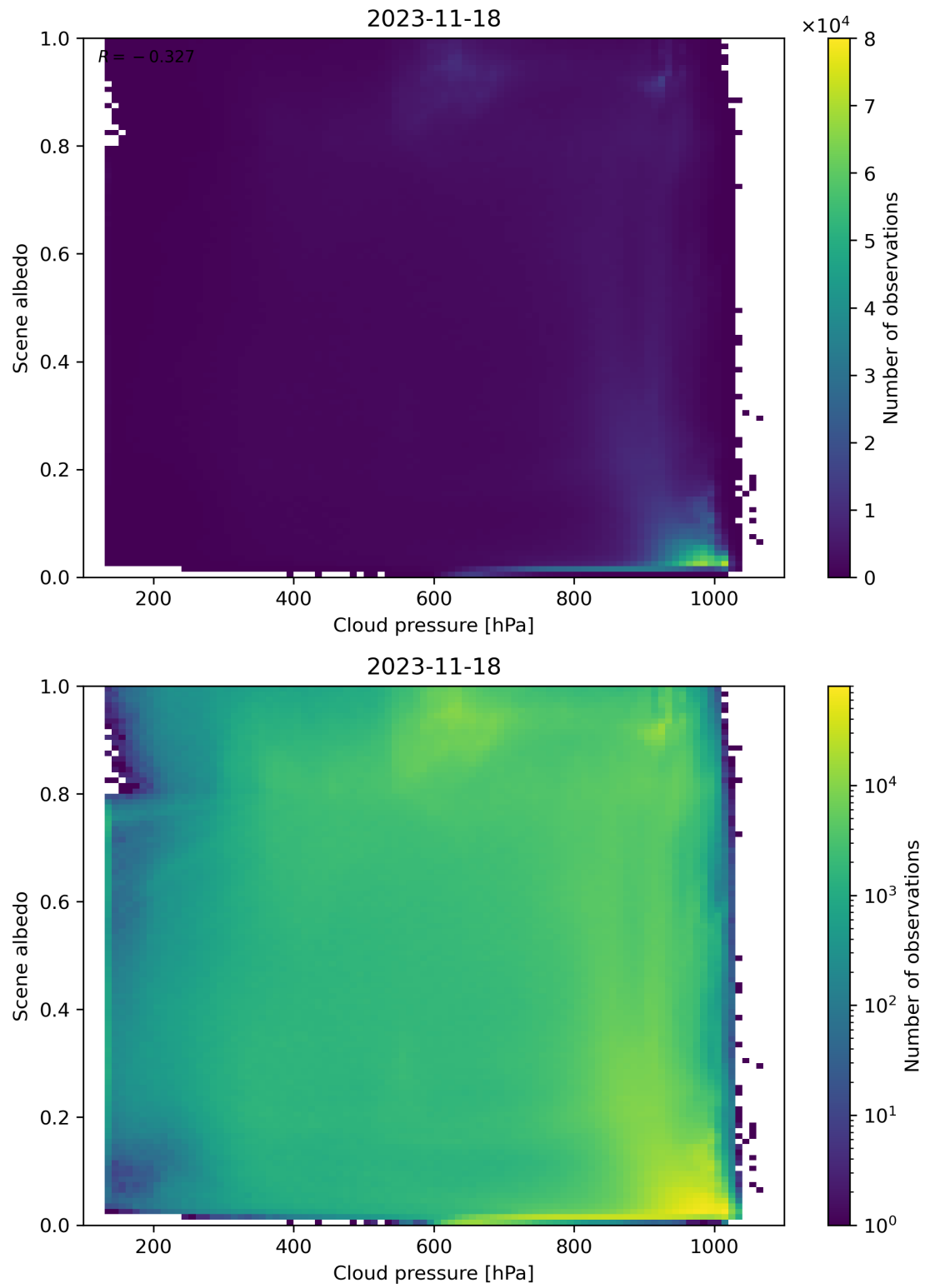
Figure 91: Scatter density plot of “Cloud pressure” against “Scene albedo” for 2023-11-18 to 2023-11-19.
