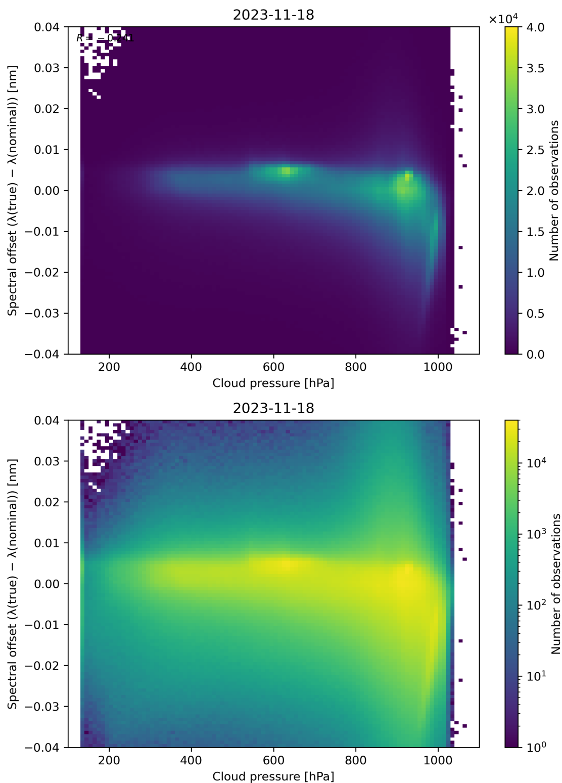
Figure 92: Scatter density plot of “Cloud pressure” against “Spectral offset ( \lambda(\text{true}) - \lambda(\text{nominal}) )” for 2023-11-18 to 2023-11-19.
