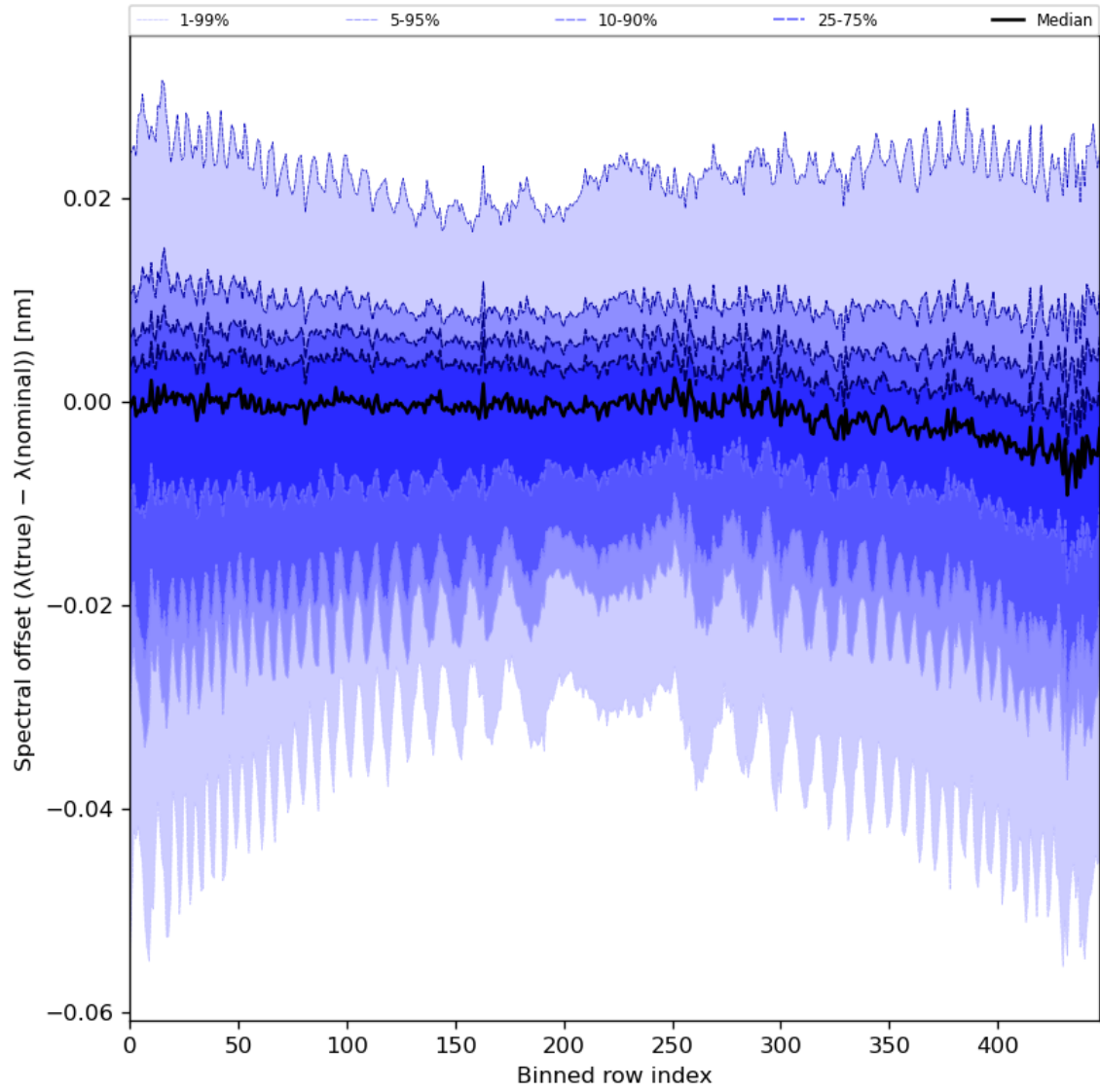
Figure 62: Along track statistics of “Spectral offset ( \lambda(\text{true}) - \lambda(\text{nominal}) )” for 2023-11-18 to 2023-11-19
