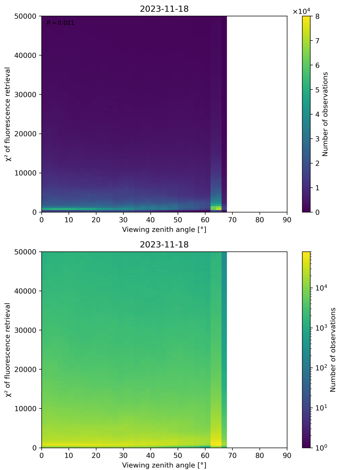
Figure 131: Scatter density plot of “Viewing zenith angle” against “ \chi^2 of fluorescence retrieval” for 2023-11-18 to 2023-11-19.
