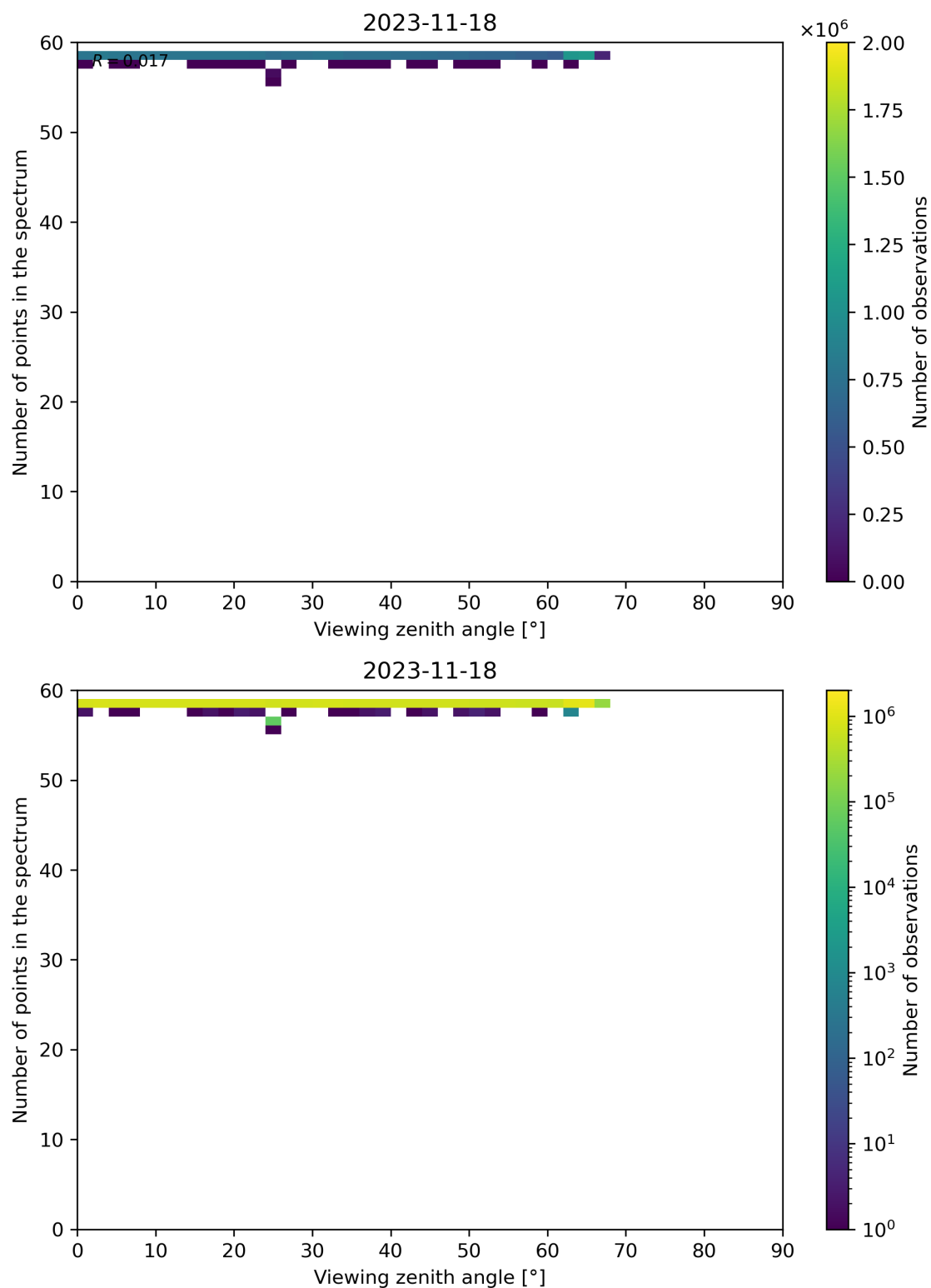
Figure 137: Scatter density plot of “Viewing zenith angle” against “Number of points in the spectrum” for 2023-11-18 to 2023-11-19.
