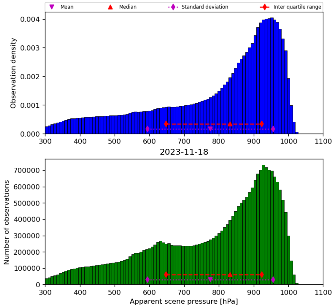
Figure 36: Histogram of “Apparent scene pressure” for 2023-11-18 to 2023-11-19
