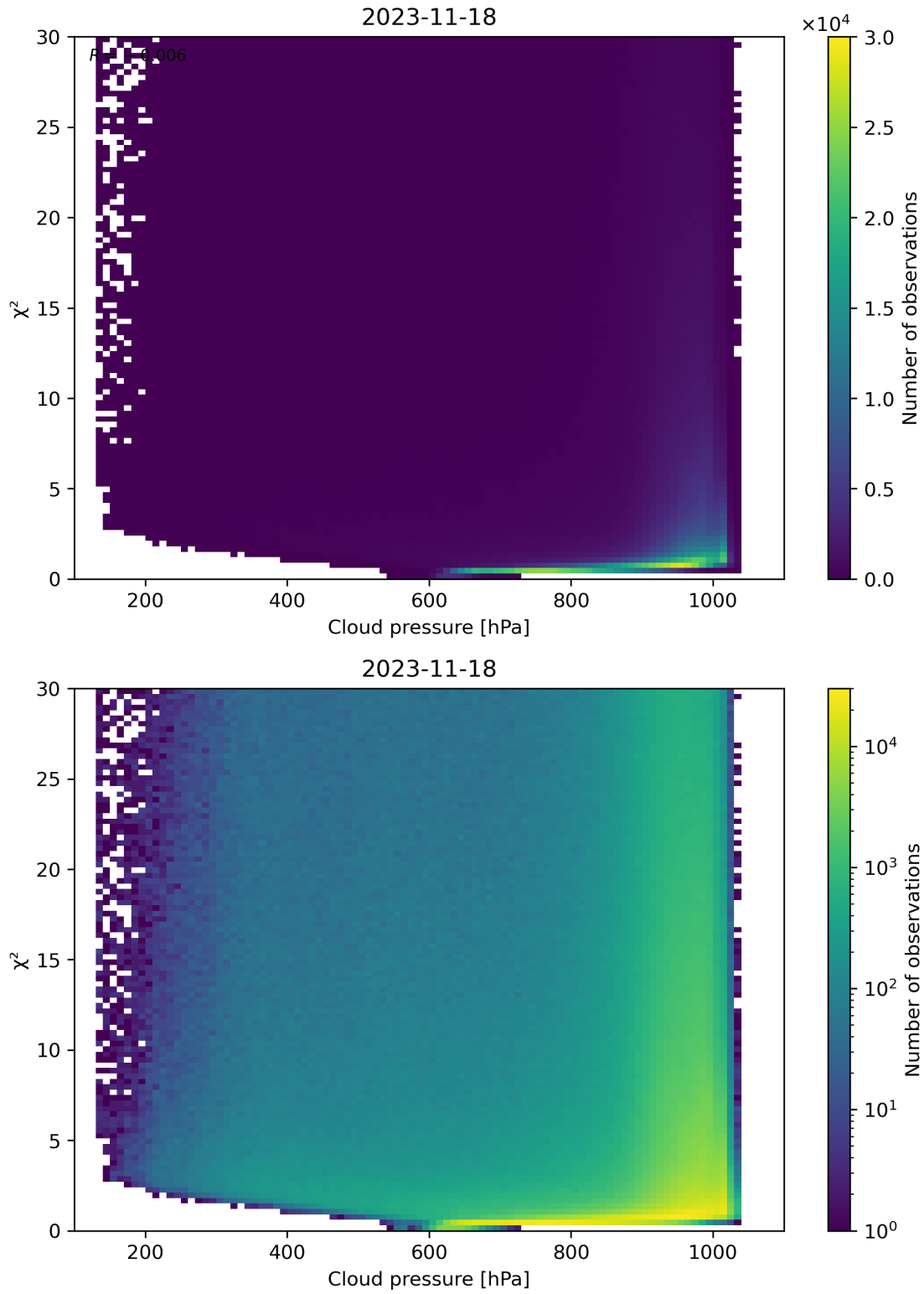
Figure 85: Scatter density plot of “Cloud pressure” against “ \chi^2 ” for 2023-11-18 to 2023-11-19.
