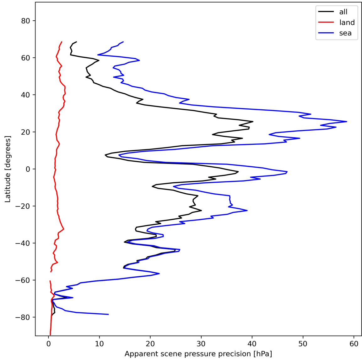
Figure 20: Zonal average of “Apparent scene pressure precision” for 2023-11-18 to 2023-11-19.
