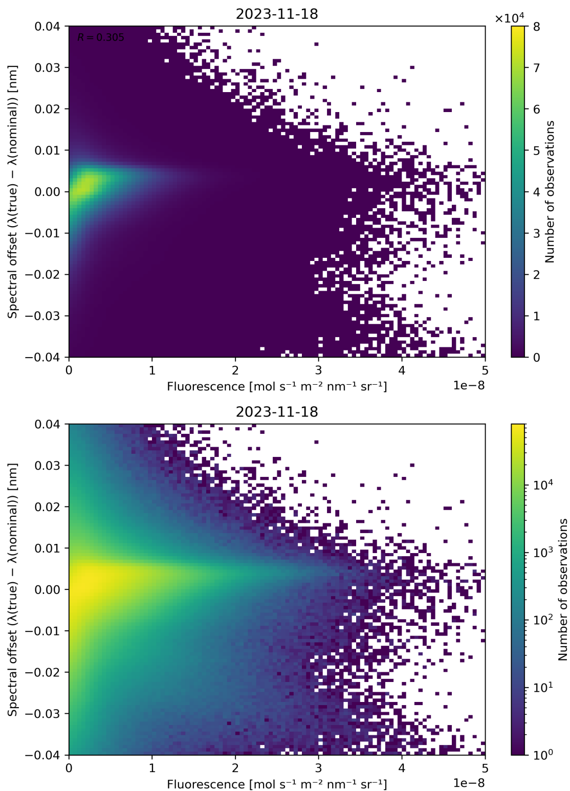
Figure 95: Scatter density plot of “Fluorescence” against “Spectral offset ( \lambda(\text{true}) - \lambda(\text{nominal}) )” for 2023-11-18 to 2023-11-19.
