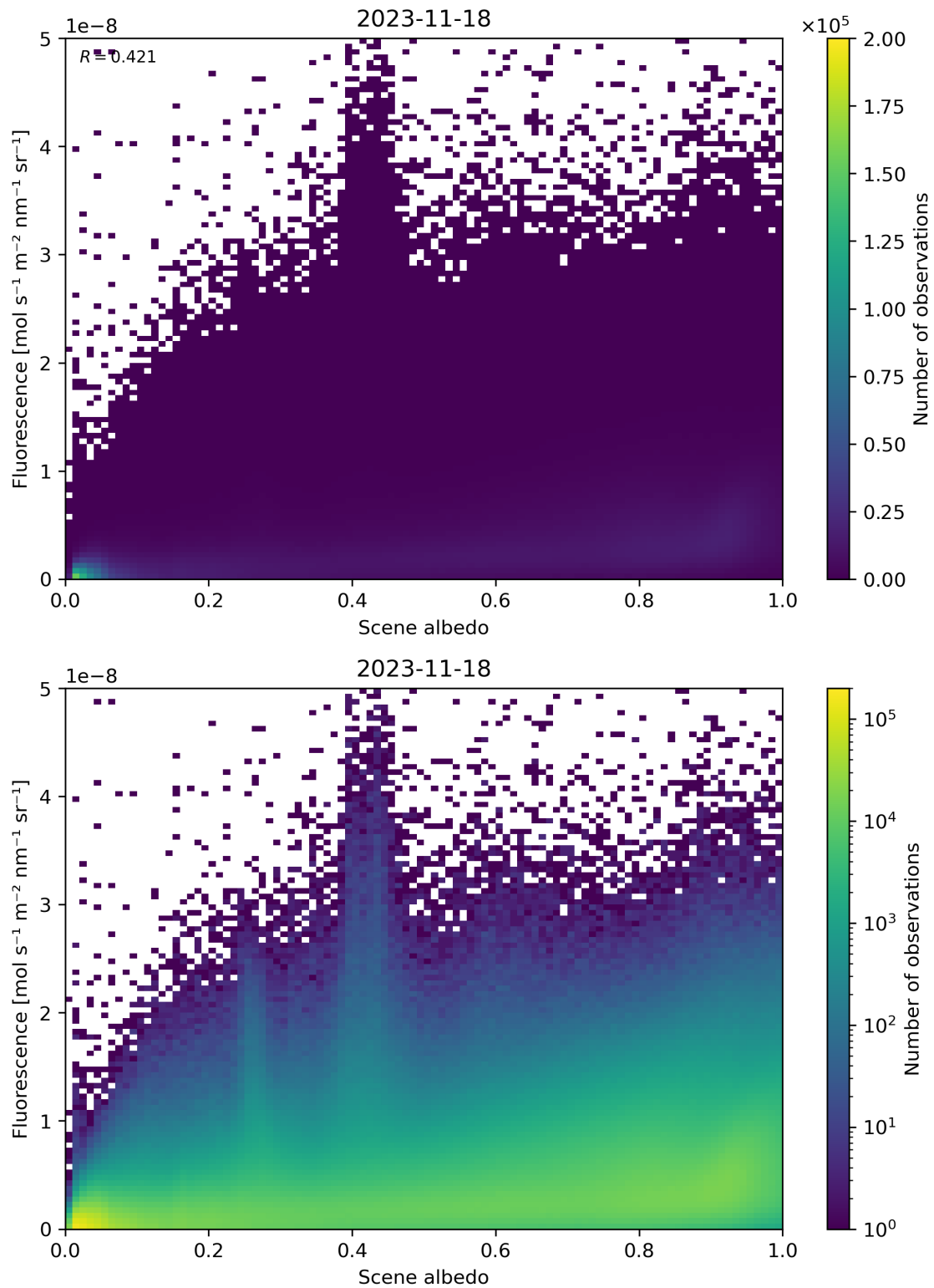
Figure 114: Scatter density plot of “Scene albedo” against “Fluorescence” for 2023-11-18 to 2023-11-19.
