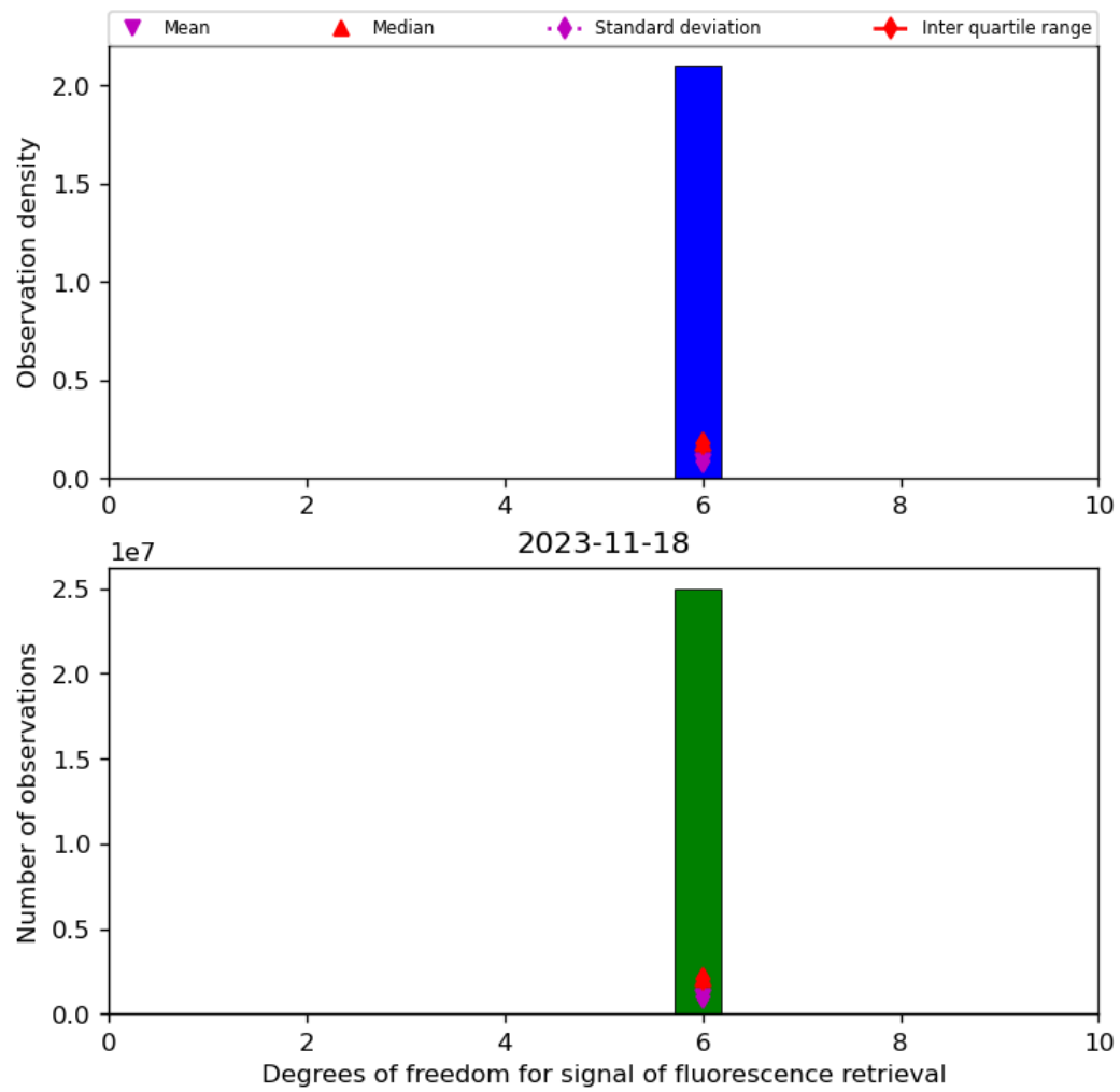
Figure 43: Histogram of “Degrees of freedom for signal of fluorescence retrieval” for 2023-11-18 to 2023-11-19
