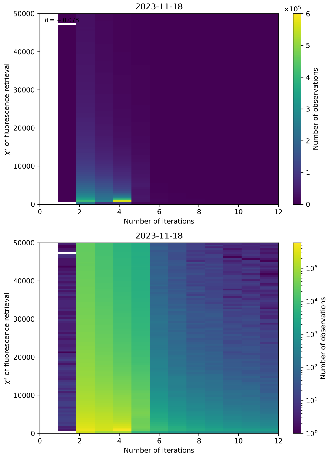
Figure 106: Scatter density plot of “Number of iterations” against “ \chi^2 of fluorescence retrieval” for 2023-11-18 to 2023-11-19.
