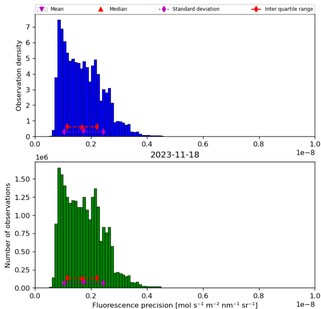
Figure 41: Histogram of “Fluorescence precision” for 2023-11-18 to 2023-11-19
