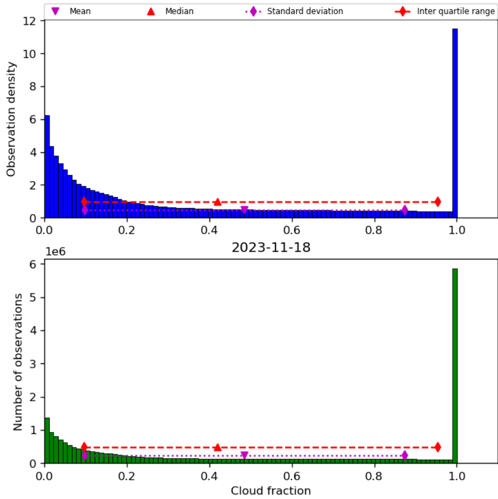
Figure 32: Histogram of “Cloud fraction” for 2023-11-18 to 2023-11-19
