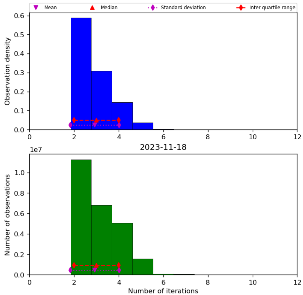
Figure 39: Histogram of “Number of iterations” for 2023-11-18 to 2023-11-19
