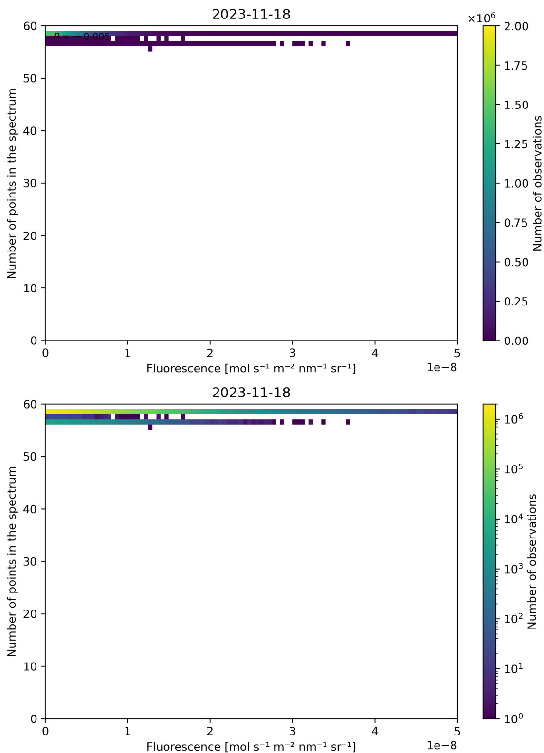
Figure 94: Scatter density plot of “Fluorescence” against “Number of points in the spectrum” for 2023-11-18 to 2023-11-19.
