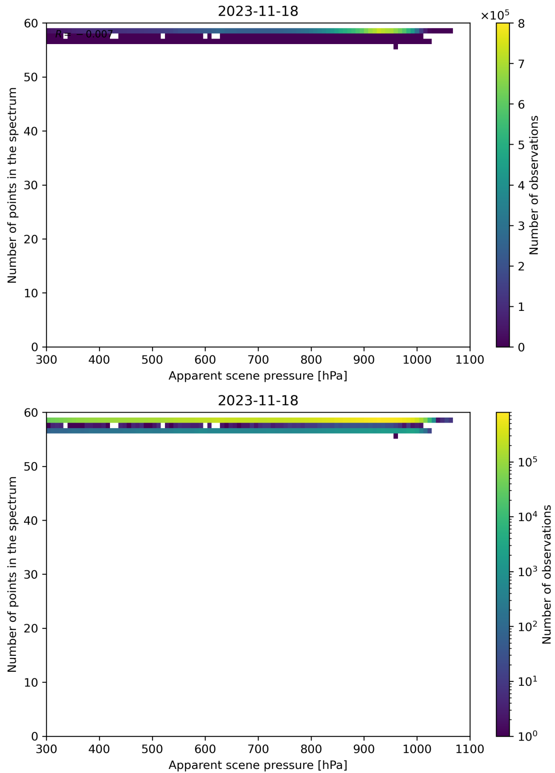
Figure 67: Scatter density plot of “Apparent scene pressure” against “Number of points in the spectrum” for 2023-11-18 to 2023-11-19.
