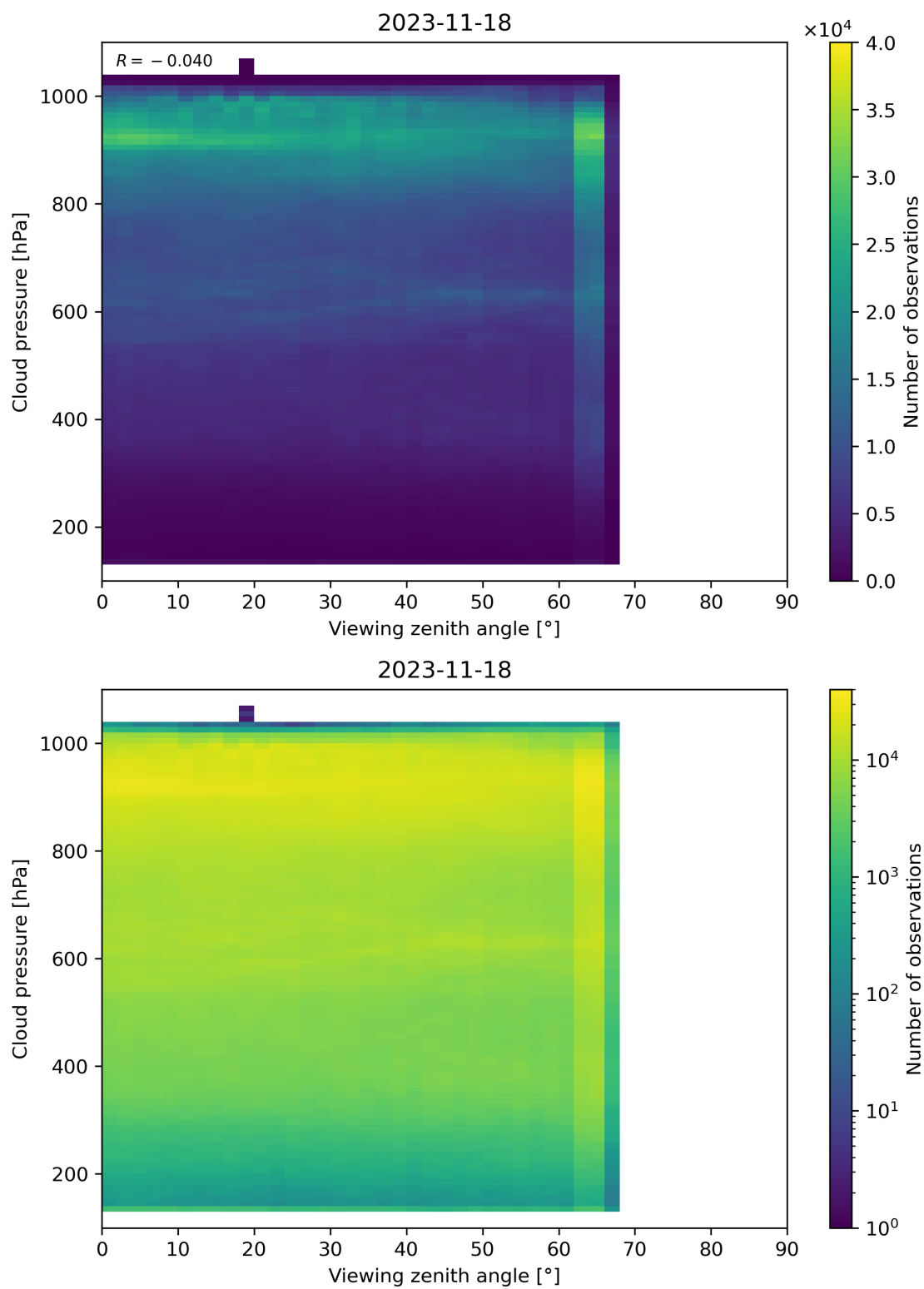
Figure 133: Scatter density plot of “Viewing zenith angle” against “Cloud pressure” for 2023-11-18 to 2023-11-19.
