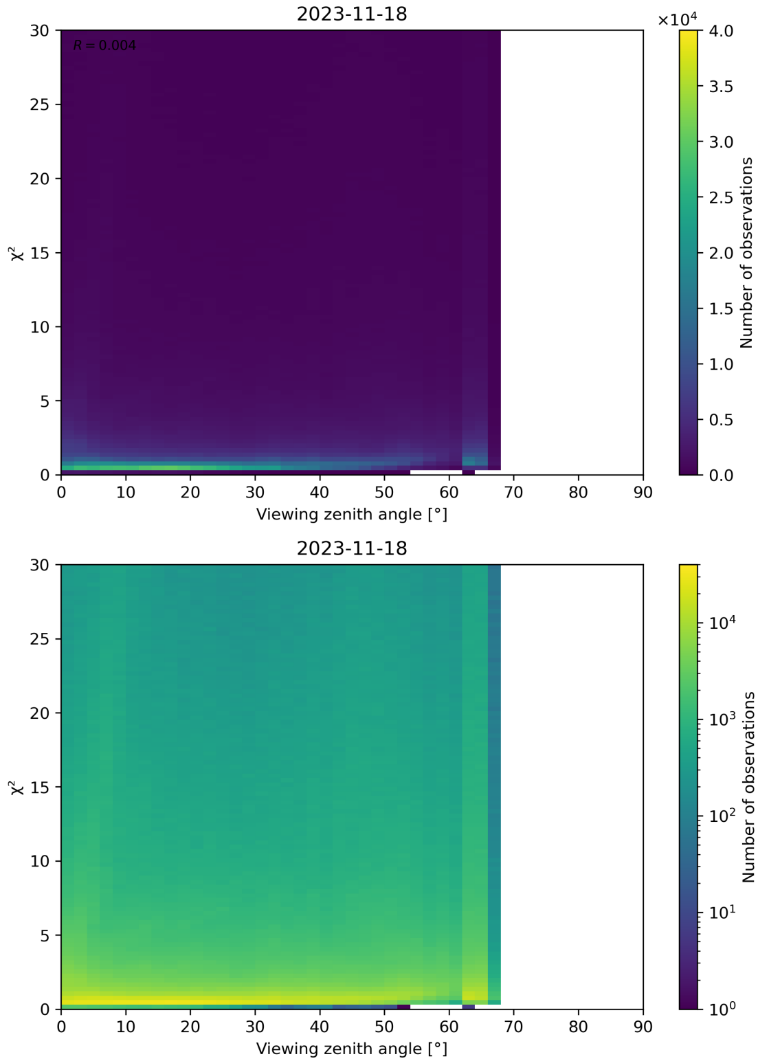
Figure 130: Scatter density plot of “Viewing zenith angle” against “ \chi^2 ” for 2023-11-18 to 2023-11-19.
