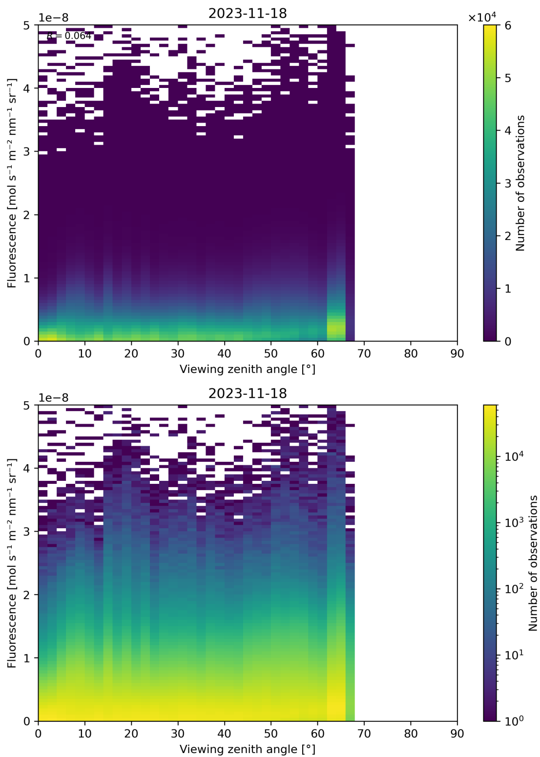
Figure 134: Scatter density plot of “Viewing zenith angle” against “Fluorescence” for 2023-11-18 to 2023-11-19.
