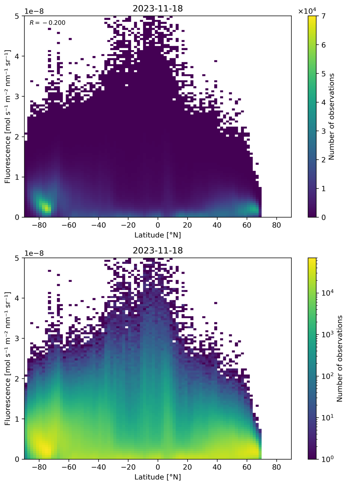
Figure 101: Scatter density plot of “Latitude” against “Fluorescence” for 2023-11-18 to 2023-11-19.
