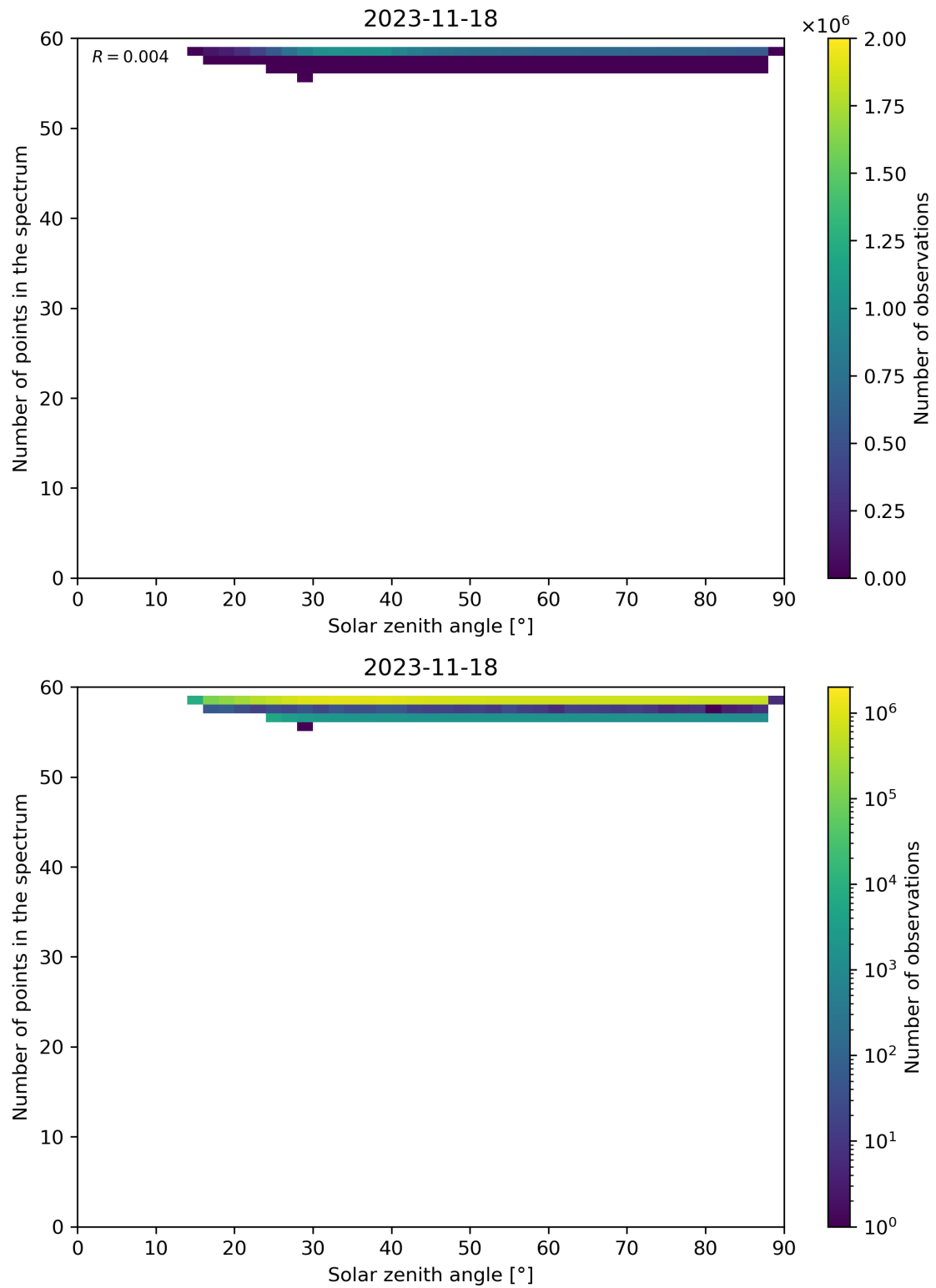
Figure 126: Scatter density plot of “Solar zenith angle” against “Number of points in the spectrum” for 2023-11-18 to 2023-11-19.
