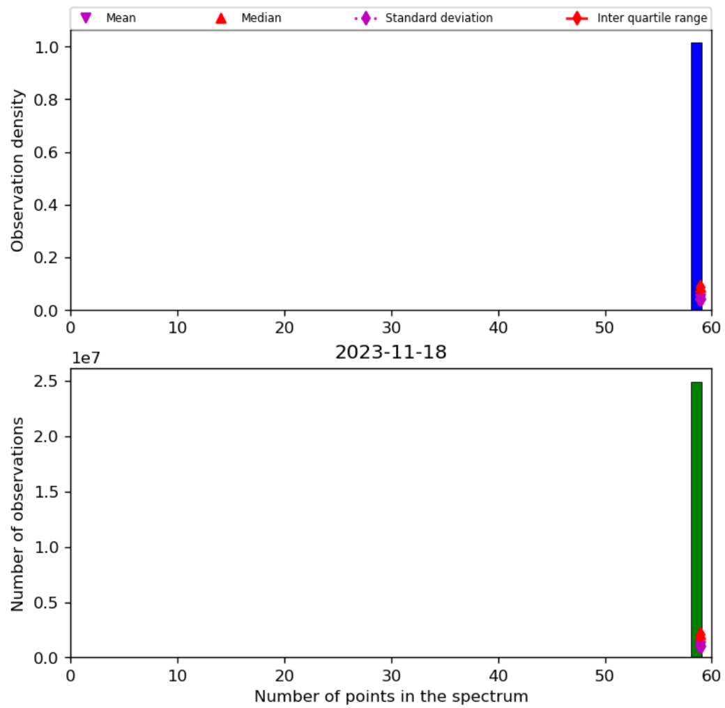
Figure 44: Histogram of “Number of points in the spectrum” for 2023-11-18 to 2023-11-19
