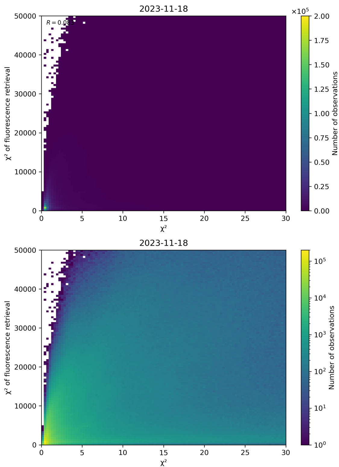
Figure 69: Scatter density plot of “ \chi^2 ” against “ \chi^2 of fluorescence retrieval” for 2023-11-18 to 2023-11-19.
