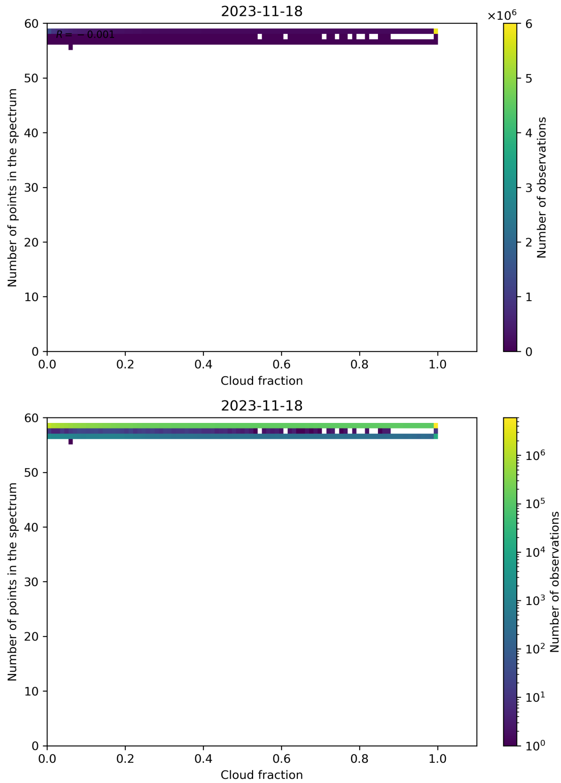
Figure 81: Scatter density plot of “Cloud fraction” against “Number of points in the spectrum” for 2023-11-18 to 2023-11-19.
