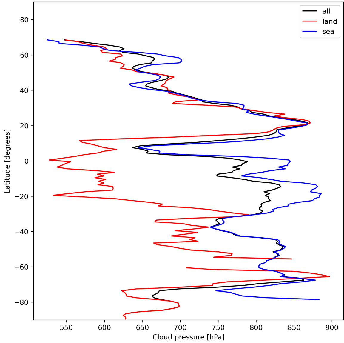
Figure 13: Zonal average of “Cloud pressure” for 2023-11-18 to 2023-11-19.
