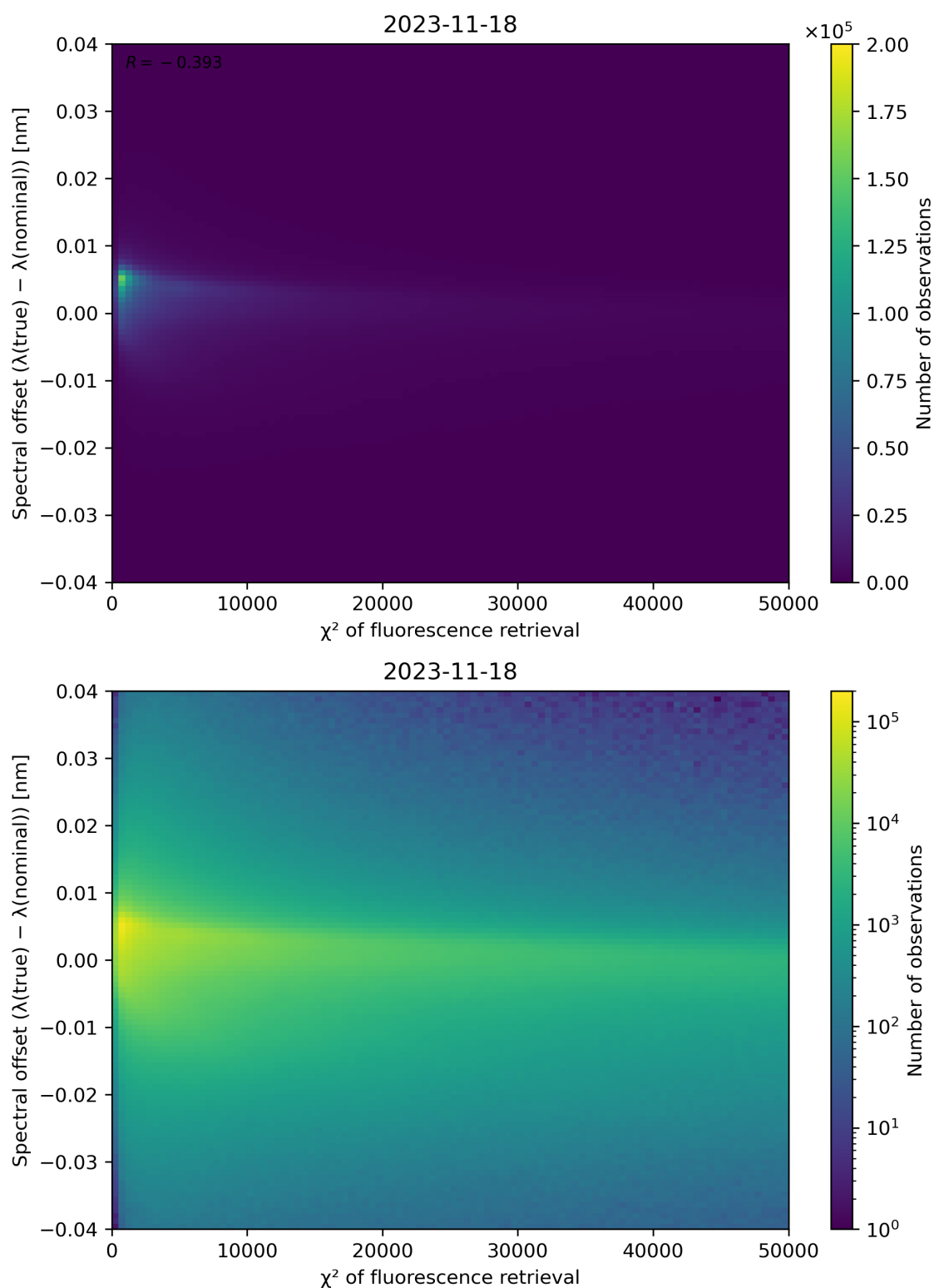
Figure 72: Scatter density plot of " \chi^2 of fluorescence retrieval" against "Spectral offset ( \lambda(\text{true}) - \lambda(\text{nominal})) " for 2023-11-18 to 2023-11-19.
