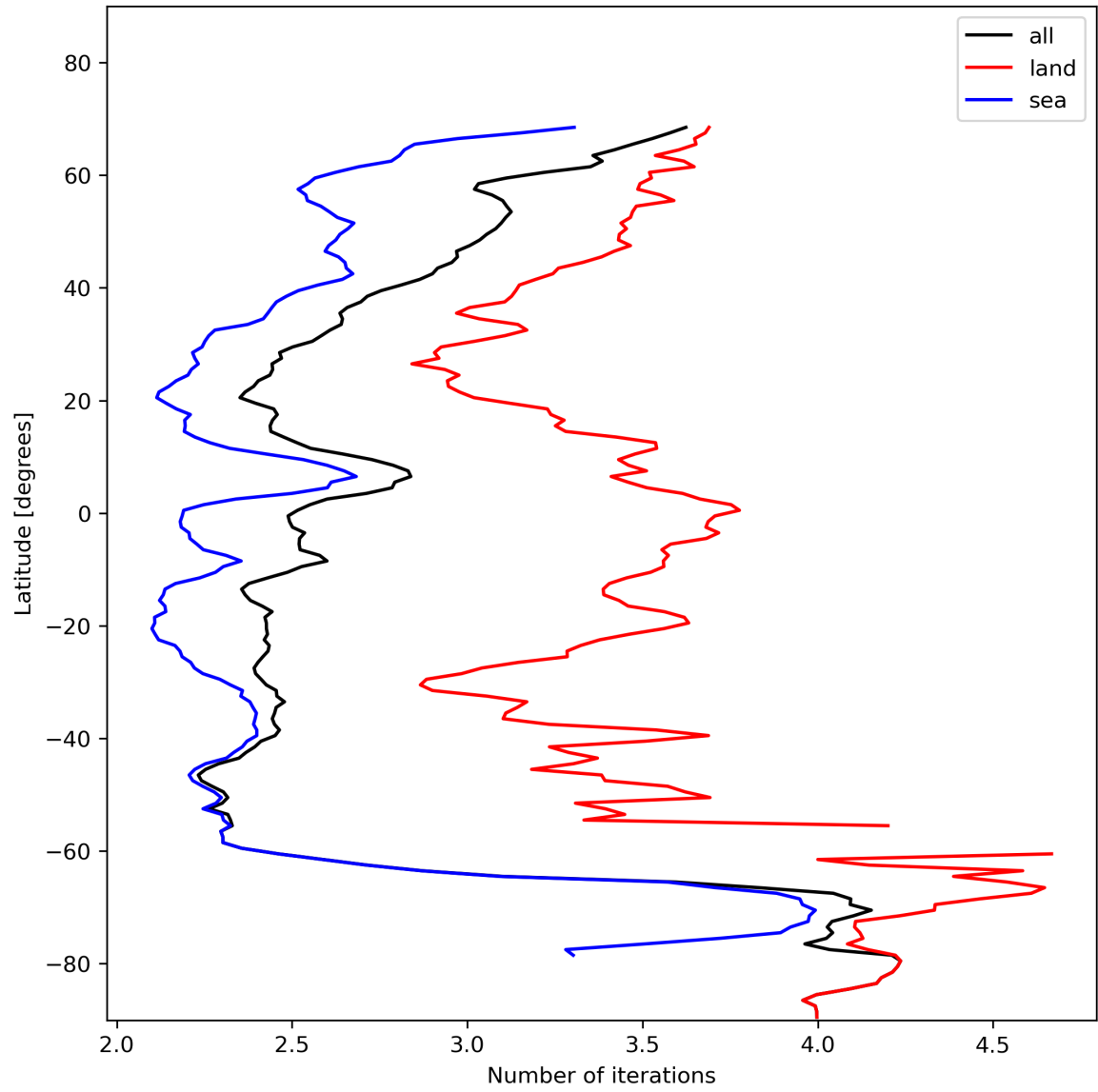
Figure 22: Zonal average of “Number of iterations” for 2023-11-18 to 2023-11-19.
