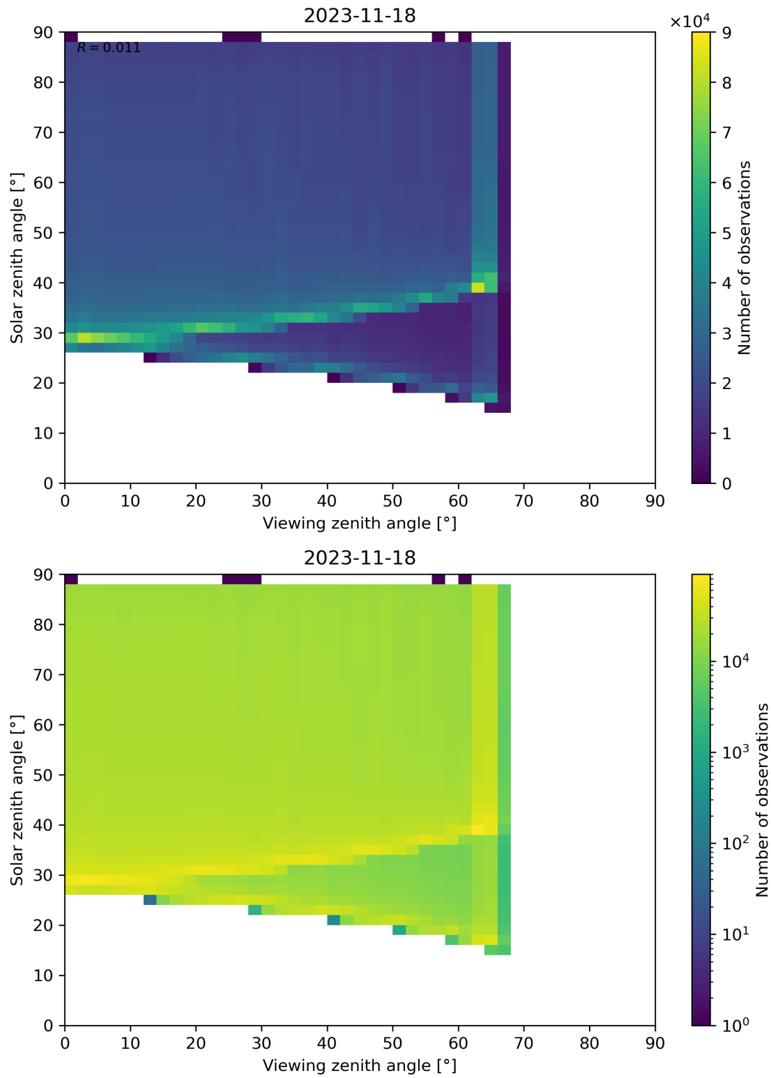
Figure 139: Scatter density plot of “Viewing zenith angle” against “Solar zenith angle” for 2023-11-18 to 2023-11-19.
