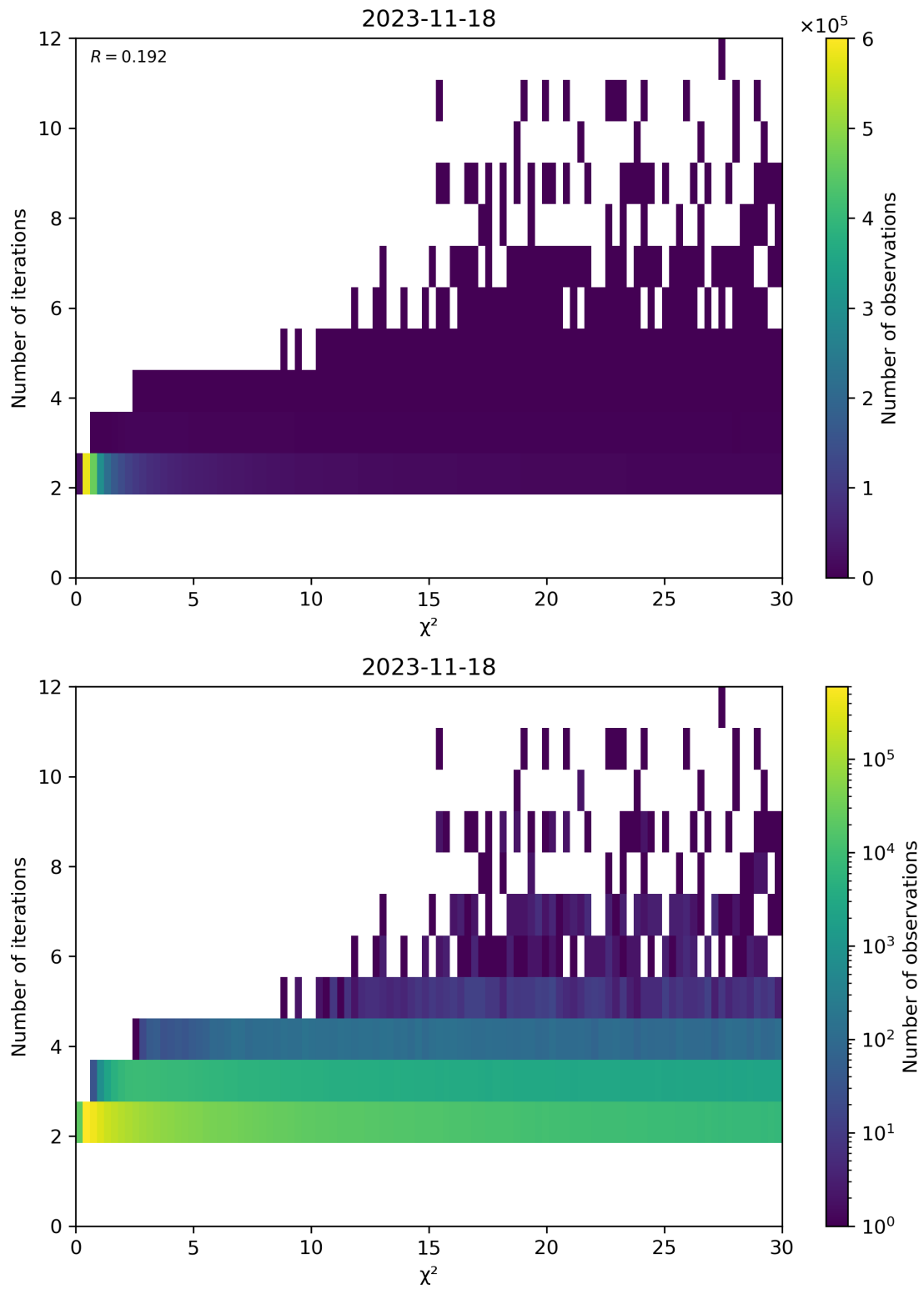
Figure 73: Scatter density plot of “ \chi^2 ” against “Number of iterations” for 2023-11-18 to 2023-11-19.
