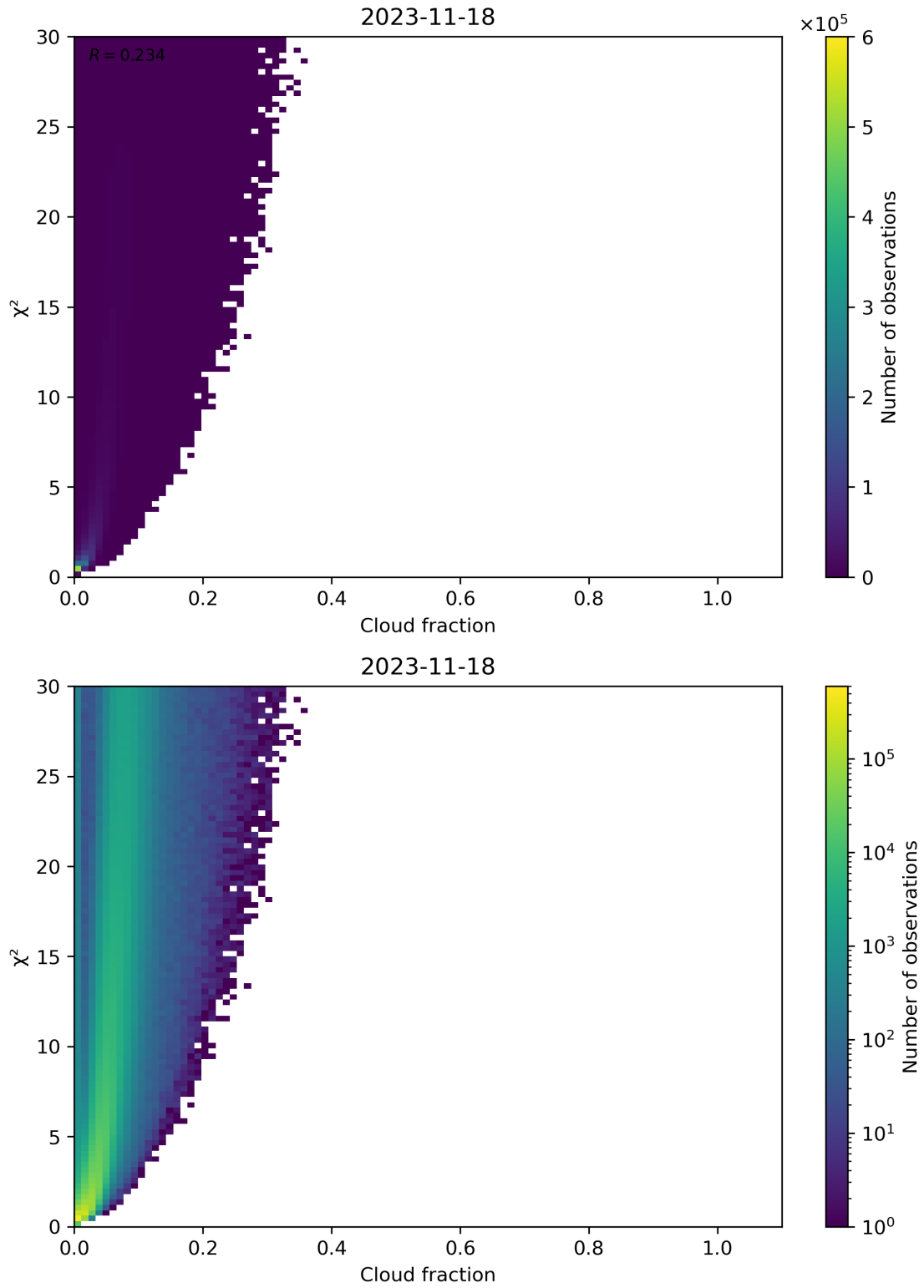
Figure 77: Scatter density plot of “Cloud fraction” against “ \chi^2 ” for 2023-11-18 to 2023-11-19.
