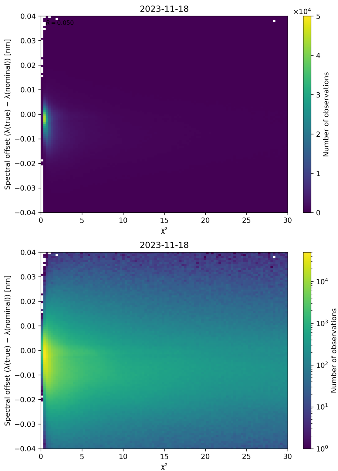
Figure 75: Scatter density plot of “ \chi^2 ” against “Spectral offset ( \lambda(\text{true}) - \lambda(\text{nominal}) )” for 2023-11-18 to 2023-11-19.
