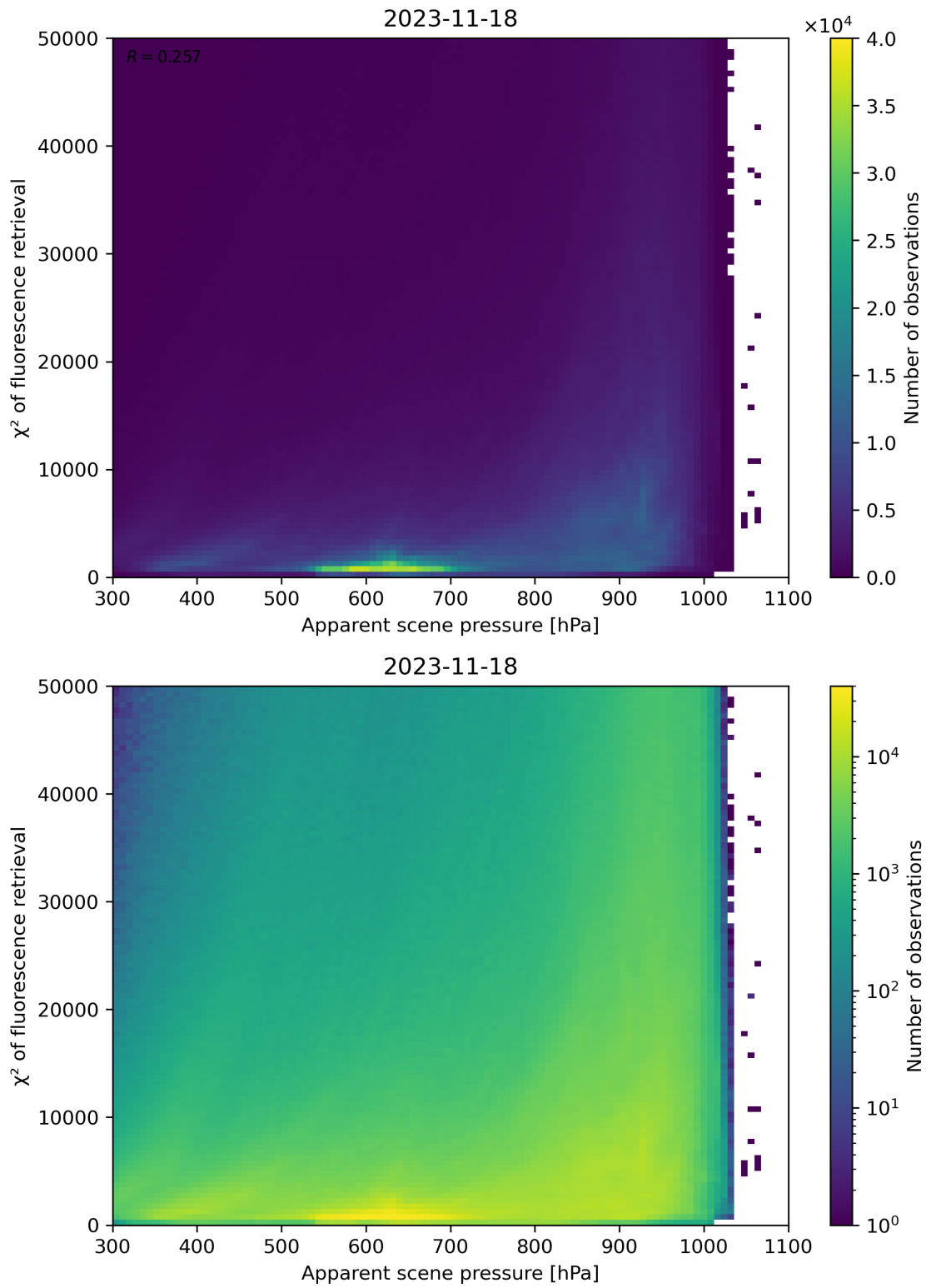
Figure 64: Scatter density plot of “Apparent scene pressure” against “ \chi^2 of fluorescence retrieval” for 2023-11-18 to 2023-11-19.
