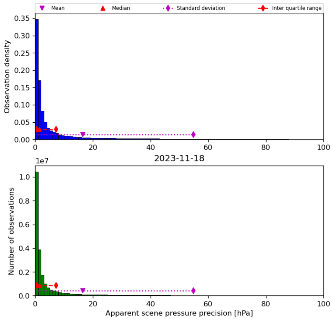
Figure 37: Histogram of “Apparent scene pressure precision” for 2023-11-18 to 2023-11-19
