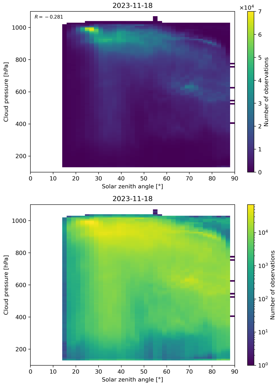
Figure 122: Scatter density plot of “Solar zenith angle” against “Cloud pressure” for 2023-11-18 to 2023-11-19.
