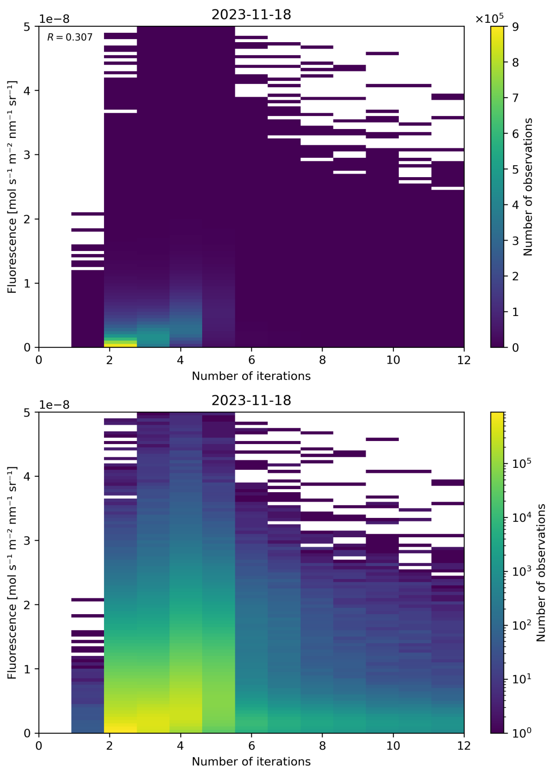
Figure 107: Scatter density plot of “Number of iterations” against “Fluorescence” for 2023-11-18 to 2023-11-19.
