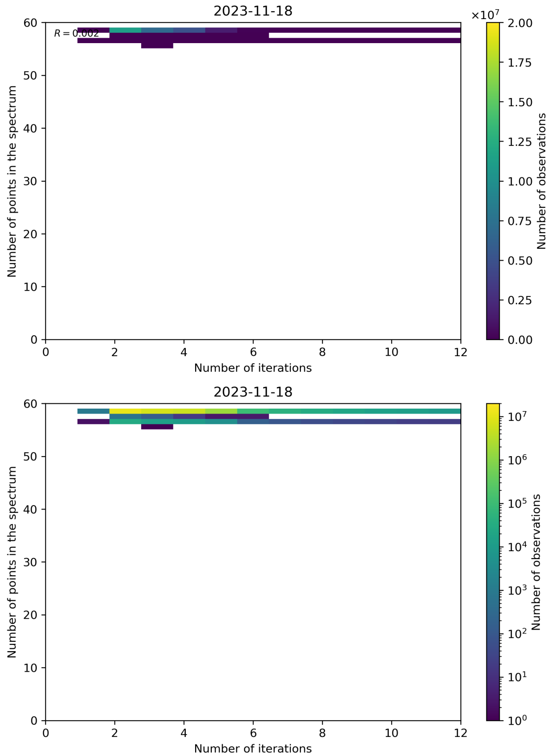
Figure 108: Scatter density plot of “Number of iterations” against “Number of points in the spectrum” for 2023-11-18 to 2023-11-19.
