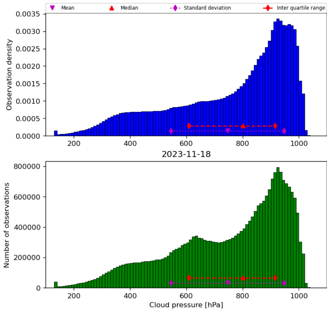
Figure 30: Histogram of “Cloud pressure” for 2023-11-18 to 2023-11-19
