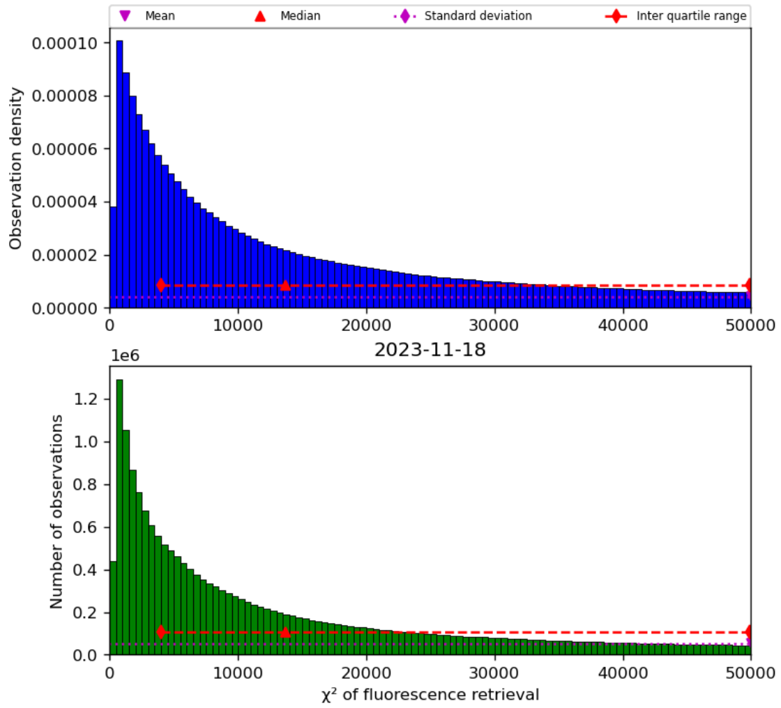
Figure 42: Histogram of “ \chi^2 of fluorescence retrieval” for 2023-11-18 to 2023-11-19
