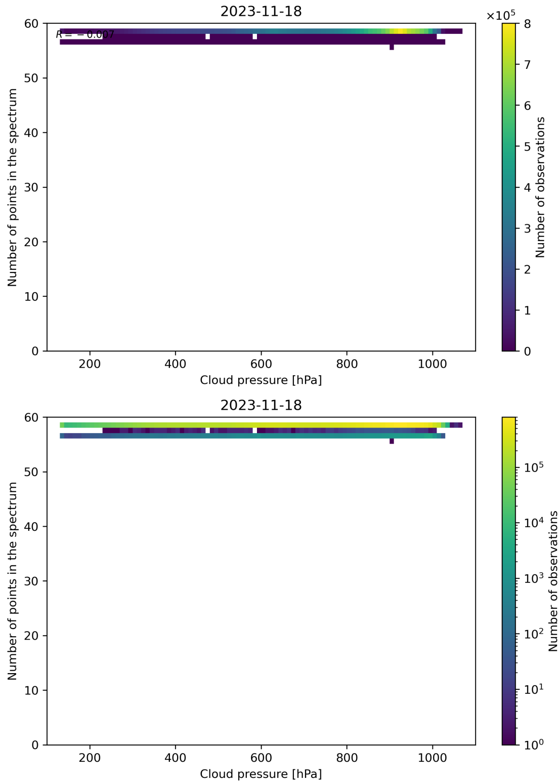
Figure 90: Scatter density plot of “Cloud pressure” against “Number of points in the spectrum” for 2023-11-18 to 2023-11-19.
