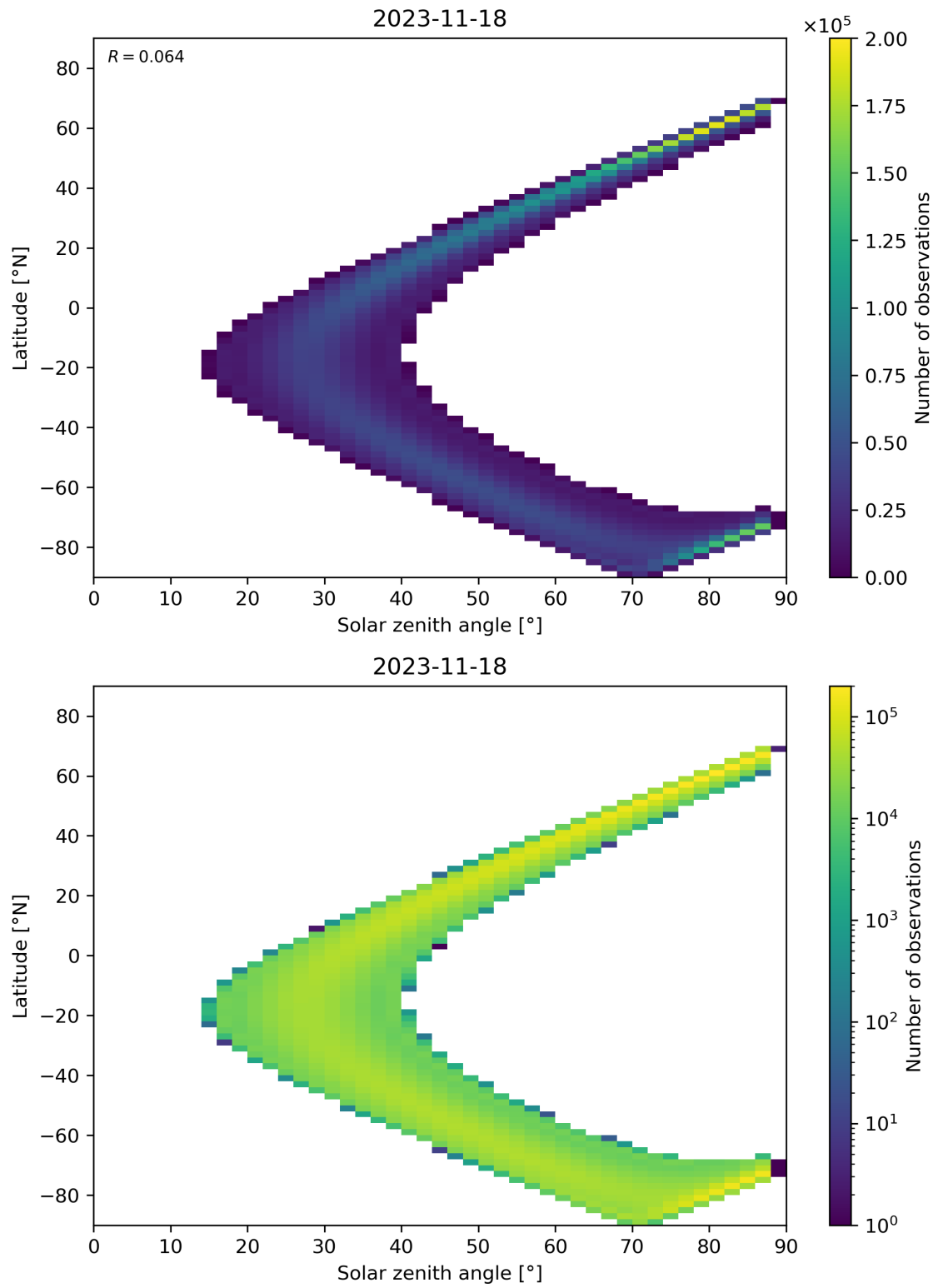
Figure 124: Scatter density plot of “Solar zenith angle” against “Latitude” for 2023-11-18 to 2023-11-19.
