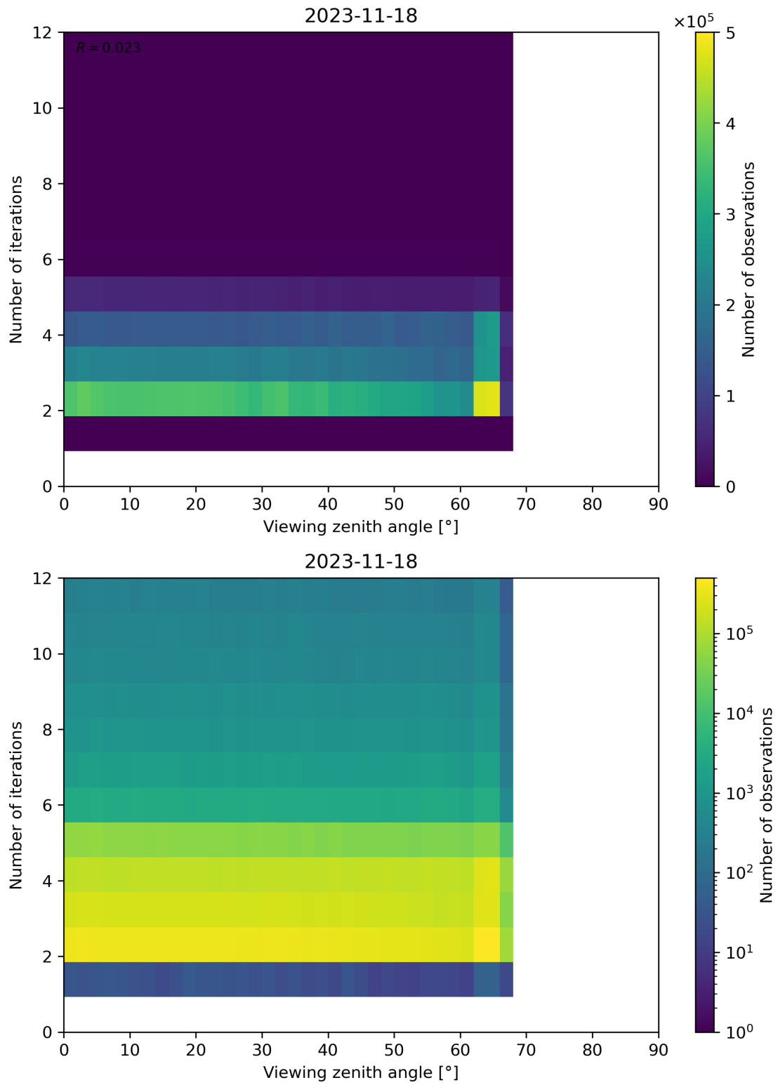
Figure 136: Scatter density plot of “Viewing zenith angle” against “Number of iterations” for 2023-11-18 to 2023-11-19.
