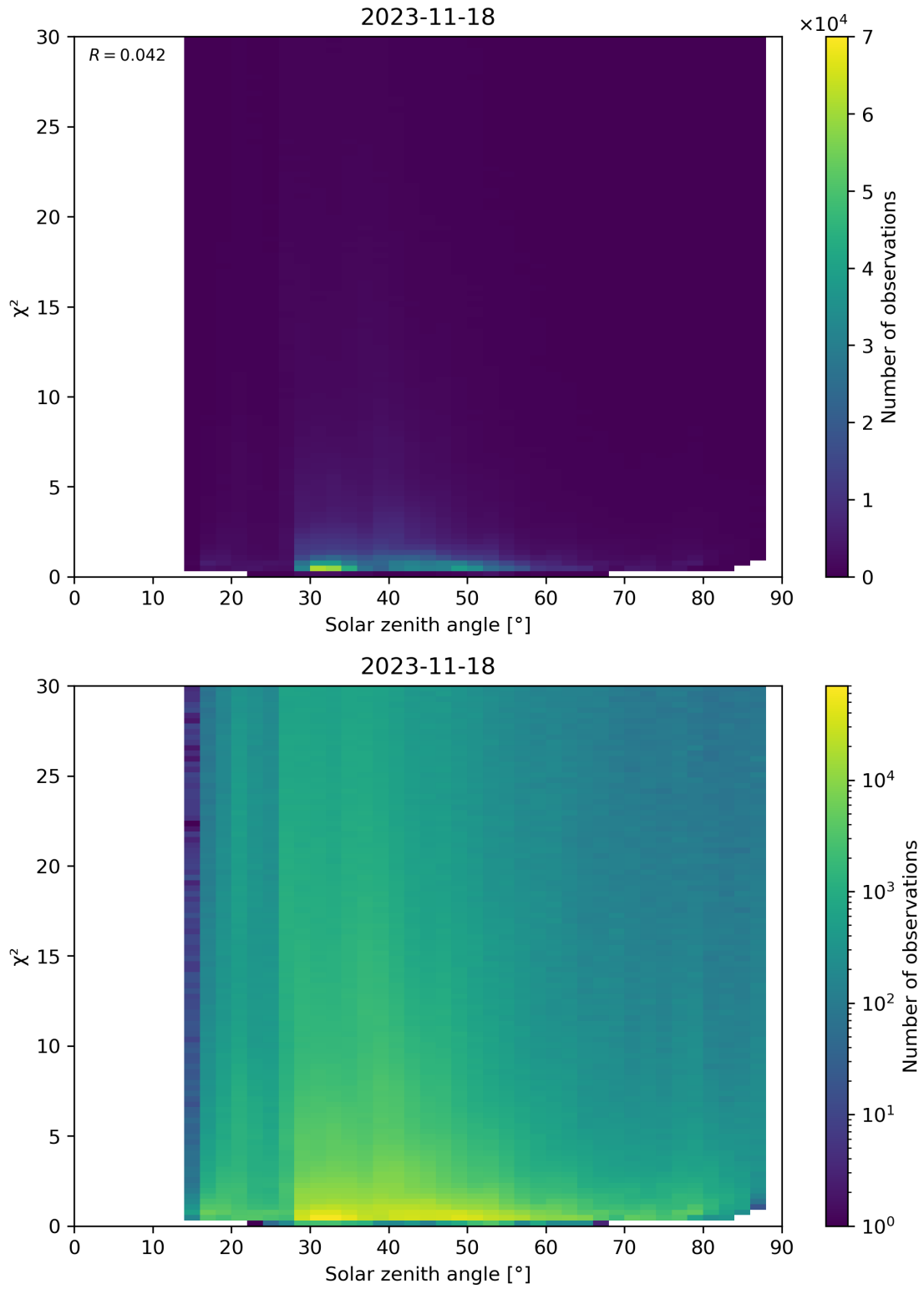
Figure 119: Scatter density plot of “Solar zenith angle” against “ \chi^2 ” for 2023-11-18 to 2023-11-19.
