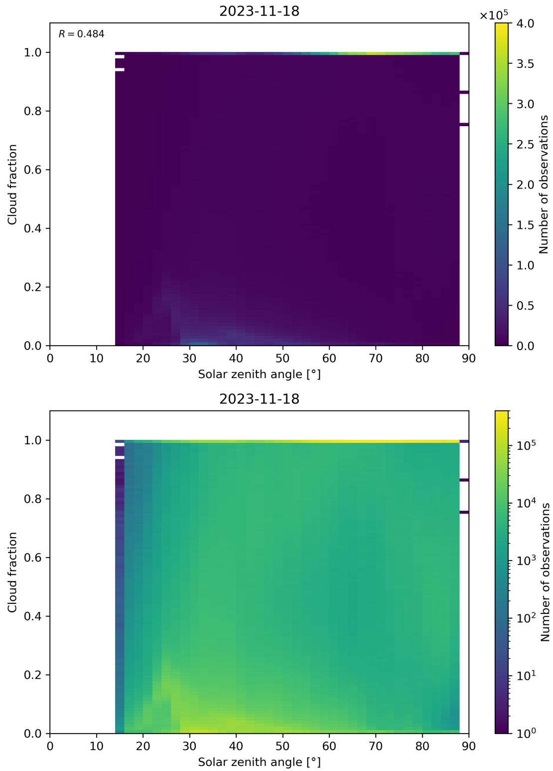
Figure 121: Scatter density plot of “Solar zenith angle” against “Cloud fraction” for 2023-11-18 to 2023-11-19.
