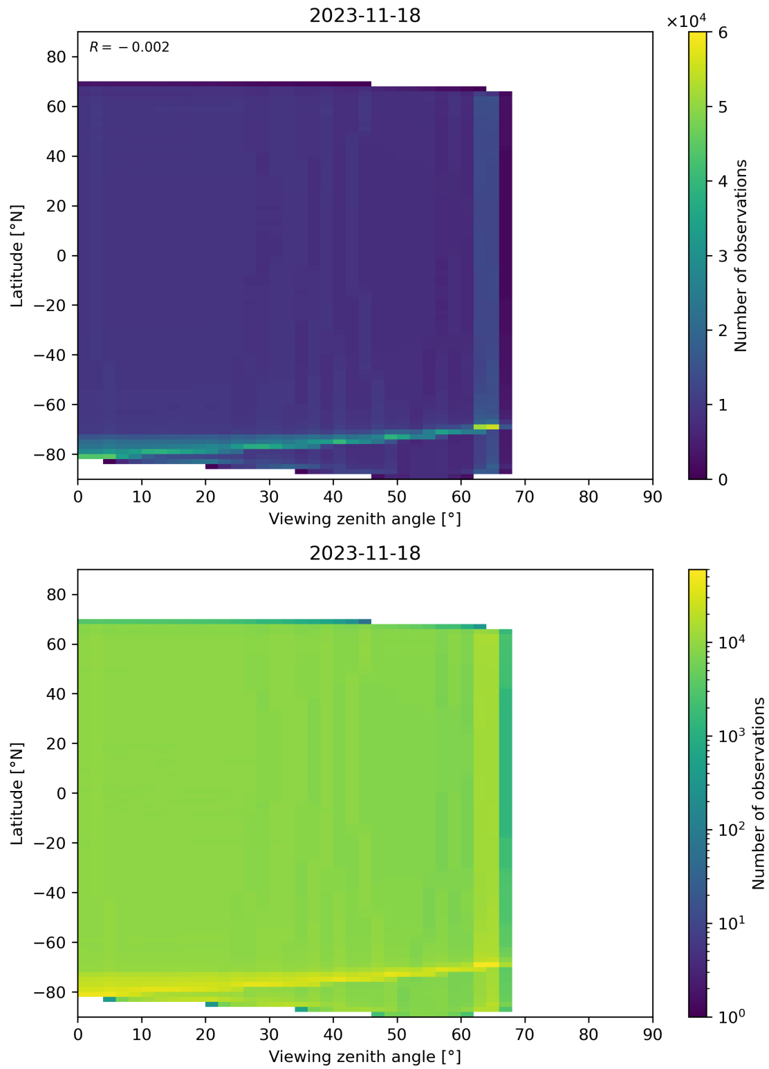
Figure 135: Scatter density plot of “Viewing zenith angle” against “Latitude” for 2023-11-18 to 2023-11-19.
