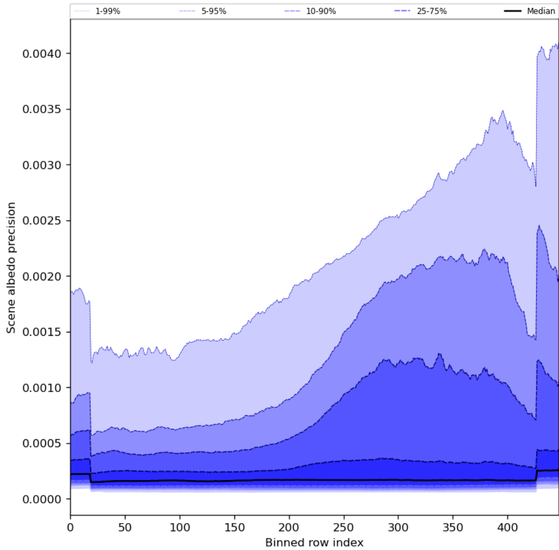
Figure 52: Along track statistics of “Scene albedo precision” for 2023-11-18 to 2023-11-19
