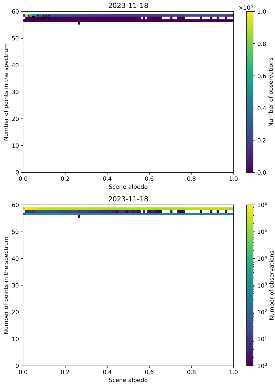
Figure 116: Scatter density plot of “Scene albedo” against “Number of points in the spectrum” for 2023-11-18 to 2023-11-19.
