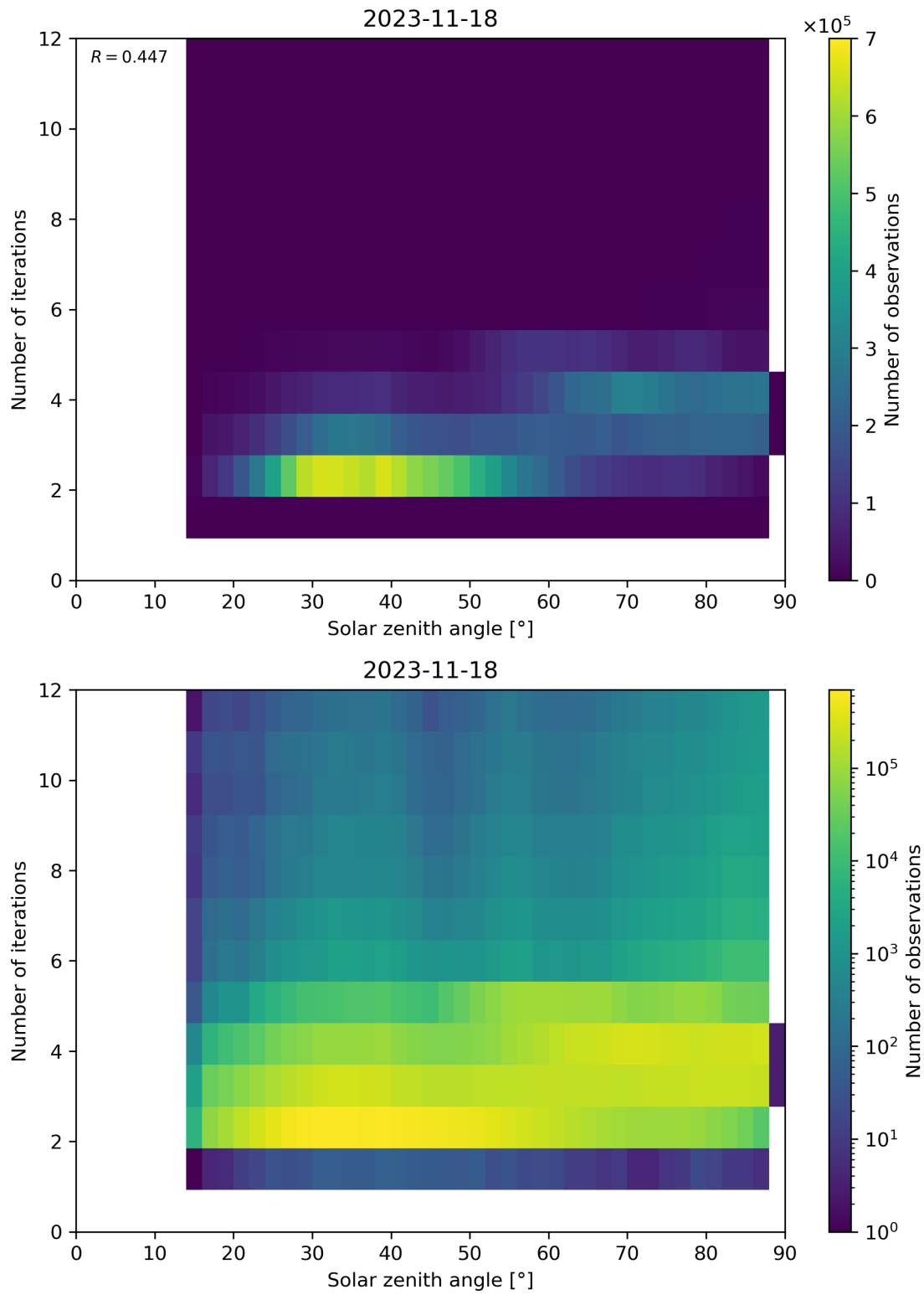
Figure 125: Scatter density plot of “Solar zenith angle” against “Number of iterations” for 2023-11-18 to 2023-11-19.
