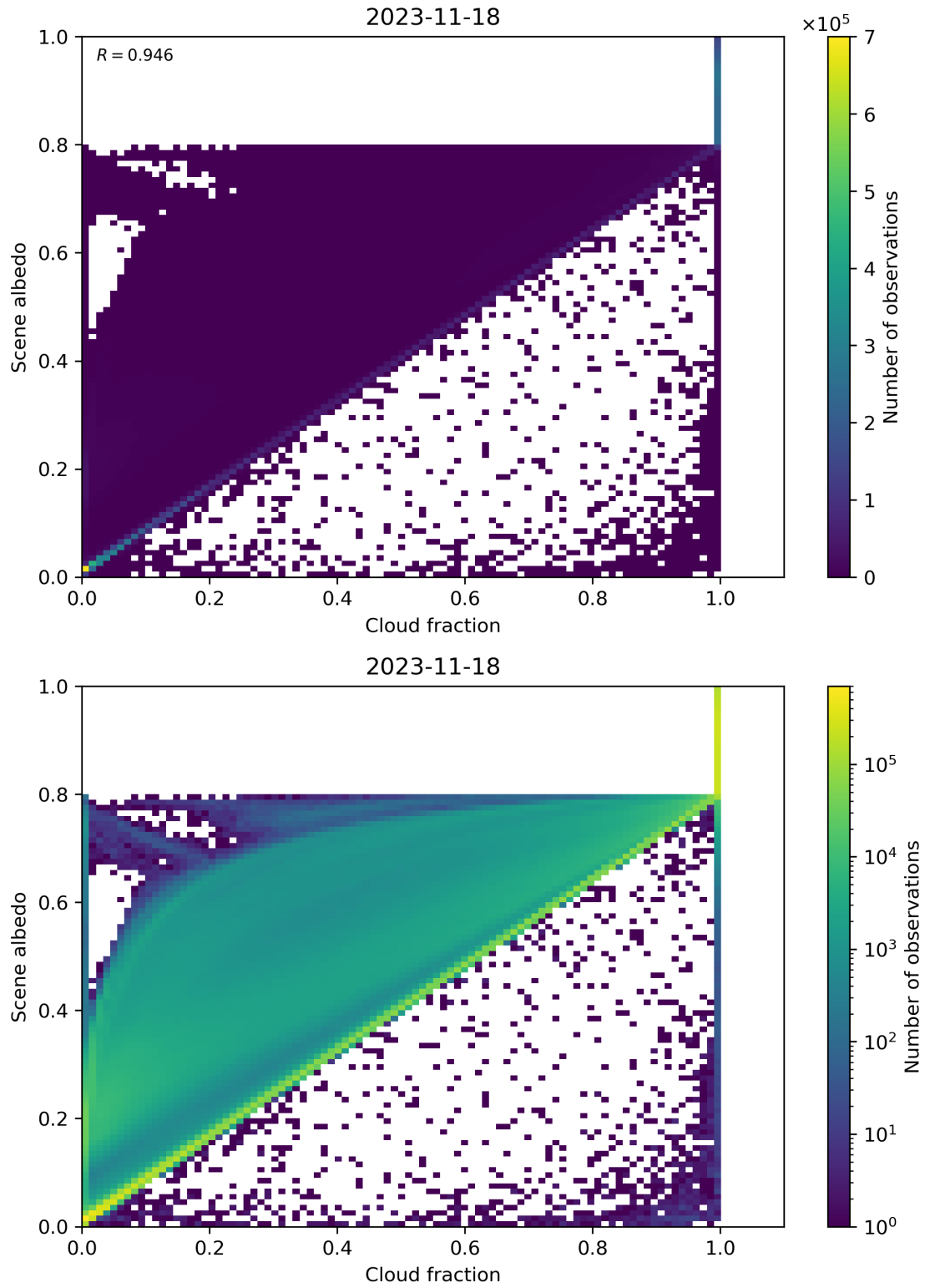
Figure 82: Scatter density plot of “Cloud fraction” against “Scene albedo” for 2023-11-18 to 2023-11-19.
