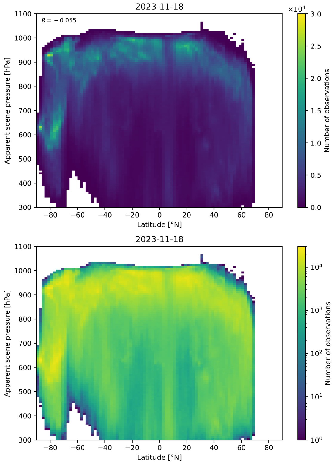
Figure 96: Scatter density plot of “Latitude” against “Apparent scene pressure” for 2023-11-18 to 2023-11-19.
