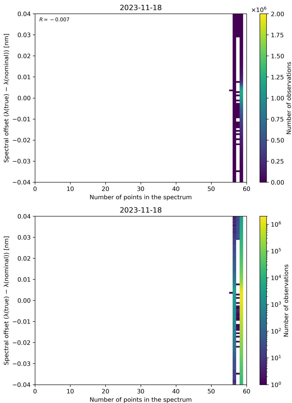
Figure 110: Scatter density plot of “Number of points in the spectrum” against “Spectral offset ( \lambda(\text{true}) - \lambda(\text{nominal}) )” for 2023-11-18 to 2023-11-19.
