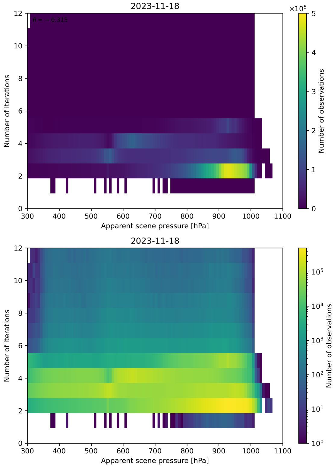
Figure 66: Scatter density plot of “Apparent scene pressure” against “Number of iterations” for 2023-11-18 to 2023-11-19.
