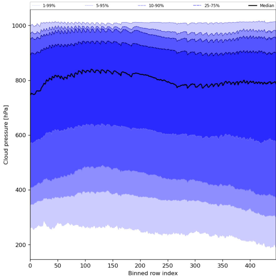
Figure 47: Along track statistics of “Cloud pressure” for 2023-11-18 to 2023-11-19
