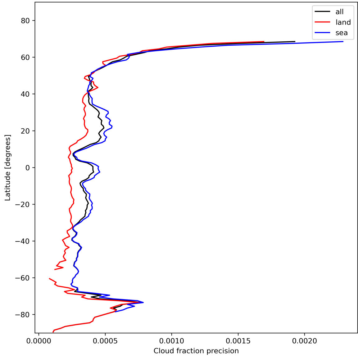
Figure 16: Zonal average of “Cloud fraction precision” for 2023-11-18 to 2023-11-19.
