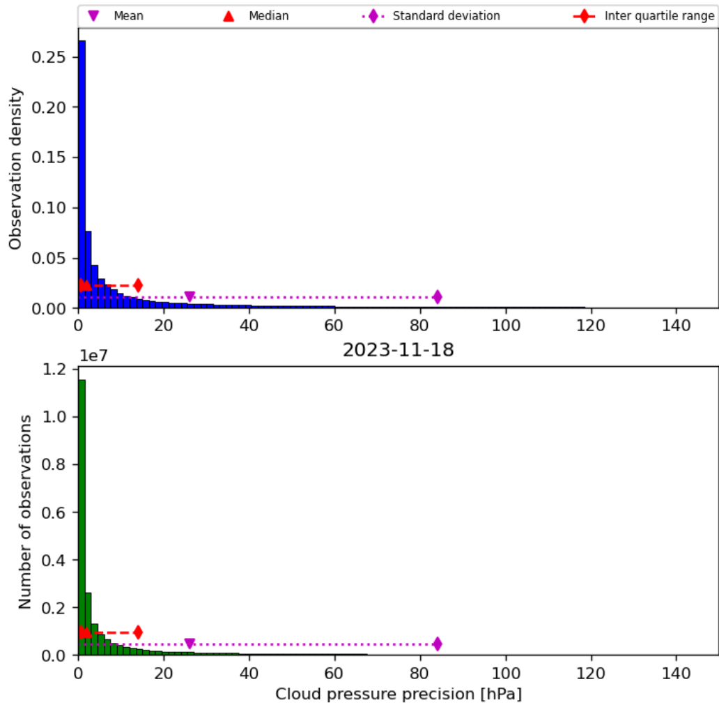
Figure 31: Histogram of “Cloud pressure precision” for 2023-11-18 to 2023-11-19
