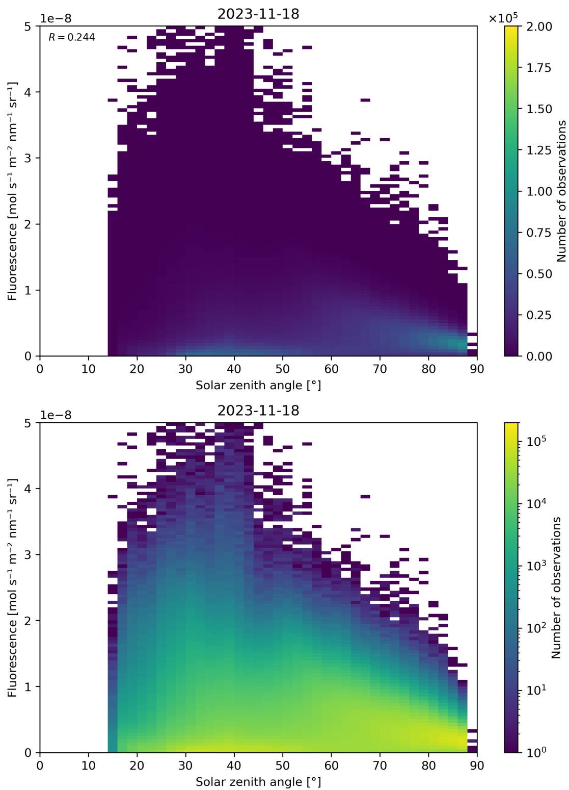
Figure 123: Scatter density plot of “Solar zenith angle” against “Fluorescence” for 2023-11-18 to 2023-11-19.
