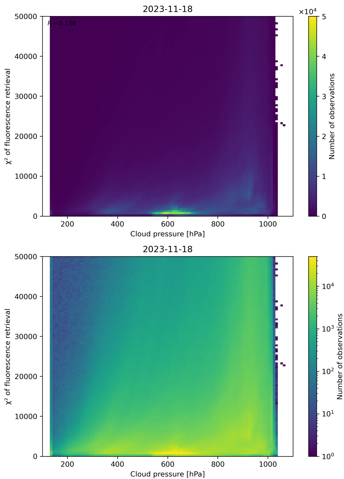
Figure 86: Scatter density plot of “Cloud pressure” against “ \chi^2 of fluorescence retrieval” for 2023-11-18 to 2023-11-19.
