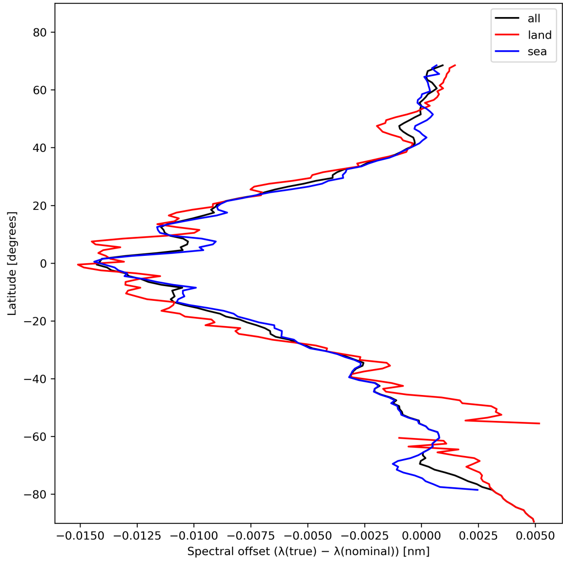
Figure 28: Zonal average of “Spectral offset ( \lambda(\text{true}) - \lambda(\text{nominal}) )” for 2023-11-18 to 2023-11-19.
