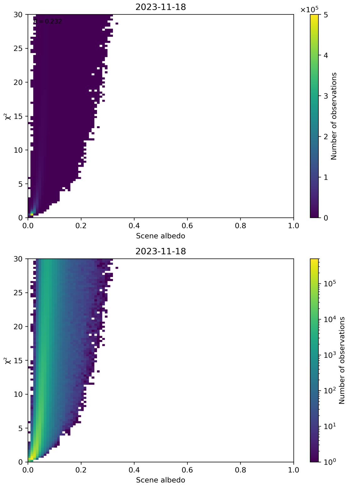
Figure 112: Scatter density plot of “Scene albedo” against “ \chi^2 ” for 2023-11-18 to 2023-11-19.
