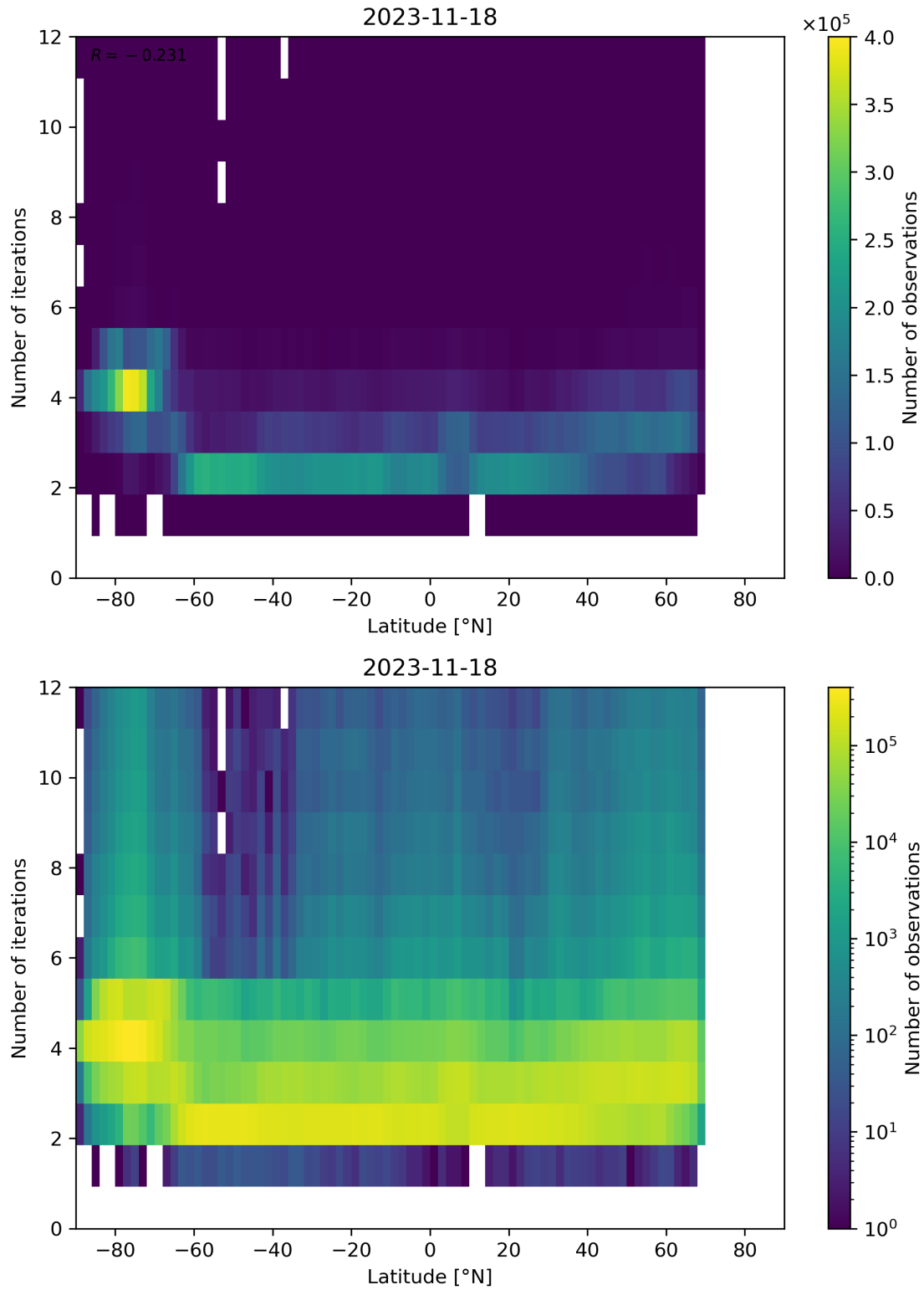
Figure 102: Scatter density plot of “Latitude” against “Number of iterations” for 2023-11-18 to 2023-11-19.
