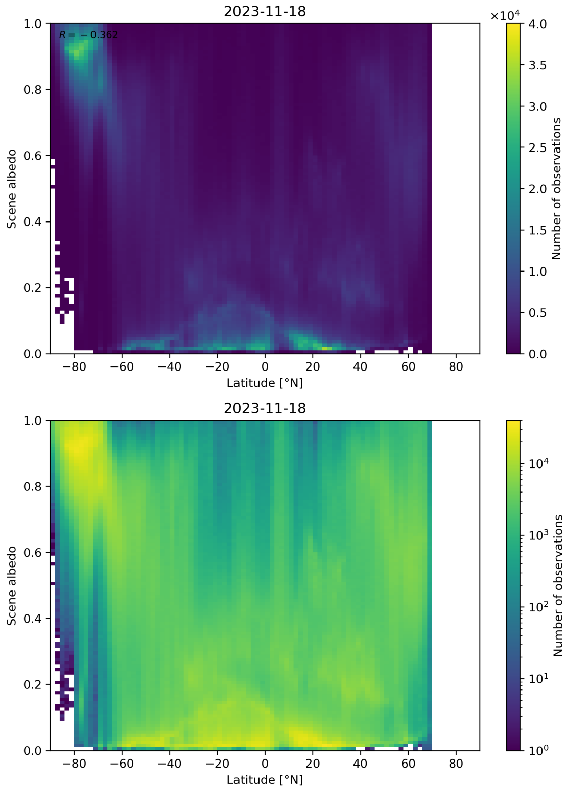
Figure 104: Scatter density plot of “Latitude” against “Scene albedo” for 2023-11-18 to 2023-11-19.
