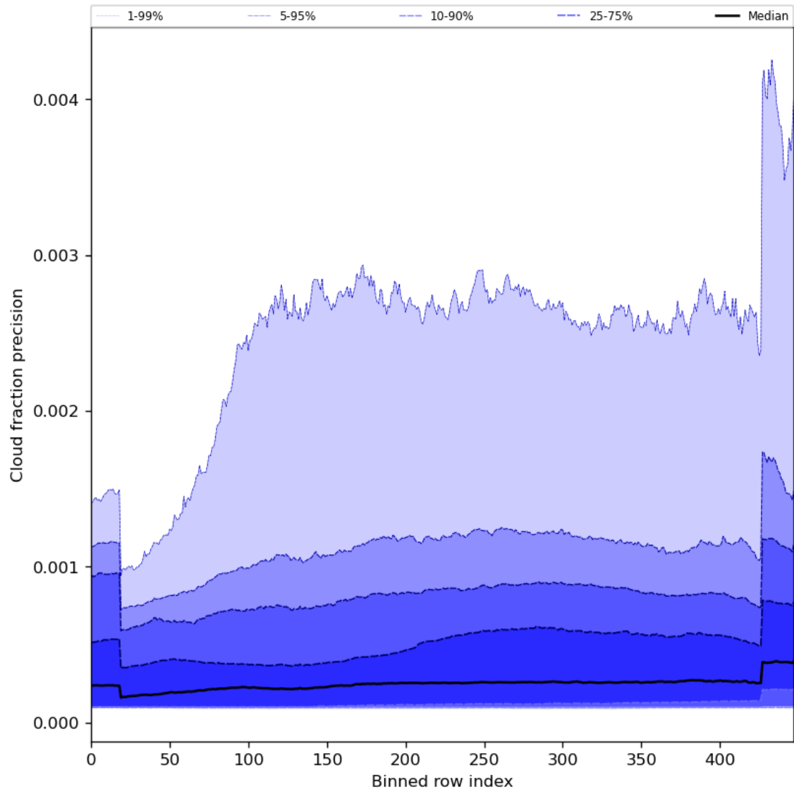
Figure 50: Along track statistics of “Cloud fraction precision” for 2023-11-18 to 2023-11-19
