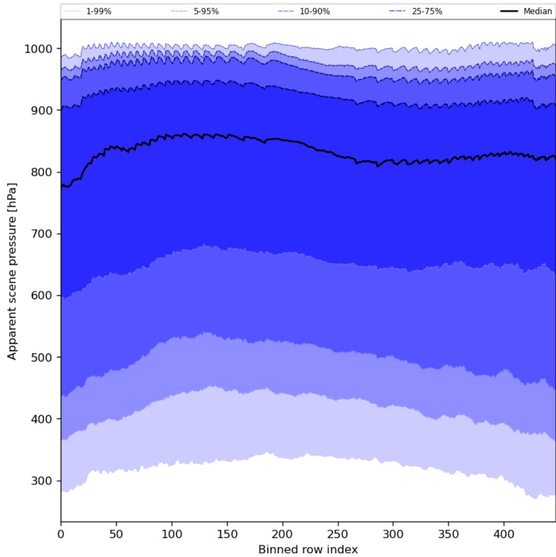
Figure 53: Along track statistics of “Apparent scene pressure” for 2023-11-18 to 2023-11-19
