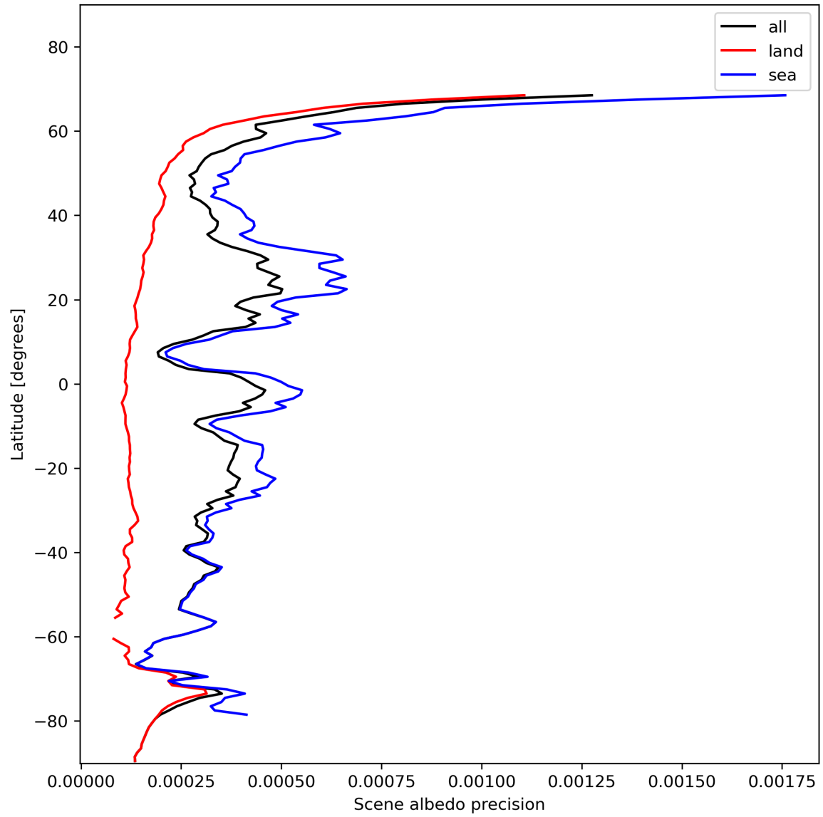
Figure 18: Zonal average of “Scene albedo precision” for 2023-11-18 to 2023-11-19.
