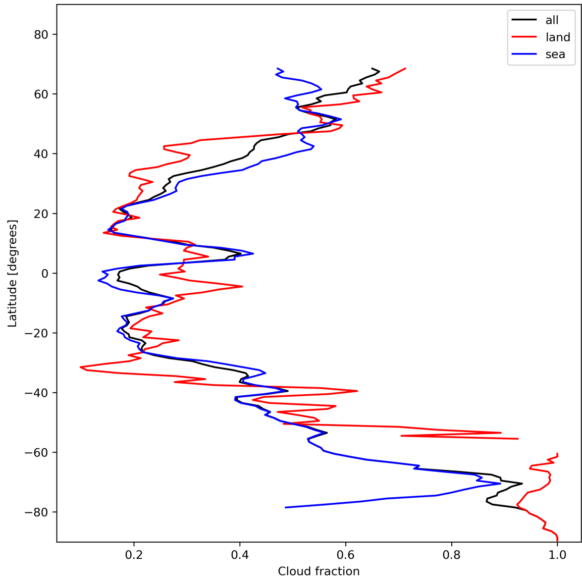
Figure 15: Zonal average of “Cloud fraction” for 2023-11-18 to 2023-11-19.
