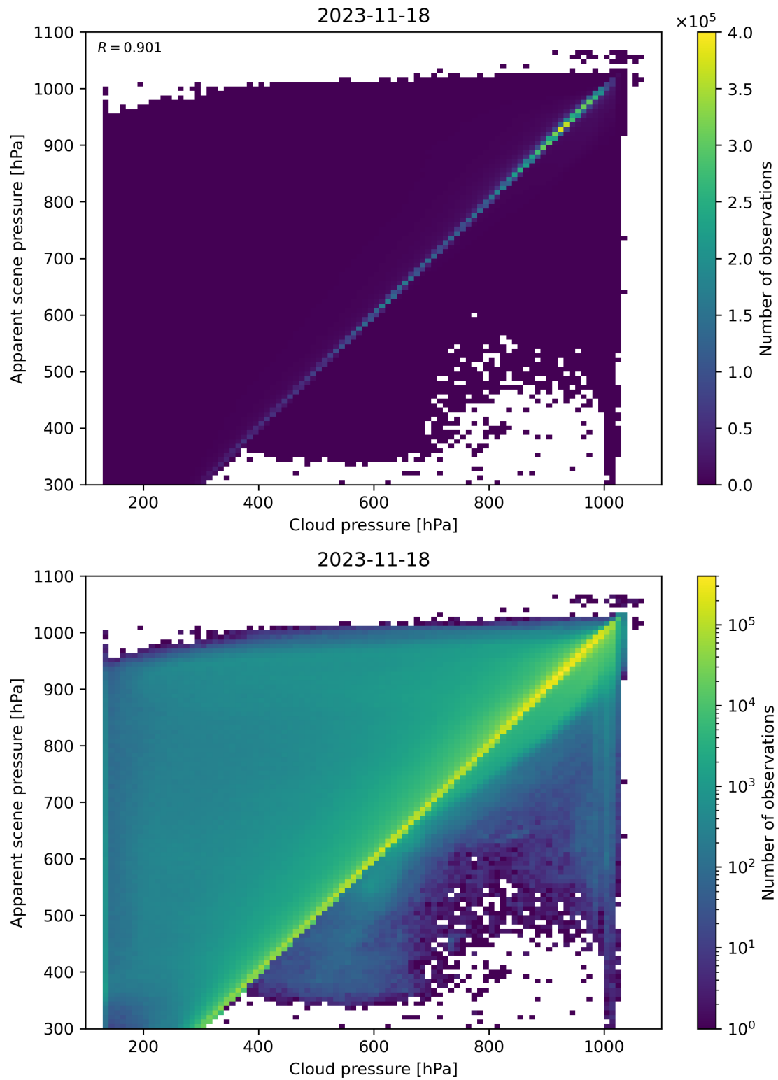
Figure 84: Scatter density plot of “Cloud pressure” against “Apparent scene pressure” for 2023-11-18 to 2023-11-19.
