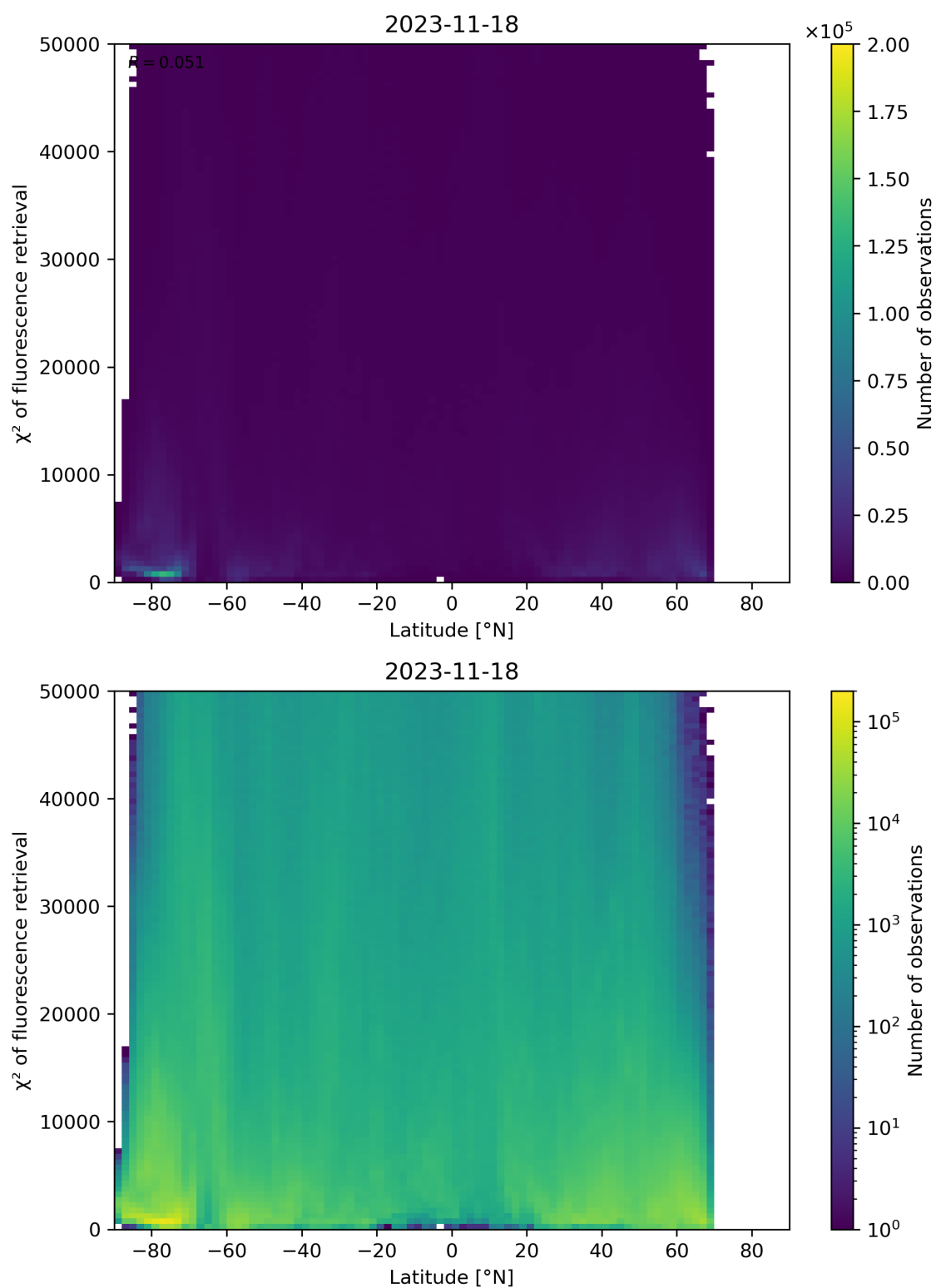
Figure 98: Scatter density plot of “Latitude” against “ \chi^2 of fluorescence retrieval” for 2023-11-18 to 2023-11-19.
