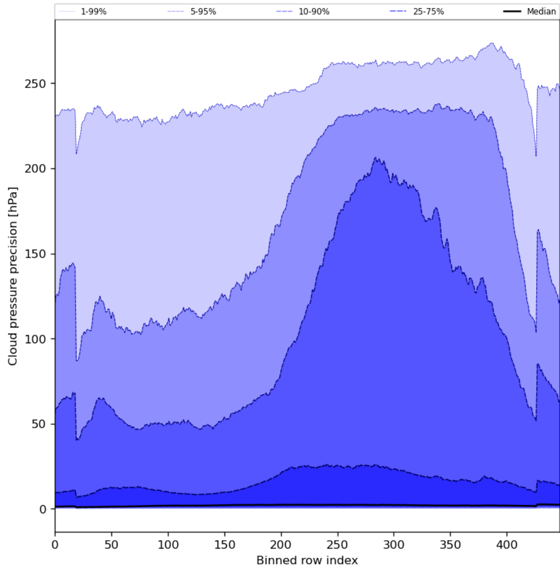
Figure 48: Along track statistics of “Cloud pressure precision” for 2023-11-18 to 2023-11-19
