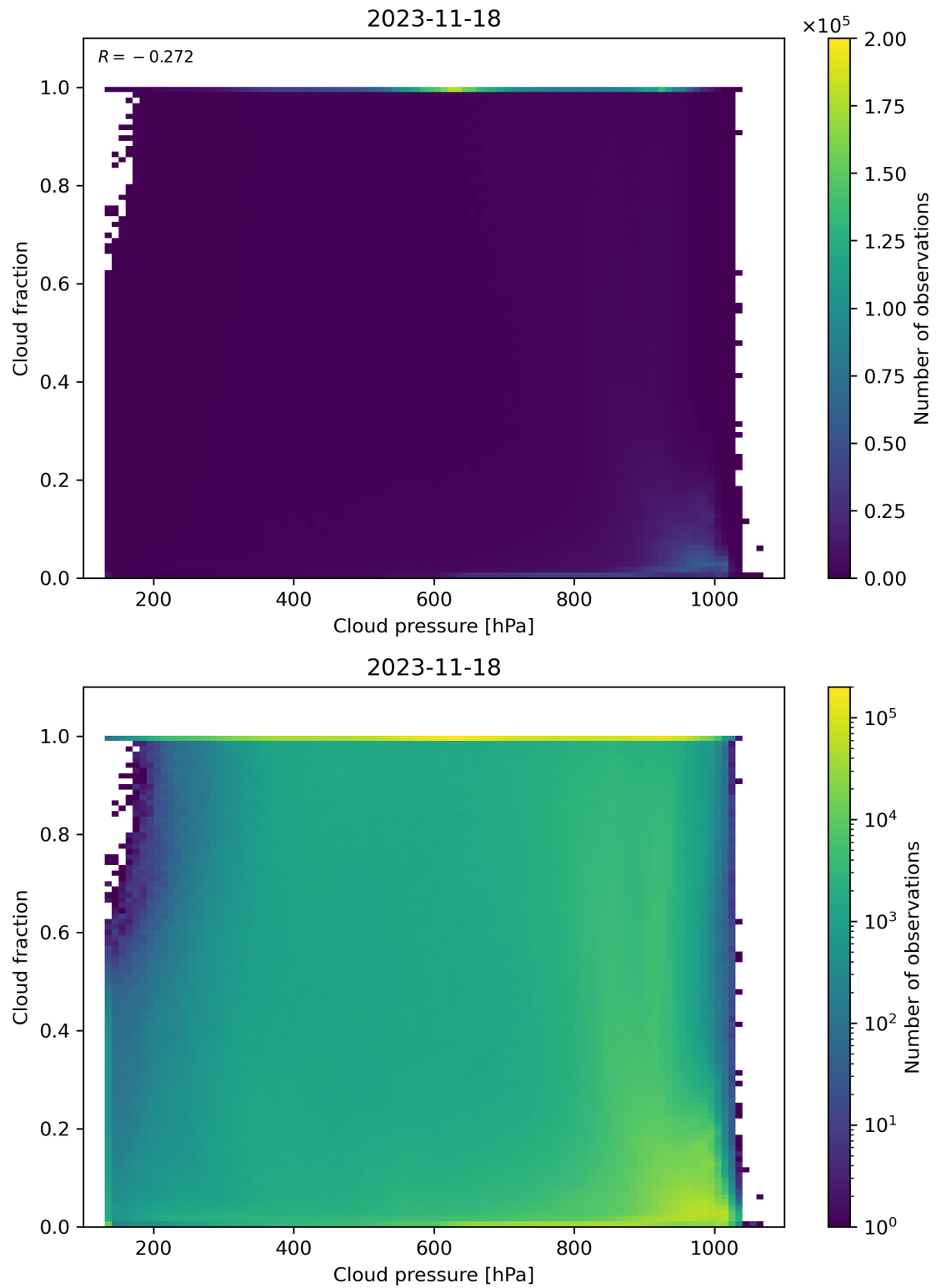
Figure 87: Scatter density plot of “Cloud pressure” against “Cloud fraction” for 2023-11-18 to 2023-11-19.
