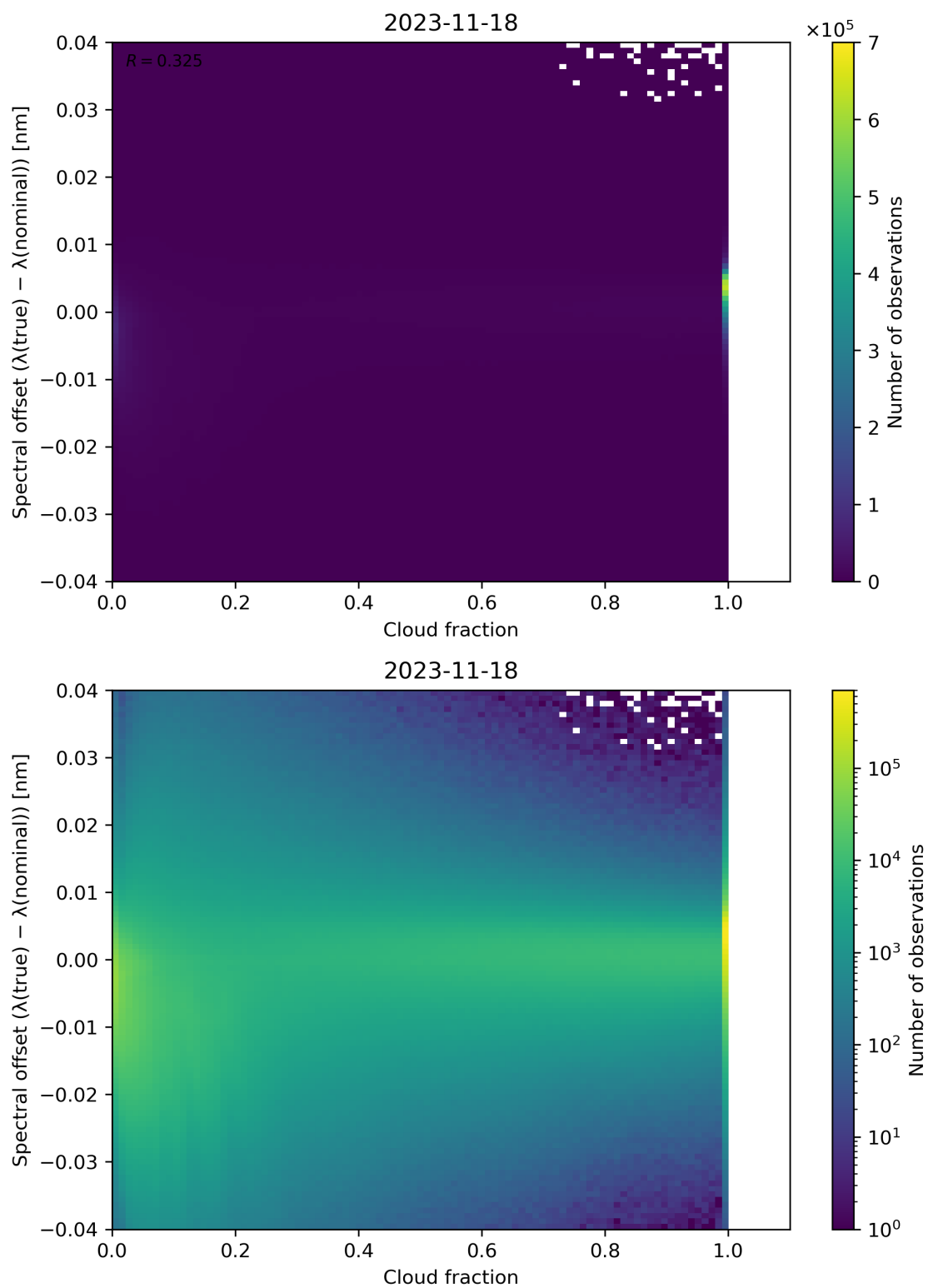
Figure 83: Scatter density plot of “Cloud fraction” against “Spectral offset ( \lambda(\text{true}) - \lambda(\text{nominal}) )” for 2023-11-18 to 2023-11-19.
