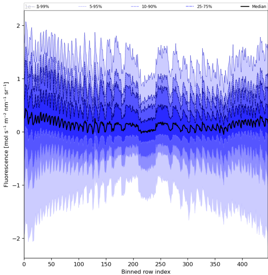
Figure 57: Along track statistics of “Fluorescence” for 2023-11-18 to 2023-11-19
