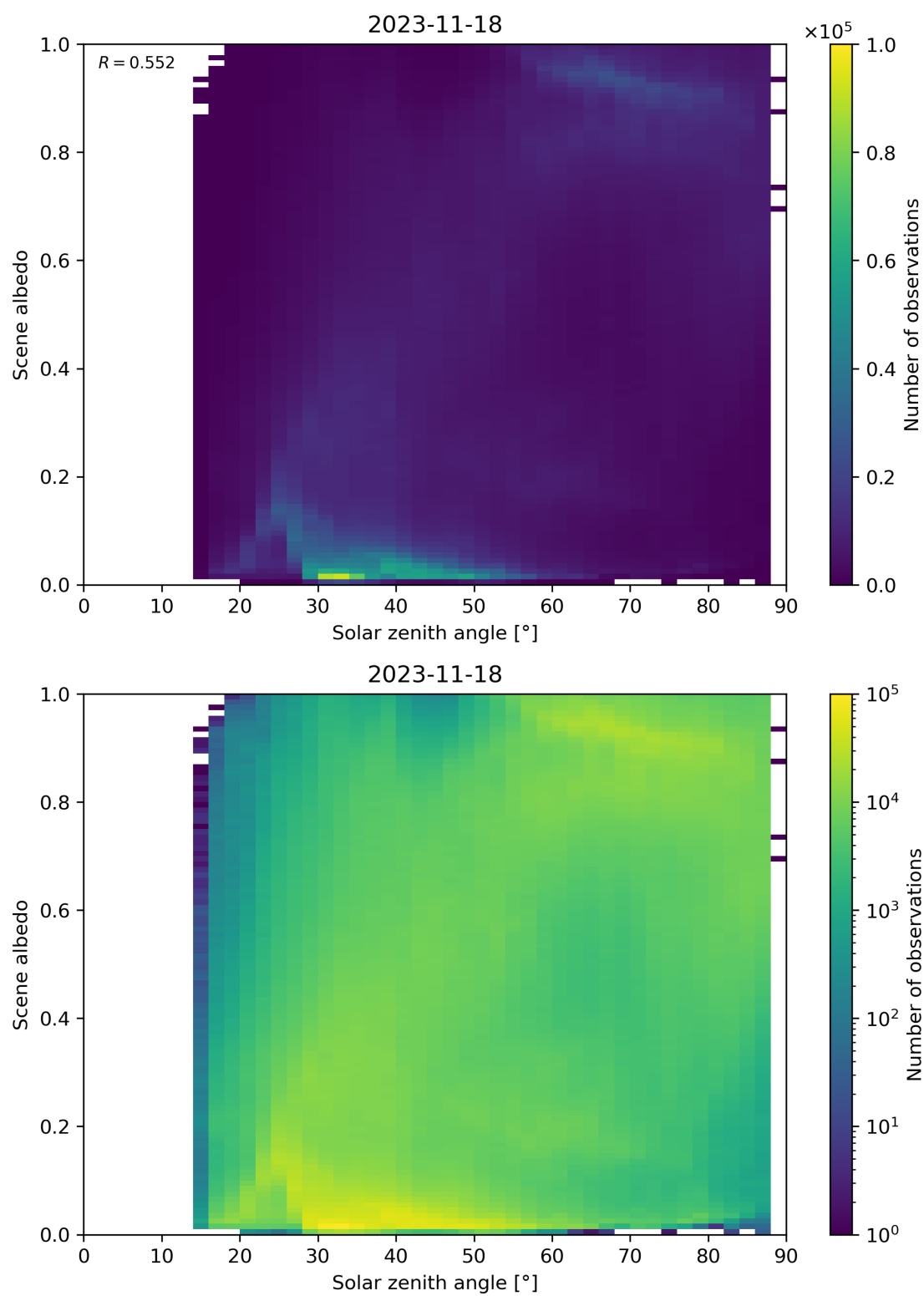
Figure 127: Scatter density plot of “Solar zenith angle” against “Scene albedo” for 2023-11-18 to 2023-11-19.
