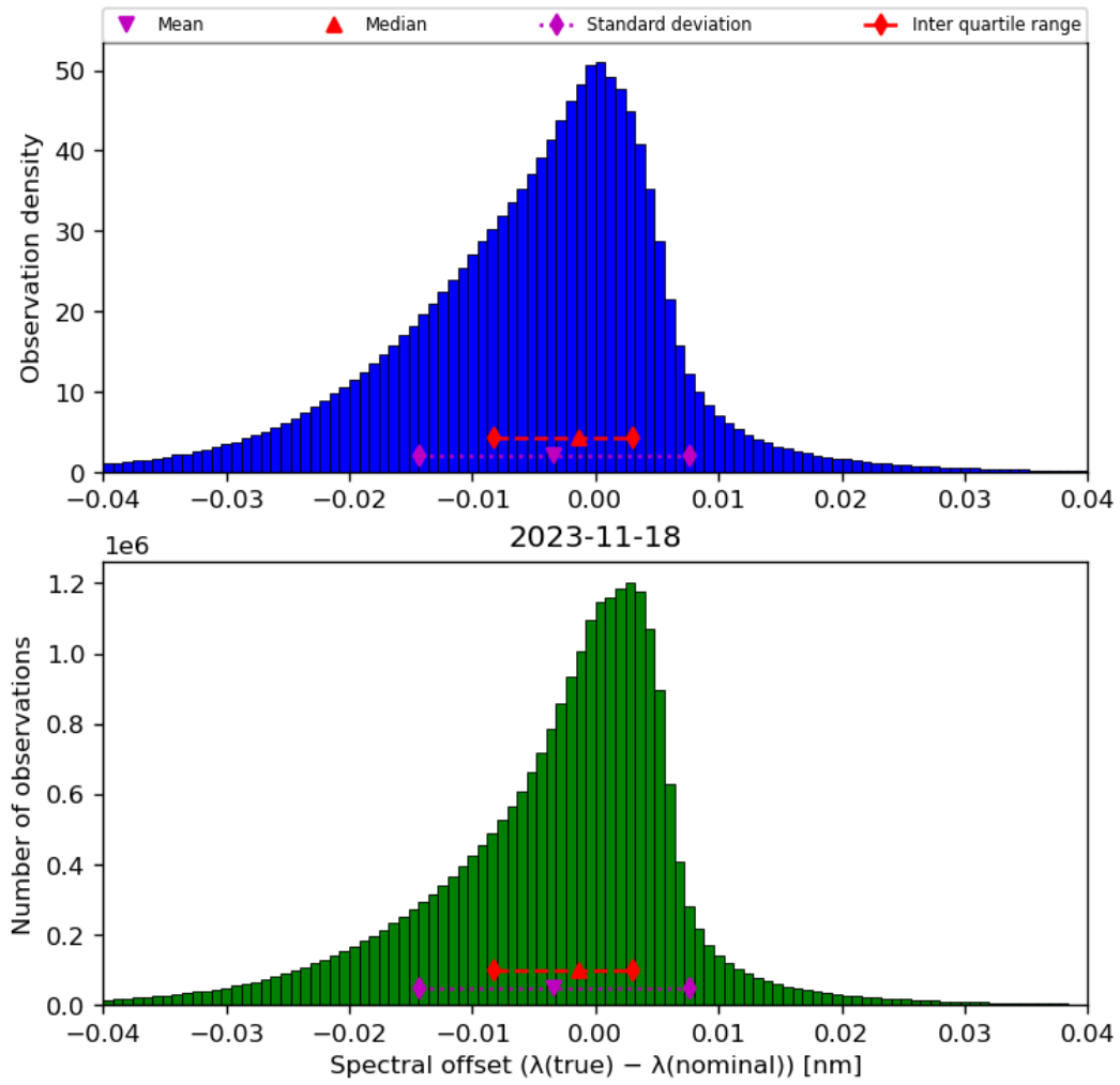
Figure 45: Histogram of “Spectral offset ( \lambda(\text{true}) - \lambda(\text{nominal}) )” for 2023-11-18 to 2023-11-19
