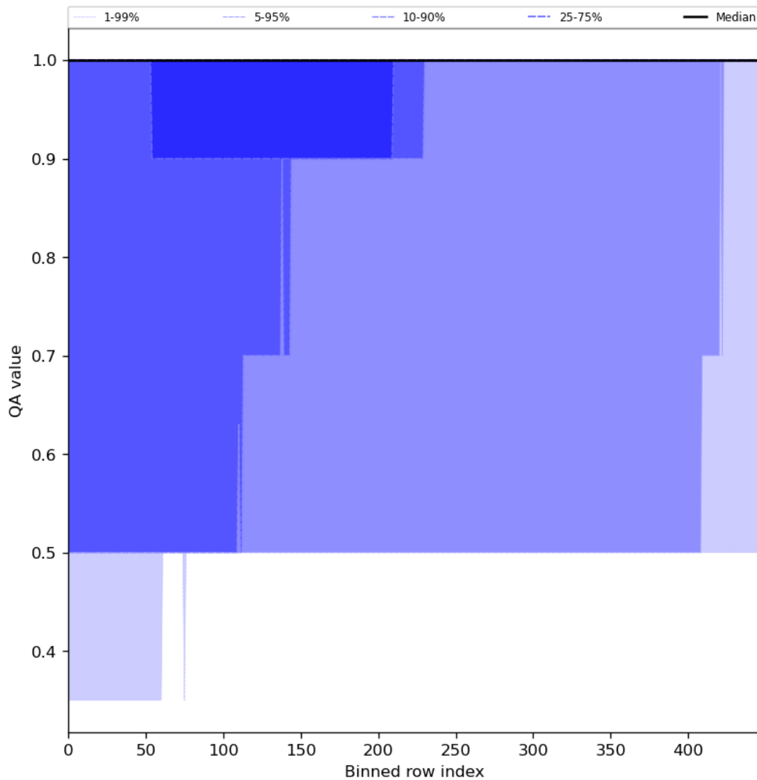
Figure 46: Along track statistics of “QA value” for 2023-11-18 to 2023-11-19
