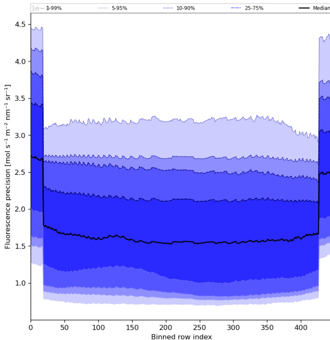
Figure 58: Along track statistics of “Fluorescence precision” for 2023-11-18 to 2023-11-19
