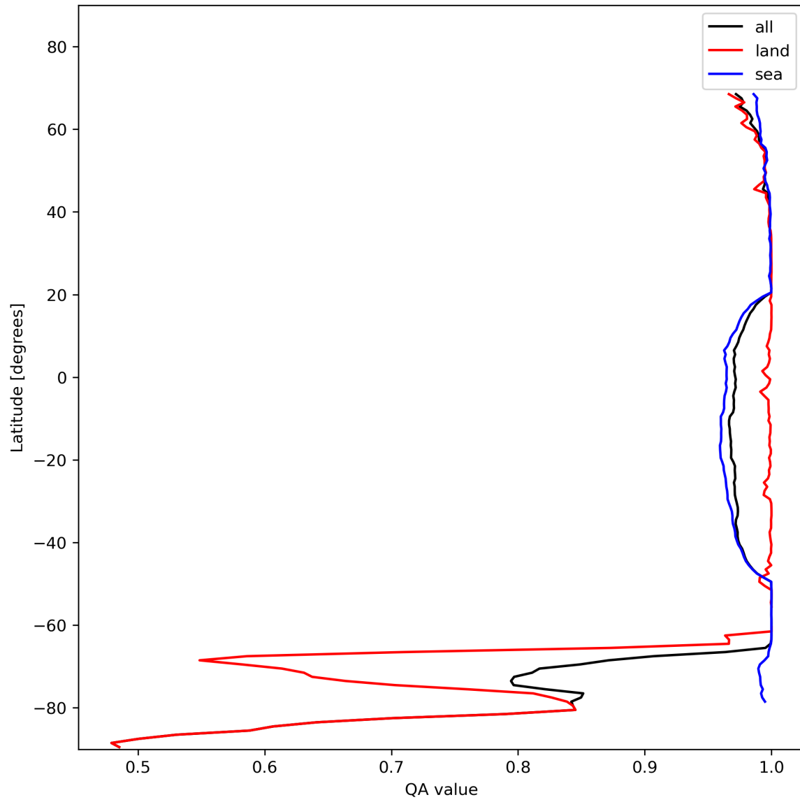
Figure 12: Zonal average of “QA value” for 2023-11-18 to 2023-11-19.
