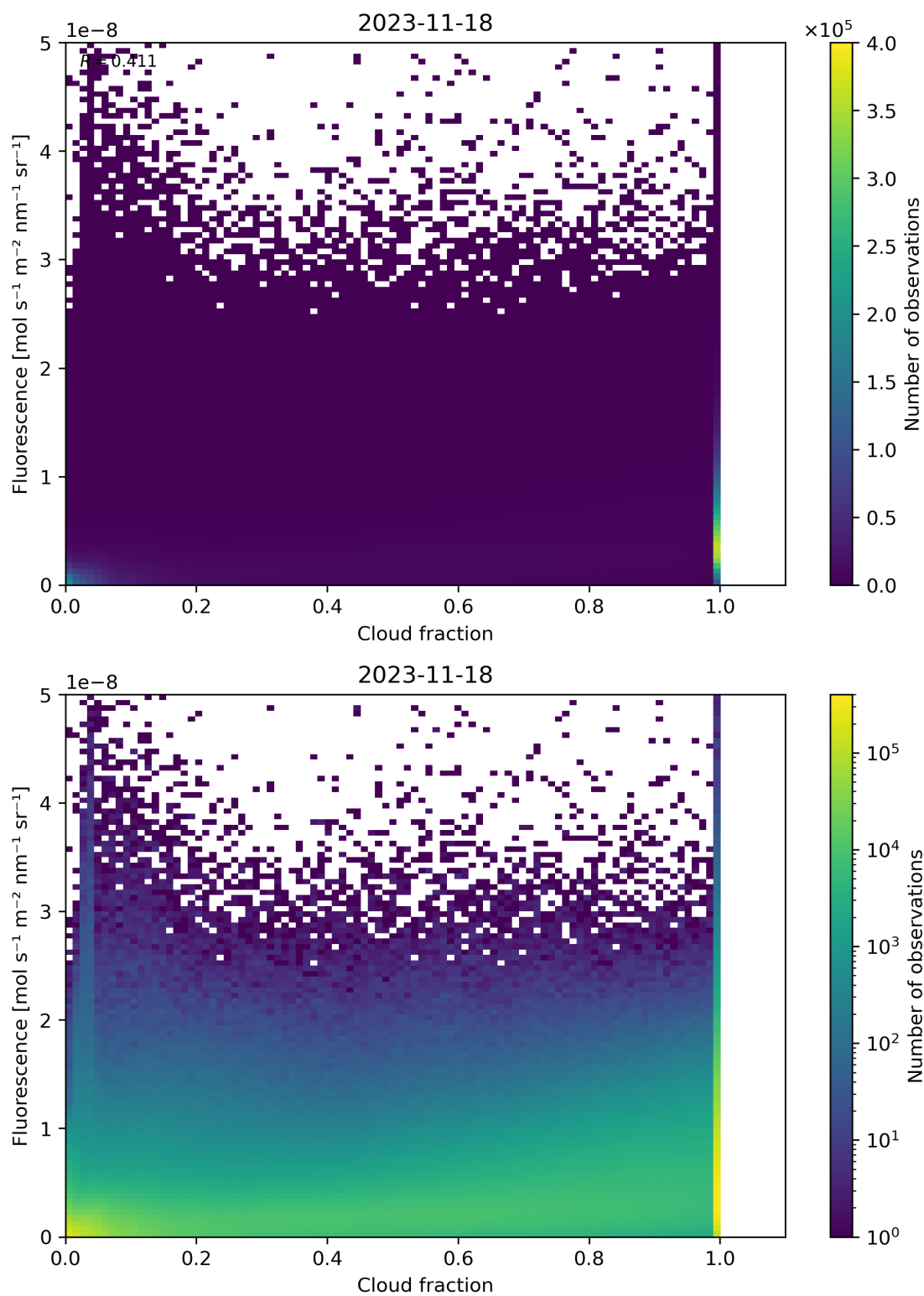
Figure 79: Scatter density plot of “Cloud fraction” against “Fluorescence” for 2023-11-18 to 2023-11-19.
