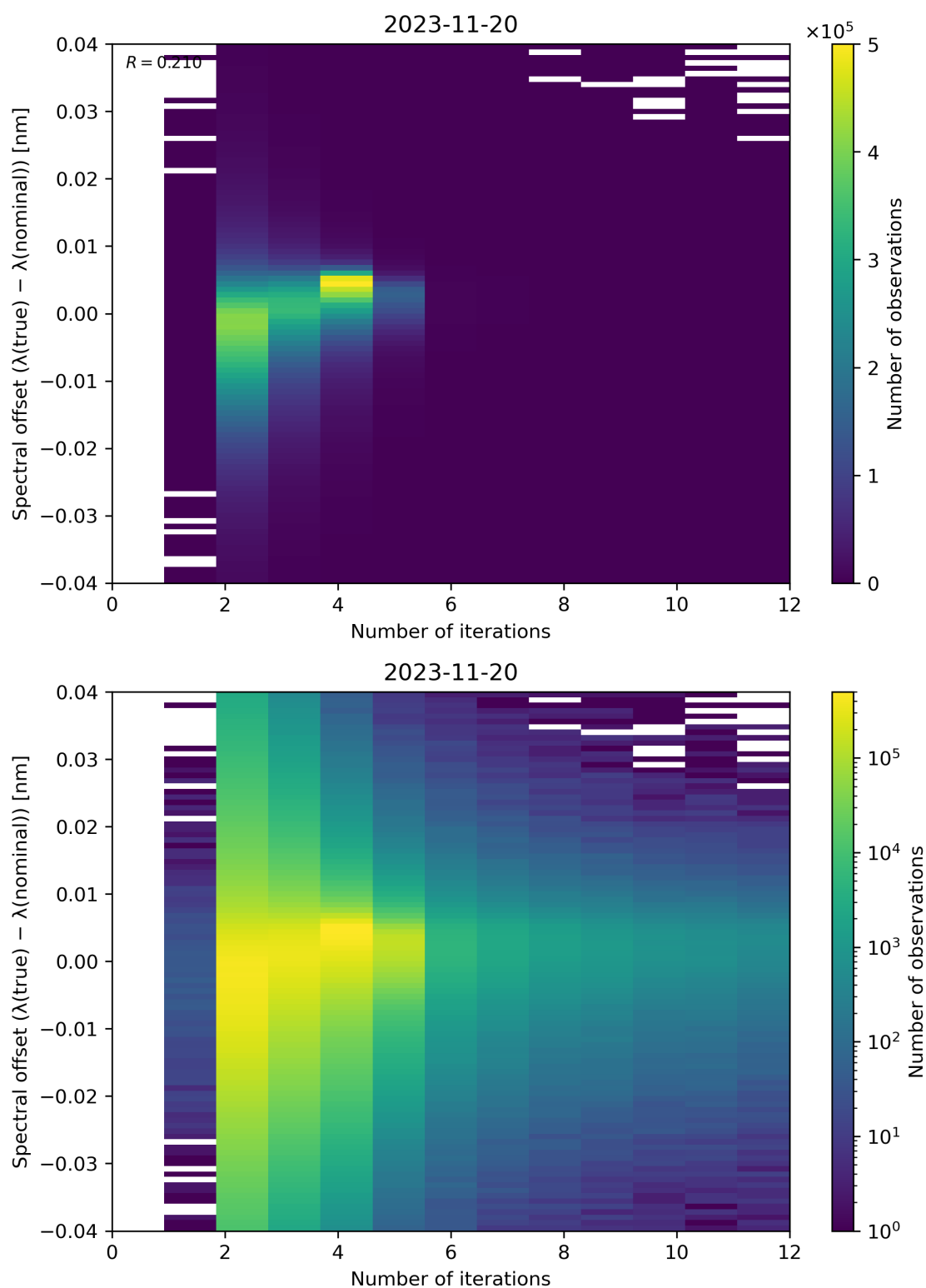
Figure 109: Scatter density plot of “Number of iterations” against “Spectral offset ( \lambda(\text{true}) - \lambda(\text{nominal}) )” for 2023-11-19 to 2023-11-21.
