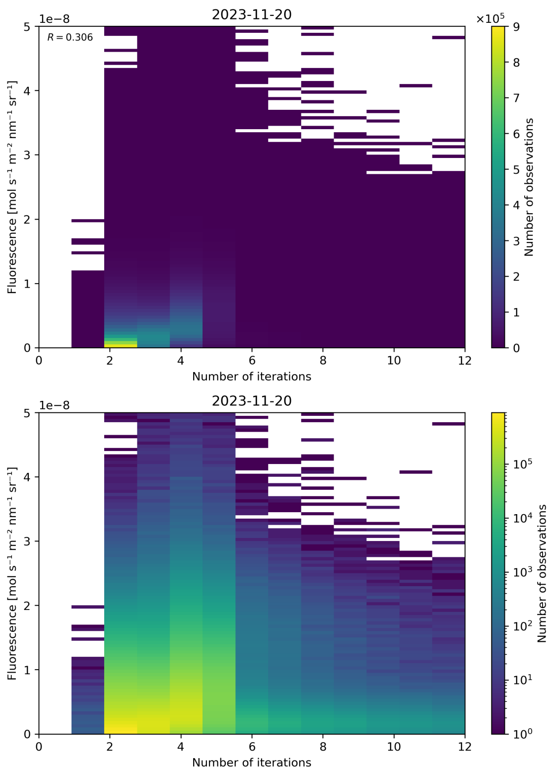
Figure 107: Scatter density plot of “Number of iterations” against “Fluorescence” for 2023-11-19 to 2023-11-21.
