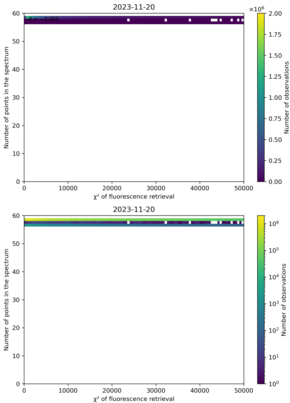
Figure 71: Scatter density plot of " \chi^2 of fluorescence retrieval" against "Number of points in the spectrum" for 2023-11-19 to 2023-11-21.
