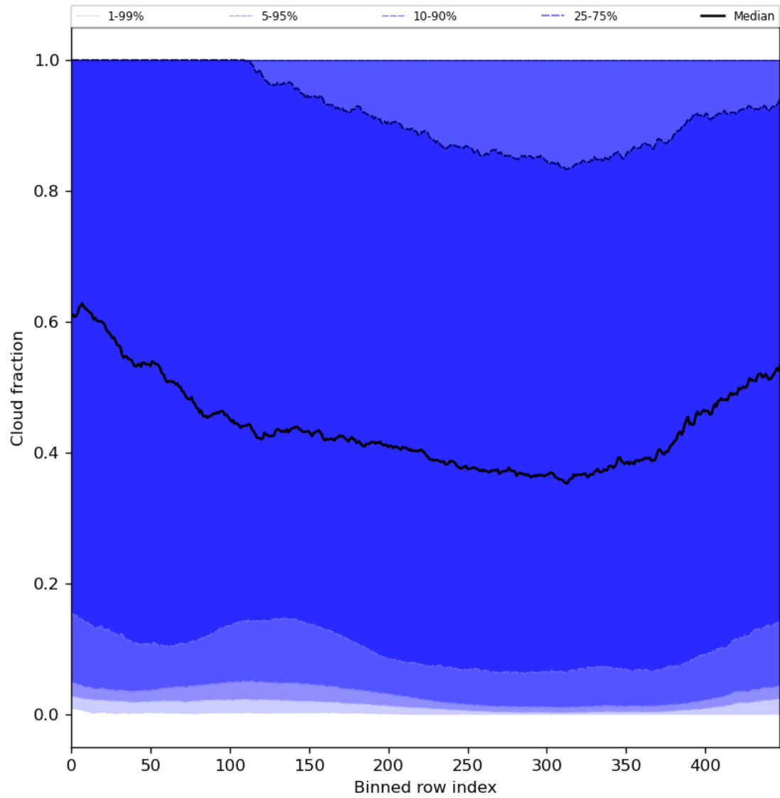
Figure 49: Along track statistics of “Cloud fraction” for 2023-11-19 to 2023-11-21
