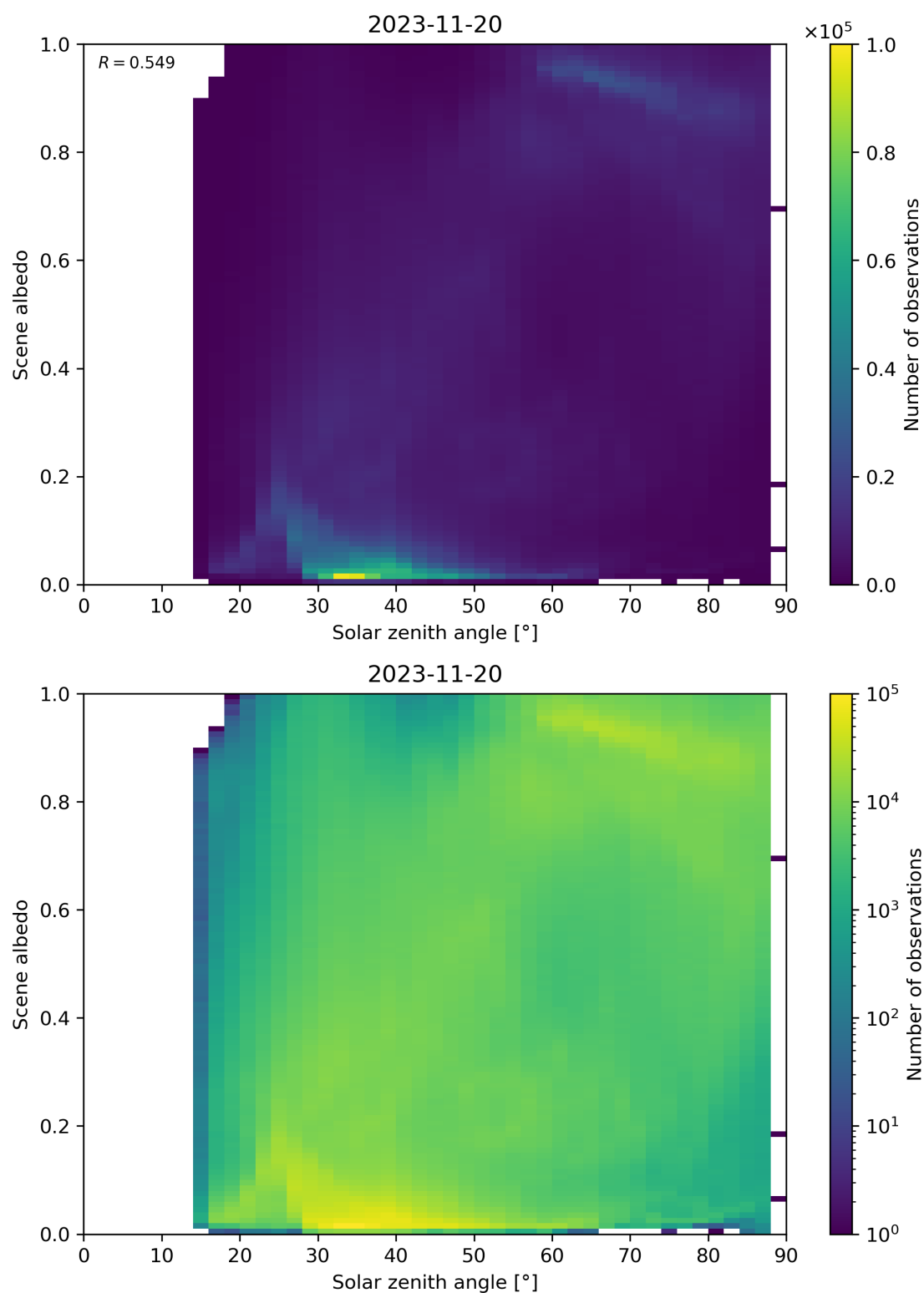
Figure 127: Scatter density plot of “Solar zenith angle” against “Scene albedo” for 2023-11-19 to 2023-11-21.
