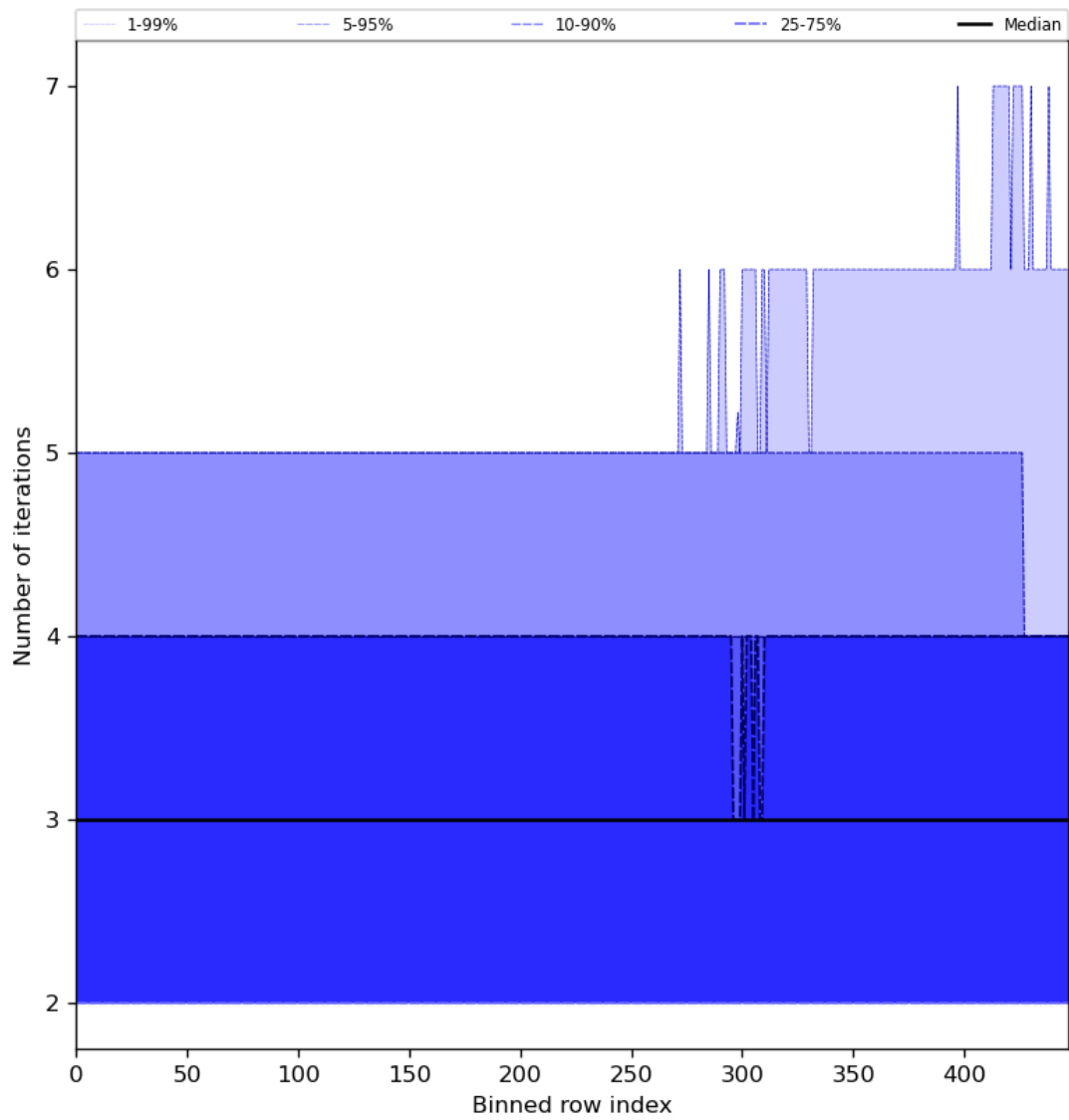
Figure 56: Along track statistics of “Number of iterations” for 2023-11-19 to 2023-11-21
