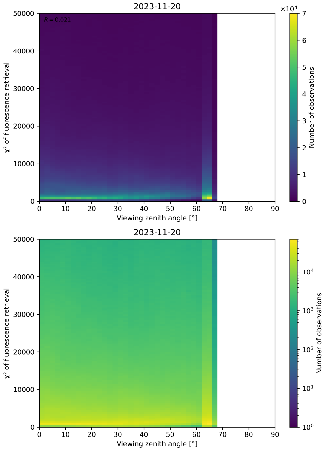
Figure 131: Scatter density plot of “Viewing zenith angle” against “ \chi^2 of fluorescence retrieval” for 2023-11-19 to 2023-11-21.
