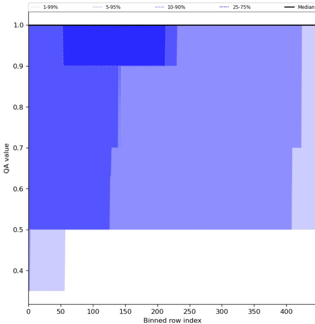
Figure 46: Along track statistics of “QA value” for 2023-11-19 to 2023-11-21
