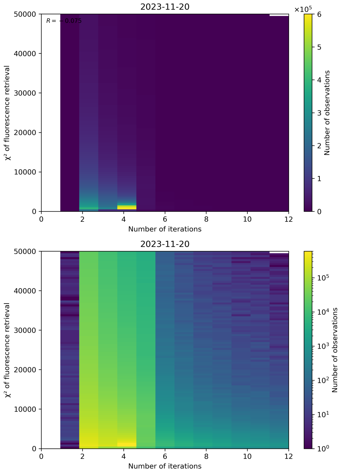
Figure 106: Scatter density plot of “Number of iterations” against “ \chi^2 of fluorescence retrieval” for 2023-11-19 to 2023-11-21.
