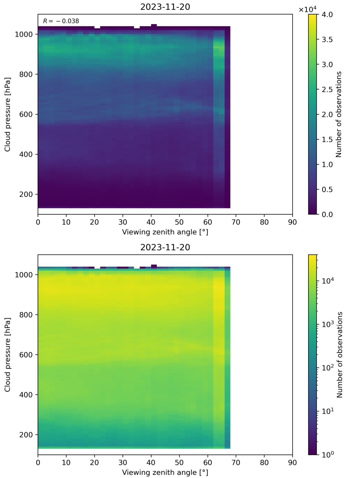
Figure 133: Scatter density plot of “Viewing zenith angle” against “Cloud pressure” for 2023-11-19 to 2023-11-21.
