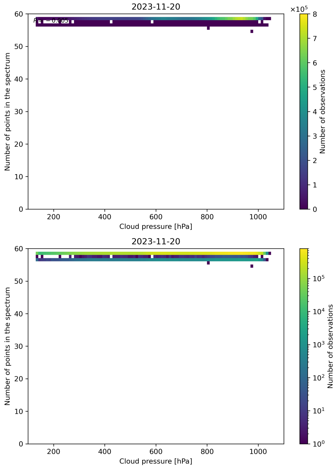
Figure 90: Scatter density plot of “Cloud pressure” against “Number of points in the spectrum” for 2023-11-19 to 2023-11-21.
