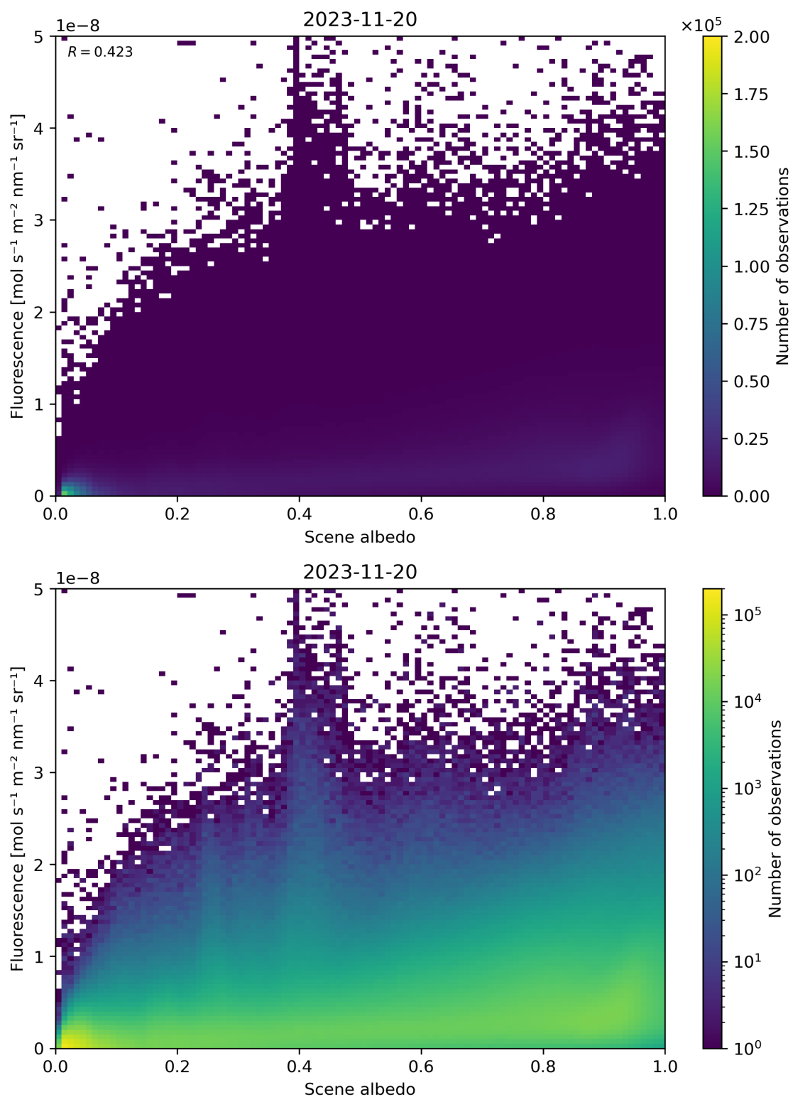
Figure 114: Scatter density plot of “Scene albedo” against “Fluorescence” for 2023-11-19 to 2023-11-21.
