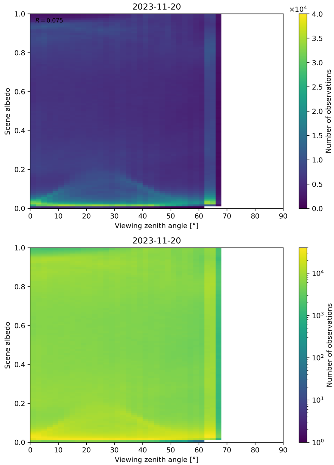
Figure 138: Scatter density plot of “Viewing zenith angle” against “Scene albedo” for 2023-11-19 to 2023-11-21.
