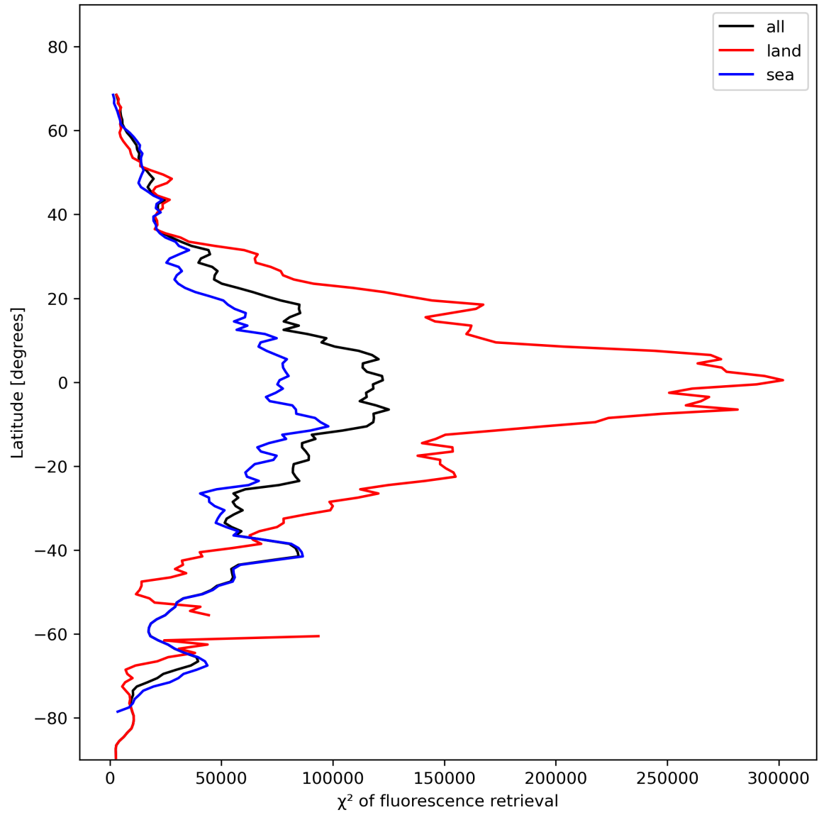
Figure 25: Zonal average of “ \chi^2 of fluorescence retrieval” for 2023-11-19 to 2023-11-21.
