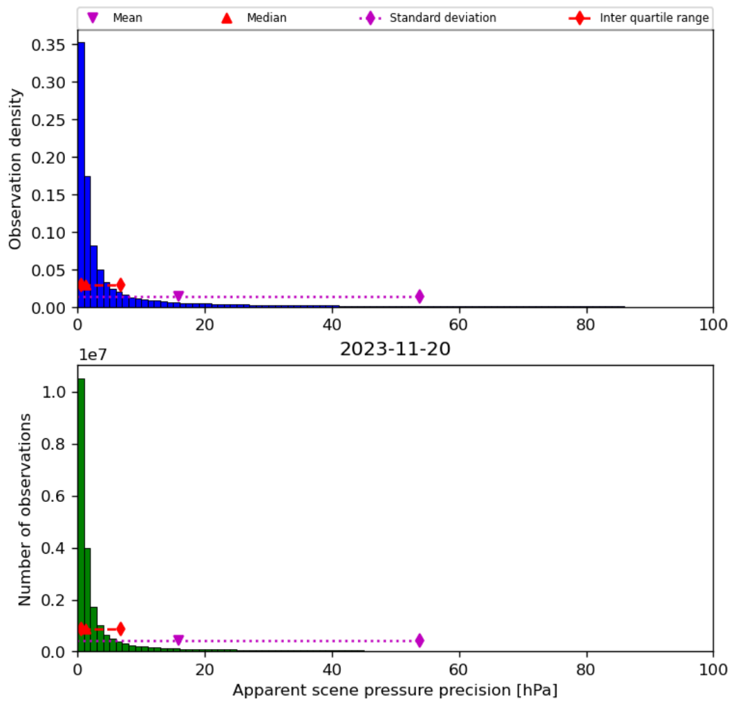
Figure 37: Histogram of “Apparent scene pressure precision” for 2023-11-19 to 2023-11-21
