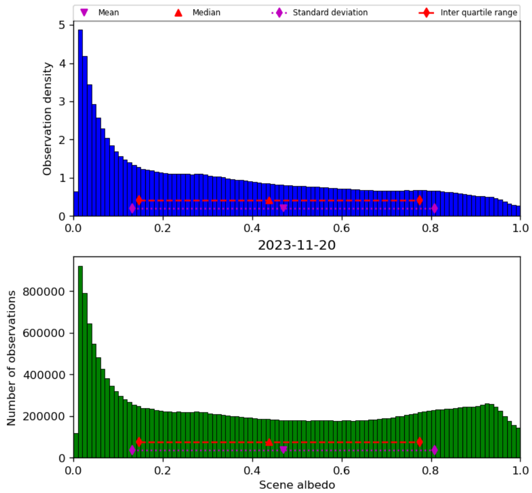
Figure 34: Histogram of “Scene albedo” for 2023-11-19 to 2023-11-21
