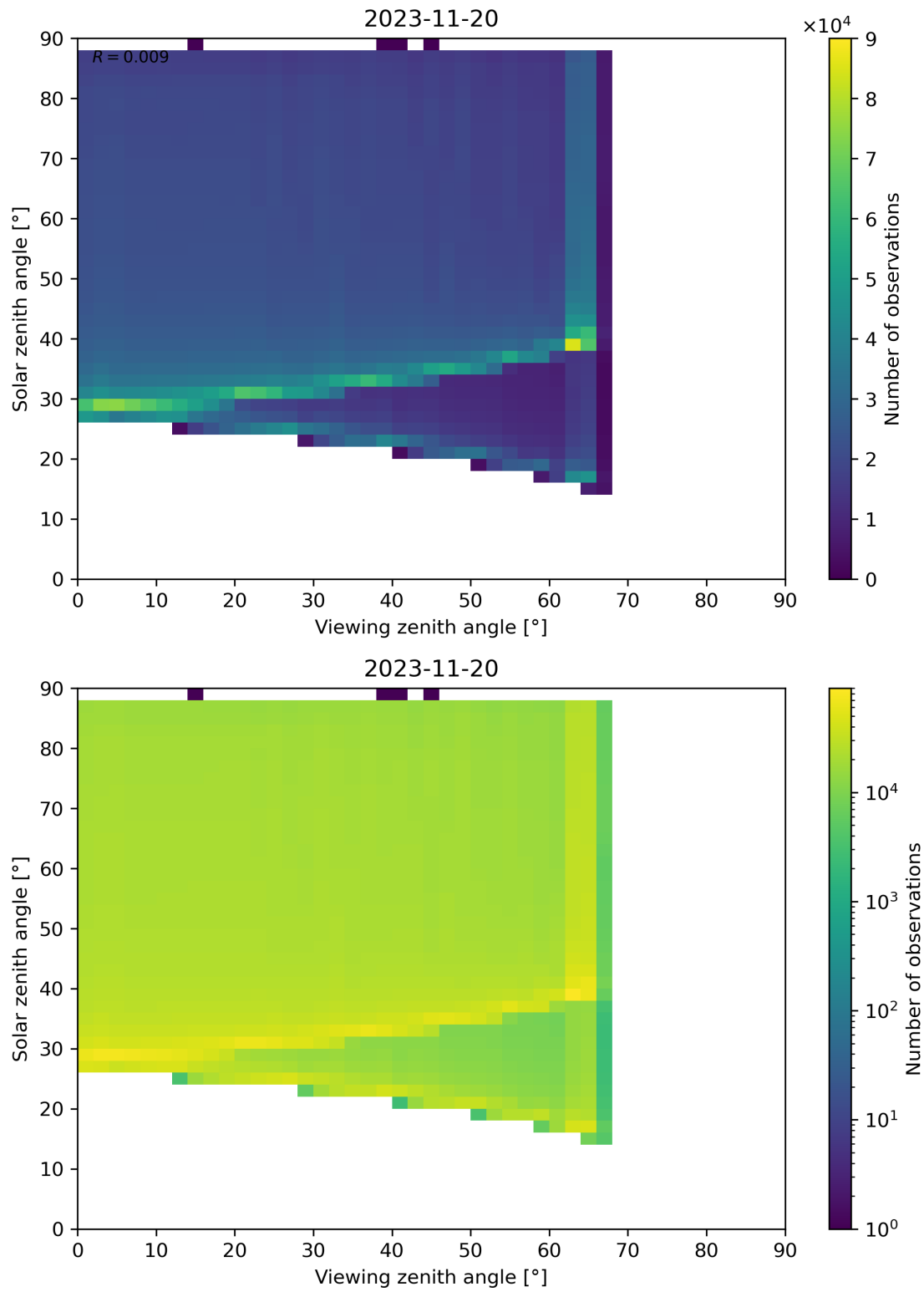
Figure 139: Scatter density plot of “Viewing zenith angle” against “Solar zenith angle” for 2023-11-19 to 2023-11-21.
