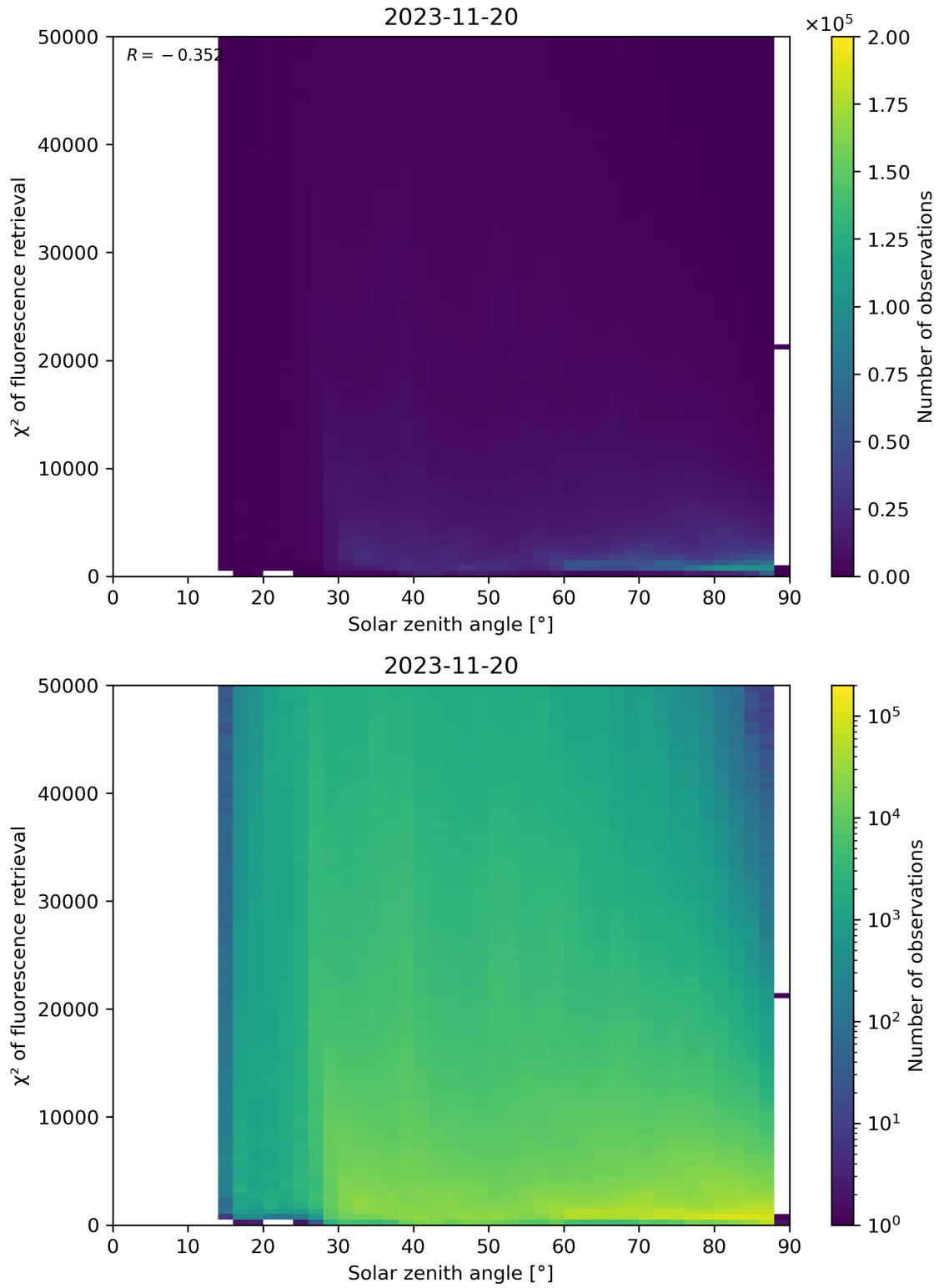
Figure 120: Scatter density plot of “Solar zenith angle” against “ \chi^2 of fluorescence retrieval” for 2023-11-19 to 2023-11-21.
