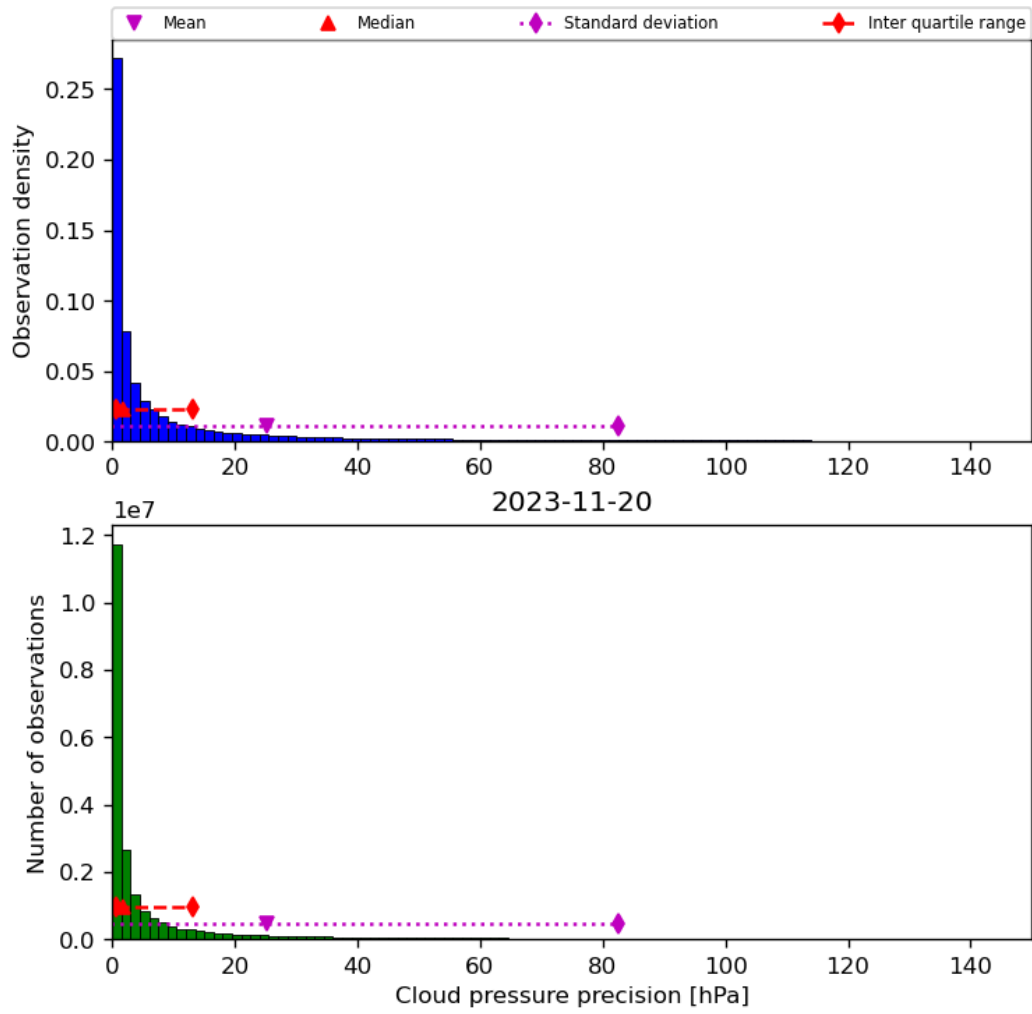
Figure 31: Histogram of “Cloud pressure precision” for 2023-11-19 to 2023-11-21
