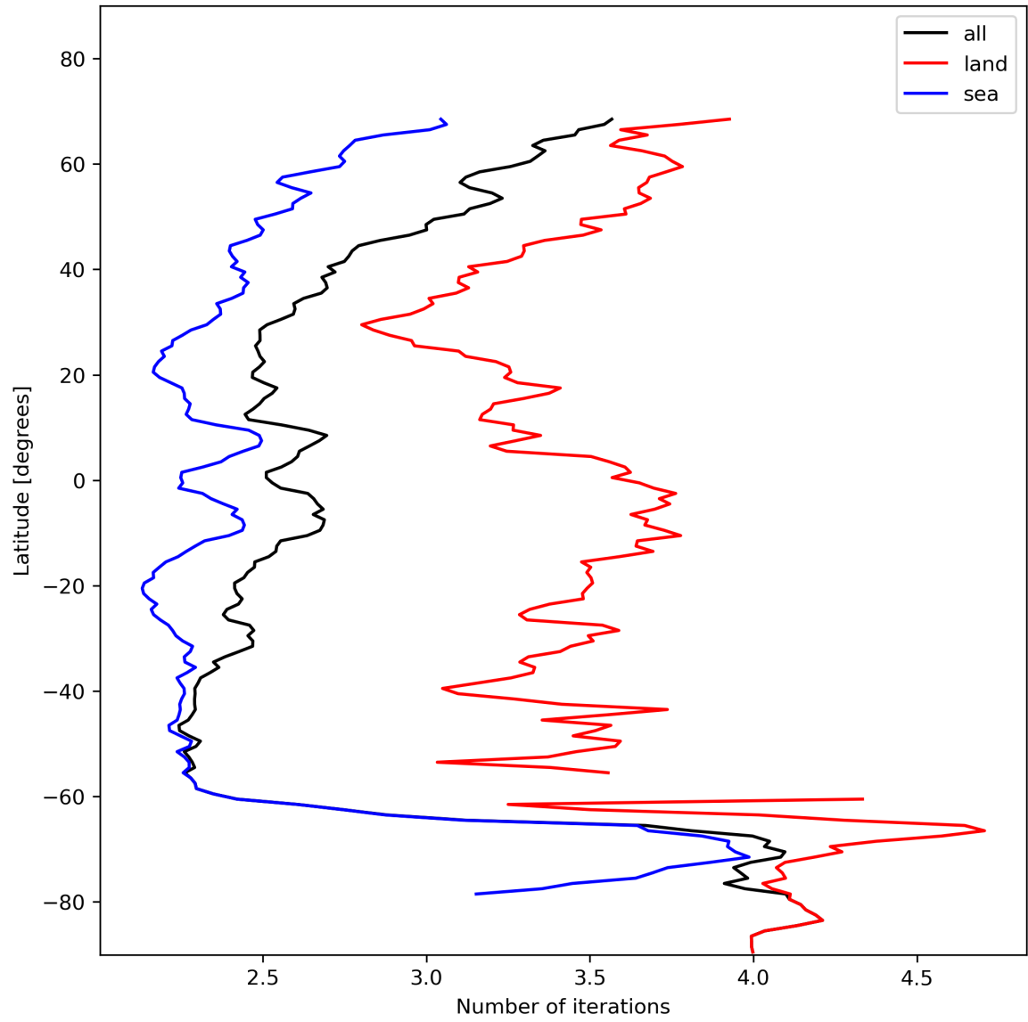
Figure 22: Zonal average of “Number of iterations” for 2023-11-19 to 2023-11-21.
