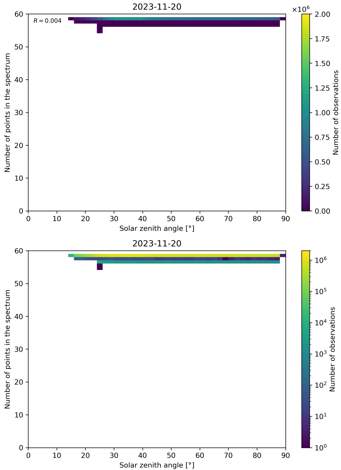
Figure 126: Scatter density plot of “Solar zenith angle” against “Number of points in the spectrum” for 2023-11-19 to 2023-11-21.
