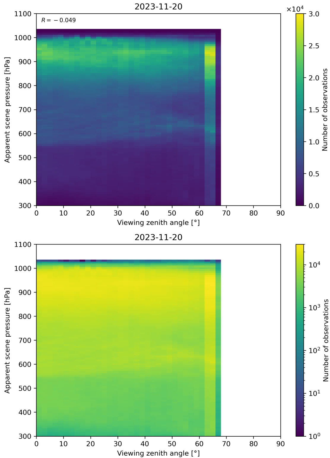
Figure 129: Scatter density plot of “Viewing zenith angle” against “Apparent scene pressure” for 2023-11-19 to 2023-11-21.
