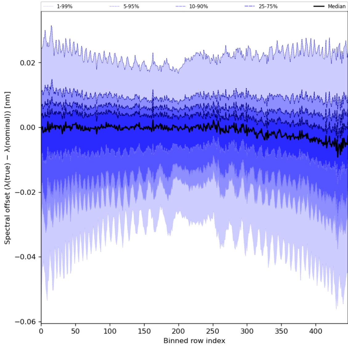
Figure 62: Along track statistics of “Spectral offset ( \lambda(\text{true}) - \lambda(\text{nominal}) )” for 2023-11-19 to 2023-11-21
