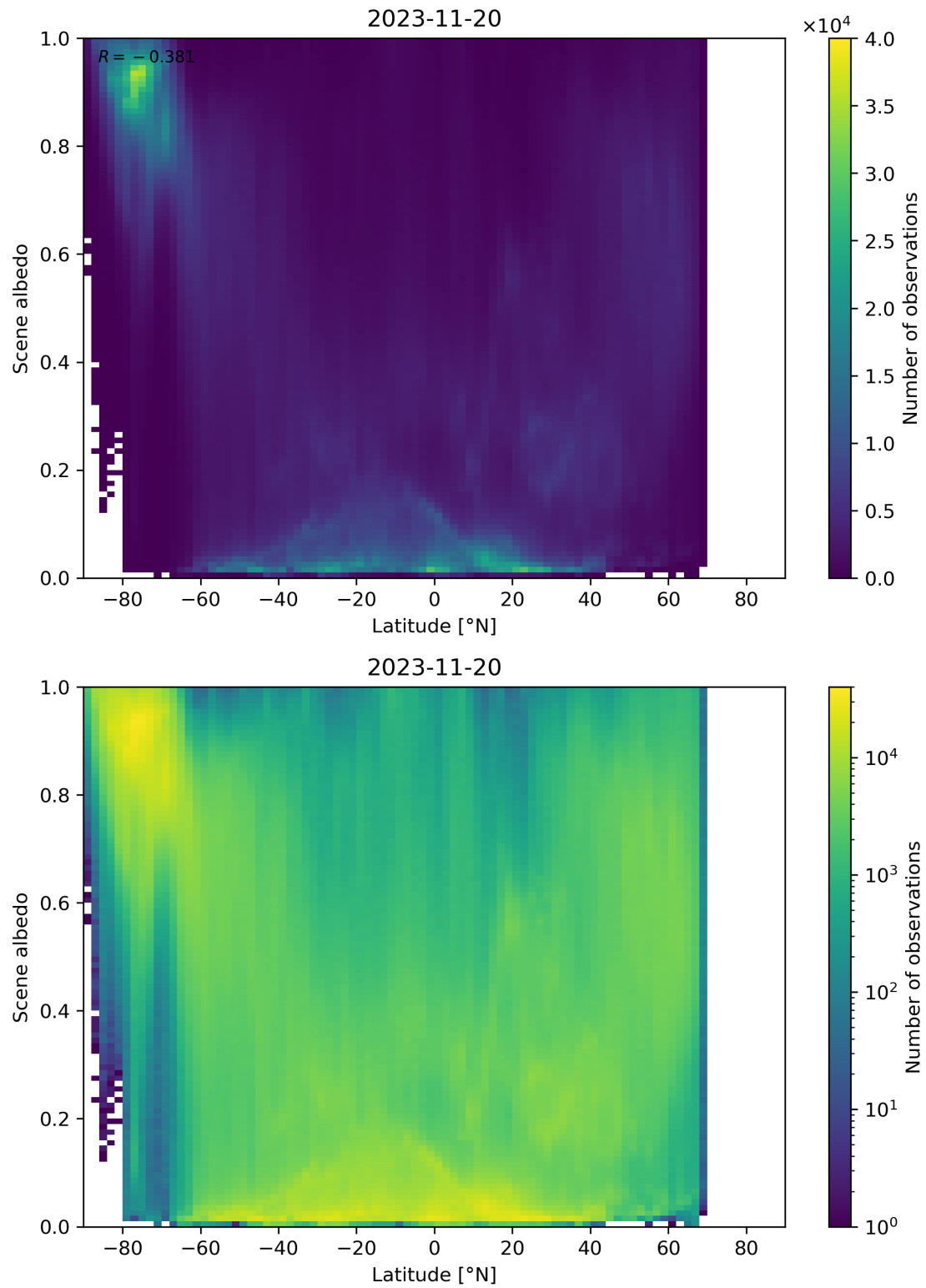
Figure 104: Scatter density plot of “Latitude” against “Scene albedo” for 2023-11-19 to 2023-11-21.
