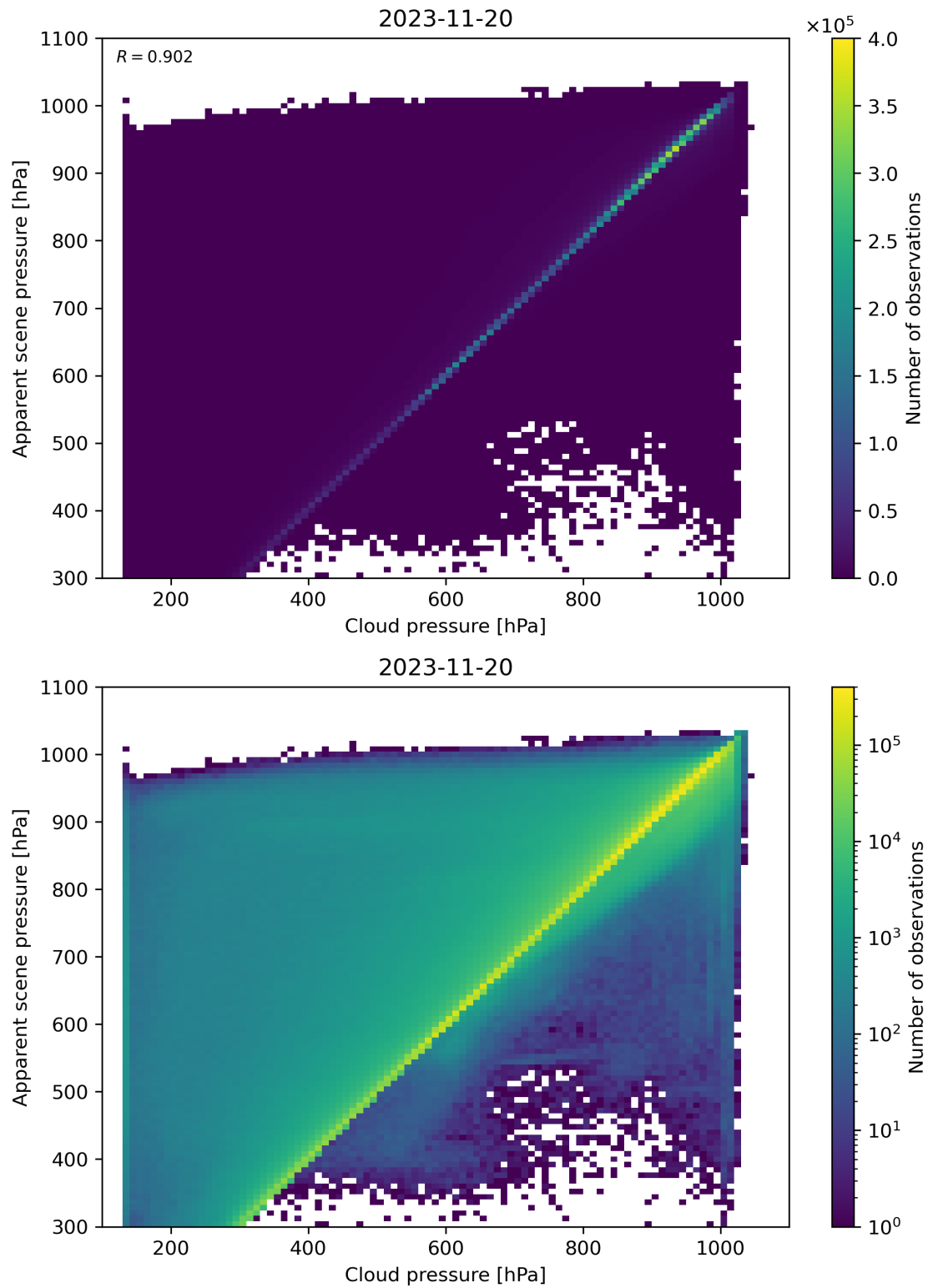
Figure 84: Scatter density plot of “Cloud pressure” against “Apparent scene pressure” for 2023-11-19 to 2023-11-21.
