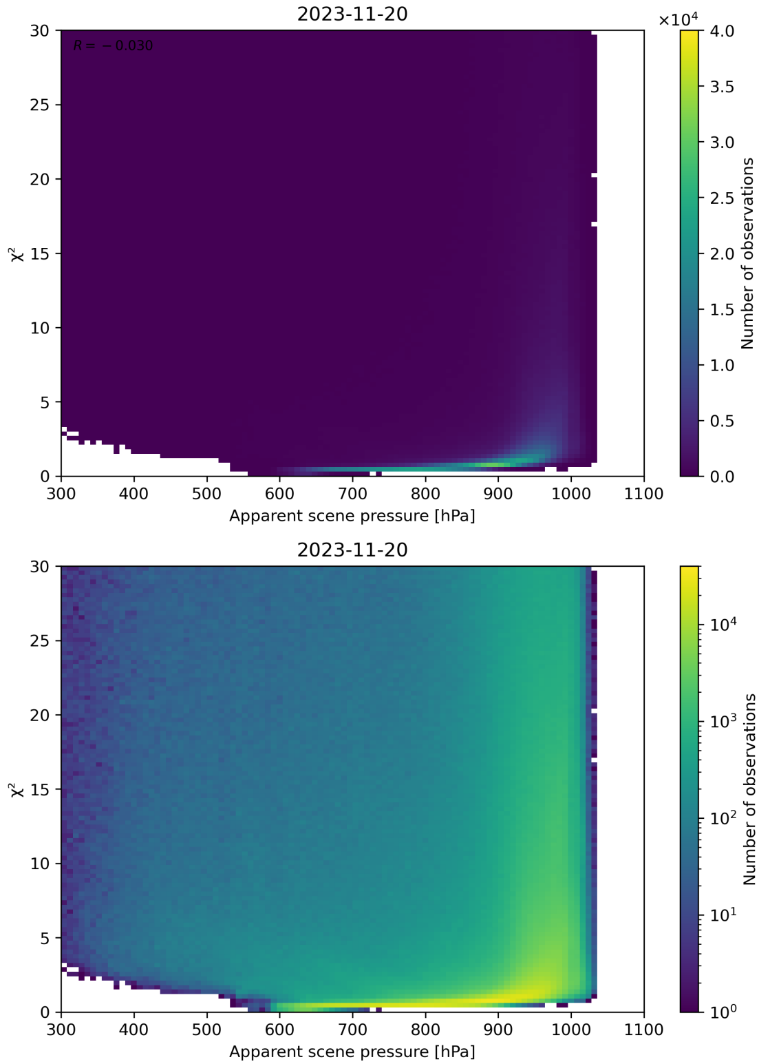
Figure 63: Scatter density plot of “Apparent scene pressure” against “ \chi^2 ” for 2023-11-19 to 2023-11-21.
