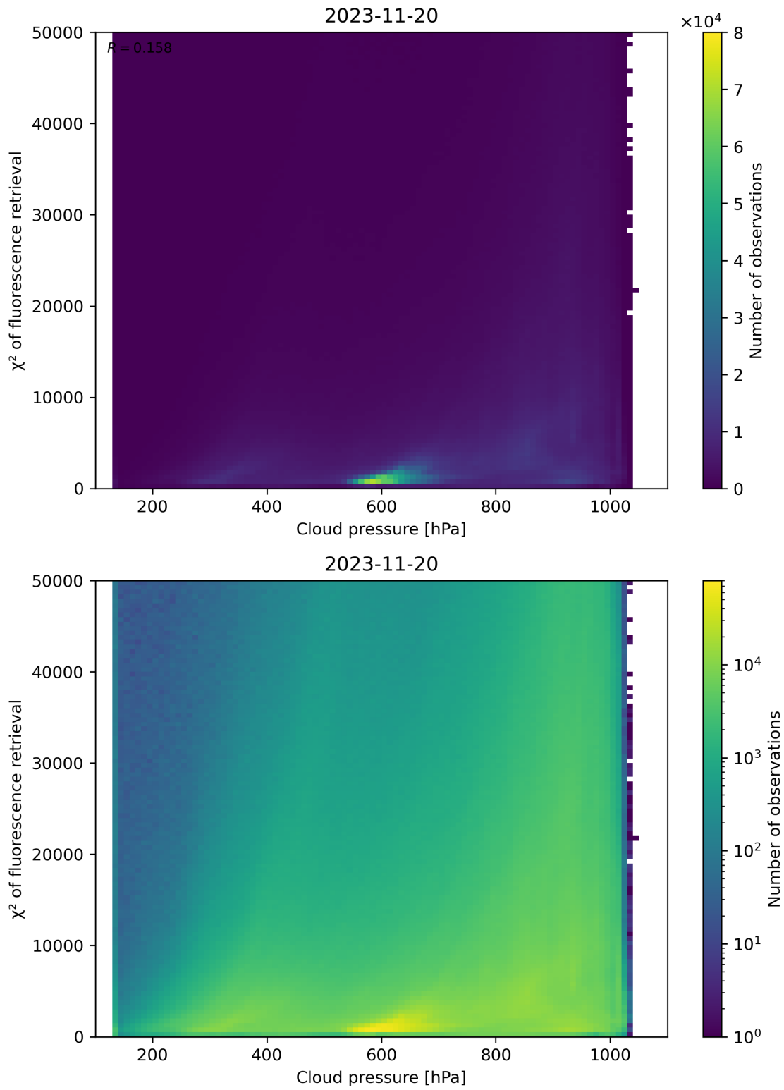
Figure 86: Scatter density plot of “Cloud pressure” against “ \chi^2 of fluorescence retrieval” for 2023-11-19 to 2023-11-21.
