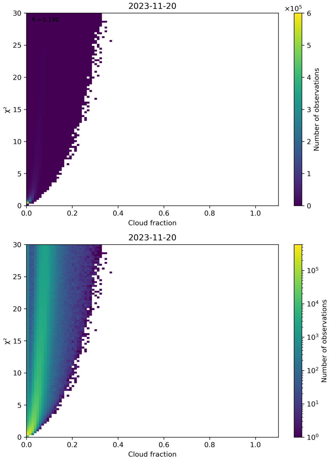
Figure 77: Scatter density plot of “Cloud fraction” against “ \chi^2 ” for 2023-11-19 to 2023-11-21.
