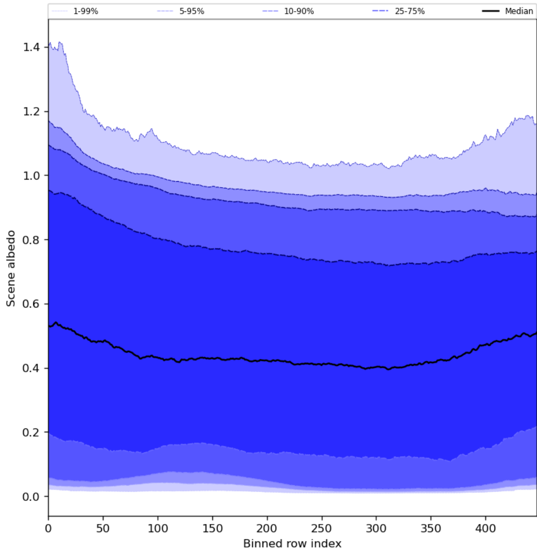
Figure 51: Along track statistics of “Scene albedo” for 2023-11-19 to 2023-11-21
