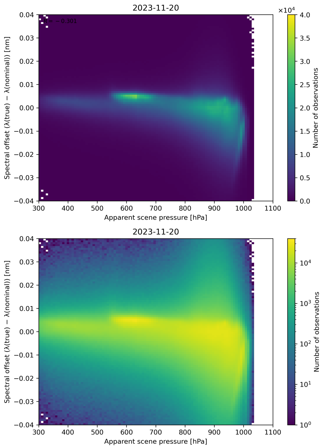
Figure 68: Scatter density plot of “Apparent scene pressure” against “Spectral offset ( \lambda(\text{true}) - \lambda(\text{nominal}) )” for 2023-11-19 to 2023-11-21.
