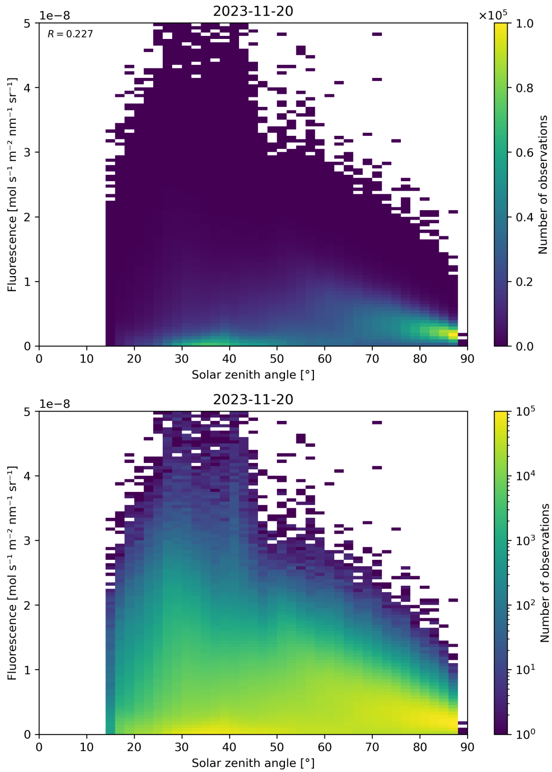
Figure 123: Scatter density plot of “Solar zenith angle” against “Fluorescence” for 2023-11-19 to 2023-11-21.
