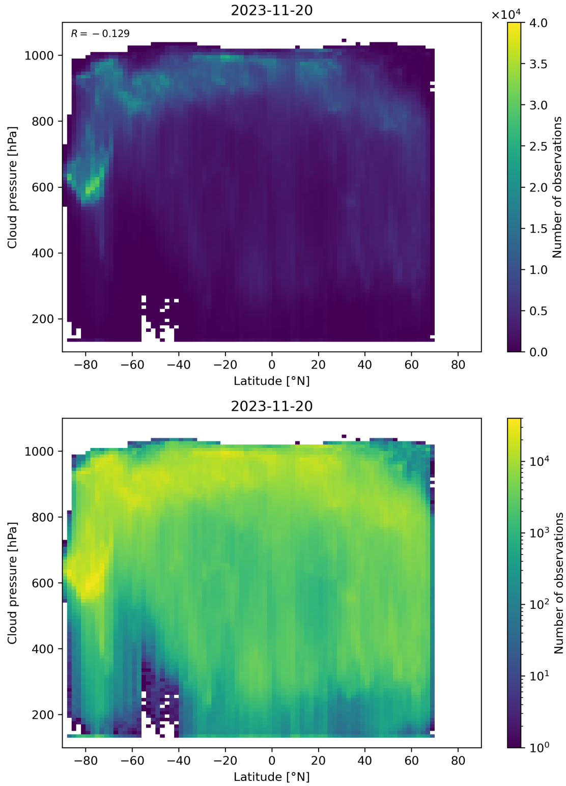
Figure 100: Scatter density plot of “Latitude” against “Cloud pressure” for 2023-11-19 to 2023-11-21.
