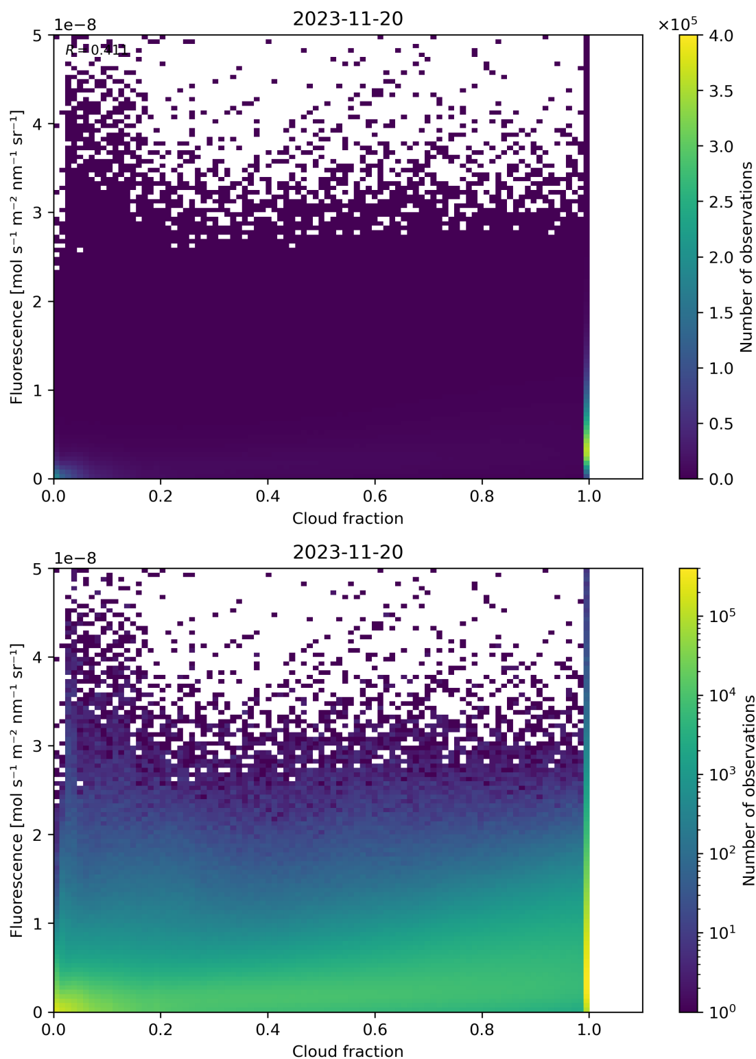
Figure 79: Scatter density plot of “Cloud fraction” against “Fluorescence” for 2023-11-19 to 2023-11-21.
