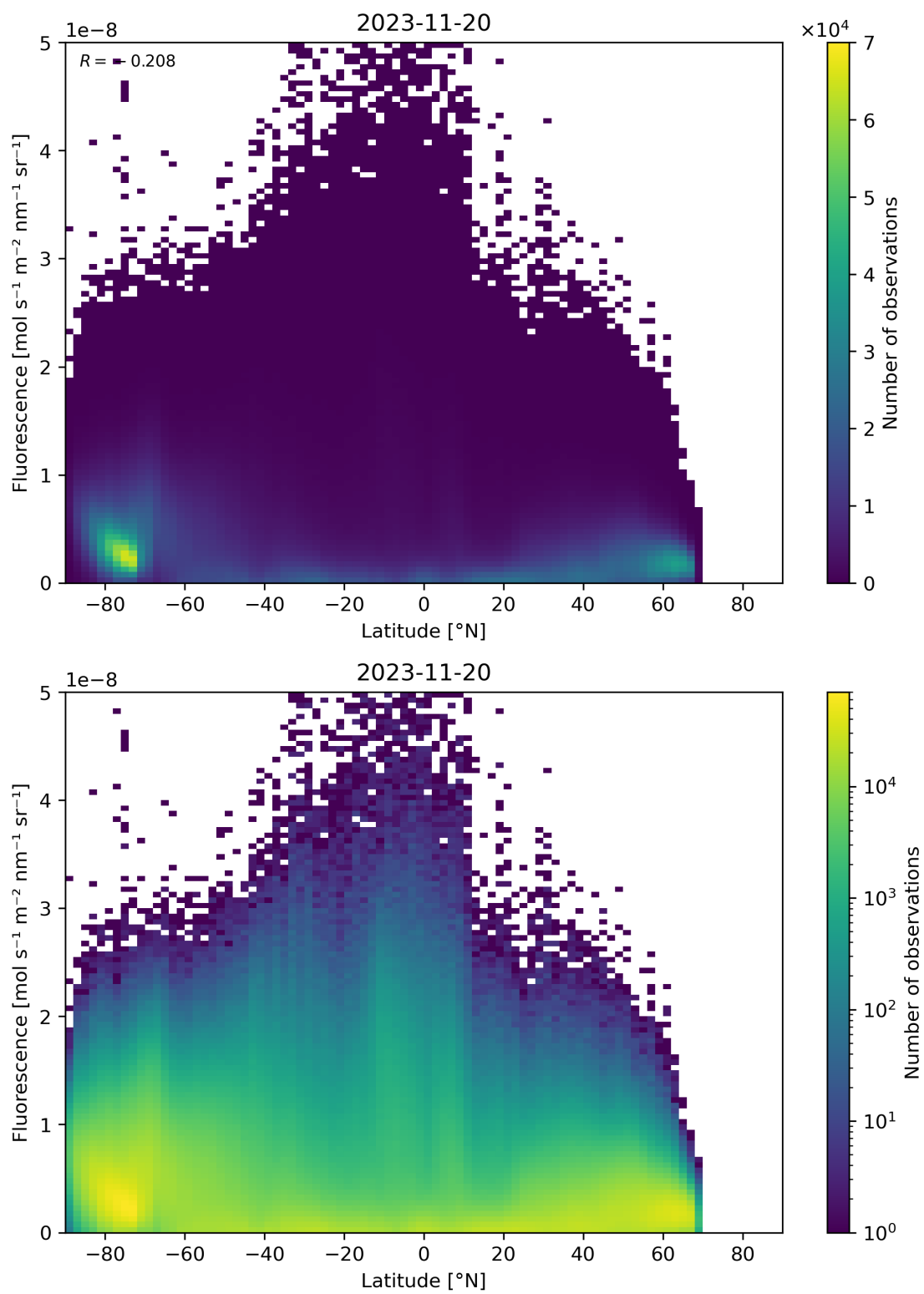
Figure 101: Scatter density plot of “Latitude” against “Fluorescence” for 2023-11-19 to 2023-11-21.
