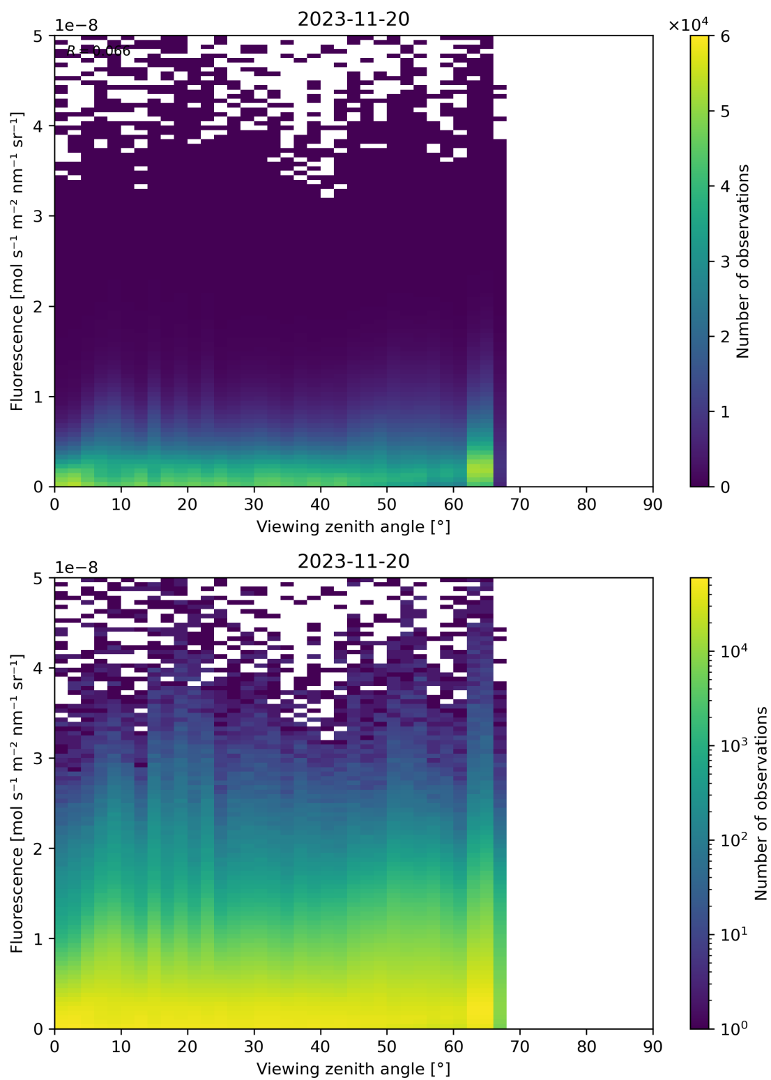
Figure 134: Scatter density plot of “Viewing zenith angle” against “Fluorescence” for 2023-11-19 to 2023-11-21.
