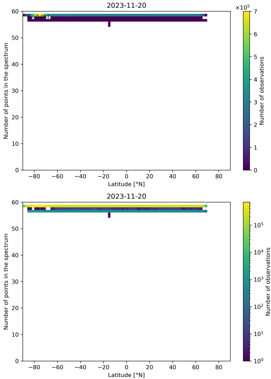
Figure 103: Scatter density plot of “Latitude” against “Number of points in the spectrum” for 2023-11-19 to 2023-11-21.
