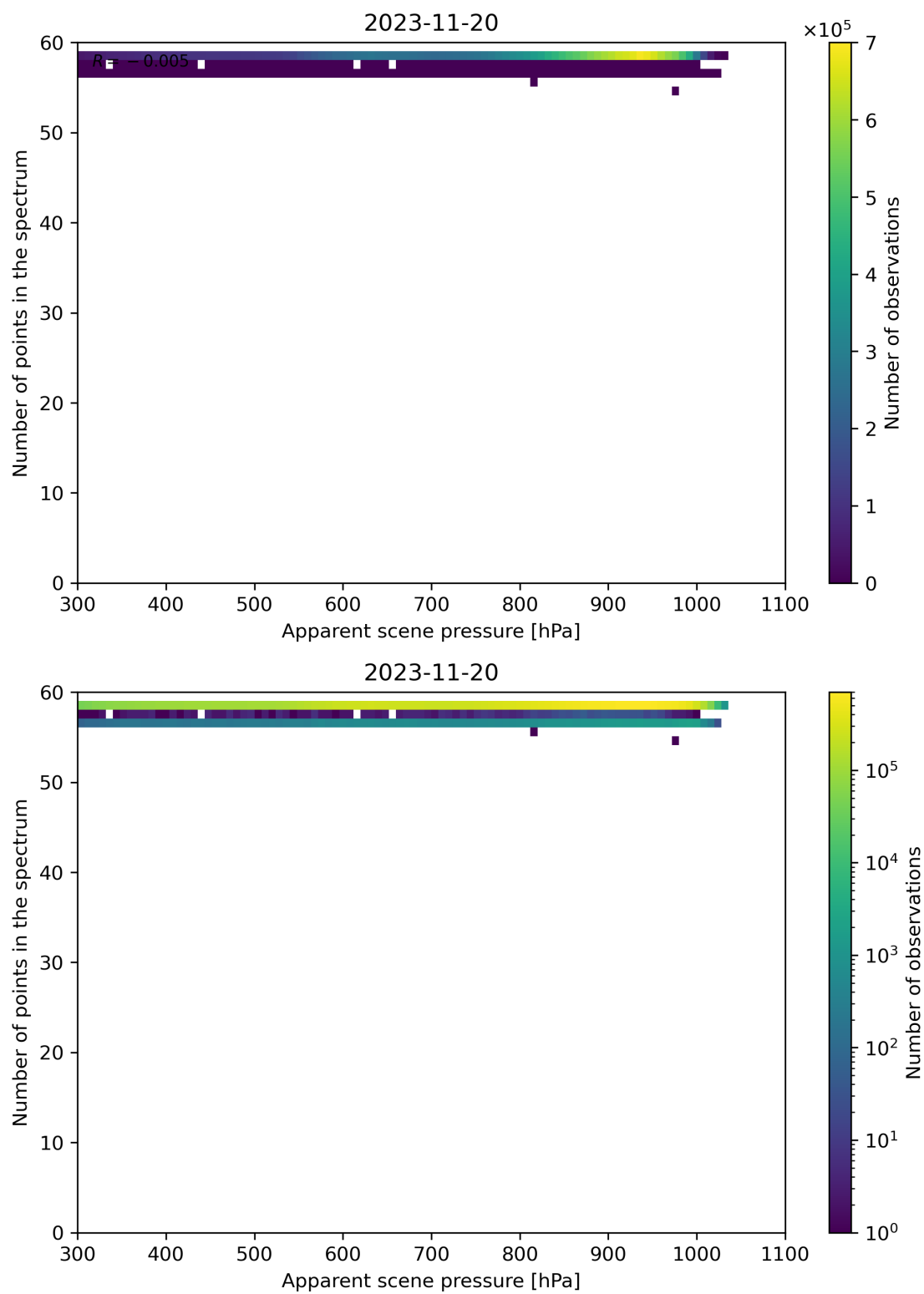
Figure 67: Scatter density plot of “Apparent scene pressure” against “Number of points in the spectrum” for 2023-11-19 to 2023-11-21.
