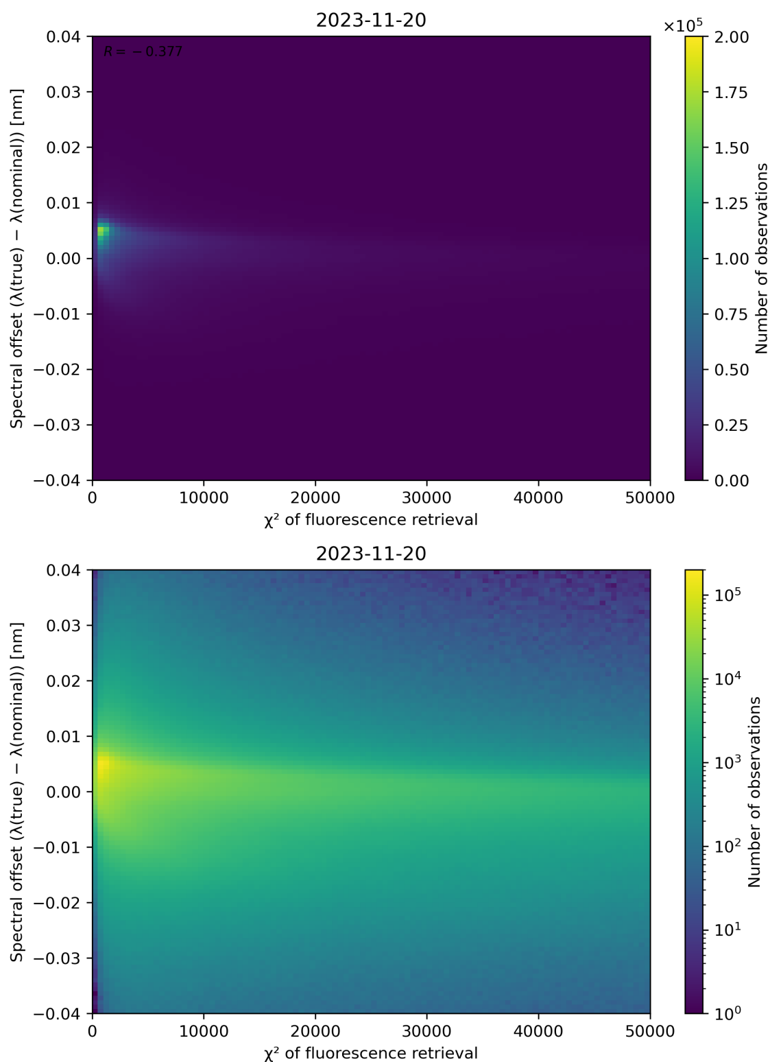
Figure 72: Scatter density plot of " \chi^2 of fluorescence retrieval" against "Spectral offset ( \lambda(\text{true}) - \lambda(\text{nominal})) " for 2023-11-19 to 2023-11-21.
