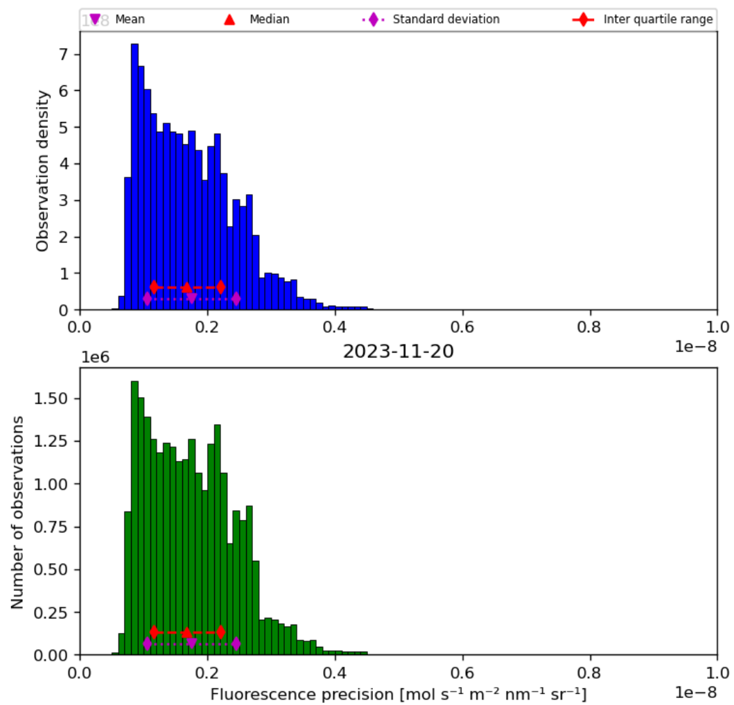
Figure 41: Histogram of “Fluorescence precision” for 2023-11-19 to 2023-11-21
