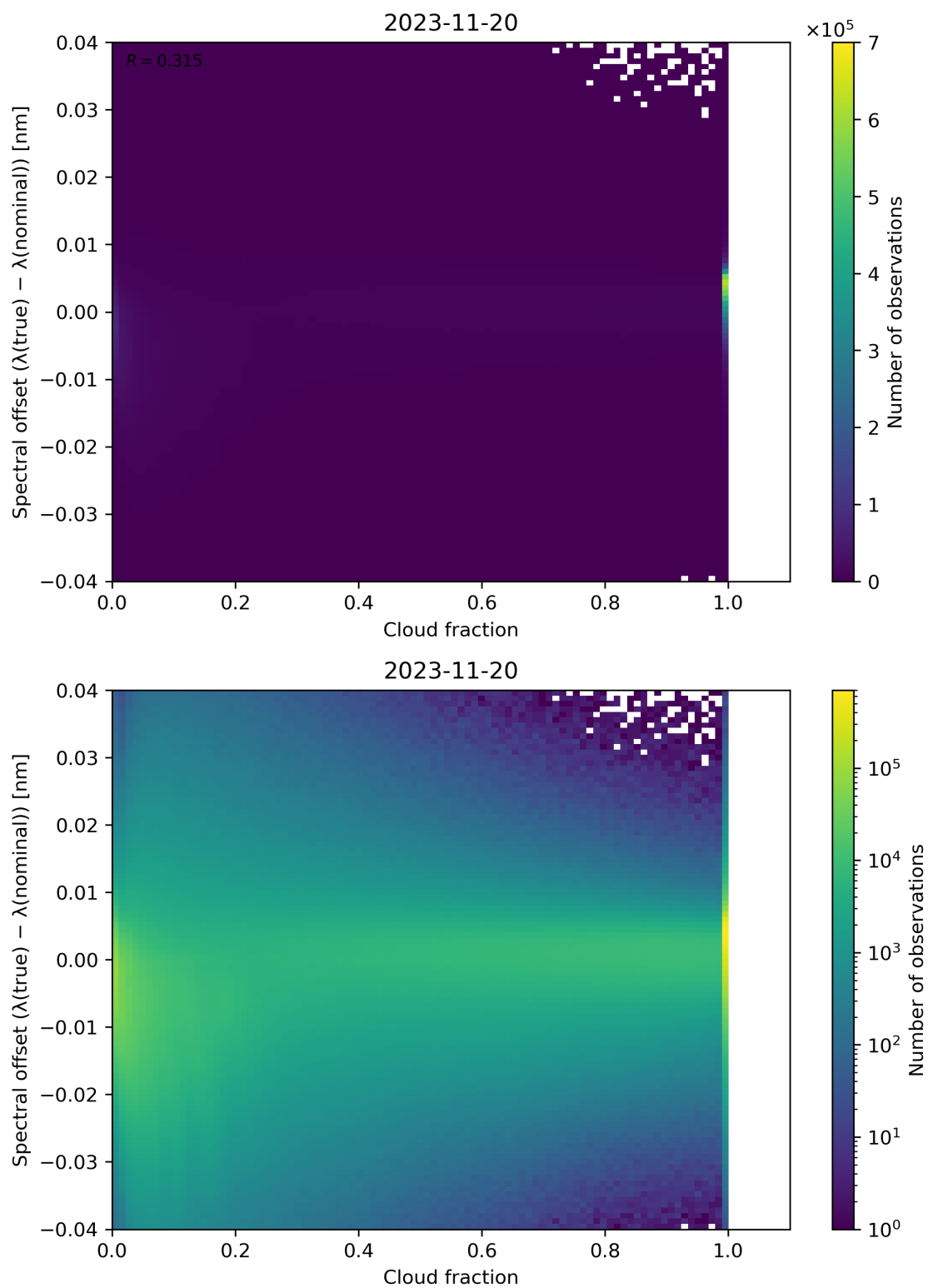
Figure 83: Scatter density plot of “Cloud fraction” against “Spectral offset ( \lambda(\text{true}) - \lambda(\text{nominal}) )” for 2023-11-19 to 2023-11-21.
