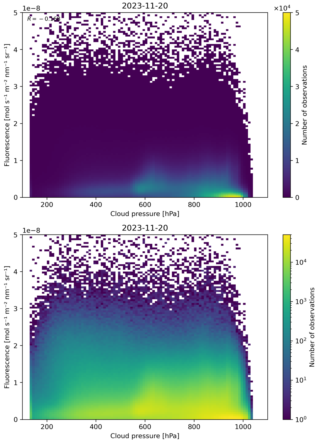
Figure 88: Scatter density plot of “Cloud pressure” against “Fluorescence” for 2023-11-19 to 2023-11-21.
