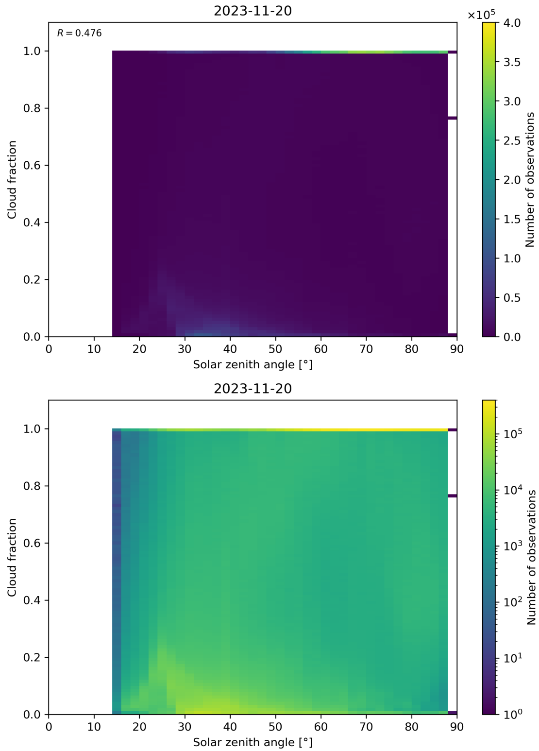
Figure 121: Scatter density plot of “Solar zenith angle” against “Cloud fraction” for 2023-11-19 to 2023-11-21.
