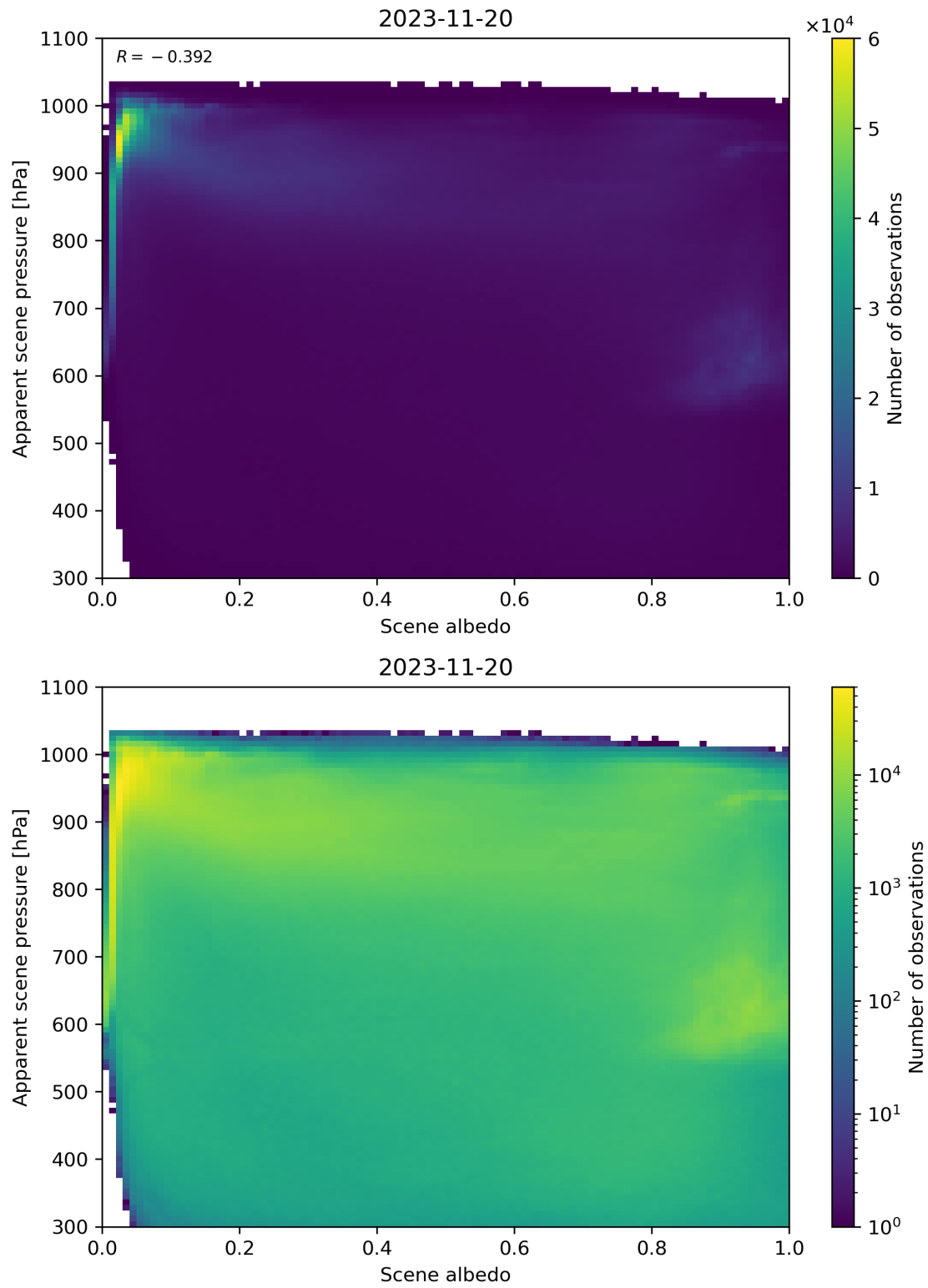
Figure 111: Scatter density plot of “Scene albedo” against “Apparent scene pressure” for 2023-11-19 to 2023-11-21.
