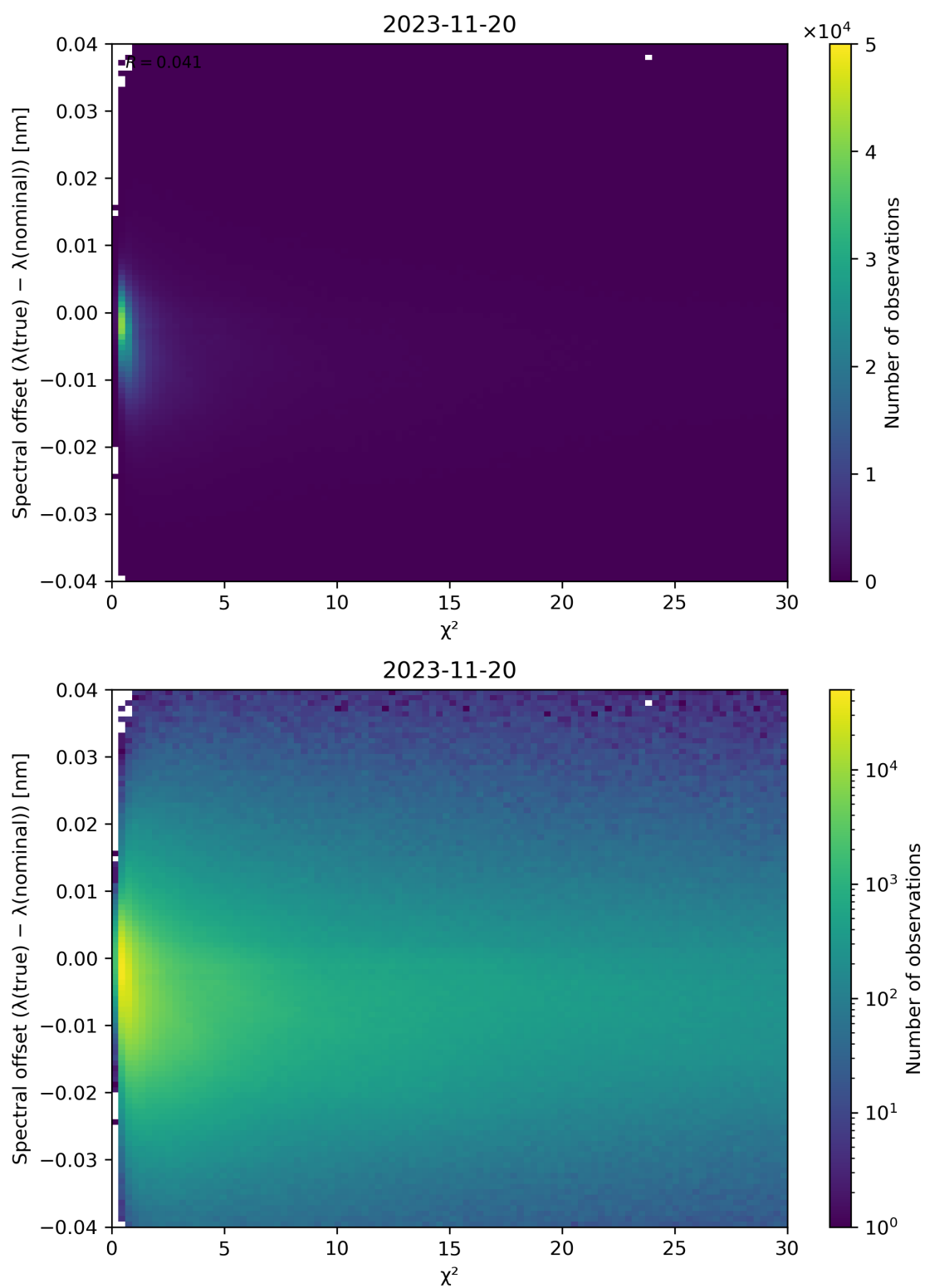
Figure 75: Scatter density plot of “ \chi^2 ” against “Spectral offset ( \lambda(\text{true}) - \lambda(\text{nominal}) )” for 2023-11-19 to 2023-11-21.
