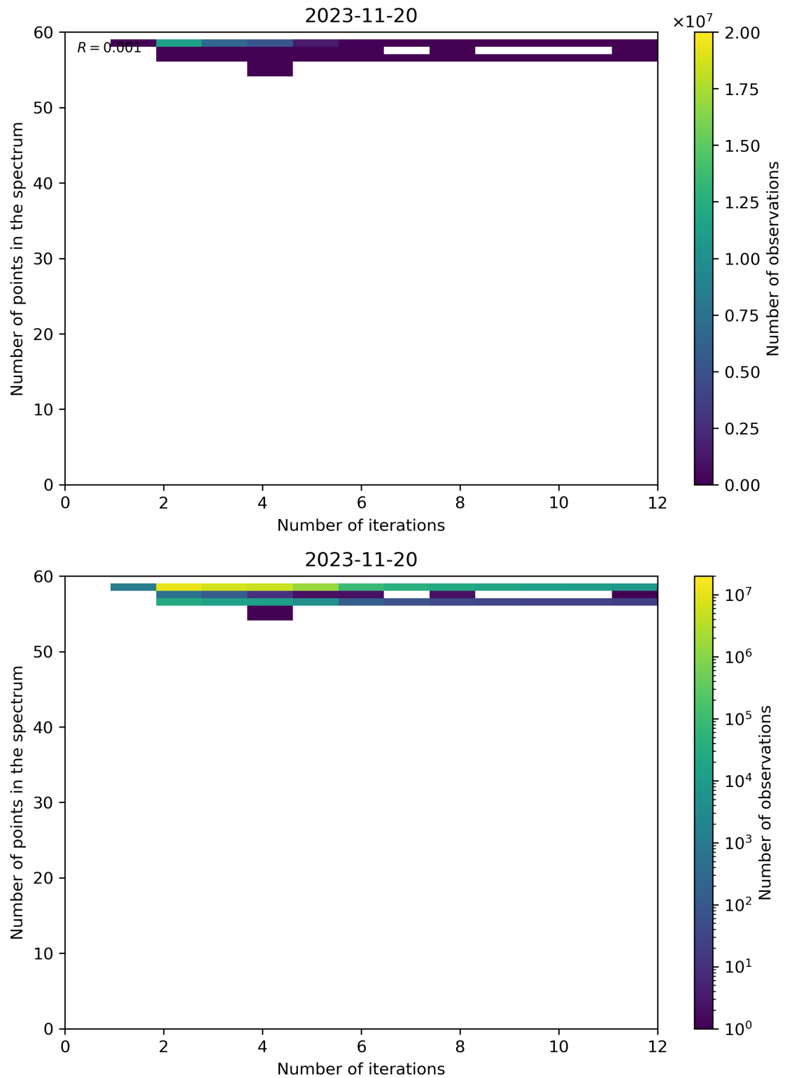
Figure 108: Scatter density plot of “Number of iterations” against “Number of points in the spectrum” for 2023-11-19 to 2023-11-21.
