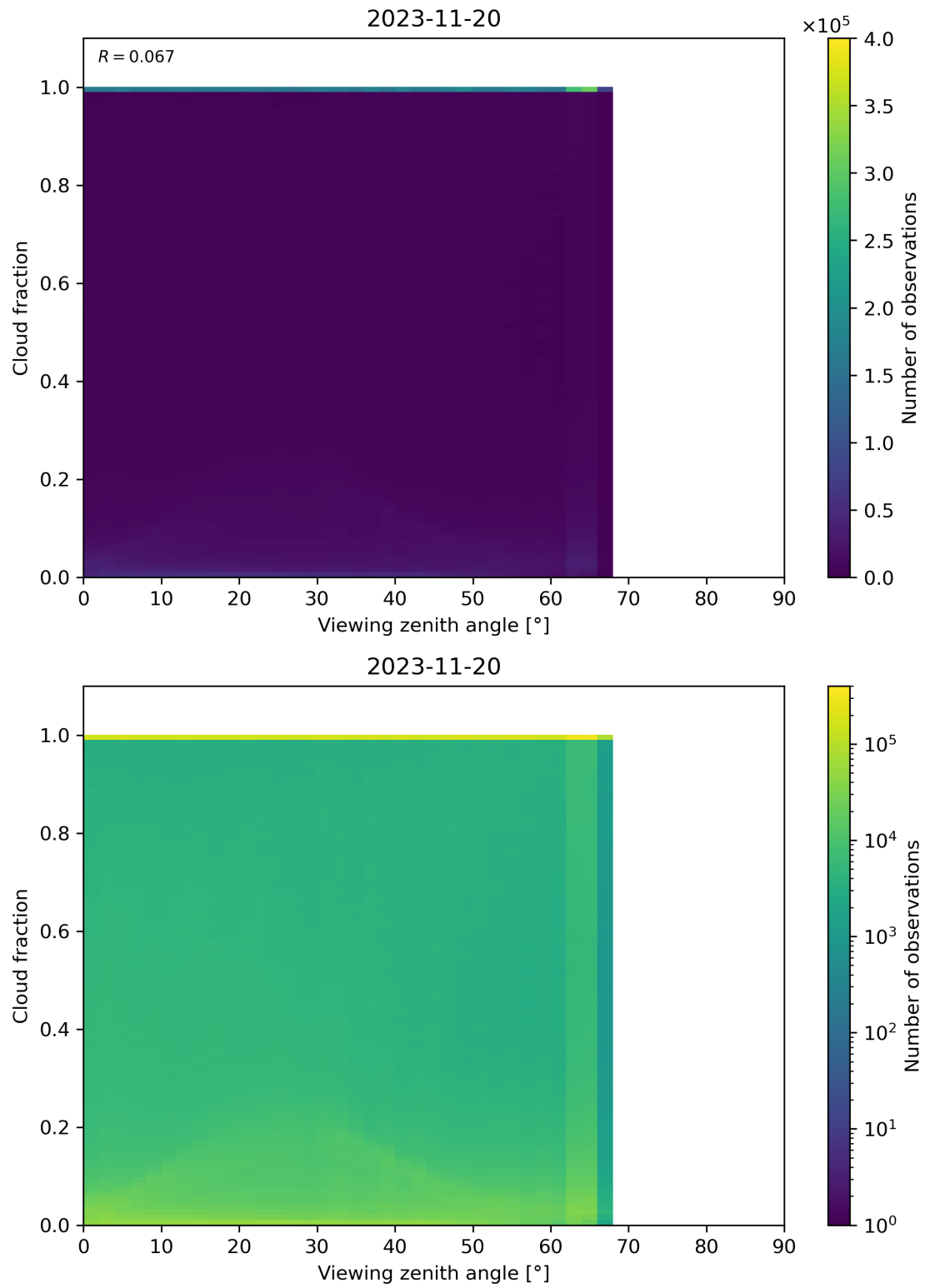
Figure 132: Scatter density plot of “Viewing zenith angle” against “Cloud fraction” for 2023-11-19 to 2023-11-21.
