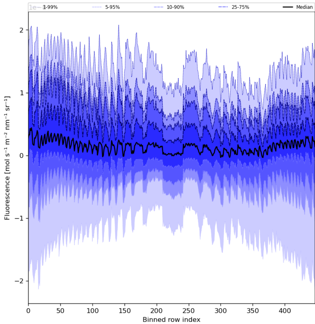
Figure 57: Along track statistics of “Fluorescence” for 2023-11-19 to 2023-11-21
