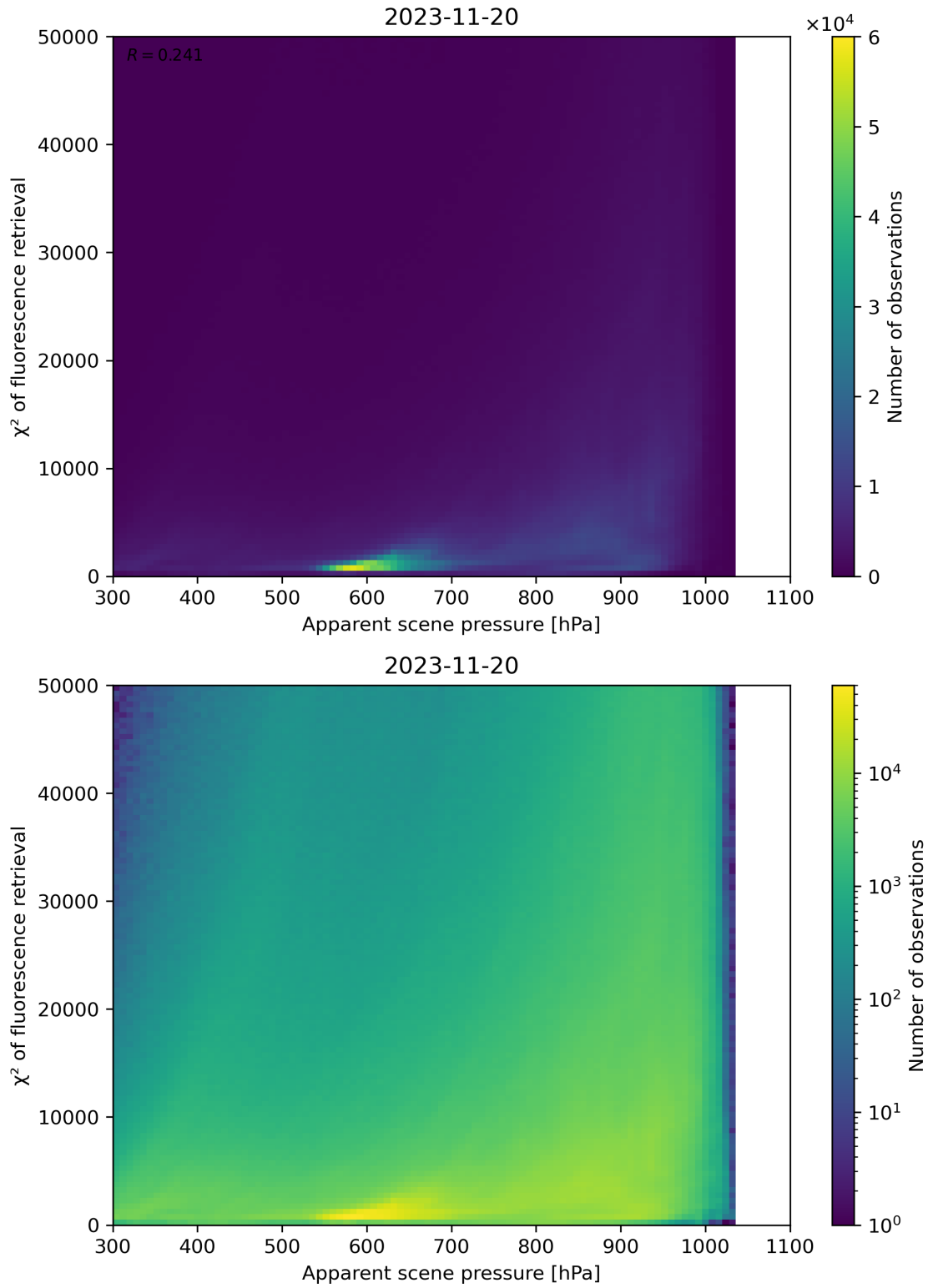
Figure 64: Scatter density plot of “Apparent scene pressure” against “ \chi^2 of fluorescence retrieval” for 2023-11-19 to 2023-11-21.
