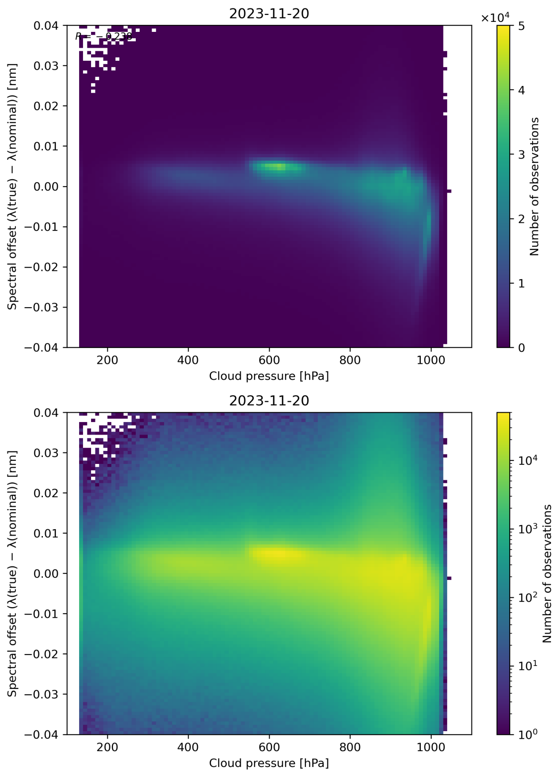
Figure 92: Scatter density plot of “Cloud pressure” against “Spectral offset ( \lambda(\text{true}) - \lambda(\text{nominal}) )” for 2023-11-19 to 2023-11-21.
