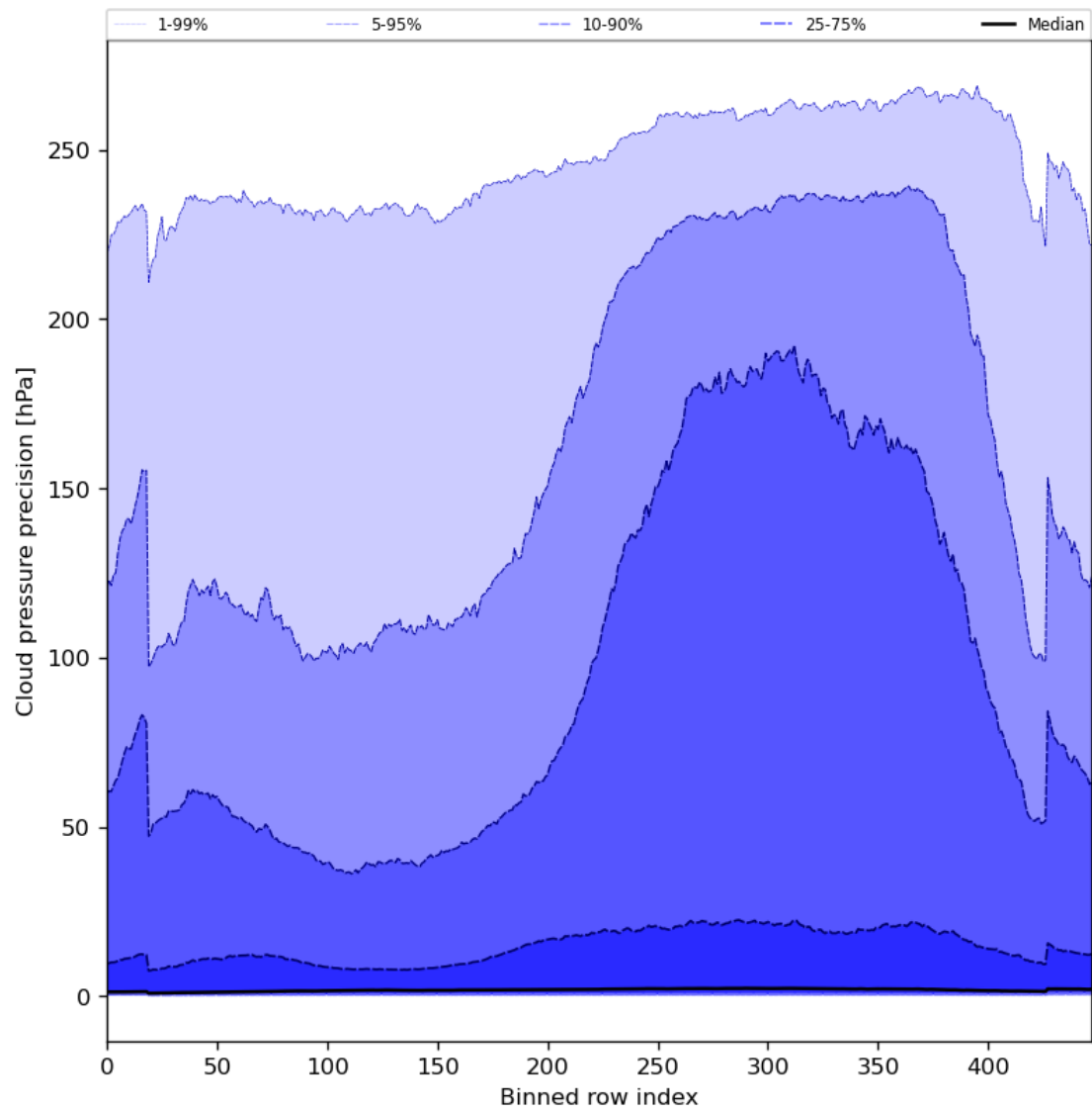
Figure 48: Along track statistics of “Cloud pressure precision” for 2023-11-19 to 2023-11-21
