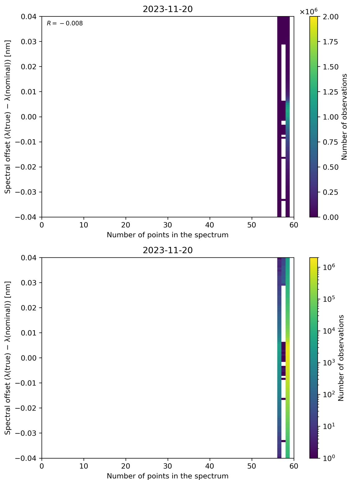
Figure 110: Scatter density plot of “Number of points in the spectrum” against “Spectral offset ( \lambda(\text{true}) - \lambda(\text{nominal}) )” for 2023-11-19 to 2023-11-21.
