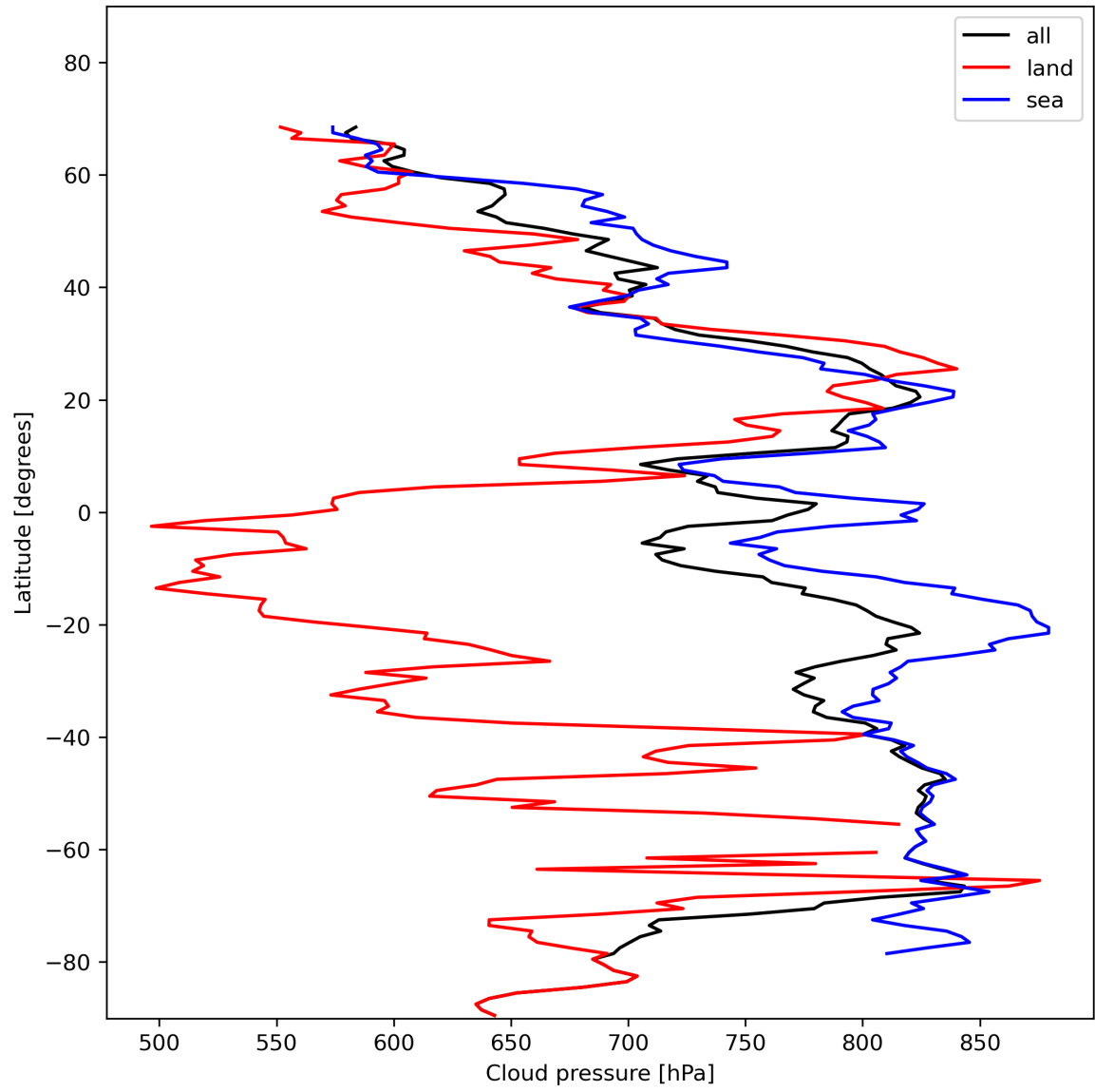
Figure 13: Zonal average of “Cloud pressure” for 2023-11-19 to 2023-11-21.
