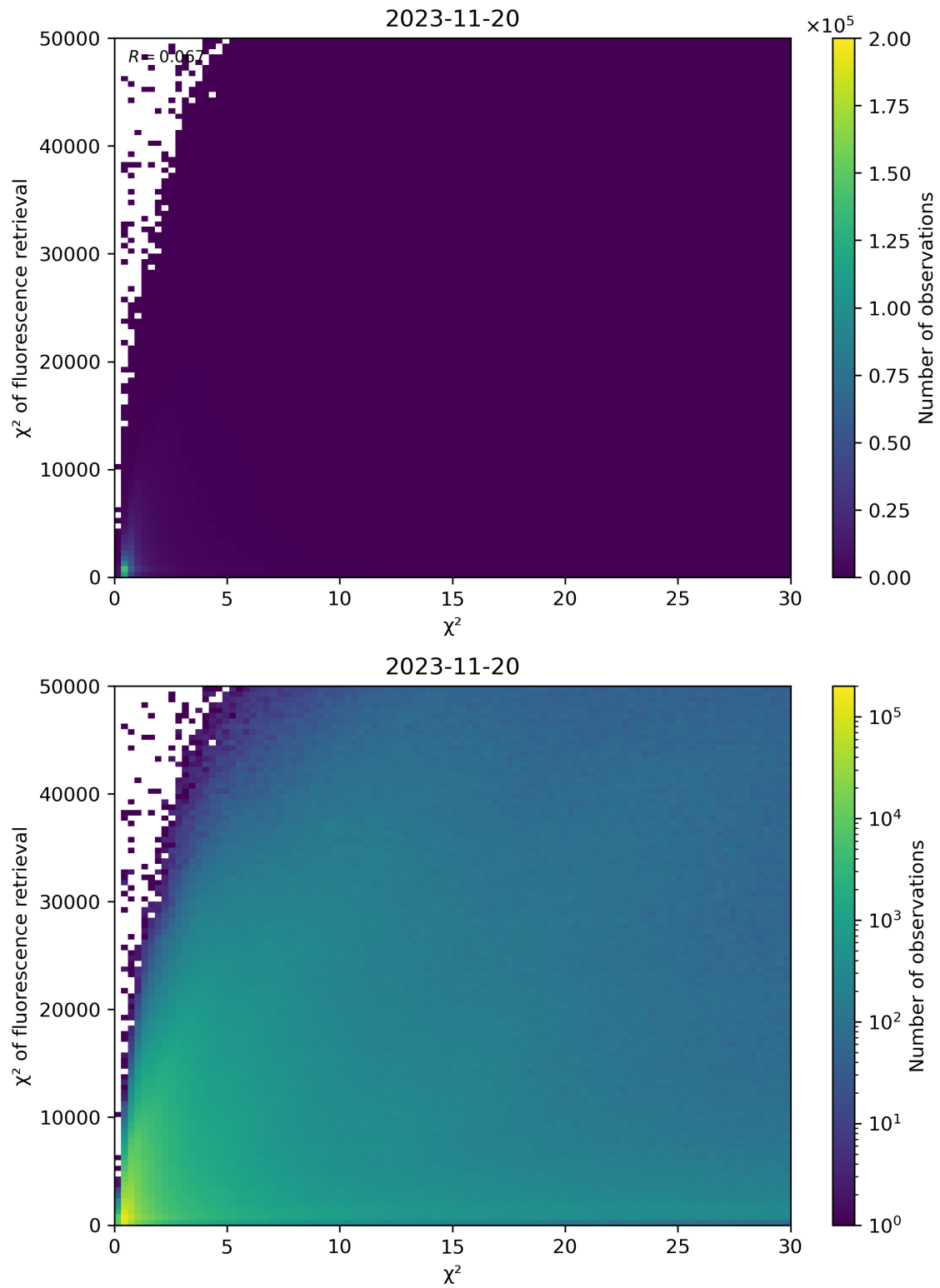
Figure 69: Scatter density plot of “ \chi^2 ” against “ \chi^2 of fluorescence retrieval” for 2023-11-19 to 2023-11-21.
