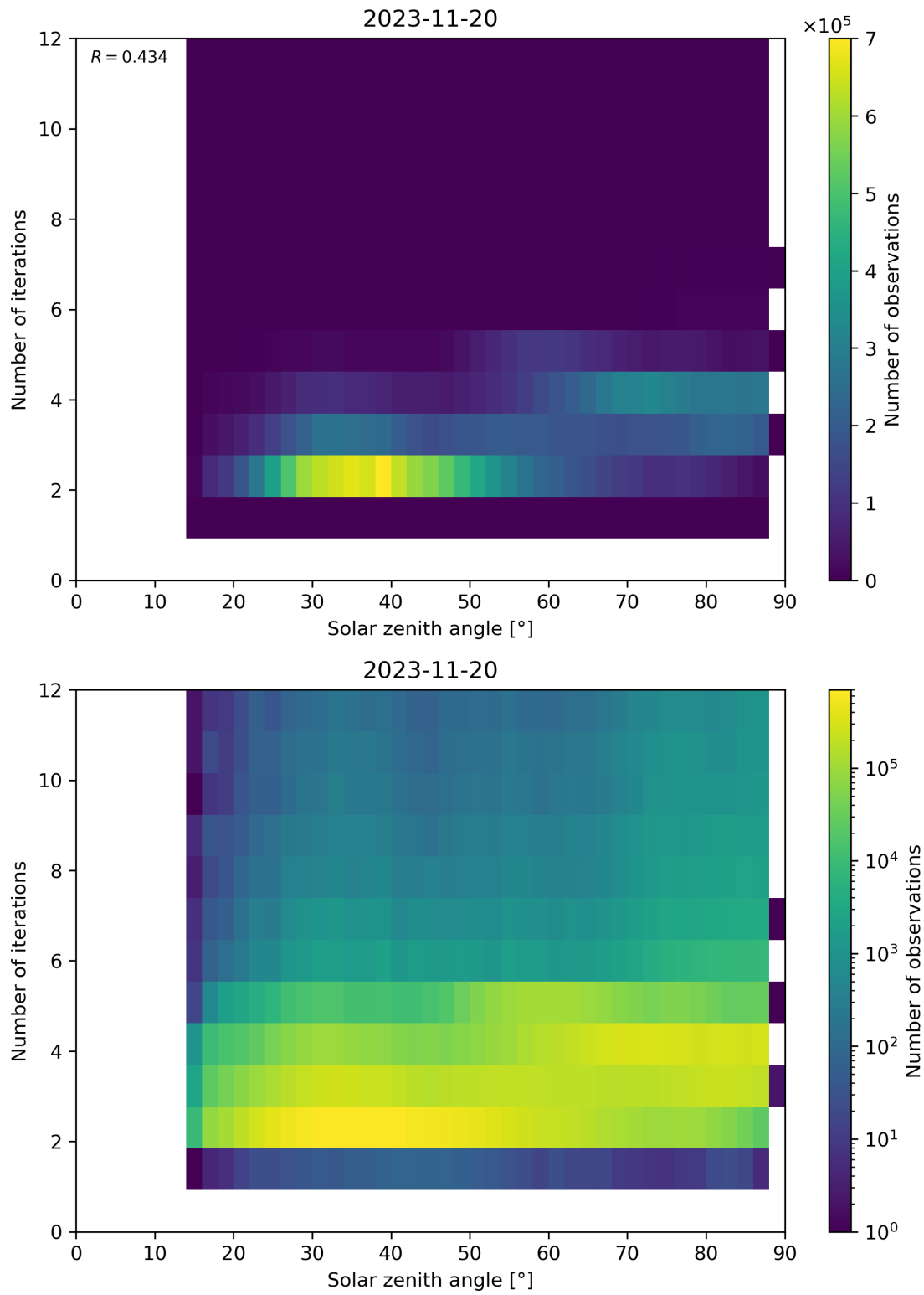
Figure 125: Scatter density plot of “Solar zenith angle” against “Number of iterations” for 2023-11-19 to 2023-11-21.
