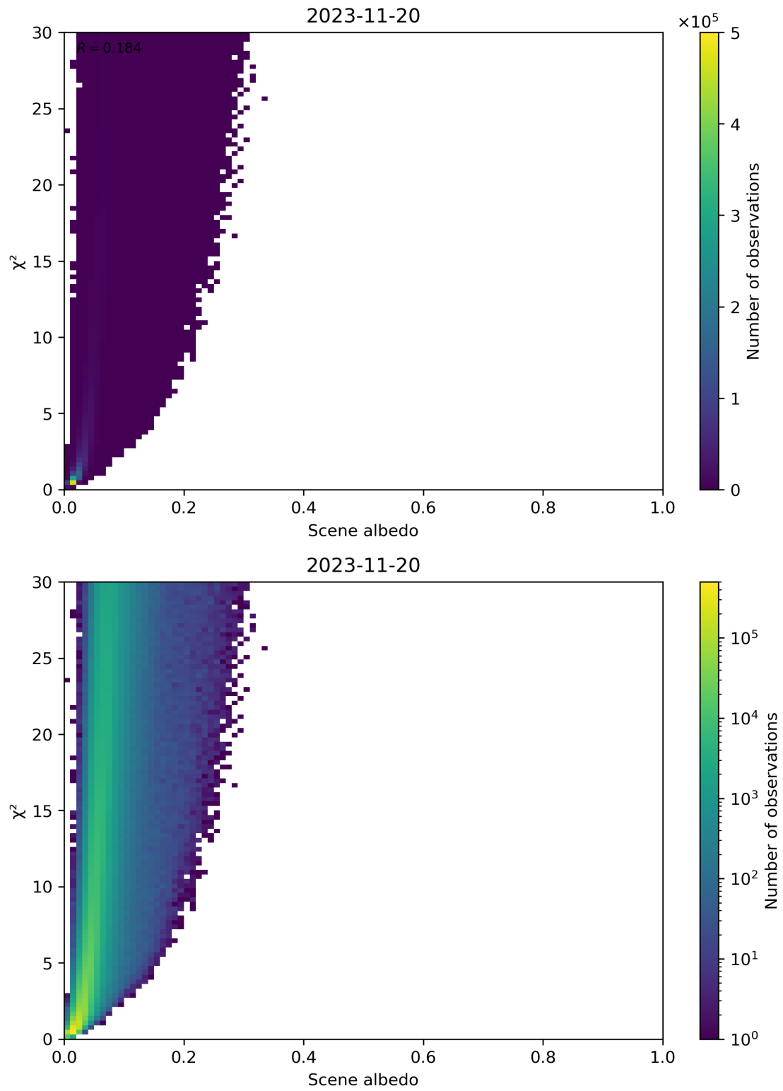
Figure 112: Scatter density plot of “Scene albedo” against “ \chi^2 ” for 2023-11-19 to 2023-11-21.
