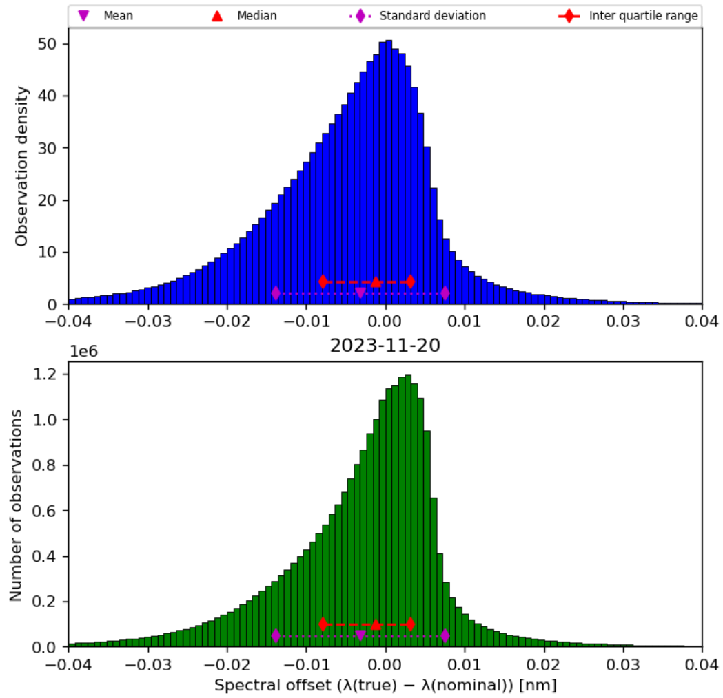
Figure 45: Histogram of “Spectral offset ( \lambda(\text{true}) - \lambda(\text{nominal}) )” for 2023-11-19 to 2023-11-21
