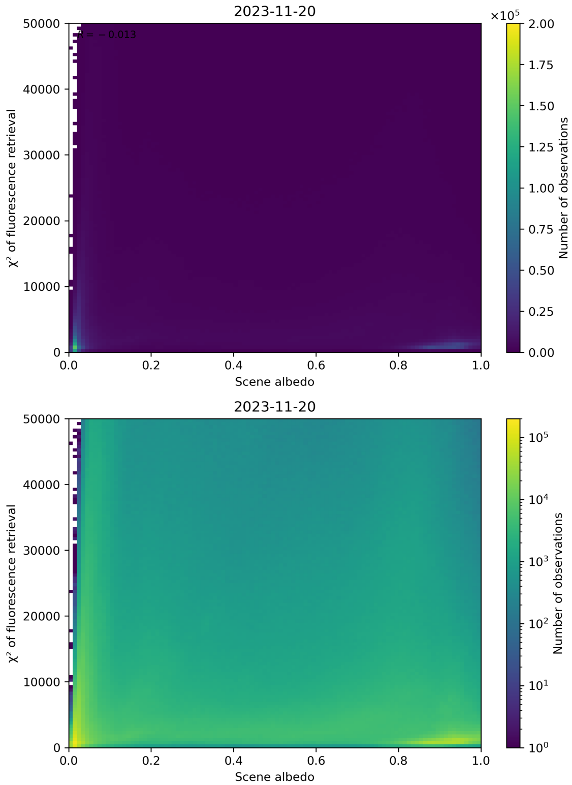
Figure 113: Scatter density plot of “Scene albedo” against “ \chi^2 of fluorescence retrieval” for 2023-11-19 to 2023-11-21.
