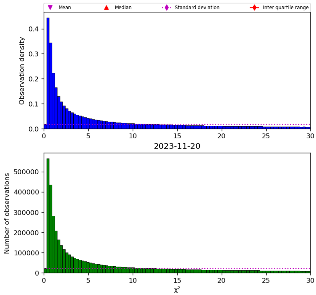
Figure 38: Histogram of “ \chi^2 ” for 2023-11-19 to 2023-11-21
