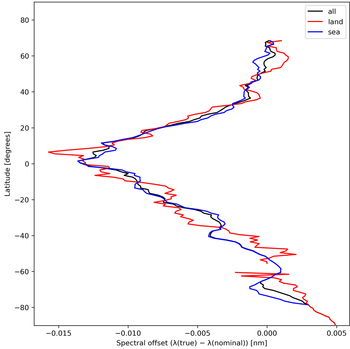
Figure 28: Zonal average of “Spectral offset ( \lambda(\text{true}) - \lambda(\text{nominal}) )” for 2023-11-19 to 2023-11-21.
