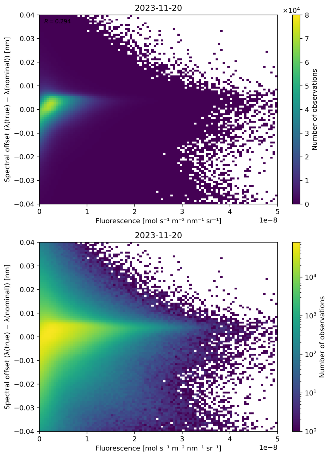
Figure 95: Scatter density plot of “Fluorescence” against “Spectral offset ( \lambda(\text{true}) - \lambda(\text{nominal}) )” for 2023-11-19 to 2023-11-21.
