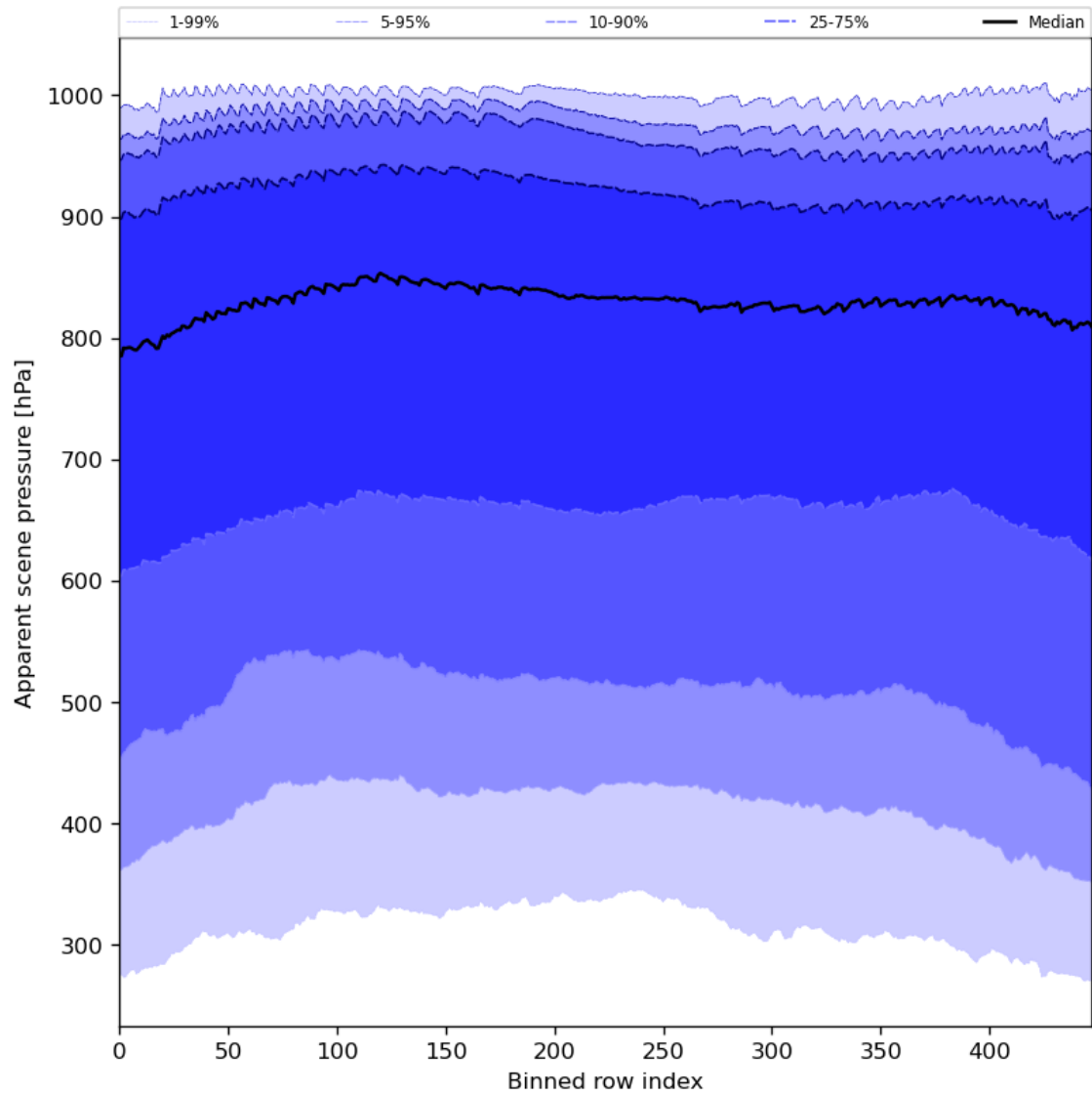
Figure 53: Along track statistics of “Apparent scene pressure” for 2023-11-19 to 2023-11-21
