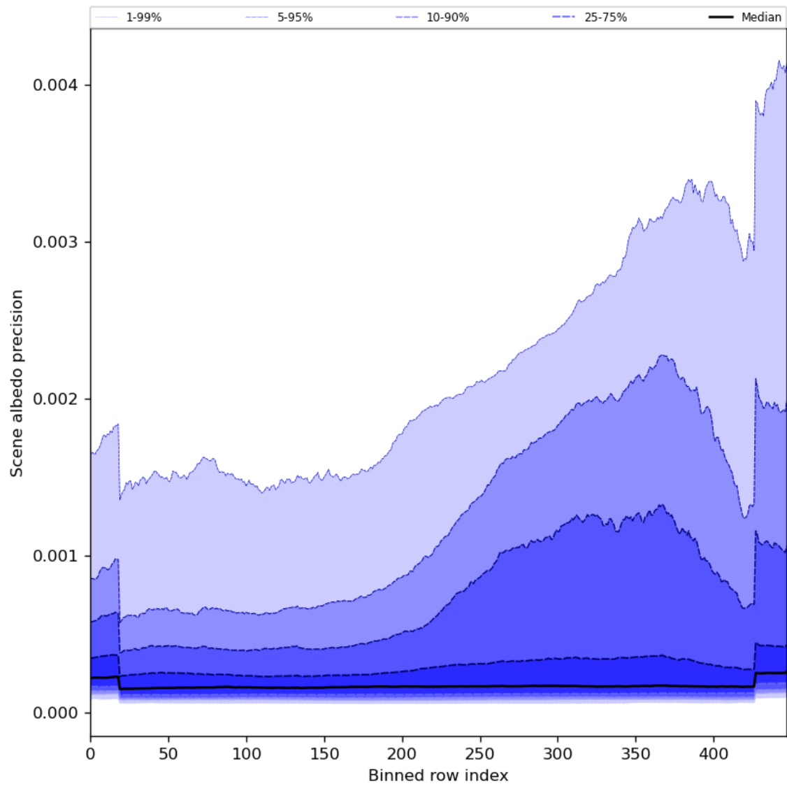
Figure 52: Along track statistics of “Scene albedo precision” for 2023-11-19 to 2023-11-21
