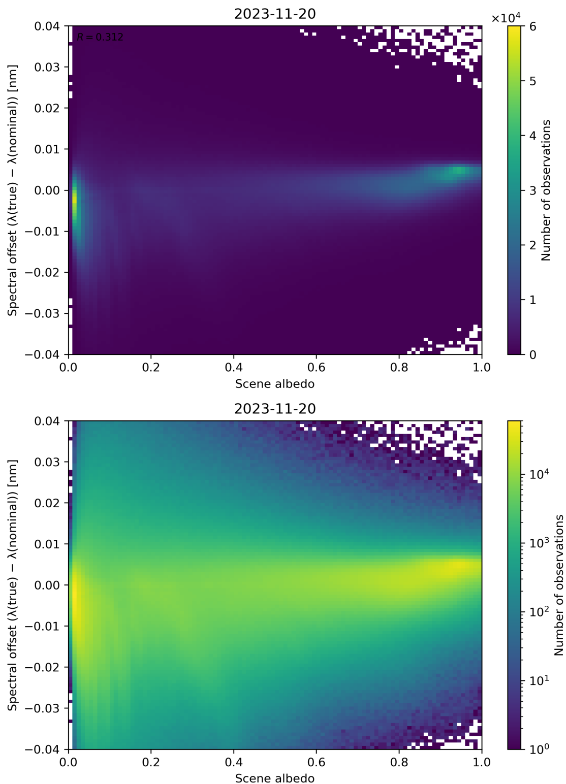
Figure 117: Scatter density plot of “Scene albedo” against “Spectral offset ( \lambda(\text{true}) - \lambda(\text{nominal}) )” for 2023-11-19 to 2023-11-21.
