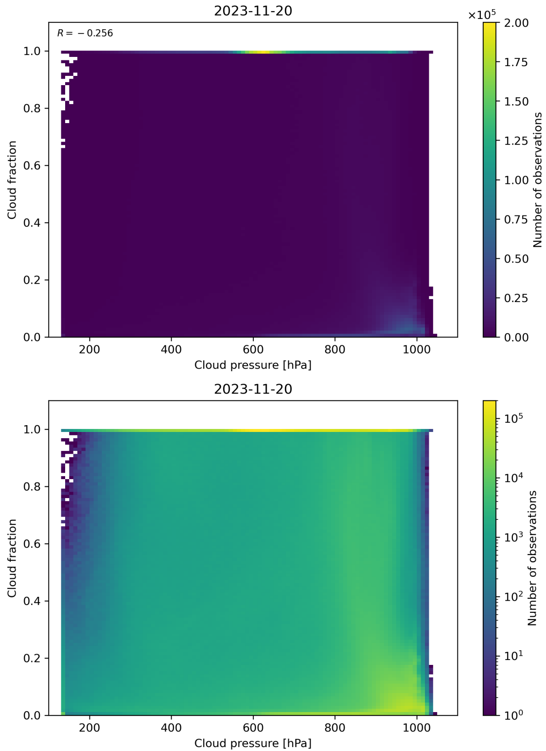
Figure 87: Scatter density plot of “Cloud pressure” against “Cloud fraction” for 2023-11-19 to 2023-11-21.
