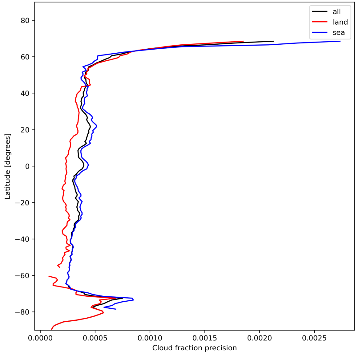
Figure 16: Zonal average of “Cloud fraction precision” for 2023-11-19 to 2023-11-21.
