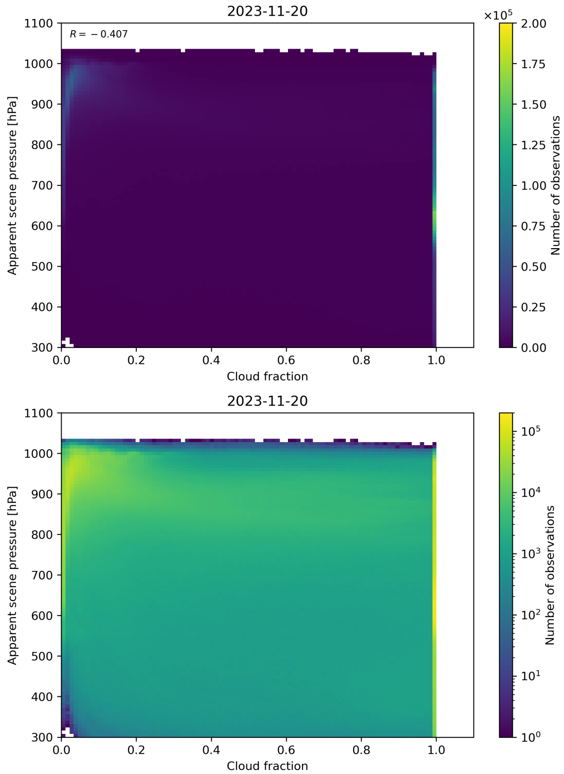
Figure 76: Scatter density plot of “Cloud fraction” against “Apparent scene pressure” for 2023-11-19 to 2023-11-21.
