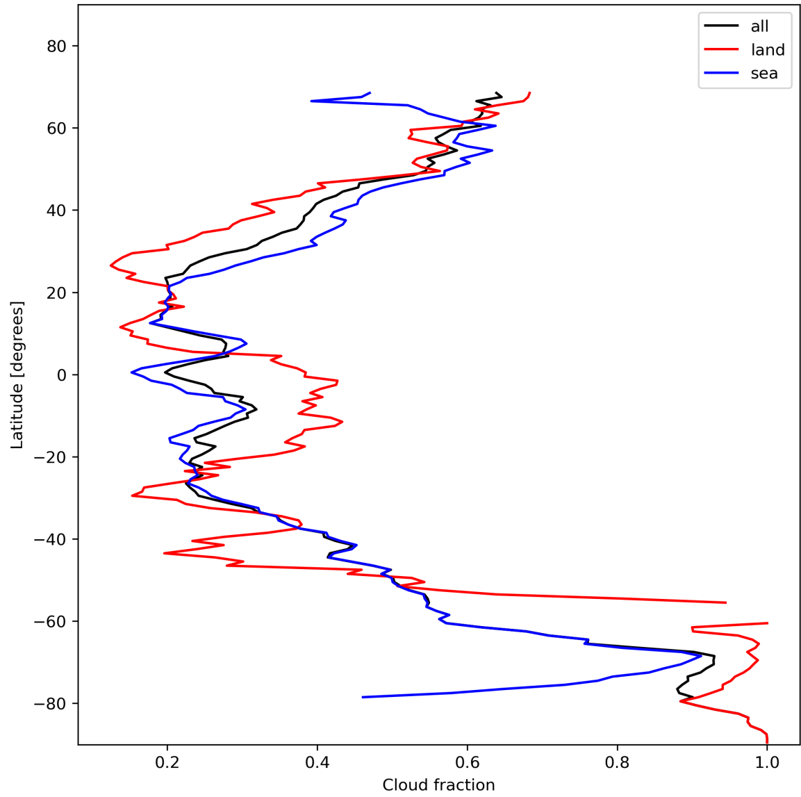
Figure 15: Zonal average of “Cloud fraction” for 2023-11-19 to 2023-11-21.
