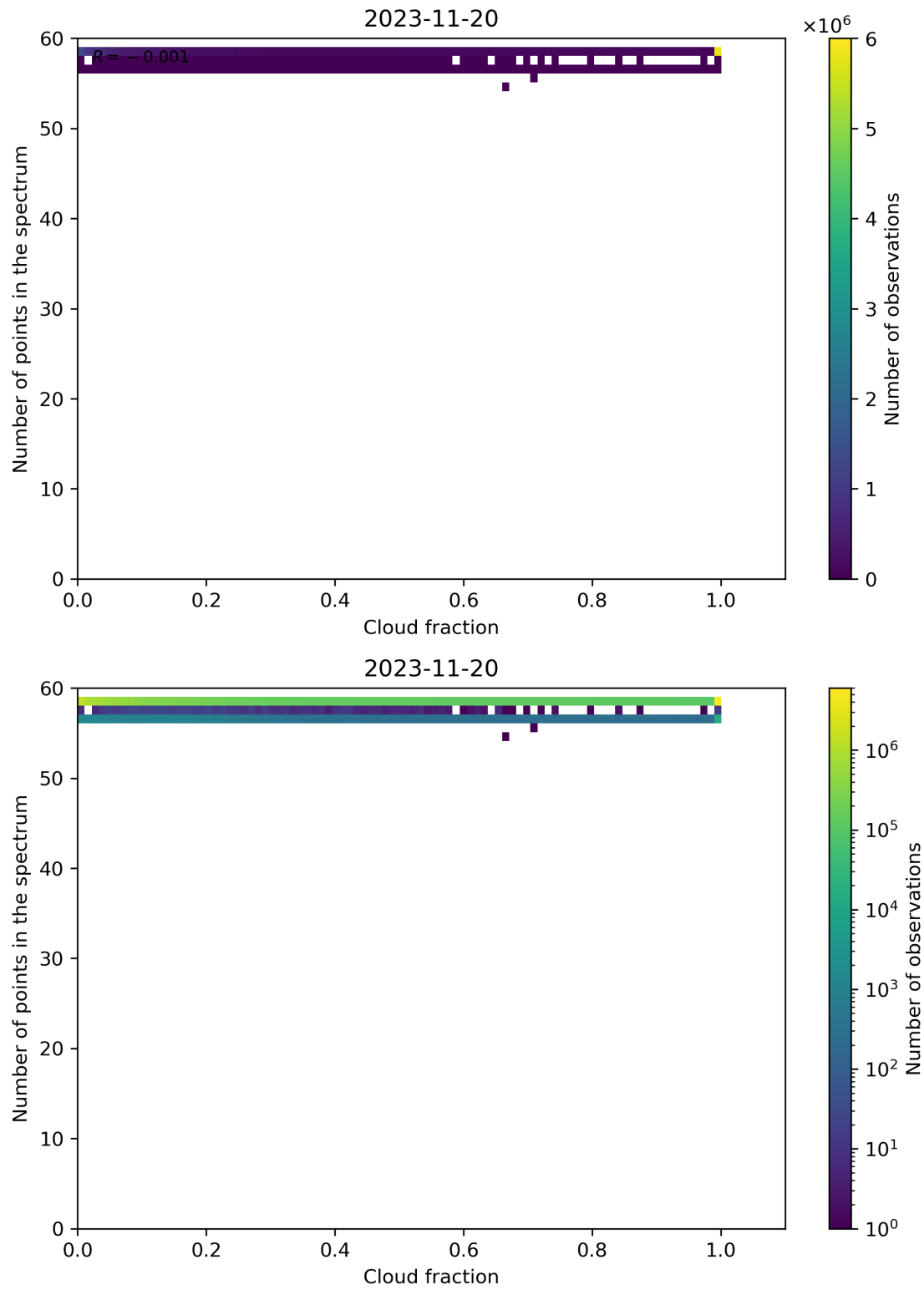
Figure 81: Scatter density plot of “Cloud fraction” against “Number of points in the spectrum” for 2023-11-19 to 2023-11-21.
