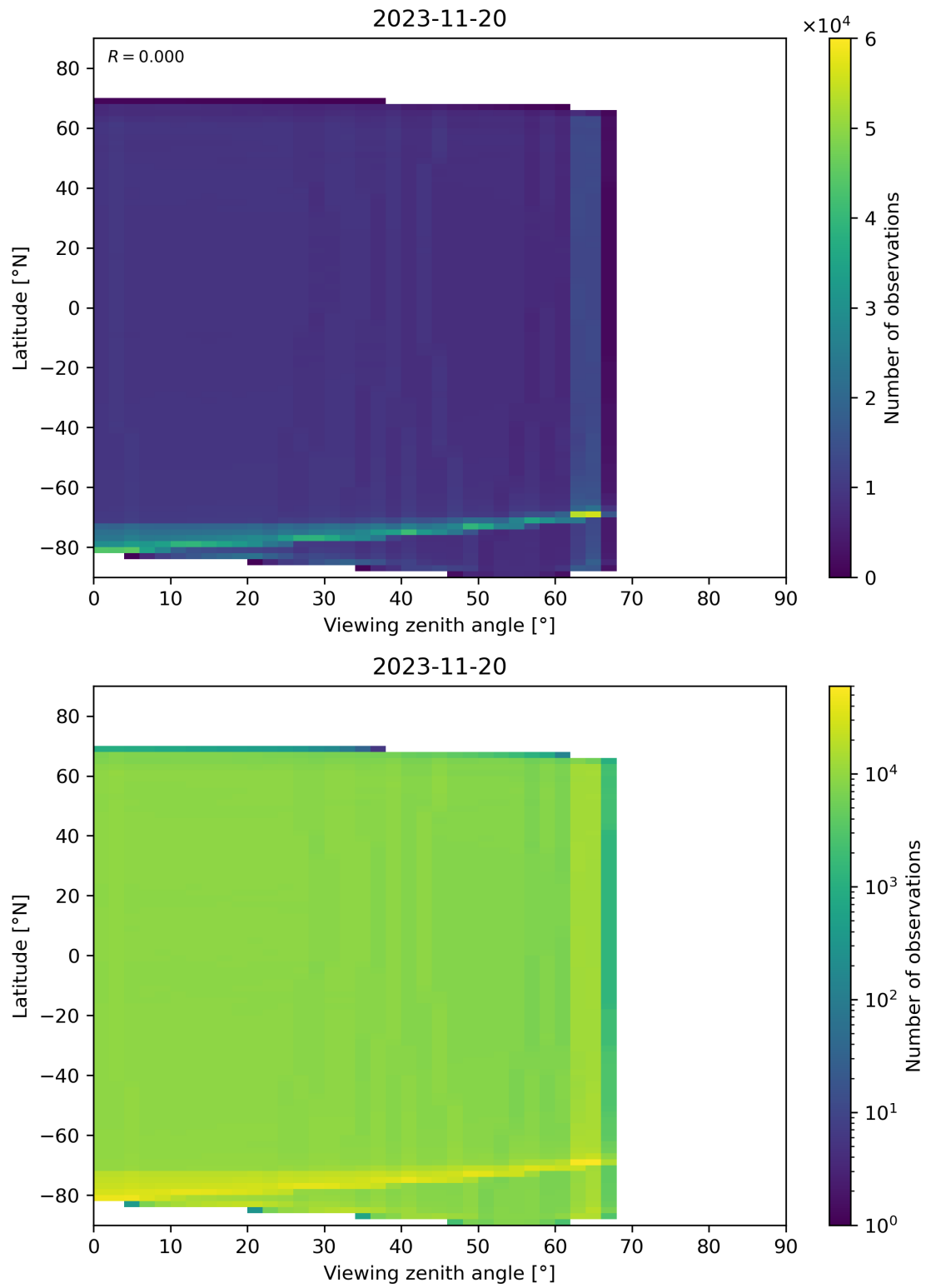
Figure 135: Scatter density plot of “Viewing zenith angle” against “Latitude” for 2023-11-19 to 2023-11-21.
