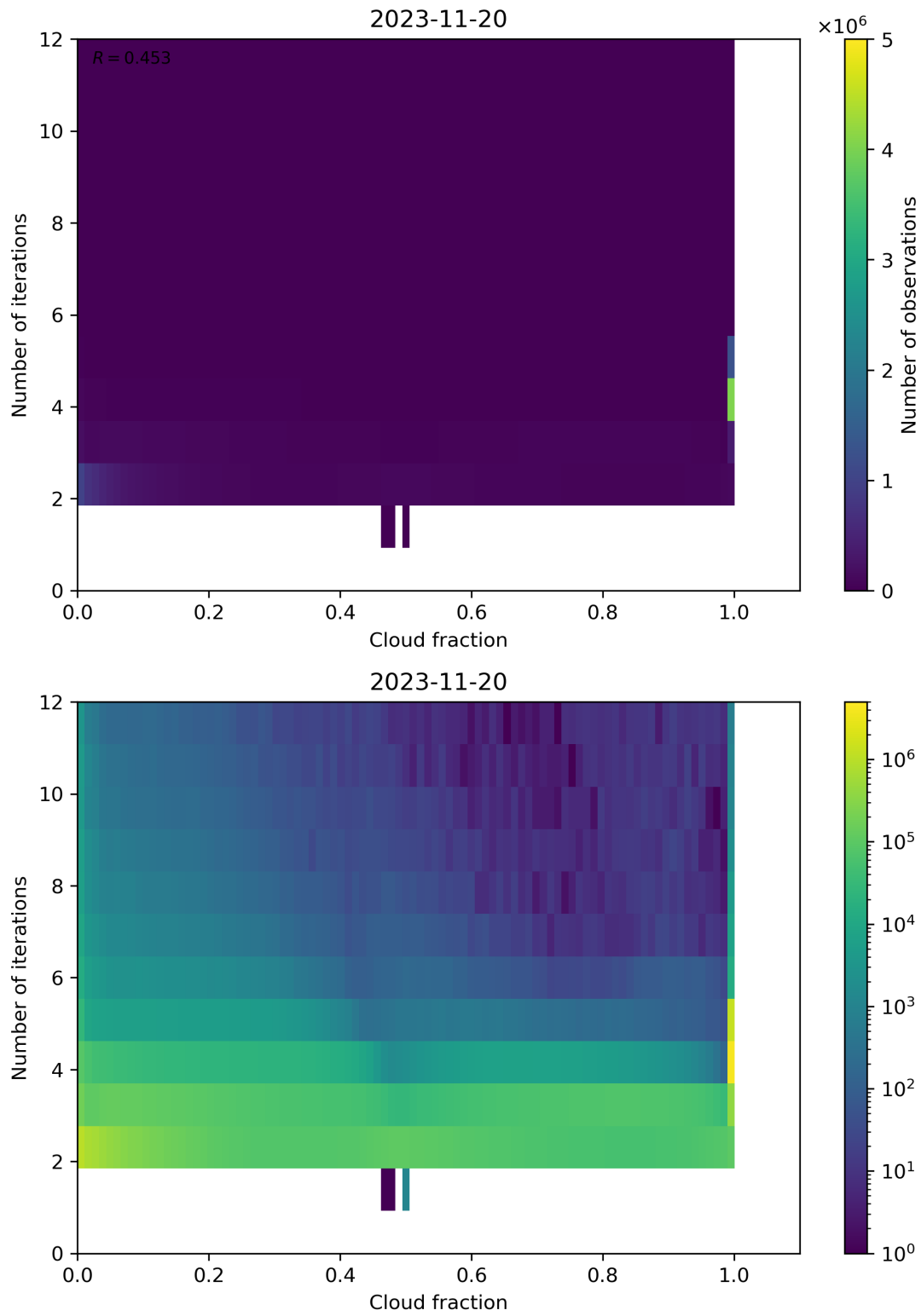
Figure 80: Scatter density plot of “Cloud fraction” against “Number of iterations” for 2023-11-19 to 2023-11-21.
