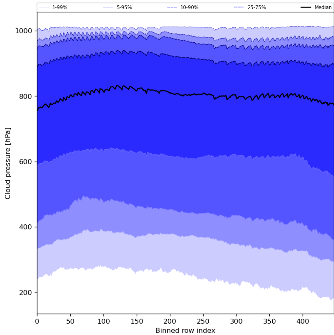
Figure 47: Along track statistics of "Cloud pressure" for 2023-11-19 to 2023-11-21
