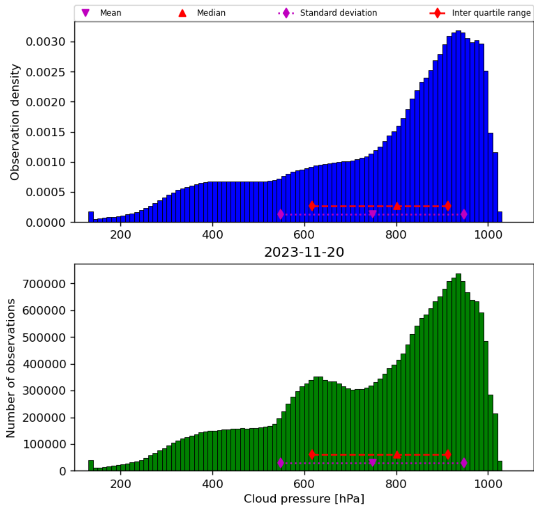
Figure 30: Histogram of “Cloud pressure” for 2023-11-19 to 2023-11-21
