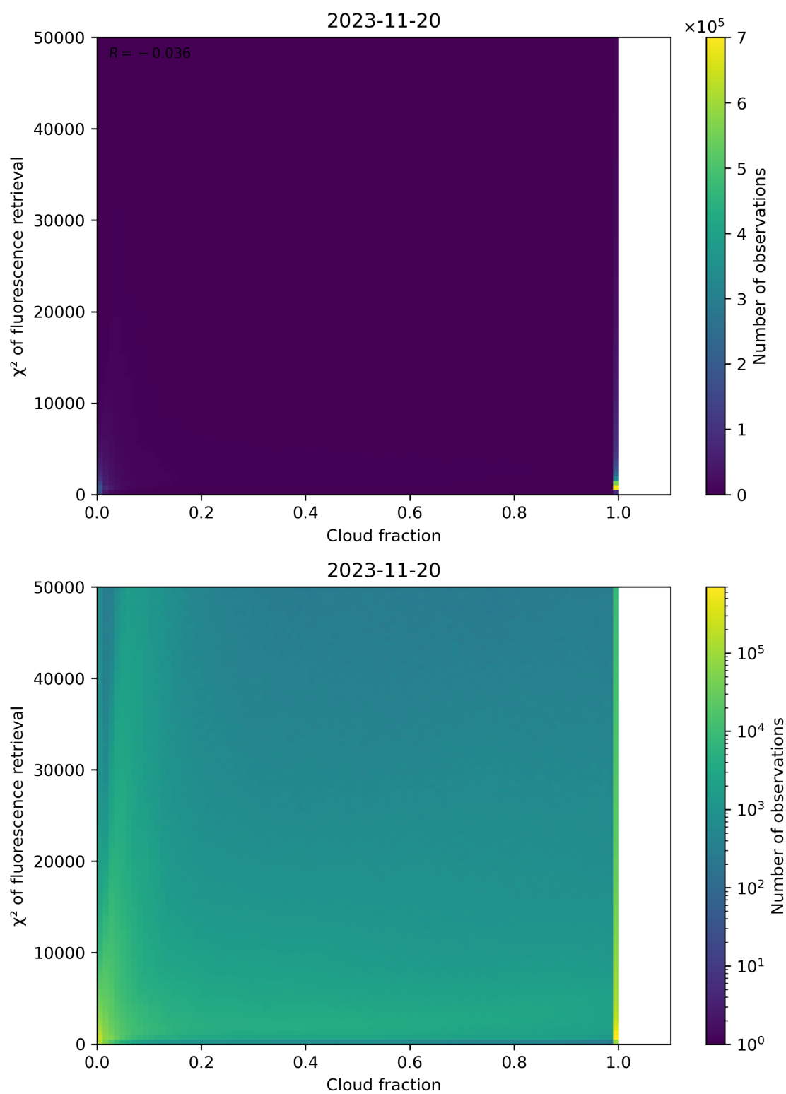
Figure 78: Scatter density plot of “Cloud fraction” against “ \chi^2 of fluorescence retrieval” for 2023-11-19 to 2023-11-21.
