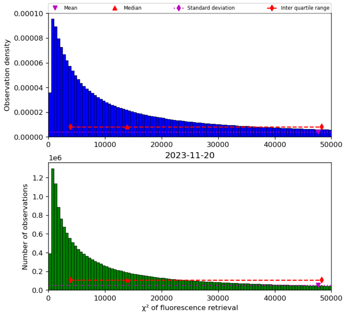
Figure 42: Histogram of “ \chi^2 of fluorescence retrieval” for 2023-11-19 to 2023-11-21
