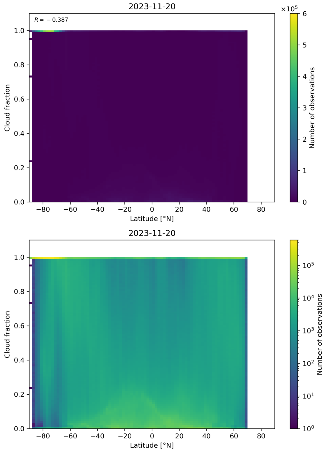
Figure 99: Scatter density plot of “Latitude” against “Cloud fraction” for 2023-11-19 to 2023-11-21.
