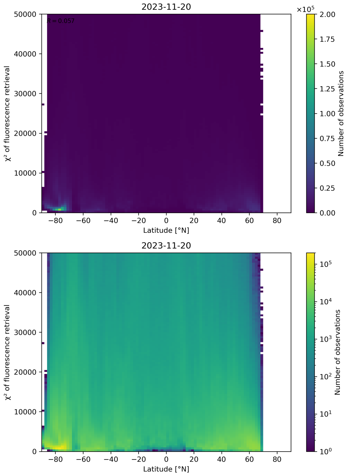
Figure 98: Scatter density plot of “Latitude” against “ \chi^2 of fluorescence retrieval” for 2023-11-19 to 2023-11-21.
