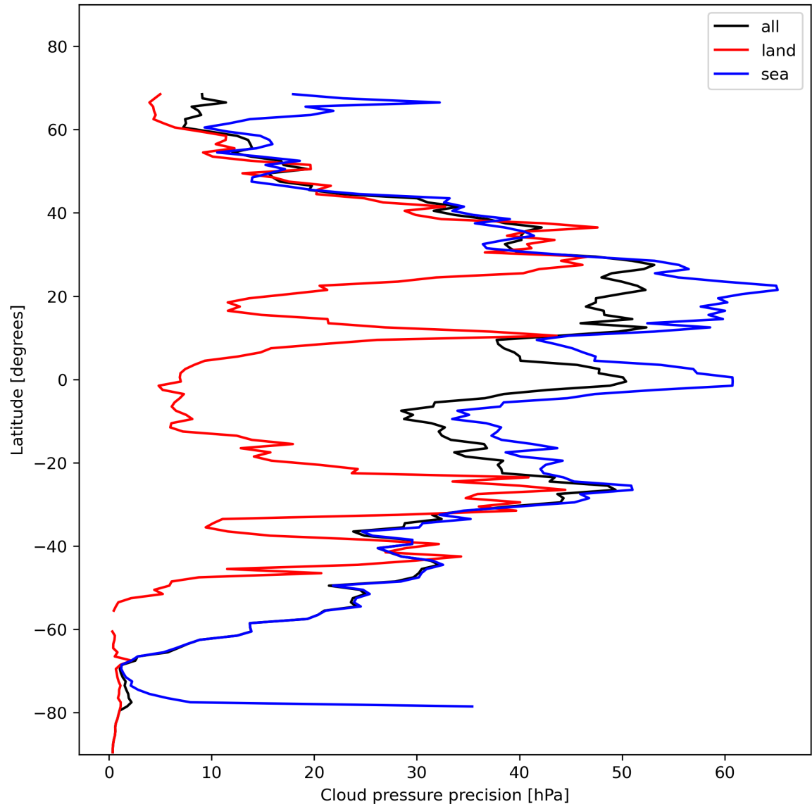
Figure 14: Zonal average of “Cloud pressure precision” for 2023-11-19 to 2023-11-21.
