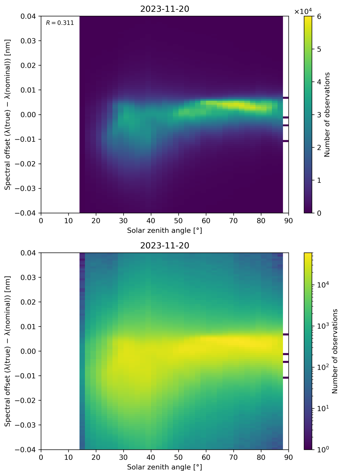
Figure 128: Scatter density plot of “Solar zenith angle” against “Spectral offset ( \lambda(\text{true}) - \lambda(\text{nominal}) )” for 2023-11-19 to 2023-11-21.
