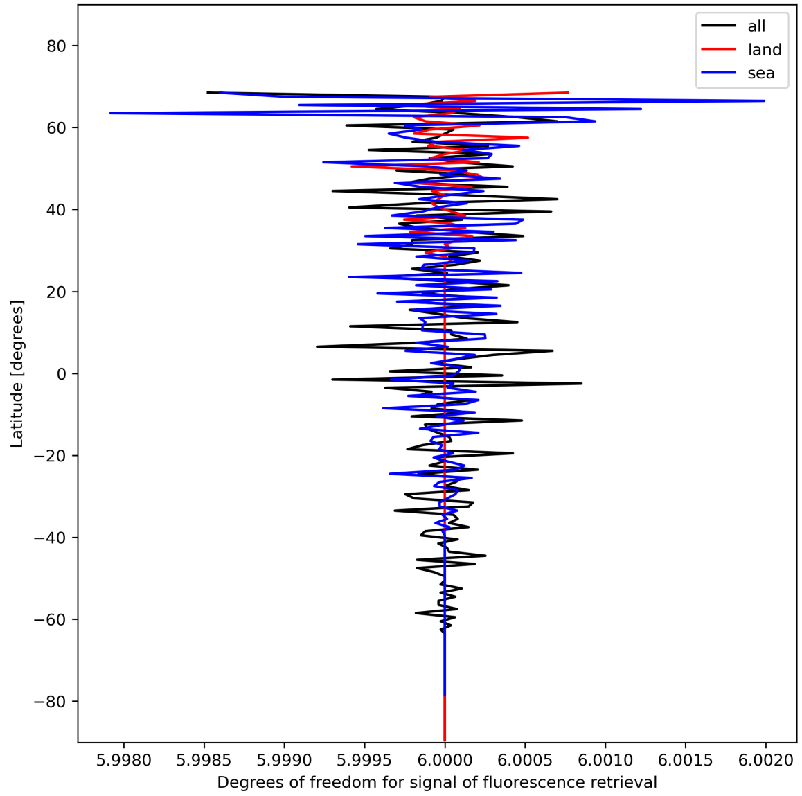
Figure 26: Zonal average of “Degrees of freedom for signal of fluorescence retrieval” for 2023-11-19 to 2023-11-21.
