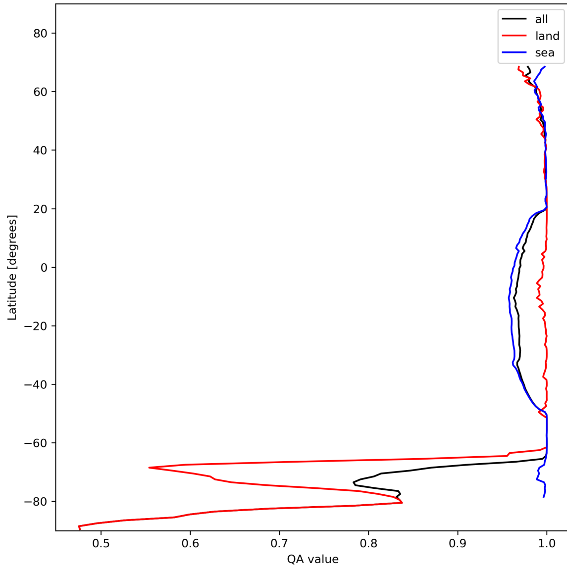
Figure 12: Zonal average of “QA value” for 2023-11-19 to 2023-11-21.
