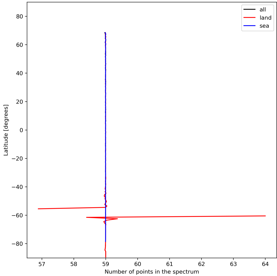
Figure 27: Zonal average of “Number of points in the spectrum” for 2023-11-19 to 2023-11-21.
