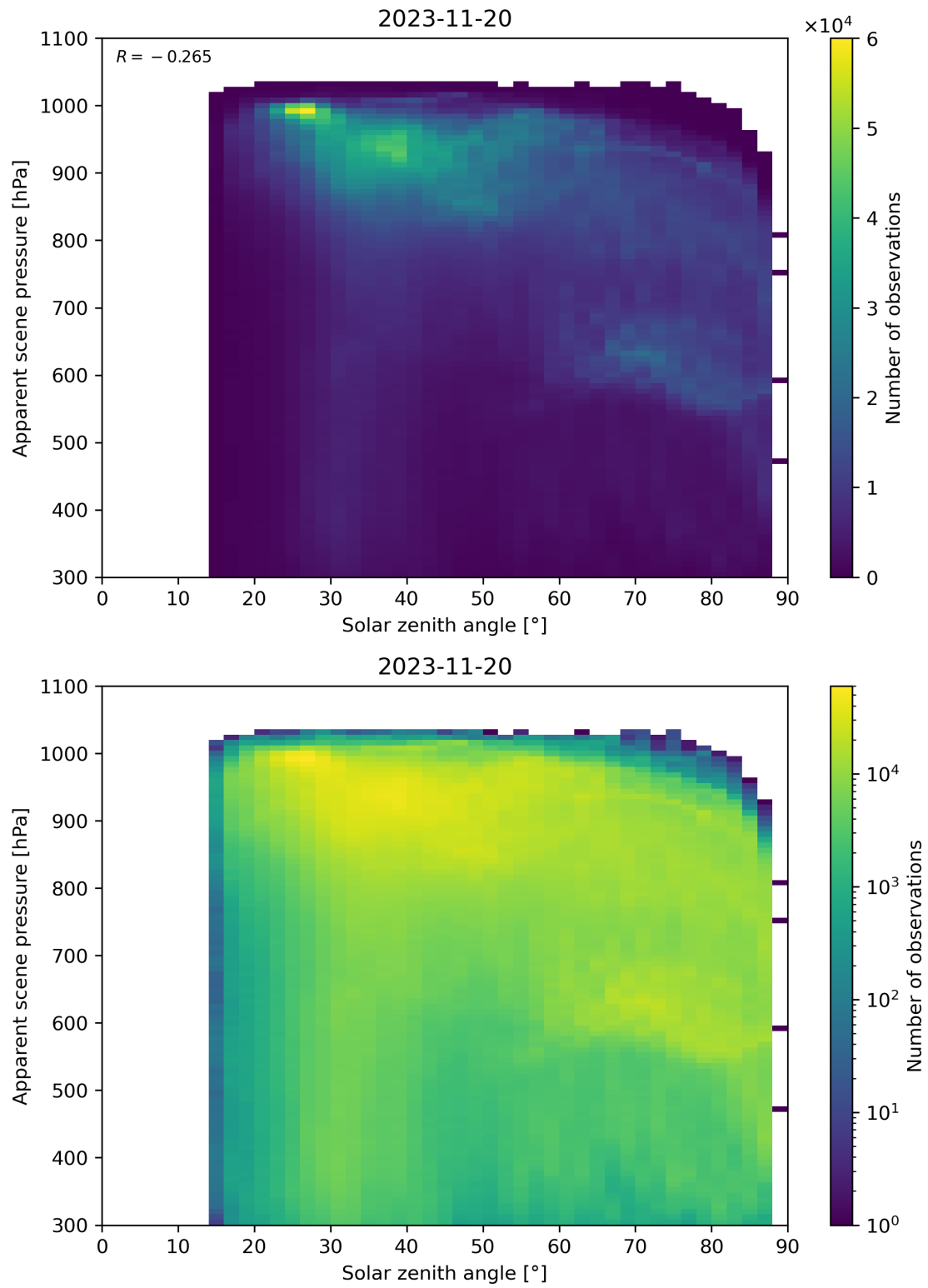
Figure 118: Scatter density plot of “Solar zenith angle” against “Apparent scene pressure” for 2023-11-19 to 2023-11-21.
