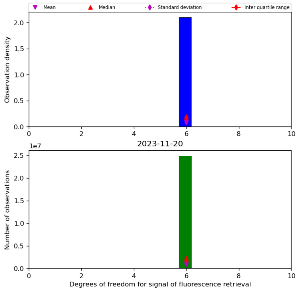
Figure 43: Histogram of “Degrees of freedom for signal of fluorescence retrieval” for 2023-11-19 to 2023-11-21
