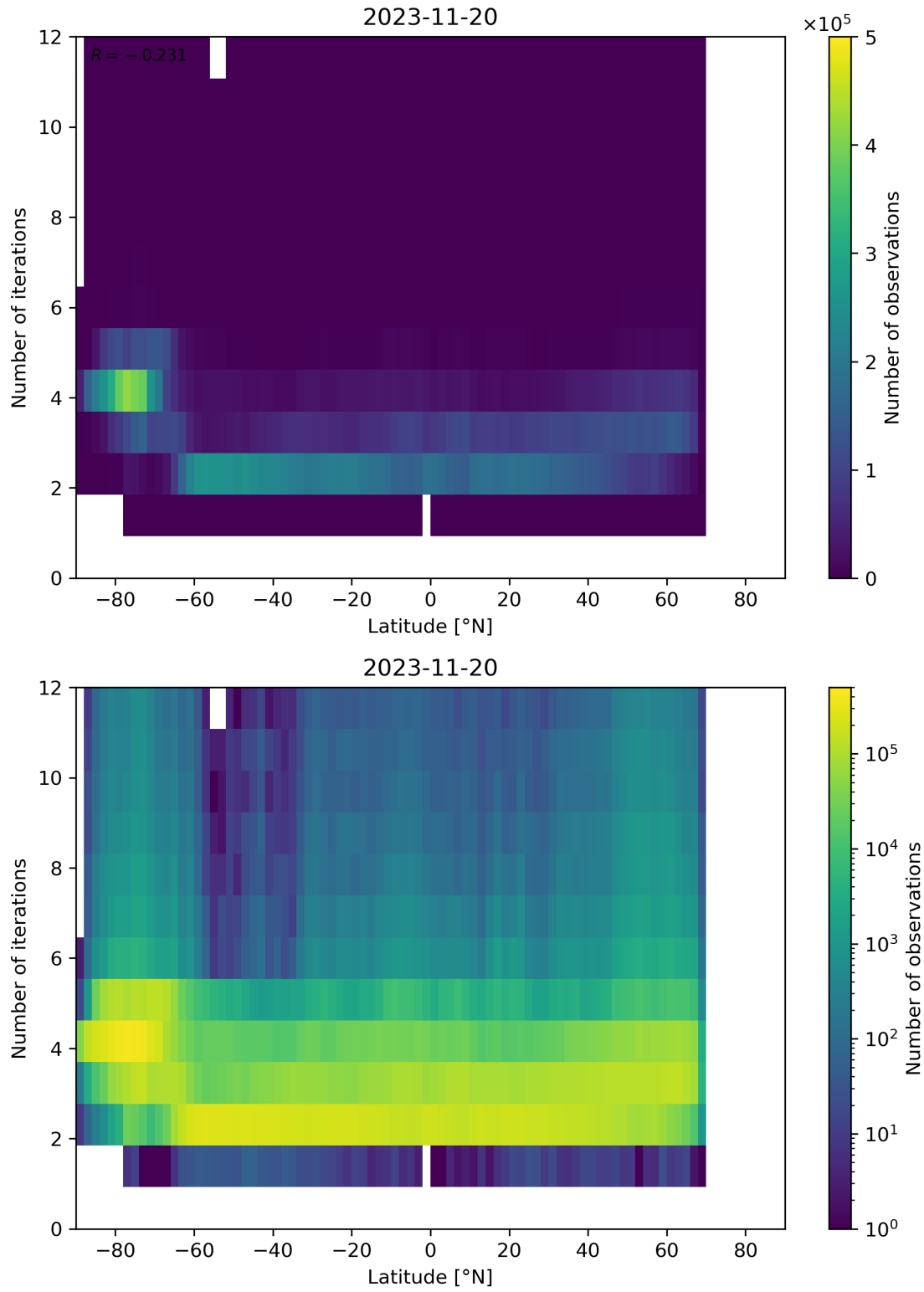
Figure 102: Scatter density plot of “Latitude” against “Number of iterations” for 2023-11-19 to 2023-11-21.
