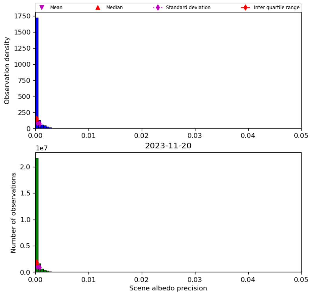
Figure 35: Histogram of “Scene albedo precision” for 2023-11-19 to 2023-11-21
