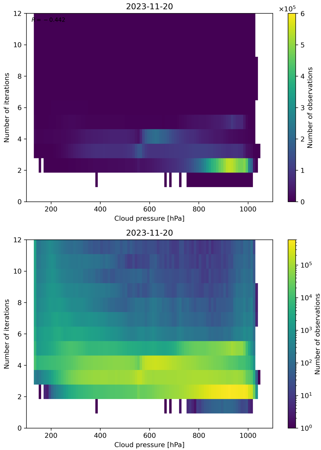
Figure 89: Scatter density plot of “Cloud pressure” against “Number of iterations” for 2023-11-19 to 2023-11-21.
