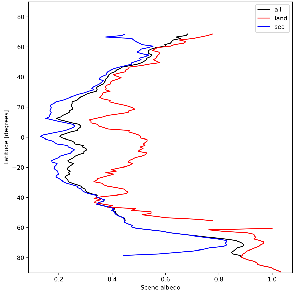
Figure 17: Zonal average of “Scene albedo” for 2023-11-19 to 2023-11-21.
