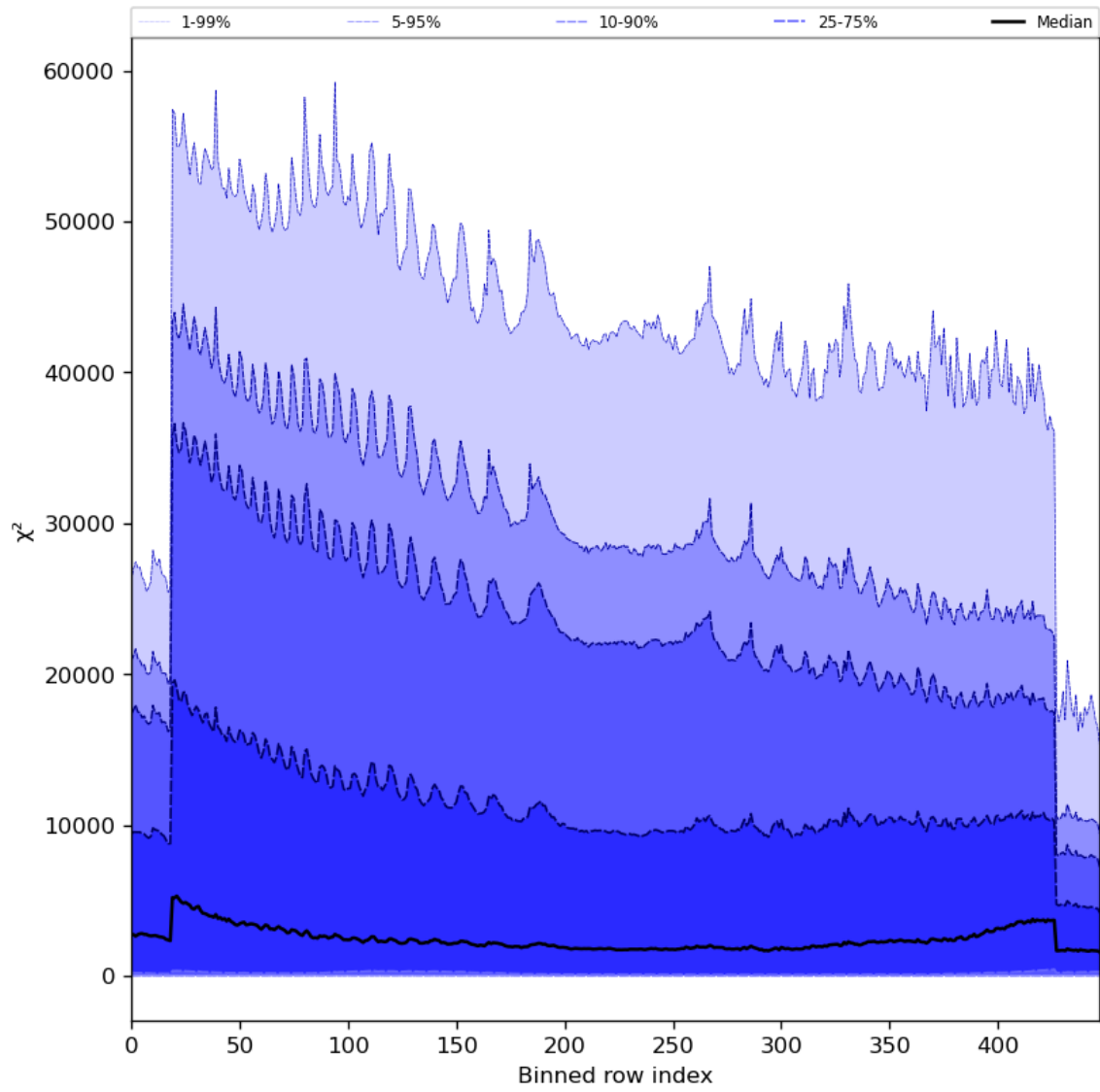
Figure 55: Along track statistics of “ \chi^2 ” for 2023-11-19 to 2023-11-21
