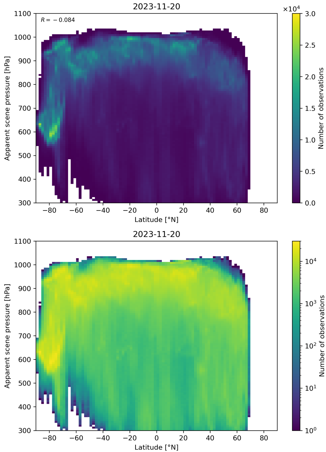
Figure 96: Scatter density plot of “Latitude” against “Apparent scene pressure” for 2023-11-19 to 2023-11-21.
