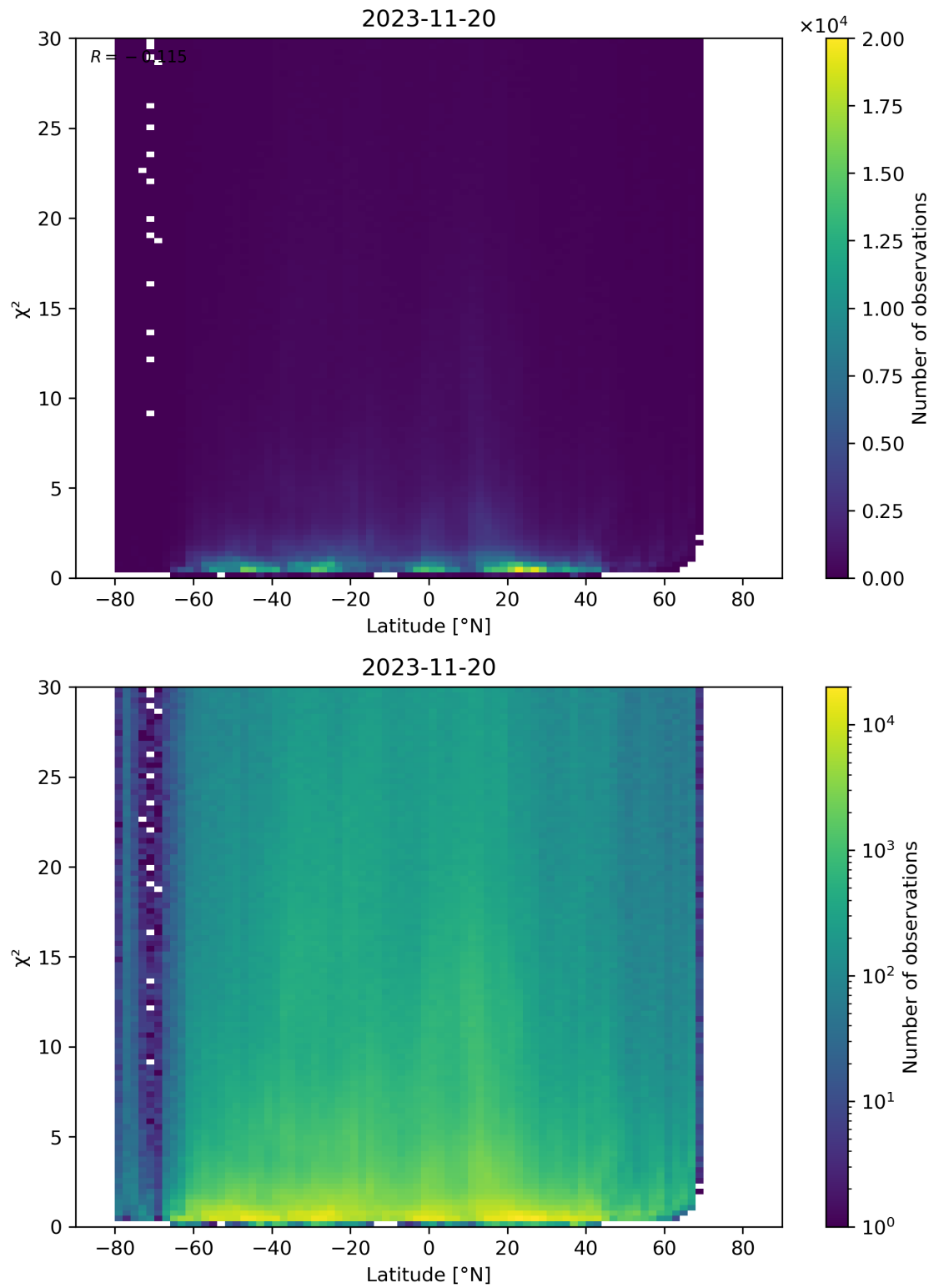
Figure 97: Scatter density plot of “Latitude” against “ \chi^2 ” for 2023-11-19 to 2023-11-21.
