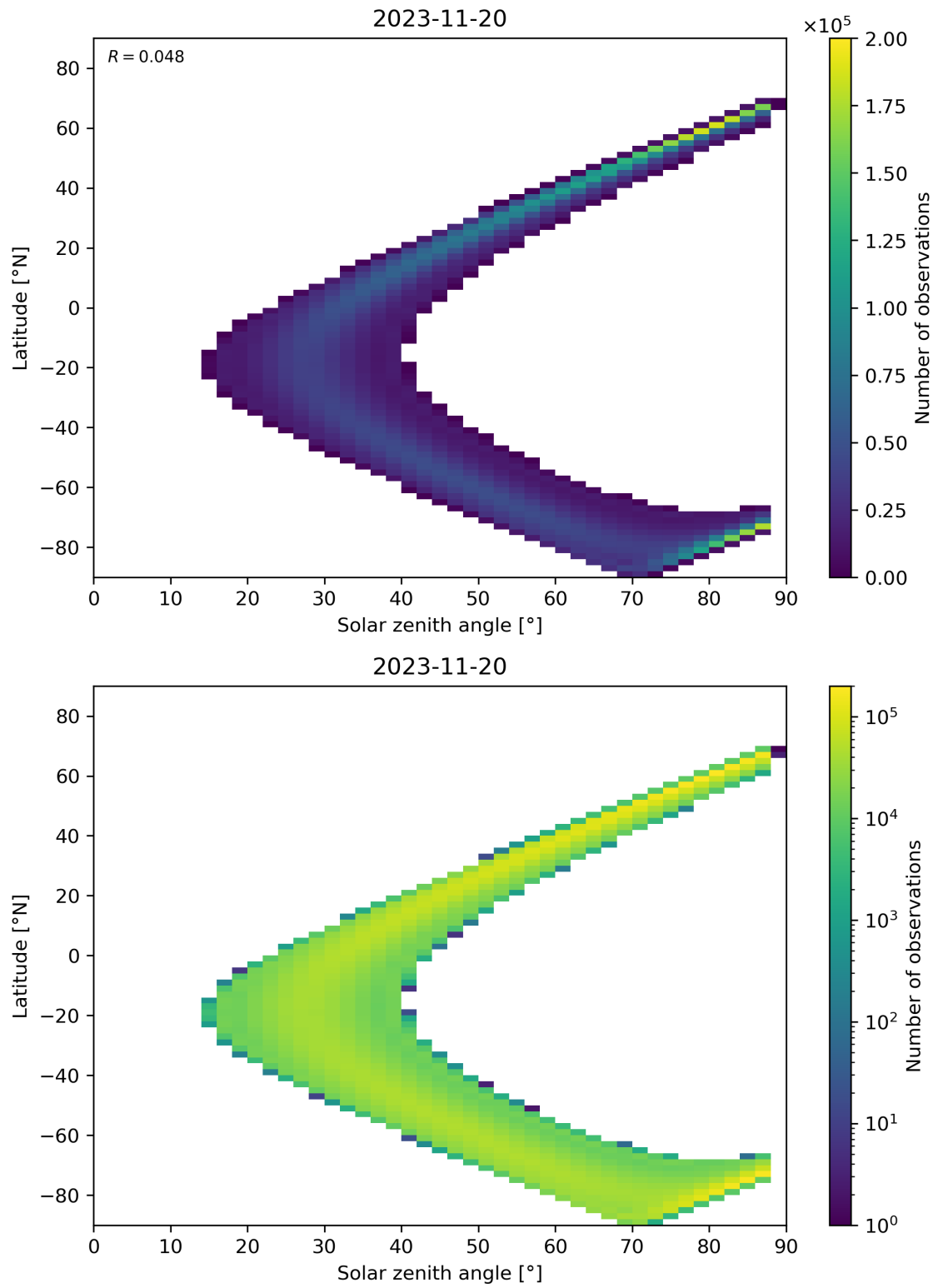
Figure 124: Scatter density plot of “Solar zenith angle” against “Latitude” for 2023-11-19 to 2023-11-21.
