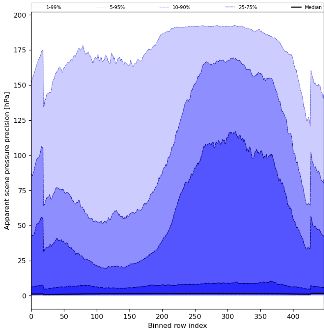
Figure 54: Along track statistics of “Apparent scene pressure precision” for 2023-11-19 to 2023-11-21
