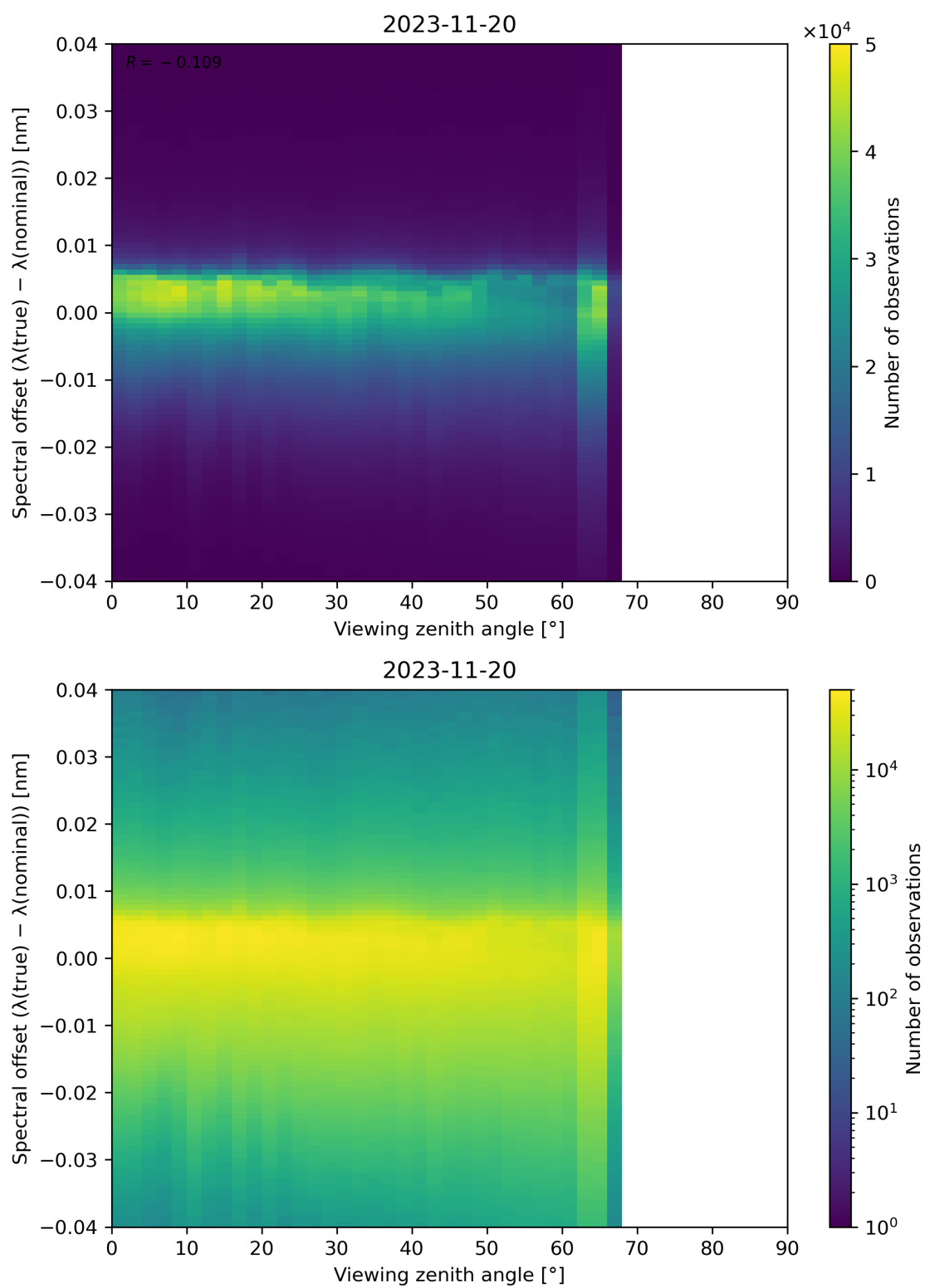
Figure 140: Scatter density plot of “Viewing zenith angle” against “Spectral offset ( \lambda(\text{true}) - \lambda(\text{nominal}) )” for 2023-11-19 to 2023-11-21.
