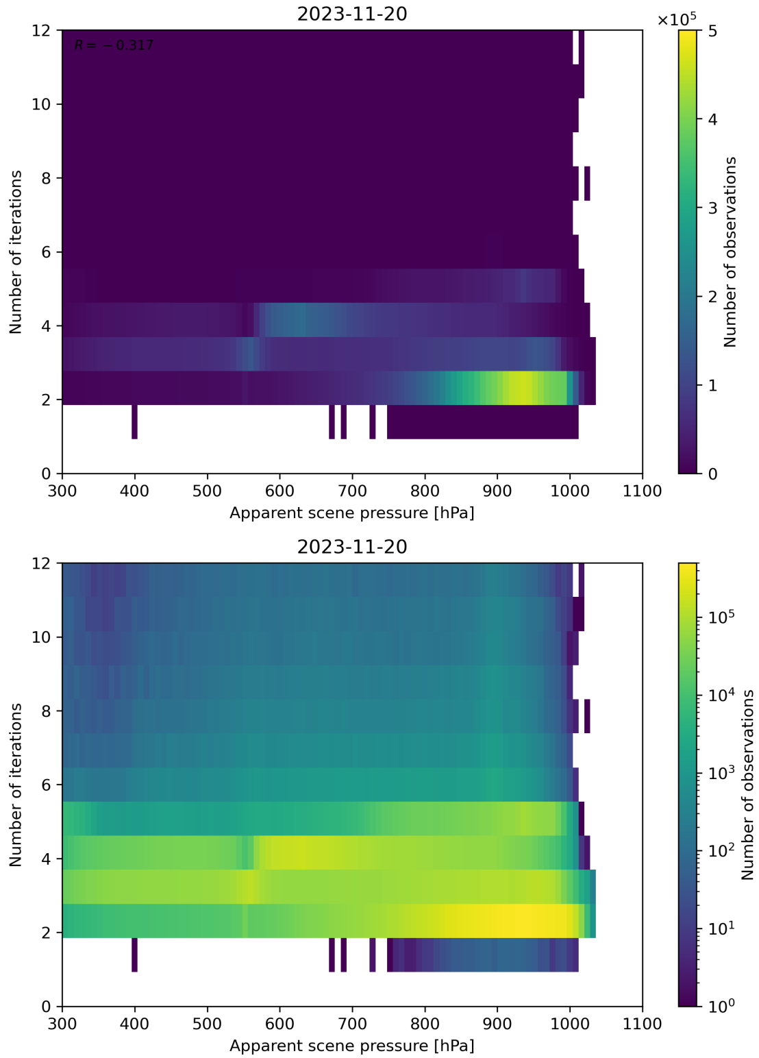
Figure 66: Scatter density plot of “Apparent scene pressure” against “Number of iterations” for 2023-11-19 to 2023-11-21.
