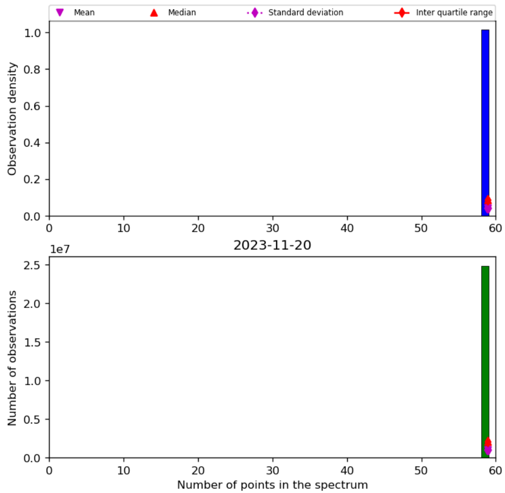
Figure 44: Histogram of "Number of points in the spectrum" for 2023-11-19 to 2023-11-21
