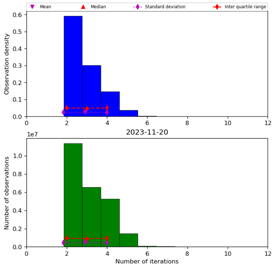
Figure 39: Histogram of “Number of iterations” for 2023-11-19 to 2023-11-21
