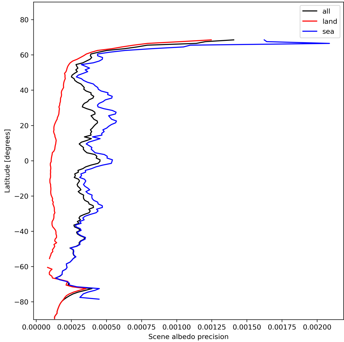
Figure 18: Zonal average of “Scene albedo precision” for 2023-11-19 to 2023-11-21.
