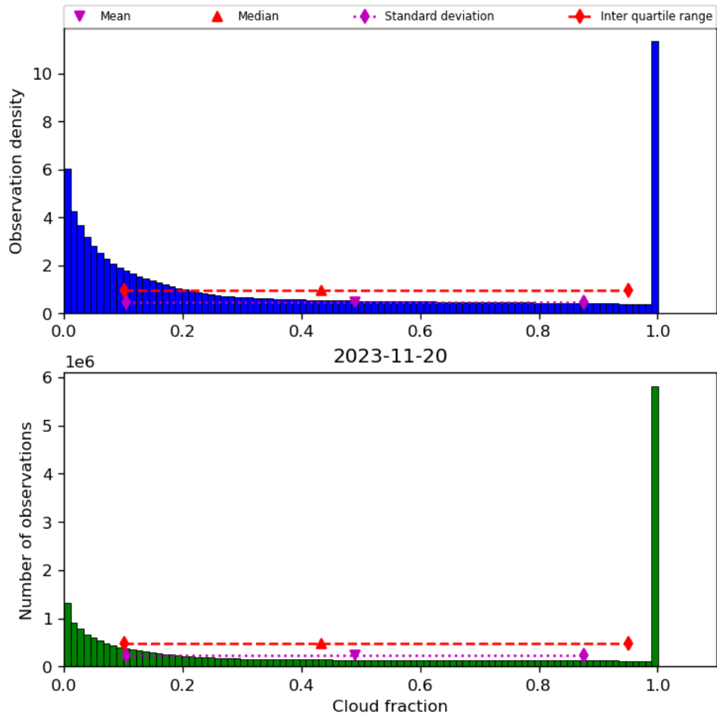
Figure 32: Histogram of “Cloud fraction” for 2023-11-19 to 2023-11-21
