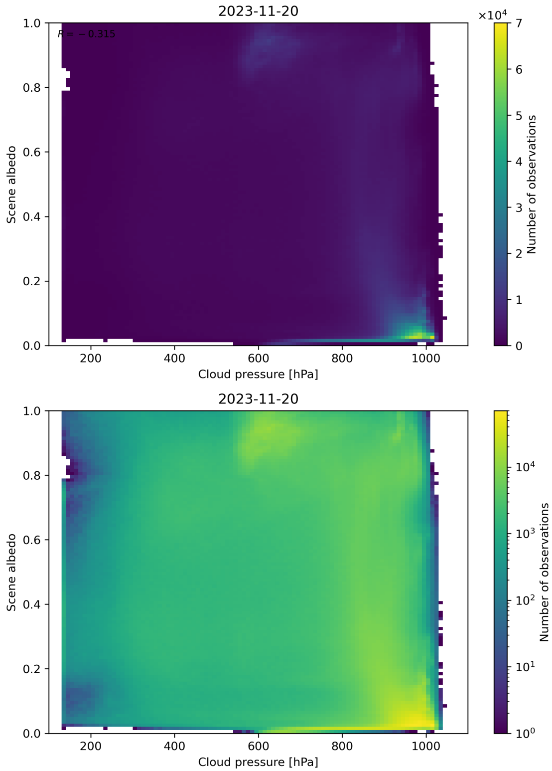
Figure 91: Scatter density plot of “Cloud pressure” against “Scene albedo” for 2023-11-19 to 2023-11-21.
