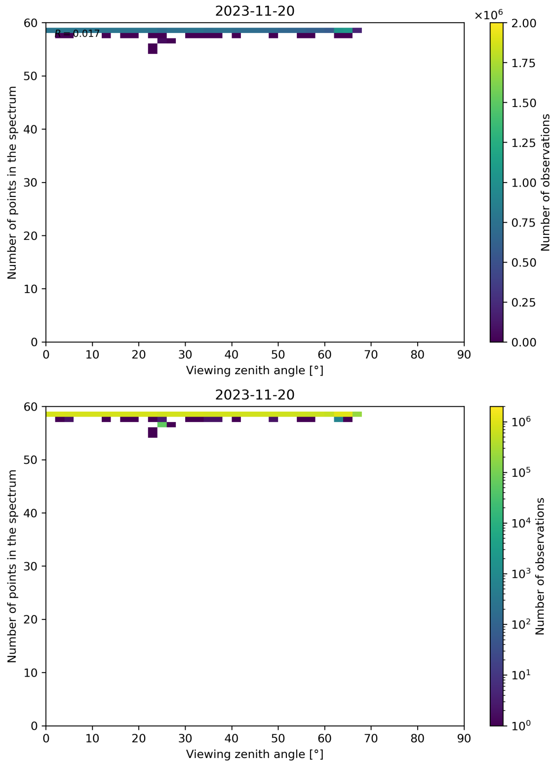
Figure 137: Scatter density plot of “Viewing zenith angle” against “Number of points in the spectrum” for 2023-11-19 to 2023-11-21.
