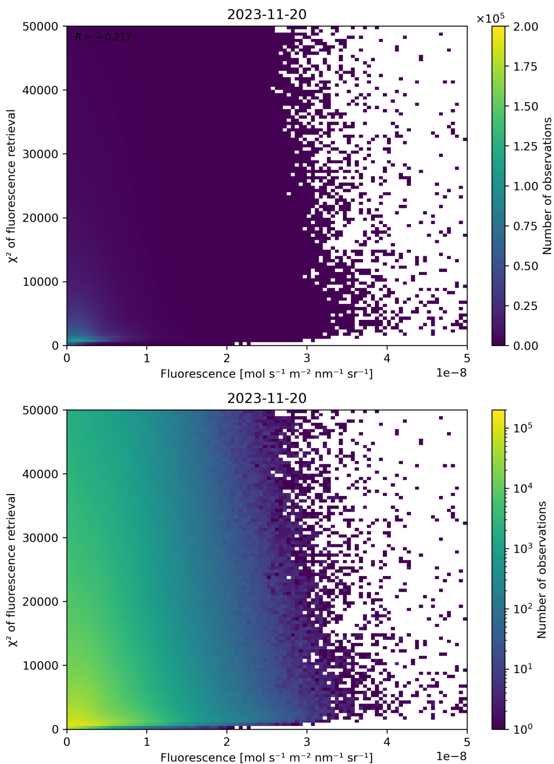
Figure 93: Scatter density plot of “Fluorescence” against “ \chi^2 of fluorescence retrieval” for 2023-11-19 to 2023-11-21.
