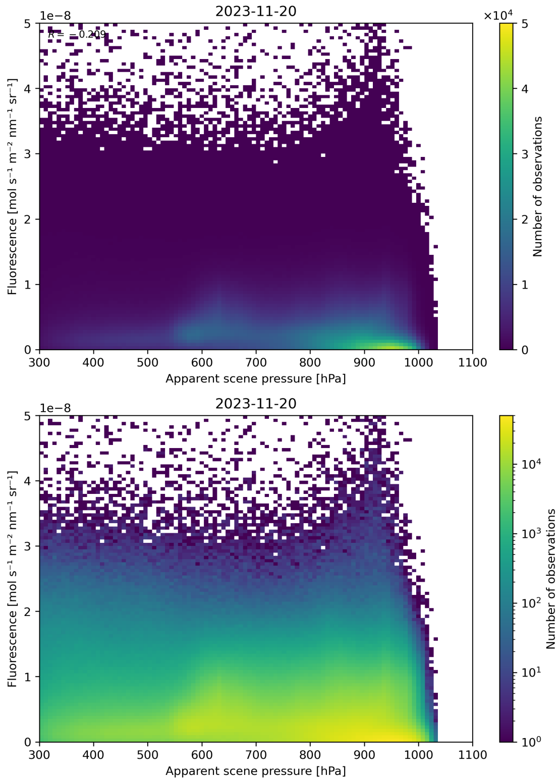
Figure 65: Scatter density plot of “Apparent scene pressure” against “Fluorescence” for 2023-11-19 to 2023-11-21.
