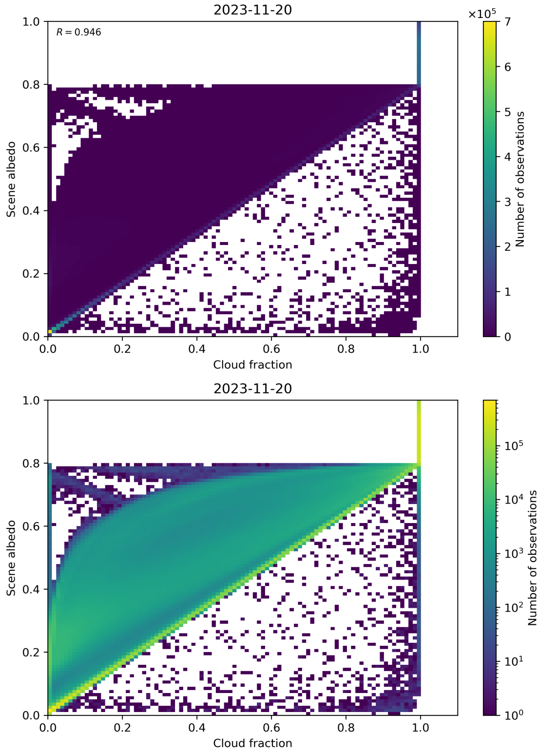
Figure 82: Scatter density plot of “Cloud fraction” against “Scene albedo” for 2023-11-19 to 2023-11-21.
