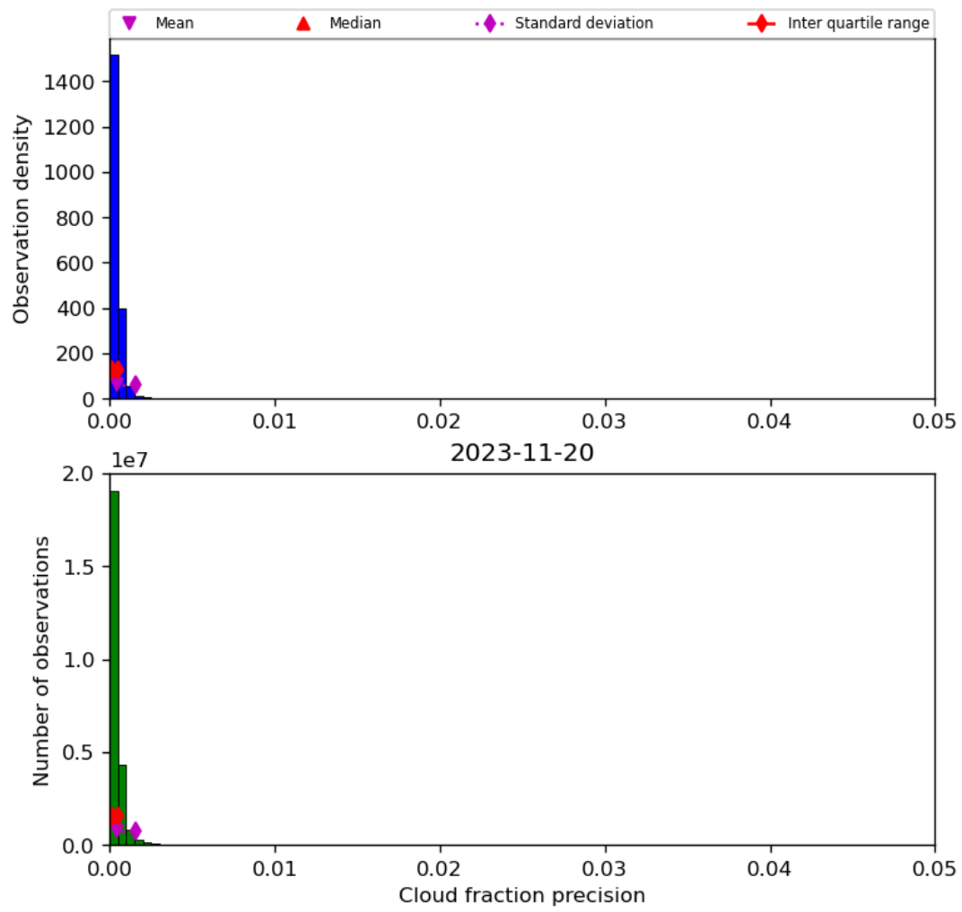
Figure 33: Histogram of “Cloud fraction precision” for 2023-11-19 to 2023-11-21
