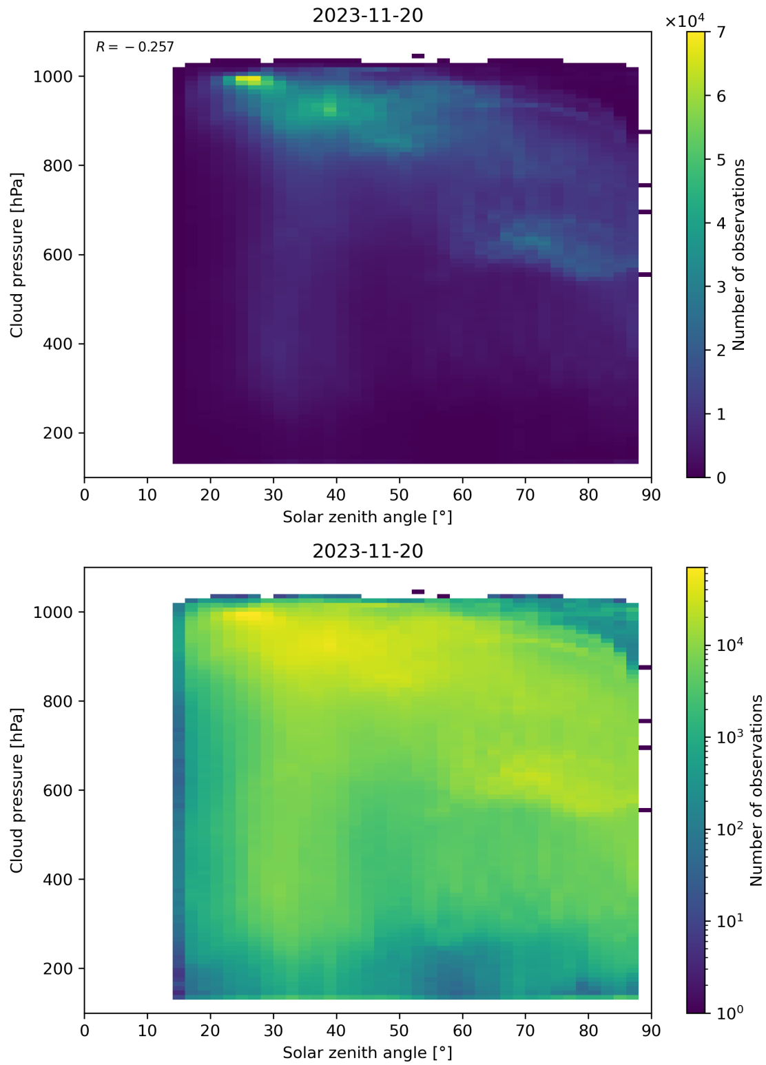
Figure 122: Scatter density plot of “Solar zenith angle” against “Cloud pressure” for 2023-11-19 to 2023-11-21.
