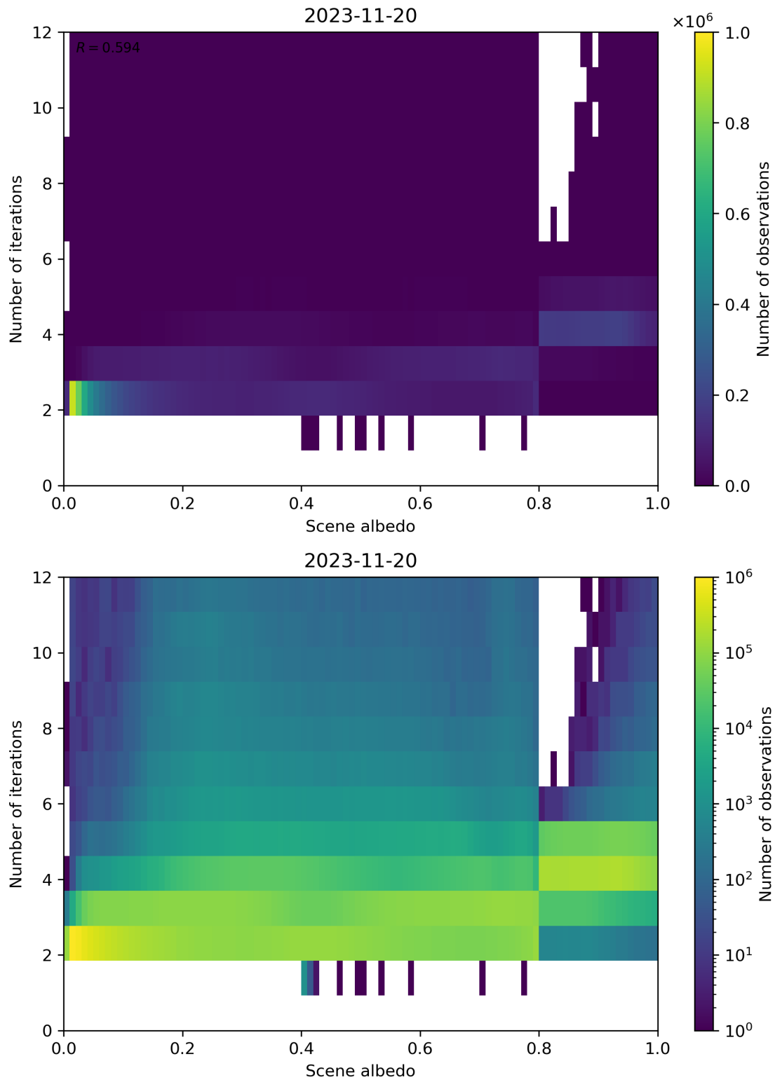
Figure 115: Scatter density plot of “Scene albedo” against “Number of iterations” for 2023-11-19 to 2023-11-21.
