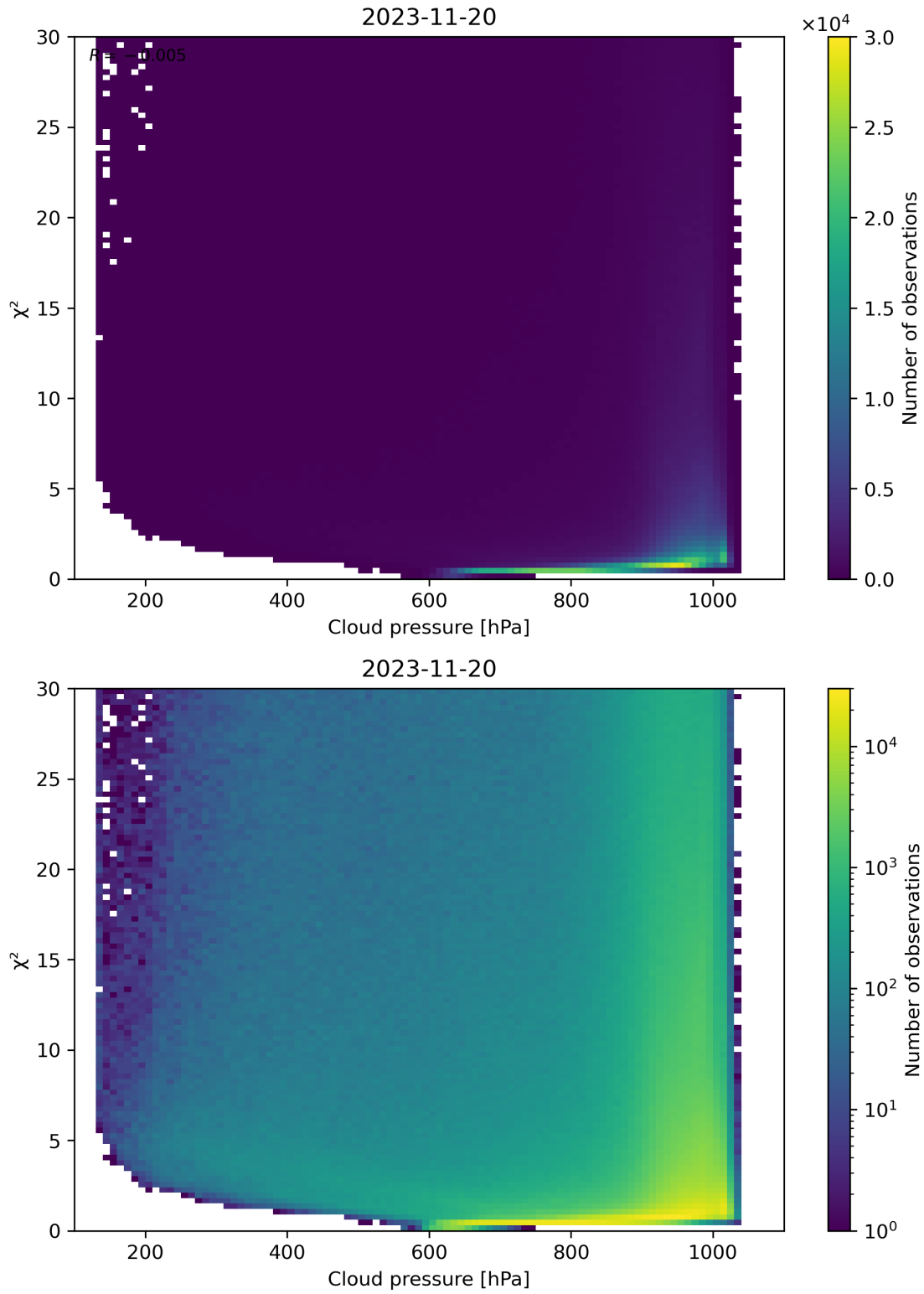
Figure 85: Scatter density plot of “Cloud pressure” against “ \chi^2 ” for 2023-11-19 to 2023-11-21.
