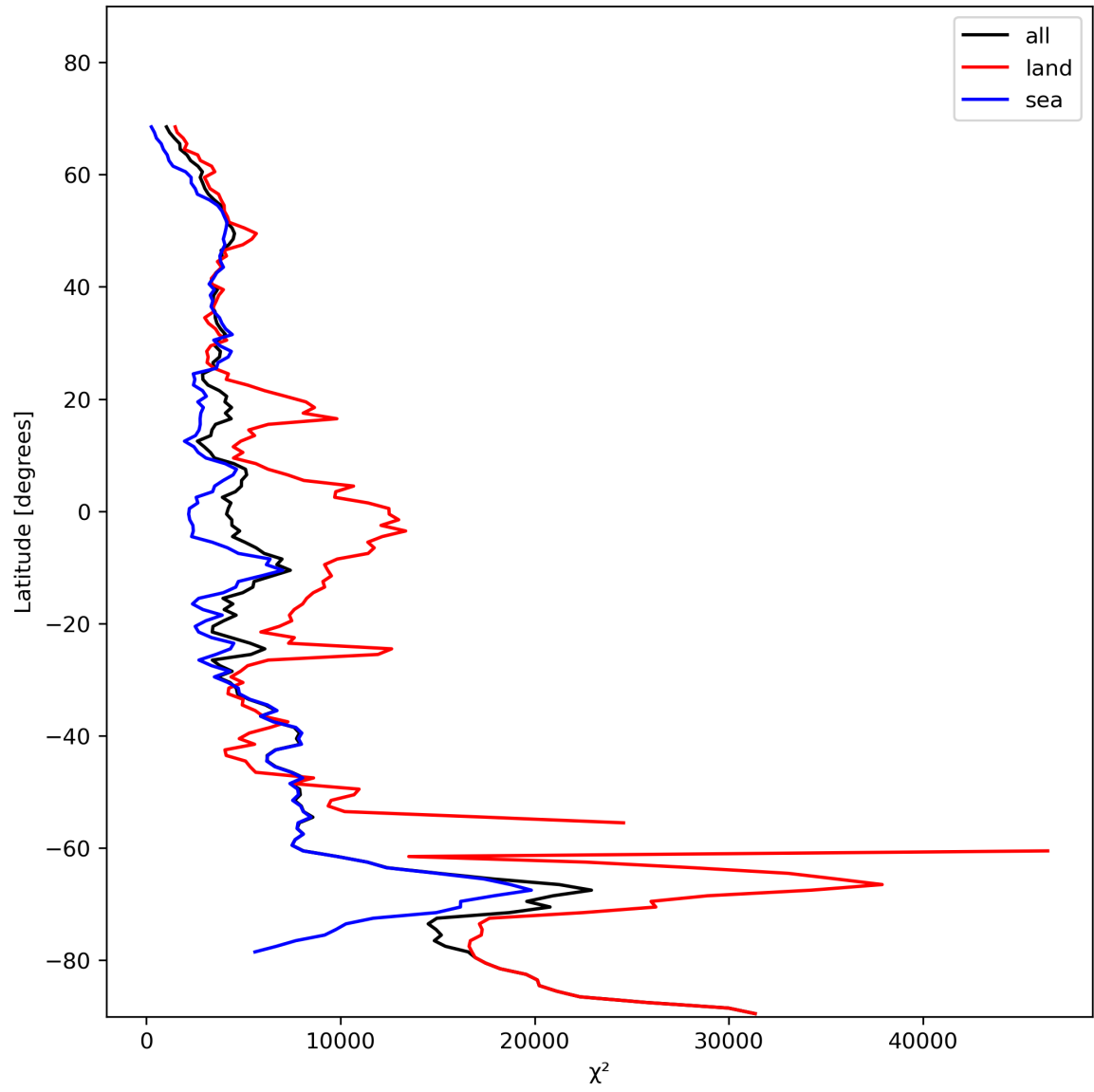
Figure 21: Zonal average of “ \chi^2 ” for 2023-11-19 to 2023-11-21.
