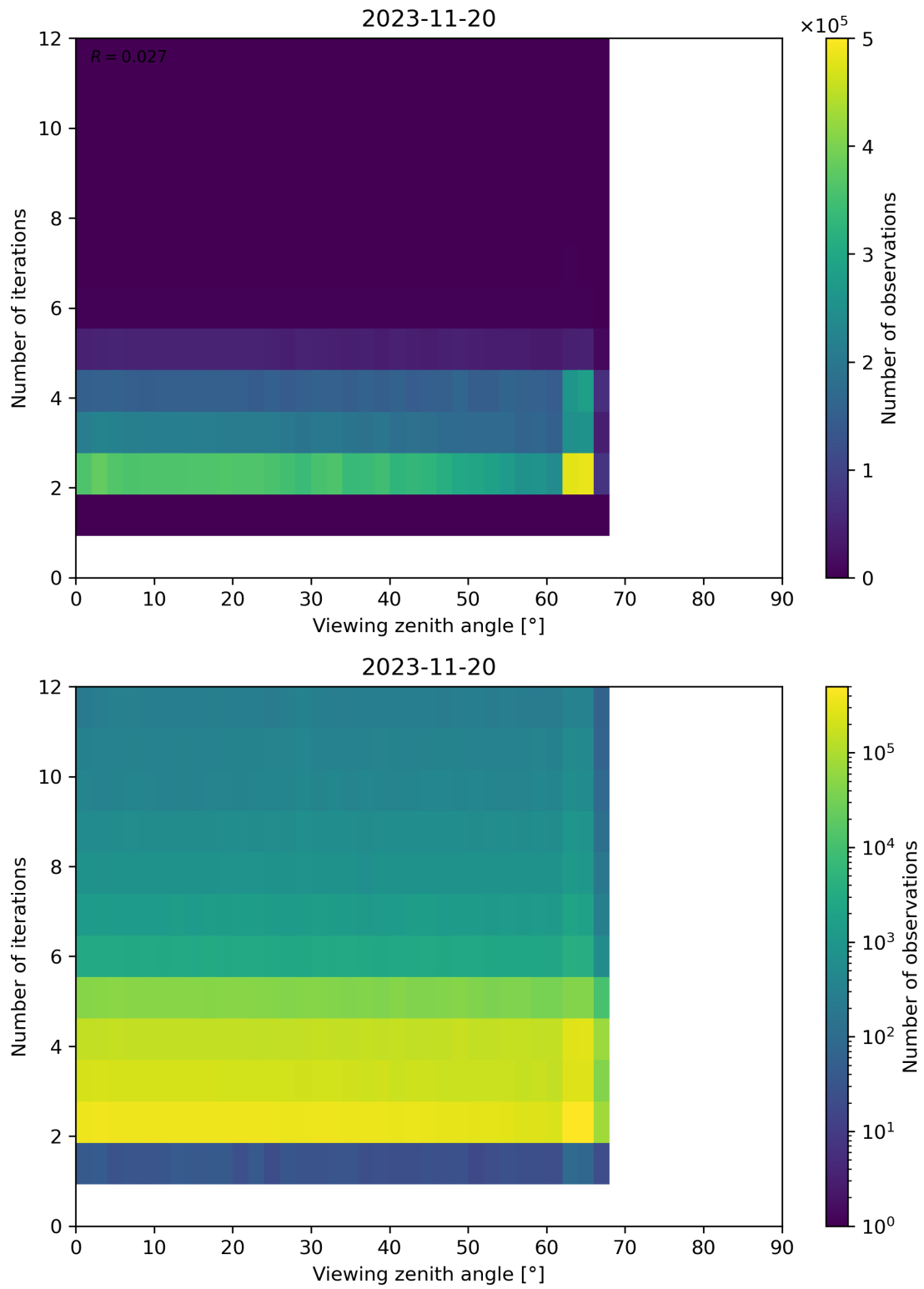
Figure 136: Scatter density plot of “Viewing zenith angle” against “Number of iterations” for 2023-11-19 to 2023-11-21.
