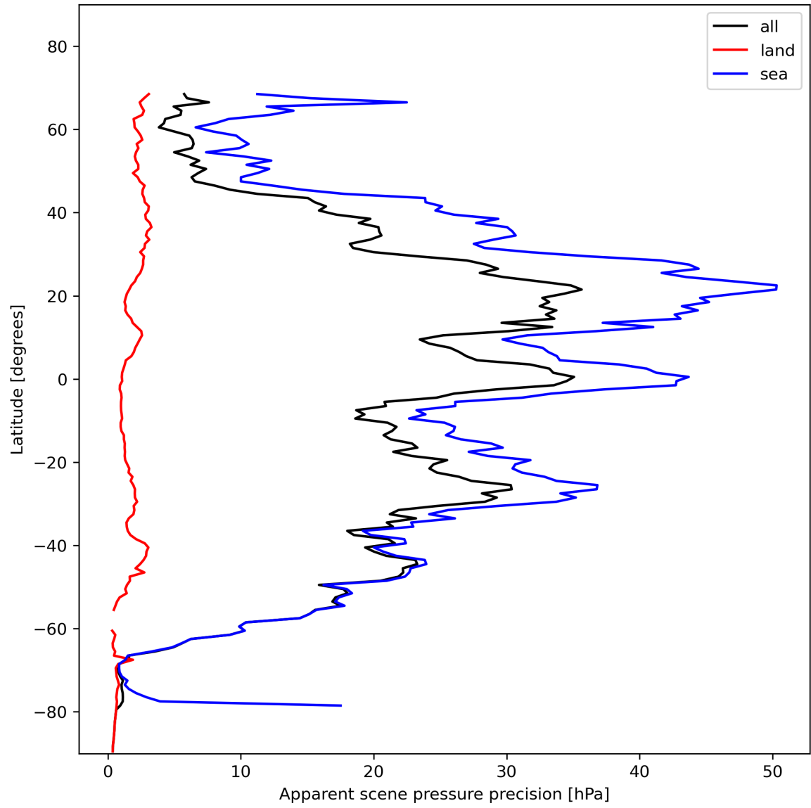
Figure 20: Zonal average of “Apparent scene pressure precision” for 2023-11-19 to 2023-11-21.
