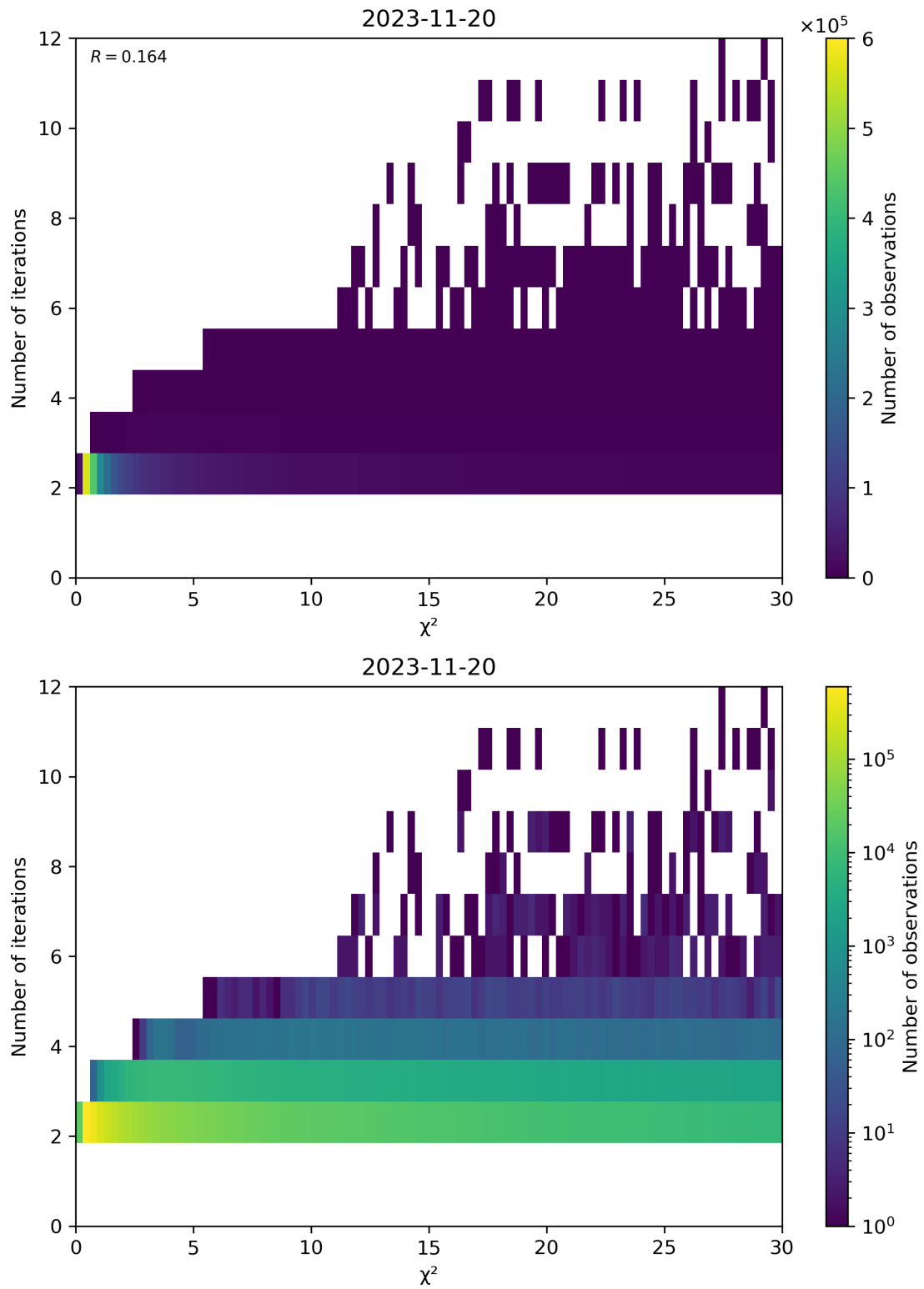
Figure 73: Scatter density plot of “ \chi^2 ” against “Number of iterations” for 2023-11-19 to 2023-11-21.
