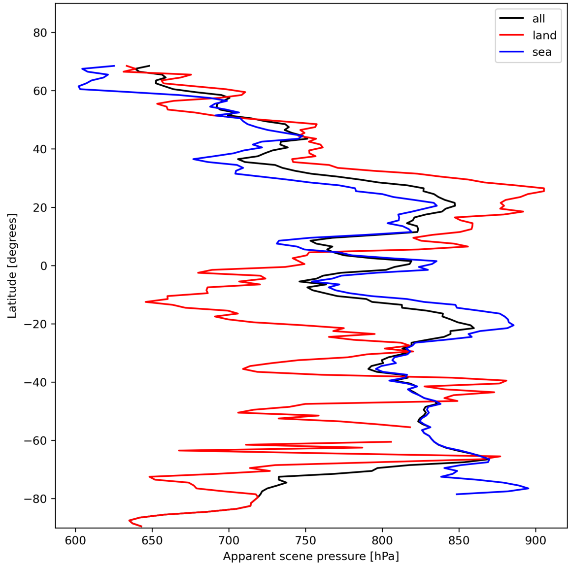
Figure 19: Zonal average of “Apparent scene pressure” for 2023-11-19 to 2023-11-21.
