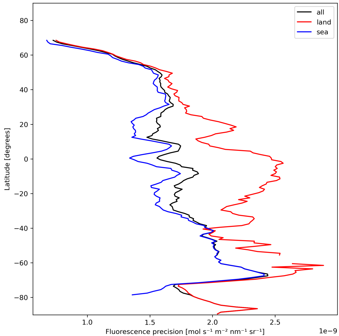
Figure 24: Zonal average of “Fluorescence precision” for 2023-11-19 to 2023-11-21.
