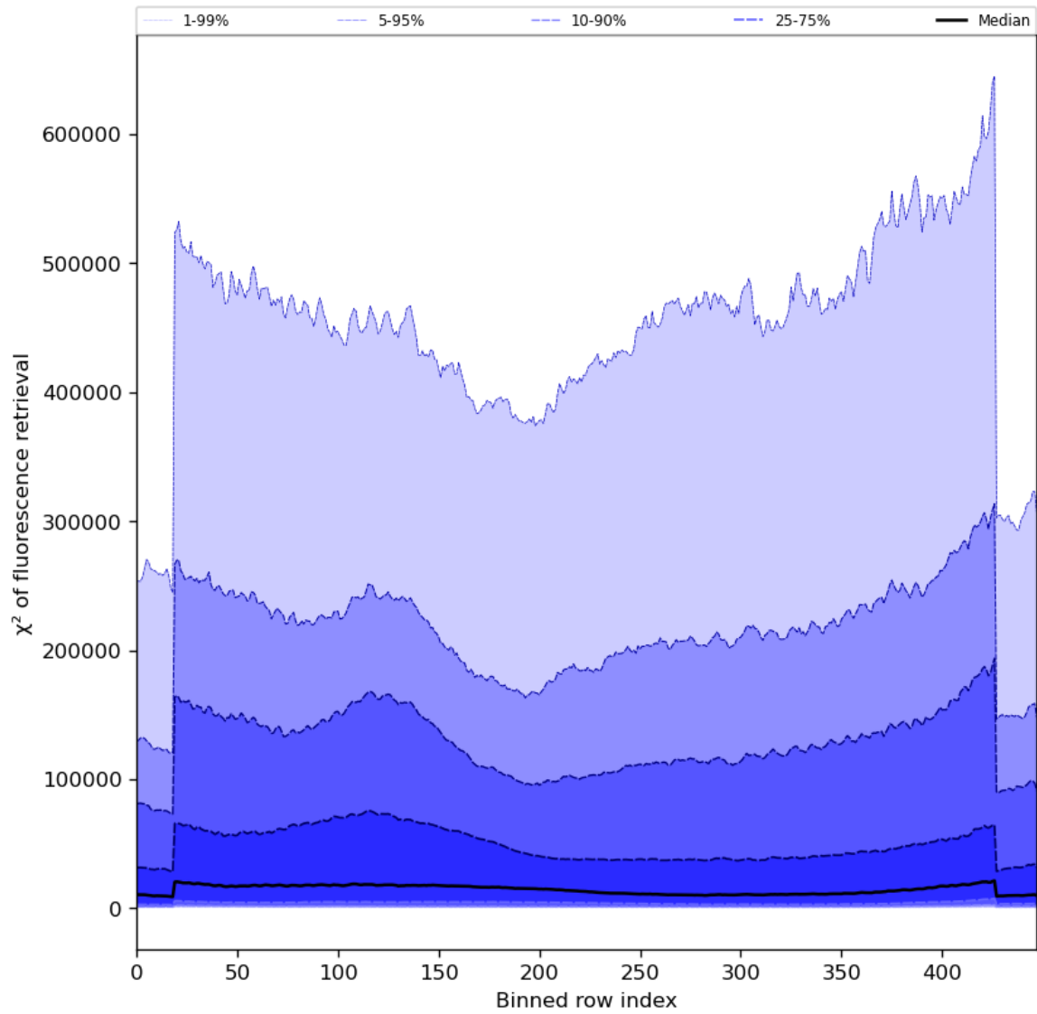
Figure 59: Along track statistics of “ \chi^2 of fluorescence retrieval” for 2023-11-19 to 2023-11-21
