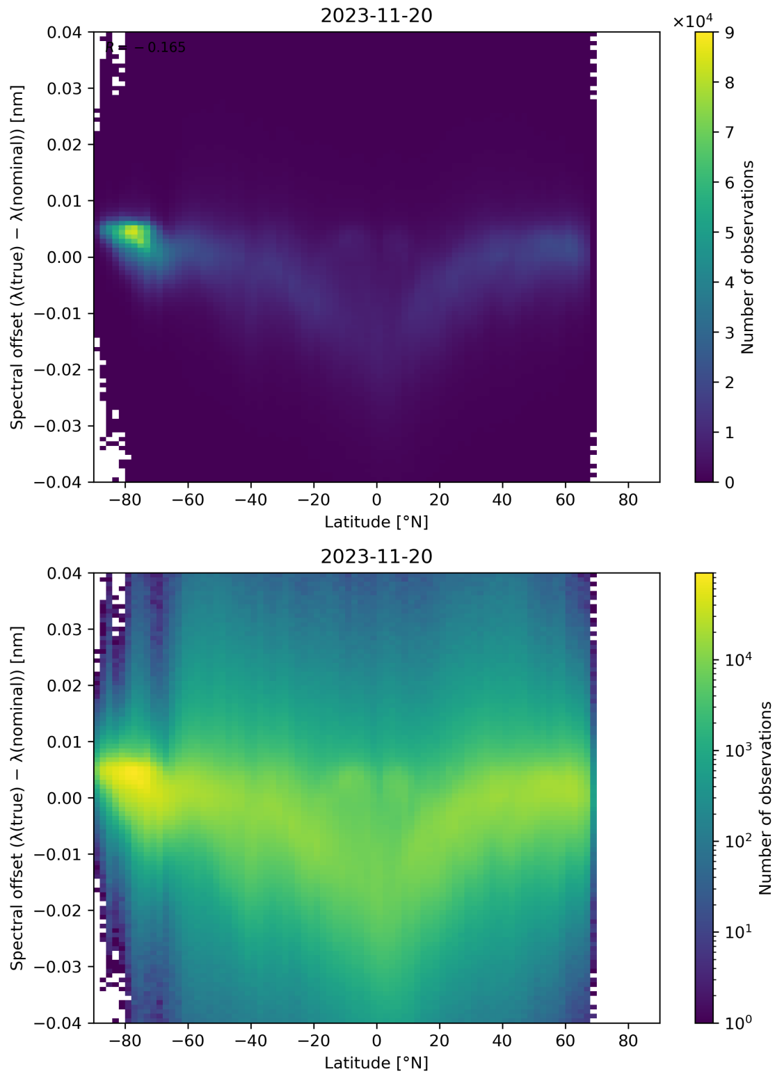
Figure 105: Scatter density plot of “Latitude” against “Spectral offset ( \lambda(\text{true}) - \lambda(\text{nominal}) )” for 2023-11-19 to 2023-11-21.
