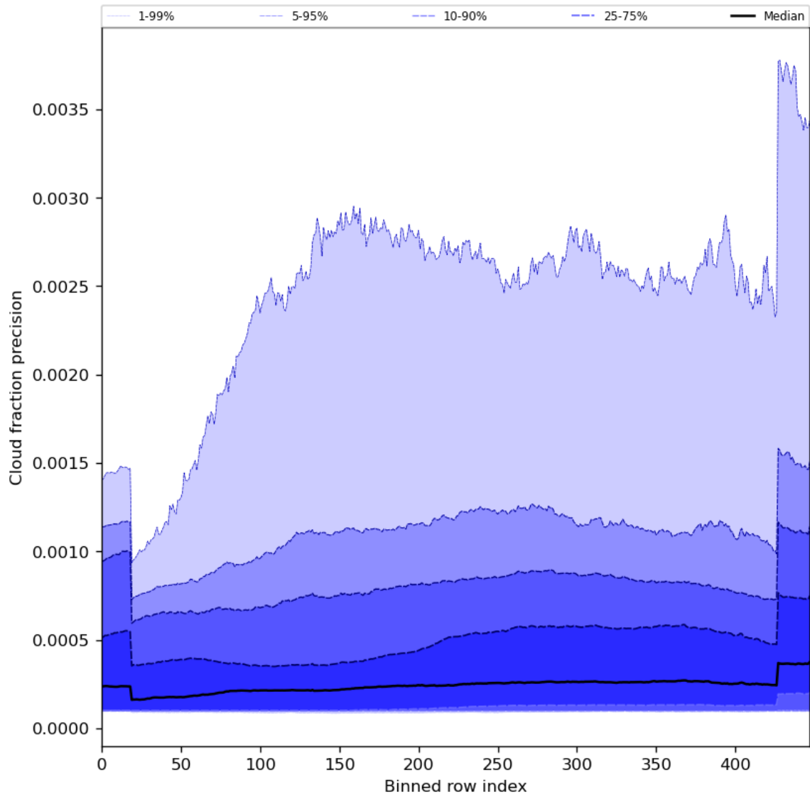
Figure 50: Along track statistics of “Cloud fraction precision” for 2023-11-19 to 2023-11-21
