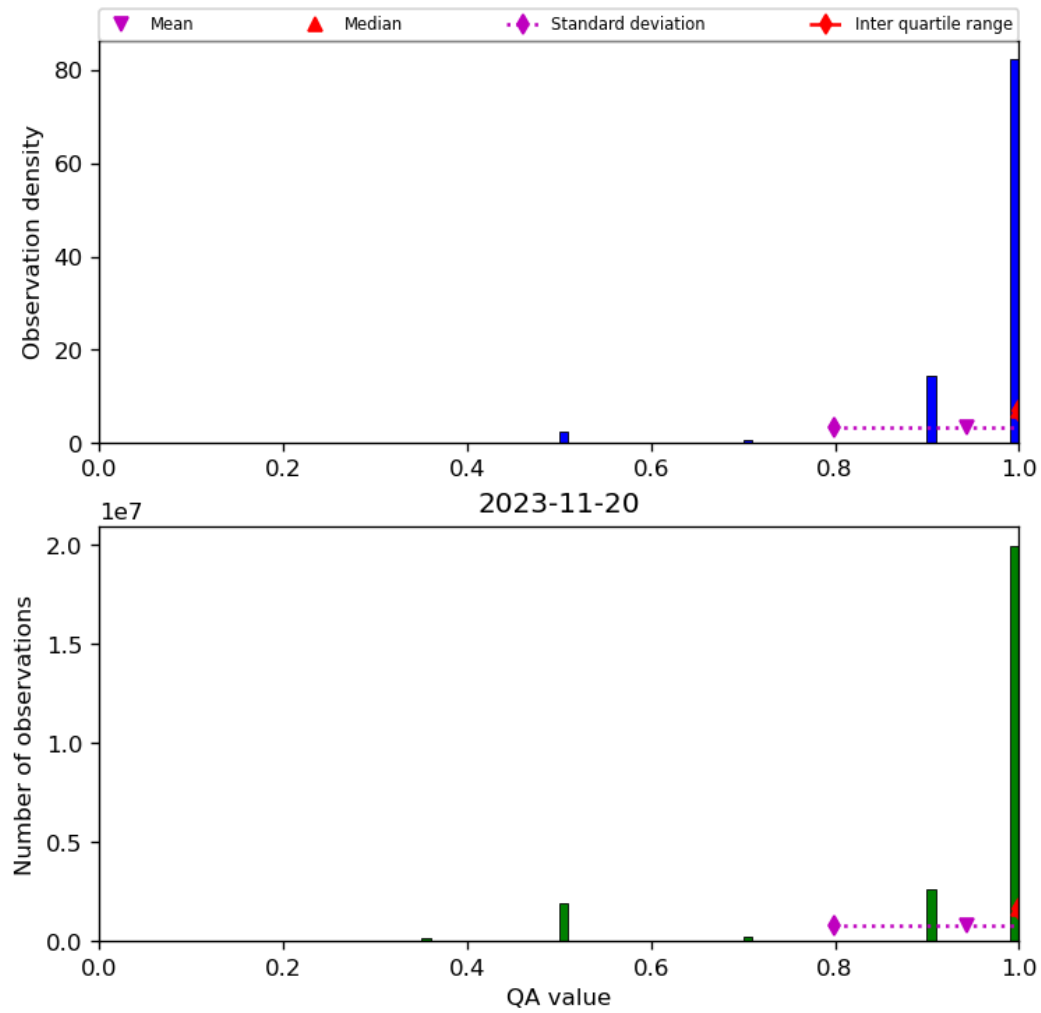
Figure 29: Histogram of “QA value” for 2023-11-19 to 2023-11-21
