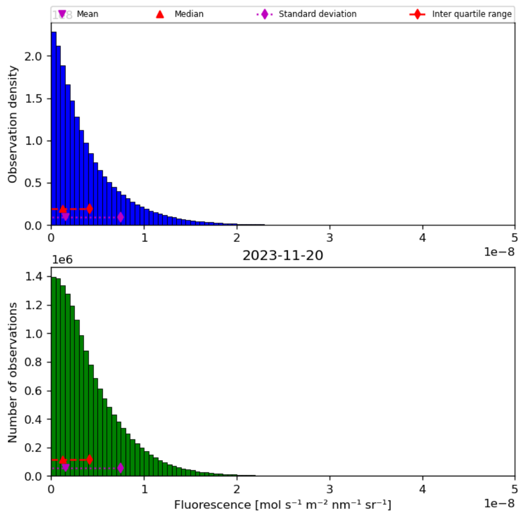
Figure 40: Histogram of “Fluorescence” for 2023-11-19 to 2023-11-21
