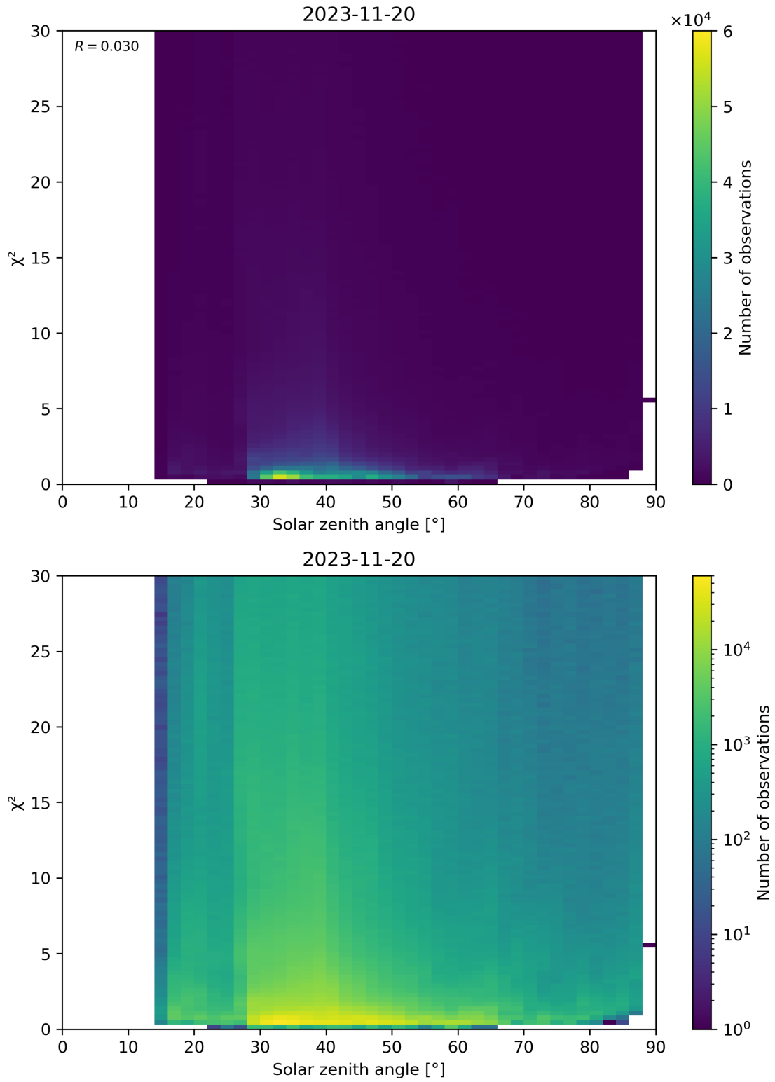
Figure 119: Scatter density plot of “Solar zenith angle” against “ \chi^2 ” for 2023-11-19 to 2023-11-21.
