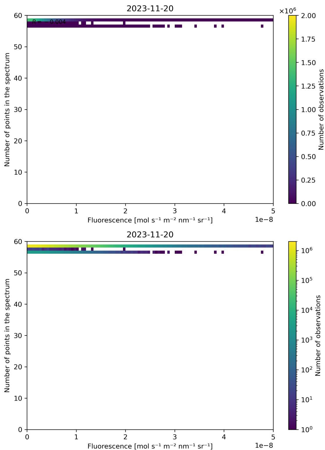
Figure 94: Scatter density plot of “Fluorescence” against “Number of points in the spectrum” for 2023-11-19 to 2023-11-21.
