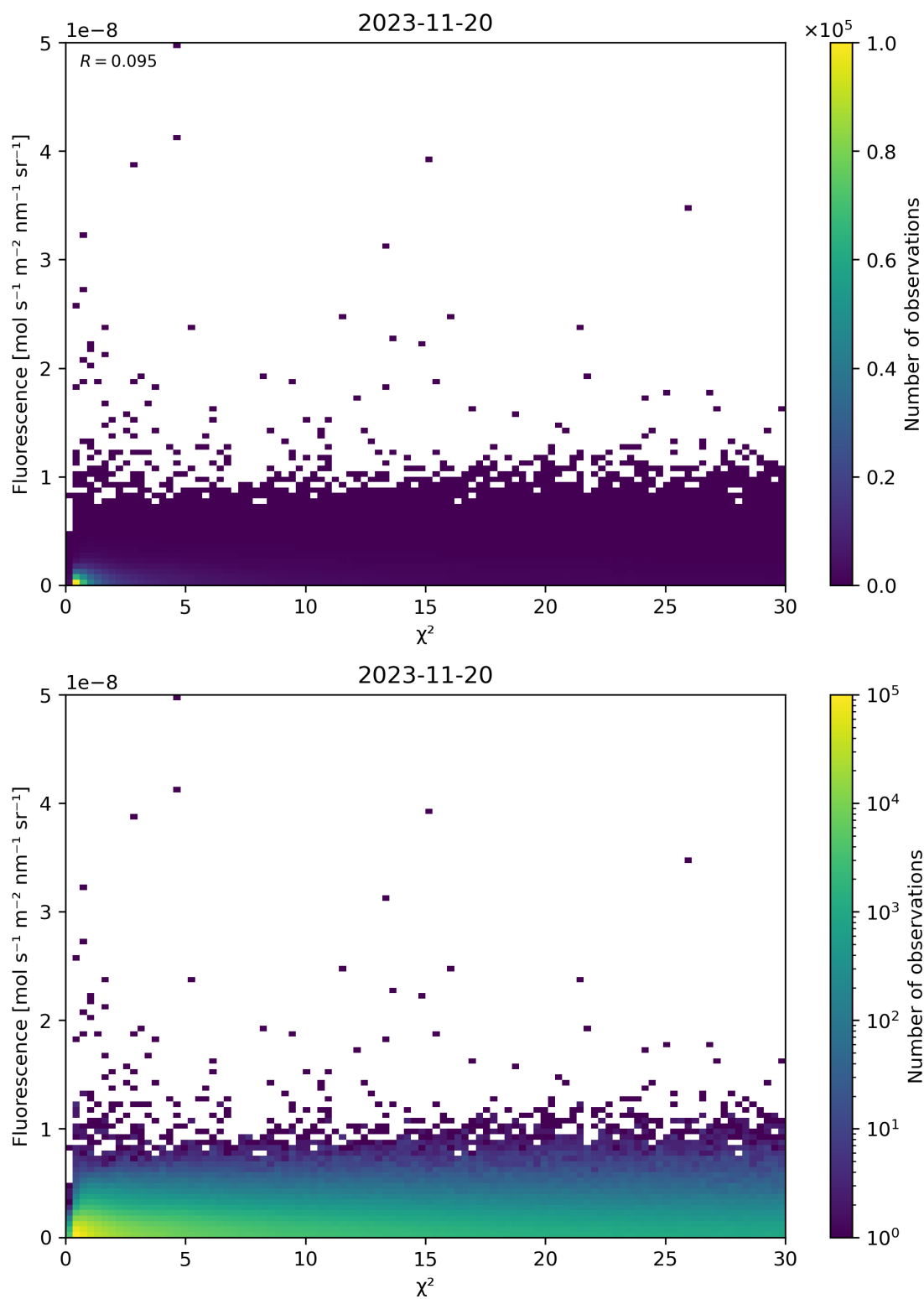
Figure 70: Scatter density plot of “ \chi^2 ” against “Fluorescence” for 2023-11-19 to 2023-11-21.
