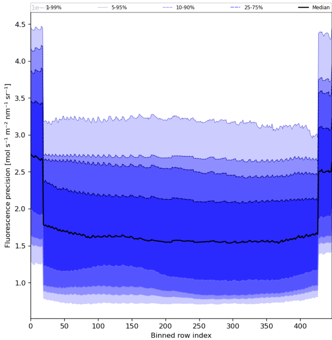
Figure 58: Along track statistics of “Fluorescence precision” for 2023-11-19 to 2023-11-21
