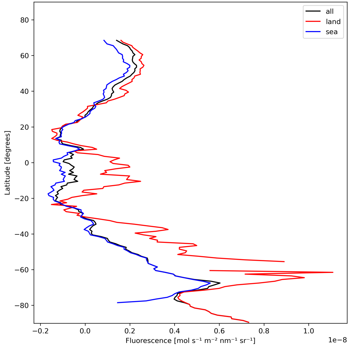
Figure 23: Zonal average of “Fluorescence” for 2023-11-19 to 2023-11-21.
