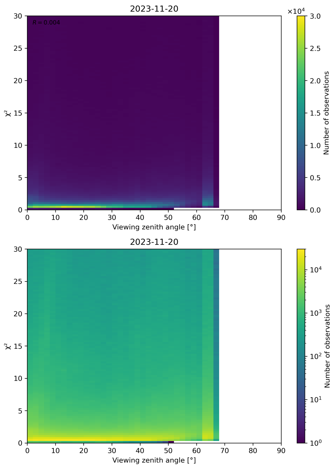
Figure 130: Scatter density plot of “Viewing zenith angle” against “ \chi^2 ” for 2023-11-19 to 2023-11-21.
