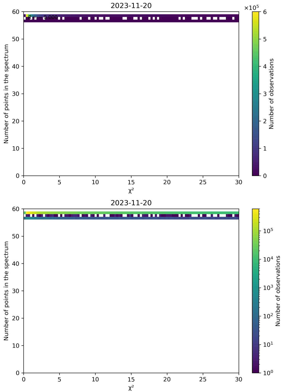
Figure 74: Scatter density plot of " \chi^2 " against "Number of points in the spectrum" for 2023-11-19 to 2023-11-21.
