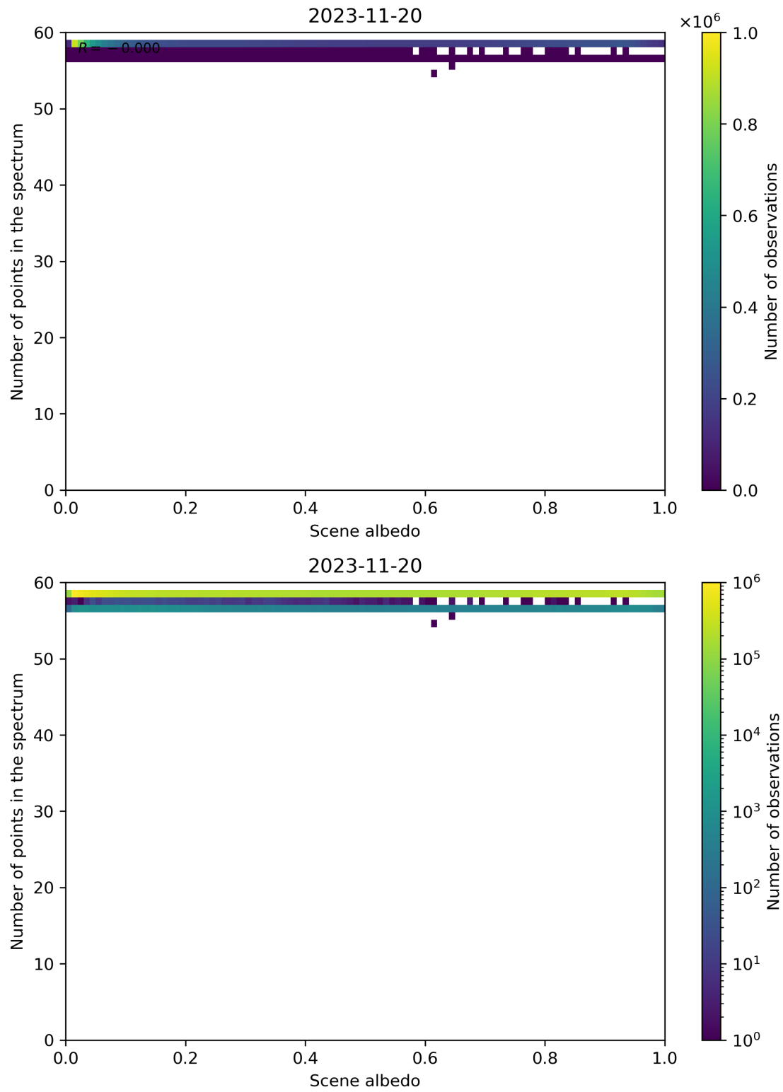
Figure 116: Scatter density plot of “Scene albedo” against “Number of points in the spectrum” for 2023-11-19 to 2023-11-21.
