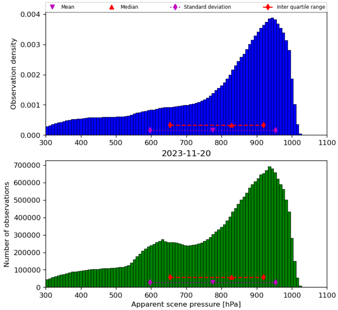
Figure 36: Histogram of “Apparent scene pressure” for 2023-11-19 to 2023-11-21
