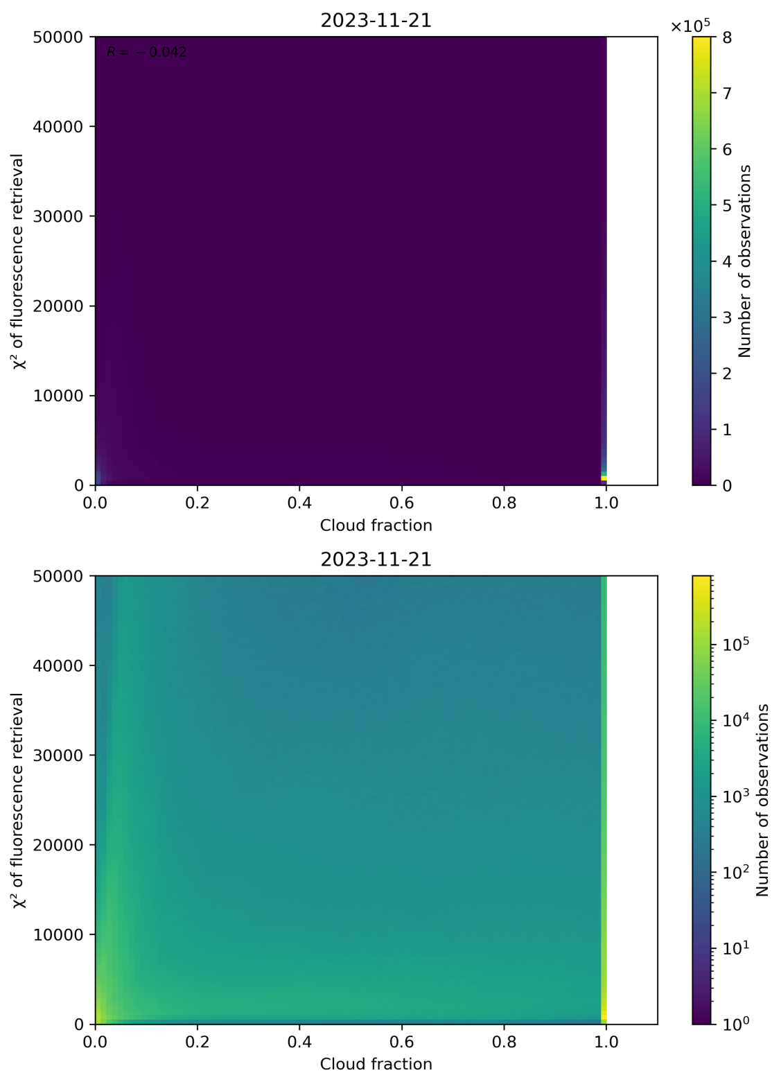
Figure 78: Scatter density plot of “Cloud fraction” against “ \chi^2 of fluorescence retrieval” for 2023-11-20 to 2023-11-22.
