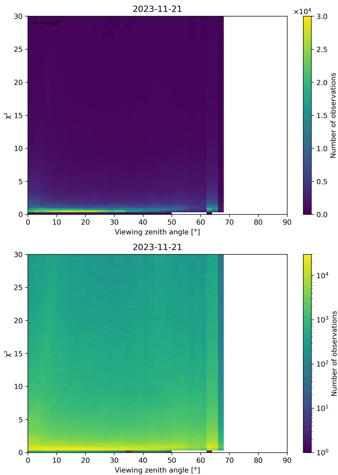
Figure 130: Scatter density plot of “Viewing zenith angle” against “ \chi^2 ” for 2023-11-20 to 2023-11-22.
