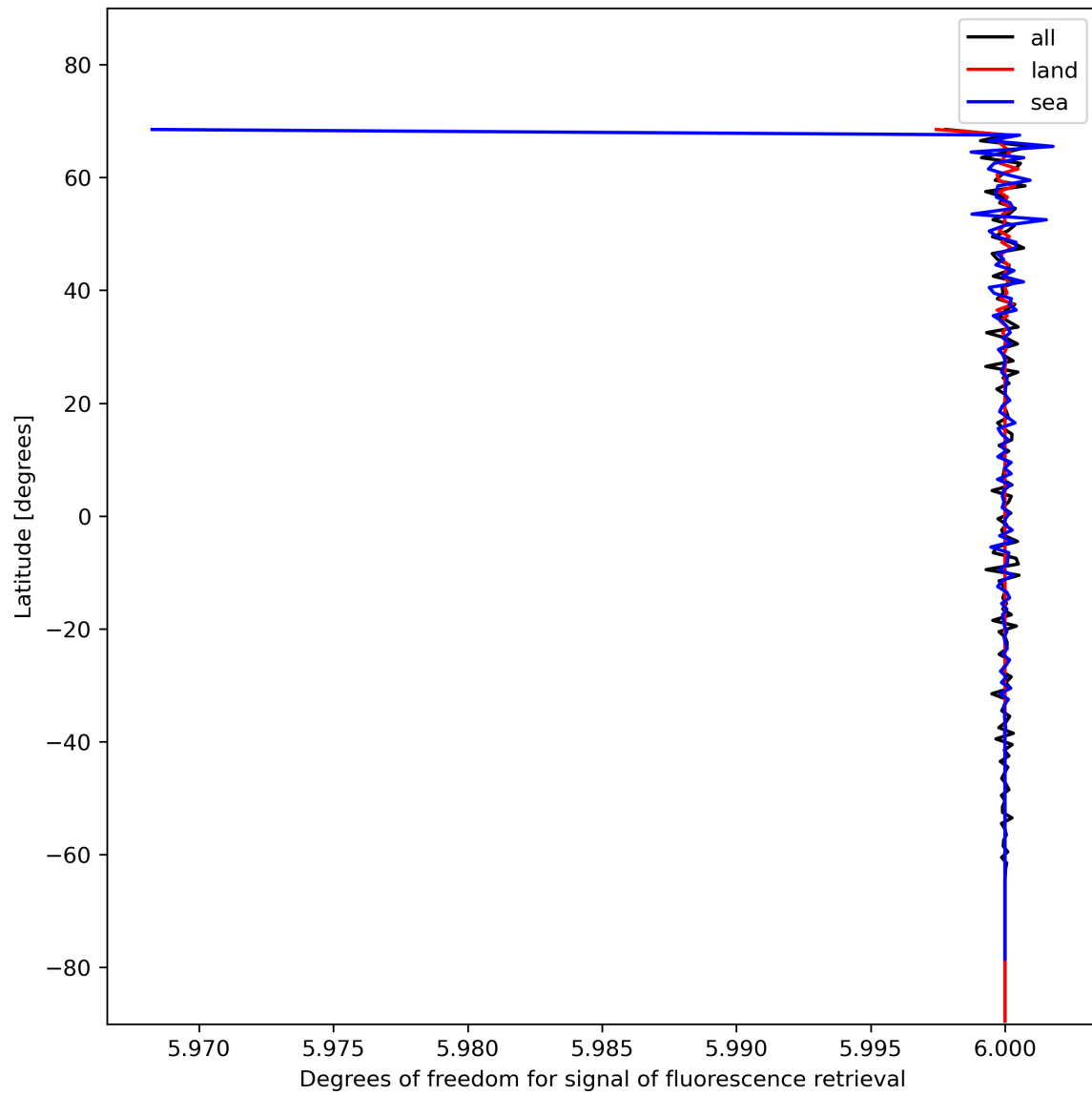
Figure 26: Zonal average of “Degrees of freedom for signal of fluorescence retrieval” for 2023-11-20 to 2023-11-22.
