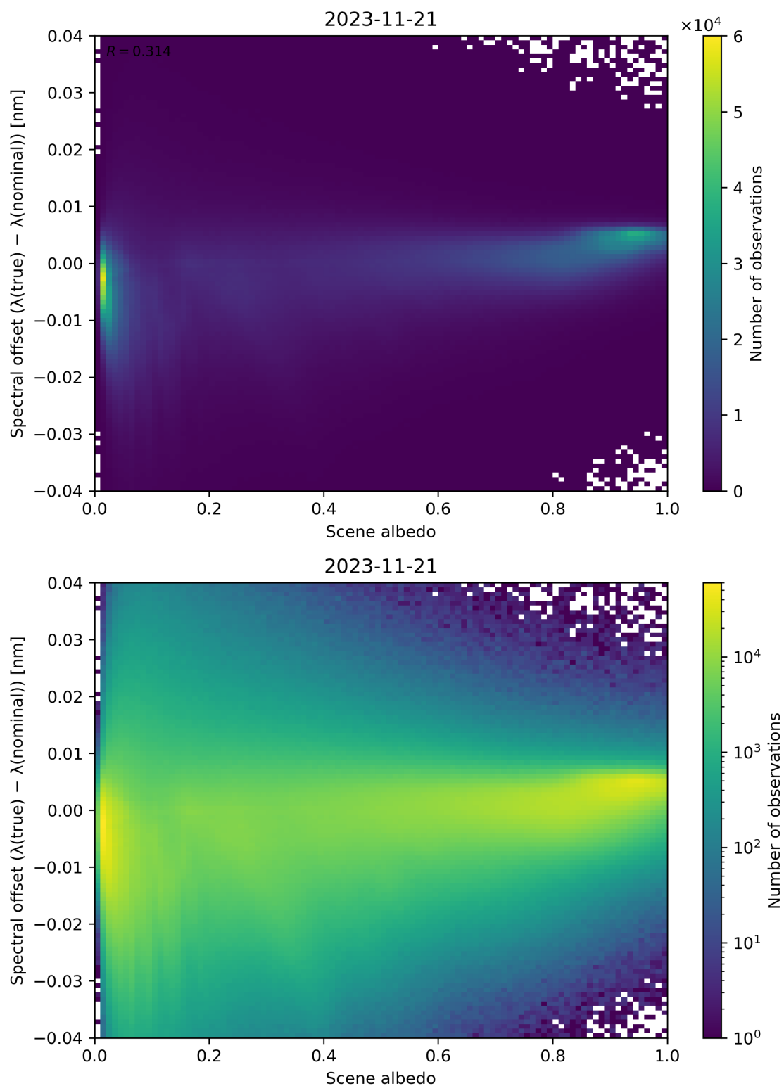
Figure 117: Scatter density plot of “Scene albedo” against “Spectral offset ( \lambda(\text{true}) - \lambda(\text{nominal}) )” for 2023-11-20 to 2023-11-22.
