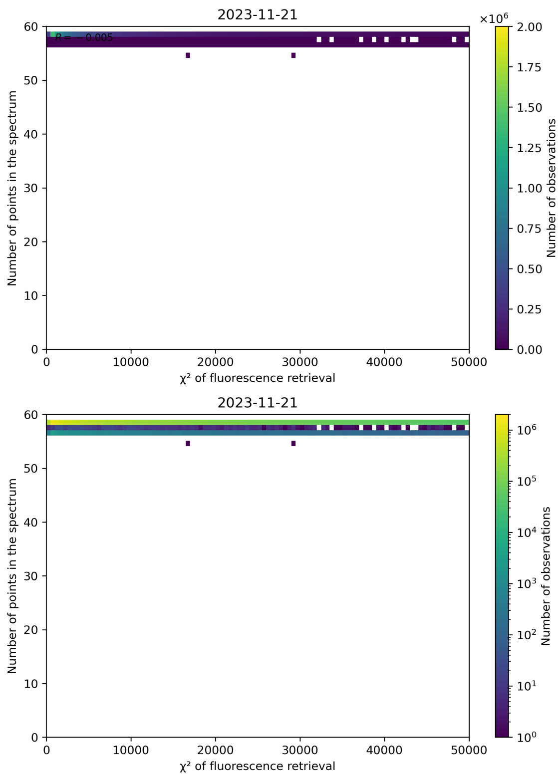
Figure 71: Scatter density plot of “ \chi^2 of fluorescence retrieval” against “Number of points in the spectrum” for 2023-11-20 to 2023-11-22.
