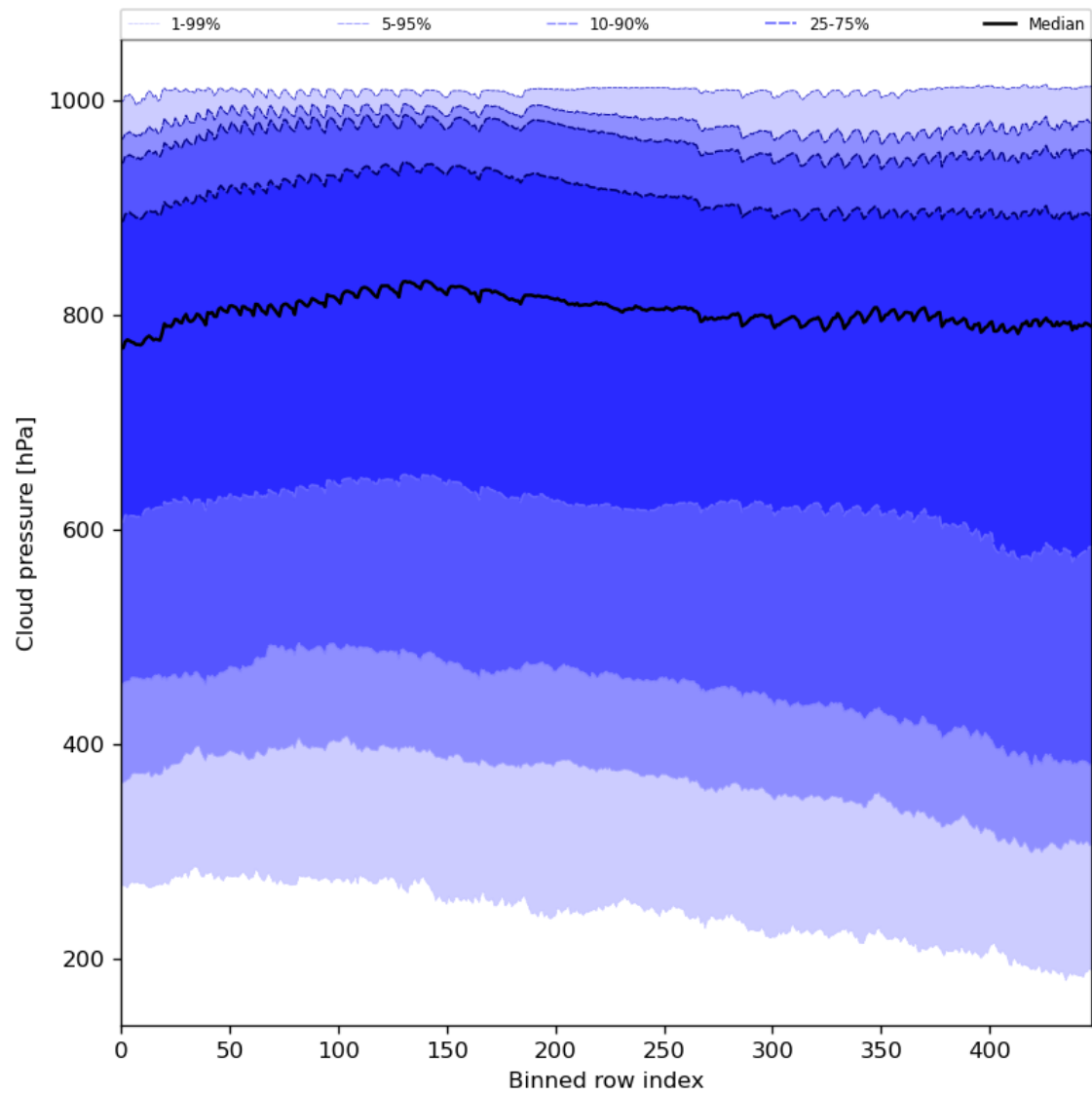
Figure 47: Along track statistics of “Cloud pressure” for 2023-11-20 to 2023-11-22
