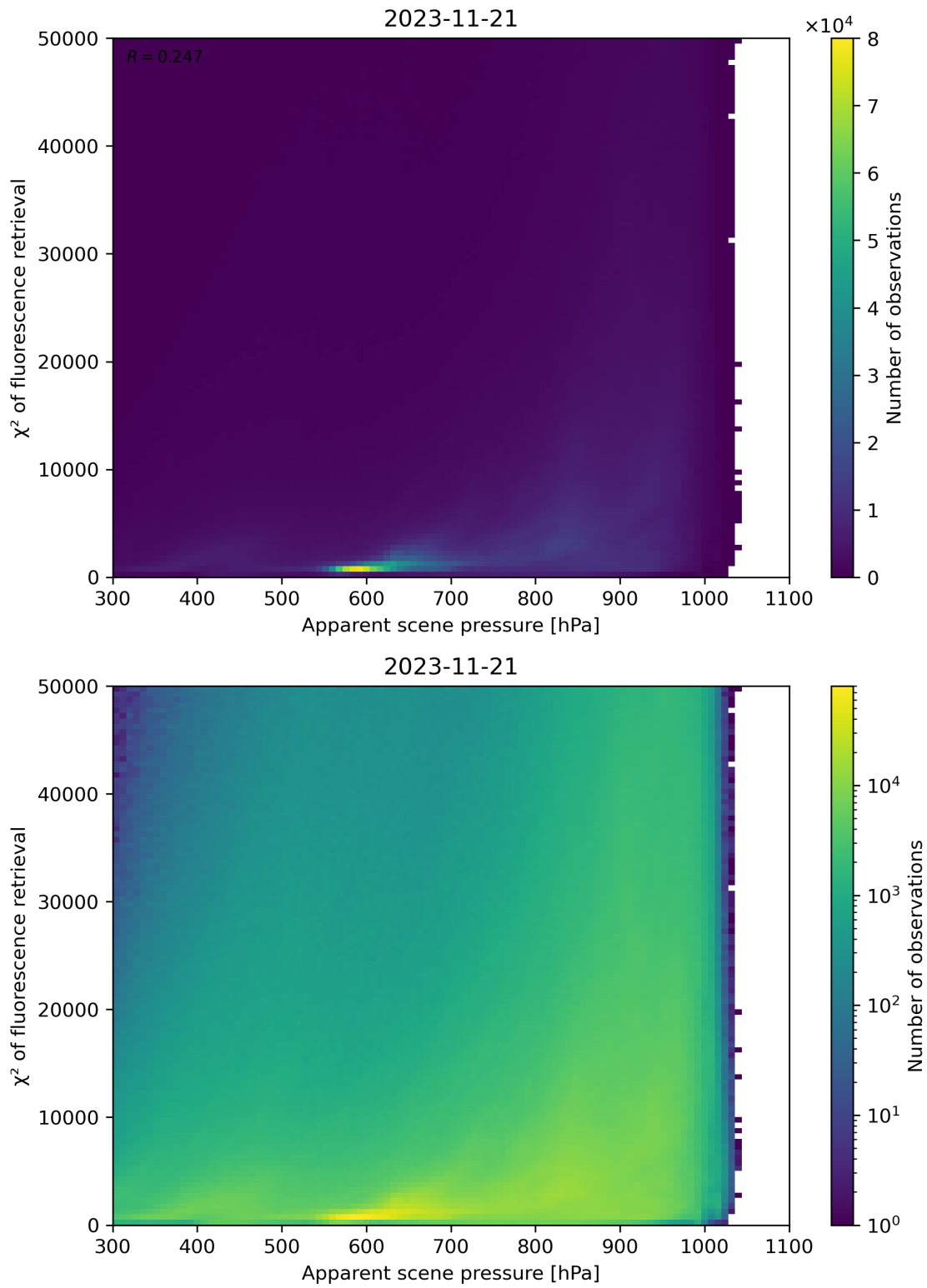
Figure 64: Scatter density plot of “Apparent scene pressure” against “ \chi^2 of fluorescence retrieval” for 2023-11-20 to 2023-11-22.
