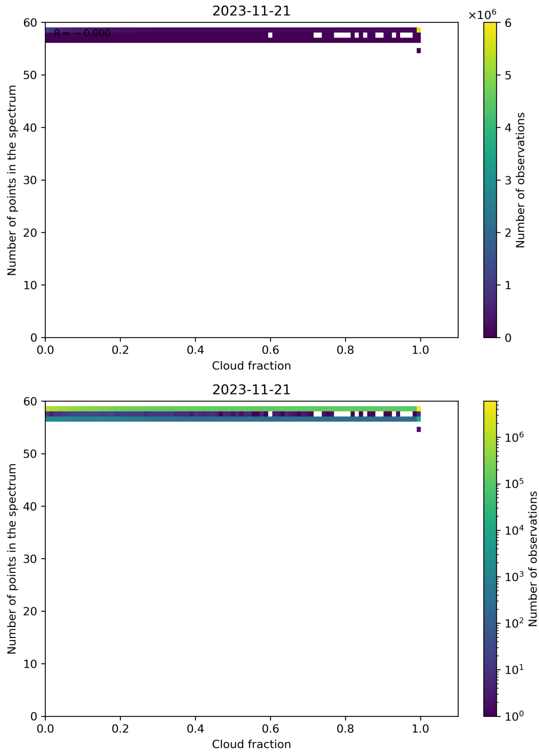
Figure 81: Scatter density plot of “Cloud fraction” against “Number of points in the spectrum” for 2023-11-20 to 2023-11-22.
