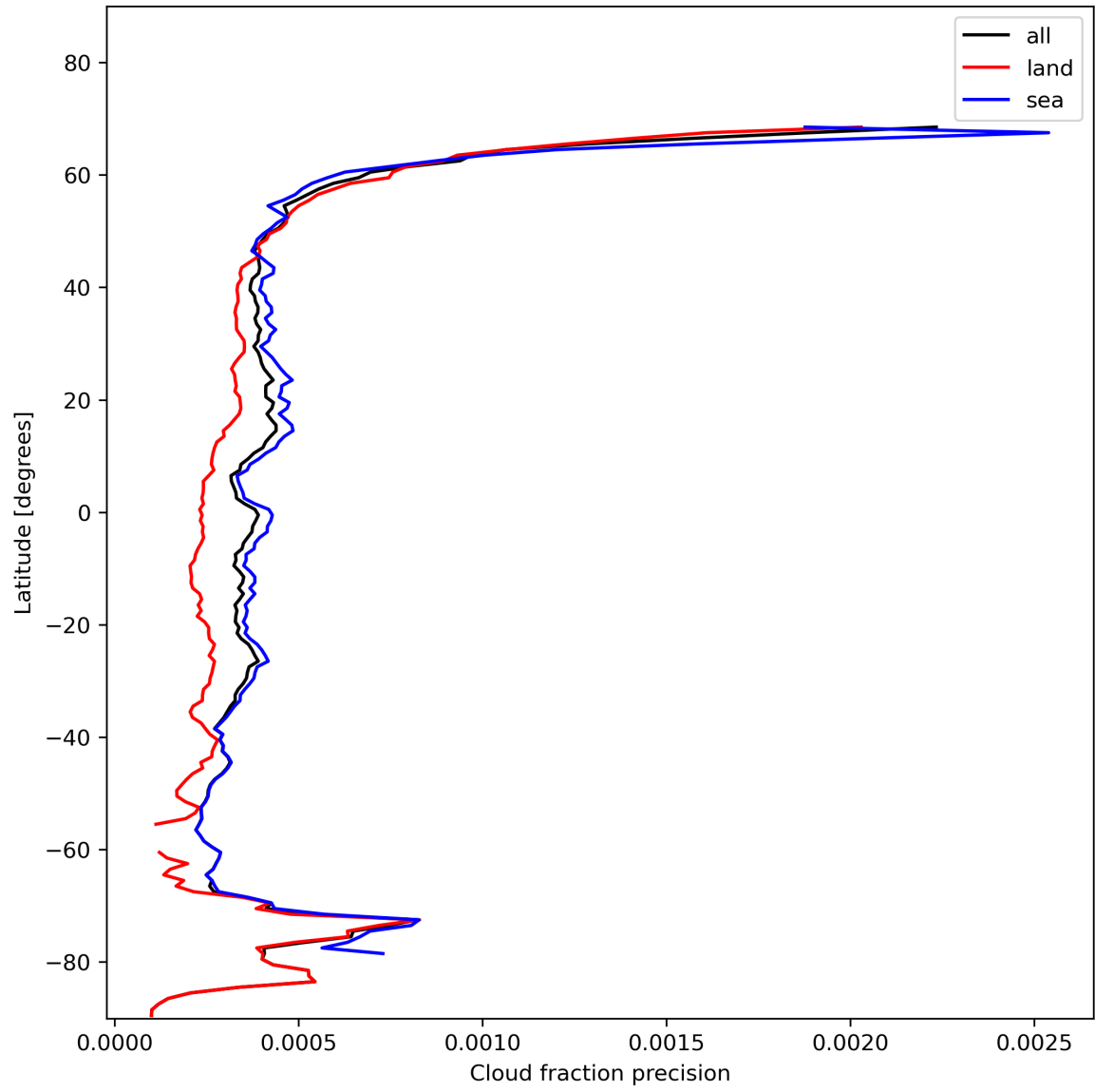
Figure 16: Zonal average of “Cloud fraction precision” for 2023-11-20 to 2023-11-22.
