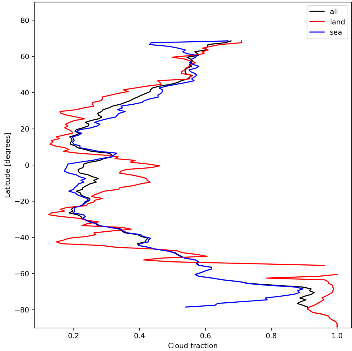
Figure 15: Zonal average of “Cloud fraction” for 2023-11-20 to 2023-11-22.
