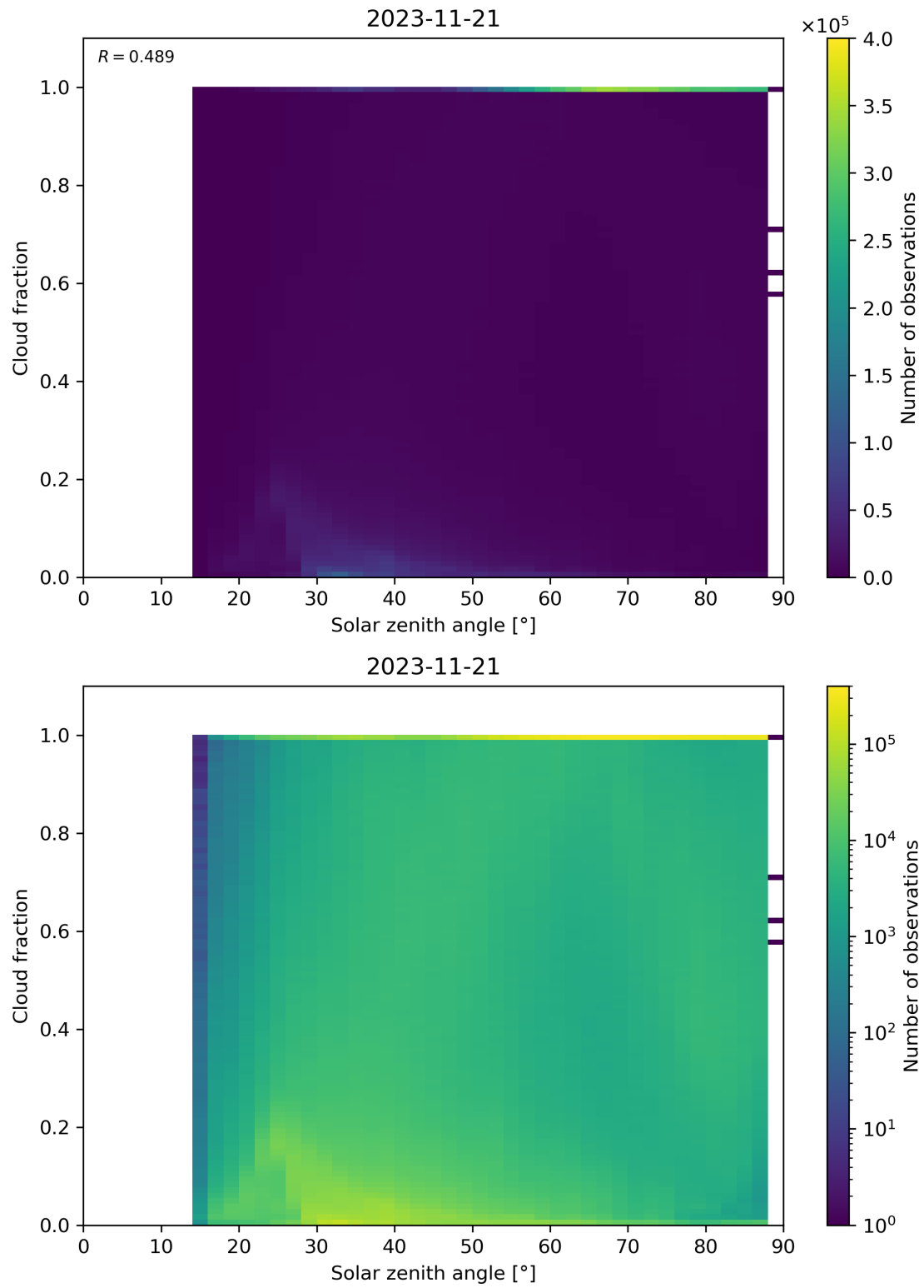
Figure 121: Scatter density plot of “Solar zenith angle” against “Cloud fraction” for 2023-11-20 to 2023-11-22.
