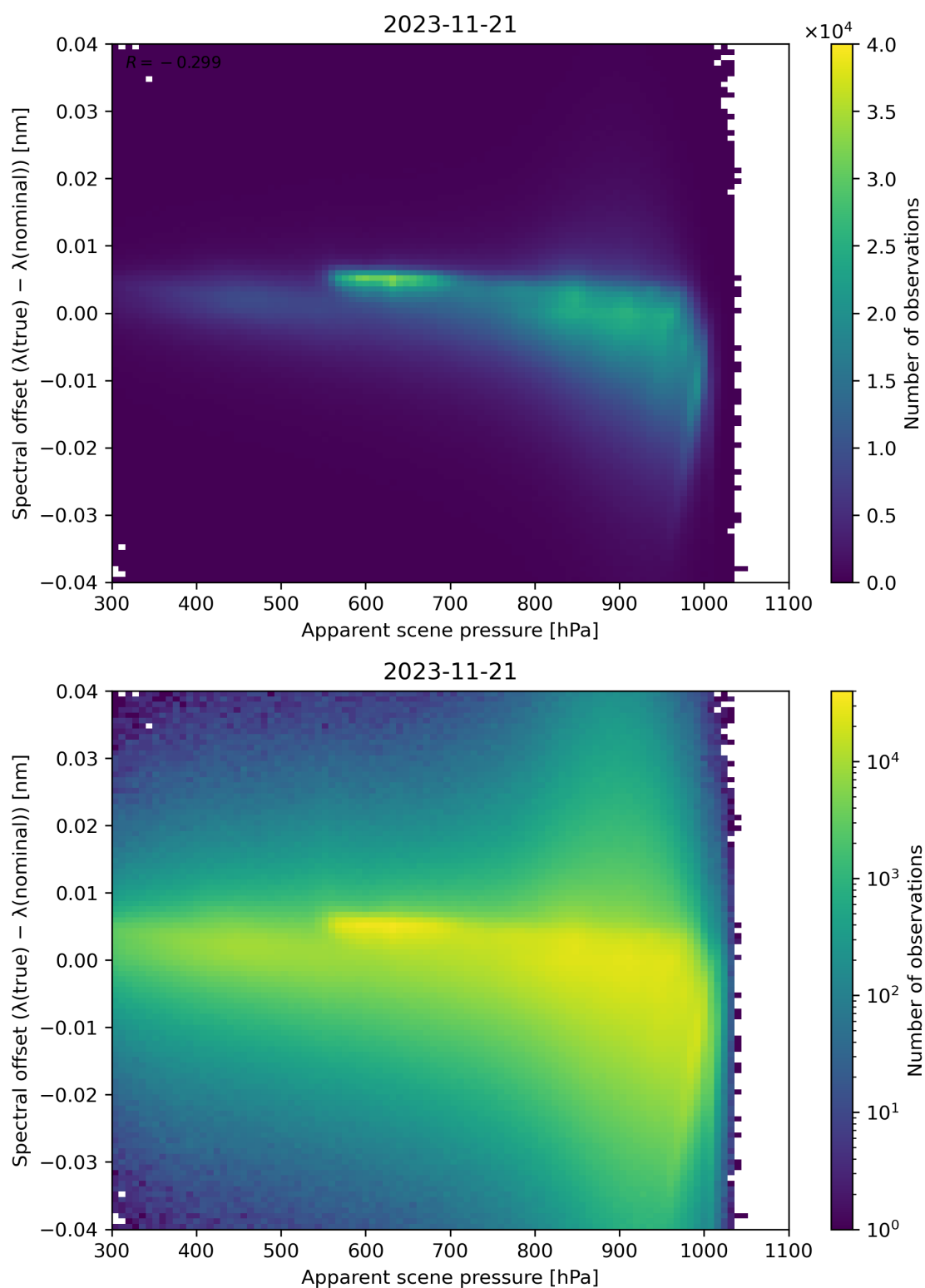
Figure 68: Scatter density plot of “Apparent scene pressure” against “Spectral offset ( \lambda(\text{true}) - \lambda(\text{nominal}) )” for 2023-11-20 to 2023-11-22.
