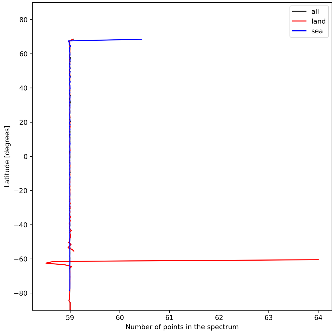
Figure 27: Zonal average of “Number of points in the spectrum” for 2023-11-20 to 2023-11-22.
