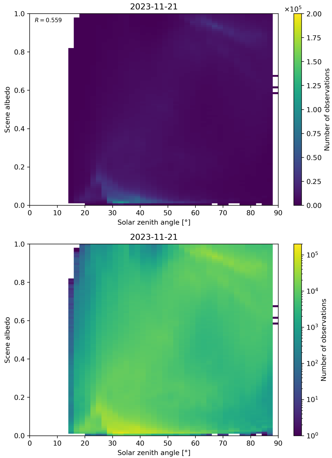
Figure 127: Scatter density plot of “Solar zenith angle” against “Scene albedo” for 2023-11-20 to 2023-11-22.
