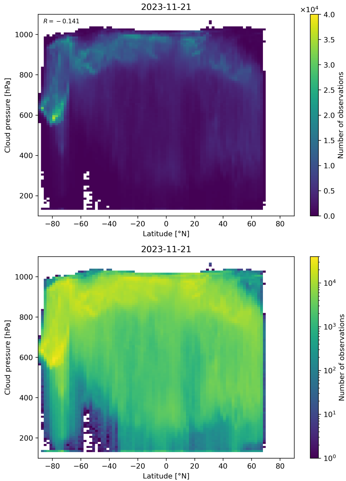
Figure 100: Scatter density plot of “Latitude” against “Cloud pressure” for 2023-11-20 to 2023-11-22.
