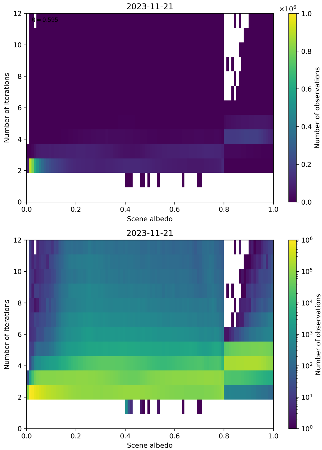
Figure 115: Scatter density plot of “Scene albedo” against “Number of iterations” for 2023-11-20 to 2023-11-22.
