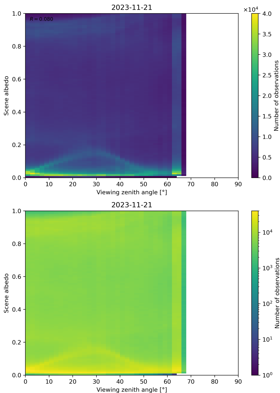
Figure 138: Scatter density plot of “Viewing zenith angle” against “Scene albedo” for 2023-11-20 to 2023-11-22.
