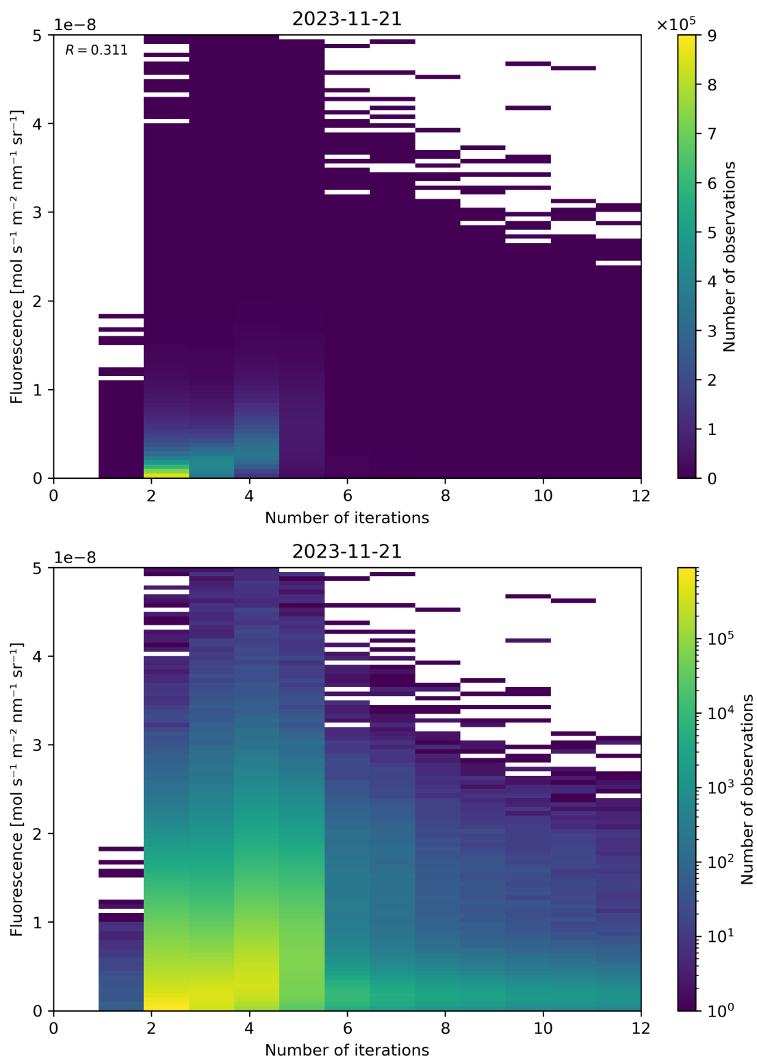
Figure 107: Scatter density plot of “Number of iterations” against “Fluorescence” for 2023-11-20 to 2023-11-22.
