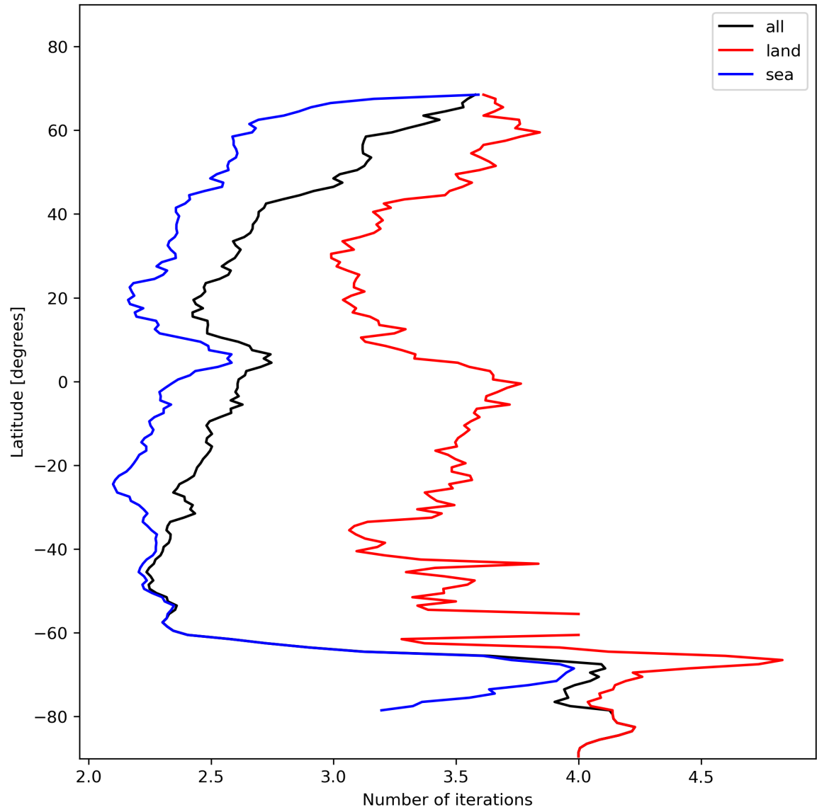
Figure 22: Zonal average of “Number of iterations” for 2023-11-20 to 2023-11-22.
