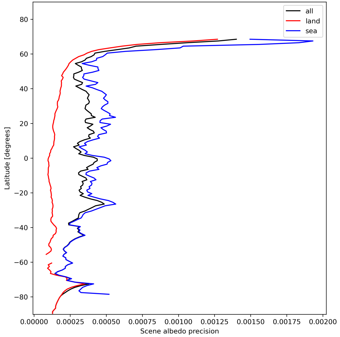
Figure 18: Zonal average of “Scene albedo precision” for 2023-11-20 to 2023-11-22.
