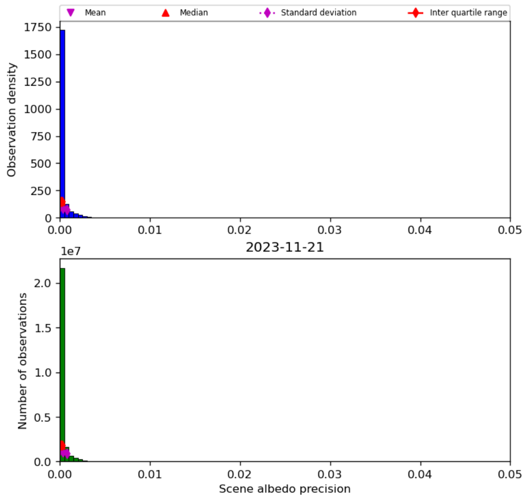
Figure 35: Histogram of “Scene albedo precision” for 2023-11-20 to 2023-11-22
