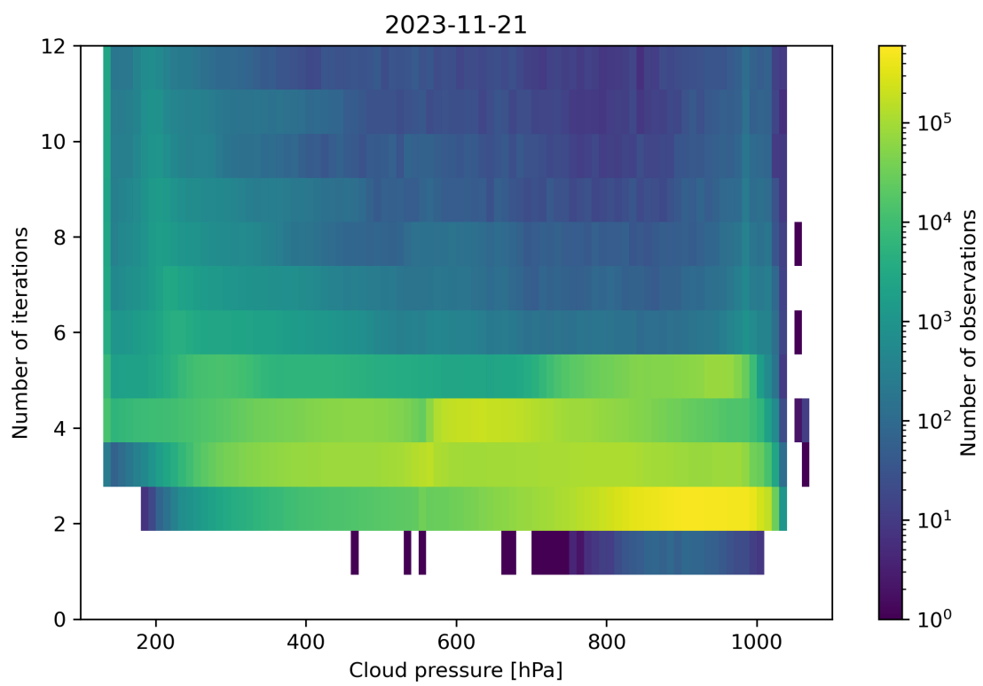
Figure 89: Scatter density plot of “Cloud pressure” against “Number of iterations” for 2023-11-20 to 2023-11-22.
