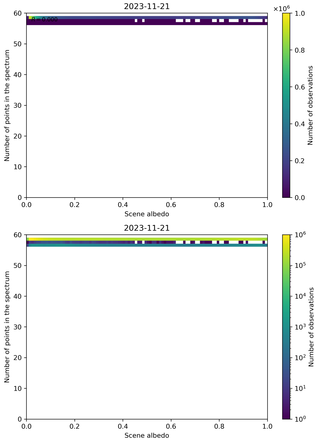
Figure 116: Scatter density plot of “Scene albedo” against “Number of points in the spectrum” for 2023-11-20 to 2023-11-22.
