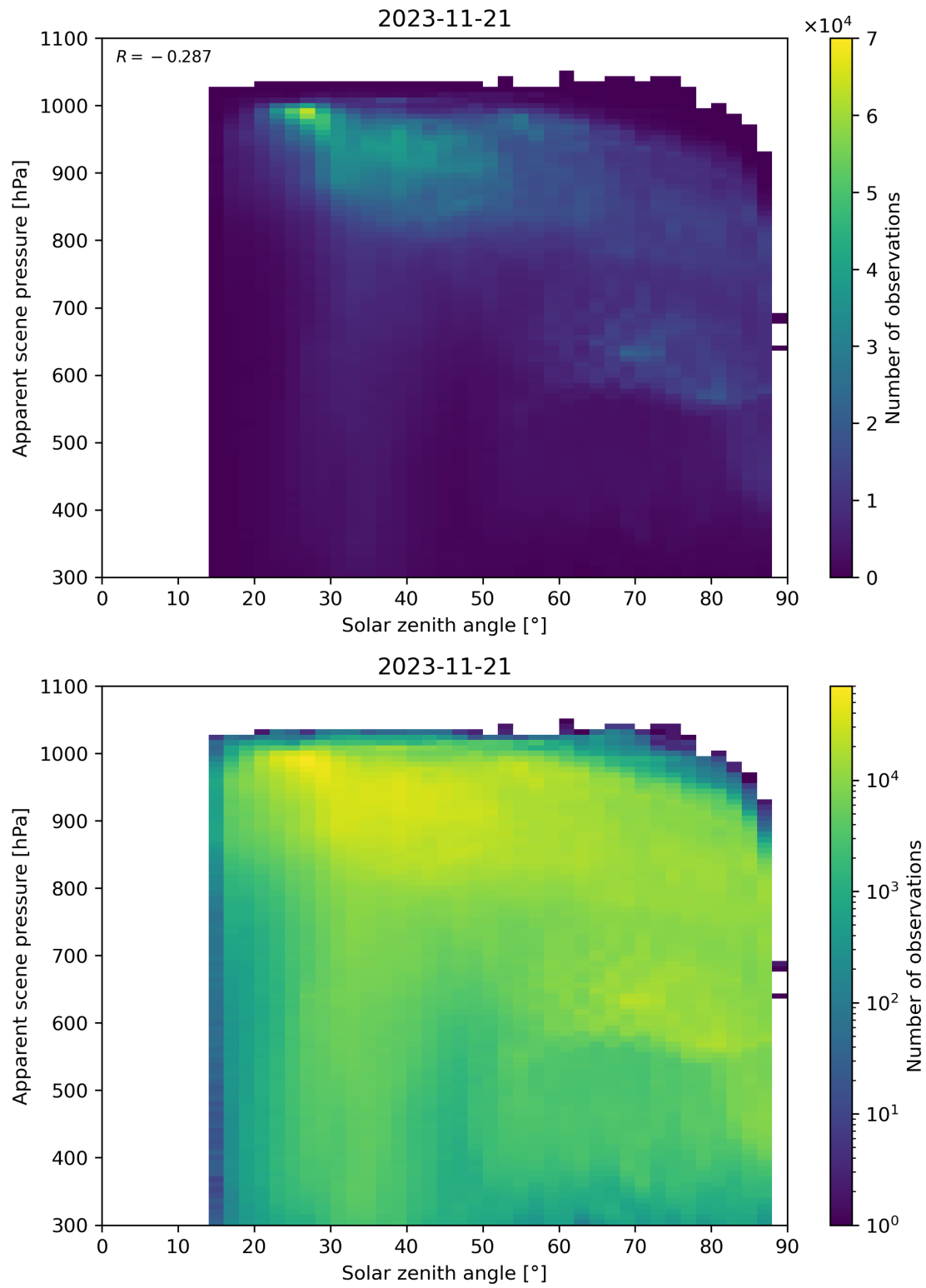
Figure 118: Scatter density plot of “Solar zenith angle” against “Apparent scene pressure” for 2023-11-20 to 2023-11-22.
