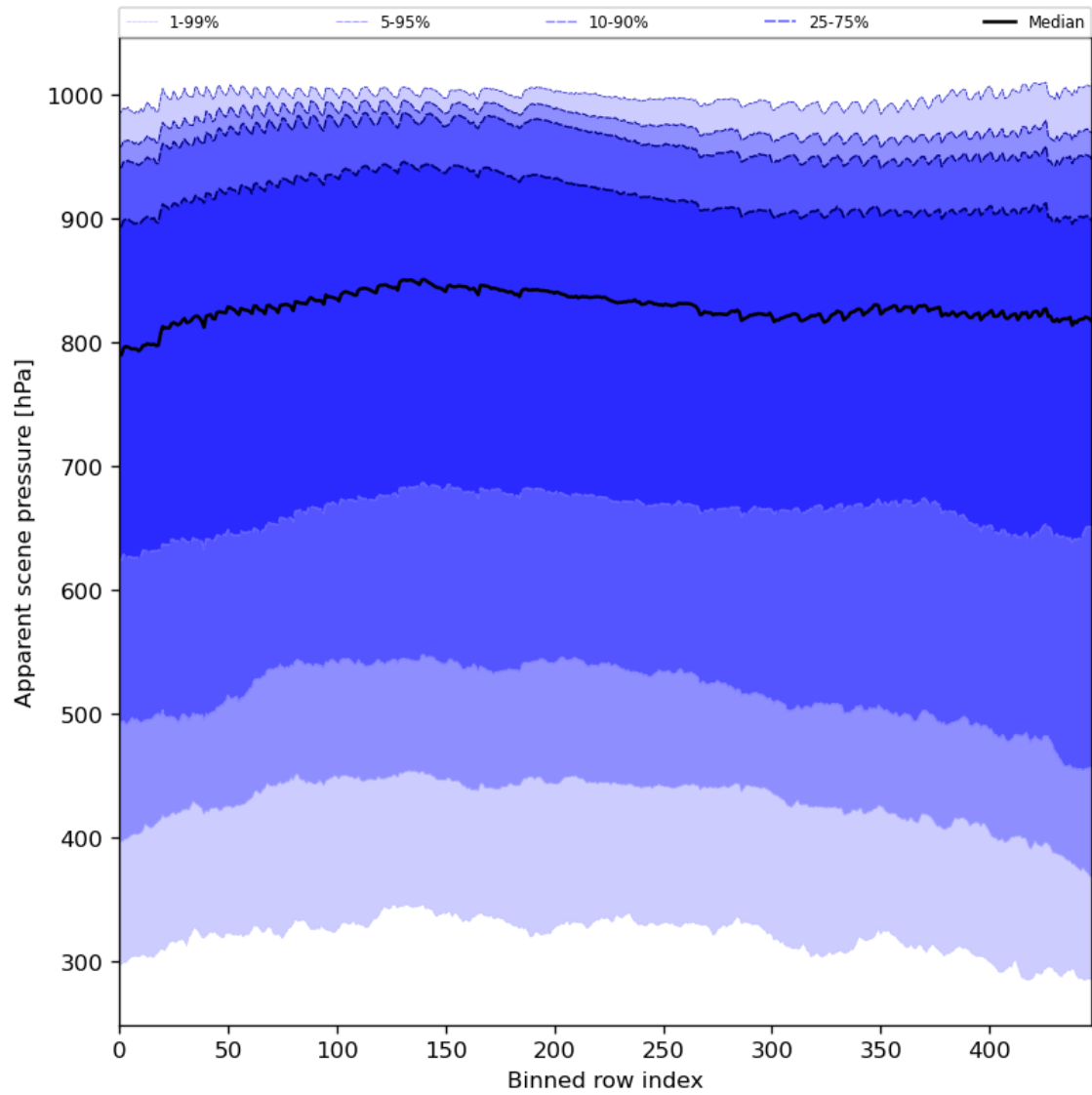
Figure 53: Along track statistics of “Apparent scene pressure” for 2023-11-20 to 2023-11-22
