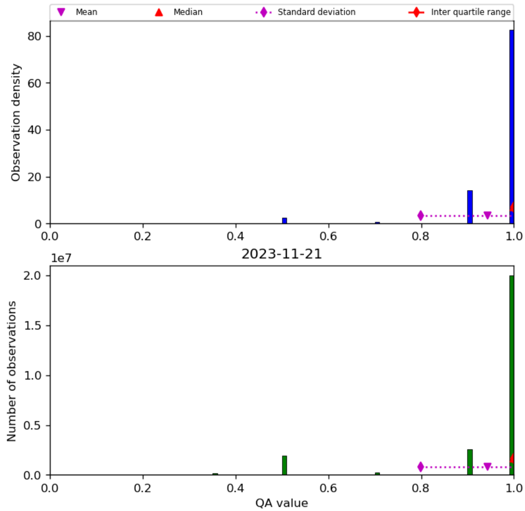
Figure 29: Histogram of “QA value” for 2023-11-20 to 2023-11-22
