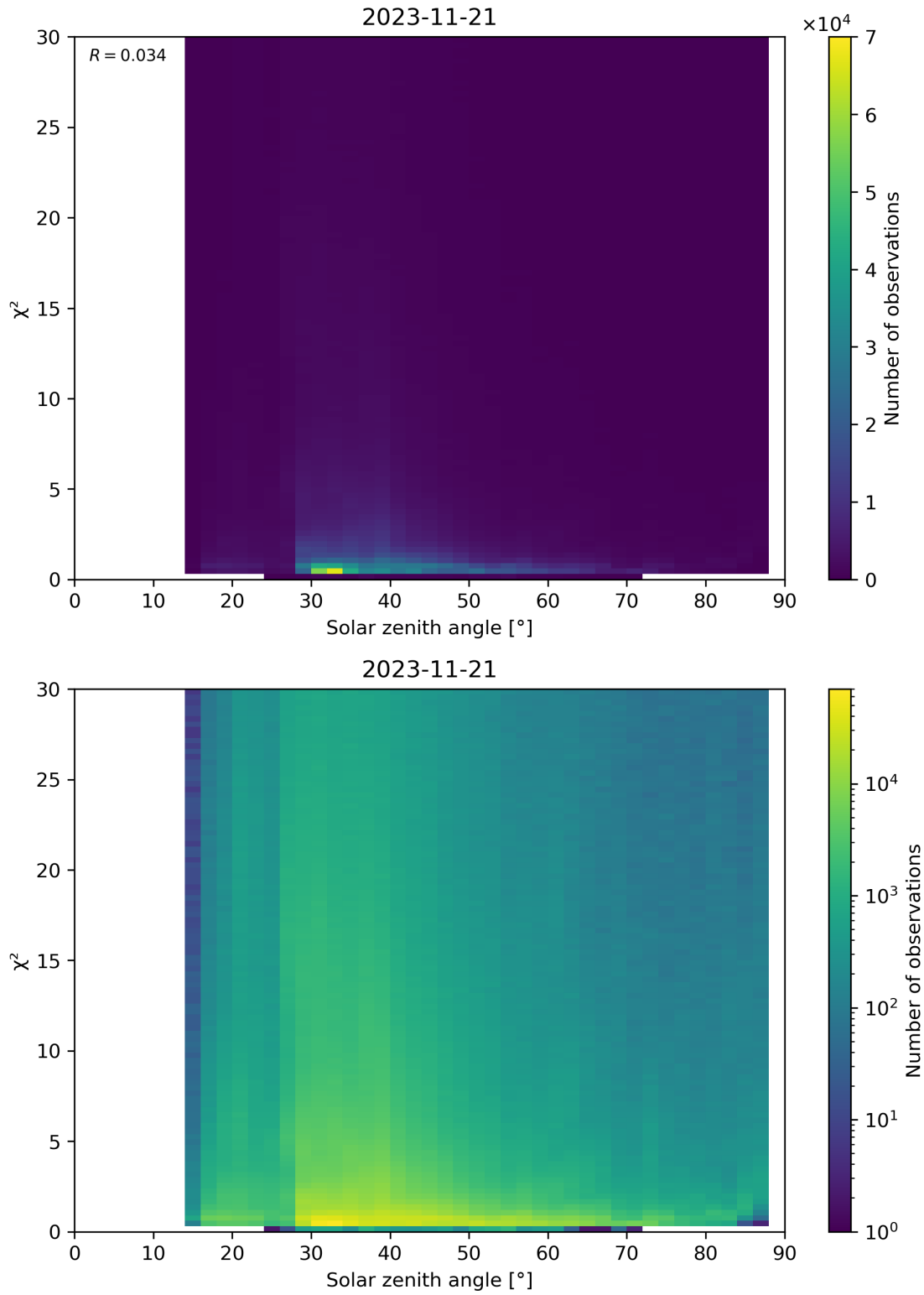
Figure 119: Scatter density plot of “Solar zenith angle” against “ \chi^2 ” for 2023-11-20 to 2023-11-22.
