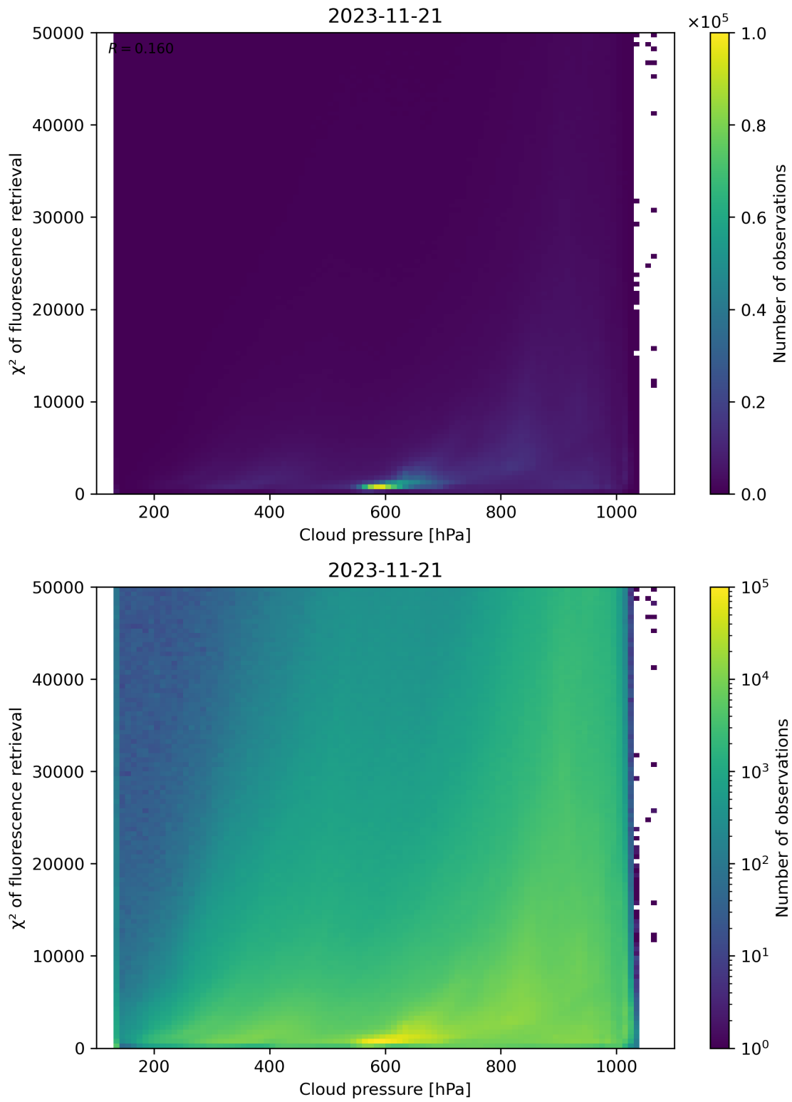
Figure 86: Scatter density plot of “Cloud pressure” against “ \chi^2 of fluorescence retrieval” for 2023-11-20 to 2023-11-22.
