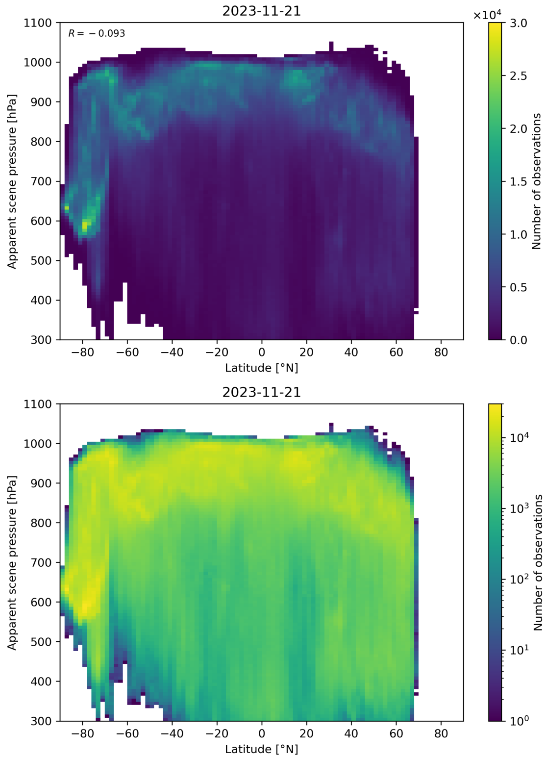
Figure 96: Scatter density plot of “Latitude” against “Apparent scene pressure” for 2023-11-20 to 2023-11-22.
