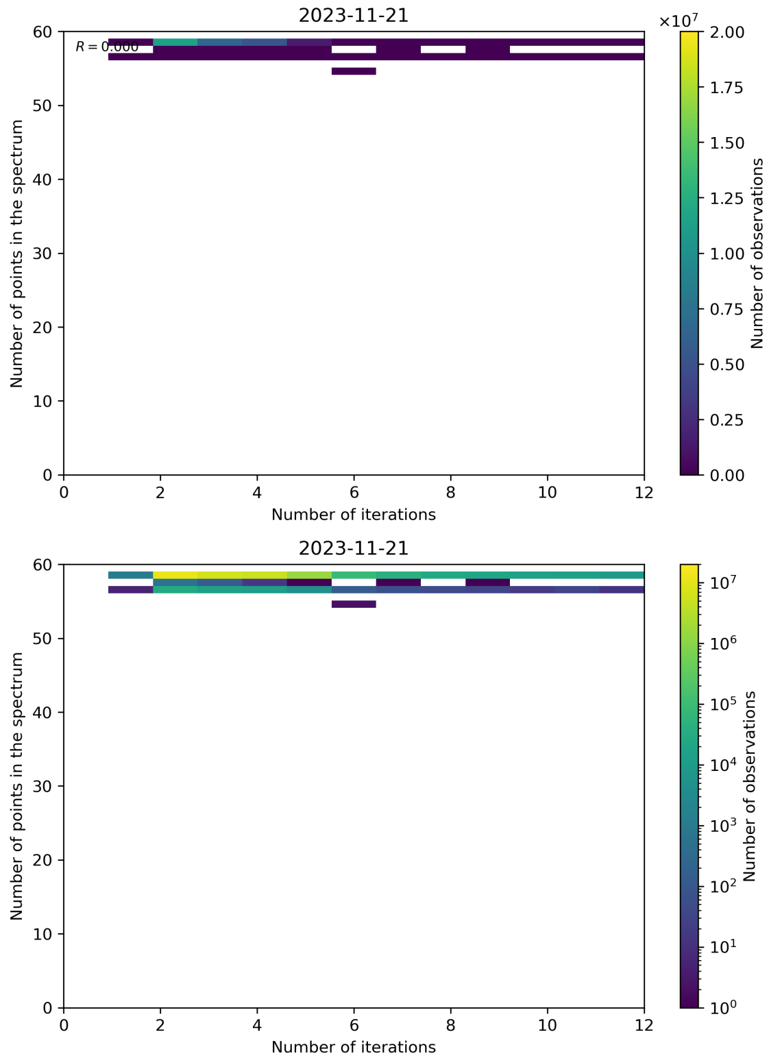
Figure 108: Scatter density plot of “Number of iterations” against “Number of points in the spectrum” for 2023-11-20 to 2023-11-22.
