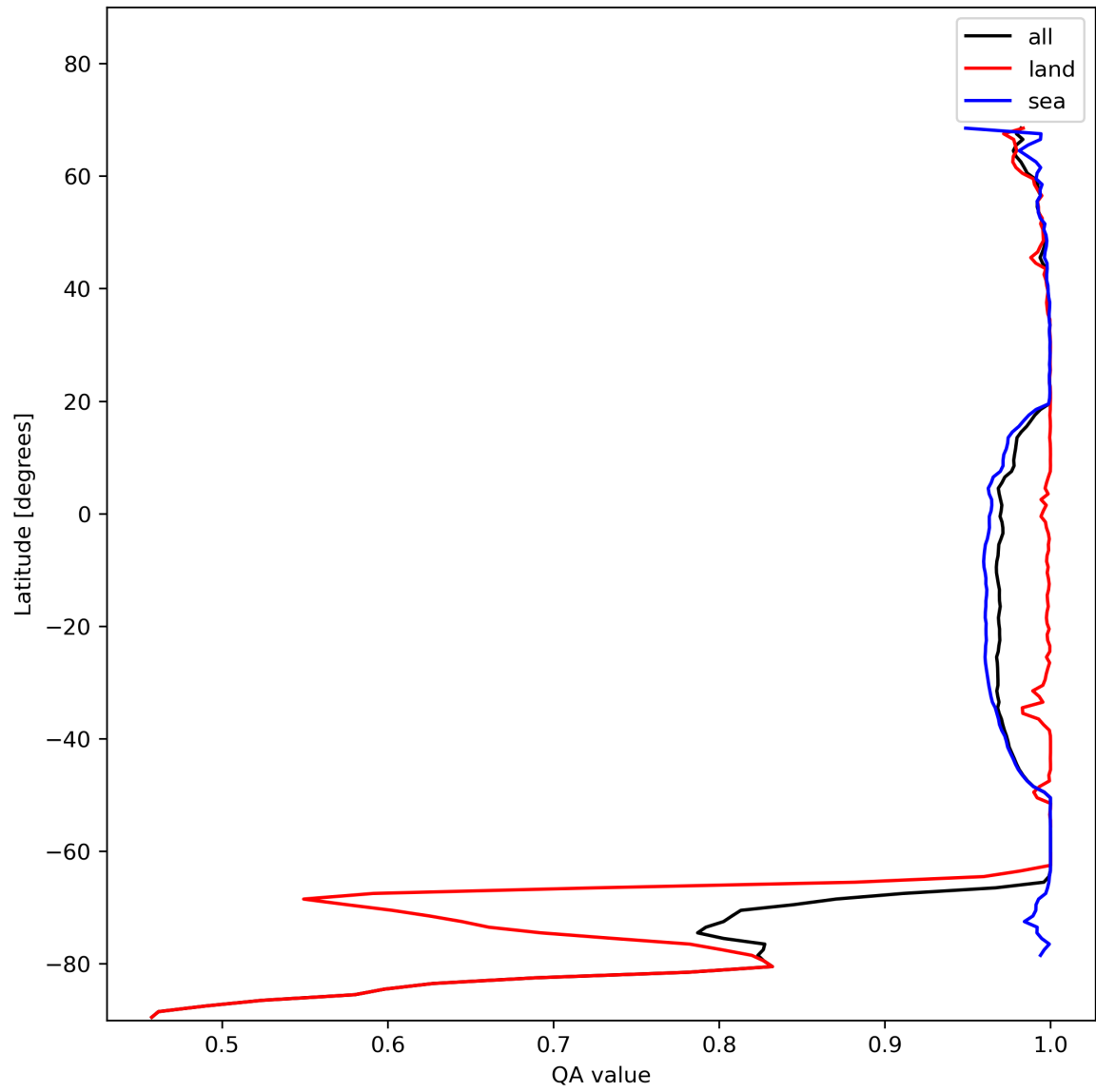
Figure 12: Zonal average of “QA value” for 2023-11-20 to 2023-11-22.
