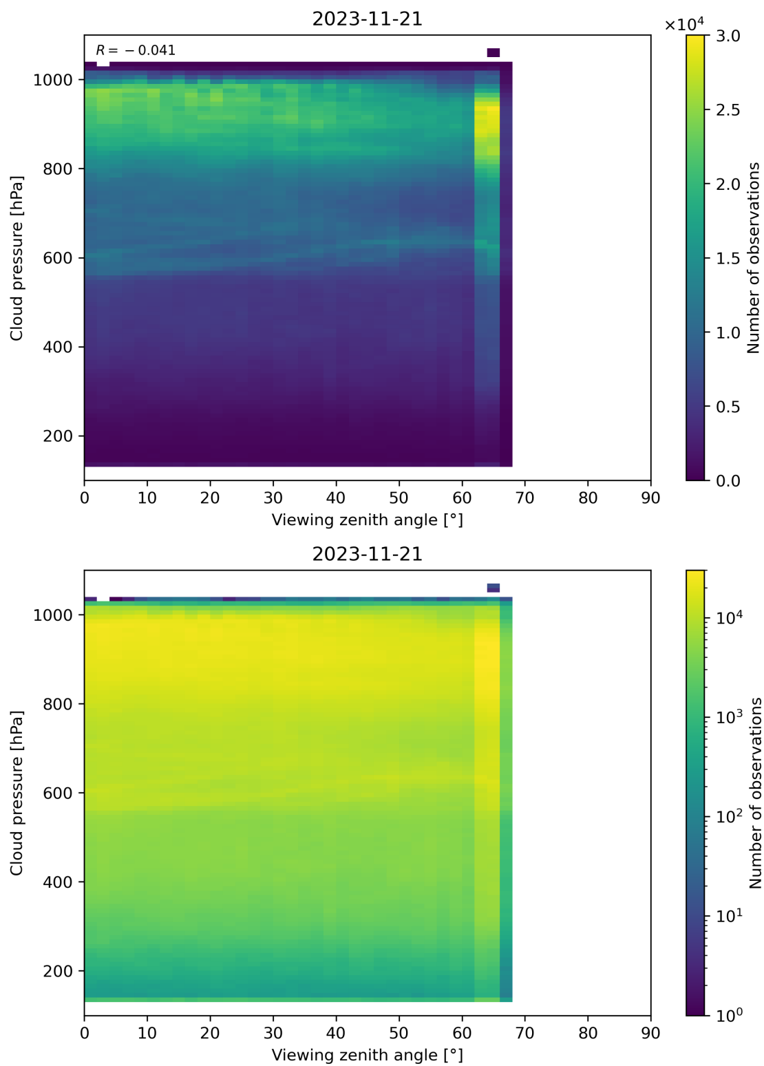
Figure 133: Scatter density plot of “Viewing zenith angle” against “Cloud pressure” for 2023-11-20 to 2023-11-22.
