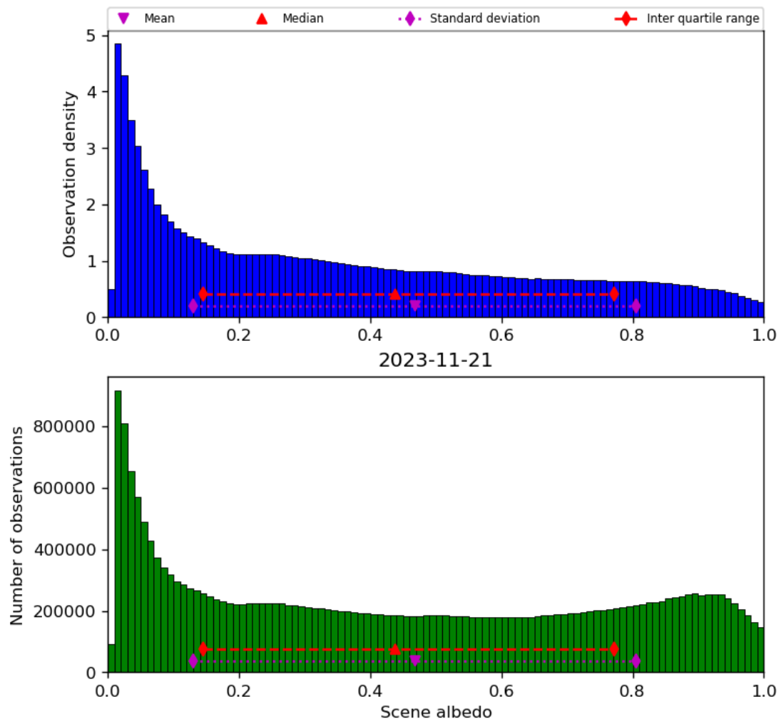
Figure 34: Histogram of “Scene albedo” for 2023-11-20 to 2023-11-22
