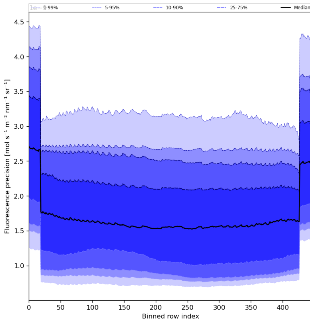
Figure 58: Along track statistics of “Fluorescence precision” for 2023-11-20 to 2023-11-22
