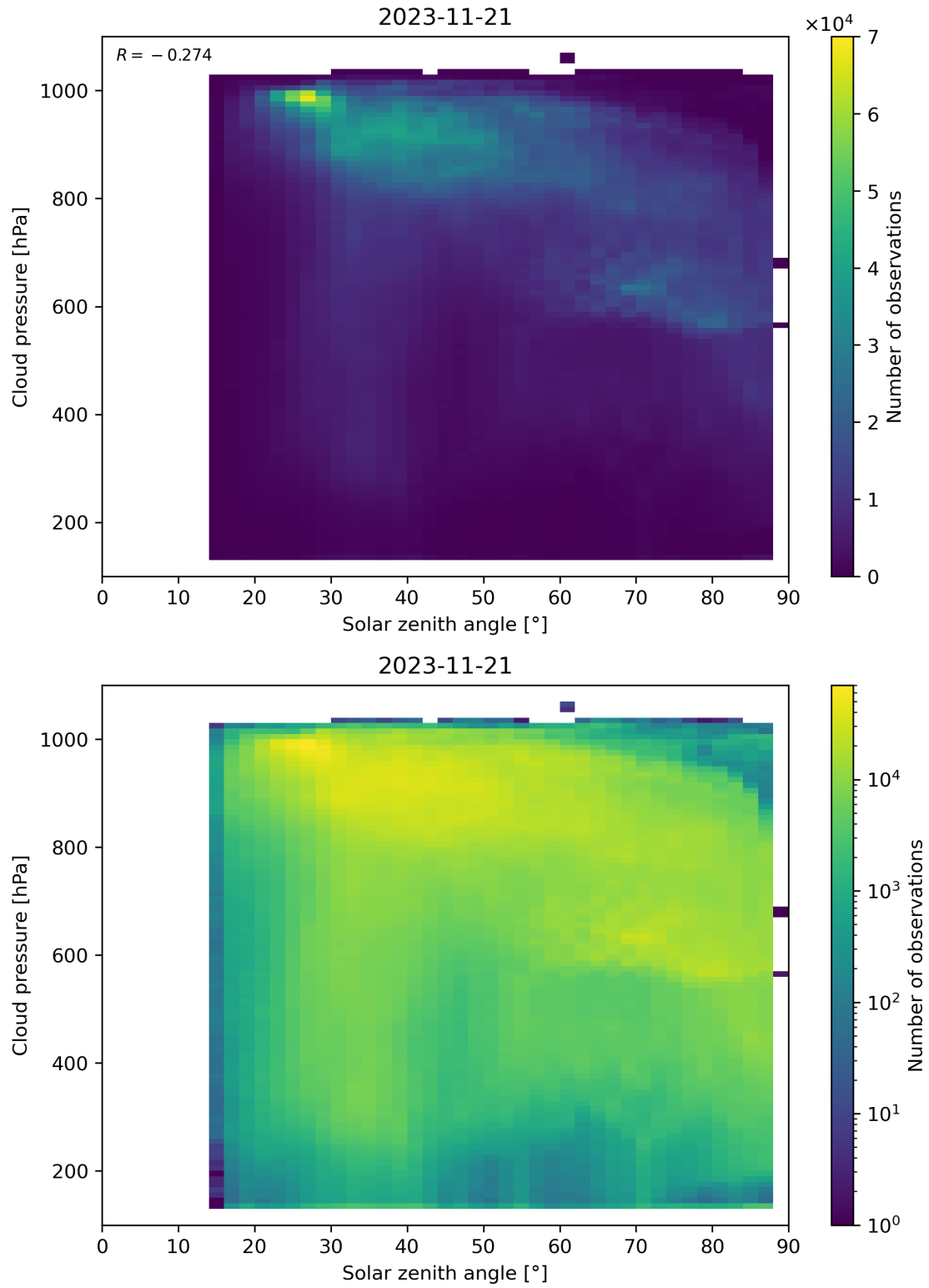
Figure 122: Scatter density plot of “Solar zenith angle” against “Cloud pressure” for 2023-11-20 to 2023-11-22.
