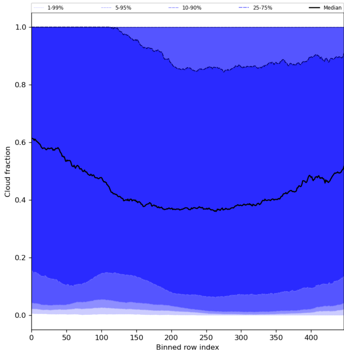
Figure 49: Along track statistics of “Cloud fraction” for 2023-11-20 to 2023-11-22
