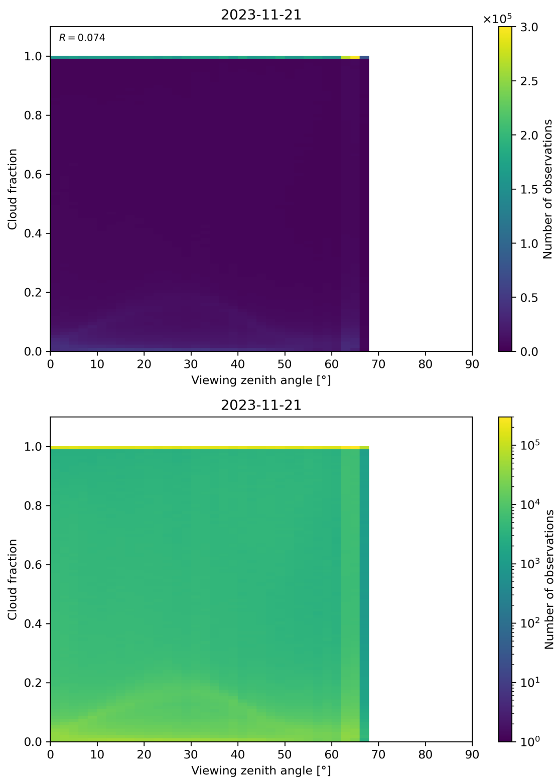
Figure 132: Scatter density plot of “Viewing zenith angle” against “Cloud fraction” for 2023-11-20 to 2023-11-22.
