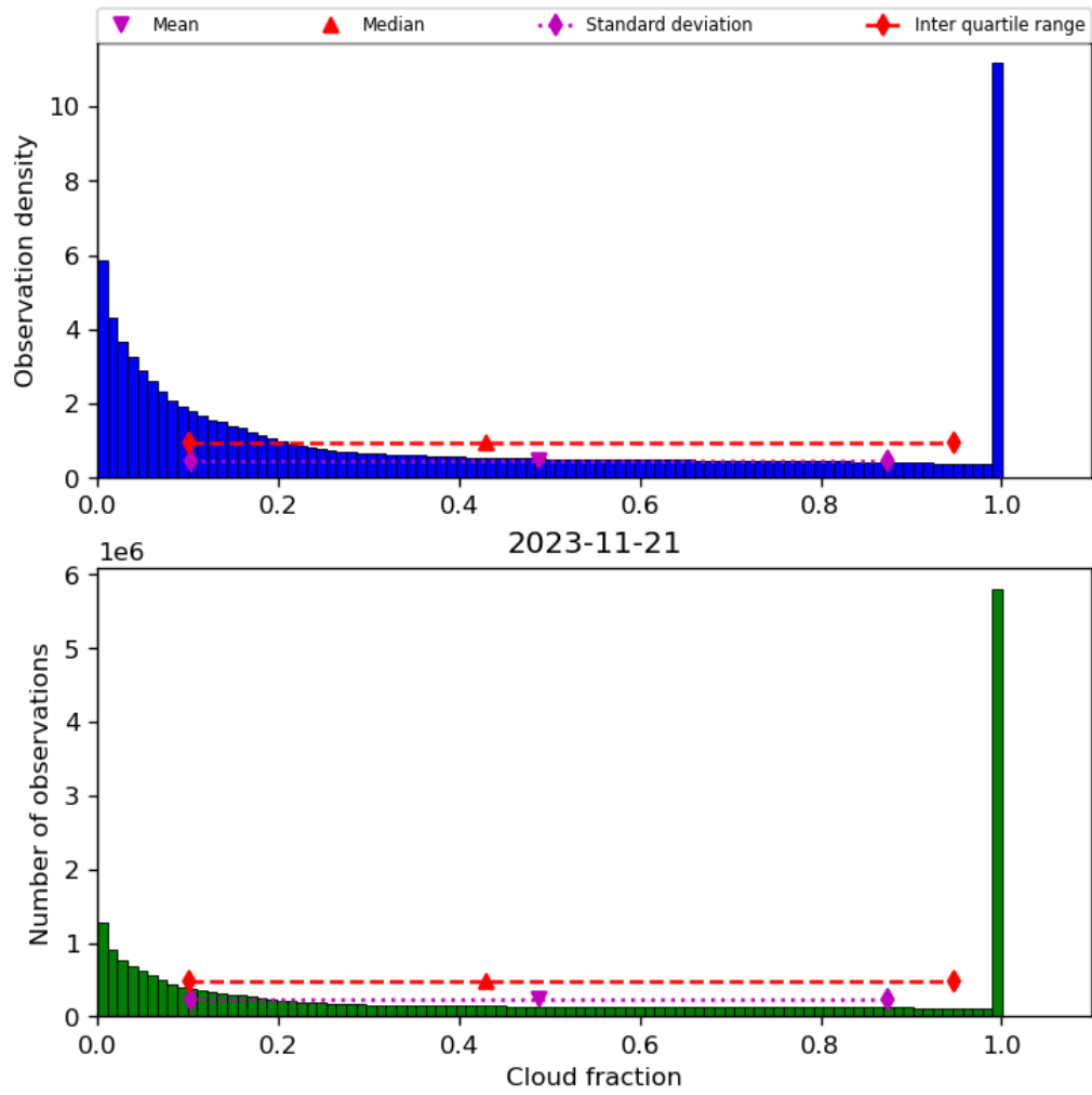
Figure 32: Histogram of “Cloud fraction” for 2023-11-20 to 2023-11-22
