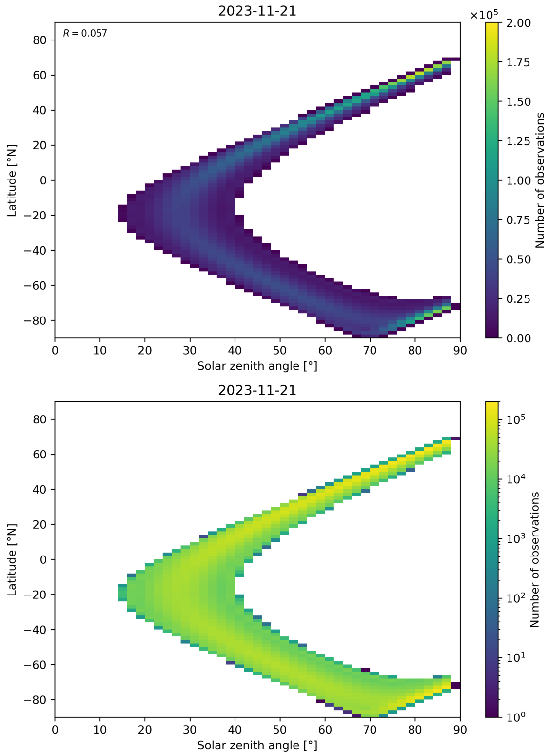
Figure 124: Scatter density plot of “Solar zenith angle” against “Latitude” for 2023-11-20 to 2023-11-22.
