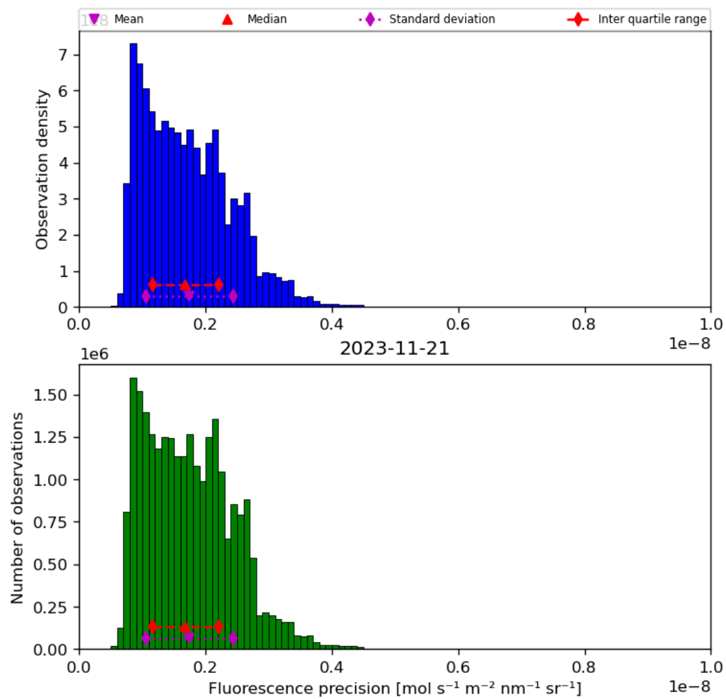
Figure 41: Histogram of “Fluorescence precision” for 2023-11-20 to 2023-11-22
