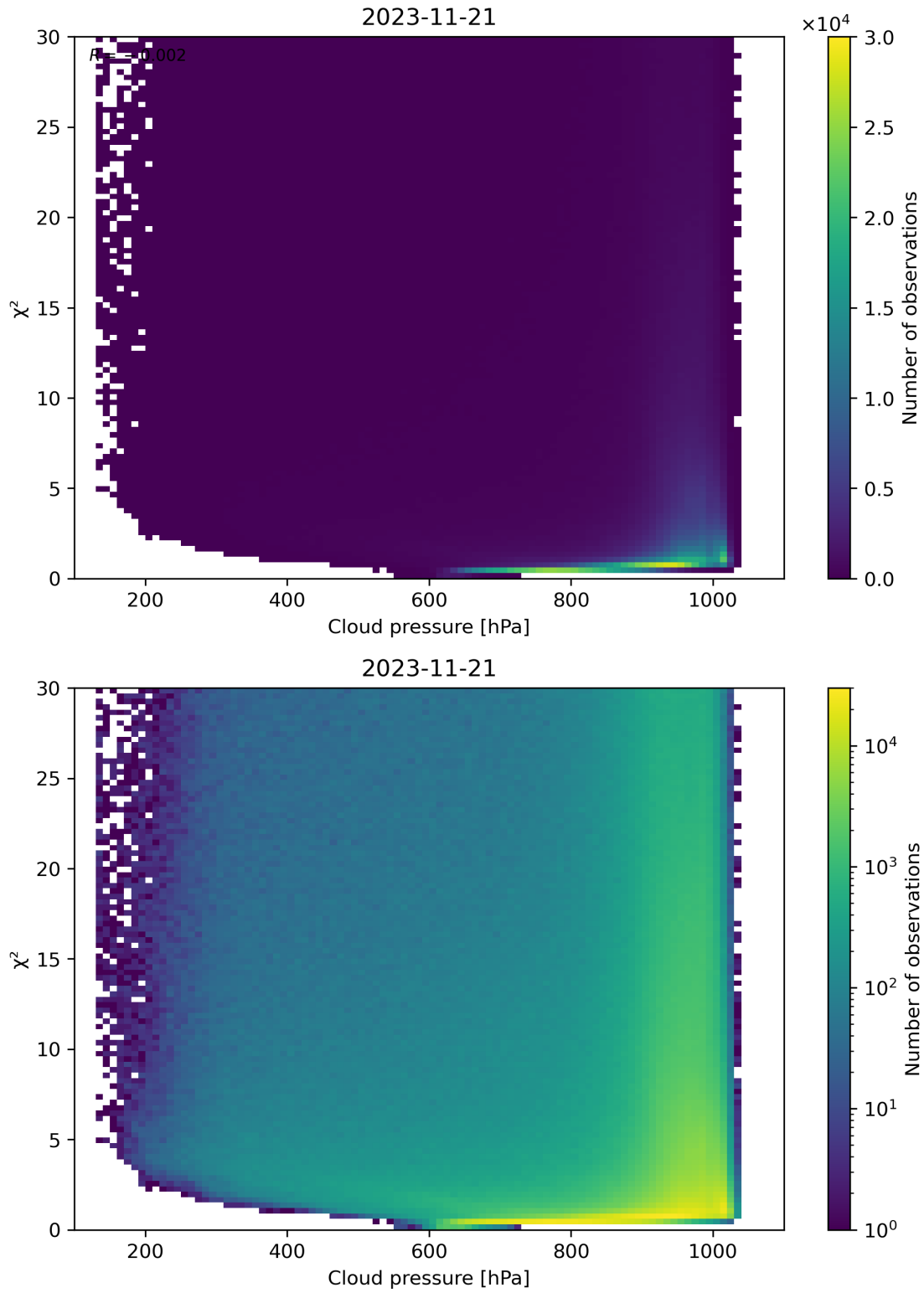
Figure 85: Scatter density plot of “Cloud pressure” against “ \chi^2 ” for 2023-11-20 to 2023-11-22.
