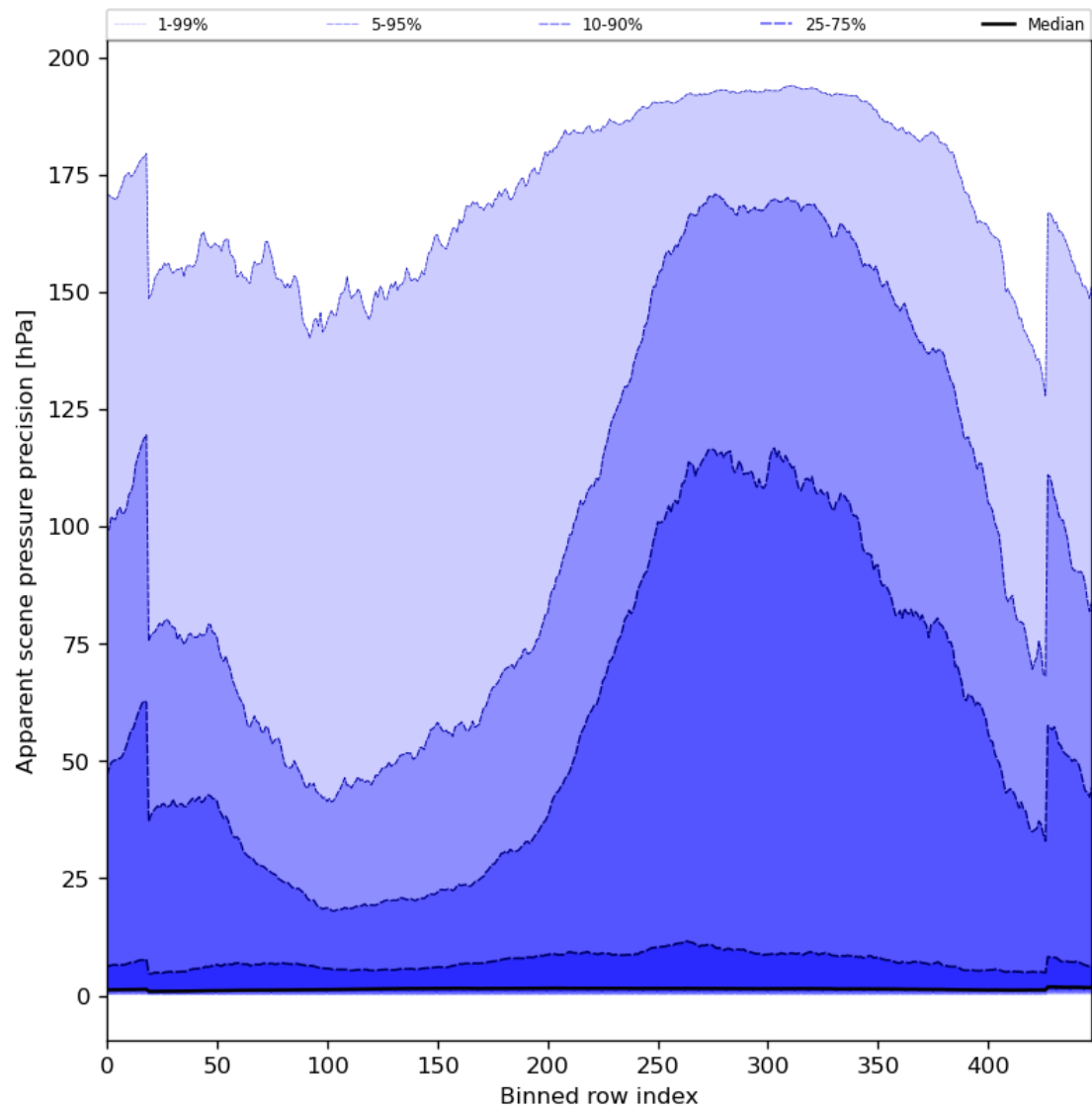
Figure 54: Along track statistics of “Apparent scene pressure precision” for 2023-11-20 to 2023-11-22
