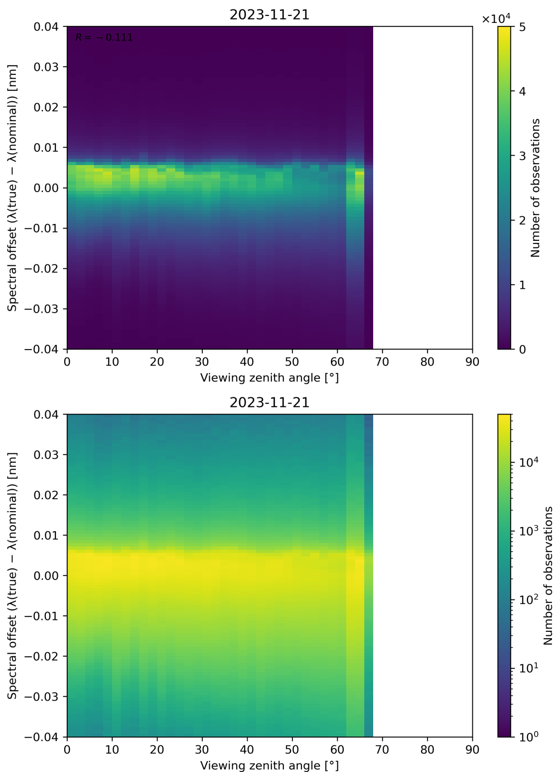
Figure 140: Scatter density plot of “Viewing zenith angle” against “Spectral offset ( \lambda(\text{true}) - \lambda(\text{nominal}) )” for 2023-11-20 to 2023-11-22.
