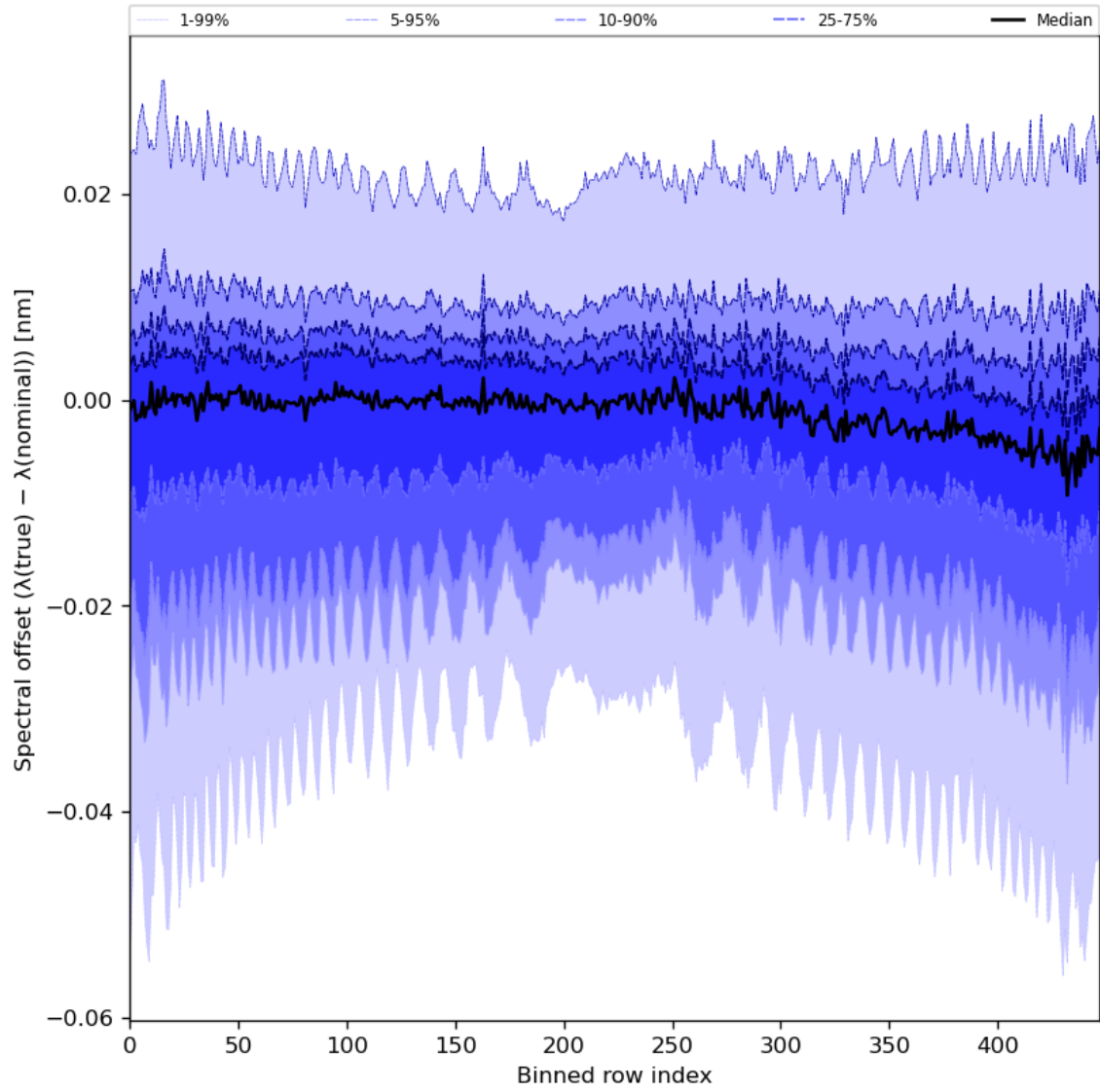
Figure 62: Along track statistics of “Spectral offset ( \lambda(\text{true}) - \lambda(\text{nominal}) )” for 2023-11-20 to 2023-11-22
