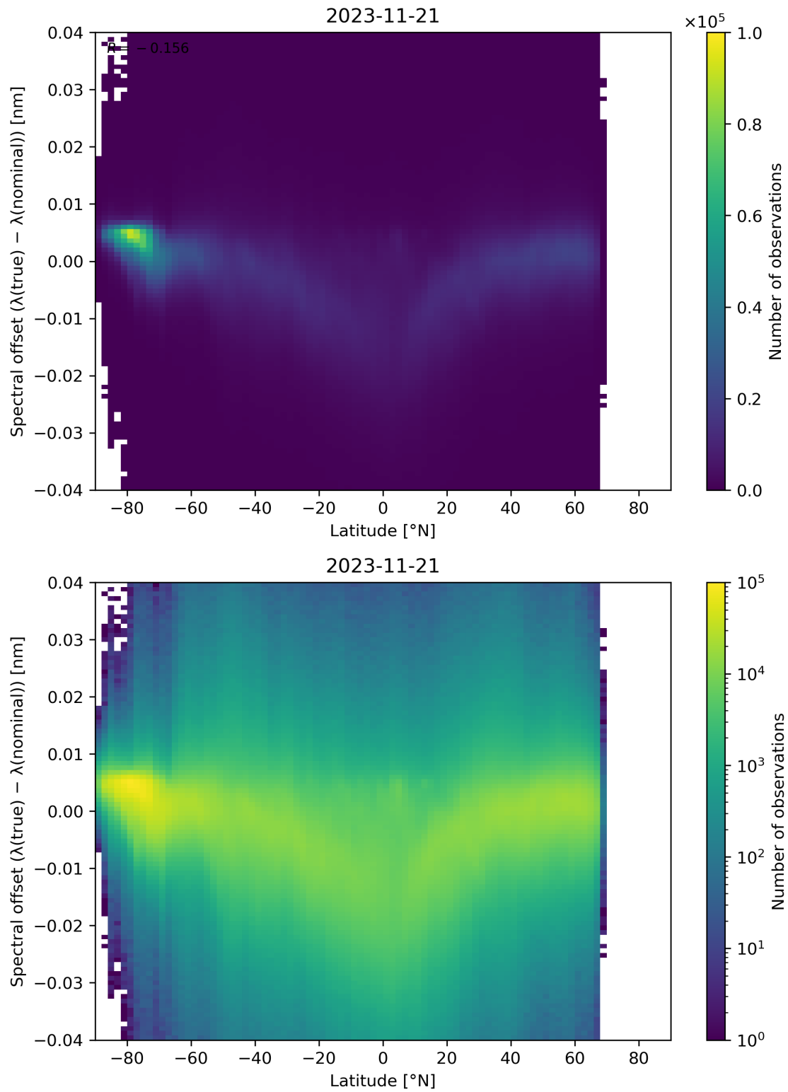
Figure 105: Scatter density plot of “Latitude” against “Spectral offset ( \lambda(\text{true}) - \lambda(\text{nominal}) )” for 2023-11-20 to 2023-11-22.
