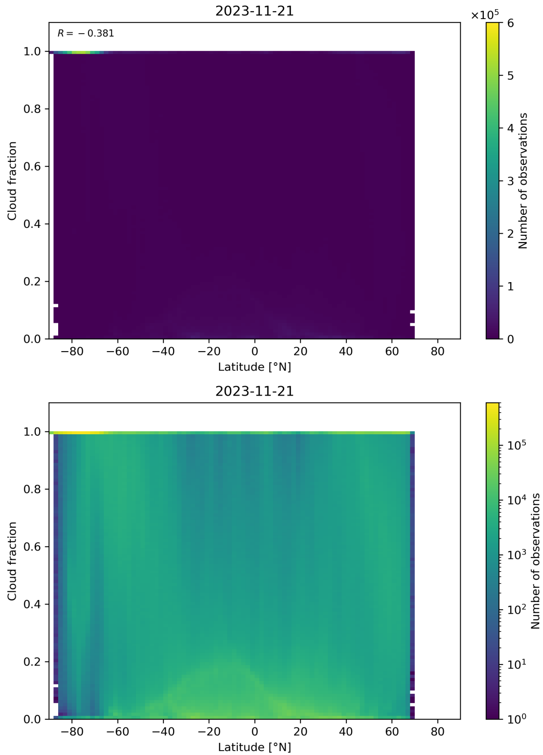
Figure 99: Scatter density plot of “Latitude” against “Cloud fraction” for 2023-11-20 to 2023-11-22.
