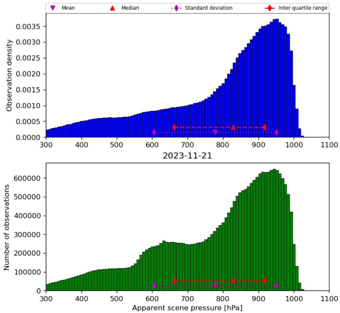
Figure 36: Histogram of “Apparent scene pressure” for 2023-11-20 to 2023-11-22
