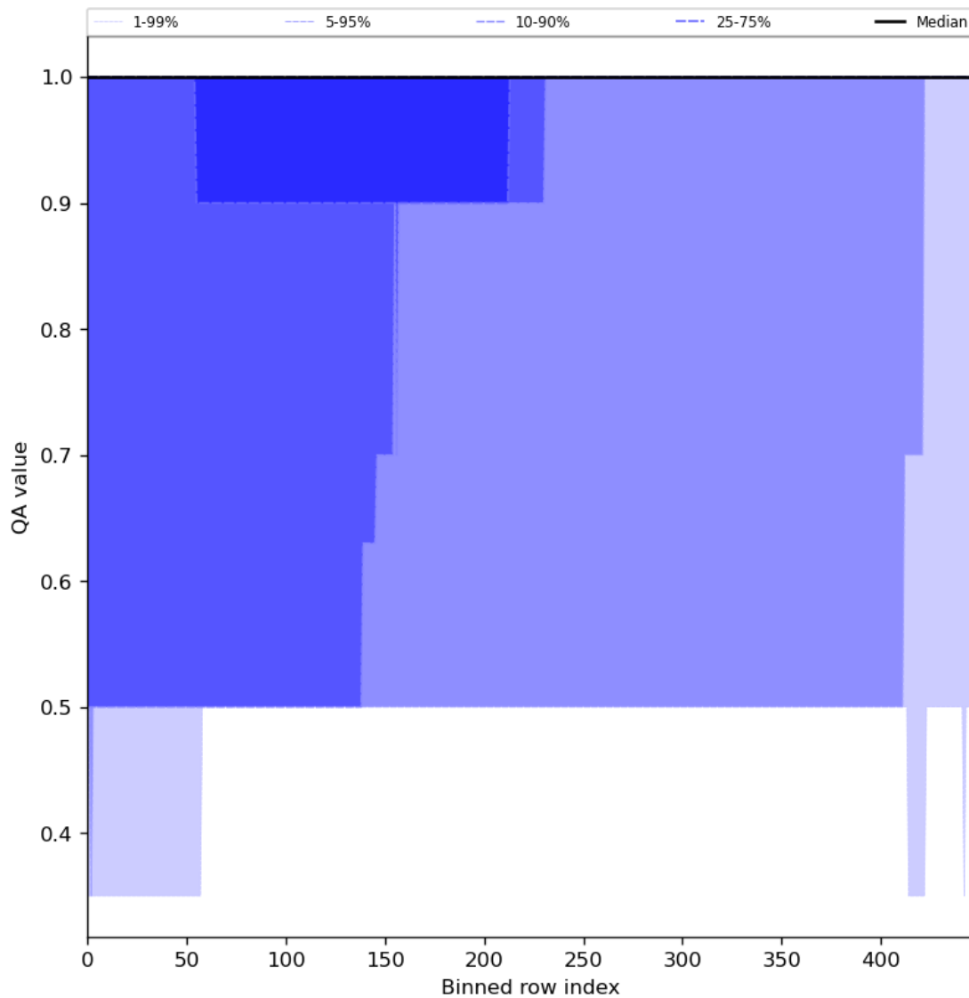
Figure 46: Along track statistics of “QA value” for 2023-11-20 to 2023-11-22
