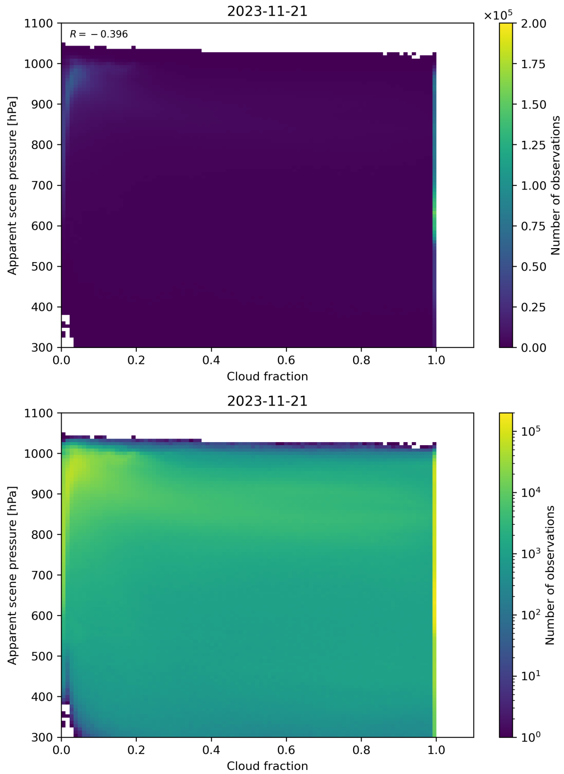
Figure 76: Scatter density plot of “Cloud fraction” against “Apparent scene pressure” for 2023-11-20 to 2023-11-22.
