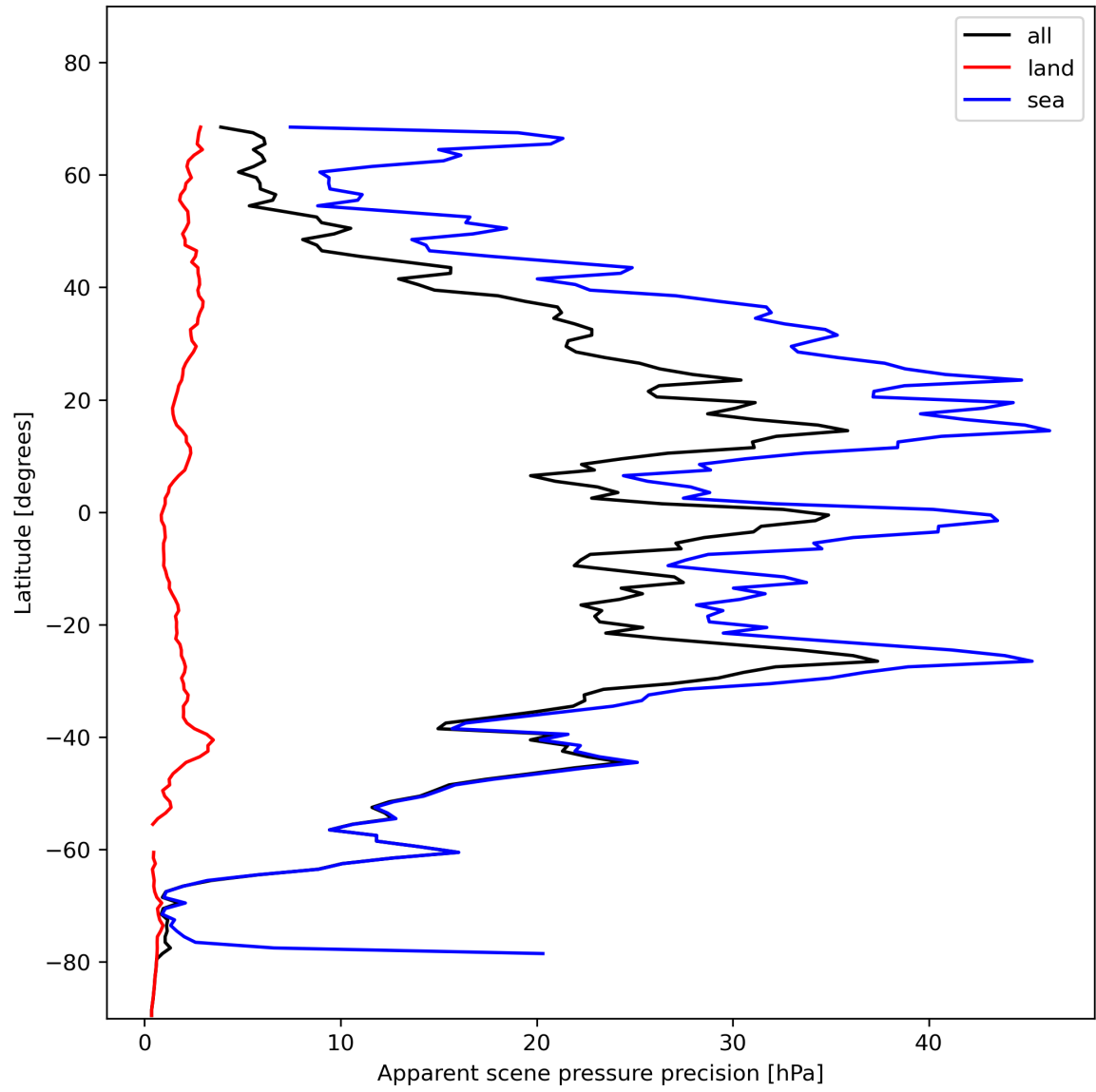
Figure 20: Zonal average of “Apparent scene pressure precision” for 2023-11-20 to 2023-11-22.
