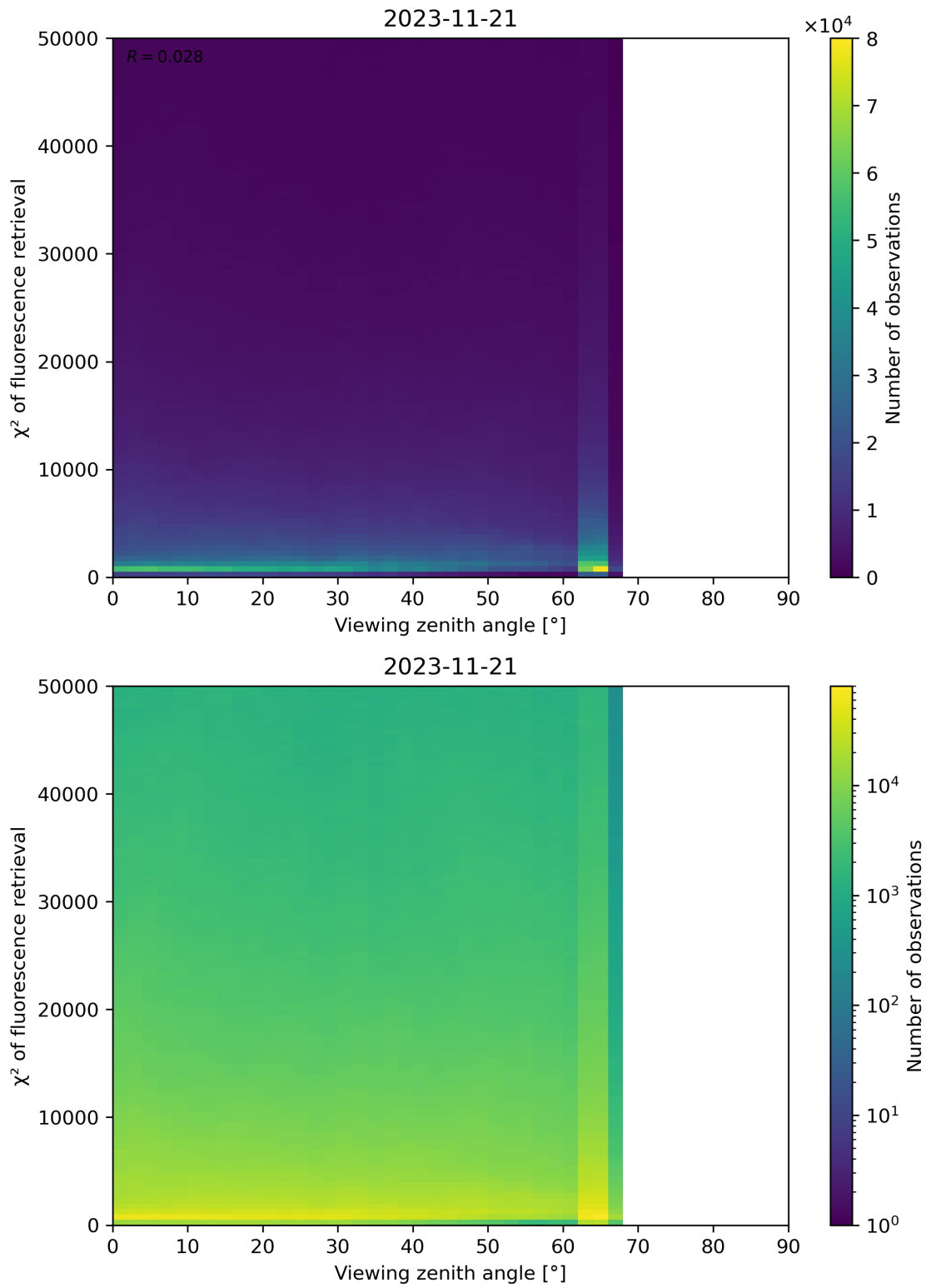
Figure 131: Scatter density plot of “Viewing zenith angle” against “ \chi^2 of fluorescence retrieval” for 2023-11-20 to 2023-11-22.
