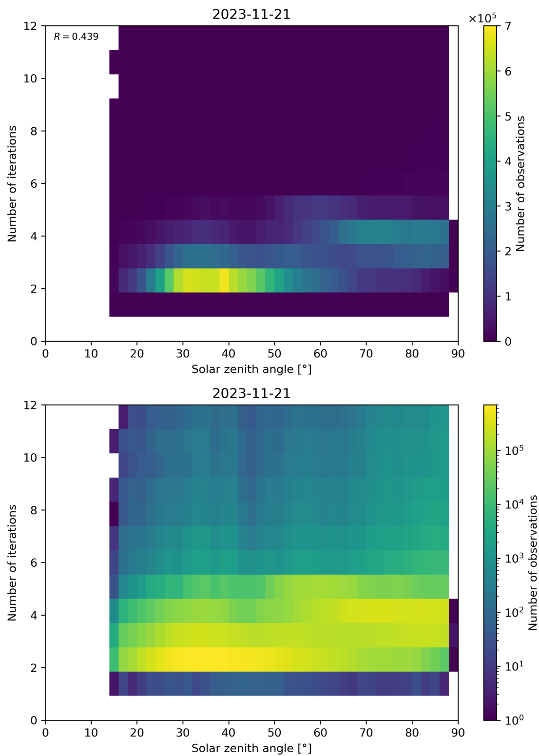
Figure 125: Scatter density plot of “Solar zenith angle” against “Number of iterations” for 2023-11-20 to 2023-11-22.
