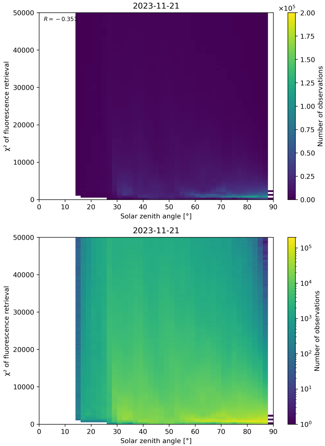
Figure 120: Scatter density plot of “Solar zenith angle” against “ \chi^2 of fluorescence retrieval” for 2023-11-20 to 2023-11-22.
