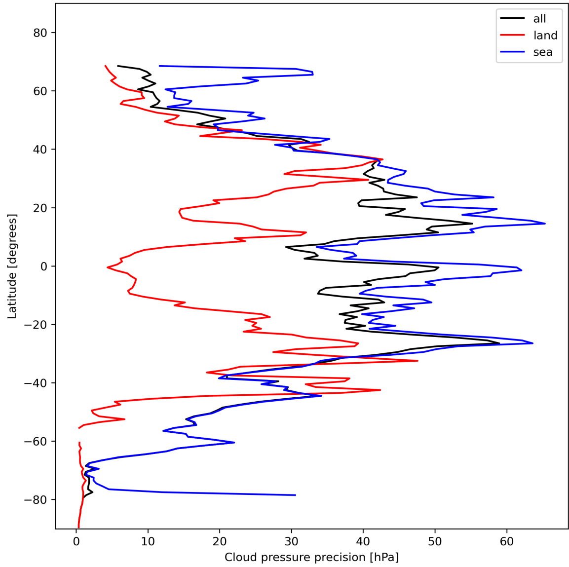
Figure 14: Zonal average of “Cloud pressure precision” for 2023-11-20 to 2023-11-22.
