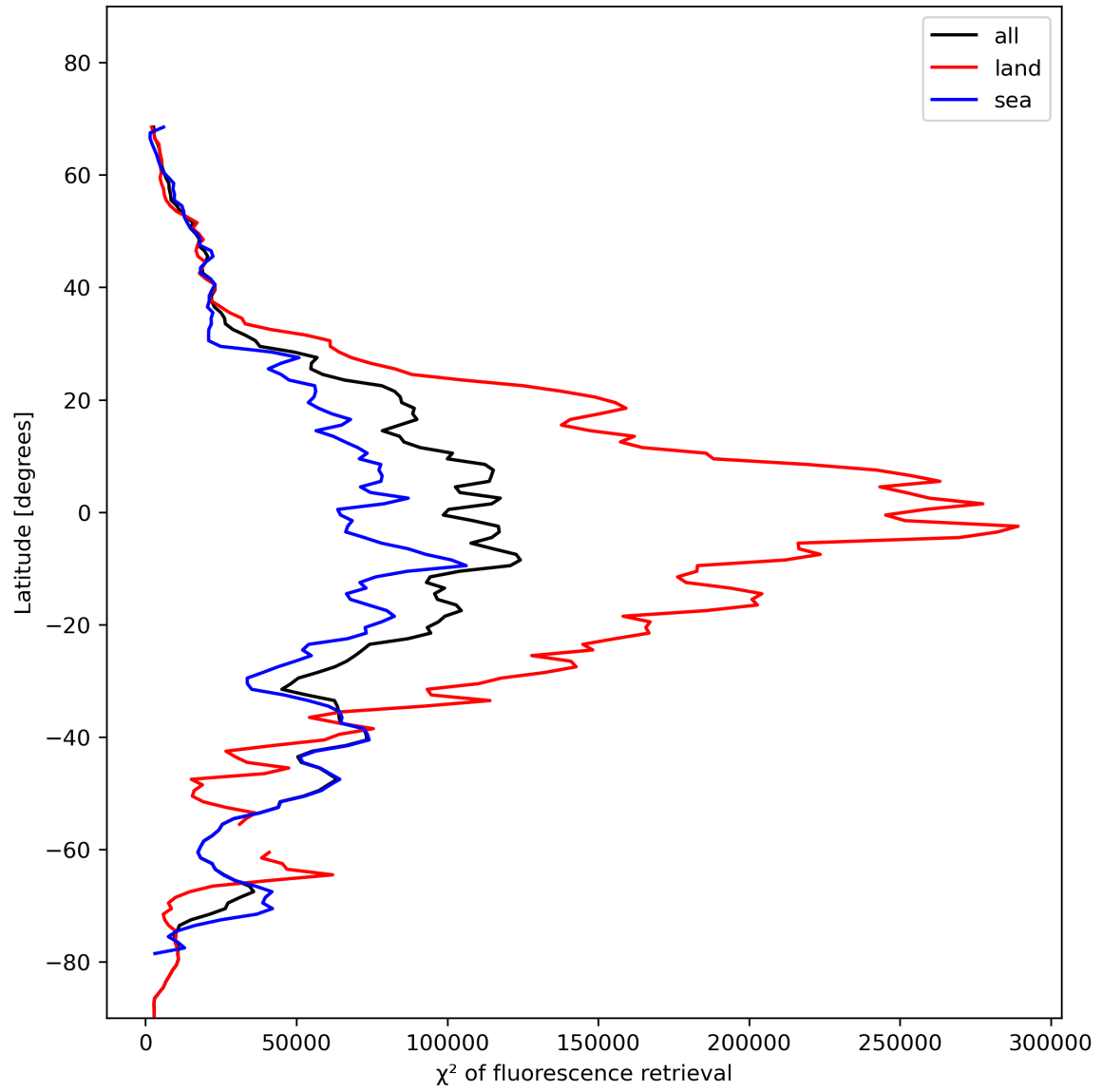
Figure 25: Zonal average of “ \chi^2 of fluorescence retrieval” for 2023-11-20 to 2023-11-22.
