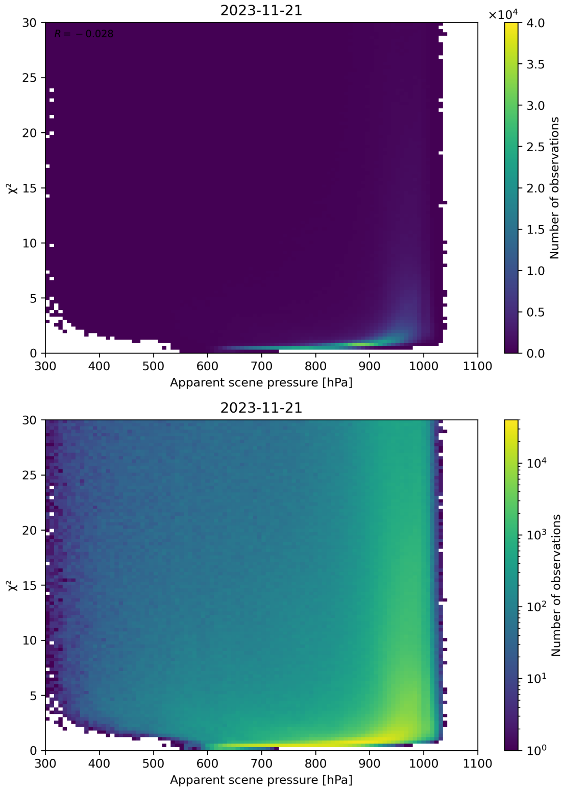
Figure 63: Scatter density plot of “Apparent scene pressure” against “ \chi^2 ” for 2023-11-20 to 2023-11-22.
