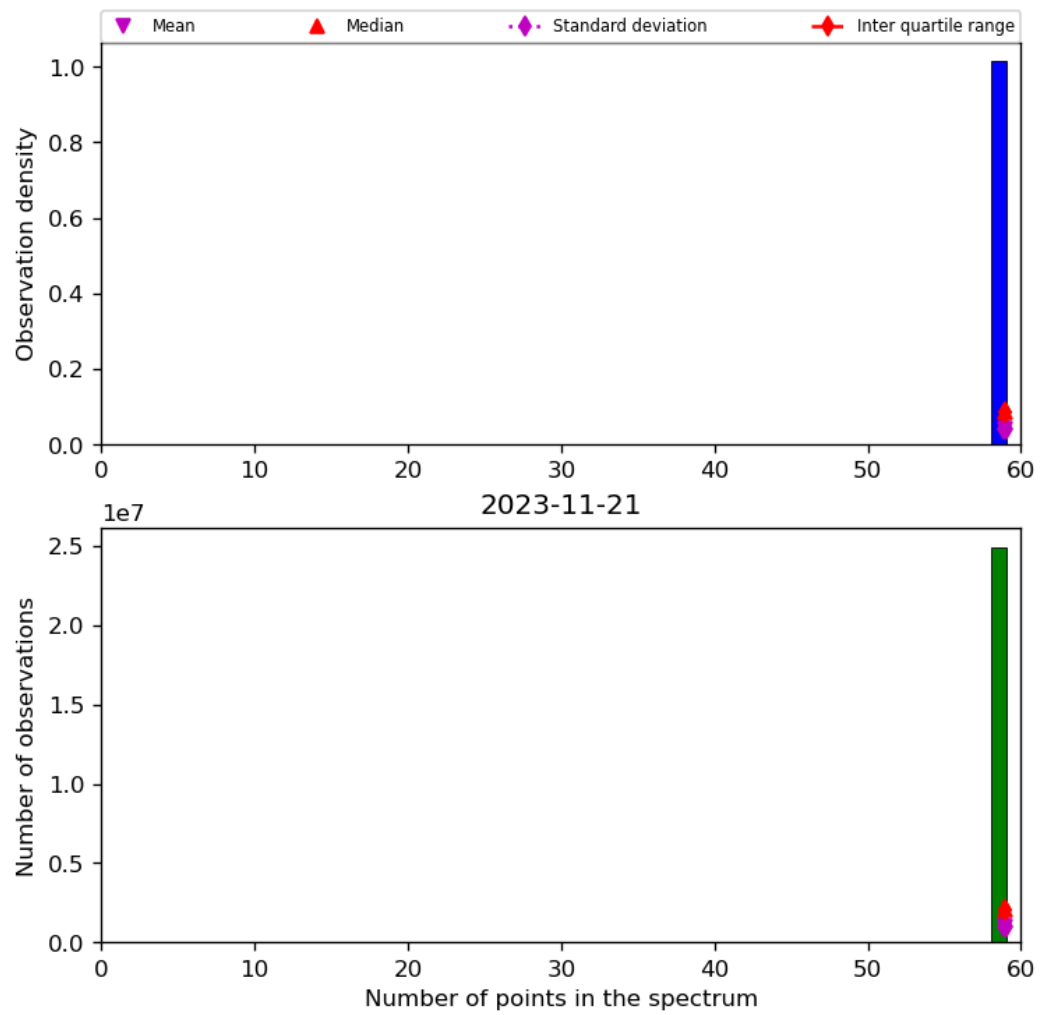
Figure 44: Histogram of “Number of points in the spectrum” for 2023-11-20 to 2023-11-22
