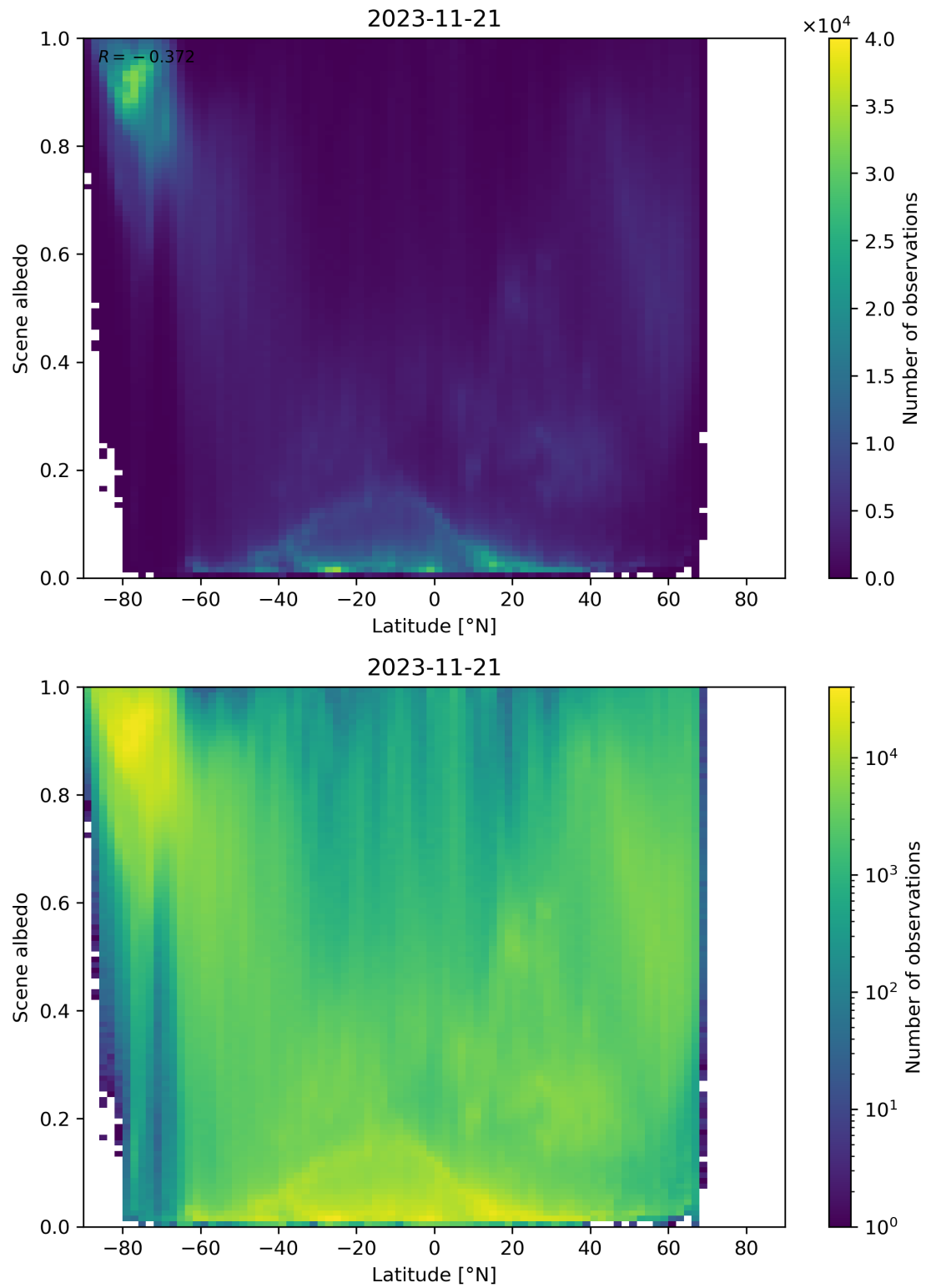
Figure 104: Scatter density plot of “Latitude” against “Scene albedo” for 2023-11-20 to 2023-11-22.
