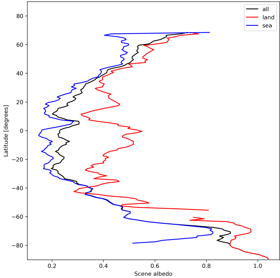
Figure 17: Zonal average of “Scene albedo” for 2023-11-20 to 2023-11-22.
