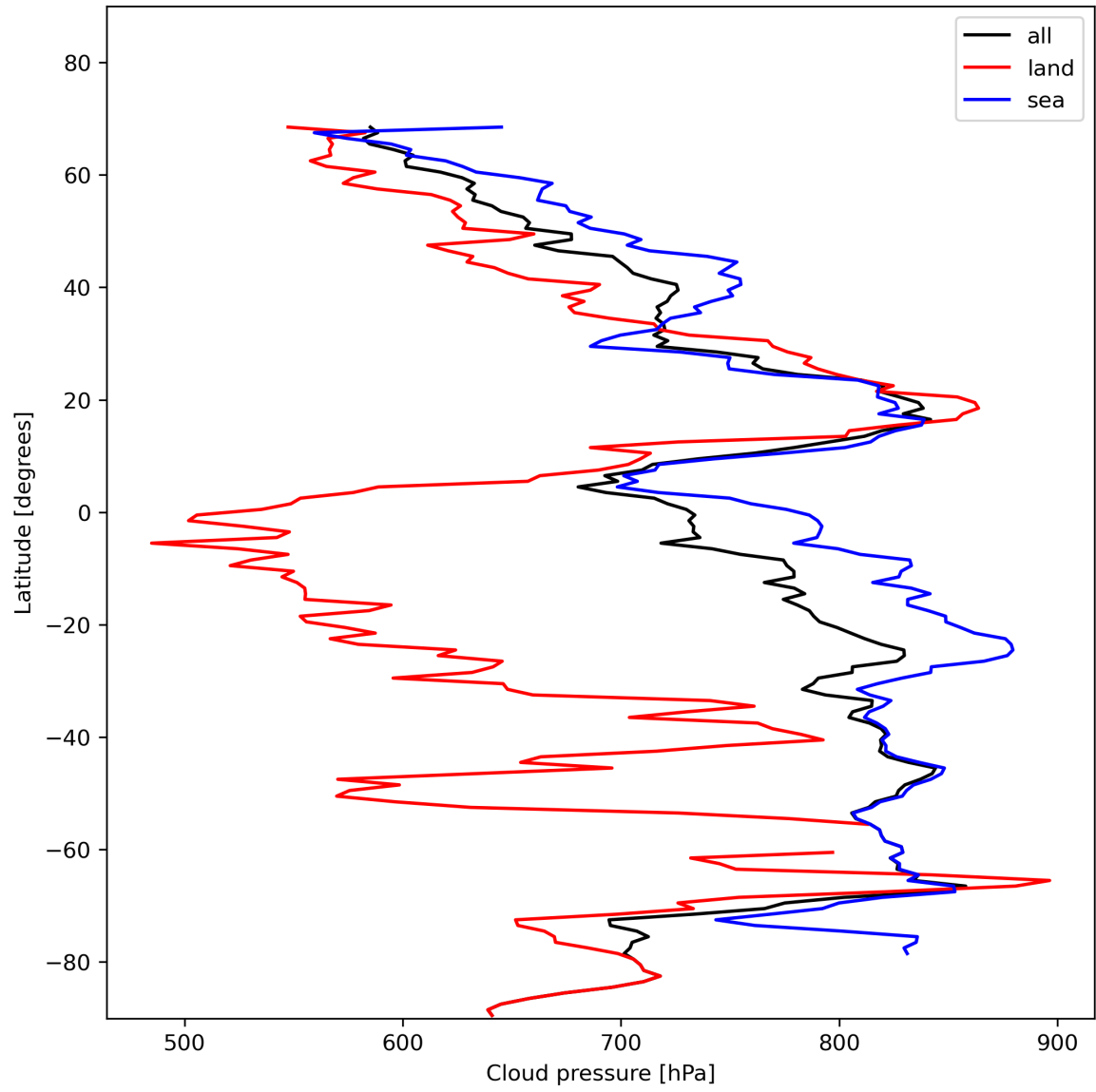
Figure 13: Zonal average of “Cloud pressure” for 2023-11-20 to 2023-11-22.
