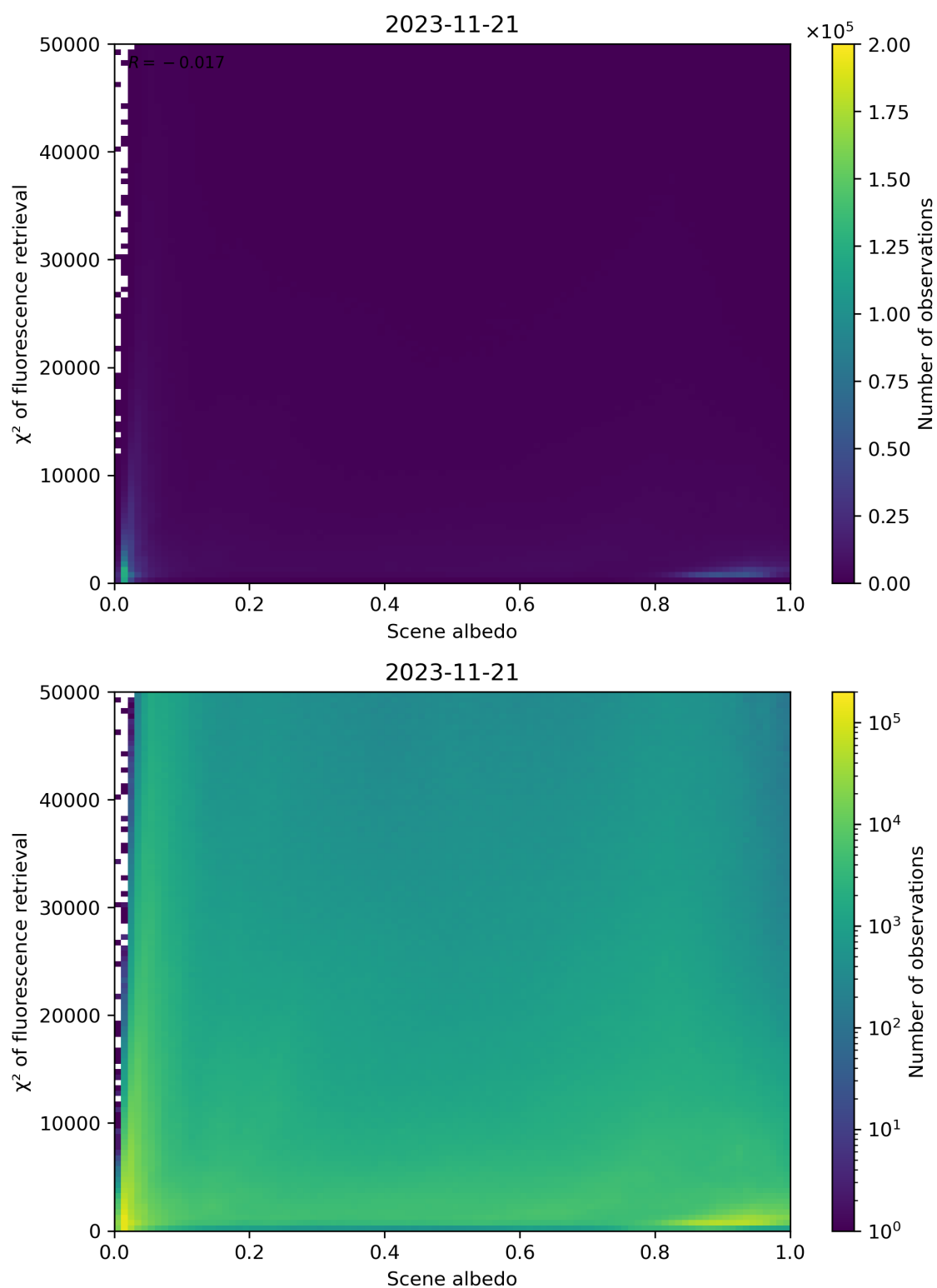
Figure 113: Scatter density plot of “Scene albedo” against “ \chi^2 of fluorescence retrieval” for 2023-11-20 to 2023-11-22.
