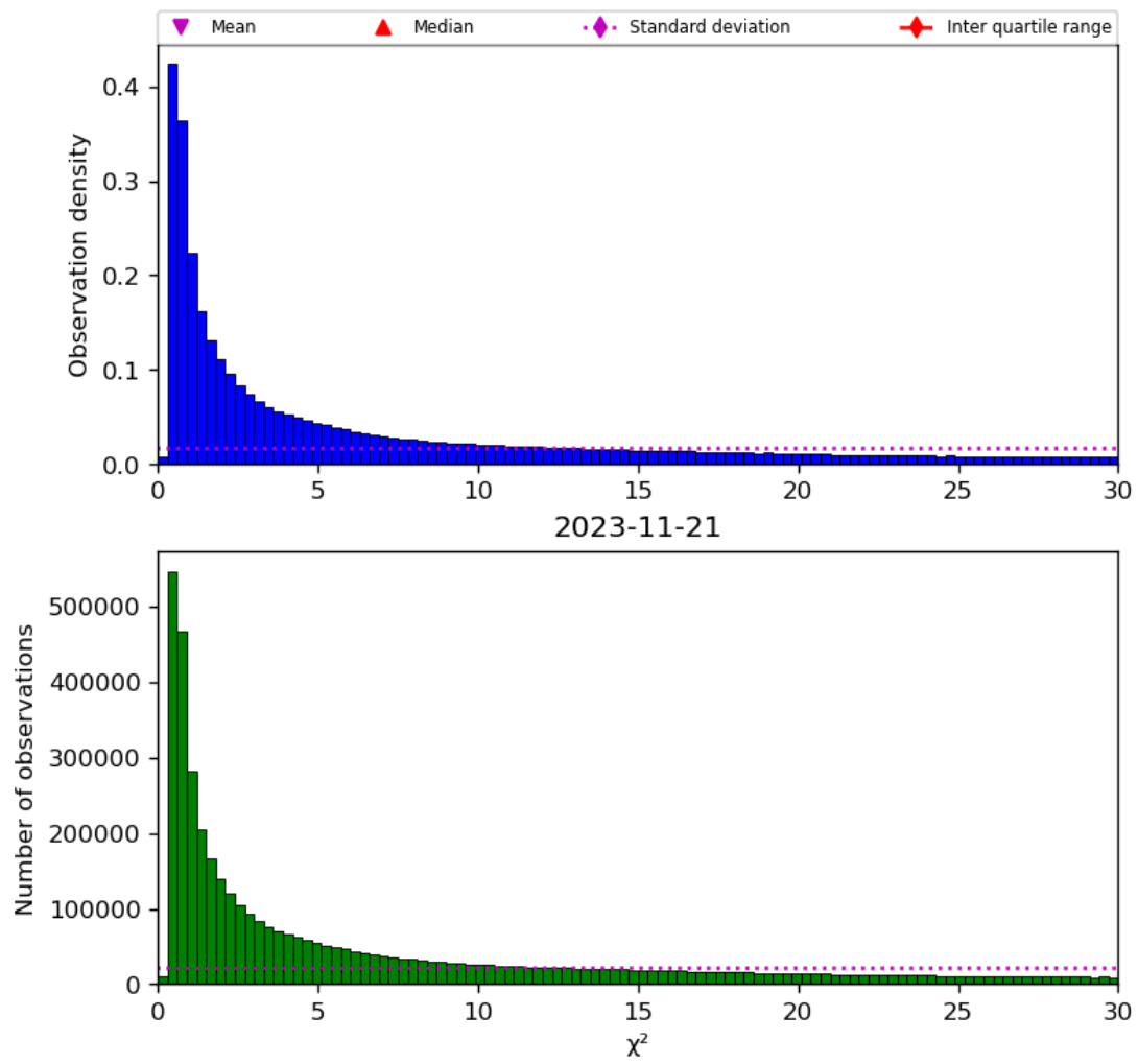
Figure 38: Histogram of “ \chi^2 ” for 2023-11-20 to 2023-11-22
