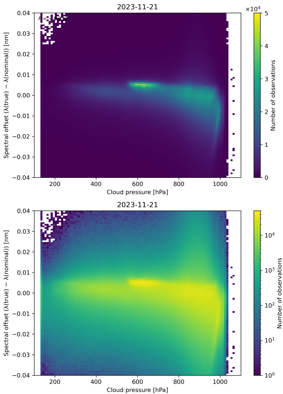
Figure 92: Scatter density plot of “Cloud pressure” against “Spectral offset ( \lambda(\text{true}) - \lambda(\text{nominal}) )” for 2023-11-20 to 2023-11-22.
