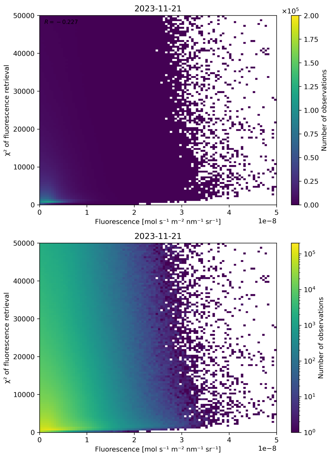
Figure 93: Scatter density plot of “Fluorescence” against “ \chi^2 of fluorescence retrieval” for 2023-11-20 to 2023-11-22.
