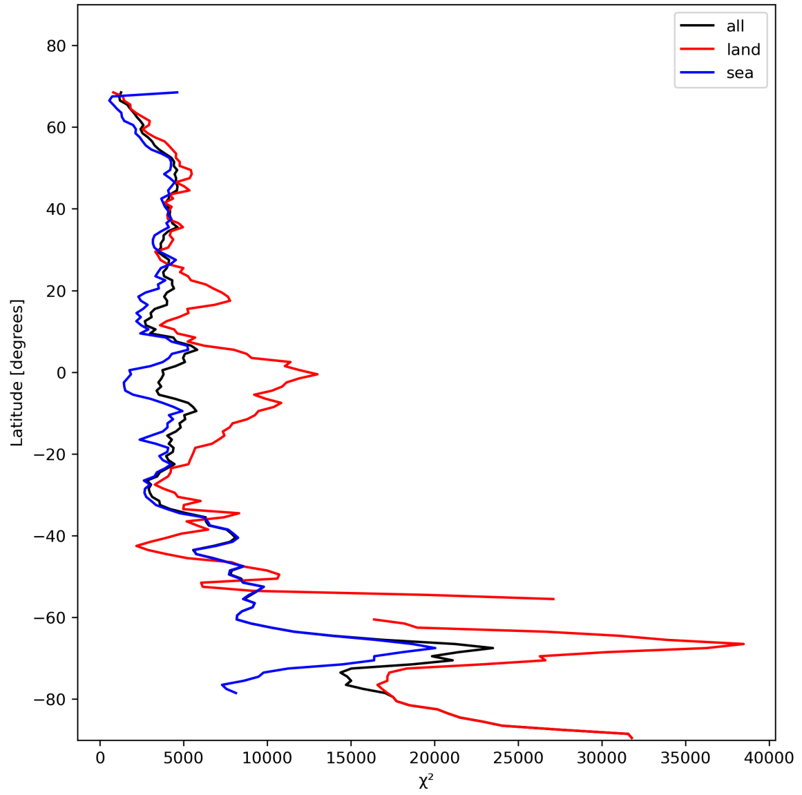
Figure 21: Zonal average of “ \chi^2 ” for 2023-11-20 to 2023-11-22.
