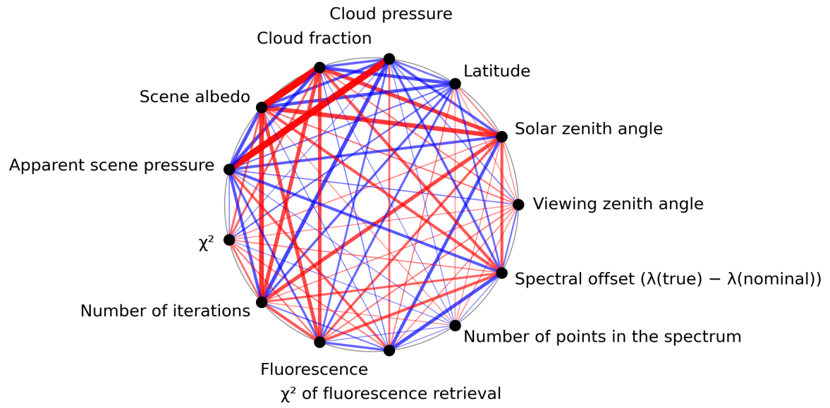
Figure 1: Map of correlation graph for 2023-11-20 to 2023-11-22.
