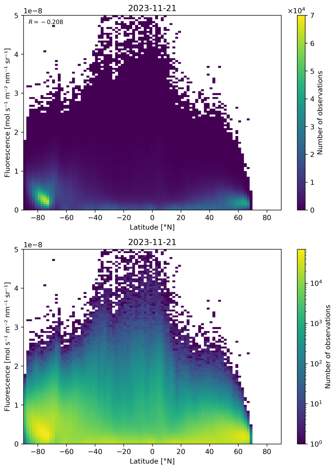
Figure 101: Scatter density plot of “Latitude” against “Fluorescence” for 2023-11-20 to 2023-11-22.
