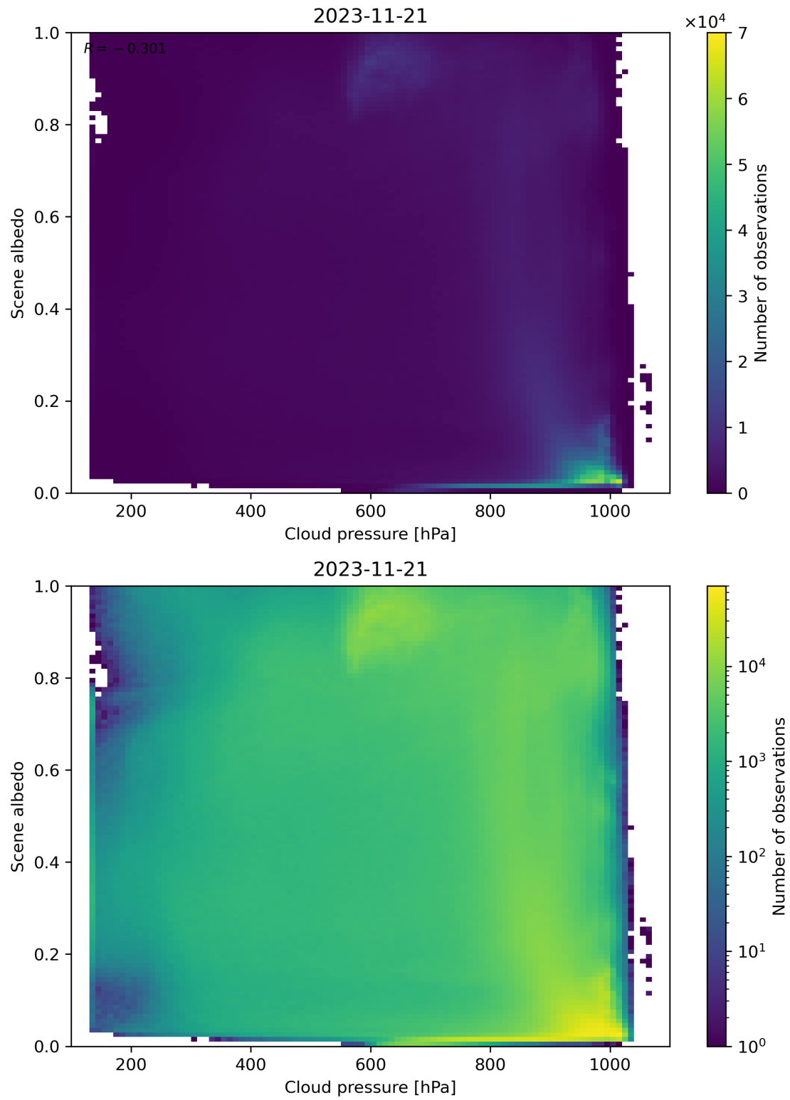
Figure 91: Scatter density plot of “Cloud pressure” against “Scene albedo” for 2023-11-20 to 2023-11-22.
