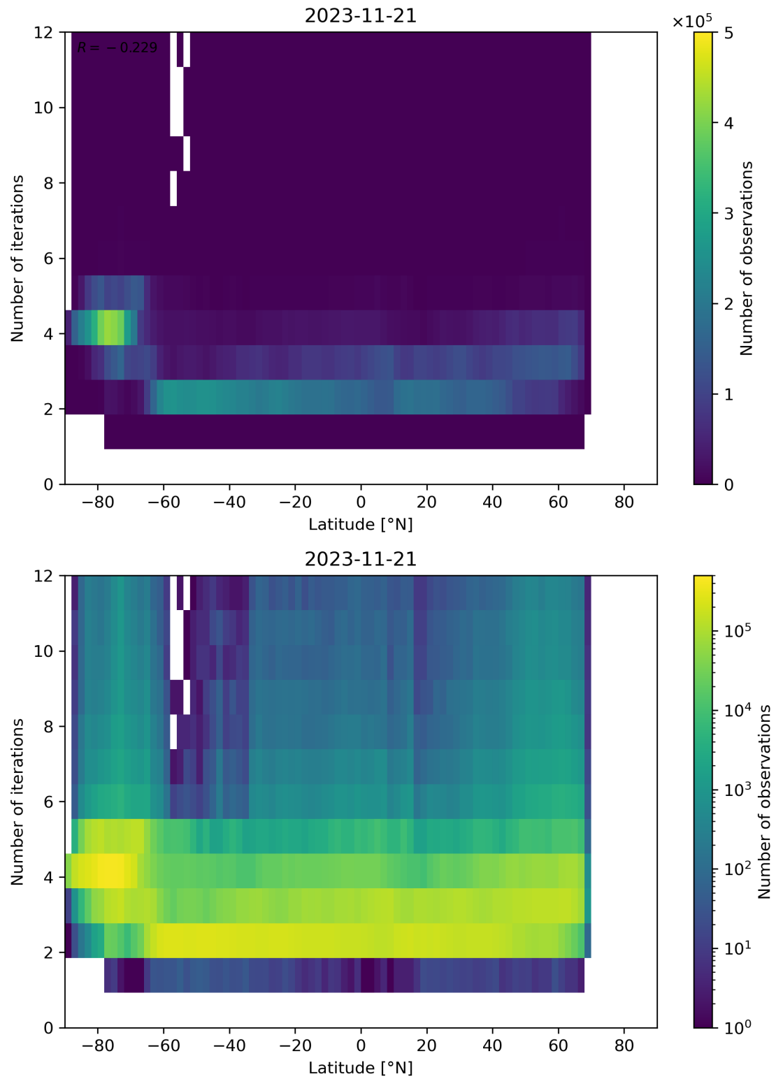
Figure 102: Scatter density plot of “Latitude” against “Number of iterations” for 2023-11-20 to 2023-11-22.
