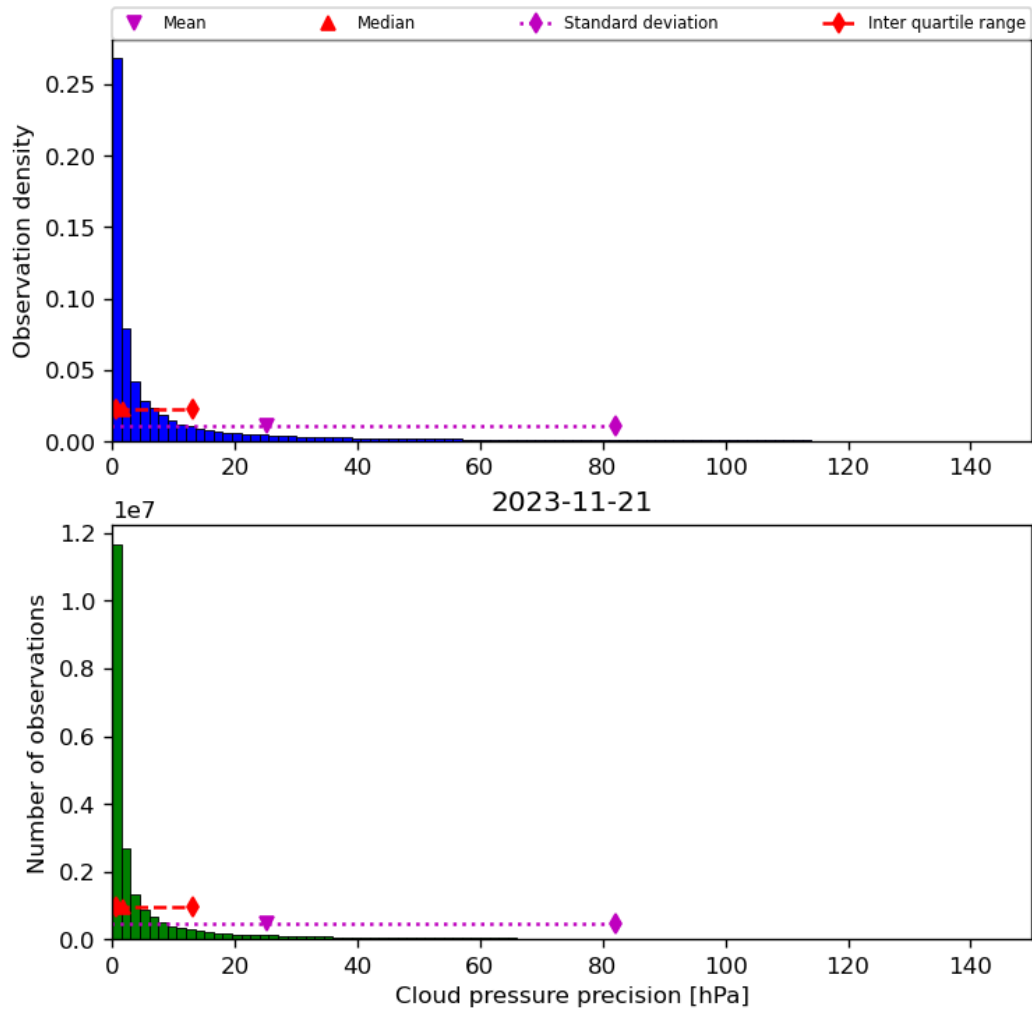
Figure 31: Histogram of “Cloud pressure precision” for 2023-11-20 to 2023-11-22
