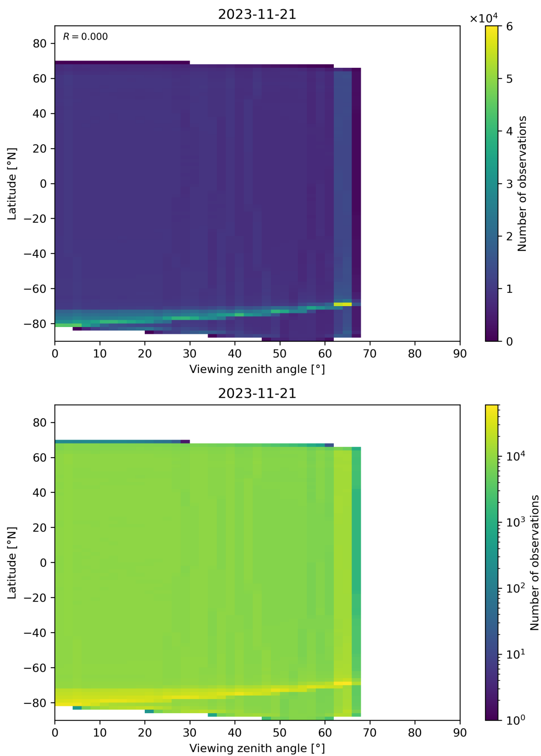
Figure 135: Scatter density plot of “Viewing zenith angle” against “Latitude” for 2023-11-20 to 2023-11-22.
