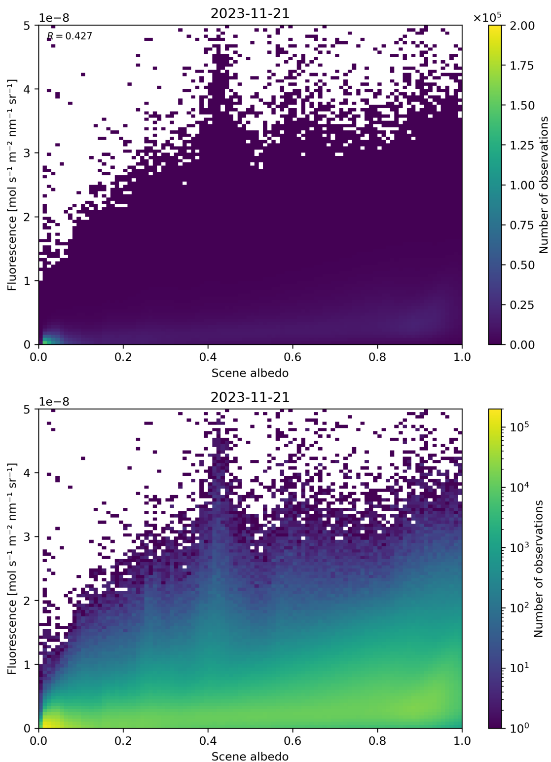
Figure 114: Scatter density plot of “Scene albedo” against “Fluorescence” for 2023-11-20 to 2023-11-22.
