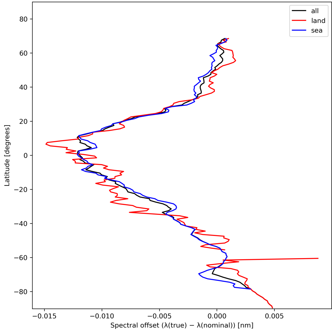
Figure 28: Zonal average of “Spectral offset ( \lambda(\text{true}) - \lambda(\text{nominal}) )” for 2023-11-20 to 2023-11-22.
