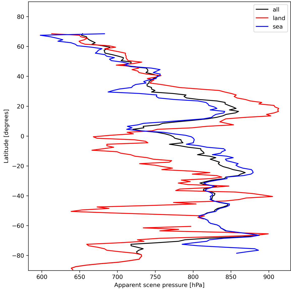
Figure 19: Zonal average of “Apparent scene pressure” for 2023-11-20 to 2023-11-22.
