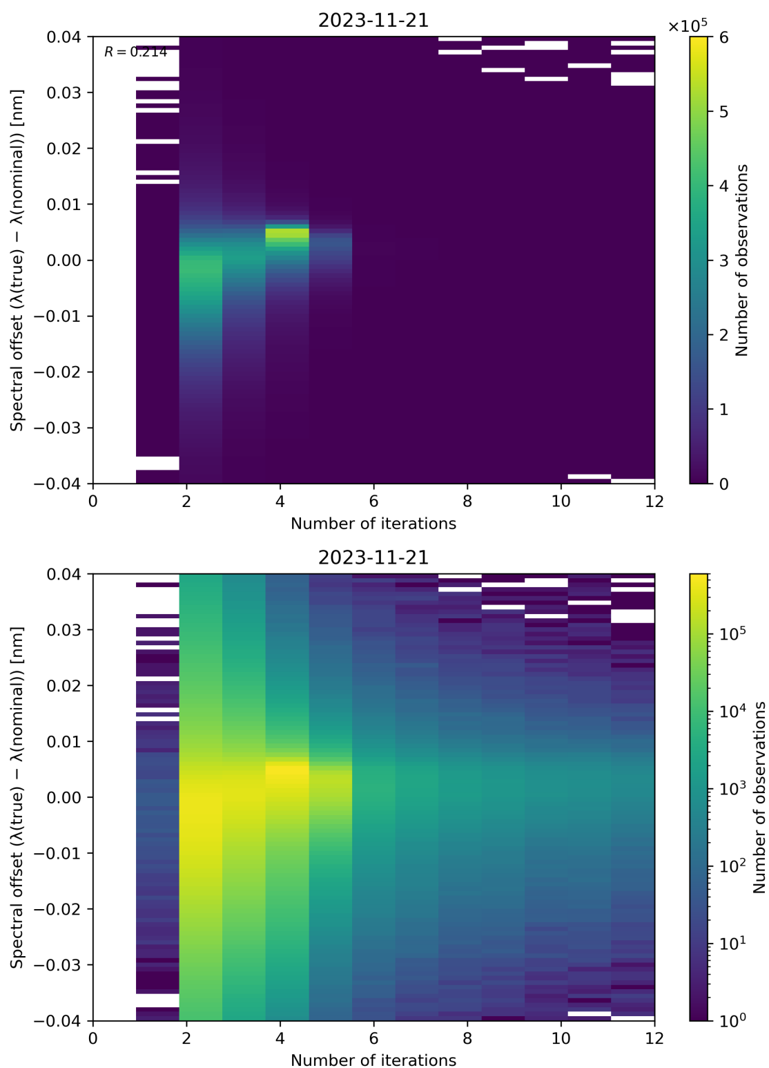
Figure 109: Scatter density plot of “Number of iterations” against “Spectral offset ( \lambda(\text{true}) - \lambda(\text{nominal}) )” for 2023-11-20 to 2023-11-22.
