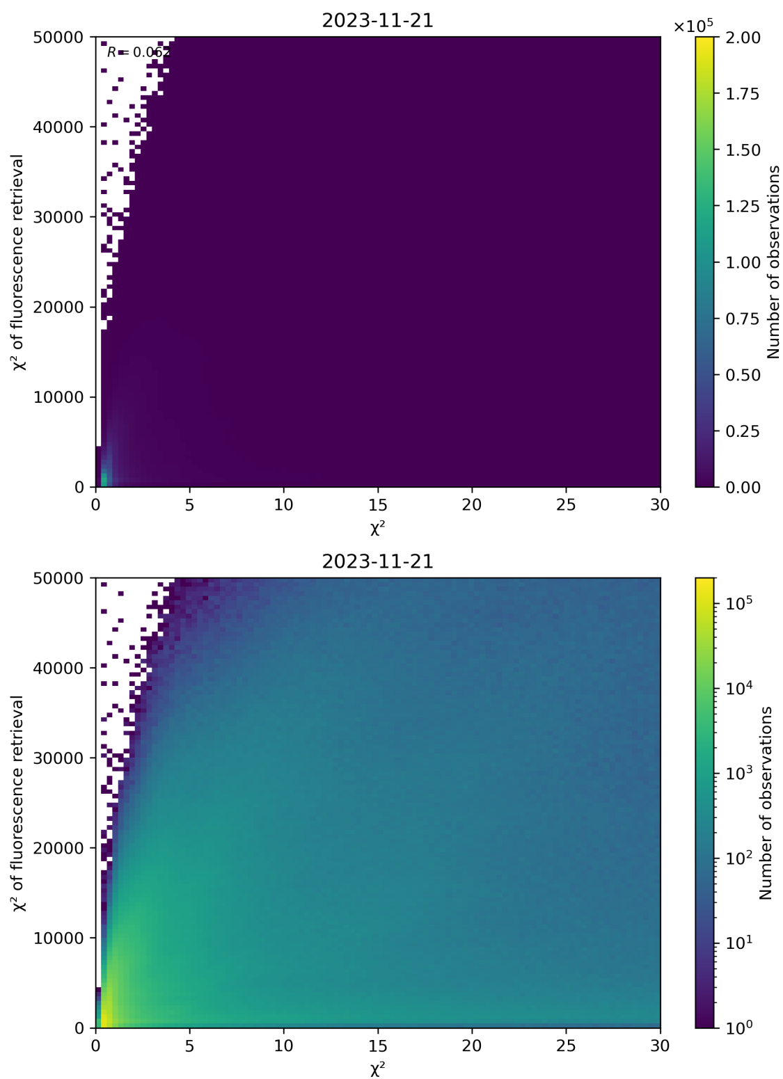
Figure 69: Scatter density plot of “ \chi^2 ” against “ \chi^2 of fluorescence retrieval” for 2023-11-20 to 2023-11-22.
