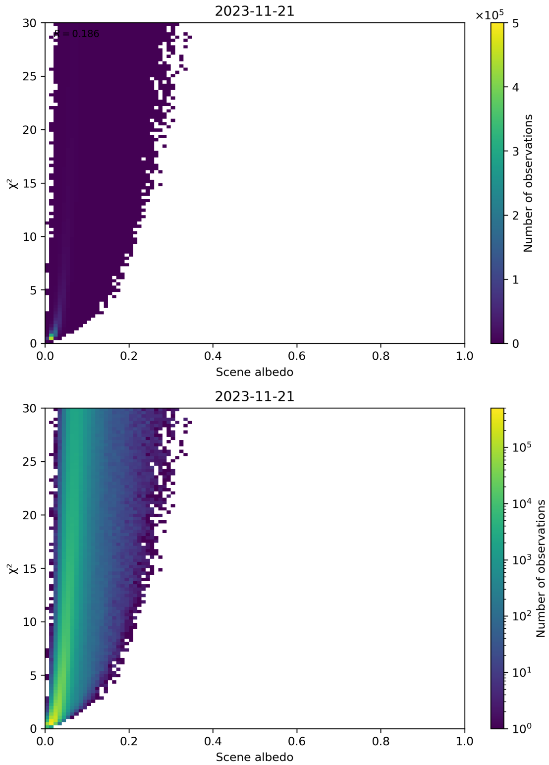
Figure 112: Scatter density plot of “Scene albedo” against “ \chi^2 ” for 2023-11-20 to 2023-11-22.
