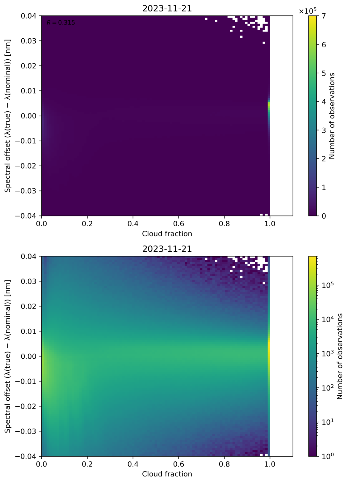
Figure 83: Scatter density plot of “Cloud fraction” against “Spectral offset ( \lambda(\text{true}) - \lambda(\text{nominal}) )” for 2023-11-20 to 2023-11-22.
