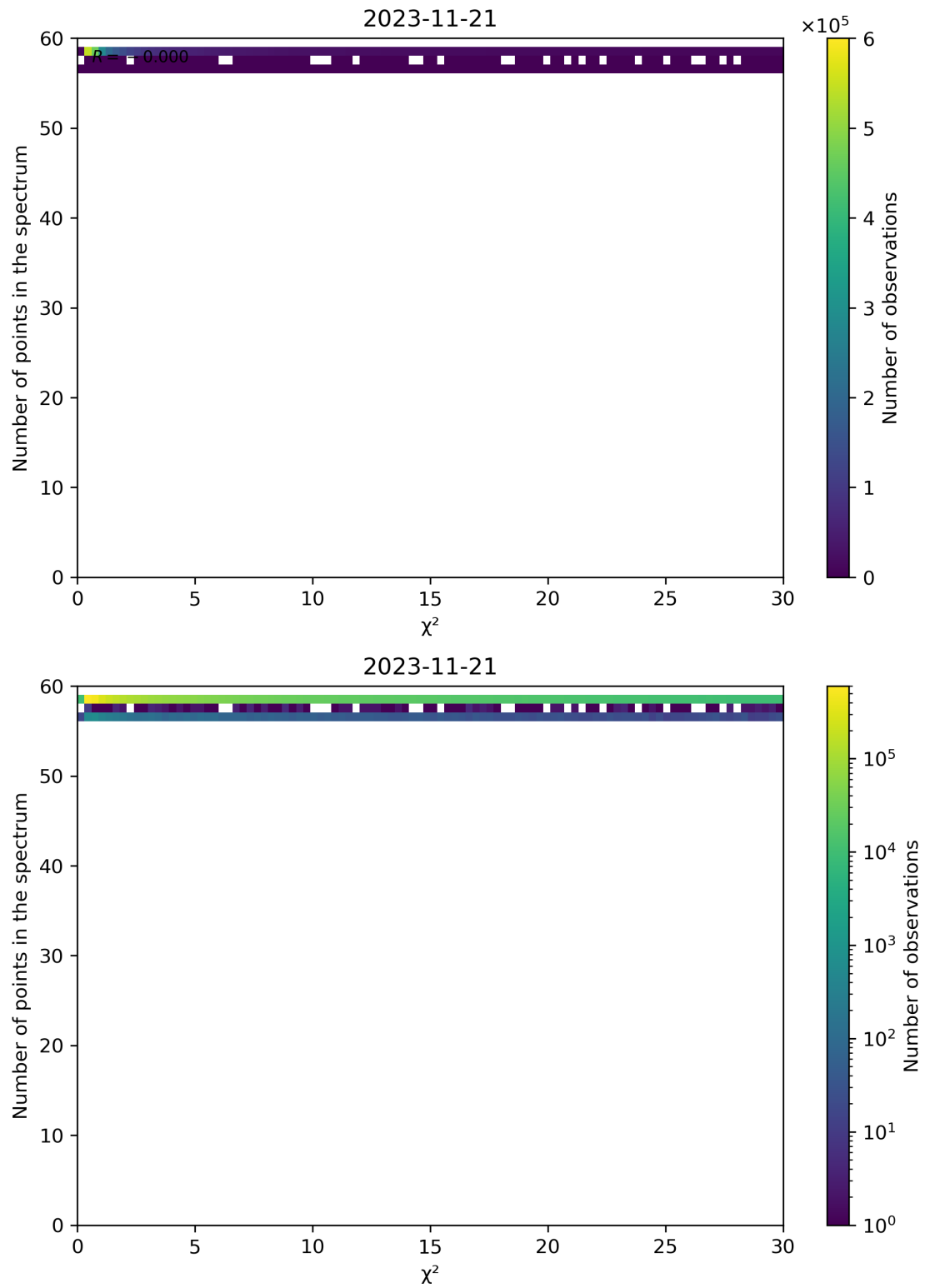
Figure 74: Scatter density plot of " \chi^2 " against "Number of points in the spectrum" for 2023-11-20 to 2023-11-22.
