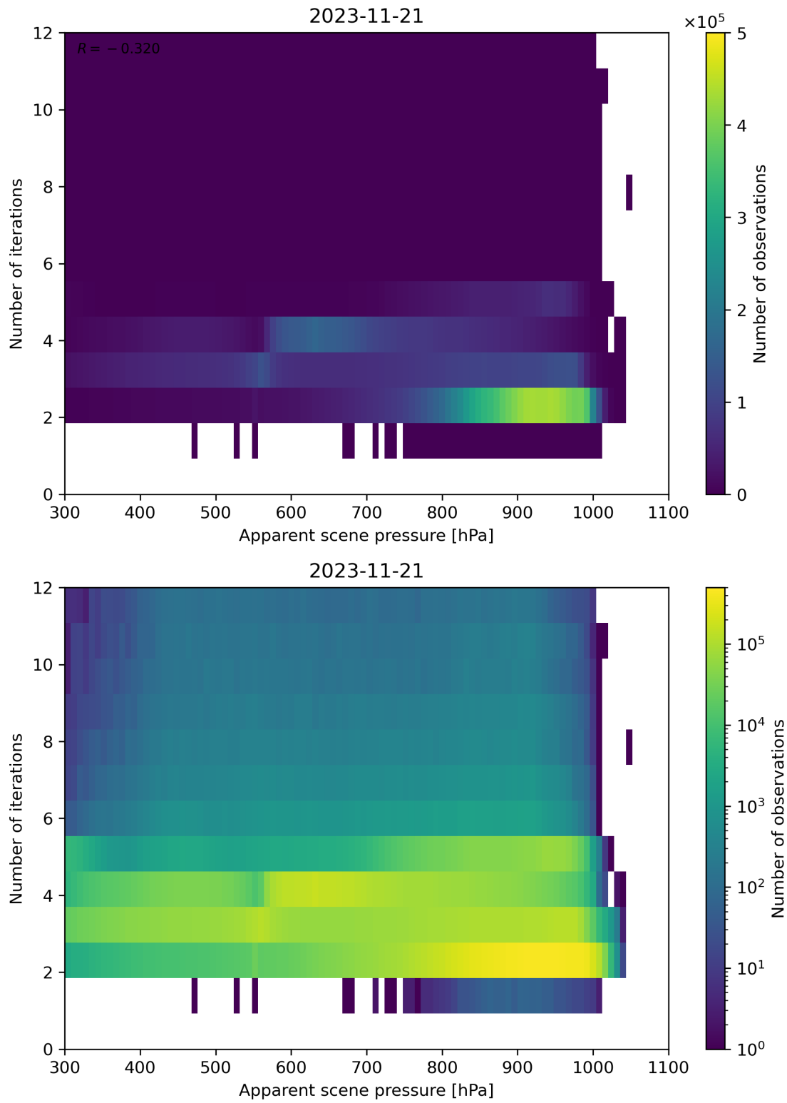
Figure 66: Scatter density plot of “Apparent scene pressure” against “Number of iterations” for 2023-11-20 to 2023-11-22.
