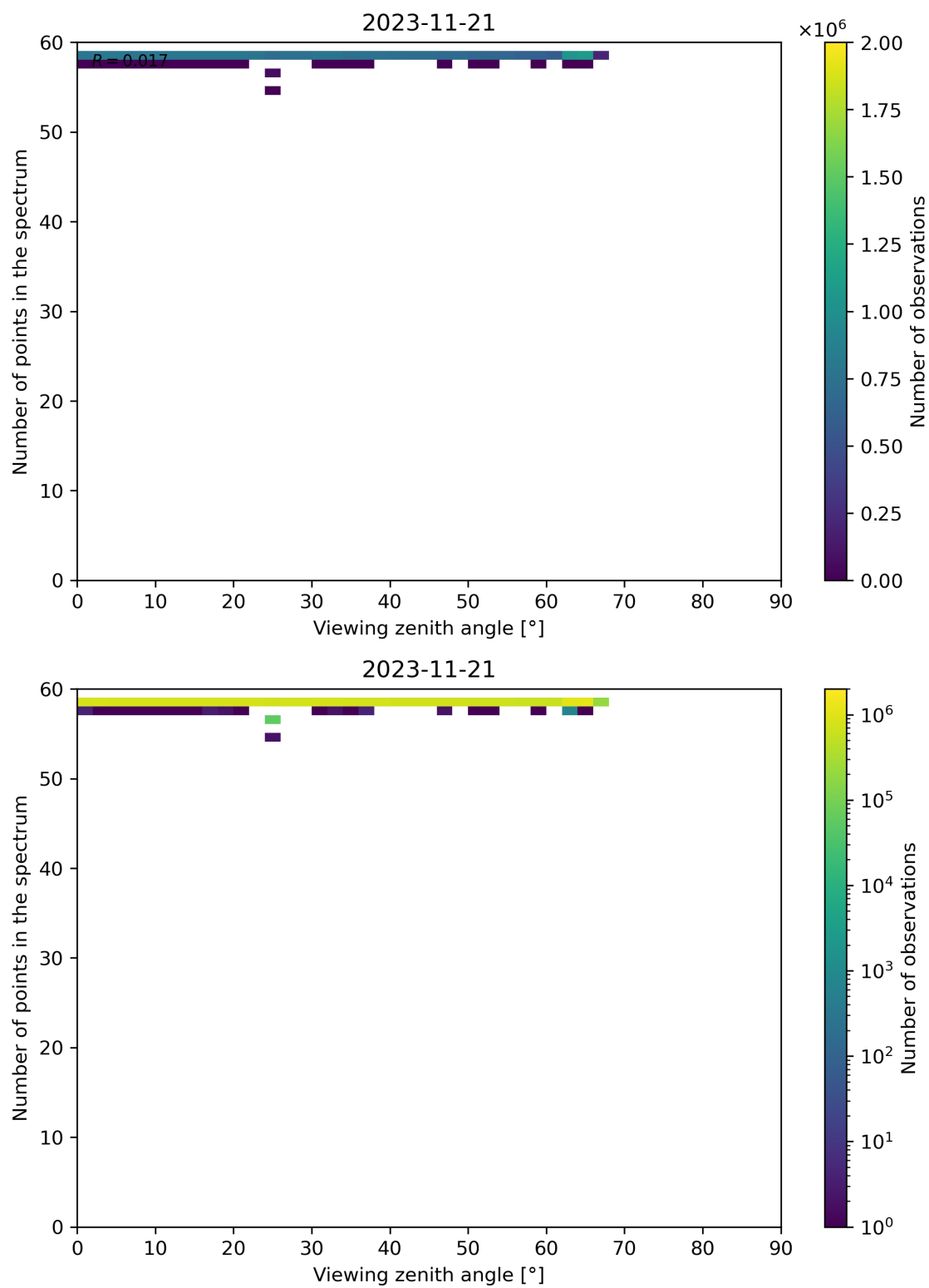
Figure 137: Scatter density plot of “Viewing zenith angle” against “Number of points in the spectrum” for 2023-11-20 to 2023-11-22.
