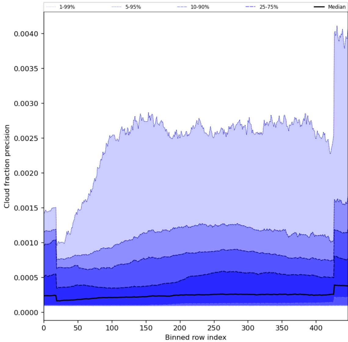
Figure 50: Along track statistics of “Cloud fraction precision” for 2023-11-20 to 2023-11-22
