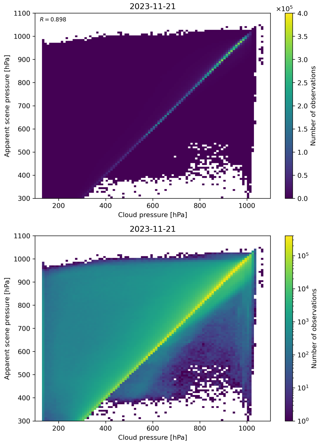
Figure 84: Scatter density plot of “Cloud pressure” against “Apparent scene pressure” for 2023-11-20 to 2023-11-22.
