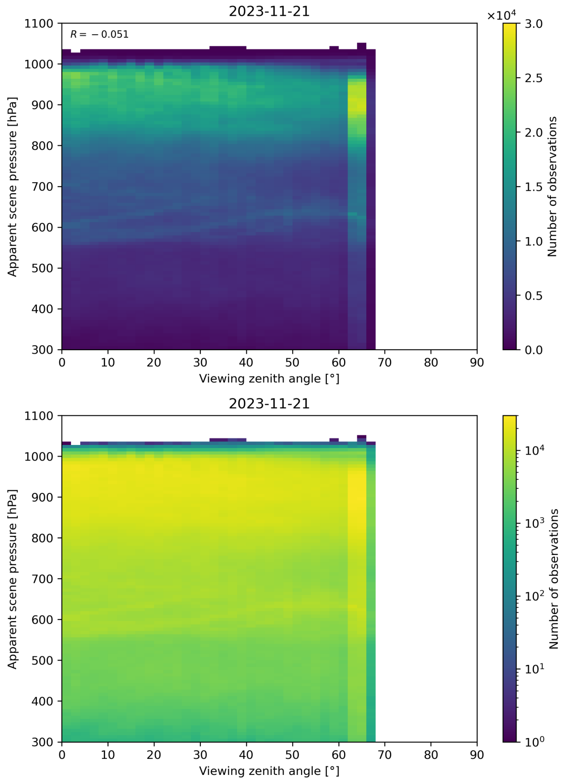
Figure 129: Scatter density plot of “Viewing zenith angle” against “Apparent scene pressure” for 2023-11-20 to 2023-11-22.
