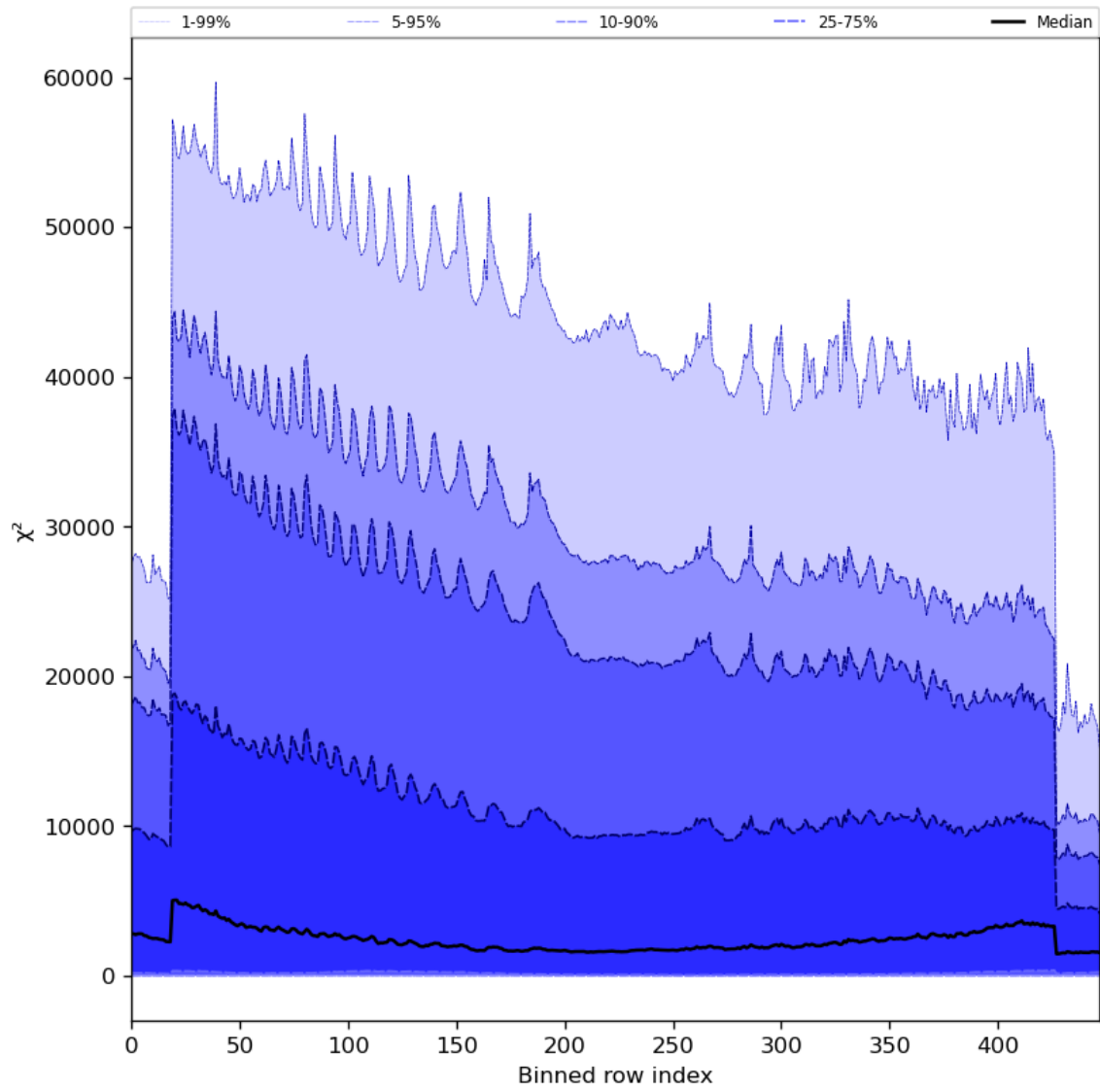
Figure 55: Along track statistics of “ \chi^2 ” for 2023-11-20 to 2023-11-22
