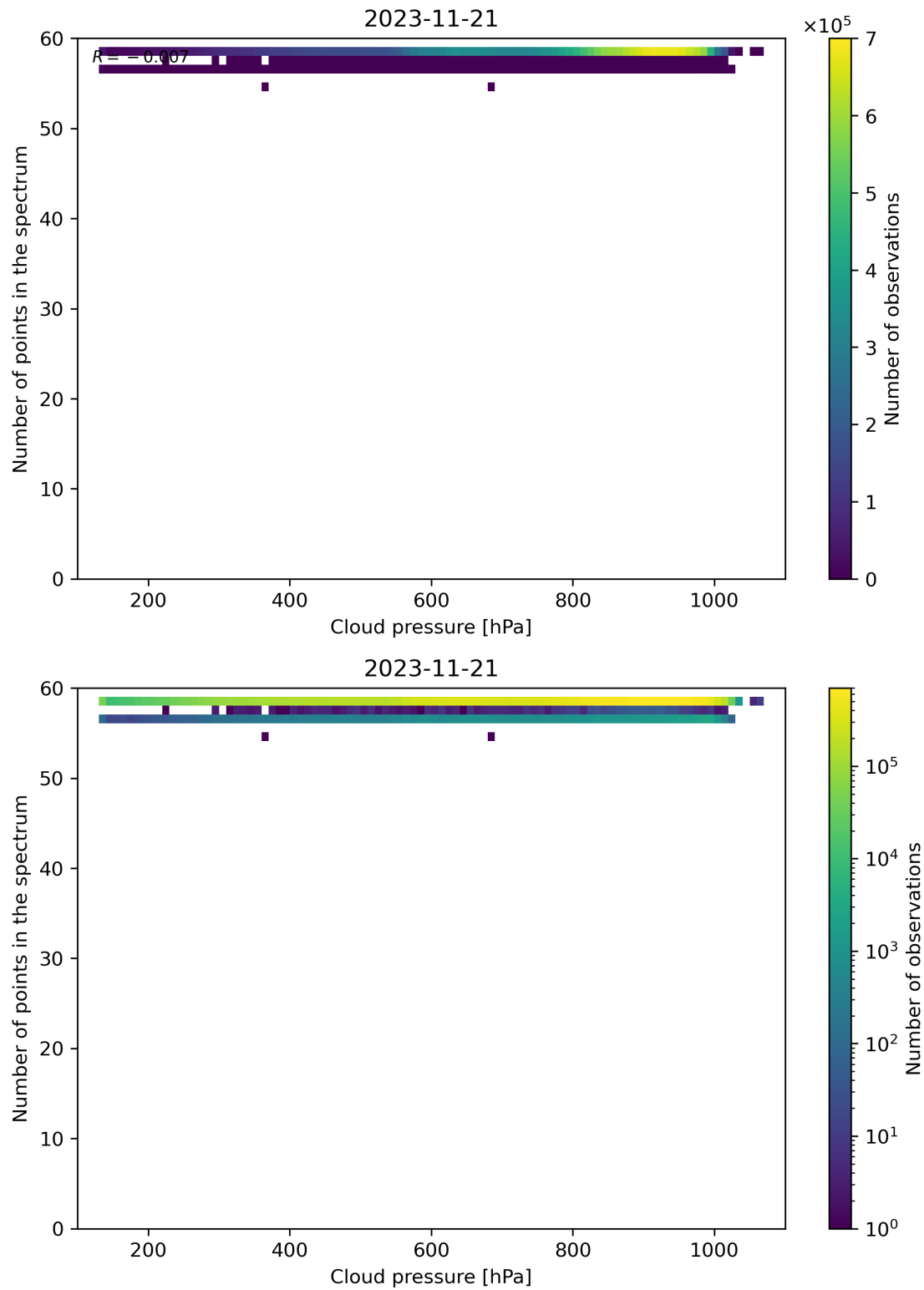
Figure 90: Scatter density plot of “Cloud pressure” against “Number of points in the spectrum” for 2023-11-20 to 2023-11-22.
