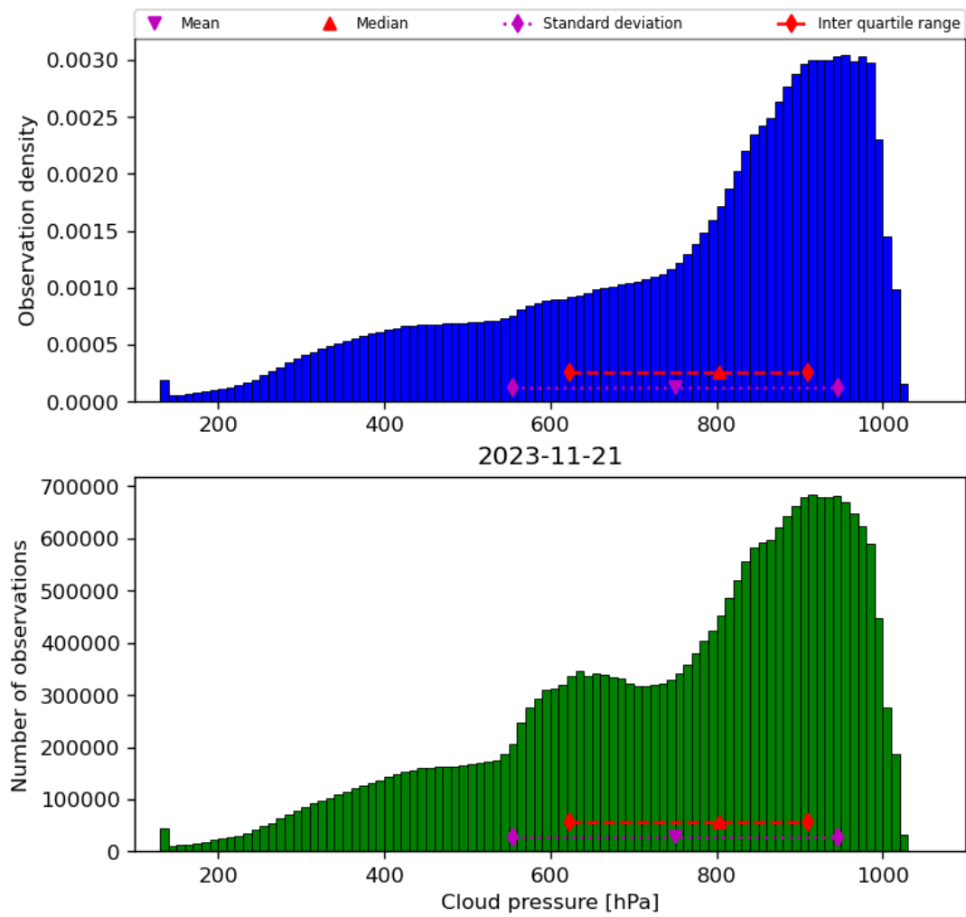
Figure 30: Histogram of “Cloud pressure” for 2023-11-20 to 2023-11-22
