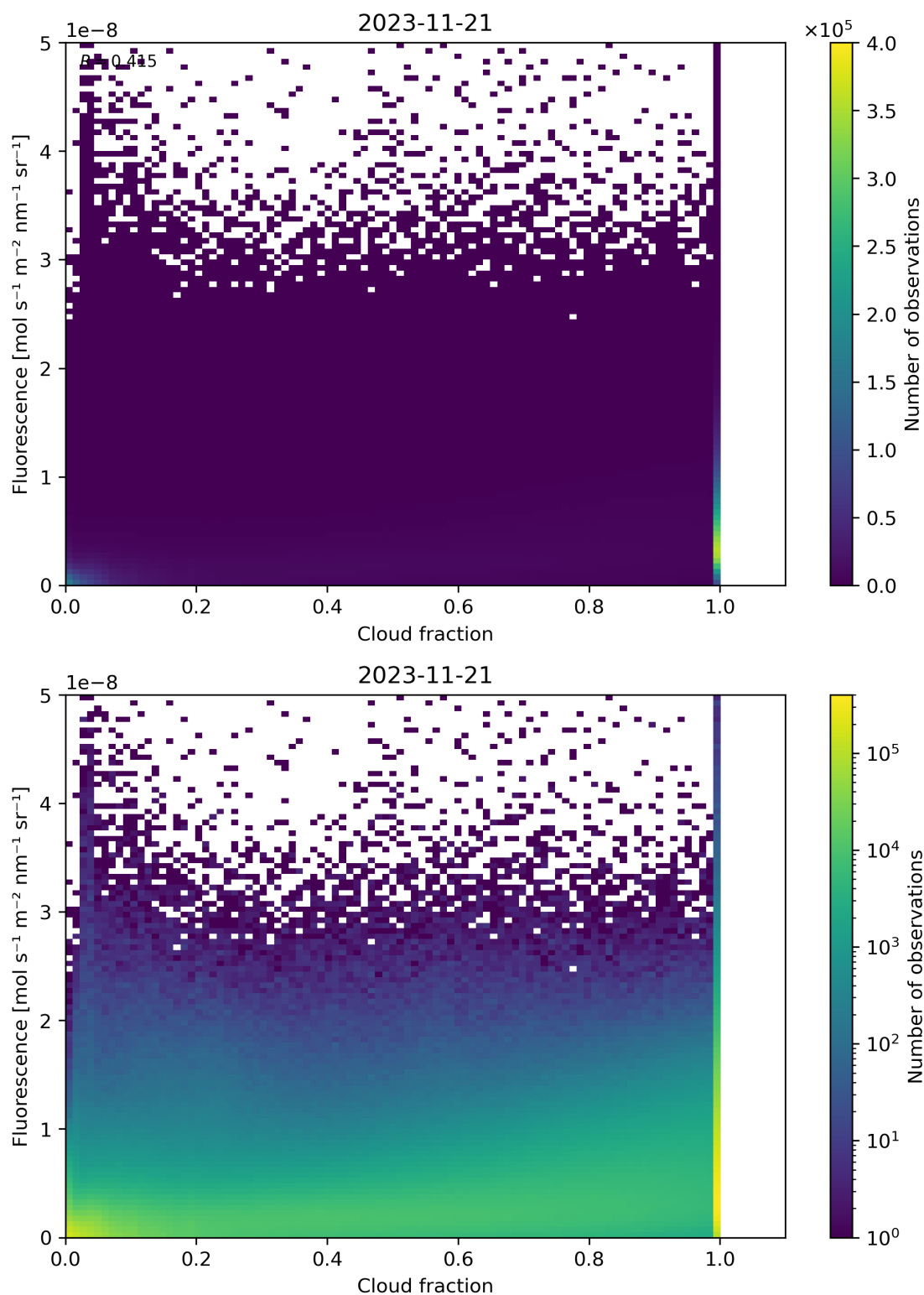
Figure 79: Scatter density plot of “Cloud fraction” against “Fluorescence” for 2023-11-20 to 2023-11-22.
