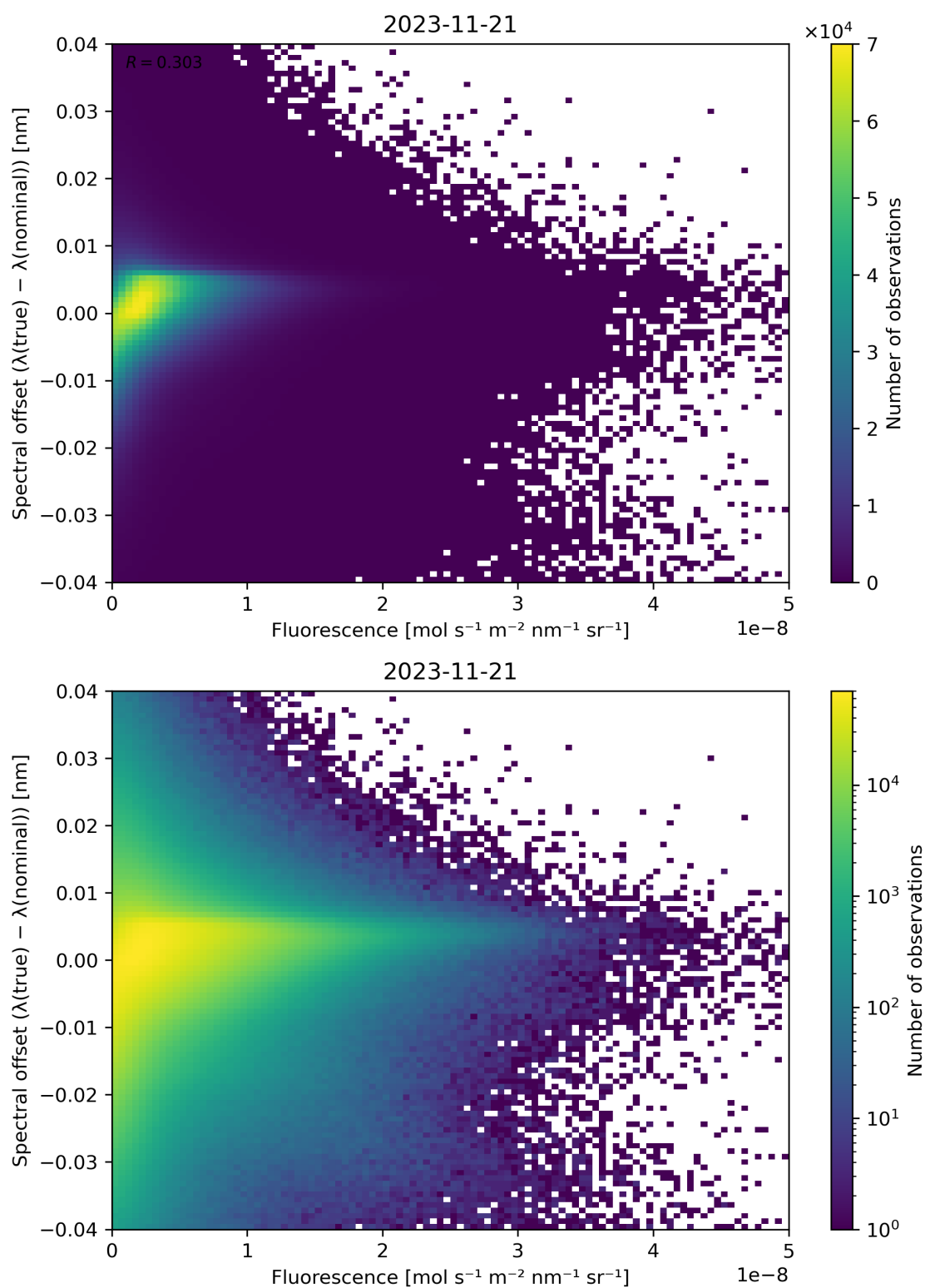
Figure 95: Scatter density plot of “Fluorescence” against “Spectral offset ( \lambda(\text{true}) - \lambda(\text{nominal}) )” for 2023-11-20 to 2023-11-22.
