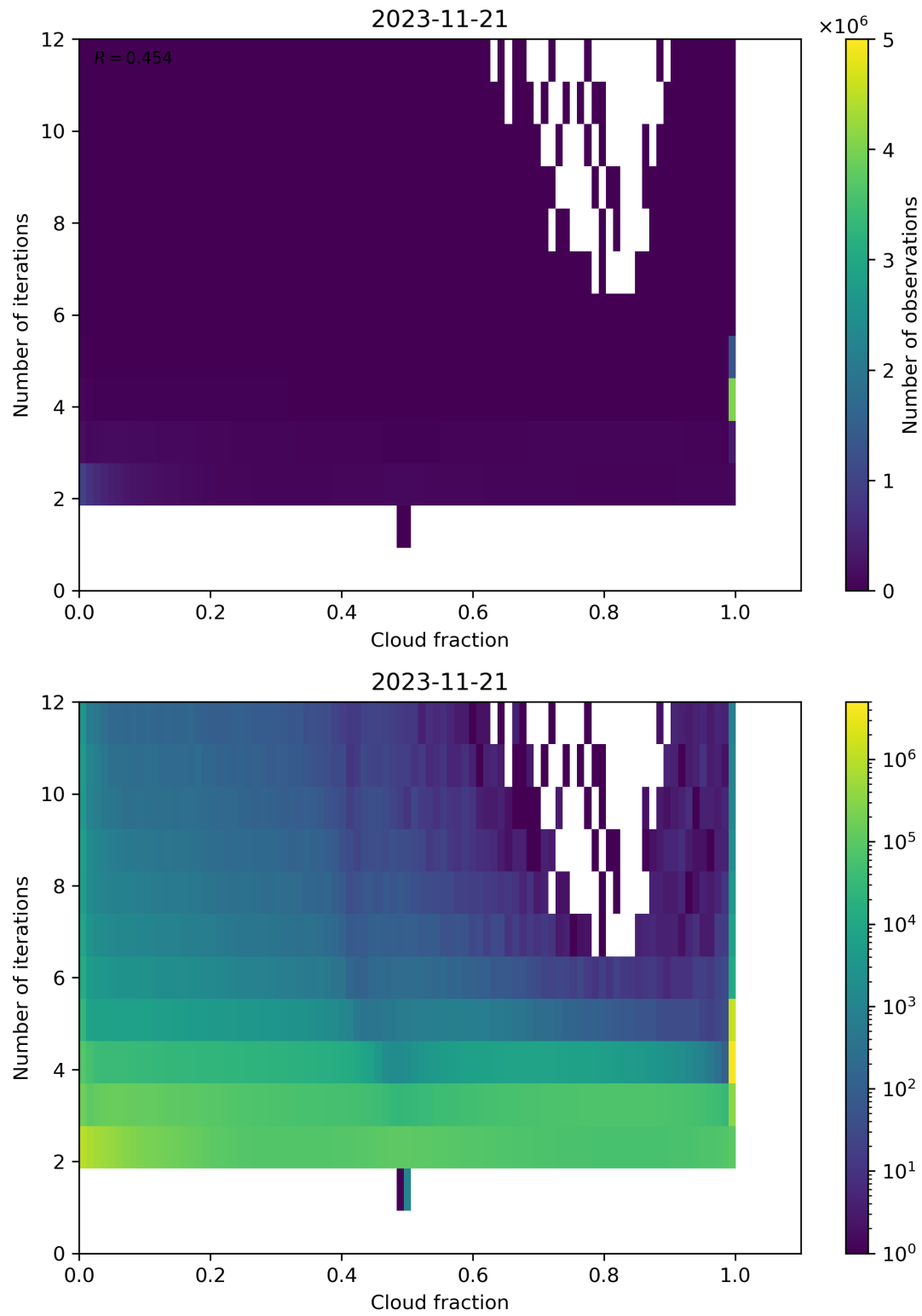
Figure 80: Scatter density plot of “Cloud fraction” against “Number of iterations” for 2023-11-20 to 2023-11-22.
