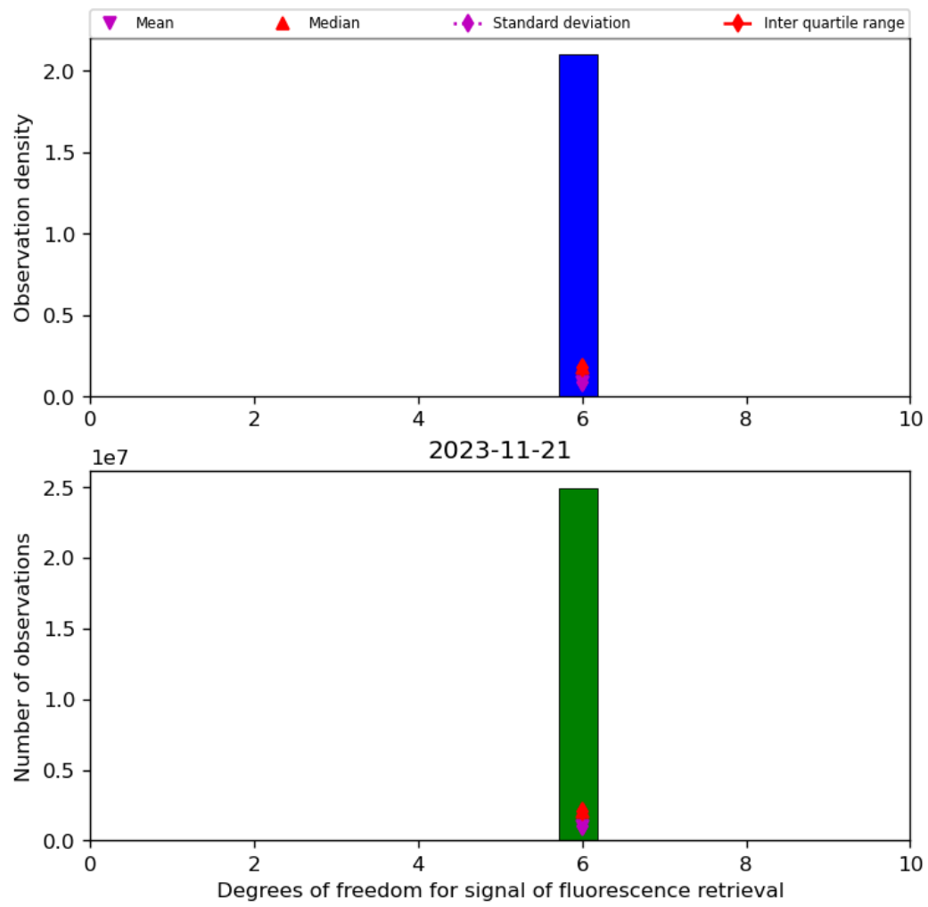
Figure 43: Histogram of “Degrees of freedom for signal of fluorescence retrieval” for 2023-11-20 to 2023-11-22
