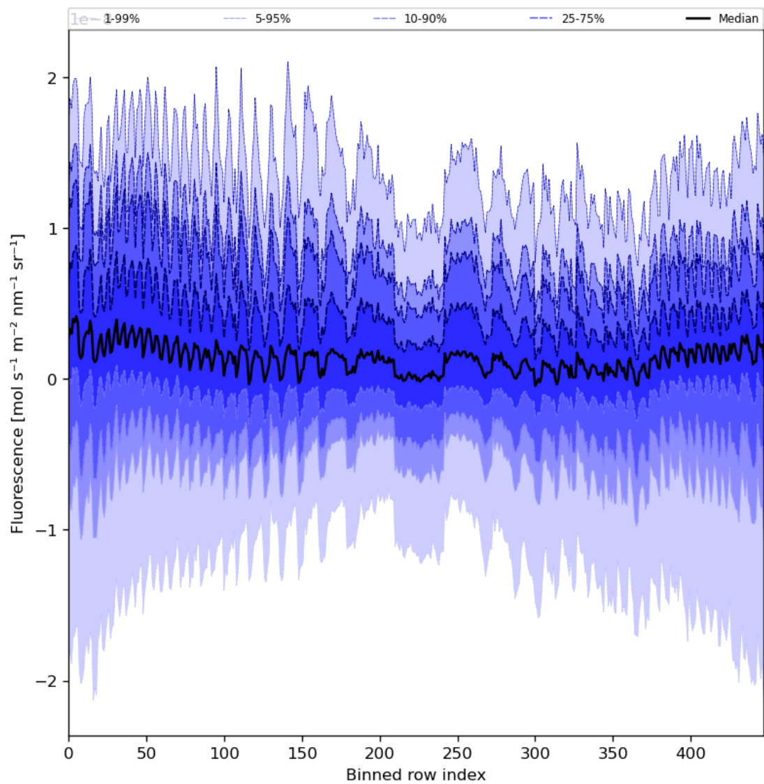
Figure 57: Along track statistics of “Fluorescence” for 2023-11-20 to 2023-11-22
