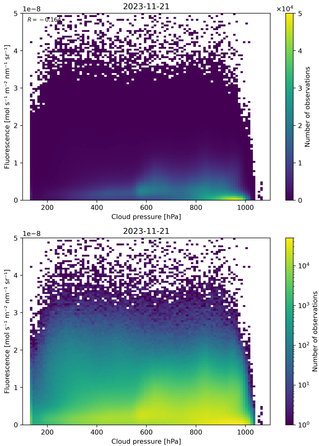
Figure 88: Scatter density plot of “Cloud pressure” against “Fluorescence” for 2023-11-20 to 2023-11-22.
