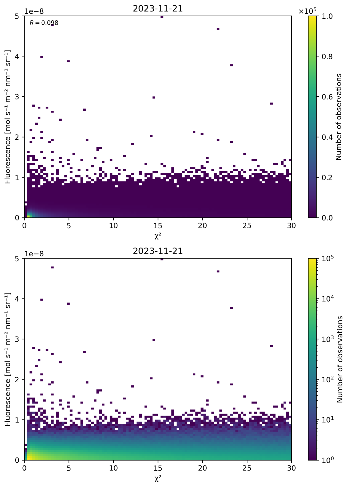
Figure 70: Scatter density plot of “ \chi^2 ” against “Fluorescence” for 2023-11-20 to 2023-11-22.
