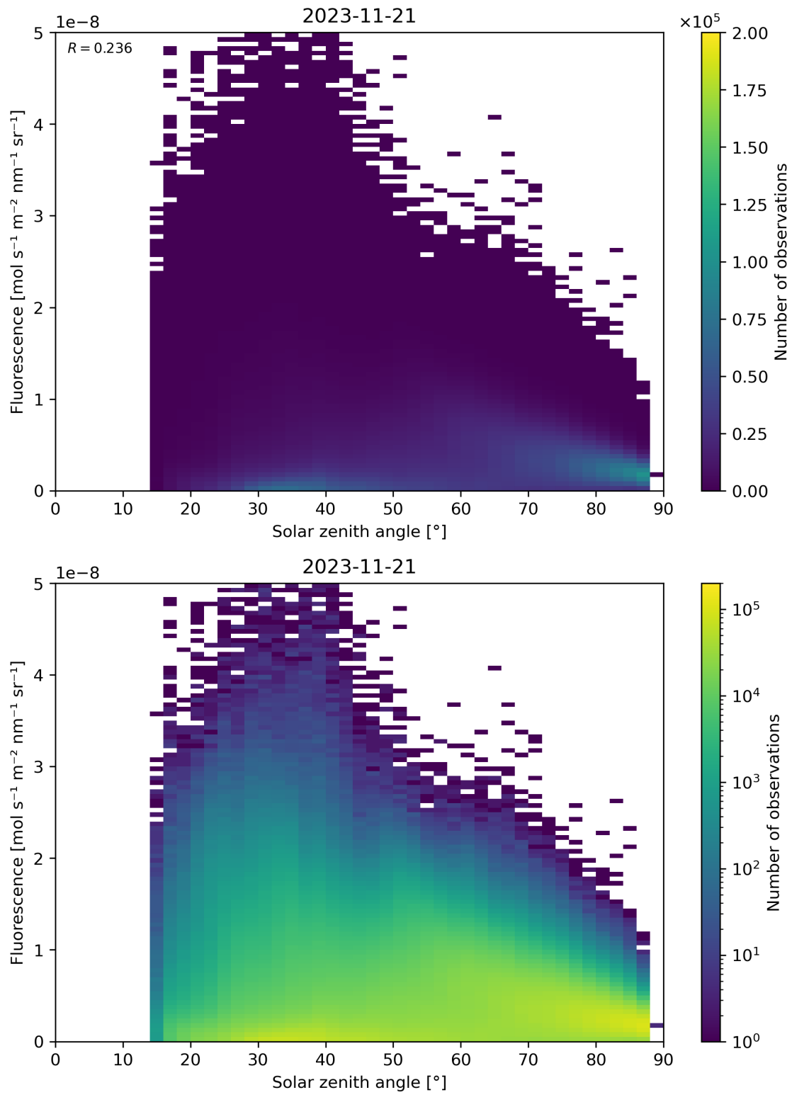
Figure 123: Scatter density plot of “Solar zenith angle” against “Fluorescence” for 2023-11-20 to 2023-11-22.
