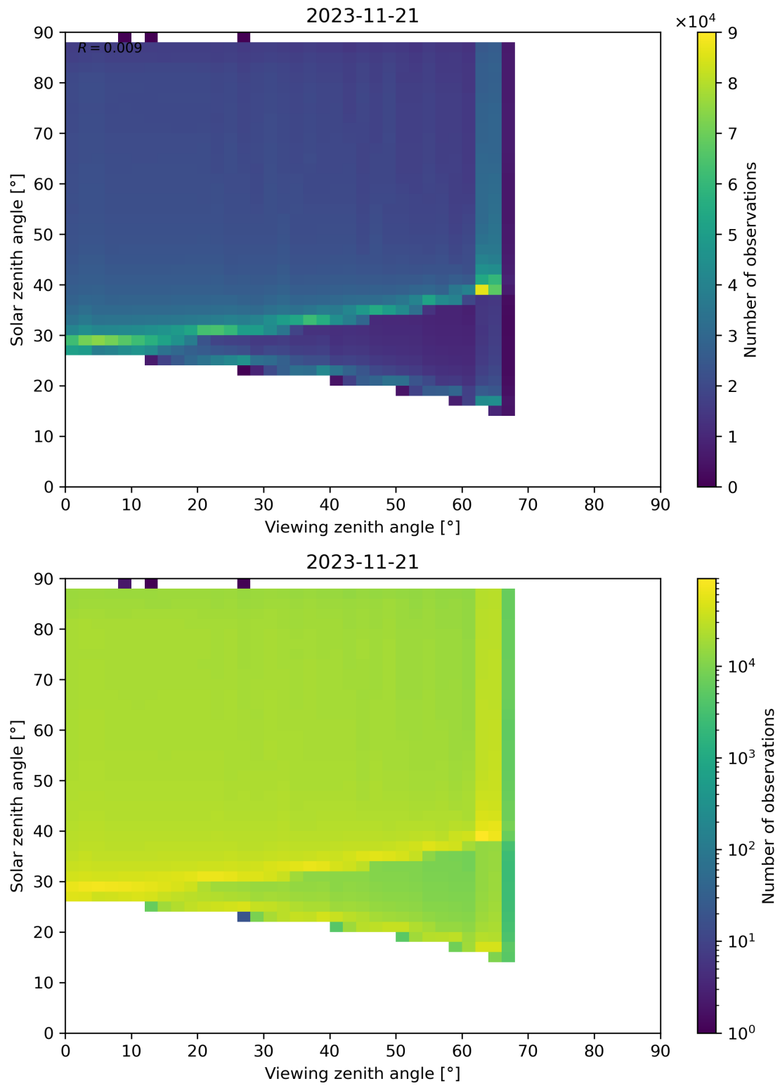
Figure 139: Scatter density plot of “Viewing zenith angle” against “Solar zenith angle” for 2023-11-20 to 2023-11-22.
