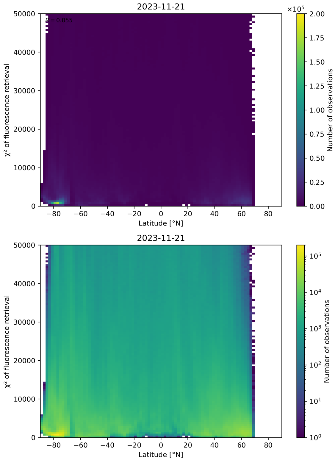
Figure 98: Scatter density plot of “Latitude” against “ \chi^2 of fluorescence retrieval” for 2023-11-20 to 2023-11-22.
