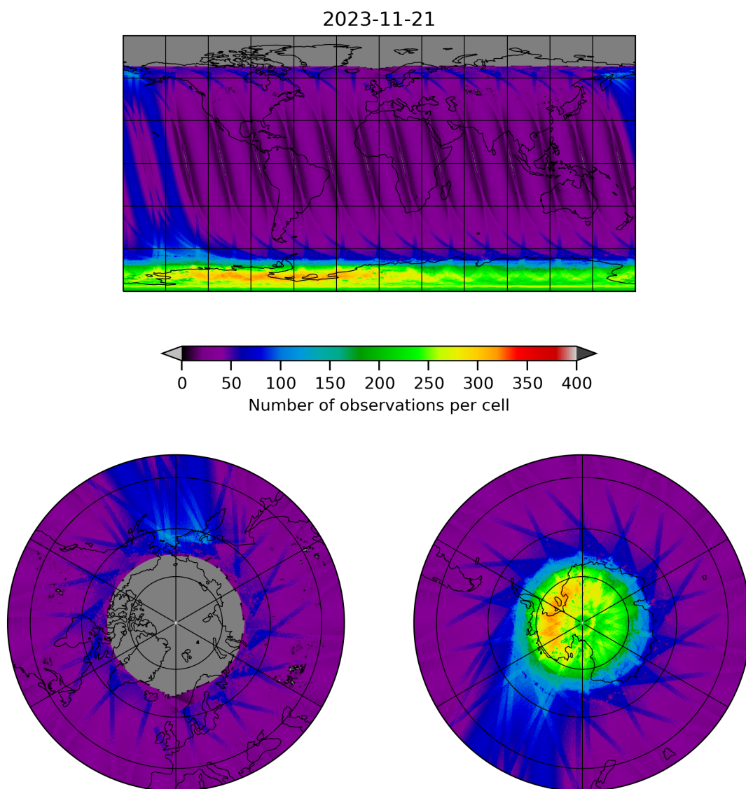
Figure 11: Map of the number of observations for 2023-11-20 to 2023-11-22
