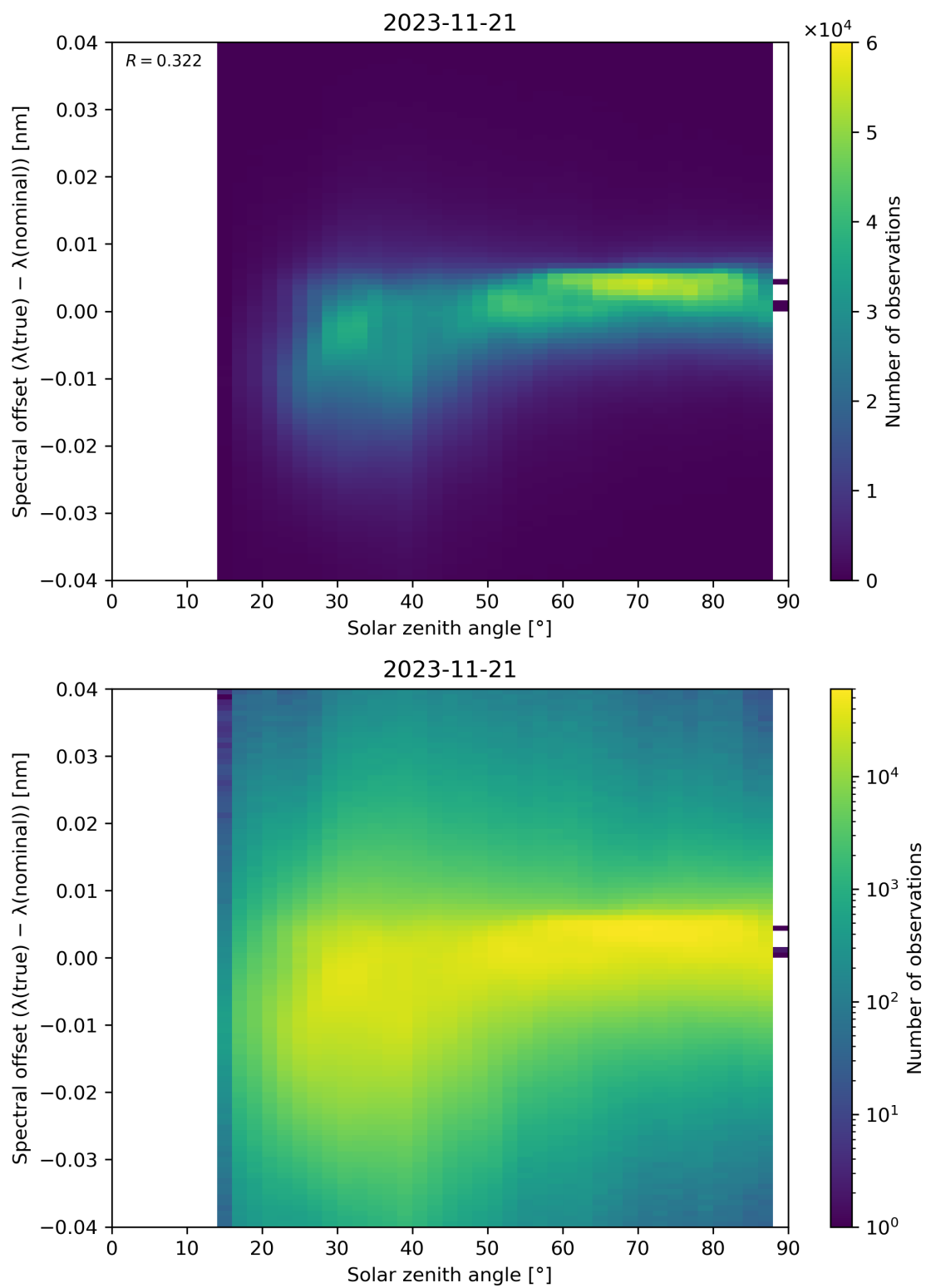
Figure 128: Scatter density plot of “Solar zenith angle” against “Spectral offset ( \lambda(\text{true}) - \lambda(\text{nominal}) )” for 2023-11-20 to 2023-11-22.
