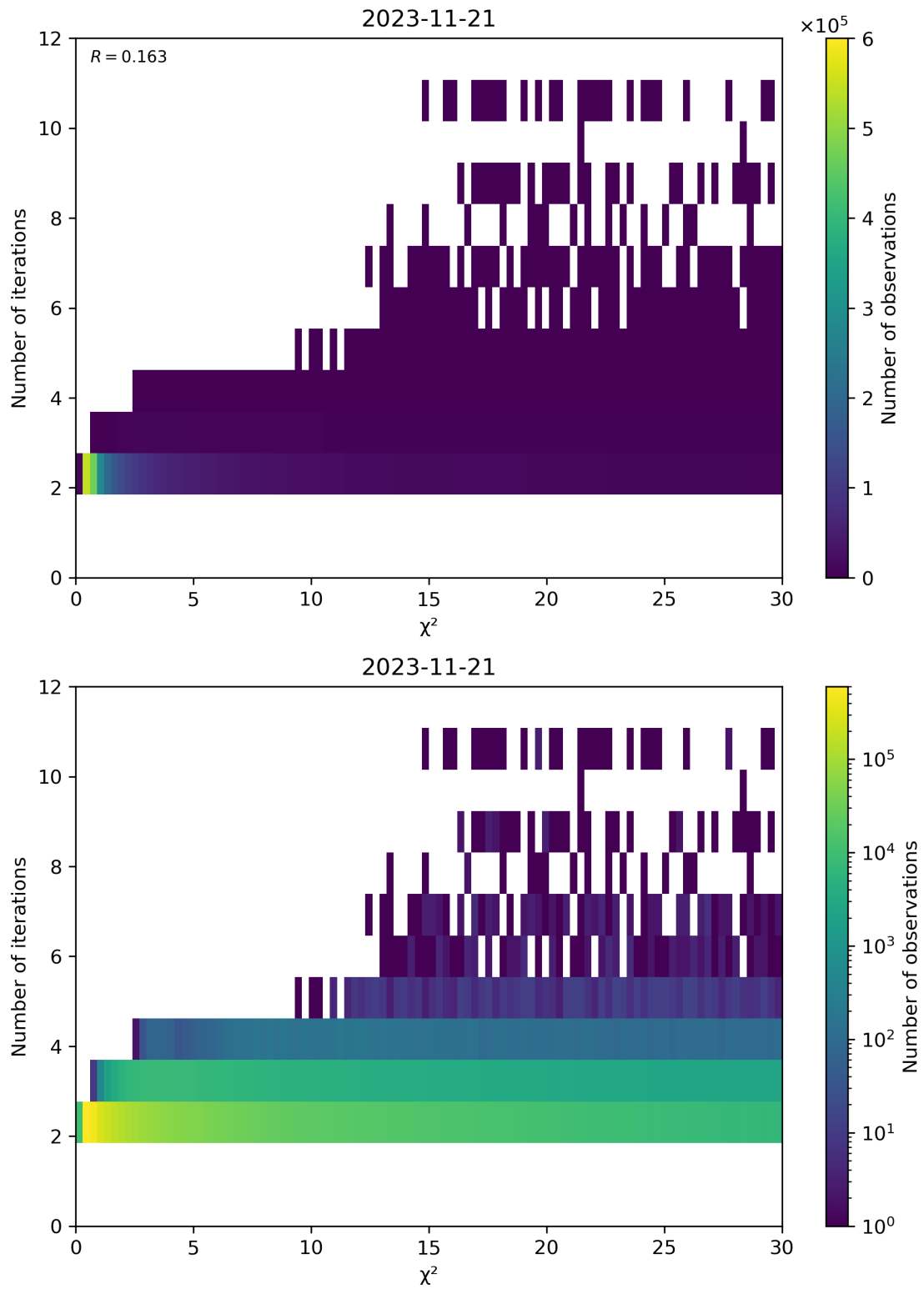
Figure 73: Scatter density plot of “ \chi^2 ” against “Number of iterations” for 2023-11-20 to 2023-11-22.
