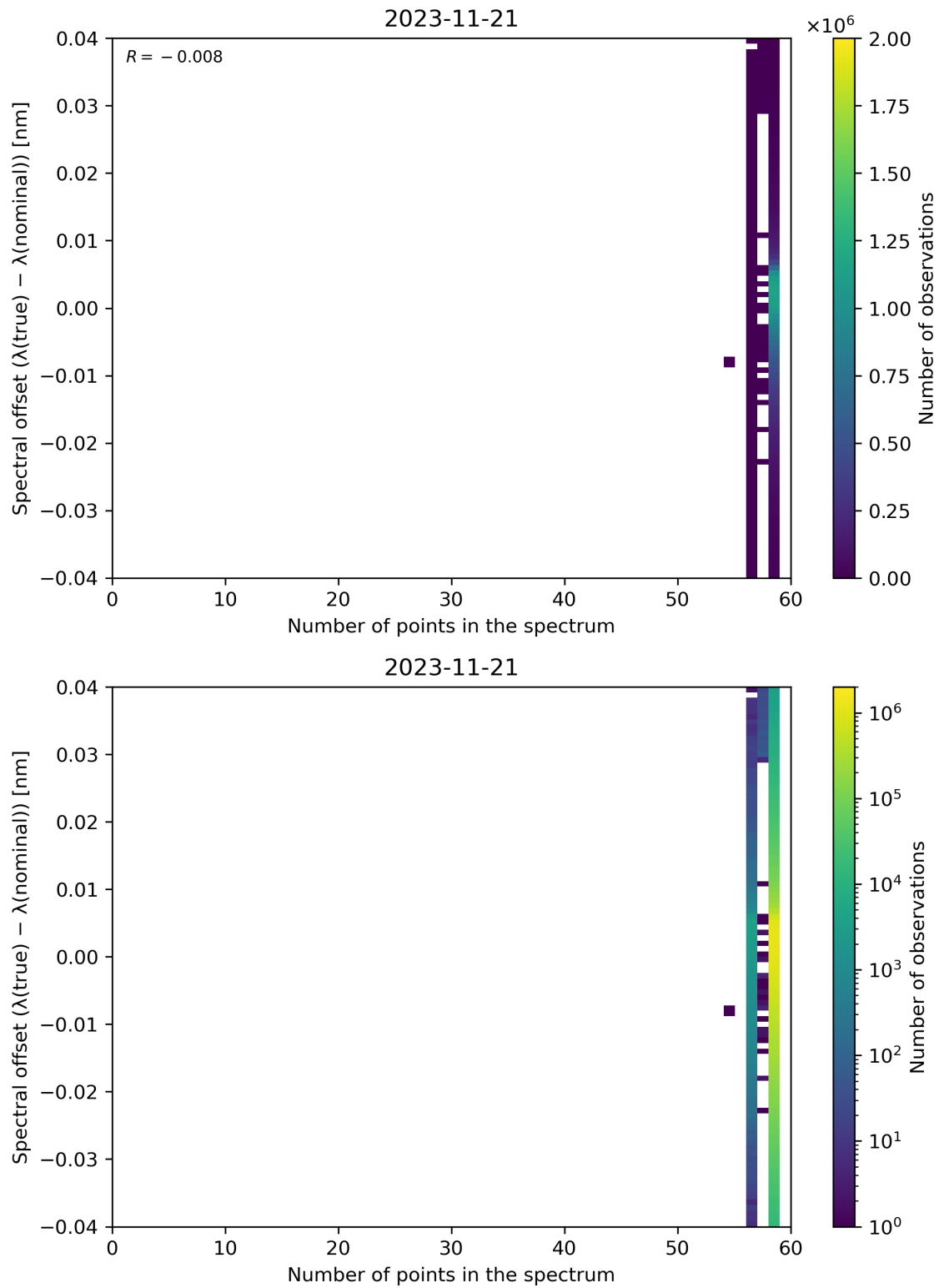
Figure 110: Scatter density plot of “Number of points in the spectrum” against “Spectral offset ( \lambda(\text{true}) - \lambda(\text{nominal}) )” for 2023-11-20 to 2023-11-22.
