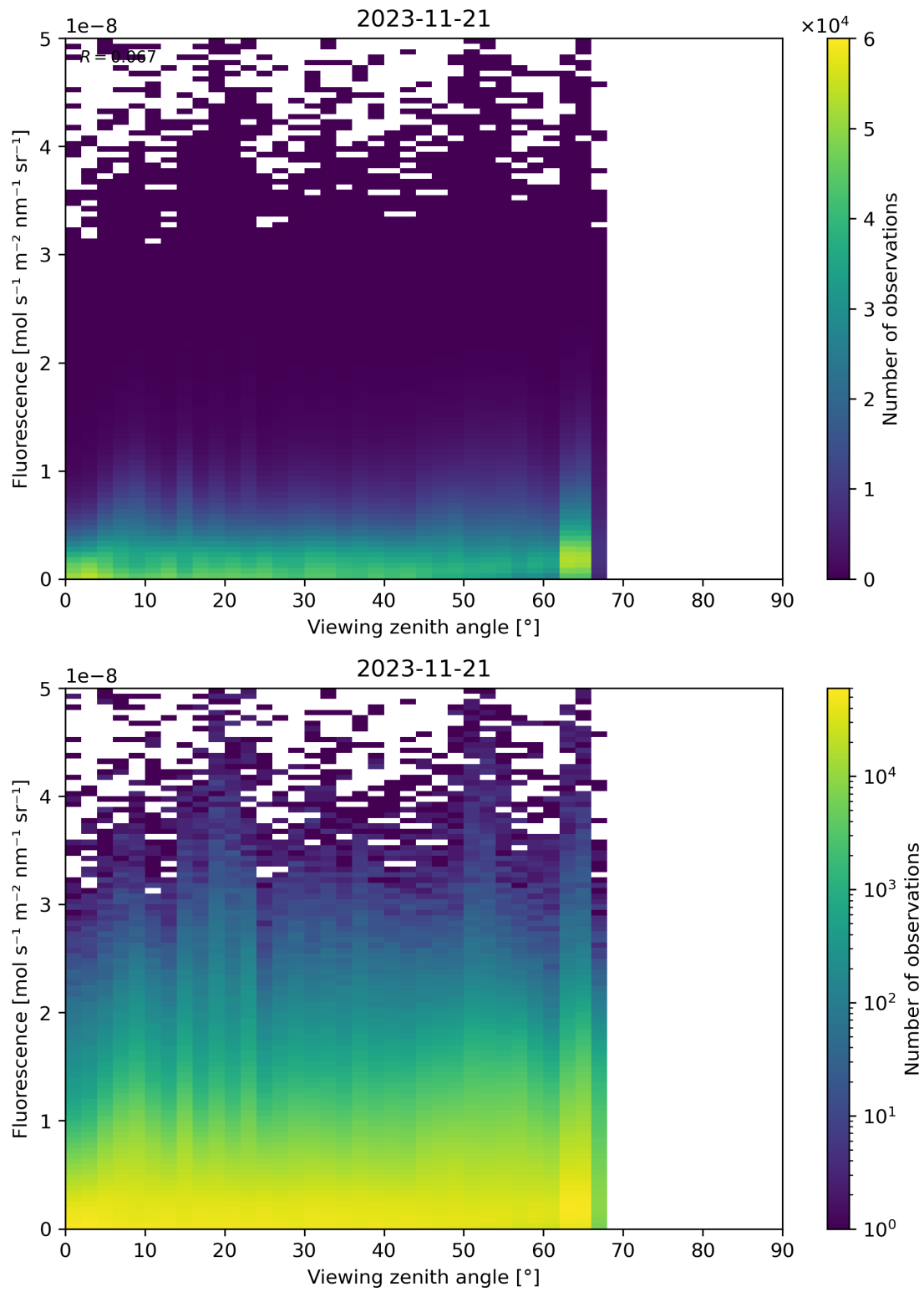
Figure 134: Scatter density plot of “Viewing zenith angle” against “Fluorescence” for 2023-11-20 to 2023-11-22.
