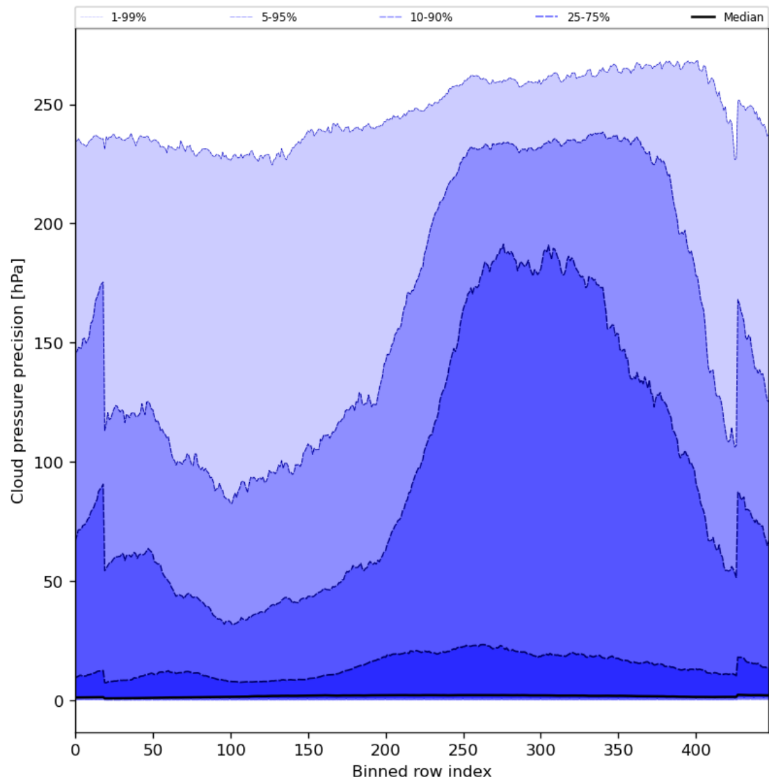
Figure 48: Along track statistics of “Cloud pressure precision” for 2023-11-20 to 2023-11-22
