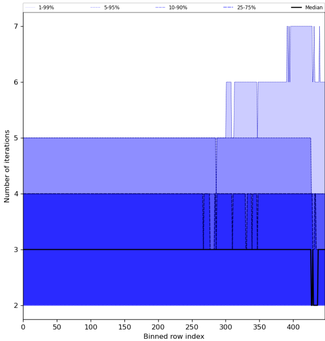
Figure 56: Along track statistics of “Number of iterations” for 2023-11-20 to 2023-11-22
