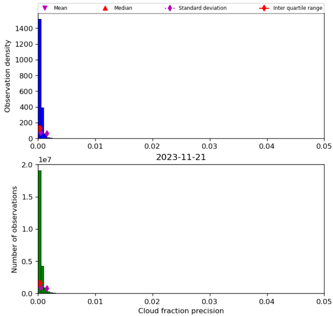
Figure 33: Histogram of “Cloud fraction precision” for 2023-11-20 to 2023-11-22
