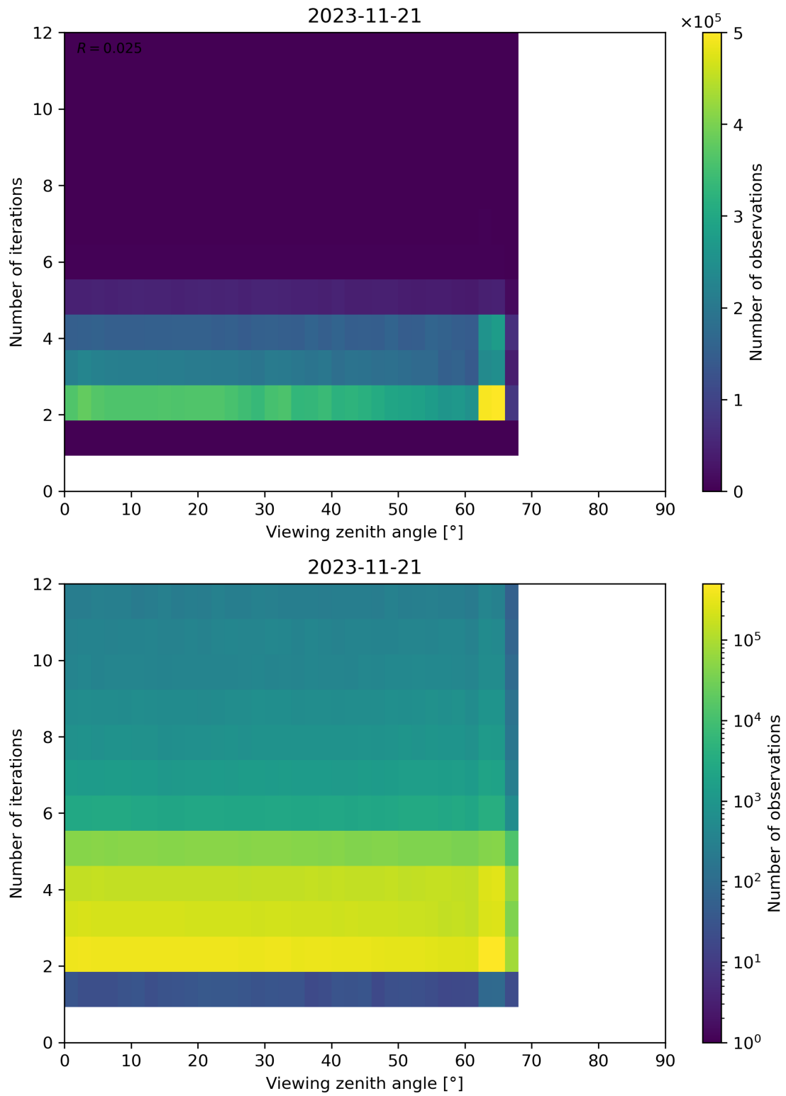
Figure 136: Scatter density plot of “Viewing zenith angle” against “Number of iterations” for 2023-11-20 to 2023-11-22.
