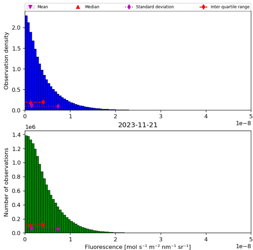
Figure 40: Histogram of “Fluorescence” for 2023-11-20 to 2023-11-22
