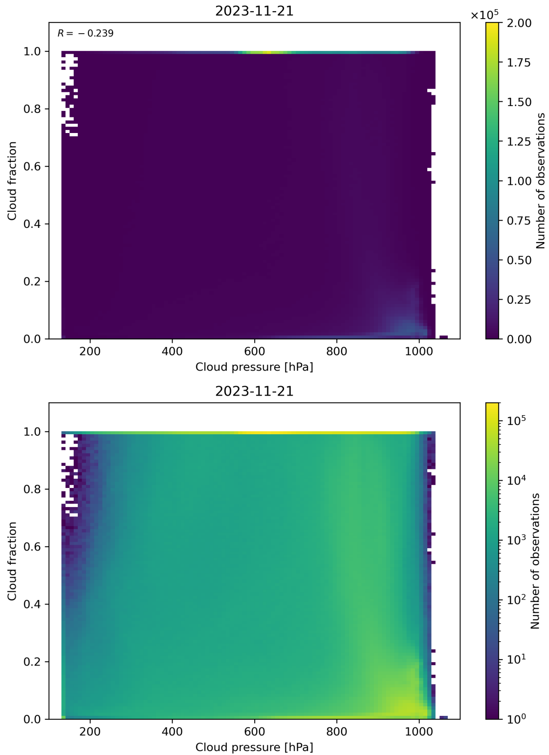
Figure 87: Scatter density plot of “Cloud pressure” against “Cloud fraction” for 2023-11-20 to 2023-11-22.
