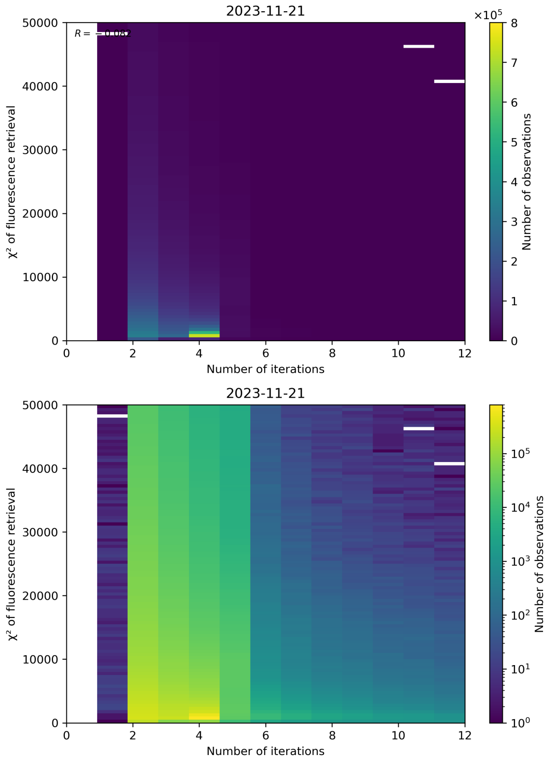
Figure 106: Scatter density plot of “Number of iterations” against “ \chi^2 of fluorescence retrieval” for 2023-11-20 to 2023-11-22.
