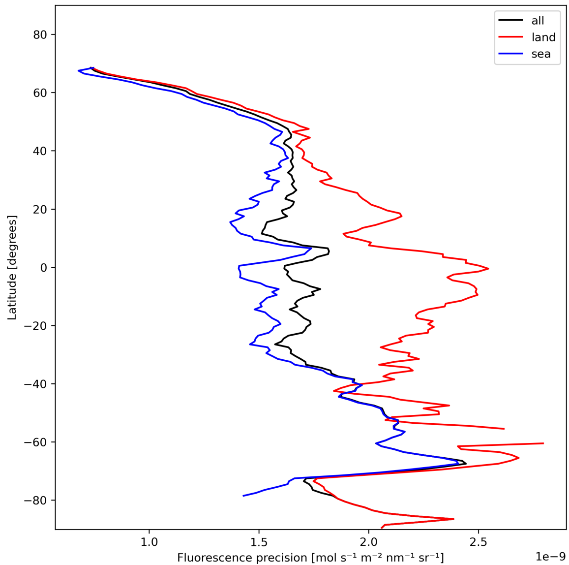
Figure 24: Zonal average of “Fluorescence precision” for 2023-11-20 to 2023-11-22.
