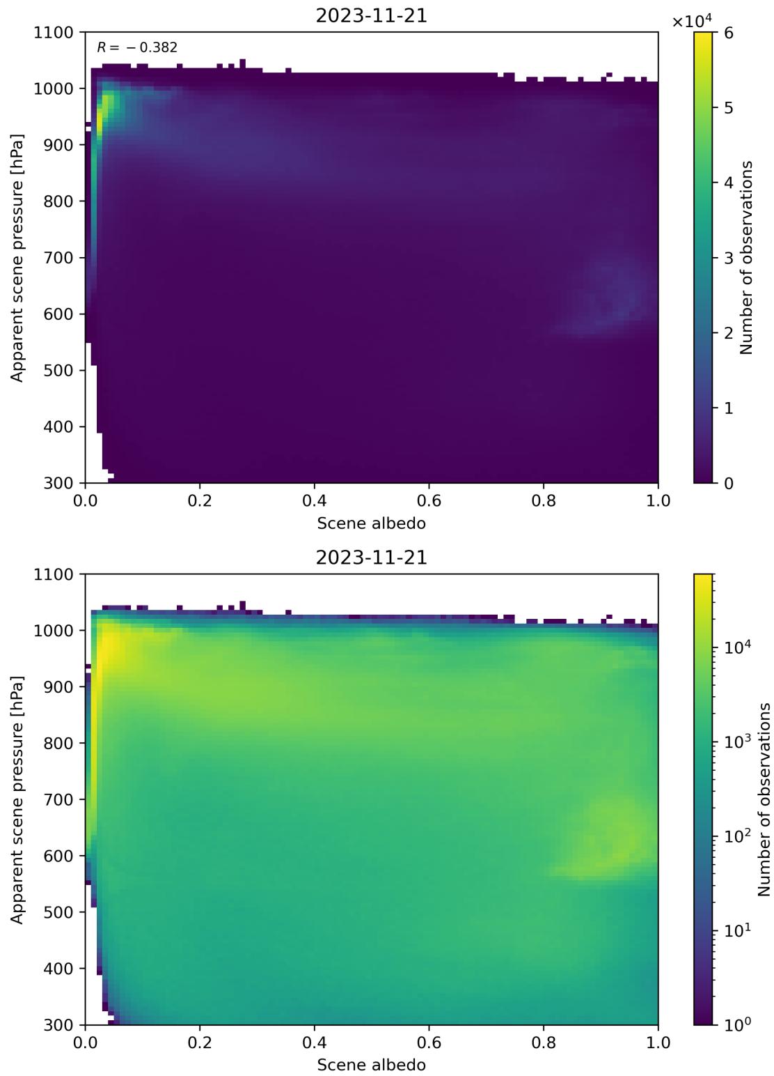
Figure 111: Scatter density plot of “Scene albedo” against “Apparent scene pressure” for 2023-11-20 to 2023-11-22.
