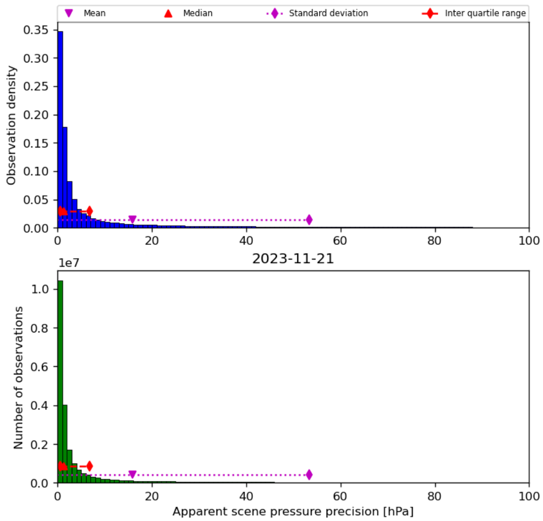
Figure 37: Histogram of “Apparent scene pressure precision” for 2023-11-20 to 2023-11-22
