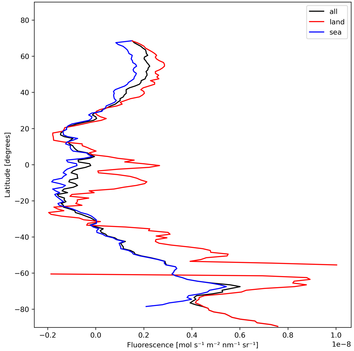
Figure 23: Zonal average of “Fluorescence” for 2023-11-20 to 2023-11-22.
