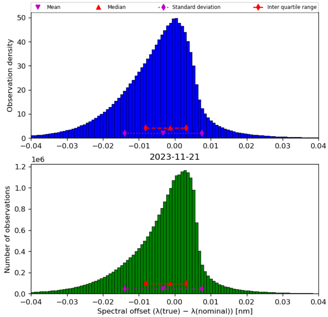
Figure 45: Histogram of “Spectral offset ( \lambda(\text{true}) - \lambda(\text{nominal}) )” for 2023-11-20 to 2023-11-22
