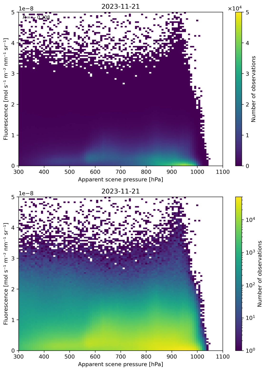
Figure 65: Scatter density plot of “Apparent scene pressure” against “Fluorescence” for 2023-11-20 to 2023-11-22.
