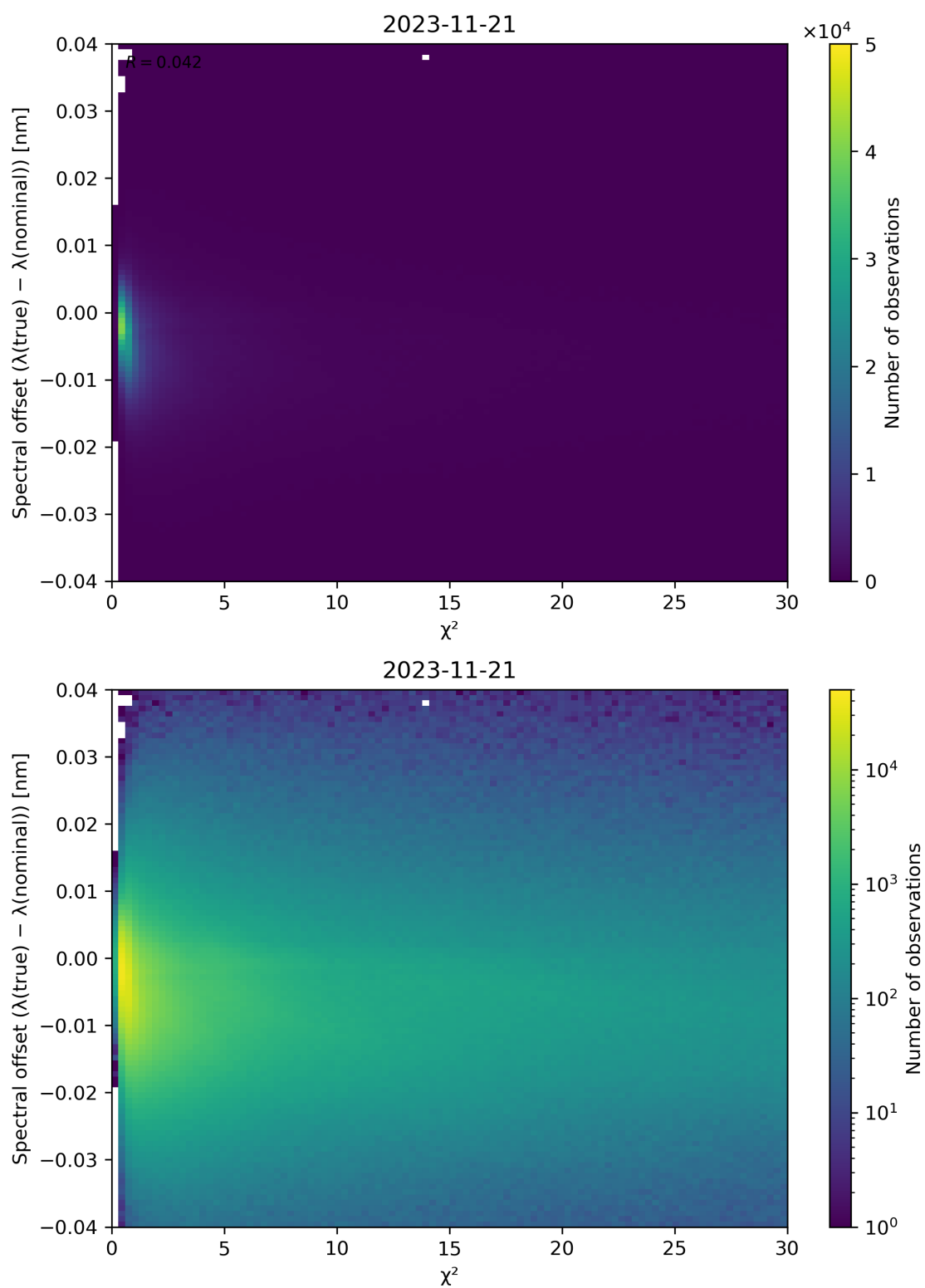
Figure 75: Scatter density plot of “ \chi^2 ” against “Spectral offset ( \lambda(\text{true}) - \lambda(\text{nominal}) )” for 2023-11-20 to 2023-11-22.
