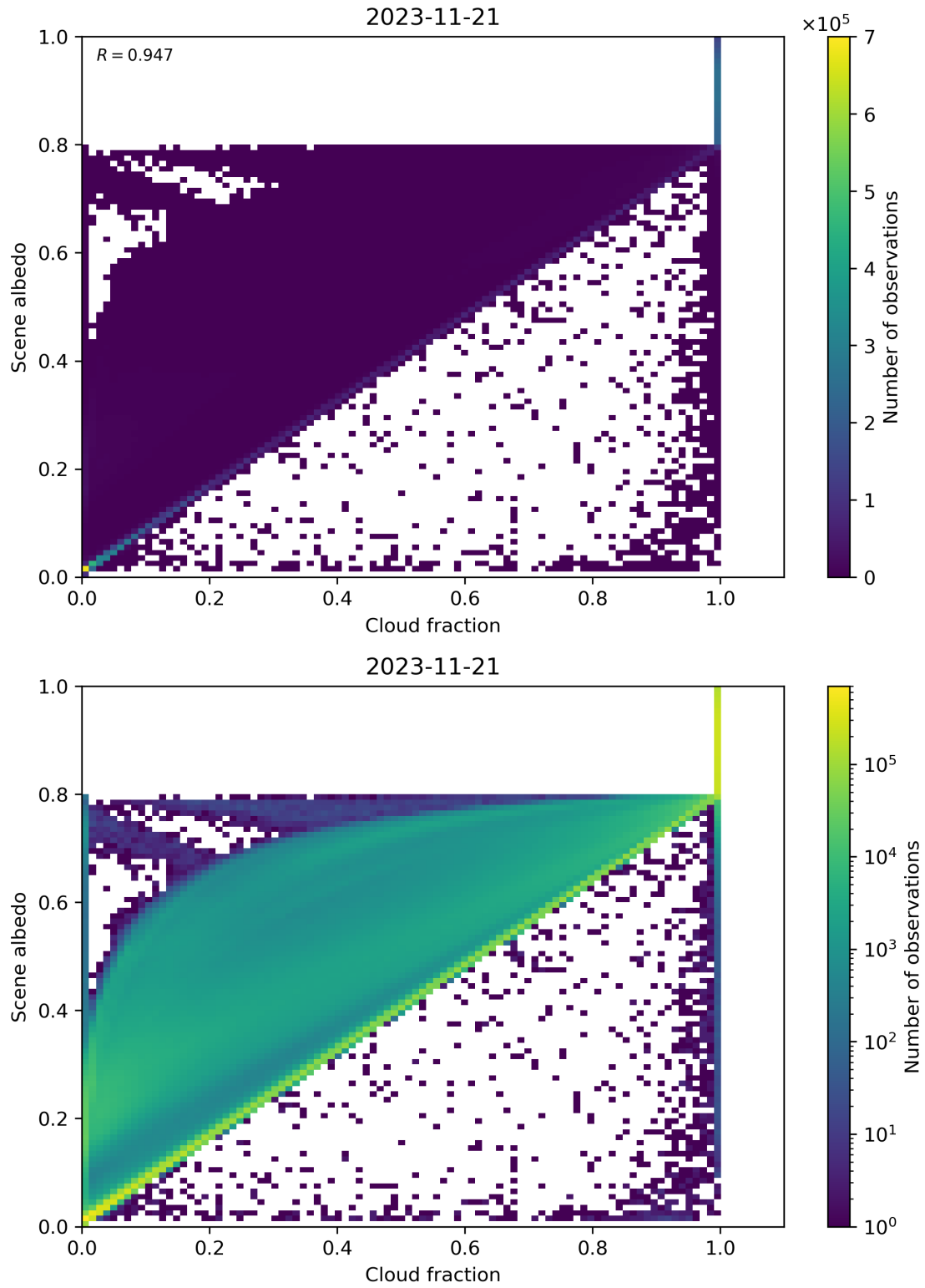
Figure 82: Scatter density plot of “Cloud fraction” against “Scene albedo” for 2023-11-20 to 2023-11-22.
