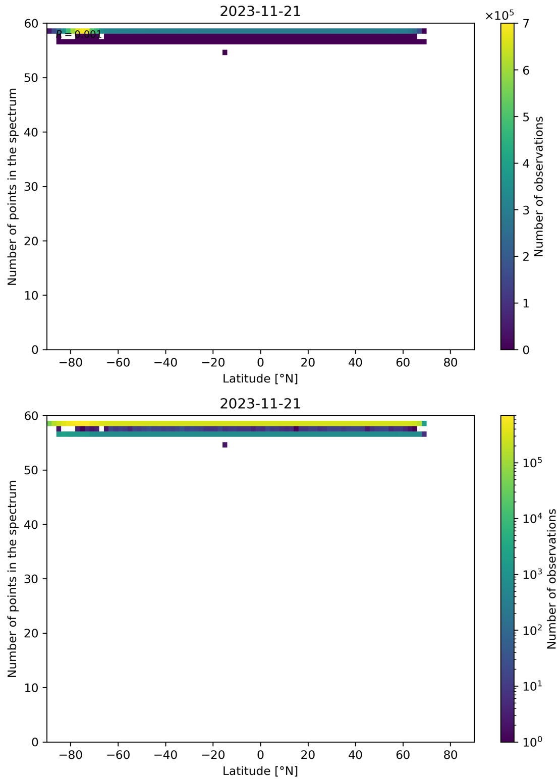
Figure 103: Scatter density plot of “Latitude” against “Number of points in the spectrum” for 2023-11-20 to 2023-11-22.
