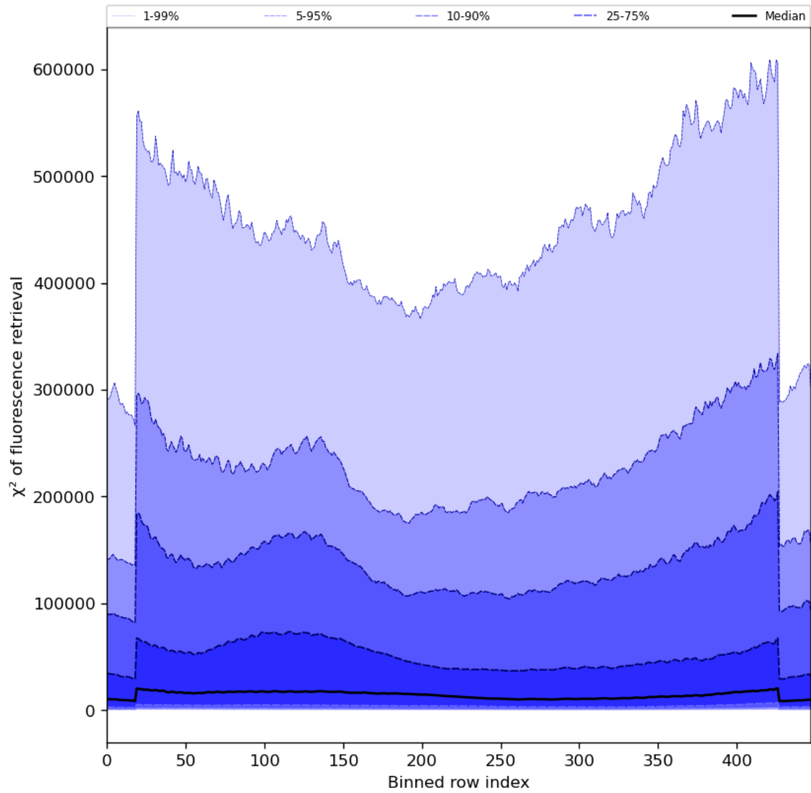
Figure 59: Along track statistics of “ \chi^2 of fluorescence retrieval” for 2023-11-20 to 2023-11-22
