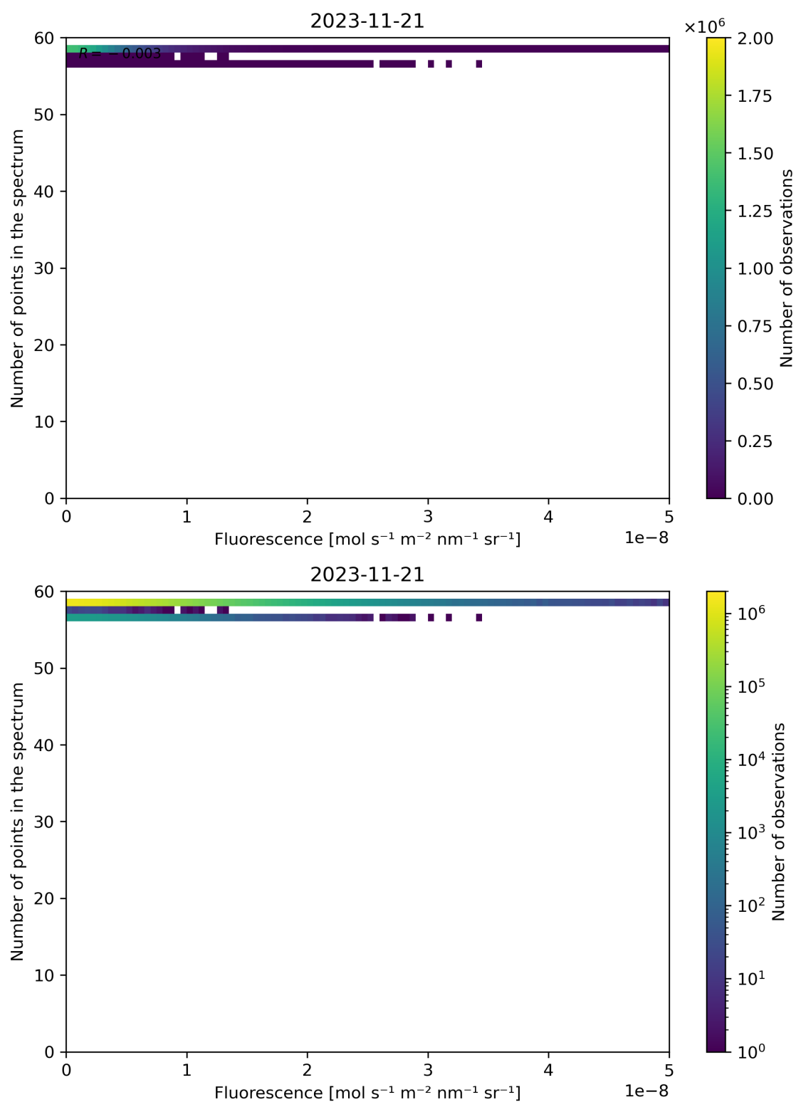
Figure 94: Scatter density plot of “Fluorescence” against “Number of points in the spectrum” for 2023-11-20 to 2023-11-22.
