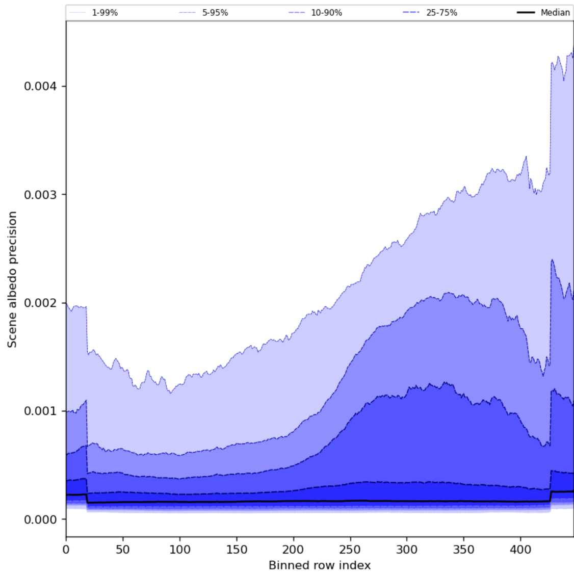
Figure 52: Along track statistics of “Scene albedo precision” for 2023-11-20 to 2023-11-22
