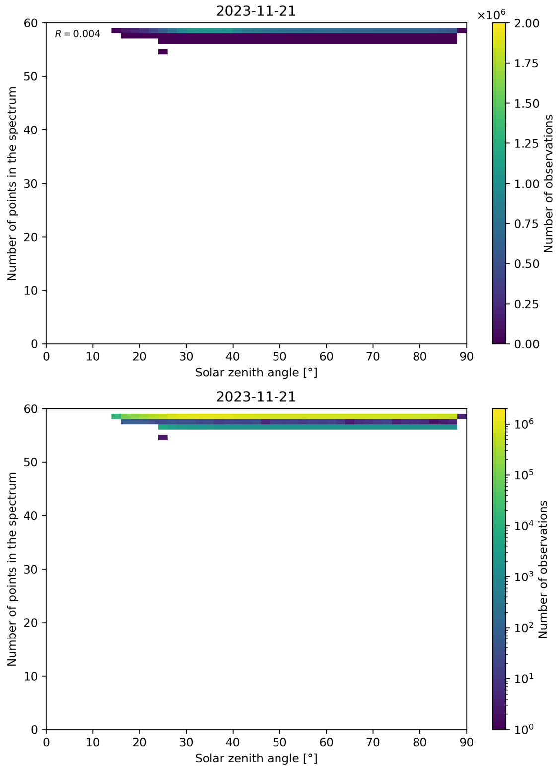
Figure 126: Scatter density plot of “Solar zenith angle” against “Number of points in the spectrum” for 2023-11-20 to 2023-11-22.
