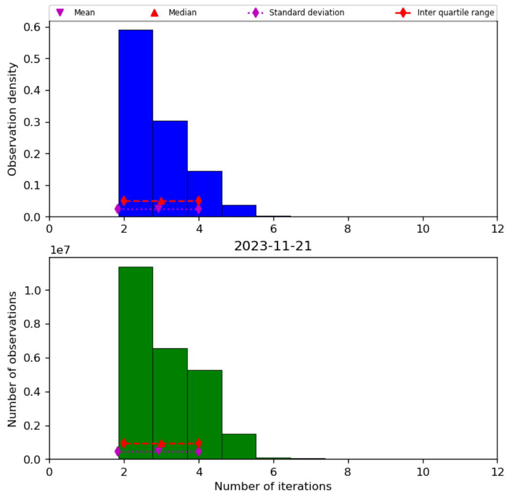
Figure 39: Histogram of “Number of iterations” for 2023-11-20 to 2023-11-22
