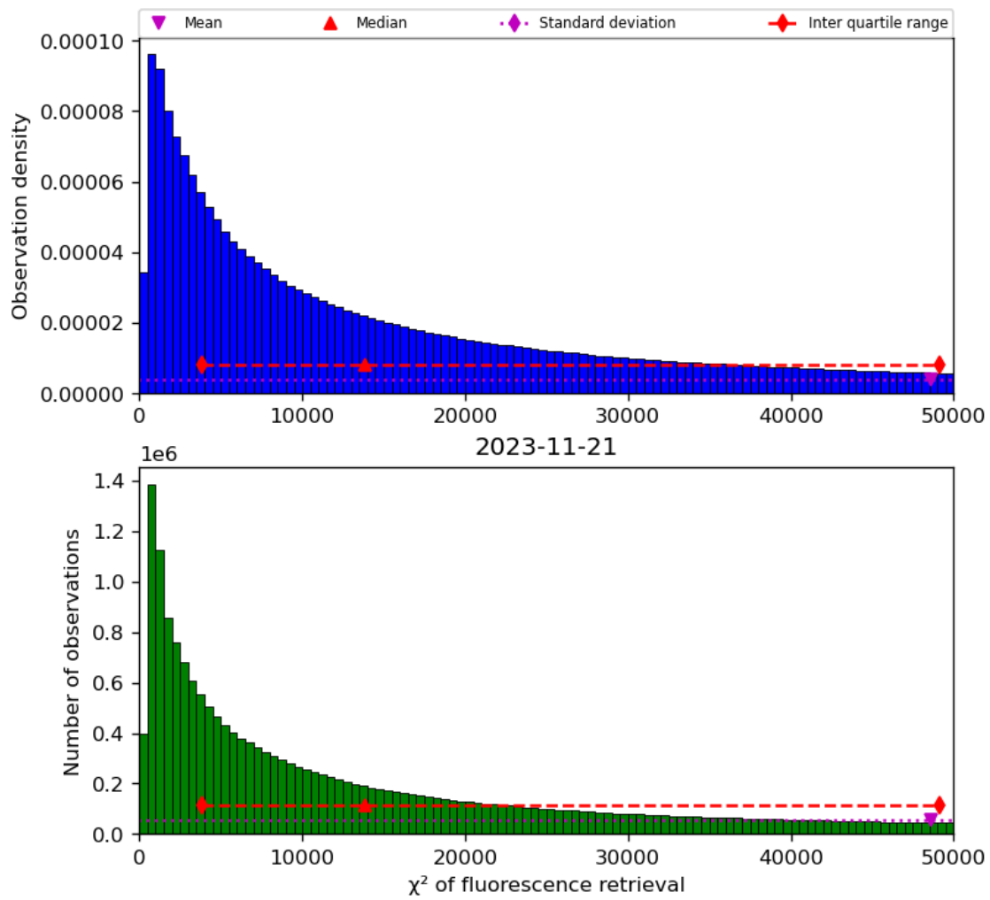
Figure 42: Histogram of “ \chi^2 of fluorescence retrieval” for 2023-11-20 to 2023-11-22
