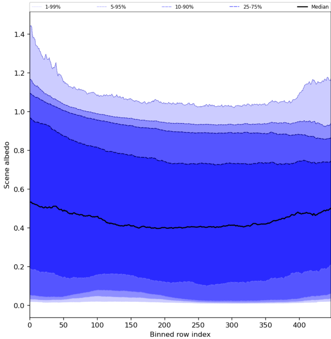
Figure 51: Along track statistics of “Scene albedo” for 2023-11-20 to 2023-11-22
