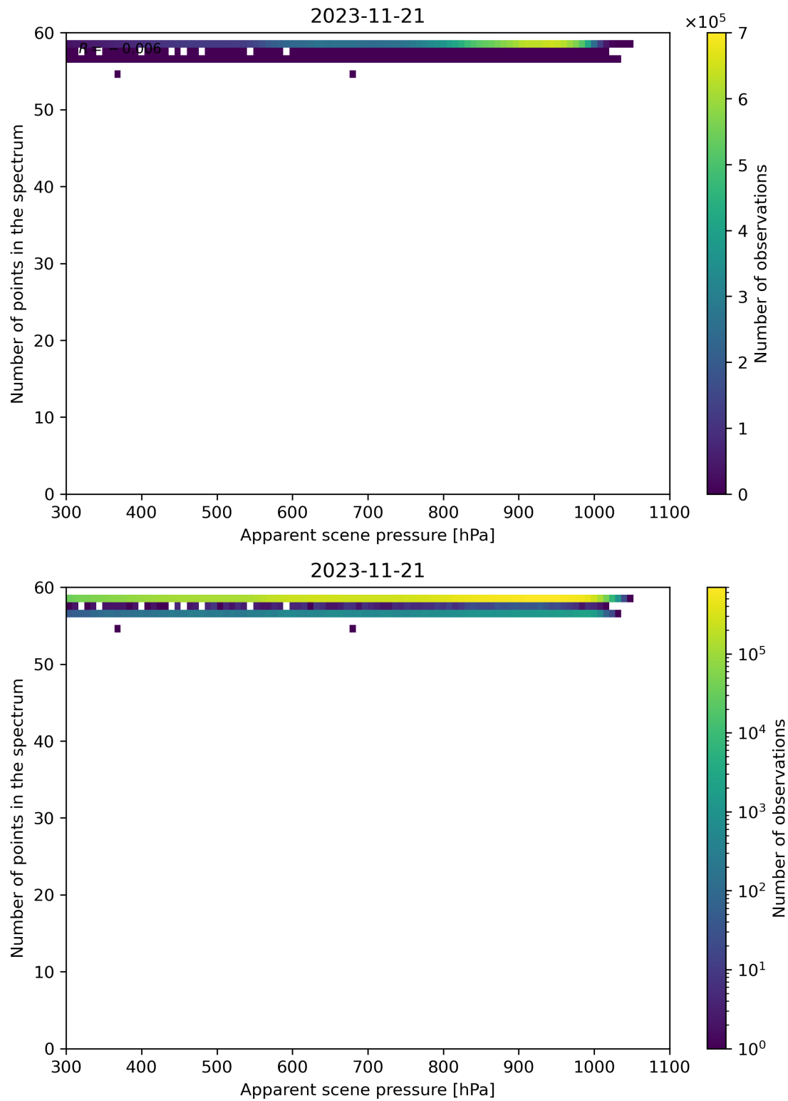
Figure 67: Scatter density plot of “Apparent scene pressure” against “Number of points in the spectrum” for 2023-11-20 to 2023-11-22.
