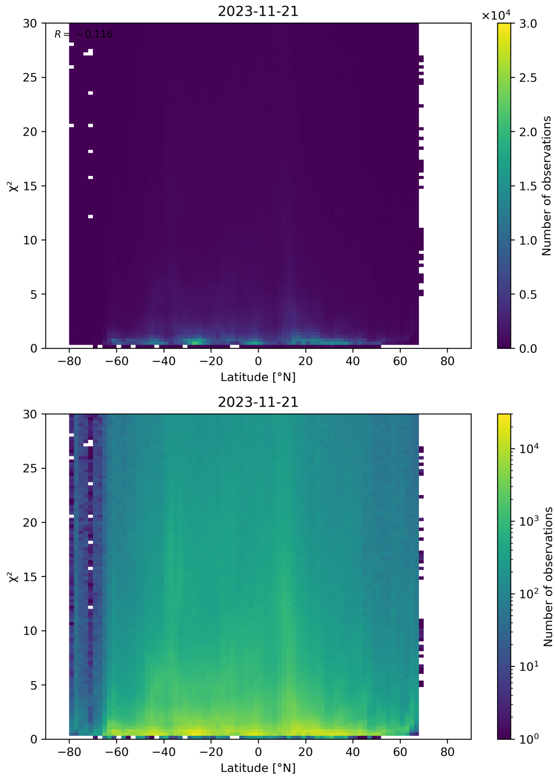
Figure 97: Scatter density plot of “Latitude” against “ \chi^2 ” for 2023-11-20 to 2023-11-22.
