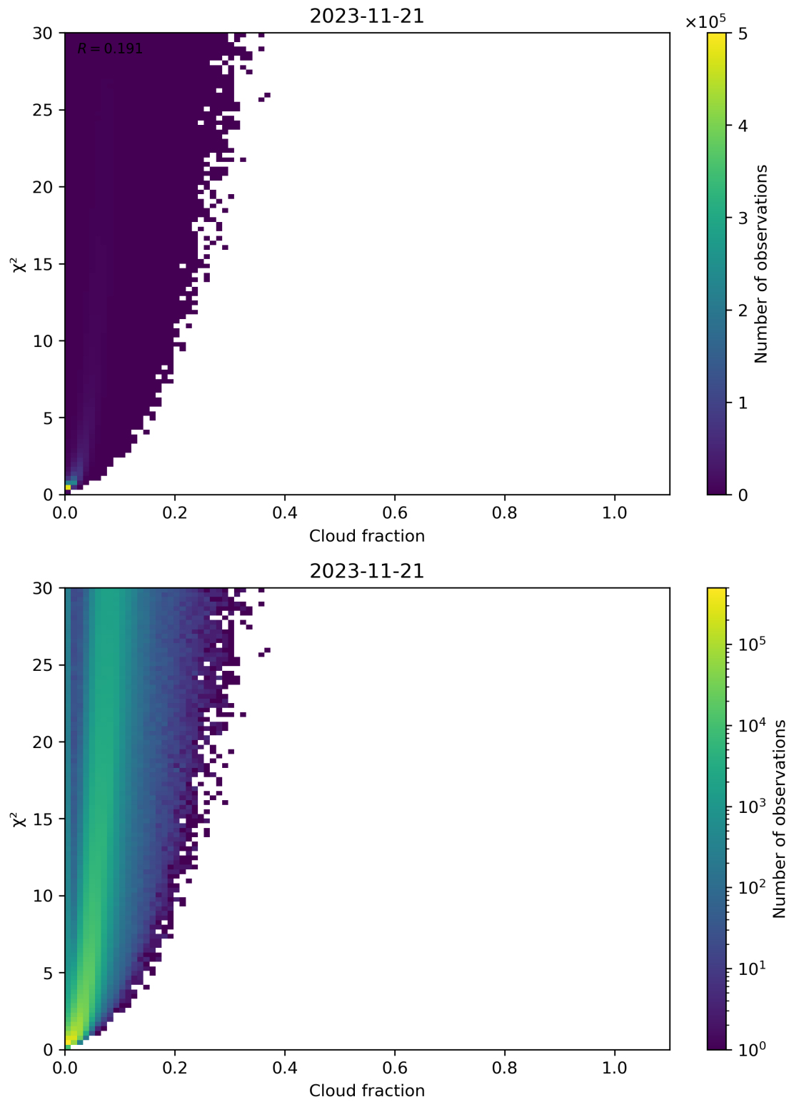
Figure 77: Scatter density plot of “Cloud fraction” against “ \chi^2 ” for 2023-11-20 to 2023-11-22.
