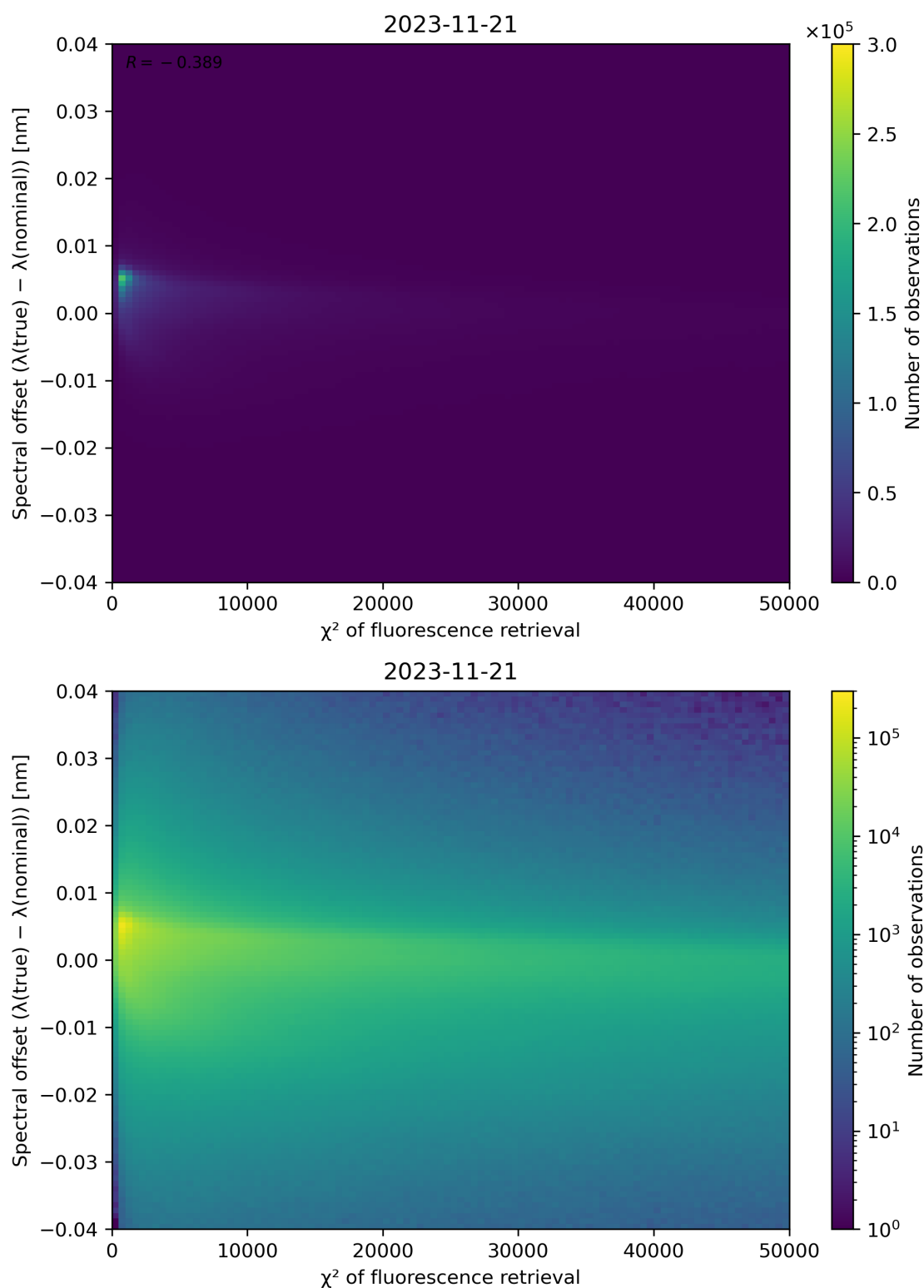
Figure 72: Scatter density plot of " \chi^2 of fluorescence retrieval" against "Spectral offset ( \lambda(\text{true}) - \lambda(\text{nominal})) " for 2023-11-20 to 2023-11-22.
