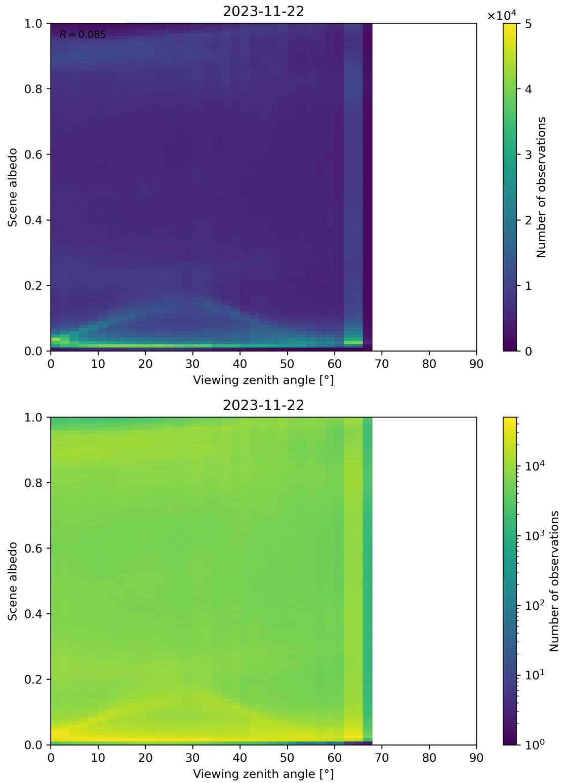
Figure 138: Scatter density plot of “Viewing zenith angle” against “Scene albedo” for 2023-11-21 to 2023-11-23.
