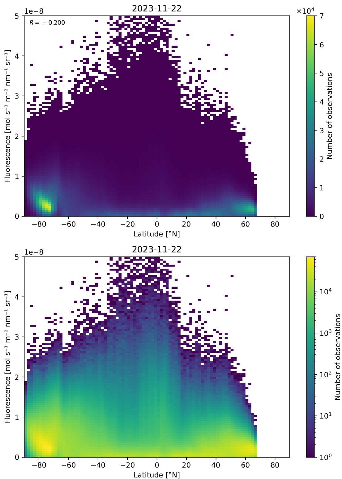
Figure 101: Scatter density plot of “Latitude” against “Fluorescence” for 2023-11-21 to 2023-11-23.
