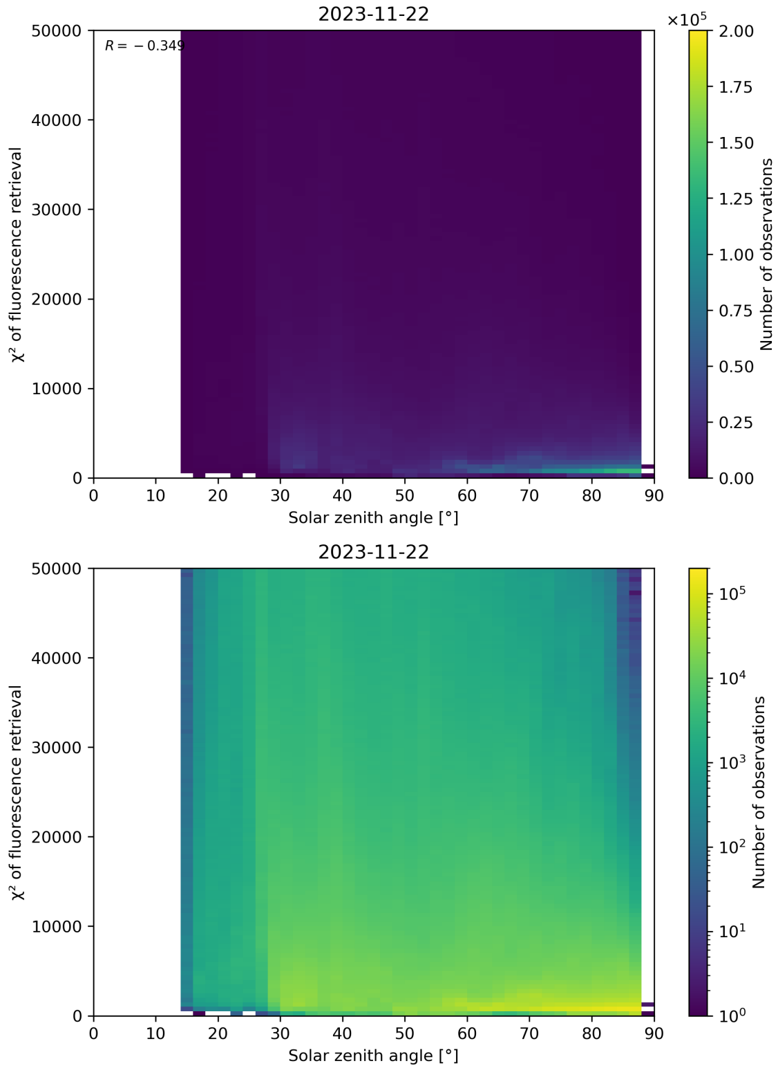
Figure 120: Scatter density plot of “Solar zenith angle” against “ \chi^2 of fluorescence retrieval” for 2023-11-21 to 2023-11-23.
