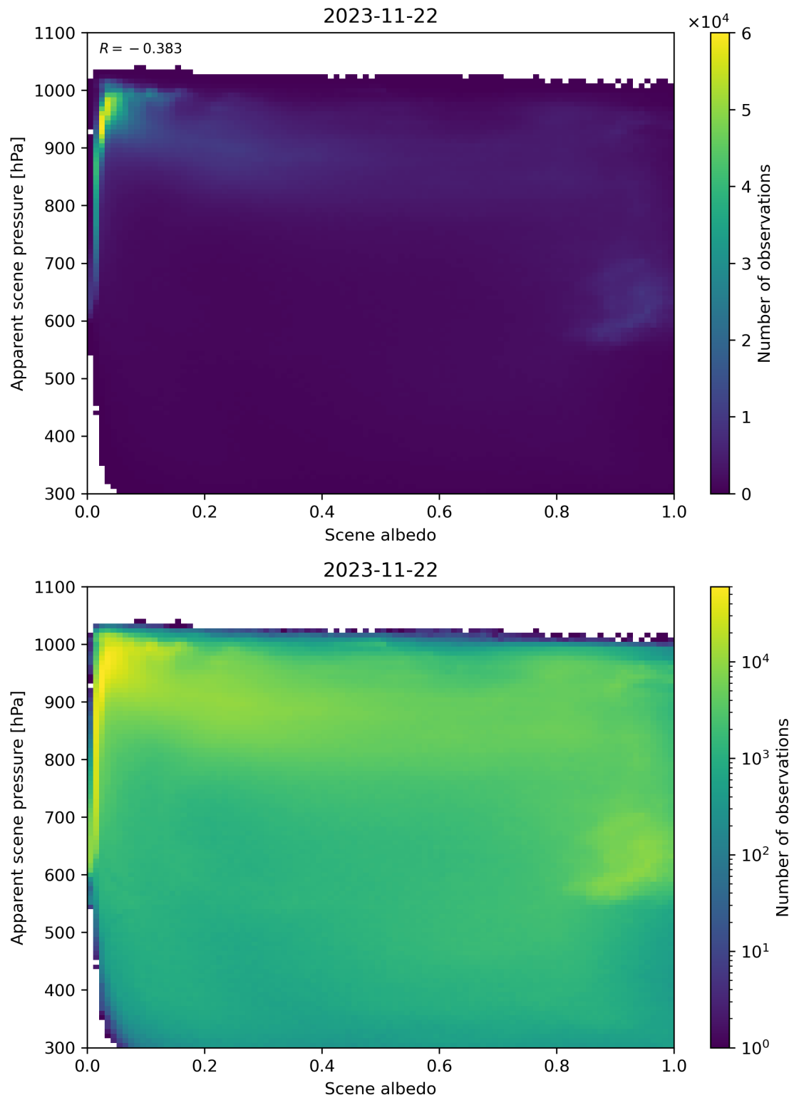
Figure 111: Scatter density plot of “Scene albedo” against “Apparent scene pressure” for 2023-11-21 to 2023-11-23.
