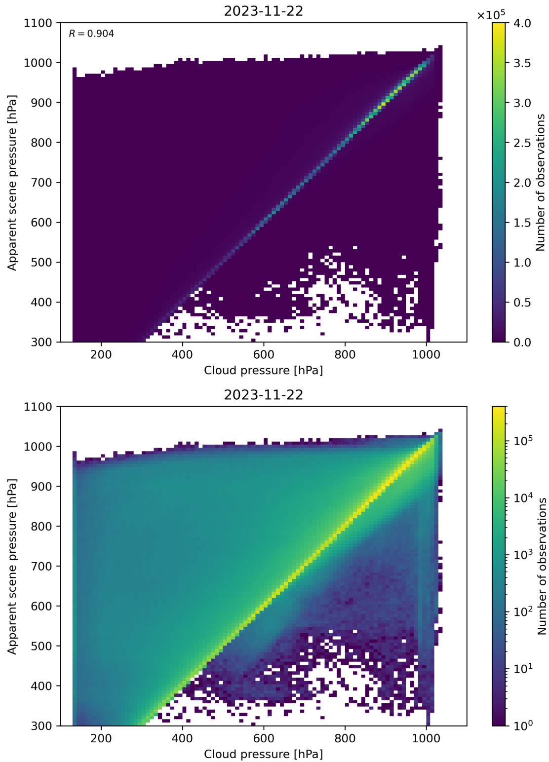
Figure 84: Scatter density plot of “Cloud pressure” against “Apparent scene pressure” for 2023-11-21 to 2023-11-23.
