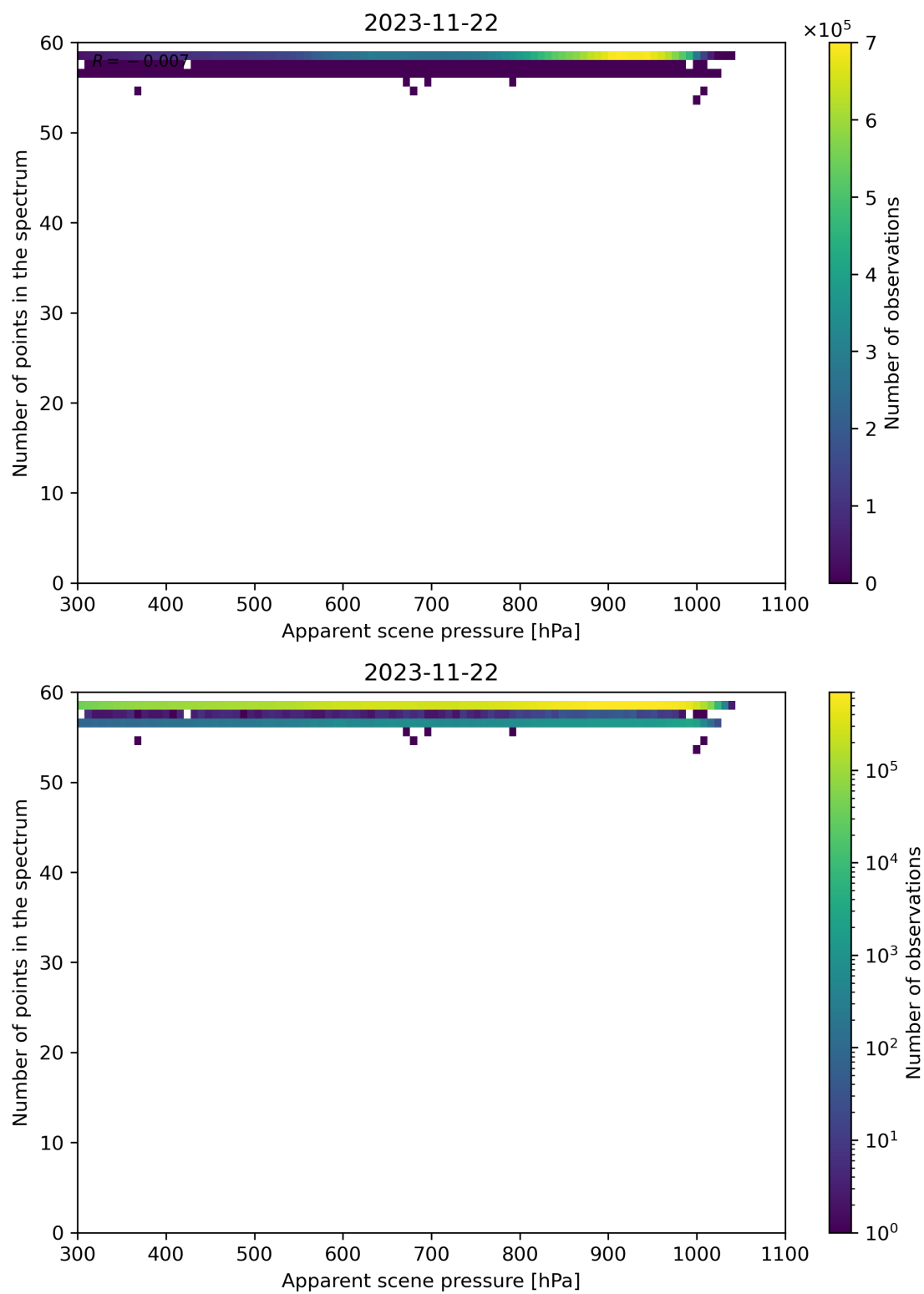
Figure 67: Scatter density plot of “Apparent scene pressure” against “Number of points in the spectrum” for 2023-11-21 to 2023-11-23.
