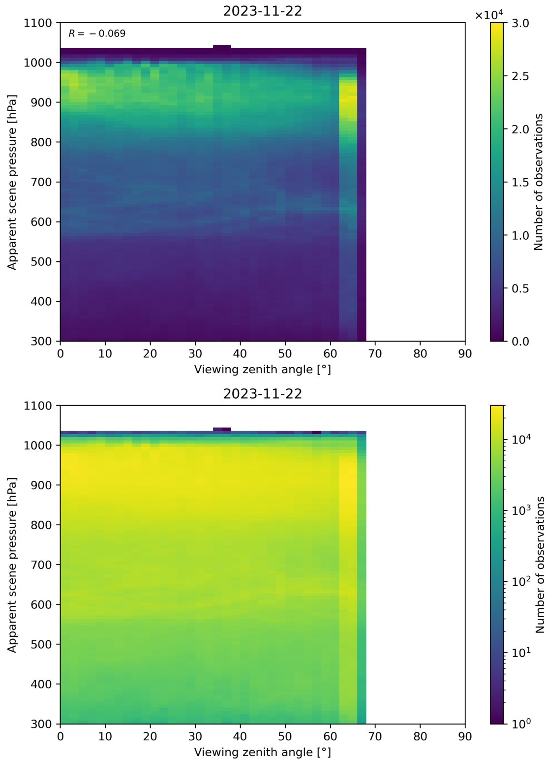
Figure 129: Scatter density plot of “Viewing zenith angle” against “Apparent scene pressure” for 2023-11-21 to 2023-11-23.
