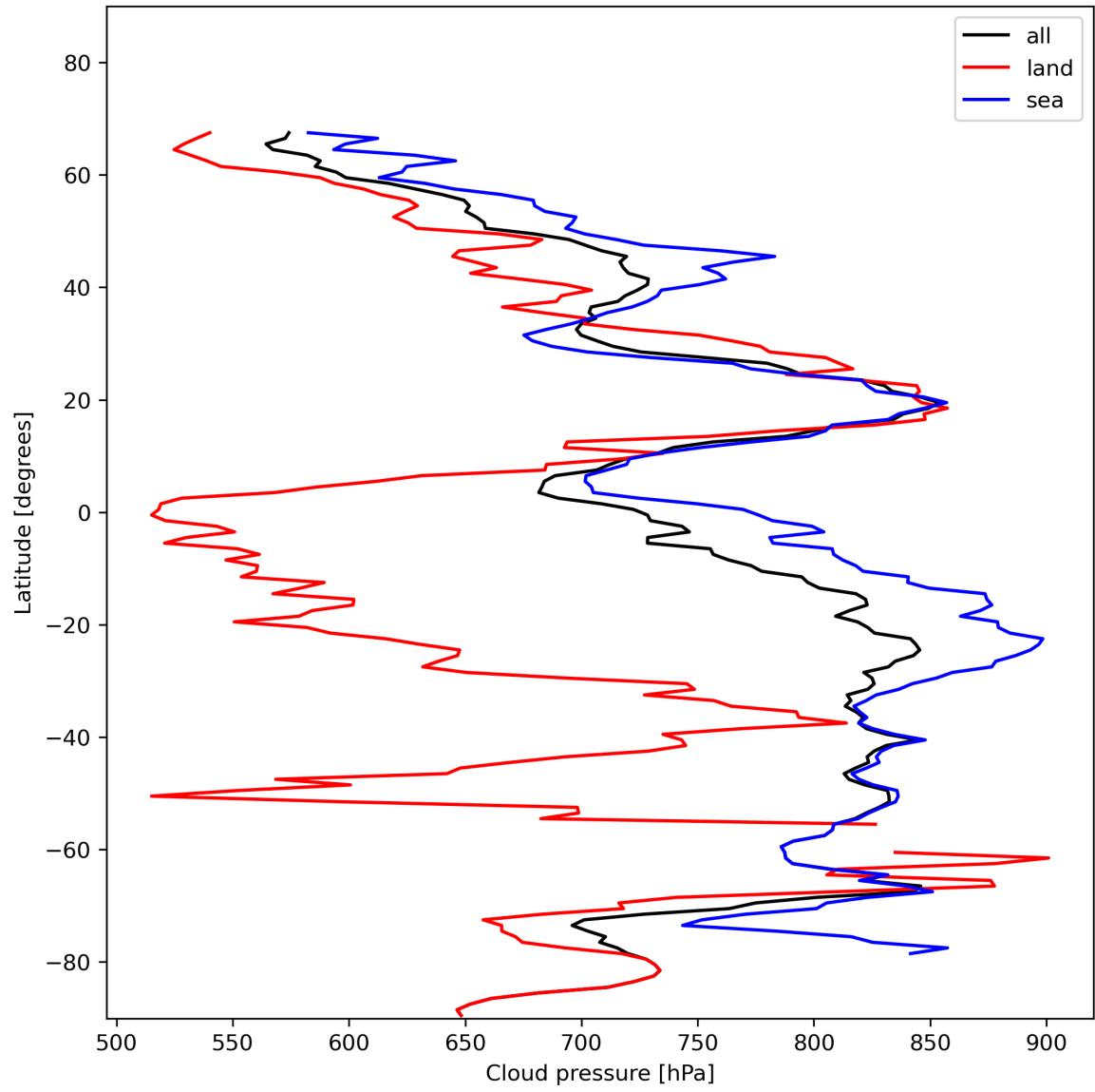
Figure 13: Zonal average of “Cloud pressure” for 2023-11-21 to 2023-11-23.
