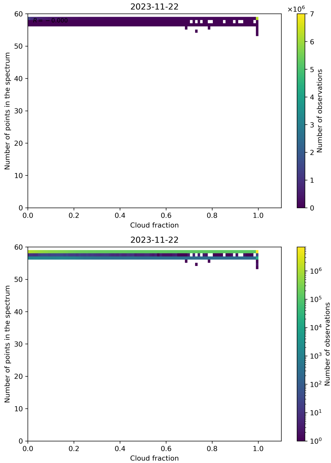
Figure 81: Scatter density plot of “Cloud fraction” against “Number of points in the spectrum” for 2023-11-21 to 2023-11-23.
