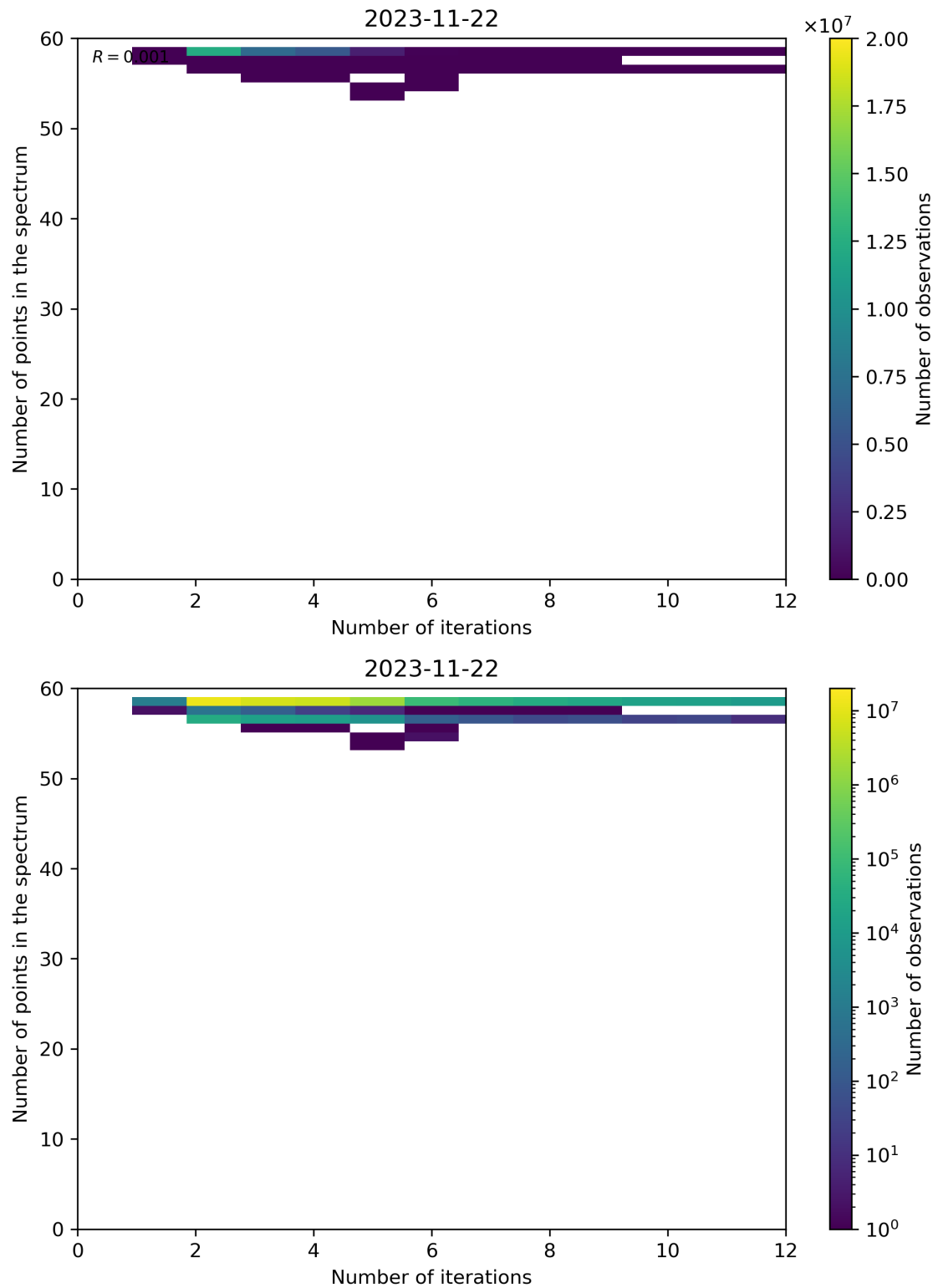
Figure 108: Scatter density plot of “Number of iterations” against “Number of points in the spectrum” for 2023-11-21 to 2023-11-23.
