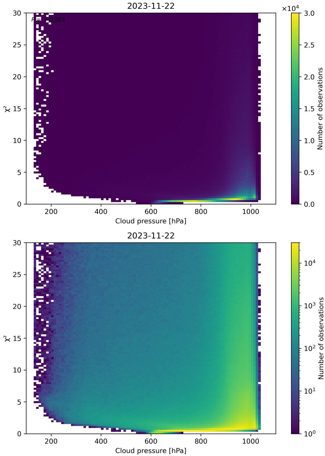
Figure 85: Scatter density plot of “Cloud pressure” against “ \chi^2 ” for 2023-11-21 to 2023-11-23.
