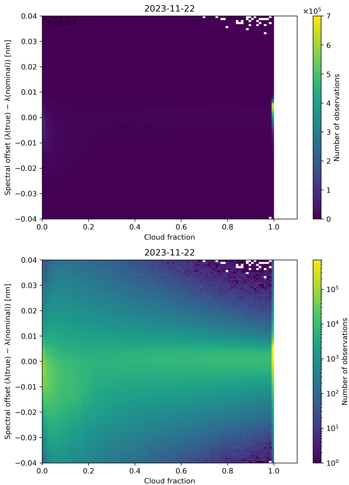
Figure 83: Scatter density plot of “Cloud fraction” against “Spectral offset ( \lambda(\text{true}) - \lambda(\text{nominal}) )” for 2023-11-21 to 2023-11-23.
