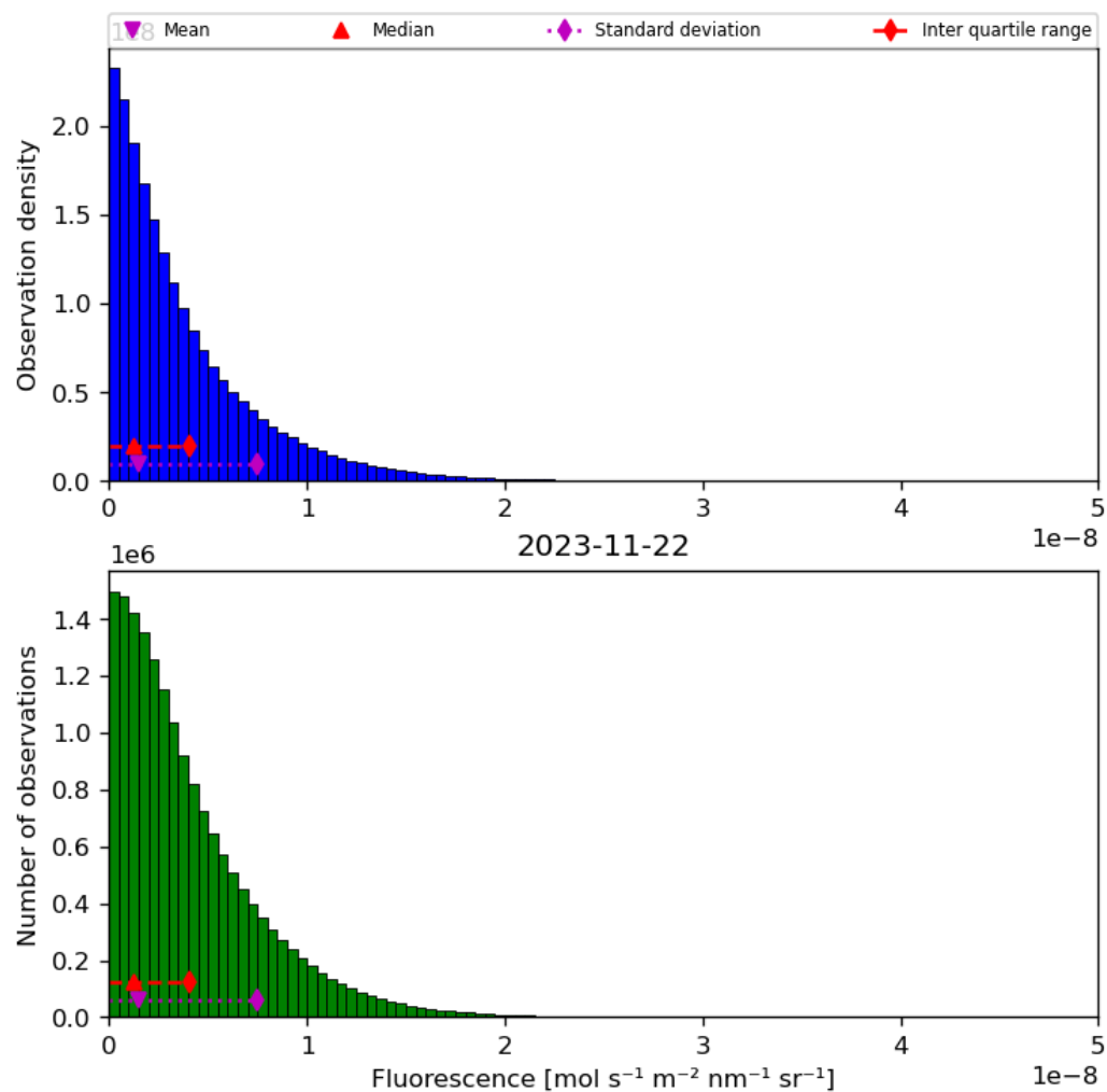
Figure 40: Histogram of “Fluorescence” for 2023-11-21 to 2023-11-23
