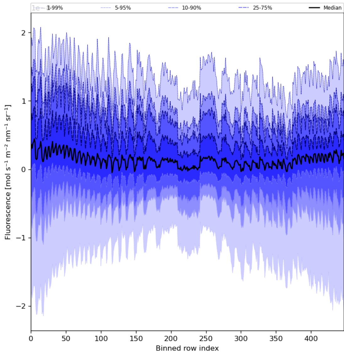
Figure 57: Along track statistics of “Fluorescence” for 2023-11-21 to 2023-11-23
