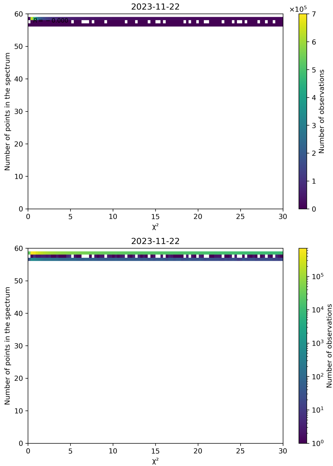
Figure 74: Scatter density plot of " \chi^2 " against "Number of points in the spectrum" for 2023-11-21 to 2023-11-23.
