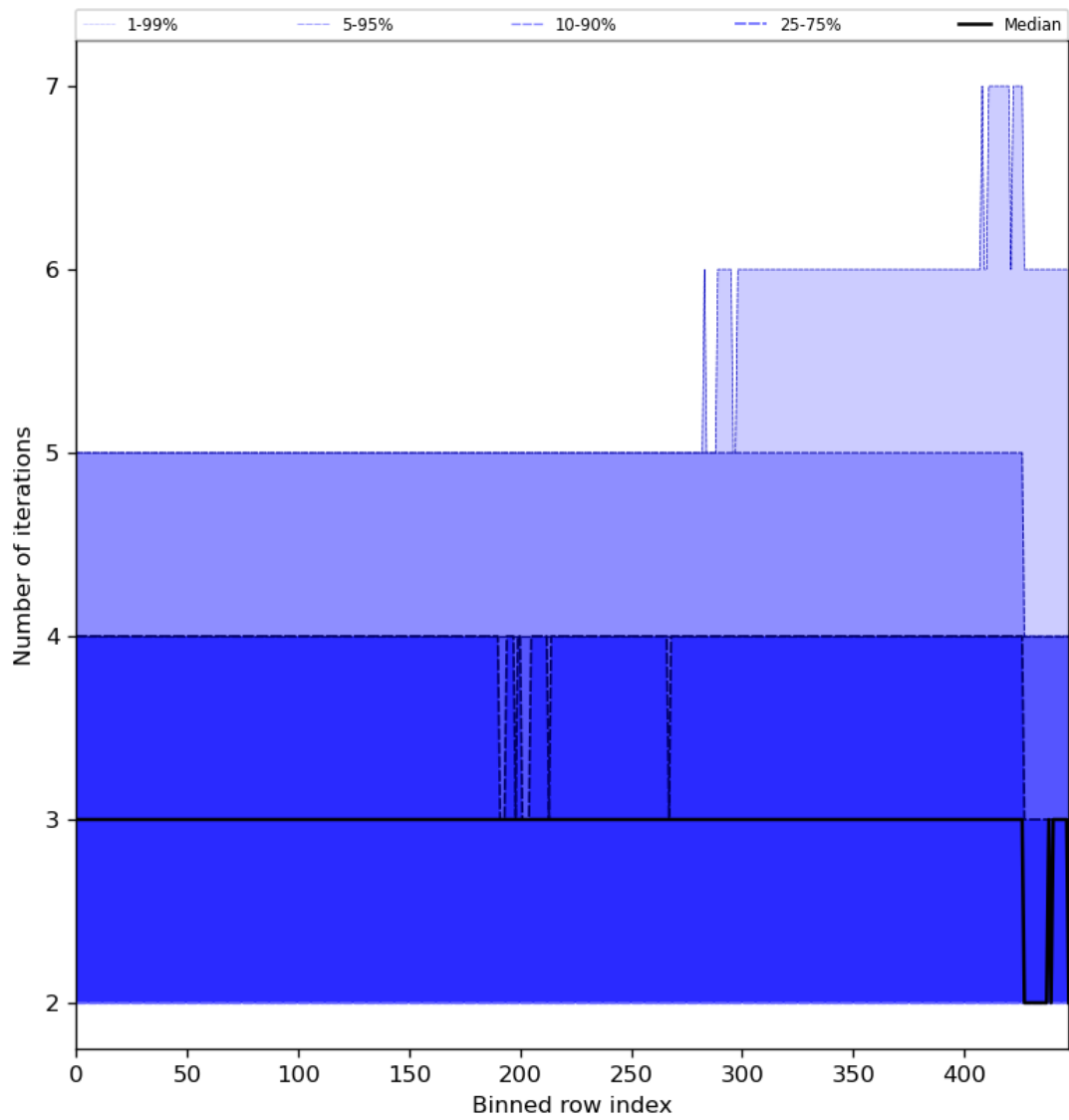
Figure 56: Along track statistics of “Number of iterations” for 2023-11-21 to 2023-11-23
