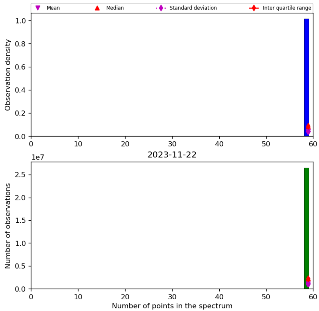
Figure 44: Histogram of “Number of points in the spectrum” for 2023-11-21 to 2023-11-23
