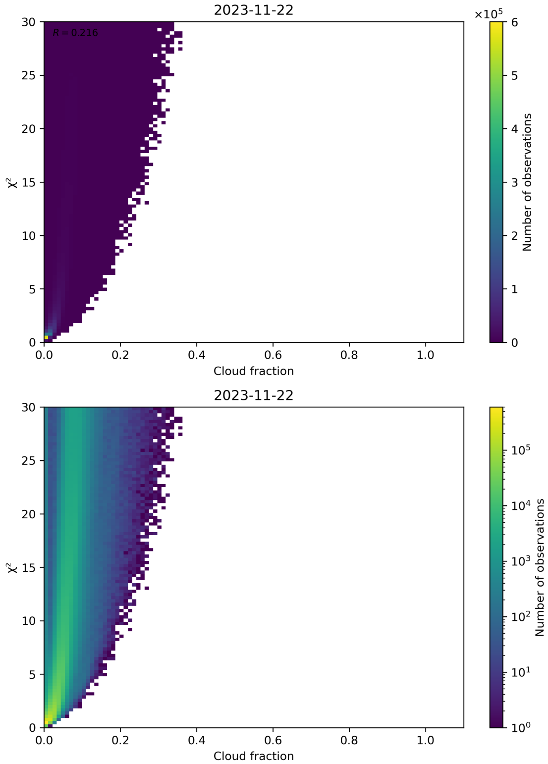
Figure 77: Scatter density plot of “Cloud fraction” against “ \chi^2 ” for 2023-11-21 to 2023-11-23.
