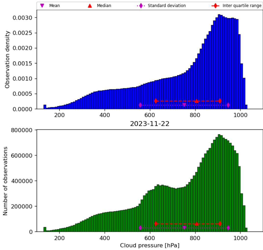
Figure 30: Histogram of “Cloud pressure” for 2023-11-21 to 2023-11-23
