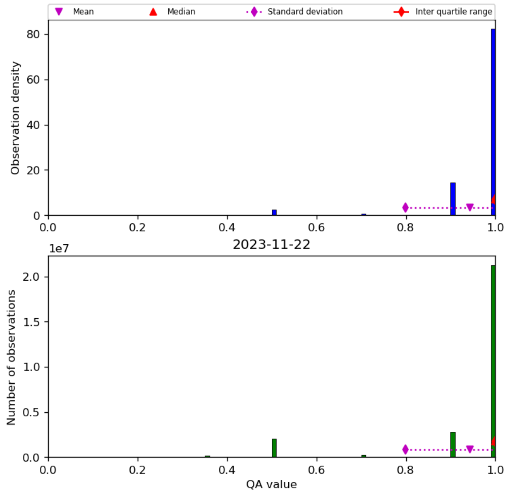
Figure 29: Histogram of “QA value” for 2023-11-21 to 2023-11-23
