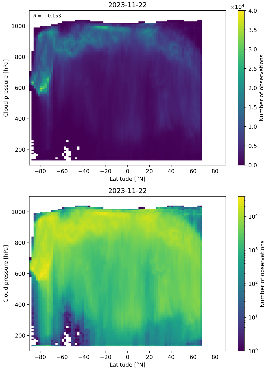
Figure 100: Scatter density plot of “Latitude” against “Cloud pressure” for 2023-11-21 to 2023-11-23.
