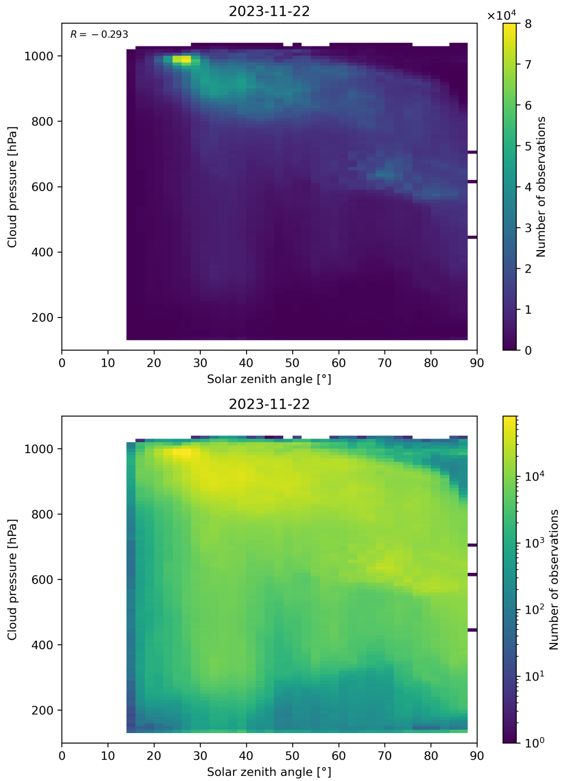
Figure 122: Scatter density plot of “Solar zenith angle” against “Cloud pressure” for 2023-11-21 to 2023-11-23.
