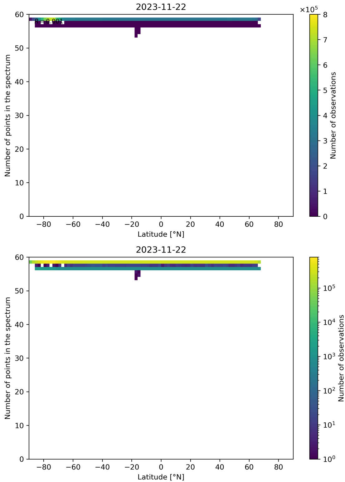
Figure 103: Scatter density plot of “Latitude” against “Number of points in the spectrum” for 2023-11-21 to 2023-11-23.
