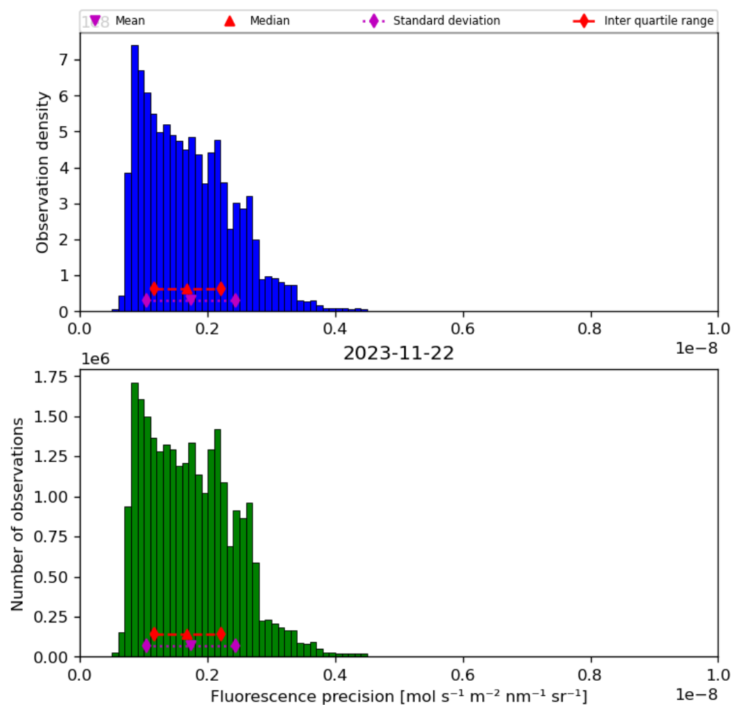
Figure 41: Histogram of “Fluorescence precision” for 2023-11-21 to 2023-11-23
