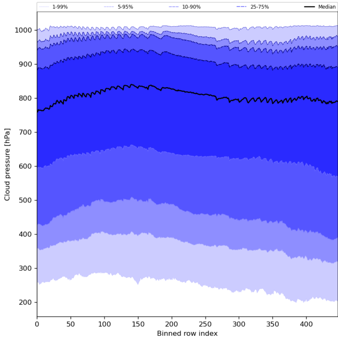
Figure 47: Along track statistics of “Cloud pressure” for 2023-11-21 to 2023-11-23
