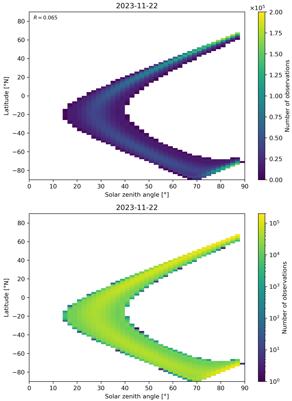
Figure 124: Scatter density plot of “Solar zenith angle” against “Latitude” for 2023-11-21 to 2023-11-23.
