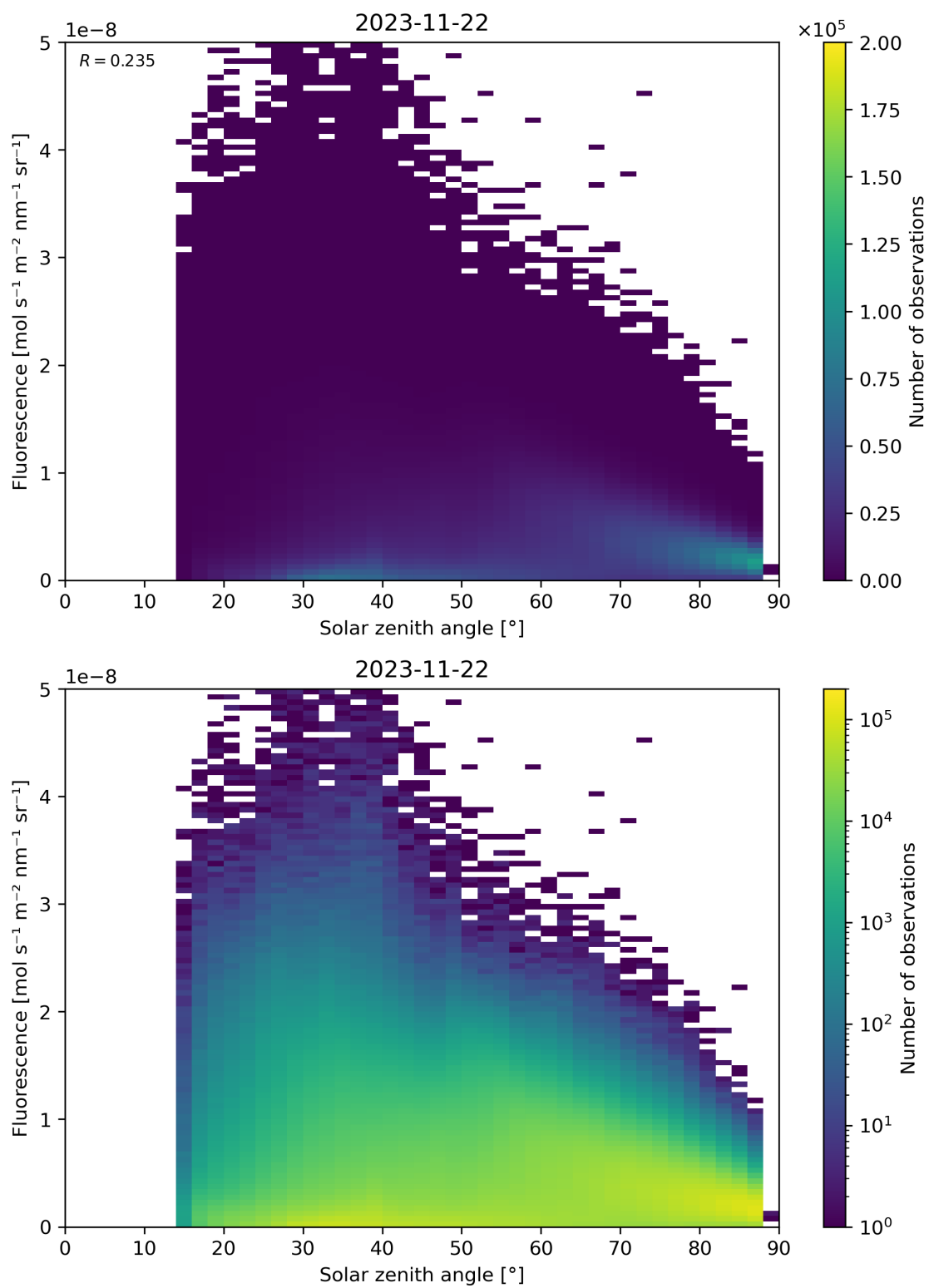
Figure 123: Scatter density plot of “Solar zenith angle” against “Fluorescence” for 2023-11-21 to 2023-11-23.
