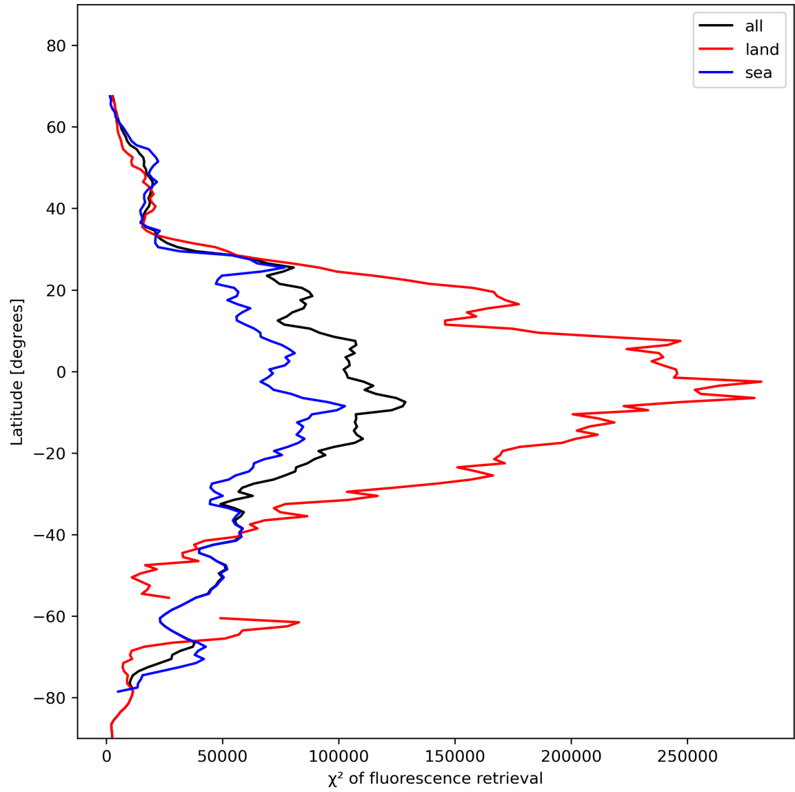
Figure 25: Zonal average of “ \chi^2 of fluorescence retrieval” for 2023-11-21 to 2023-11-23.
