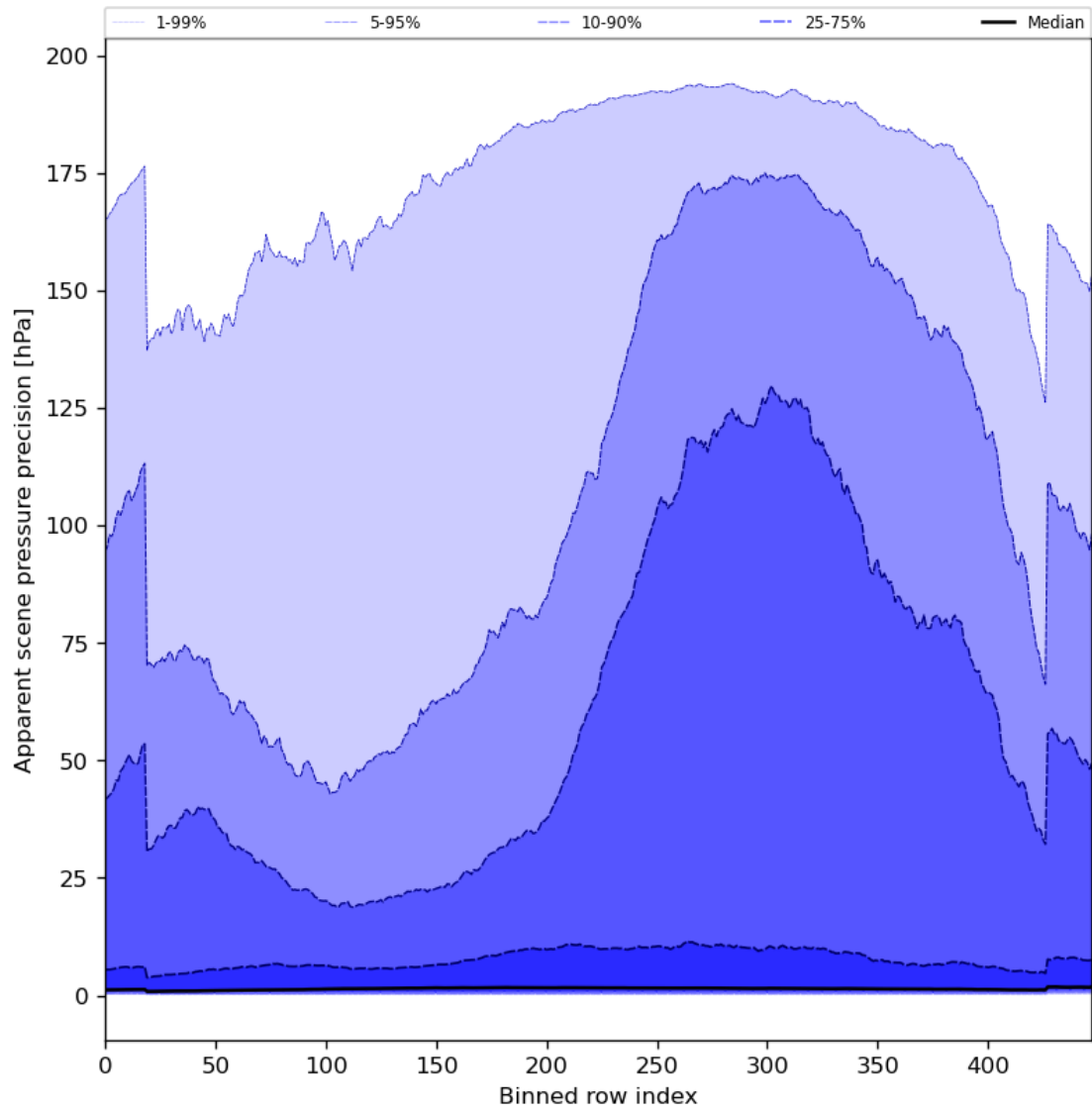
Figure 54: Along track statistics of “Apparent scene pressure precision” for 2023-11-21 to 2023-11-23
