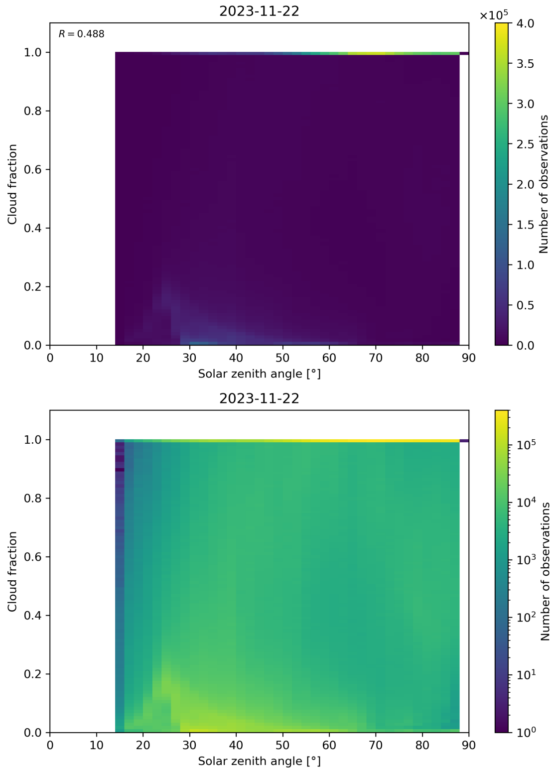
Figure 121: Scatter density plot of “Solar zenith angle” against “Cloud fraction” for 2023-11-21 to 2023-11-23.
