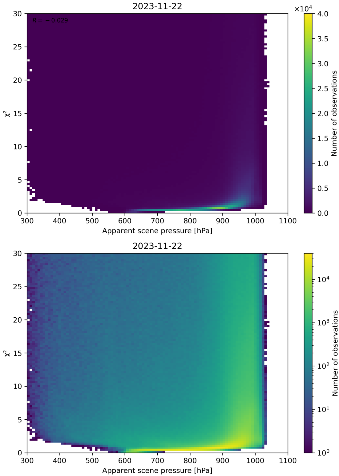
Figure 63: Scatter density plot of “Apparent scene pressure” against “ \chi^2 ” for 2023-11-21 to 2023-11-23.
