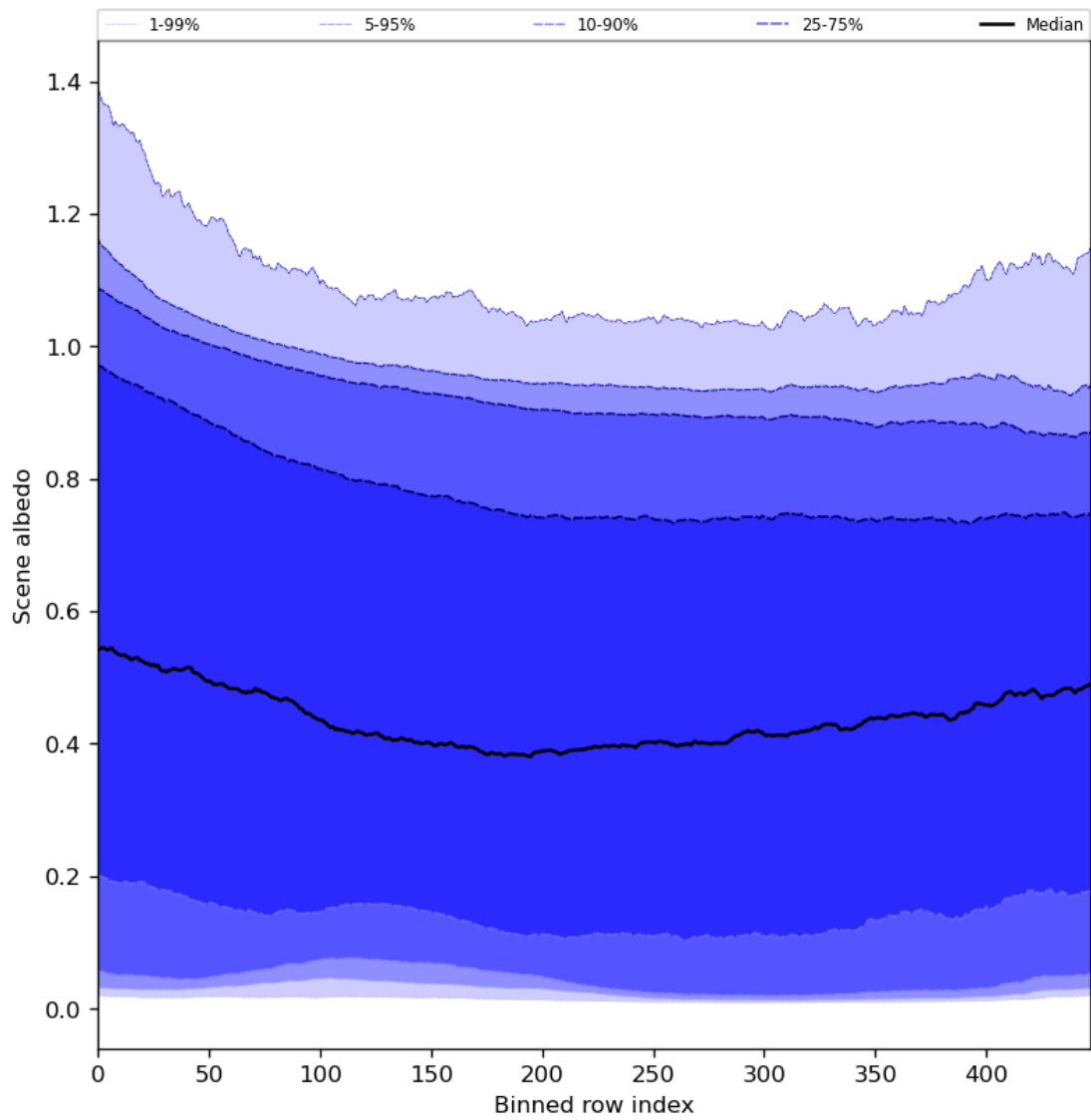
Figure 51: Along track statistics of “Scene albedo” for 2023-11-21 to 2023-11-23
