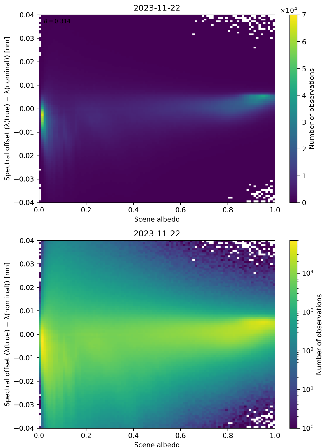
Figure 117: Scatter density plot of “Scene albedo” against “Spectral offset ( \lambda(\text{true}) - \lambda(\text{nominal}) )” for 2023-11-21 to 2023-11-23.
