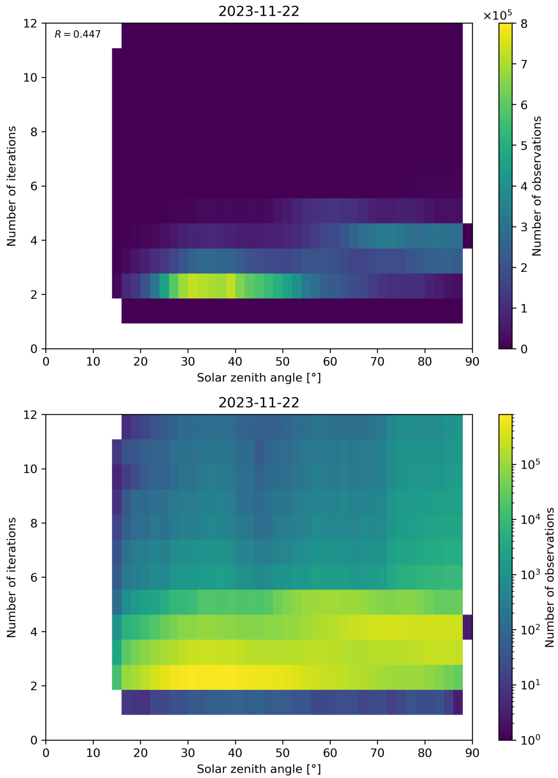
Figure 125: Scatter density plot of “Solar zenith angle” against “Number of iterations” for 2023-11-21 to 2023-11-23.
