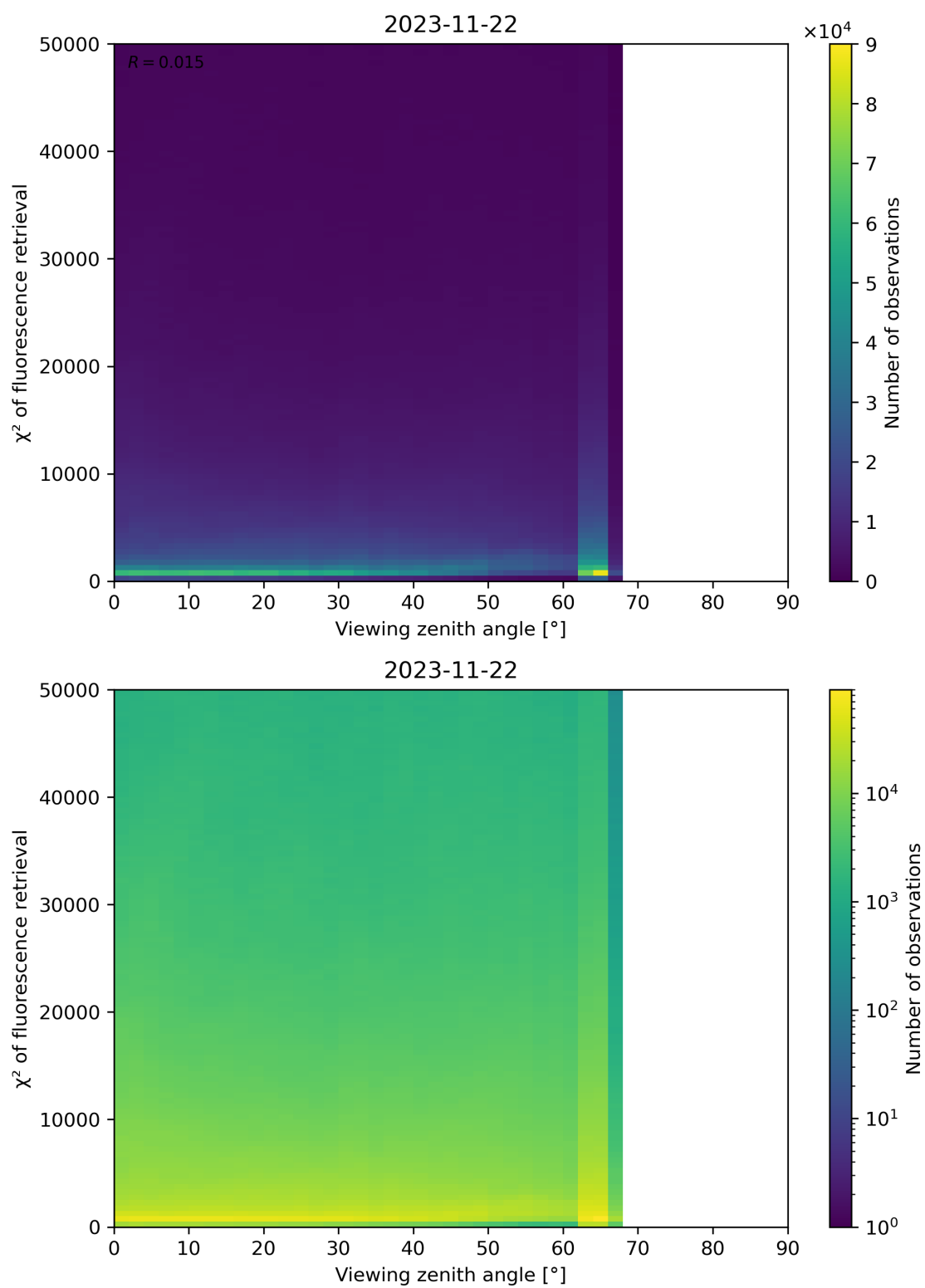
Figure 131: Scatter density plot of “Viewing zenith angle” against “ \chi^2 of fluorescence retrieval” for 2023-11-21 to 2023-11-23.
