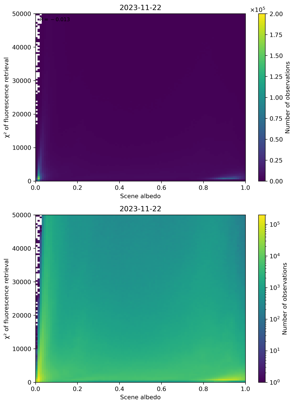
Figure 113: Scatter density plot of “Scene albedo” against “ \chi^2 of fluorescence retrieval” for 2023-11-21 to 2023-11-23.
