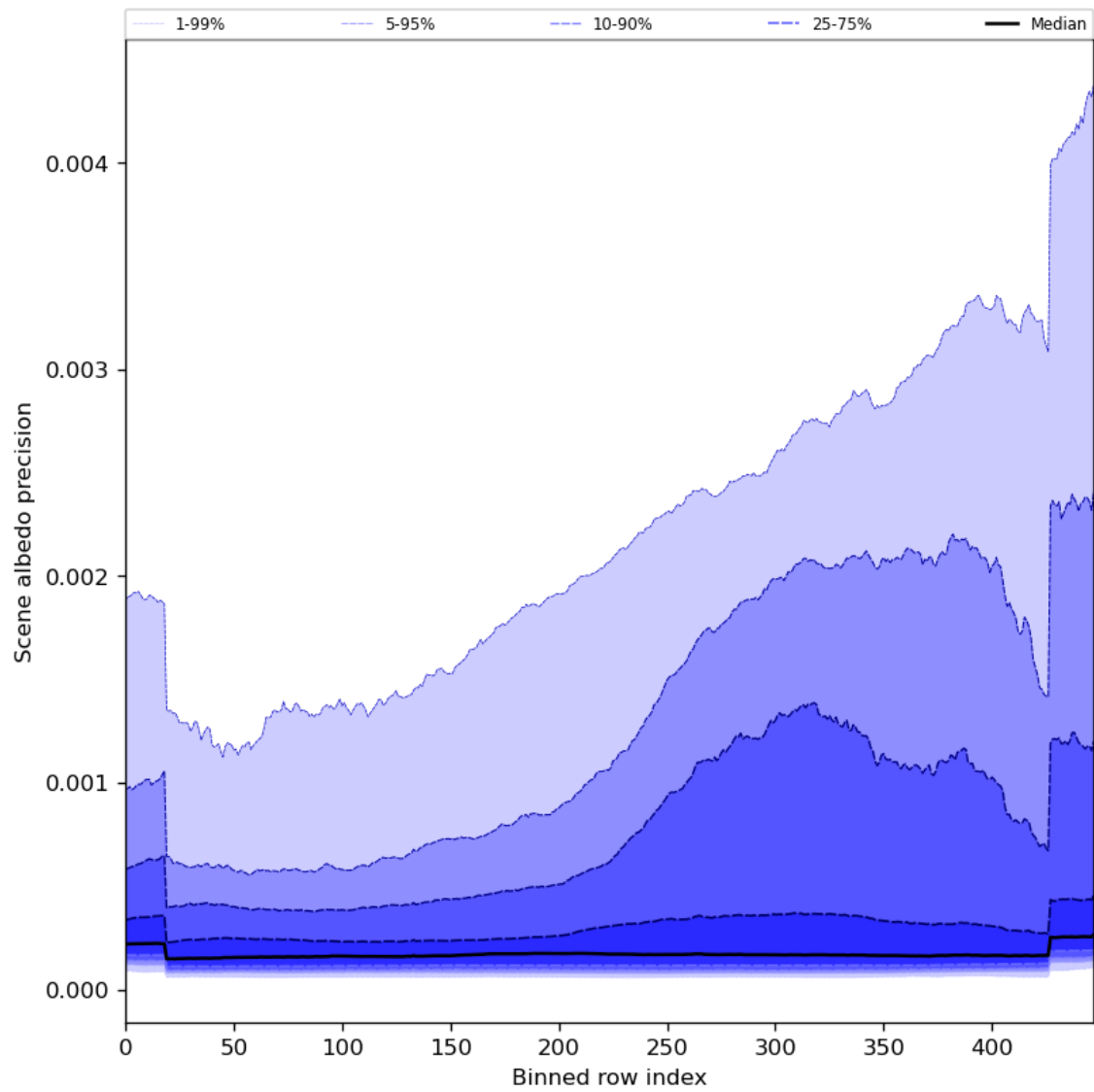
Figure 52: Along track statistics of “Scene albedo precision” for 2023-11-21 to 2023-11-23
