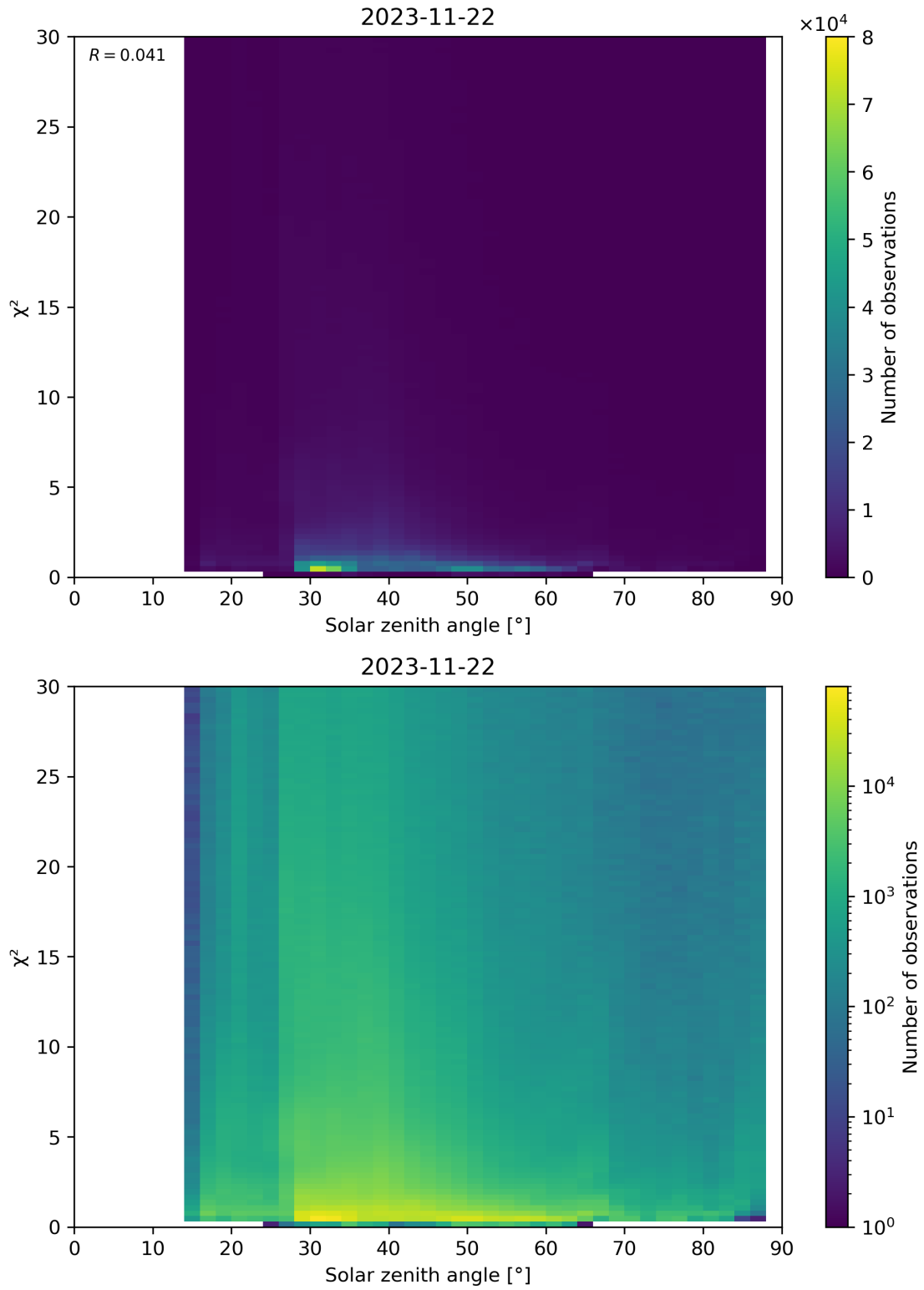
Figure 119: Scatter density plot of “Solar zenith angle” against “ \chi^2 ” for 2023-11-21 to 2023-11-23.
