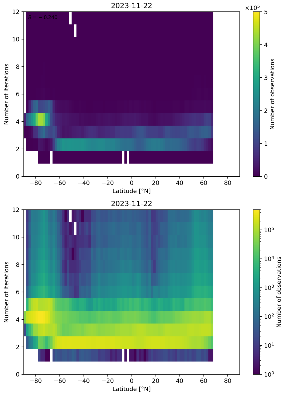
Figure 102: Scatter density plot of “Latitude” against “Number of iterations” for 2023-11-21 to 2023-11-23.
