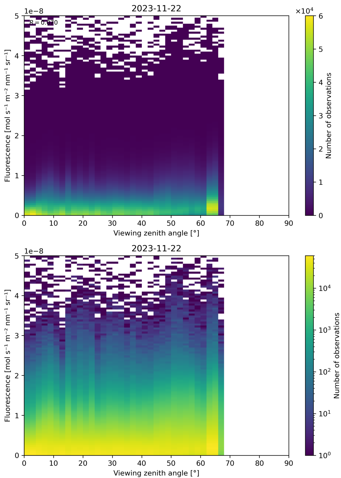
Figure 134: Scatter density plot of “Viewing zenith angle” against “Fluorescence” for 2023-11-21 to 2023-11-23.
