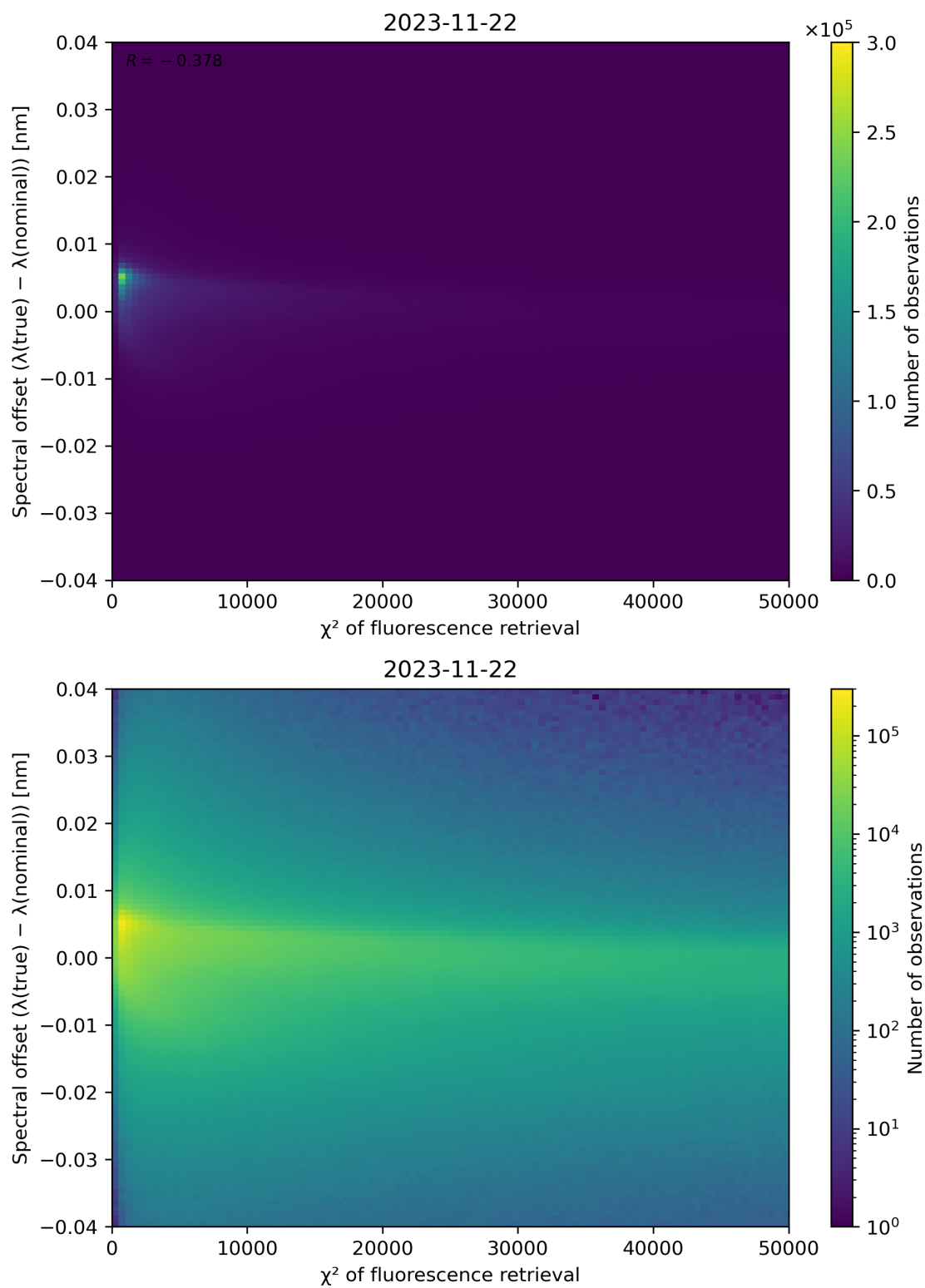
Figure 72: Scatter density plot of " \chi^2 of fluorescence retrieval" against "Spectral offset ( \lambda(\text{true}) - \lambda(\text{nominal}) )" for 2023-11-21 to 2023-11-23.
