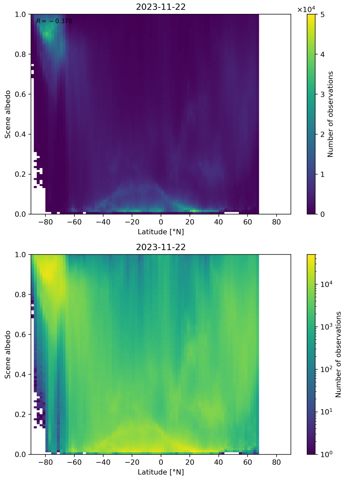
Figure 104: Scatter density plot of “Latitude” against “Scene albedo” for 2023-11-21 to 2023-11-23.
