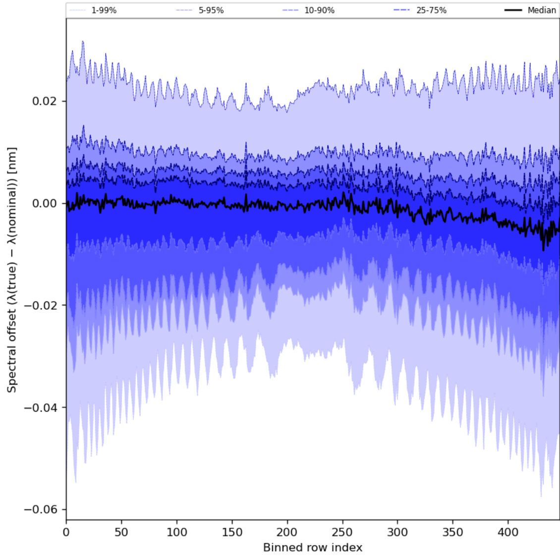
Figure 62: Along track statistics of “Spectral offset ( \lambda(\text{true}) - \lambda(\text{nominal}) )” for 2023-11-21 to 2023-11-23
