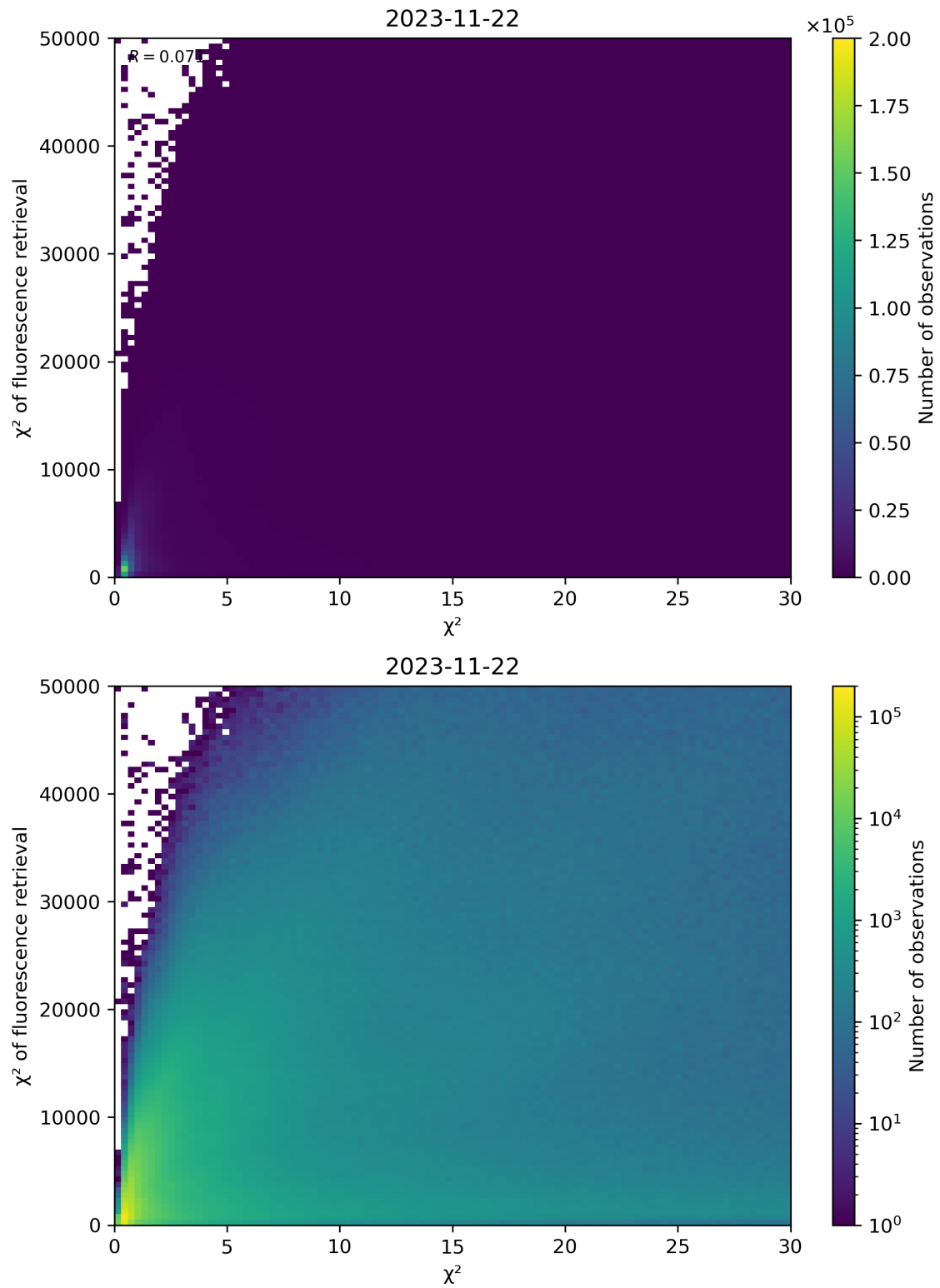
Figure 69: Scatter density plot of “ \chi^2 ” against “ \chi^2 of fluorescence retrieval” for 2023-11-21 to 2023-11-23.
