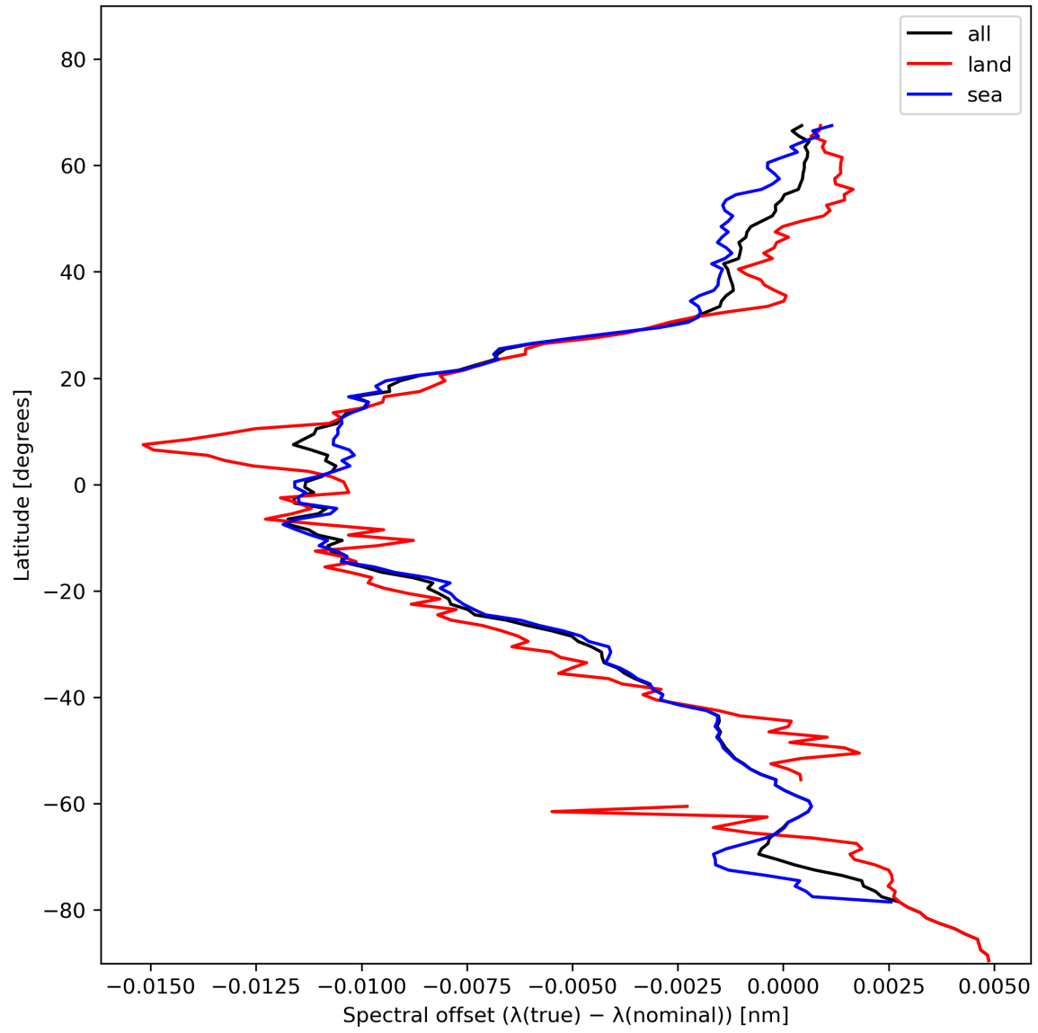
Figure 28: Zonal average of “Spectral offset ( \lambda(\text{true}) - \lambda(\text{nominal}) )” for 2023-11-21 to 2023-11-23.
