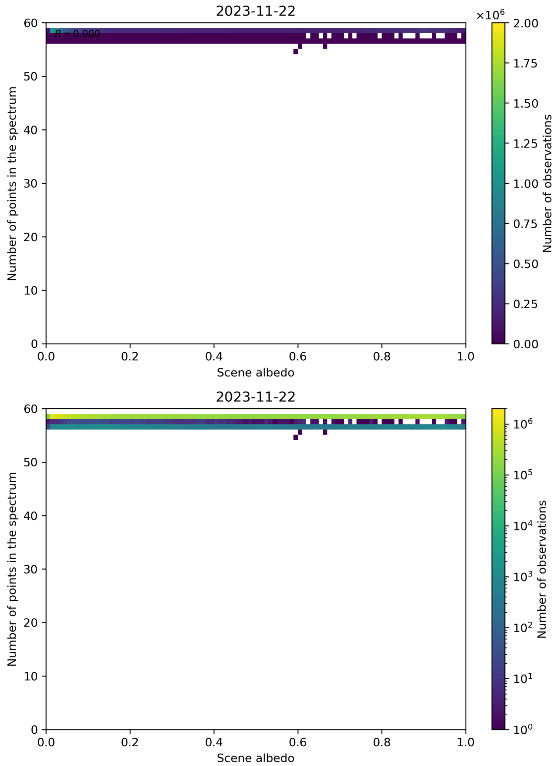
Figure 116: Scatter density plot of “Scene albedo” against “Number of points in the spectrum” for 2023-11-21 to 2023-11-23.
