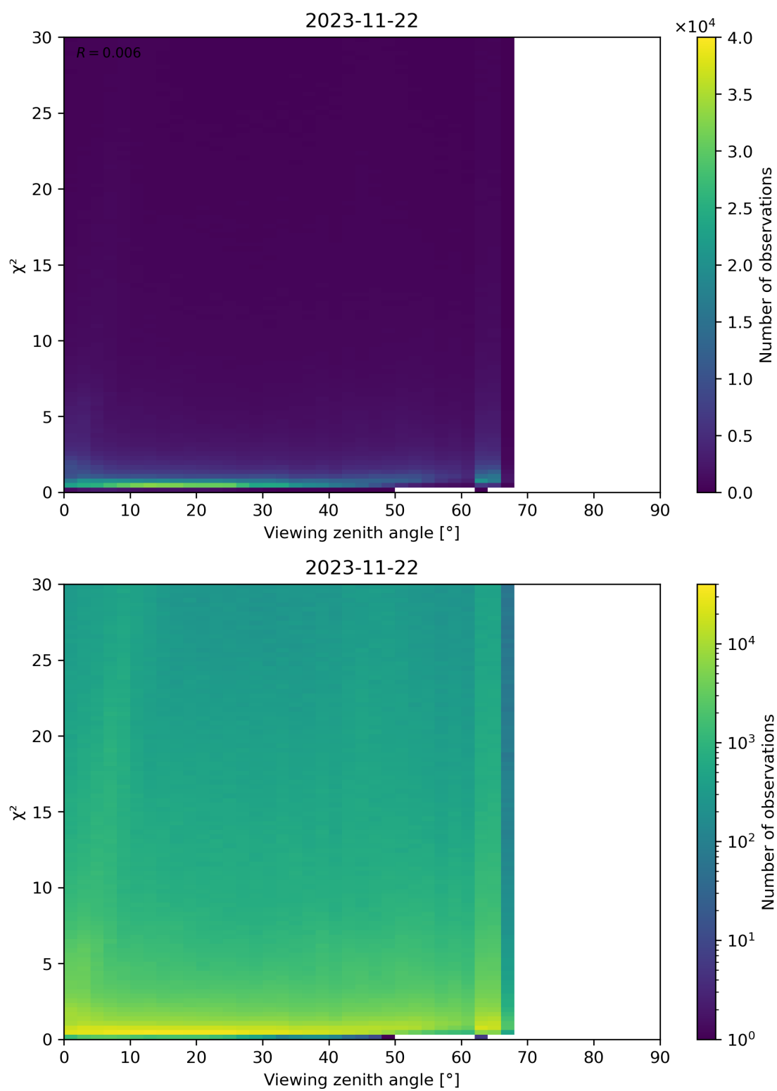
Figure 130: Scatter density plot of “Viewing zenith angle” against “ \chi^2 ” for 2023-11-21 to 2023-11-23.
