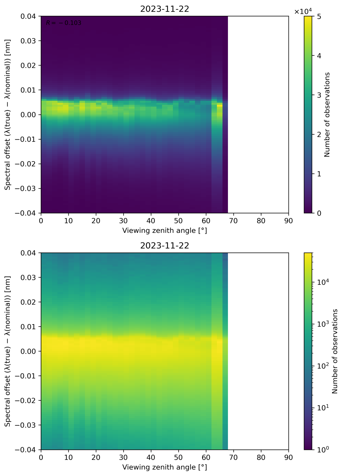
Figure 140: Scatter density plot of “Viewing zenith angle” against “Spectral offset ( \lambda(\text{true}) - \lambda(\text{nominal}) )” for 2023-11-21 to 2023-11-23.
