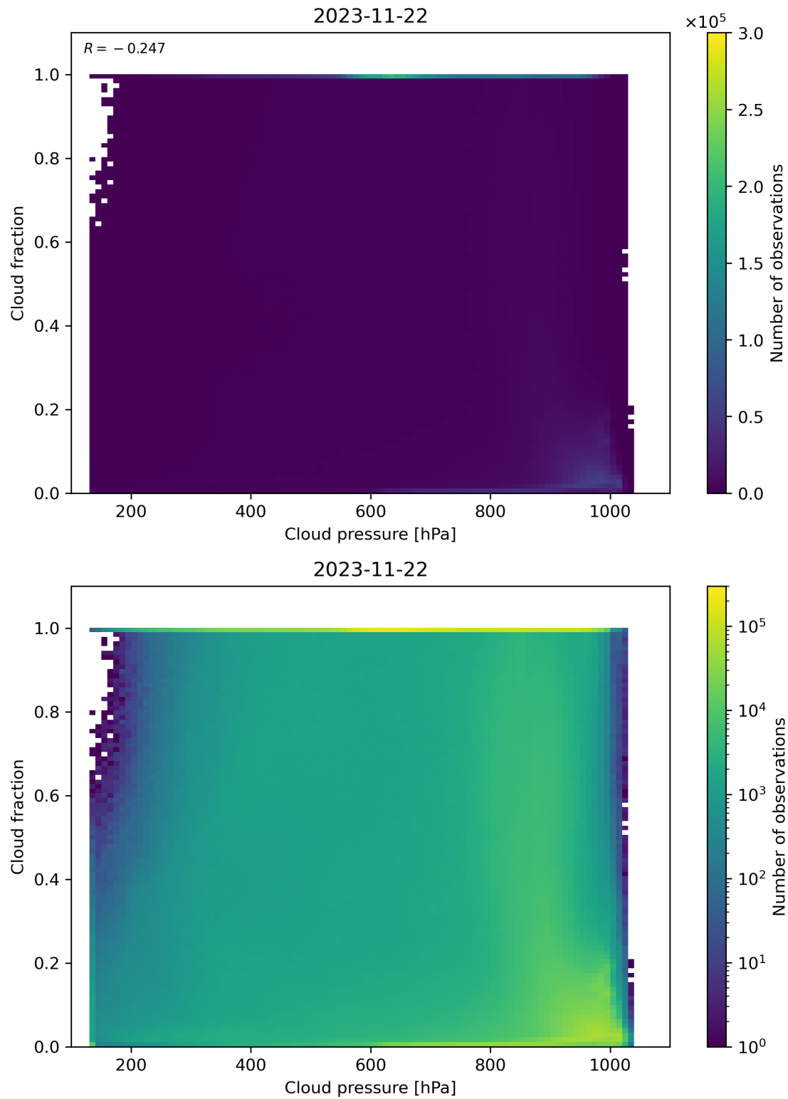
Figure 87: Scatter density plot of “Cloud pressure” against “Cloud fraction” for 2023-11-21 to 2023-11-23.
