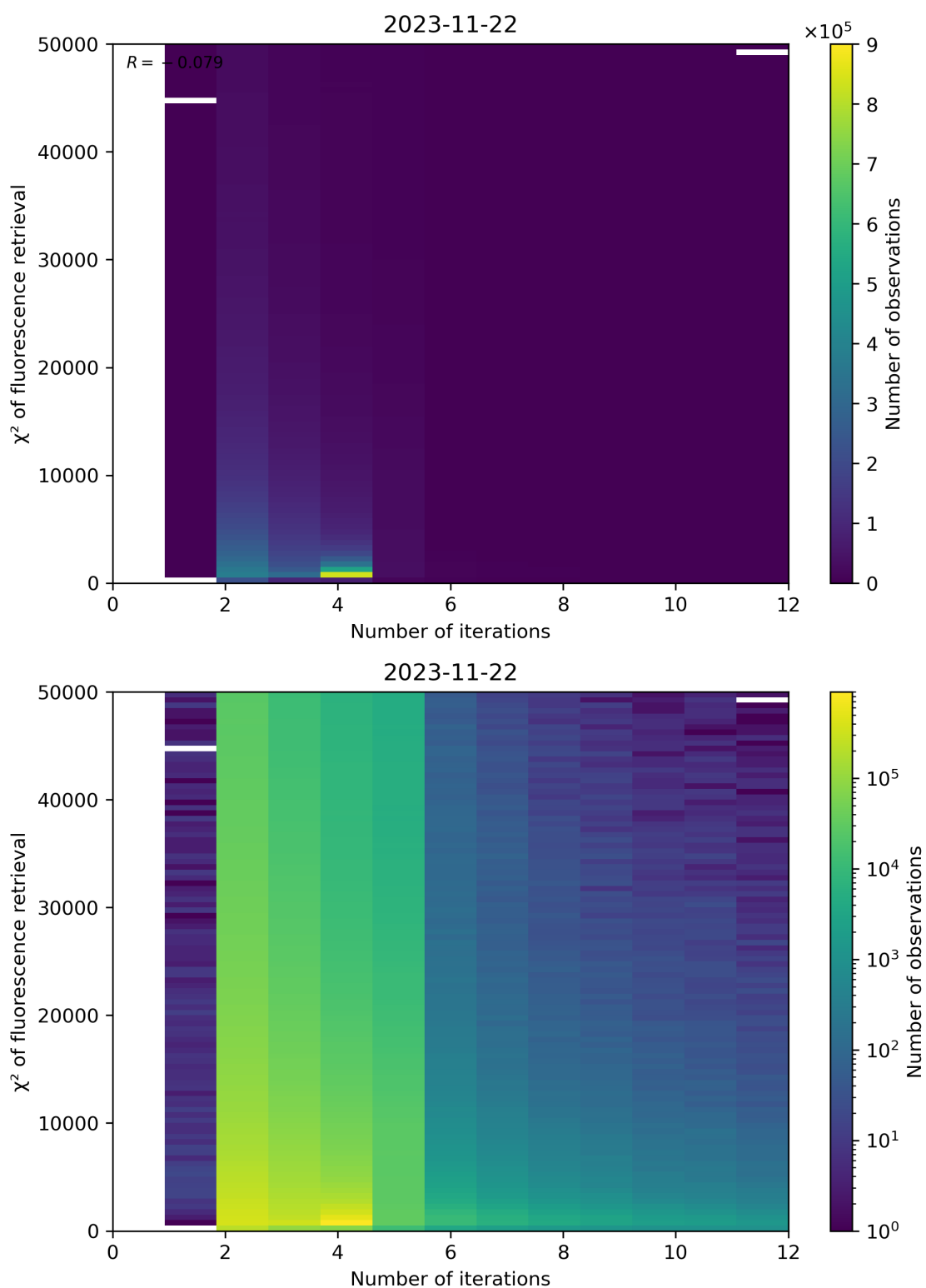
Figure 106: Scatter density plot of “Number of iterations” against “ \chi^2 of fluorescence retrieval” for 2023-11-21 to 2023-11-23.
