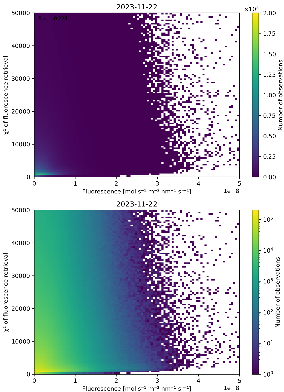
Figure 93: Scatter density plot of “Fluorescence” against “ \chi^2 of fluorescence retrieval” for 2023-11-21 to 2023-11-23.
