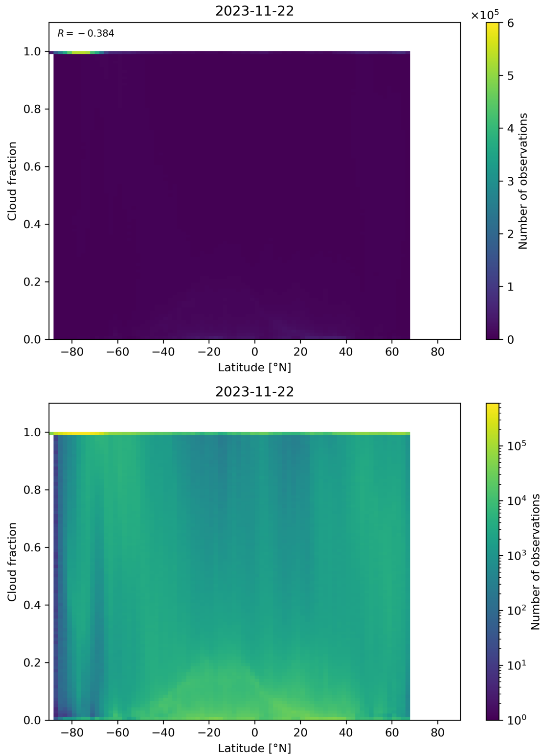
Figure 99: Scatter density plot of “Latitude” against “Cloud fraction” for 2023-11-21 to 2023-11-23.
