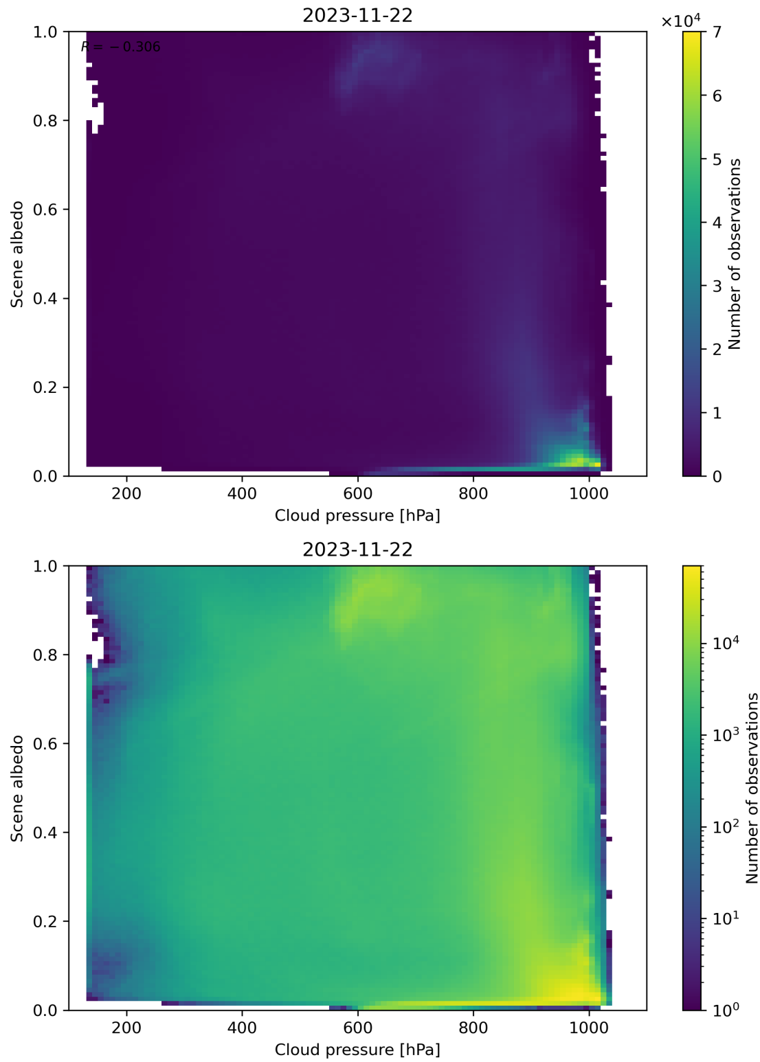
Figure 91: Scatter density plot of “Cloud pressure” against “Scene albedo” for 2023-11-21 to 2023-11-23.
