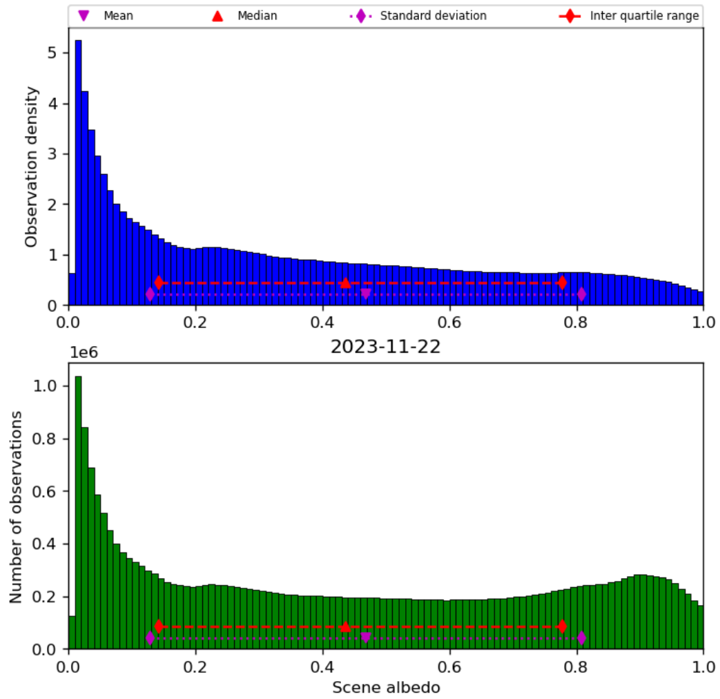
Figure 34: Histogram of “Scene albedo” for 2023-11-21 to 2023-11-23
