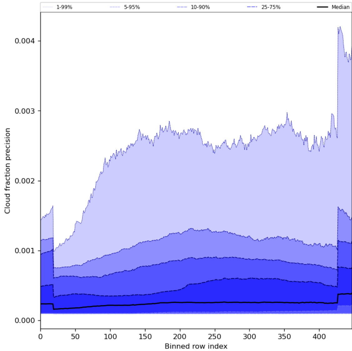
Figure 50: Along track statistics of “Cloud fraction precision” for 2023-11-21 to 2023-11-23
