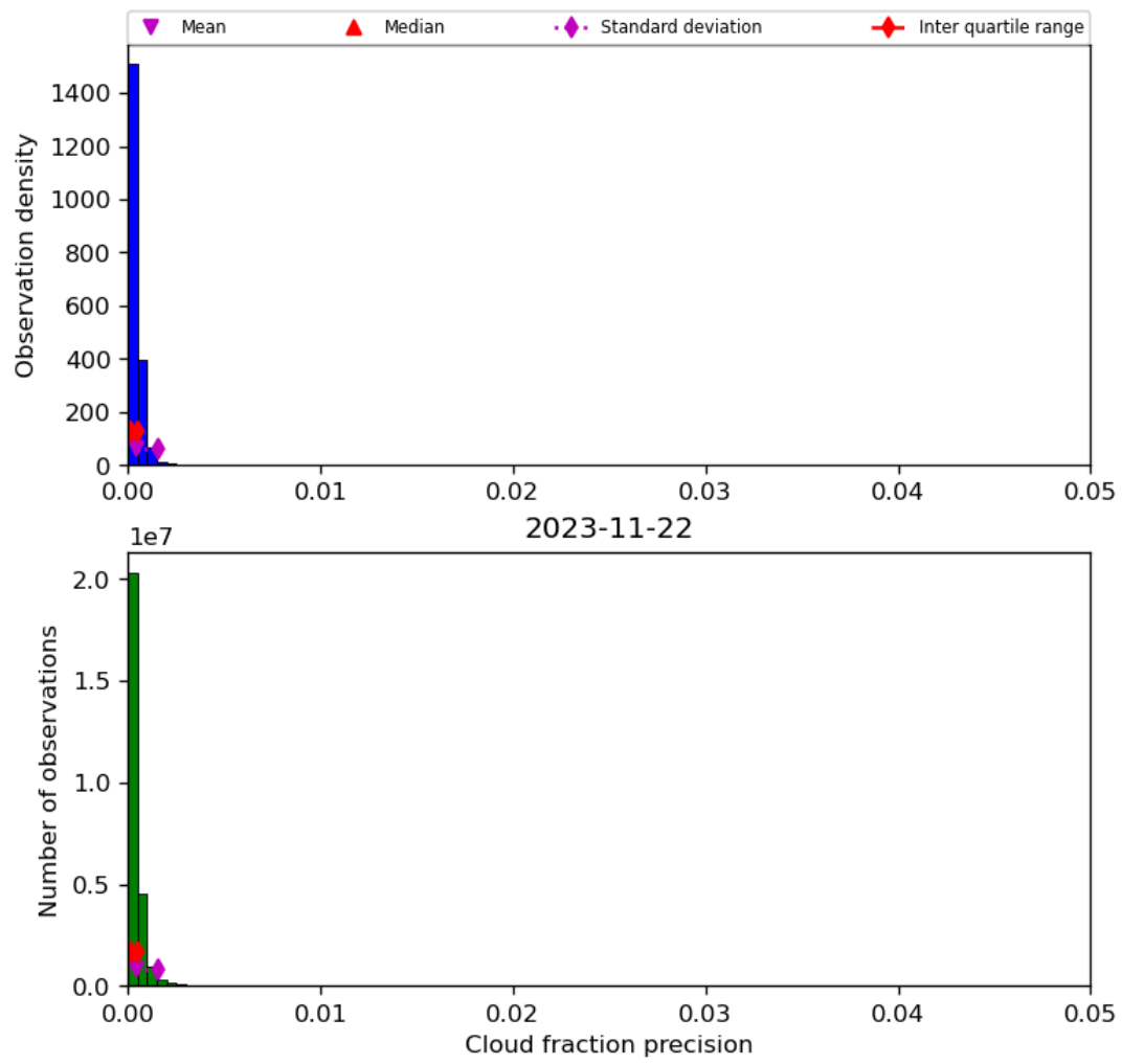
Figure 33: Histogram of “Cloud fraction precision” for 2023-11-21 to 2023-11-23
