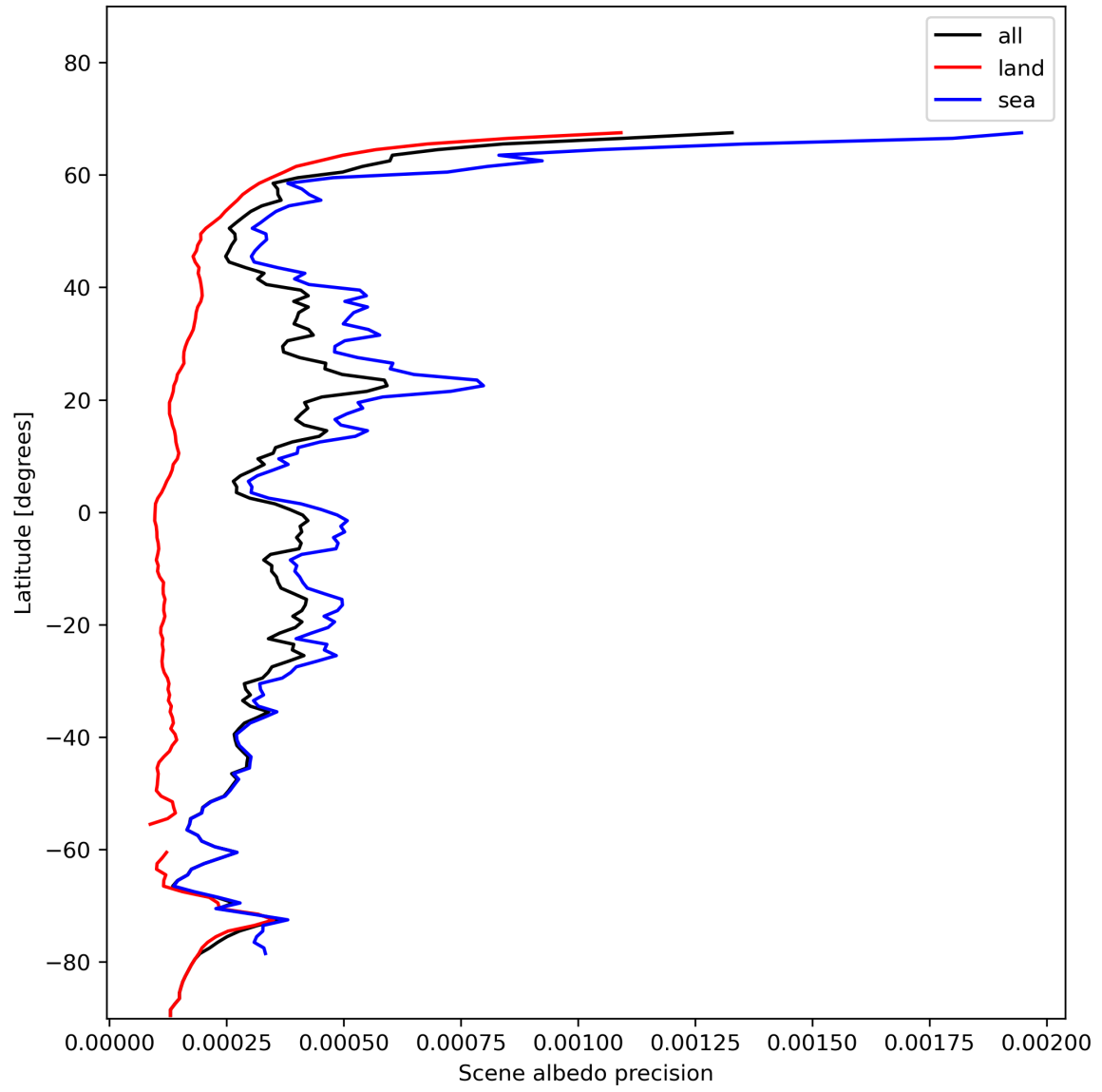
Figure 18: Zonal average of "Scene albedo precision" for 2023-11-21 to 2023-11-23.
