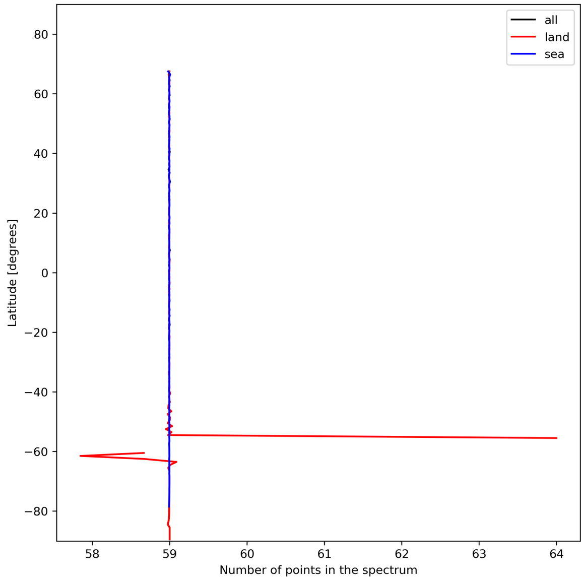
Figure 27: Zonal average of “Number of points in the spectrum” for 2023-11-21 to 2023-11-23.
