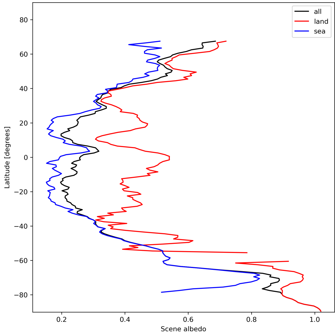
Figure 17: Zonal average of "Scene albedo" for 2023-11-21 to 2023-11-23.
