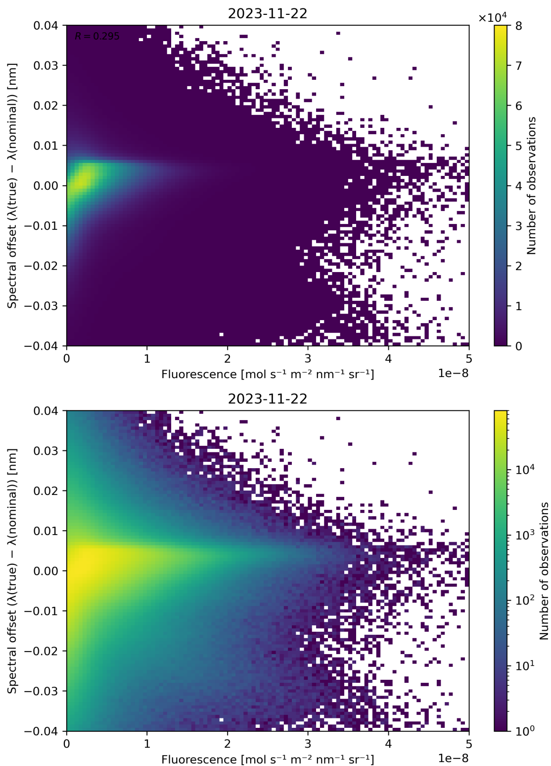
Figure 95: Scatter density plot of “Fluorescence” against “Spectral offset ( \lambda(\text{true}) - \lambda(\text{nominal}) )” for 2023-11-21 to 2023-11-23.
