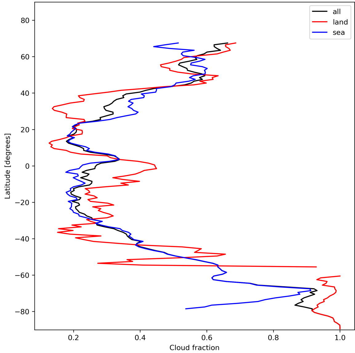
Figure 15: Zonal average of “Cloud fraction” for 2023-11-21 to 2023-11-23.
