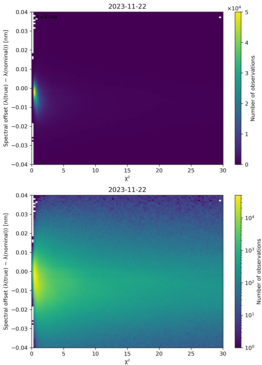
Figure 75: Scatter density plot of “ \chi^2 ” against “Spectral offset ( \lambda(\text{true}) - \lambda(\text{nominal}) )” for 2023-11-21 to 2023-11-23.
