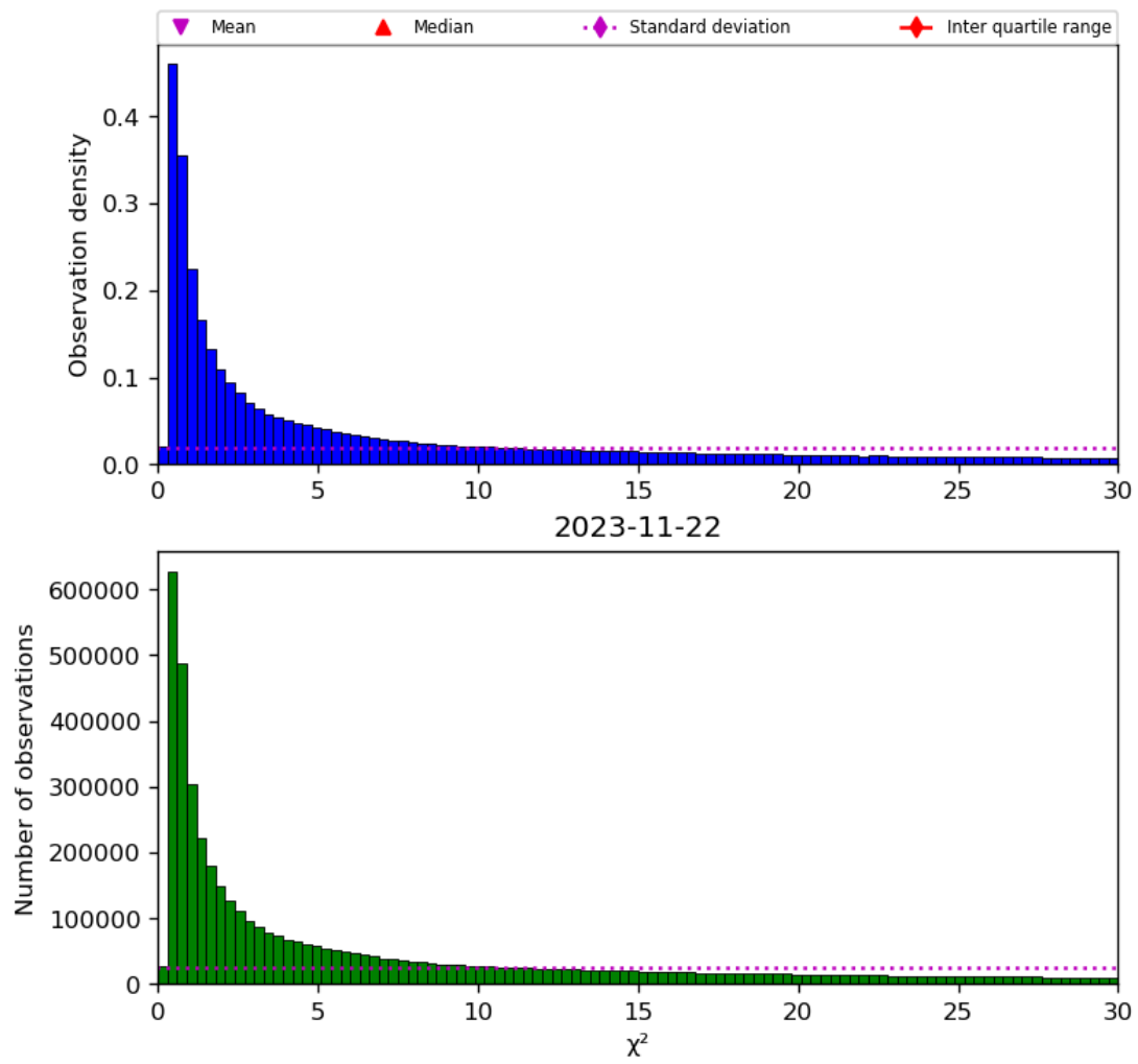
Figure 38: Histogram of " \chi^2 " for 2023-11-21 to 2023-11-23
