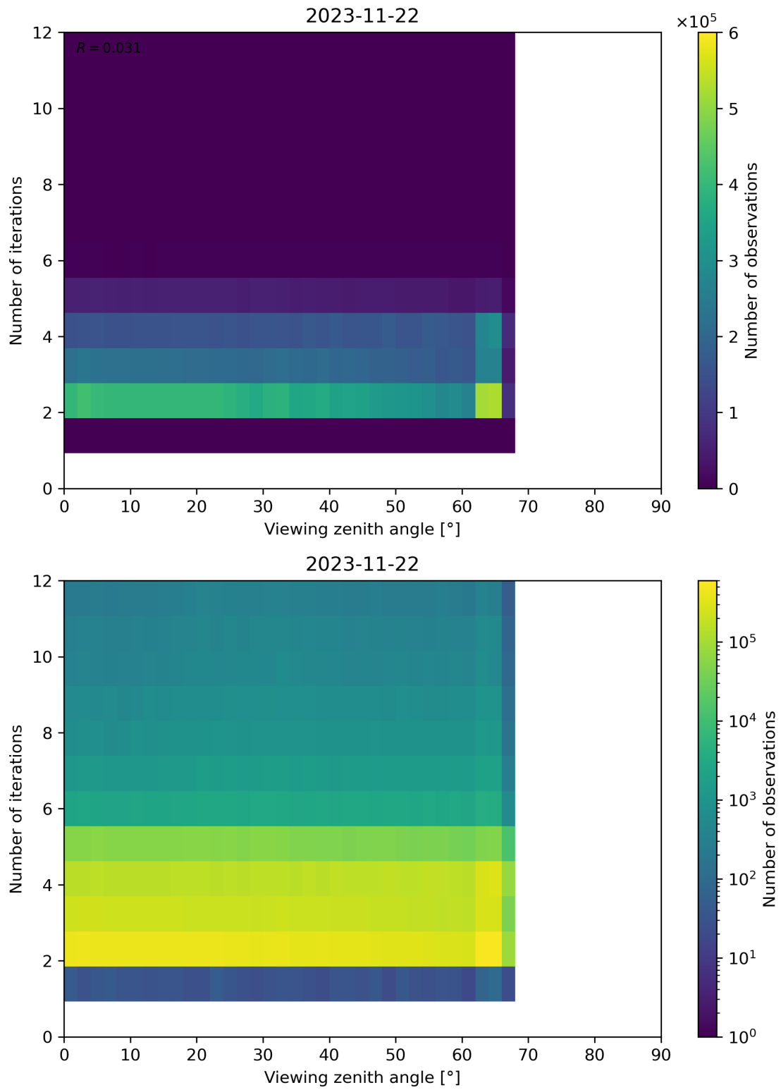
Figure 136: Scatter density plot of “Viewing zenith angle” against “Number of iterations” for 2023-11-21 to 2023-11-23.
