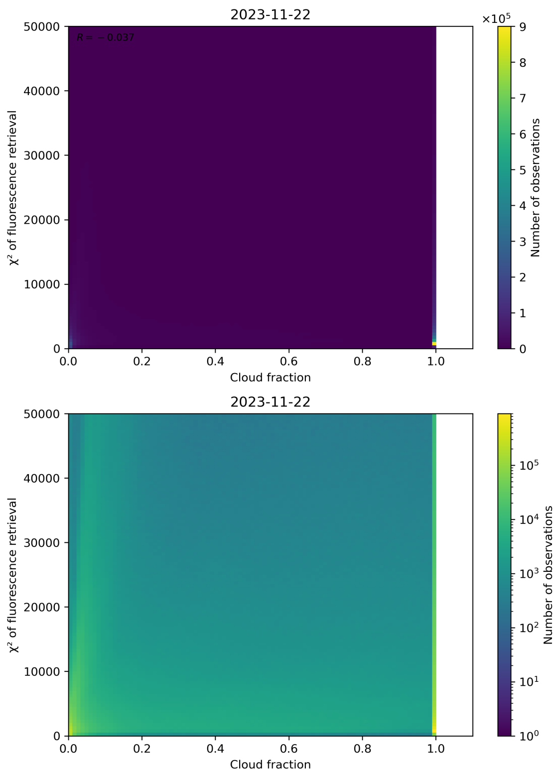
Figure 78: Scatter density plot of “Cloud fraction” against “ \chi^2 of fluorescence retrieval” for 2023-11-21 to 2023-11-23.
