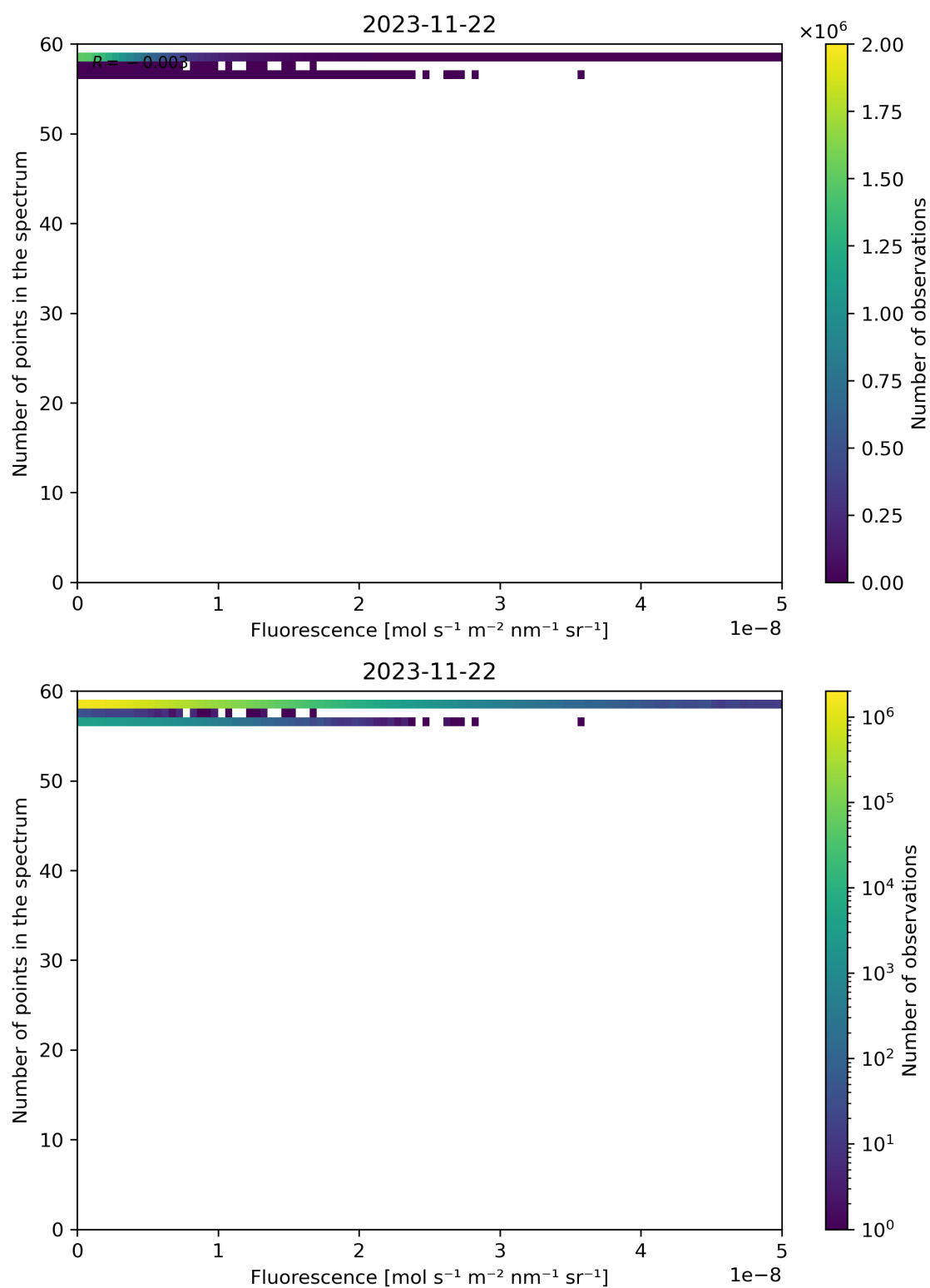
Figure 94: Scatter density plot of “Fluorescence” against “Number of points in the spectrum” for 2023-11-21 to 2023-11-23.
