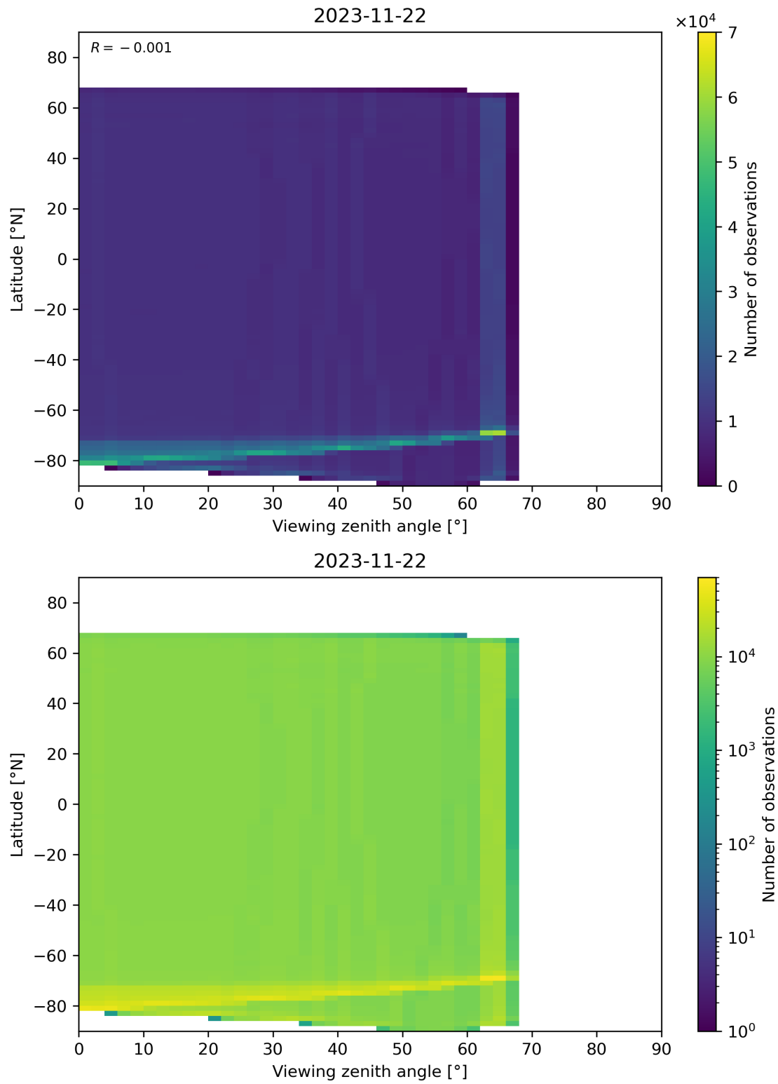
Figure 135: Scatter density plot of “Viewing zenith angle” against “Latitude” for 2023-11-21 to 2023-11-23.
