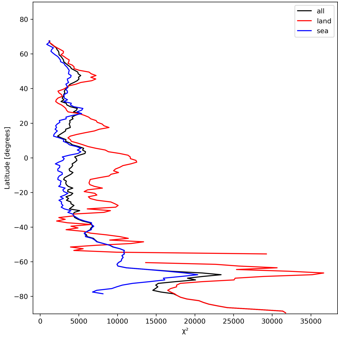
Figure 21: Zonal average of “ \chi^2 ” for 2023-11-21 to 2023-11-23.
