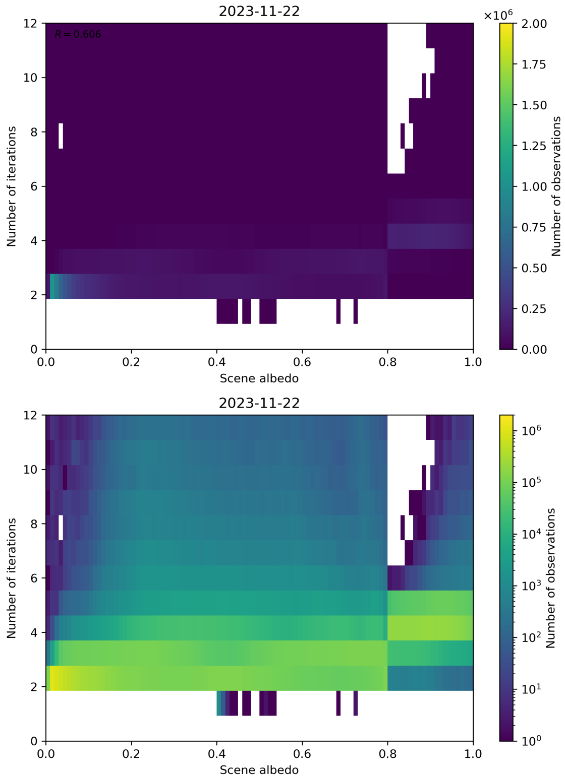
Figure 115: Scatter density plot of “Scene albedo” against “Number of iterations” for 2023-11-21 to 2023-11-23.
