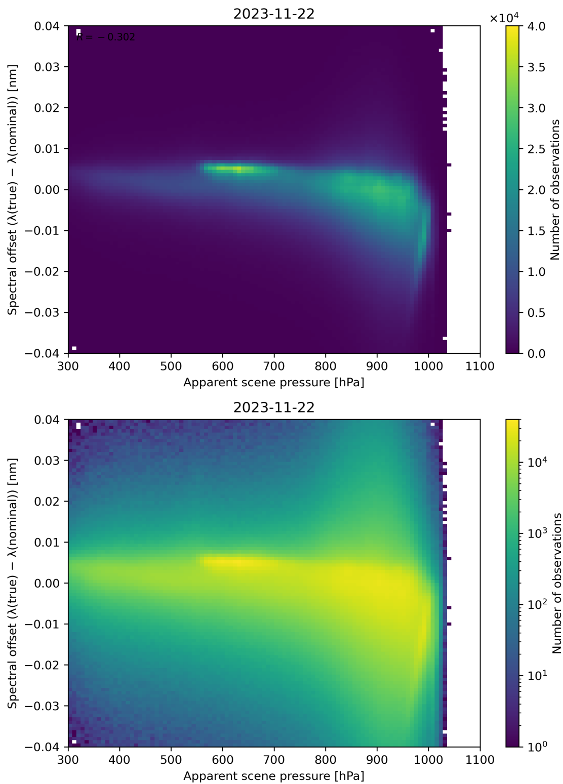
Figure 68: Scatter density plot of “Apparent scene pressure” against “Spectral offset ( \lambda(\text{true}) - \lambda(\text{nominal}) )” for 2023-11-21 to 2023-11-23.
