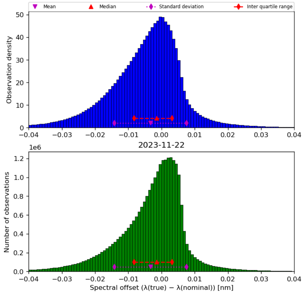
Figure 45: Histogram of “Spectral offset ( \lambda(\text{true}) - \lambda(\text{nominal}) )” for 2023-11-21 to 2023-11-23
