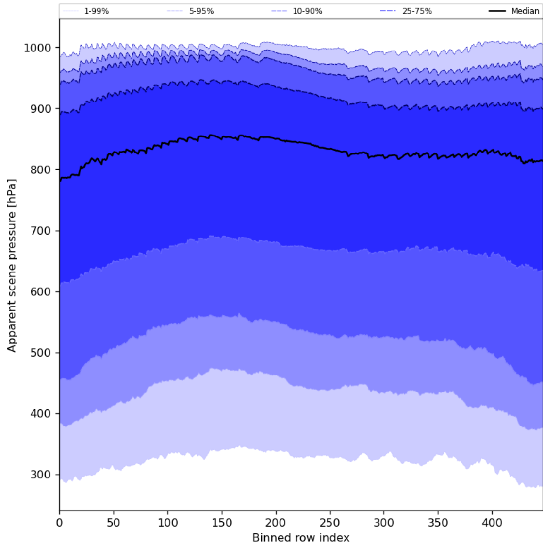
Figure 53: Along track statistics of “Apparent scene pressure” for 2023-11-21 to 2023-11-23
