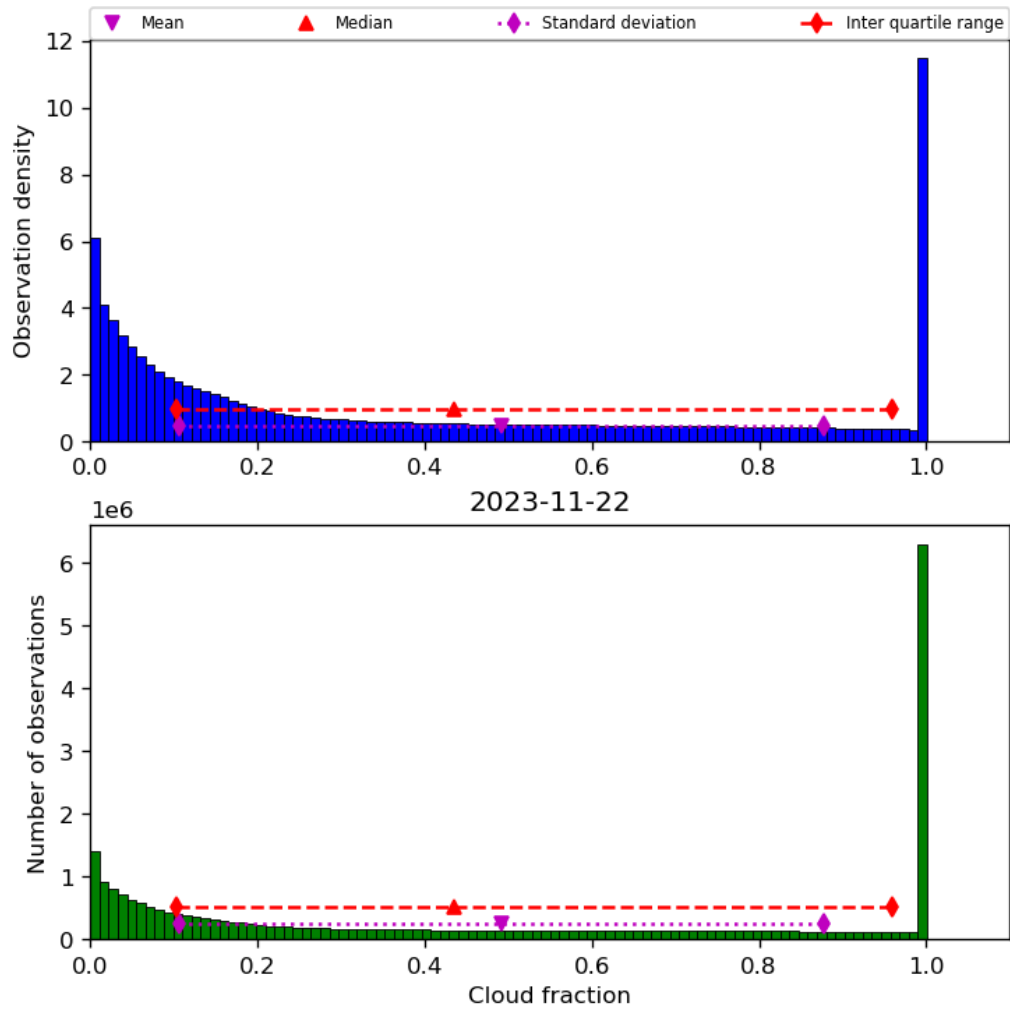
Figure 32: Histogram of “Cloud fraction” for 2023-11-21 to 2023-11-23
