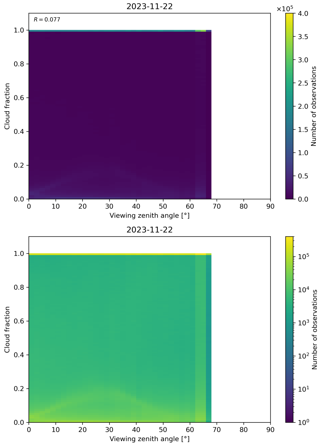
Figure 132: Scatter density plot of “Viewing zenith angle” against “Cloud fraction” for 2023-11-21 to 2023-11-23.
