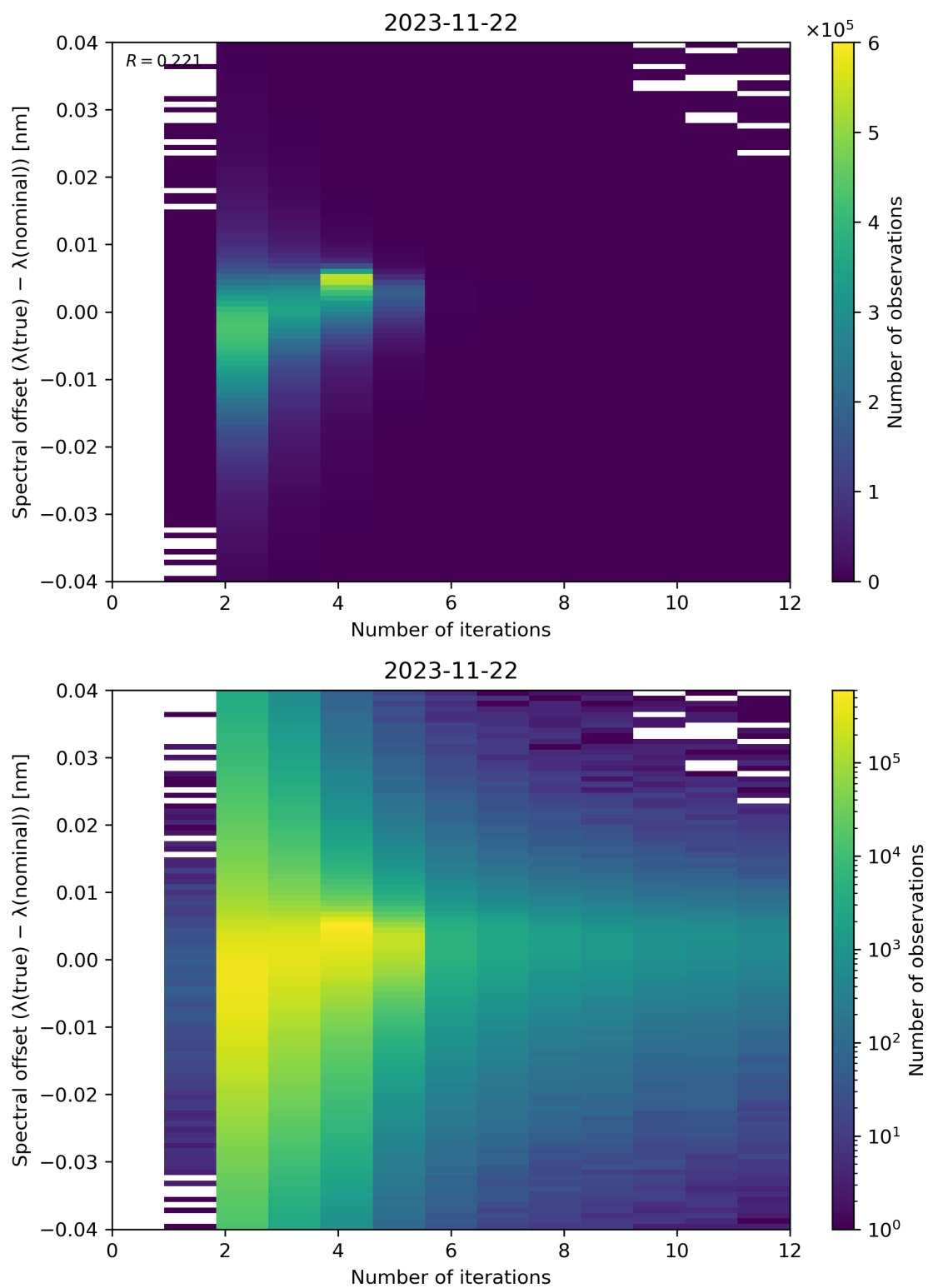
Figure 109: Scatter density plot of “Number of iterations” against “Spectral offset ( \lambda(\text{true}) - \lambda(\text{nominal}) )” for 2023-11-21 to 2023-11-23.
