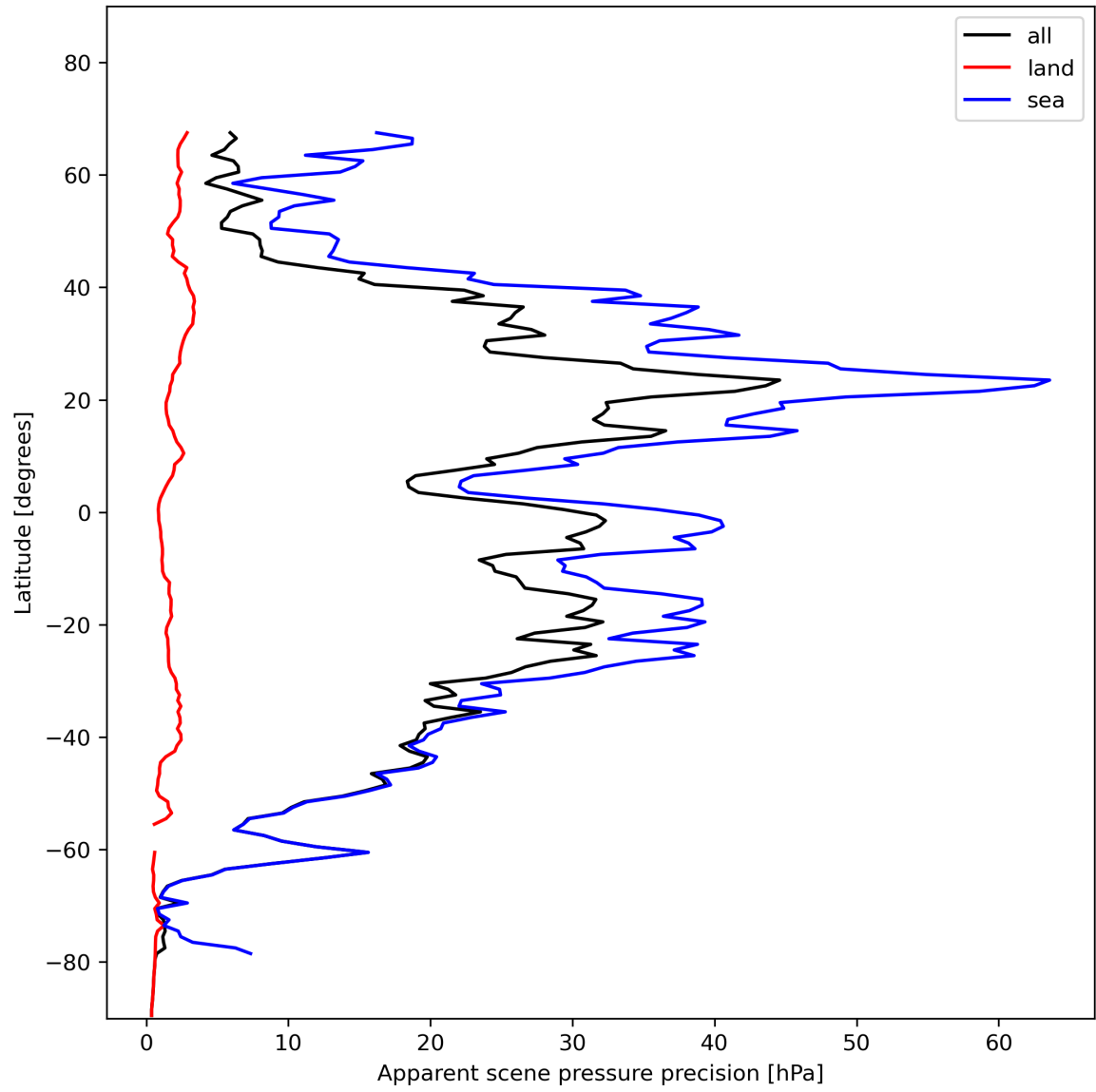
Figure 20: Zonal average of “Apparent scene pressure precision” for 2023-11-21 to 2023-11-23.
