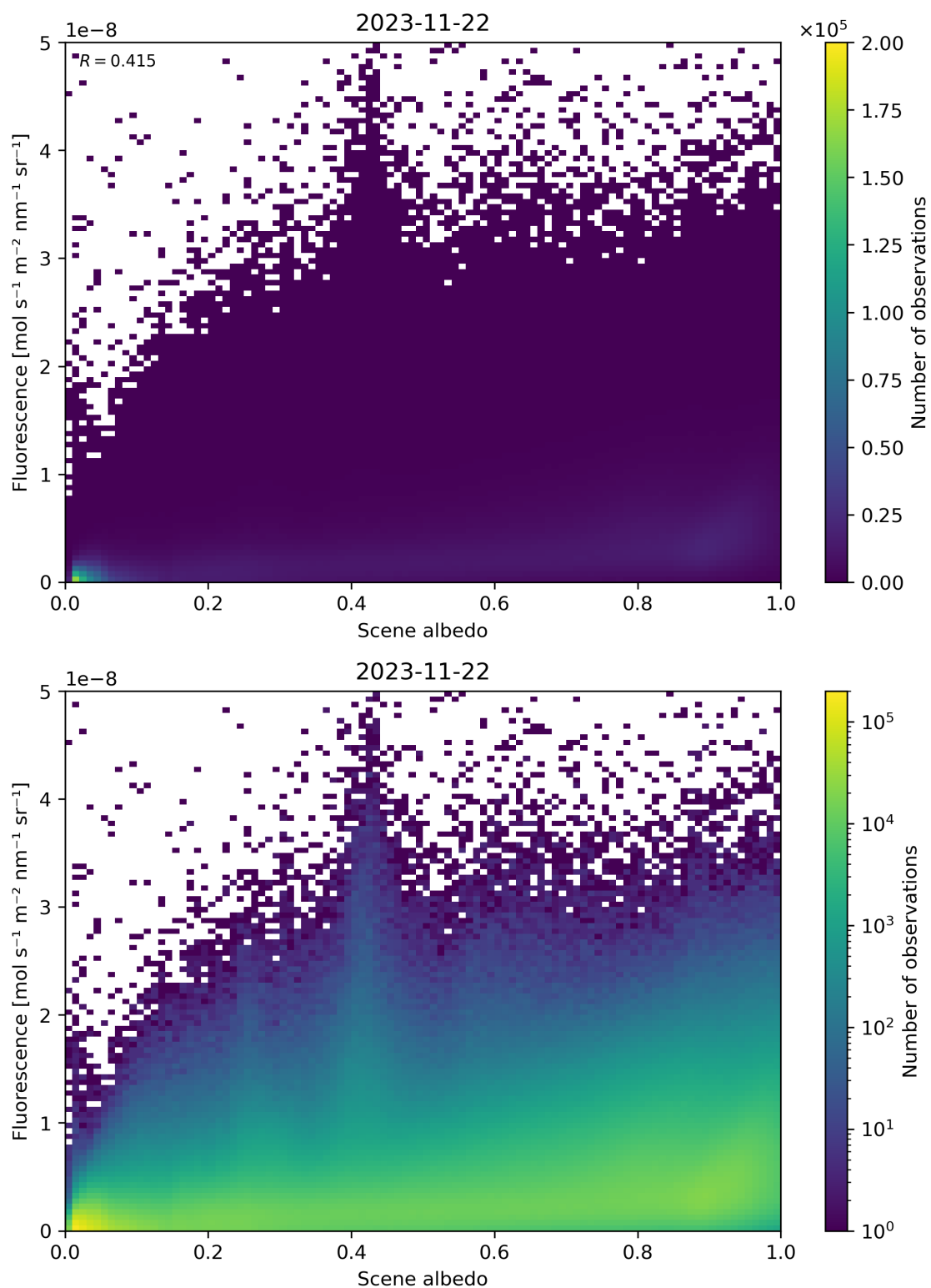
Figure 114: Scatter density plot of “Scene albedo” against “Fluorescence” for 2023-11-21 to 2023-11-23.
