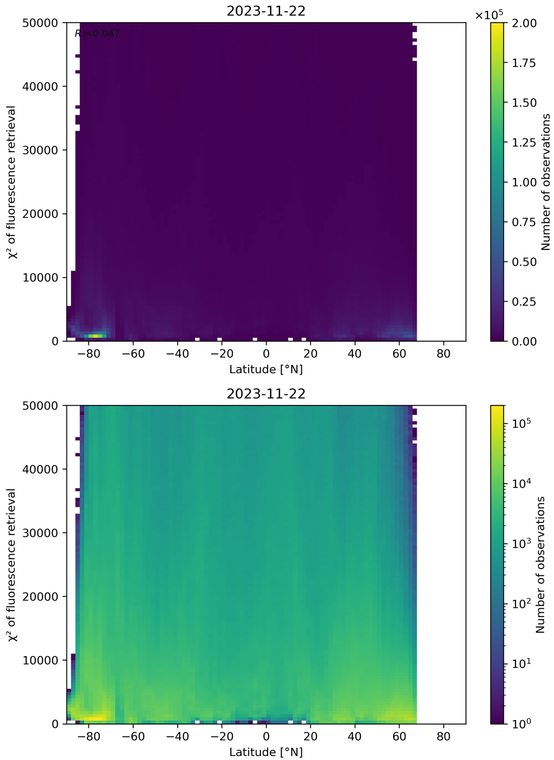
Figure 98: Scatter density plot of “Latitude” against “ \chi^2 of fluorescence retrieval” for 2023-11-21 to 2023-11-23.
