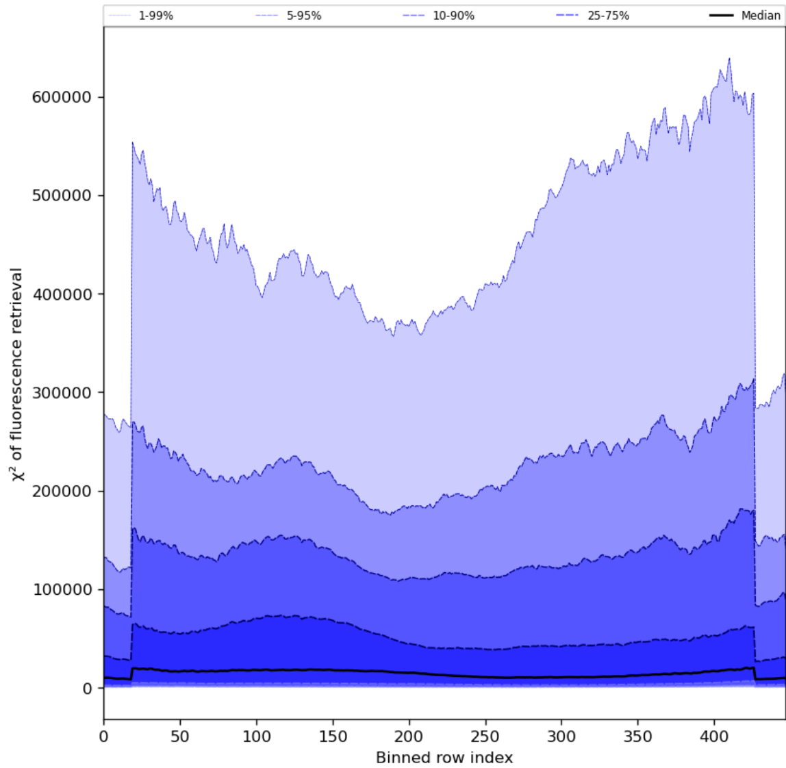
Figure 59: Along track statistics of “ \chi^2 of fluorescence retrieval” for 2023-11-21 to 2023-11-23
