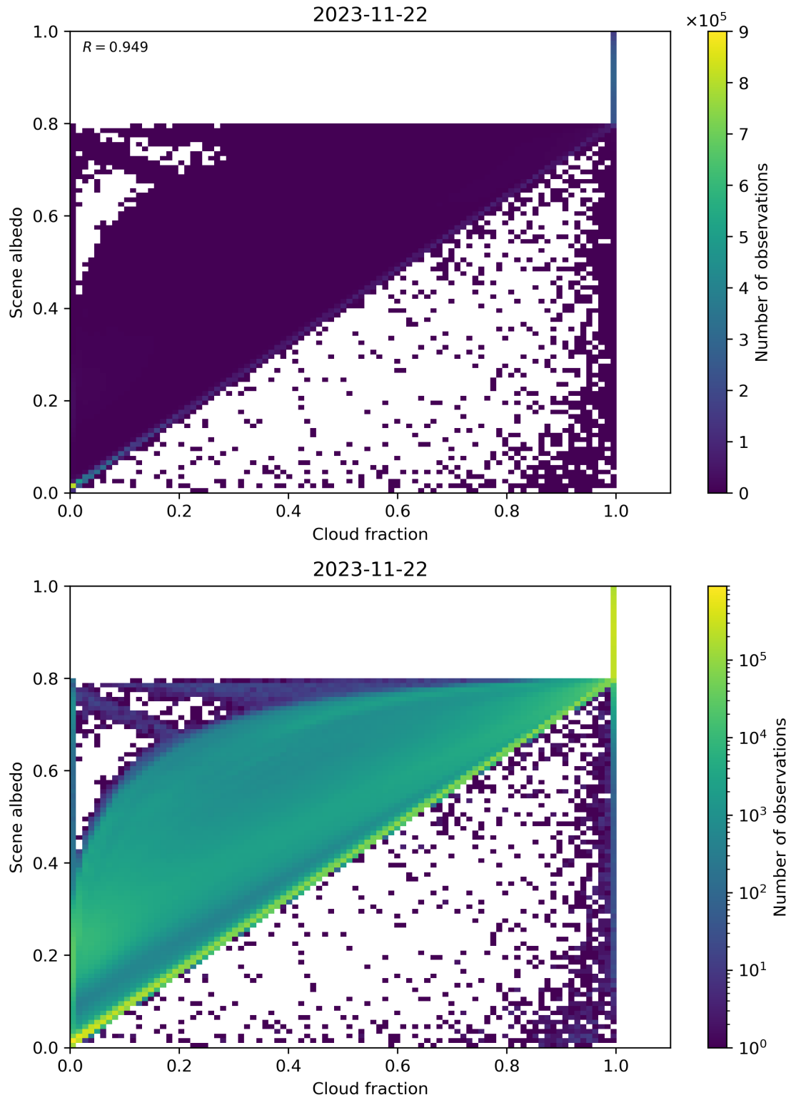
Figure 82: Scatter density plot of “Cloud fraction” against “Scene albedo” for 2023-11-21 to 2023-11-23.
