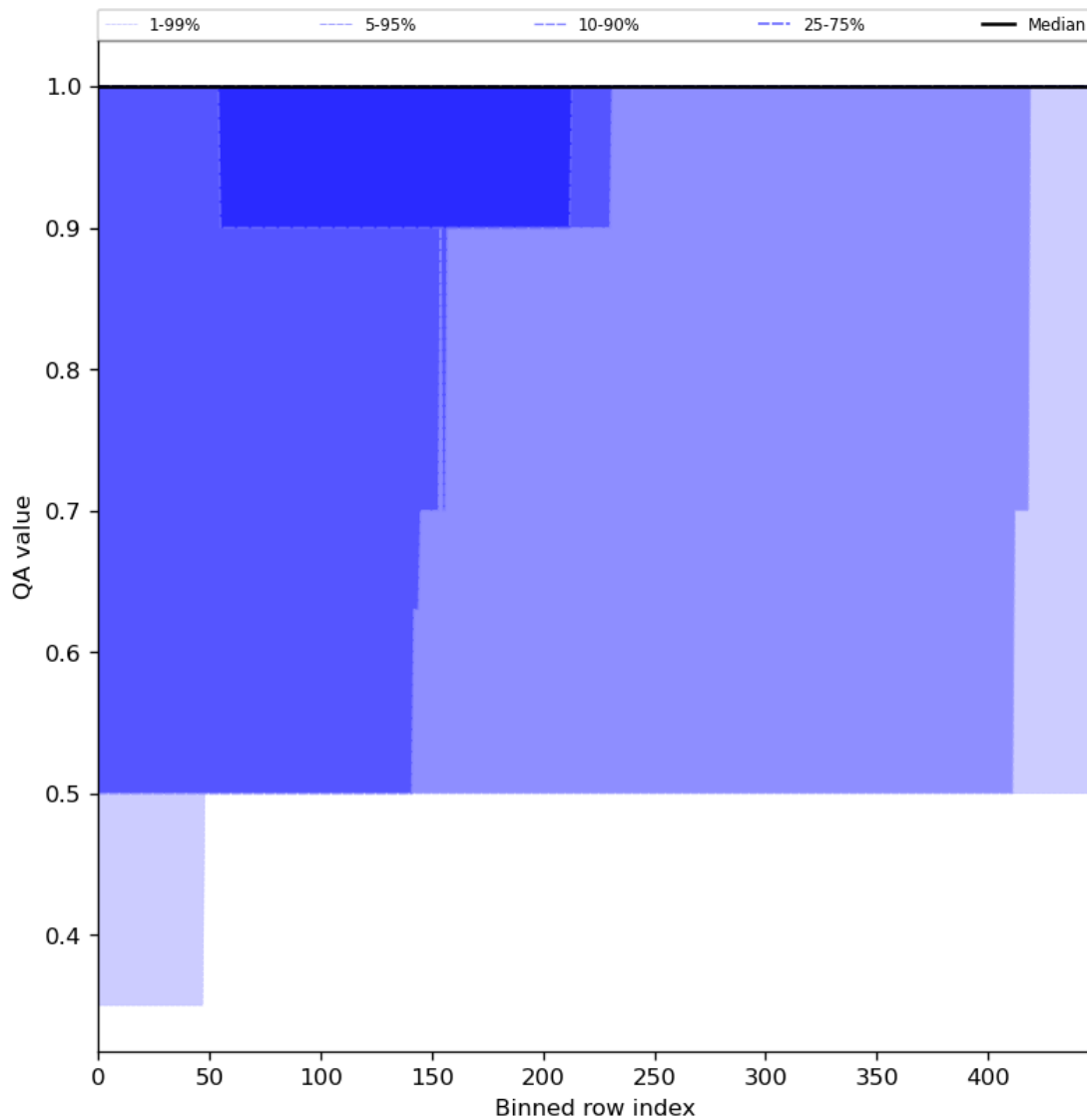
Figure 46: Along track statistics of “QA value” for 2023-11-21 to 2023-11-23
