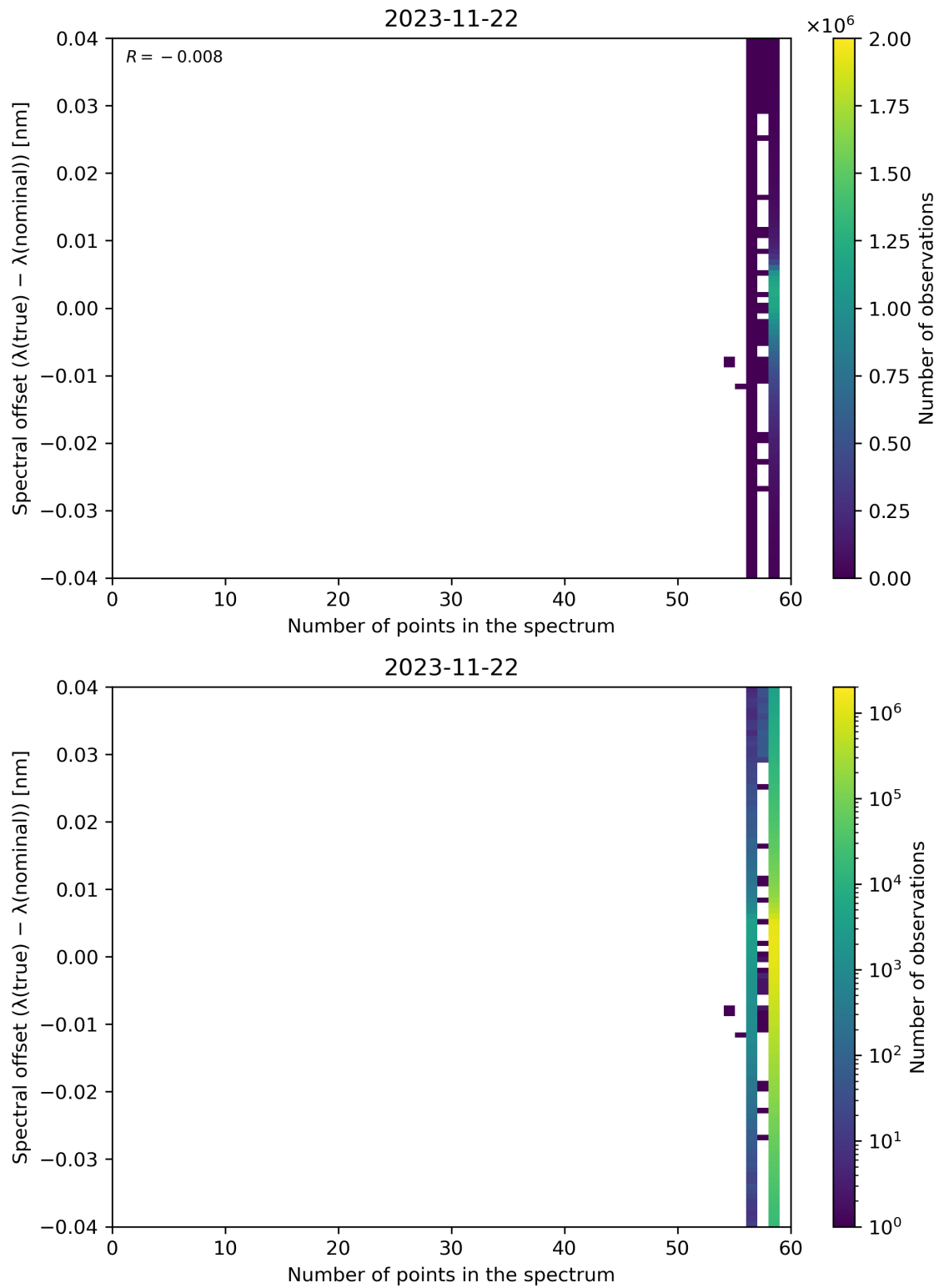
Figure 110: Scatter density plot of “Number of points in the spectrum” against “Spectral offset ( \lambda(\text{true}) - \lambda(\text{nominal}) )” for 2023-11-21 to 2023-11-23.
