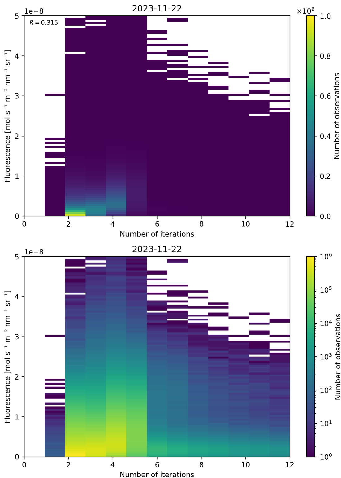
Figure 107: Scatter density plot of “Number of iterations” against “Fluorescence” for 2023-11-21 to 2023-11-23.
