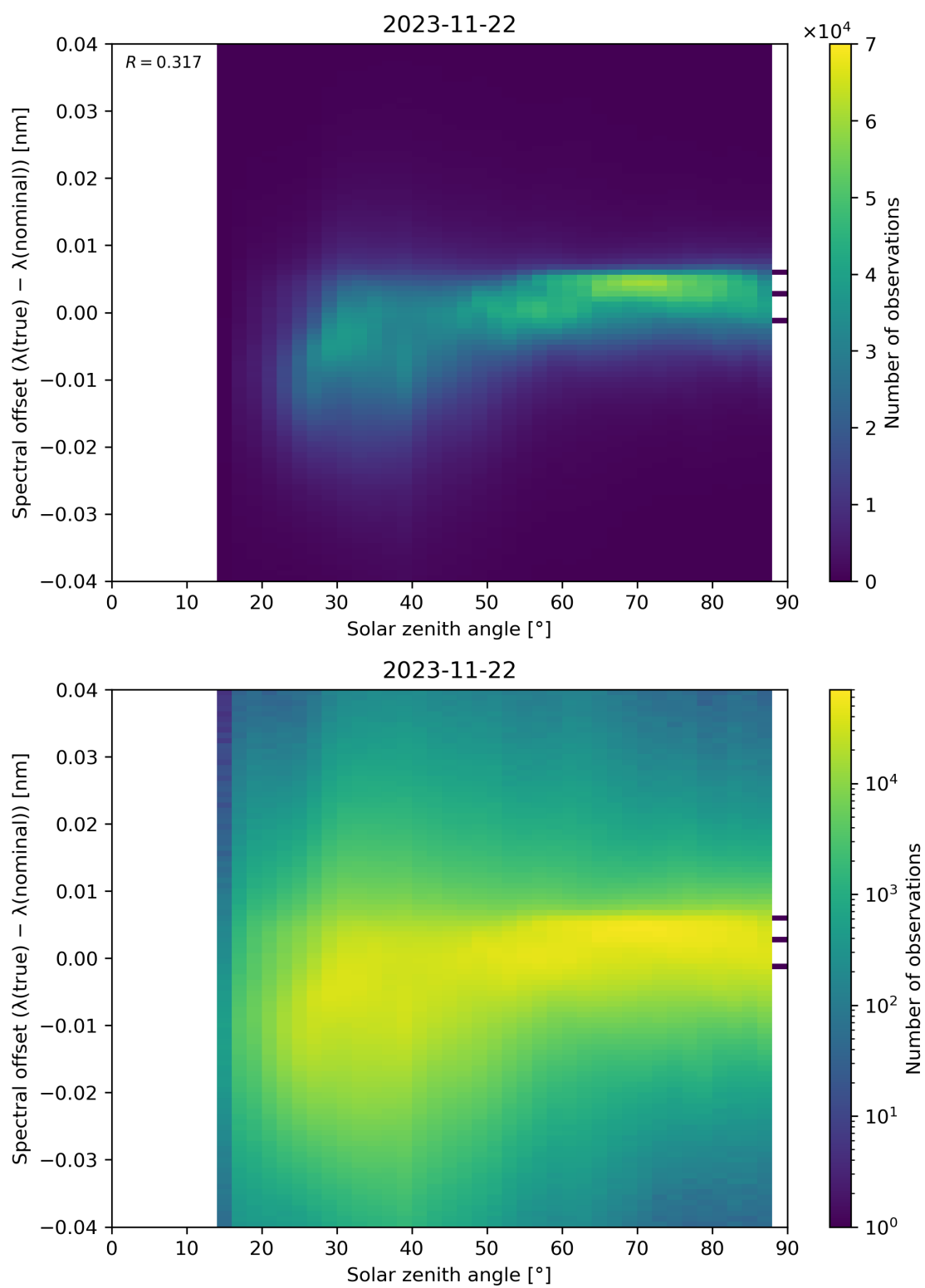
Figure 128: Scatter density plot of “Solar zenith angle” against “Spectral offset ( \lambda(\text{true}) - \lambda(\text{nominal}) )” for 2023-11-21 to 2023-11-23.
