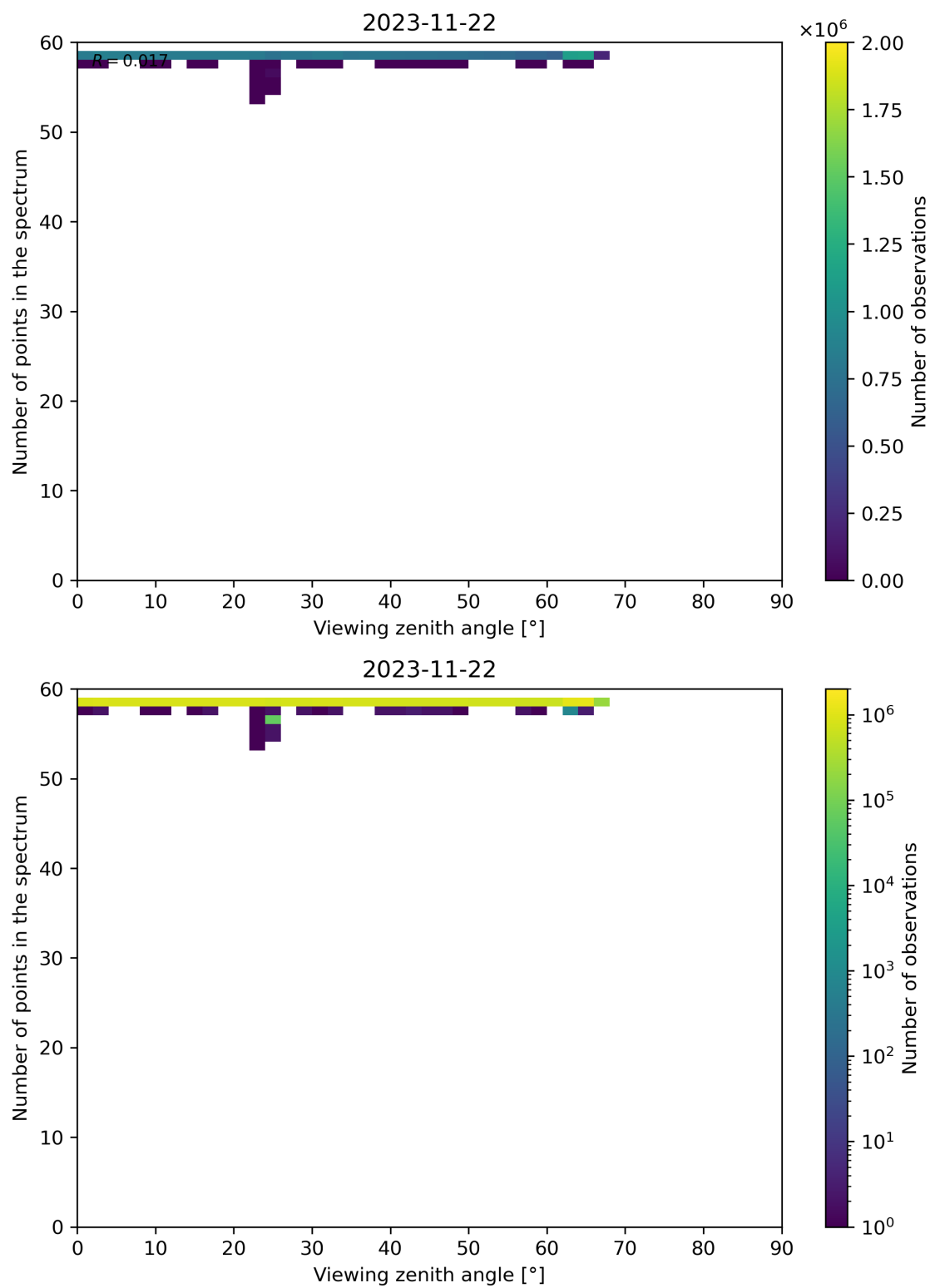
Figure 137: Scatter density plot of “Viewing zenith angle” against “Number of points in the spectrum” for 2023-11-21 to 2023-11-23.
