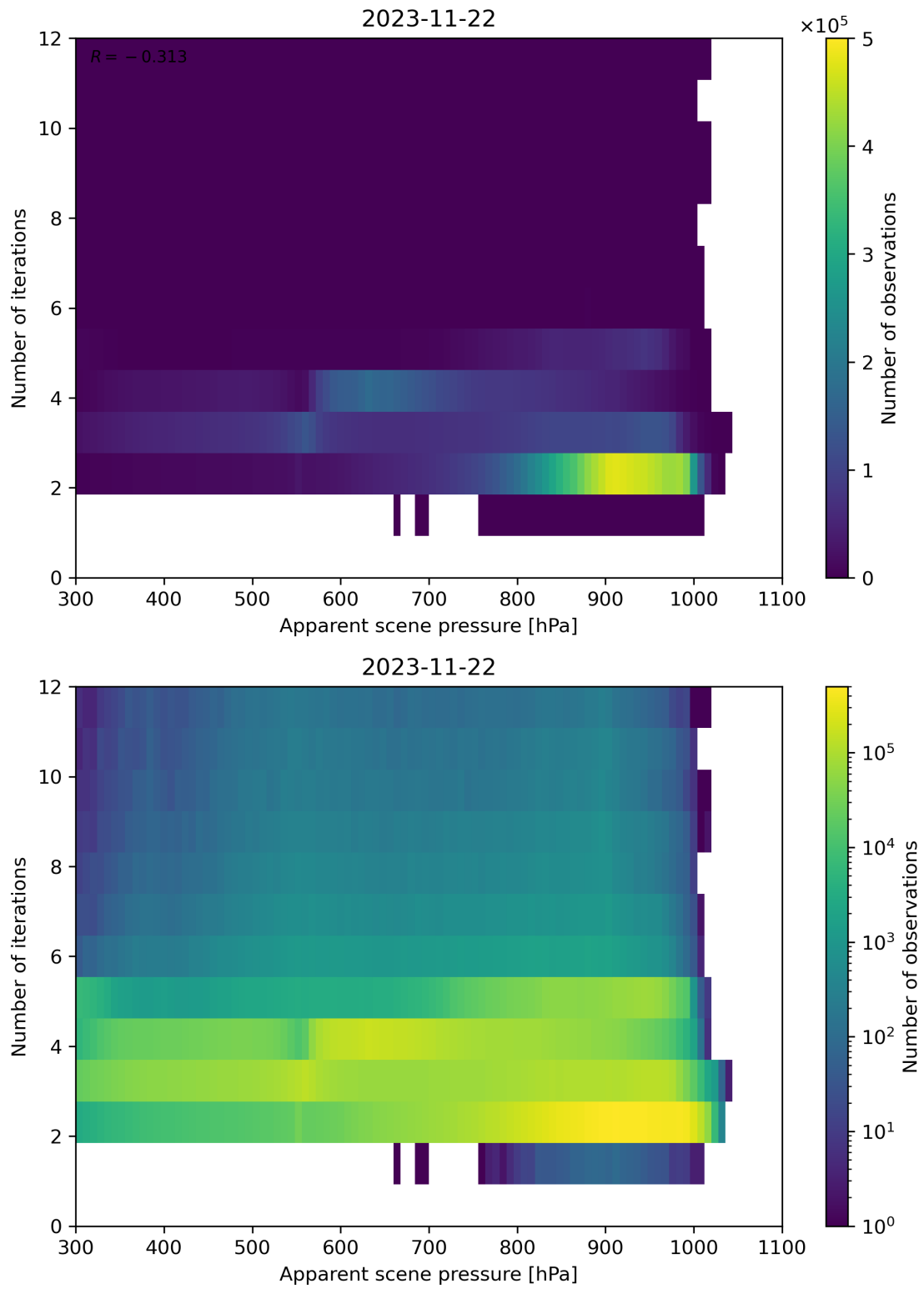
Figure 66: Scatter density plot of “Apparent scene pressure” against “Number of iterations” for 2023-11-21 to 2023-11-23.
