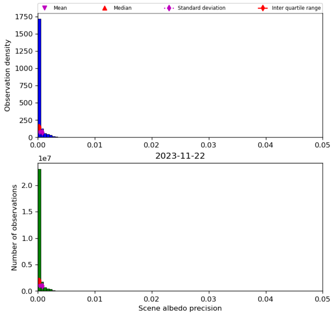
Figure 35: Histogram of “Scene albedo precision” for 2023-11-21 to 2023-11-23
