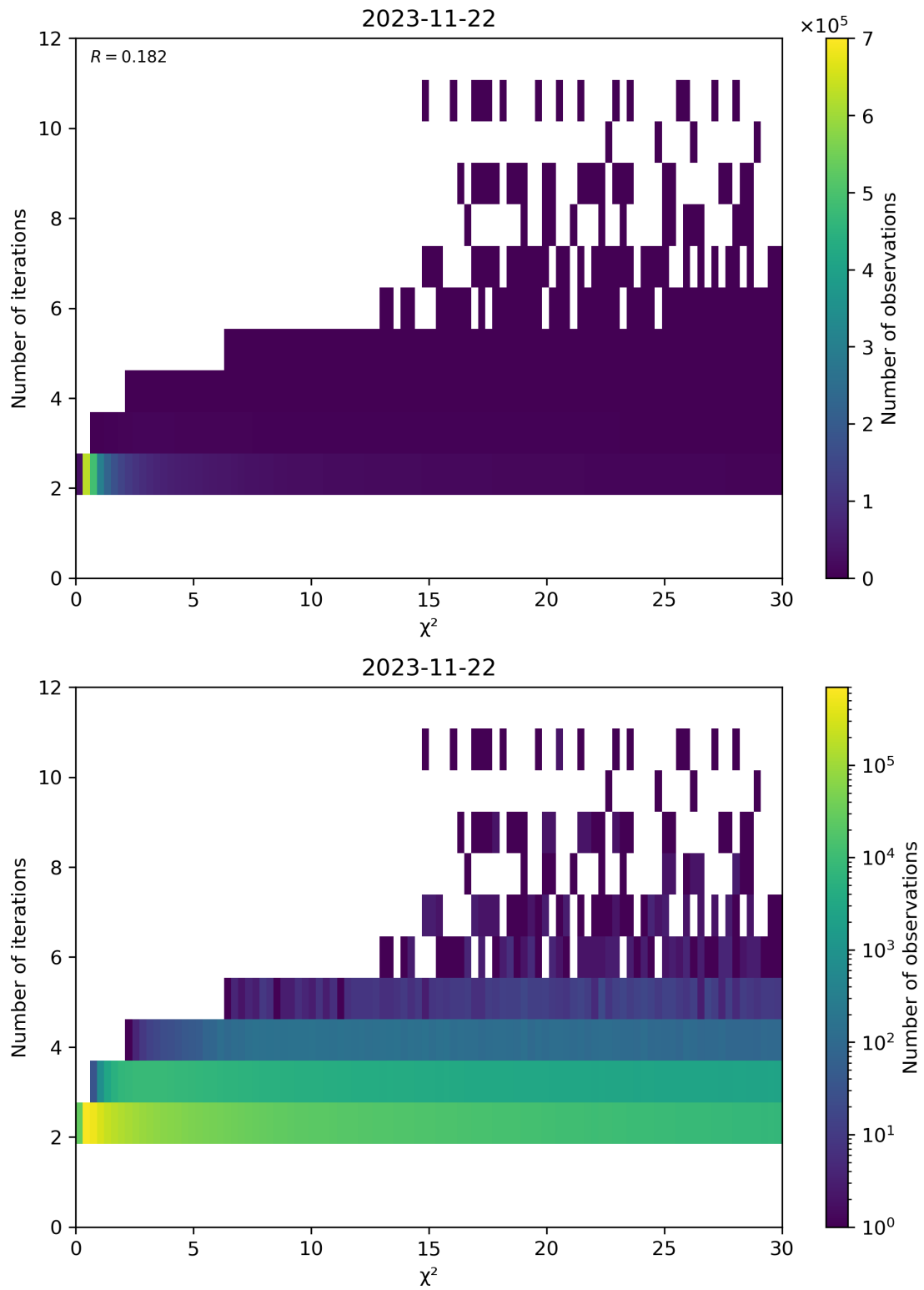
Figure 73: Scatter density plot of “ \chi^2 ” against “Number of iterations” for 2023-11-21 to 2023-11-23.
