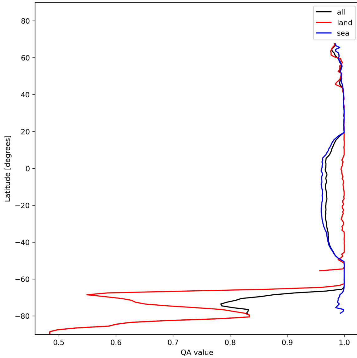
Figure 12: Zonal average of “QA value” for 2023-11-21 to 2023-11-23.
