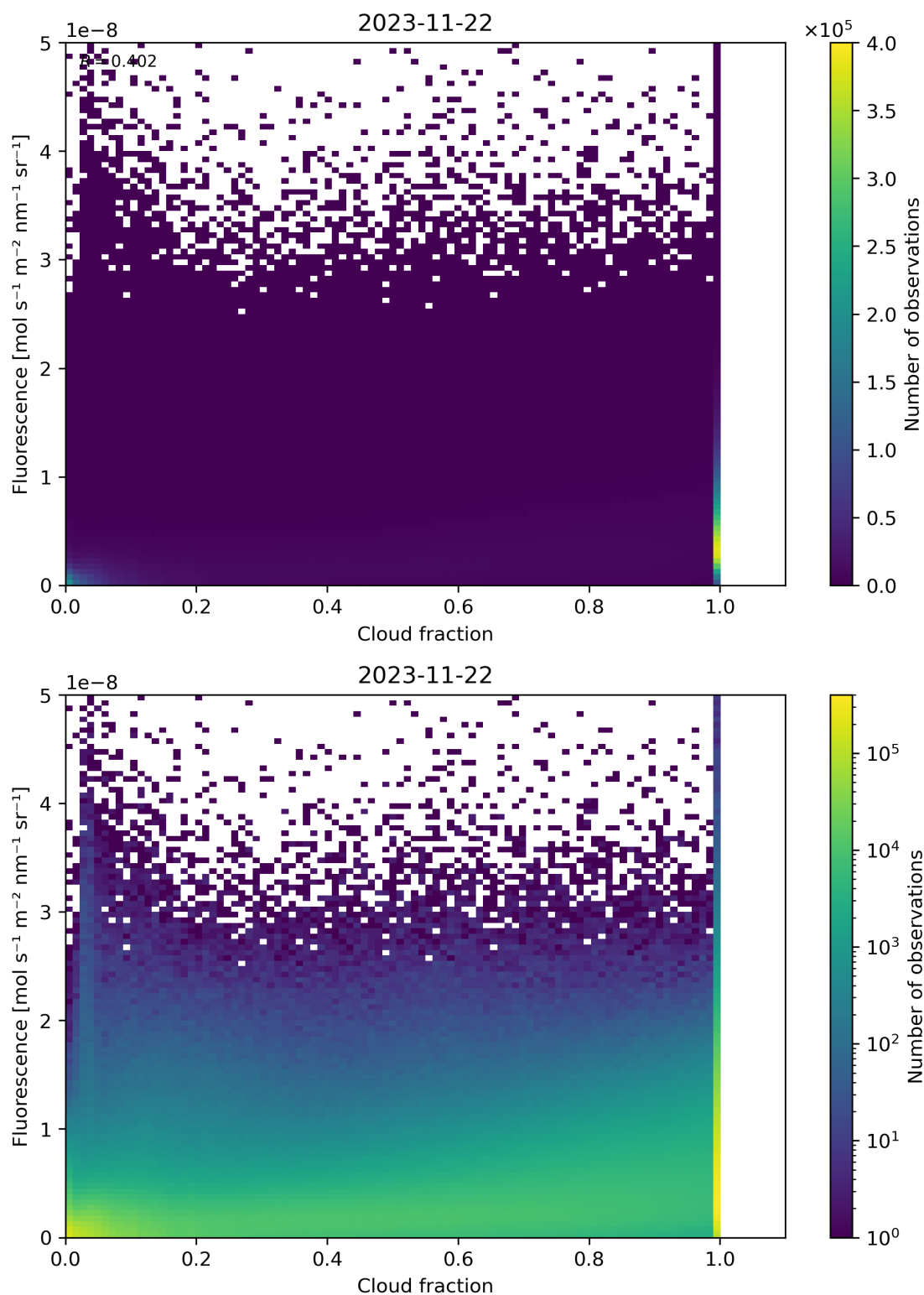
Figure 79: Scatter density plot of “Cloud fraction” against “Fluorescence” for 2023-11-21 to 2023-11-23.
