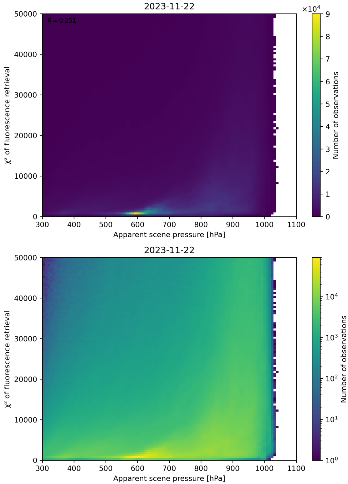
Figure 64: Scatter density plot of “Apparent scene pressure” against “ \chi^2 of fluorescence retrieval” for 2023-11-21 to 2023-11-23.
