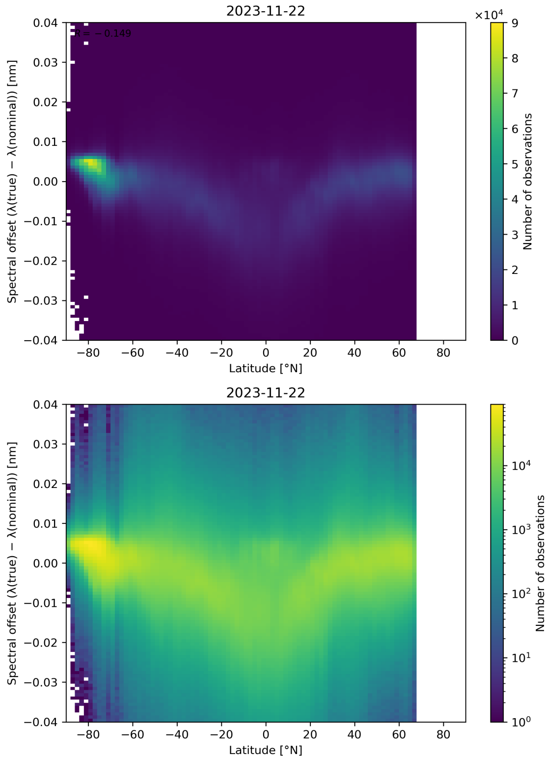
Figure 105: Scatter density plot of “Latitude” against “Spectral offset ( \lambda(\text{true}) - \lambda(\text{nominal}) )” for 2023-11-21 to 2023-11-23.
