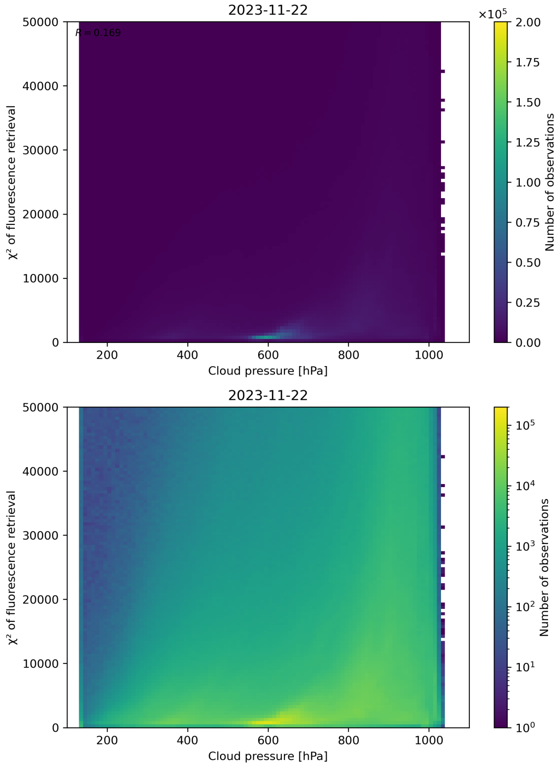
Figure 86: Scatter density plot of “Cloud pressure” against “ \chi^2 of fluorescence retrieval” for 2023-11-21 to 2023-11-23.
