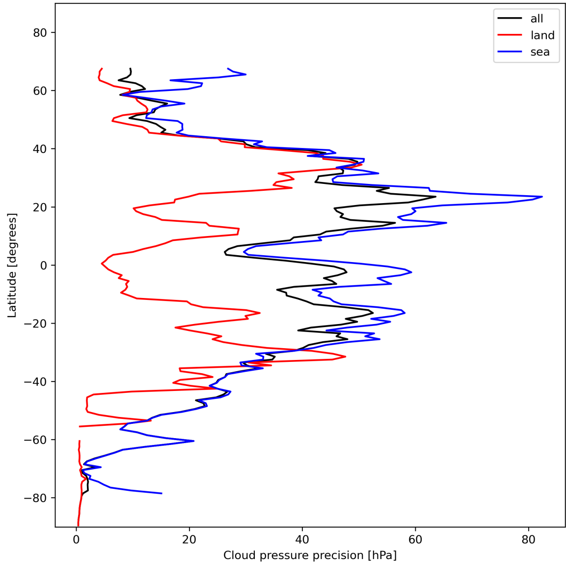
Figure 14: Zonal average of “Cloud pressure precision” for 2023-11-21 to 2023-11-23.
