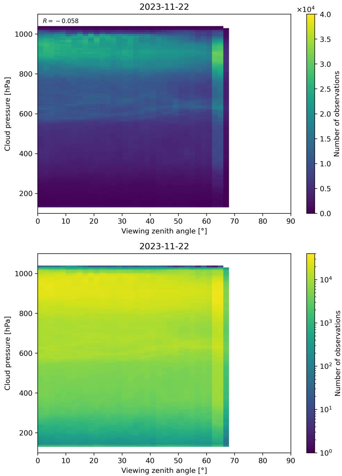
Figure 133: Scatter density plot of “Viewing zenith angle” against “Cloud pressure” for 2023-11-21 to 2023-11-23.
