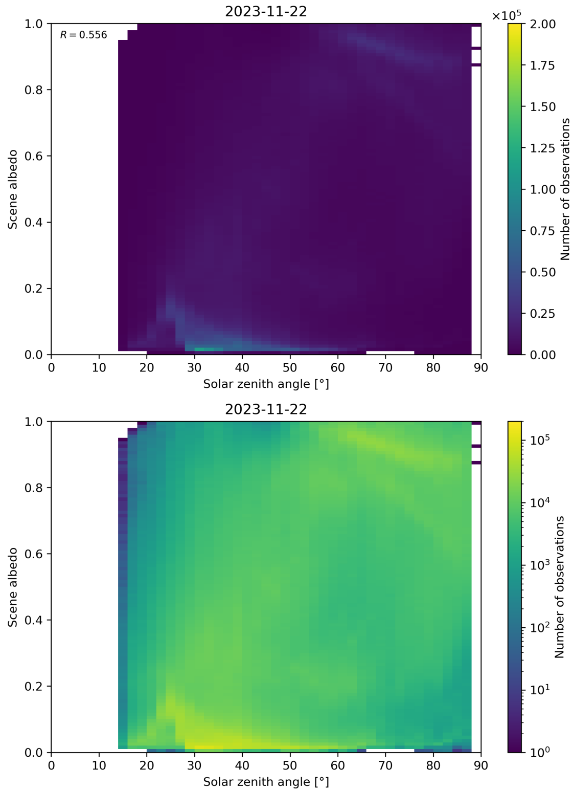
Figure 127: Scatter density plot of “Solar zenith angle” against “Scene albedo” for 2023-11-21 to 2023-11-23.
