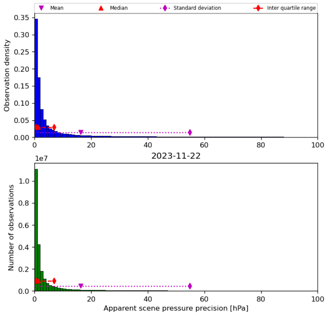
Figure 37: Histogram of “Apparent scene pressure precision” for 2023-11-21 to 2023-11-23
