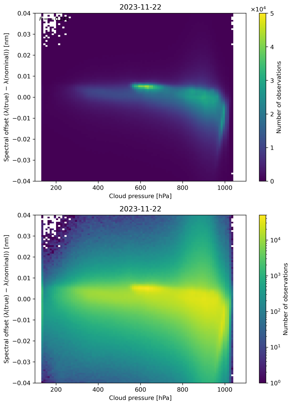
Figure 92: Scatter density plot of “Cloud pressure” against “Spectral offset ( \lambda(\text{true}) - \lambda(\text{nominal}) )” for 2023-11-21 to 2023-11-23.
