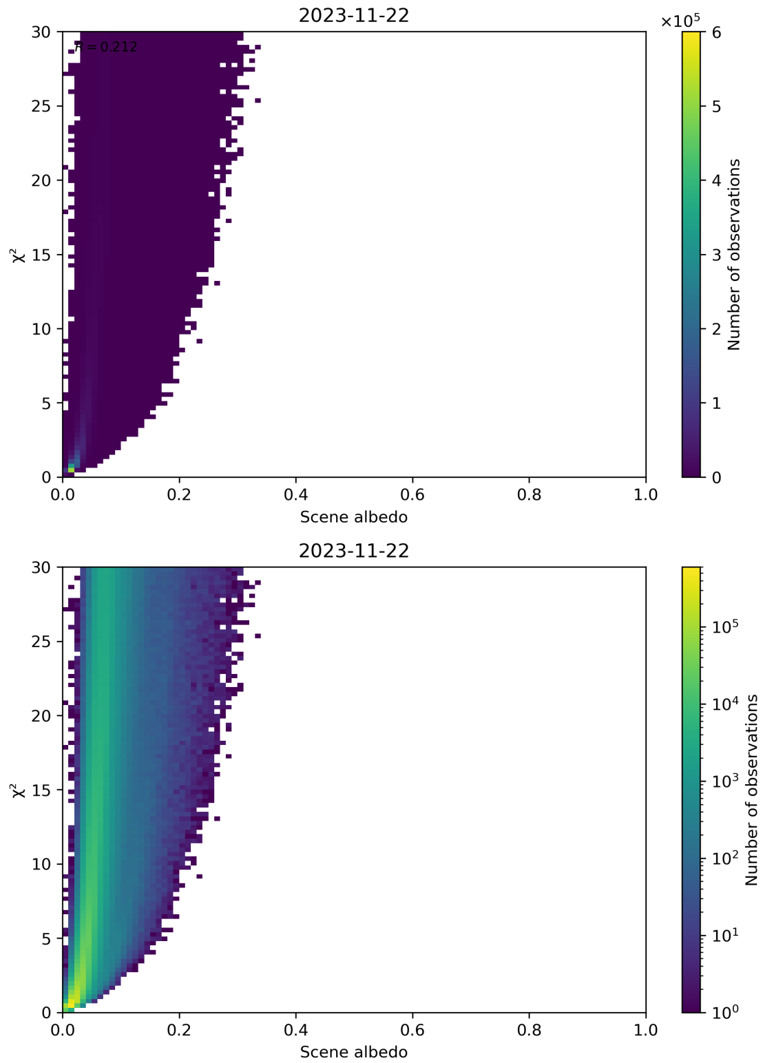
Figure 112: Scatter density plot of “Scene albedo” against “ \chi^2 ” for 2023-11-21 to 2023-11-23.
