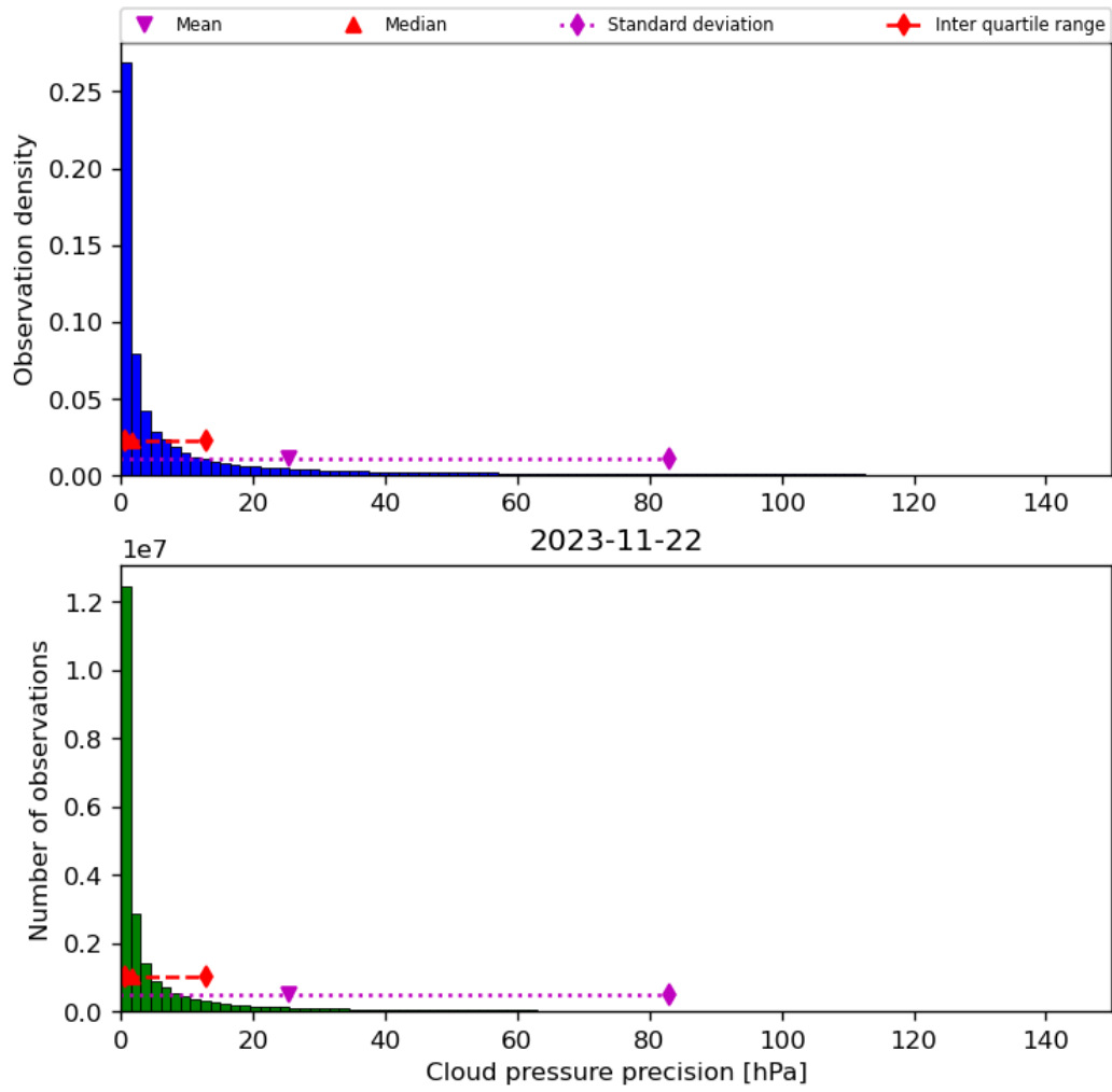
Figure 31: Histogram of “Cloud pressure precision” for 2023-11-21 to 2023-11-23
