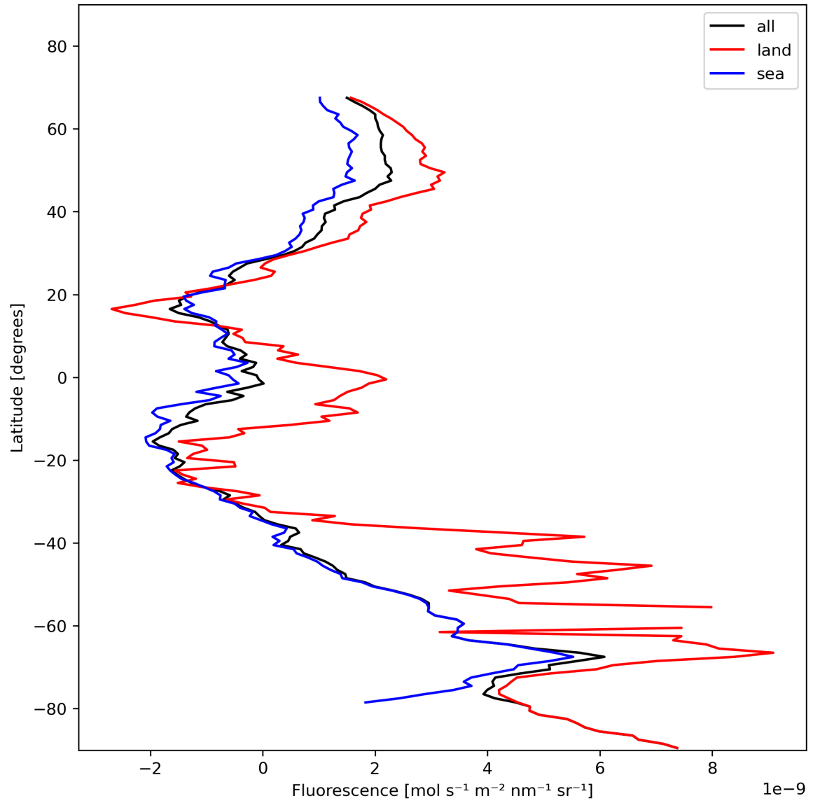
Figure 23: Zonal average of “Fluorescence” for 2023-11-21 to 2023-11-23.
