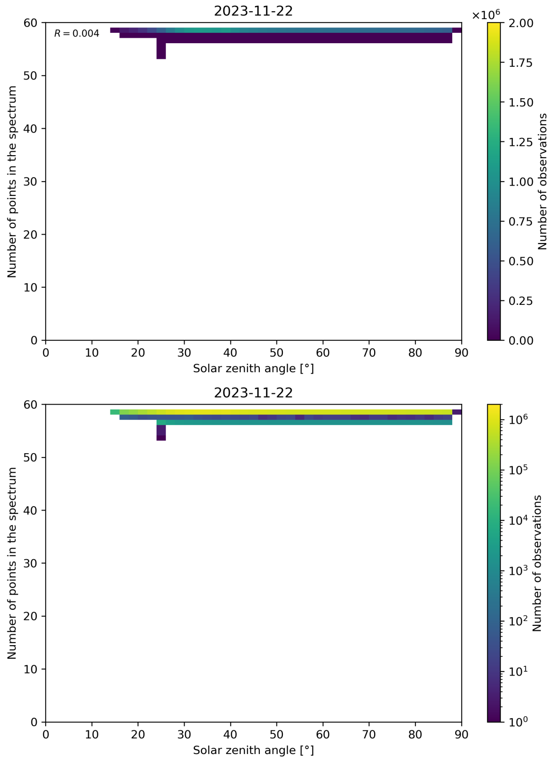
Figure 126: Scatter density plot of “Solar zenith angle” against “Number of points in the spectrum” for 2023-11-21 to 2023-11-23.
