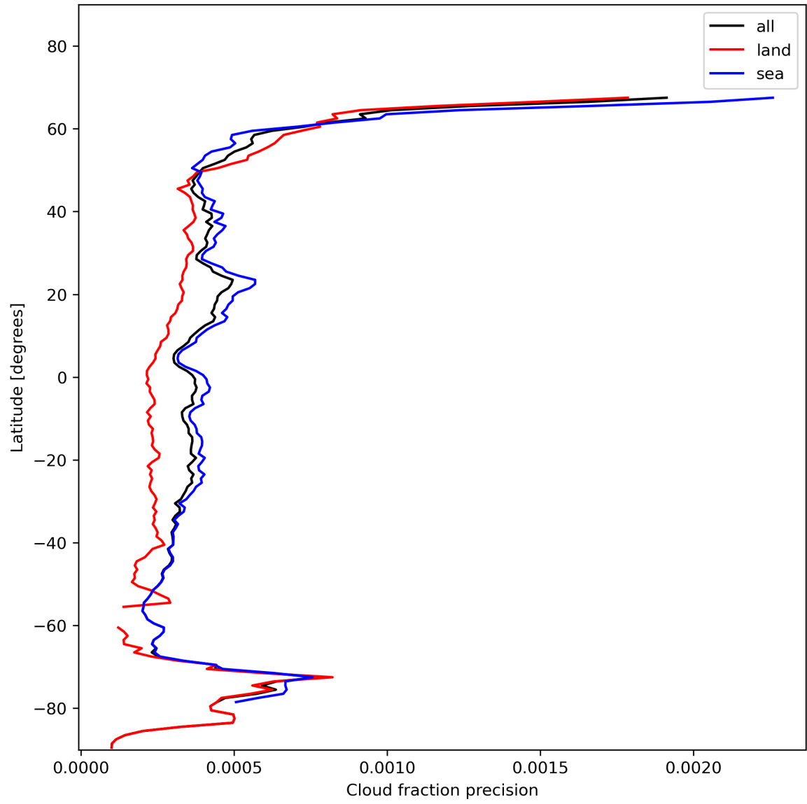
Figure 16: Zonal average of “Cloud fraction precision” for 2023-11-21 to 2023-11-23.
