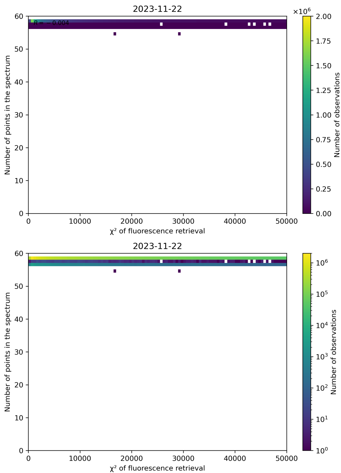
Figure 71: Scatter density plot of “ \chi^2 of fluorescence retrieval” against “Number of points in the spectrum” for 2023-11-21 to 2023-11-23.
