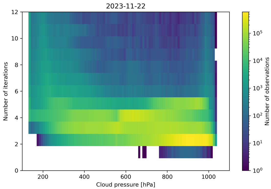
Figure 89: Scatter density plot of “Cloud pressure” against “Number of iterations” for 2023-11-21 to 2023-11-23.
