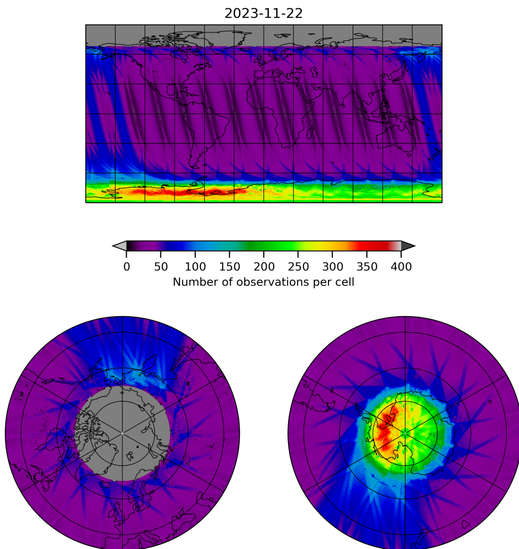
Figure 11: Map of the number of observations for 2023-11-21 to 2023-11-23
