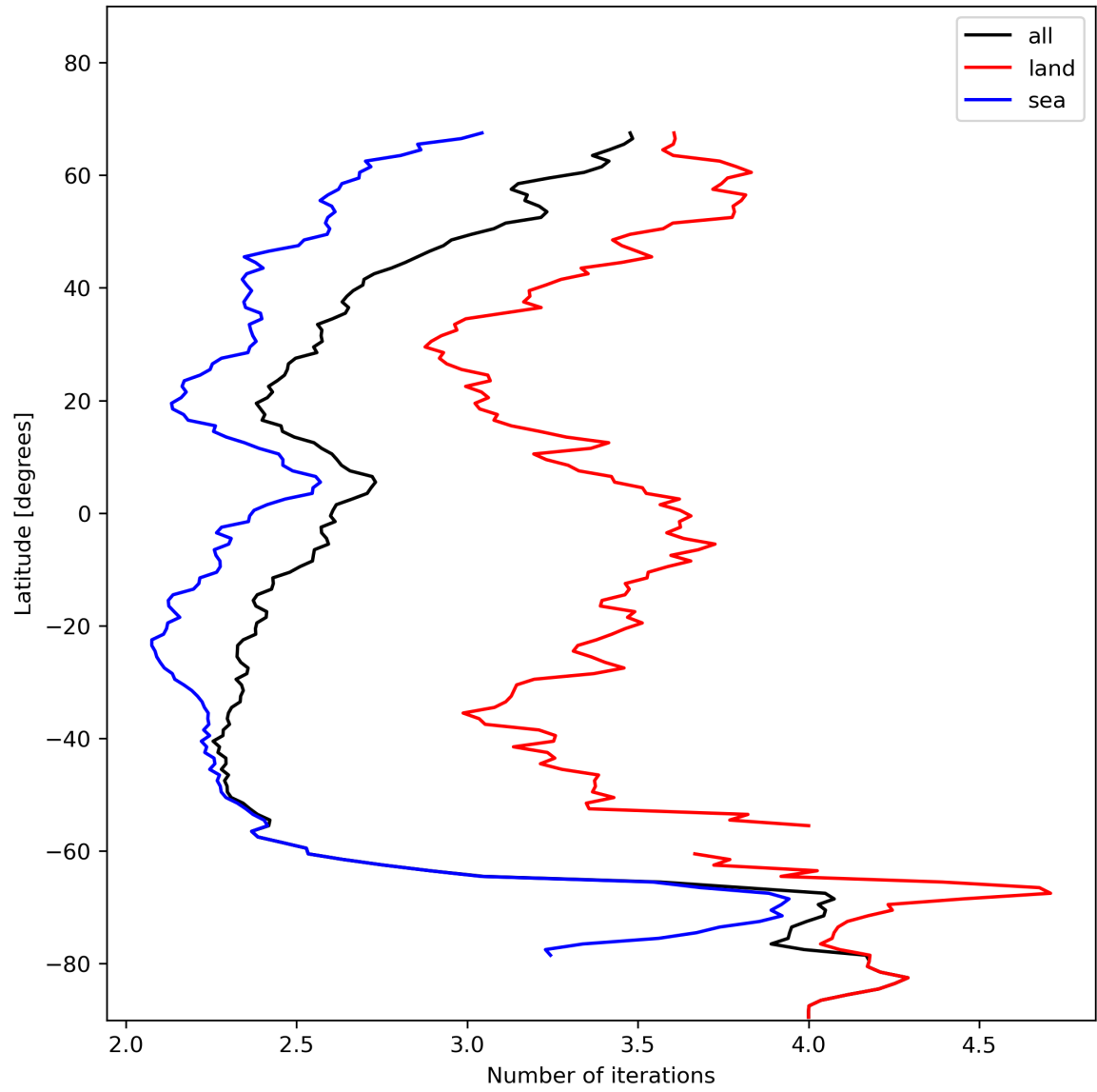
Figure 22: Zonal average of “Number of iterations” for 2023-11-21 to 2023-11-23.
