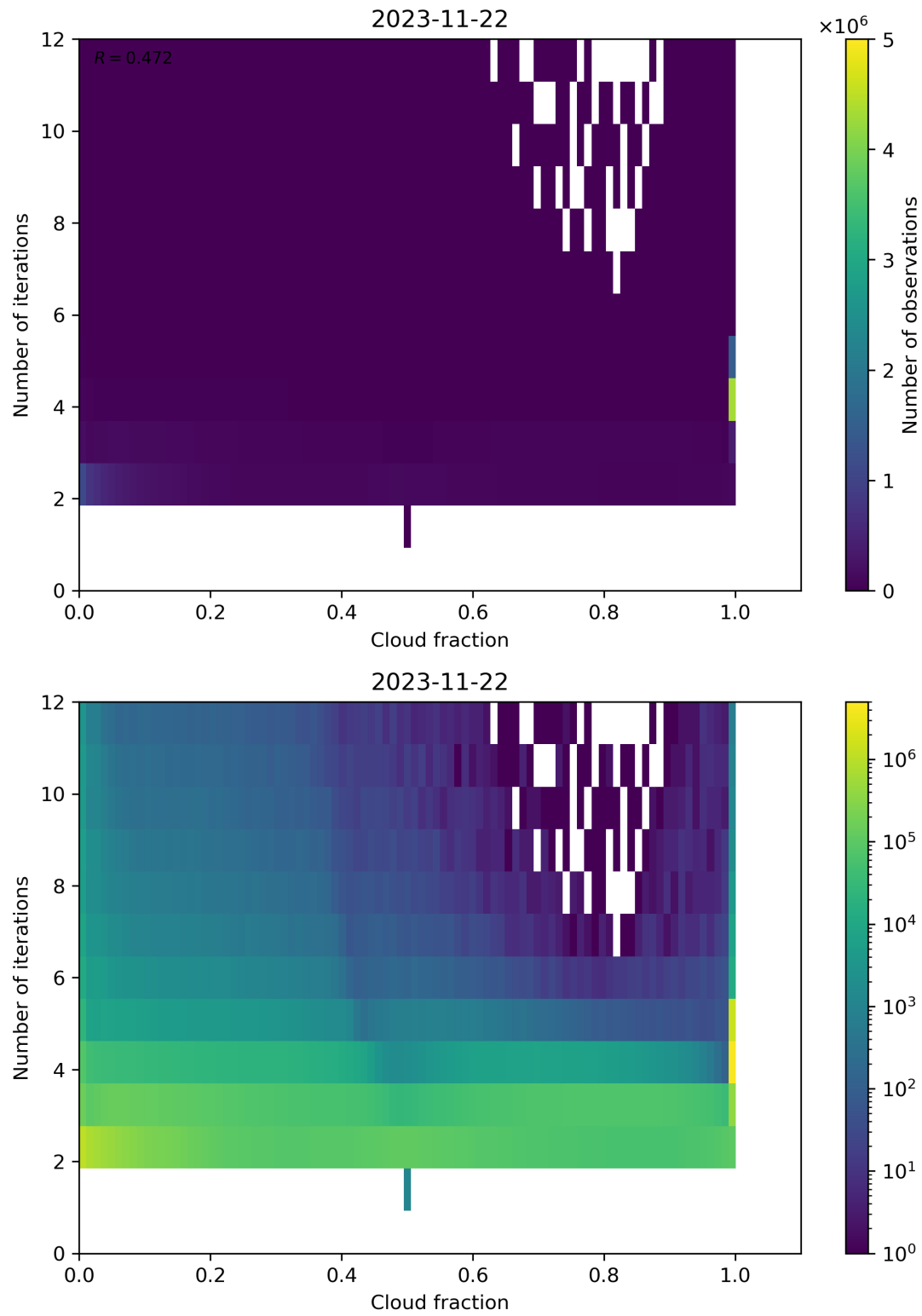
Figure 80: Scatter density plot of “Cloud fraction” against “Number of iterations” for 2023-11-21 to 2023-11-23.
