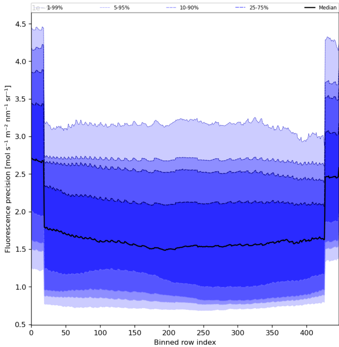
Figure 58: Along track statistics of “Fluorescence precision” for 2023-11-21 to 2023-11-23
