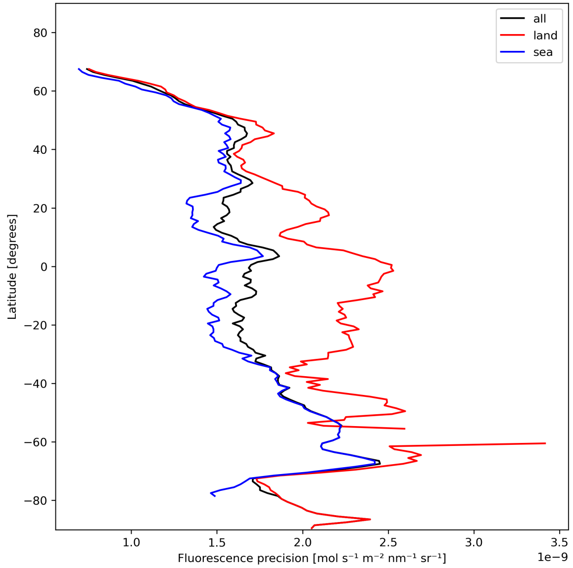
Figure 24: Zonal average of “Fluorescence precision” for 2023-11-21 to 2023-11-23.
