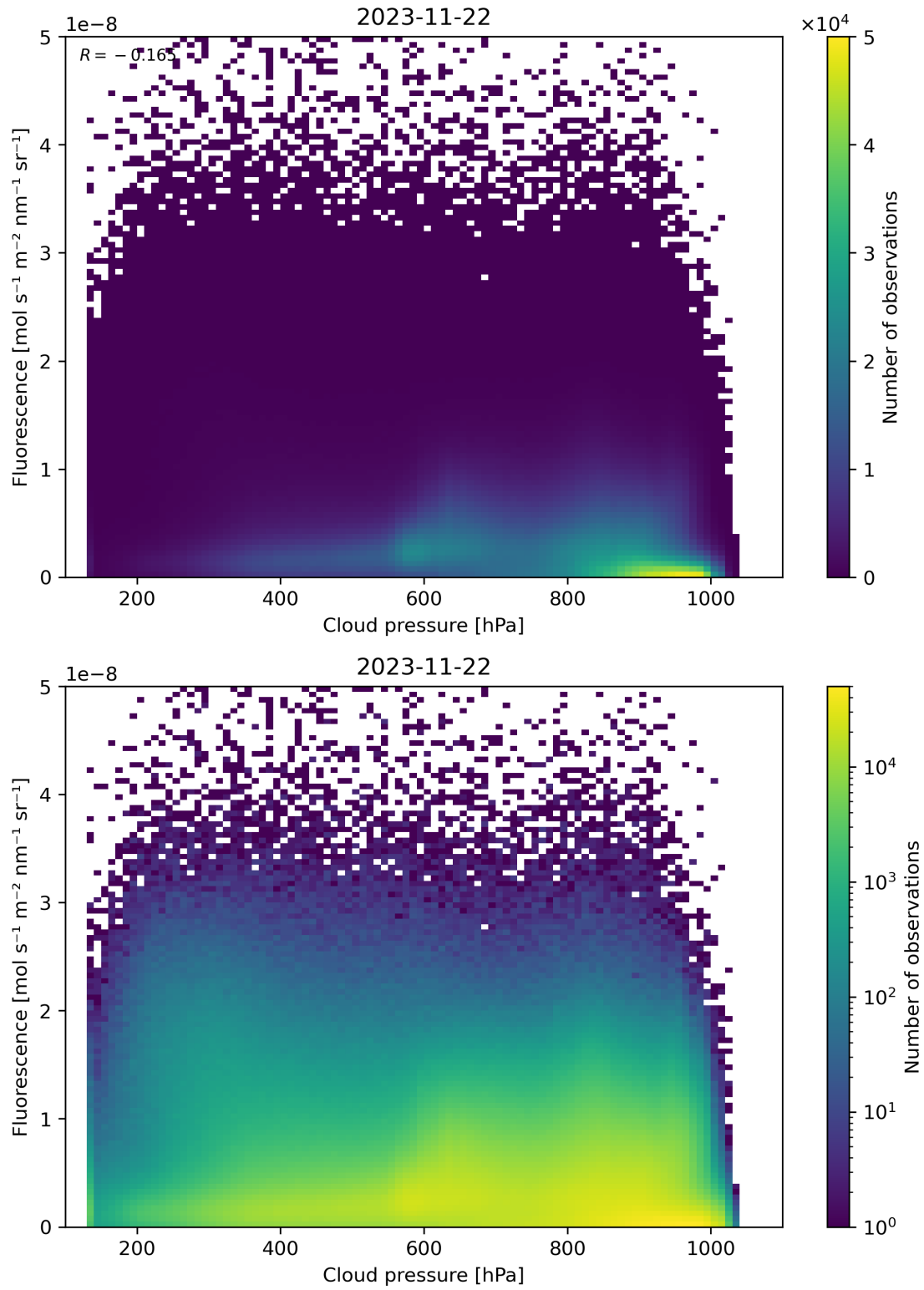
Figure 88: Scatter density plot of “Cloud pressure” against “Fluorescence” for 2023-11-21 to 2023-11-23.
