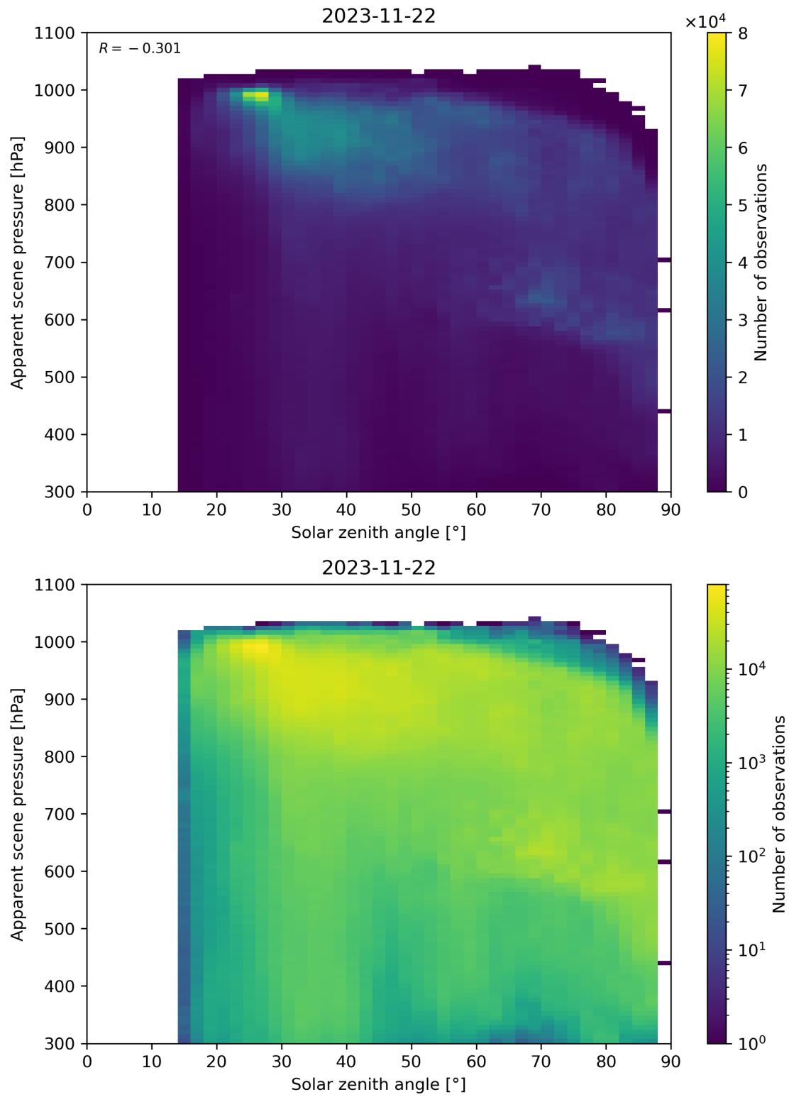
Figure 118: Scatter density plot of “Solar zenith angle” against “Apparent scene pressure” for 2023-11-21 to 2023-11-23.
