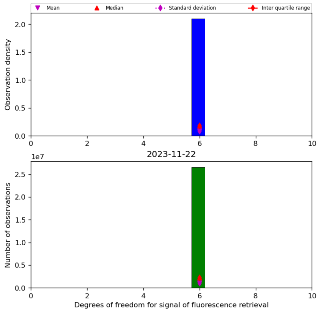
Figure 43: Histogram of “Degrees of freedom for signal of fluorescence retrieval” for 2023-11-21 to 2023-11-23
