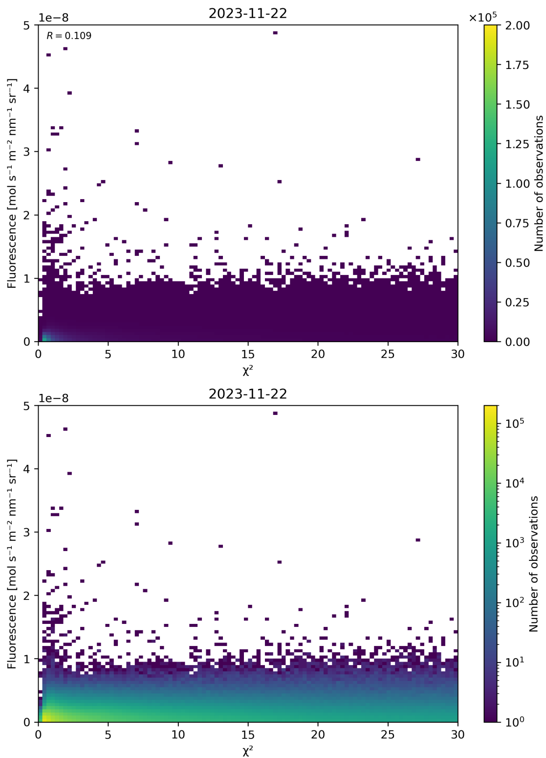
Figure 70: Scatter density plot of “ \chi^2 ” against “Fluorescence” for 2023-11-21 to 2023-11-23.
