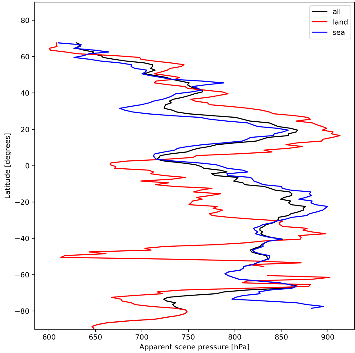
Figure 19: Zonal average of “Apparent scene pressure” for 2023-11-21 to 2023-11-23.
