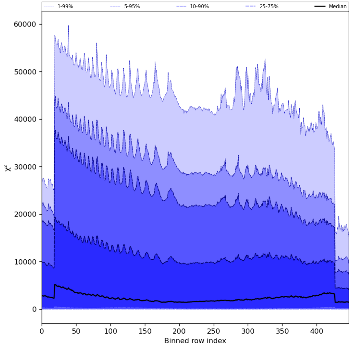
Figure 55: Along track statistics of “ \chi^2 ” for 2023-11-21 to 2023-11-23
