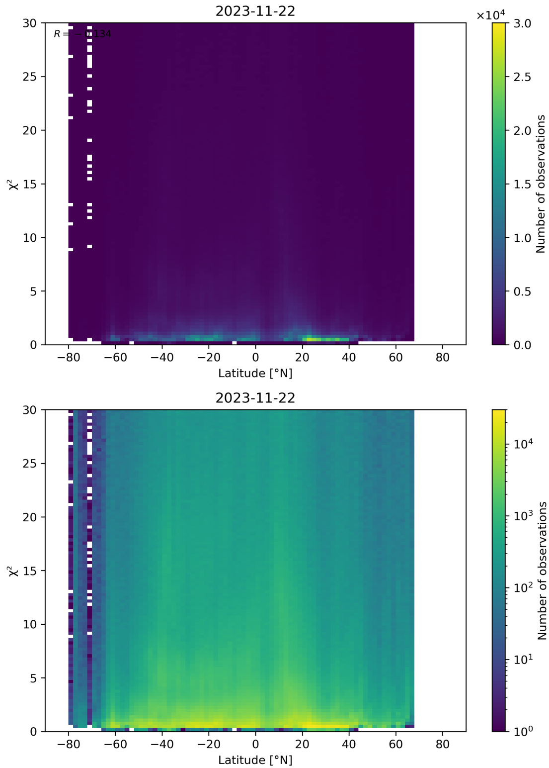
Figure 97: Scatter density plot of “Latitude” against “ \chi^2 ” for 2023-11-21 to 2023-11-23.
