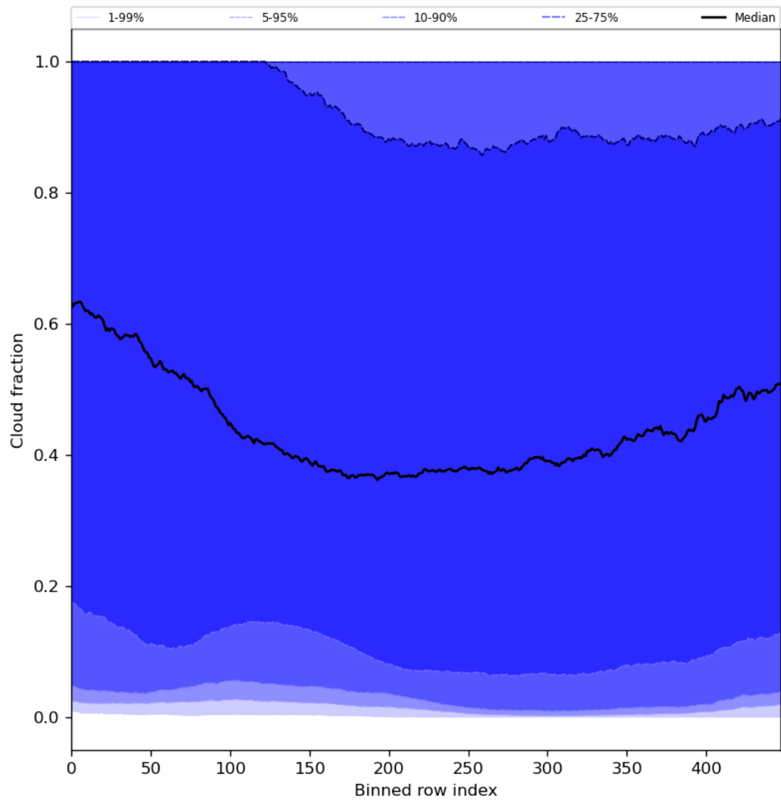
Figure 49: Along track statistics of “Cloud fraction” for 2023-11-21 to 2023-11-23
