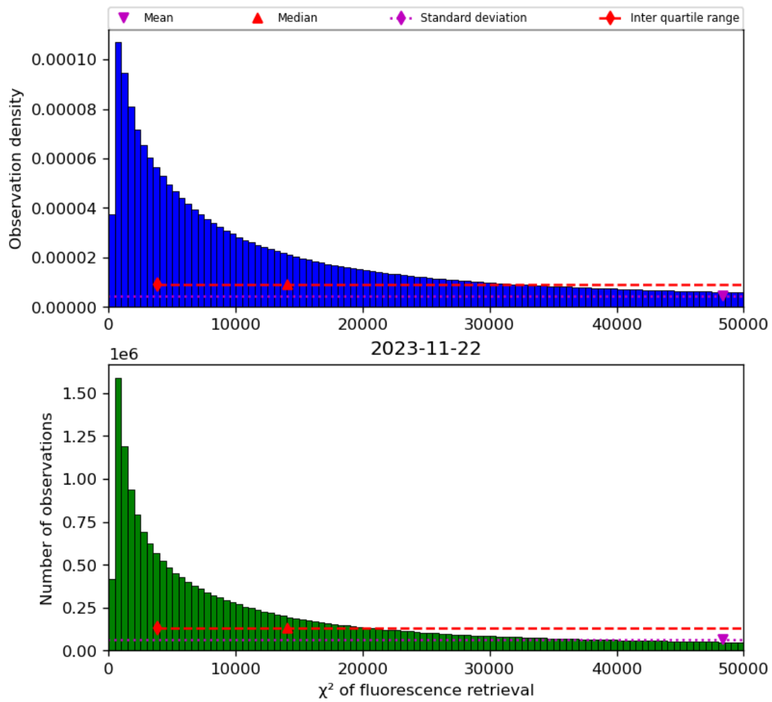
Figure 42: Histogram of “ \chi^2 of fluorescence retrieval” for 2023-11-21 to 2023-11-23
