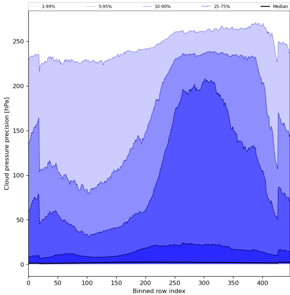
Figure 48: Along track statistics of “Cloud pressure precision” for 2023-11-21 to 2023-11-23
