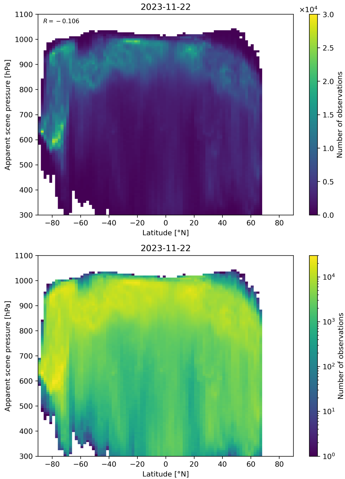
Figure 96: Scatter density plot of “Latitude” against “Apparent scene pressure” for 2023-11-21 to 2023-11-23.
