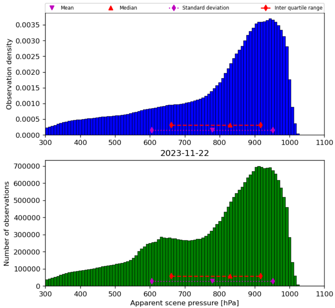
Figure 36: Histogram of “Apparent scene pressure” for 2023-11-21 to 2023-11-23
