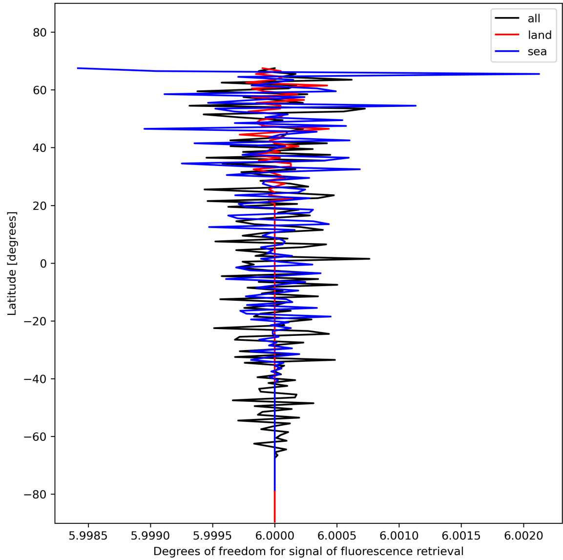
Figure 26: Zonal average of “Degrees of freedom for signal of fluorescence retrieval” for 2023-11-21 to 2023-11-23.
