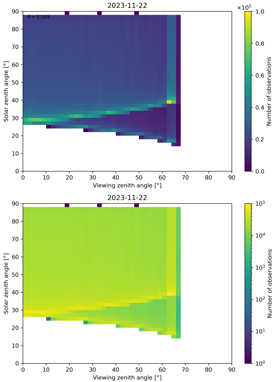
Figure 139: Scatter density plot of “Viewing zenith angle” against “Solar zenith angle” for 2023-11-21 to 2023-11-23.
