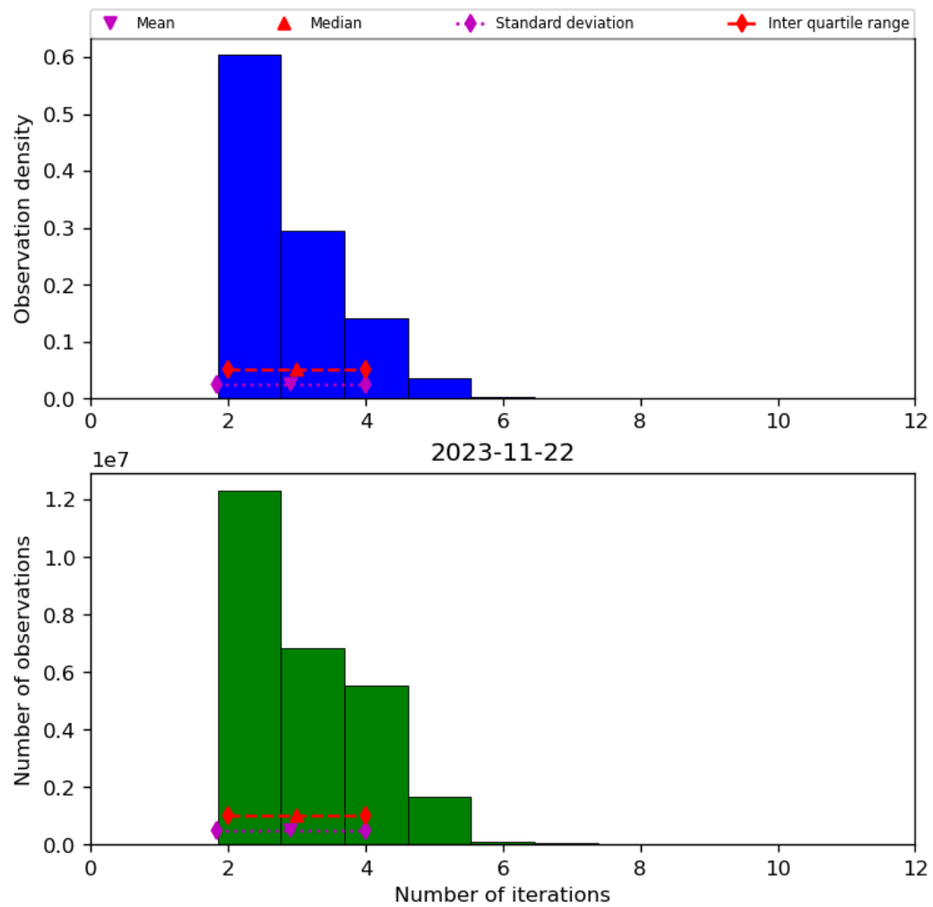
Figure 39: Histogram of “Number of iterations” for 2023-11-21 to 2023-11-23
