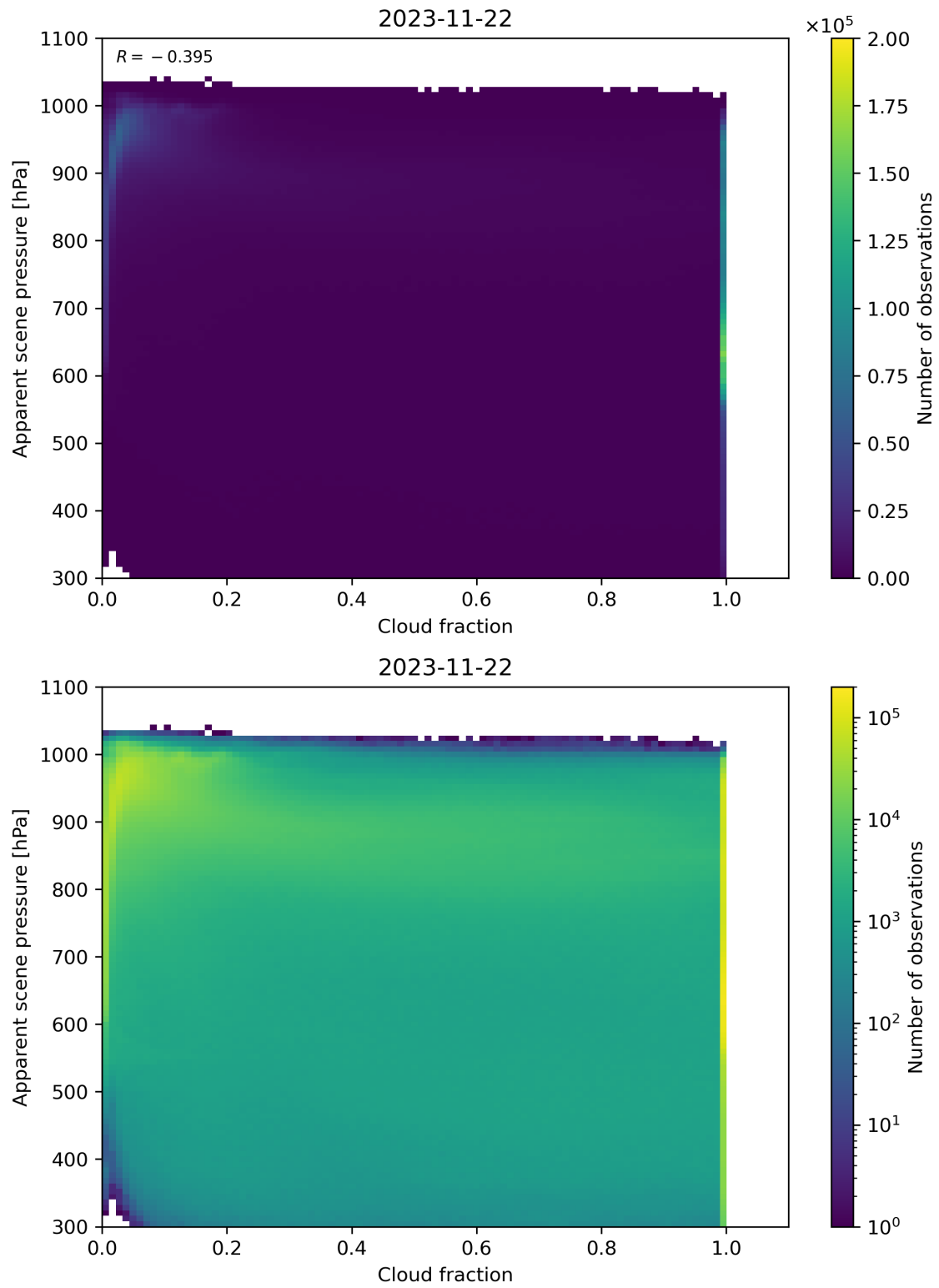
Figure 76: Scatter density plot of “Cloud fraction” against “Apparent scene pressure” for 2023-11-21 to 2023-11-23.
