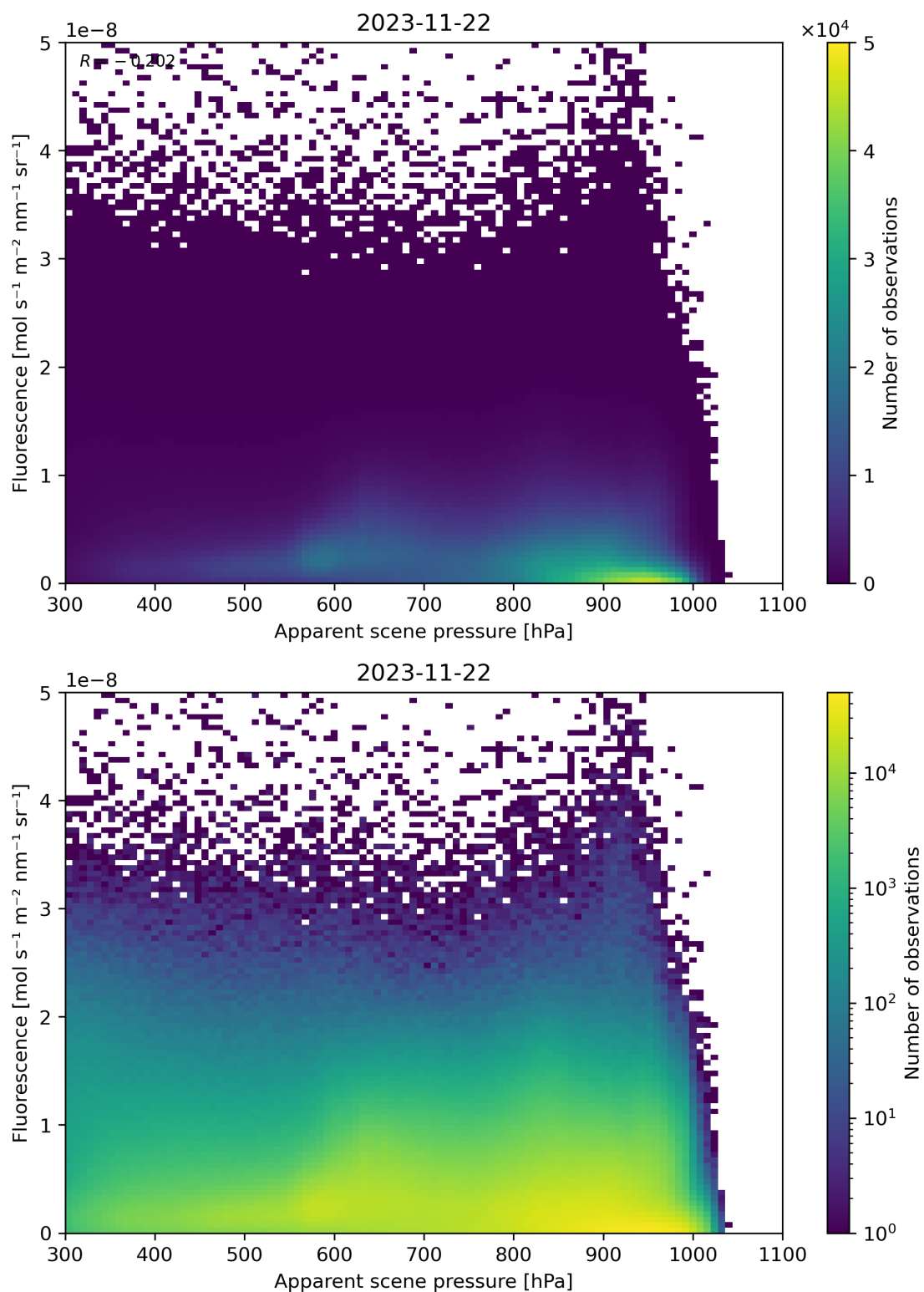
Figure 65: Scatter density plot of “Apparent scene pressure” against “Fluorescence” for 2023-11-21 to 2023-11-23.
