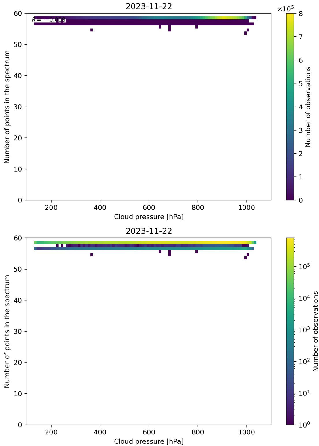
Figure 90: Scatter density plot of “Cloud pressure” against “Number of points in the spectrum” for 2023-11-21 to 2023-11-23.
