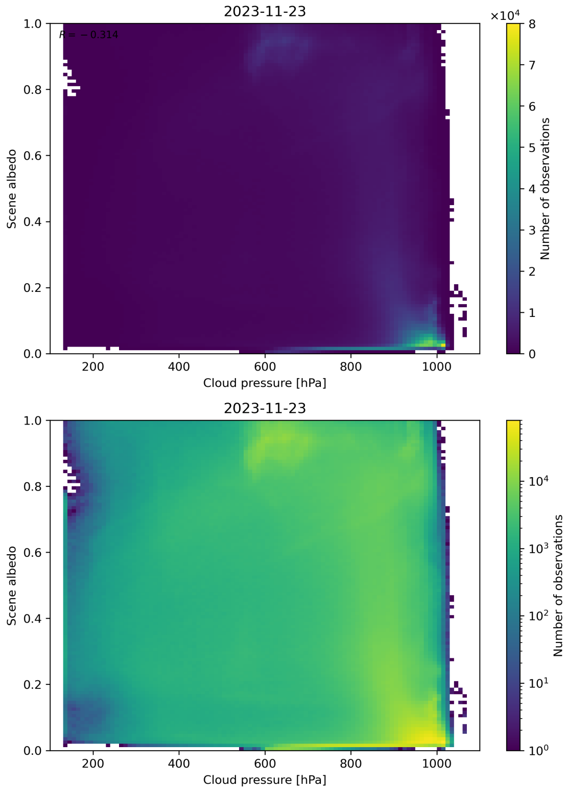
Figure 91: Scatter density plot of “Cloud pressure” against “Scene albedo” for 2023-11-23 to 2023-11-24.
