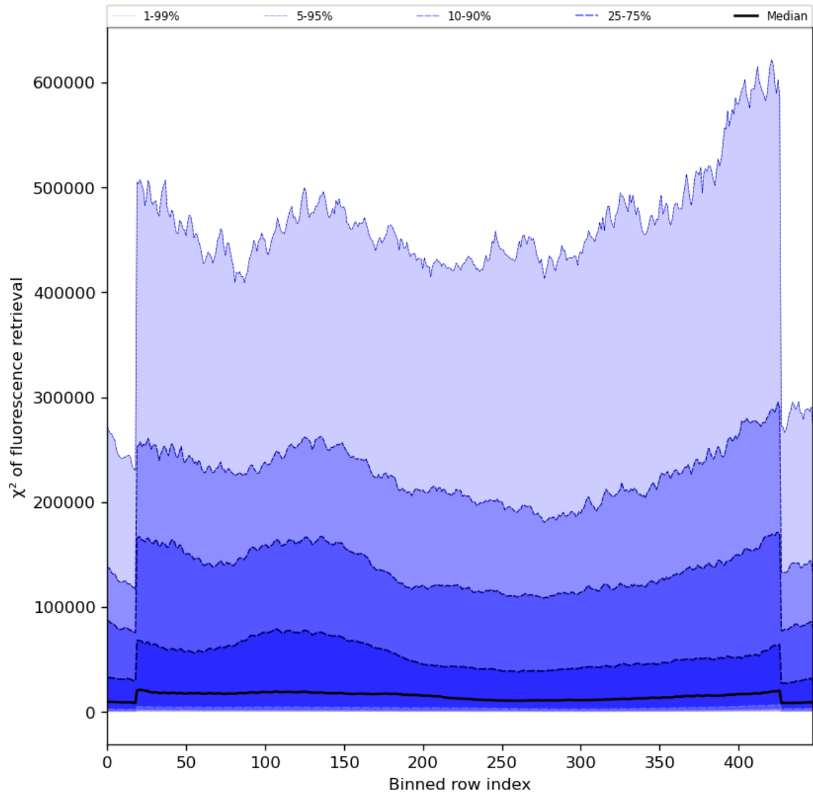
Figure 59: Along track statistics of “ \chi^2 of fluorescence retrieval” for 2023-11-23 to 2023-11-24
