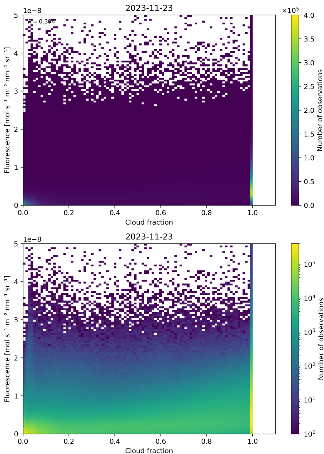
Figure 79: Scatter density plot of “Cloud fraction” against “Fluorescence” for 2023-11-23 to 2023-11-24.
