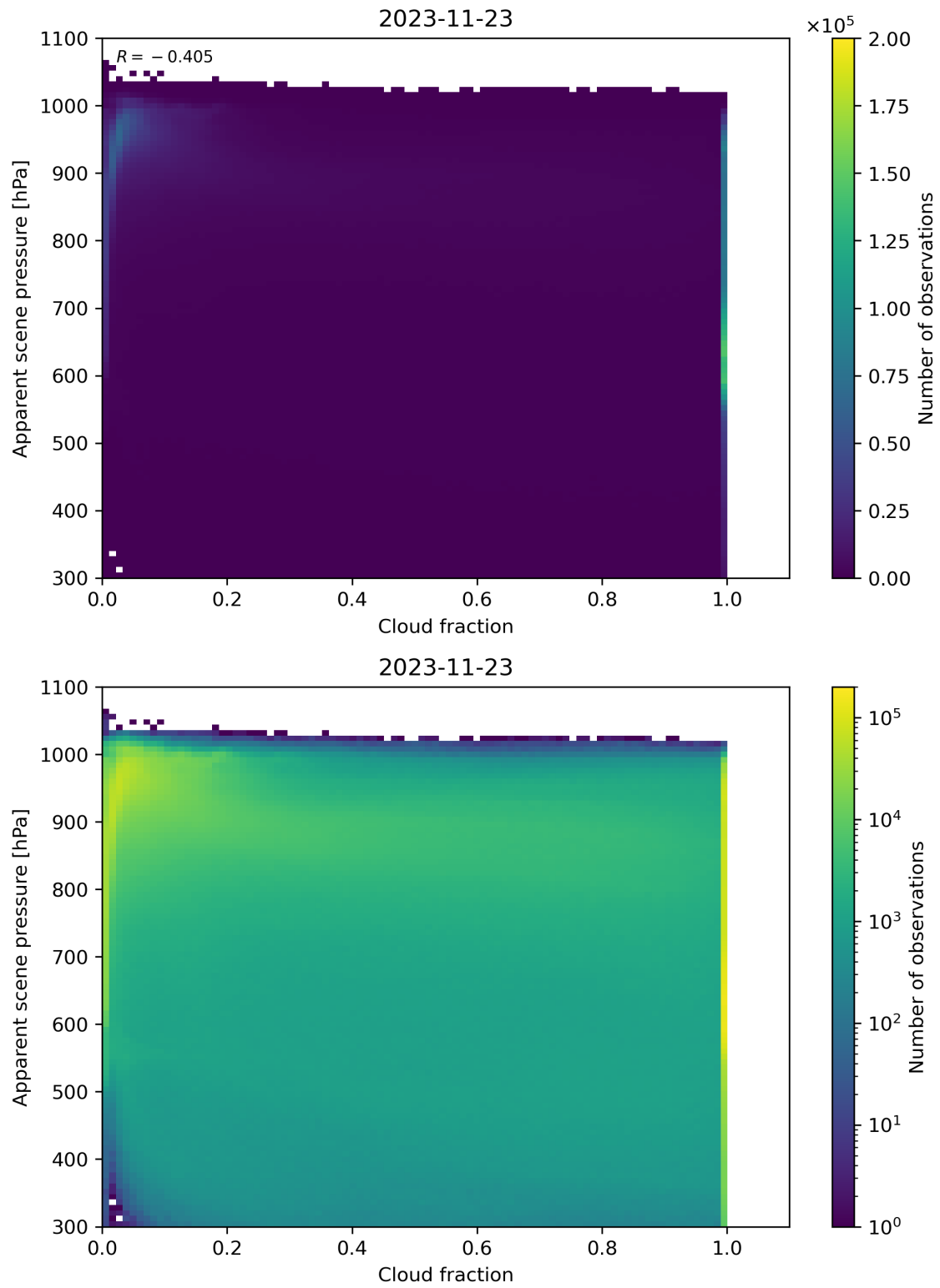
Figure 76: Scatter density plot of “Cloud fraction” against “Apparent scene pressure” for 2023-11-23 to 2023-11-24.
