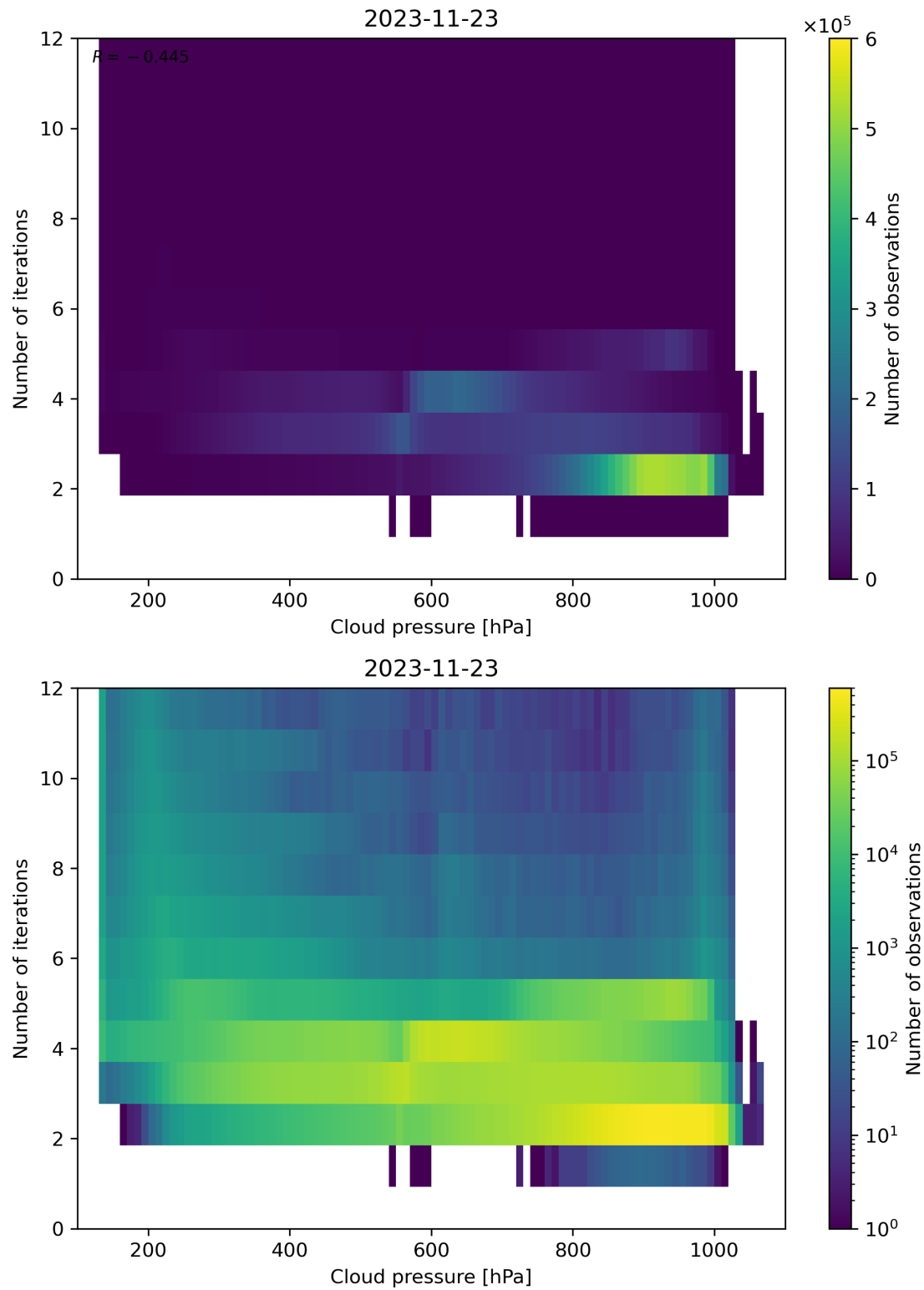
Figure 89: Scatter density plot of “Cloud pressure” against “Number of iterations” for 2023-11-23 to 2023-11-24.
