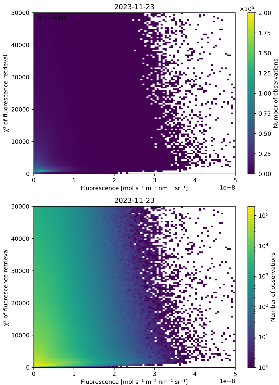
Figure 93: Scatter density plot of “Fluorescence” against “ \chi^2 of fluorescence retrieval” for 2023-11-23 to 2023-11-24.
