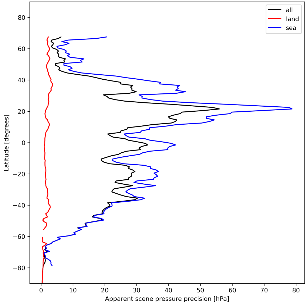
Figure 20: Zonal average of “Apparent scene pressure precision” for 2023-11-23 to 2023-11-24.
