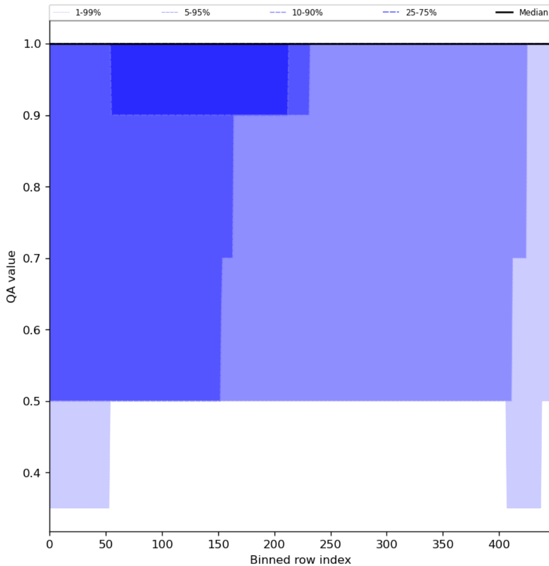
Figure 46: Along track statistics of “QA value” for 2023-11-23 to 2023-11-24
