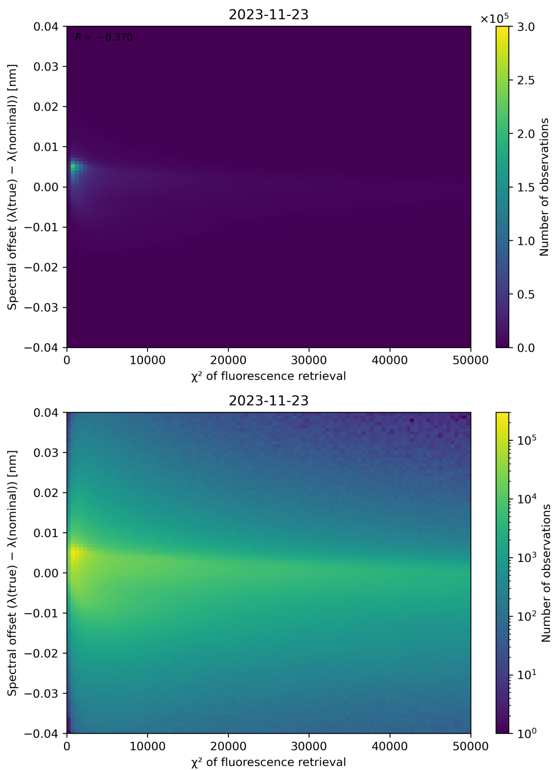
Figure 72: Scatter density plot of " \chi^2 of fluorescence retrieval" against "Spectral offset ( \lambda(\text{true}) - \lambda(\text{nominal}) )" for 2023-11-23 to 2023-11-24.
