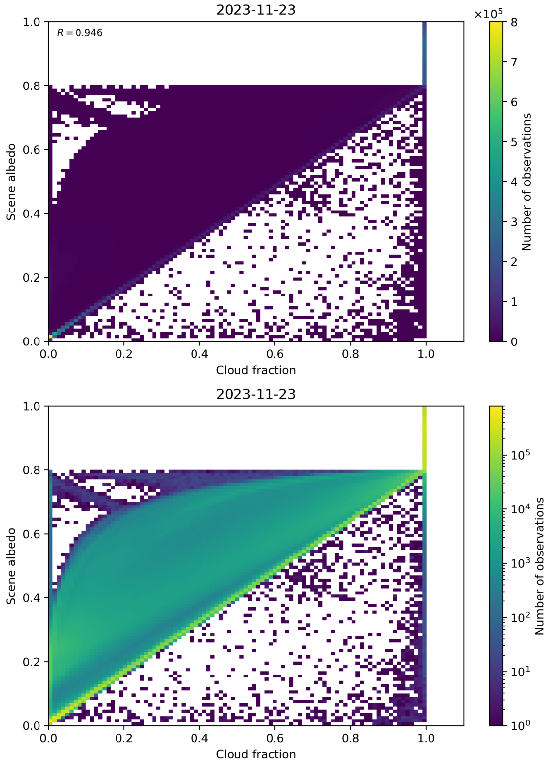
Figure 82: Scatter density plot of “Cloud fraction” against “Scene albedo” for 2023-11-23 to 2023-11-24.
