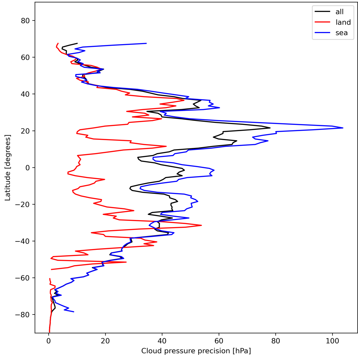
Figure 14: Zonal average of “Cloud pressure precision” for 2023-11-23 to 2023-11-24.
