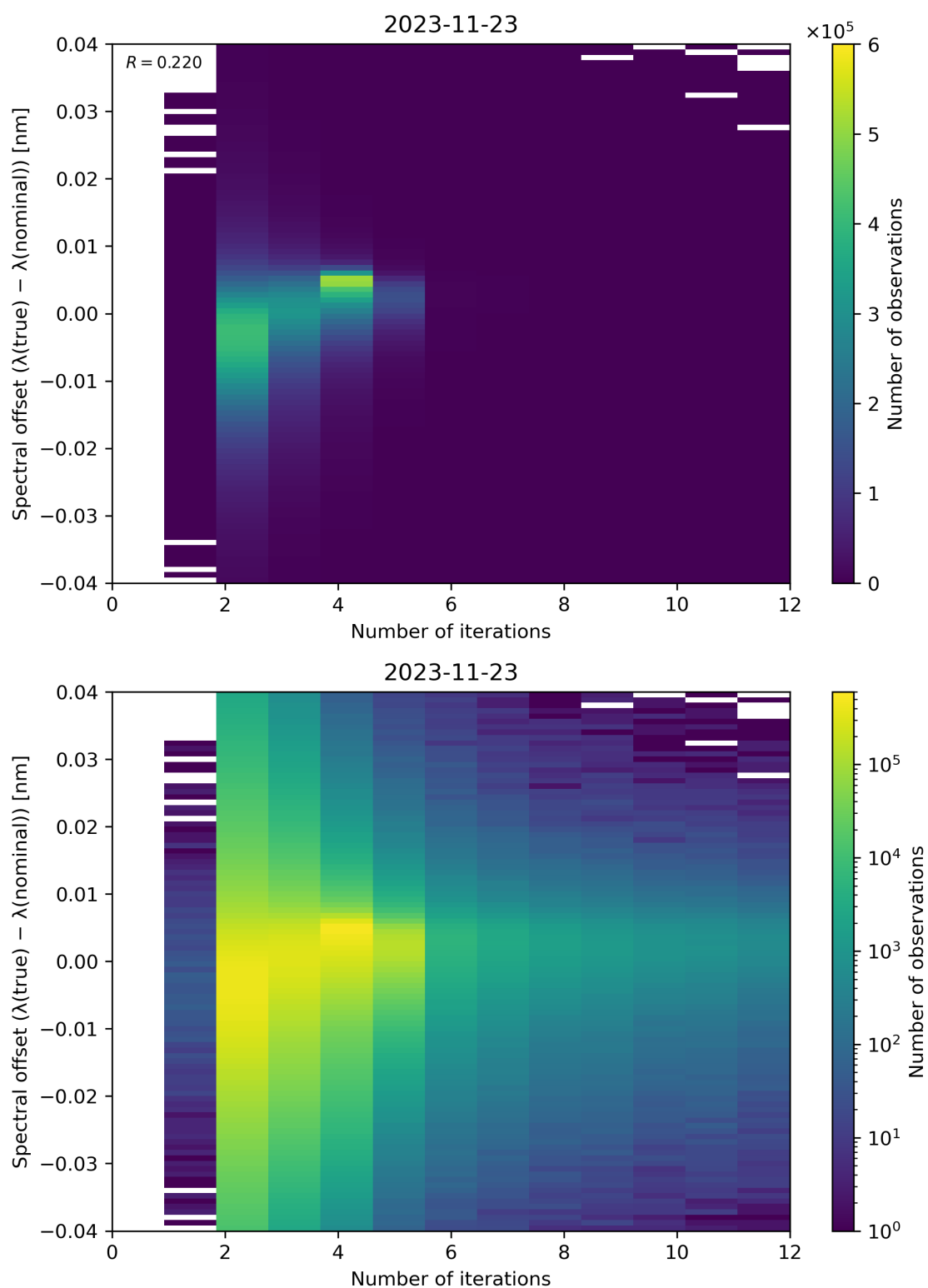
Figure 109: Scatter density plot of “Number of iterations” against “Spectral offset ( \lambda(\text{true}) - \lambda(\text{nominal}) )” for 2023-11-23 to 2023-11-24.
