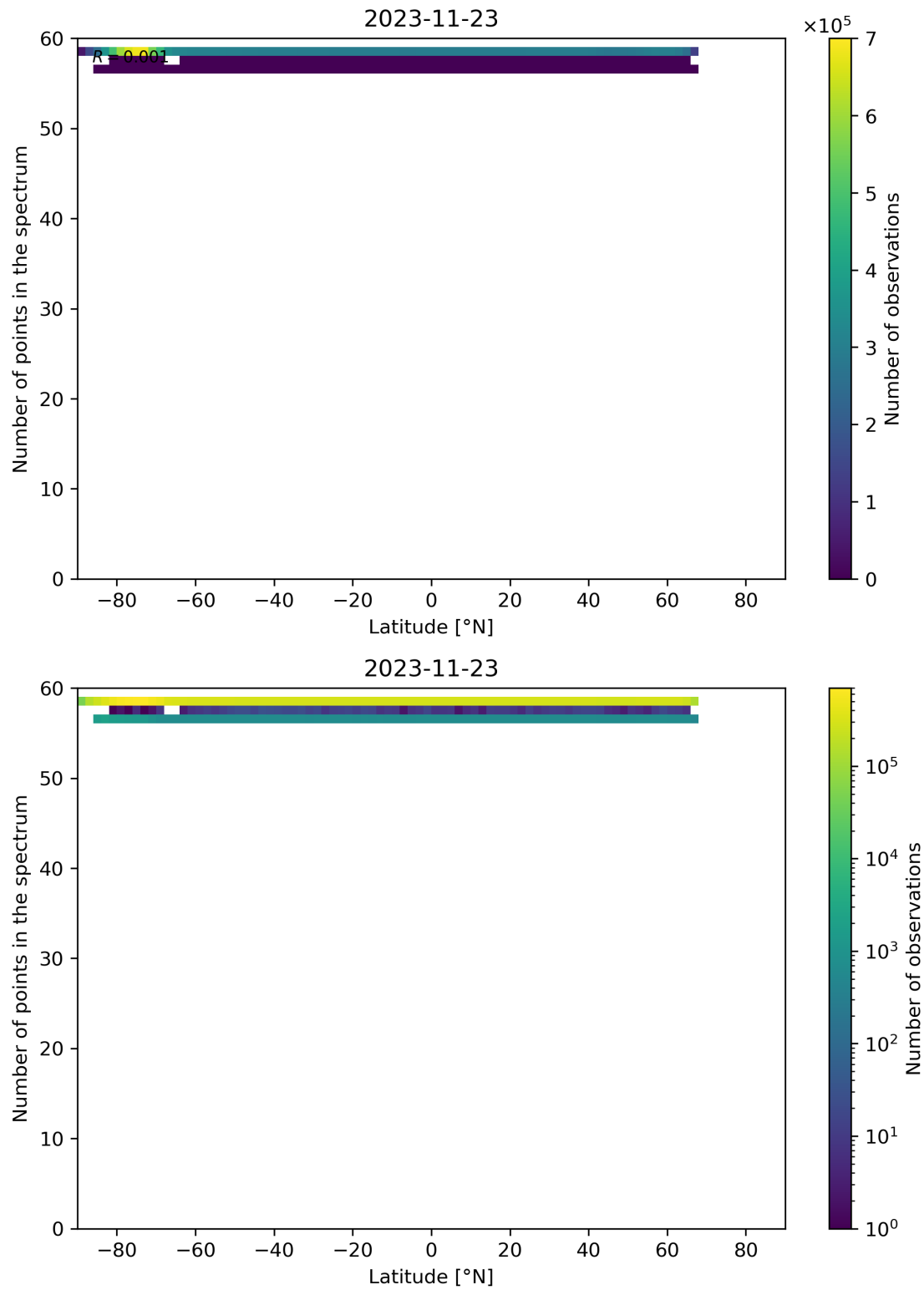
Figure 103: Scatter density plot of “Latitude” against “Number of points in the spectrum” for 2023-11-23 to 2023-11-24.
