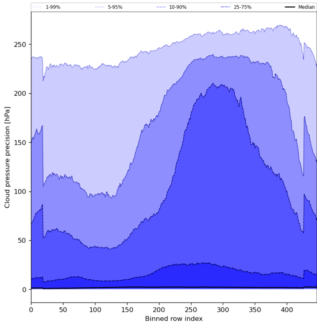
Figure 48: Along track statistics of “Cloud pressure precision” for 2023-11-23 to 2023-11-24
