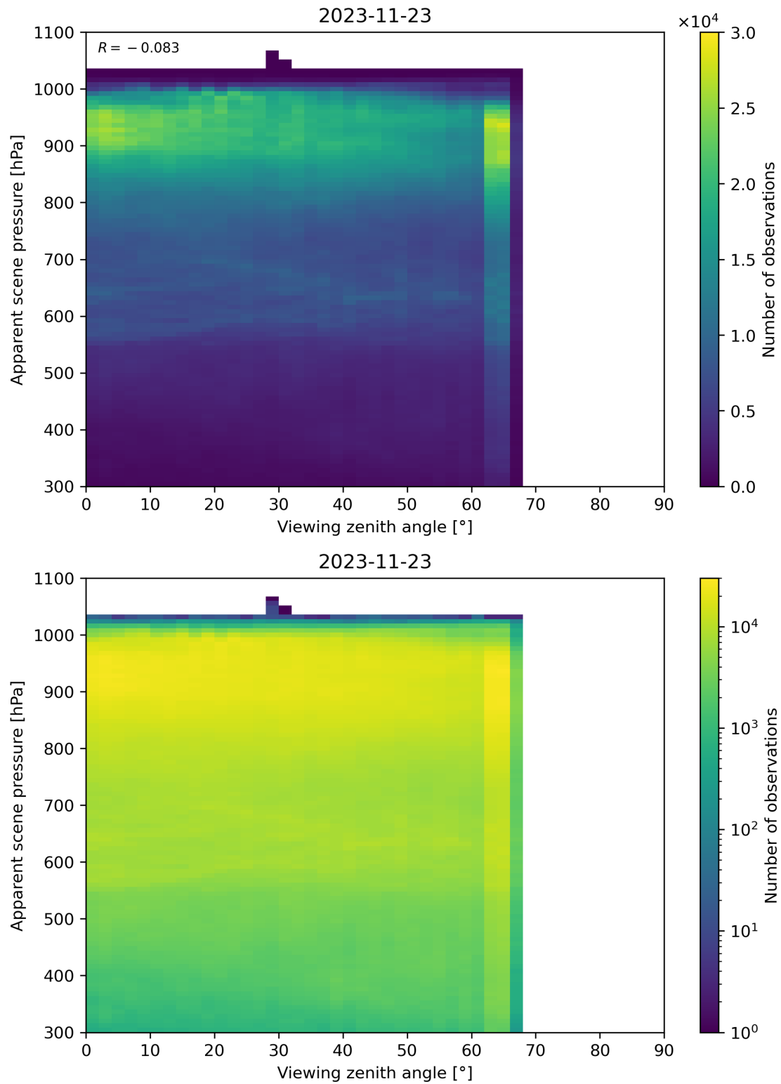
Figure 129: Scatter density plot of “Viewing zenith angle” against “Apparent scene pressure” for 2023-11-23 to 2023-11-24.
