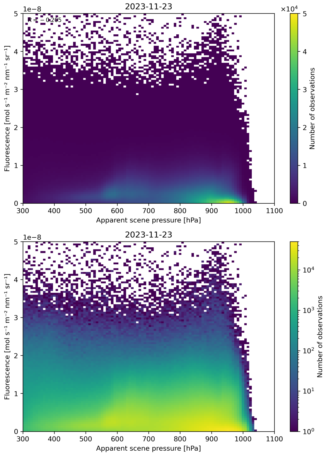
Figure 65: Scatter density plot of “Apparent scene pressure” against “Fluorescence” for 2023-11-23 to 2023-11-24.
