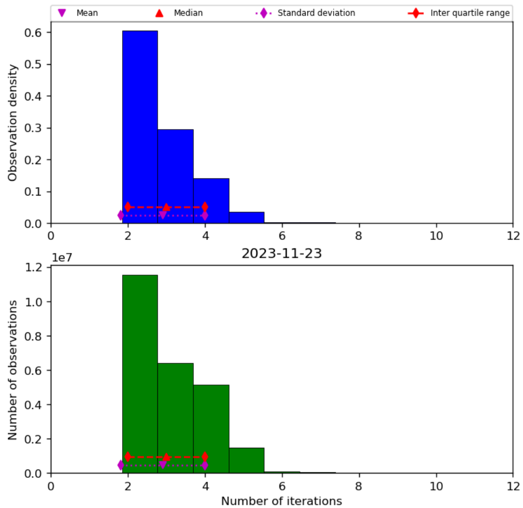
Figure 39: Histogram of “Number of iterations” for 2023-11-23 to 2023-11-24
