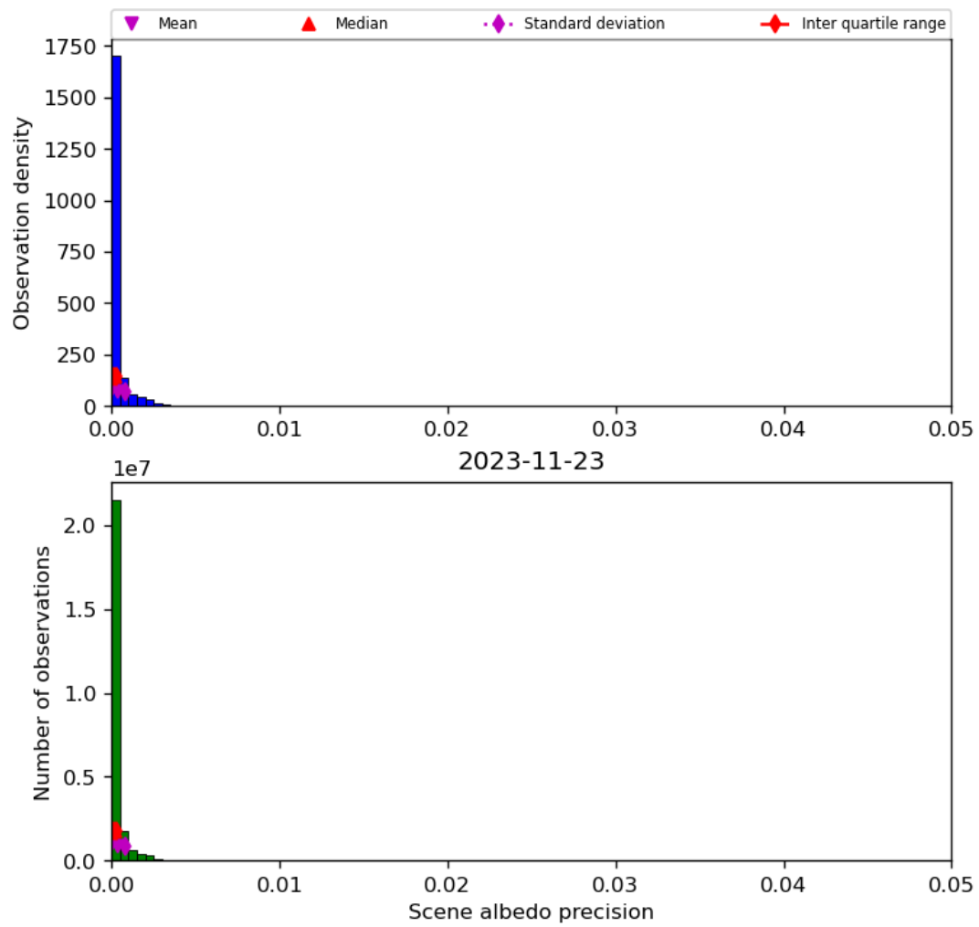
Figure 35: Histogram of “Scene albedo precision” for 2023-11-23 to 2023-11-24
