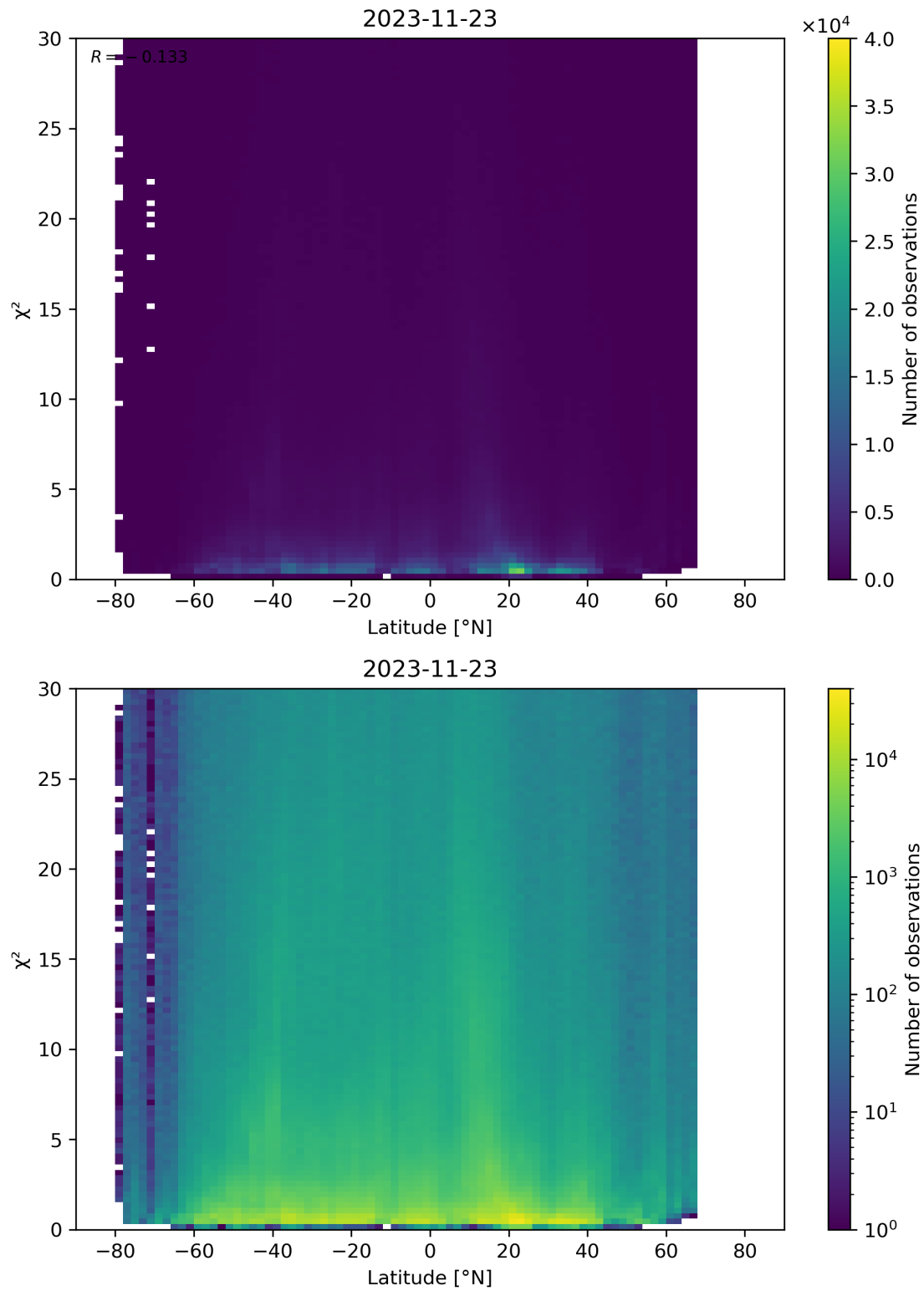
Figure 97: Scatter density plot of “Latitude” against “ \chi^2 ” for 2023-11-23 to 2023-11-24.
