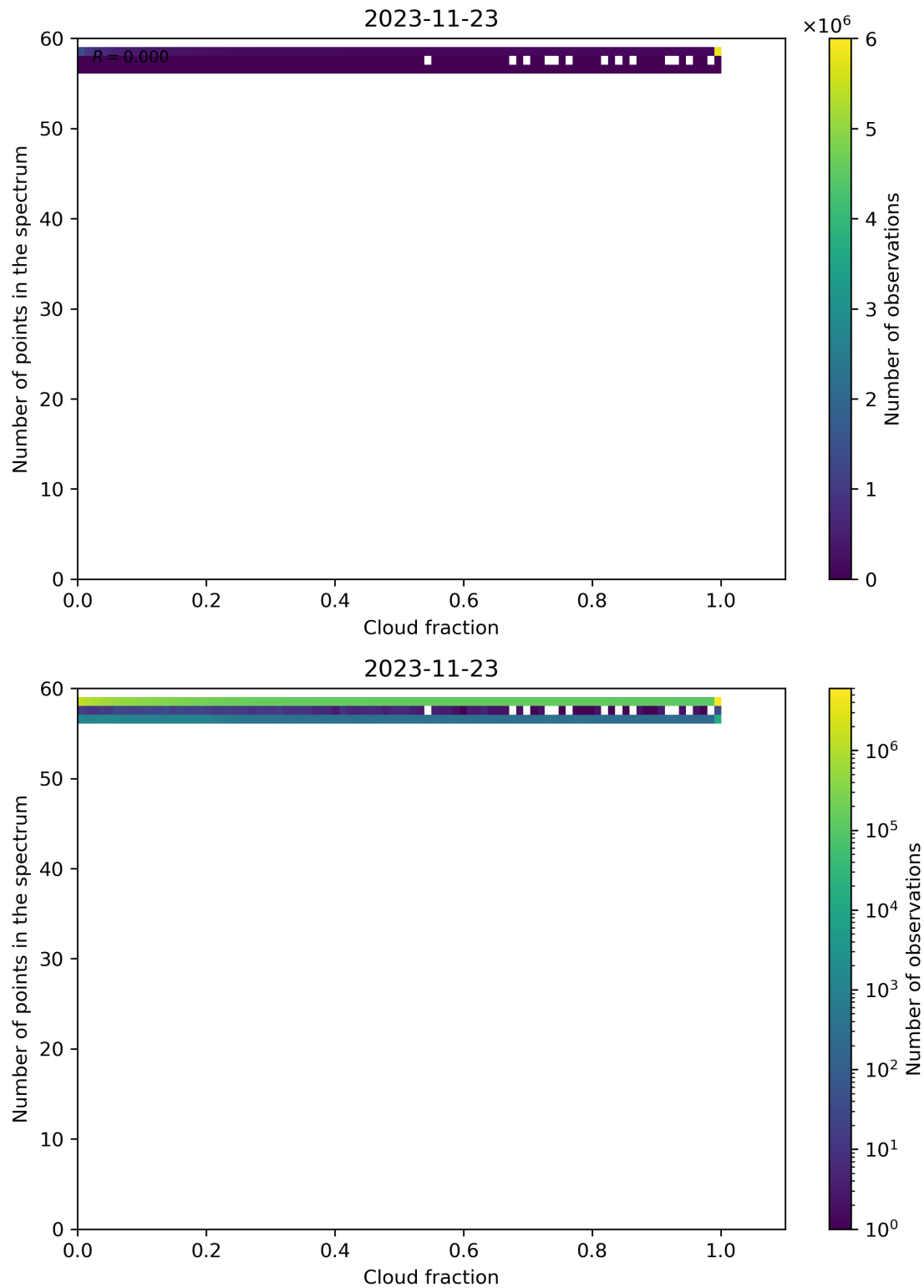
Figure 81: Scatter density plot of “Cloud fraction” against “Number of points in the spectrum” for 2023-11-23 to 2023-11-24.
