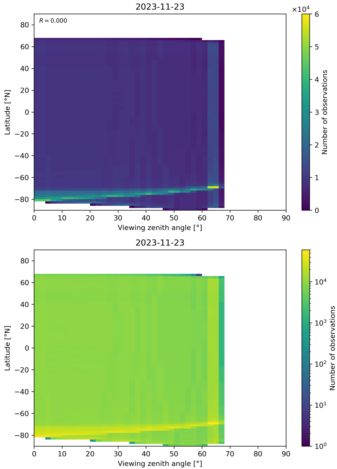
Figure 135: Scatter density plot of “Viewing zenith angle” against “Latitude” for 2023-11-23 to 2023-11-24.
