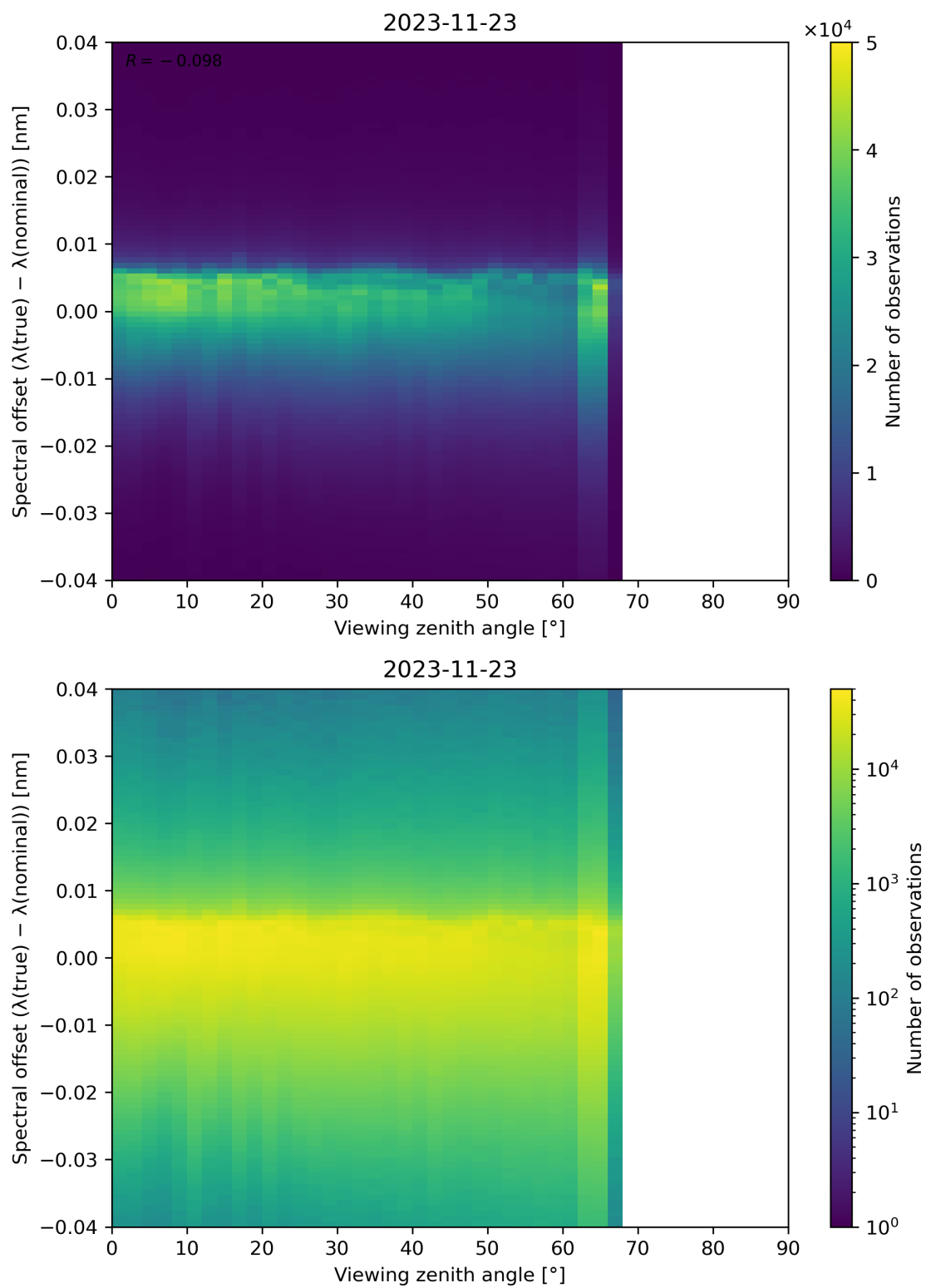
Figure 140: Scatter density plot of “Viewing zenith angle” against “Spectral offset ( \lambda(\text{true}) - \lambda(\text{nominal}) )” for 2023-11-23 to 2023-11-24.
