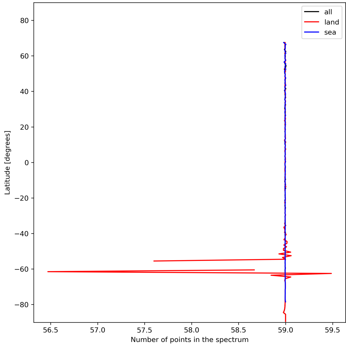
Figure 27: Zonal average of “Number of points in the spectrum” for 2023-11-23 to 2023-11-24.
