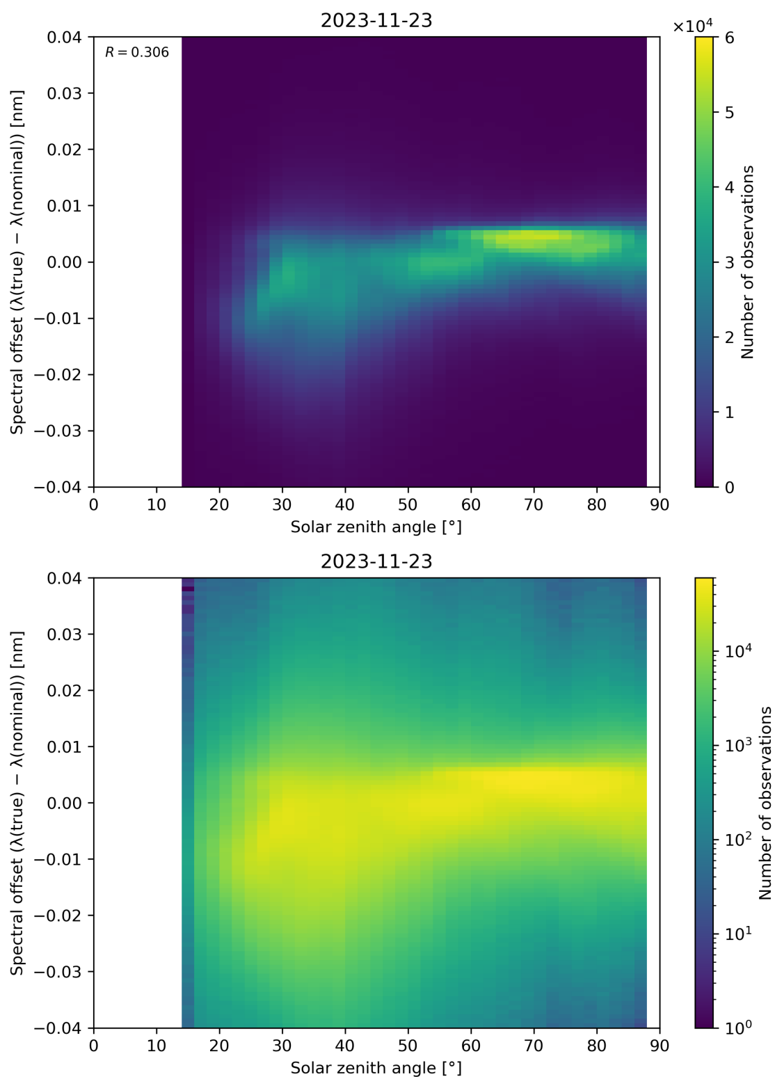
Figure 128: Scatter density plot of “Solar zenith angle” against “Spectral offset ( \lambda(\text{true}) - \lambda(\text{nominal}) )” for 2023-11-23 to 2023-11-24.
