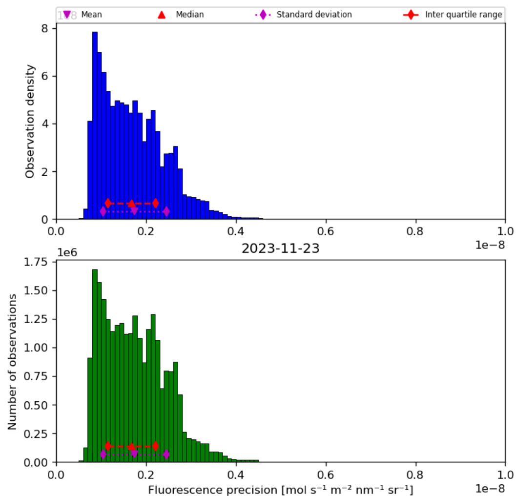
Figure 41: Histogram of “Fluorescence precision” for 2023-11-23 to 2023-11-24
