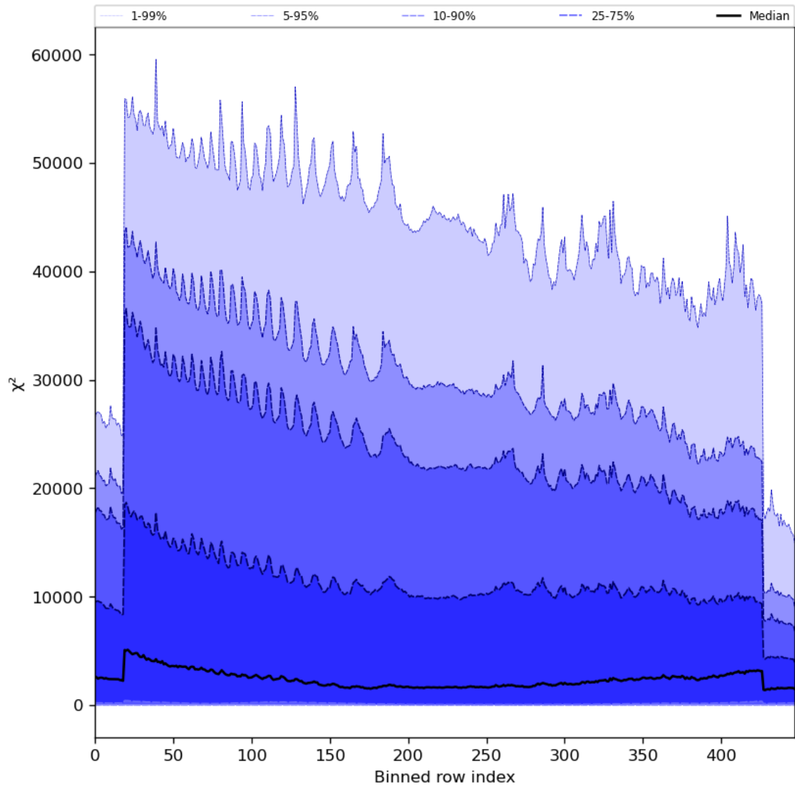
Figure 55: Along track statistics of “ \chi^2 ” for 2023-11-23 to 2023-11-24
