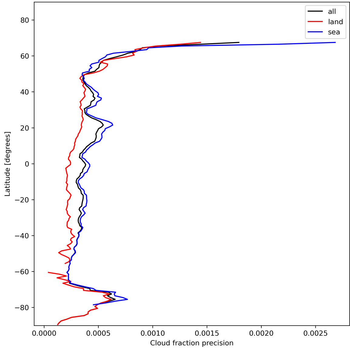
Figure 16: Zonal average of “Cloud fraction precision” for 2023-11-23 to 2023-11-24.
