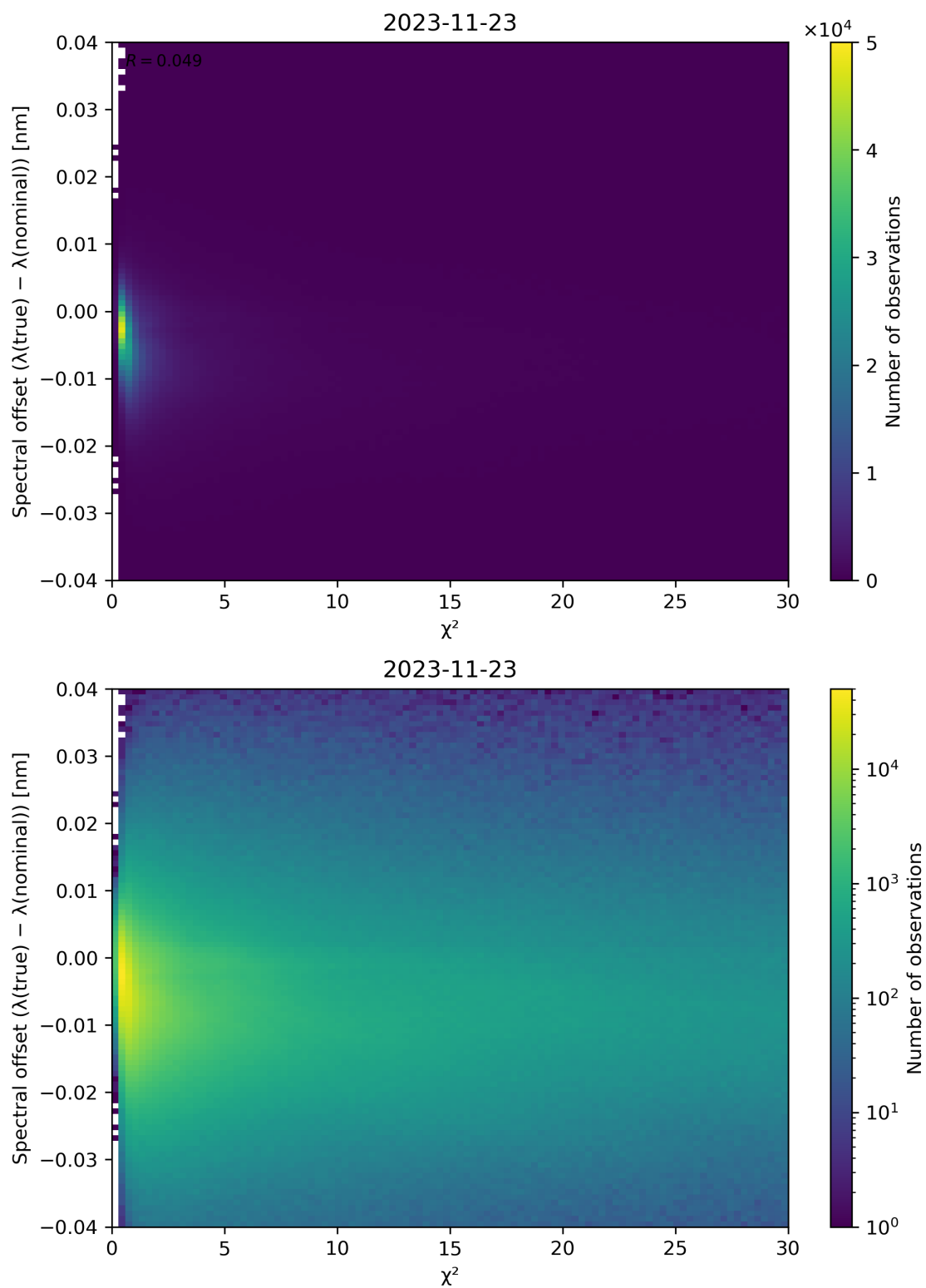
Figure 75: Scatter density plot of " \chi^2 " against "Spectral offset ( \lambda(\text{true}) - \lambda(\text{nominal}) )" for 2023-11-23 to 2023-11-24.
