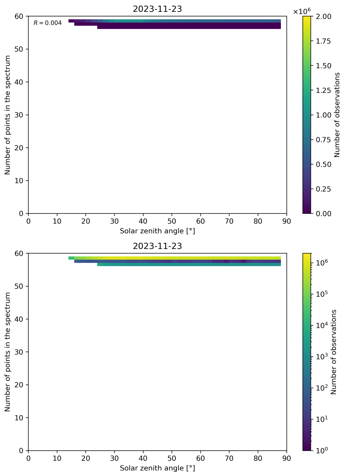
Figure 126: Scatter density plot of “Solar zenith angle” against “Number of points in the spectrum” for 2023-11-23 to 2023-11-24.
