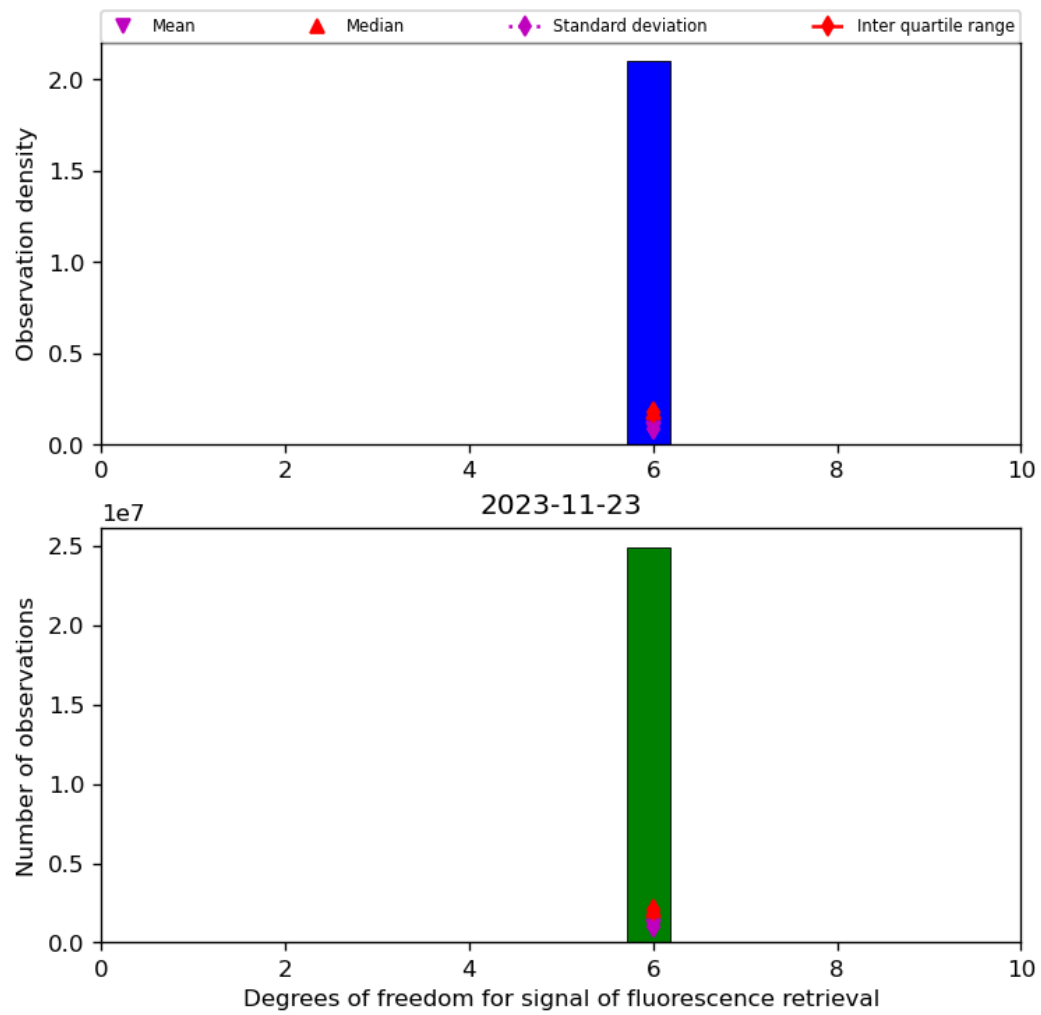
Figure 43: Histogram of “Degrees of freedom for signal of fluorescence retrieval” for 2023-11-23 to 2023-11-24
