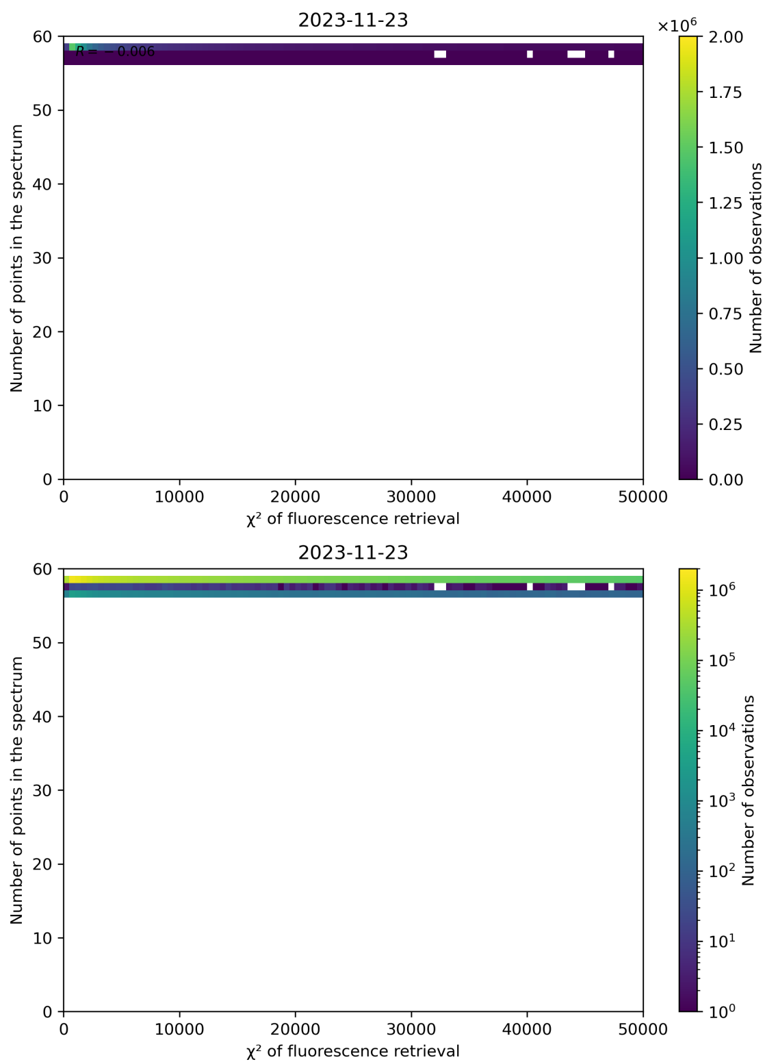
Figure 71: Scatter density plot of " \chi^2 of fluorescence retrieval" against "Number of points in the spectrum" for 2023-11-23 to 2023-11-24.
