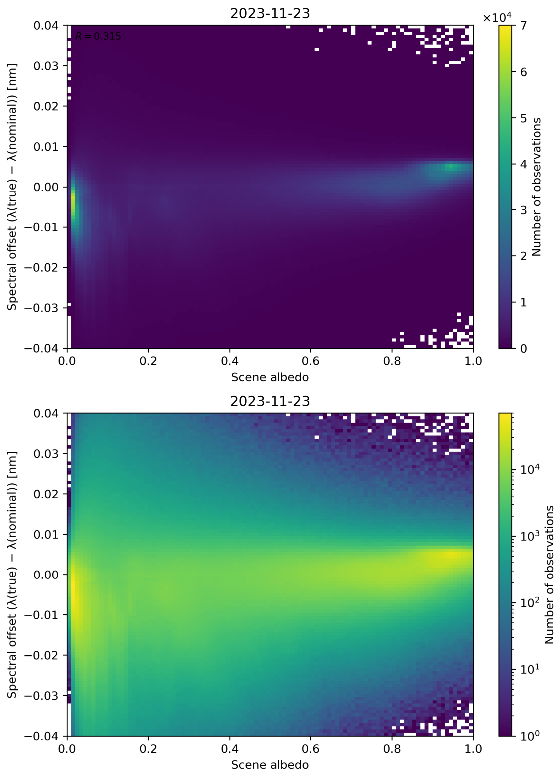
Figure 117: Scatter density plot of “Scene albedo” against “Spectral offset ( \lambda(\text{true}) - \lambda(\text{nominal}) )” for 2023-11-23 to 2023-11-24.
