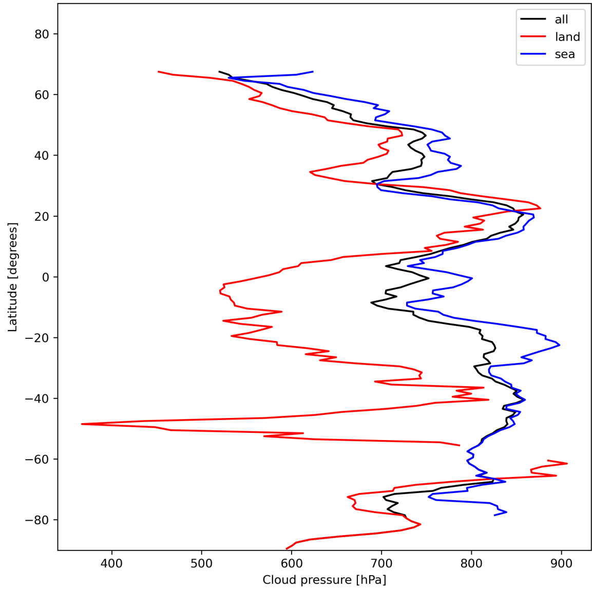
Figure 13: Zonal average of “Cloud pressure” for 2023-11-23 to 2023-11-24.
