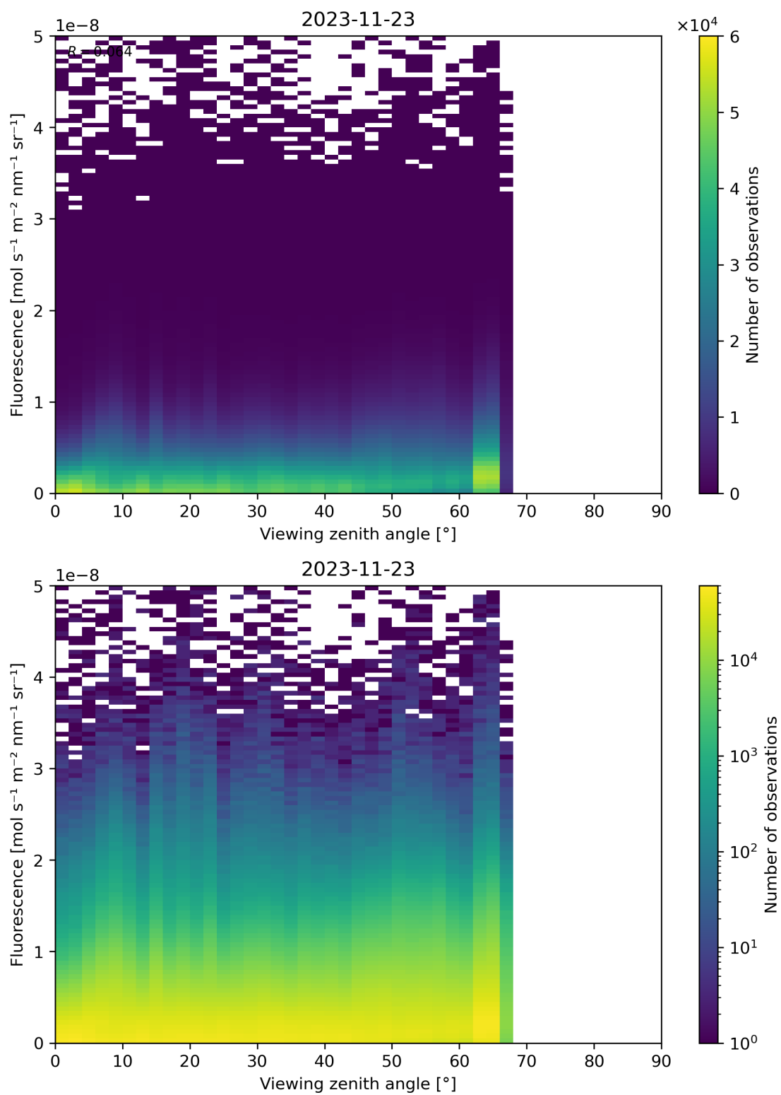
Figure 134: Scatter density plot of “Viewing zenith angle” against “Fluorescence” for 2023-11-23 to 2023-11-24.
