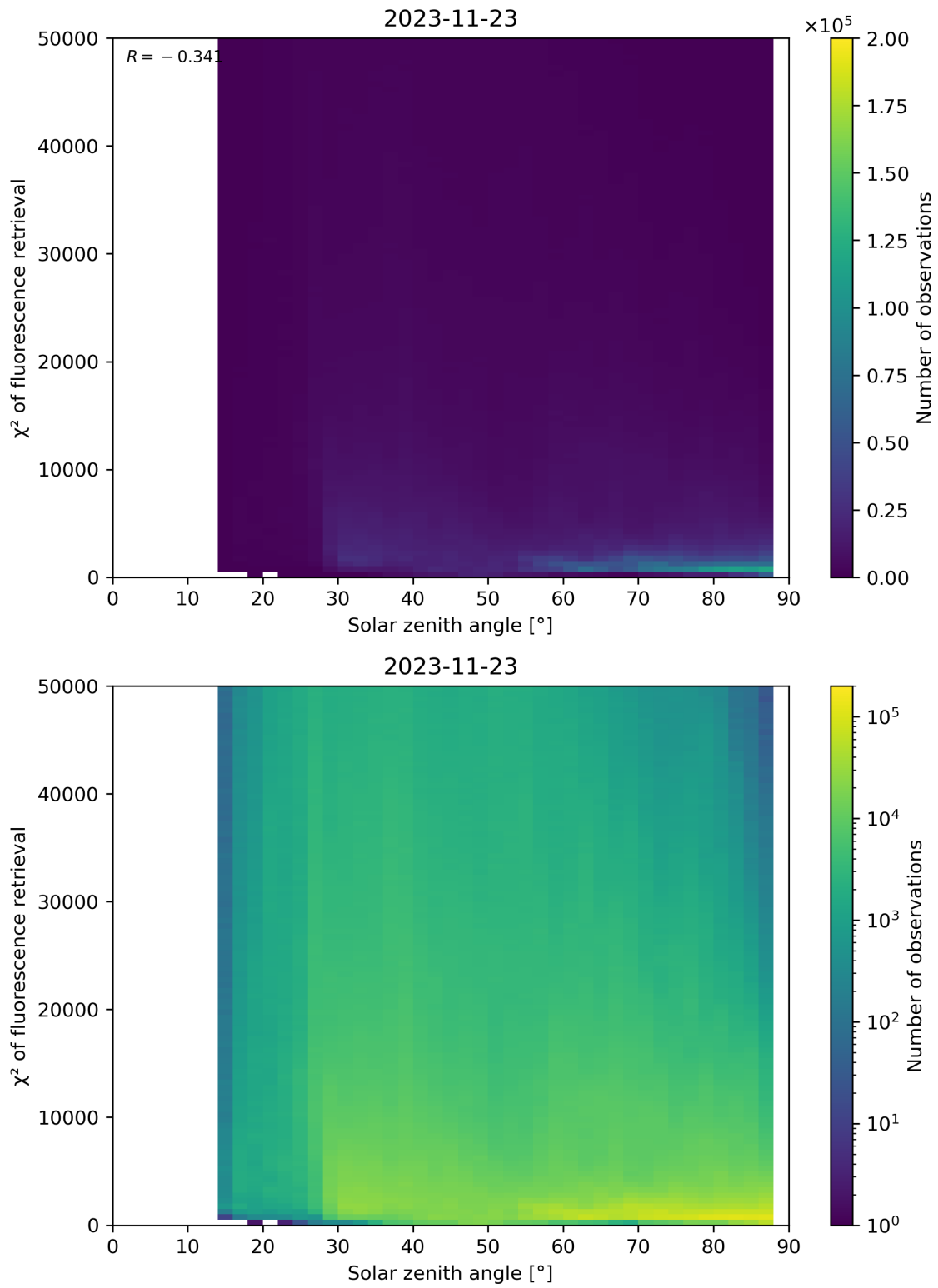
Figure 120: Scatter density plot of “Solar zenith angle” against “ \chi^2 of fluorescence retrieval” for 2023-11-23 to 2023-11-24.
