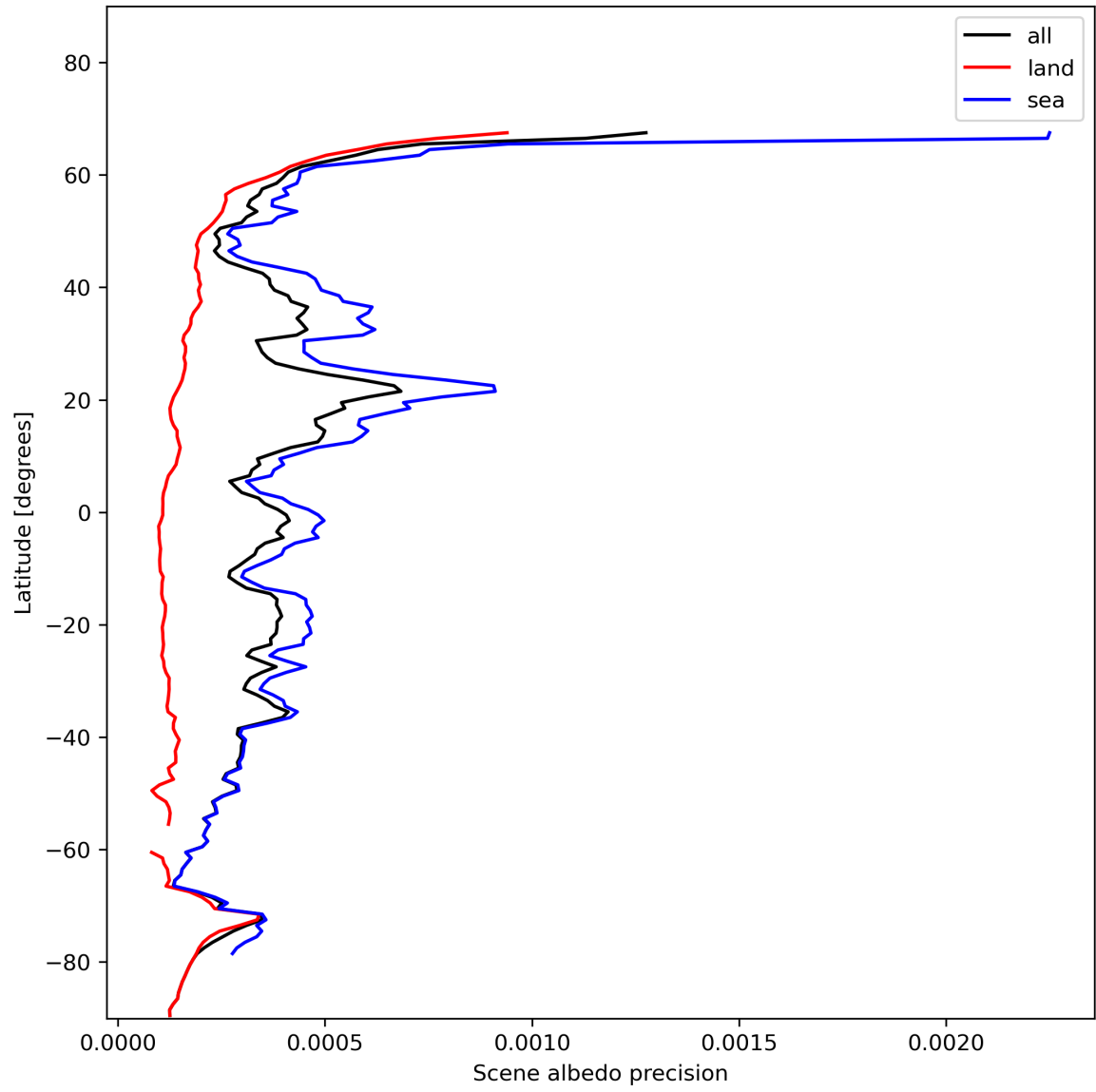
Figure 18: Zonal average of “Scene albedo precision” for 2023-11-23 to 2023-11-24.
