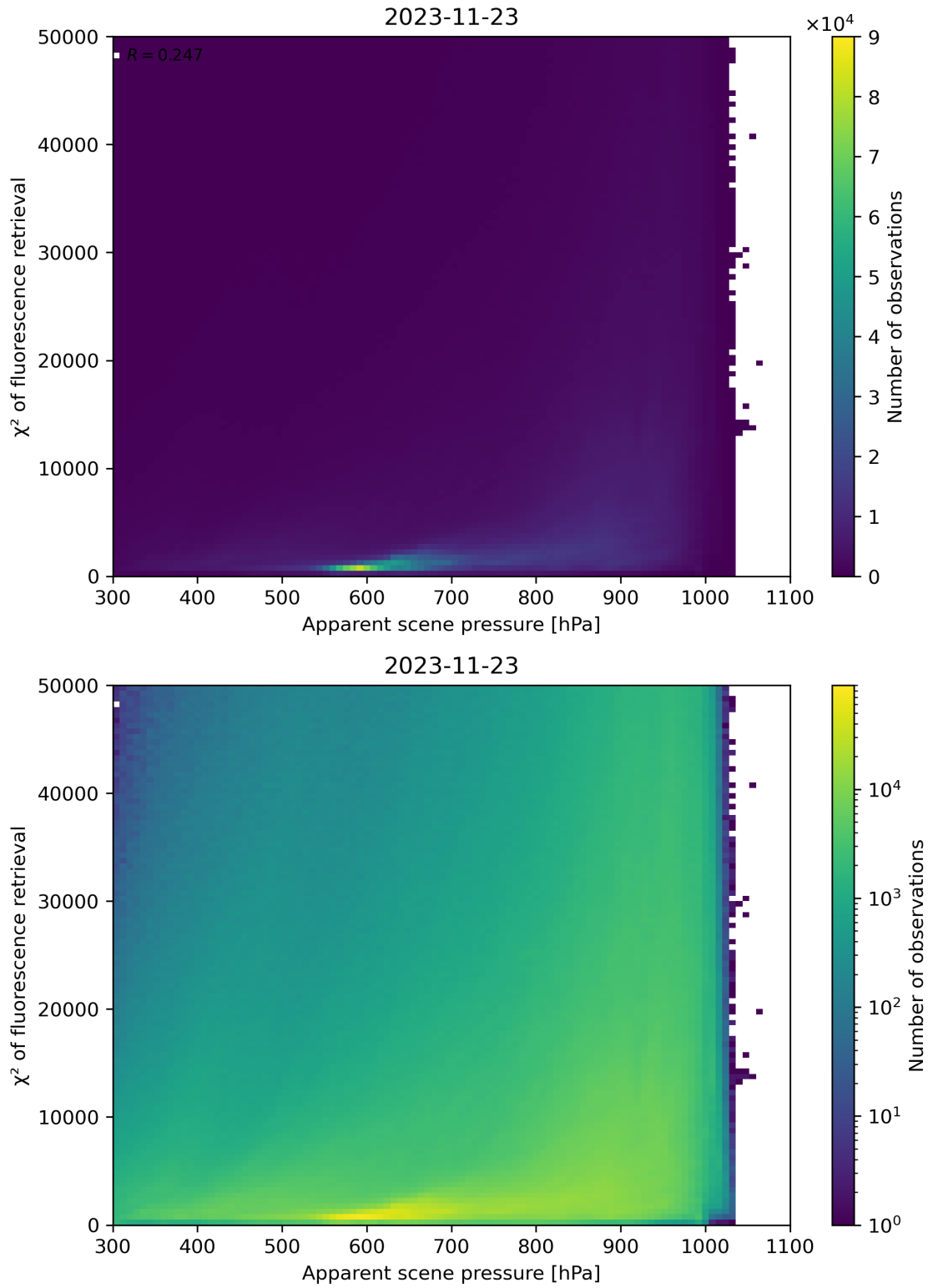
Figure 64: Scatter density plot of “Apparent scene pressure” against “ \chi^2 of fluorescence retrieval” for 2023-11-23 to 2023-11-24.
