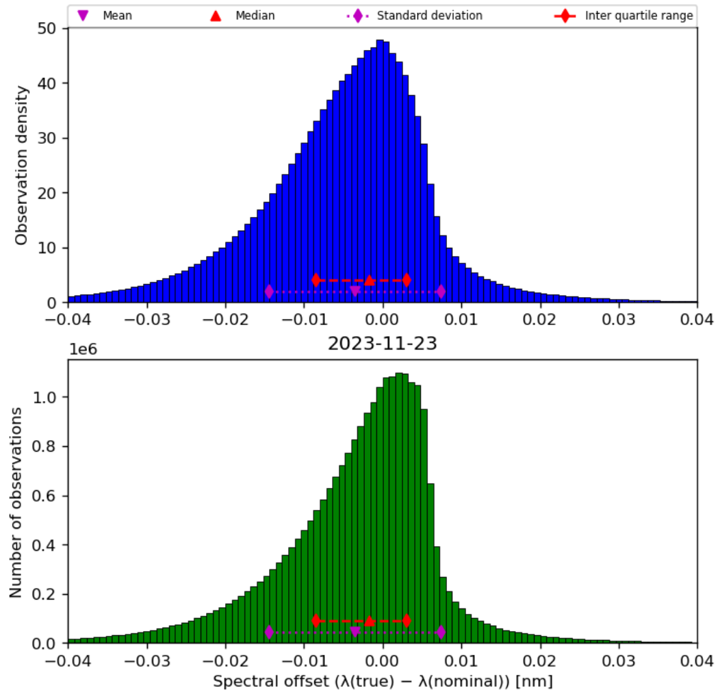
Figure 45: Histogram of “Spectral offset ( \lambda(\text{true}) - \lambda(\text{nominal}) )” for 2023-11-23 to 2023-11-24
