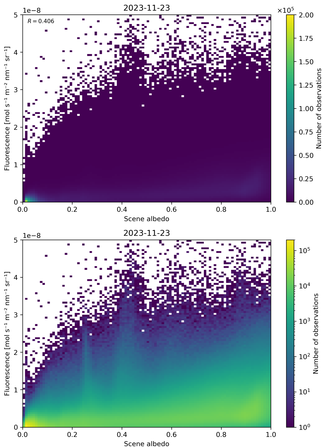
Figure 114: Scatter density plot of “Scene albedo” against “Fluorescence” for 2023-11-23 to 2023-11-24.
