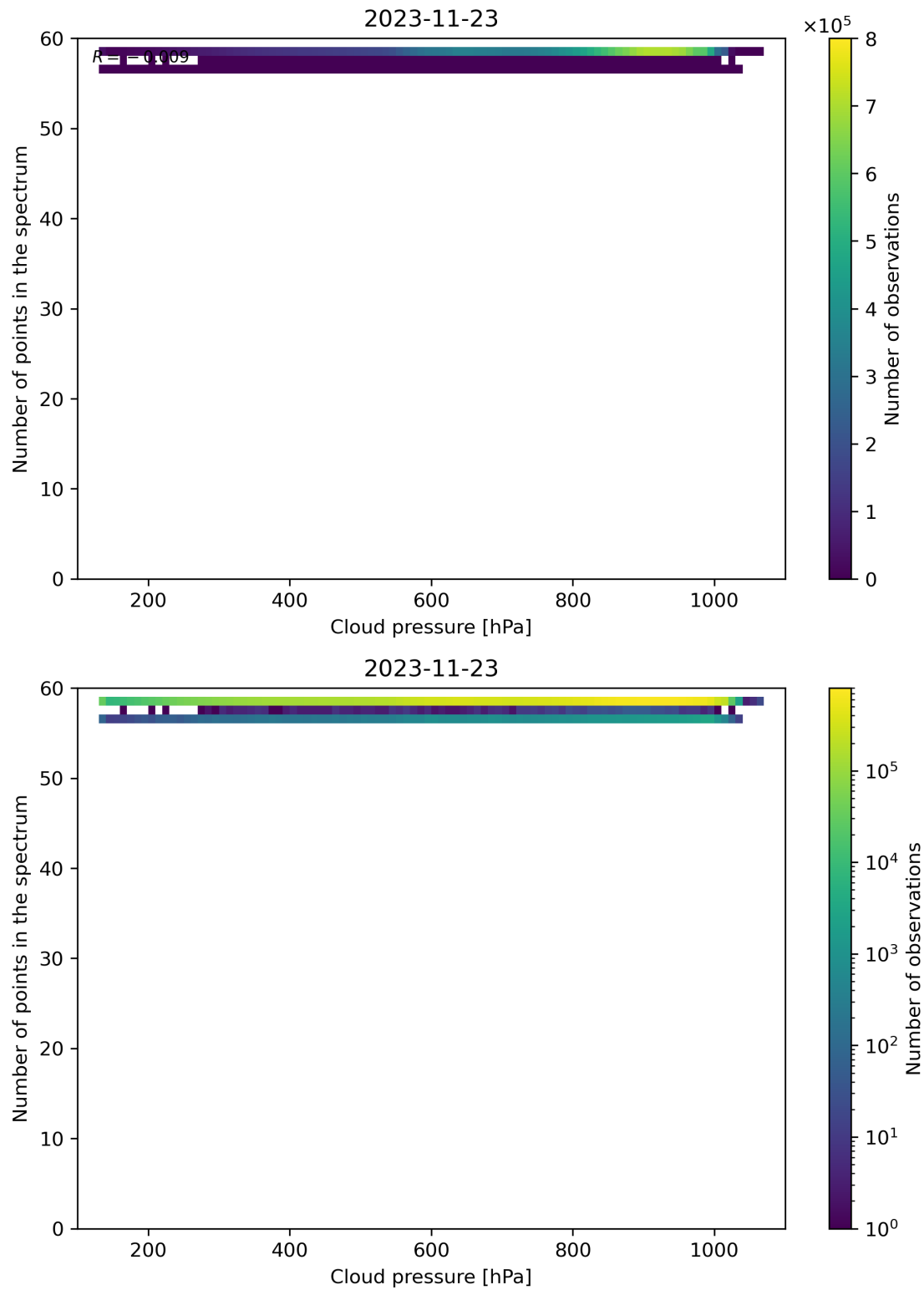
Figure 90: Scatter density plot of “Cloud pressure” against “Number of points in the spectrum” for 2023-11-23 to 2023-11-24.
