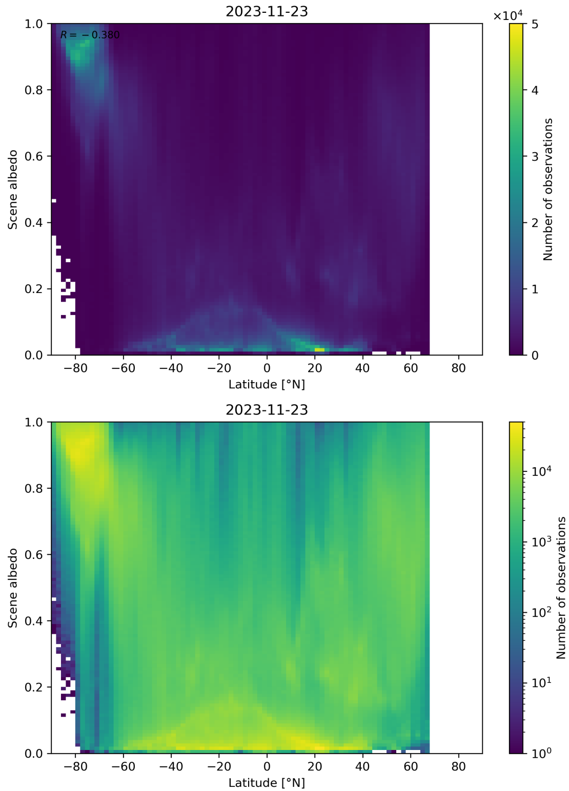
Figure 104: Scatter density plot of “Latitude” against “Scene albedo” for 2023-11-23 to 2023-11-24.
