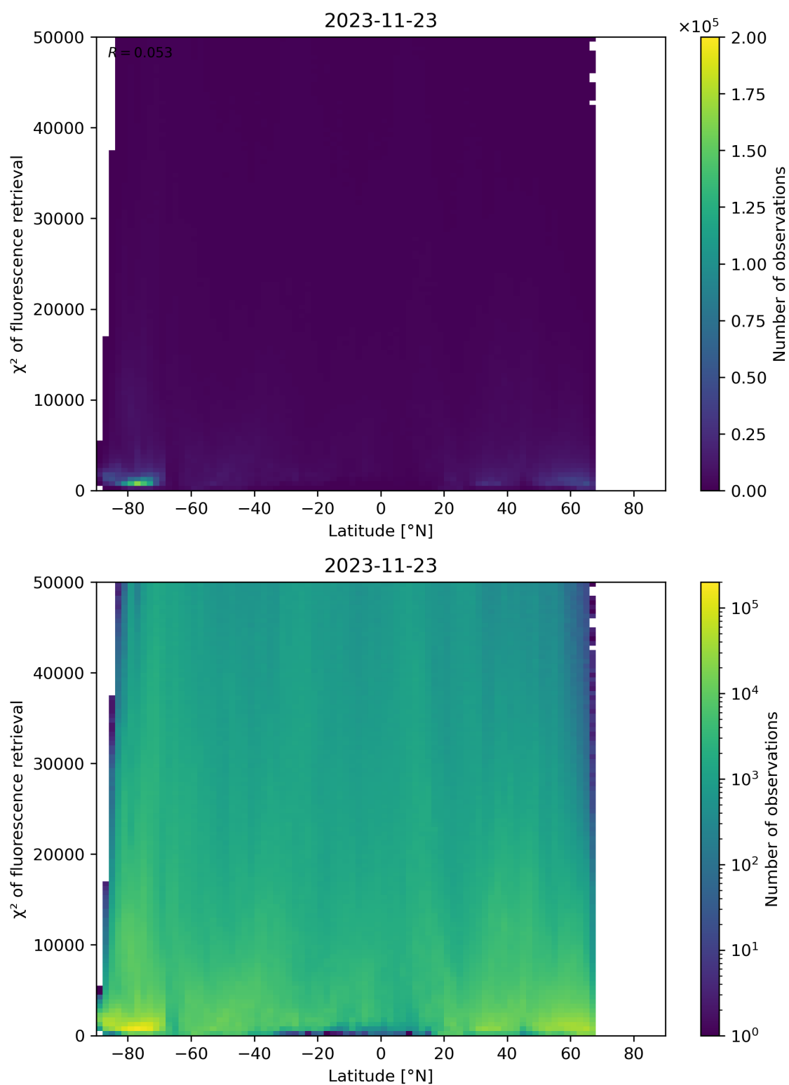
Figure 98: Scatter density plot of “Latitude” against “ \chi^2 of fluorescence retrieval” for 2023-11-23 to 2023-11-24.
