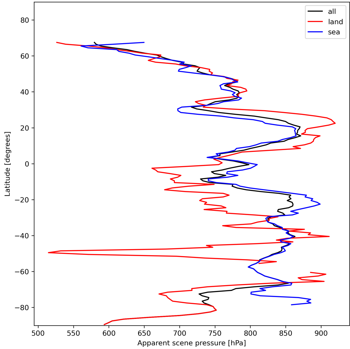
Figure 19: Zonal average of “Apparent scene pressure” for 2023-11-23 to 2023-11-24.
