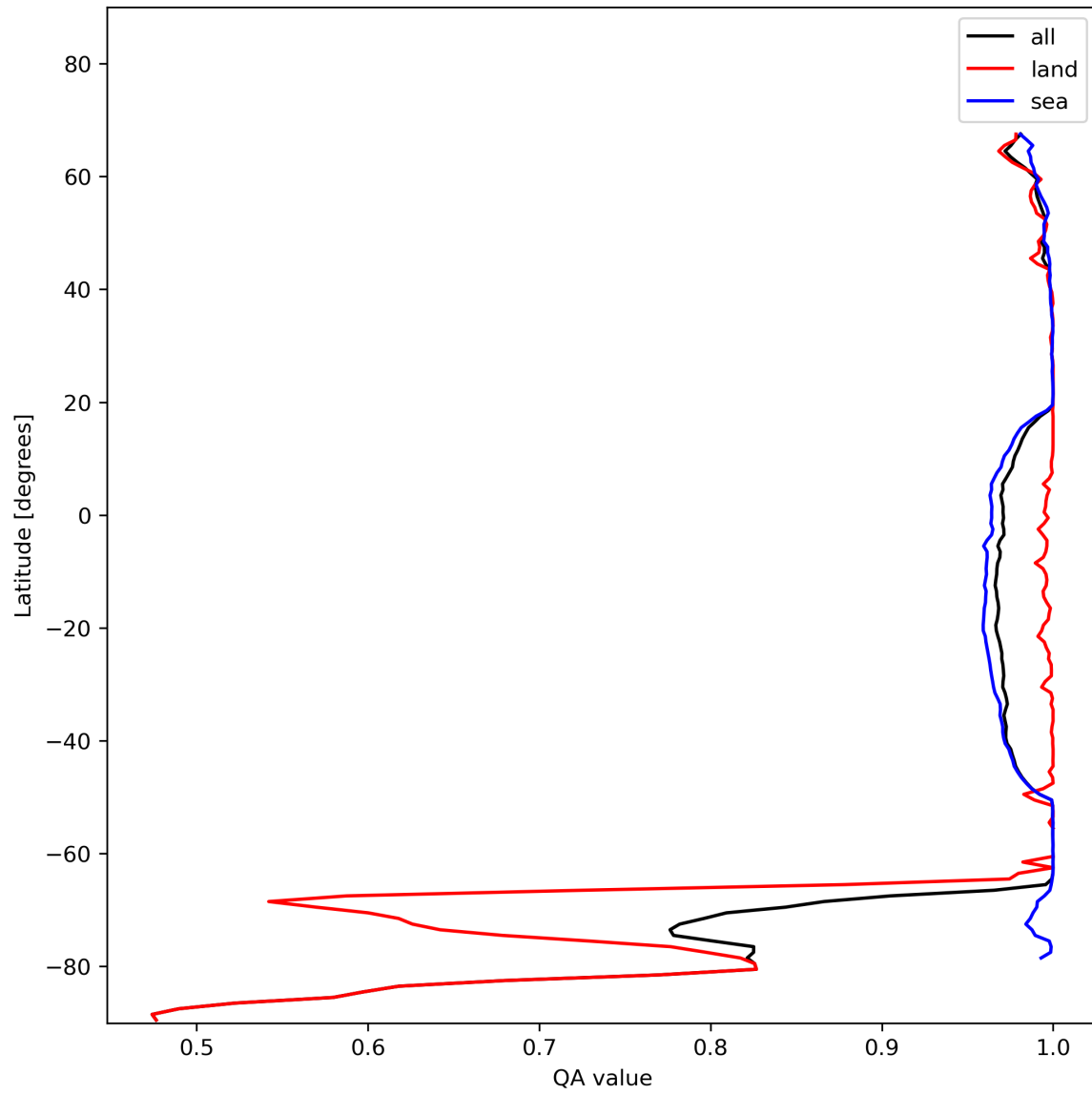
Figure 12: Zonal average of “QA value” for 2023-11-23 to 2023-11-24.
