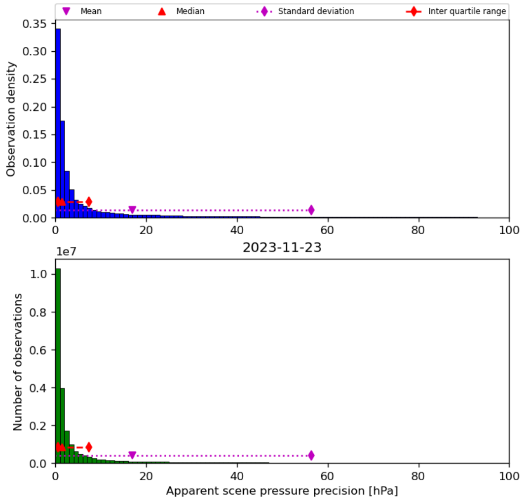
Figure 37: Histogram of “Apparent scene pressure precision” for 2023-11-23 to 2023-11-24
