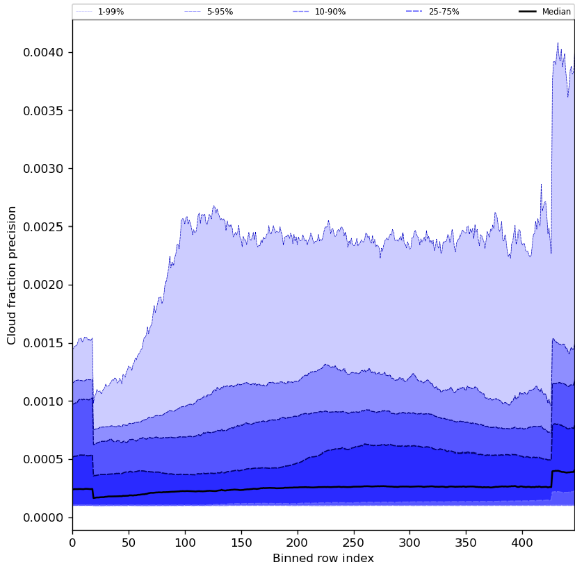
Figure 50: Along track statistics of “Cloud fraction precision” for 2023-11-23 to 2023-11-24
