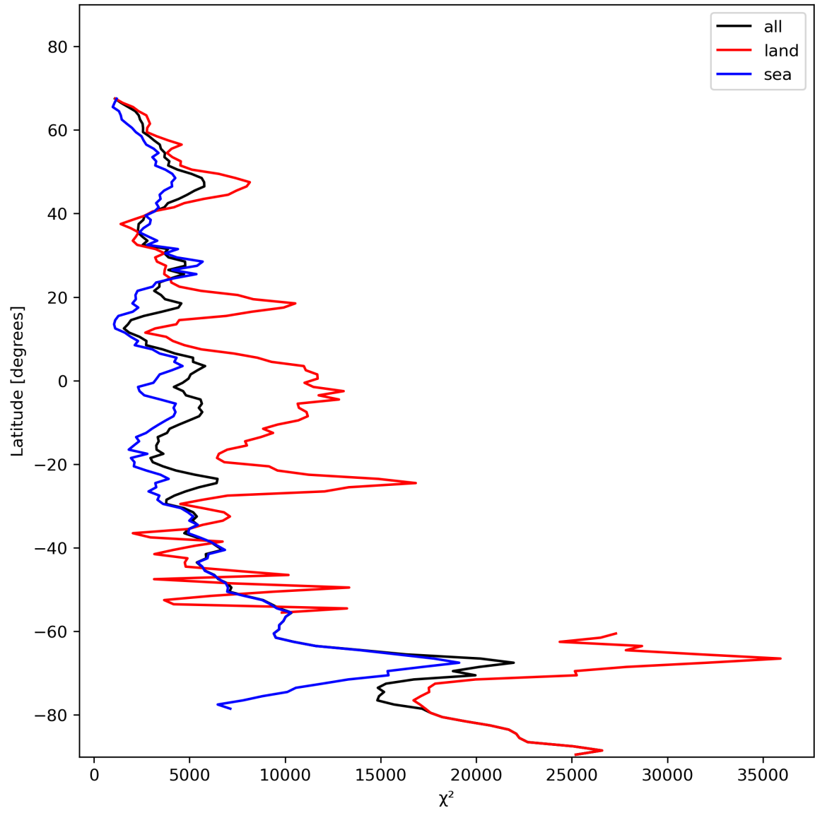
Figure 21: Zonal average of “ \chi^2 ” for 2023-11-23 to 2023-11-24.
