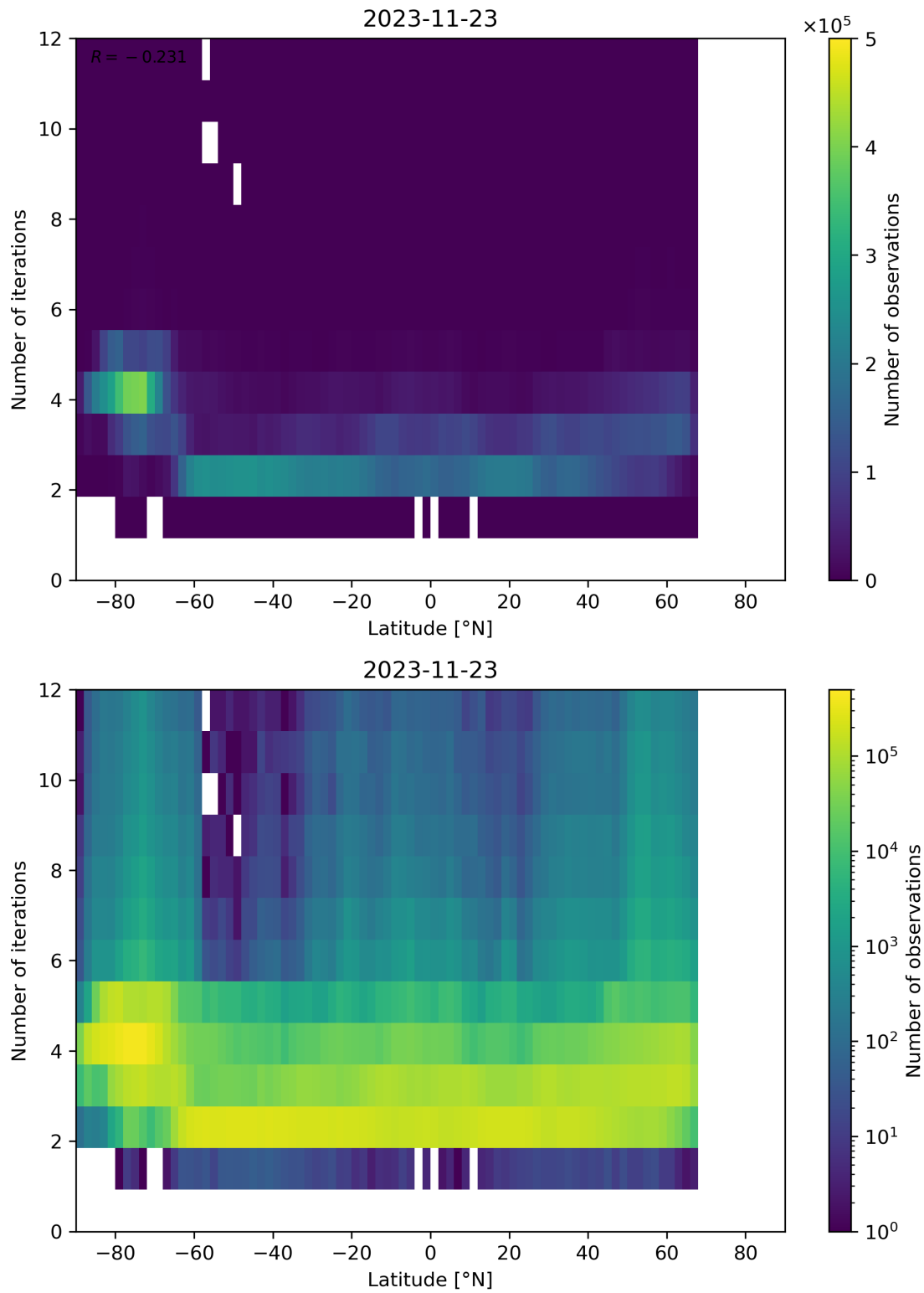
Figure 102: Scatter density plot of “Latitude” against “Number of iterations” for 2023-11-23 to 2023-11-24.
