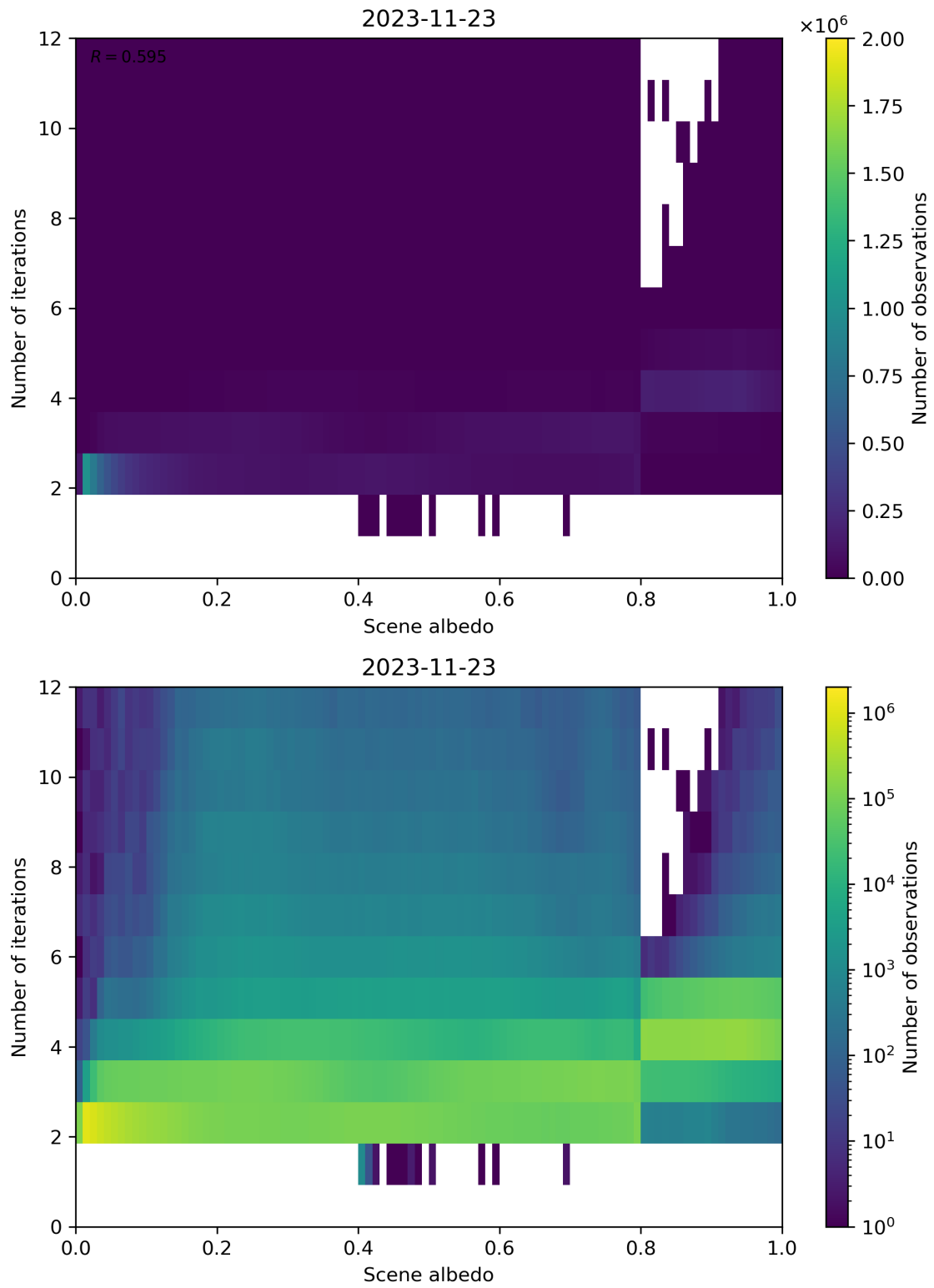
Figure 115: Scatter density plot of “Scene albedo” against “Number of iterations” for 2023-11-23 to 2023-11-24.
