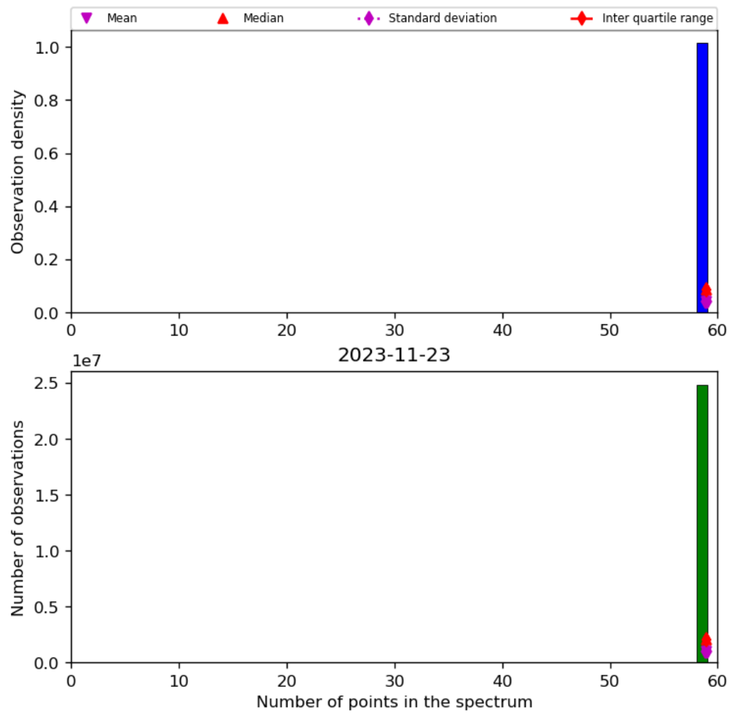
Figure 44: Histogram of “Number of points in the spectrum” for 2023-11-23 to 2023-11-24
