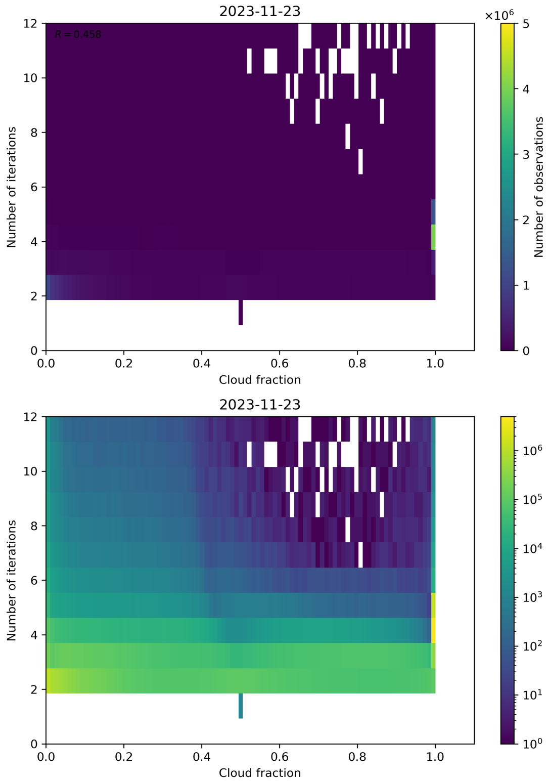
Figure 80: Scatter density plot of “Cloud fraction” against “Number of iterations” for 2023-11-23 to 2023-11-24.
