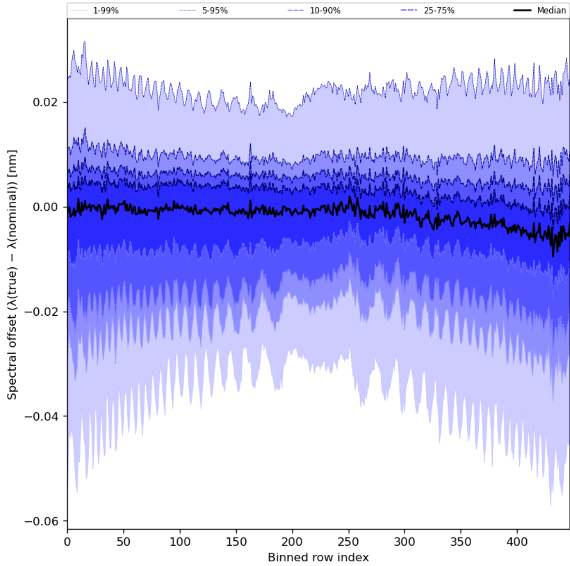
Figure 62: Along track statistics of “Spectral offset ( \lambda(\text{true}) - \lambda(\text{nominal}) )” for 2023-11-23 to 2023-11-24
