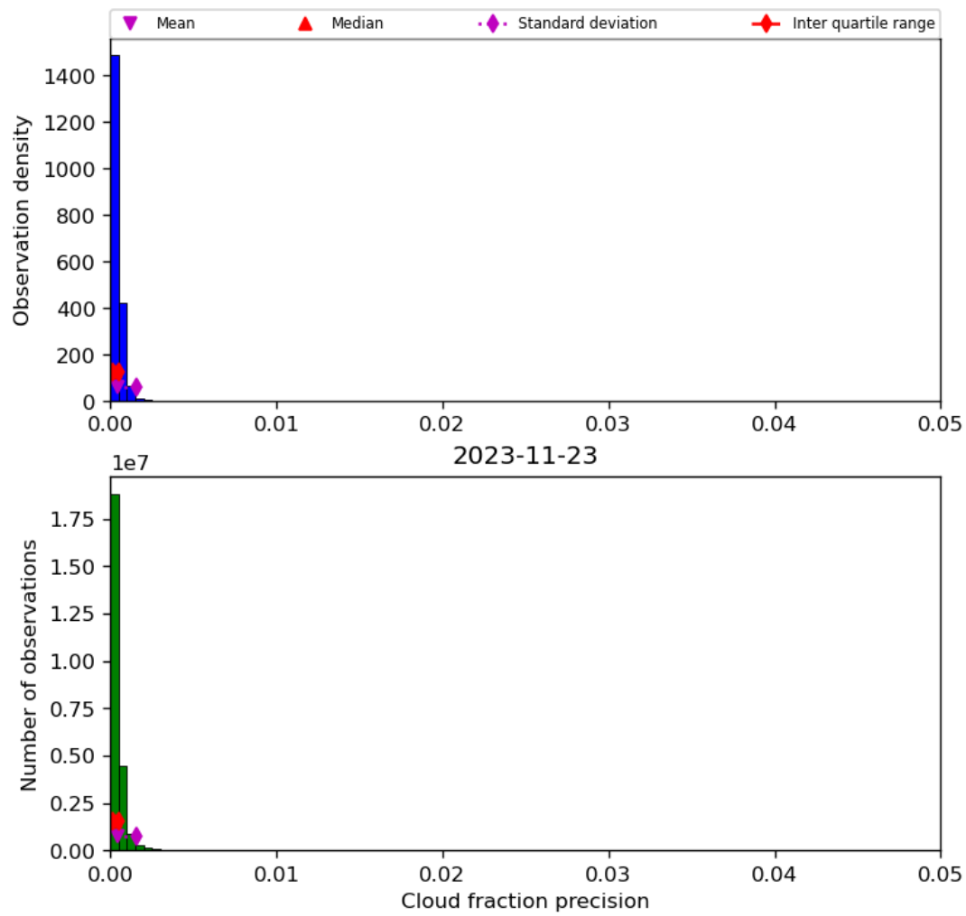
Figure 33: Histogram of “Cloud fraction precision” for 2023-11-23 to 2023-11-24
