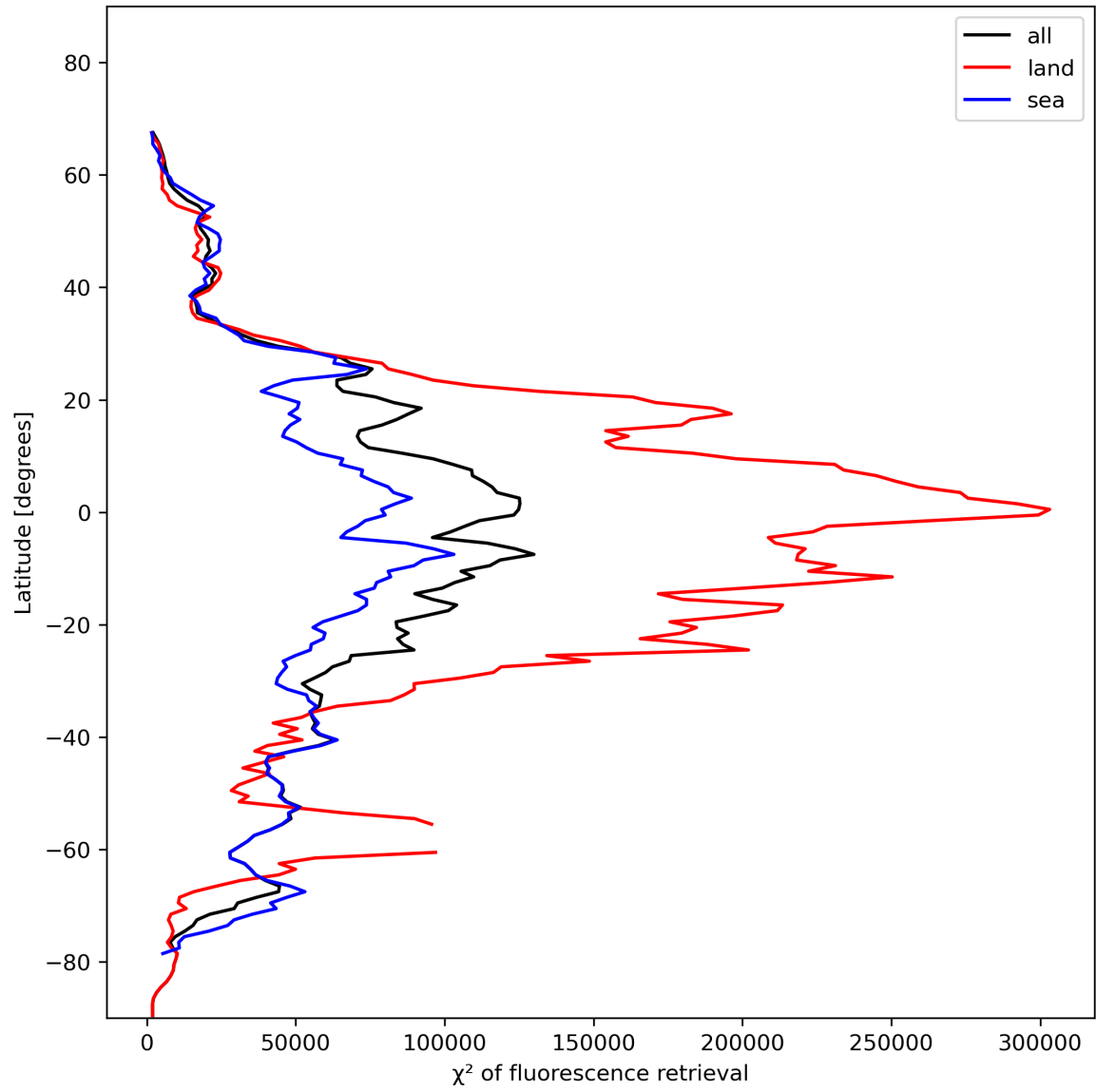
Figure 25: Zonal average of “ \chi^2 of fluorescence retrieval” for 2023-11-23 to 2023-11-24.
