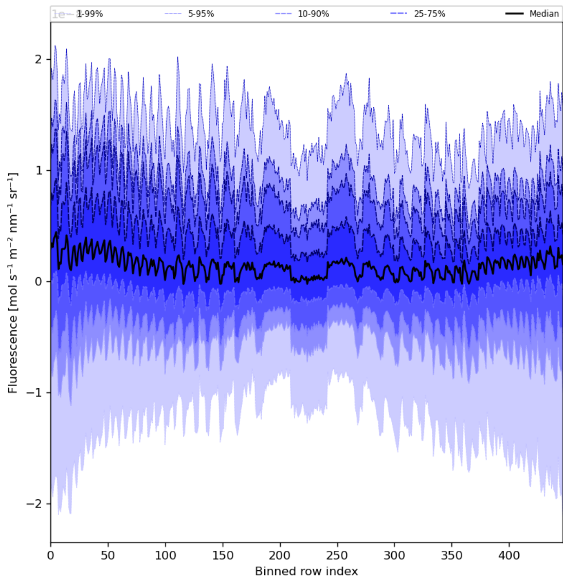
Figure 57: Along track statistics of “Fluorescence” for 2023-11-23 to 2023-11-24
