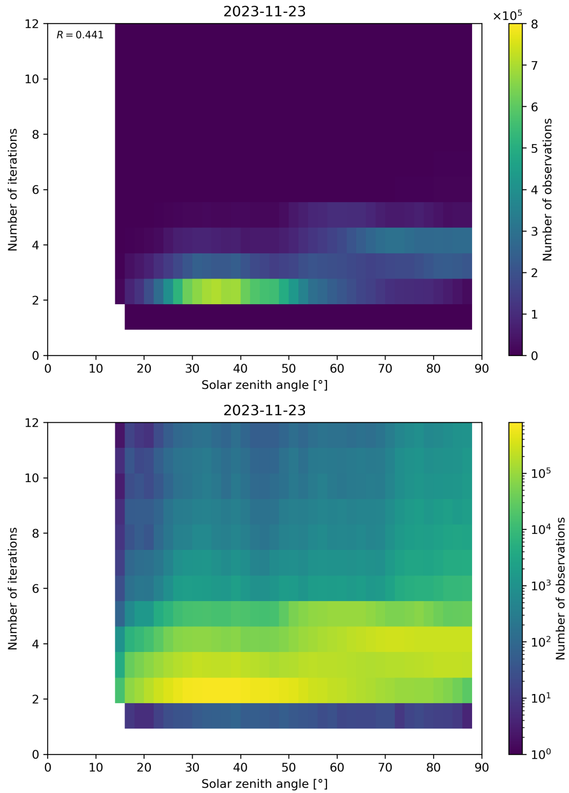
Figure 125: Scatter density plot of “Solar zenith angle” against “Number of iterations” for 2023-11-23 to 2023-11-24.
