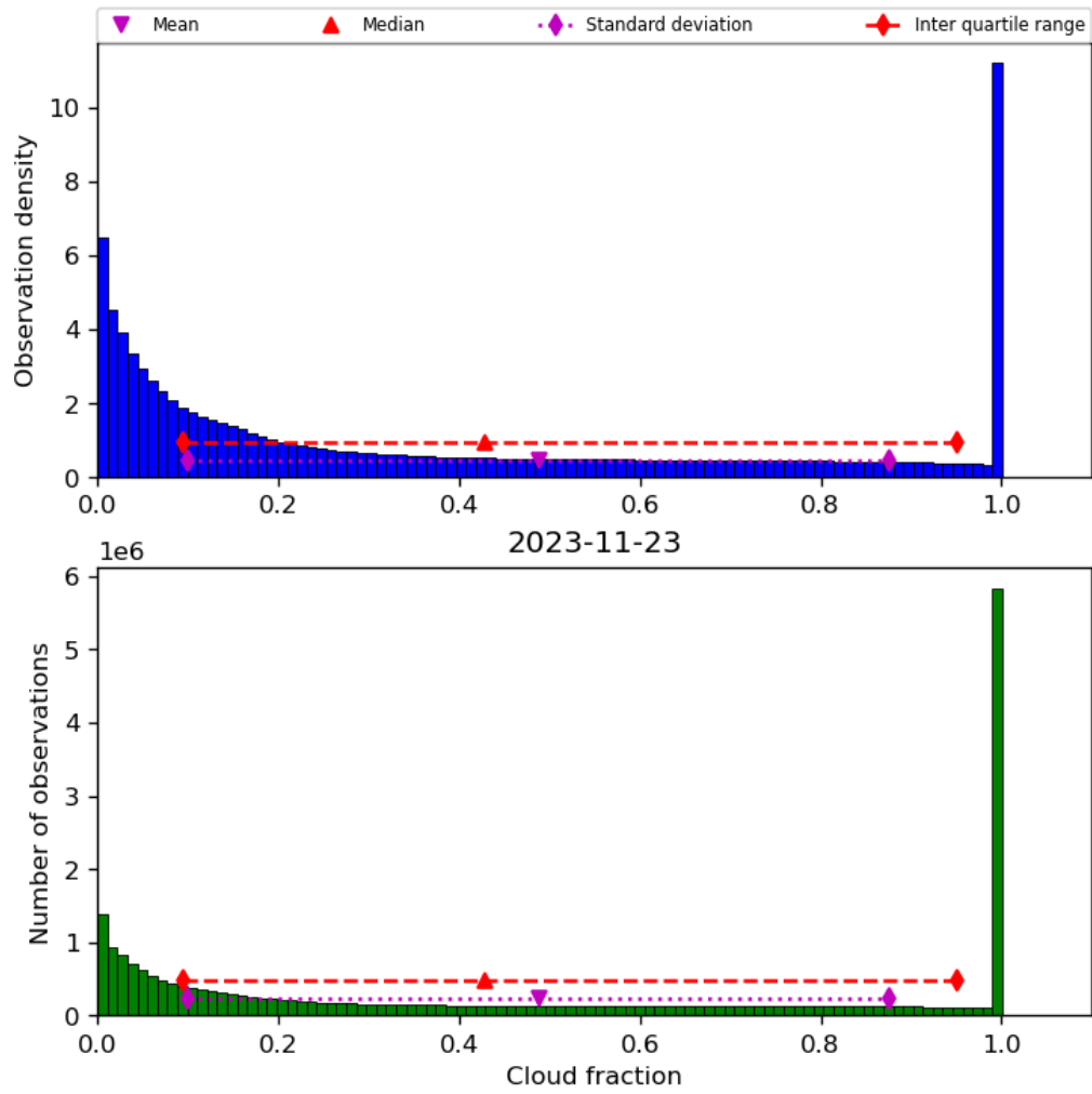
Figure 32: Histogram of “Cloud fraction” for 2023-11-23 to 2023-11-24
