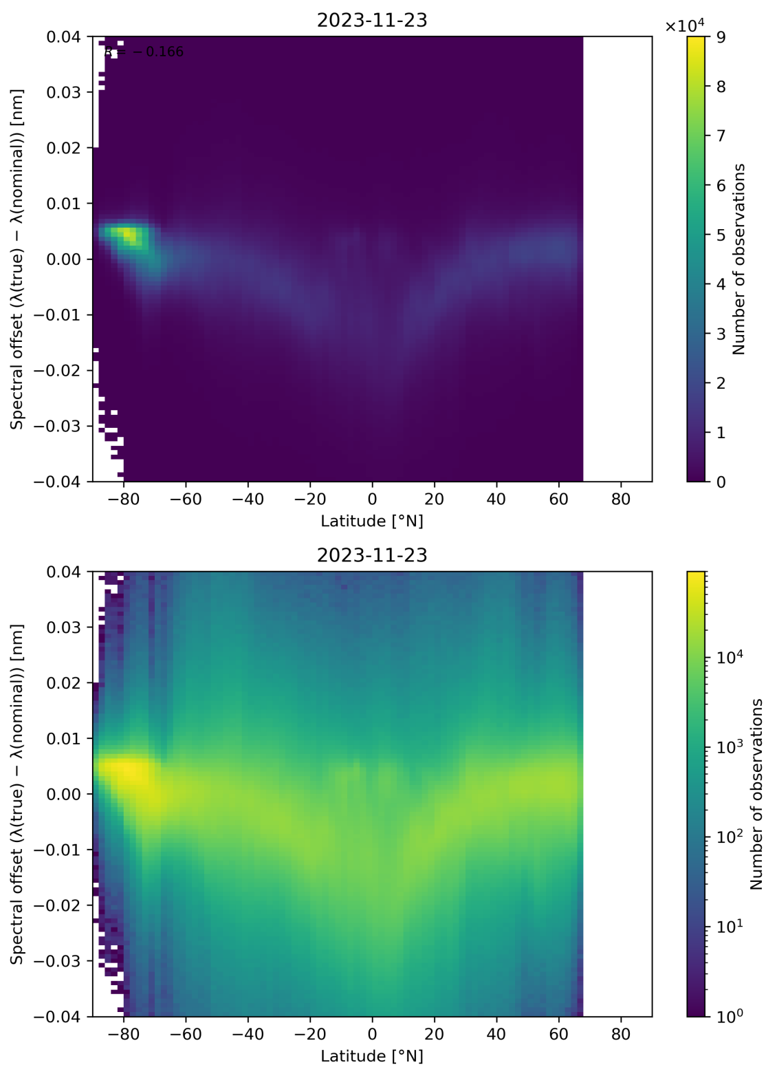
Figure 105: Scatter density plot of “Latitude” against “Spectral offset ( \lambda(\text{true}) - \lambda(\text{nominal}) )” for 2023-11-23 to 2023-11-24.
