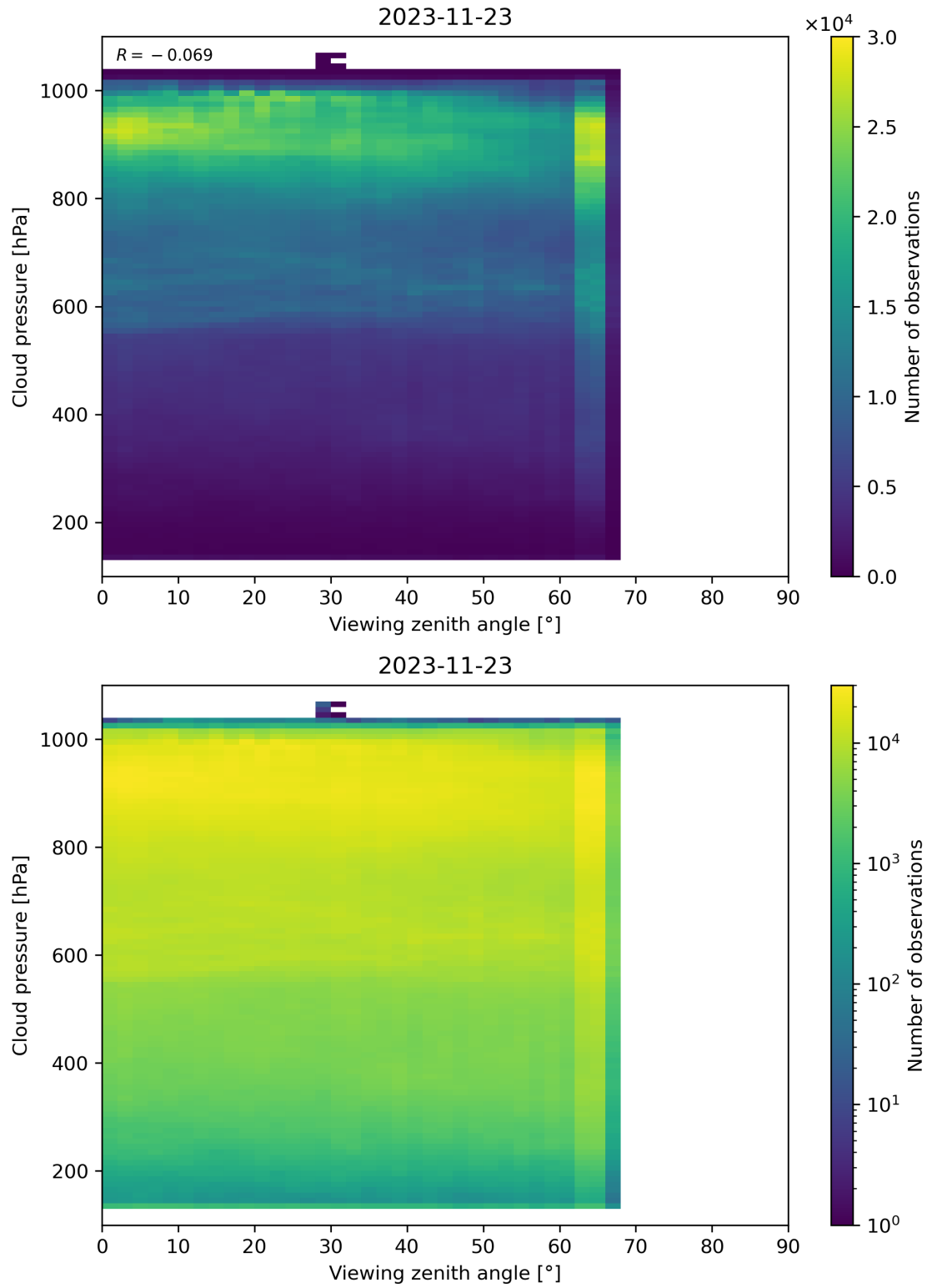
Figure 133: Scatter density plot of “Viewing zenith angle” against “Cloud pressure” for 2023-11-23 to 2023-11-24.
