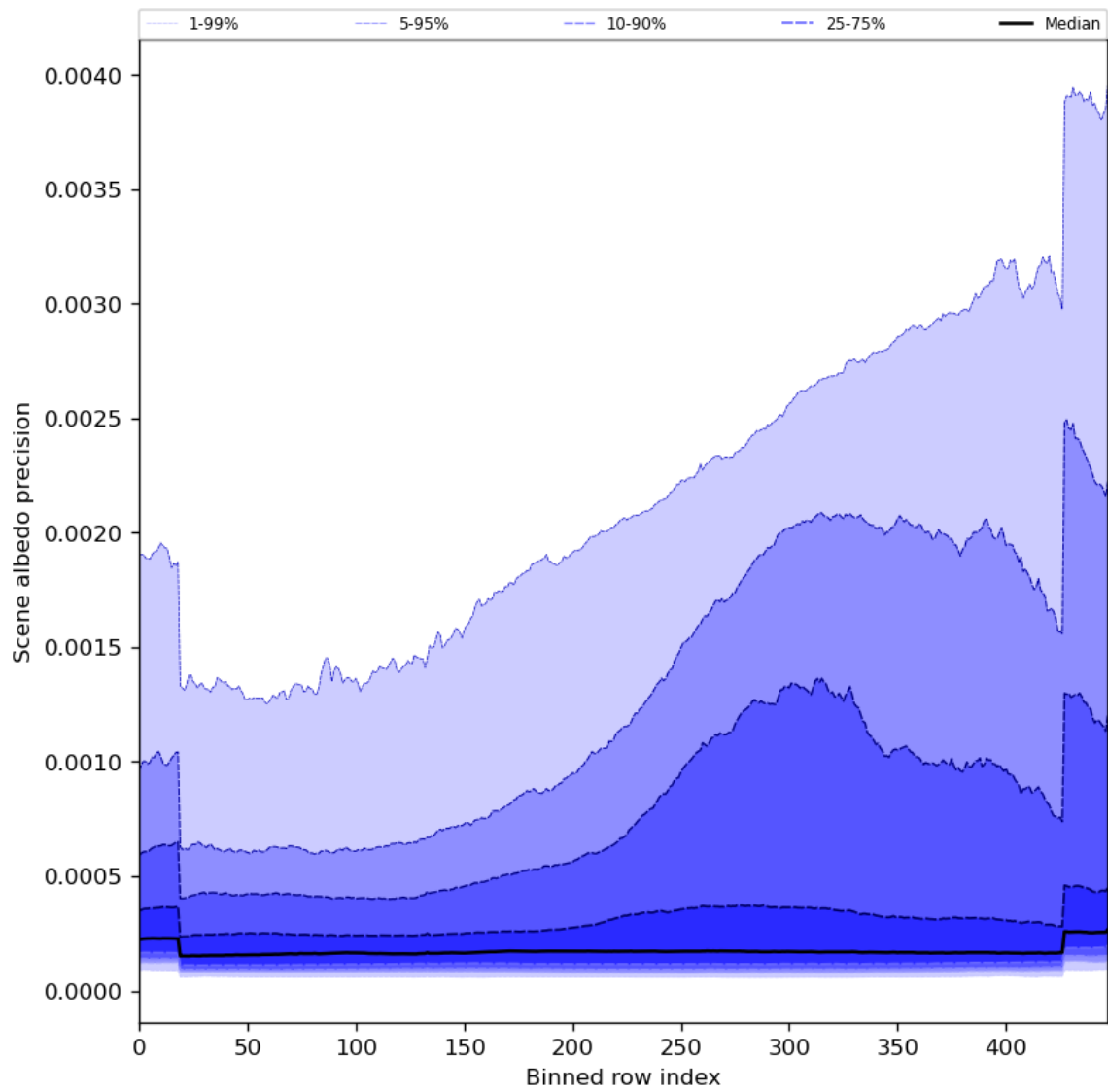
Figure 52: Along track statistics of “Scene albedo precision” for 2023-11-23 to 2023-11-24
