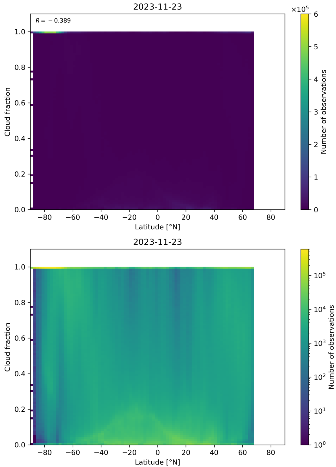
Figure 99: Scatter density plot of “Latitude” against “Cloud fraction” for 2023-11-23 to 2023-11-24.
