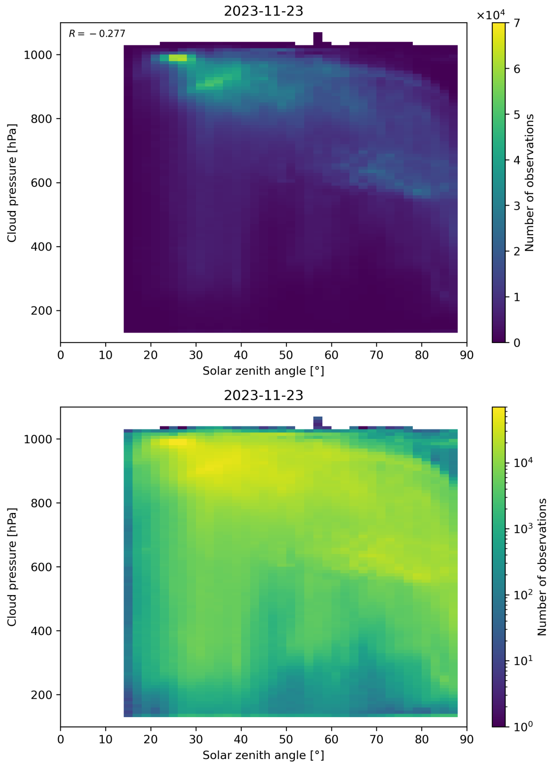
Figure 122: Scatter density plot of “Solar zenith angle” against “Cloud pressure” for 2023-11-23 to 2023-11-24.
