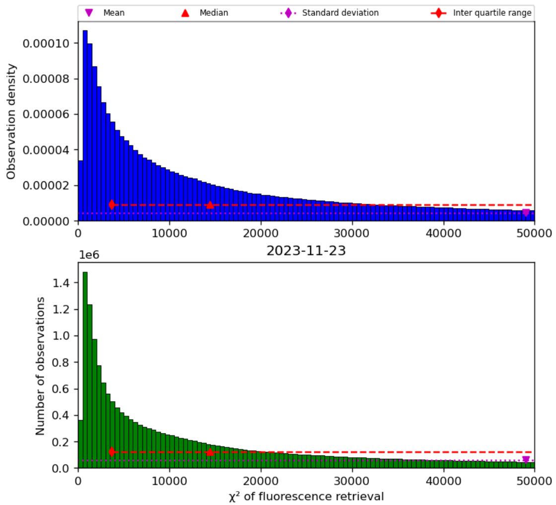
Figure 42: Histogram of “ \chi^2 of fluorescence retrieval” for 2023-11-23 to 2023-11-24
