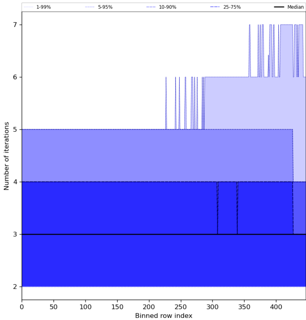
Figure 56: Along track statistics of "Number of iterations" for 2023-11-23 to 2023-11-24
