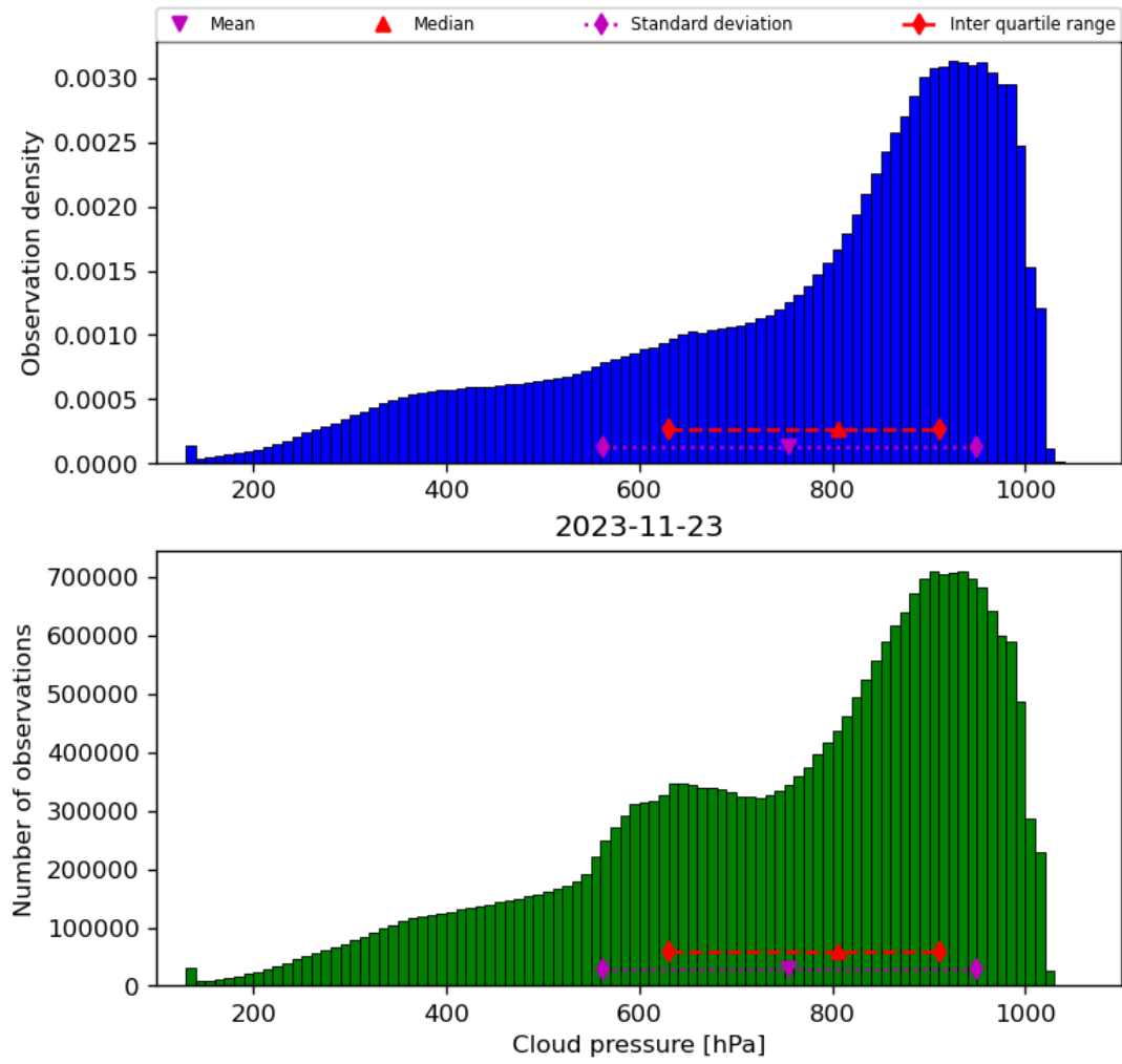
Figure 30: Histogram of “Cloud pressure” for 2023-11-23 to 2023-11-24
