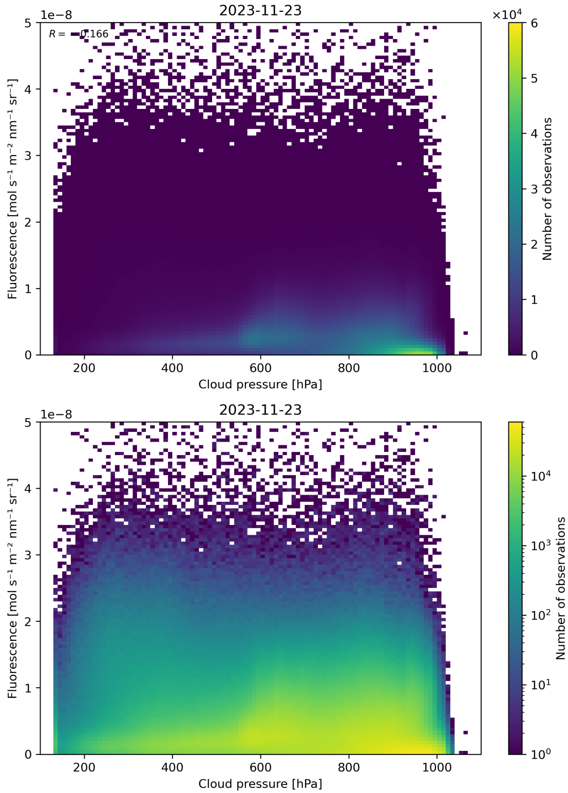
Figure 88: Scatter density plot of “Cloud pressure” against “Fluorescence” for 2023-11-23 to 2023-11-24.
