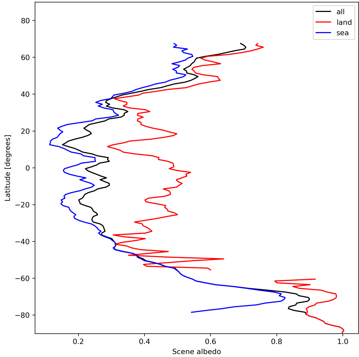
Figure 17: Zonal average of “Scene albedo” for 2023-11-23 to 2023-11-24.
