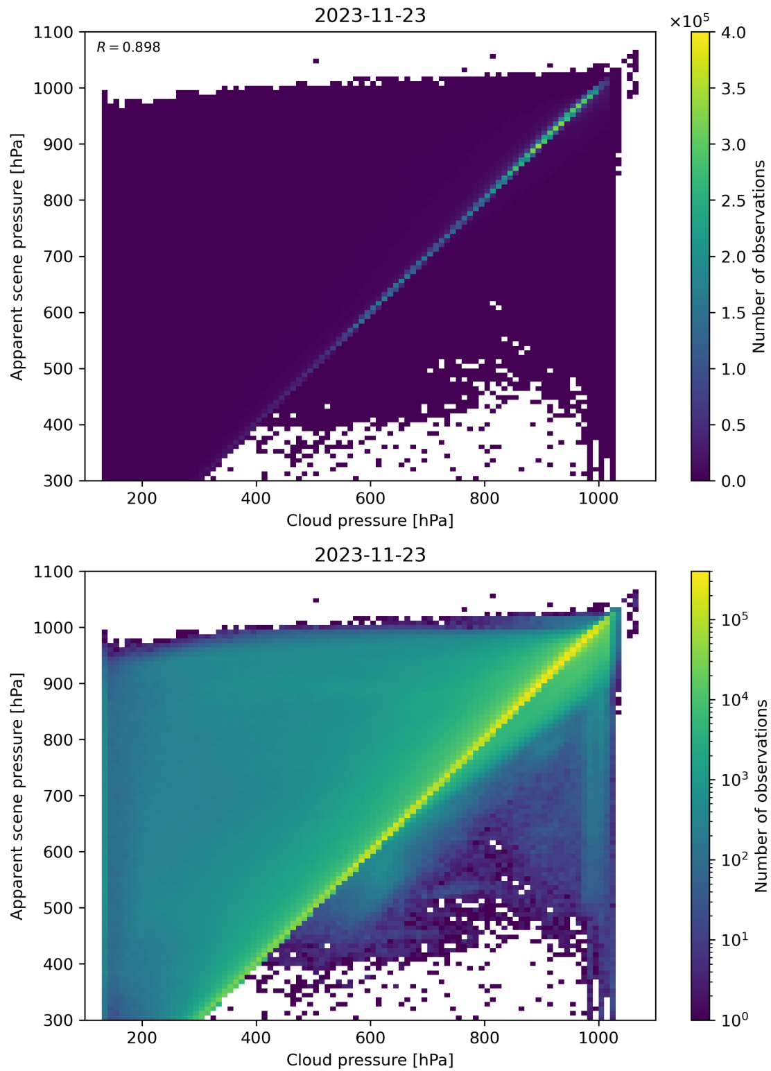
Figure 84: Scatter density plot of “Cloud pressure” against “Apparent scene pressure” for 2023-11-23 to 2023-11-24.
