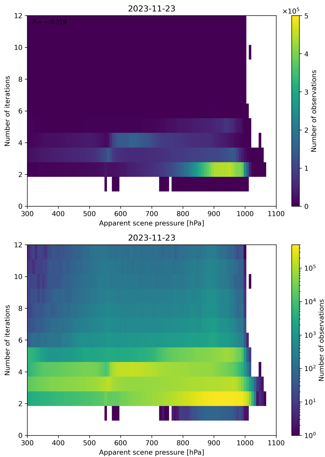
Figure 66: Scatter density plot of “Apparent scene pressure” against “Number of iterations” for 2023-11-23 to 2023-11-24.
