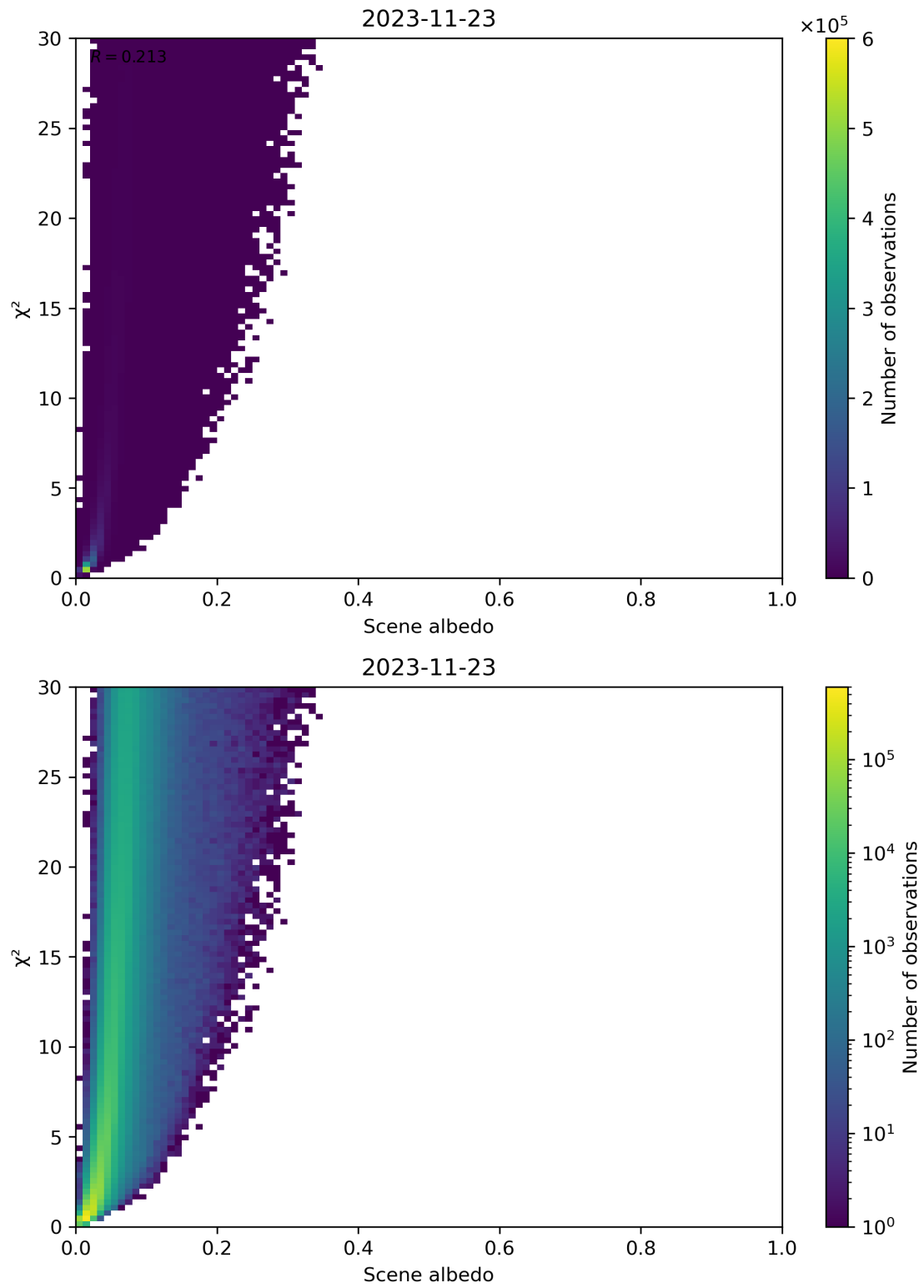
Figure 112: Scatter density plot of “Scene albedo” against “ \chi^2 ” for 2023-11-23 to 2023-11-24.
