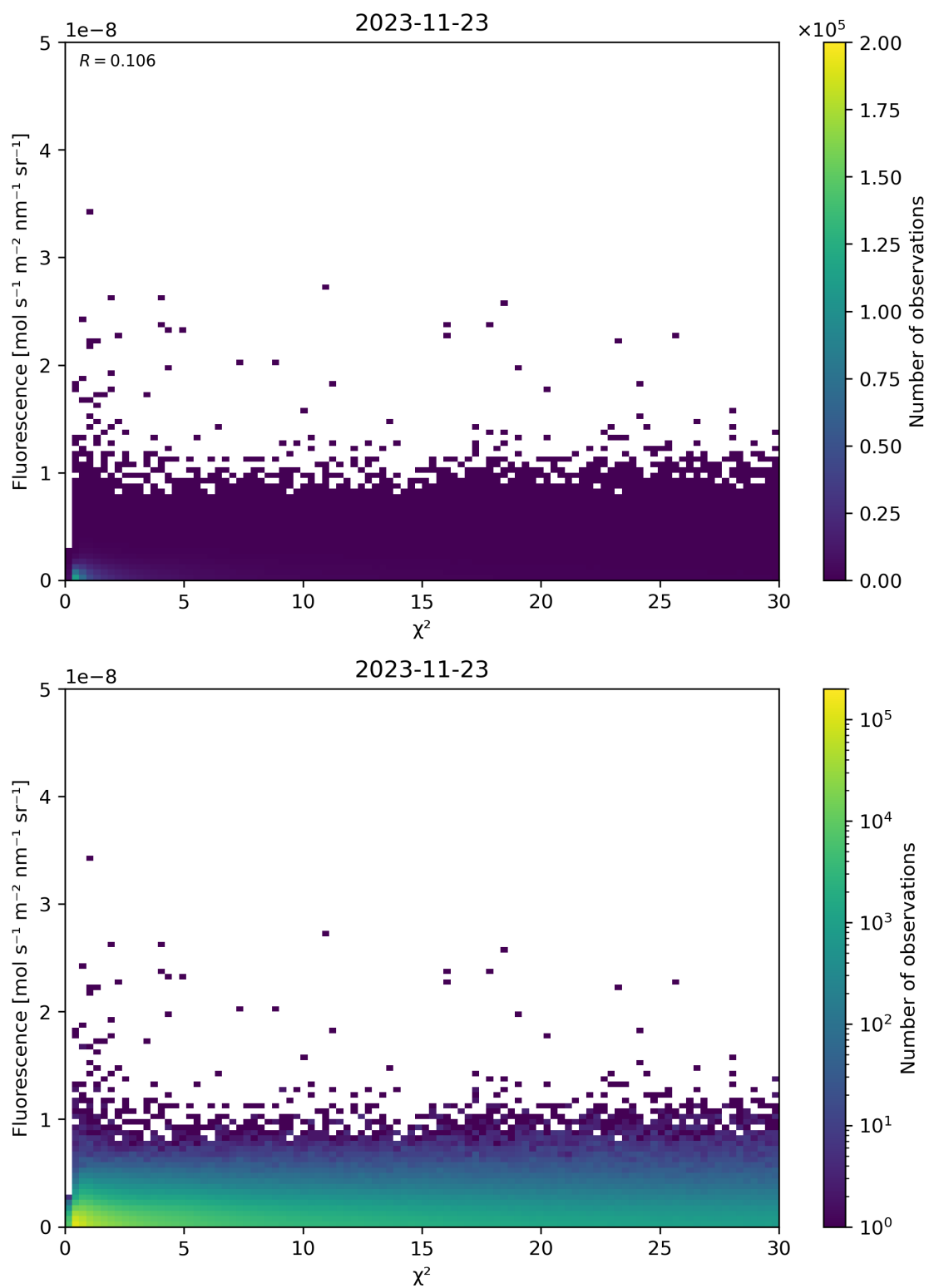
Figure 70: Scatter density plot of “ \chi^2 ” against “Fluorescence” for 2023-11-23 to 2023-11-24.
