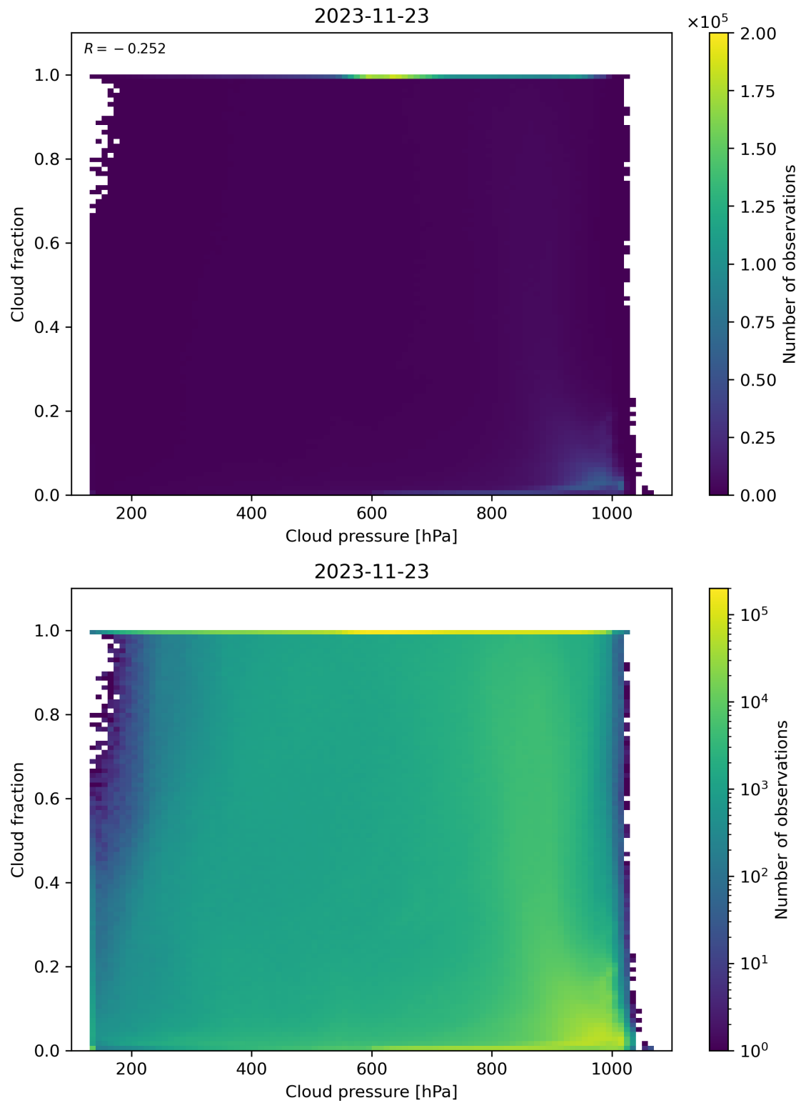
Figure 87: Scatter density plot of “Cloud pressure” against “Cloud fraction” for 2023-11-23 to 2023-11-24.
