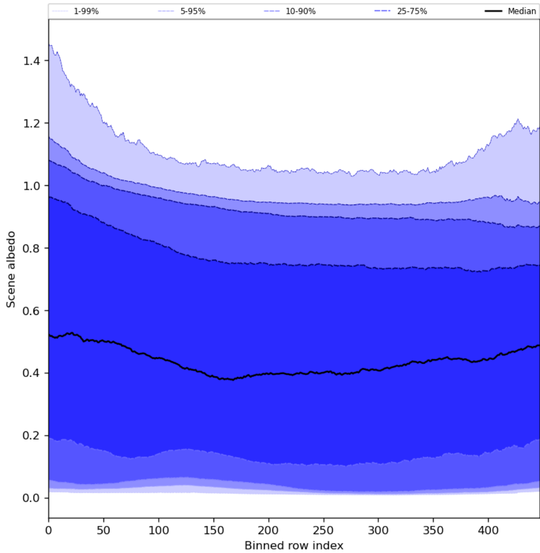
Figure 51: Along track statistics of “Scene albedo” for 2023-11-23 to 2023-11-24
