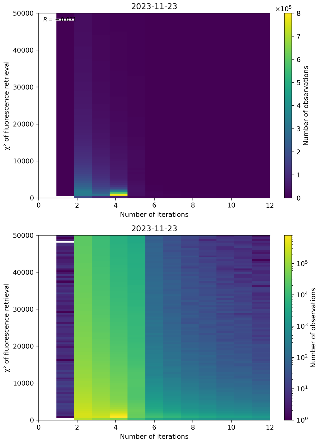
Figure 106: Scatter density plot of “Number of iterations” against “ \chi^2 of fluorescence retrieval” for 2023-11-23 to 2023-11-24.
