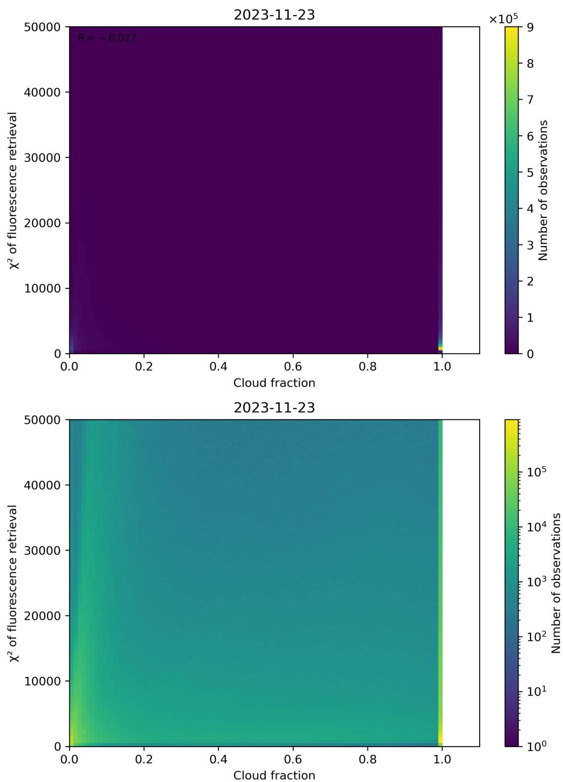
Figure 78: Scatter density plot of “Cloud fraction” against “ \chi^2 of fluorescence retrieval” for 2023-11-23 to 2023-11-24.
