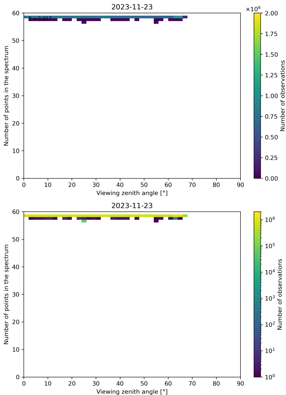
Figure 137: Scatter density plot of “Viewing zenith angle” against “Number of points in the spectrum” for 2023-11-23 to 2023-11-24.
