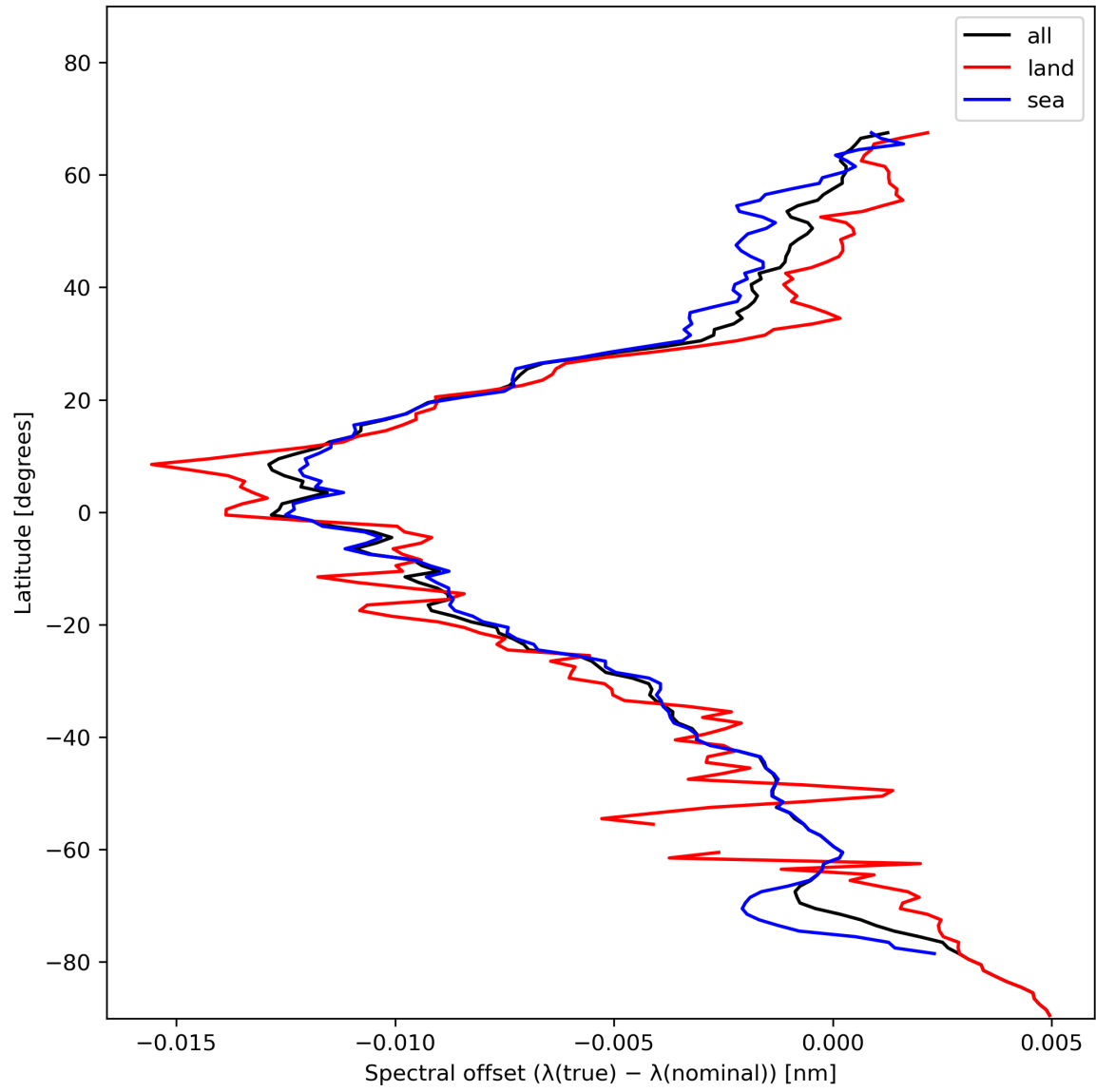
Figure 28: Zonal average of “Spectral offset ( \lambda(\text{true}) - \lambda(\text{nominal}) )” for 2023-11-23 to 2023-11-24.
