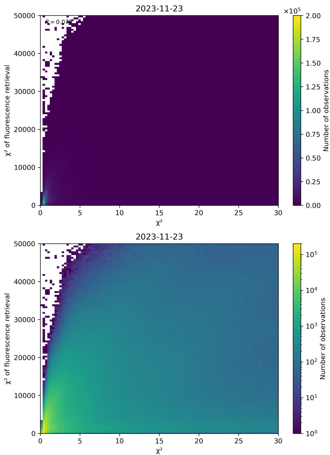
Figure 69: Scatter density plot of “ \chi^2 ” against “ \chi^2 of fluorescence retrieval” for 2023-11-23 to 2023-11-24.
