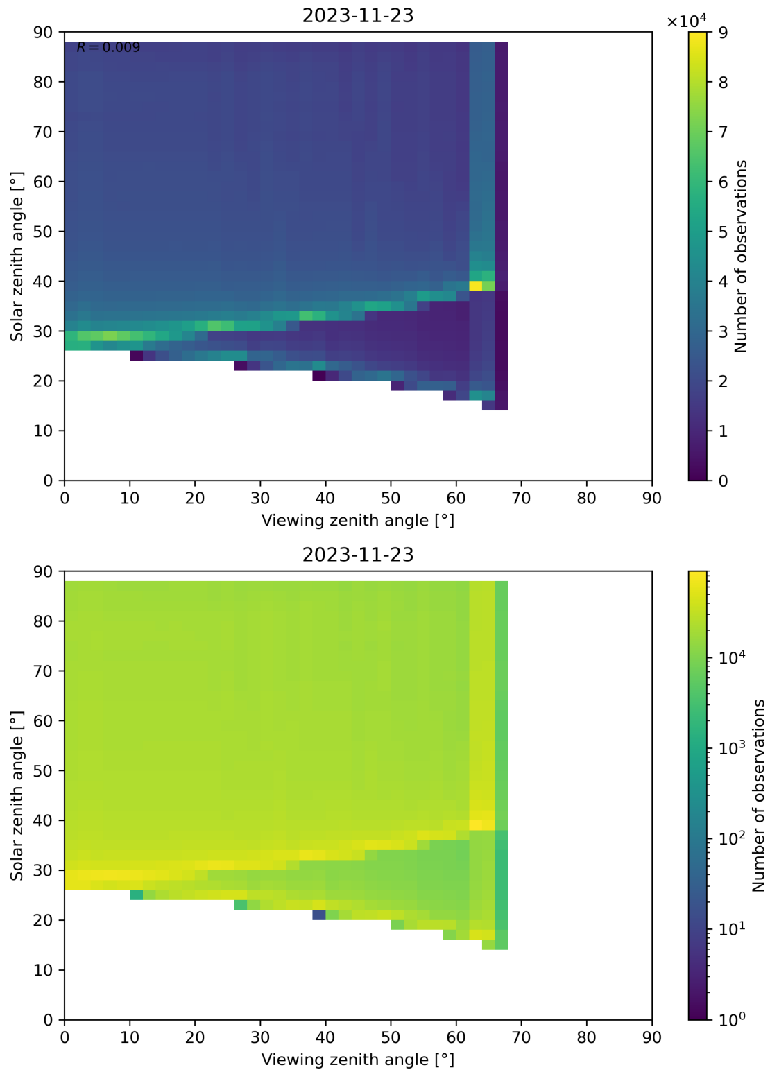
Figure 139: Scatter density plot of “Viewing zenith angle” against “Solar zenith angle” for 2023-11-23 to 2023-11-24.
