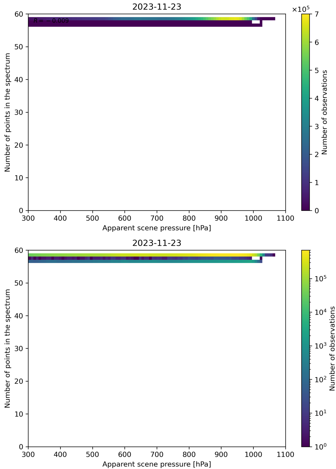
Figure 67: Scatter density plot of “Apparent scene pressure” against “Number of points in the spectrum” for 2023-11-23 to 2023-11-24.
