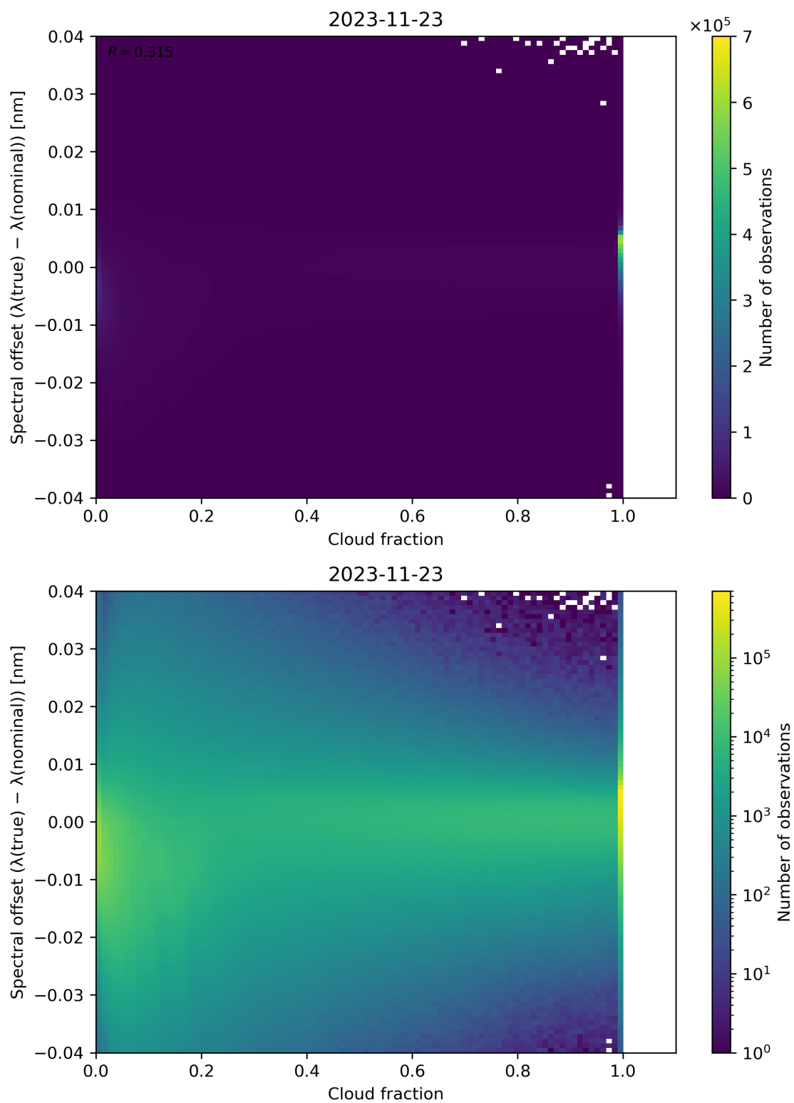
Figure 83: Scatter density plot of “Cloud fraction” against “Spectral offset ( \lambda(\text{true}) - \lambda(\text{nominal}) )” for 2023-11-23 to 2023-11-24.
