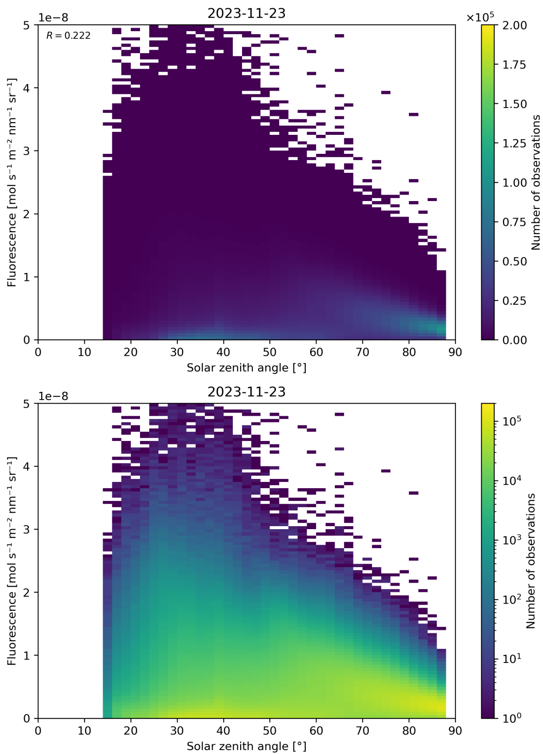
Figure 123: Scatter density plot of “Solar zenith angle” against “Fluorescence” for 2023-11-23 to 2023-11-24.
