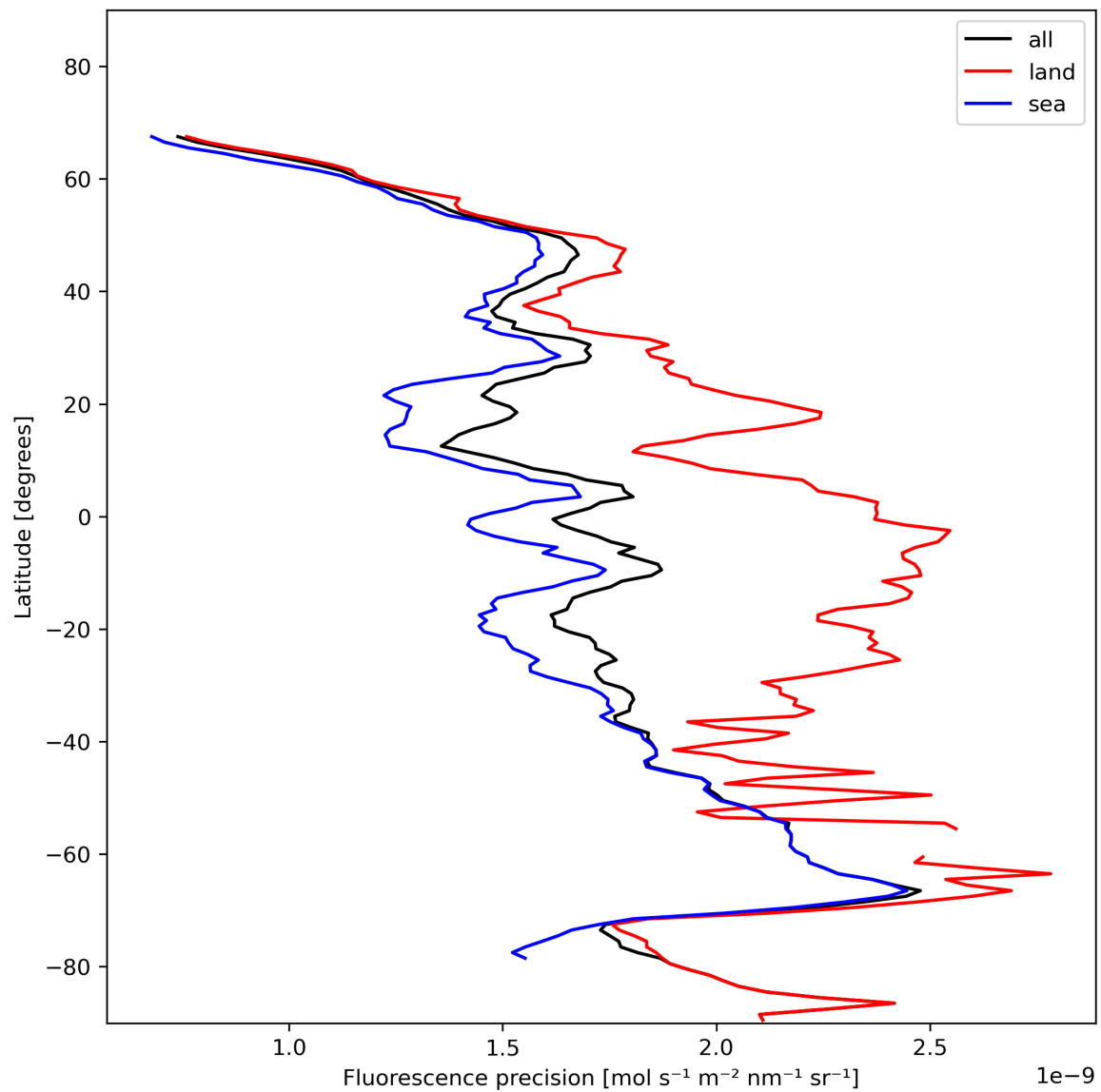
Figure 24: Zonal average of “Fluorescence precision” for 2023-11-23 to 2023-11-24.
