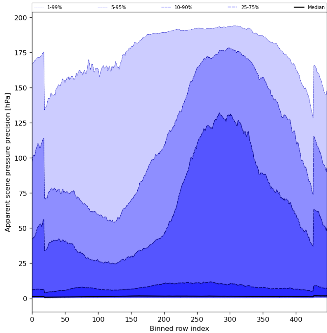
Figure 54: Along track statistics of “Apparent scene pressure precision” for 2023-11-23 to 2023-11-24
