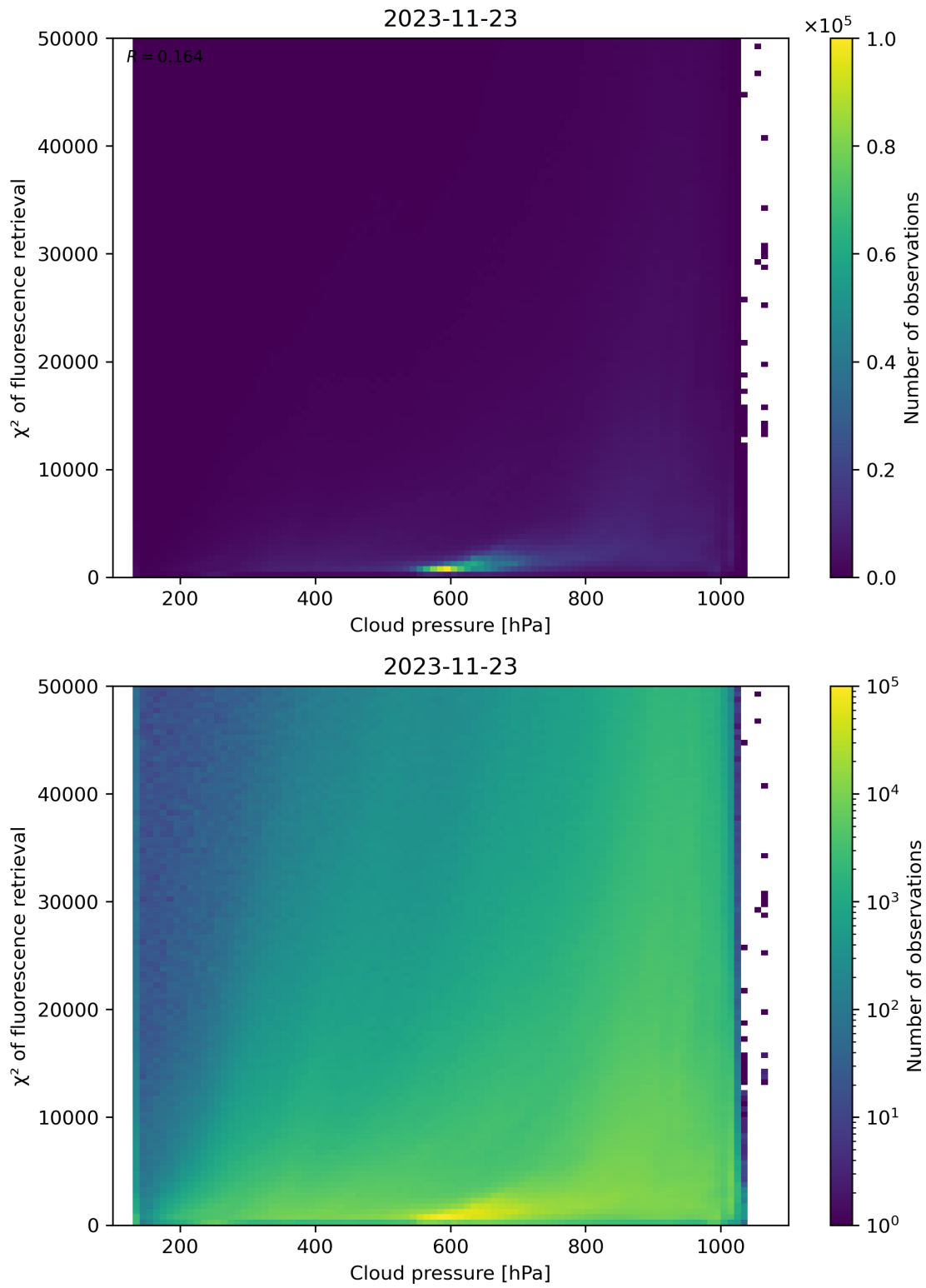
Figure 86: Scatter density plot of “Cloud pressure” against “ \chi^2 of fluorescence retrieval” for 2023-11-23 to 2023-11-24.
