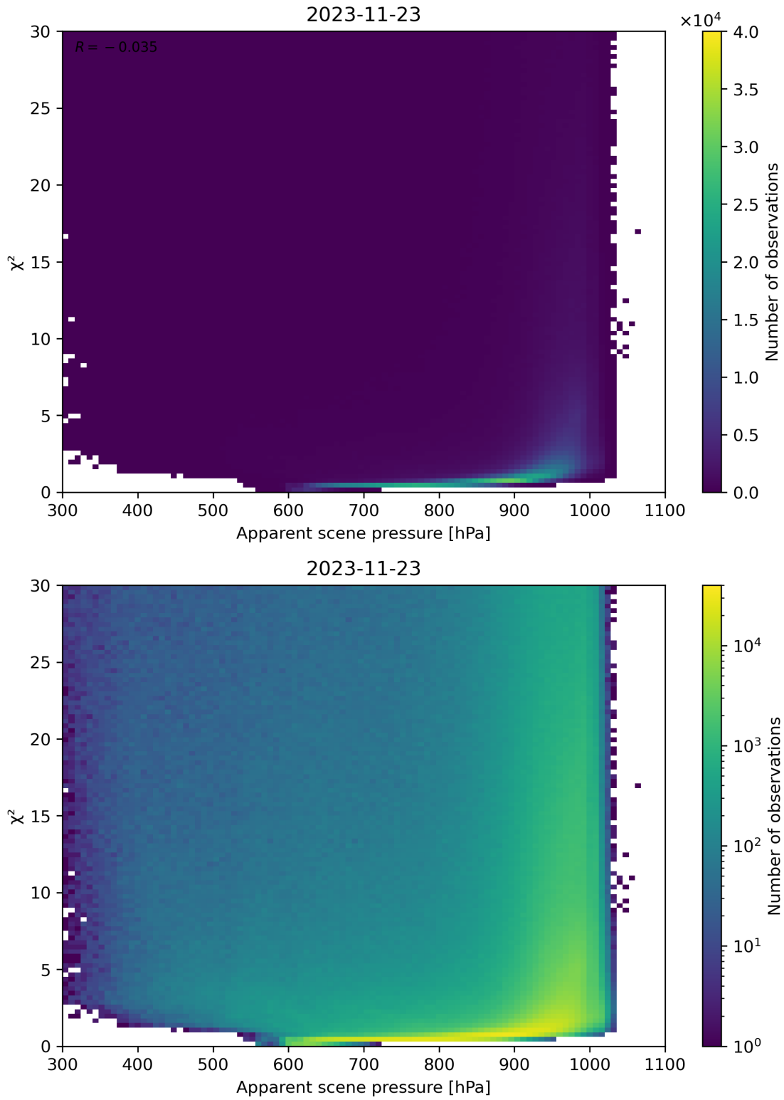
Figure 63: Scatter density plot of “Apparent scene pressure” against “ \chi^2 ” for 2023-11-23 to 2023-11-24.
