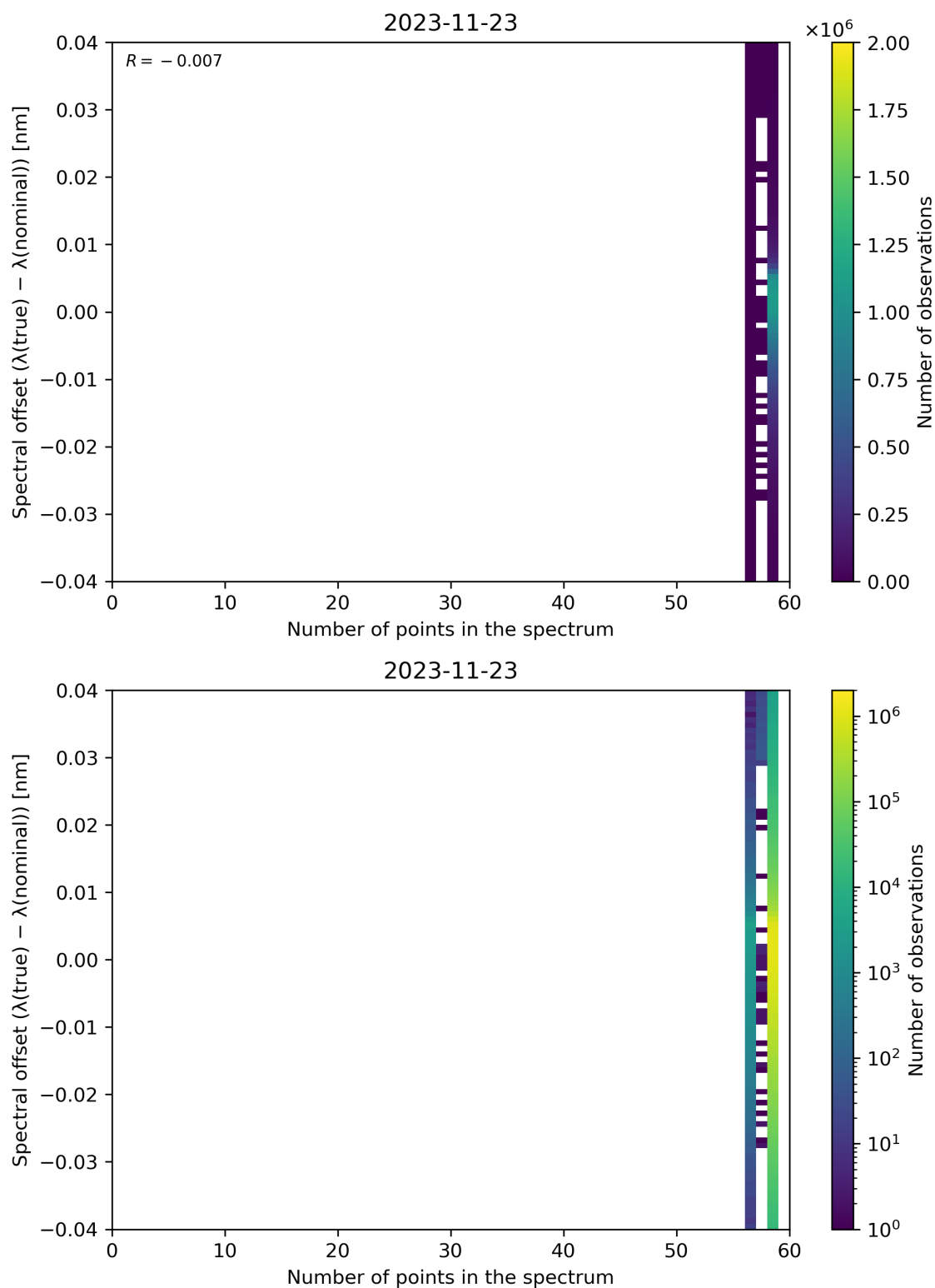
Figure 110: Scatter density plot of “Number of points in the spectrum” against “Spectral offset ( \lambda(\text{true}) - \lambda(\text{nominal}) )” for 2023-11-23 to 2023-11-24.
