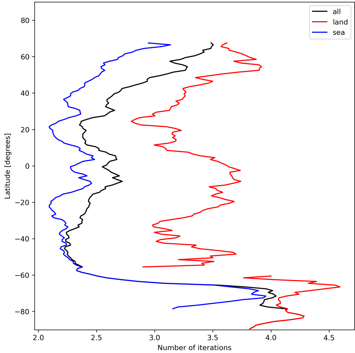
Figure 22: Zonal average of “Number of iterations” for 2023-11-23 to 2023-11-24.
