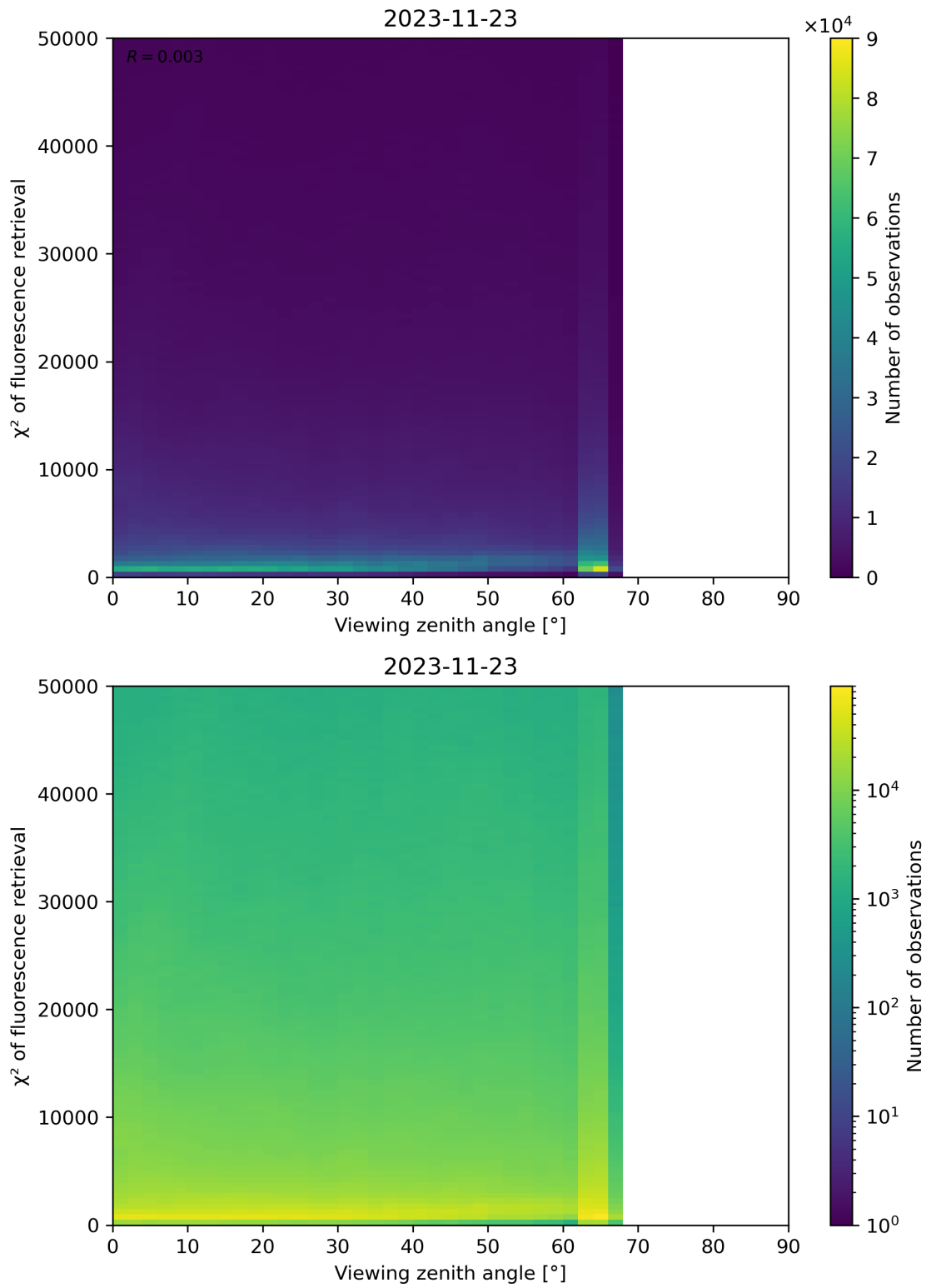
Figure 131: Scatter density plot of “Viewing zenith angle” against “ \chi^2 of fluorescence retrieval” for 2023-11-23 to 2023-11-24.
