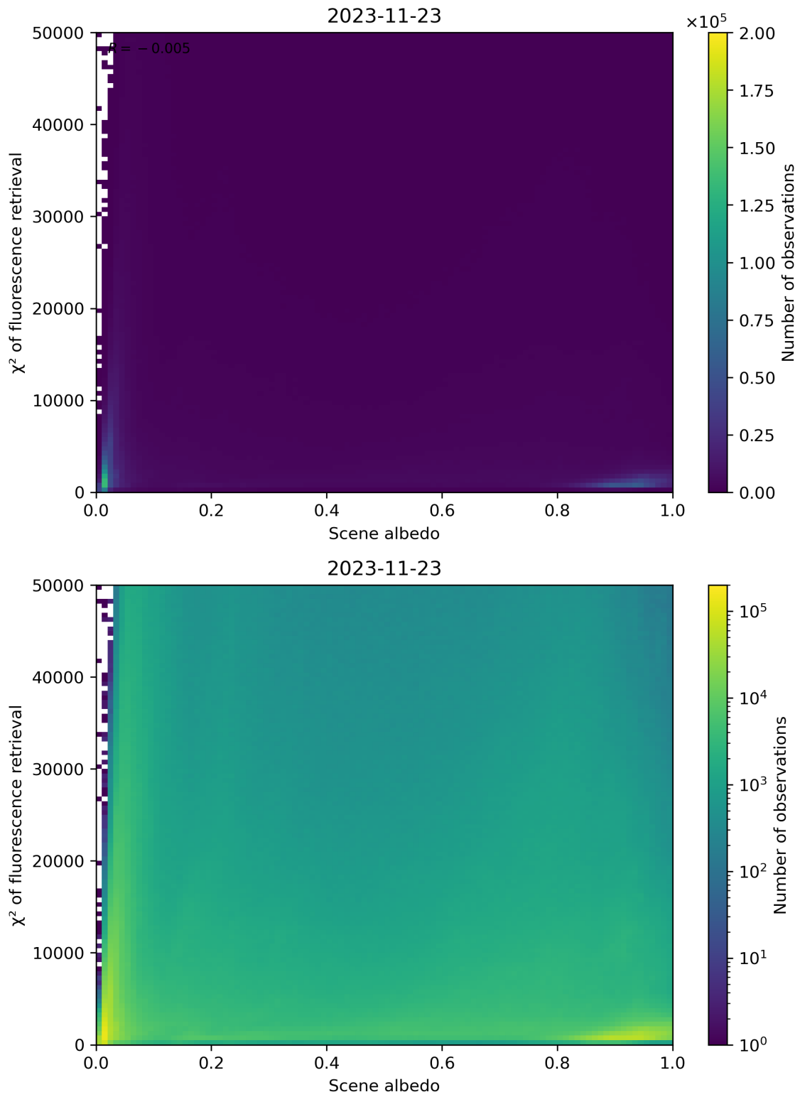
Figure 113: Scatter density plot of “Scene albedo” against “ \chi^2 of fluorescence retrieval” for 2023-11-23 to 2023-11-24.
