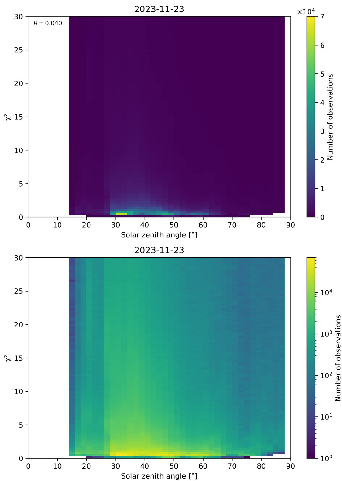
Figure 119: Scatter density plot of “Solar zenith angle” against “ \chi^2 ” for 2023-11-23 to 2023-11-24.
