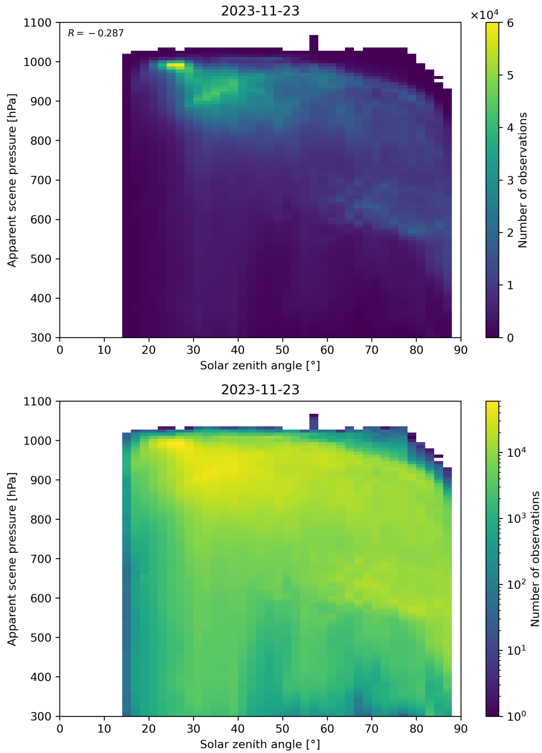
Figure 118: Scatter density plot of “Solar zenith angle” against “Apparent scene pressure” for 2023-11-23 to 2023-11-24.
