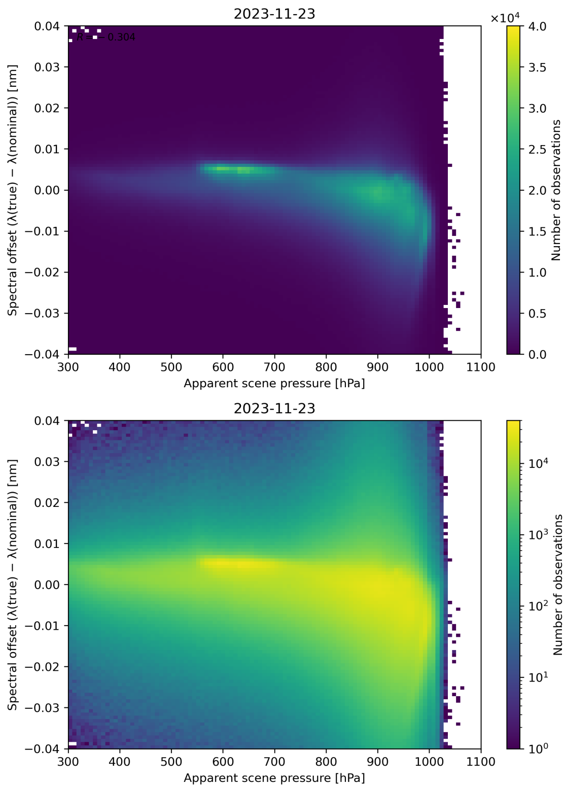
Figure 68: Scatter density plot of “Apparent scene pressure” against “Spectral offset ( \lambda(\text{true}) - \lambda(\text{nominal}) )” for 2023-11-23 to 2023-11-24.
