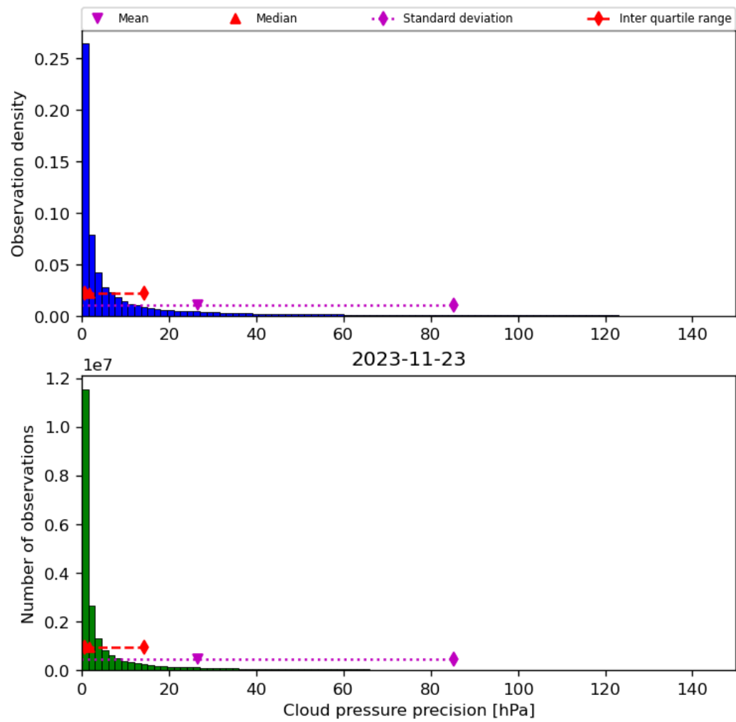
Figure 31: Histogram of “Cloud pressure precision” for 2023-11-23 to 2023-11-24
