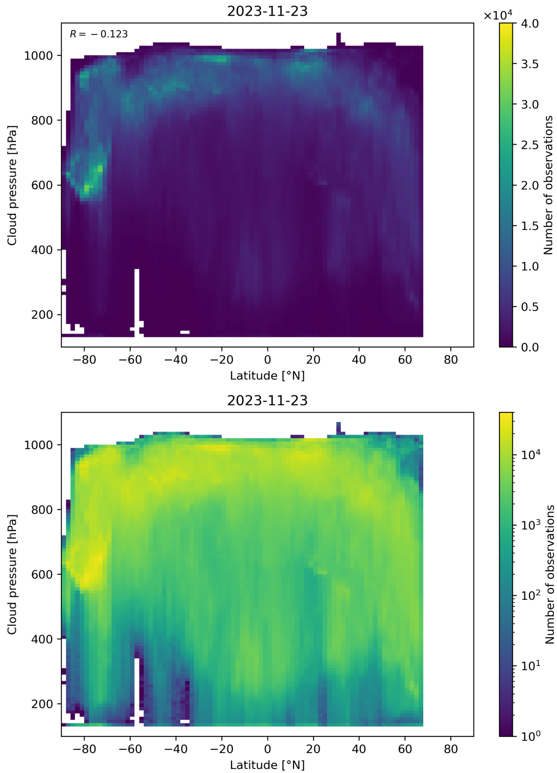
Figure 100: Scatter density plot of “Latitude” against “Cloud pressure” for 2023-11-23 to 2023-11-24.
