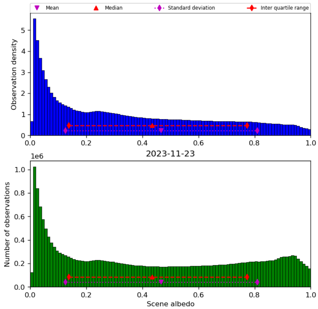
Figure 34: Histogram of “Scene albedo” for 2023-11-23 to 2023-11-24
