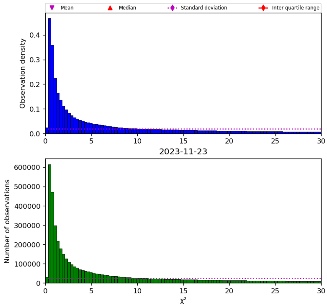
Figure 38: Histogram of “ \chi^2 ” for 2023-11-23 to 2023-11-24
