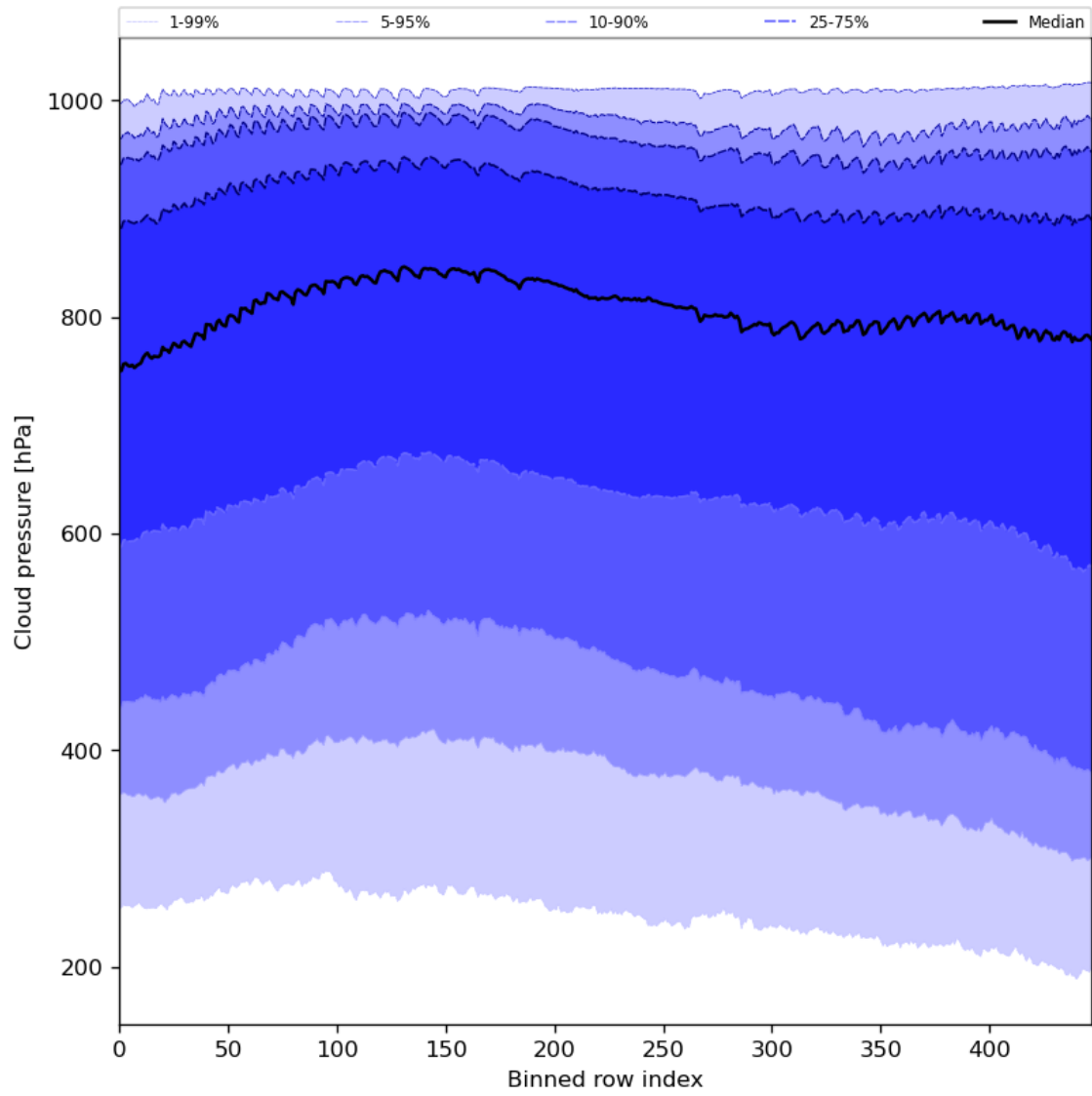
Figure 47: Along track statistics of “Cloud pressure” for 2023-11-23 to 2023-11-24
