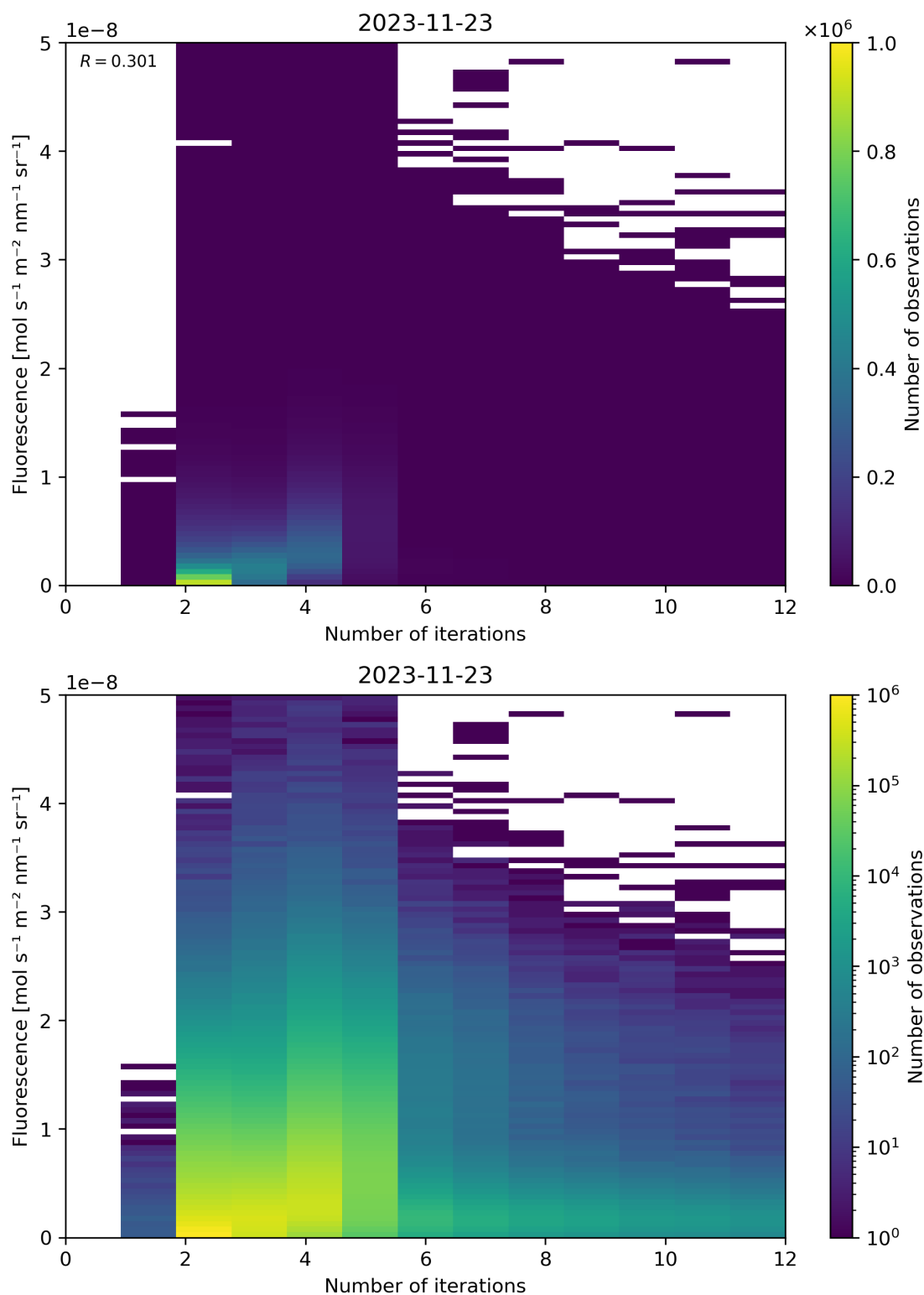
Figure 107: Scatter density plot of “Number of iterations” against “Fluorescence” for 2023-11-23 to 2023-11-24.
