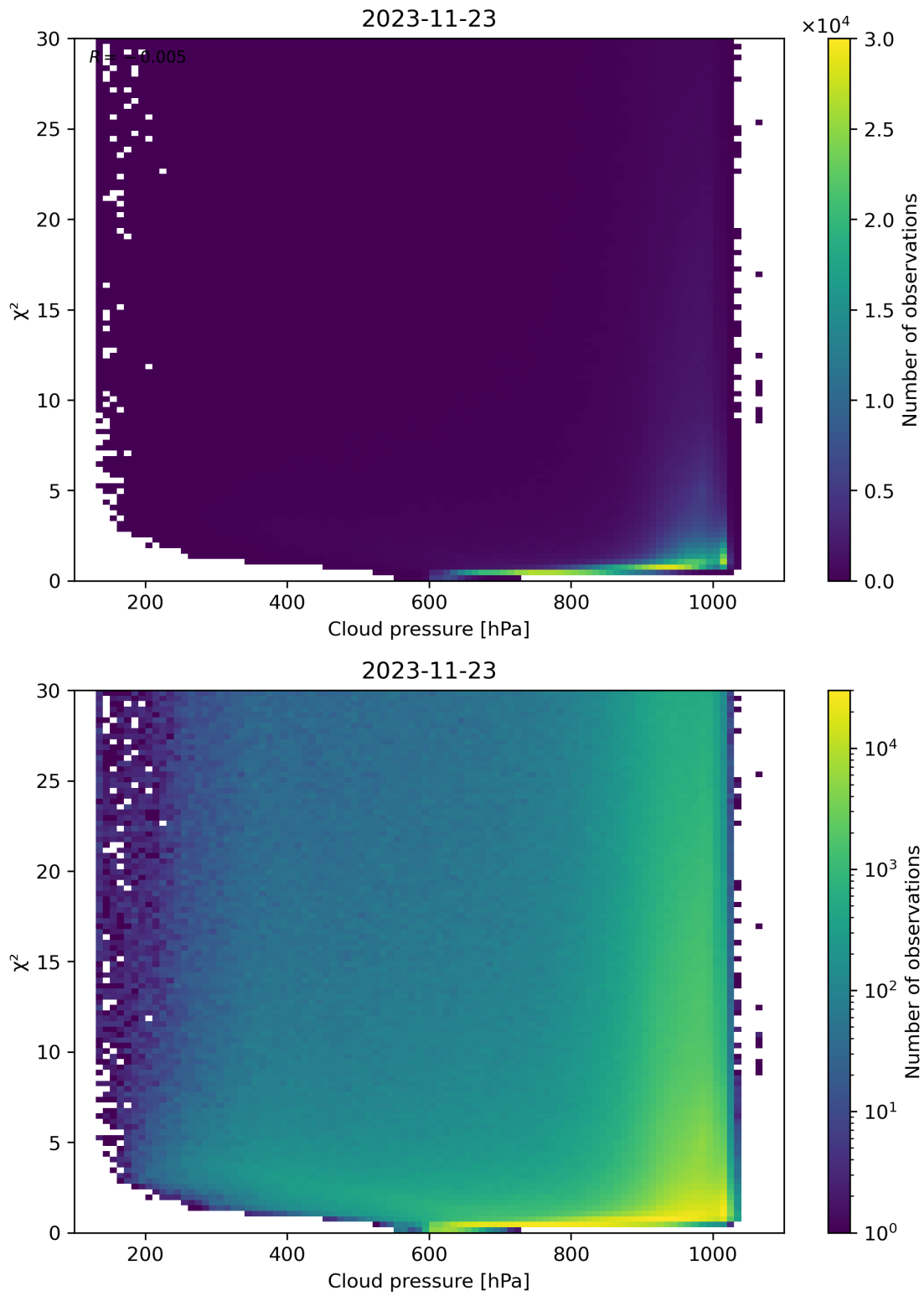
Figure 85: Scatter density plot of “Cloud pressure” against “ \chi^2 ” for 2023-11-23 to 2023-11-24.
