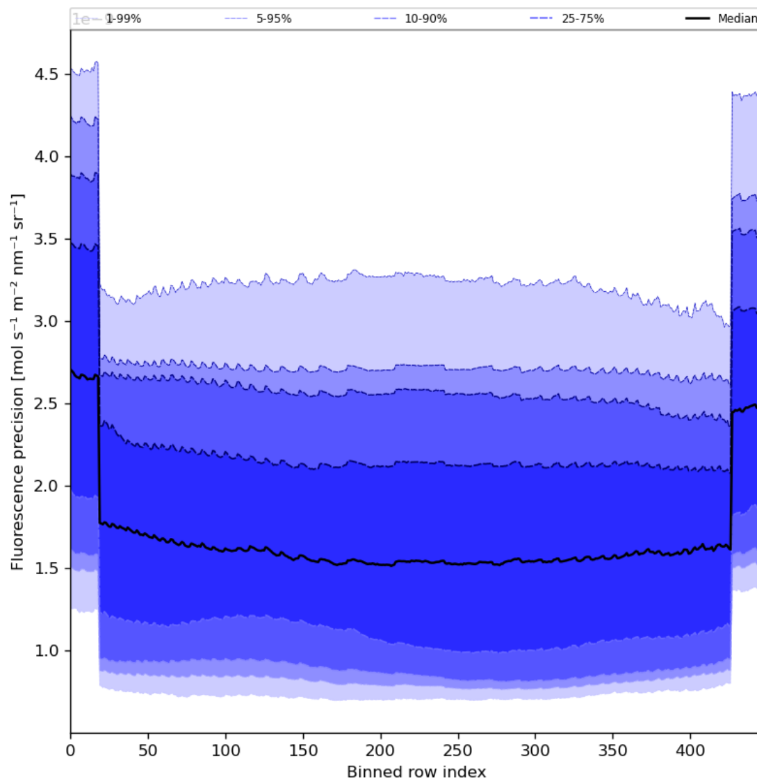
Figure 58: Along track statistics of “Fluorescence precision” for 2023-11-23 to 2023-11-24
