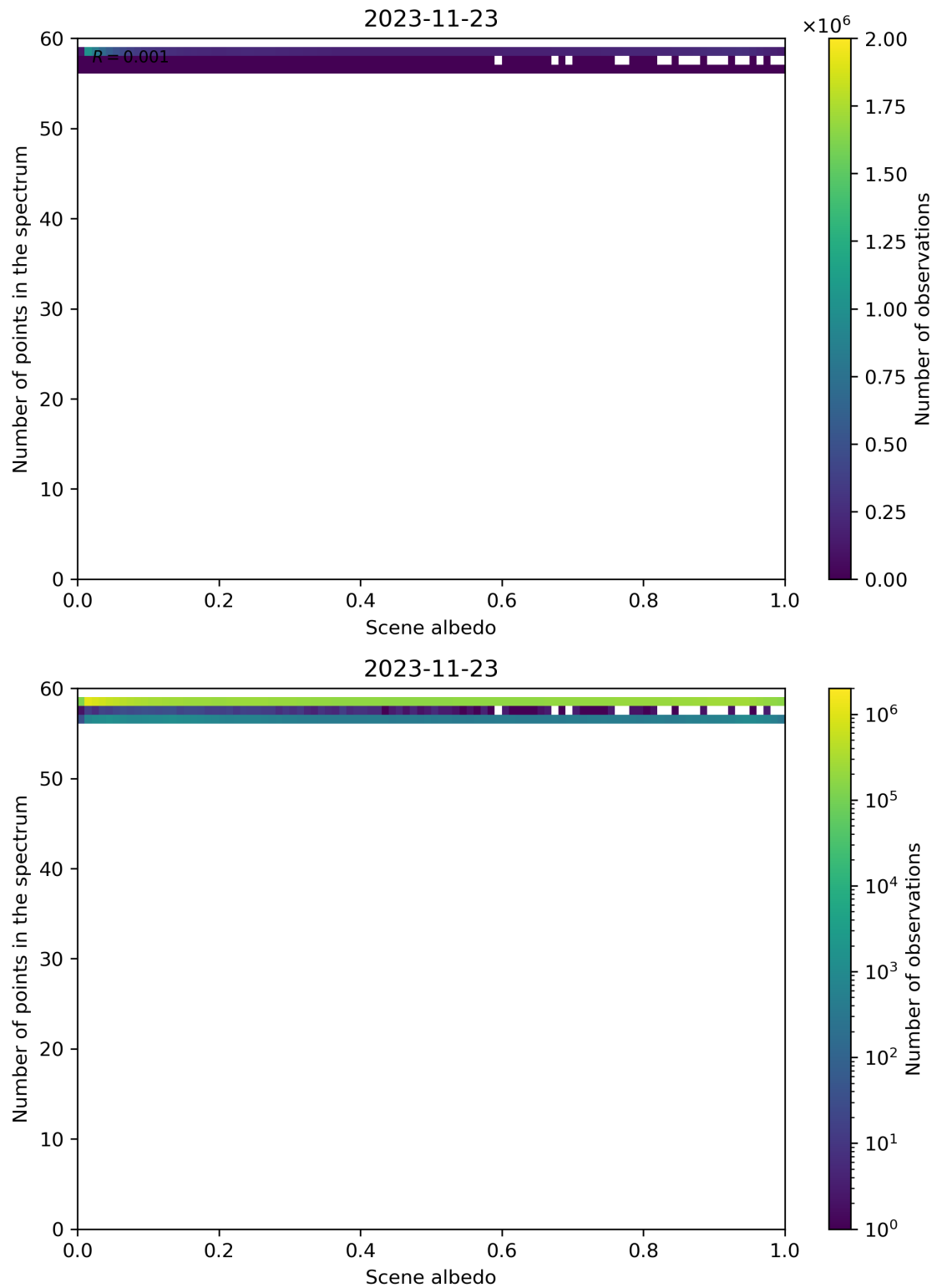
Figure 116: Scatter density plot of “Scene albedo” against “Number of points in the spectrum” for 2023-11-23 to 2023-11-24.
