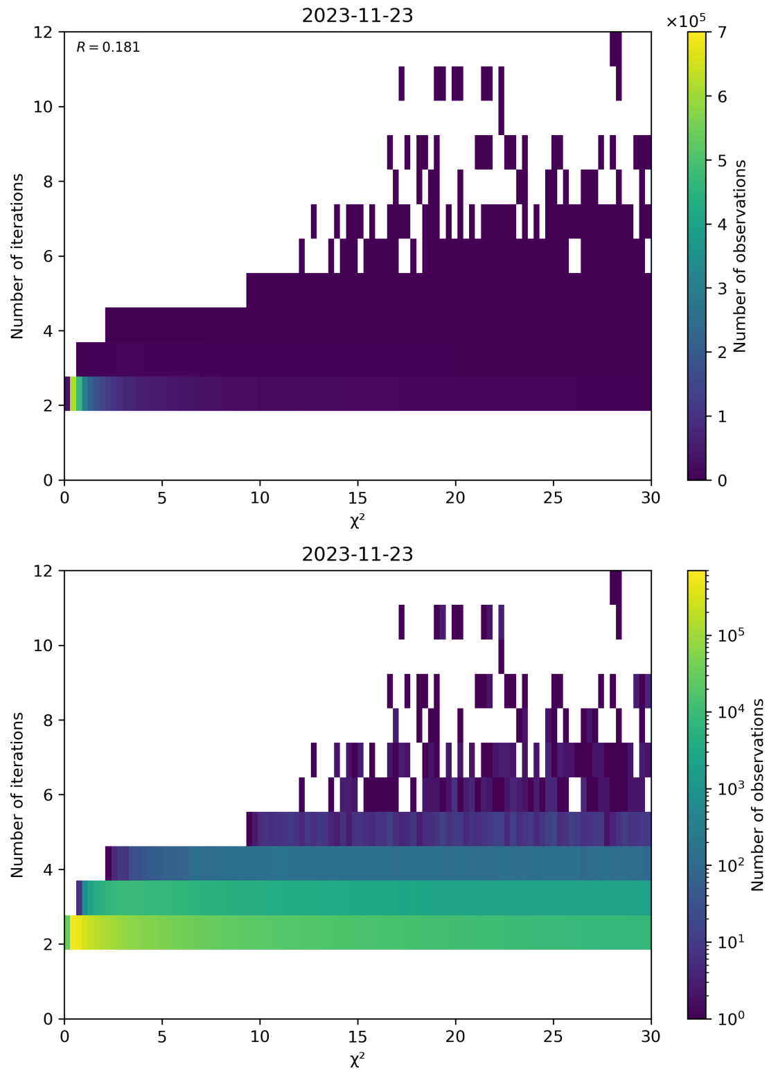
Figure 73: Scatter density plot of “ \chi^2 ” against “Number of iterations” for 2023-11-23 to 2023-11-24.
