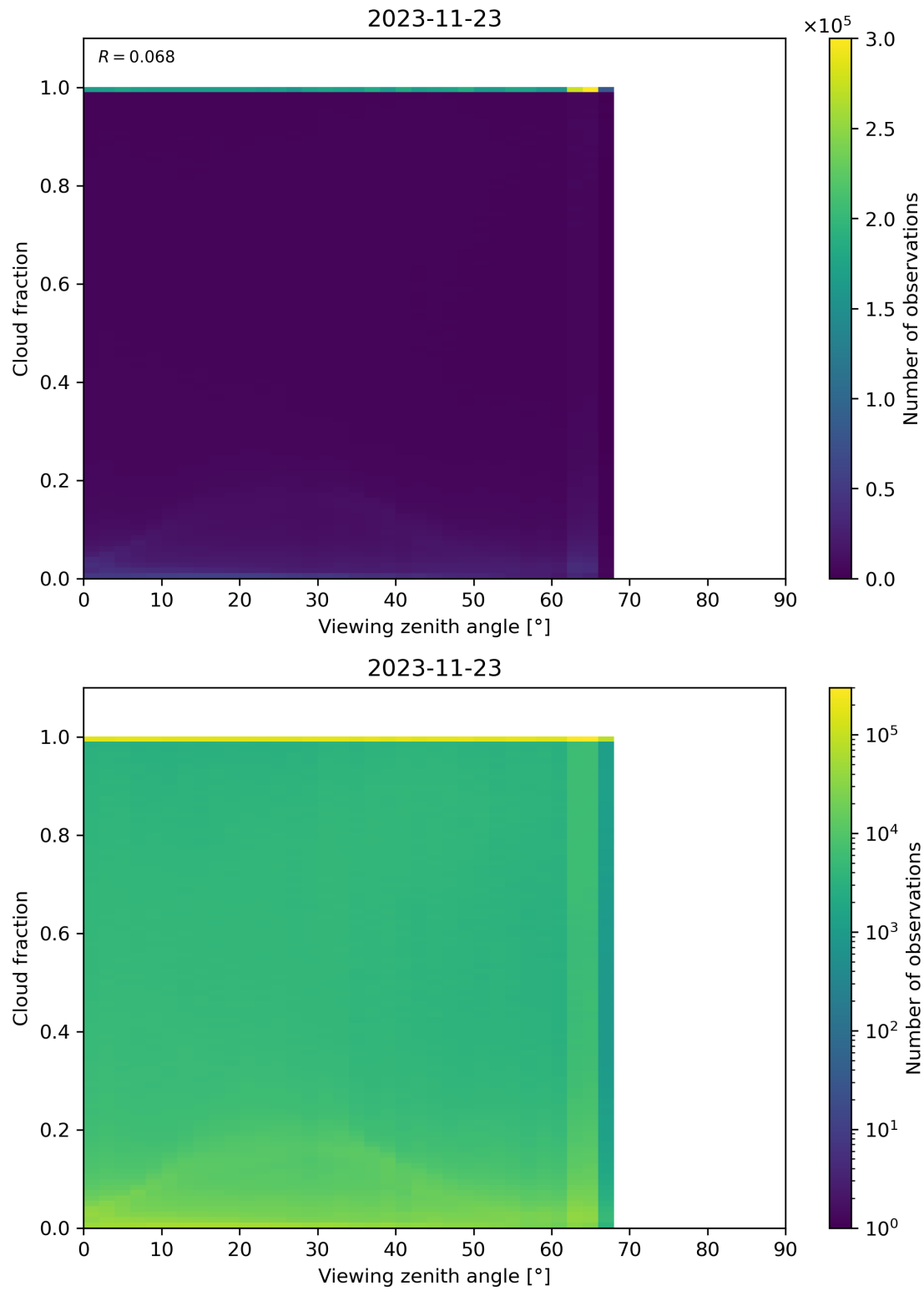
Figure 132: Scatter density plot of “Viewing zenith angle” against “Cloud fraction” for 2023-11-23 to 2023-11-24.
