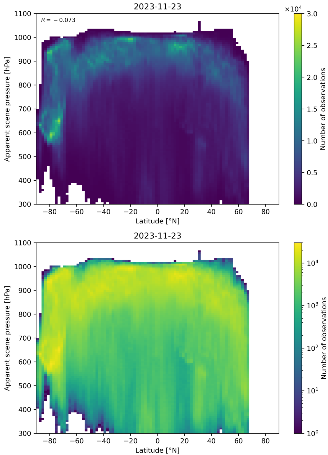
Figure 96: Scatter density plot of “Latitude” against “Apparent scene pressure” for 2023-11-23 to 2023-11-24.
