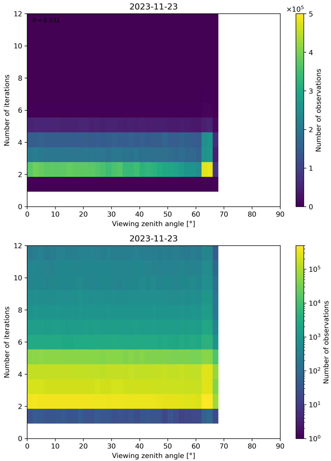
Figure 136: Scatter density plot of “Viewing zenith angle” against “Number of iterations” for 2023-11-23 to 2023-11-24.
