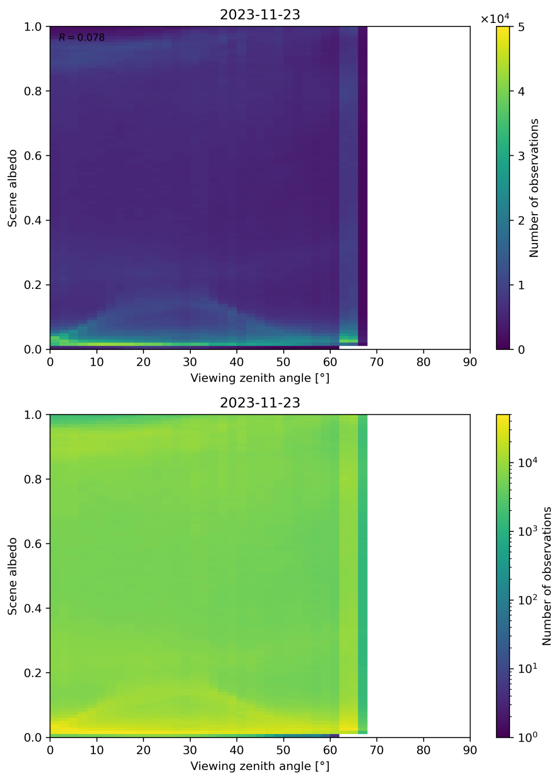
Figure 138: Scatter density plot of “Viewing zenith angle” against “Scene albedo” for 2023-11-23 to 2023-11-24.
