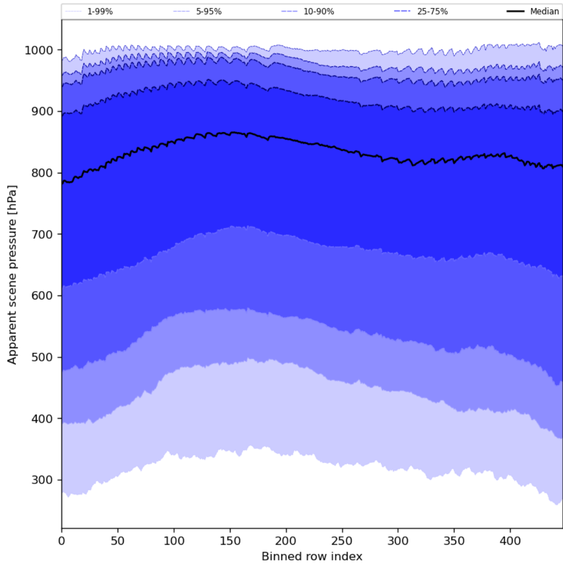
Figure 53: Along track statistics of “Apparent scene pressure” for 2023-11-23 to 2023-11-24
