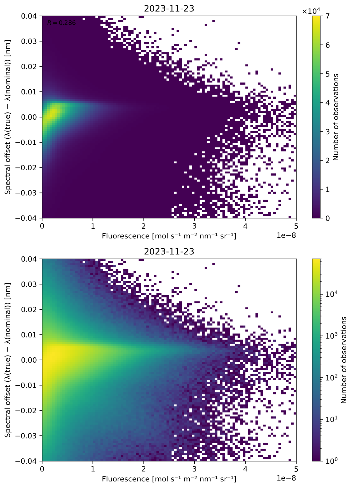
Figure 95: Scatter density plot of “Fluorescence” against “Spectral offset ( \lambda(\text{true}) - \lambda(\text{nominal}) )” for 2023-11-23 to 2023-11-24.
