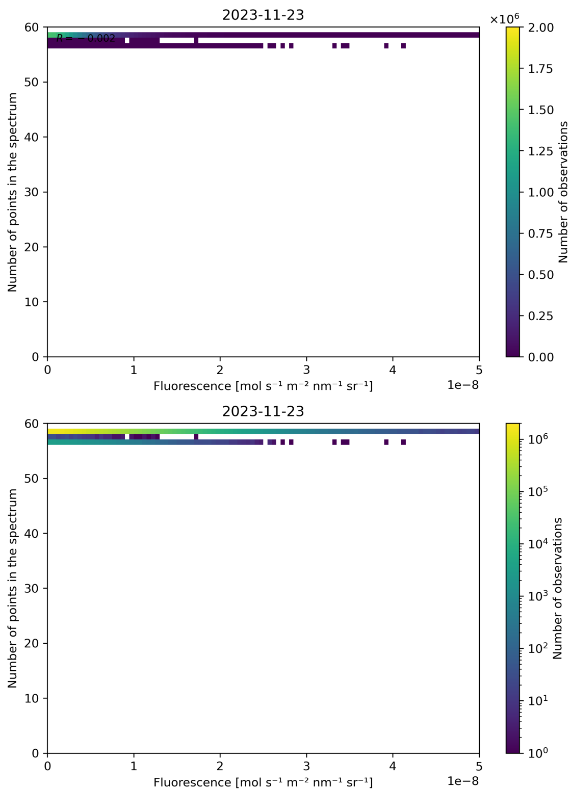
Figure 94: Scatter density plot of “Fluorescence” against “Number of points in the spectrum” for 2023-11-23 to 2023-11-24.
