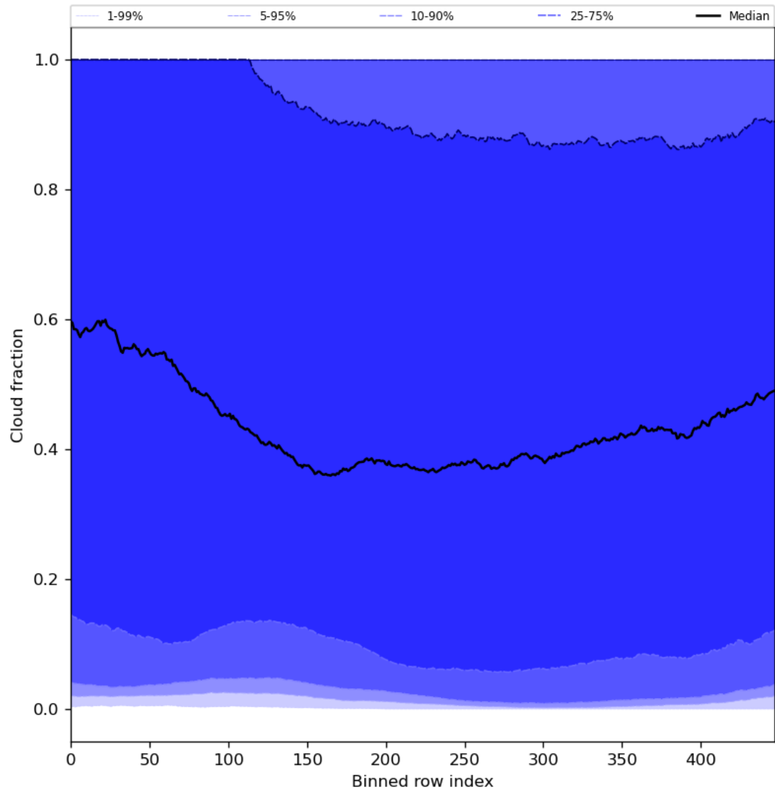
Figure 49: Along track statistics of “Cloud fraction” for 2023-11-23 to 2023-11-24
