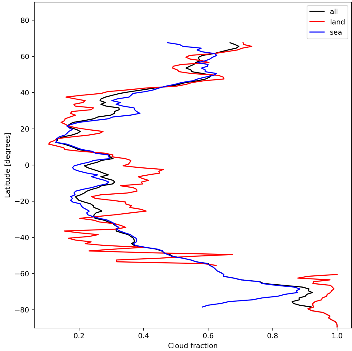
Figure 15: Zonal average of “Cloud fraction” for 2023-11-23 to 2023-11-24.
