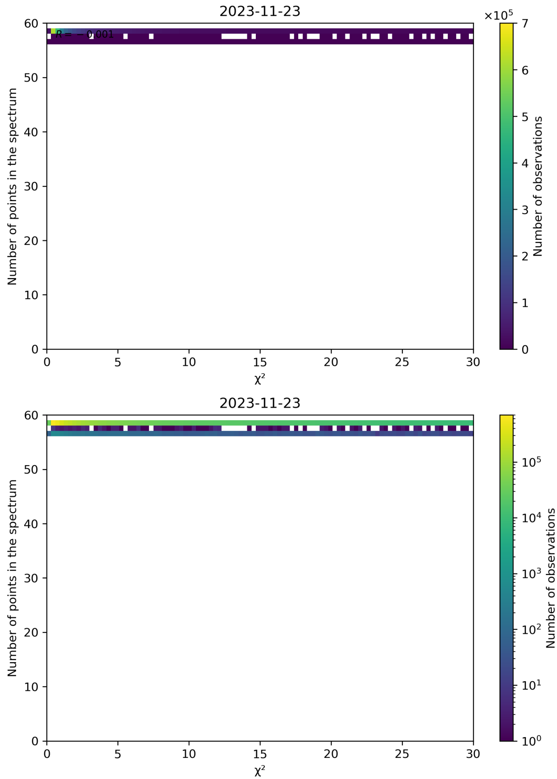
Figure 74: Scatter density plot of " \chi^2 " against "Number of points in the spectrum" for 2023-11-23 to 2023-11-24.
