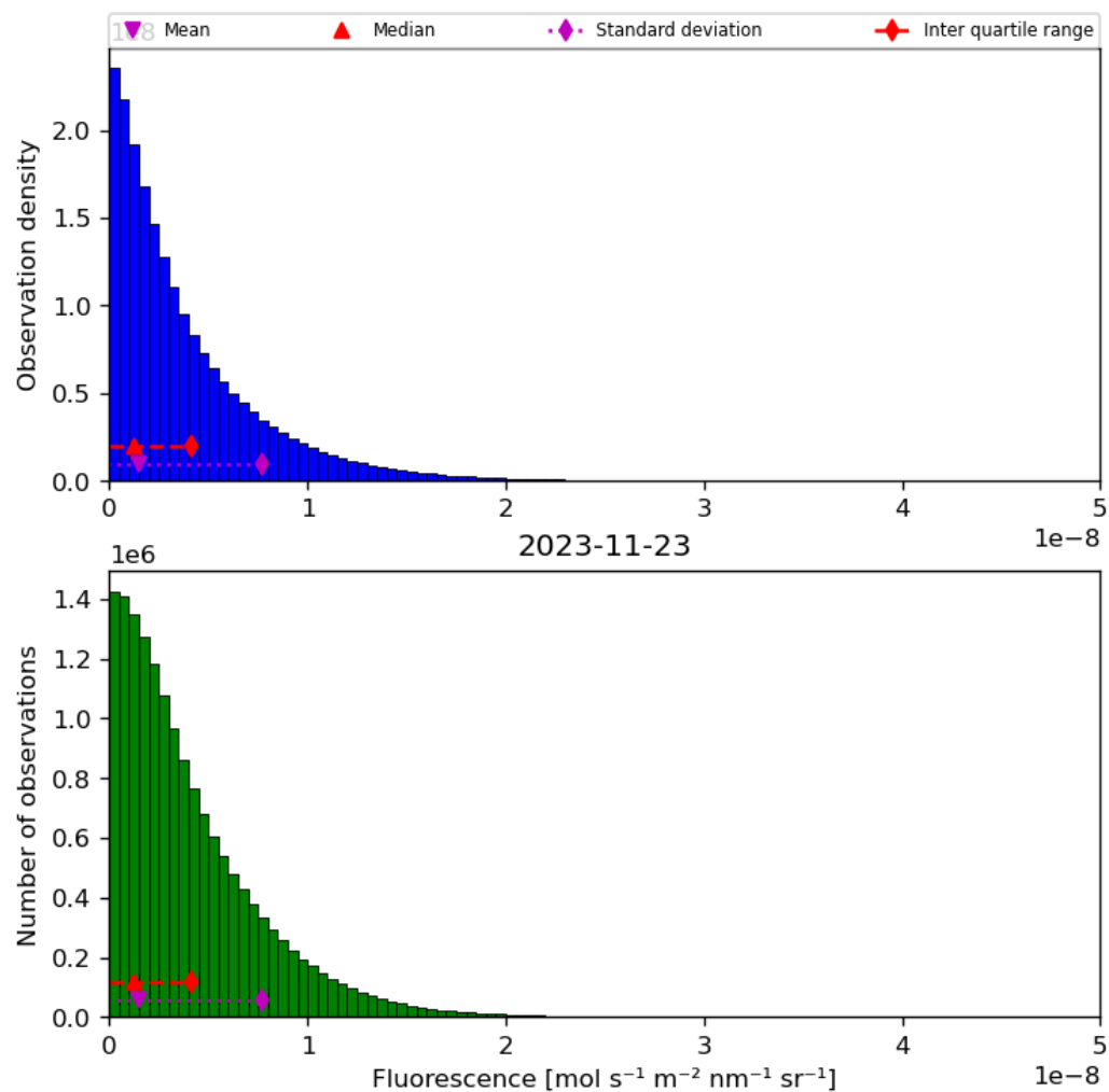
Figure 40: Histogram of “Fluorescence” for 2023-11-23 to 2023-11-24
