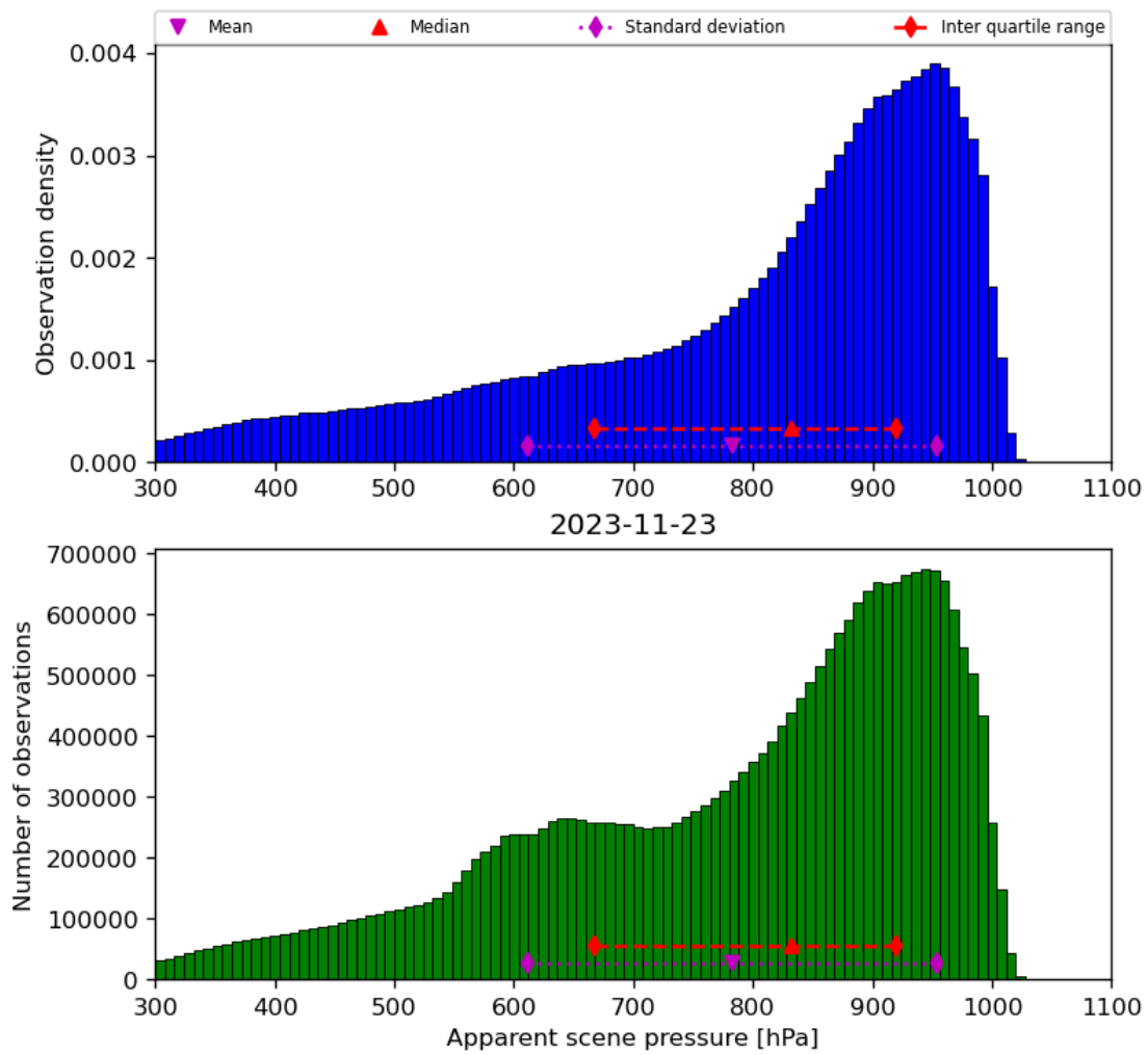
Figure 36: Histogram of “Apparent scene pressure” for 2023-11-23 to 2023-11-24
