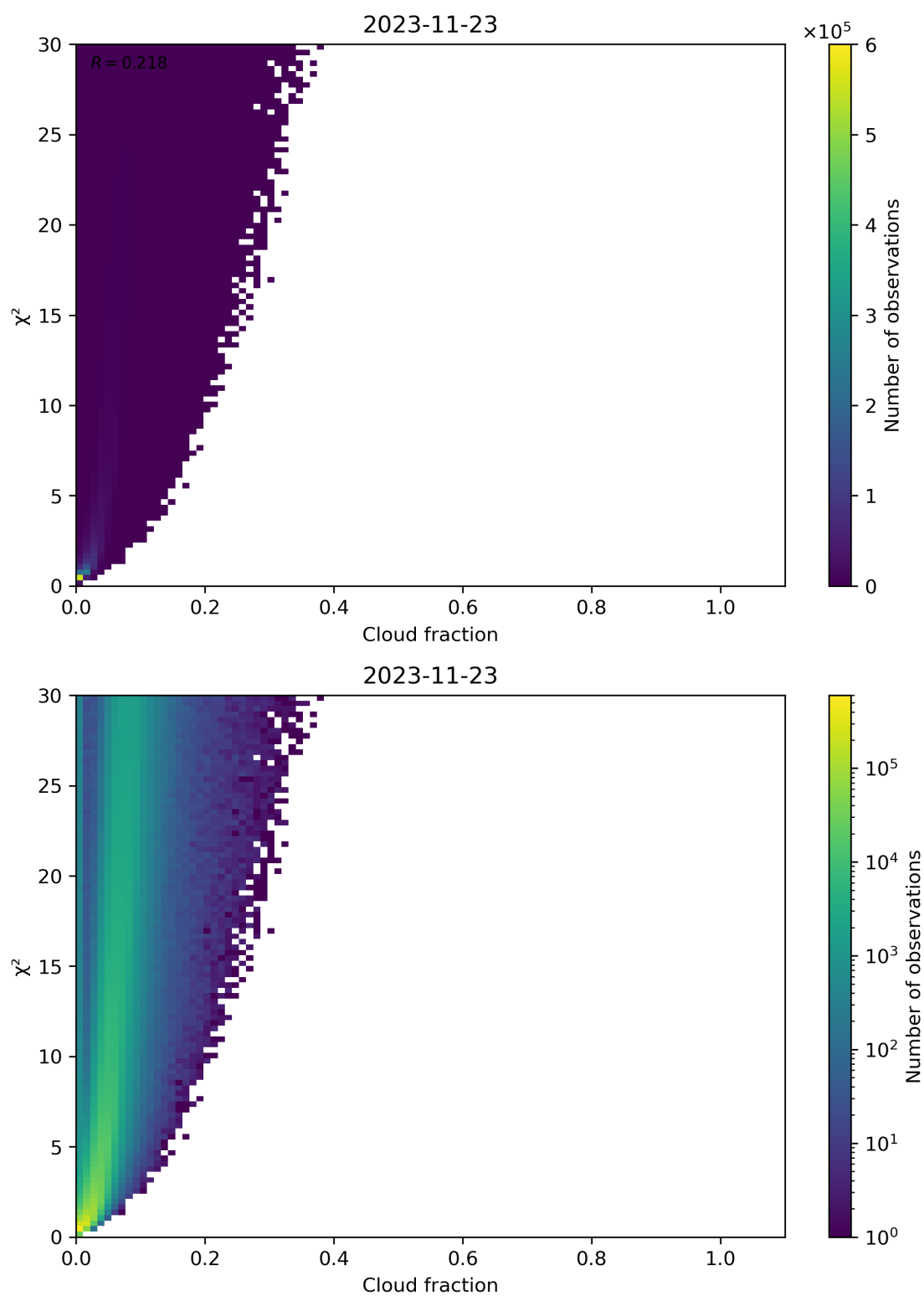
Figure 77: Scatter density plot of “Cloud fraction” against “ \chi^2 ” for 2023-11-23 to 2023-11-24.
