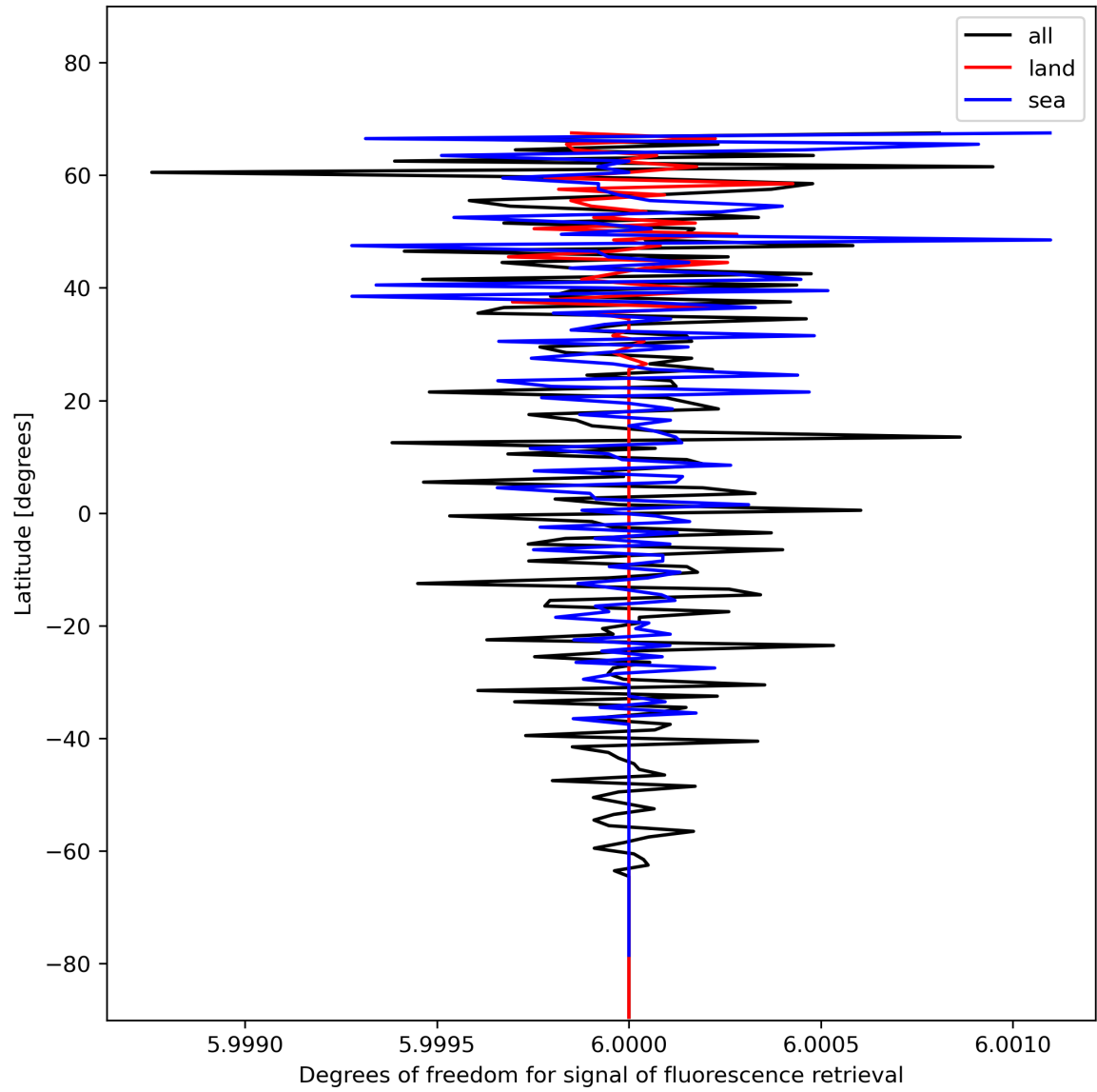
Figure 26: Zonal average of “Degrees of freedom for signal of fluorescence retrieval” for 2023-11-23 to 2023-11-24.
