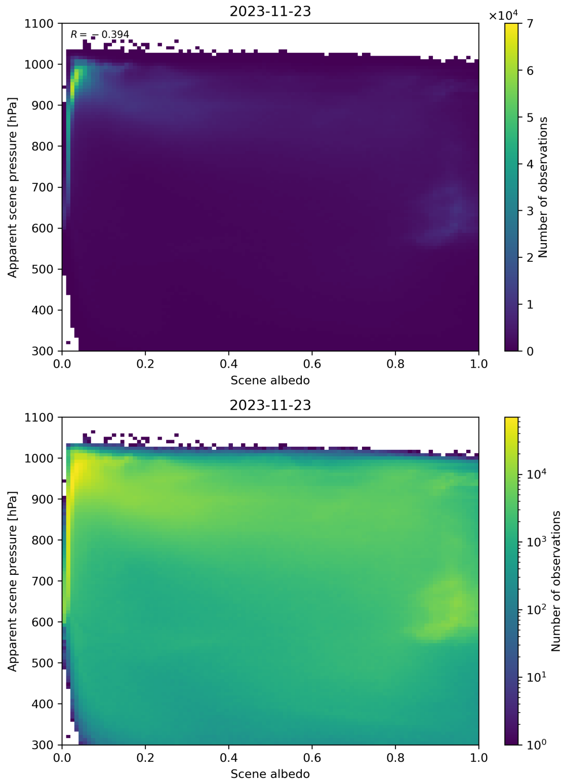
Figure 111: Scatter density plot of “Scene albedo” against “Apparent scene pressure” for 2023-11-23 to 2023-11-24.
