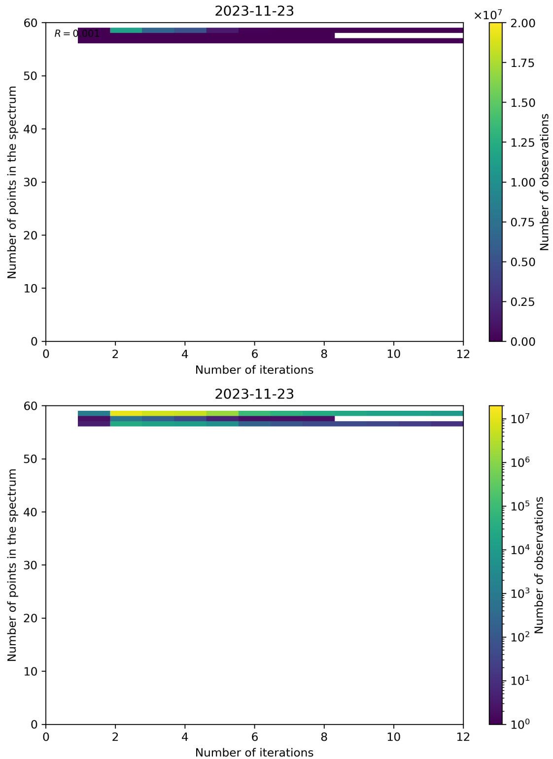
Figure 108: Scatter density plot of “Number of iterations” against “Number of points in the spectrum” for 2023-11-23 to 2023-11-24.
