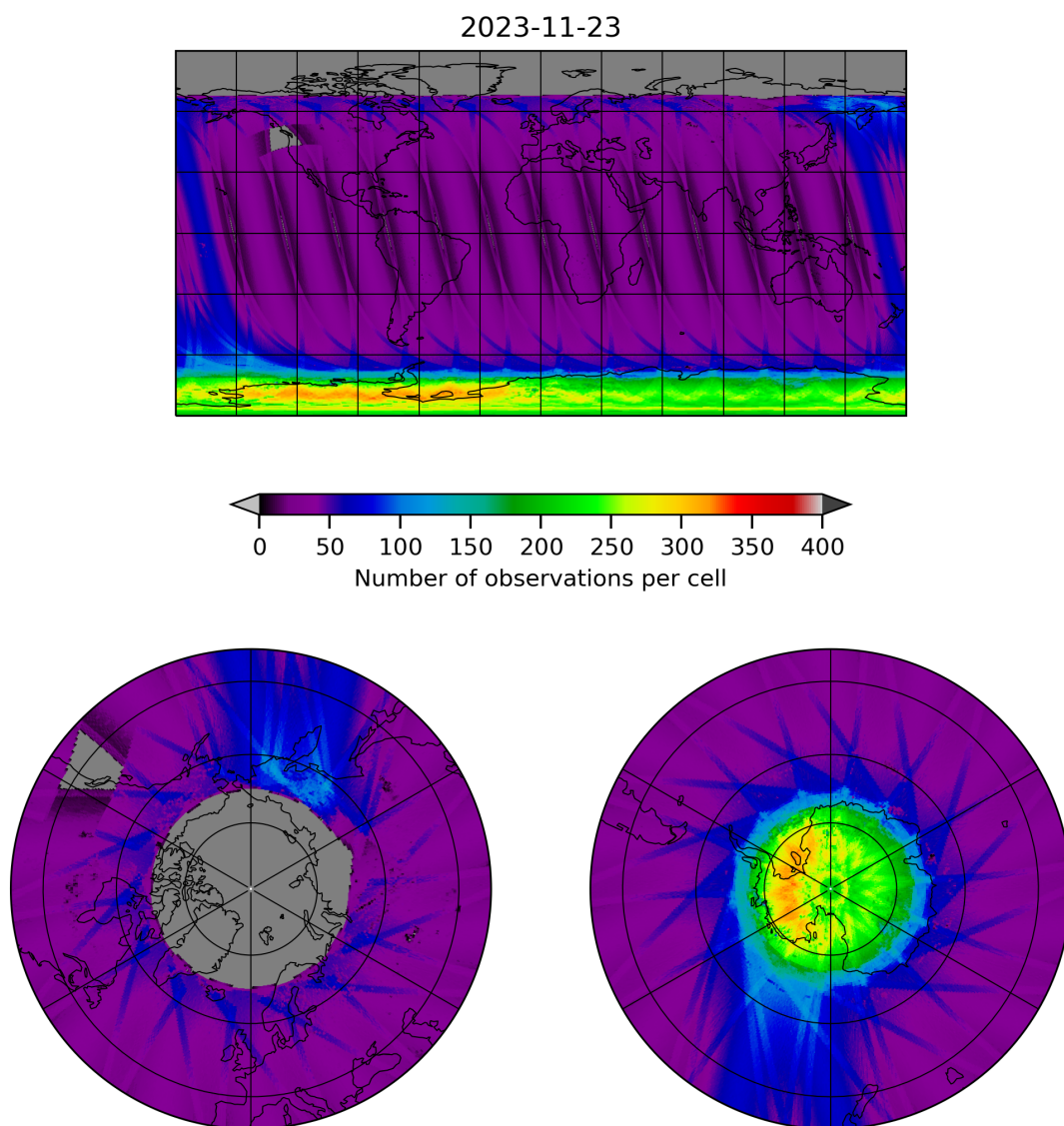
Figure 11: Map of the number of observations for 2023-11-23 to 2023-11-24
