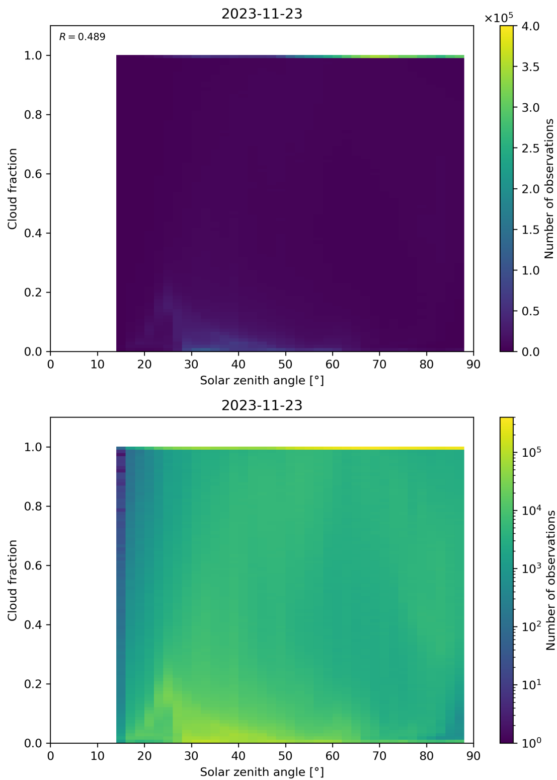
Figure 121: Scatter density plot of “Solar zenith angle” against “Cloud fraction” for 2023-11-23 to 2023-11-24.
