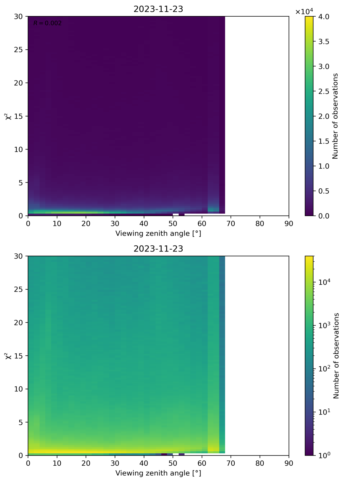
Figure 130: Scatter density plot of “Viewing zenith angle” against “ \chi^2 ” for 2023-11-23 to 2023-11-24.
