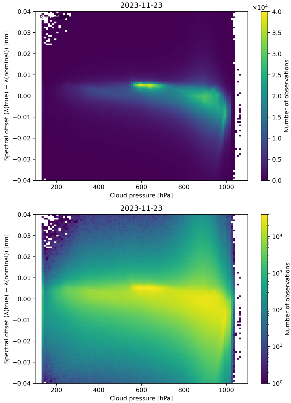
Figure 92: Scatter density plot of “Cloud pressure” against “Spectral offset ( \lambda(\text{true}) - \lambda(\text{nominal}) )” for 2023-11-23 to 2023-11-24.
