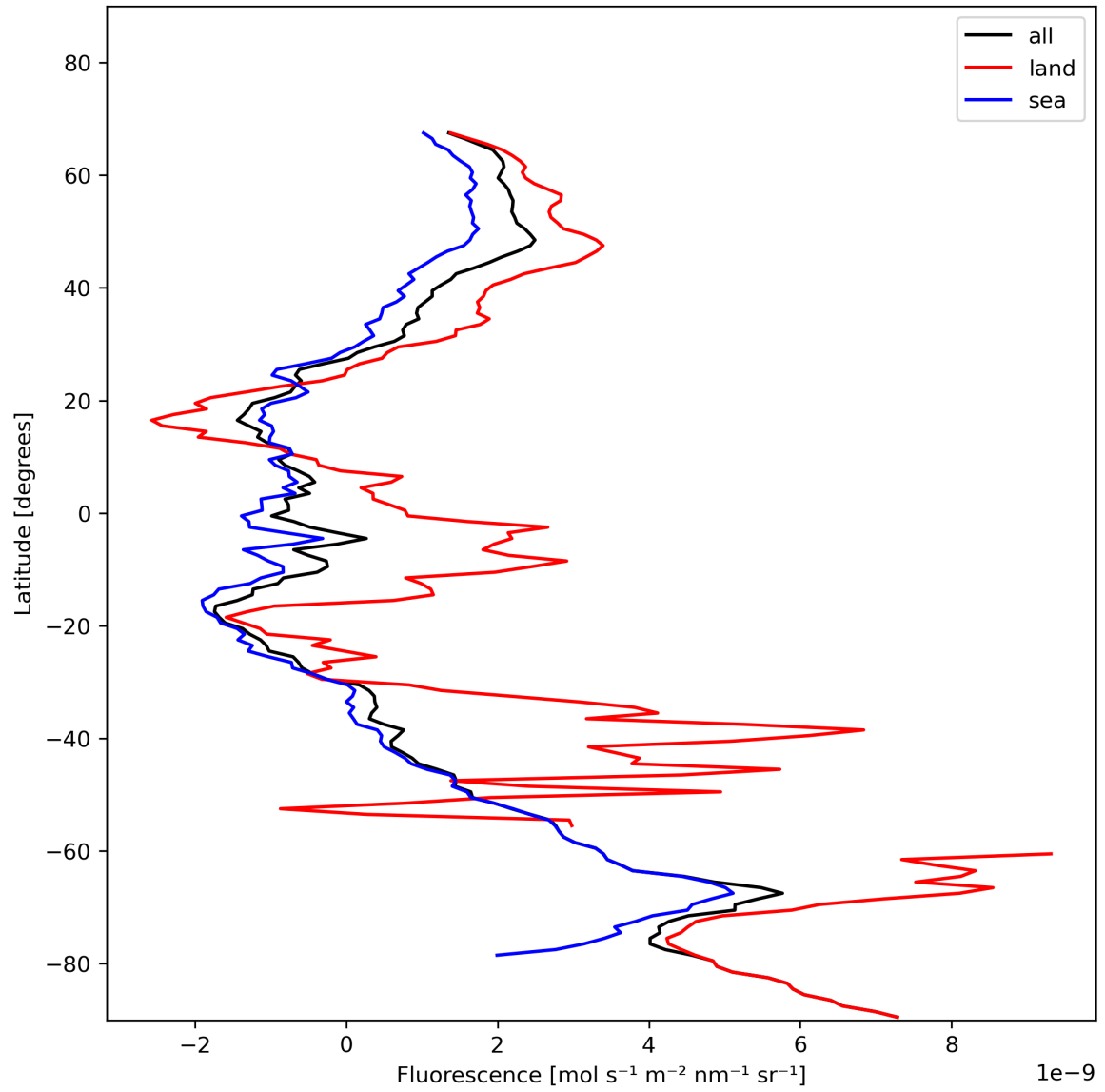
Figure 23: Zonal average of “Fluorescence” for 2023-11-23 to 2023-11-24.
