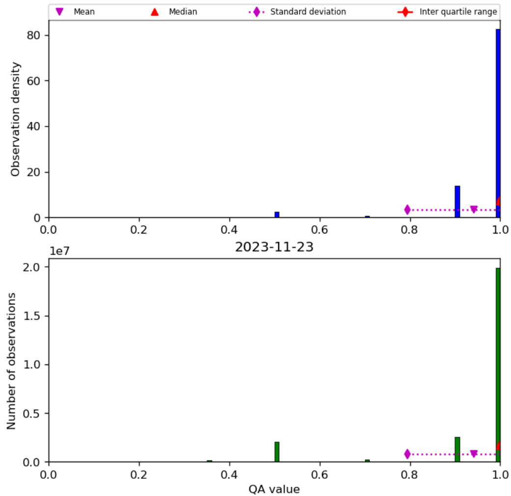
Figure 29: Histogram of “QA value” for 2023-11-23 to 2023-11-24
