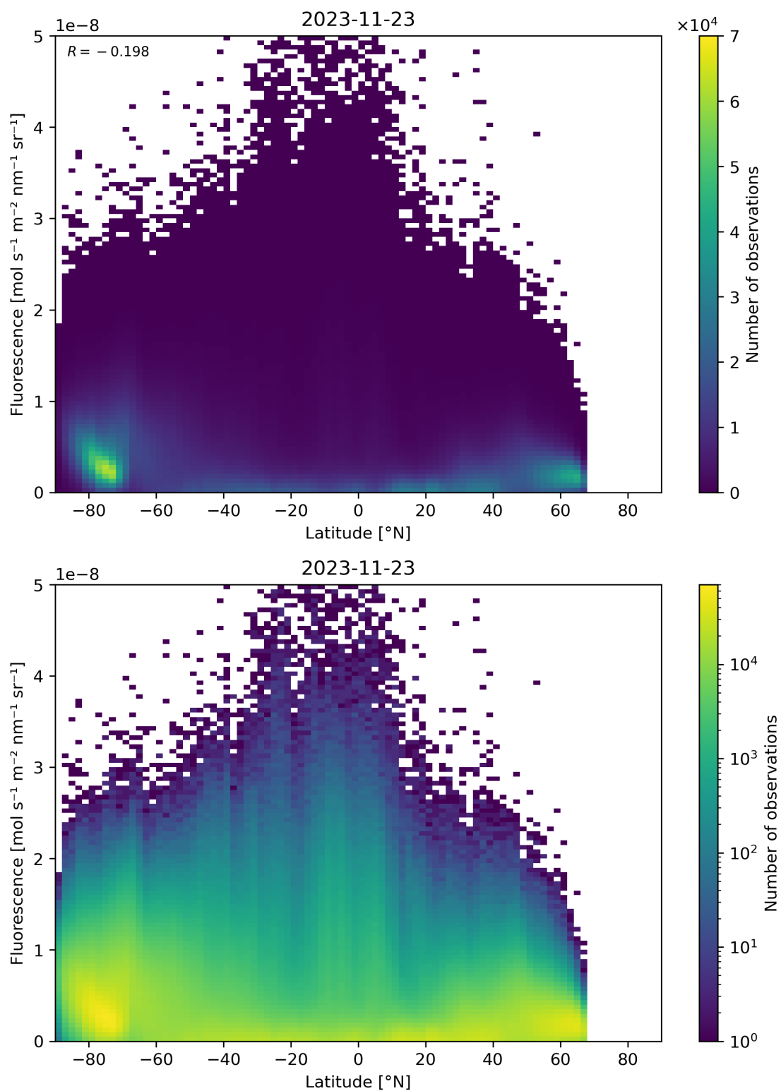
Figure 101: Scatter density plot of “Latitude” against “Fluorescence” for 2023-11-23 to 2023-11-24.
