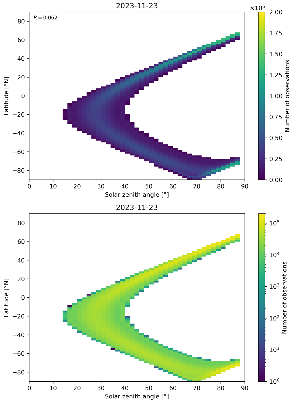
Figure 124: Scatter density plot of “Solar zenith angle” against “Latitude” for 2023-11-23 to 2023-11-24.
