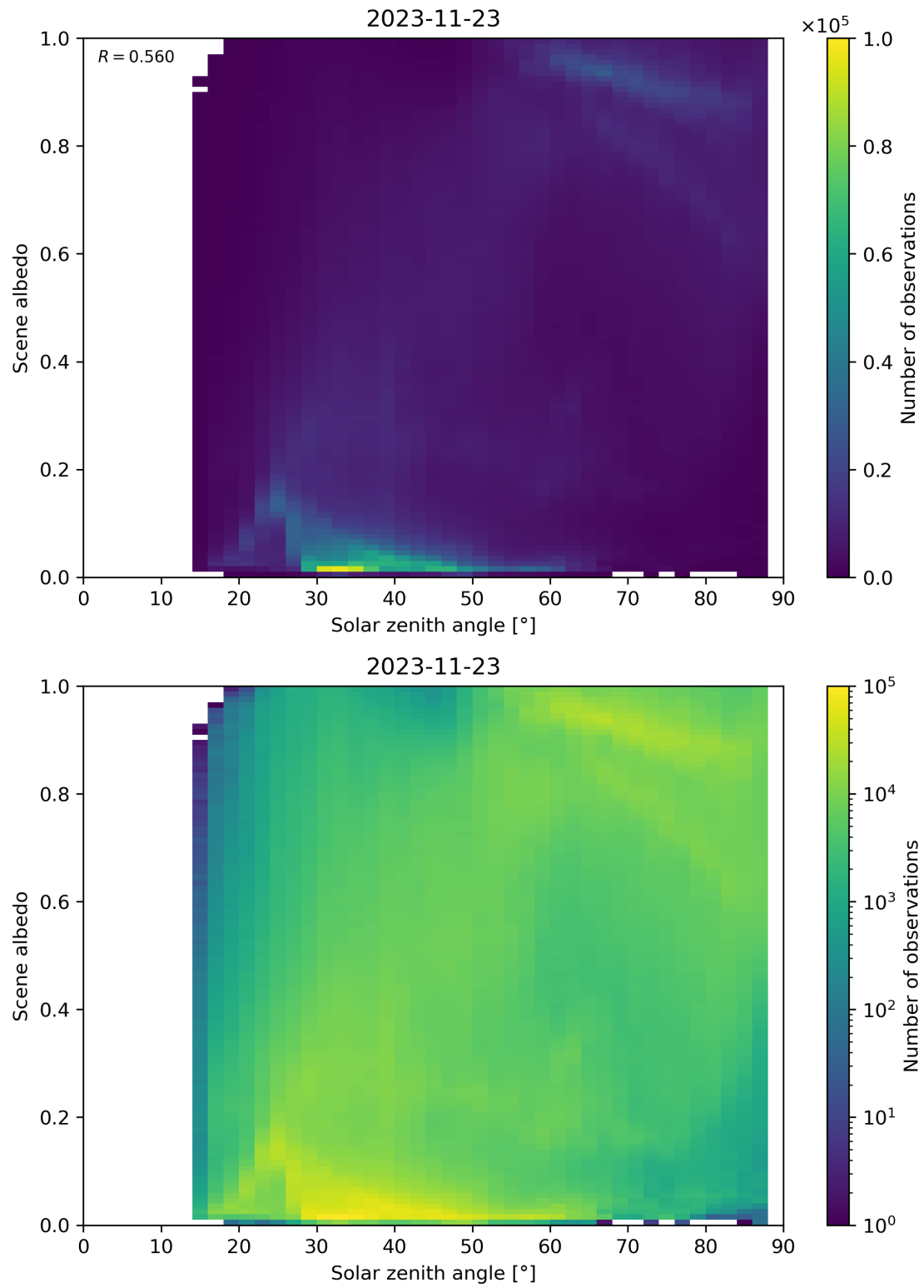
Figure 127: Scatter density plot of “Solar zenith angle” against “Scene albedo” for 2023-11-23 to 2023-11-24.
