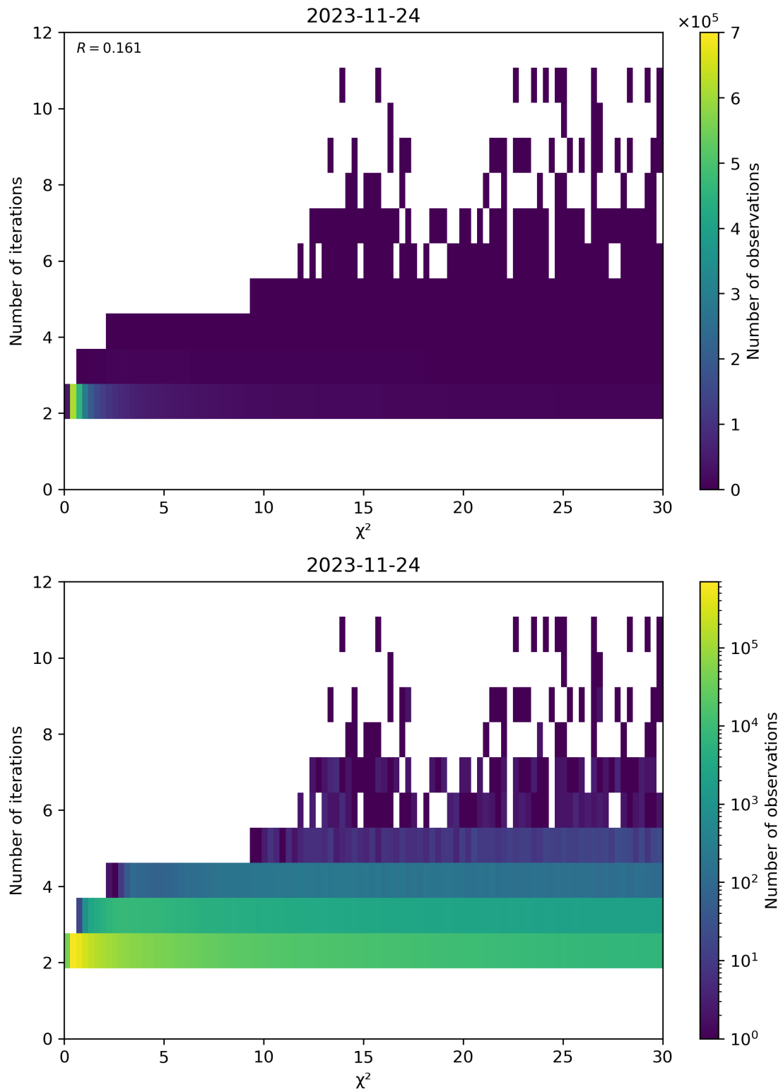
Figure 73: Scatter density plot of “ \chi^2 ” against “Number of iterations” for 2023-11-23 to 2023-11-25.
