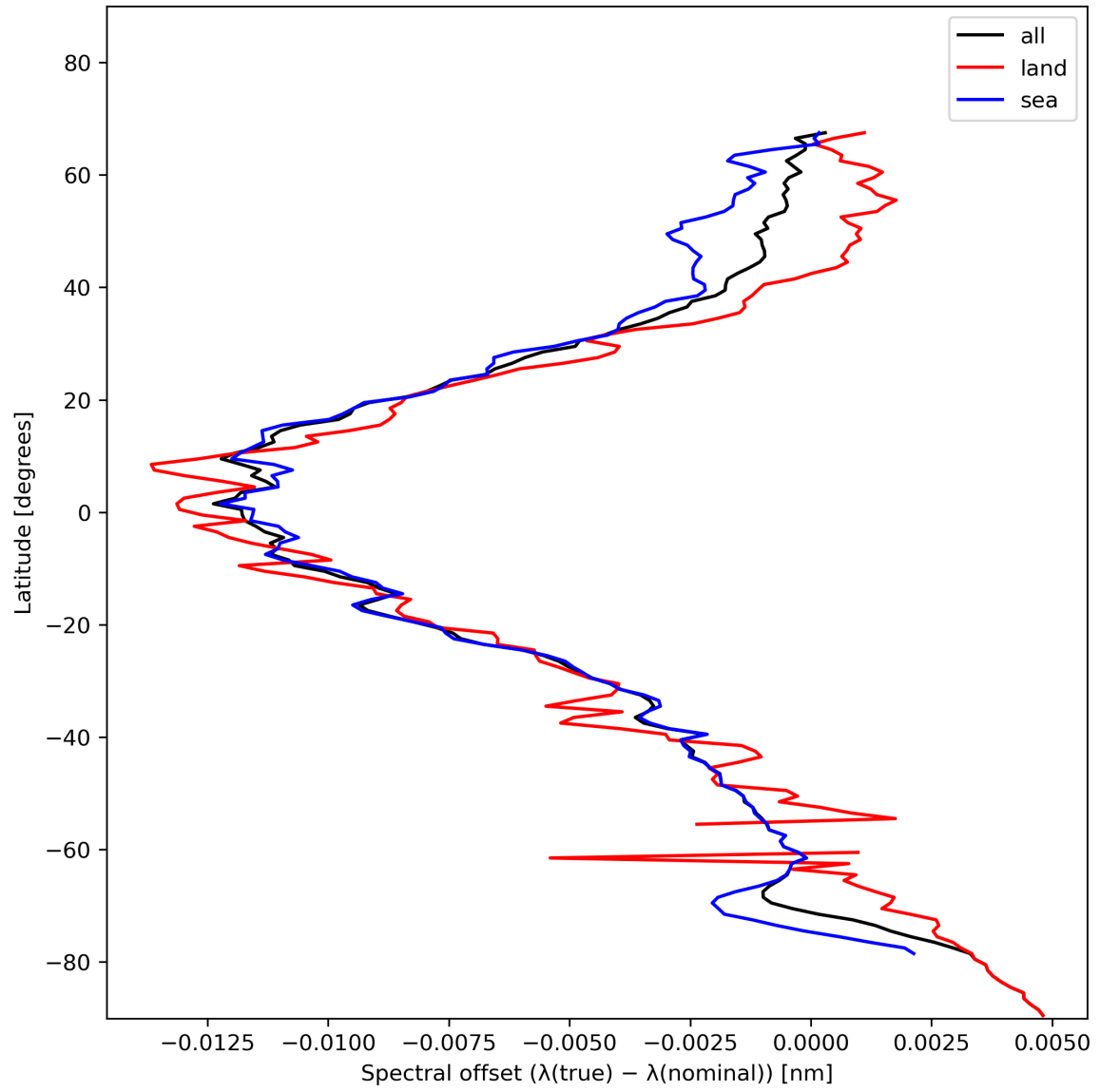
Figure 28: Zonal average of “Spectral offset ( \lambda(\text{true}) - \lambda(\text{nominal}) )” for 2023-11-23 to 2023-11-25.
