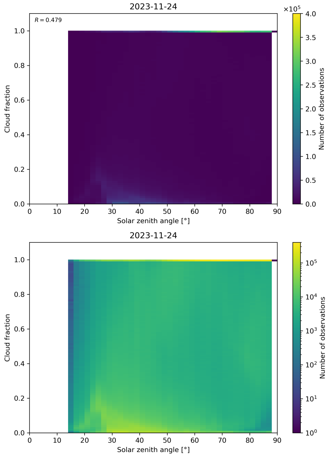
Figure 121: Scatter density plot of “Solar zenith angle” against “Cloud fraction” for 2023-11-23 to 2023-11-25.
