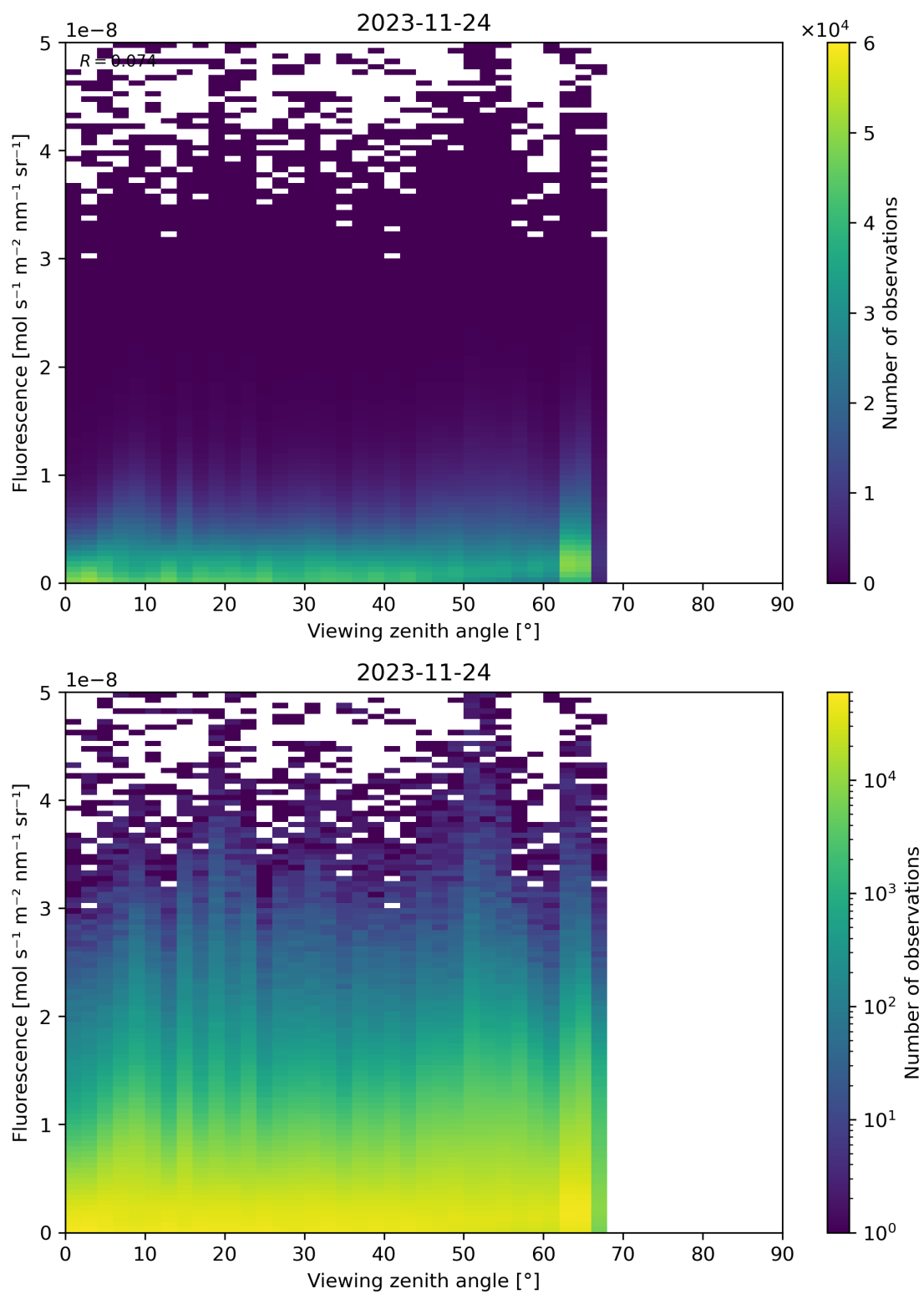
Figure 134: Scatter density plot of “Viewing zenith angle” against “Fluorescence” for 2023-11-23 to 2023-11-25.
