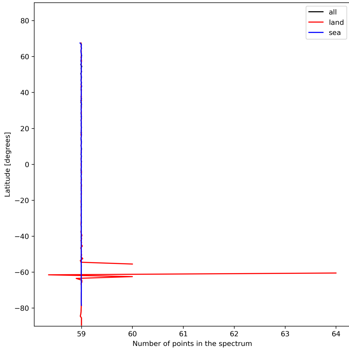
Figure 27: Zonal average of “Number of points in the spectrum” for 2023-11-23 to 2023-11-25.
