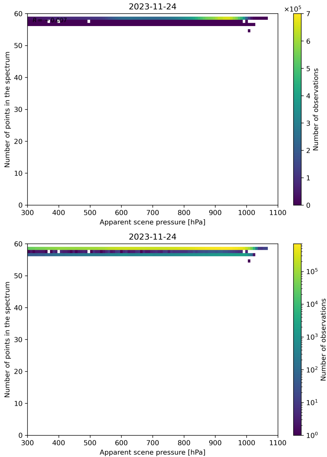
Figure 67: Scatter density plot of “Apparent scene pressure” against “Number of points in the spectrum” for 2023-11-23 to 2023-11-25.
