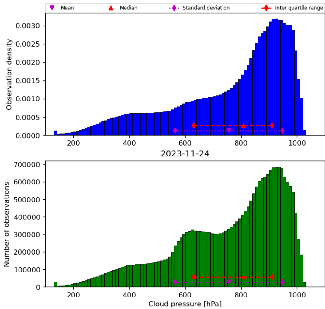
Figure 30: Histogram of “Cloud pressure” for 2023-11-23 to 2023-11-25
