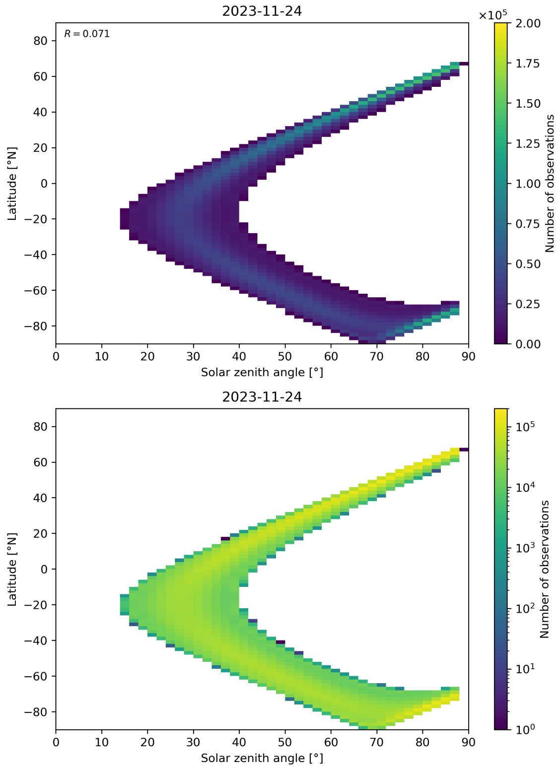
Figure 124: Scatter density plot of “Solar zenith angle” against “Latitude” for 2023-11-23 to 2023-11-25.
