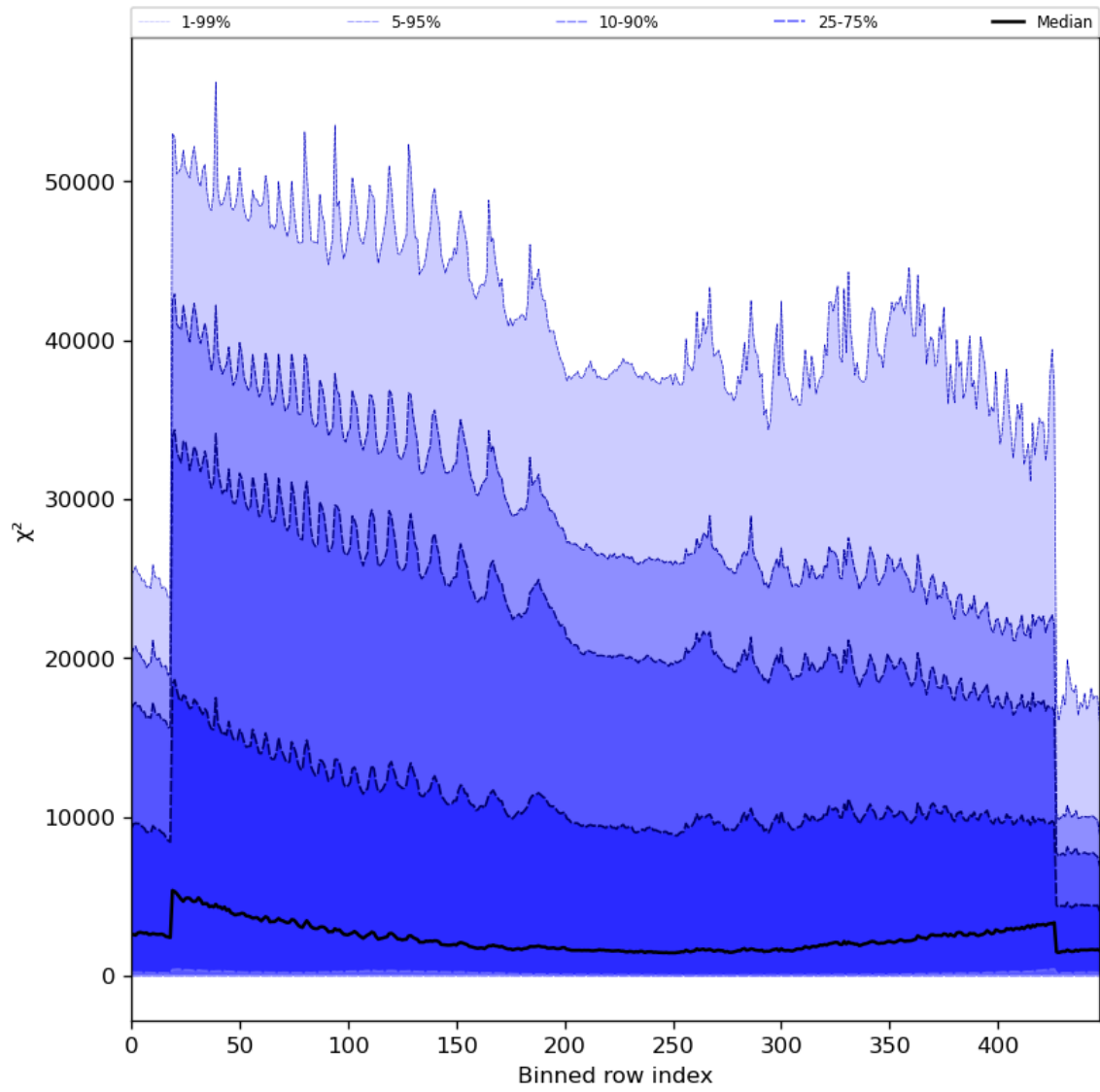
Figure 55: Along track statistics of “ \chi^2 ” for 2023-11-23 to 2023-11-25
