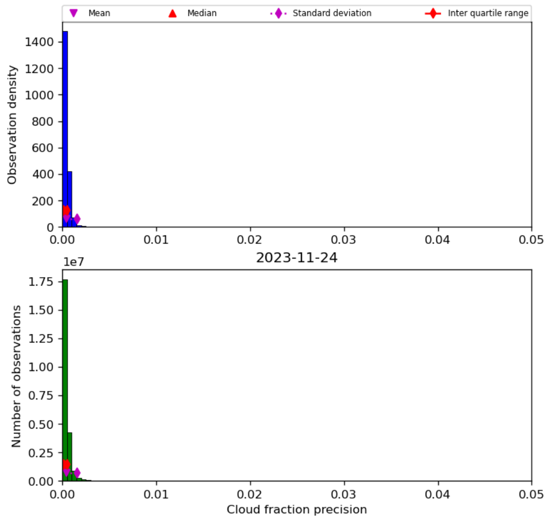
Figure 33: Histogram of “Cloud fraction precision” for 2023-11-23 to 2023-11-25
