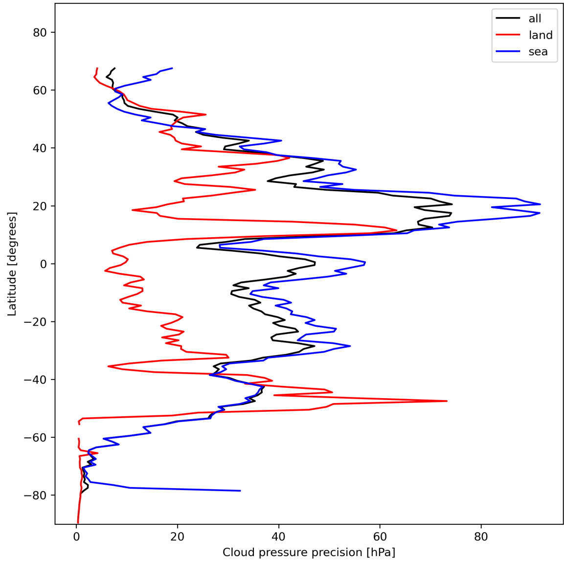
Figure 14: Zonal average of “Cloud pressure precision” for 2023-11-23 to 2023-11-25.
