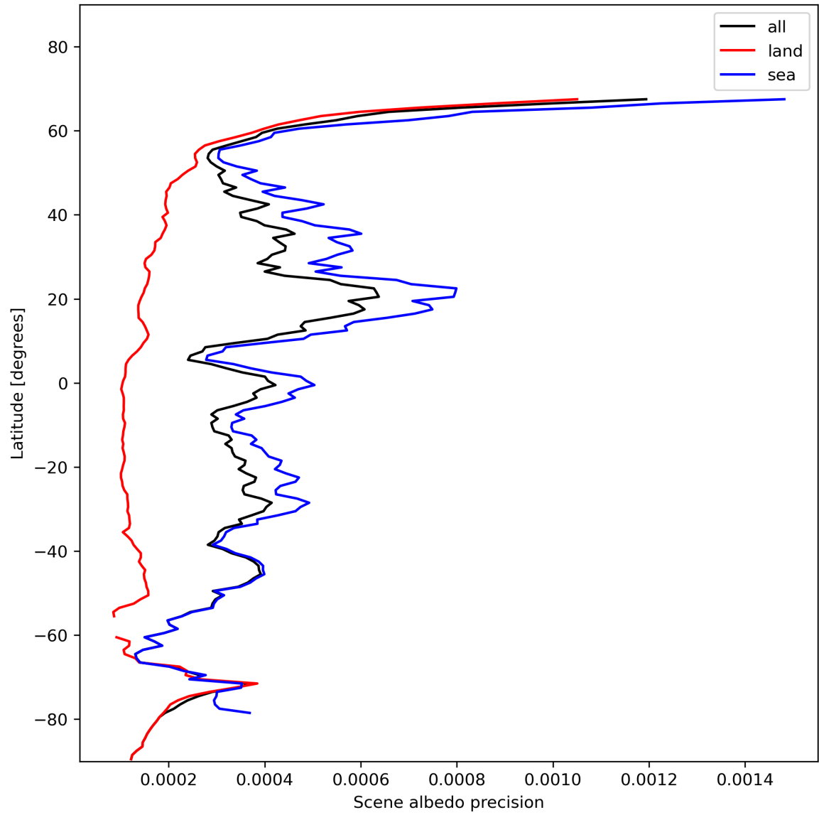
Figure 18: Zonal average of "Scene albedo precision" for 2023-11-23 to 2023-11-25.
