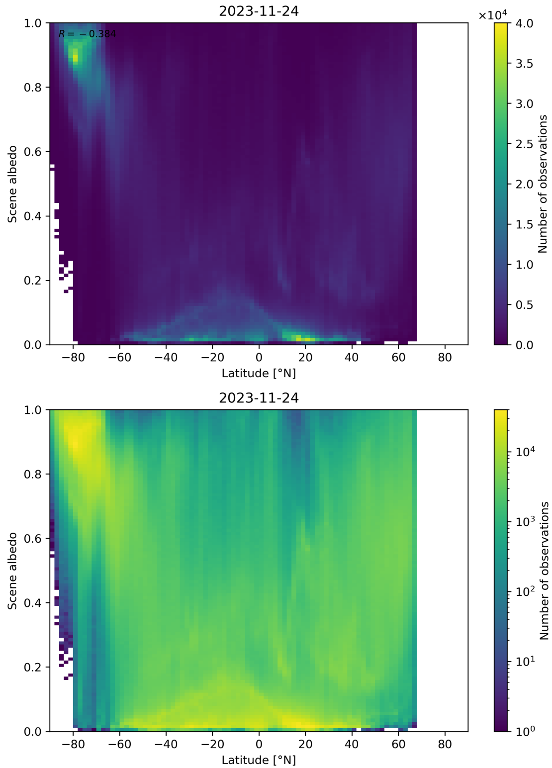
Figure 104: Scatter density plot of “Latitude” against “Scene albedo” for 2023-11-23 to 2023-11-25.
