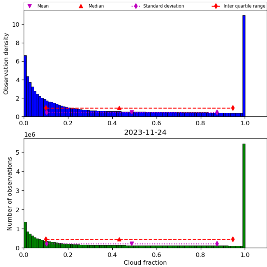
Figure 32: Histogram of “Cloud fraction” for 2023-11-23 to 2023-11-25
