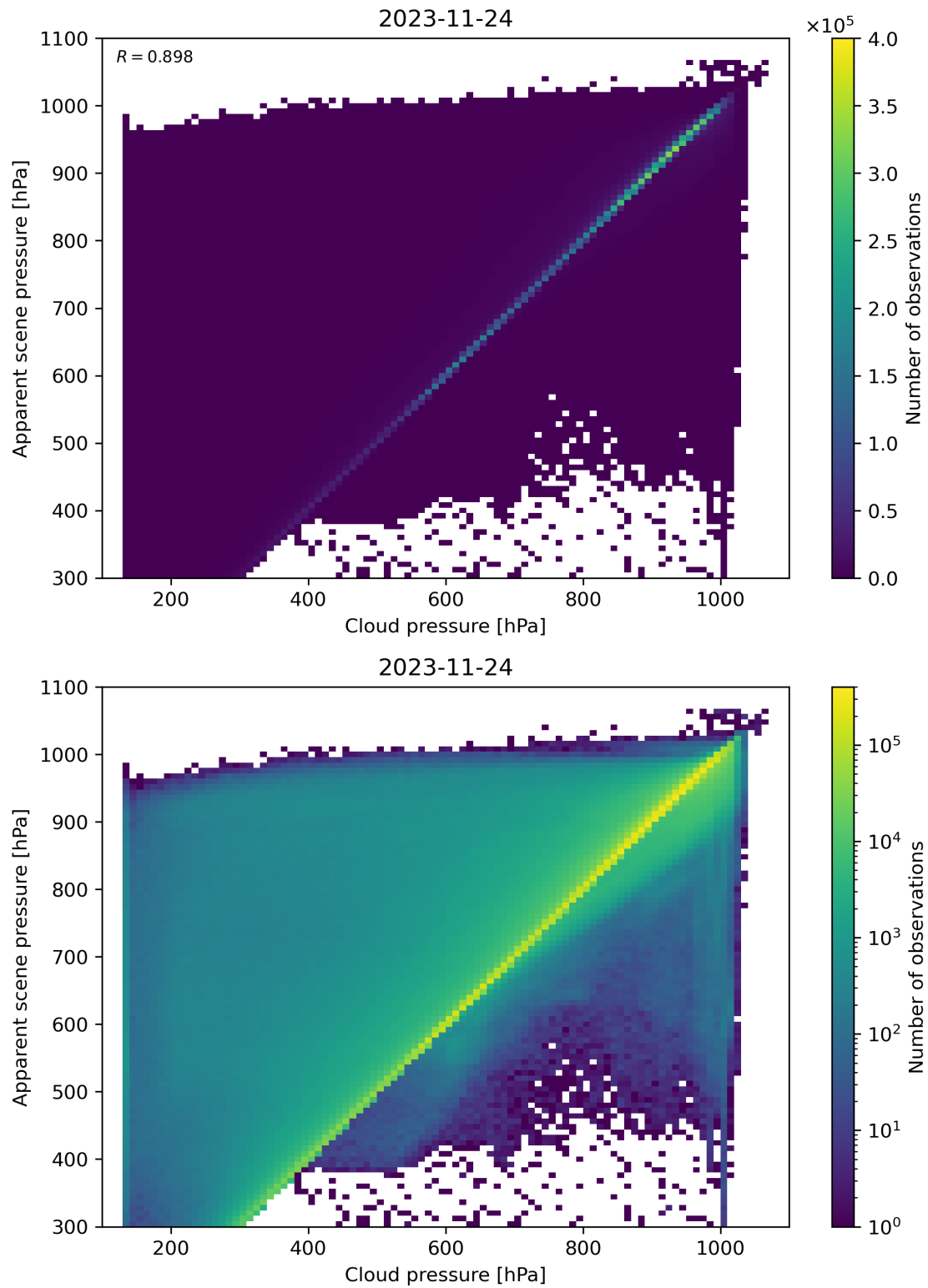
Figure 84: Scatter density plot of “Cloud pressure” against “Apparent scene pressure” for 2023-11-23 to 2023-11-25.
