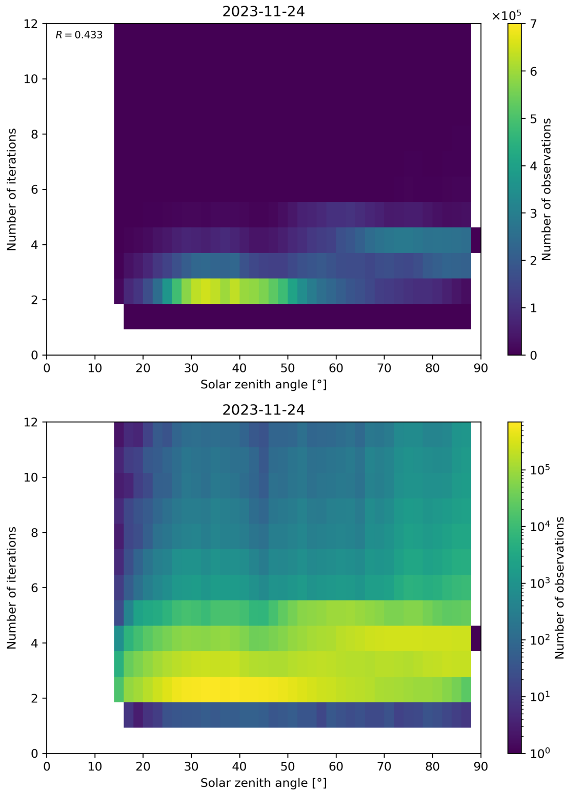
Figure 125: Scatter density plot of “Solar zenith angle” against “Number of iterations” for 2023-11-23 to 2023-11-25.
