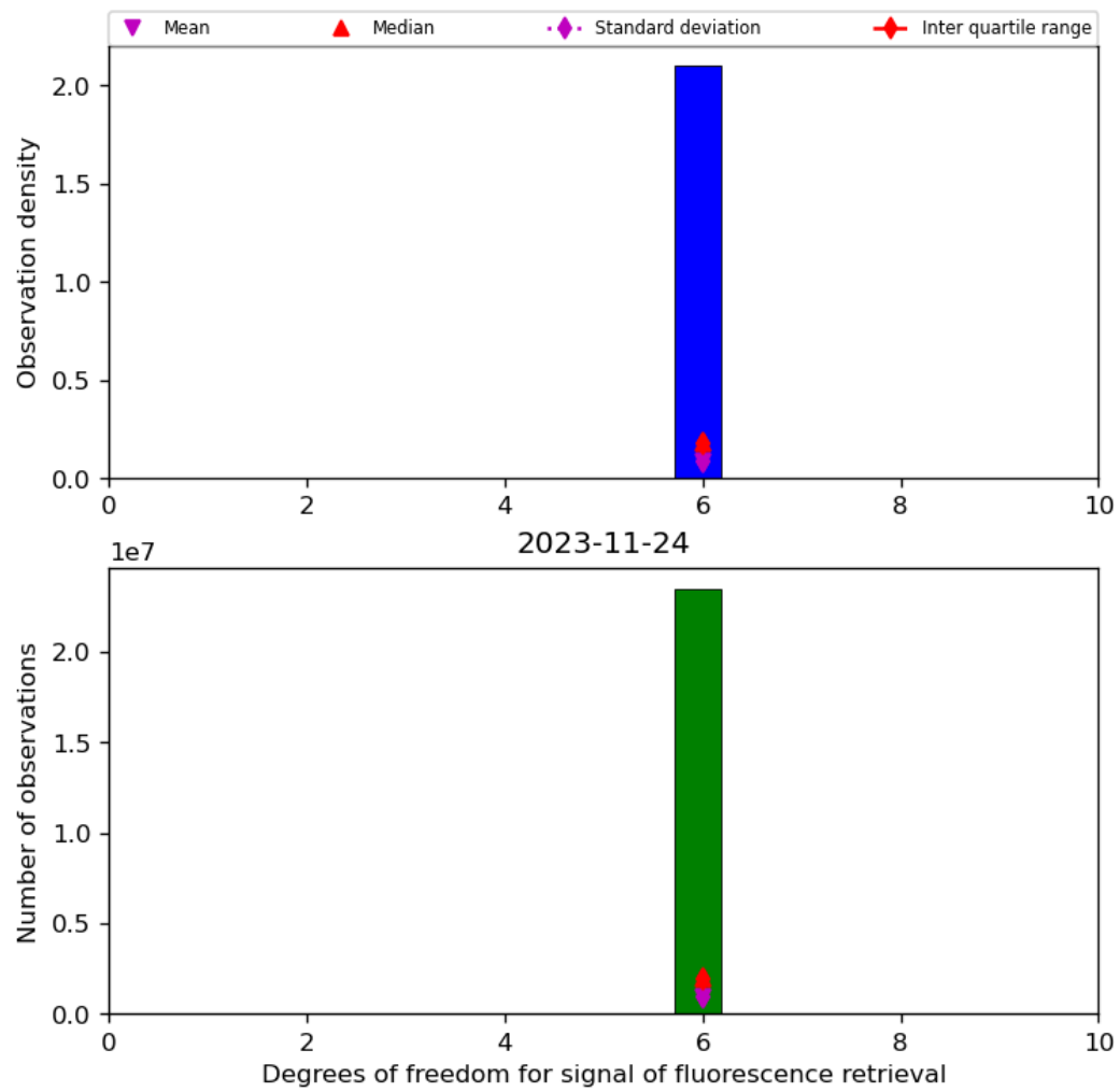
Figure 43: Histogram of “Degrees of freedom for signal of fluorescence retrieval” for 2023-11-23 to 2023-11-25
