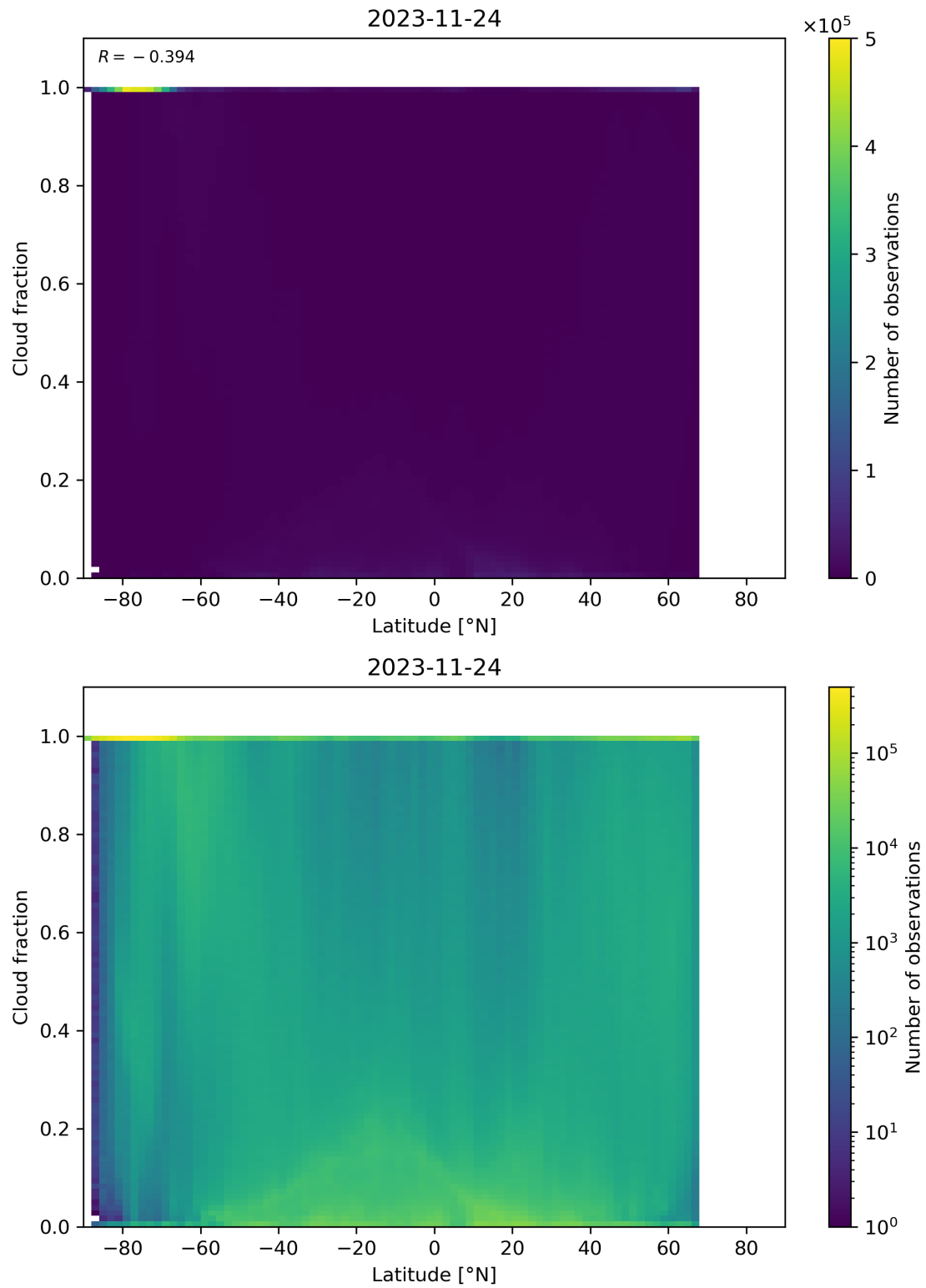
Figure 99: Scatter density plot of “Latitude” against “Cloud fraction” for 2023-11-23 to 2023-11-25.
