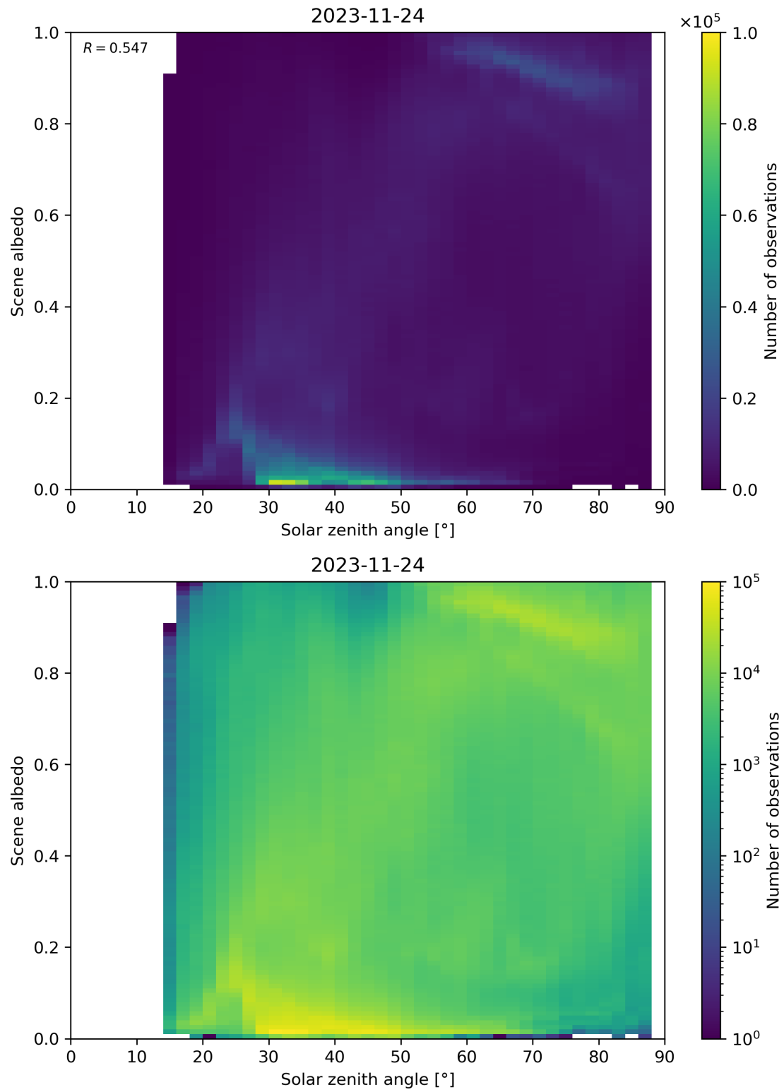
Figure 127: Scatter density plot of “Solar zenith angle” against “Scene albedo” for 2023-11-23 to 2023-11-25.
