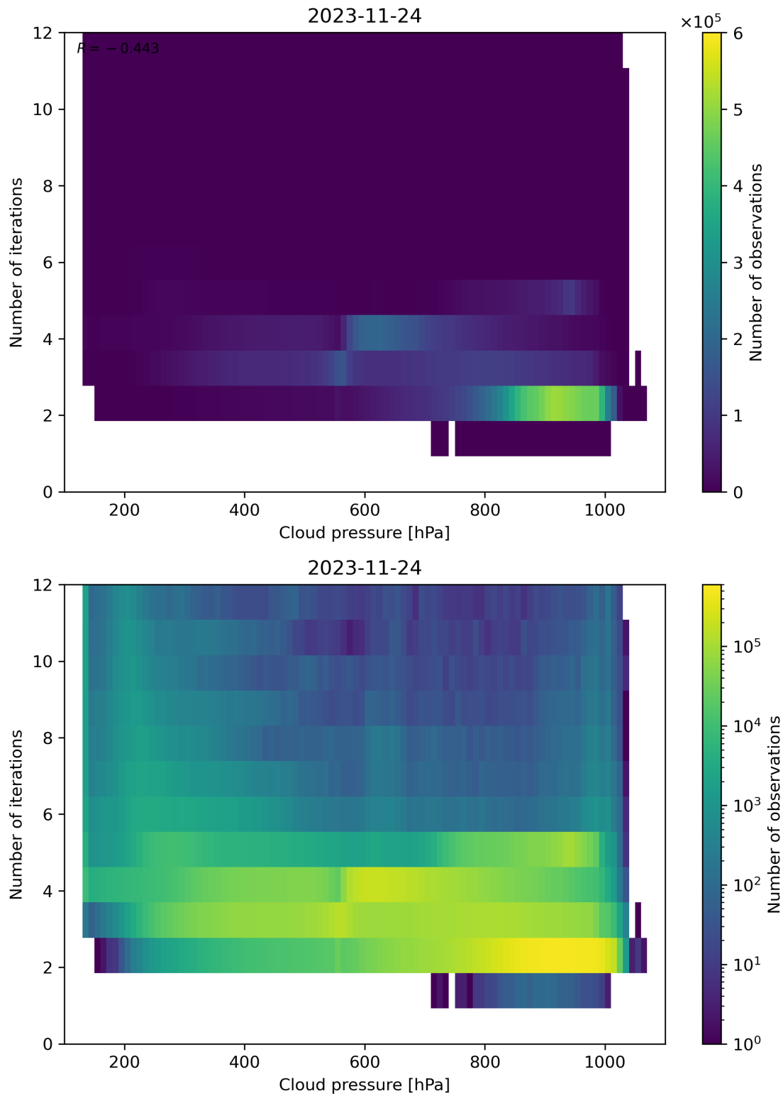
Figure 89: Scatter density plot of “Cloud pressure” against “Number of iterations” for 2023-11-23 to 2023-11-25.
