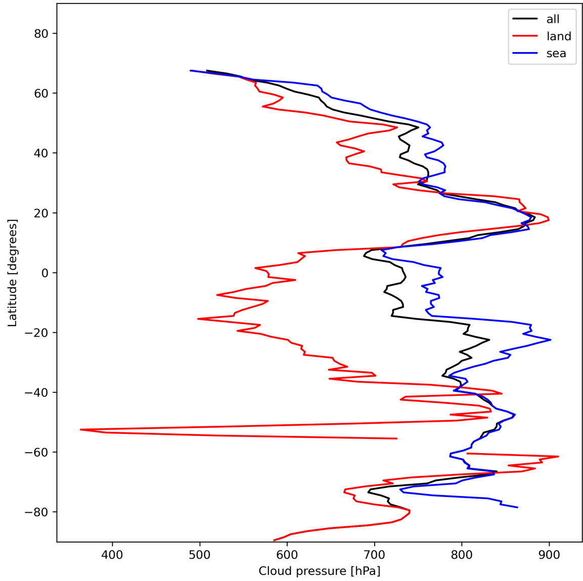
Figure 13: Zonal average of “Cloud pressure” for 2023-11-23 to 2023-11-25.
