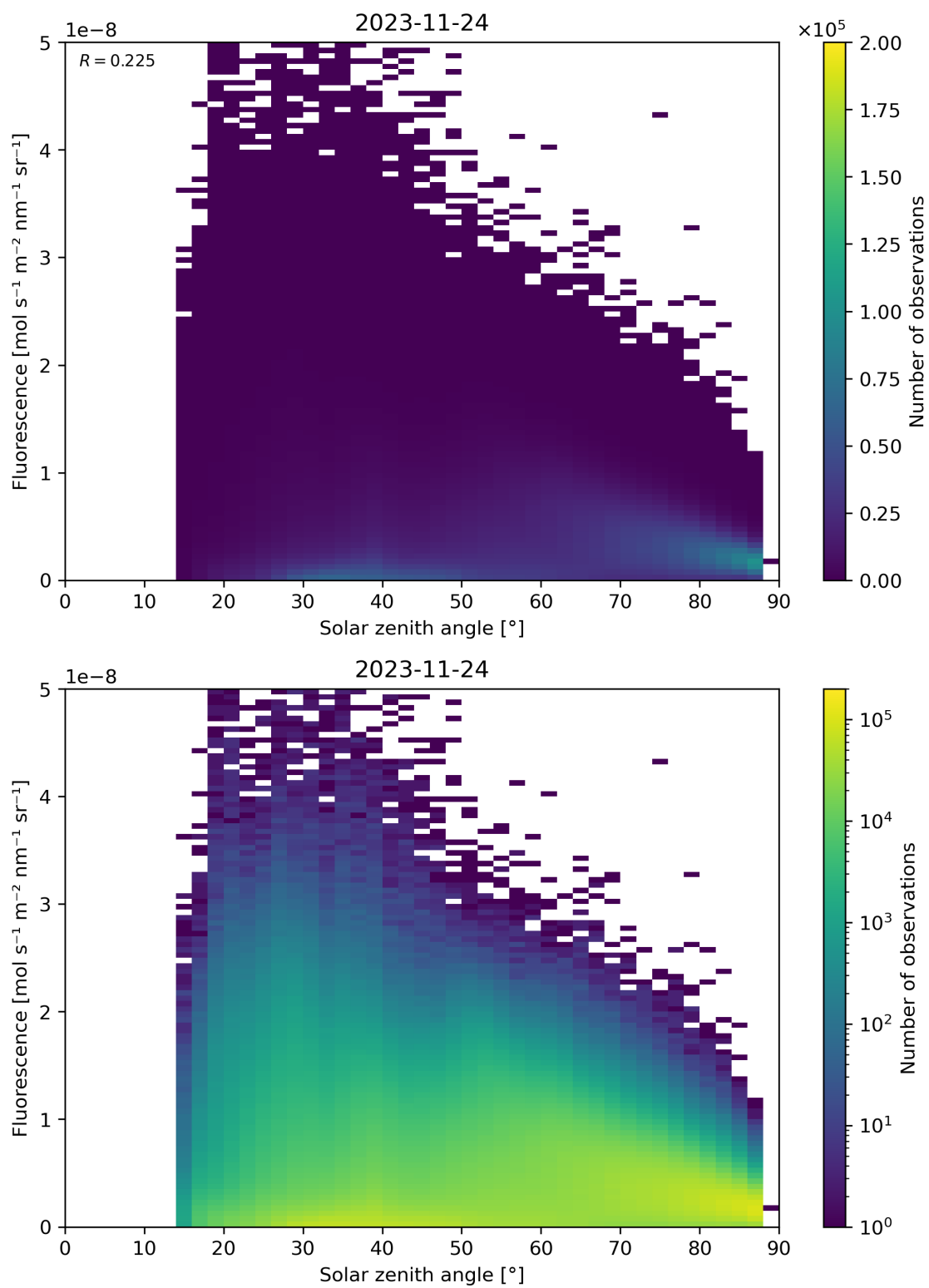
Figure 123: Scatter density plot of “Solar zenith angle” against “Fluorescence” for 2023-11-23 to 2023-11-25.
