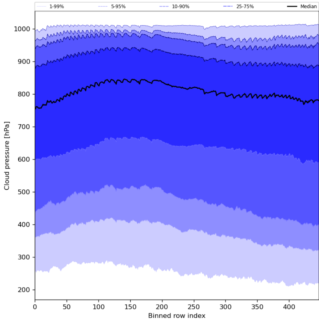
Figure 47: Along track statistics of “Cloud pressure” for 2023-11-23 to 2023-11-25
