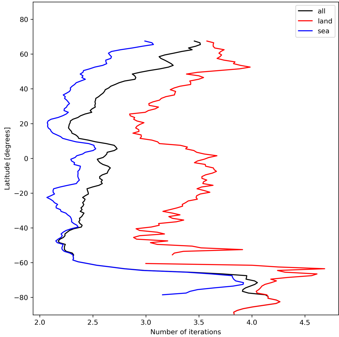
Figure 22: Zonal average of “Number of iterations” for 2023-11-23 to 2023-11-25.
