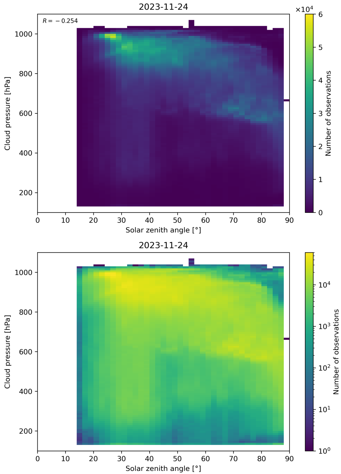
Figure 122: Scatter density plot of “Solar zenith angle” against “Cloud pressure” for 2023-11-23 to 2023-11-25.
