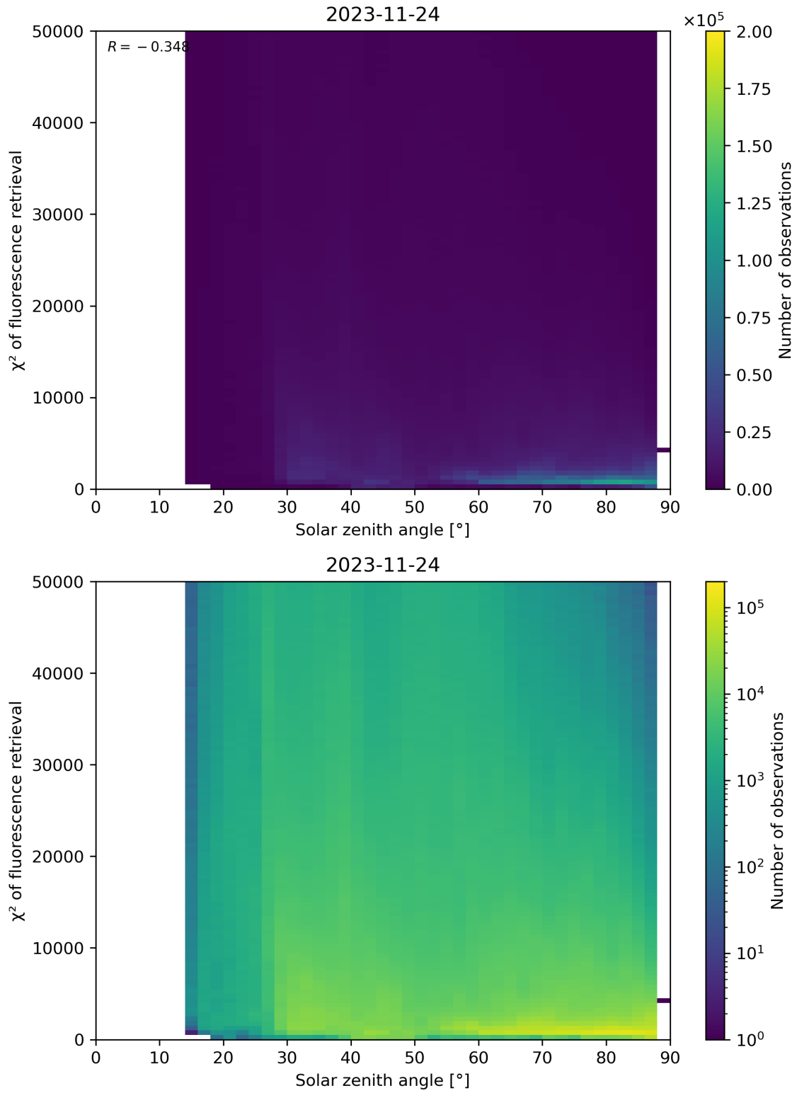
Figure 120: Scatter density plot of “Solar zenith angle” against “ \chi^2 of fluorescence retrieval” for 2023-11-23 to 2023-11-25.
