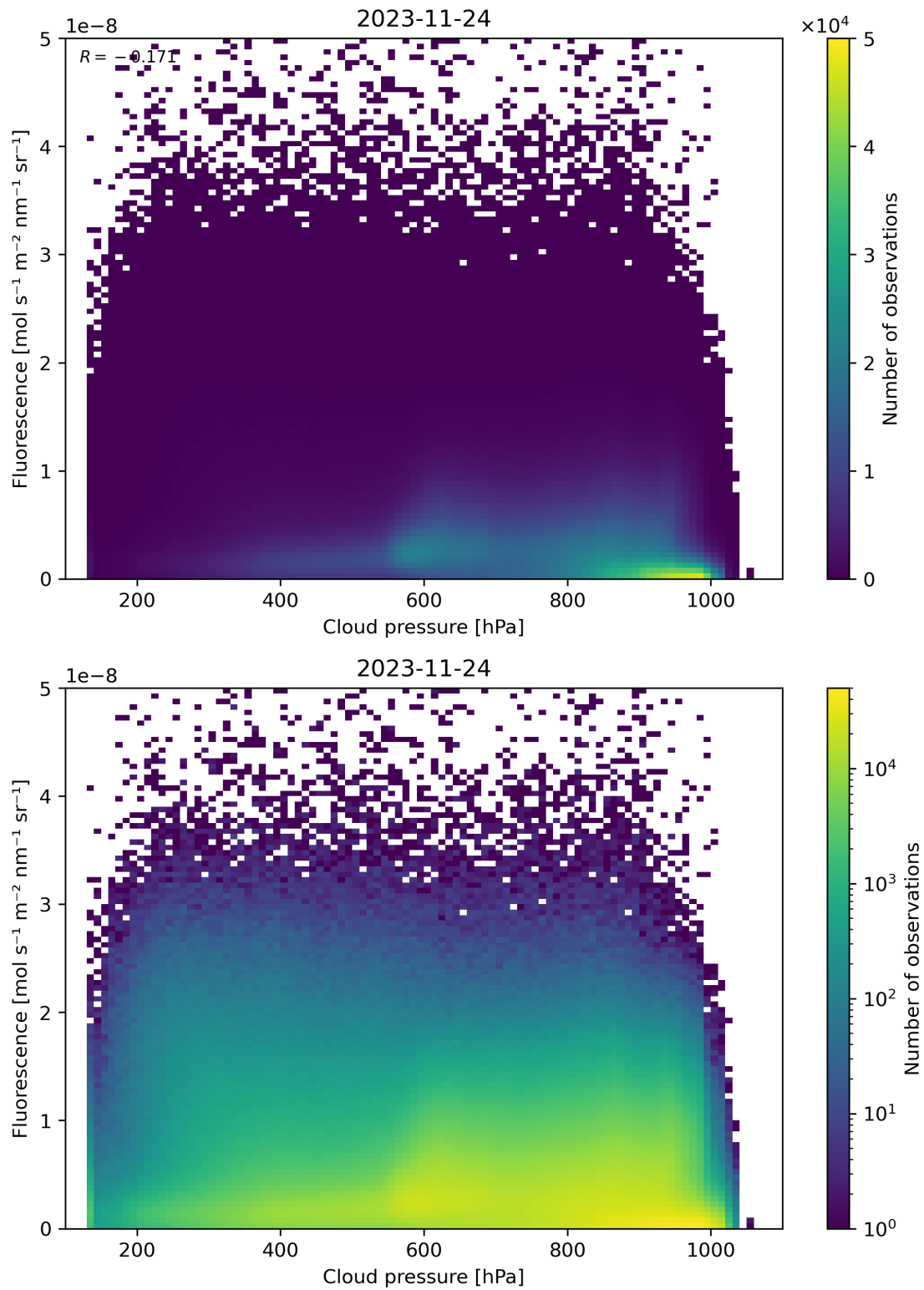
Figure 88: Scatter density plot of “Cloud pressure” against “Fluorescence” for 2023-11-23 to 2023-11-25.
