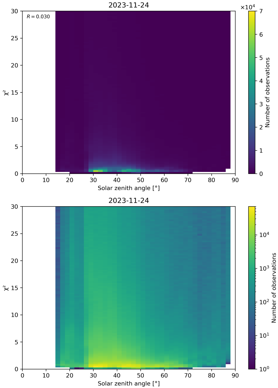
Figure 119: Scatter density plot of “Solar zenith angle” against “ \chi^2 ” for 2023-11-23 to 2023-11-25.
