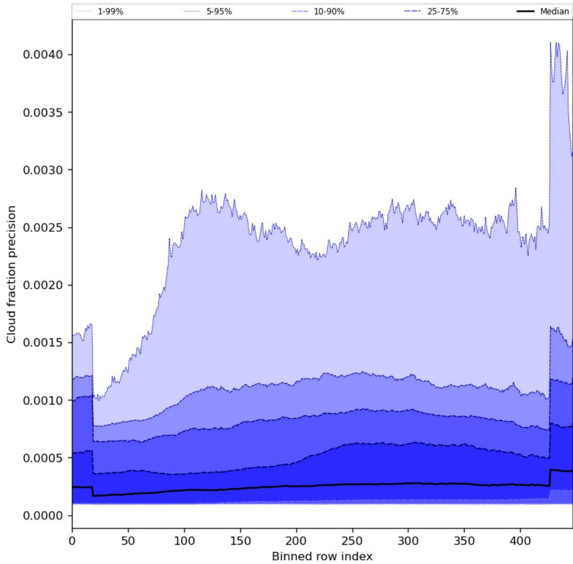
Figure 50: Along track statistics of “Cloud fraction precision” for 2023-11-23 to 2023-11-25
