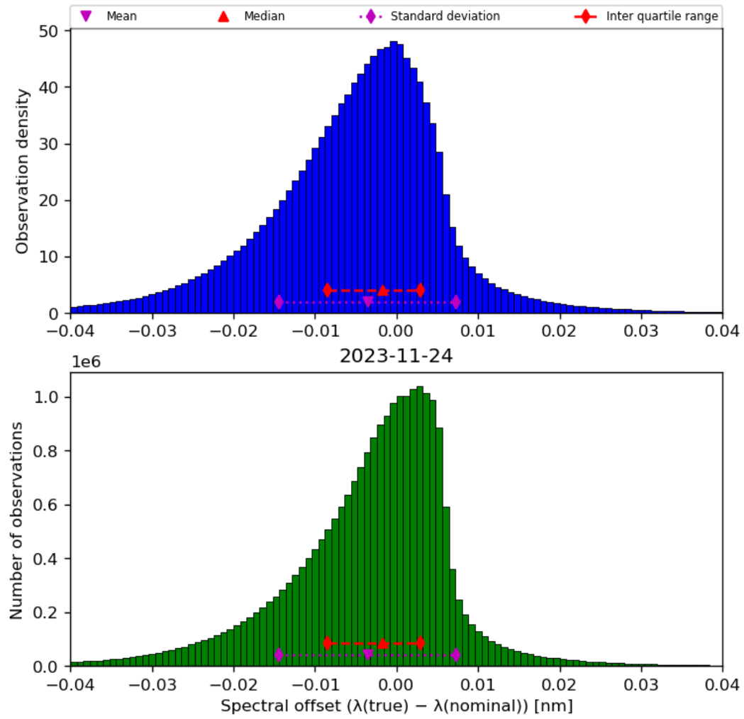
Figure 45: Histogram of “Spectral offset ( \lambda(\text{true}) - \lambda(\text{nominal}) )” for 2023-11-23 to 2023-11-25
