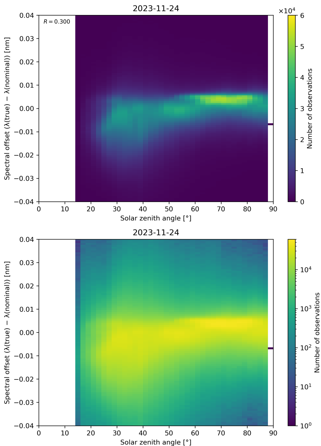
Figure 128: Scatter density plot of “Solar zenith angle” against “Spectral offset ( \lambda(\text{true}) - \lambda(\text{nominal}) )” for 2023-11-23 to 2023-11-25.
