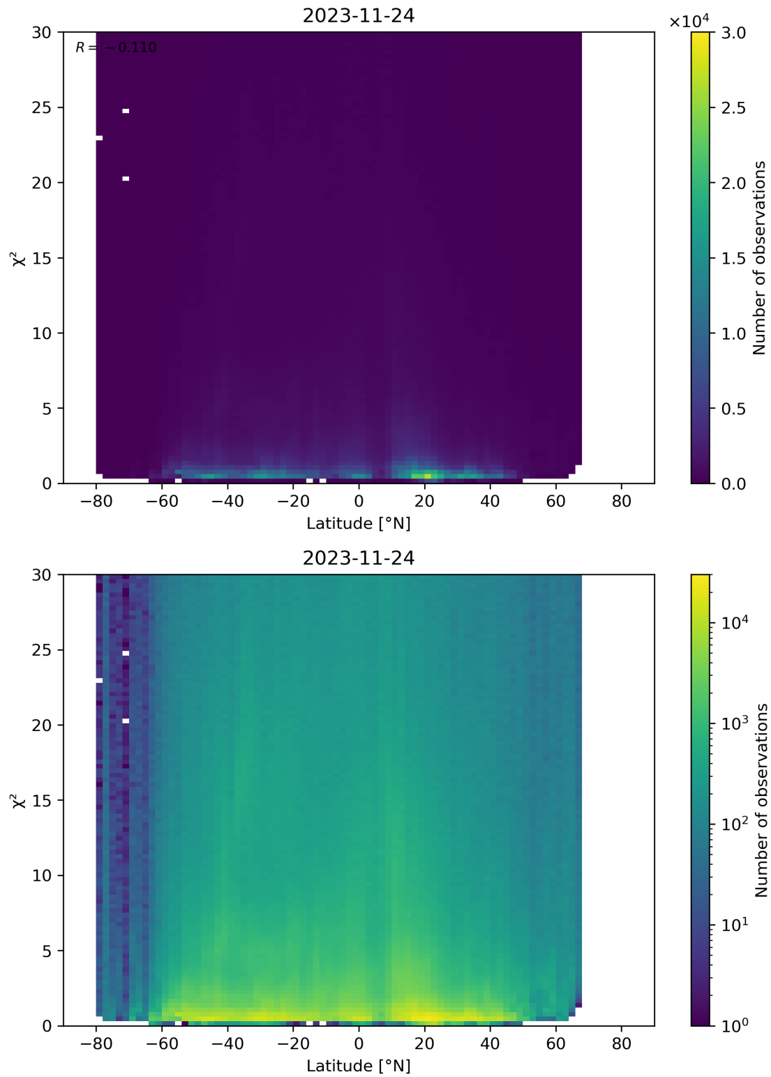
Figure 97: Scatter density plot of “Latitude” against “ \chi^2 ” for 2023-11-23 to 2023-11-25.
