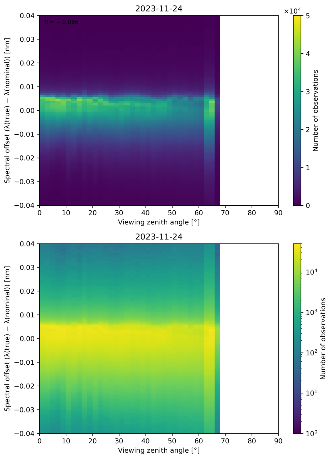
Figure 140: Scatter density plot of “Viewing zenith angle” against “Spectral offset ( \lambda(\text{true}) - \lambda(\text{nominal}) )” for 2023-11-23 to 2023-11-25.
