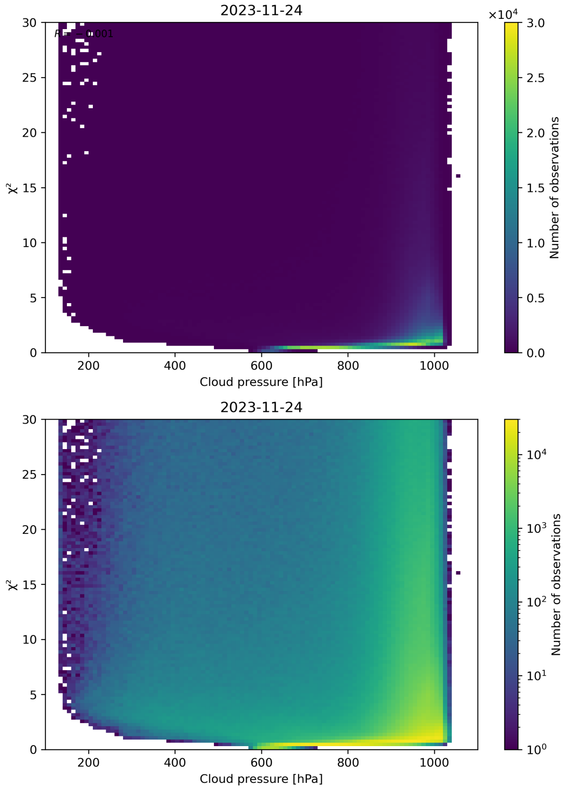
Figure 85: Scatter density plot of “Cloud pressure” against “ \chi^2 ” for 2023-11-23 to 2023-11-25.
