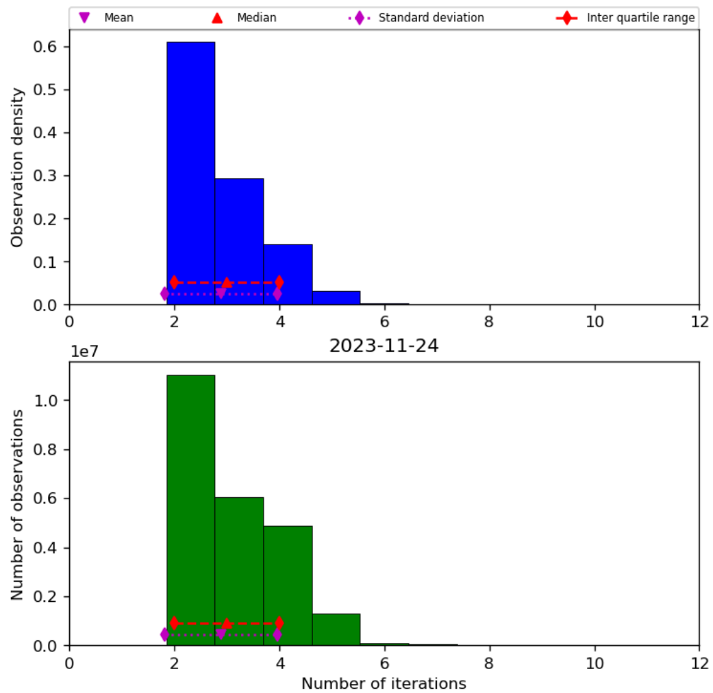
Figure 39: Histogram of “Number of iterations” for 2023-11-23 to 2023-11-25
