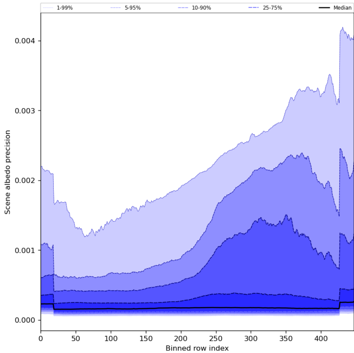
Figure 52: Along track statistics of “Scene albedo precision” for 2023-11-23 to 2023-11-25
