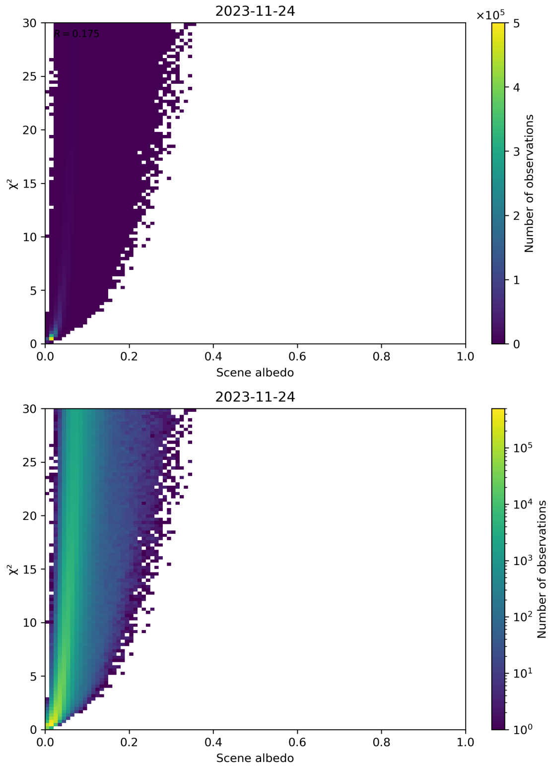
Figure 112: Scatter density plot of “Scene albedo” against “ \chi^2 ” for 2023-11-23 to 2023-11-25.
