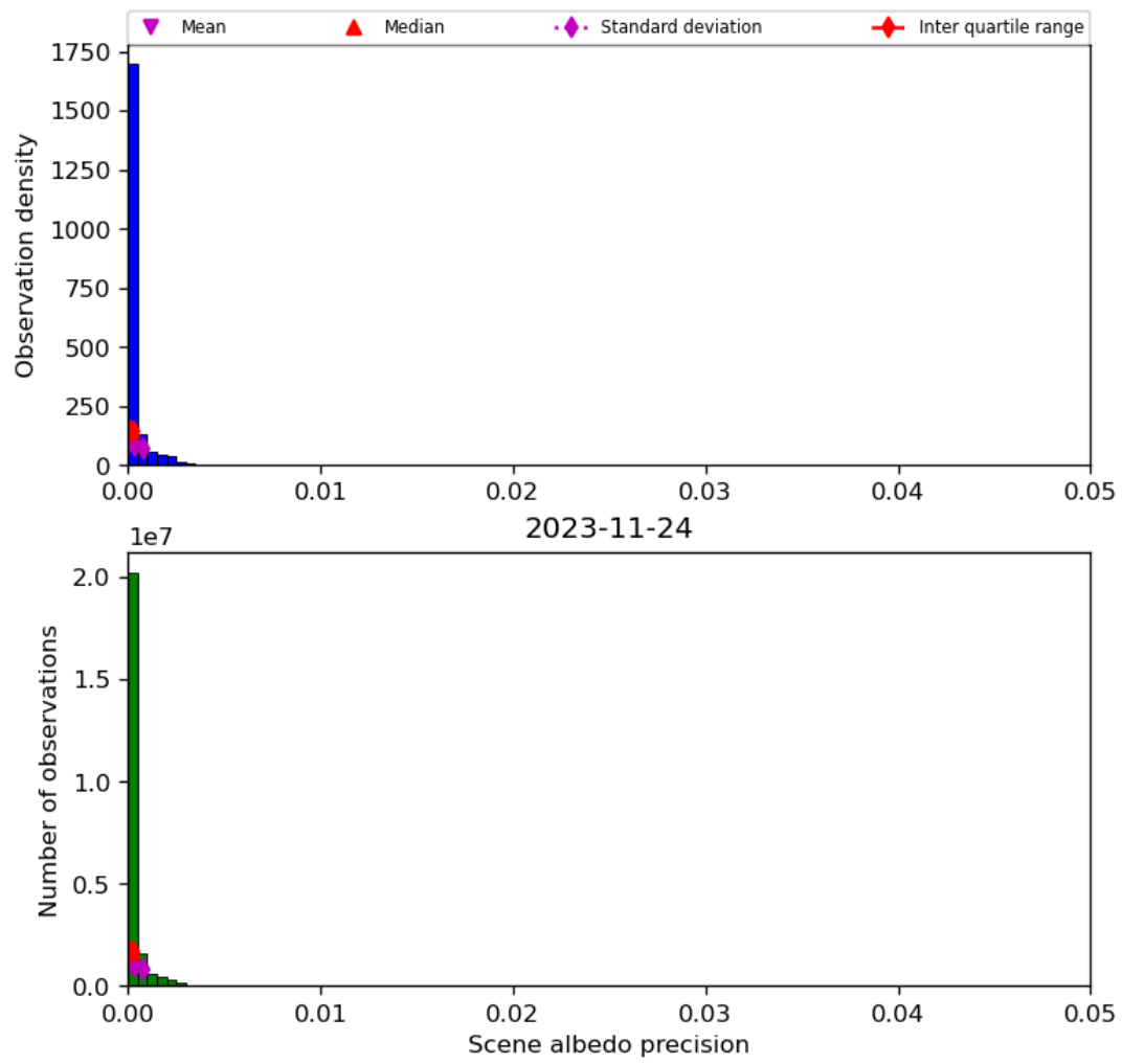
Figure 35: Histogram of “Scene albedo precision” for 2023-11-23 to 2023-11-25
