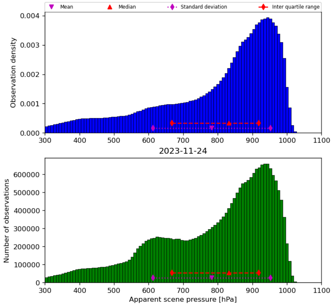
Figure 36: Histogram of “Apparent scene pressure” for 2023-11-23 to 2023-11-25
