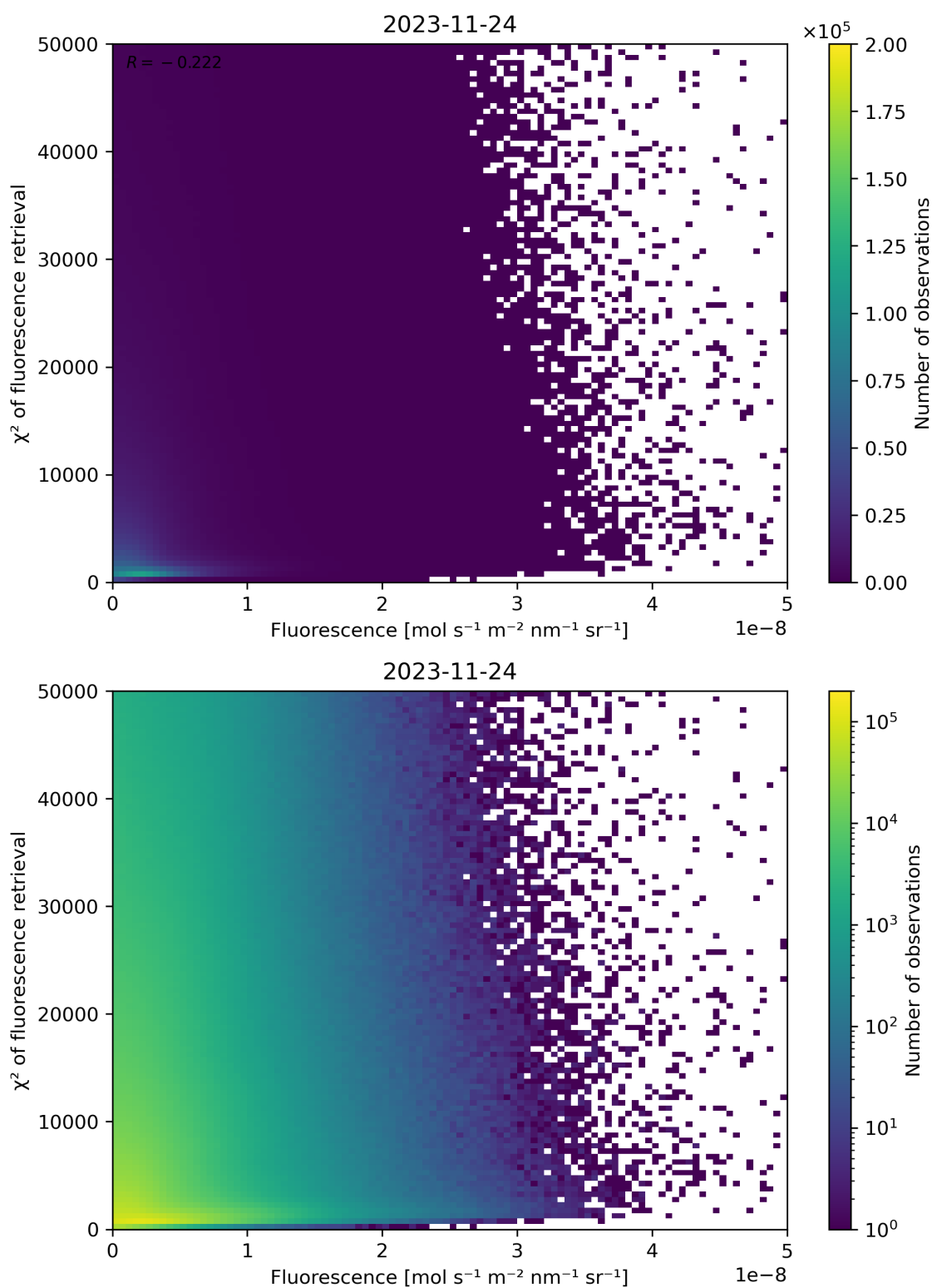
Figure 93: Scatter density plot of “Fluorescence” against “ \chi^2 of fluorescence retrieval” for 2023-11-23 to 2023-11-25.
