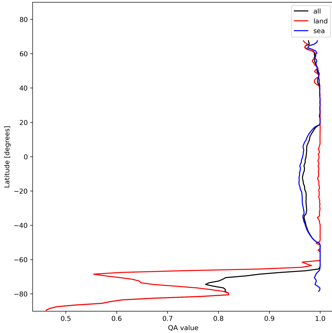
Figure 12: Zonal average of “QA value” for 2023-11-23 to 2023-11-25.
