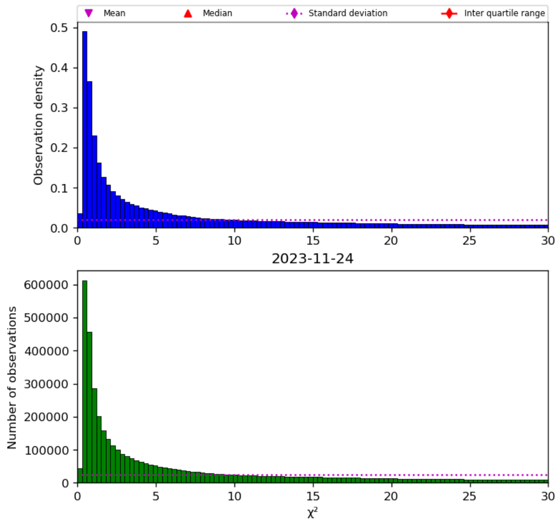
Figure 38: Histogram of “ \chi^2 ” for 2023-11-23 to 2023-11-25
