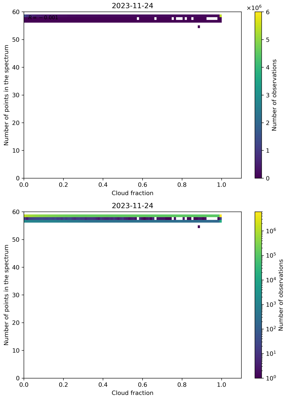
Figure 81: Scatter density plot of “Cloud fraction” against “Number of points in the spectrum” for 2023-11-23 to 2023-11-25.
