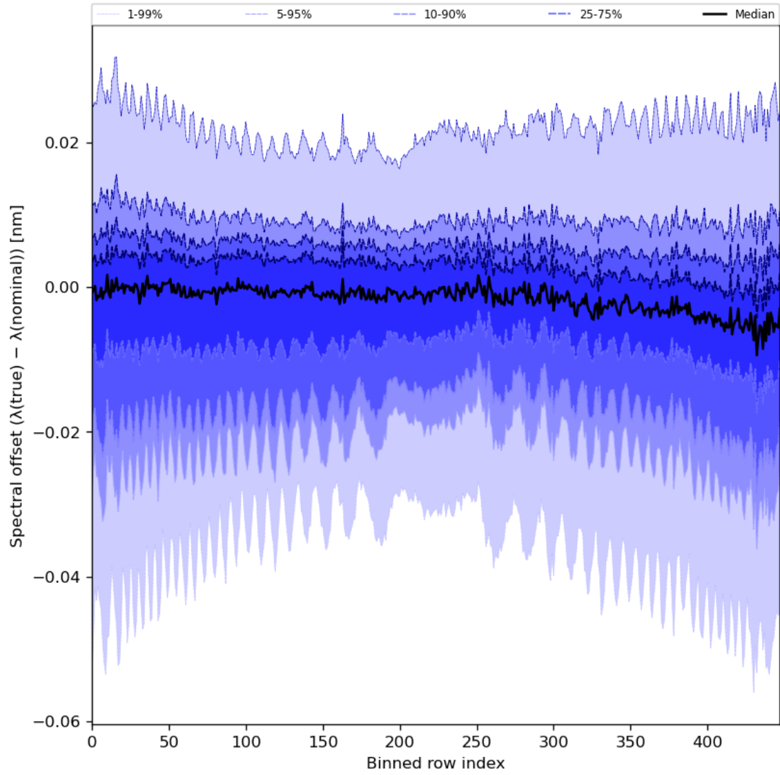
Figure 62: Along track statistics of “Spectral offset ( \lambda(\text{true}) - \lambda(\text{nominal}) )” for 2023-11-23 to 2023-11-25
