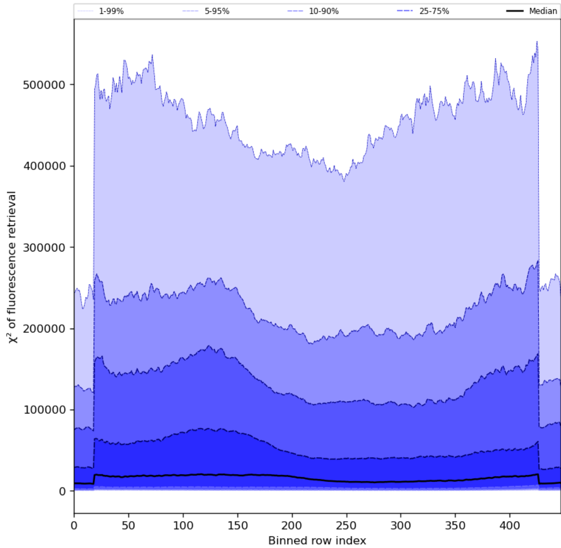
Figure 59: Along track statistics of “ \chi^2 of fluorescence retrieval” for 2023-11-23 to 2023-11-25
