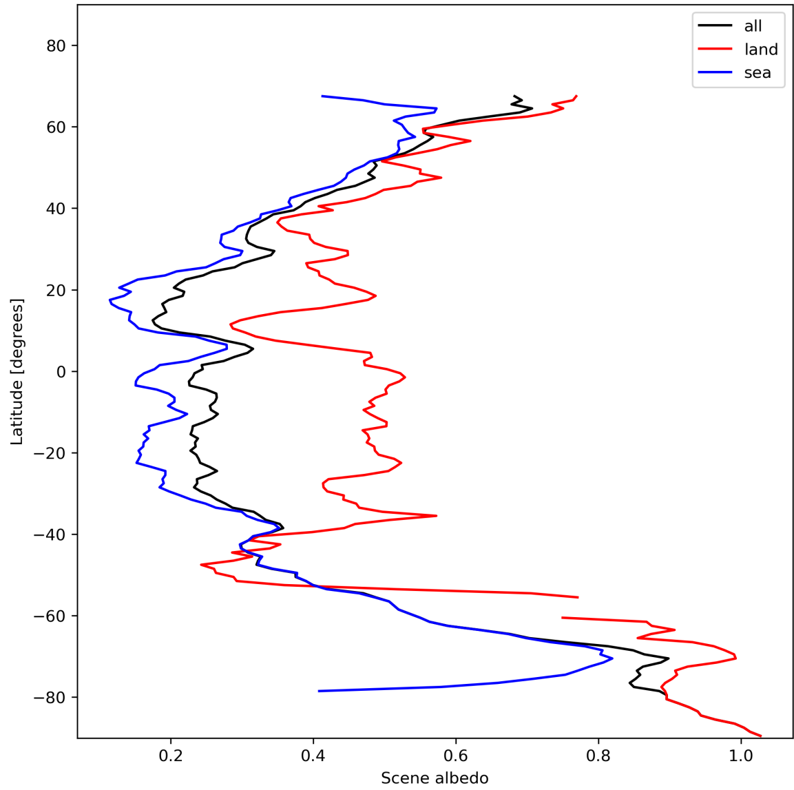
Figure 17: Zonal average of “Scene albedo” for 2023-11-23 to 2023-11-25.
