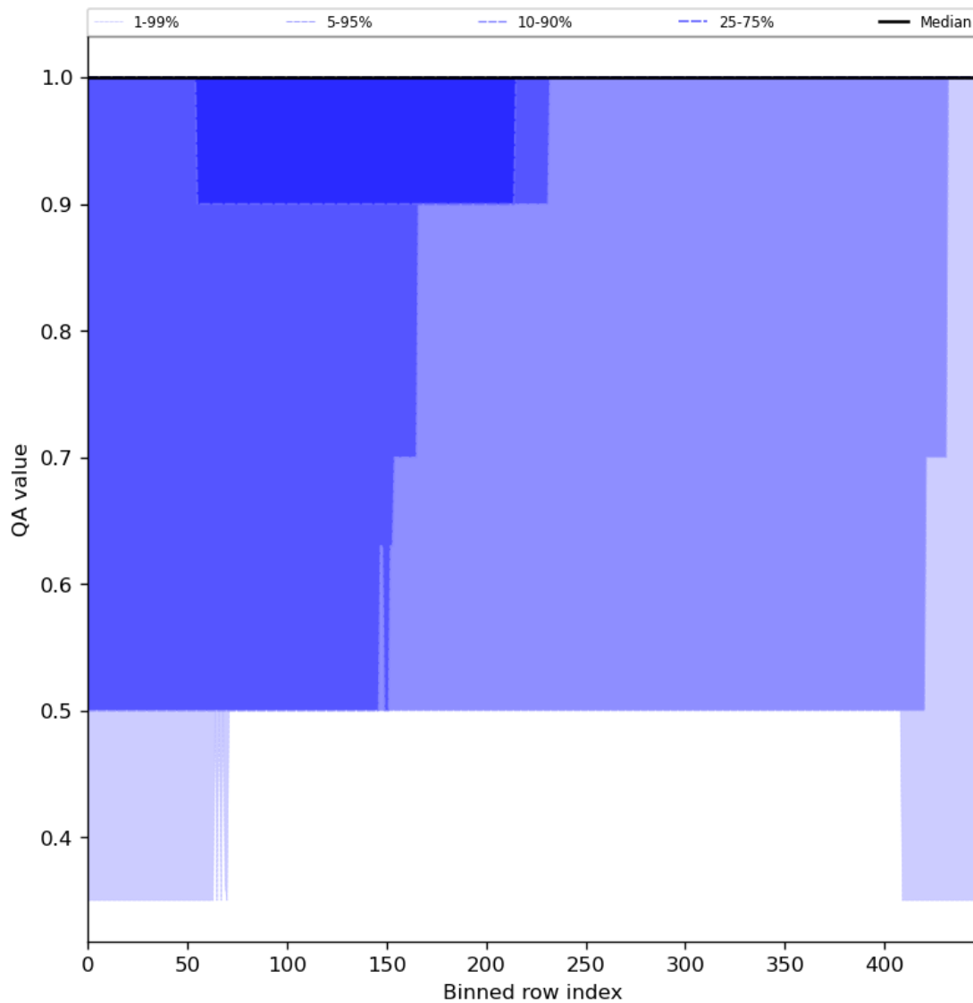
Figure 46: Along track statistics of “QA value” for 2023-11-23 to 2023-11-25
