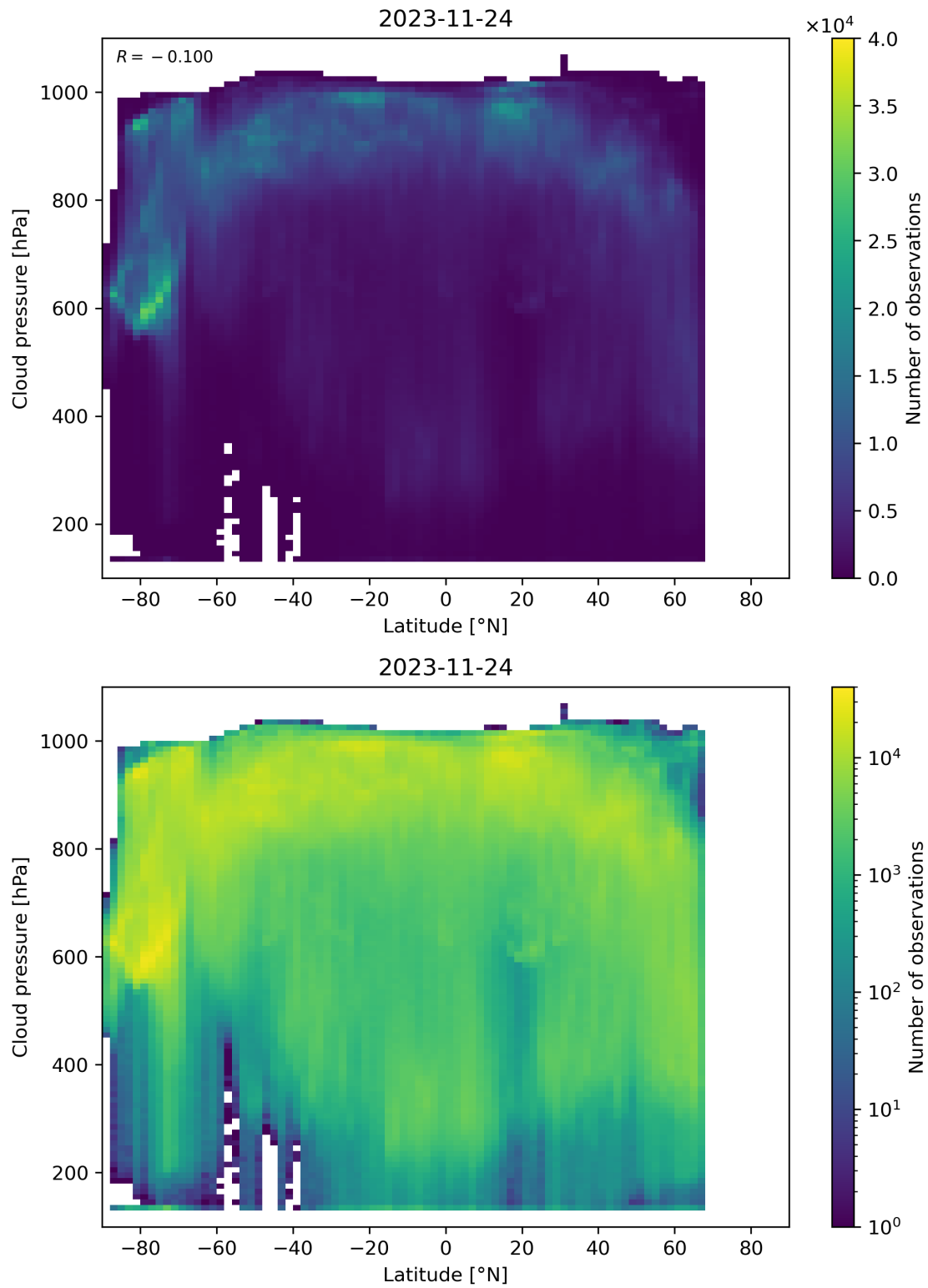
Figure 100: Scatter density plot of “Latitude” against “Cloud pressure” for 2023-11-23 to 2023-11-25.
