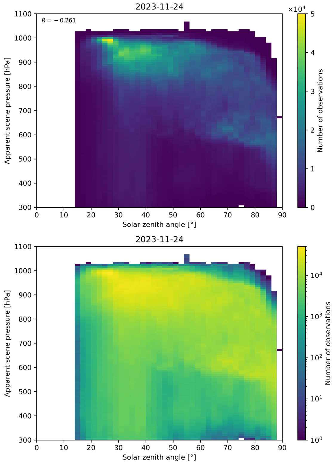
Figure 118: Scatter density plot of “Solar zenith angle” against “Apparent scene pressure” for 2023-11-23 to 2023-11-25.
