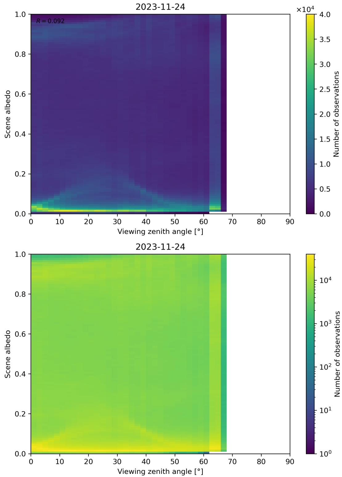
Figure 138: Scatter density plot of “Viewing zenith angle” against “Scene albedo” for 2023-11-23 to 2023-11-25.
