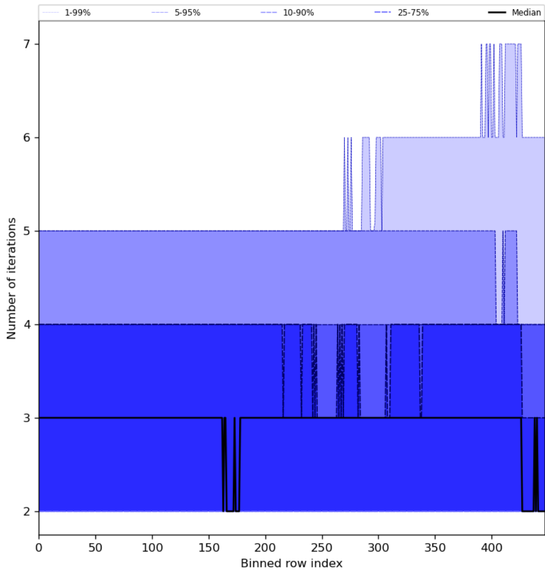
Figure 56: Along track statistics of “Number of iterations” for 2023-11-23 to 2023-11-25
