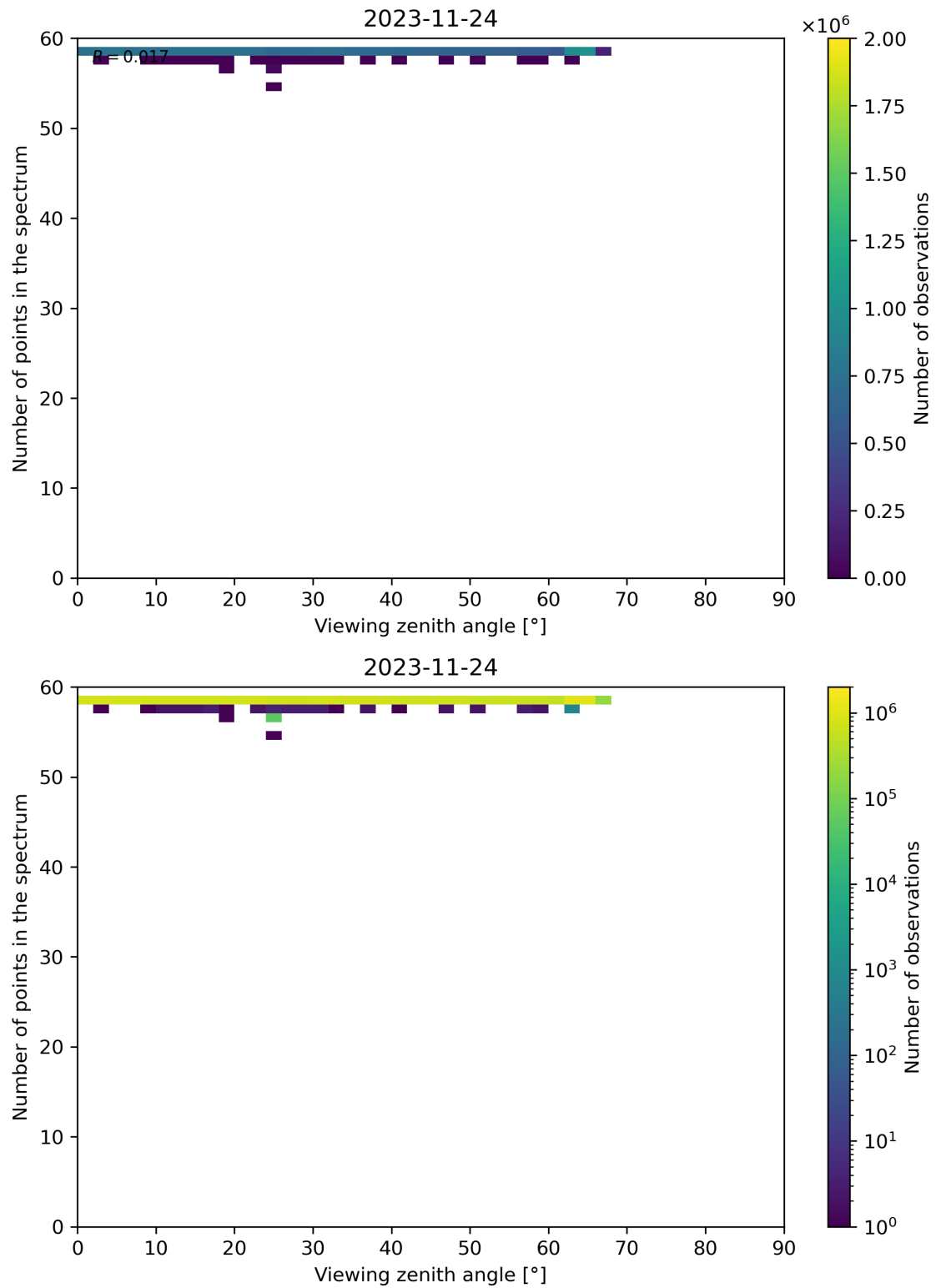
Figure 137: Scatter density plot of “Viewing zenith angle” against “Number of points in the spectrum” for 2023-11-23 to 2023-11-25.
