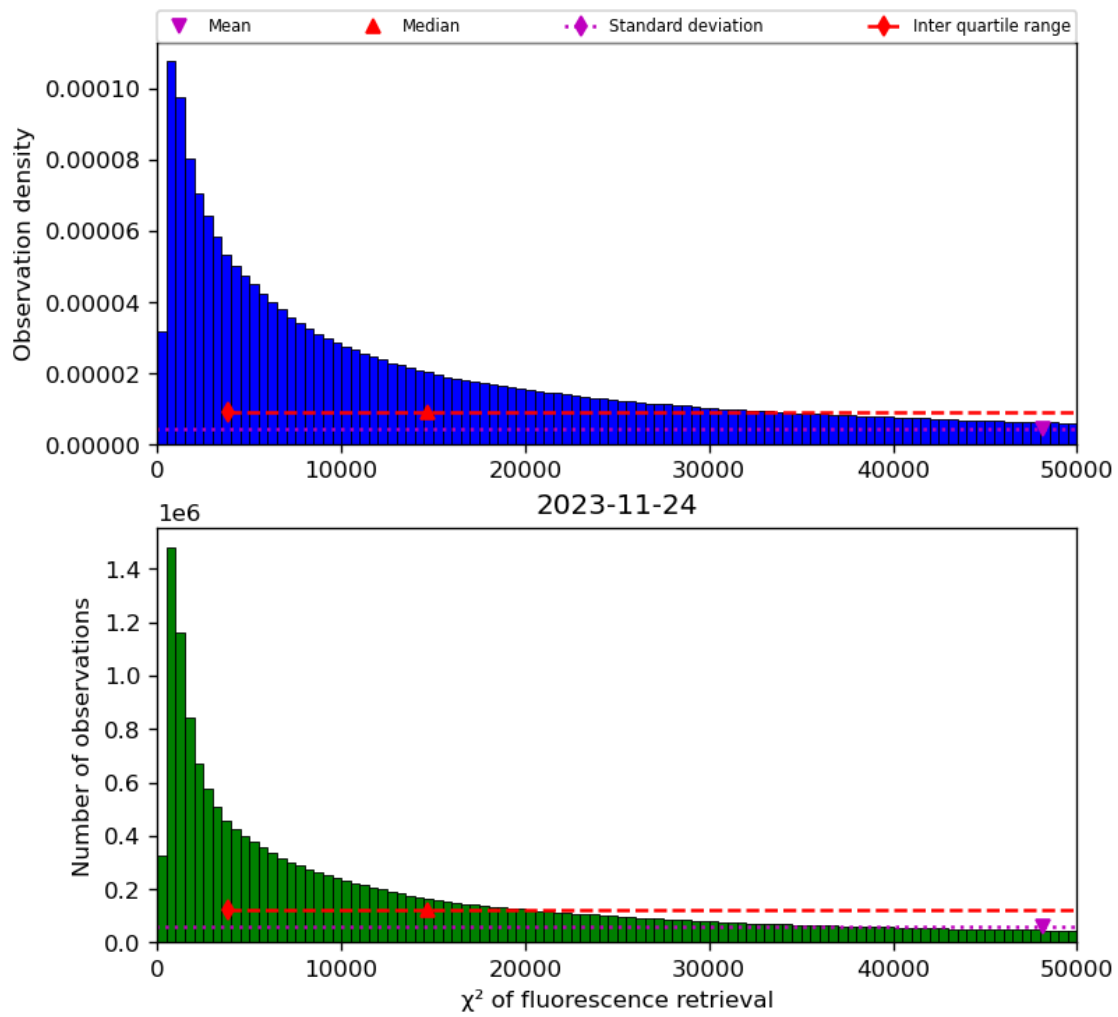
Figure 42: Histogram of “ \chi^2 of fluorescence retrieval” for 2023-11-23 to 2023-11-25
