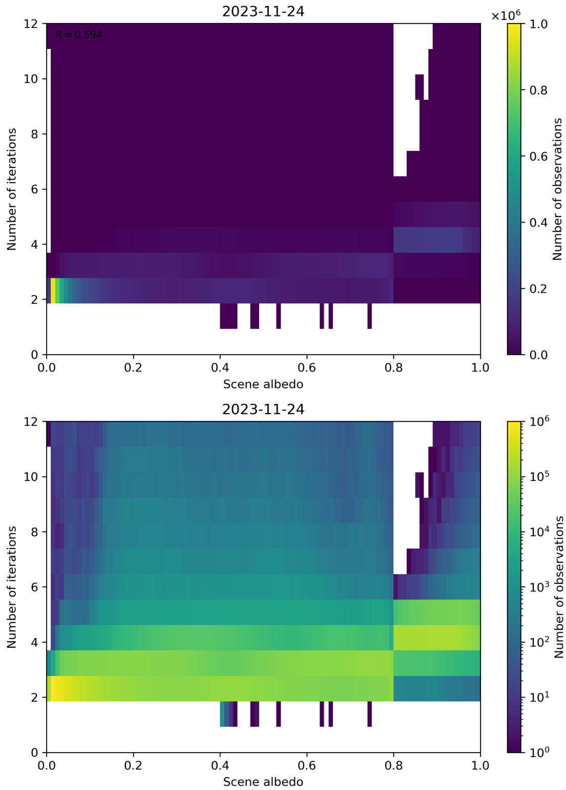
Figure 115: Scatter density plot of “Scene albedo” against “Number of iterations” for 2023-11-23 to 2023-11-25.
