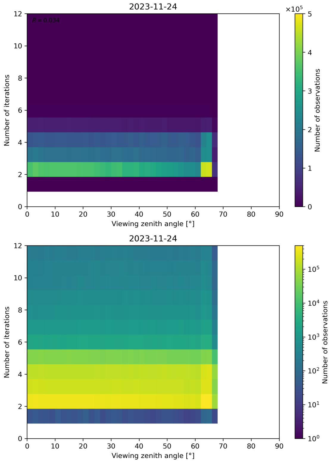
Figure 136: Scatter density plot of “Viewing zenith angle” against “Number of iterations” for 2023-11-23 to 2023-11-25.
