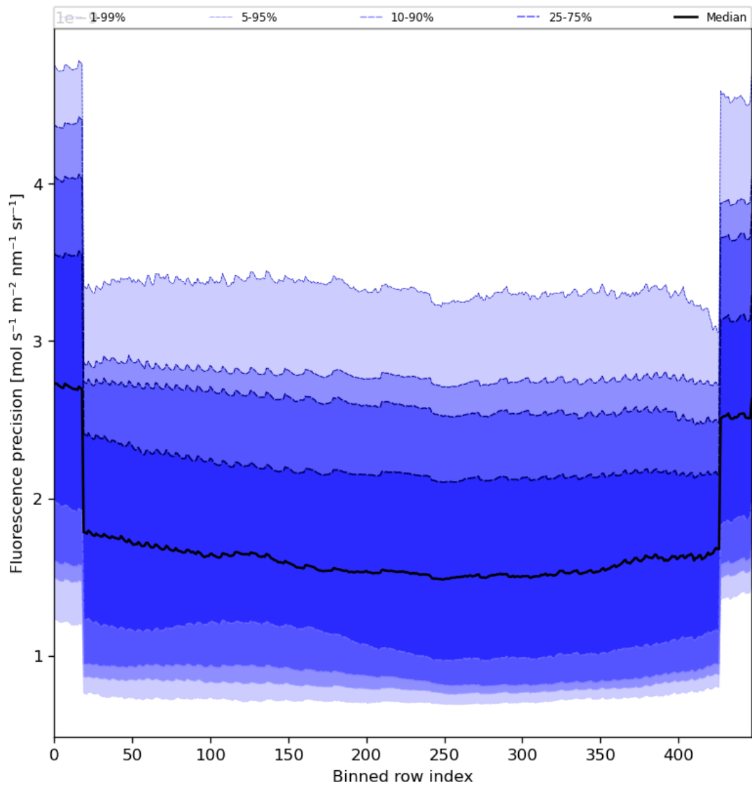
Figure 58: Along track statistics of “Fluorescence precision” for 2023-11-23 to 2023-11-25
