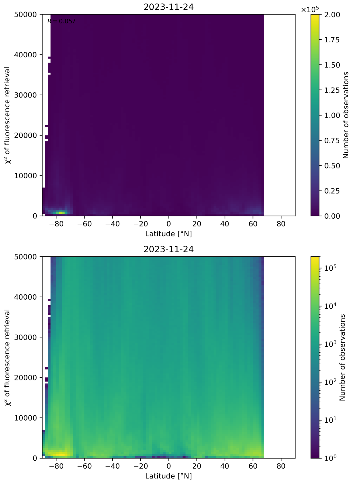
Figure 98: Scatter density plot of “Latitude” against “ \chi^2 of fluorescence retrieval” for 2023-11-23 to 2023-11-25.
