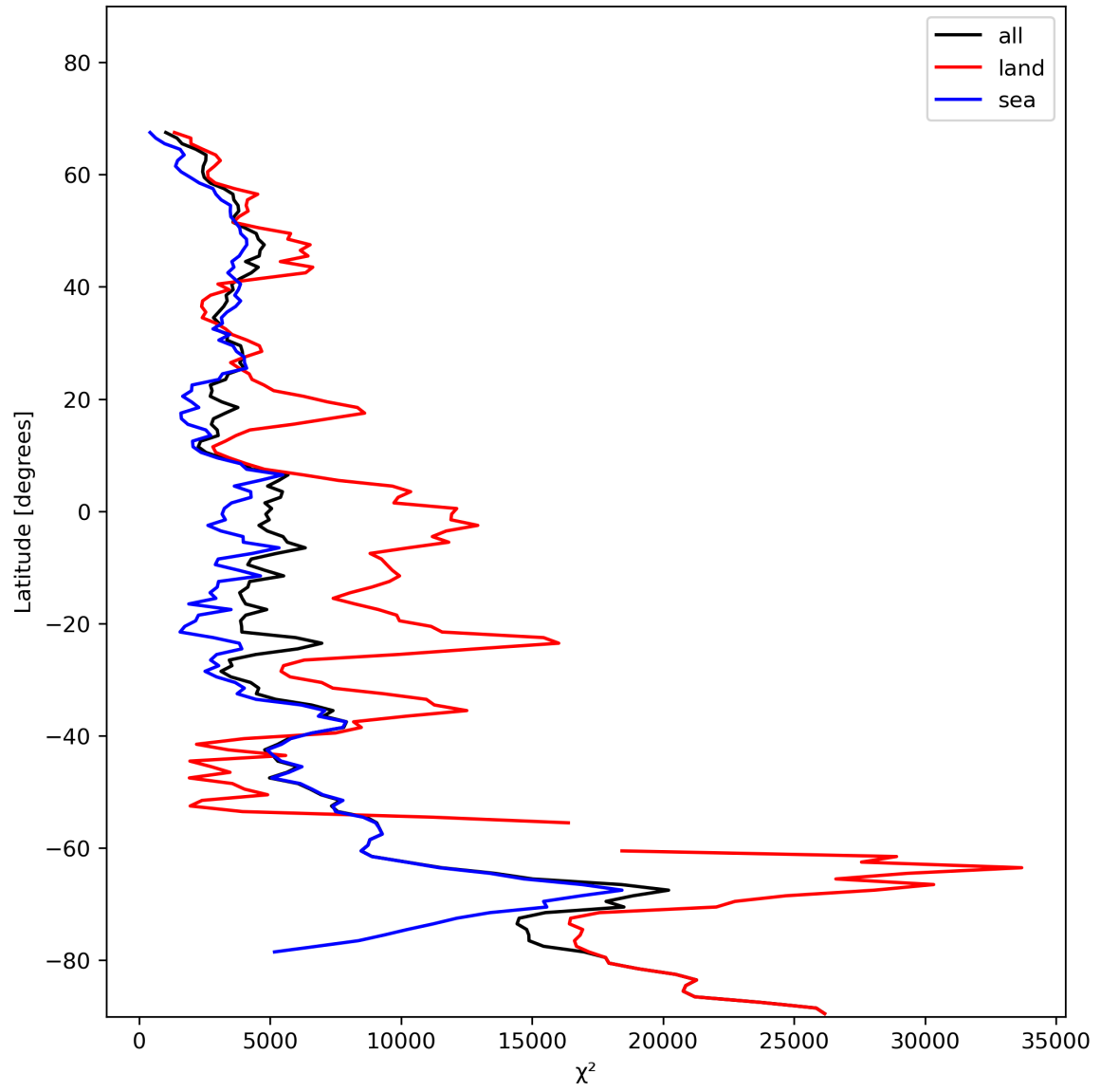
Figure 21: Zonal average of “ \chi^2 ” for 2023-11-23 to 2023-11-25.
