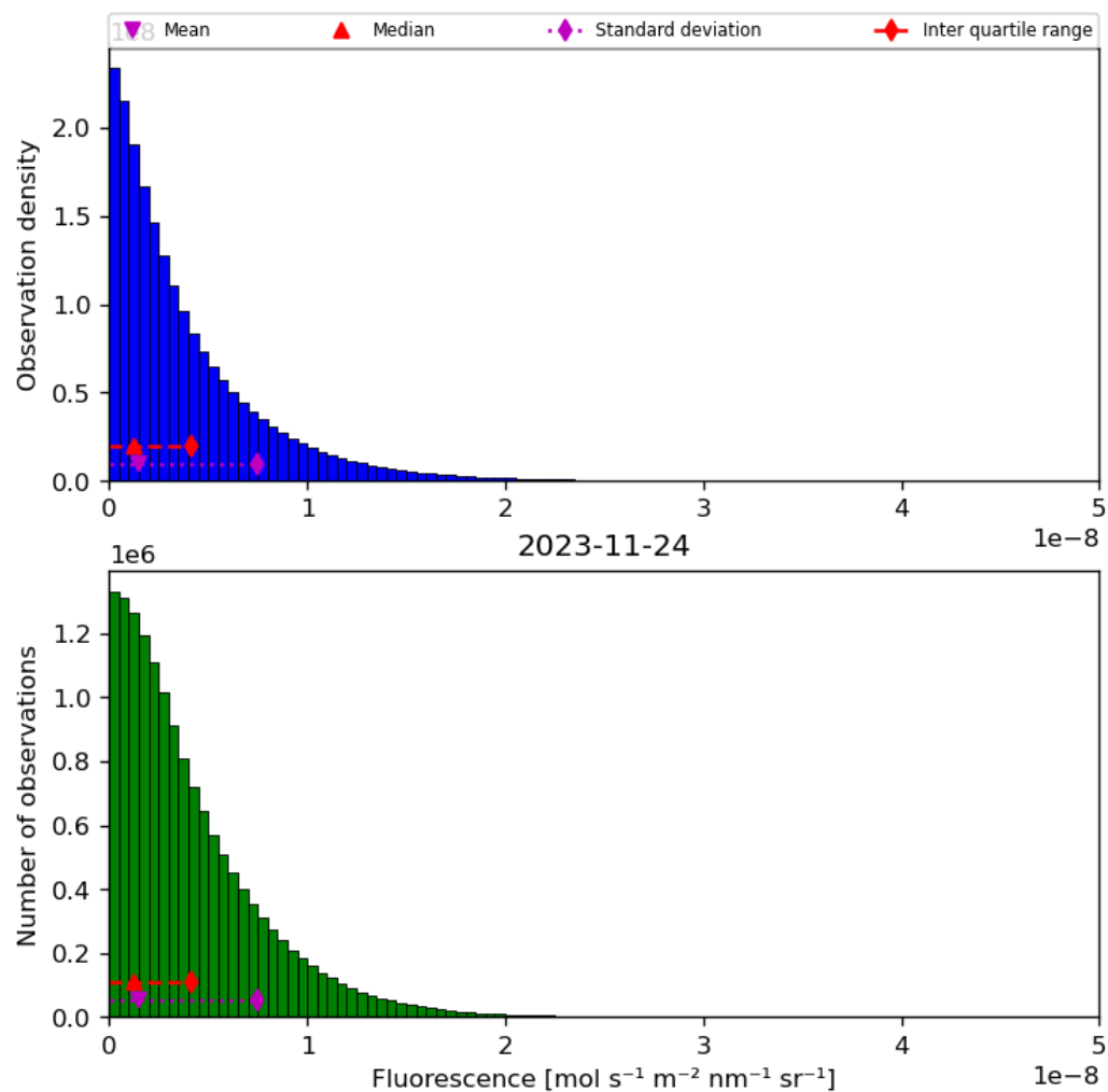
Figure 40: Histogram of “Fluorescence” for 2023-11-23 to 2023-11-25
