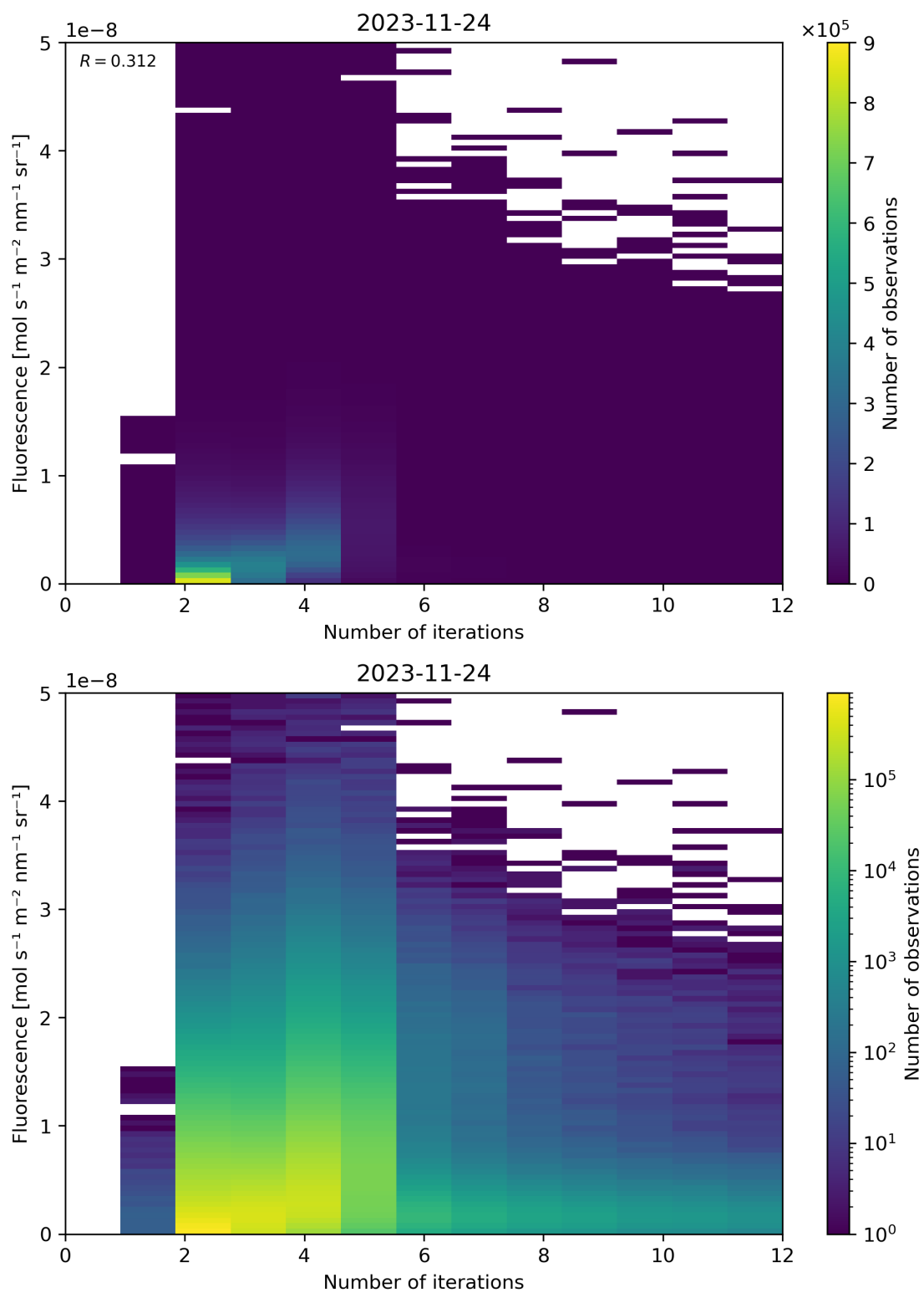
Figure 107: Scatter density plot of “Number of iterations” against “Fluorescence” for 2023-11-23 to 2023-11-25.
