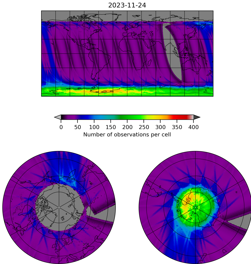
Figure 11: Map of the number of observations for 2023-11-23 to 2023-11-25
