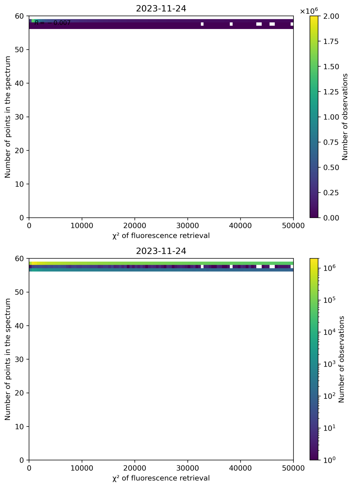
Figure 71: Scatter density plot of " \chi^2 of fluorescence retrieval" against "Number of points in the spectrum" for 2023-11-23 to 2023-11-25.
