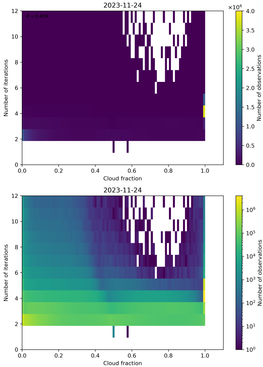
Figure 80: Scatter density plot of “Cloud fraction” against “Number of iterations” for 2023-11-23 to 2023-11-25.
