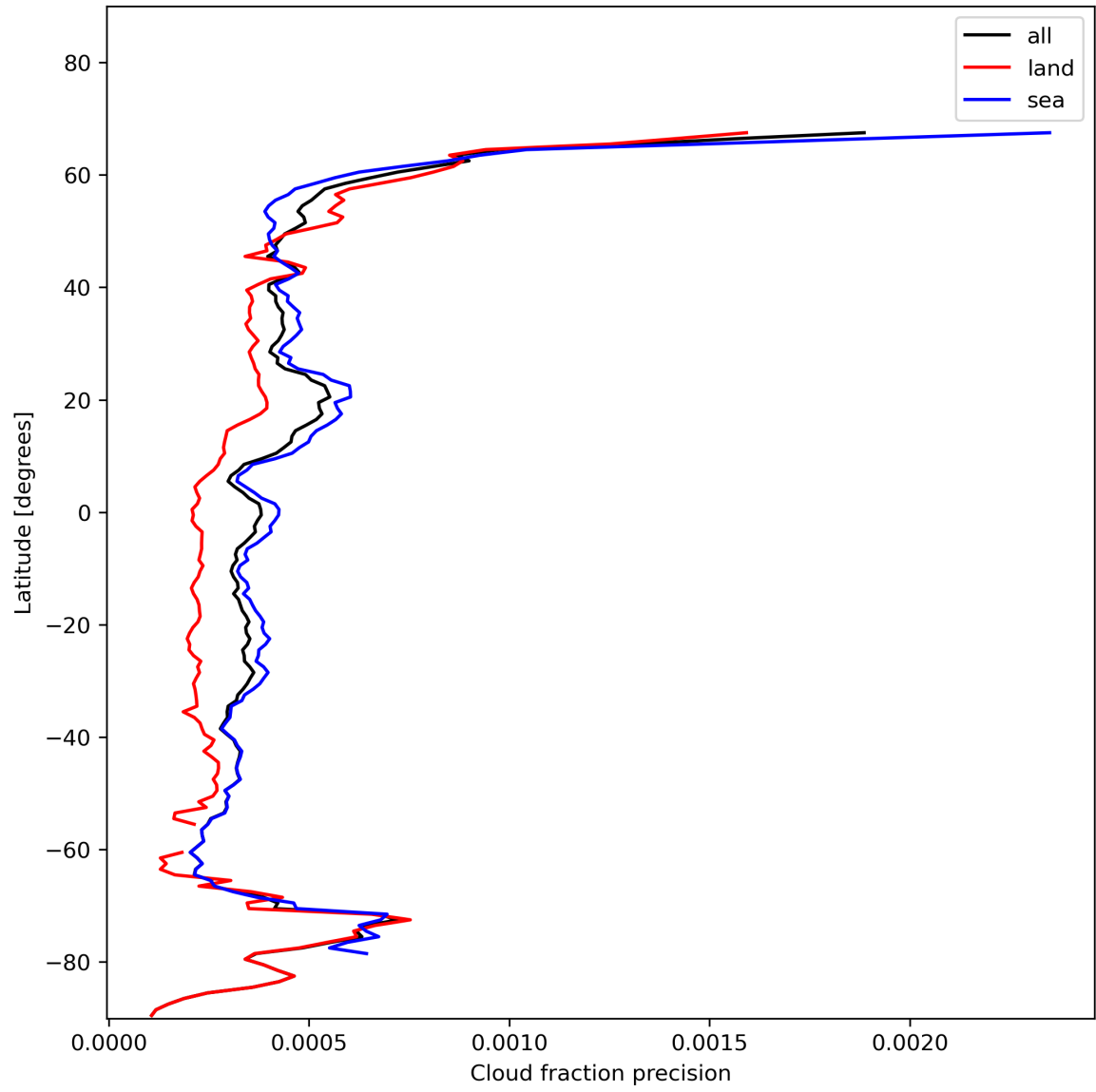
Figure 16: Zonal average of “Cloud fraction precision” for 2023-11-23 to 2023-11-25.
