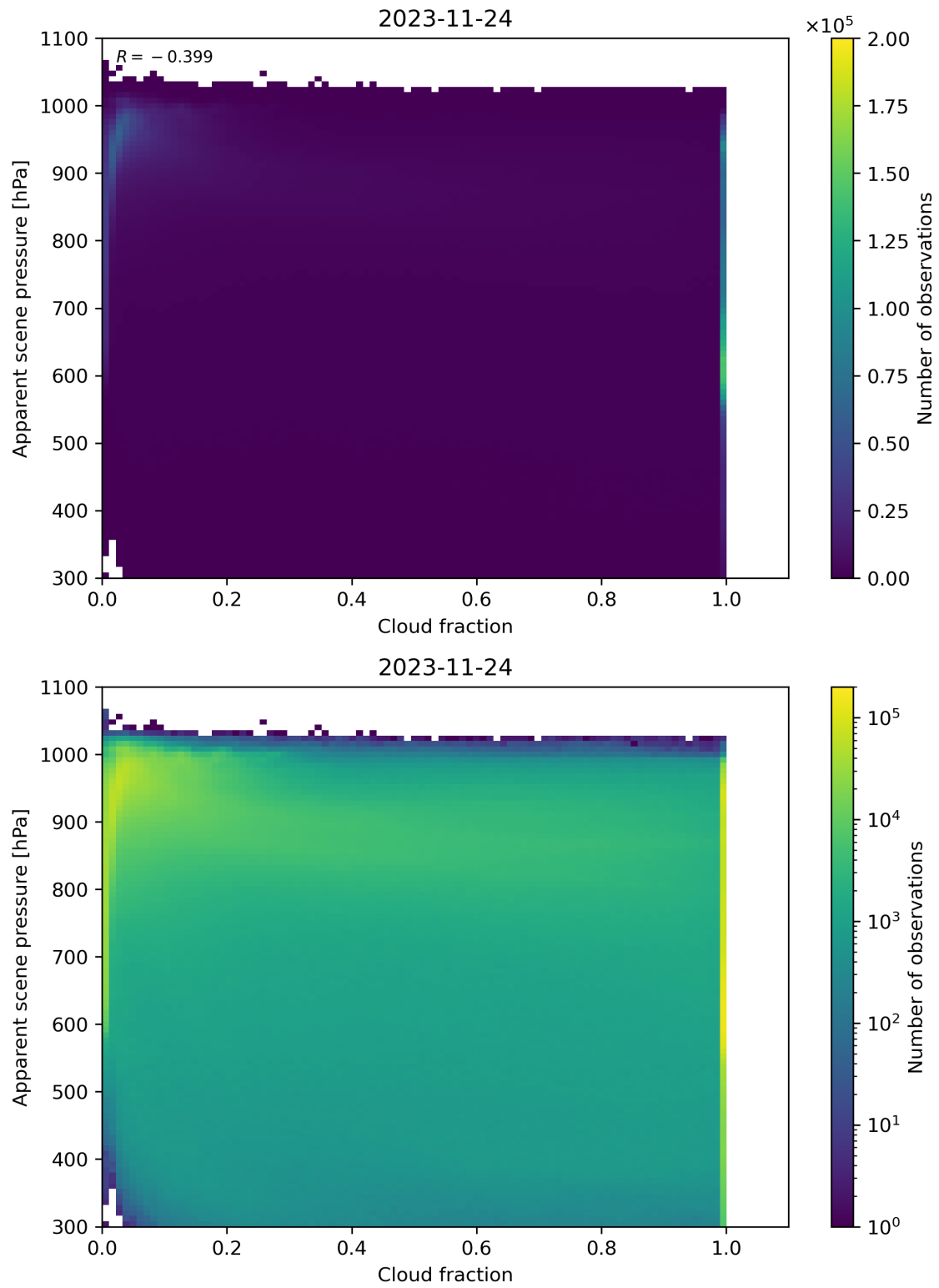
Figure 76: Scatter density plot of “Cloud fraction” against “Apparent scene pressure” for 2023-11-23 to 2023-11-25.
