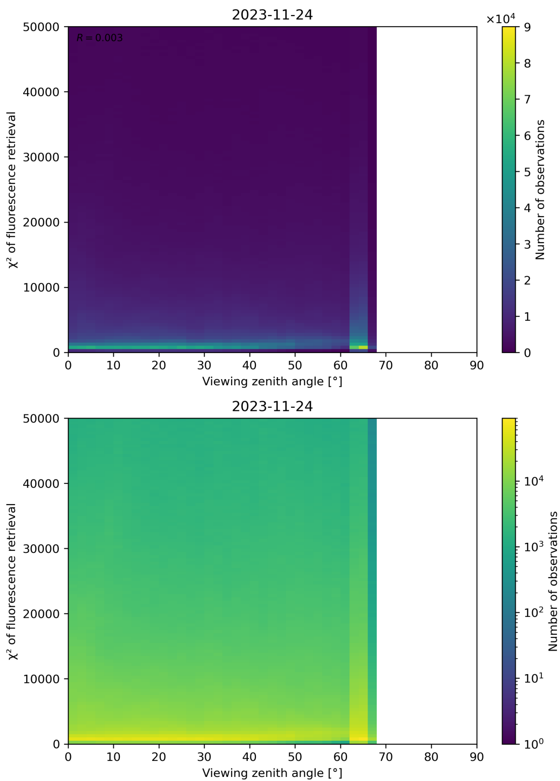
Figure 131: Scatter density plot of “Viewing zenith angle” against “ \chi^2 of fluorescence retrieval” for 2023-11-23 to 2023-11-25.
