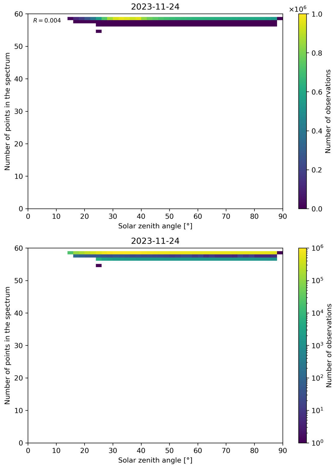
Figure 126: Scatter density plot of “Solar zenith angle” against “Number of points in the spectrum” for 2023-11-23 to 2023-11-25.
