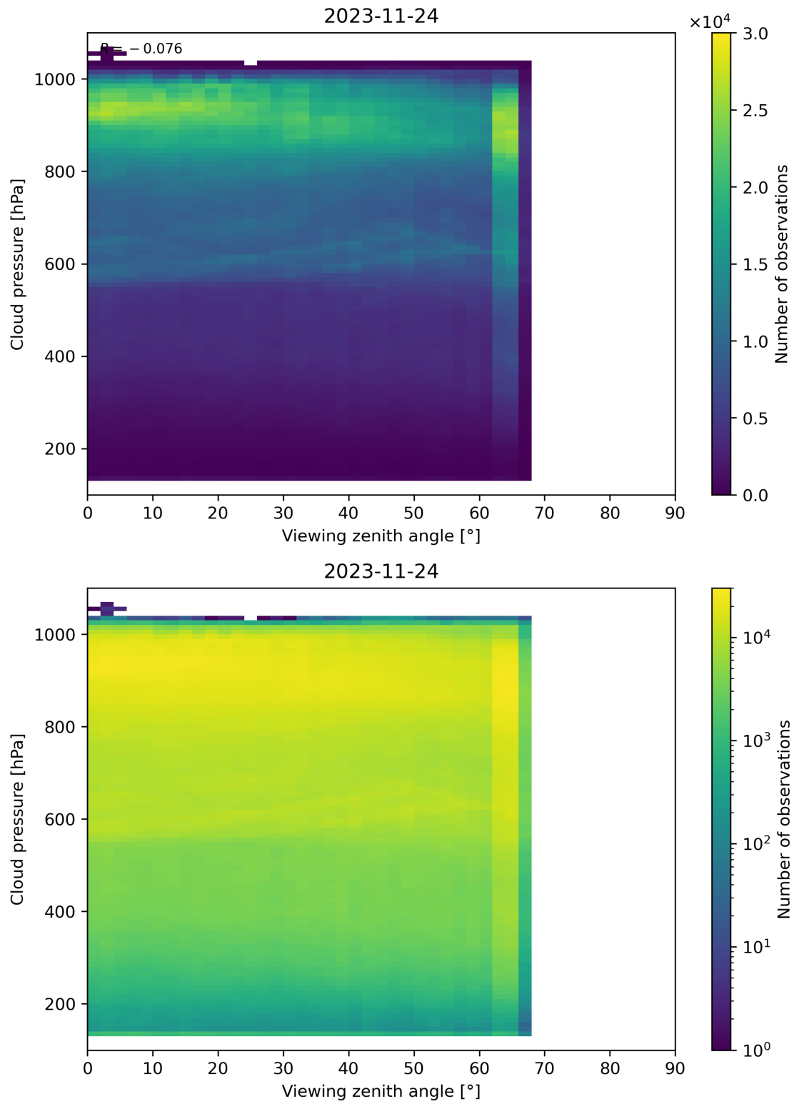
Figure 133: Scatter density plot of “Viewing zenith angle” against “Cloud pressure” for 2023-11-23 to 2023-11-25.
