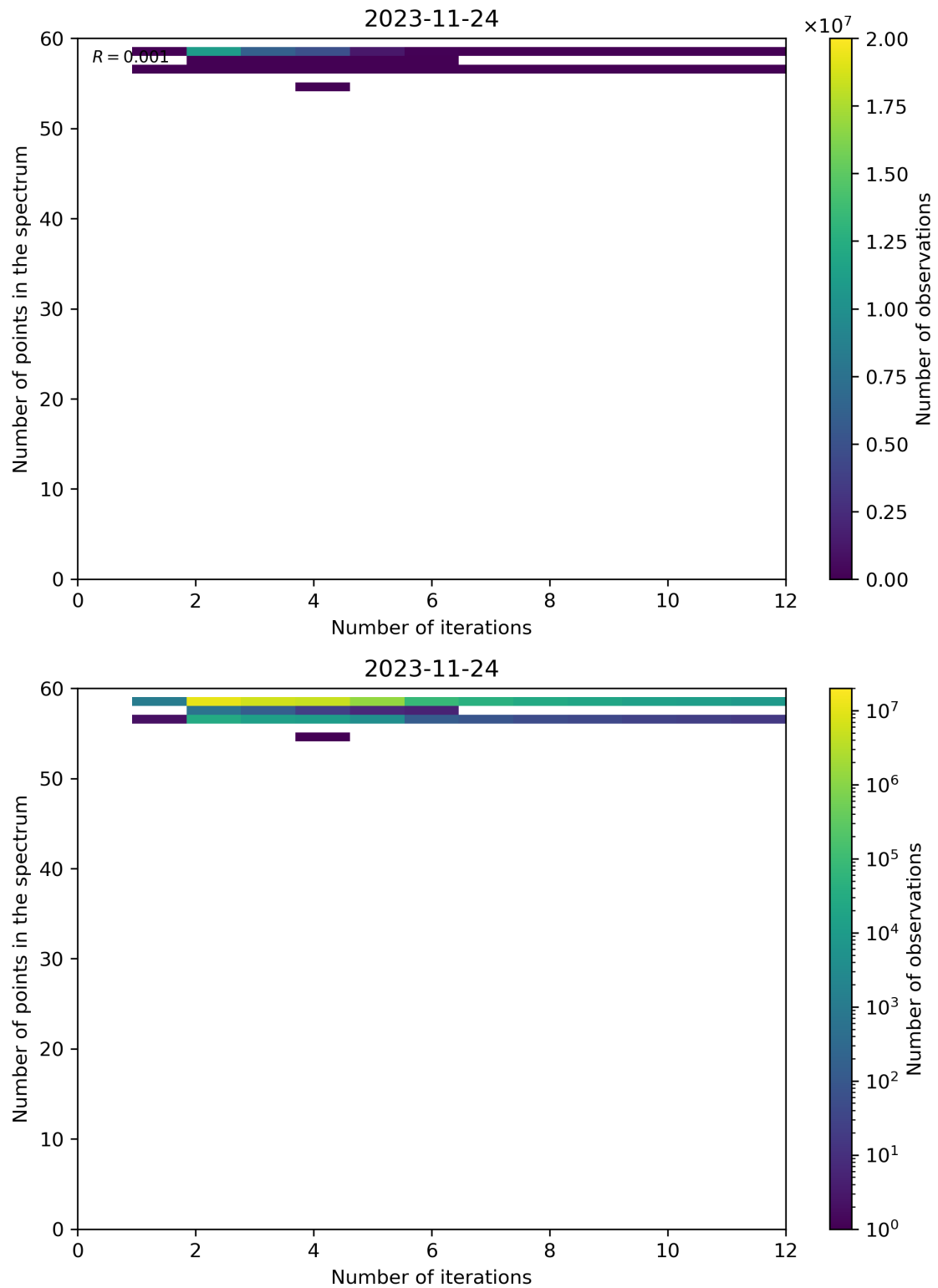
Figure 108: Scatter density plot of “Number of iterations” against “Number of points in the spectrum” for 2023-11-23 to 2023-11-25.
