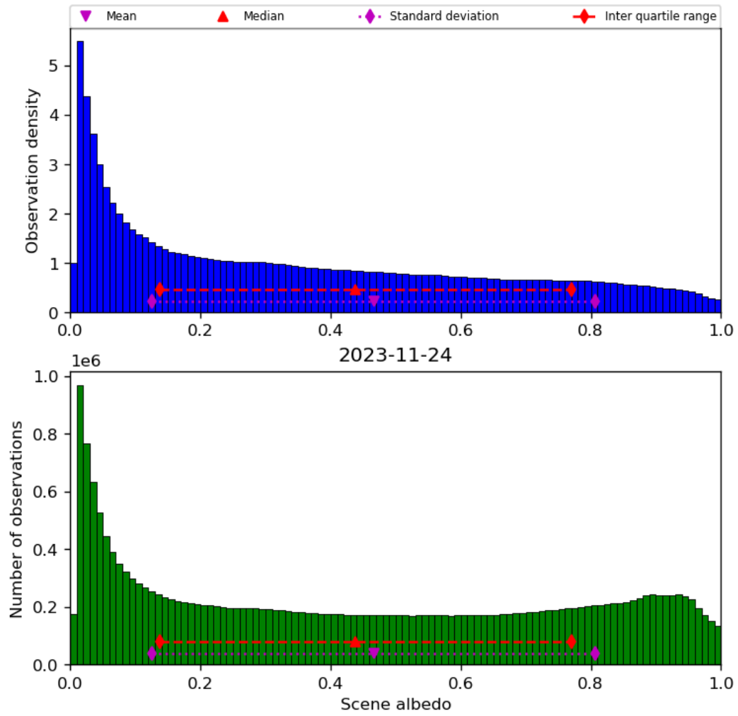
Figure 34: Histogram of “Scene albedo” for 2023-11-23 to 2023-11-25
