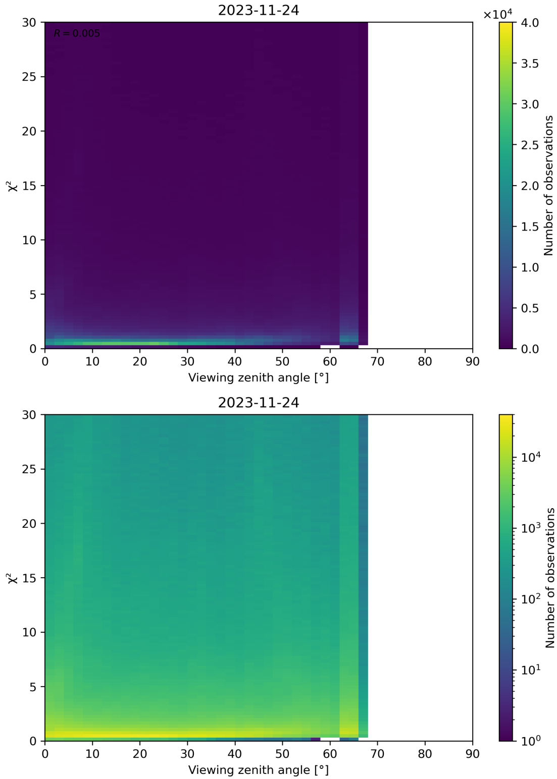
Figure 130: Scatter density plot of “Viewing zenith angle” against “ \chi^2 ” for 2023-11-23 to 2023-11-25.
