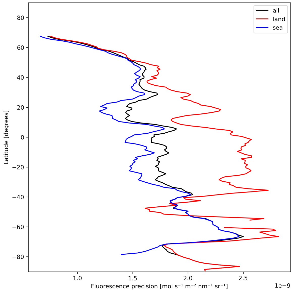
Figure 24: Zonal average of “Fluorescence precision” for 2023-11-23 to 2023-11-25.
