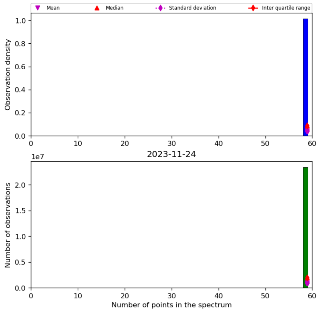
Figure 44: Histogram of “Number of points in the spectrum” for 2023-11-23 to 2023-11-25
