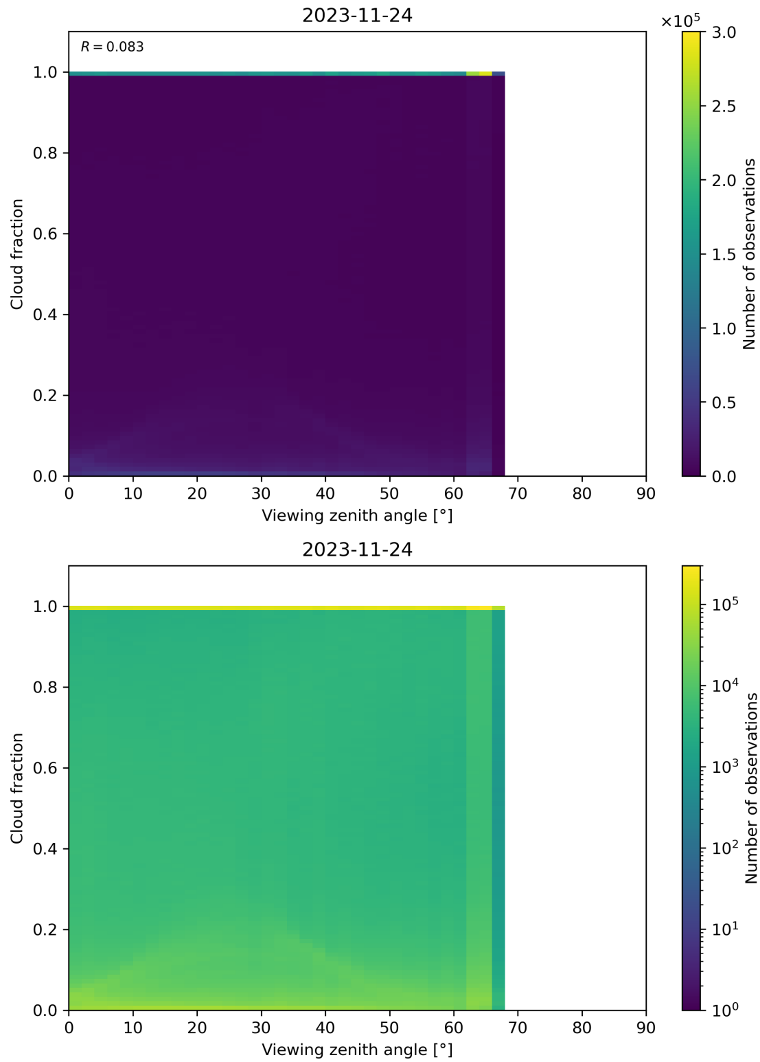
Figure 132: Scatter density plot of “Viewing zenith angle” against “Cloud fraction” for 2023-11-23 to 2023-11-25.
