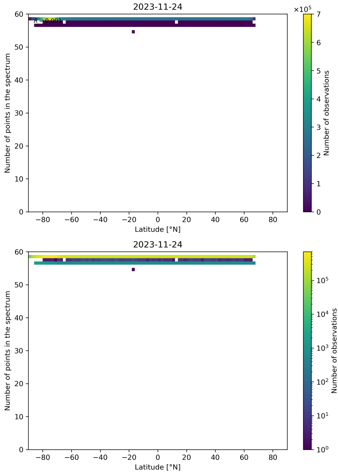
Figure 103: Scatter density plot of “Latitude” against “Number of points in the spectrum” for 2023-11-23 to 2023-11-25.
