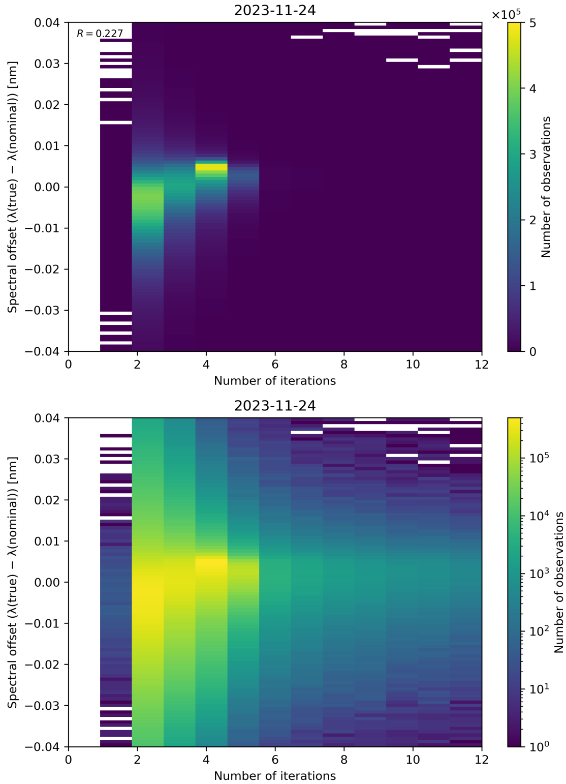
Figure 109: Scatter density plot of “Number of iterations” against “Spectral offset ( \lambda(\text{true}) - \lambda(\text{nominal}) )” for 2023-11-23 to 2023-11-25.
