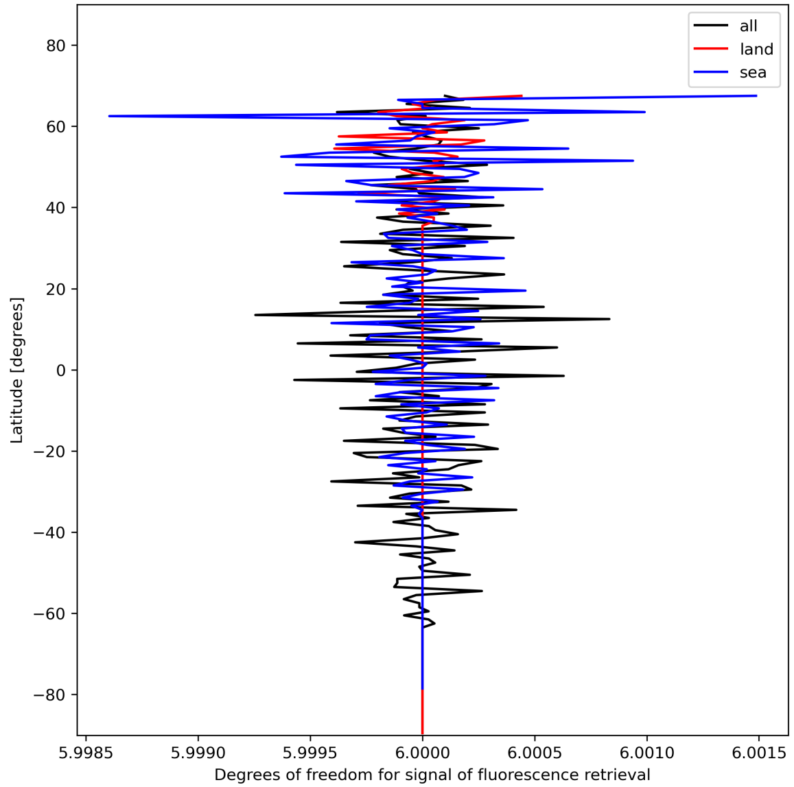
Figure 26: Zonal average of “Degrees of freedom for signal of fluorescence retrieval” for 2023-11-23 to 2023-11-25.
