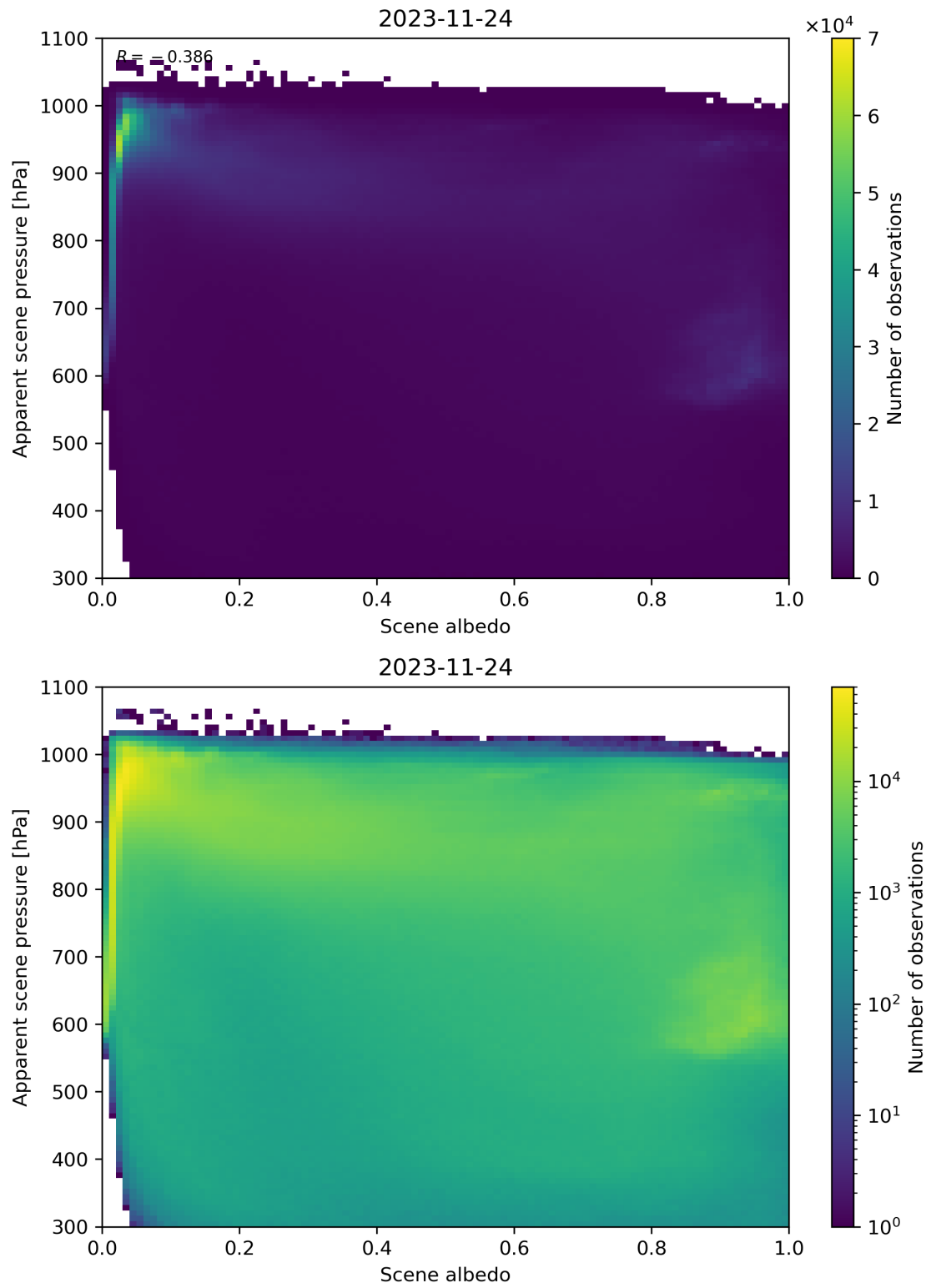
Figure 111: Scatter density plot of “Scene albedo” against “Apparent scene pressure” for 2023-11-23 to 2023-11-25.
