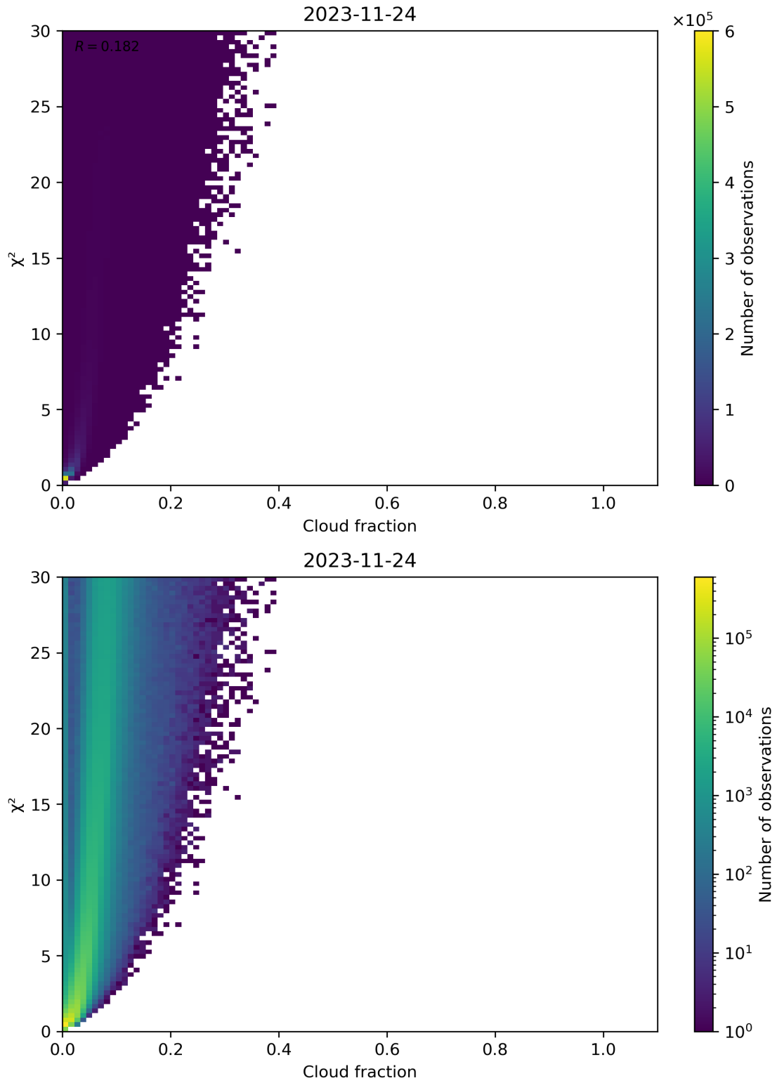
Figure 77: Scatter density plot of “Cloud fraction” against “ \chi^2 ” for 2023-11-23 to 2023-11-25.
