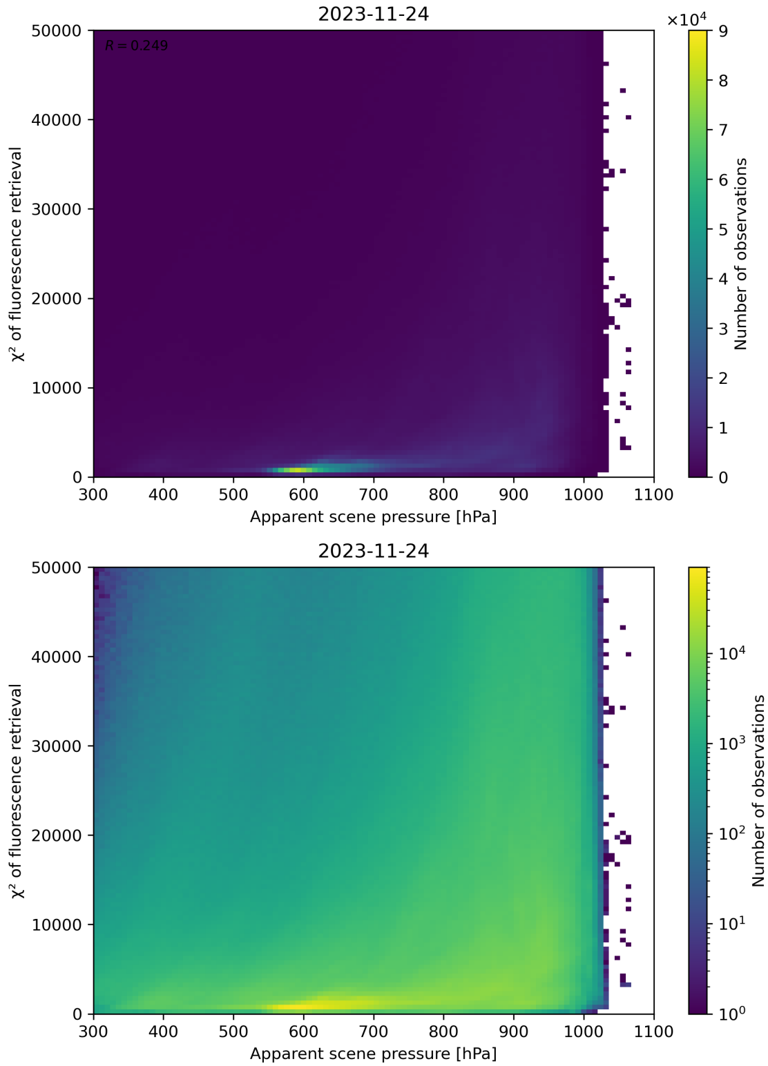
Figure 64: Scatter density plot of “Apparent scene pressure” against “ \chi^2 of fluorescence retrieval” for 2023-11-23 to 2023-11-25.
