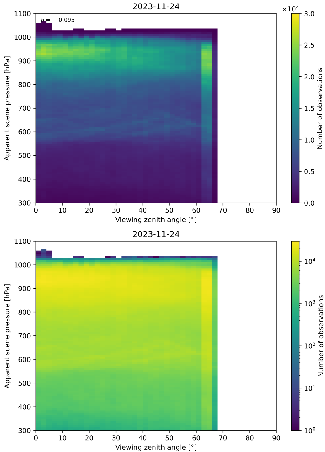
Figure 129: Scatter density plot of “Viewing zenith angle” against “Apparent scene pressure” for 2023-11-23 to 2023-11-25.
