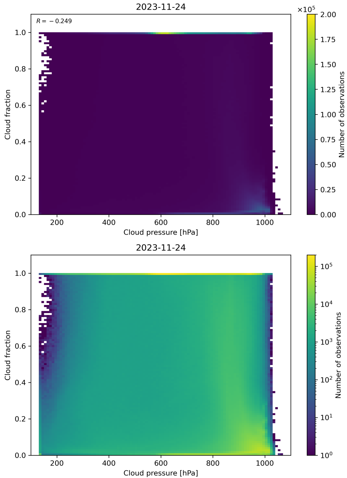
Figure 87: Scatter density plot of “Cloud pressure” against “Cloud fraction” for 2023-11-23 to 2023-11-25.
