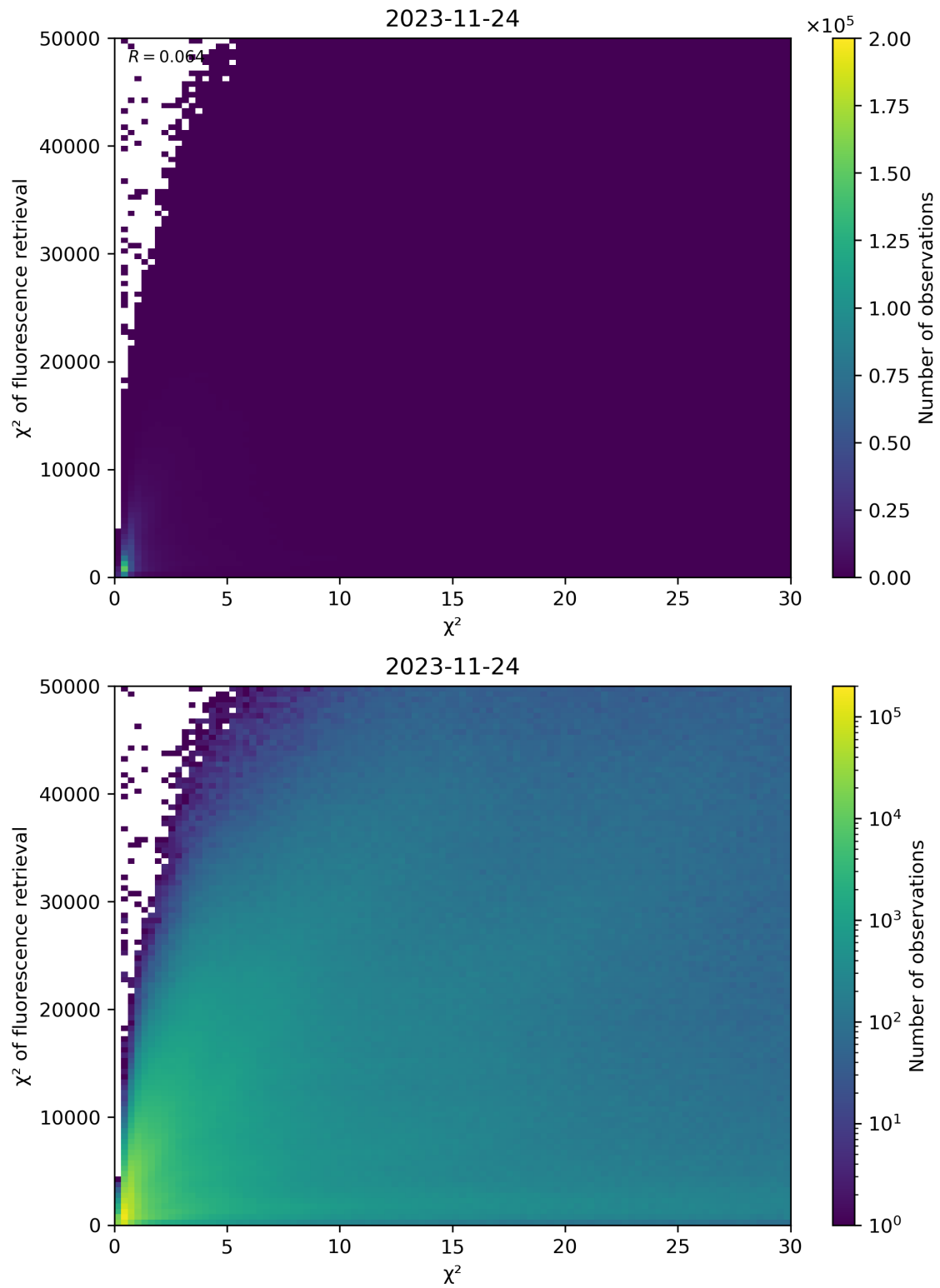
Figure 69: Scatter density plot of “ \chi^2 ” against “ \chi^2 of fluorescence retrieval” for 2023-11-23 to 2023-11-25.
