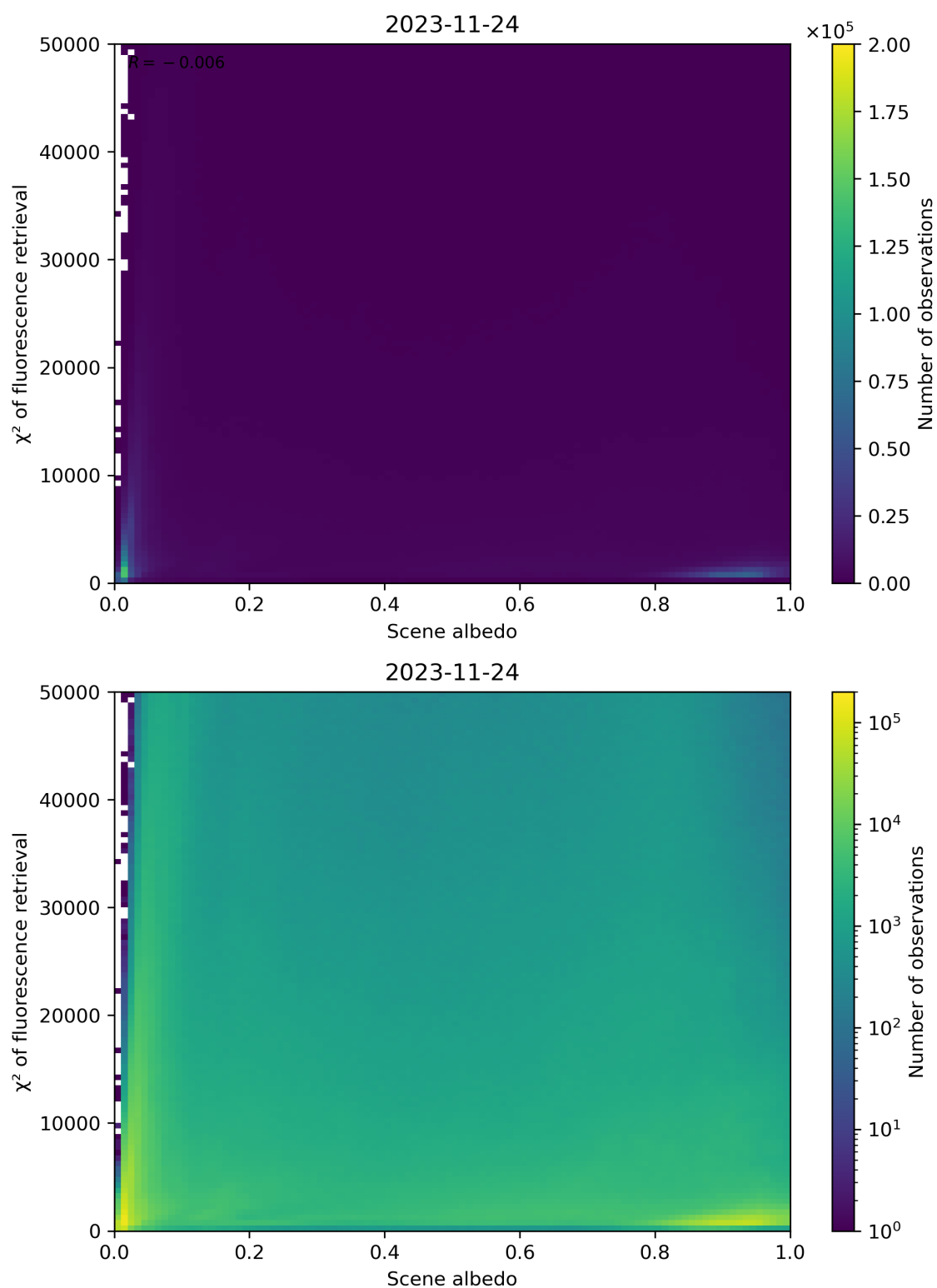
Figure 113: Scatter density plot of “Scene albedo” against “ \chi^2 of fluorescence retrieval” for 2023-11-23 to 2023-11-25.
