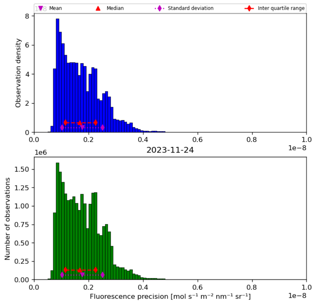
Figure 41: Histogram of “Fluorescence precision” for 2023-11-23 to 2023-11-25
