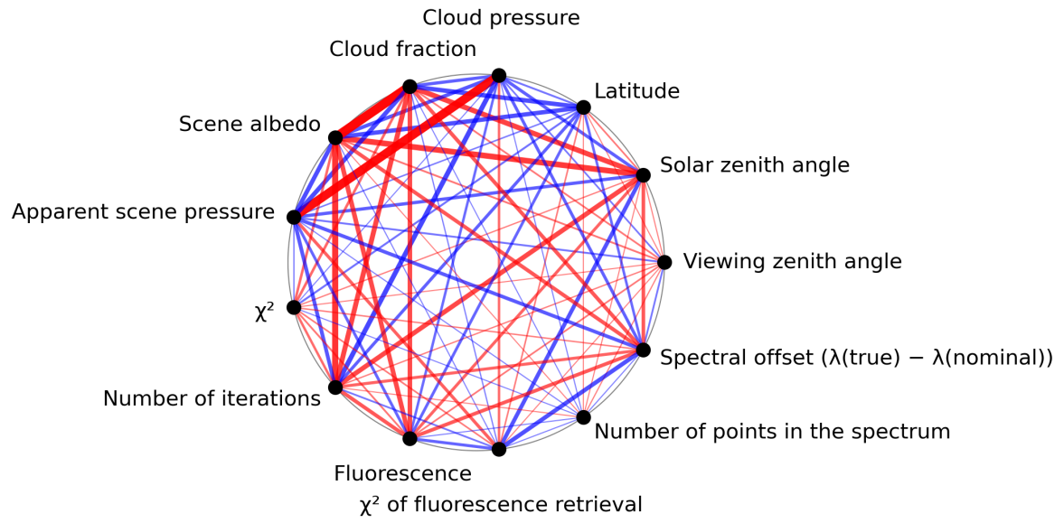
Figure 1: Map of correlation graph for 2023-11-23 to 2023-11-25.
