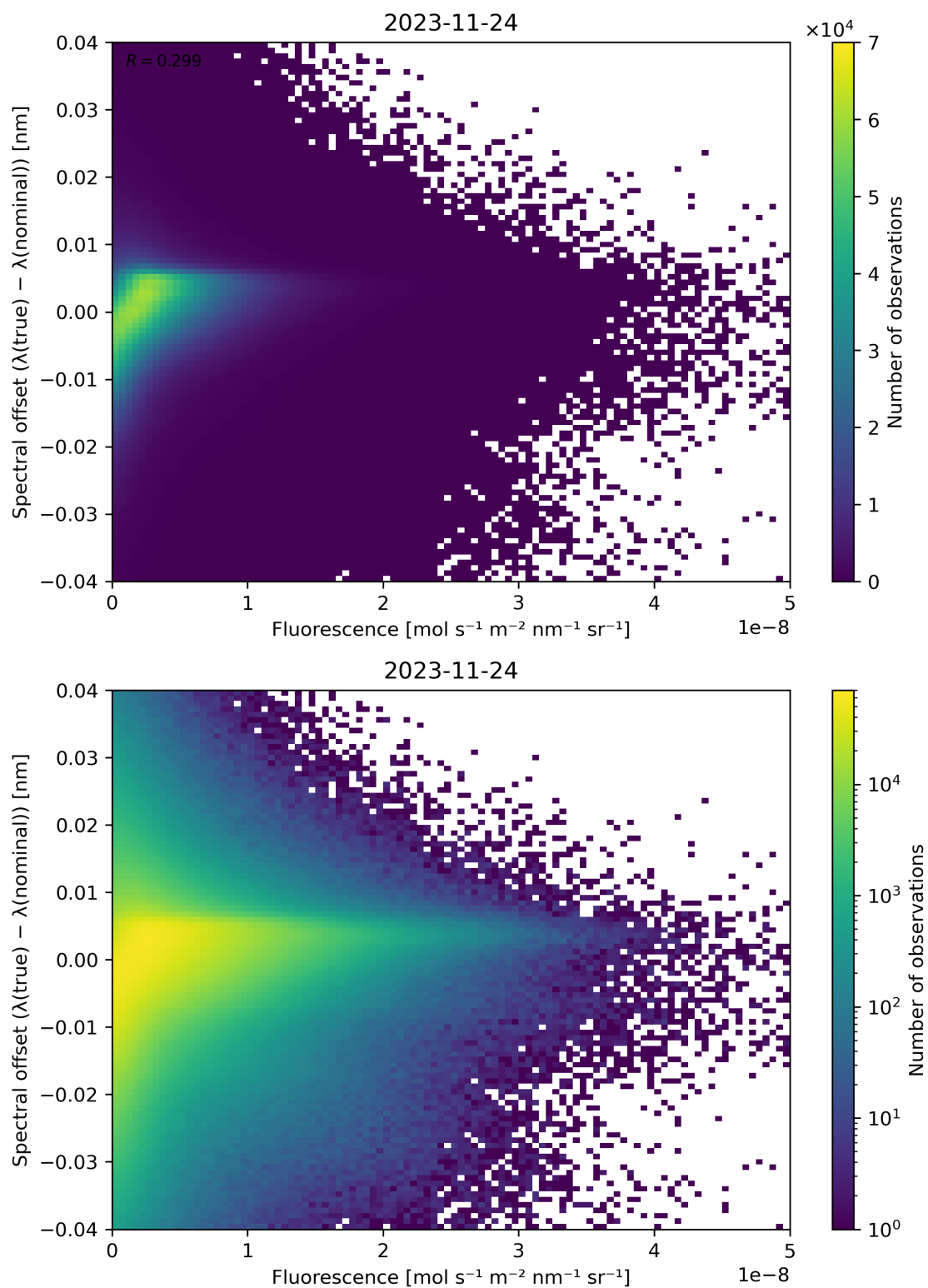
Figure 95: Scatter density plot of “Fluorescence” against “Spectral offset ( \lambda(\text{true}) - \lambda(\text{nominal}) )” for 2023-11-23 to 2023-11-25.
