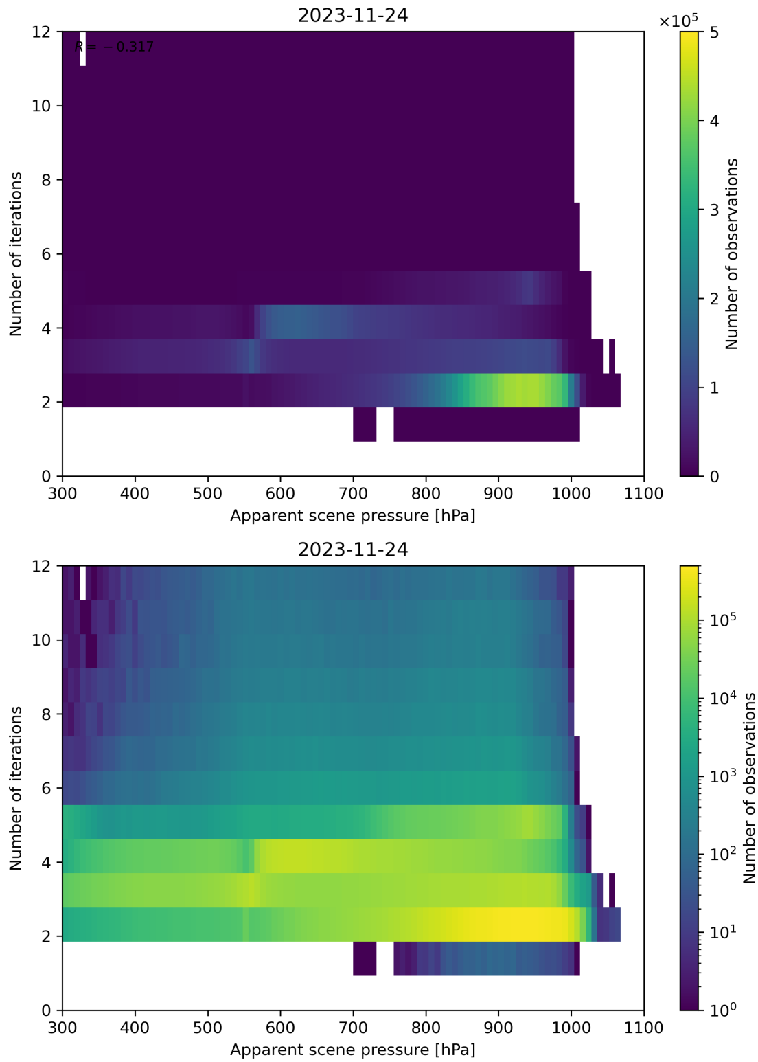
Figure 66: Scatter density plot of “Apparent scene pressure” against “Number of iterations” for 2023-11-23 to 2023-11-25.
