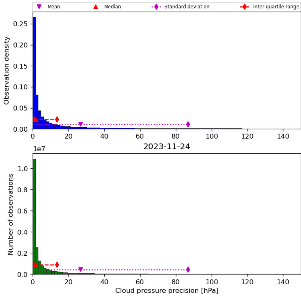
Figure 31: Histogram of “Cloud pressure precision” for 2023-11-23 to 2023-11-25
