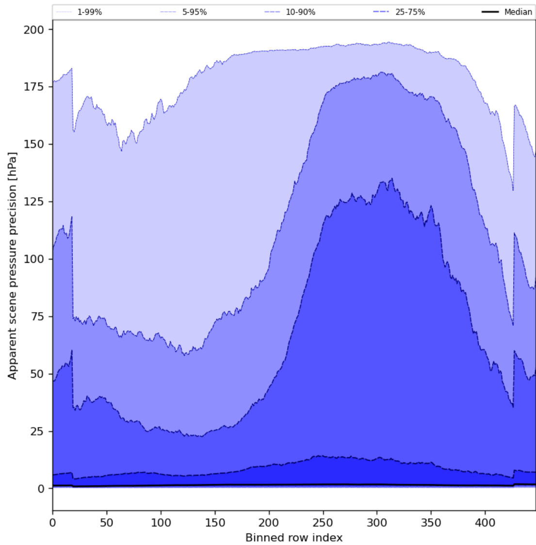
Figure 54: Along track statistics of “Apparent scene pressure precision” for 2023-11-23 to 2023-11-25
