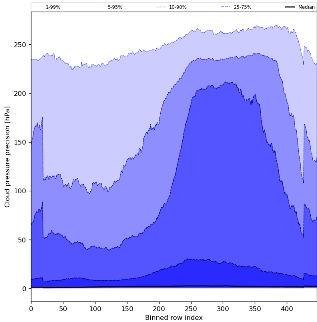
Figure 48: Along track statistics of “Cloud pressure precision” for 2023-11-23 to 2023-11-25
