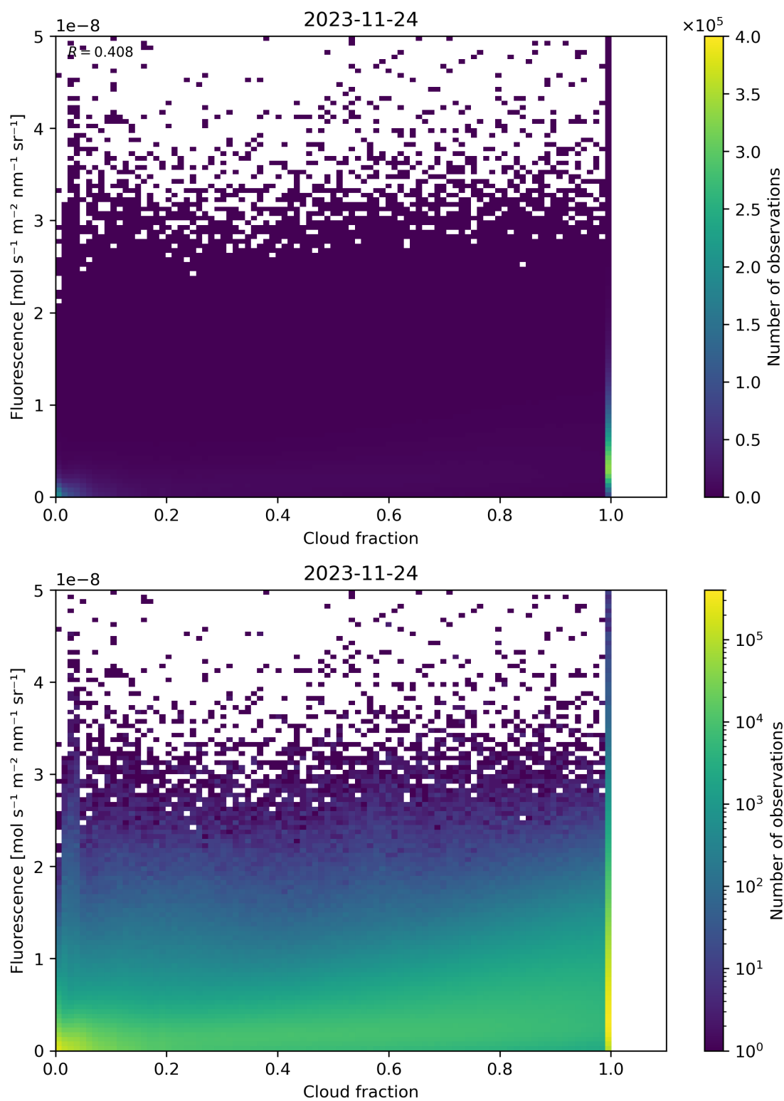
Figure 79: Scatter density plot of “Cloud fraction” against “Fluorescence” for 2023-11-23 to 2023-11-25.
