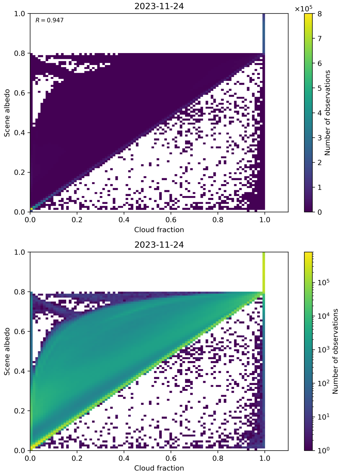
Figure 82: Scatter density plot of “Cloud fraction” against “Scene albedo” for 2023-11-23 to 2023-11-25.
