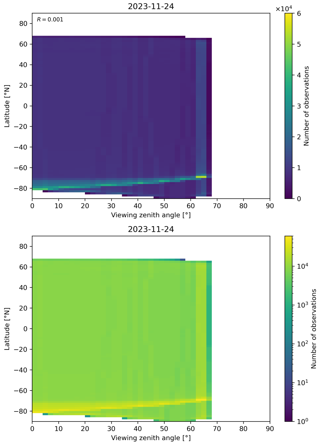
Figure 135: Scatter density plot of “Viewing zenith angle” against “Latitude” for 2023-11-23 to 2023-11-25.
