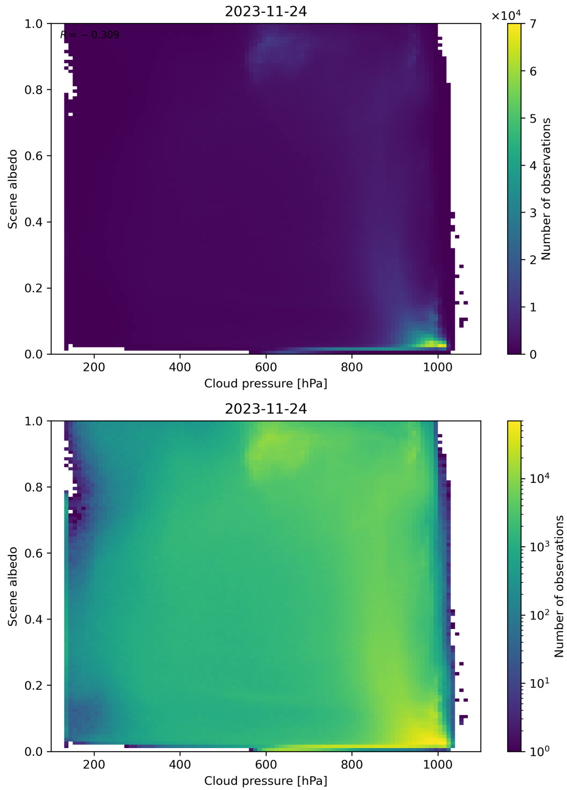
Figure 91: Scatter density plot of “Cloud pressure” against “Scene albedo” for 2023-11-23 to 2023-11-25.
