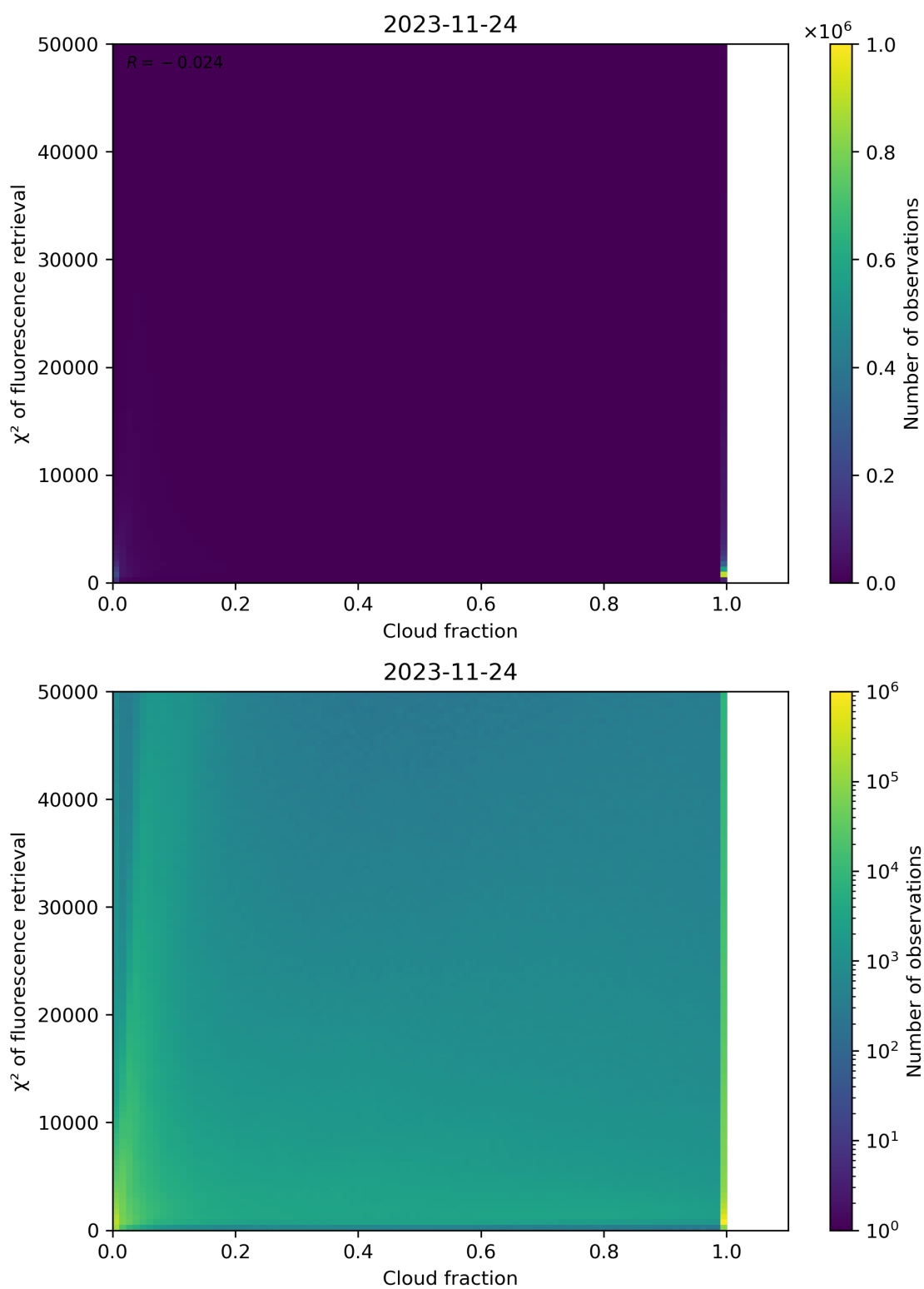
Figure 78: Scatter density plot of “Cloud fraction” against “ \chi^2 of fluorescence retrieval” for 2023-11-23 to 2023-11-25.
