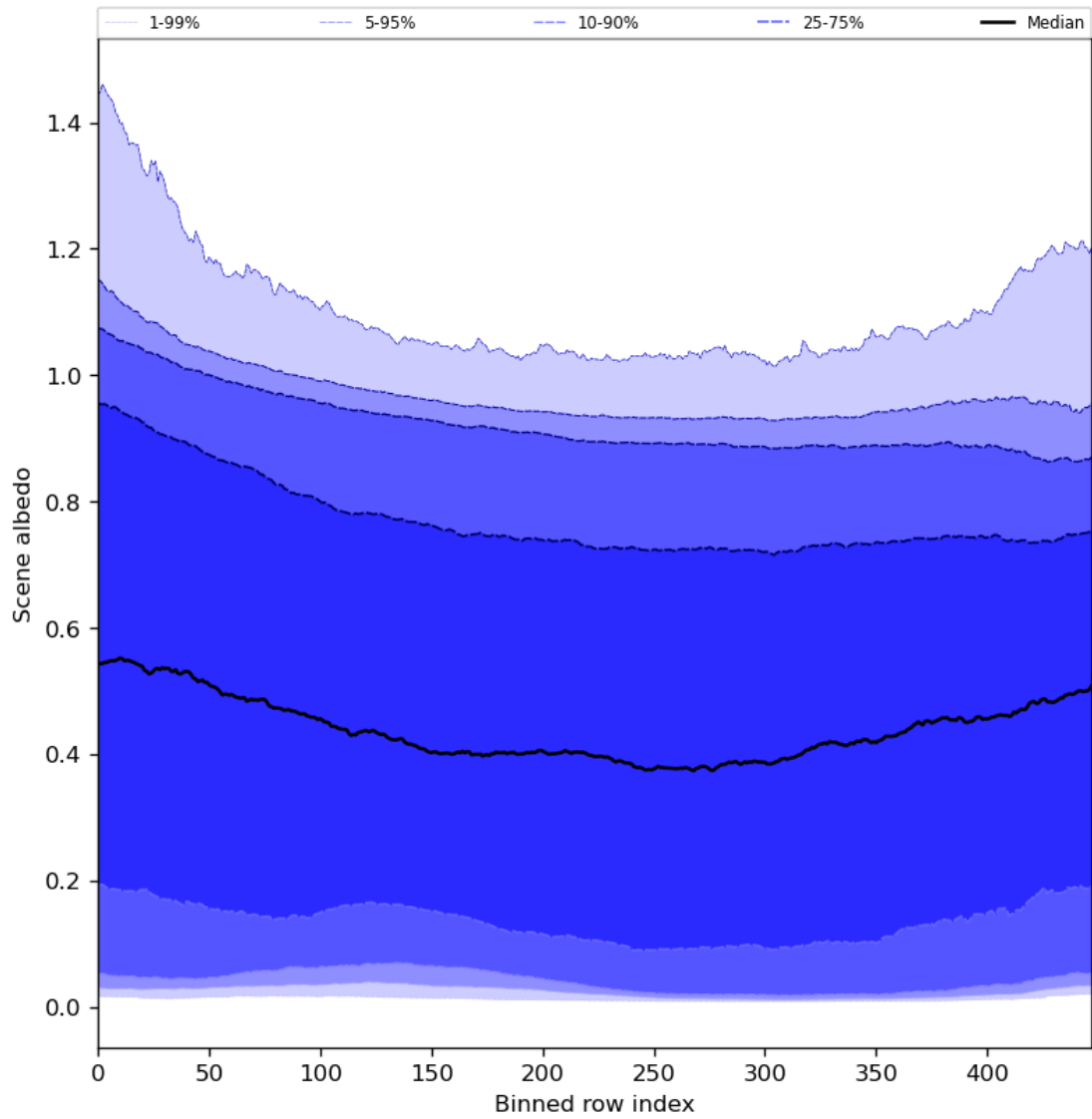
Figure 51: Along track statistics of “Scene albedo” for 2023-11-23 to 2023-11-25
