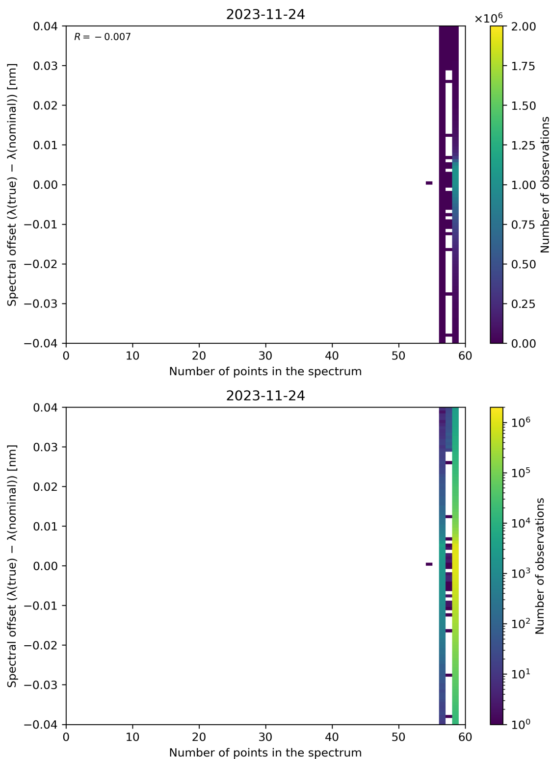
Figure 110: Scatter density plot of “Number of points in the spectrum” against “Spectral offset ( \lambda(\text{true}) - \lambda(\text{nominal}) )” for 2023-11-23 to 2023-11-25.
