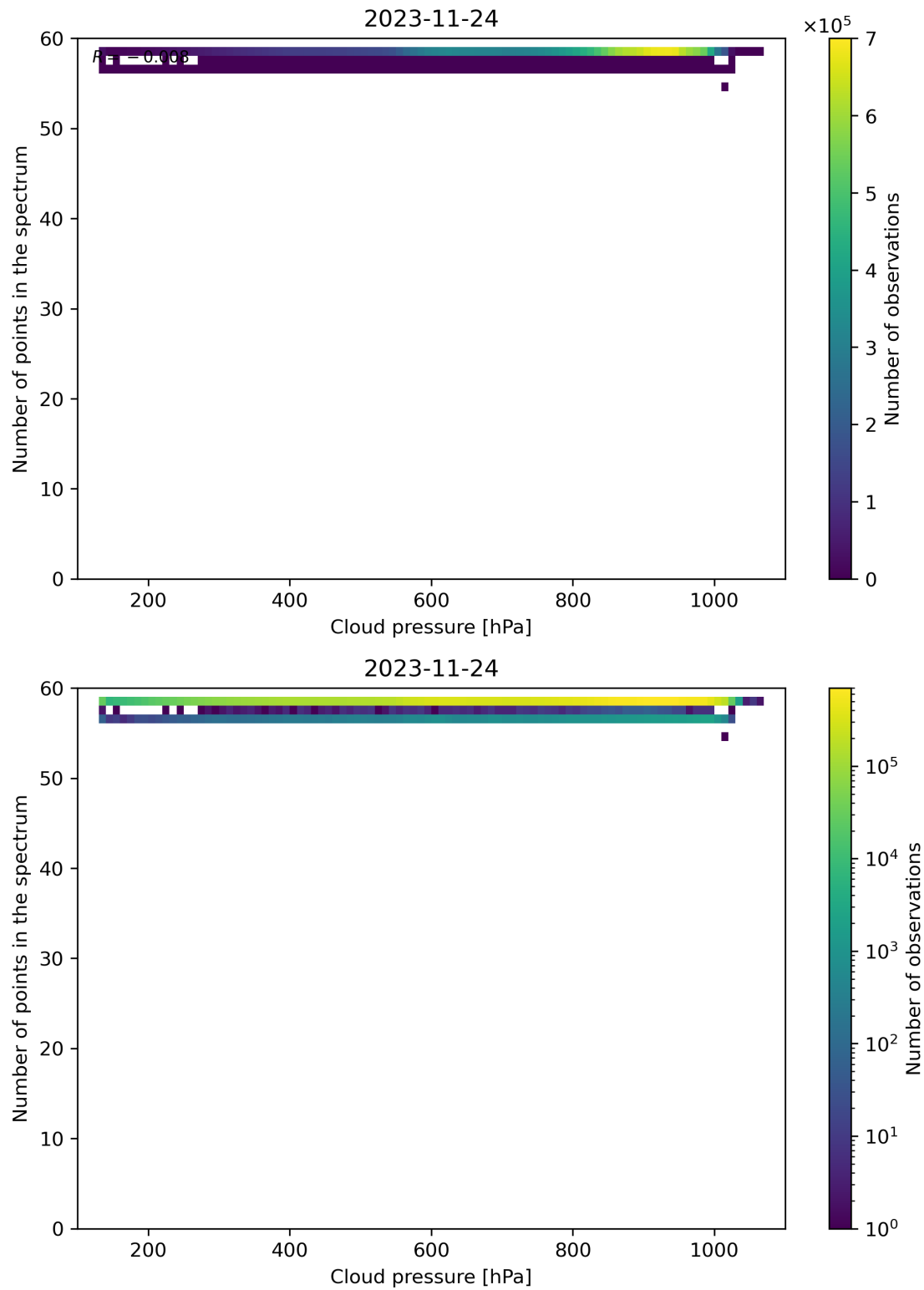
Figure 90: Scatter density plot of “Cloud pressure” against “Number of points in the spectrum” for 2023-11-23 to 2023-11-25.
