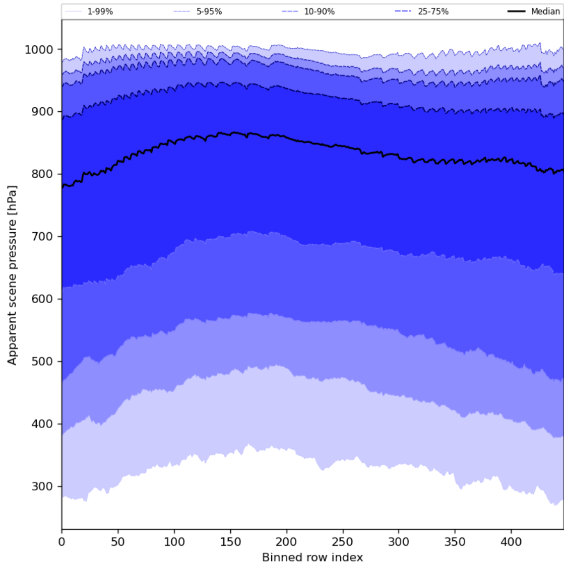
Figure 53: Along track statistics of “Apparent scene pressure” for 2023-11-23 to 2023-11-25
