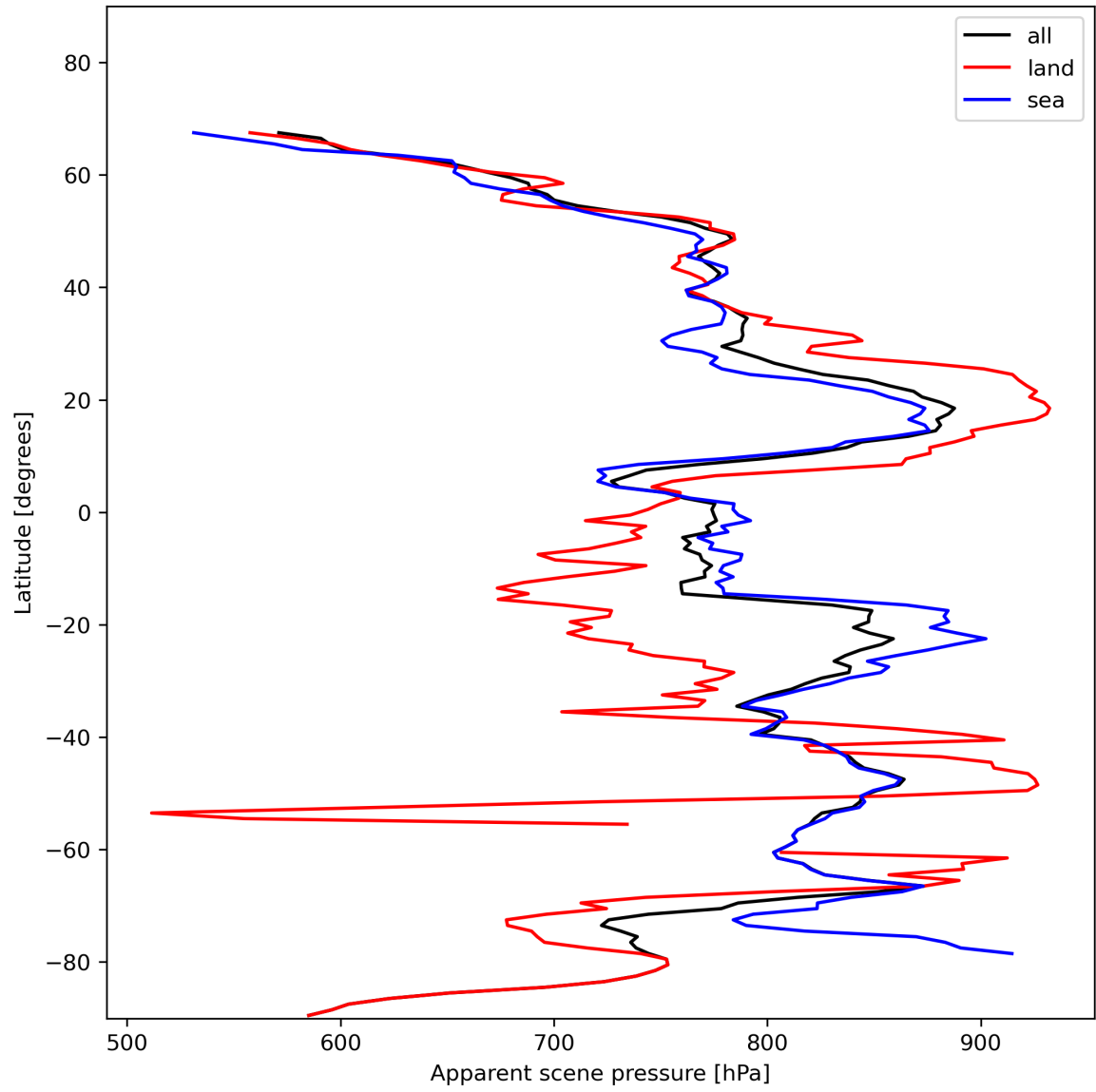
Figure 19: Zonal average of “Apparent scene pressure” for 2023-11-23 to 2023-11-25.
