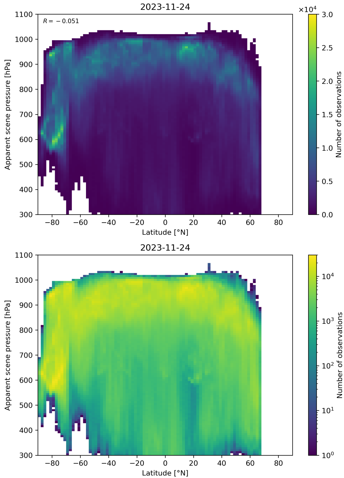
Figure 96: Scatter density plot of “Latitude” against “Apparent scene pressure” for 2023-11-23 to 2023-11-25.
