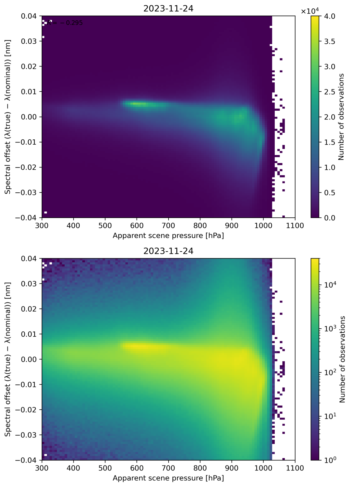
Figure 68: Scatter density plot of “Apparent scene pressure” against “Spectral offset ( \lambda(\text{true}) - \lambda(\text{nominal}) )” for 2023-11-23 to 2023-11-25.
