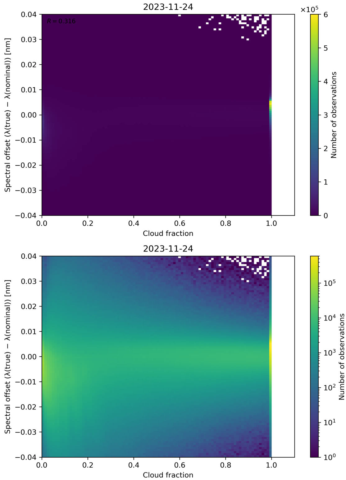
Figure 83: Scatter density plot of “Cloud fraction” against “Spectral offset ( \lambda(\text{true}) - \lambda(\text{nominal}) )” for 2023-11-23 to 2023-11-25.
