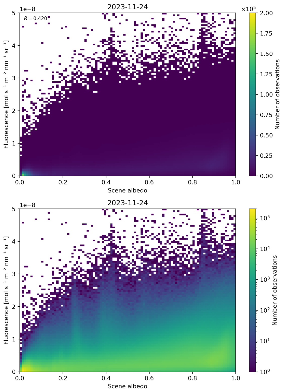
Figure 114: Scatter density plot of “Scene albedo” against “Fluorescence” for 2023-11-23 to 2023-11-25.
