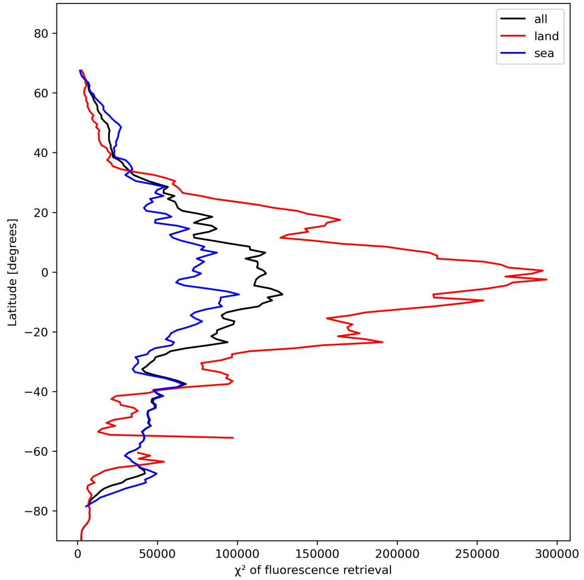
Figure 25: Zonal average of “ \chi^2 of fluorescence retrieval” for 2023-11-23 to 2023-11-25.
