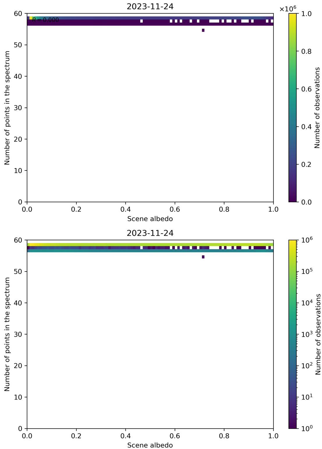
Figure 116: Scatter density plot of “Scene albedo” against “Number of points in the spectrum” for 2023-11-23 to 2023-11-25.
