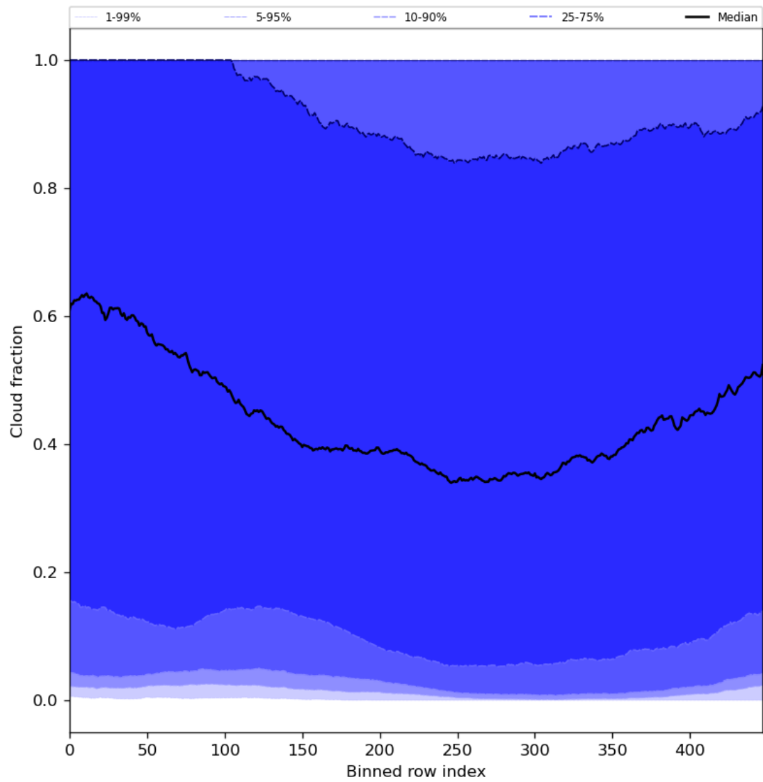
Figure 49: Along track statistics of “Cloud fraction” for 2023-11-23 to 2023-11-25
