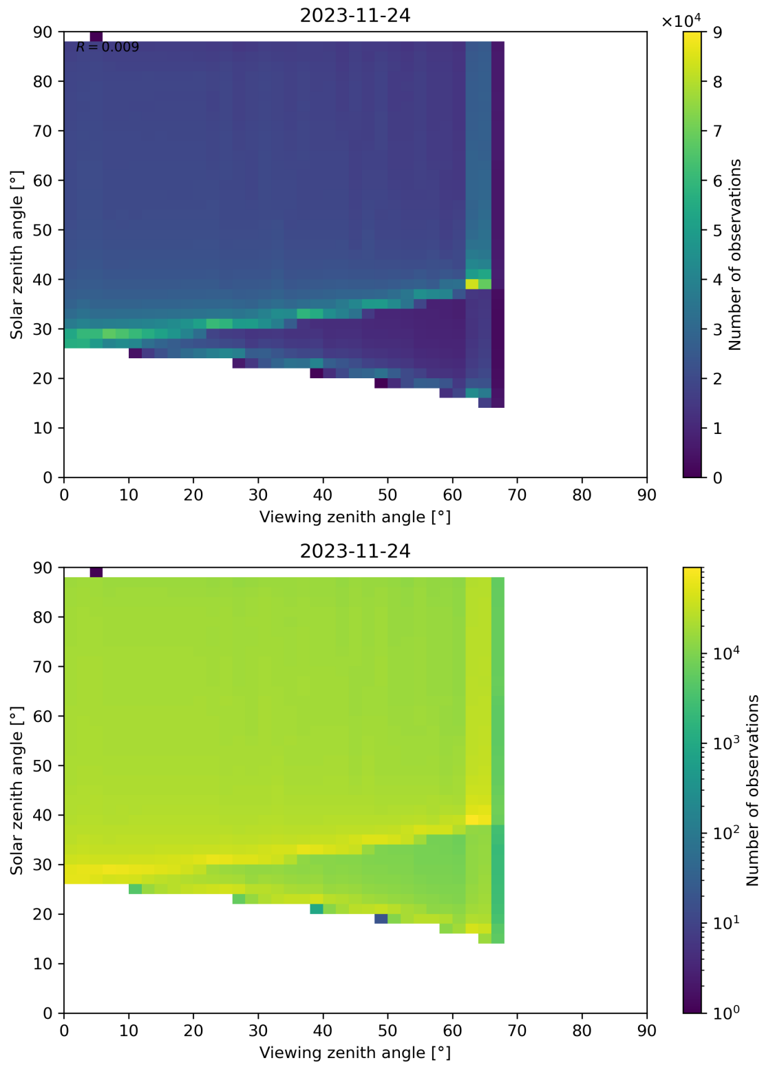
Figure 139: Scatter density plot of “Viewing zenith angle” against “Solar zenith angle” for 2023-11-23 to 2023-11-25.
