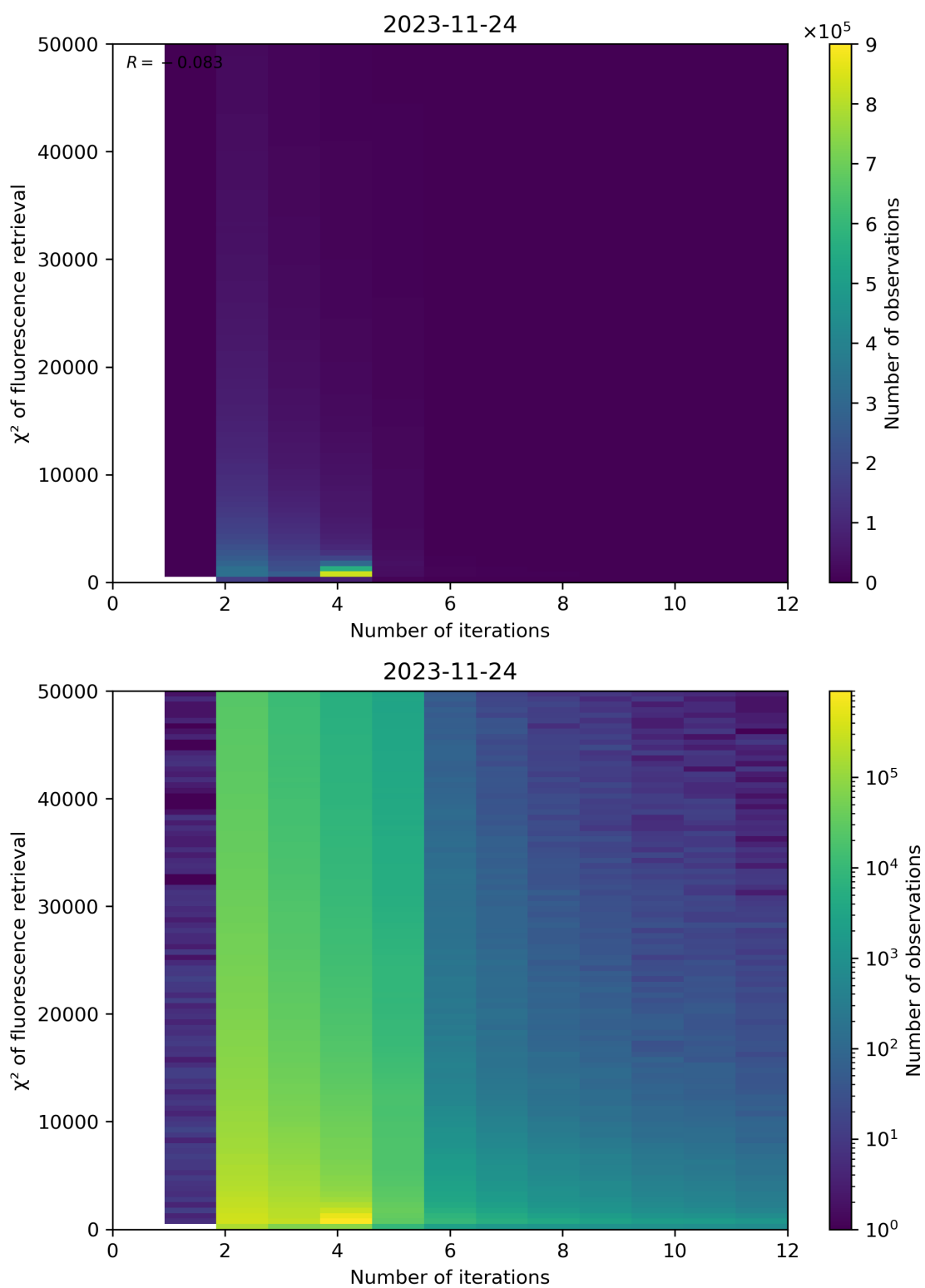
Figure 106: Scatter density plot of “Number of iterations” against “ \chi^2 of fluorescence retrieval” for 2023-11-23 to 2023-11-25.
