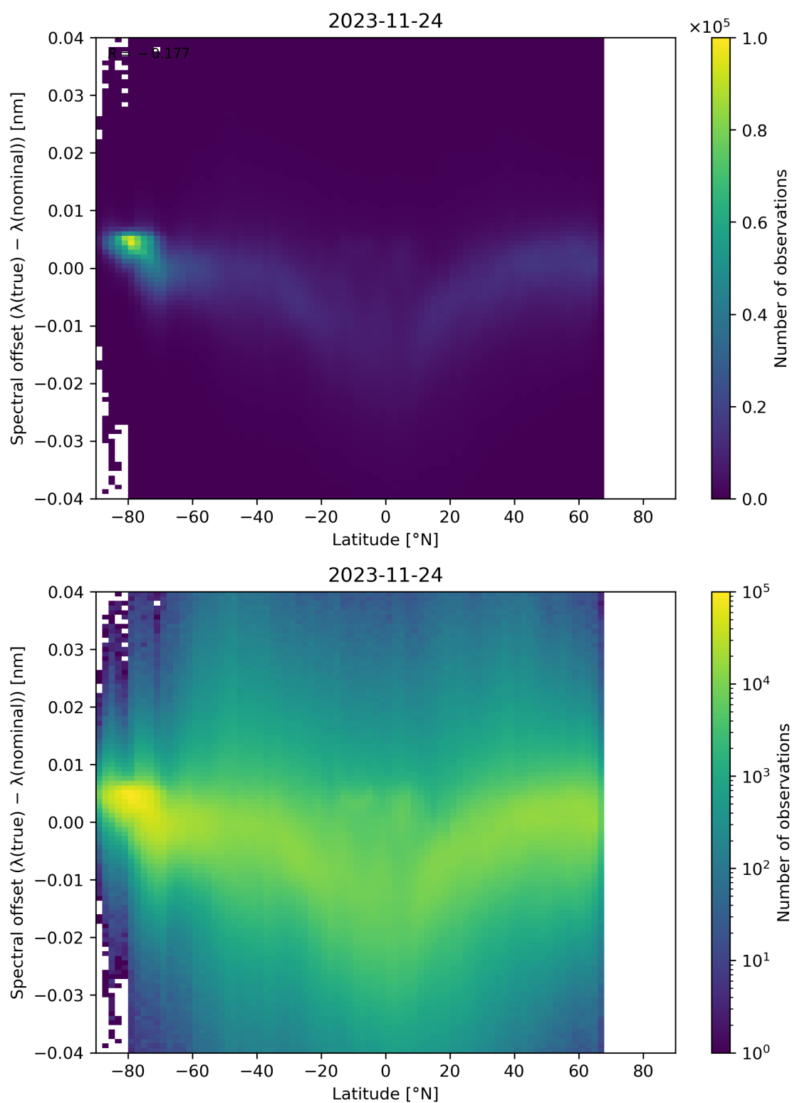
Figure 105: Scatter density plot of “Latitude” against “Spectral offset ( \lambda(\text{true}) - \lambda(\text{nominal}) )” for 2023-11-23 to 2023-11-25.
