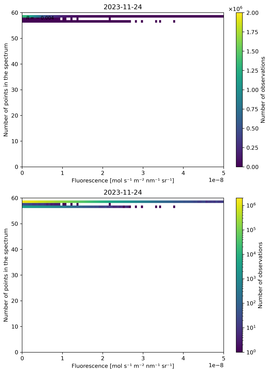
Figure 94: Scatter density plot of “Fluorescence” against “Number of points in the spectrum” for 2023-11-23 to 2023-11-25.
