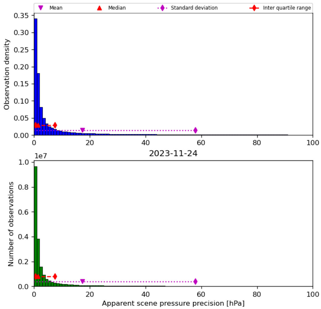
Figure 37: Histogram of “Apparent scene pressure precision” for 2023-11-23 to 2023-11-25
