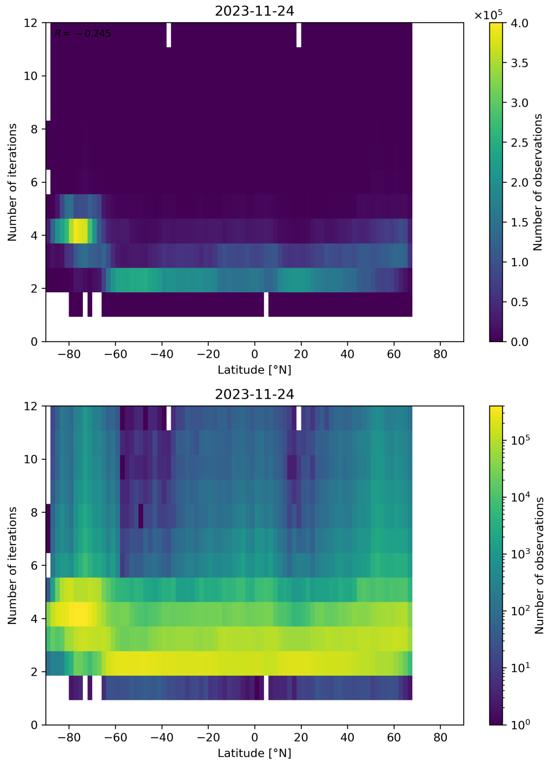
Figure 102: Scatter density plot of “Latitude” against “Number of iterations” for 2023-11-23 to 2023-11-25.
