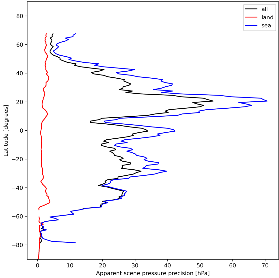
Figure 20: Zonal average of “Apparent scene pressure precision” for 2023-11-23 to 2023-11-25.
