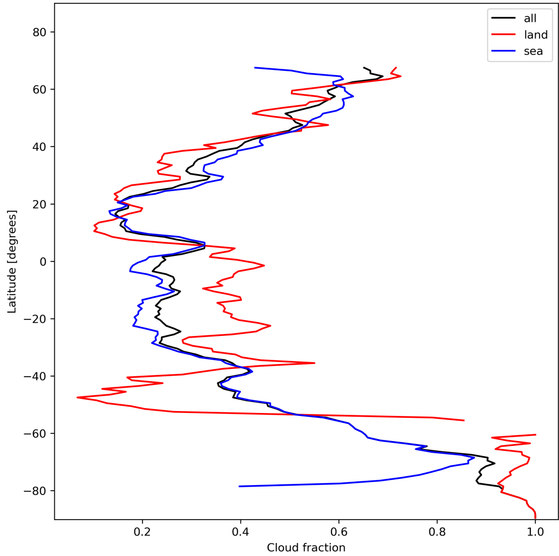
Figure 15: Zonal average of “Cloud fraction” for 2023-11-23 to 2023-11-25.
