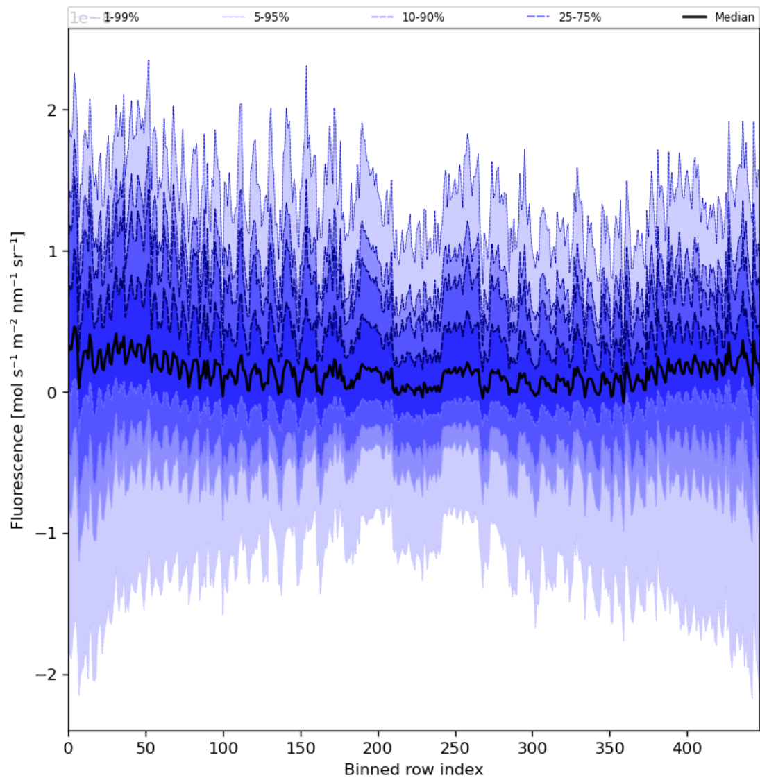
Figure 57: Along track statistics of “Fluorescence” for 2023-11-23 to 2023-11-25
