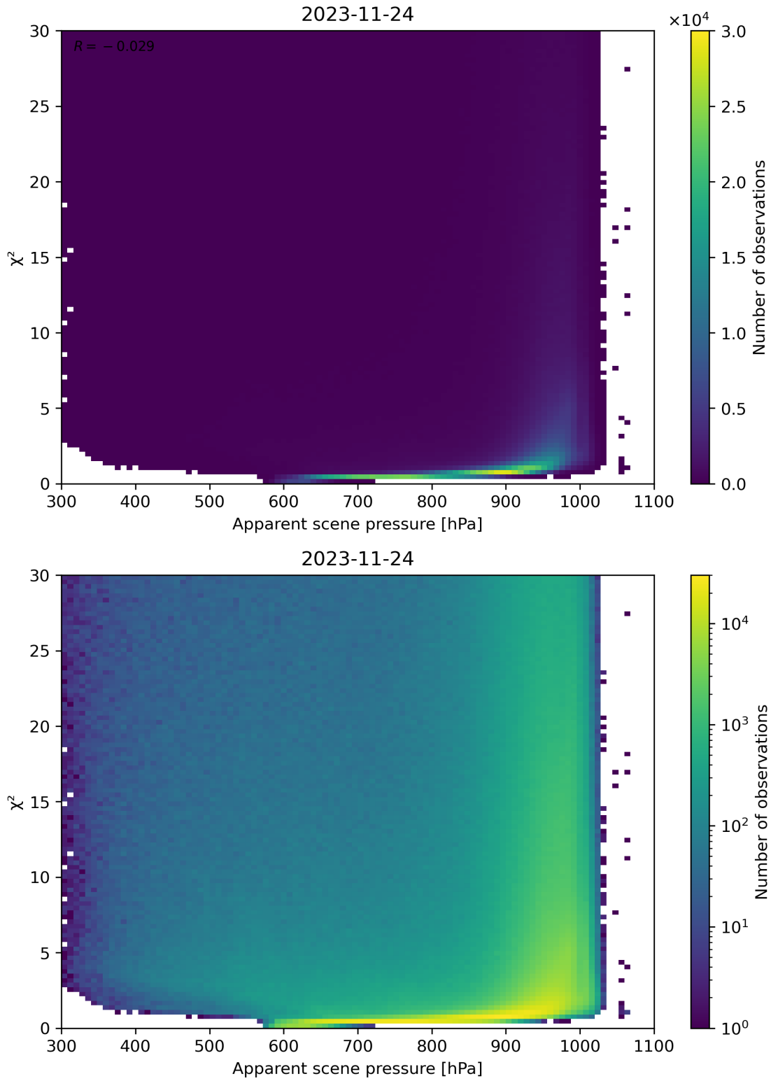
Figure 63: Scatter density plot of “Apparent scene pressure” against “ \chi^2 ” for 2023-11-23 to 2023-11-25.
