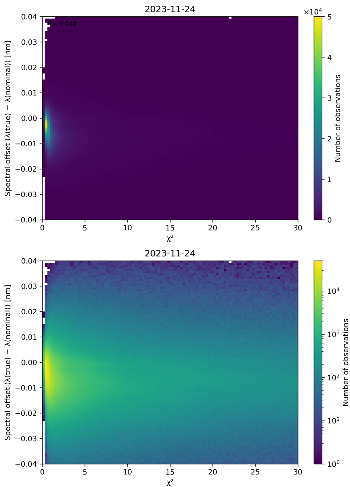
Figure 75: Scatter density plot of “ \chi^2 ” against “Spectral offset ( \lambda(\text{true}) - \lambda(\text{nominal}) )” for 2023-11-23 to 2023-11-25.
