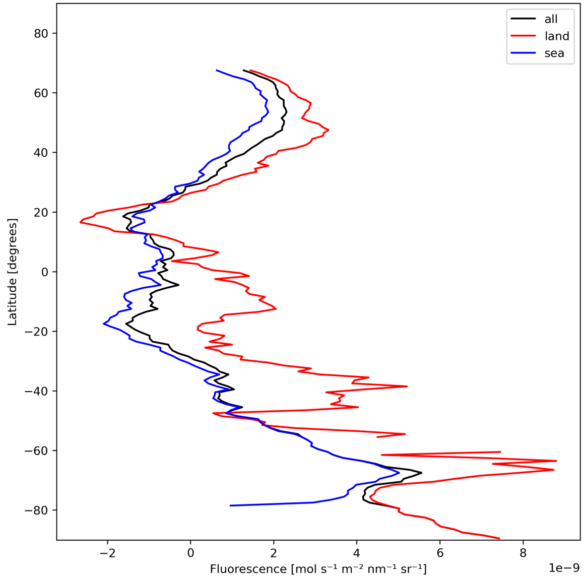
Figure 23: Zonal average of “Fluorescence” for 2023-11-23 to 2023-11-25.
