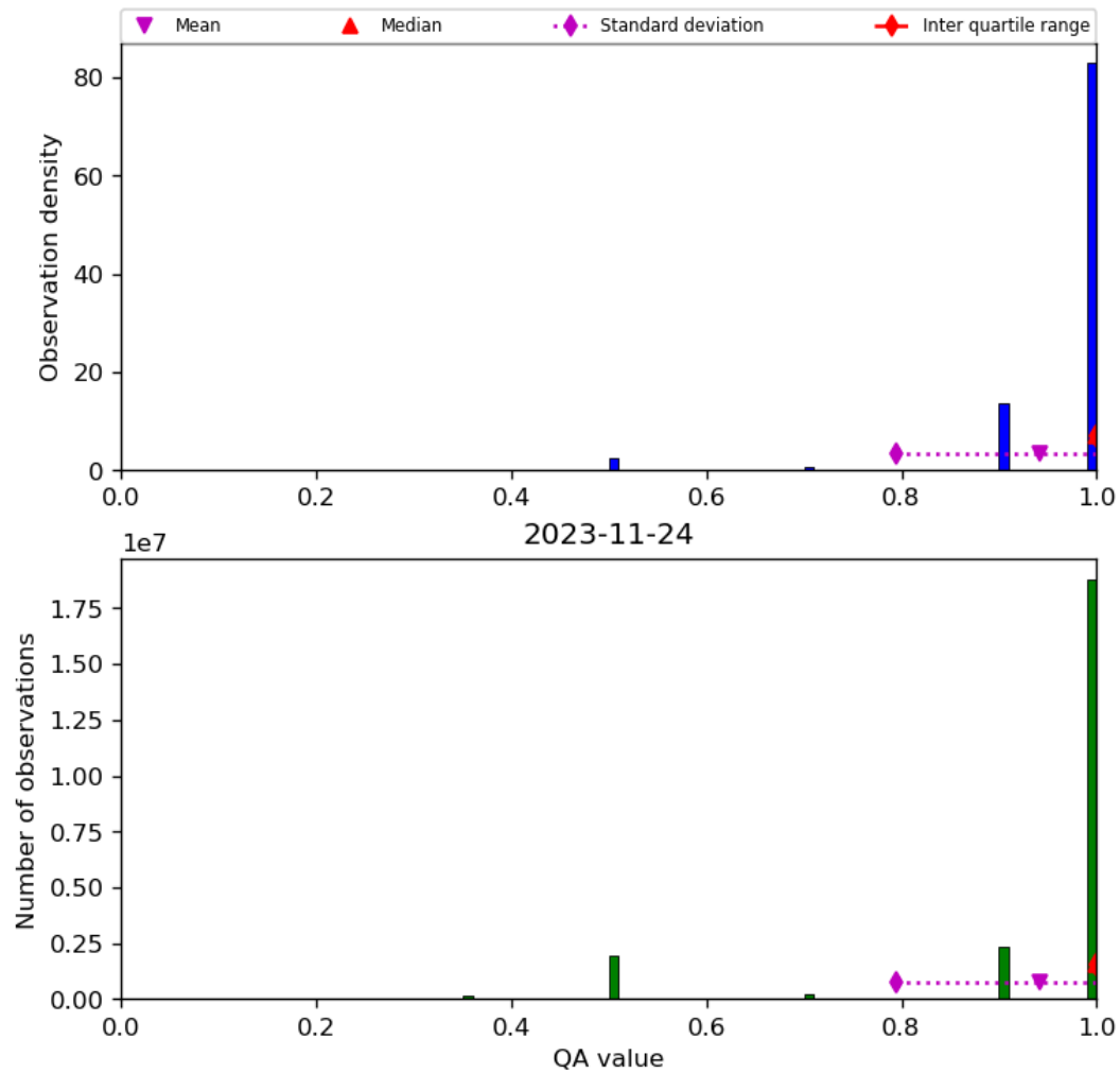
Figure 29: Histogram of “QA value” for 2023-11-23 to 2023-11-25
