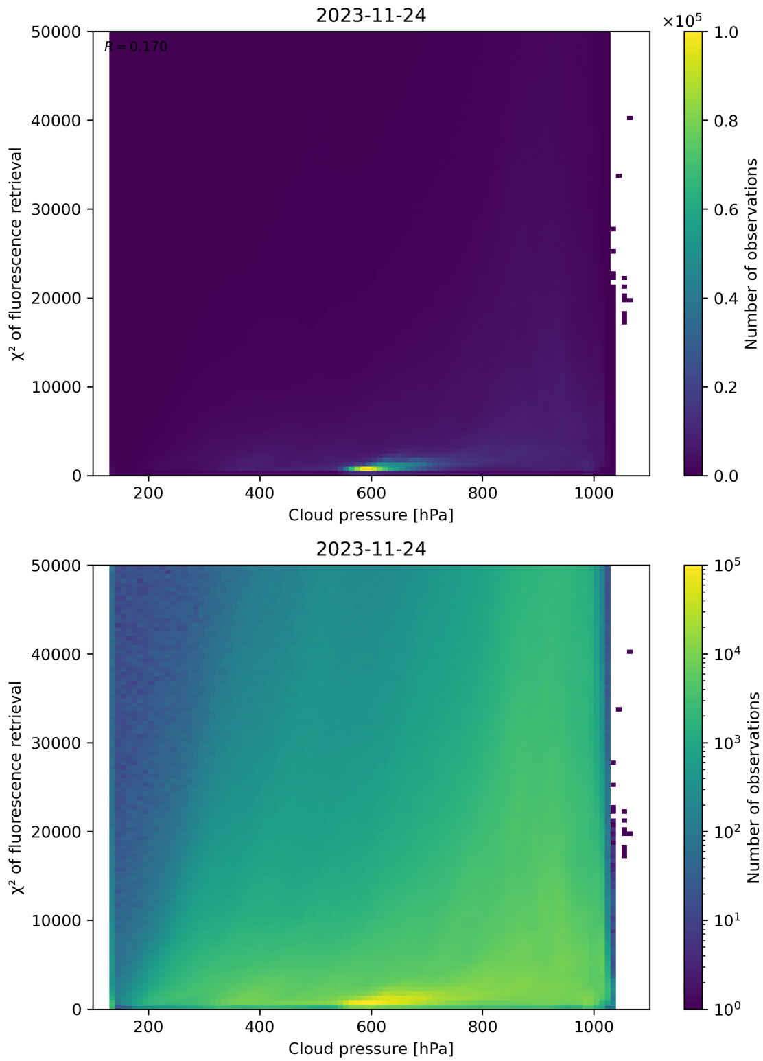
Figure 86: Scatter density plot of “Cloud pressure” against “ \chi^2 of fluorescence retrieval” for 2023-11-23 to 2023-11-25.
