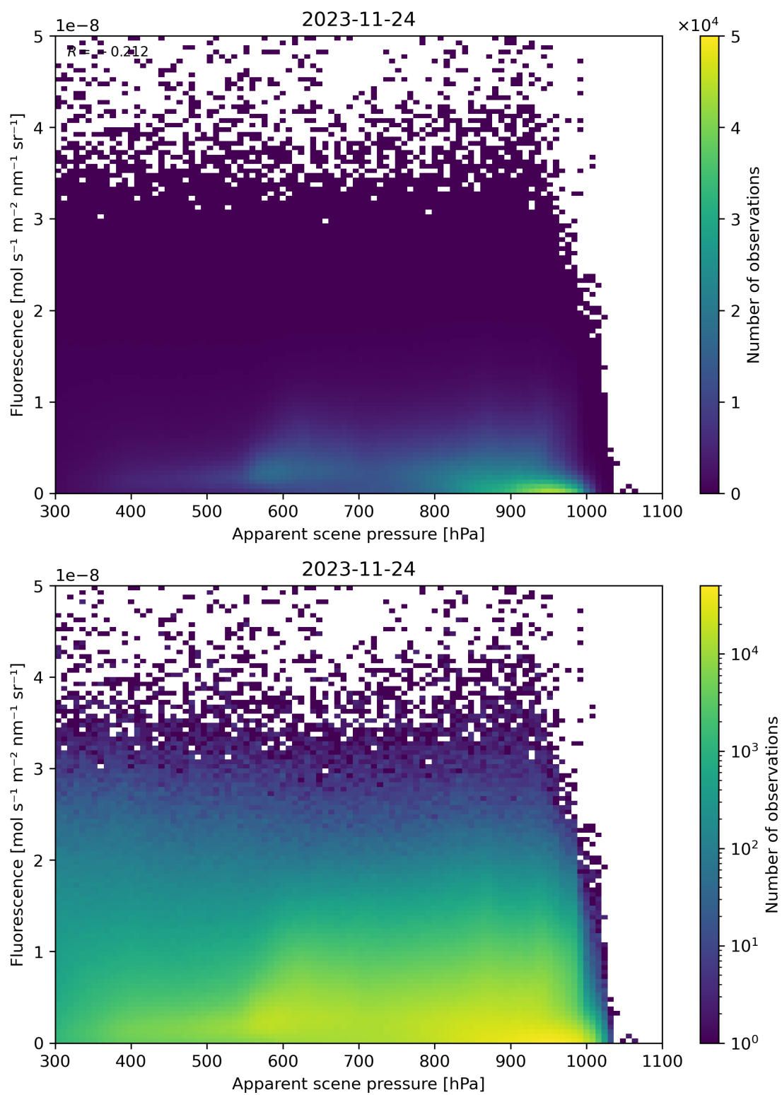
Figure 65: Scatter density plot of “Apparent scene pressure” against “Fluorescence” for 2023-11-23 to 2023-11-25.
