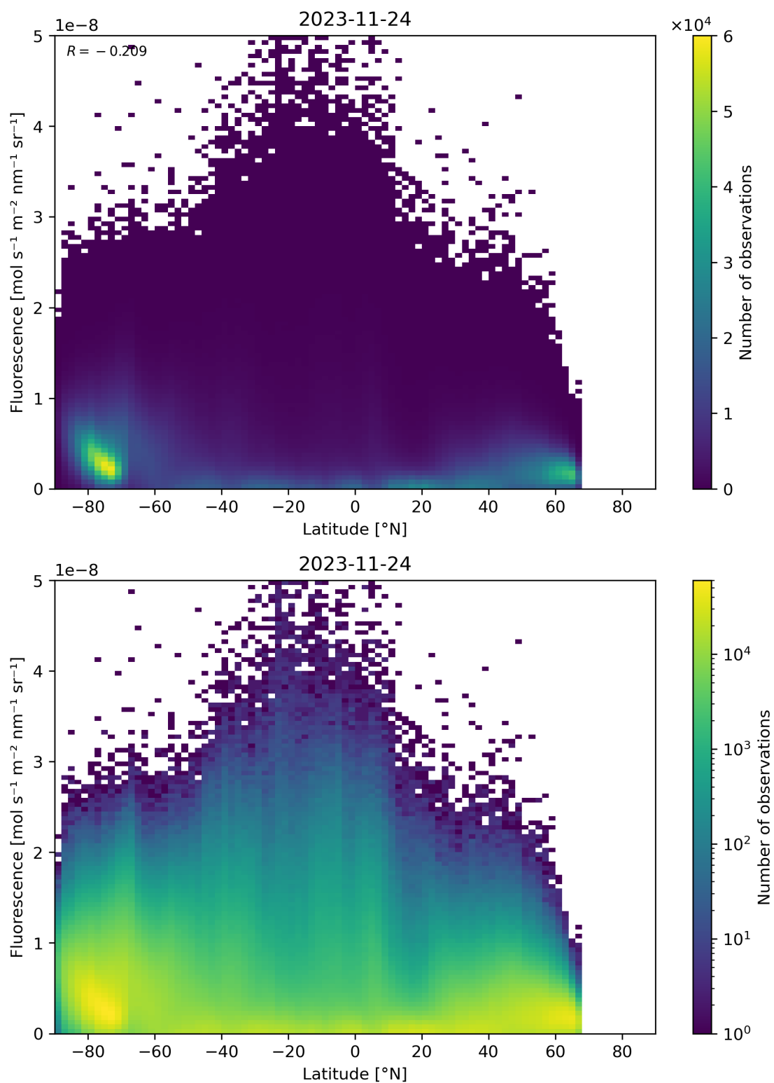
Figure 101: Scatter density plot of “Latitude” against “Fluorescence” for 2023-11-23 to 2023-11-25.
