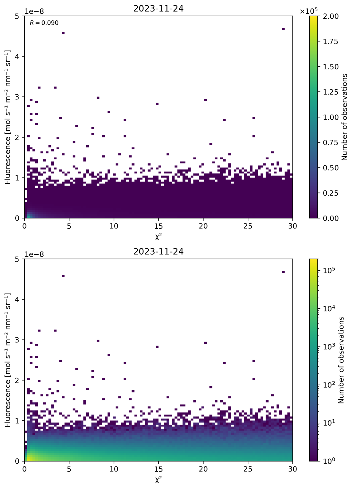
Figure 70: Scatter density plot of “ \chi^2 ” against “Fluorescence” for 2023-11-23 to 2023-11-25.
