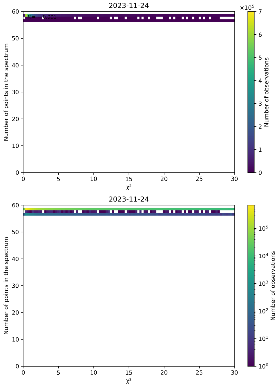
Figure 74: Scatter density plot of " \chi^2 " against "Number of points in the spectrum" for 2023-11-23 to 2023-11-25.
