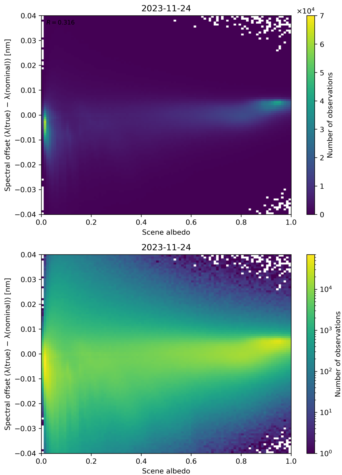
Figure 117: Scatter density plot of “Scene albedo” against “Spectral offset ( \lambda(\text{true}) - \lambda(\text{nominal}) )” for 2023-11-23 to 2023-11-25.
