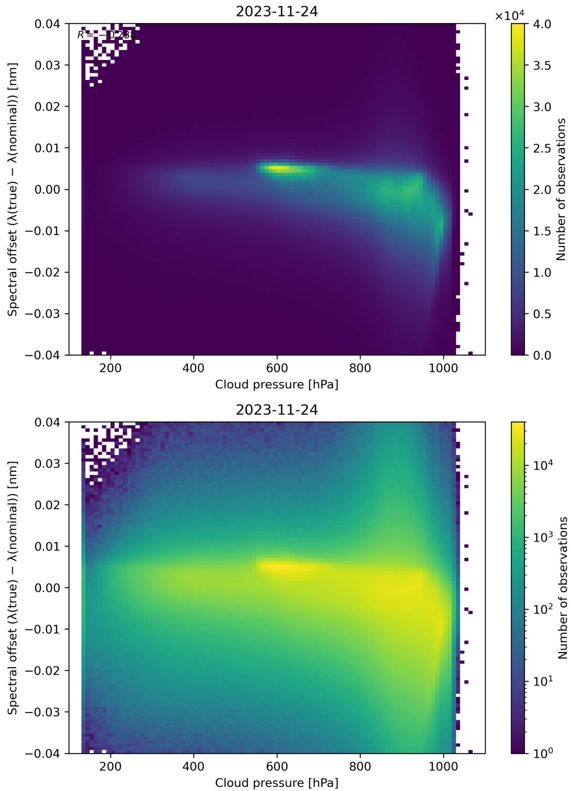
Figure 92: Scatter density plot of “Cloud pressure” against “Spectral offset ( \lambda(\text{true}) - \lambda(\text{nominal}) )” for 2023-11-23 to 2023-11-25.
