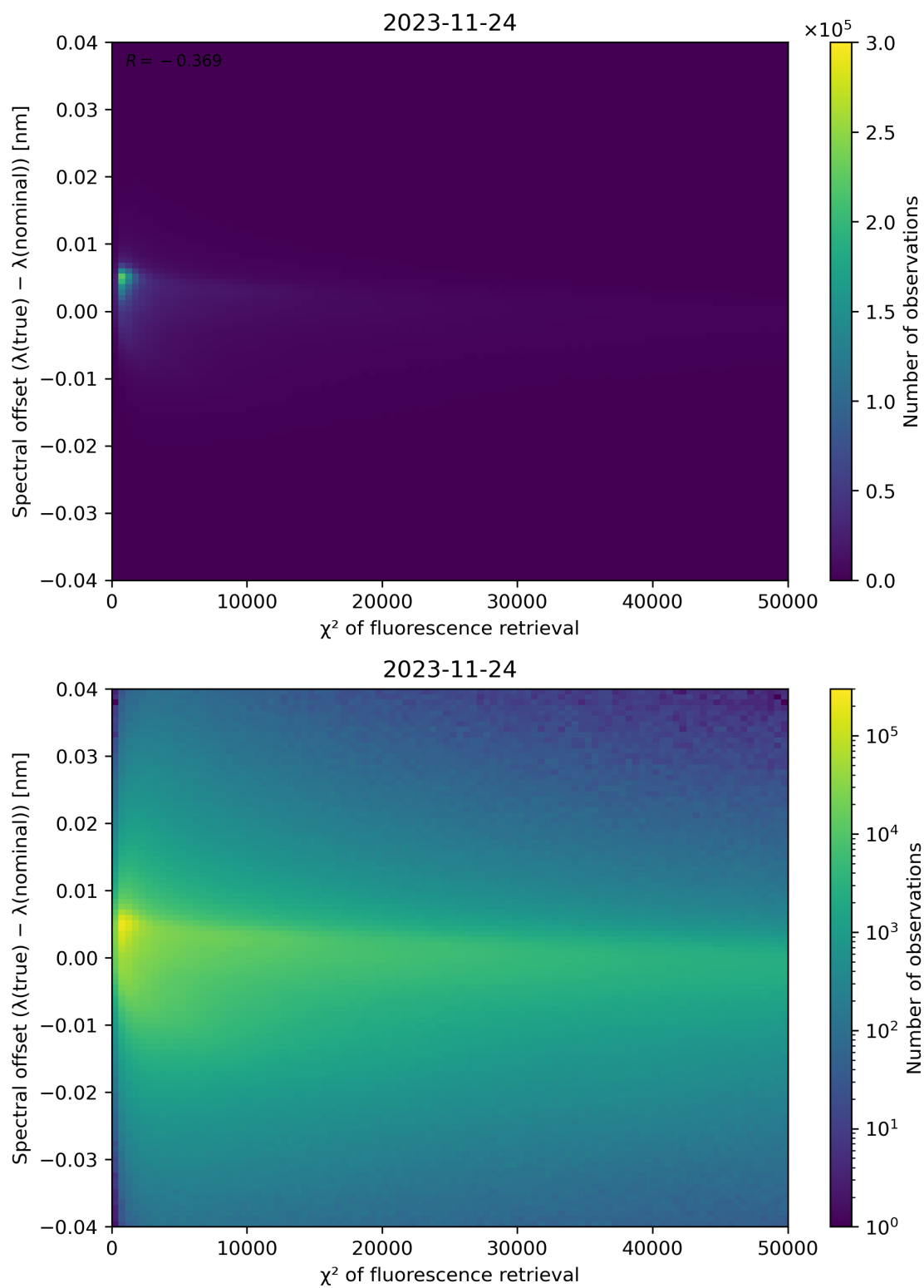
Figure 72: Scatter density plot of “ \chi^2 of fluorescence retrieval” against “Spectral offset ( \lambda(\text{true}) - \lambda(\text{nominal}) )” for 2023-11-23 to 2023-11-25.
