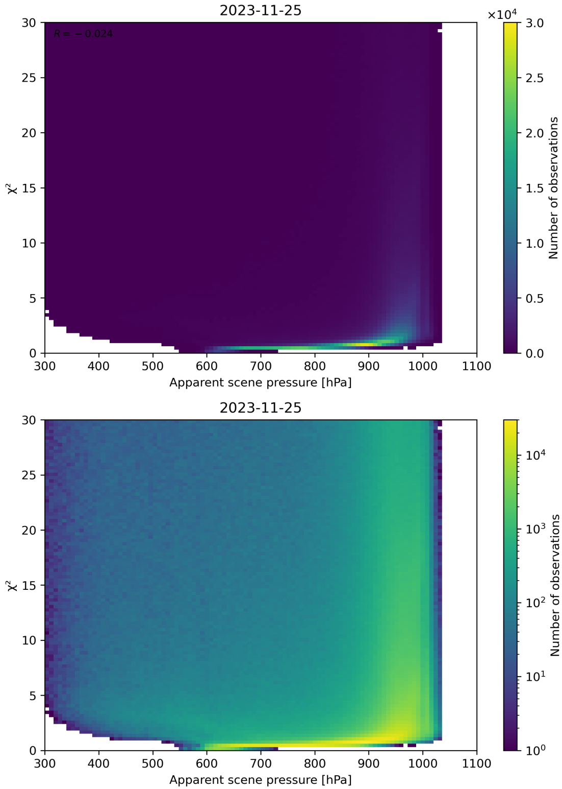
Figure 63: Scatter density plot of “Apparent scene pressure” against “ \chi^2 ” for 2023-11-24 to 2023-11-26.
