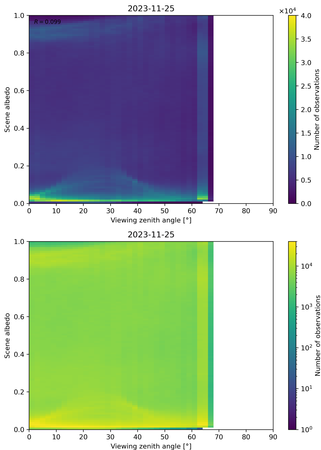
Figure 138: Scatter density plot of “Viewing zenith angle” against “Scene albedo” for 2023-11-24 to 2023-11-26.
