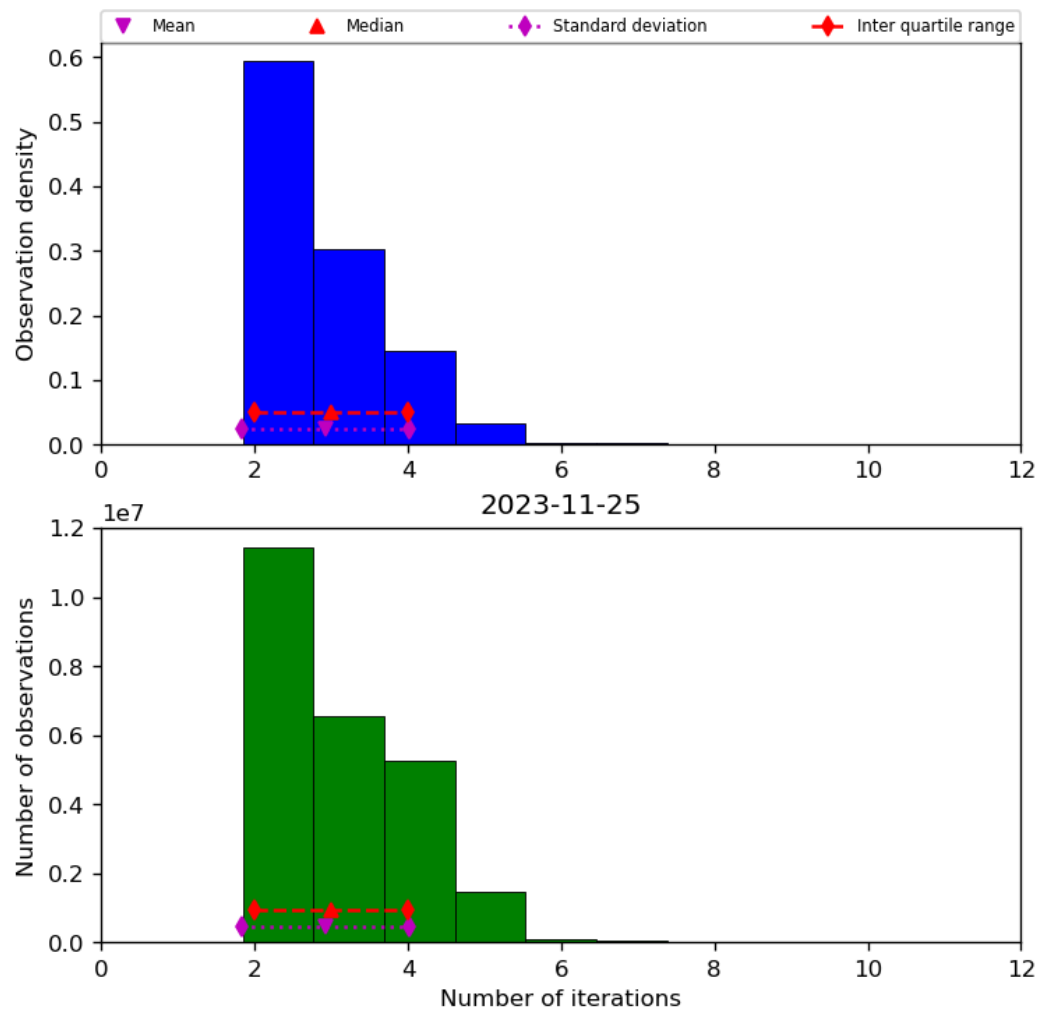
Figure 39: Histogram of “Number of iterations” for 2023-11-24 to 2023-11-26
