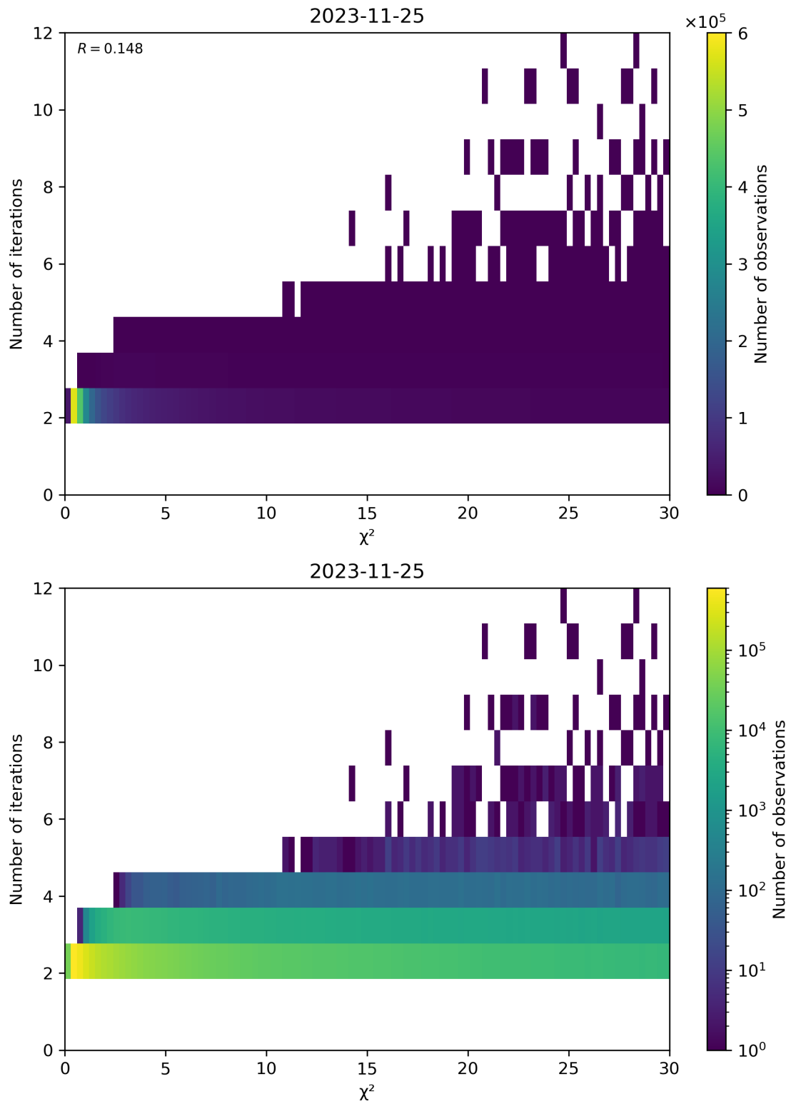
Figure 73: Scatter density plot of “ \chi^2 ” against “Number of iterations” for 2023-11-24 to 2023-11-26.
