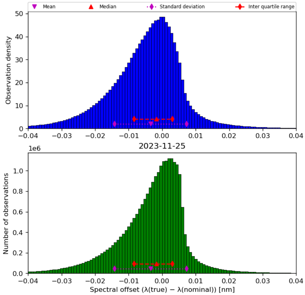
Figure 45: Histogram of “Spectral offset ( \lambda(\text{true}) - \lambda(\text{nominal}) )” for 2023-11-24 to 2023-11-26
