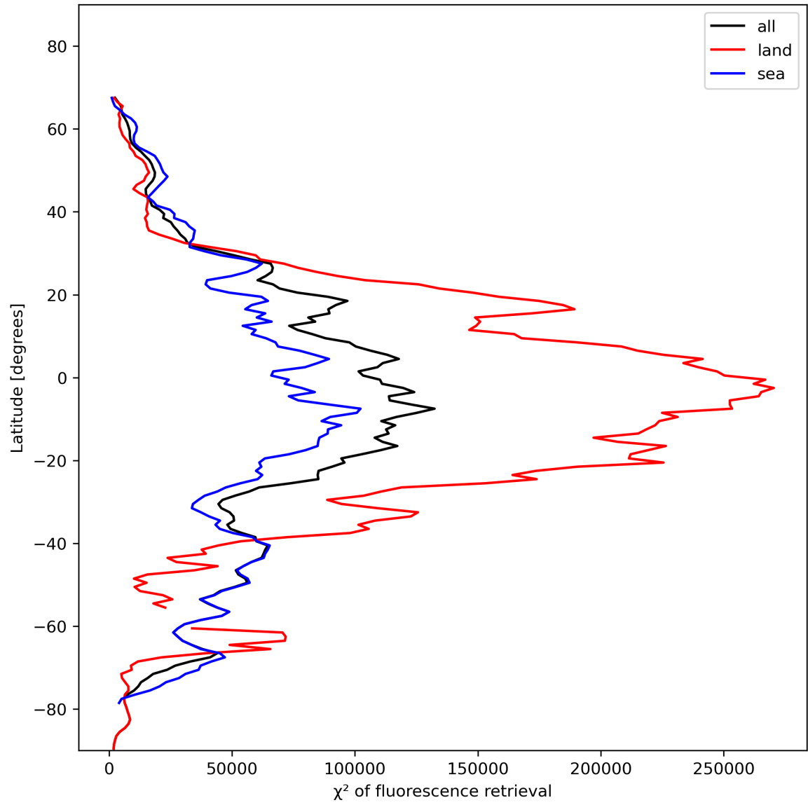
Figure 25: Zonal average of “ \chi^2 of fluorescence retrieval” for 2023-11-24 to 2023-11-26.
