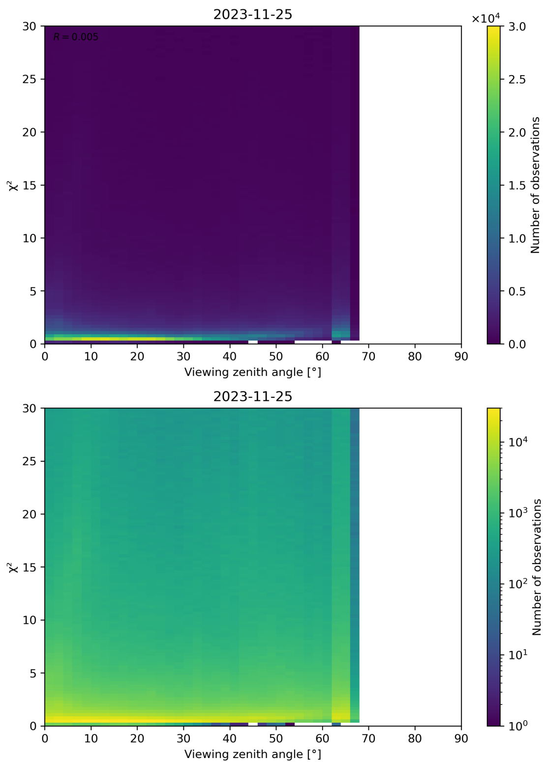
Figure 130: Scatter density plot of “Viewing zenith angle” against “ \chi^2 ” for 2023-11-24 to 2023-11-26.
