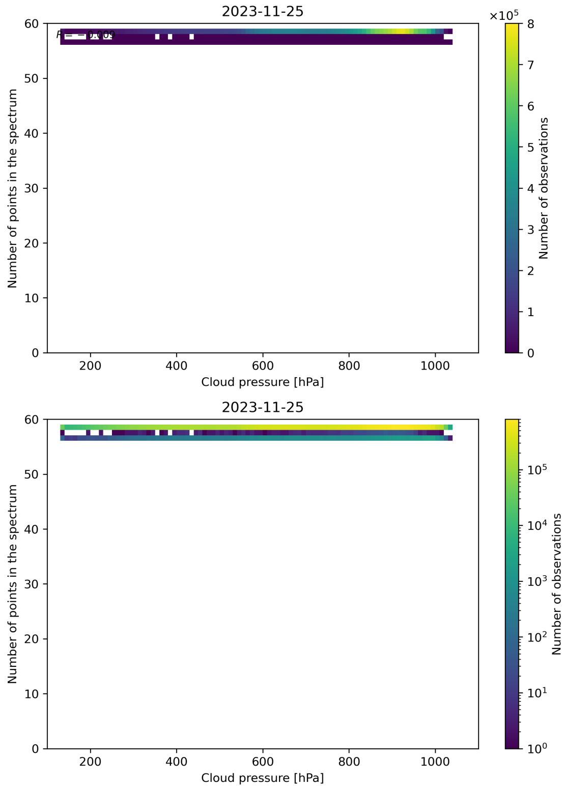
Figure 90: Scatter density plot of “Cloud pressure” against “Number of points in the spectrum” for 2023-11-24 to 2023-11-26.
