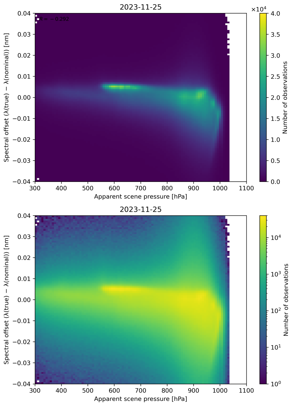
Figure 68: Scatter density plot of “Apparent scene pressure” against “Spectral offset ( \lambda(\text{true}) - \lambda(\text{nominal}) )” for 2023-11-24 to 2023-11-26.
