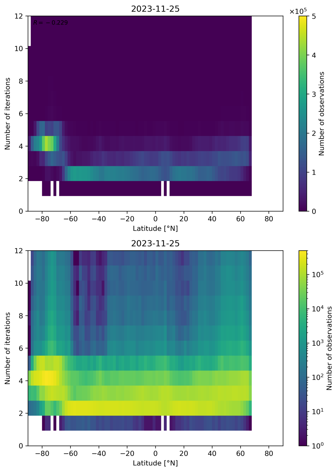
Figure 102: Scatter density plot of “Latitude” against “Number of iterations” for 2023-11-24 to 2023-11-26.
