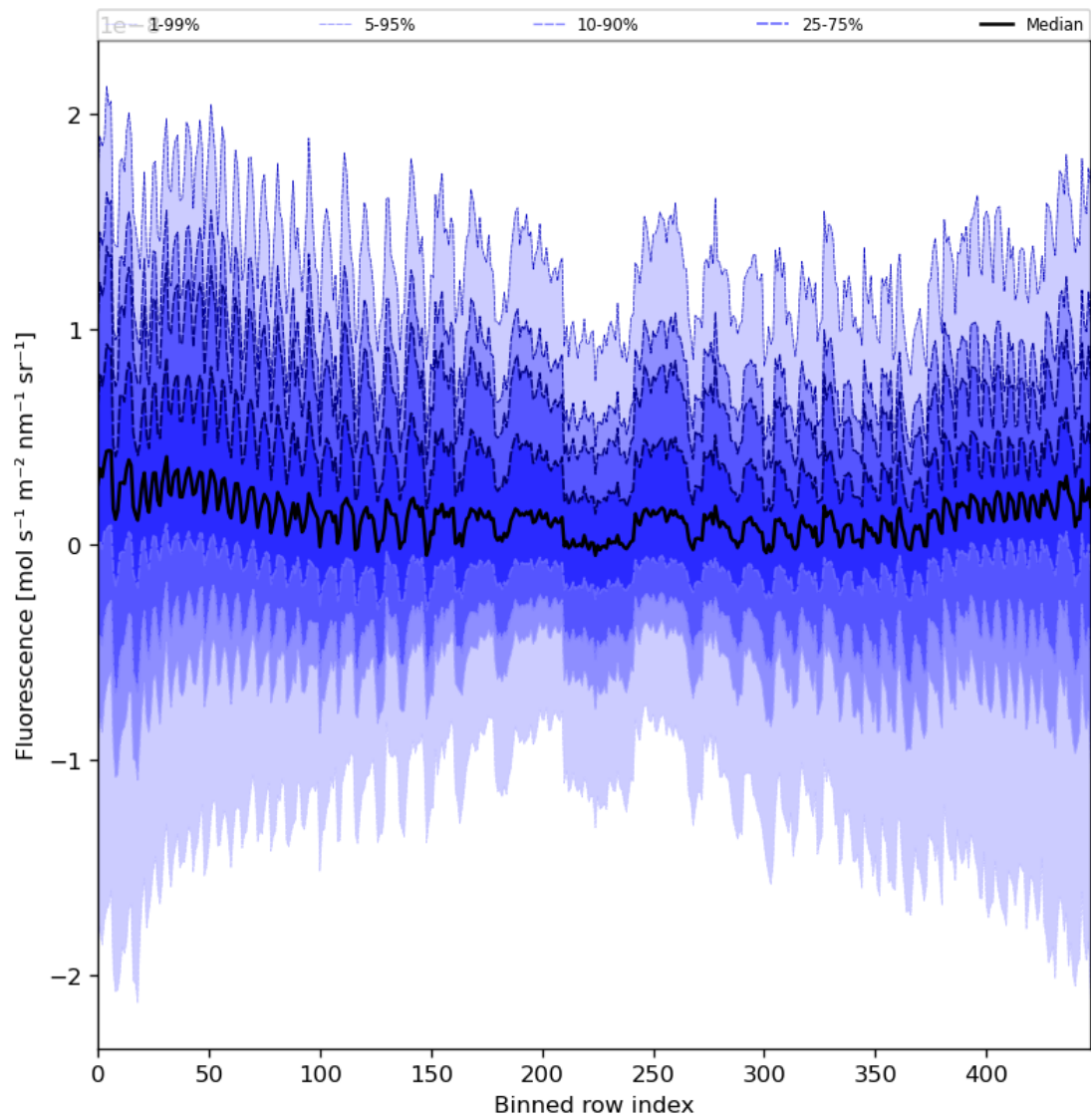
Figure 57: Along track statistics of “Fluorescence” for 2023-11-24 to 2023-11-26
