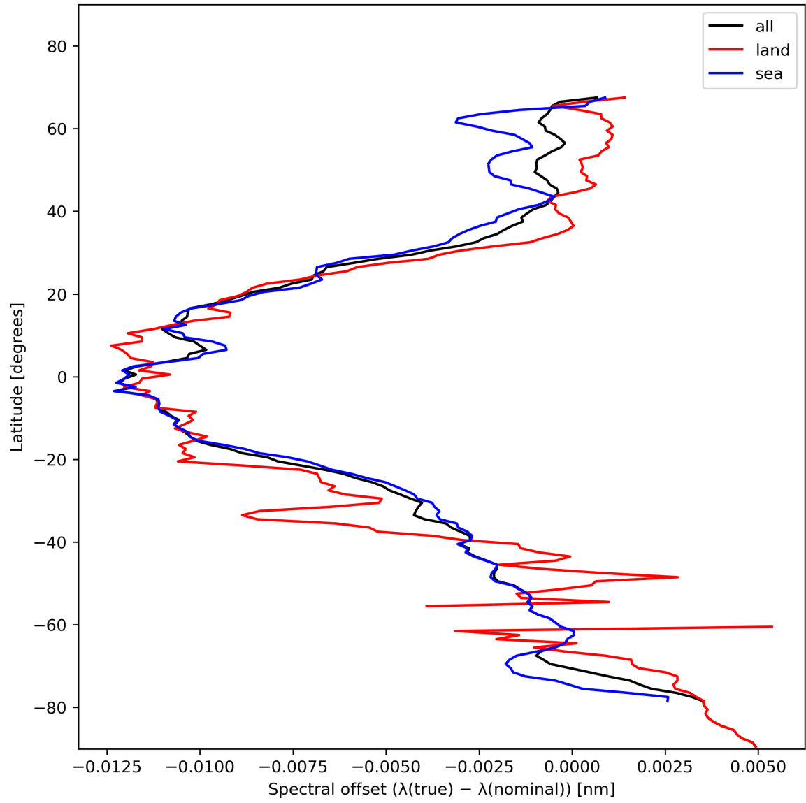
Figure 28: Zonal average of “Spectral offset ( \lambda(\text{true}) - \lambda(\text{nominal}) )” for 2023-11-24 to 2023-11-26.
