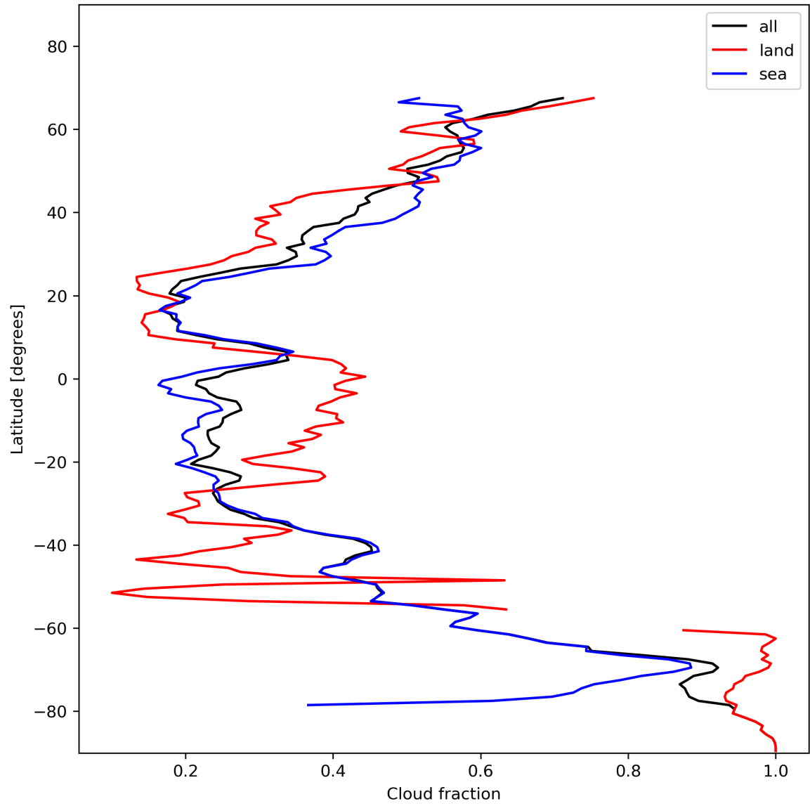
Figure 15: Zonal average of “Cloud fraction” for 2023-11-24 to 2023-11-26.
