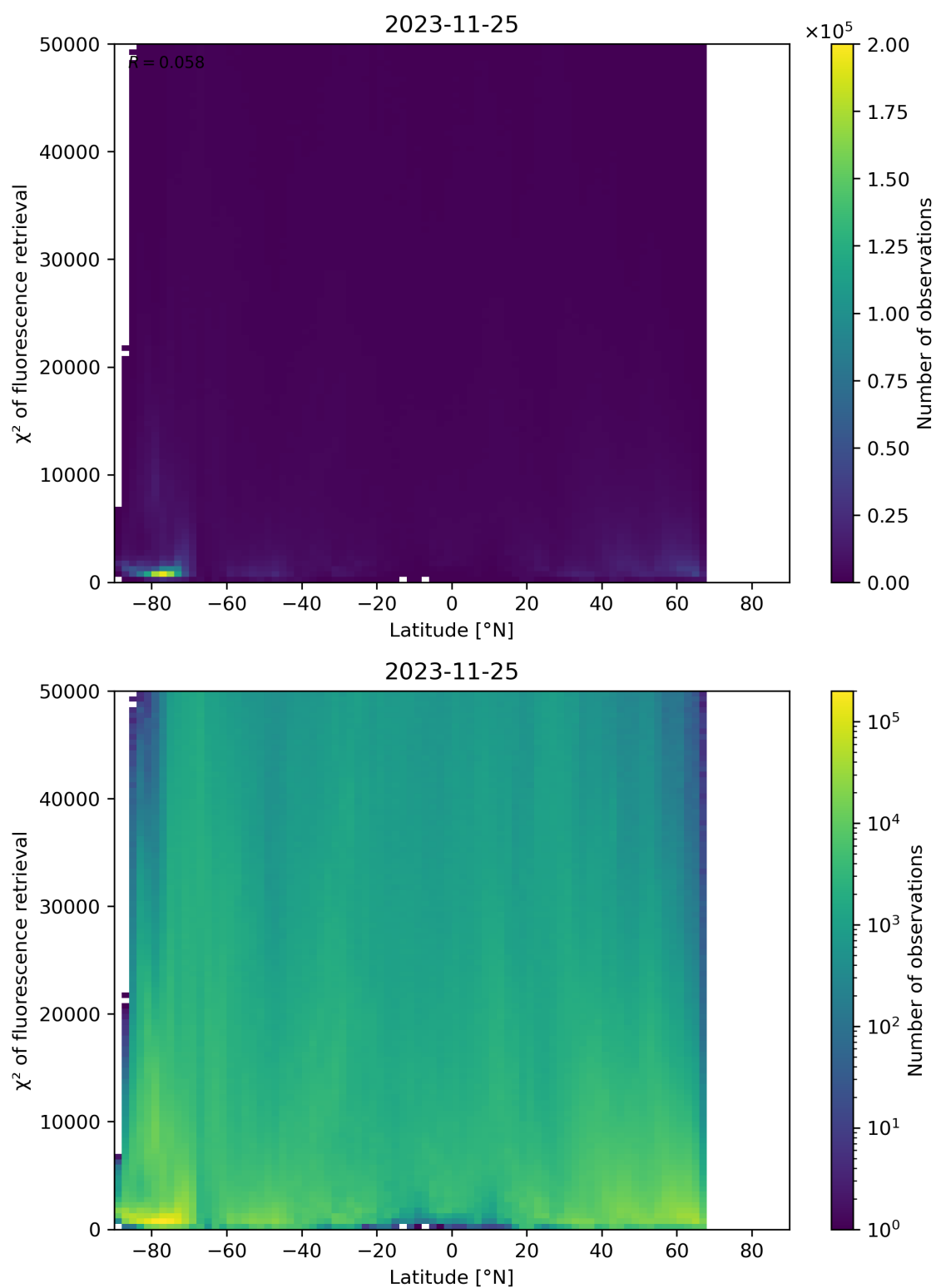
Figure 98: Scatter density plot of “Latitude” against “ \chi^2 of fluorescence retrieval” for 2023-11-24 to 2023-11-26.
