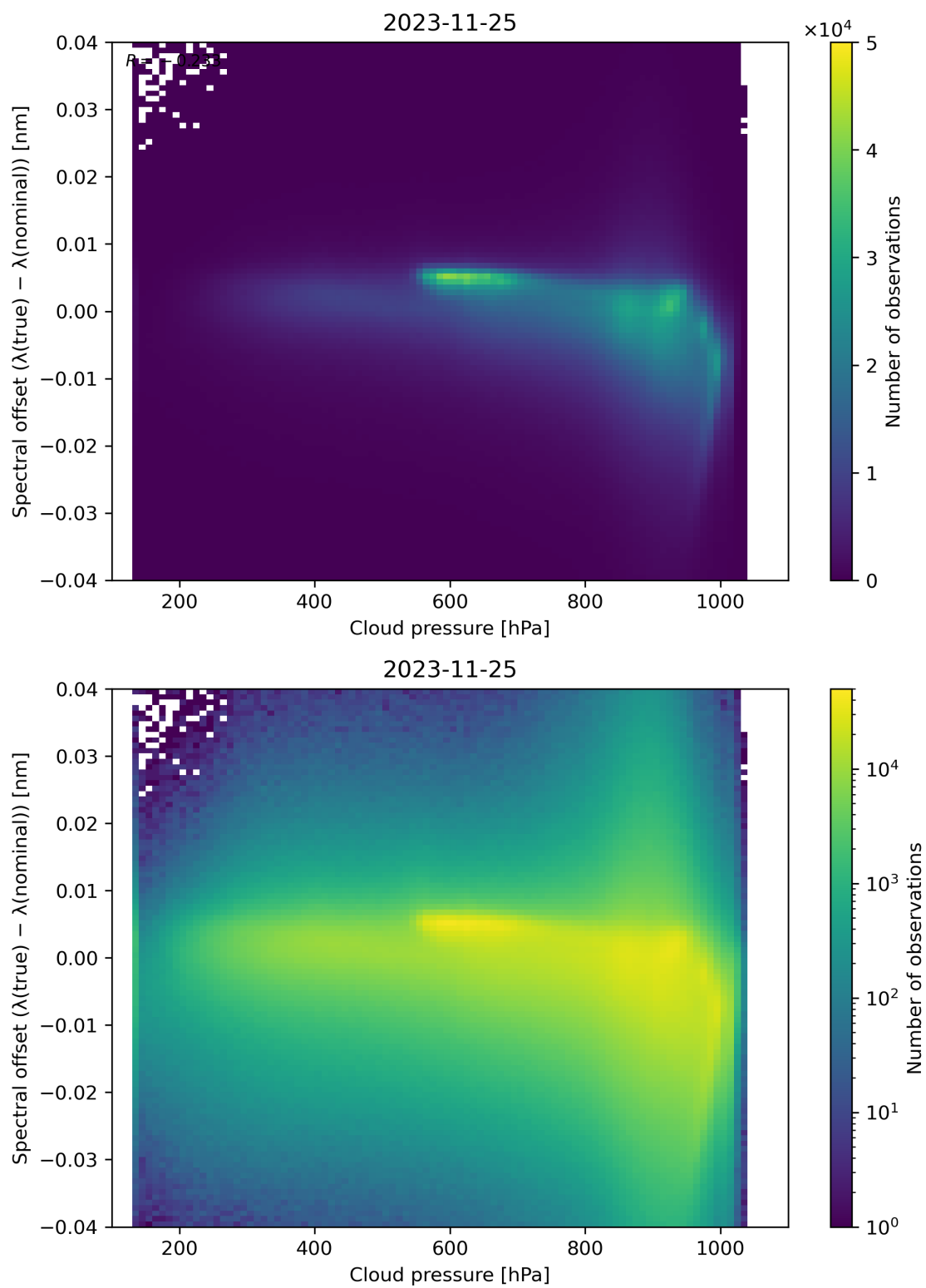
Figure 92: Scatter density plot of “Cloud pressure” against “Spectral offset ( \lambda(\text{true}) - \lambda(\text{nominal}) )” for 2023-11-24 to 2023-11-26.
