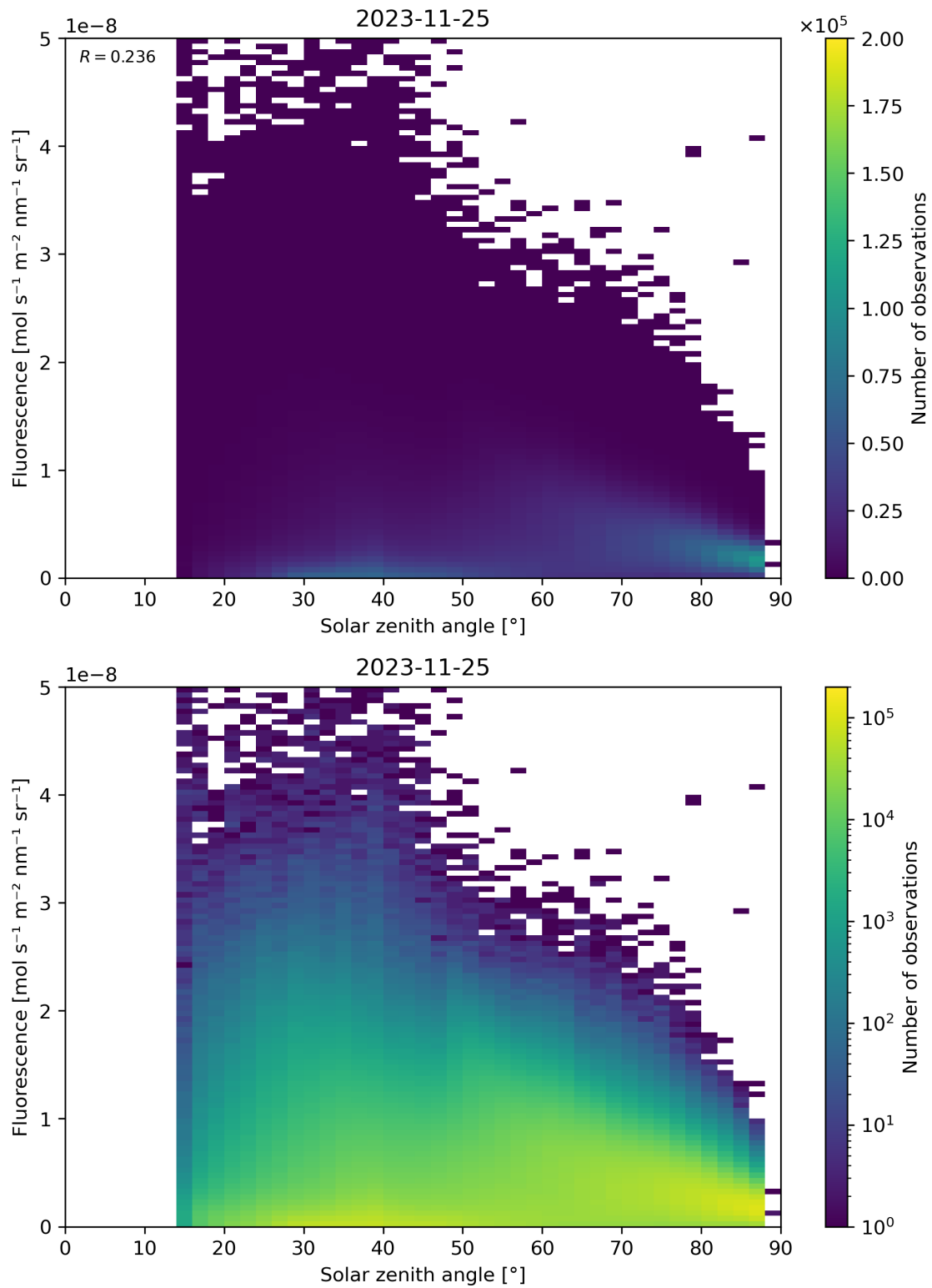
Figure 123: Scatter density plot of “Solar zenith angle” against “Fluorescence” for 2023-11-24 to 2023-11-26.
