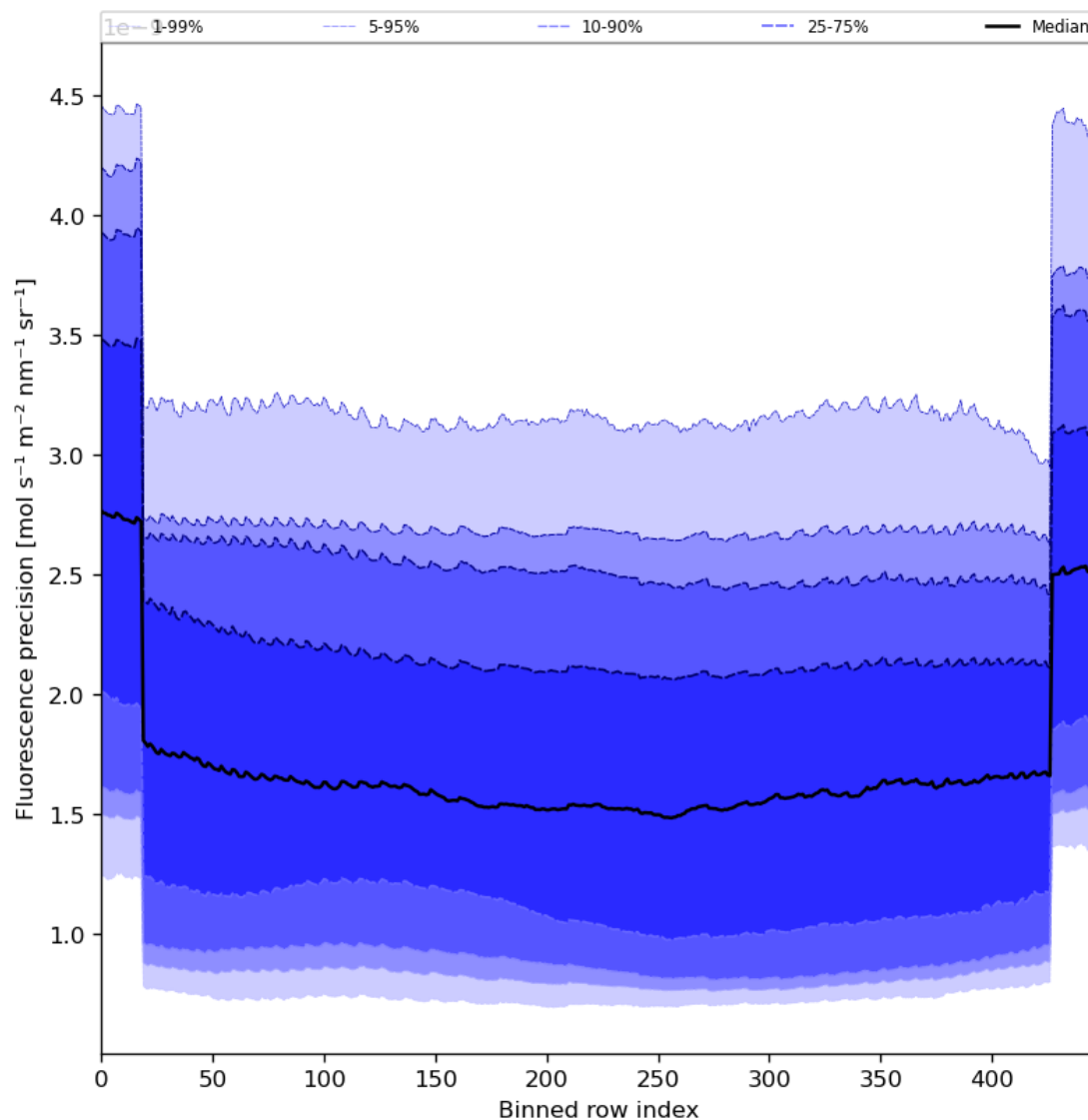
Figure 58: Along track statistics of “Fluorescence precision” for 2023-11-24 to 2023-11-26
