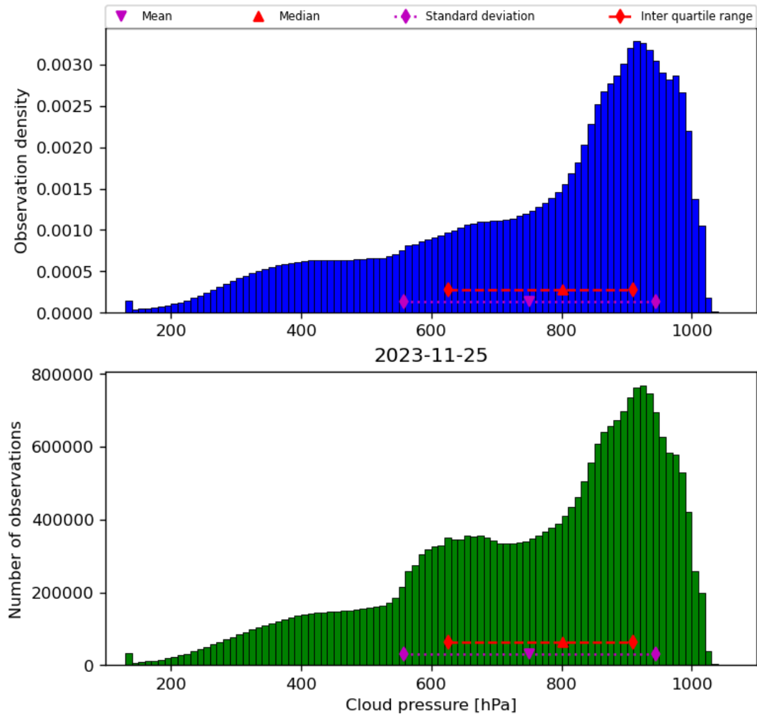
Figure 30: Histogram of “Cloud pressure” for 2023-11-24 to 2023-11-26
