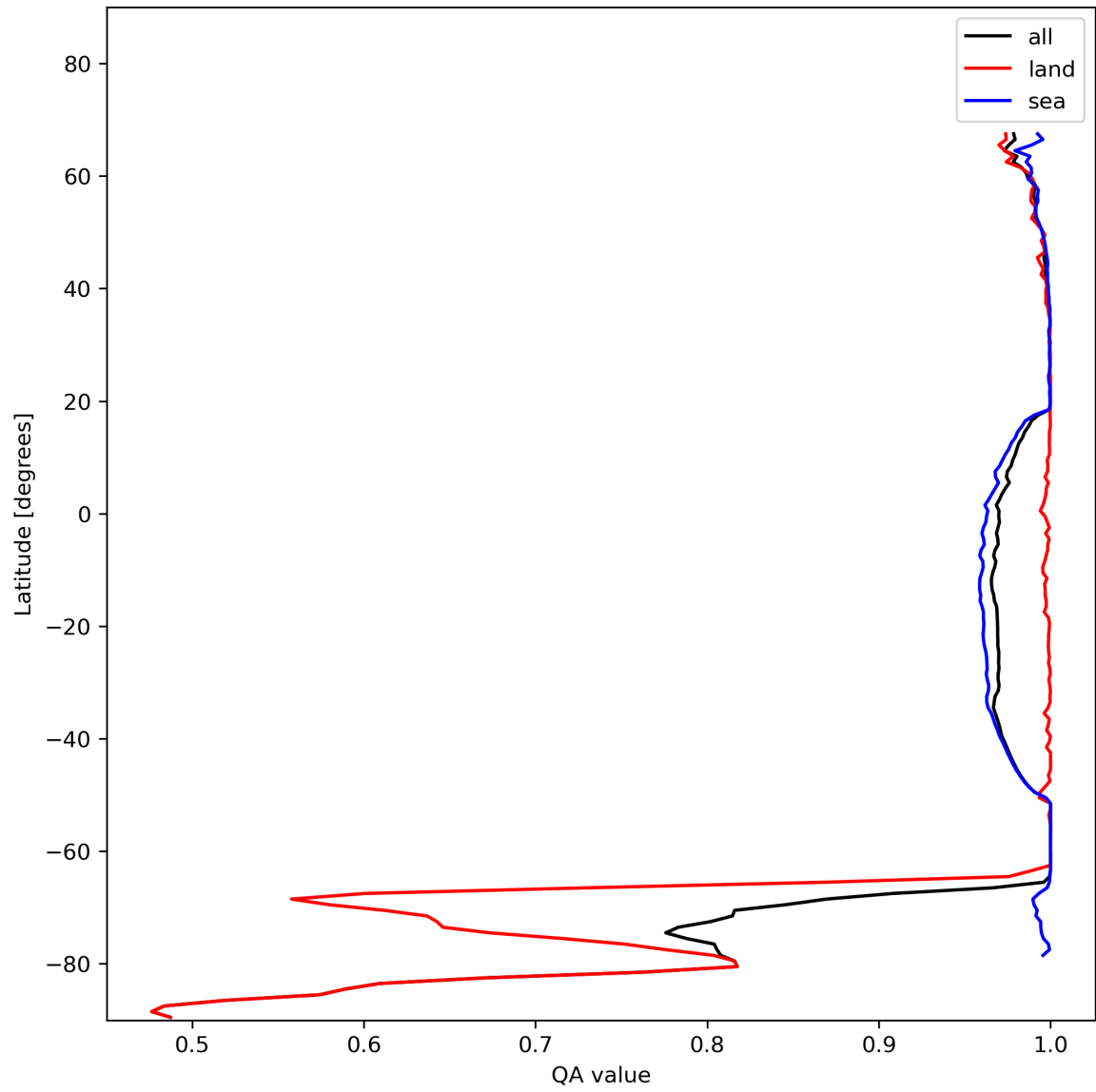
Figure 12: Zonal average of “QA value” for 2023-11-24 to 2023-11-26.
