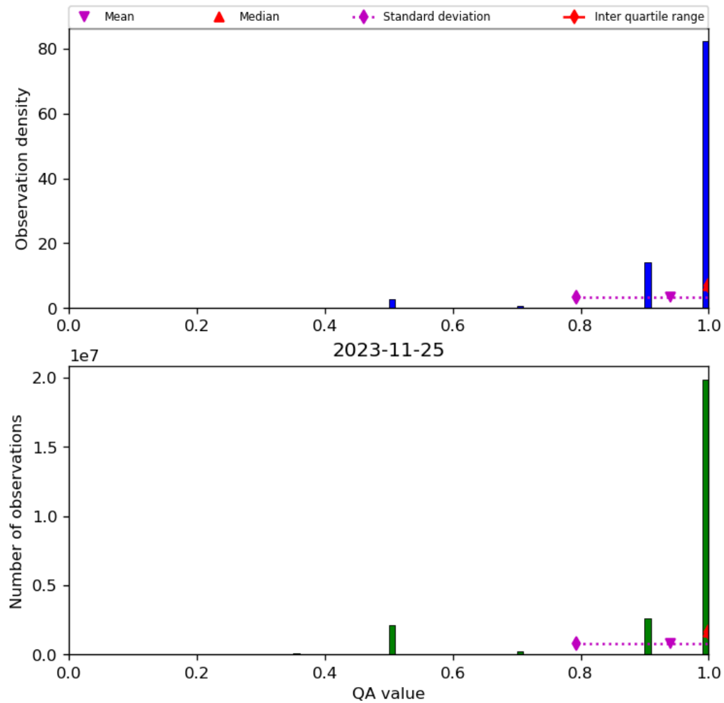
Figure 29: Histogram of “QA value” for 2023-11-24 to 2023-11-26
