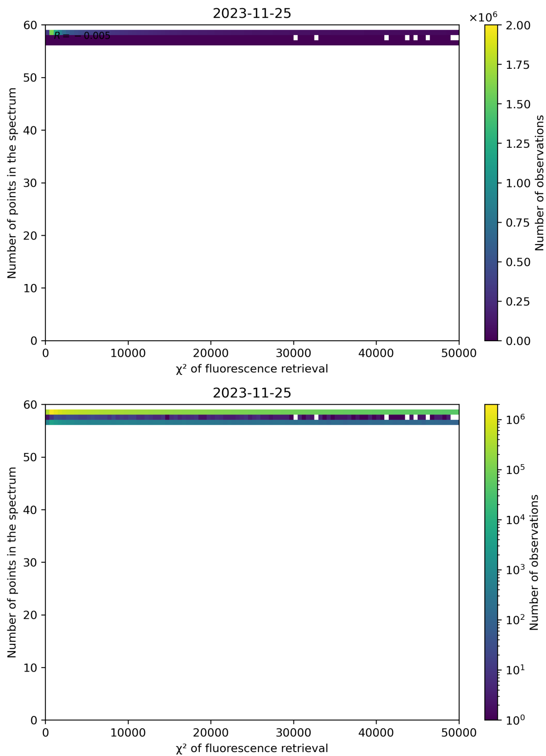
Figure 71: Scatter density plot of " \chi^2 of fluorescence retrieval" against "Number of points in the spectrum" for 2023-11-24 to 2023-11-26.
