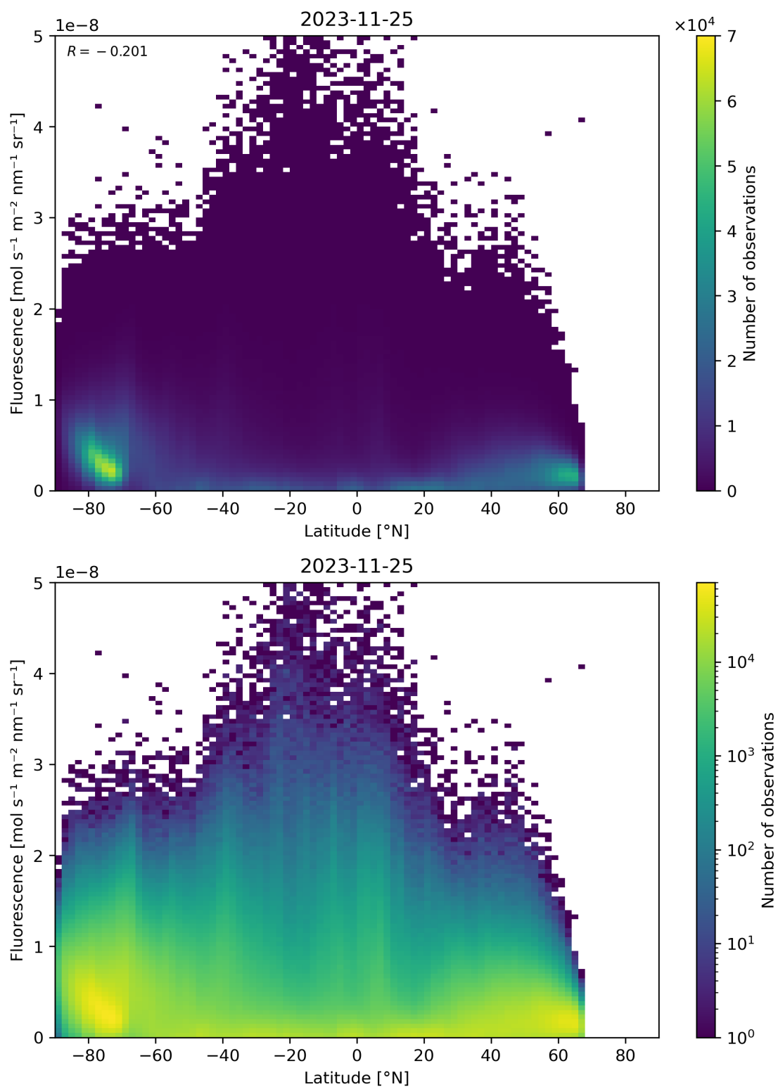
Figure 101: Scatter density plot of “Latitude” against “Fluorescence” for 2023-11-24 to 2023-11-26.
