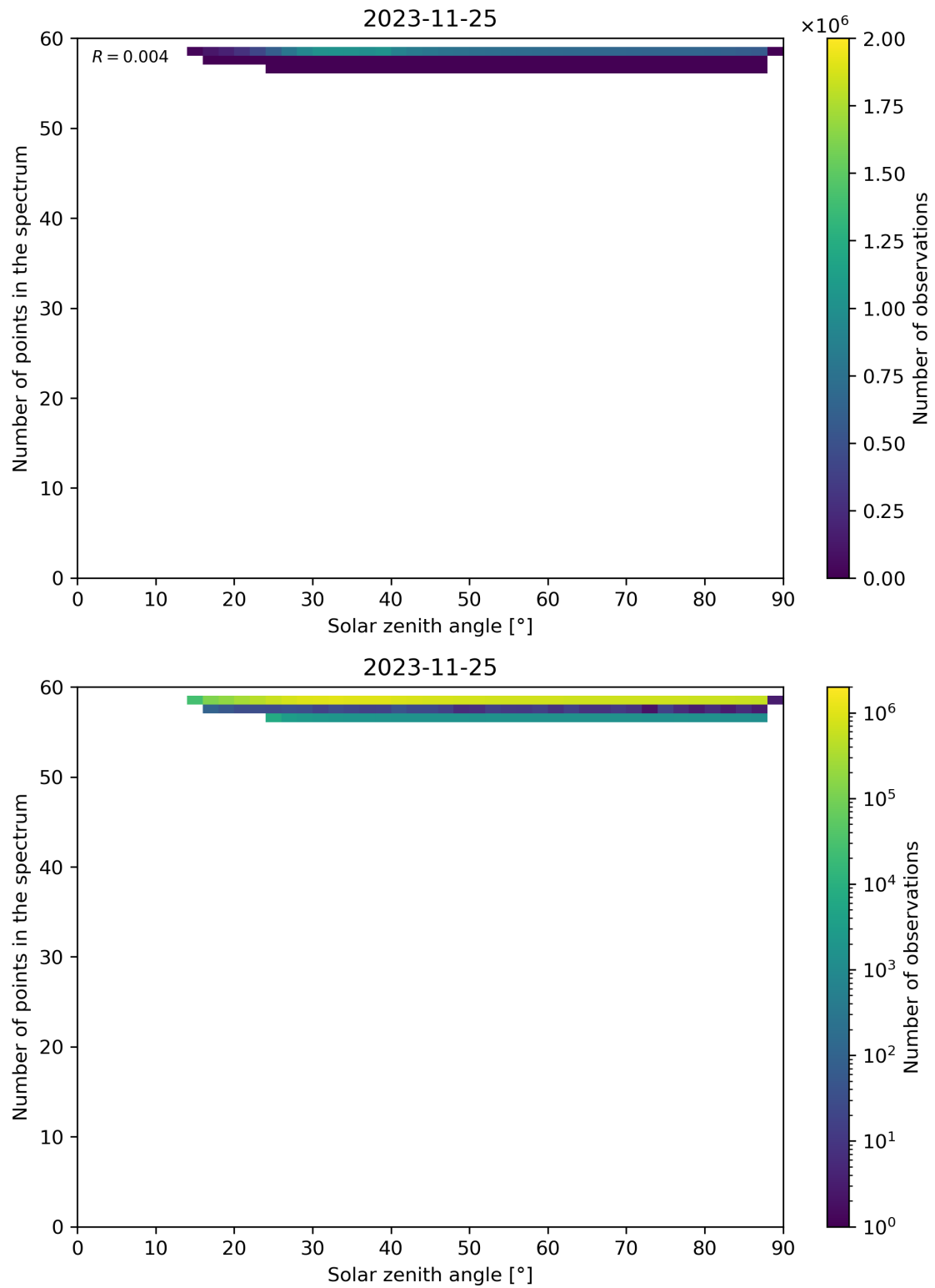
Figure 126: Scatter density plot of “Solar zenith angle” against “Number of points in the spectrum” for 2023-11-24 to 2023-11-26.
