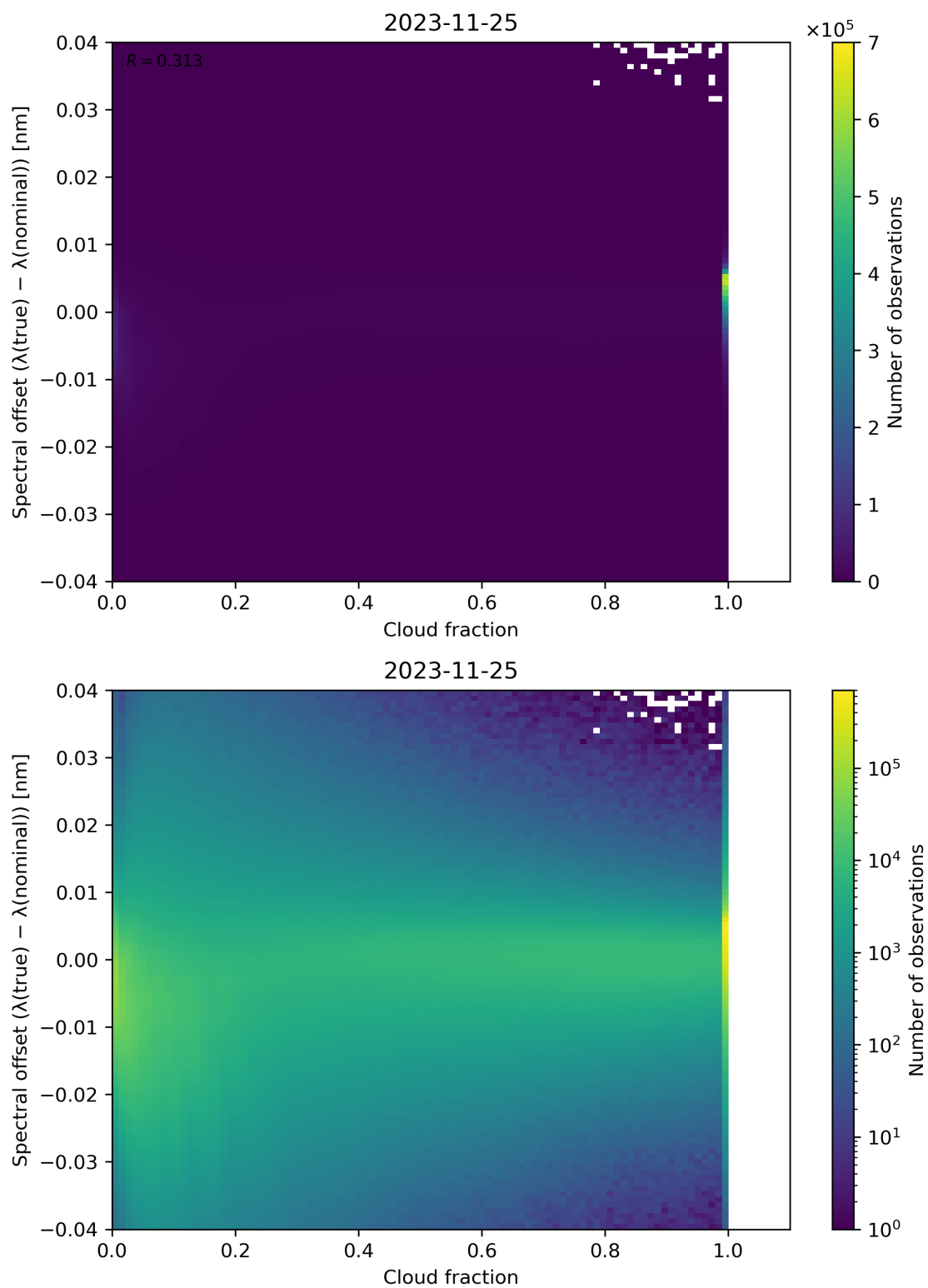
Figure 83: Scatter density plot of “Cloud fraction” against “Spectral offset ( \lambda(\text{true}) - \lambda(\text{nominal}) )” for 2023-11-24 to 2023-11-26.
