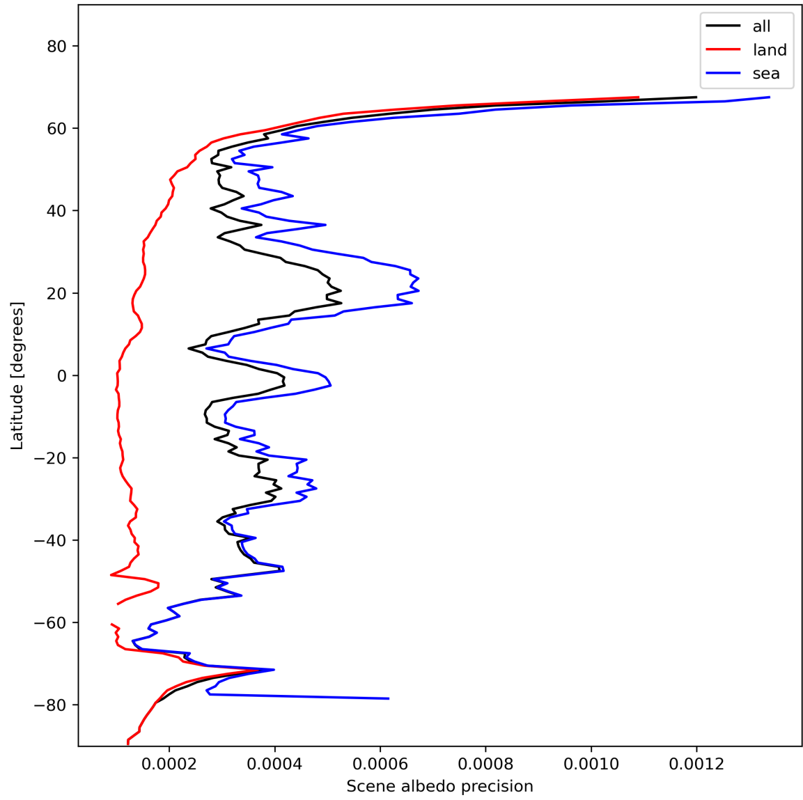
Figure 18: Zonal average of “Scene albedo precision” for 2023-11-24 to 2023-11-26.
