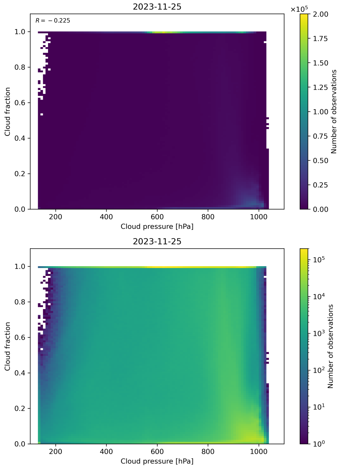
Figure 87: Scatter density plot of “Cloud pressure” against “Cloud fraction” for 2023-11-24 to 2023-11-26.
