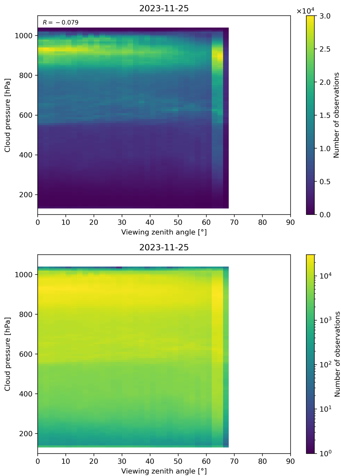
Figure 133: Scatter density plot of “Viewing zenith angle” against “Cloud pressure” for 2023-11-24 to 2023-11-26.
