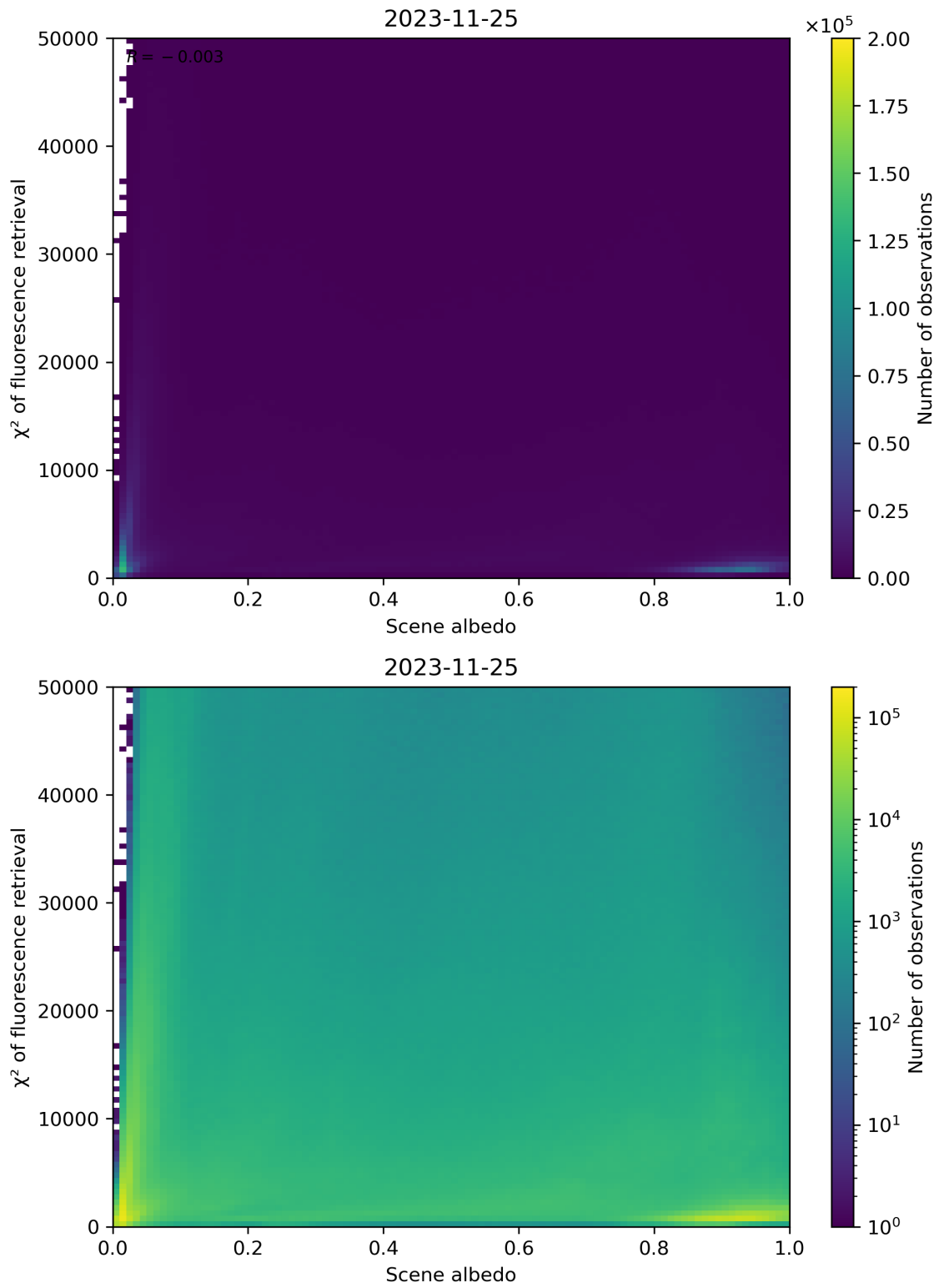
Figure 113: Scatter density plot of “Scene albedo” against “ \chi^2 of fluorescence retrieval” for 2023-11-24 to 2023-11-26.
