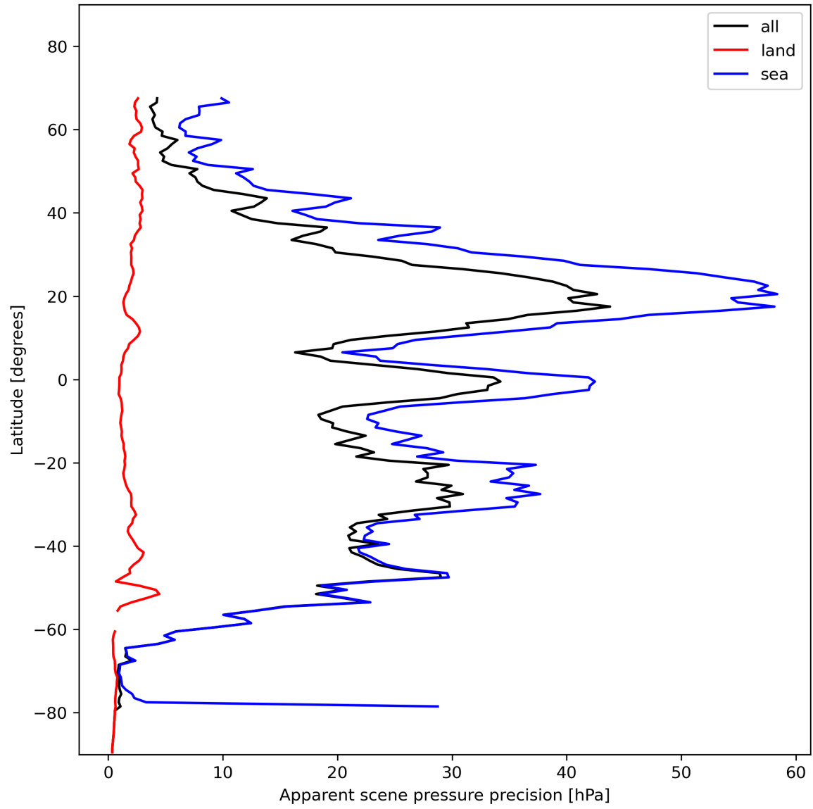
Figure 20: Zonal average of “Apparent scene pressure precision” for 2023-11-24 to 2023-11-26.
