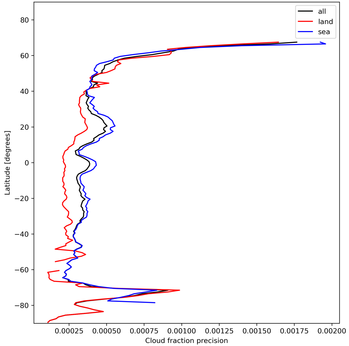
Figure 16: Zonal average of “Cloud fraction precision” for 2023-11-24 to 2023-11-26.
