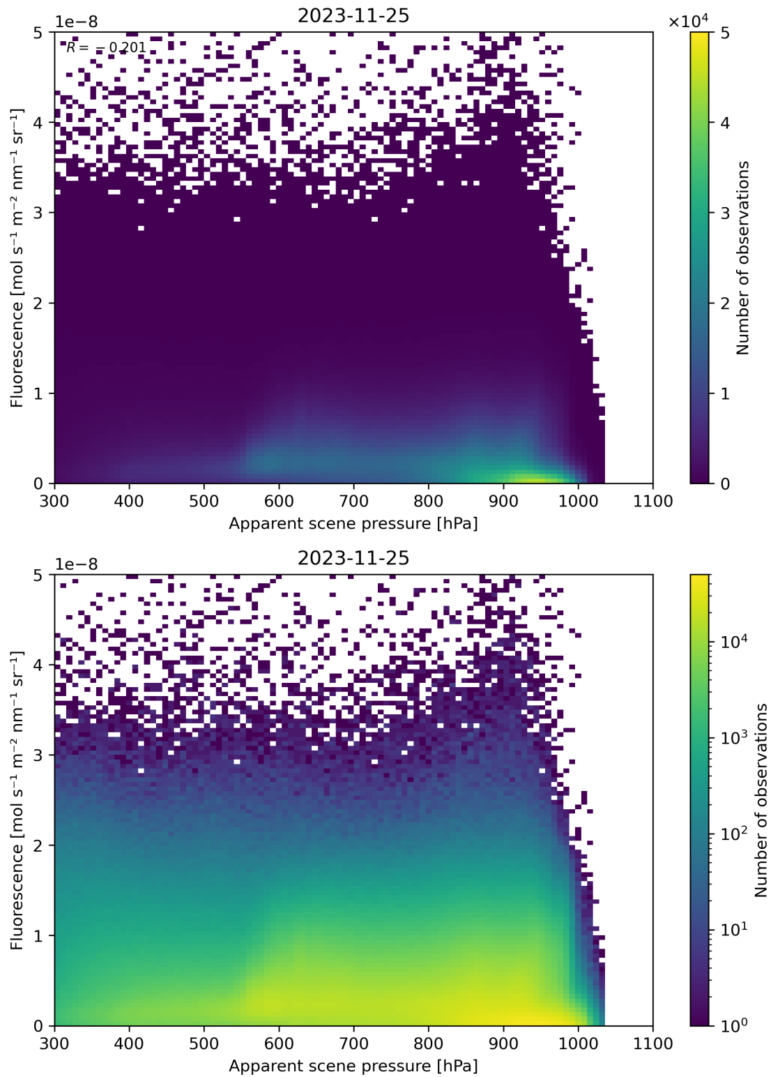
Figure 65: Scatter density plot of “Apparent scene pressure” against “Fluorescence” for 2023-11-24 to 2023-11-26.
