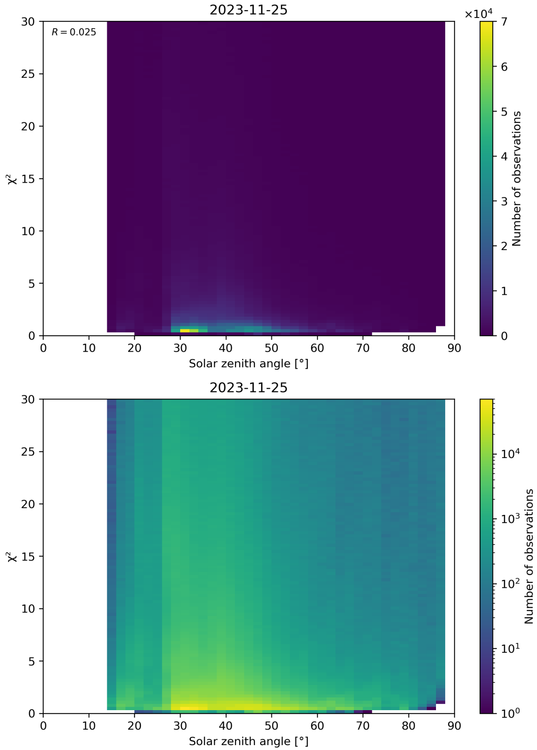
Figure 119: Scatter density plot of “Solar zenith angle” against “ \chi^2 ” for 2023-11-24 to 2023-11-26.
