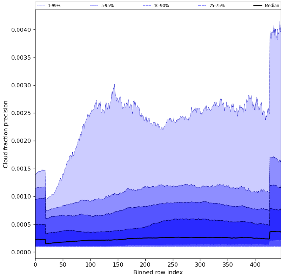
Figure 50: Along track statistics of “Cloud fraction precision” for 2023-11-24 to 2023-11-26
