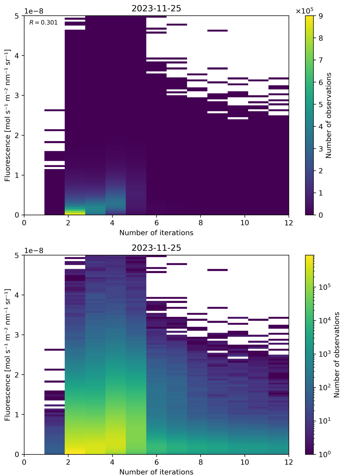
Figure 107: Scatter density plot of “Number of iterations” against “Fluorescence” for 2023-11-24 to 2023-11-26.
