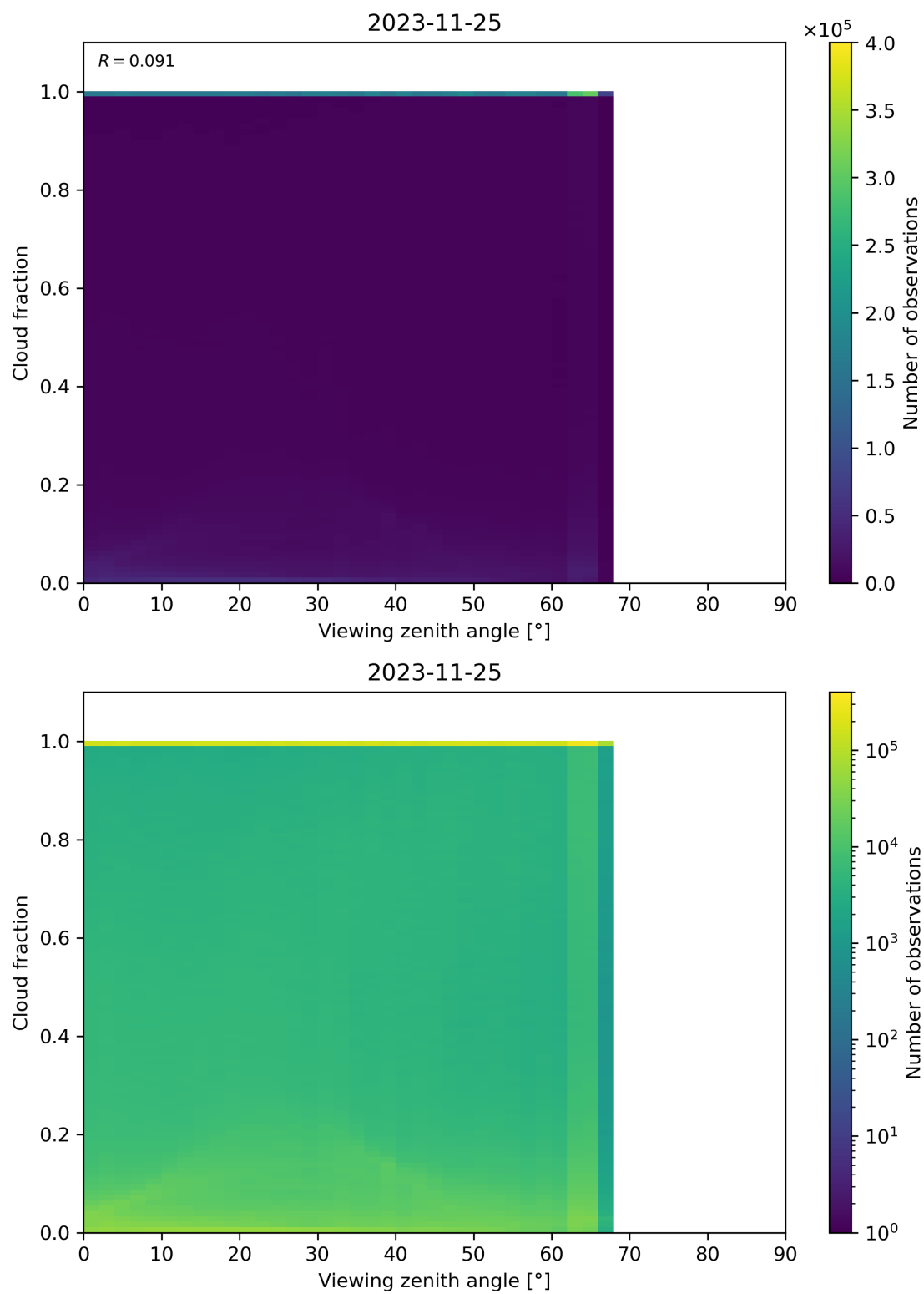
Figure 132: Scatter density plot of “Viewing zenith angle” against “Cloud fraction” for 2023-11-24 to 2023-11-26.
