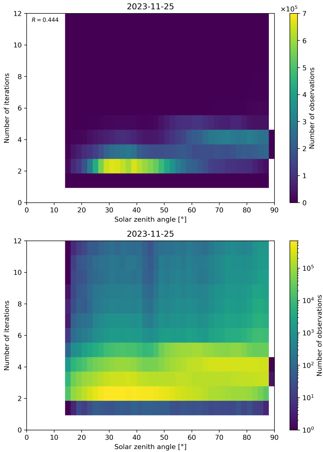
Figure 125: Scatter density plot of “Solar zenith angle” against “Number of iterations” for 2023-11-24 to 2023-11-26.
