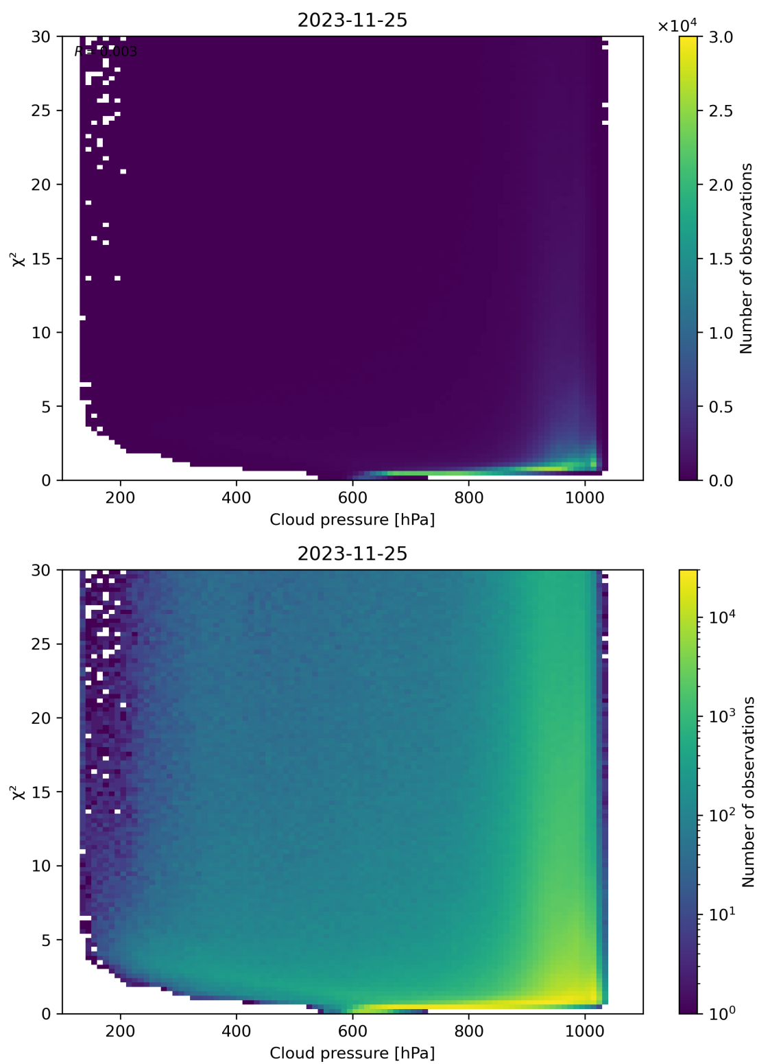
Figure 85: Scatter density plot of “Cloud pressure” against “ \chi^2 ” for 2023-11-24 to 2023-11-26.
