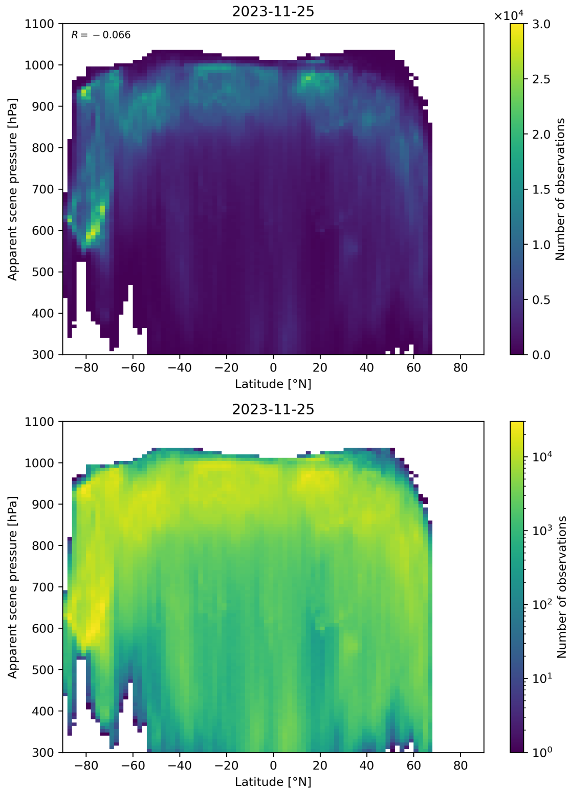
Figure 96: Scatter density plot of “Latitude” against “Apparent scene pressure” for 2023-11-24 to 2023-11-26.
