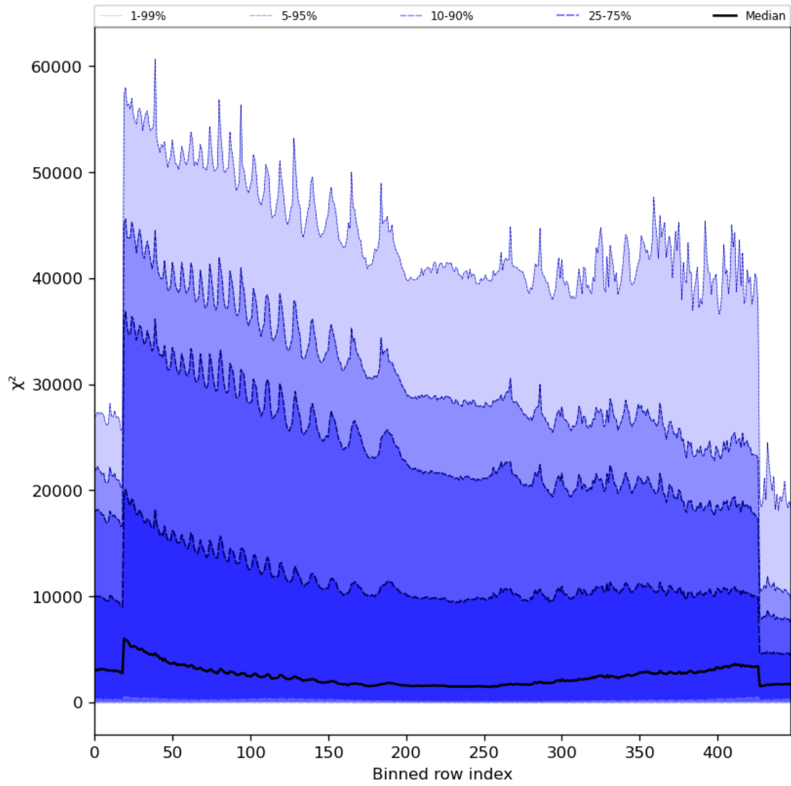
Figure 55: Along track statistics of " \chi^2 " for 2023-11-24 to 2023-11-26
