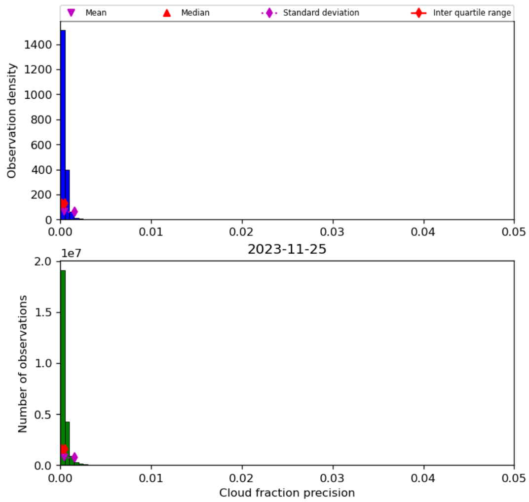
Figure 33: Histogram of “Cloud fraction precision” for 2023-11-24 to 2023-11-26
