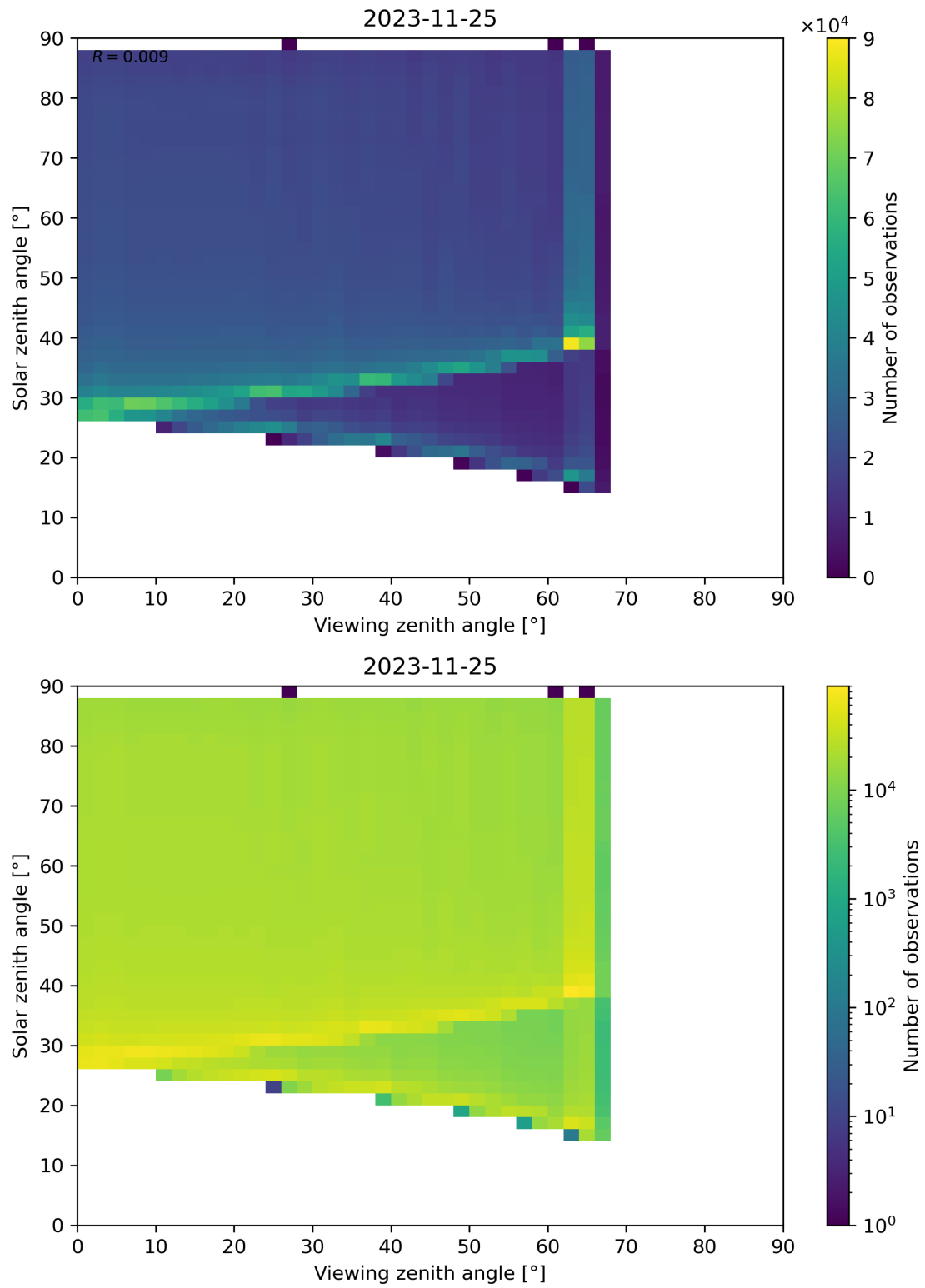
Figure 139: Scatter density plot of “Viewing zenith angle” against “Solar zenith angle” for 2023-11-24 to 2023-11-26.
