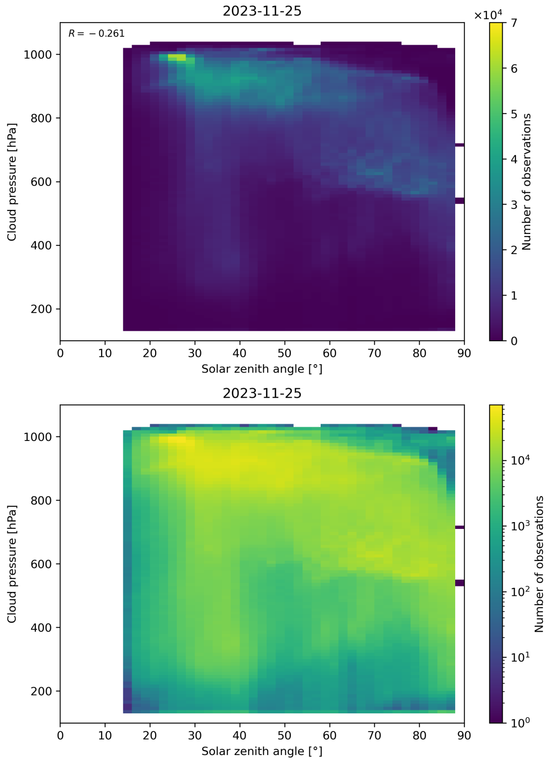
Figure 122: Scatter density plot of “Solar zenith angle” against “Cloud pressure” for 2023-11-24 to 2023-11-26.
