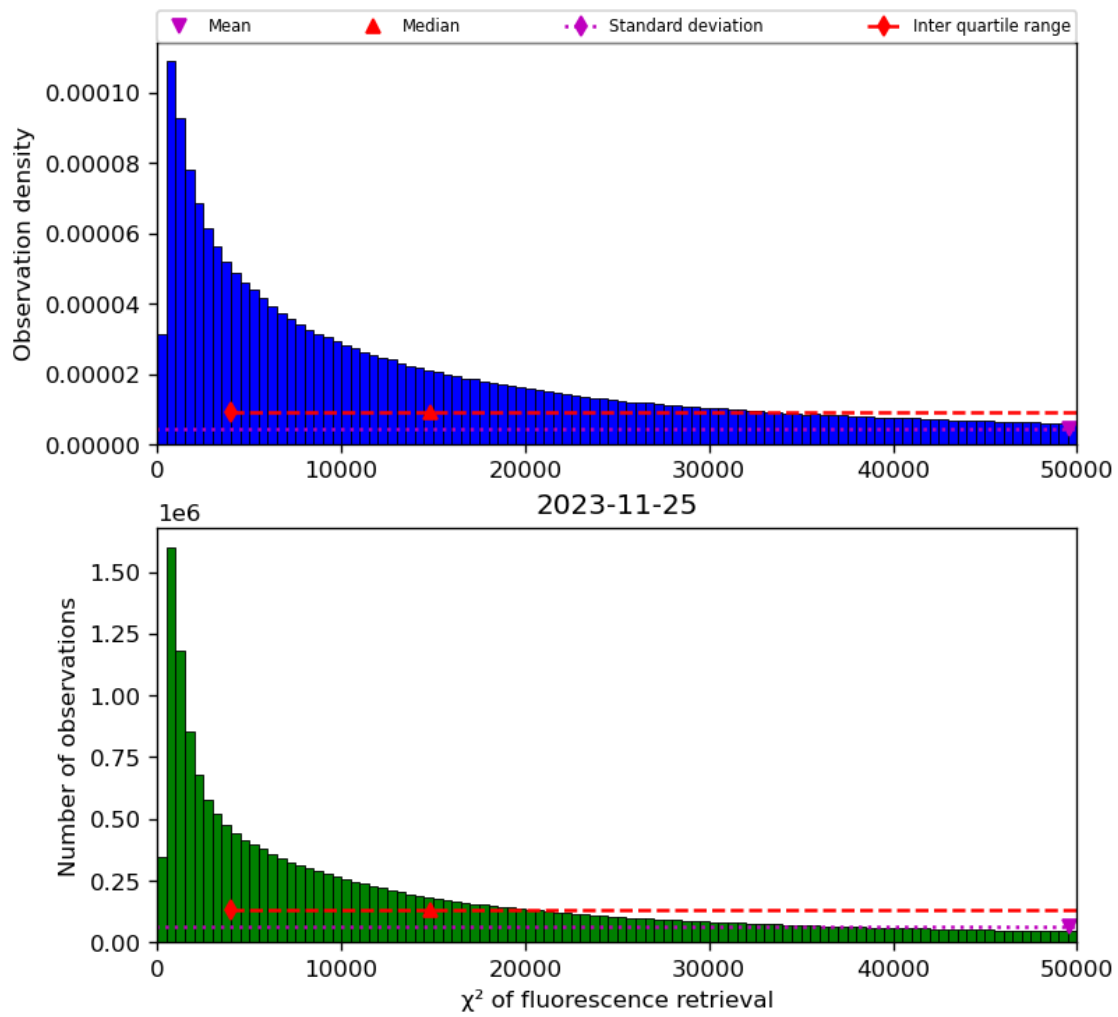
Figure 42: Histogram of “ \chi^2 of fluorescence retrieval” for 2023-11-24 to 2023-11-26
