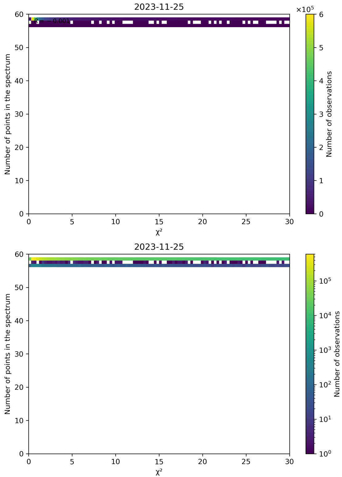
Figure 74: Scatter density plot of " \chi^2 " against "Number of points in the spectrum" for 2023-11-24 to 2023-11-26.
