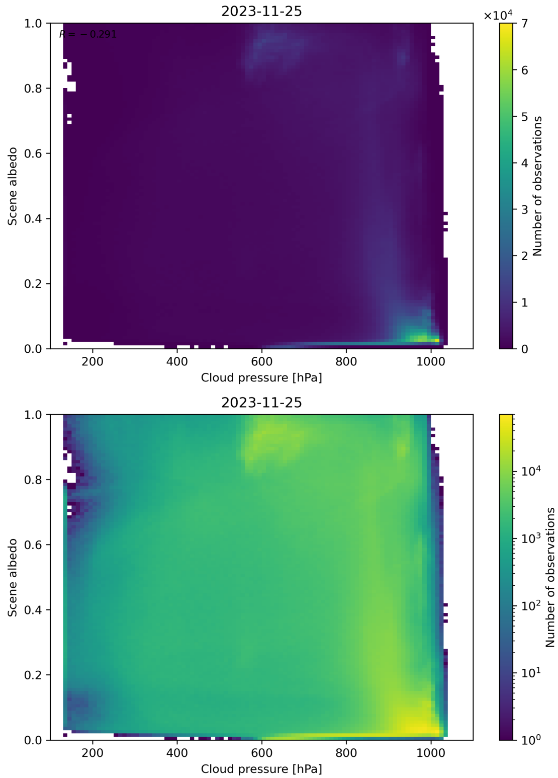
Figure 91: Scatter density plot of “Cloud pressure” against “Scene albedo” for 2023-11-24 to 2023-11-26.
