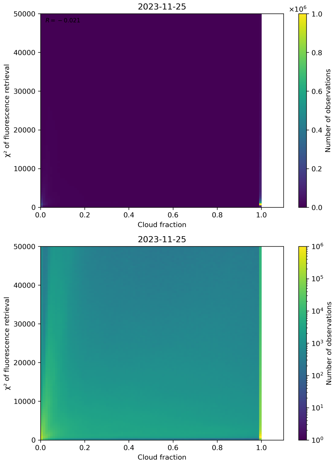
Figure 78: Scatter density plot of “Cloud fraction” against “ \chi^2 of fluorescence retrieval” for 2023-11-24 to 2023-11-26.
