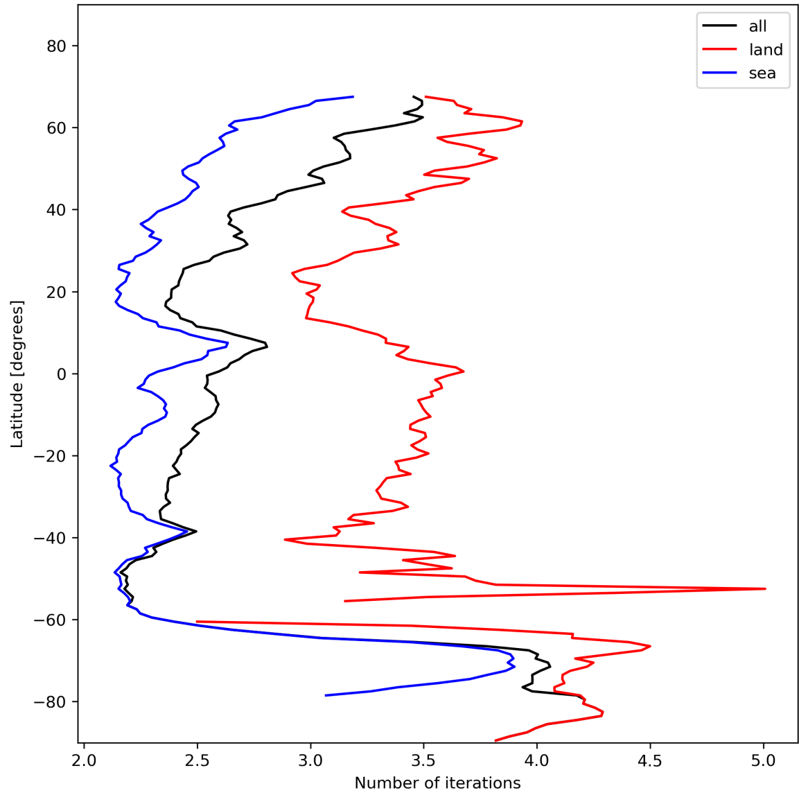
Figure 22: Zonal average of “Number of iterations” for 2023-11-24 to 2023-11-26.
