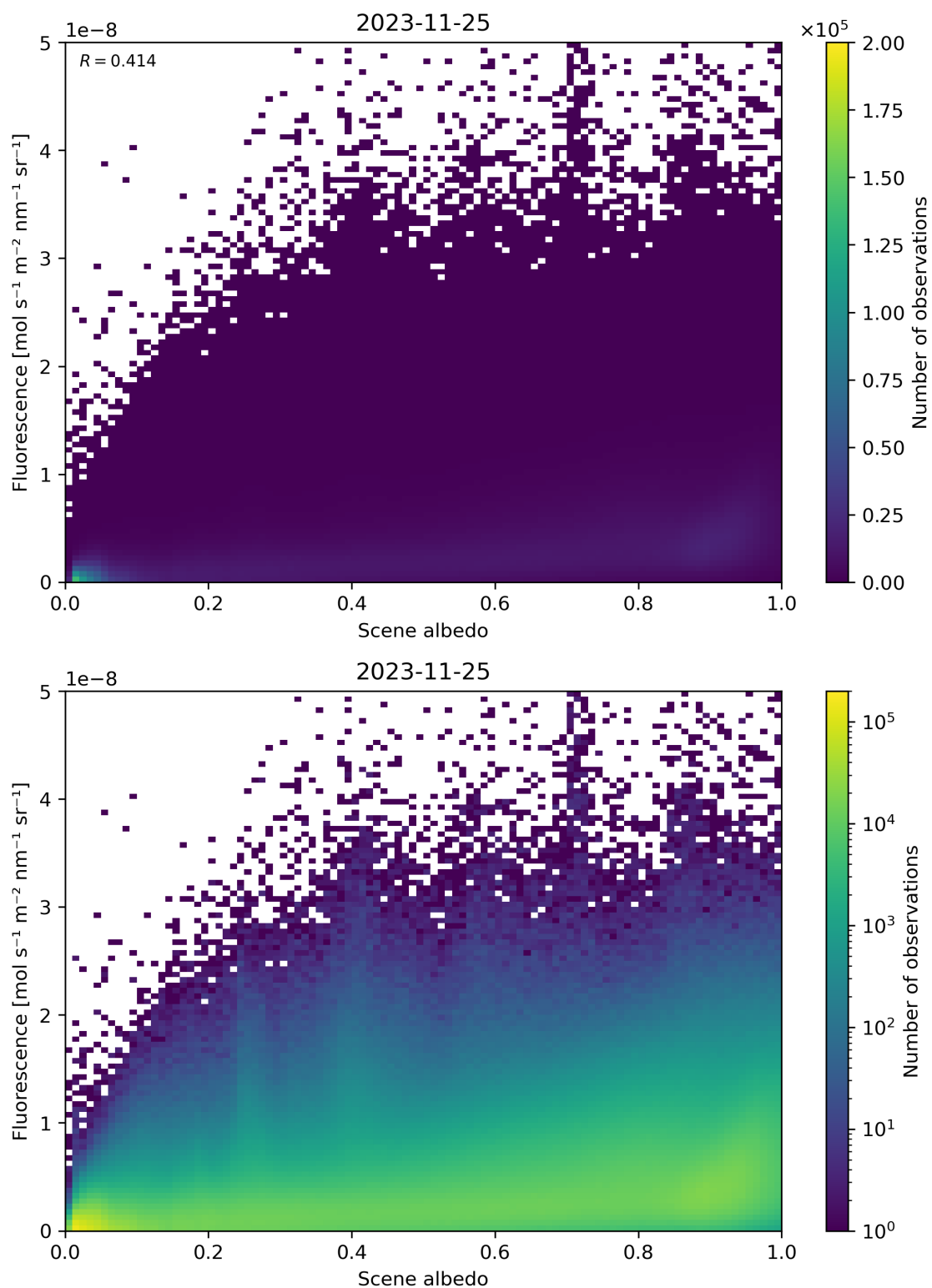
Figure 114: Scatter density plot of “Scene albedo” against “Fluorescence” for 2023-11-24 to 2023-11-26.
