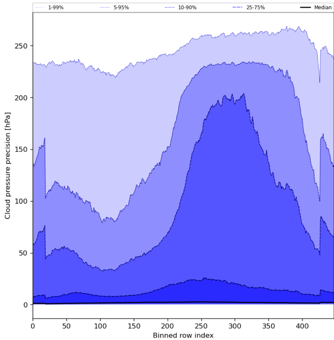
Figure 48: Along track statistics of “Cloud pressure precision” for 2023-11-24 to 2023-11-26
