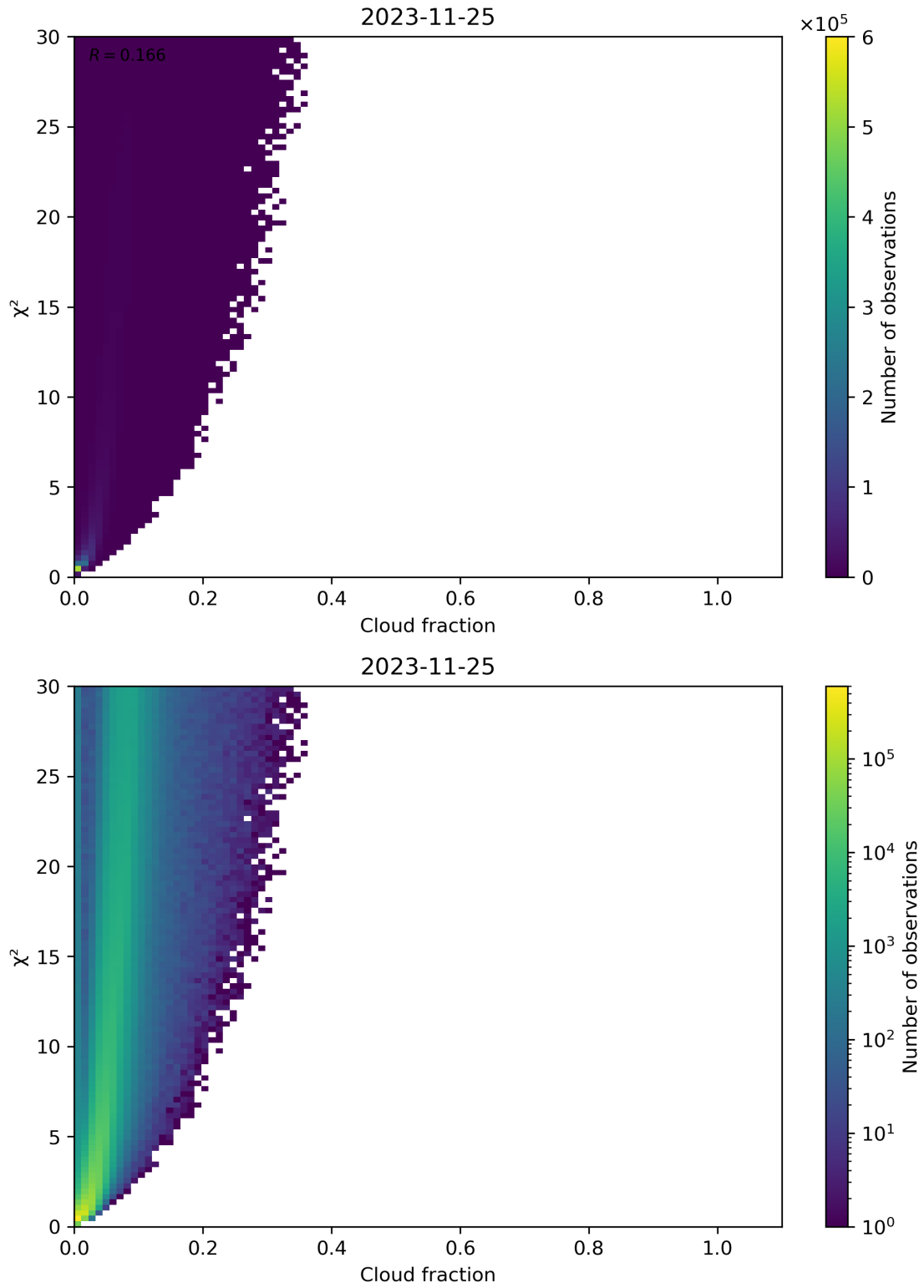
Figure 77: Scatter density plot of “Cloud fraction” against “ \chi^2 ” for 2023-11-24 to 2023-11-26.
