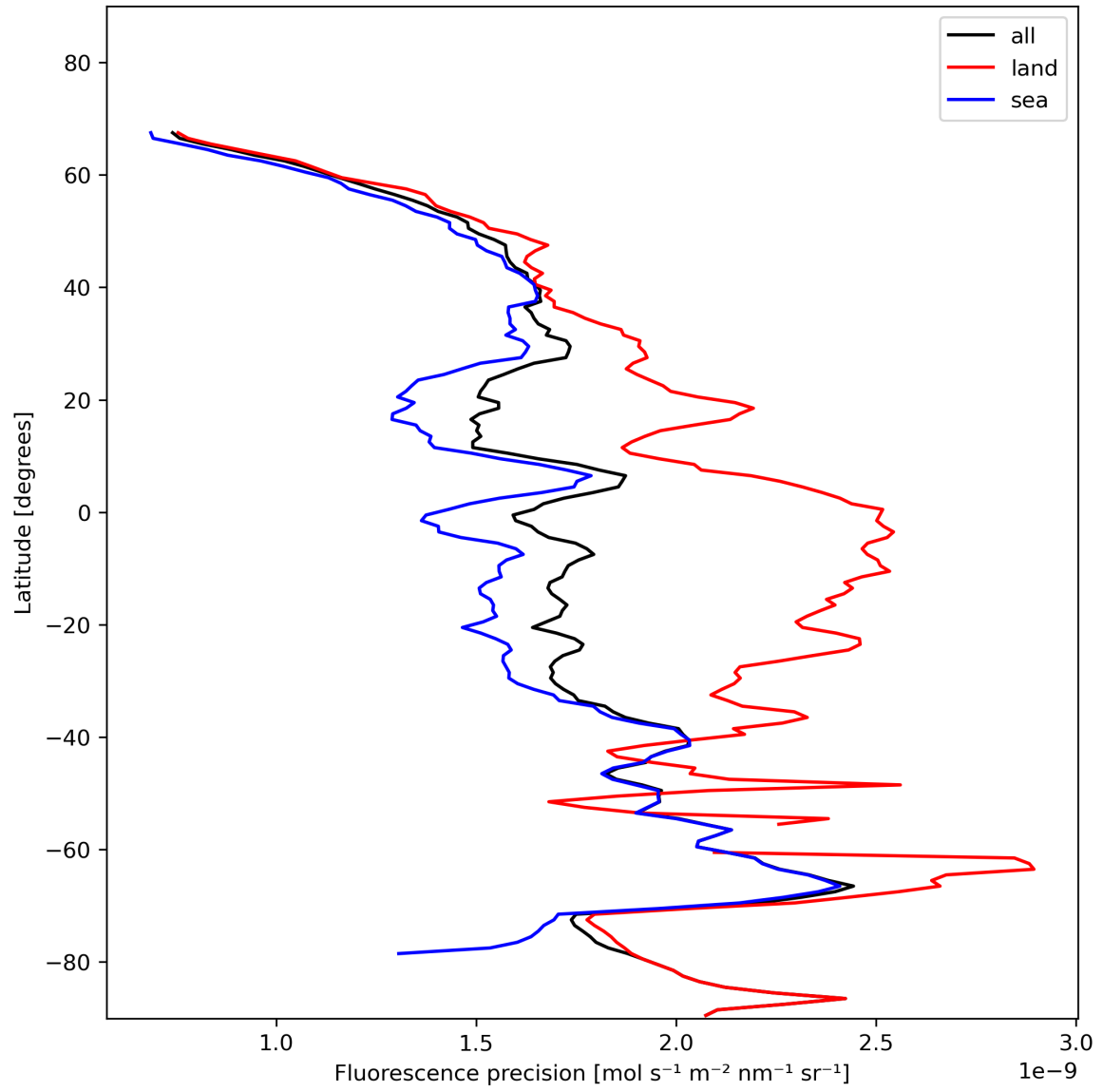
Figure 24: Zonal average of “Fluorescence precision” for 2023-11-24 to 2023-11-26.
