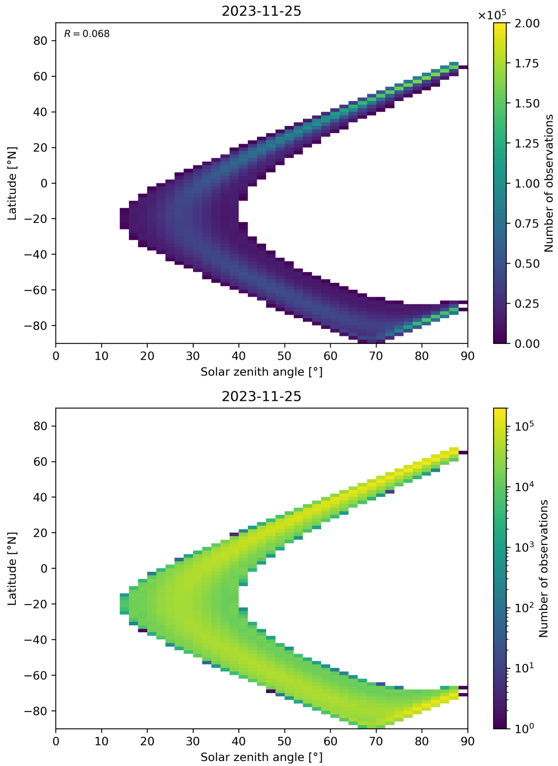
Figure 124: Scatter density plot of “Solar zenith angle” against “Latitude” for 2023-11-24 to 2023-11-26.
