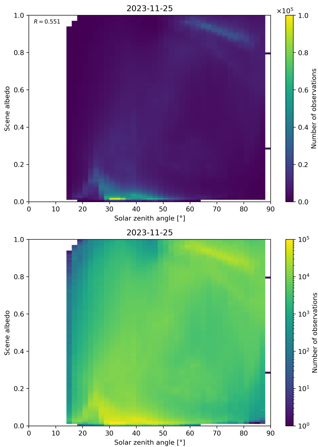
Figure 127: Scatter density plot of “Solar zenith angle” against “Scene albedo” for 2023-11-24 to 2023-11-26.
