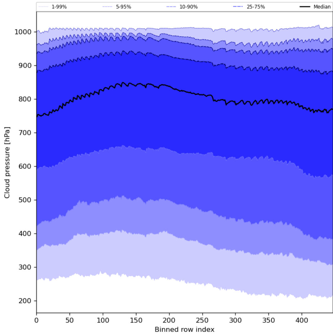
Figure 47: Along track statistics of “Cloud pressure” for 2023-11-24 to 2023-11-26
