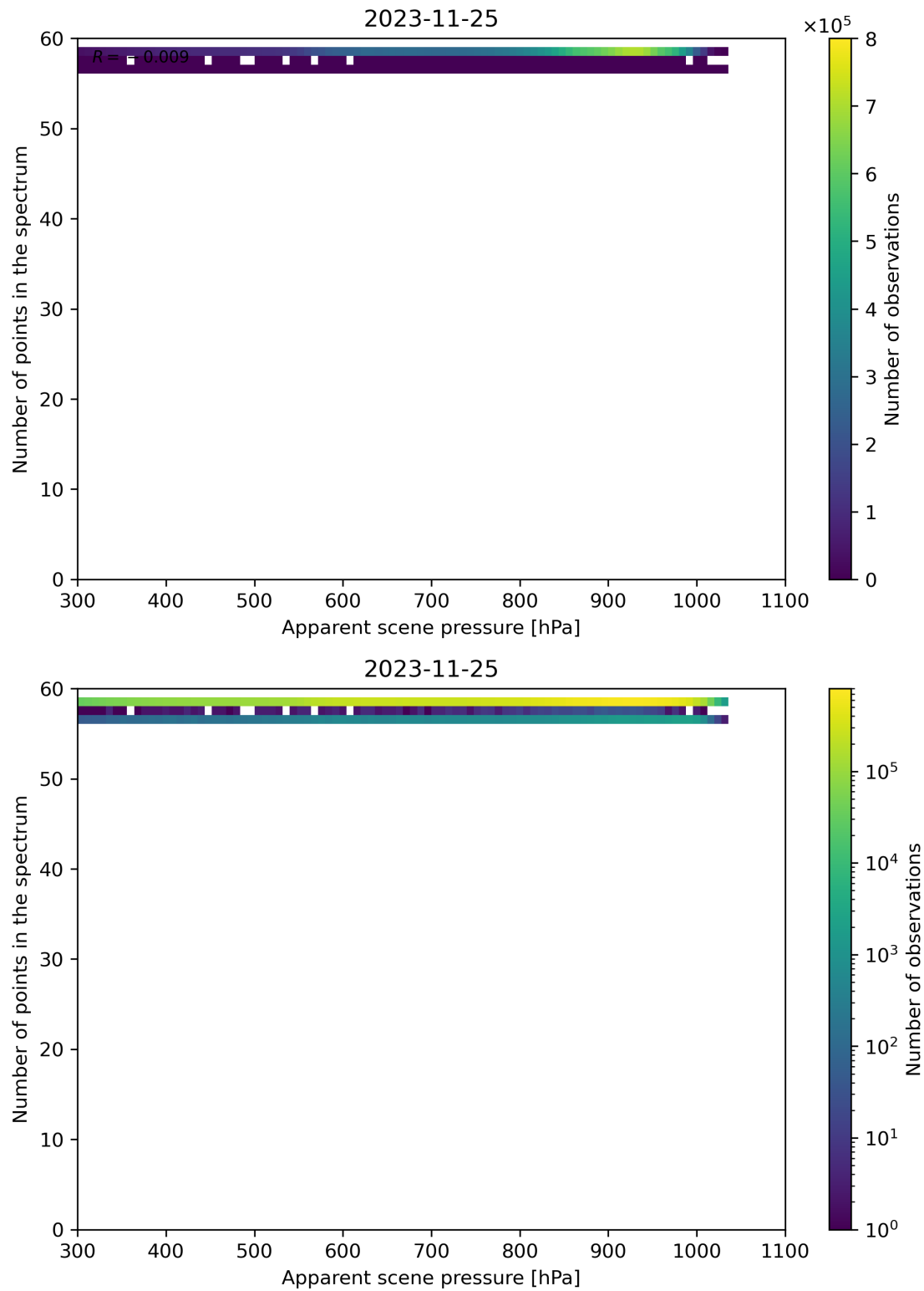
Figure 67: Scatter density plot of “Apparent scene pressure” against “Number of points in the spectrum” for 2023-11-24 to 2023-11-26.
