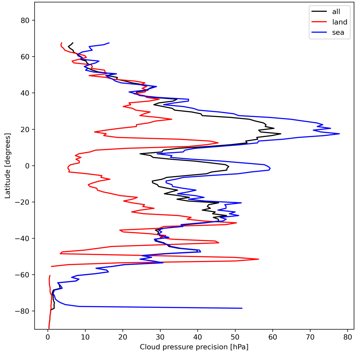
Figure 14: Zonal average of “Cloud pressure precision” for 2023-11-24 to 2023-11-26.
