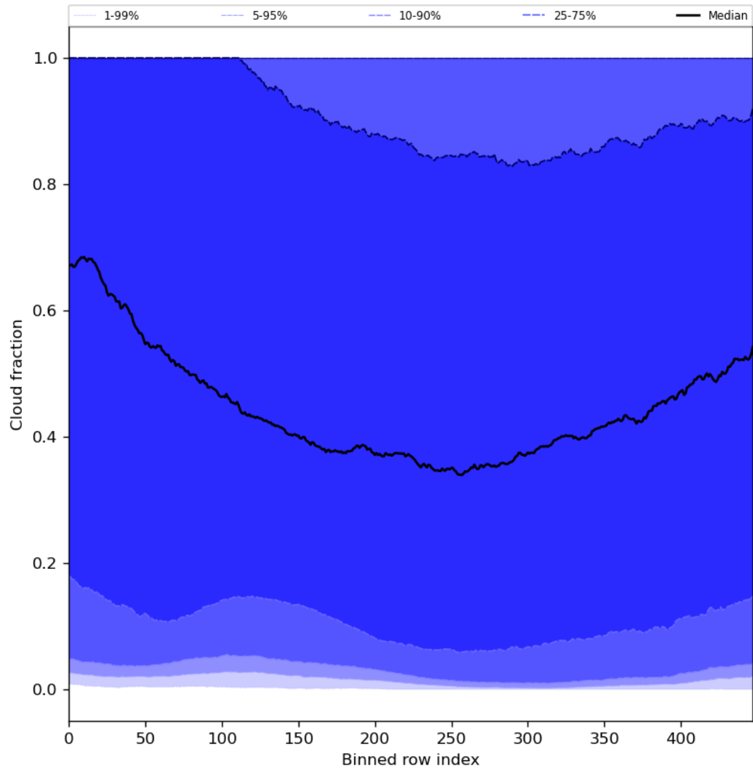
Figure 49: Along track statistics of “Cloud fraction” for 2023-11-24 to 2023-11-26
