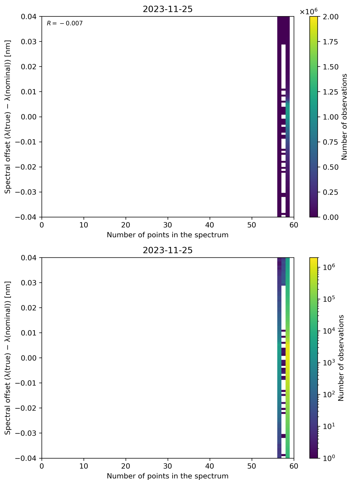
Figure 110: Scatter density plot of “Number of points in the spectrum” against “Spectral offset ( \lambda(\text{true}) - \lambda(\text{nominal}) )” for 2023-11-24 to 2023-11-26.
