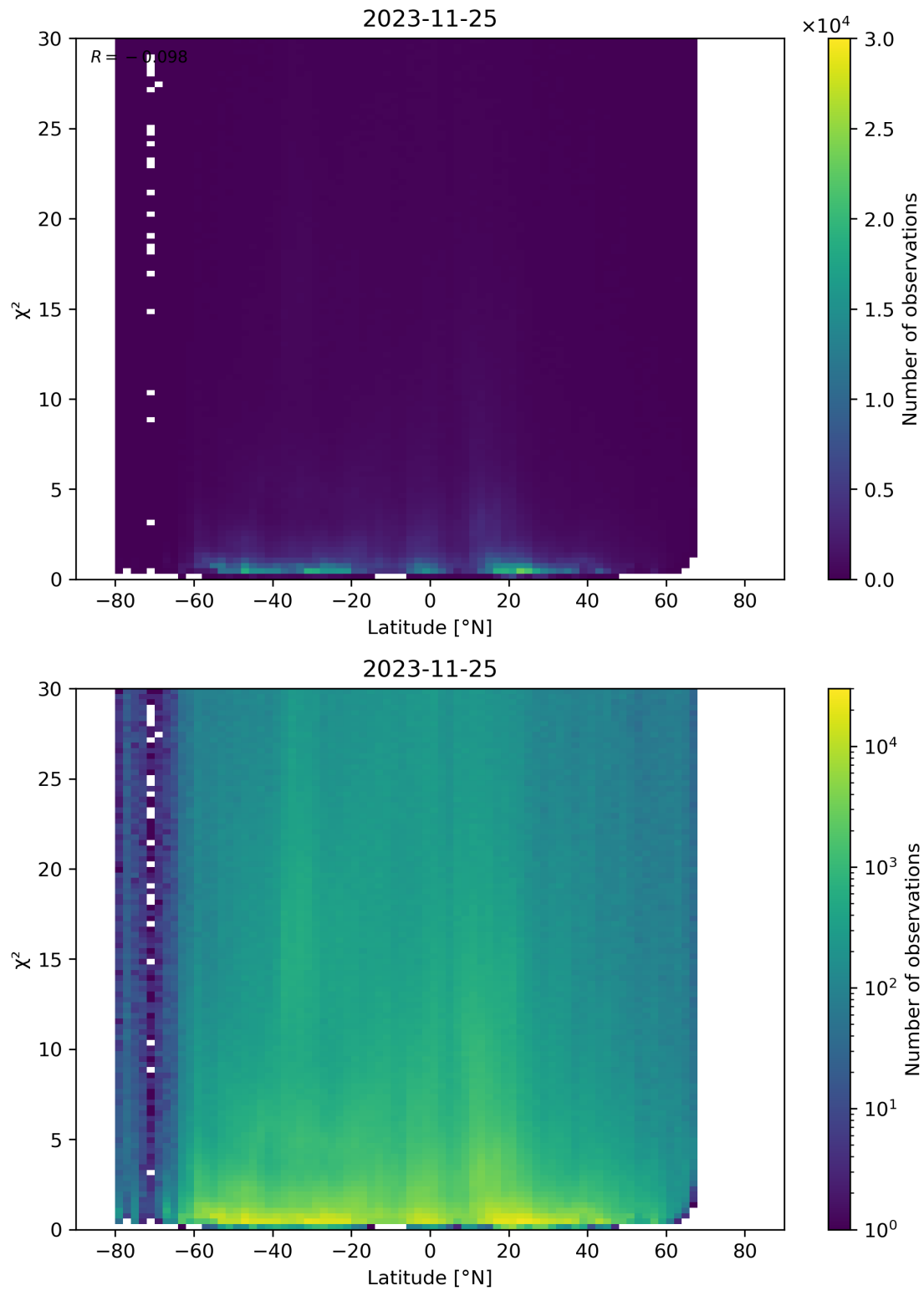
Figure 97: Scatter density plot of “Latitude” against “ \chi^2 ” for 2023-11-24 to 2023-11-26.
