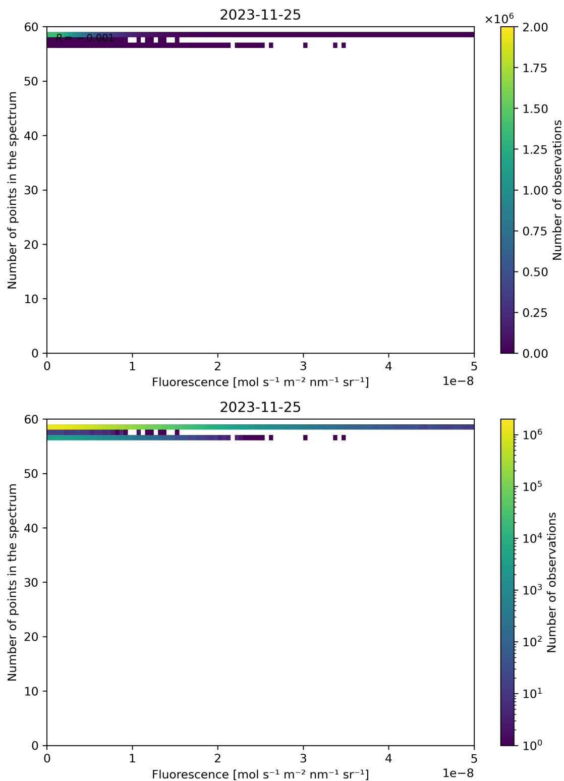
Figure 94: Scatter density plot of “Fluorescence” against “Number of points in the spectrum” for 2023-11-24 to 2023-11-26.
