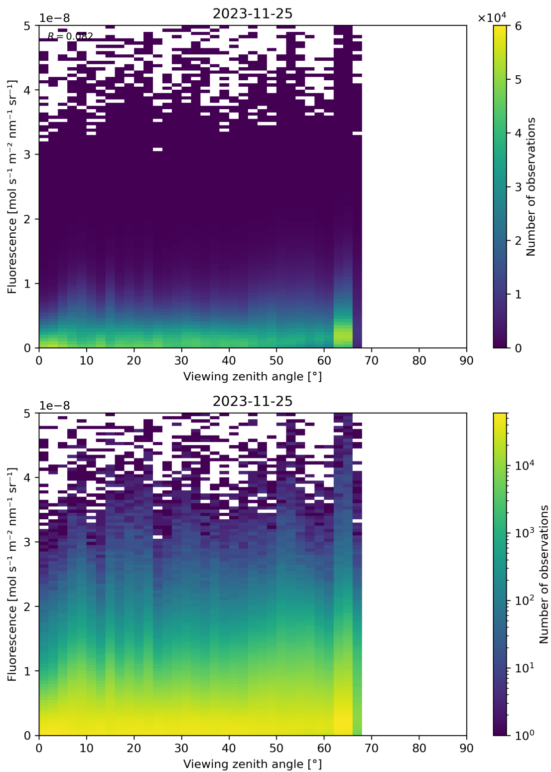
Figure 134: Scatter density plot of “Viewing zenith angle” against “Fluorescence” for 2023-11-24 to 2023-11-26.
