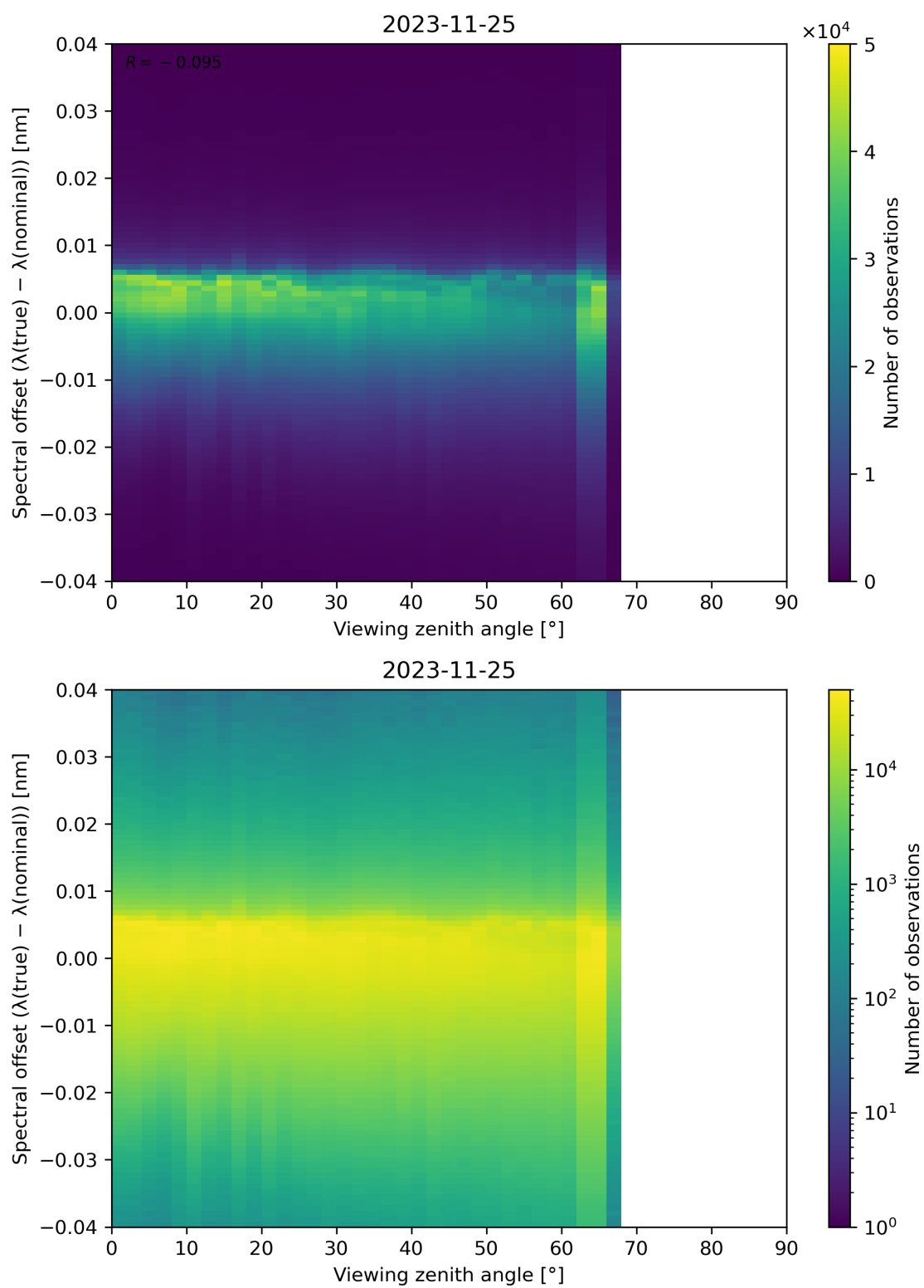
Figure 140: Scatter density plot of “Viewing zenith angle” against “Spectral offset ( \lambda(\text{true}) - \lambda(\text{nominal}) )” for 2023-11-24 to 2023-11-26.
