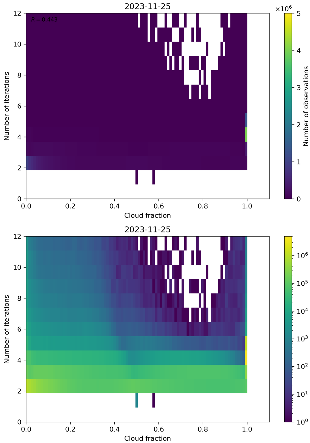
Figure 80: Scatter density plot of “Cloud fraction” against “Number of iterations” for 2023-11-24 to 2023-11-26.
