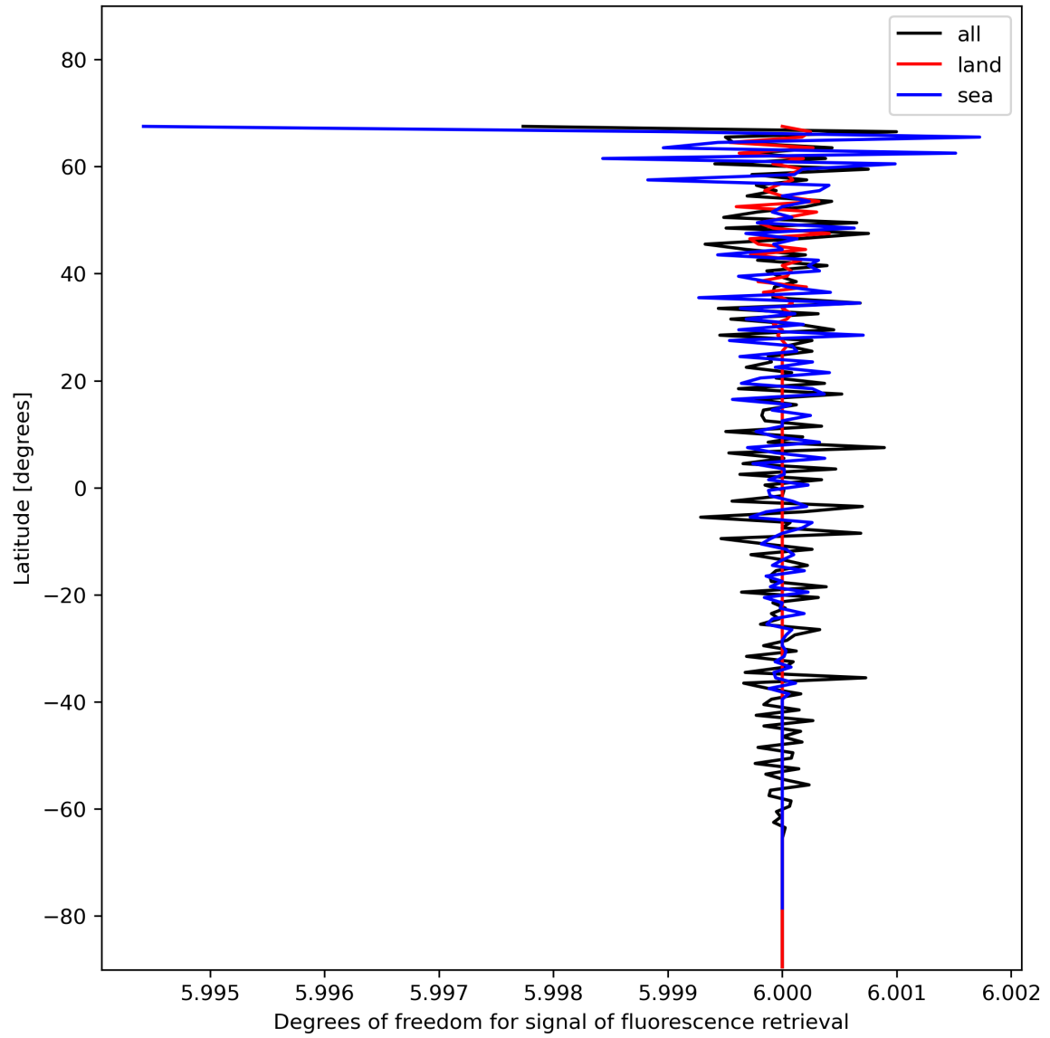
Figure 26: Zonal average of “Degrees of freedom for signal of fluorescence retrieval” for 2023-11-24 to 2023-11-26.
