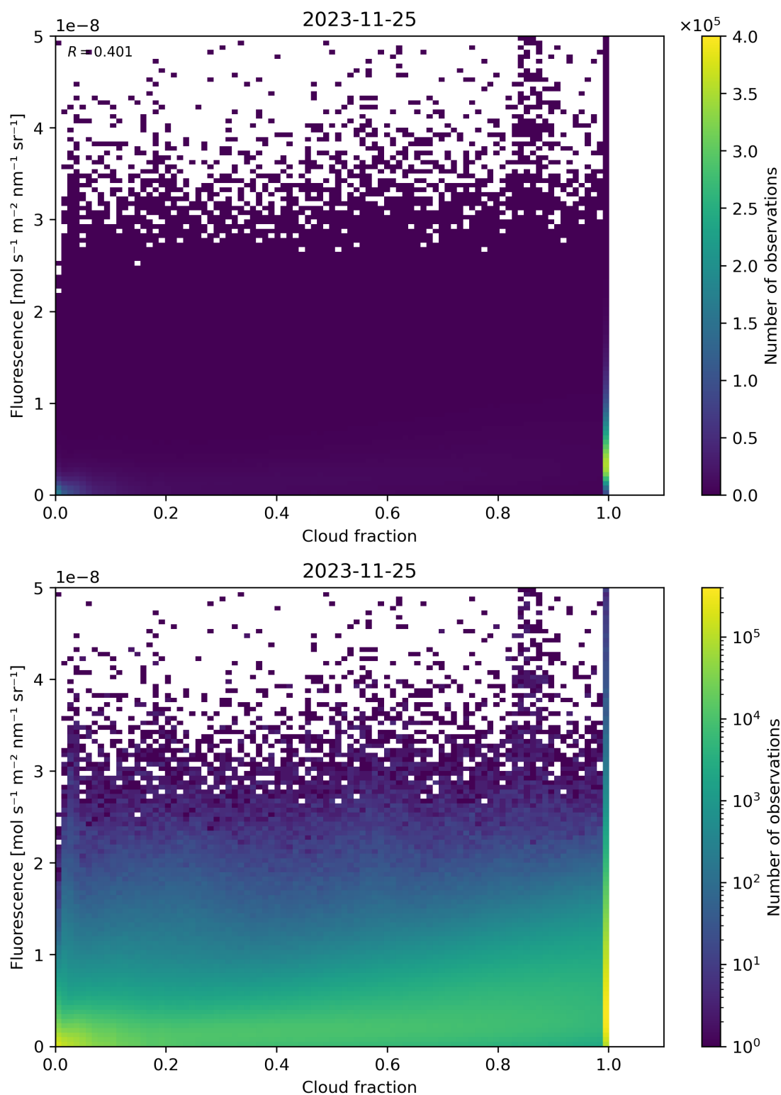
Figure 79: Scatter density plot of “Cloud fraction” against “Fluorescence” for 2023-11-24 to 2023-11-26.
