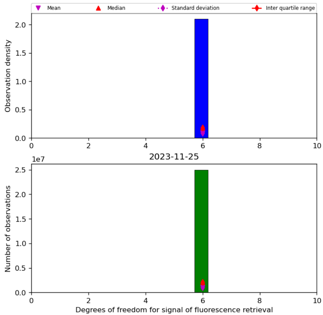
Figure 43: Histogram of “Degrees of freedom for signal of fluorescence retrieval” for 2023-11-24 to 2023-11-26
