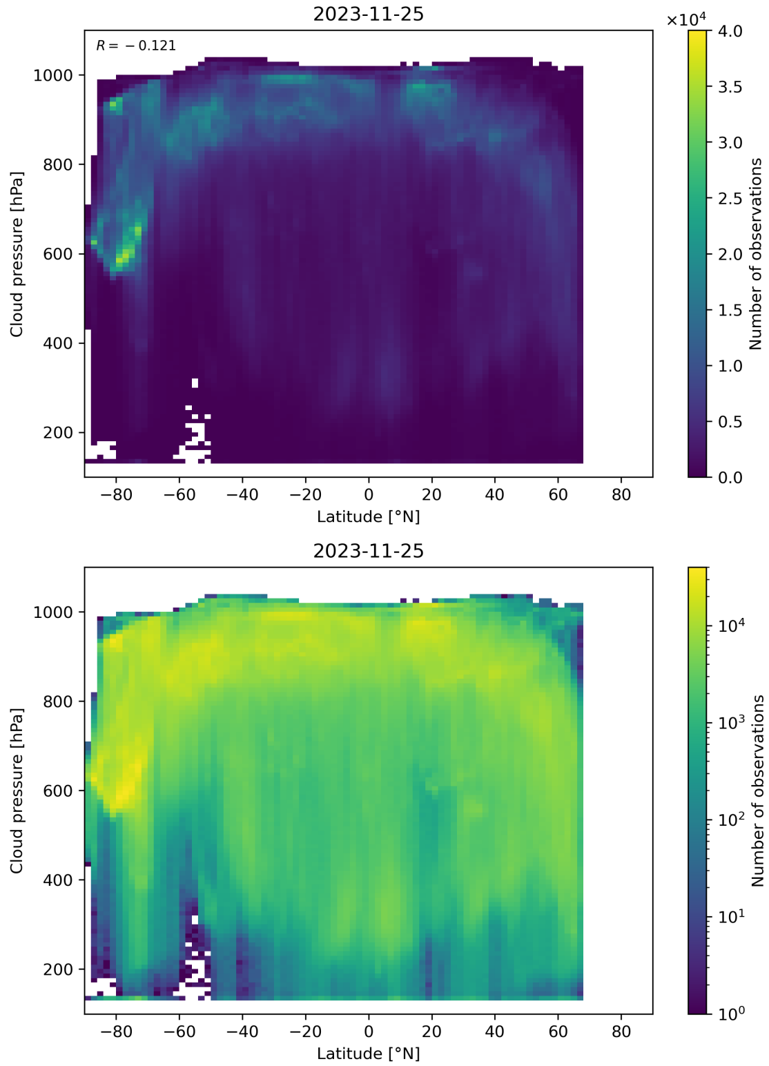
Figure 100: Scatter density plot of “Latitude” against “Cloud pressure” for 2023-11-24 to 2023-11-26.
