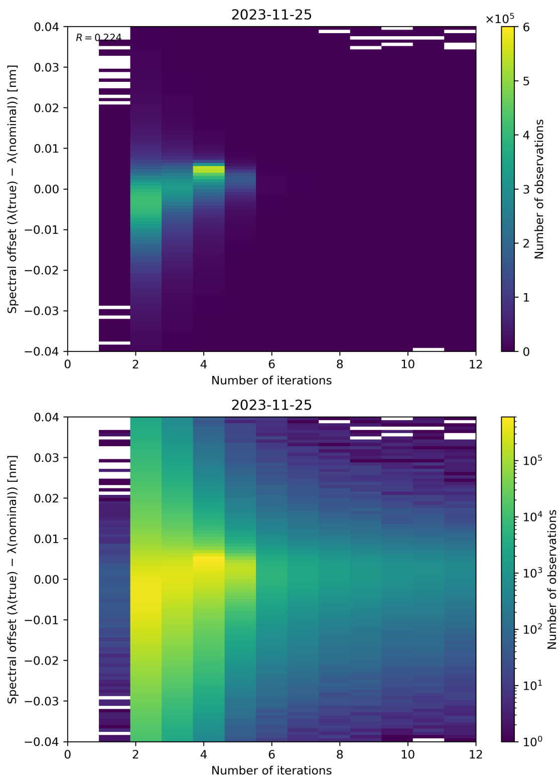
Figure 109: Scatter density plot of “Number of iterations” against “Spectral offset ( \lambda(\text{true}) - \lambda(\text{nominal}) )” for 2023-11-24 to 2023-11-26.
