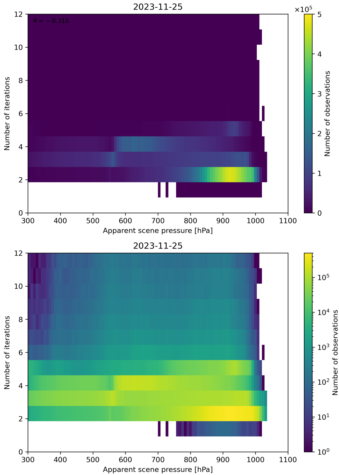
Figure 66: Scatter density plot of “Apparent scene pressure” against “Number of iterations” for 2023-11-24 to 2023-11-26.
