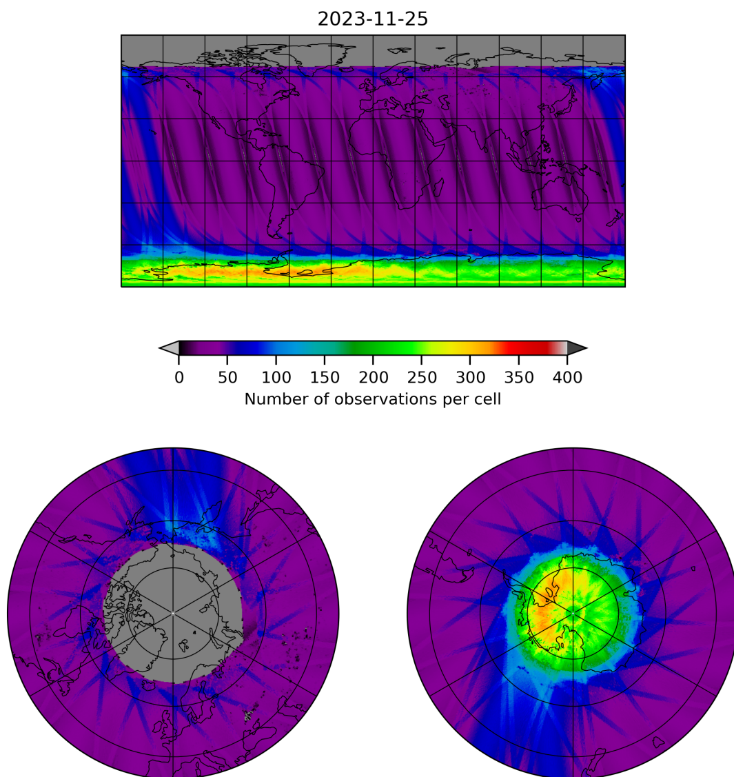
Figure 11: Map of the number of observations for 2023-11-24 to 2023-11-26
