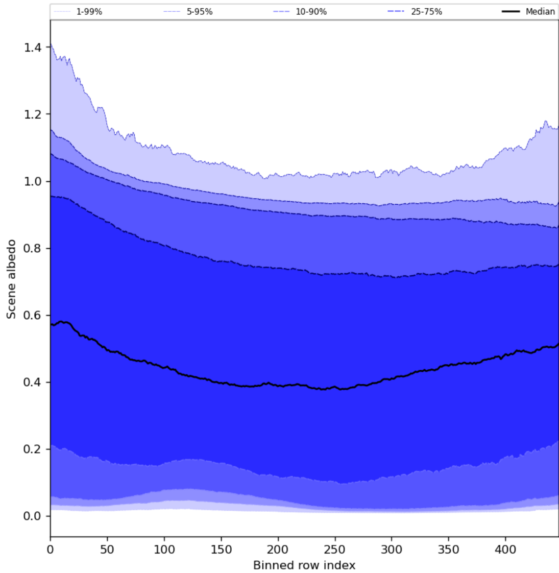
Figure 51: Along track statistics of “Scene albedo” for 2023-11-24 to 2023-11-26
