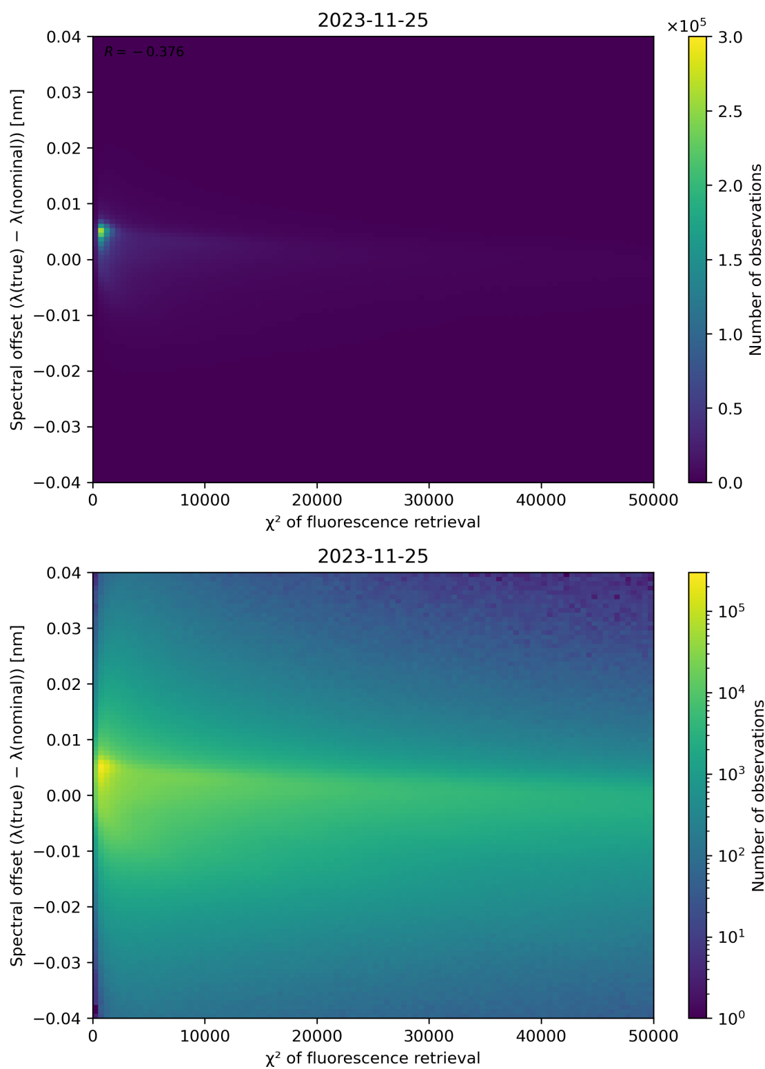
Figure 72: Scatter density plot of " \chi^2 of fluorescence retrieval" against "Spectral offset ( \lambda(\text{true}) - \lambda(\text{nominal}) )" for 2023-11-24 to 2023-11-26.
