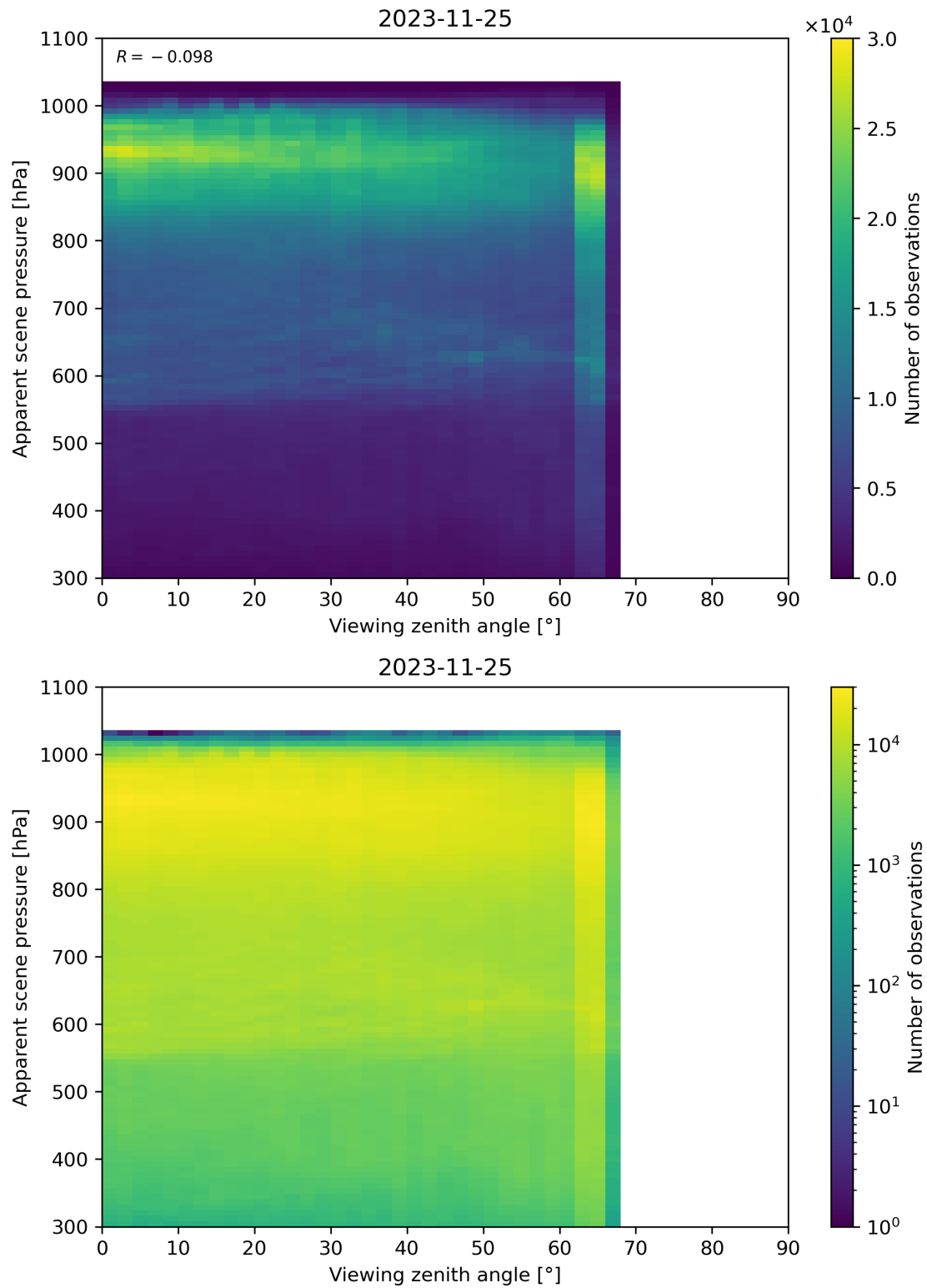
Figure 129: Scatter density plot of “Viewing zenith angle” against “Apparent scene pressure” for 2023-11-24 to 2023-11-26.
