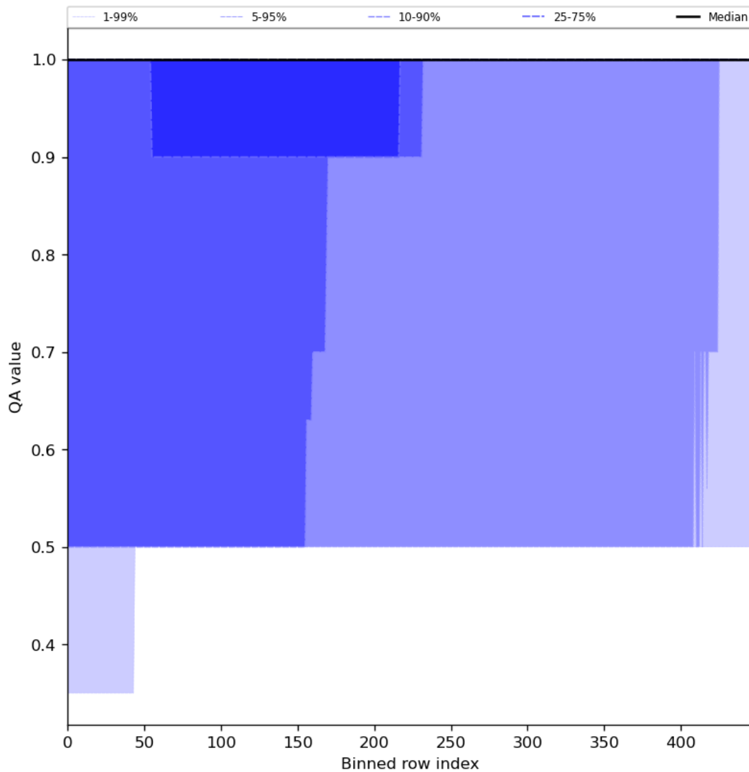
Figure 46: Along track statistics of “QA value” for 2023-11-24 to 2023-11-26
