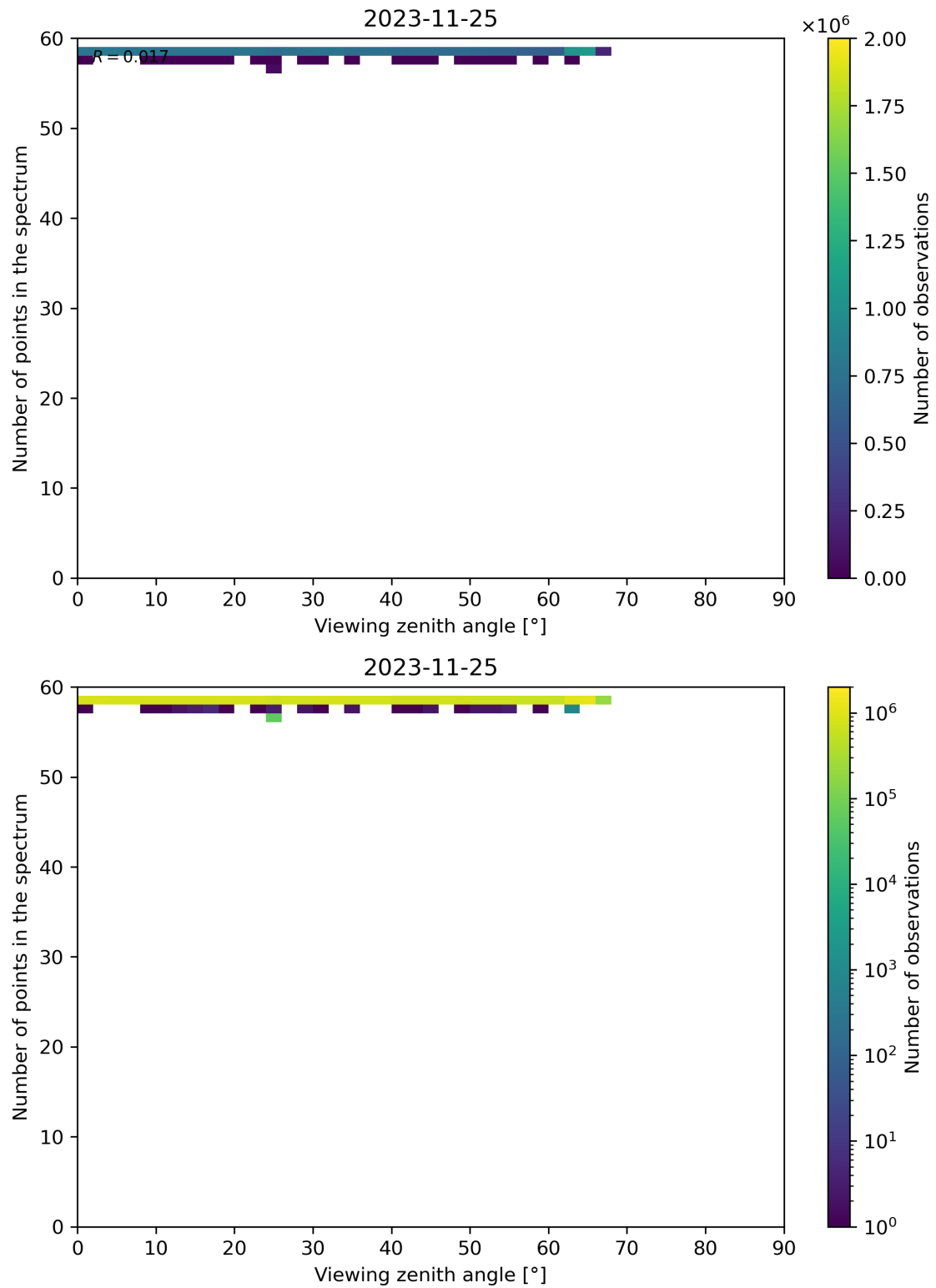
Figure 137: Scatter density plot of “Viewing zenith angle” against “Number of points in the spectrum” for 2023-11-24 to 2023-11-26.
