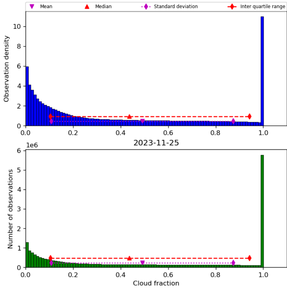
Figure 32: Histogram of “Cloud fraction” for 2023-11-24 to 2023-11-26
