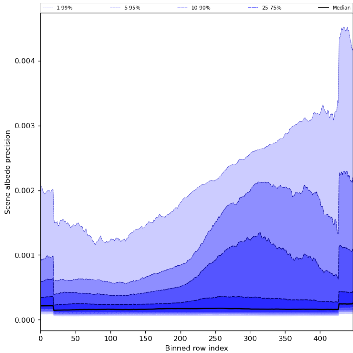
Figure 52: Along track statistics of “Scene albedo precision” for 2023-11-24 to 2023-11-26
