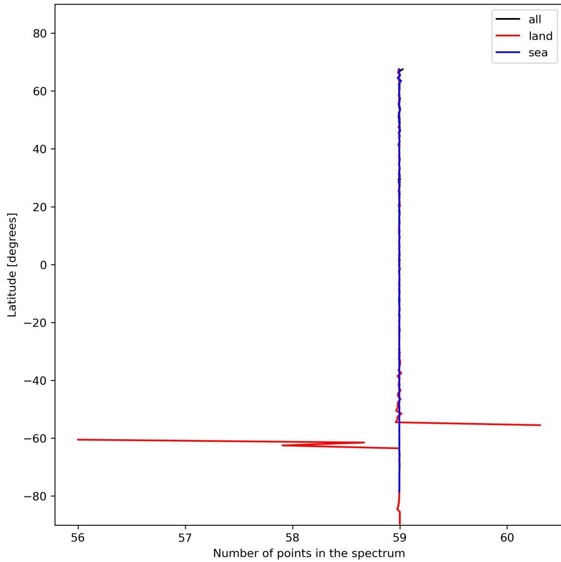
Figure 27: Zonal average of “Number of points in the spectrum” for 2023-11-24 to 2023-11-26.
