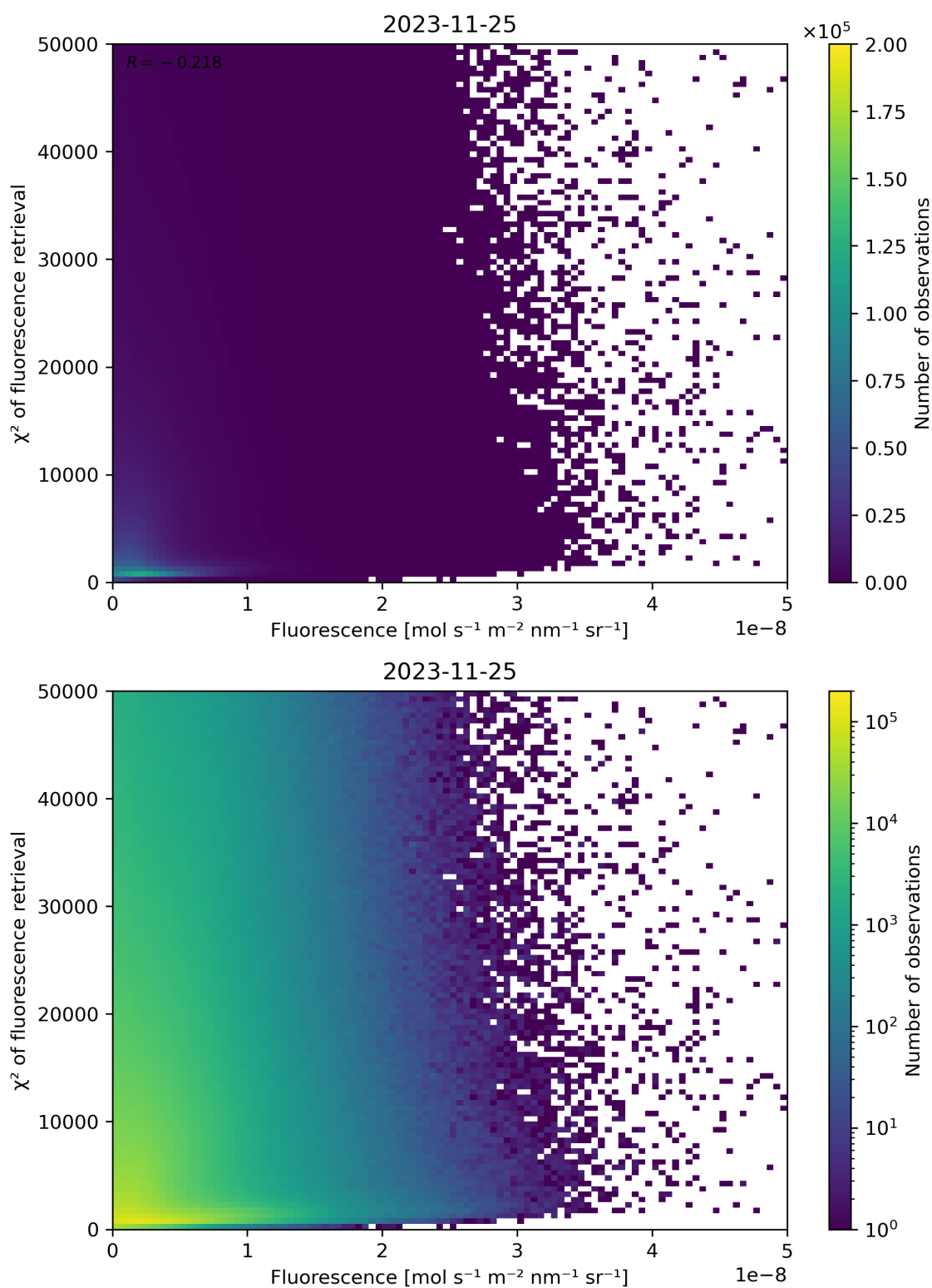
Figure 93: Scatter density plot of “Fluorescence” against “ \chi^2 of fluorescence retrieval” for 2023-11-24 to 2023-11-26.
