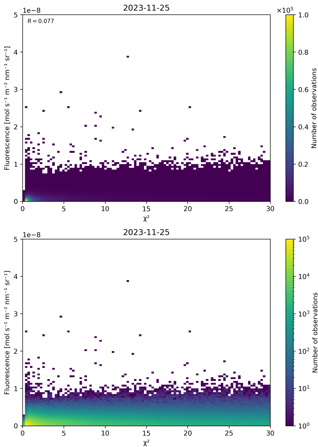
Figure 70: Scatter density plot of “ \chi^2 ” against “Fluorescence” for 2023-11-24 to 2023-11-26.
