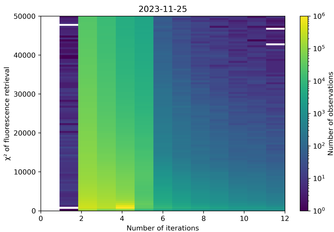
Figure 106: Scatter density plot of “Number of iterations” against “ \chi^2 of fluorescence retrieval” for 2023-11-24 to 2023-11-26.
