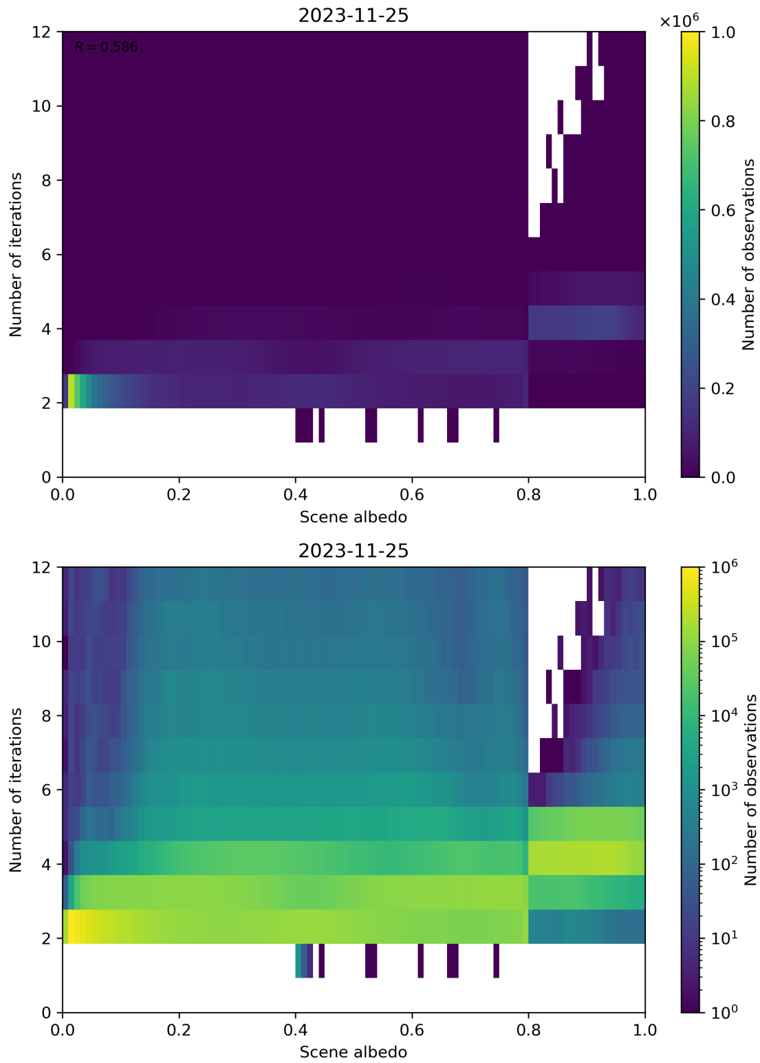
Figure 115: Scatter density plot of “Scene albedo” against “Number of iterations” for 2023-11-24 to 2023-11-26.
