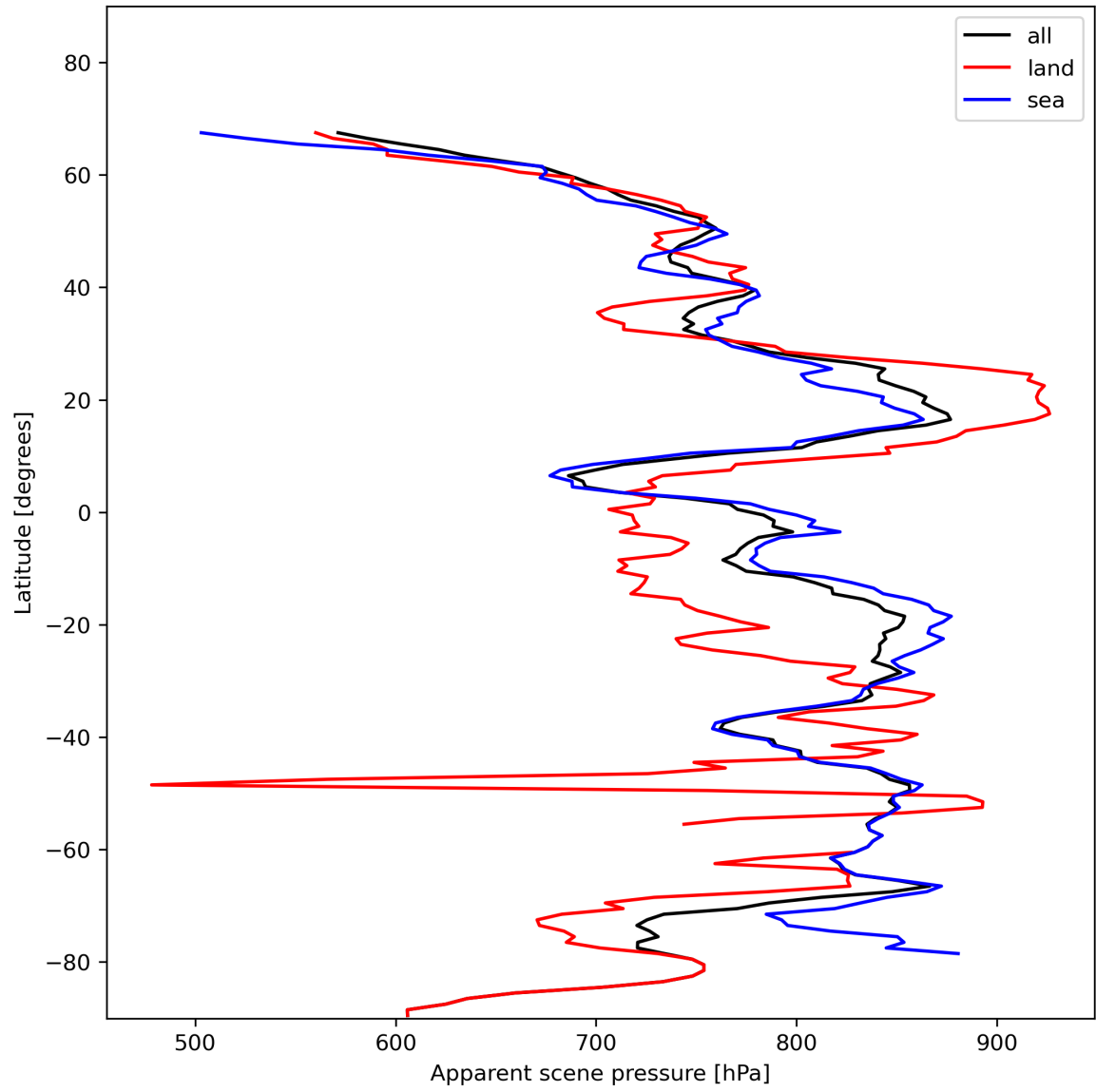
Figure 19: Zonal average of “Apparent scene pressure” for 2023-11-24 to 2023-11-26.
