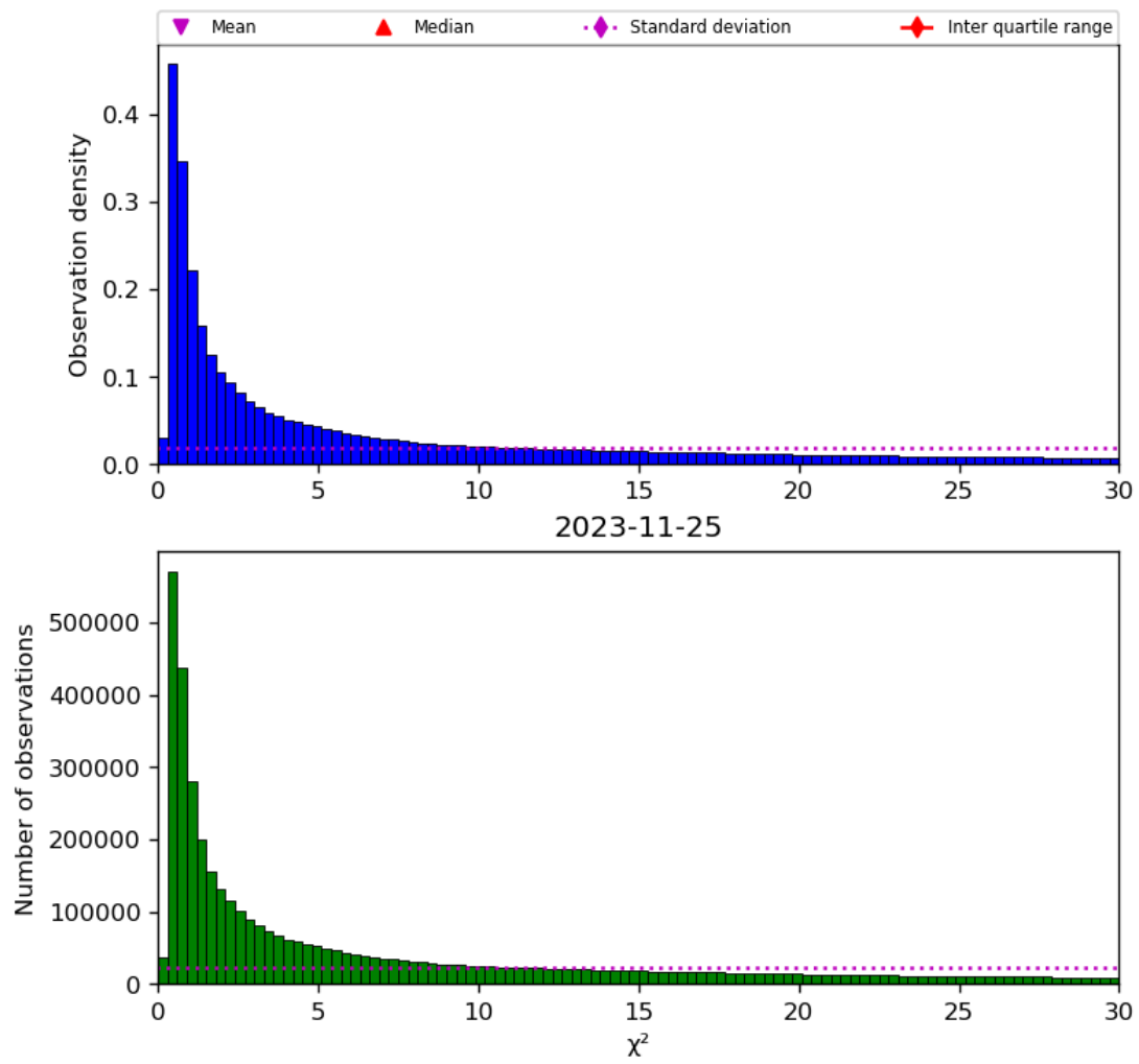
Figure 38: Histogram of " \chi^2 " for 2023-11-24 to 2023-11-26
