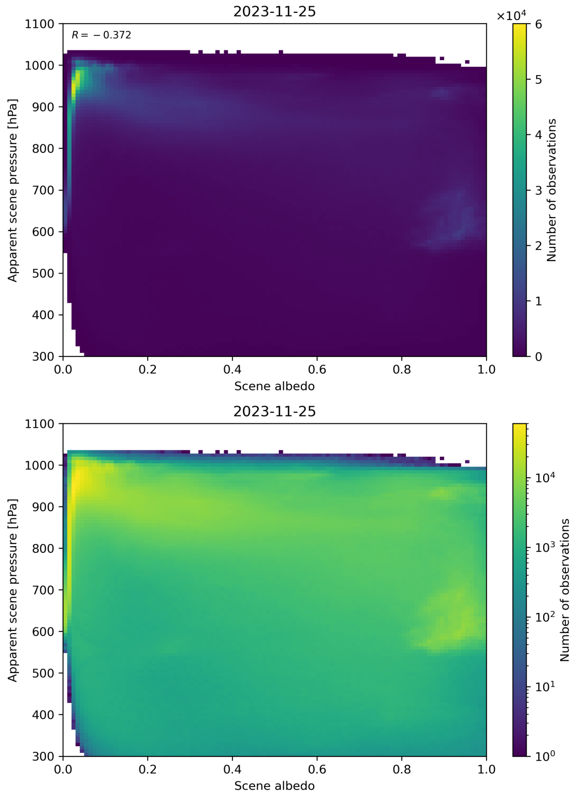
Figure 111: Scatter density plot of “Scene albedo” against “Apparent scene pressure” for 2023-11-24 to 2023-11-26.
