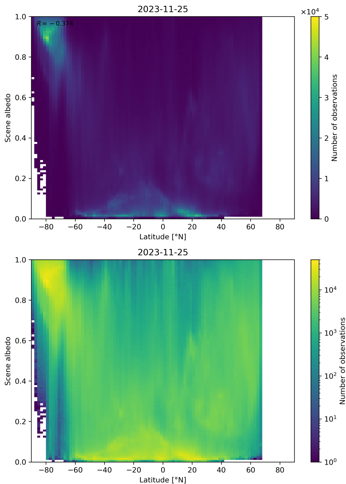
Figure 104: Scatter density plot of “Latitude” against “Scene albedo” for 2023-11-24 to 2023-11-26.
