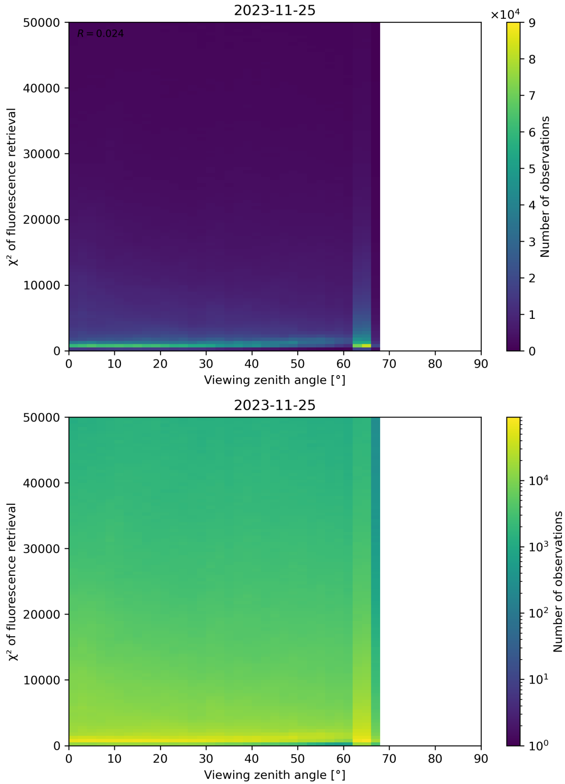
Figure 131: Scatter density plot of “Viewing zenith angle” against “ \chi^2 of fluorescence retrieval” for 2023-11-24 to 2023-11-26.
