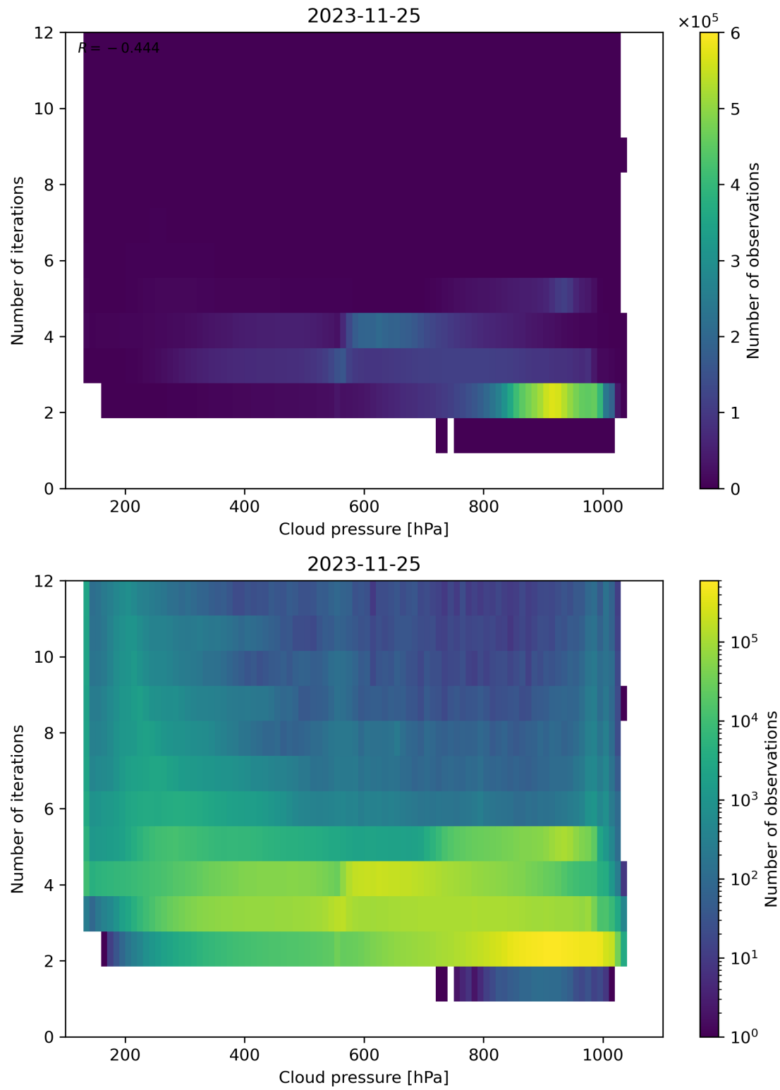
Figure 89: Scatter density plot of “Cloud pressure” against “Number of iterations” for 2023-11-24 to 2023-11-26.
