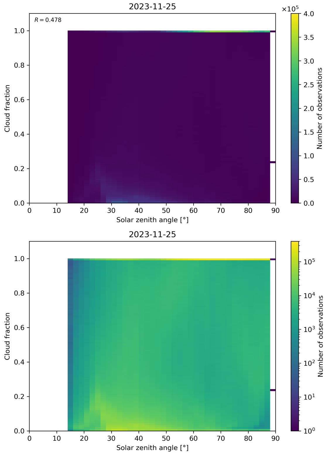
Figure 121: Scatter density plot of “Solar zenith angle” against “Cloud fraction” for 2023-11-24 to 2023-11-26.
