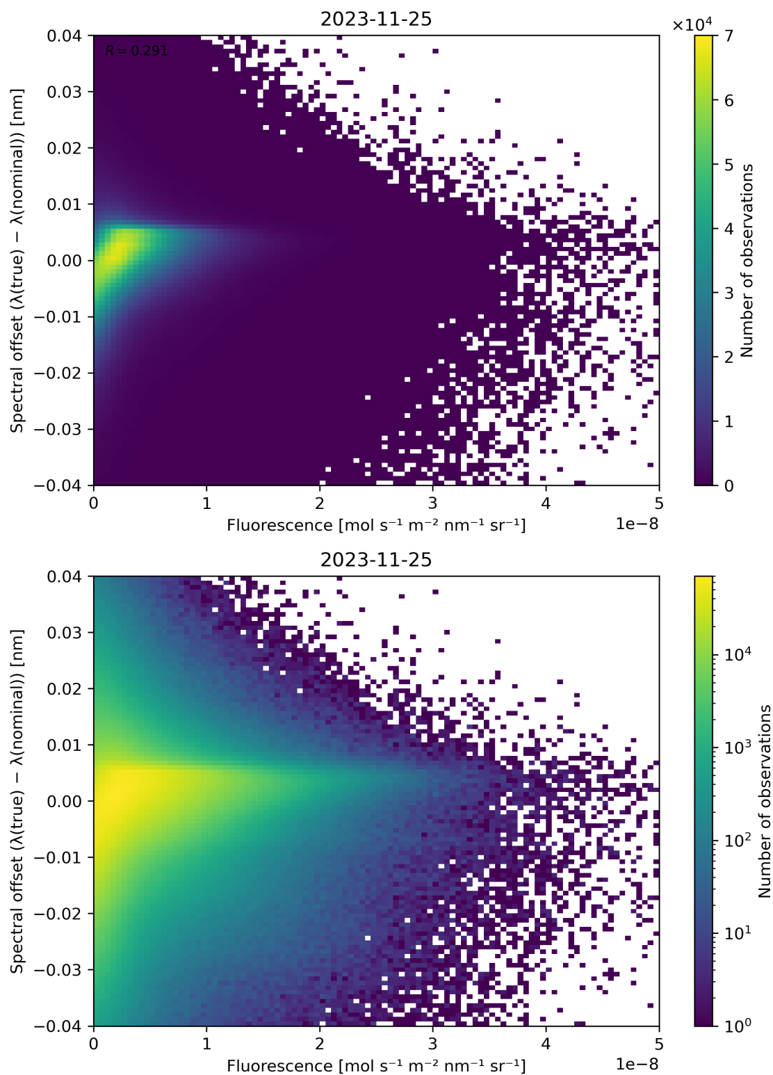
Figure 95: Scatter density plot of “Fluorescence” against “Spectral offset ( \lambda(\text{true}) - \lambda(\text{nominal}) )” for 2023-11-24 to 2023-11-26.
