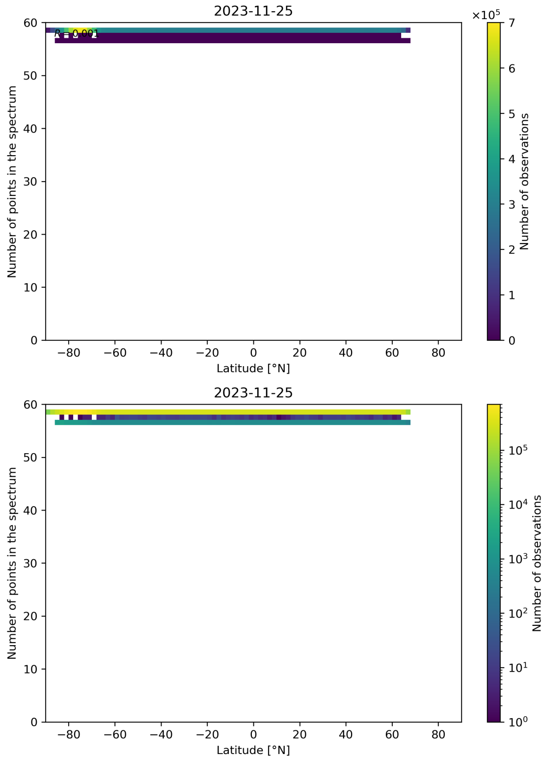
Figure 103: Scatter density plot of “Latitude” against “Number of points in the spectrum” for 2023-11-24 to 2023-11-26.
