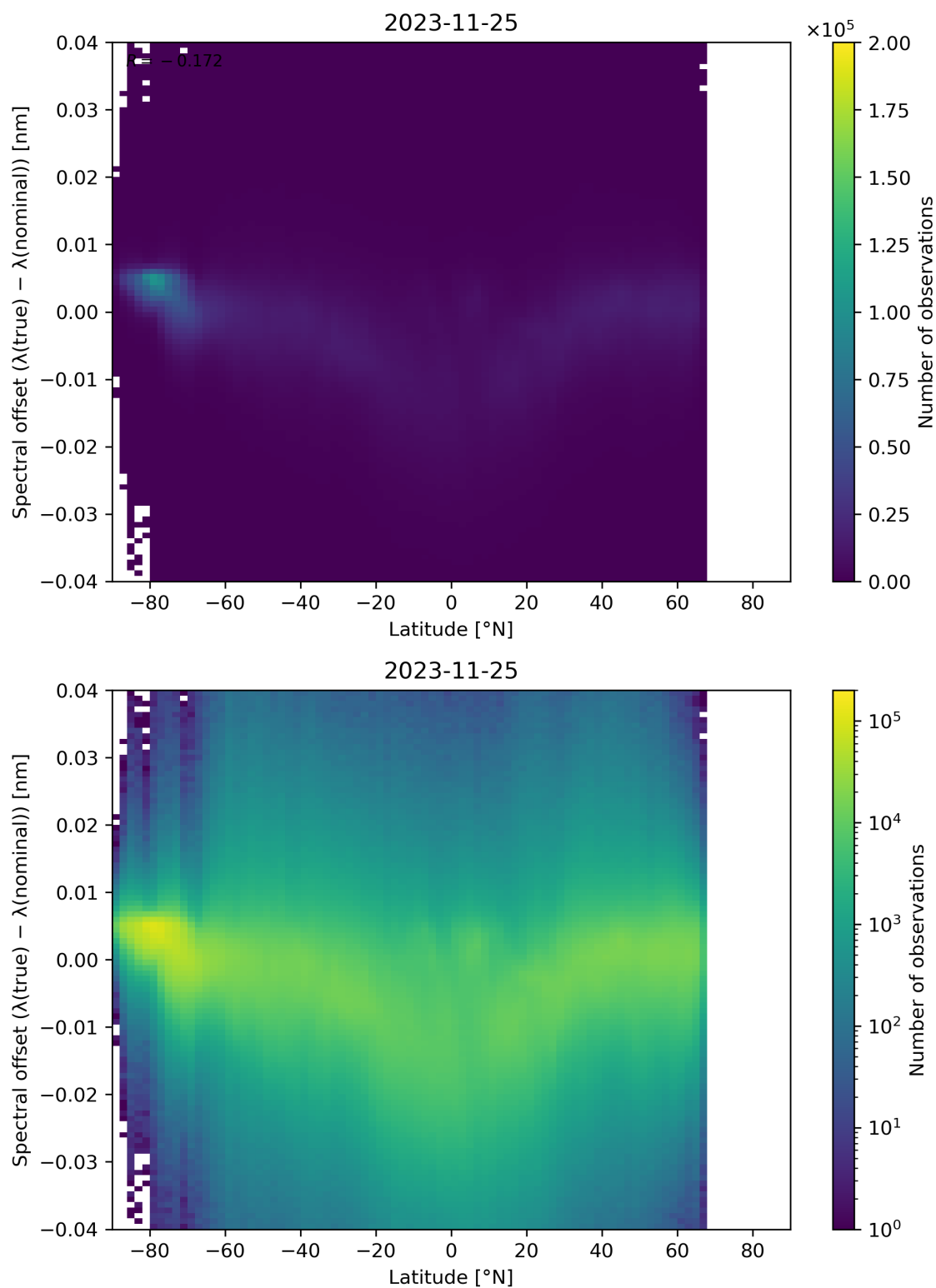
Figure 105: Scatter density plot of “Latitude” against “Spectral offset ( \lambda(\text{true}) - \lambda(\text{nominal}) )” for 2023-11-24 to 2023-11-26.
