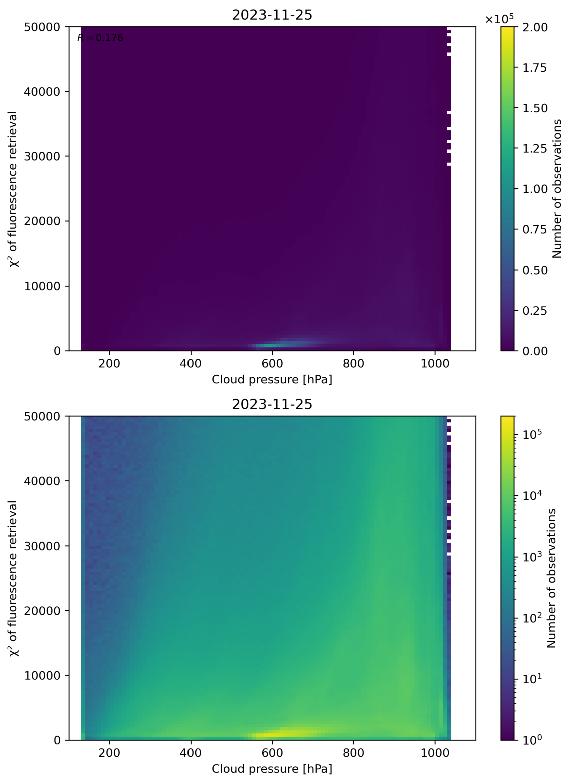
Figure 86: Scatter density plot of “Cloud pressure” against “ \chi^2 of fluorescence retrieval” for 2023-11-24 to 2023-11-26.
