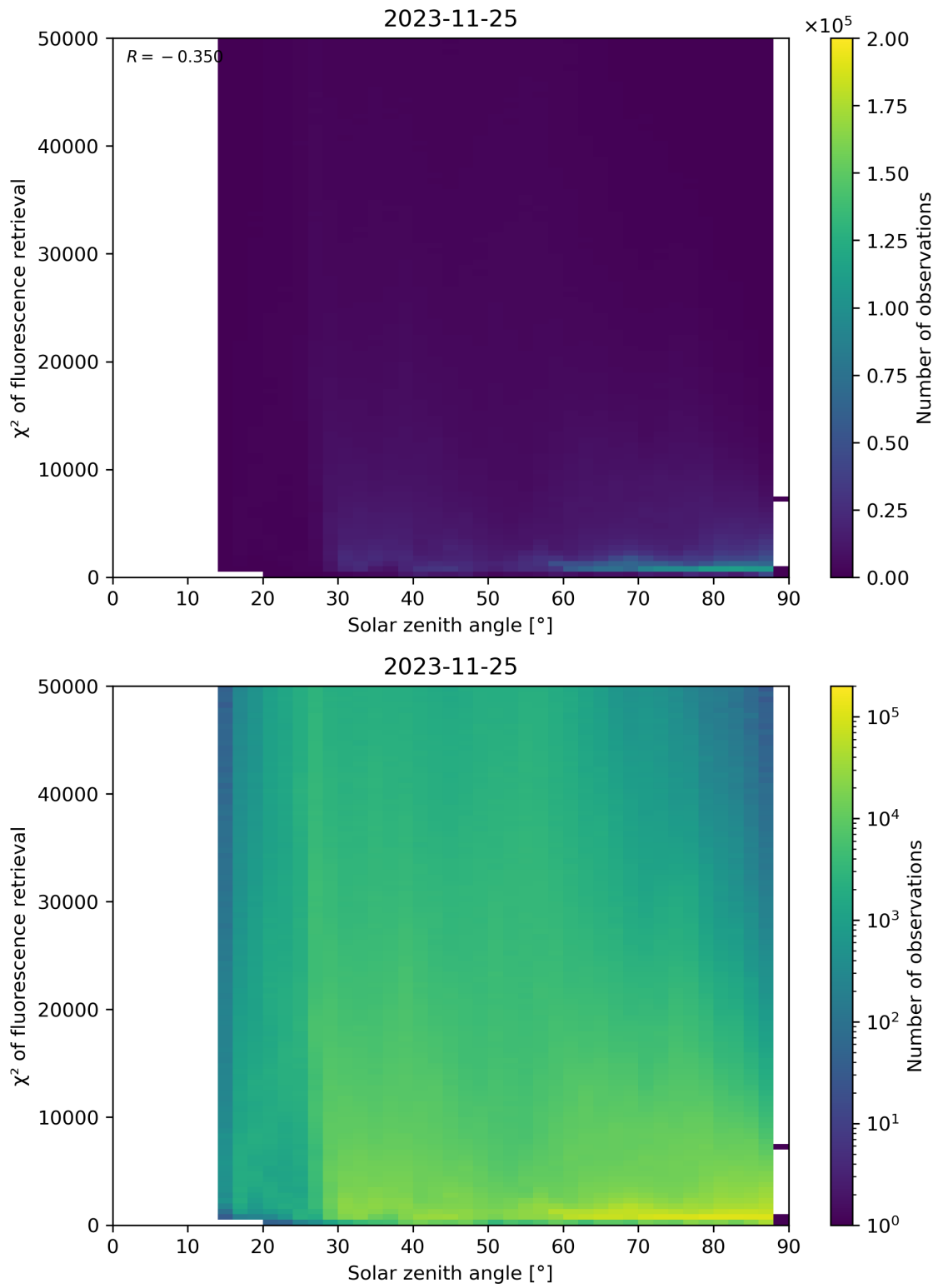
Figure 120: Scatter density plot of “Solar zenith angle” against “ \chi^2 of fluorescence retrieval” for 2023-11-24 to 2023-11-26.
