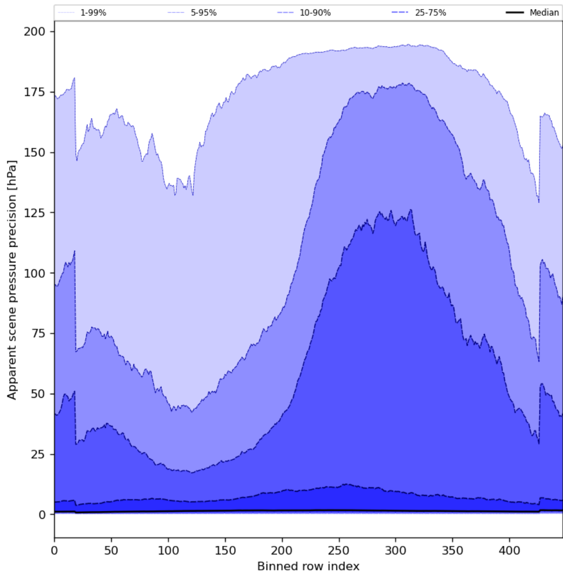
Figure 54: Along track statistics of “Apparent scene pressure precision” for 2023-11-24 to 2023-11-26
