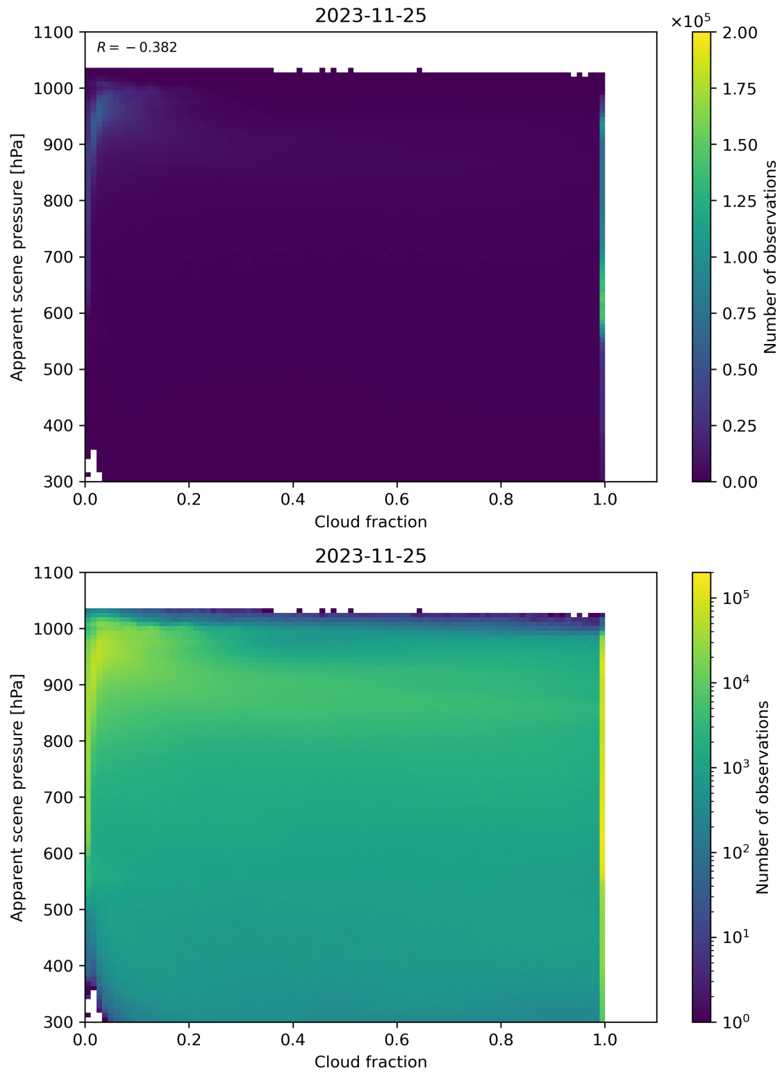
Figure 76: Scatter density plot of “Cloud fraction” against “Apparent scene pressure” for 2023-11-24 to 2023-11-26.
