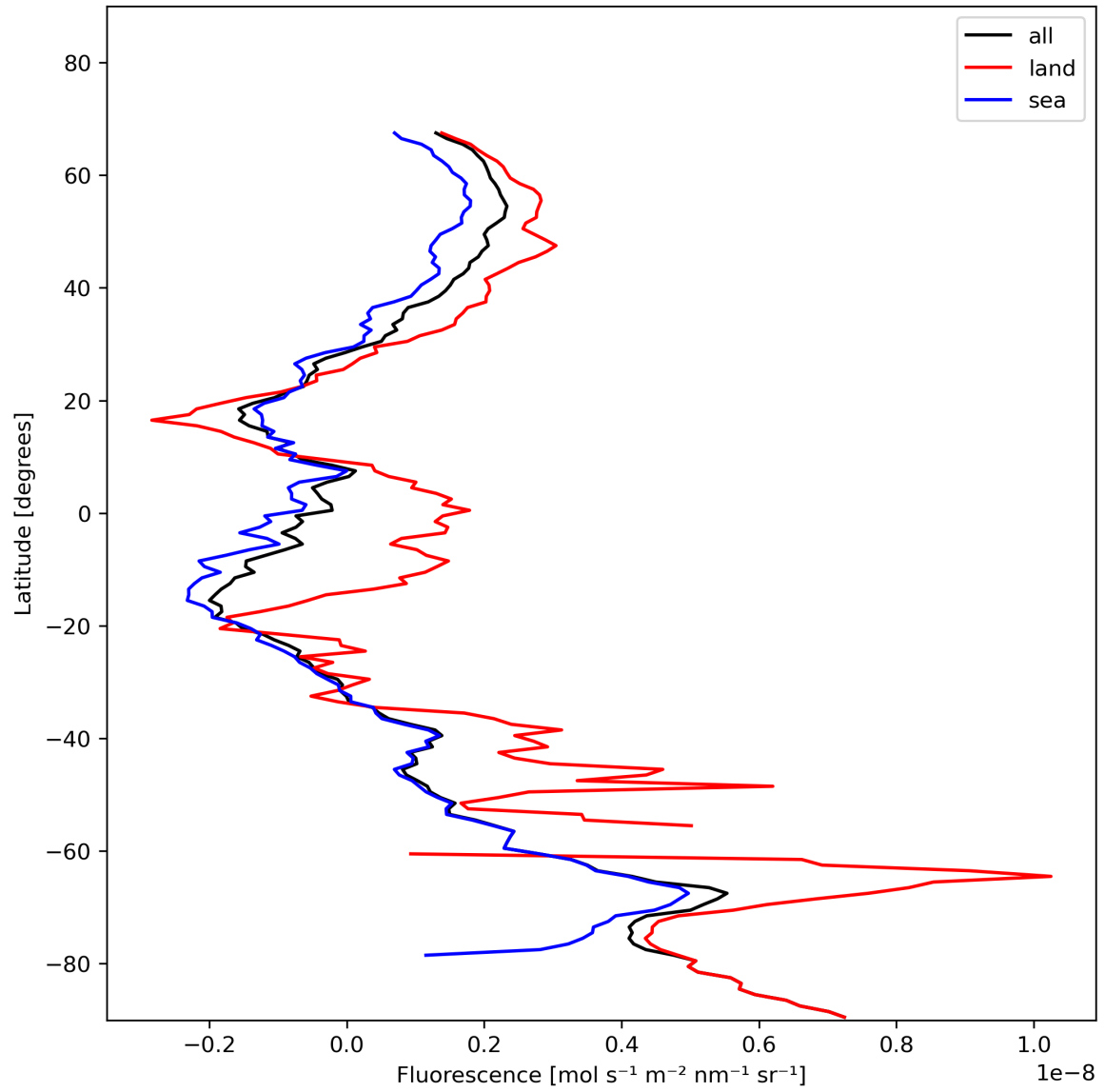
Figure 23: Zonal average of “Fluorescence” for 2023-11-24 to 2023-11-26.
