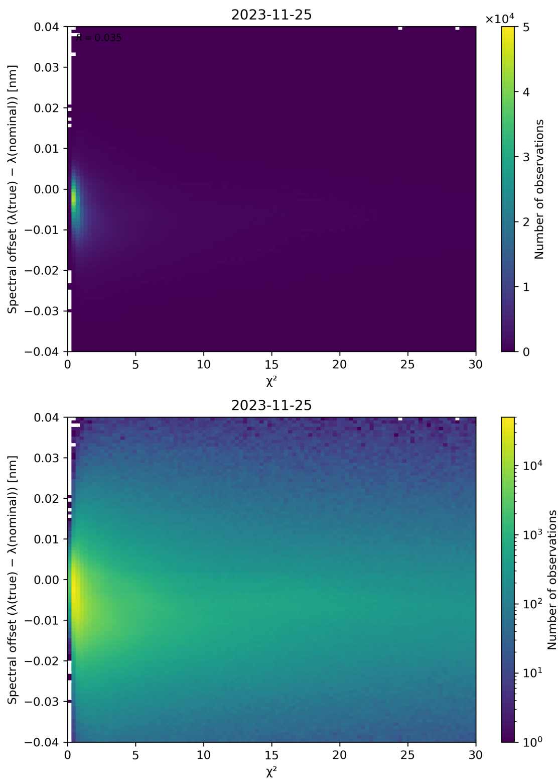
Figure 75: Scatter density plot of “ \chi^2 ” against “Spectral offset ( \lambda(\text{true}) - \lambda(\text{nominal}) )” for 2023-11-24 to 2023-11-26.
