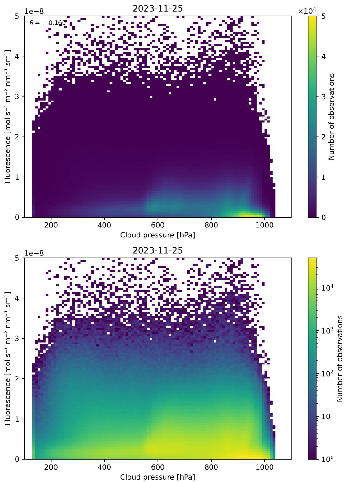
Figure 88: Scatter density plot of “Cloud pressure” against “Fluorescence” for 2023-11-24 to 2023-11-26.
