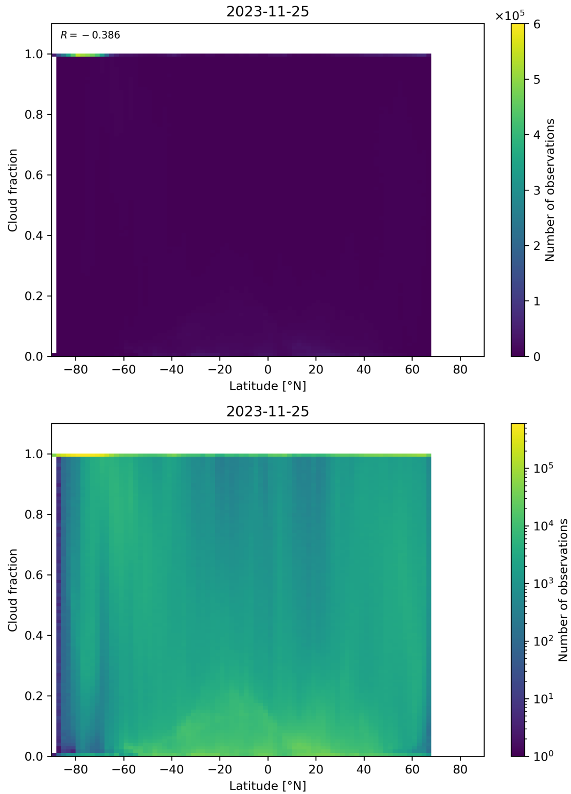
Figure 99: Scatter density plot of “Latitude” against “Cloud fraction” for 2023-11-24 to 2023-11-26.
