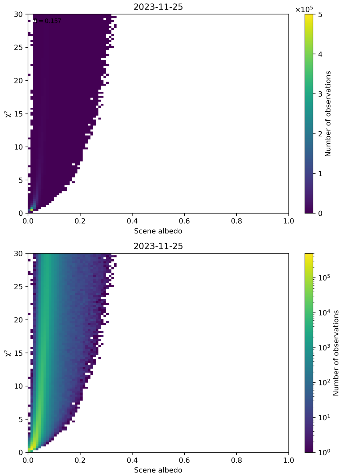
Figure 112: Scatter density plot of “Scene albedo” against “ \chi^2 ” for 2023-11-24 to 2023-11-26.
