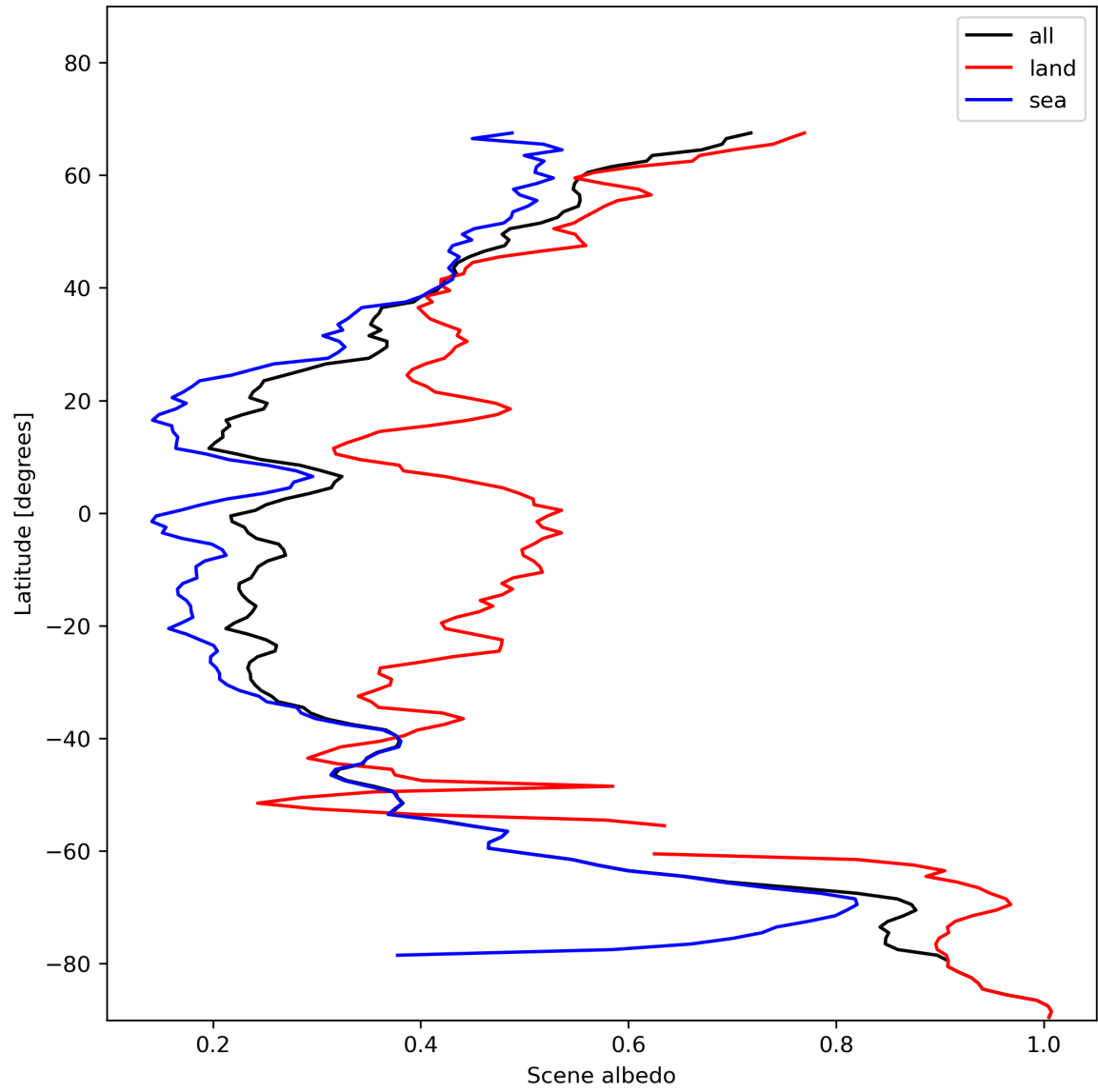
Figure 17: Zonal average of “Scene albedo” for 2023-11-24 to 2023-11-26.
