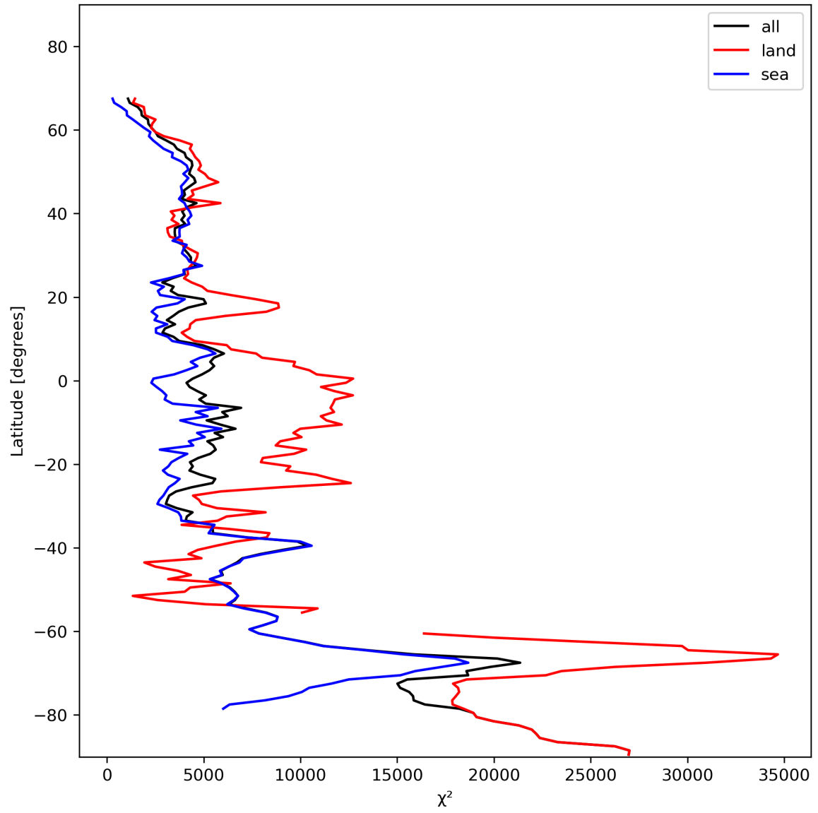
Figure 21: Zonal average of “ \chi^2 ” for 2023-11-24 to 2023-11-26.
