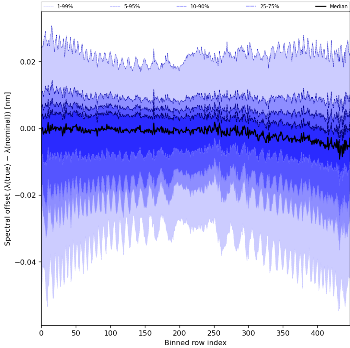
Figure 62: Along track statistics of “Spectral offset ( \lambda(\text{true}) - \lambda(\text{nominal}) )” for 2023-11-24 to 2023-11-26
