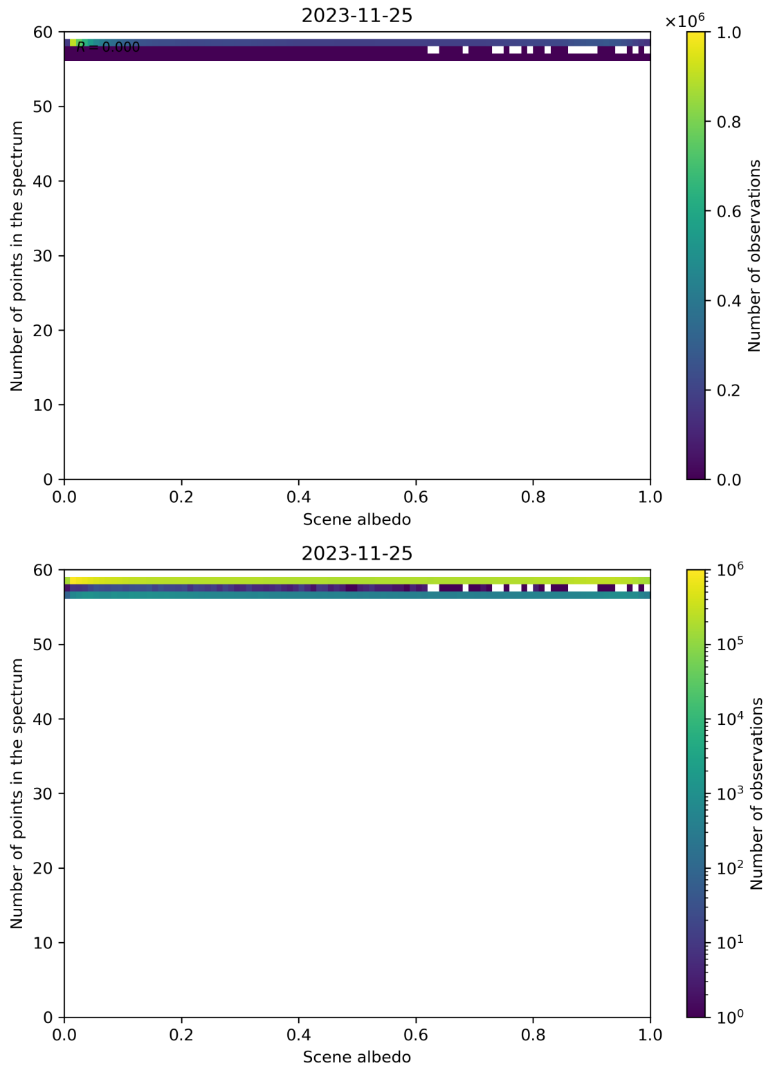
Figure 116: Scatter density plot of “Scene albedo” against “Number of points in the spectrum” for 2023-11-24 to 2023-11-26.
