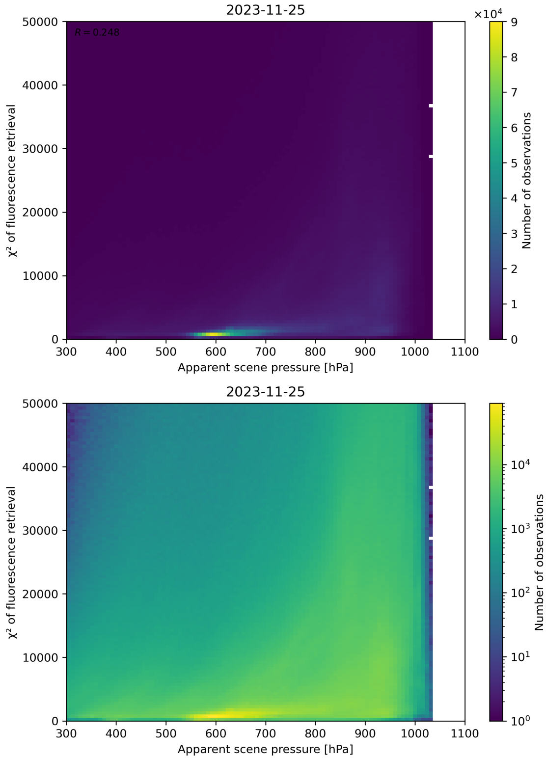
Figure 64: Scatter density plot of “Apparent scene pressure” against “ \chi^2 of fluorescence retrieval” for 2023-11-24 to 2023-11-26.
