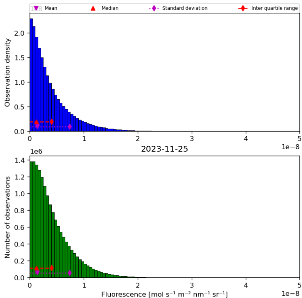
Figure 40: Histogram of “Fluorescence” for 2023-11-24 to 2023-11-26
