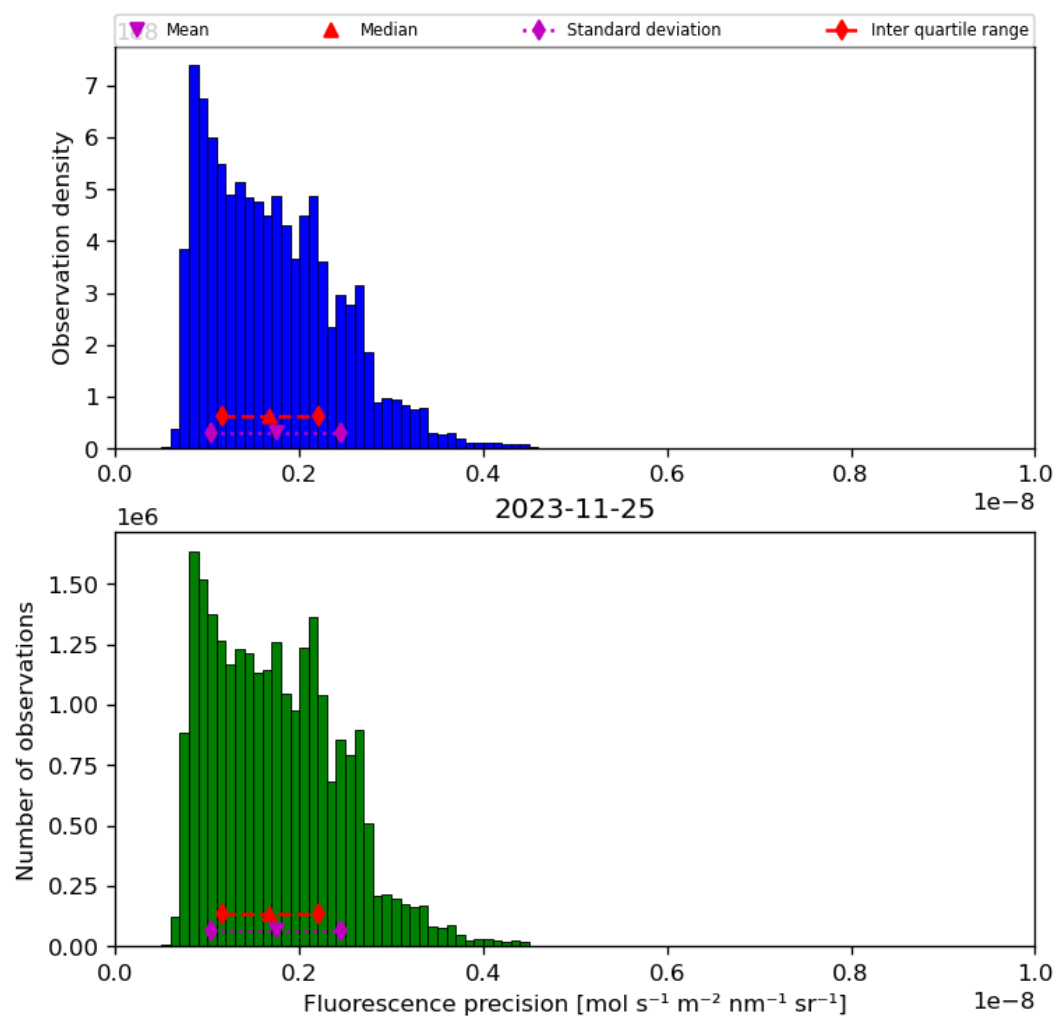
Figure 41: Histogram of “Fluorescence precision” for 2023-11-24 to 2023-11-26
