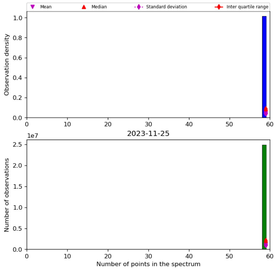
Figure 44: Histogram of “Number of points in the spectrum” for 2023-11-24 to 2023-11-26
