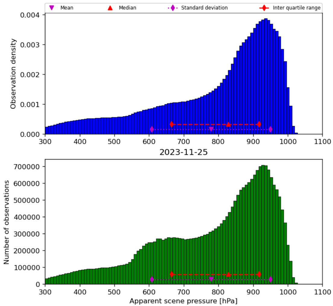
Figure 36: Histogram of “Apparent scene pressure” for 2023-11-24 to 2023-11-26
