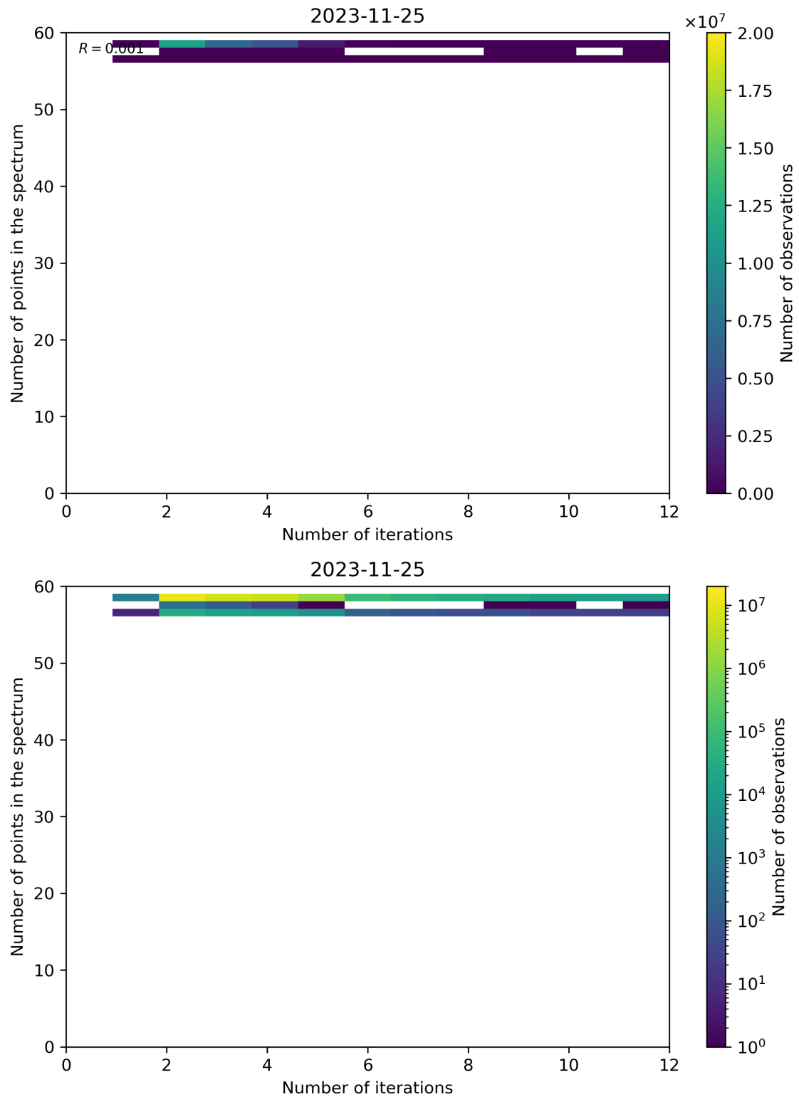
Figure 108: Scatter density plot of “Number of iterations” against “Number of points in the spectrum” for 2023-11-24 to 2023-11-26.
