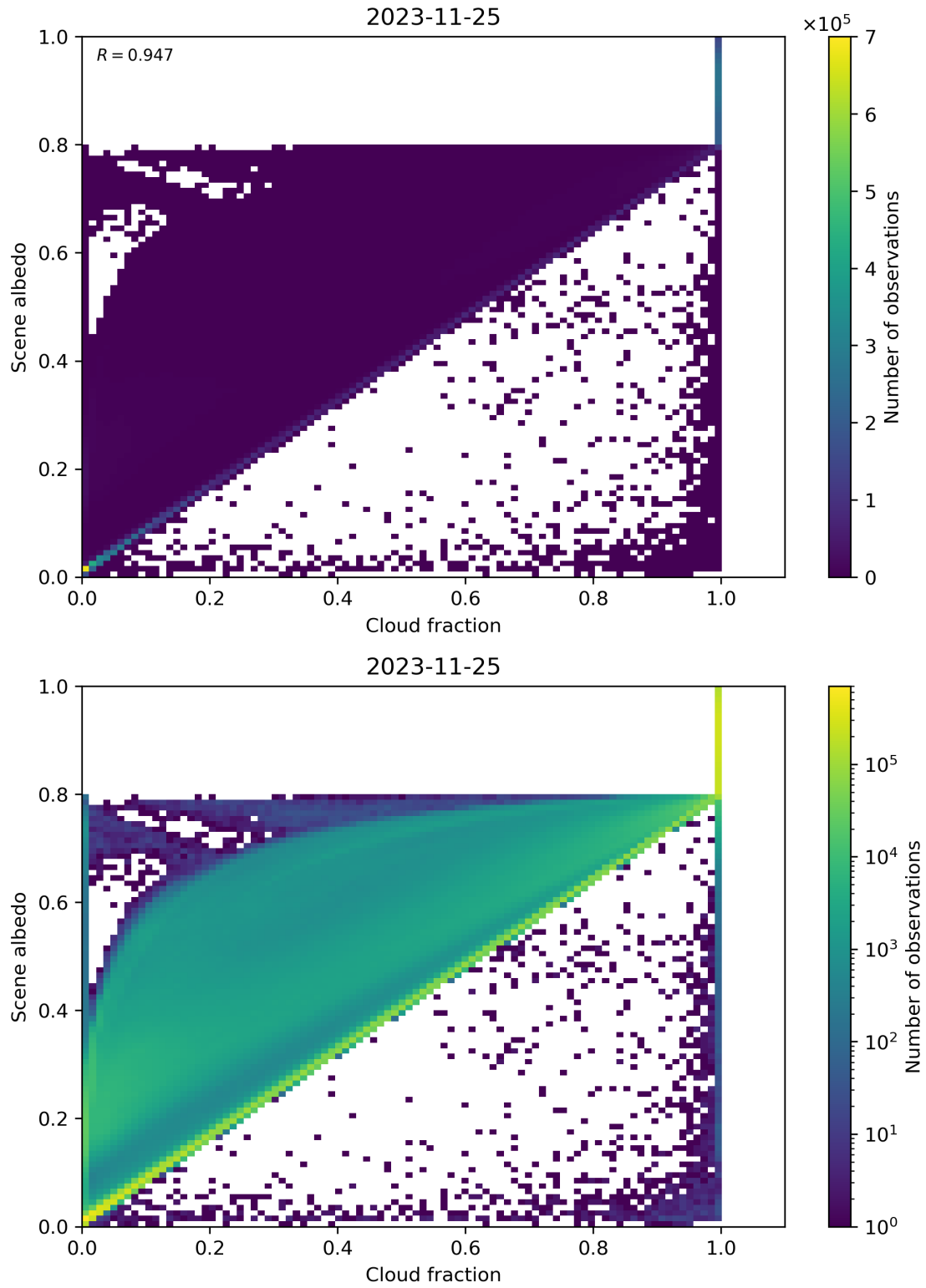
Figure 82: Scatter density plot of “Cloud fraction” against “Scene albedo” for 2023-11-24 to 2023-11-26.
