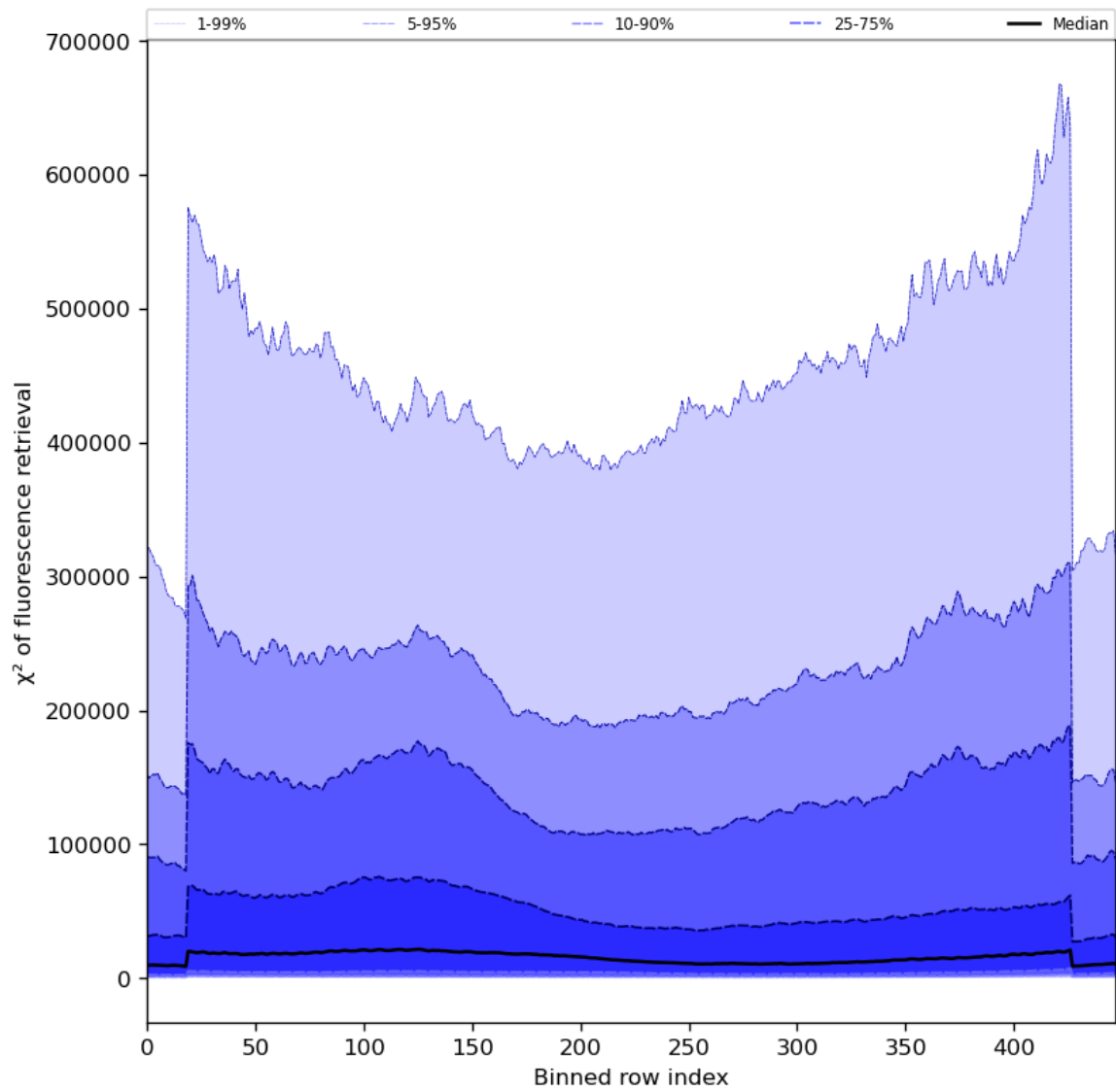
Figure 59: Along track statistics of “ \chi^2 of fluorescence retrieval” for 2023-11-24 to 2023-11-26
