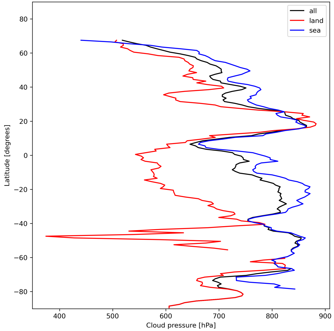
Figure 13: Zonal average of “Cloud pressure” for 2023-11-24 to 2023-11-26.
