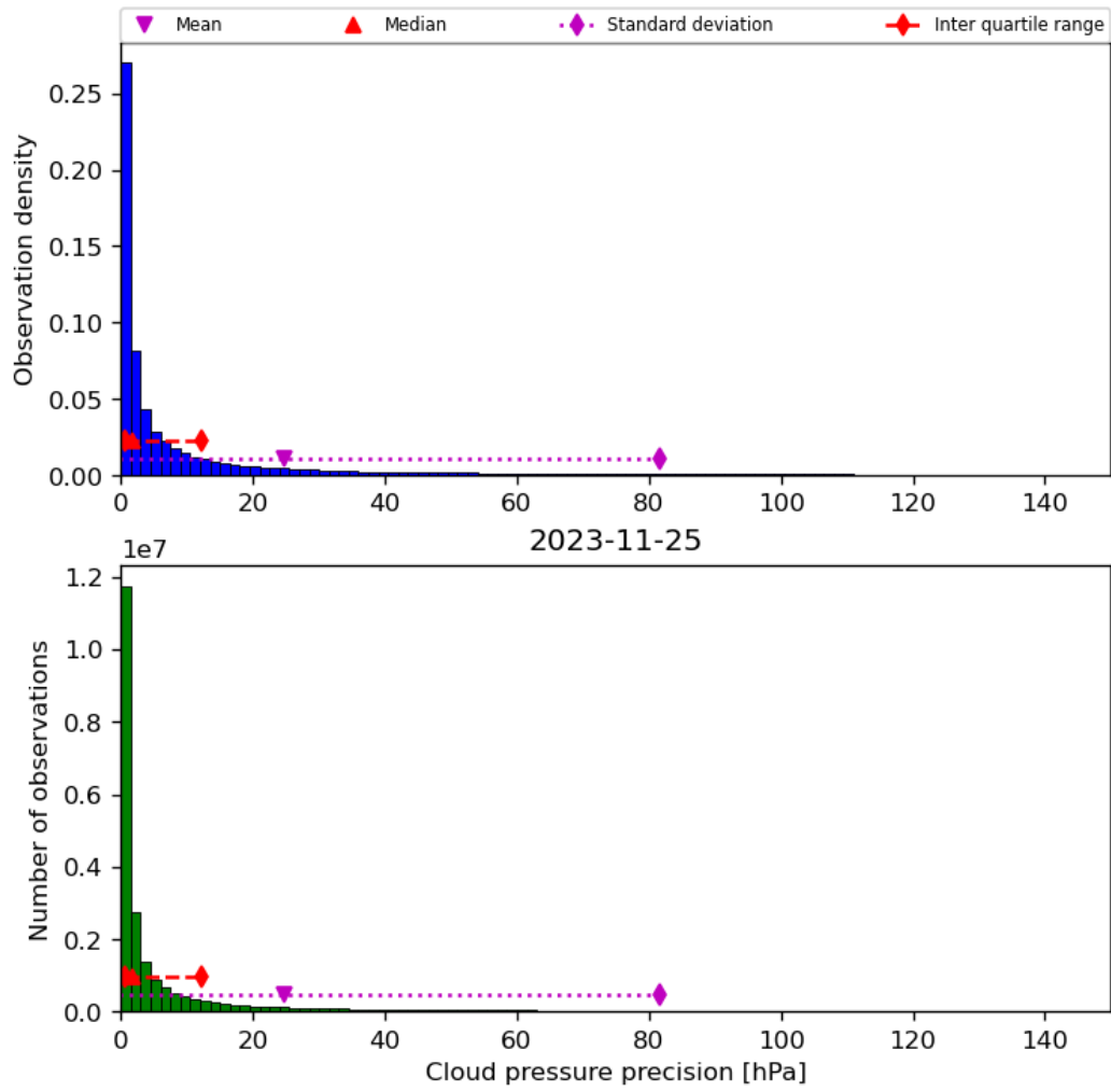
Figure 31: Histogram of “Cloud pressure precision” for 2023-11-24 to 2023-11-26
