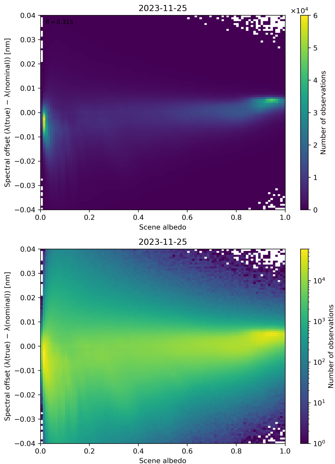
Figure 117: Scatter density plot of “Scene albedo” against “Spectral offset ( \lambda(\text{true}) - \lambda(\text{nominal}) )” for 2023-11-24 to 2023-11-26.
