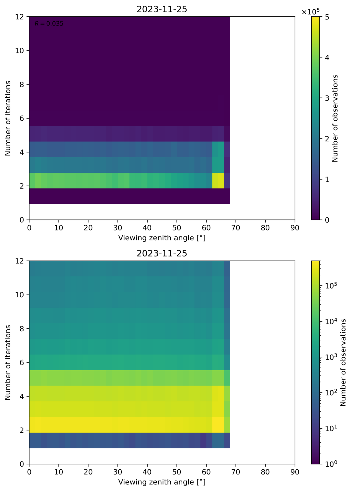
Figure 136: Scatter density plot of “Viewing zenith angle” against “Number of iterations” for 2023-11-24 to 2023-11-26.
