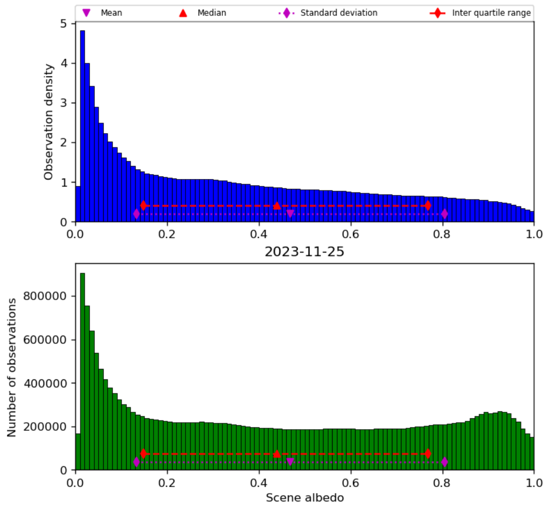
Figure 34: Histogram of “Scene albedo” for 2023-11-24 to 2023-11-26
