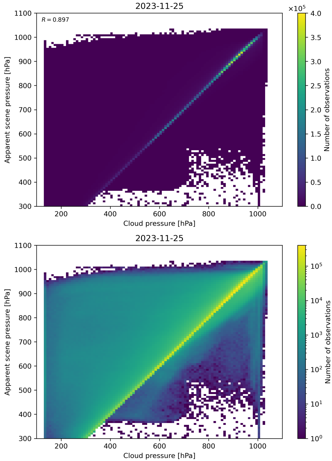
Figure 84: Scatter density plot of “Cloud pressure” against “Apparent scene pressure” for 2023-11-24 to 2023-11-26.
