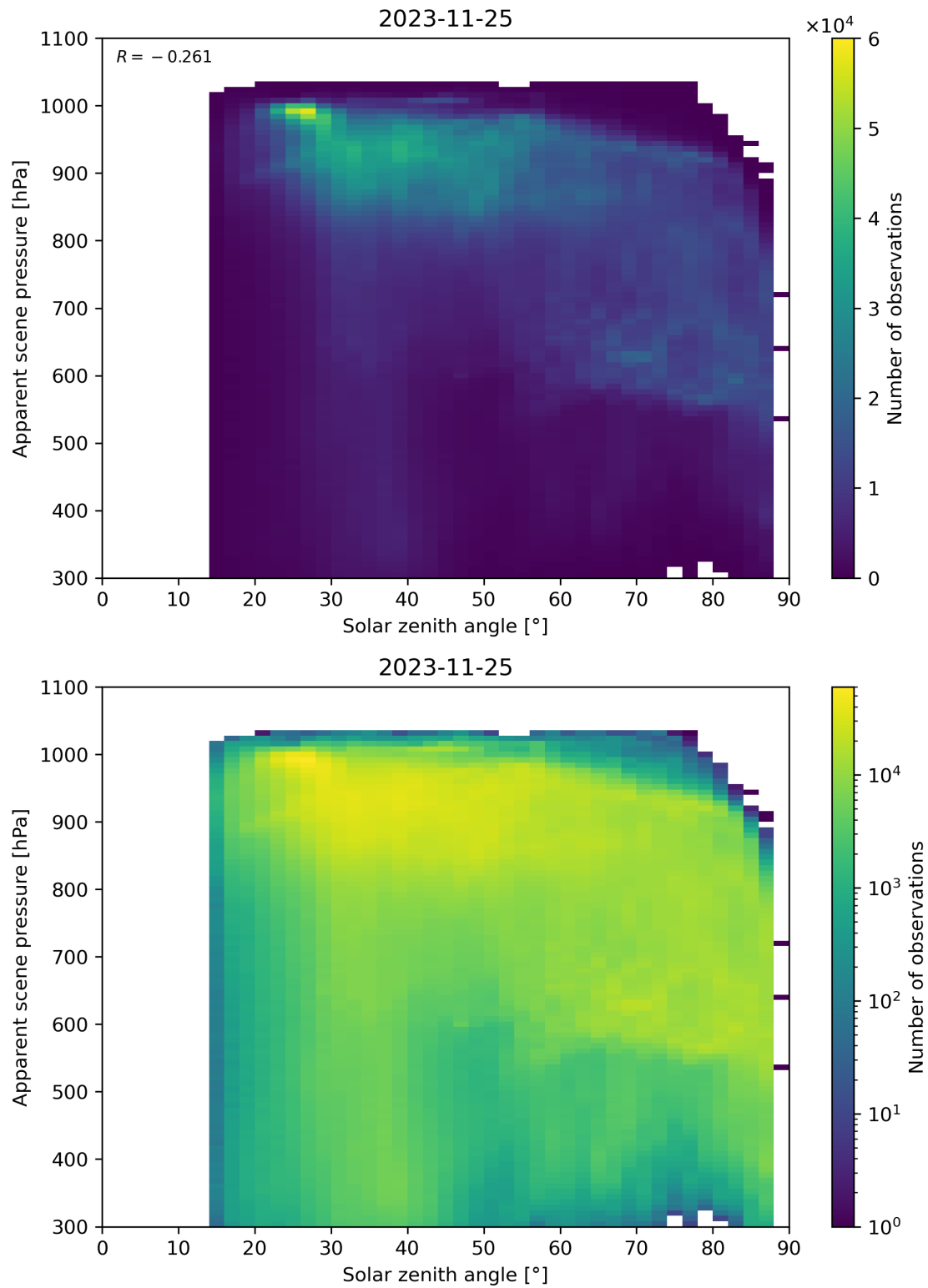
Figure 118: Scatter density plot of “Solar zenith angle” against “Apparent scene pressure” for 2023-11-24 to 2023-11-26.
