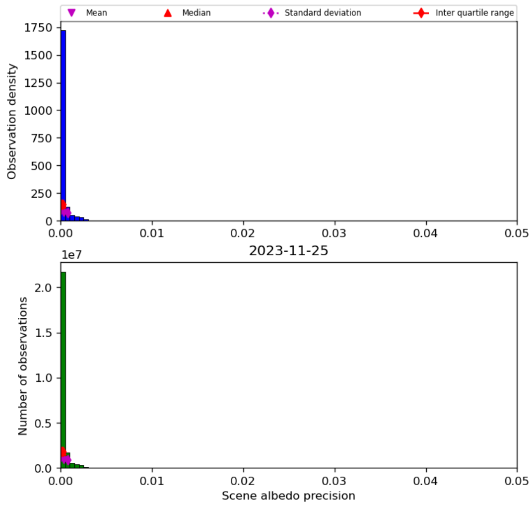
Figure 35: Histogram of “Scene albedo precision” for 2023-11-24 to 2023-11-26
