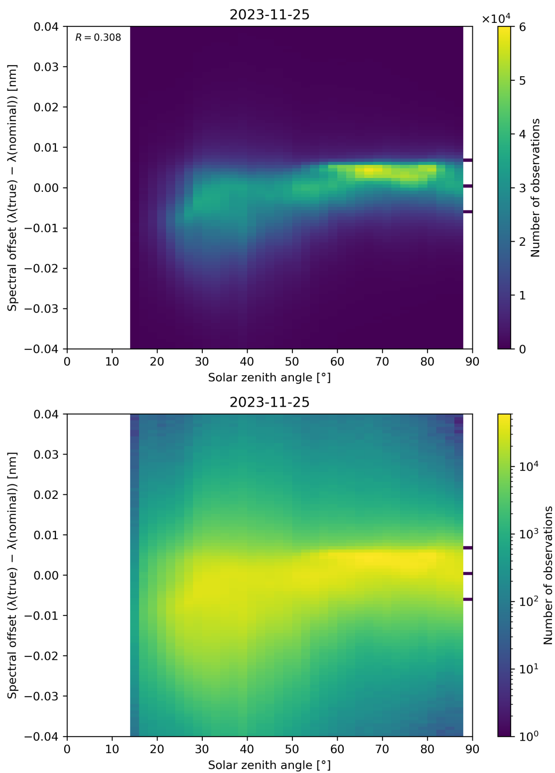
Figure 128: Scatter density plot of “Solar zenith angle” against “Spectral offset ( \lambda(\text{true}) - \lambda(\text{nominal}) )” for 2023-11-24 to 2023-11-26.
