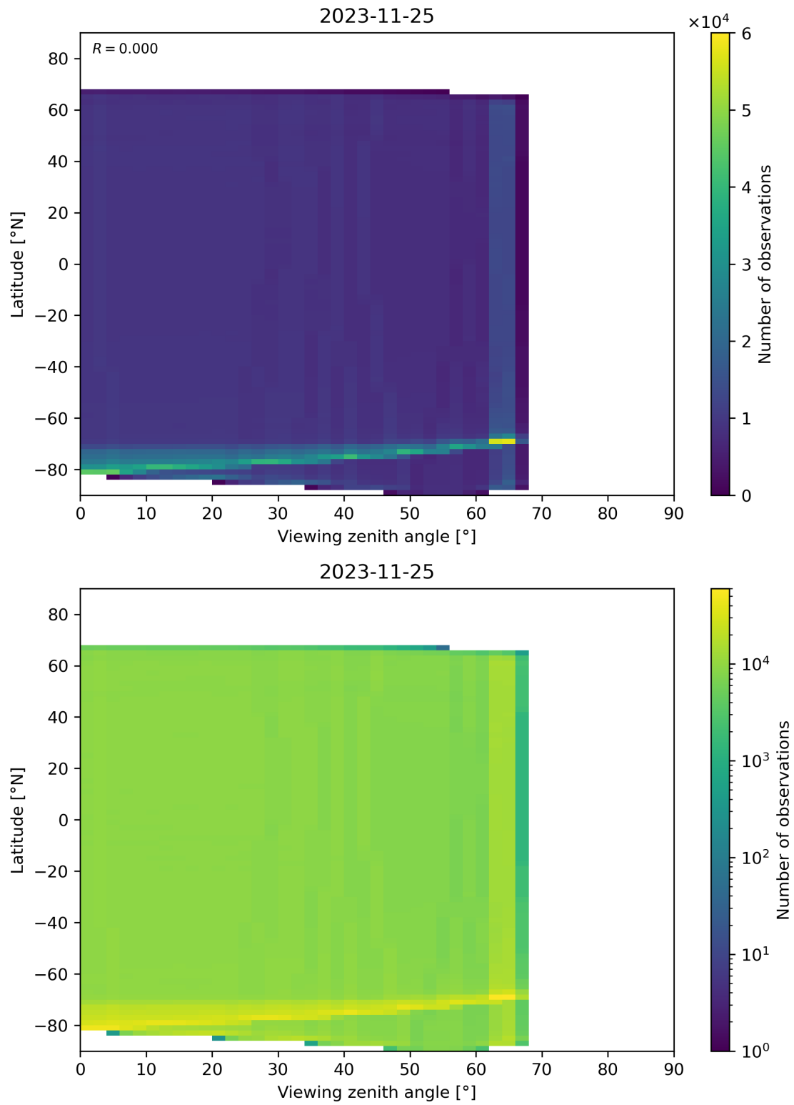
Figure 135: Scatter density plot of “Viewing zenith angle” against “Latitude” for 2023-11-24 to 2023-11-26.
