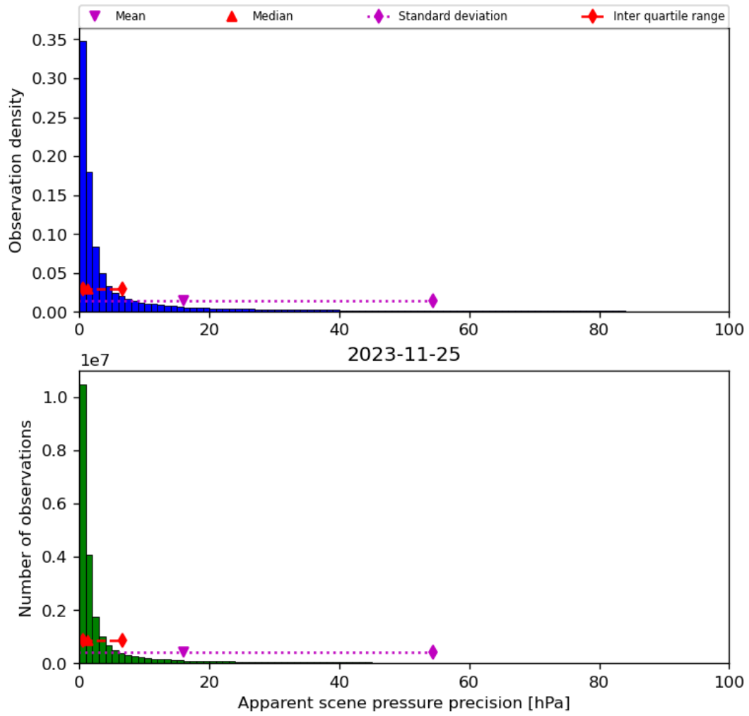
Figure 37: Histogram of “Apparent scene pressure precision” for 2023-11-24 to 2023-11-26
