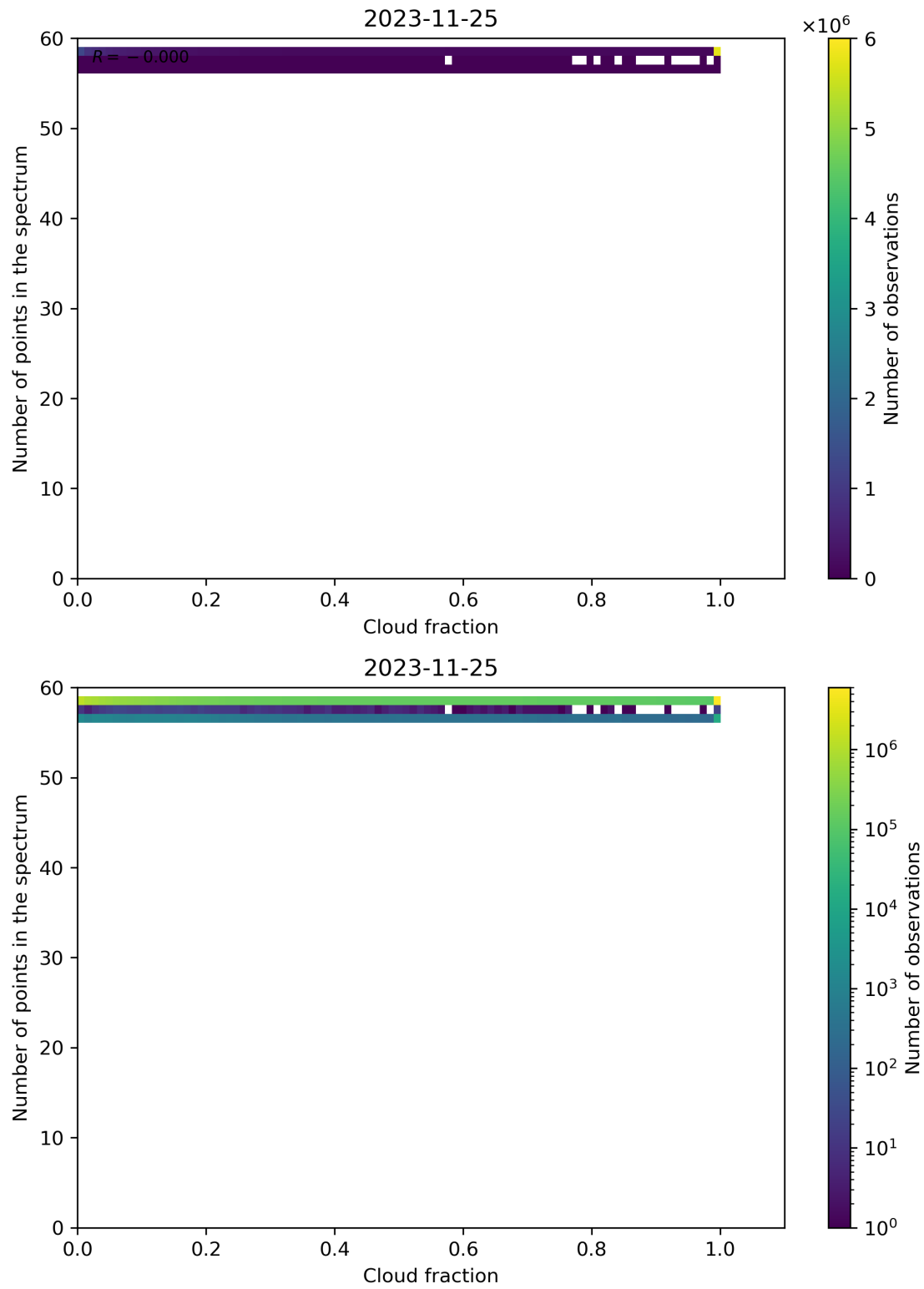
Figure 81: Scatter density plot of “Cloud fraction” against “Number of points in the spectrum” for 2023-11-24 to 2023-11-26.
