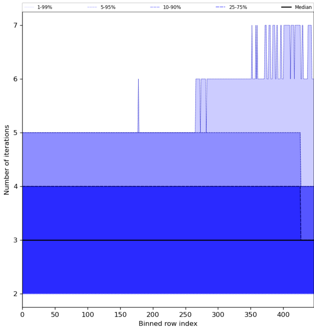
Figure 56: Along track statistics of “Number of iterations” for 2023-11-24 to 2023-11-26
