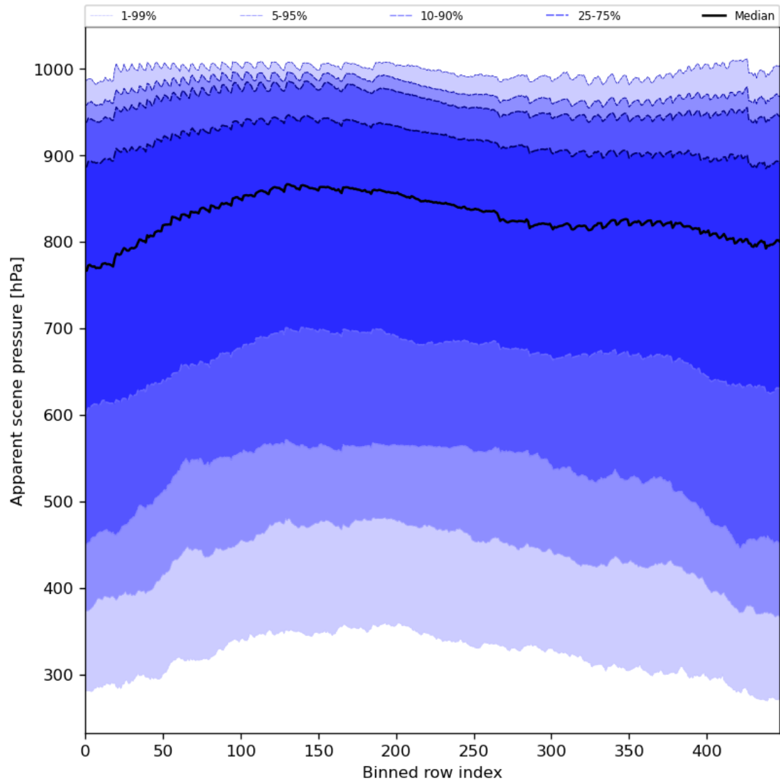
Figure 53: Along track statistics of “Apparent scene pressure” for 2023-11-24 to 2023-11-26
