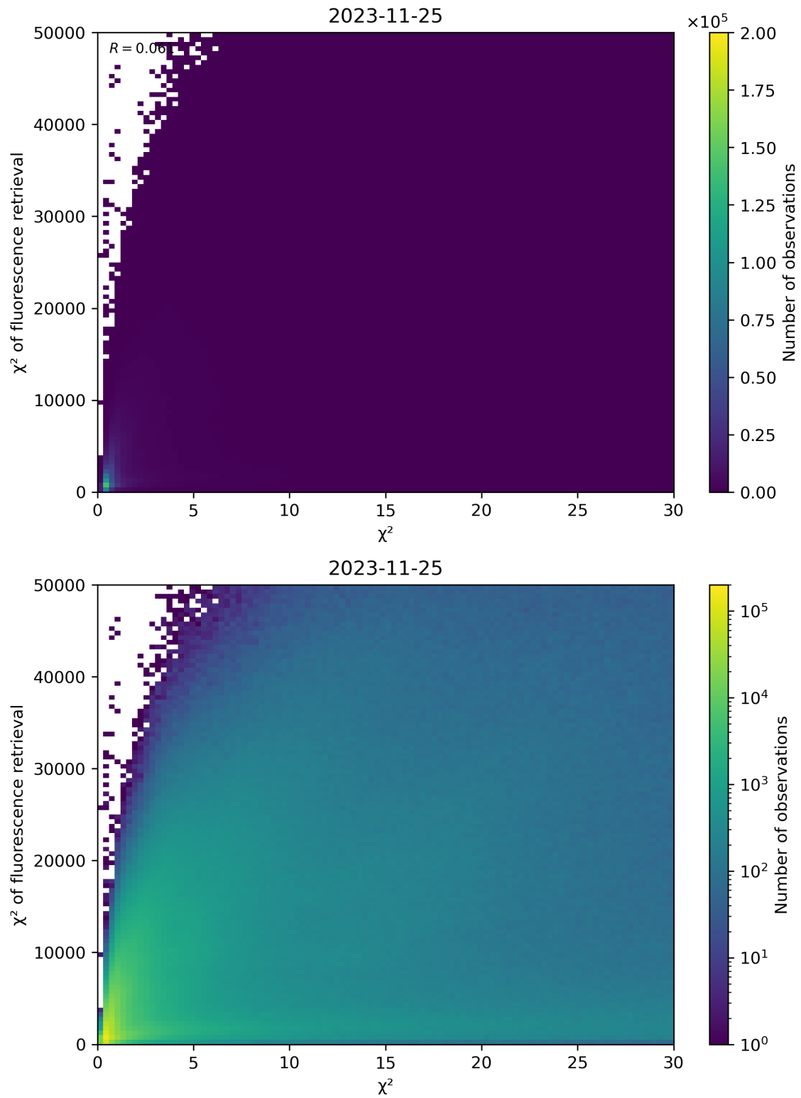
Figure 69: Scatter density plot of “ \chi^2 ” against “ \chi^2 of fluorescence retrieval” for 2023-11-24 to 2023-11-26.
