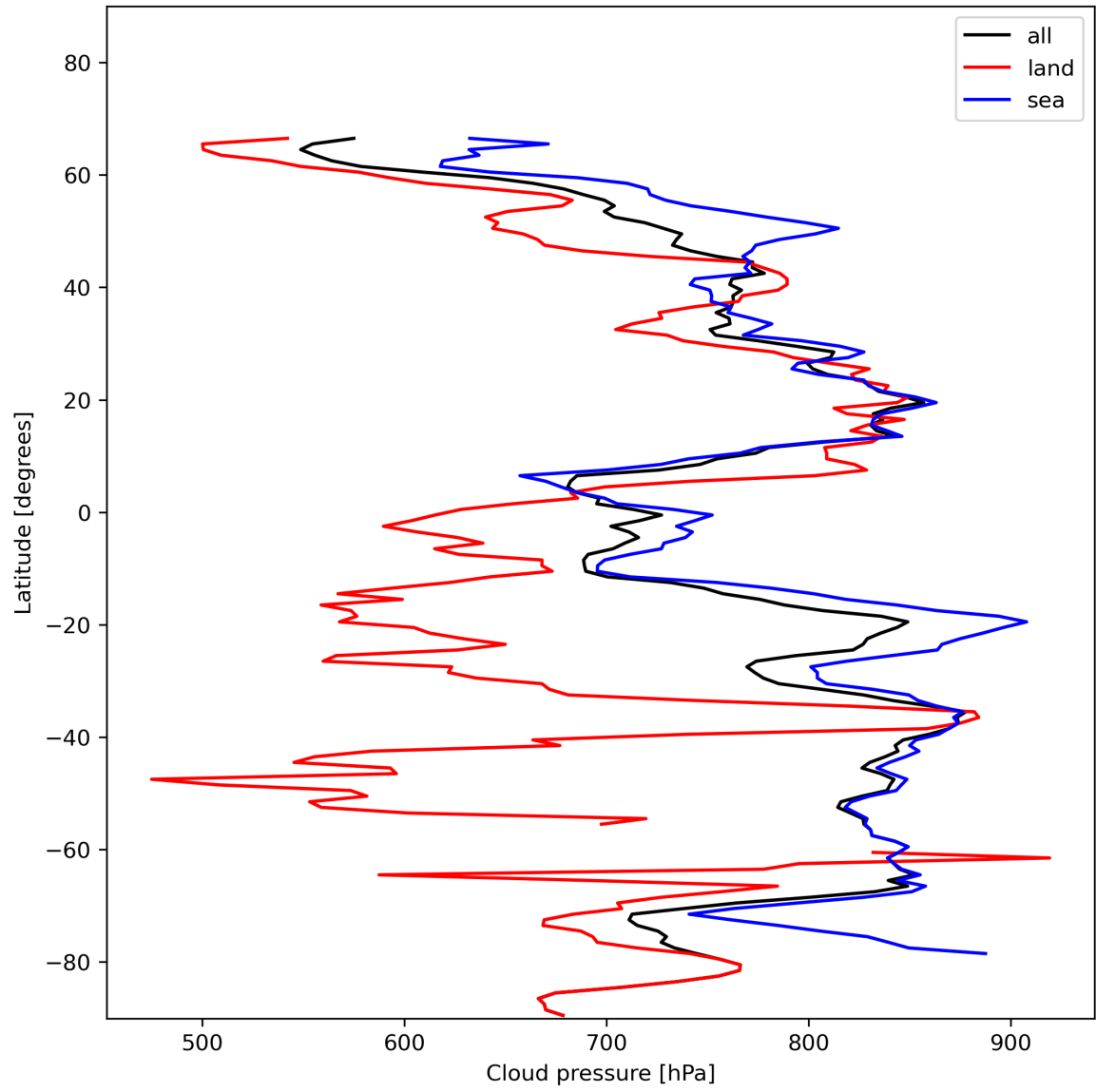
Figure 13: Zonal average of “Cloud pressure” for 2023-11-26 to 2023-11-28.
