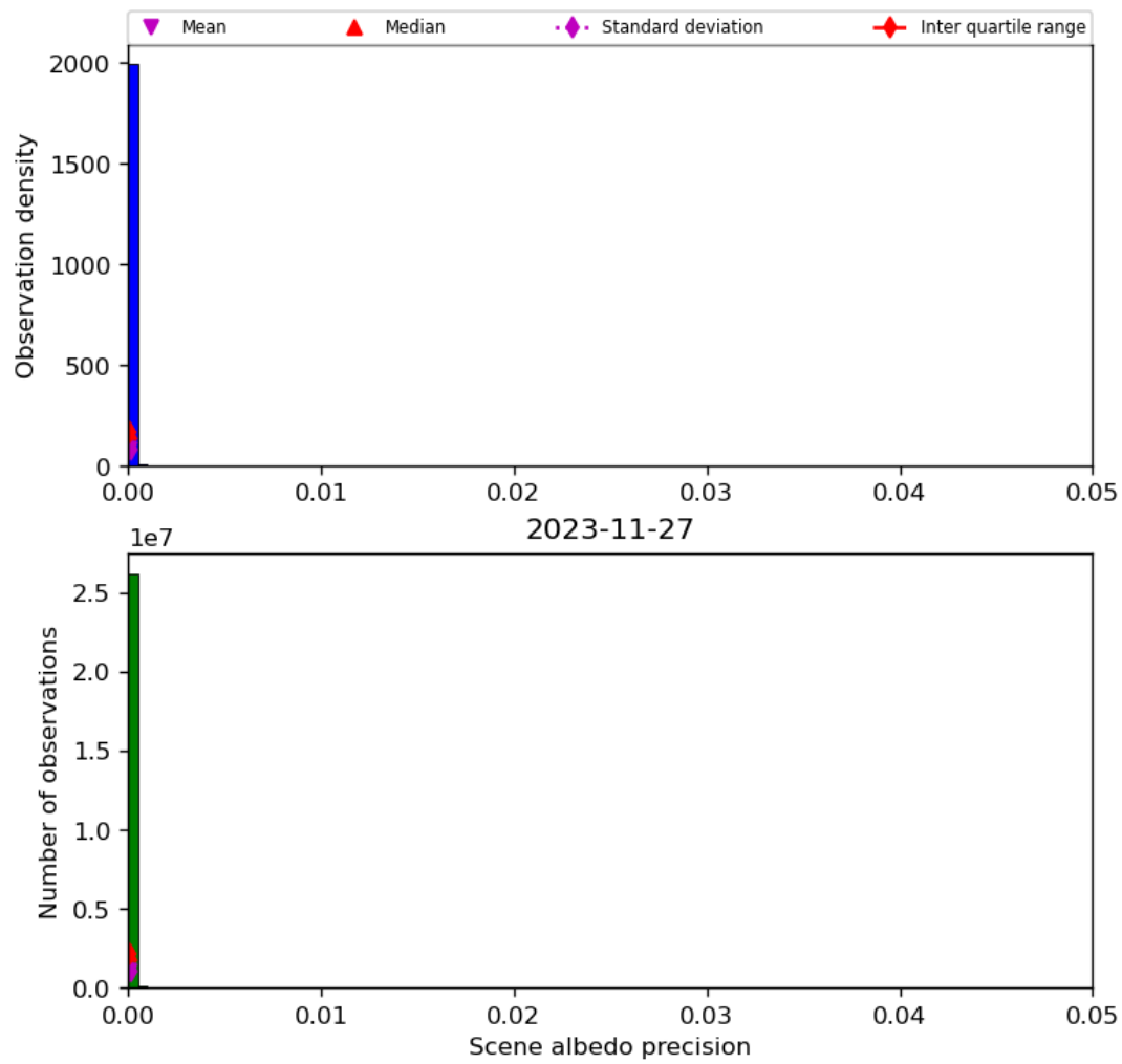
Figure 35: Histogram of “Scene albedo precision” for 2023-11-26 to 2023-11-28
