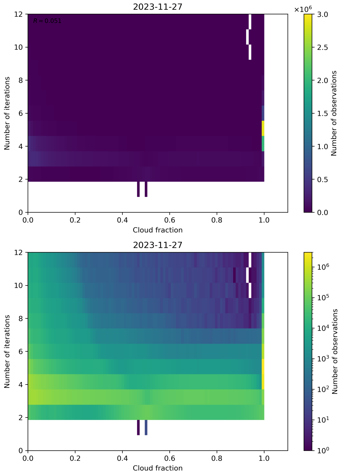
Figure 73: Scatter density plot of “Cloud fraction” against “Number of iterations” for 2023-11-26 to 2023-11-28.
