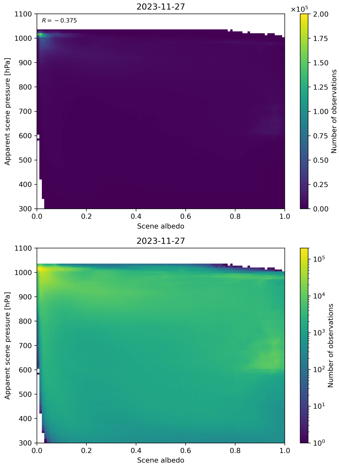
Figure 102: Scatter density plot of “Scene albedo” against “Apparent scene pressure” for 2023-11-26 to 2023-11-28.
