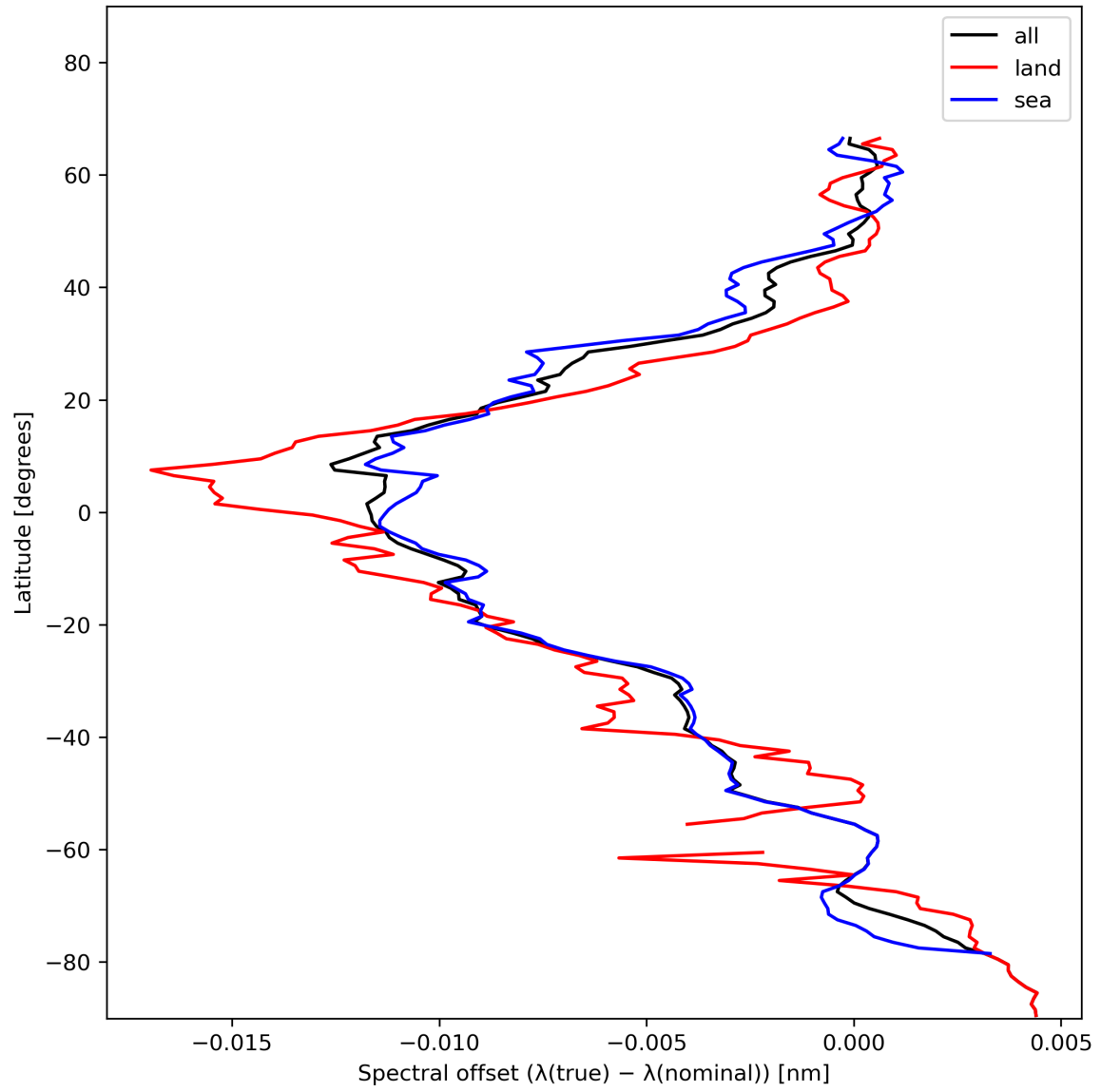
Figure 28: Zonal average of “Spectral offset ( \lambda(\text{true}) - \lambda(\text{nominal}) )” for 2023-11-26 to 2023-11-28.
