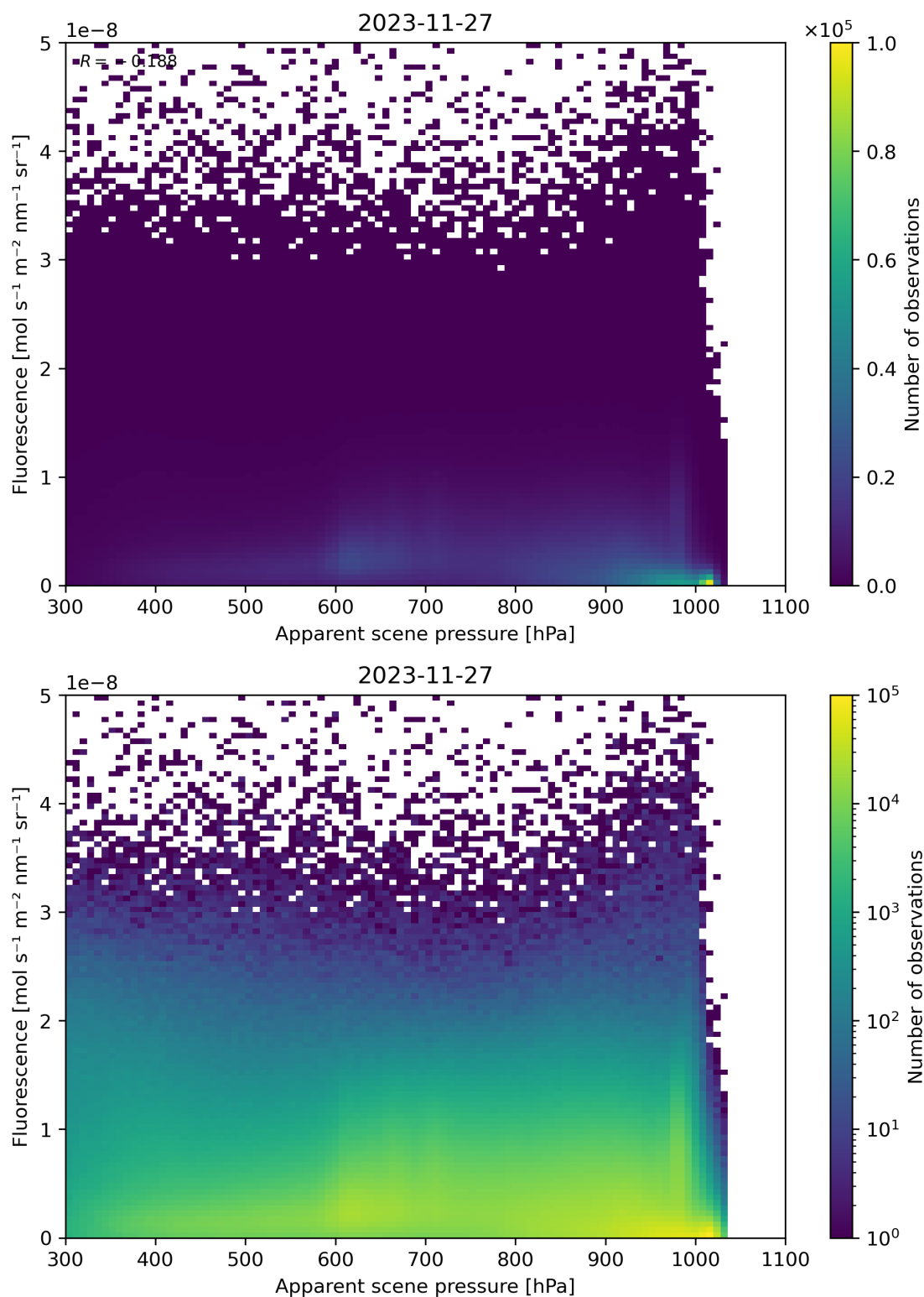
Figure 64: Scatter density plot of “Apparent scene pressure” against “Fluorescence” for 2023-11-26 to 2023-11-28.
