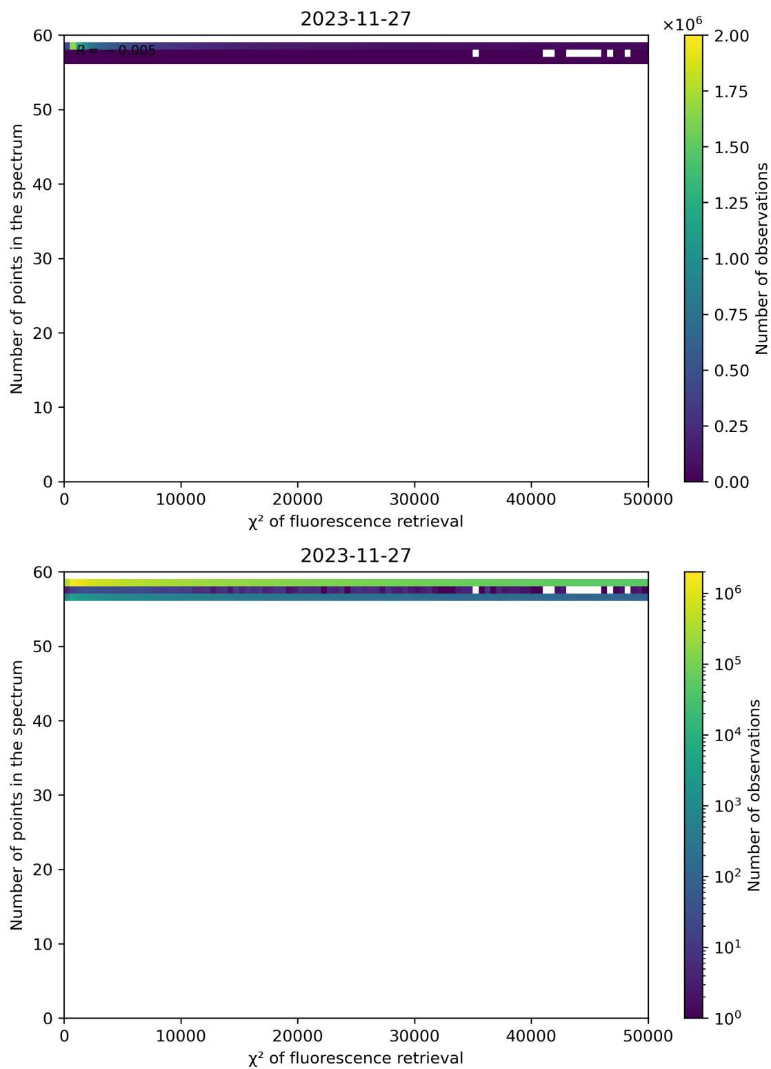
Figure 68: Scatter density plot of “ \chi^2 of fluorescence retrieval” against “Number of points in the spectrum” for 2023-11-26 to 2023-11-28.
