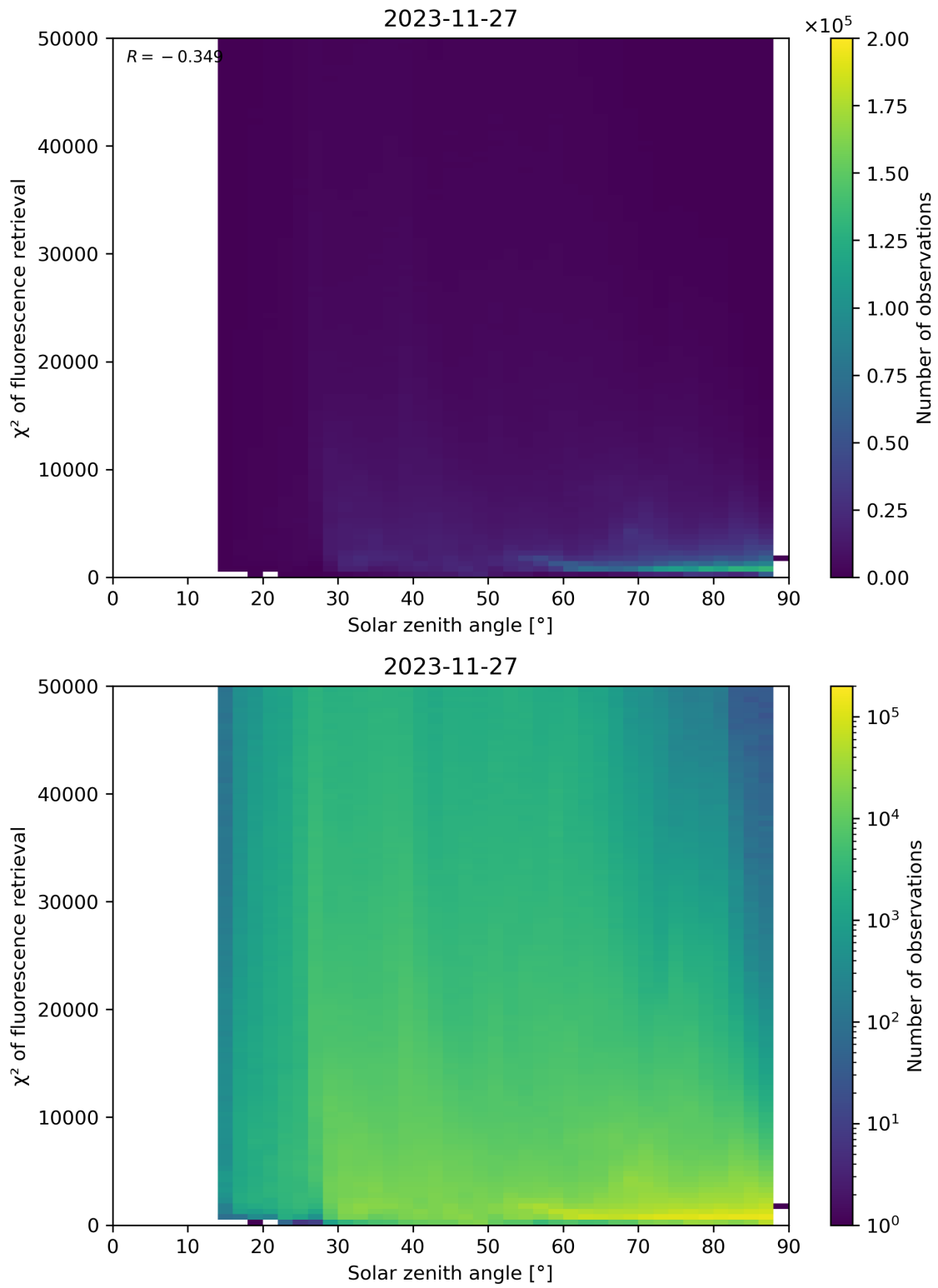
Figure 109: Scatter density plot of “Solar zenith angle” against “ \chi^2 of fluorescence retrieval” for 2023-11-26 to 2023-11-28.
