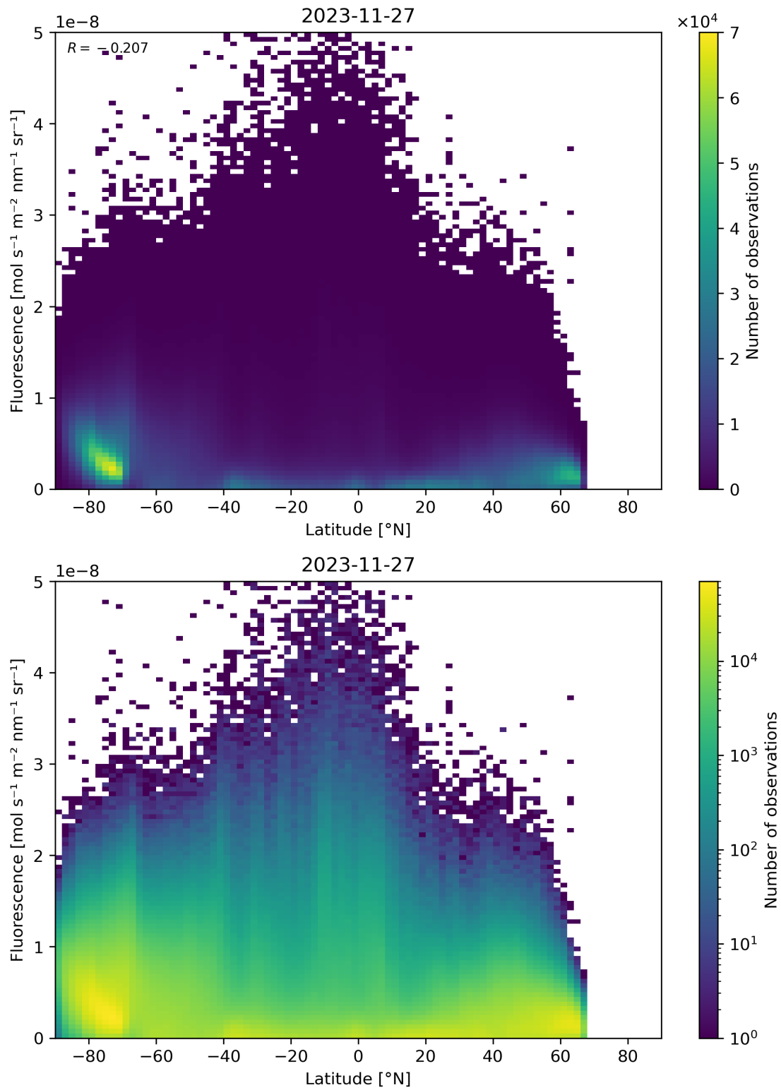
Figure 92: Scatter density plot of “Latitude” against “Fluorescence” for 2023-11-26 to 2023-11-28.
