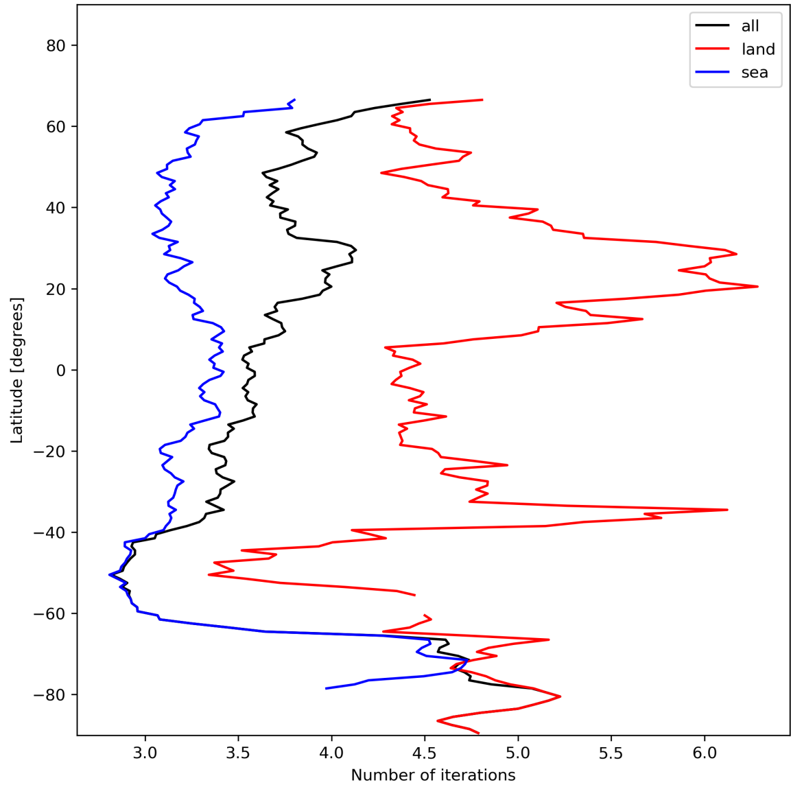
Figure 22: Zonal average of “Number of iterations” for 2023-11-26 to 2023-11-28.
