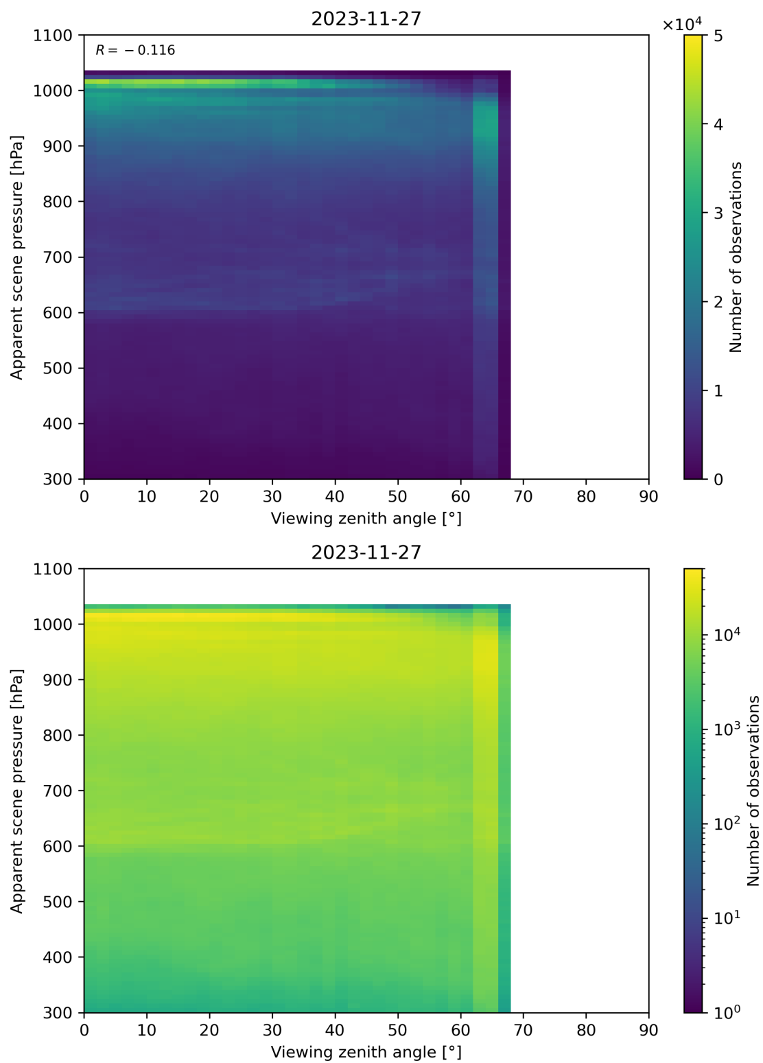
Figure 118: Scatter density plot of “Viewing zenith angle” against “Apparent scene pressure” for 2023-11-26 to 2023-11-28.
