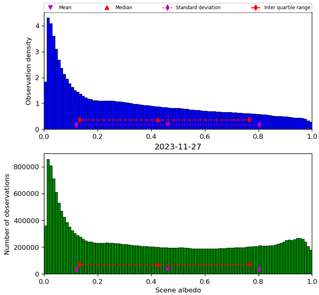
Figure 34: Histogram of “Scene albedo” for 2023-11-26 to 2023-11-28
