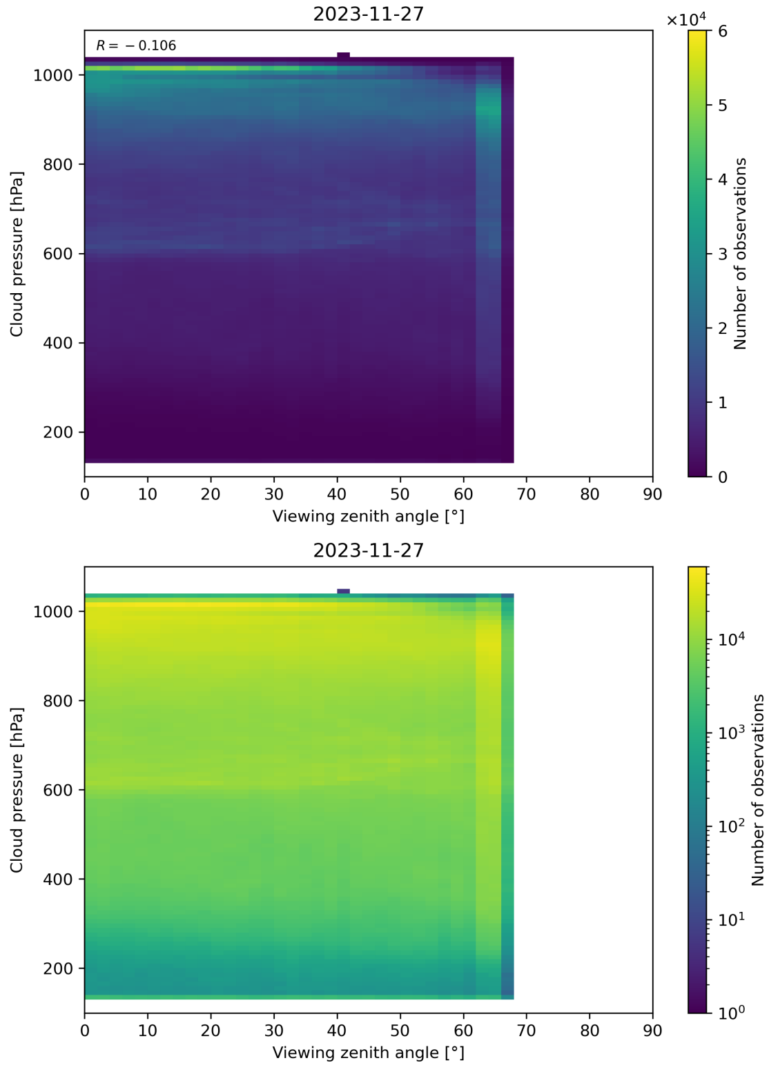
Figure 121: Scatter density plot of “Viewing zenith angle” against “Cloud pressure” for 2023-11-26 to 2023-11-28.
