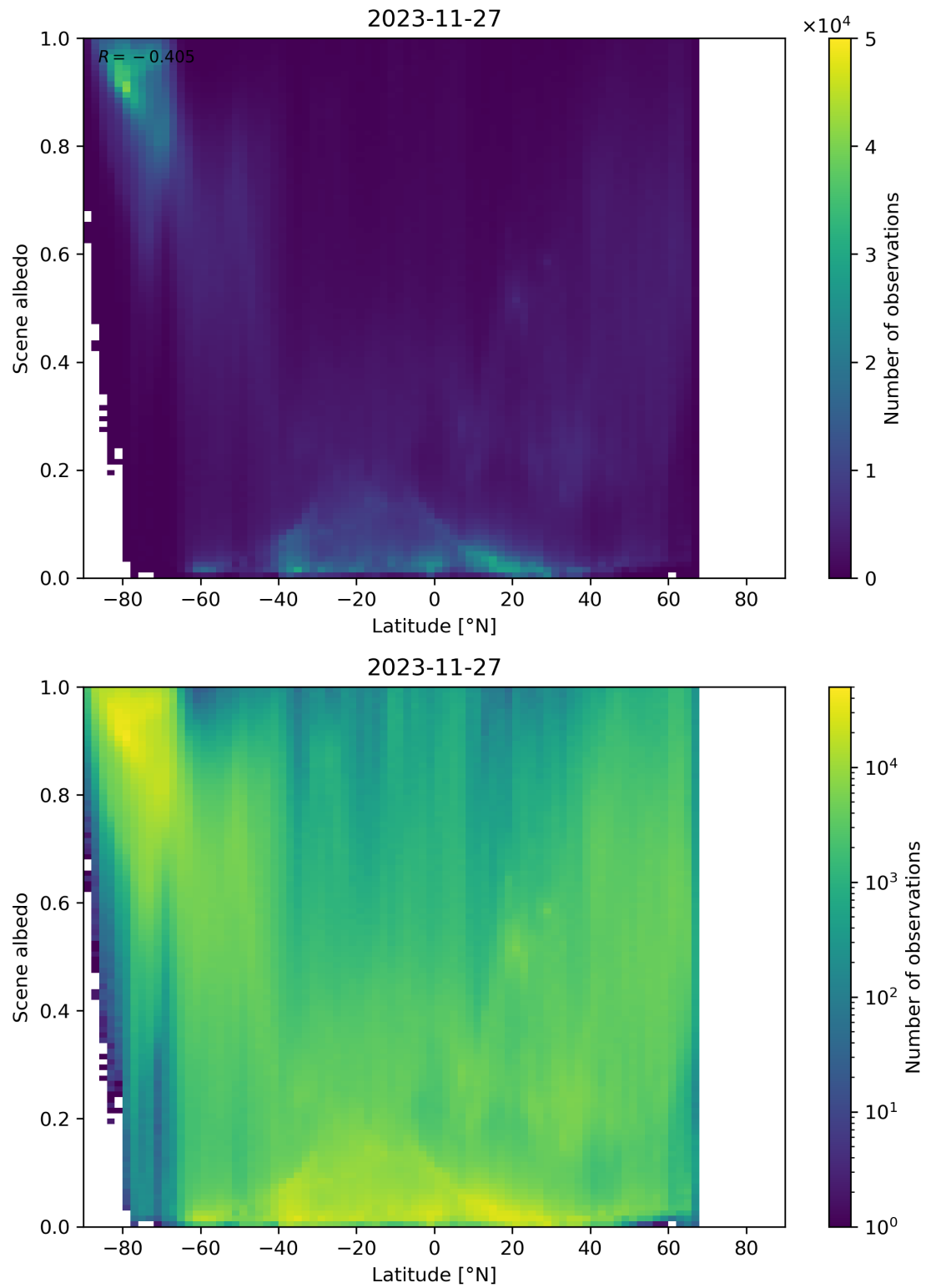
Figure 95: Scatter density plot of “Latitude” against “Scene albedo” for 2023-11-26 to 2023-11-28.
