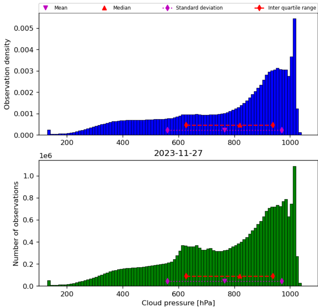
Figure 30: Histogram of “Cloud pressure” for 2023-11-26 to 2023-11-28
