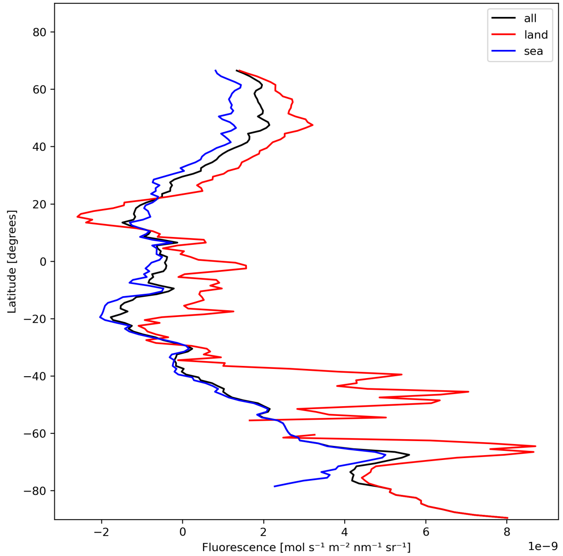
Figure 23: Zonal average of “Fluorescence” for 2023-11-26 to 2023-11-28.
