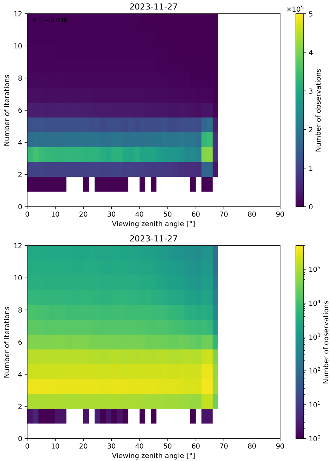
Figure 124: Scatter density plot of “Viewing zenith angle” against “Number of iterations” for 2023-11-26 to 2023-11-28.
