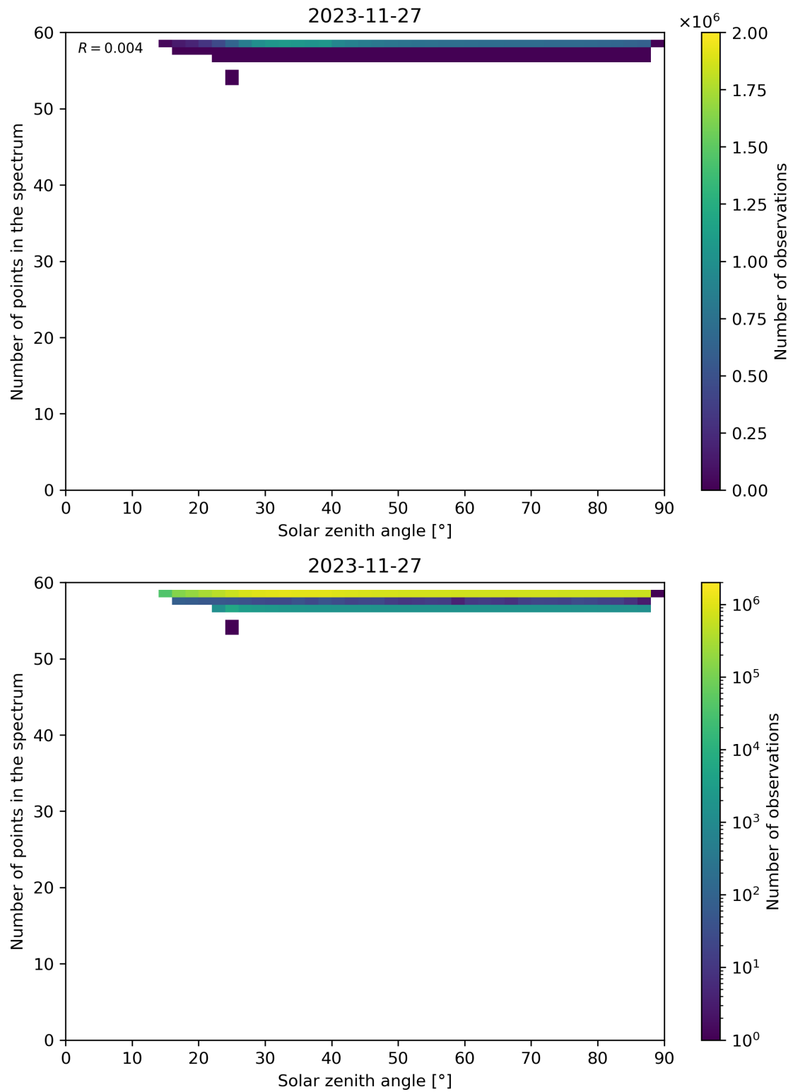
Figure 115: Scatter density plot of “Solar zenith angle” against “Number of points in the spectrum” for 2023-11-26 to 2023-11-28.
