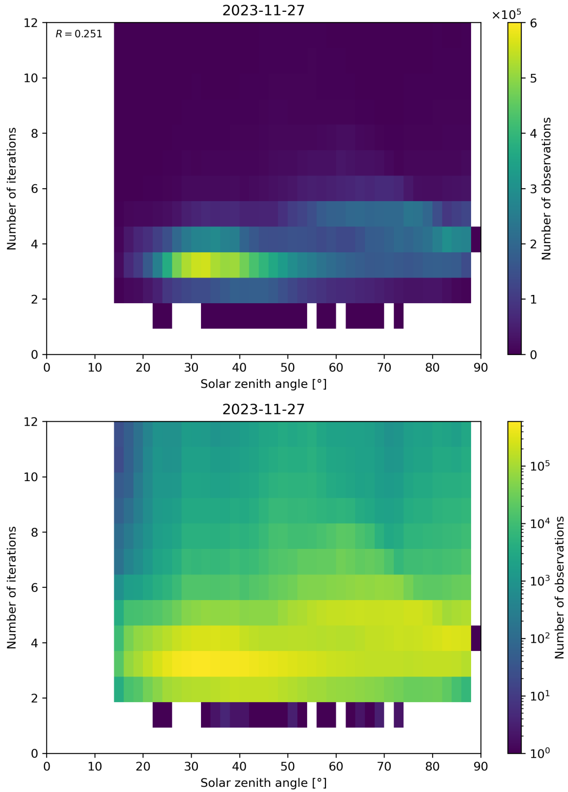
Figure 114: Scatter density plot of “Solar zenith angle” against “Number of iterations” for 2023-11-26 to 2023-11-28.
