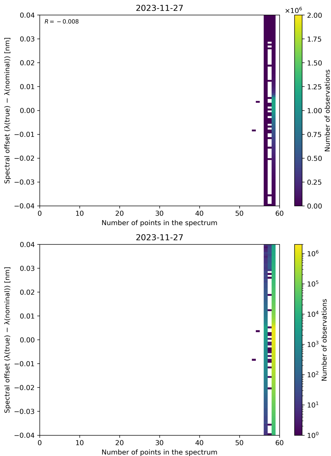
Figure 101: Scatter density plot of “Number of points in the spectrum” against “Spectral offset ( \lambda(\text{true}) - \lambda(\text{nominal}) )” for 2023-11-26 to 2023-11-28.
