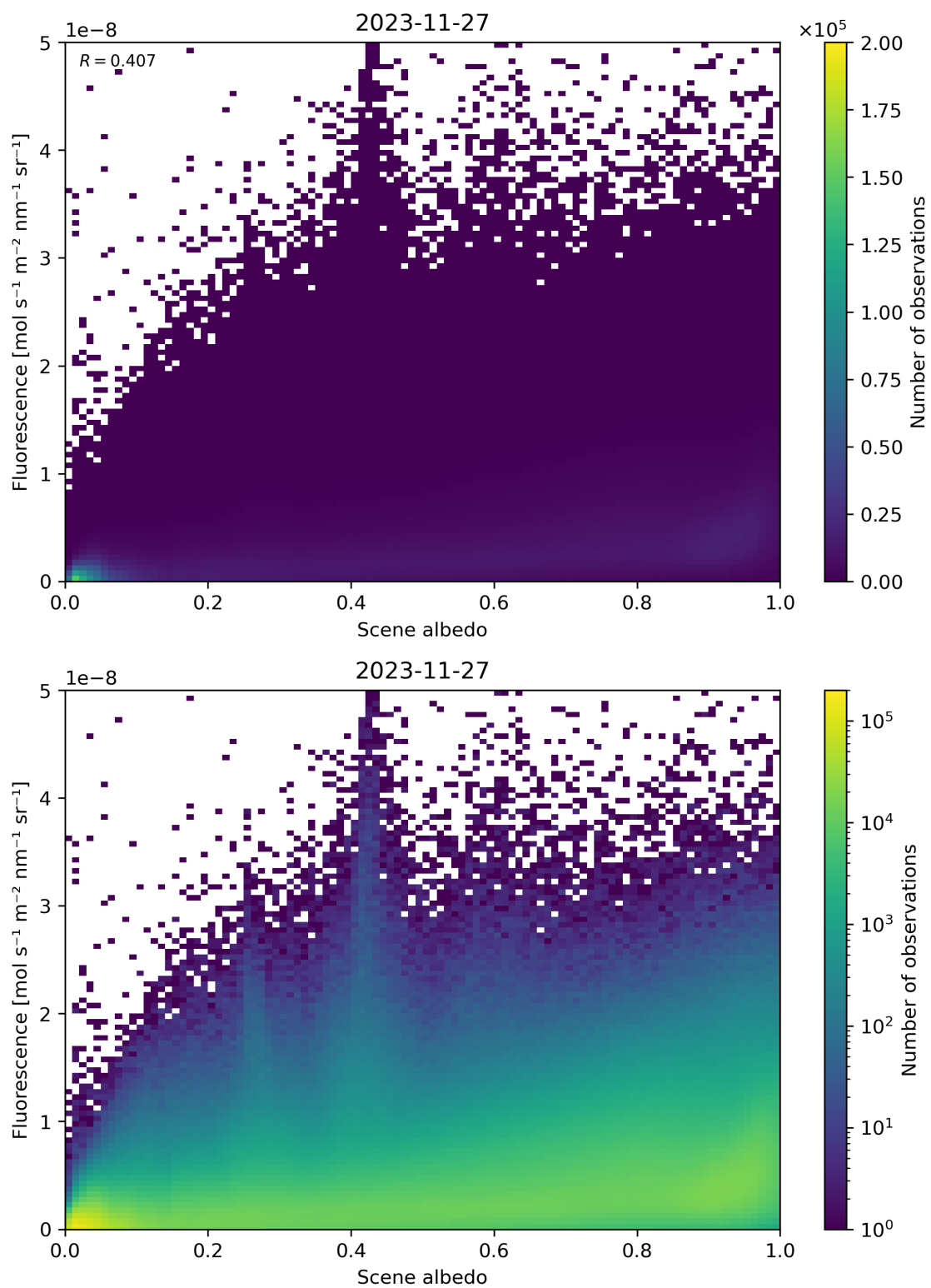
Figure 104: Scatter density plot of “Scene albedo” against “Fluorescence” for 2023-11-26 to 2023-11-28.
