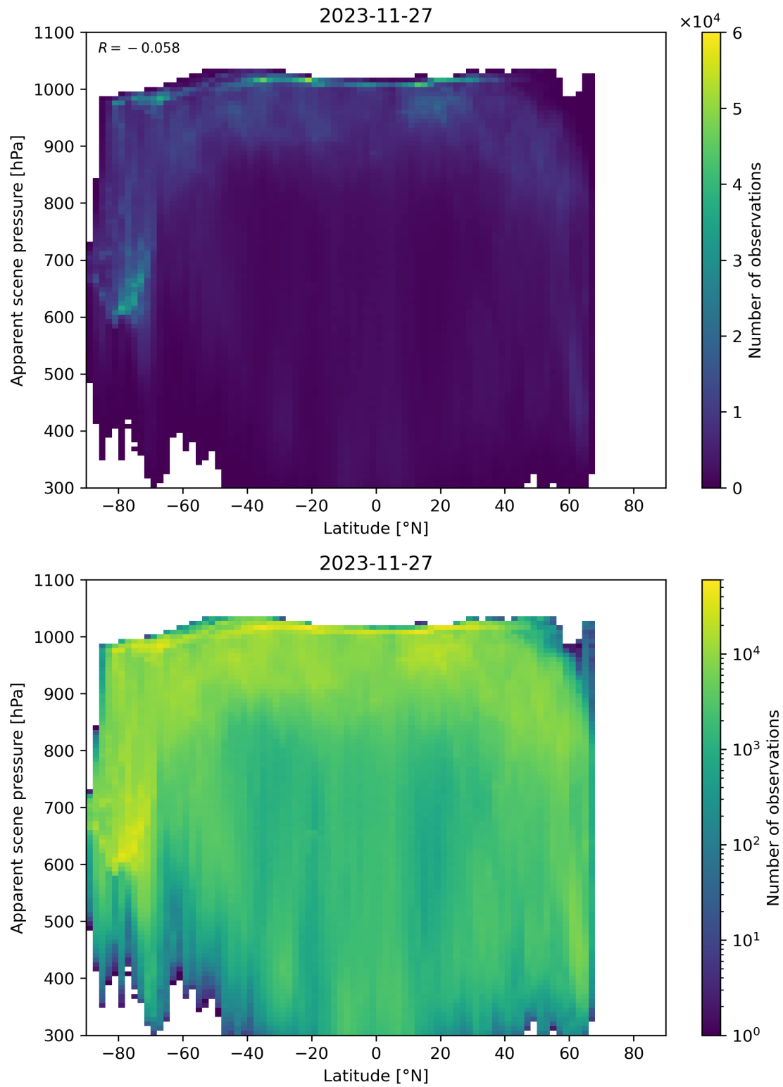
Figure 88: Scatter density plot of “Latitude” against “Apparent scene pressure” for 2023-11-26 to 2023-11-28.
