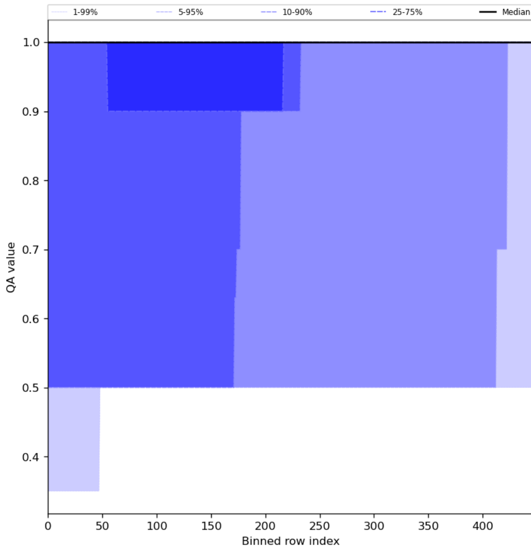
Figure 46: Along track statistics of “QA value” for 2023-11-26 to 2023-11-28
