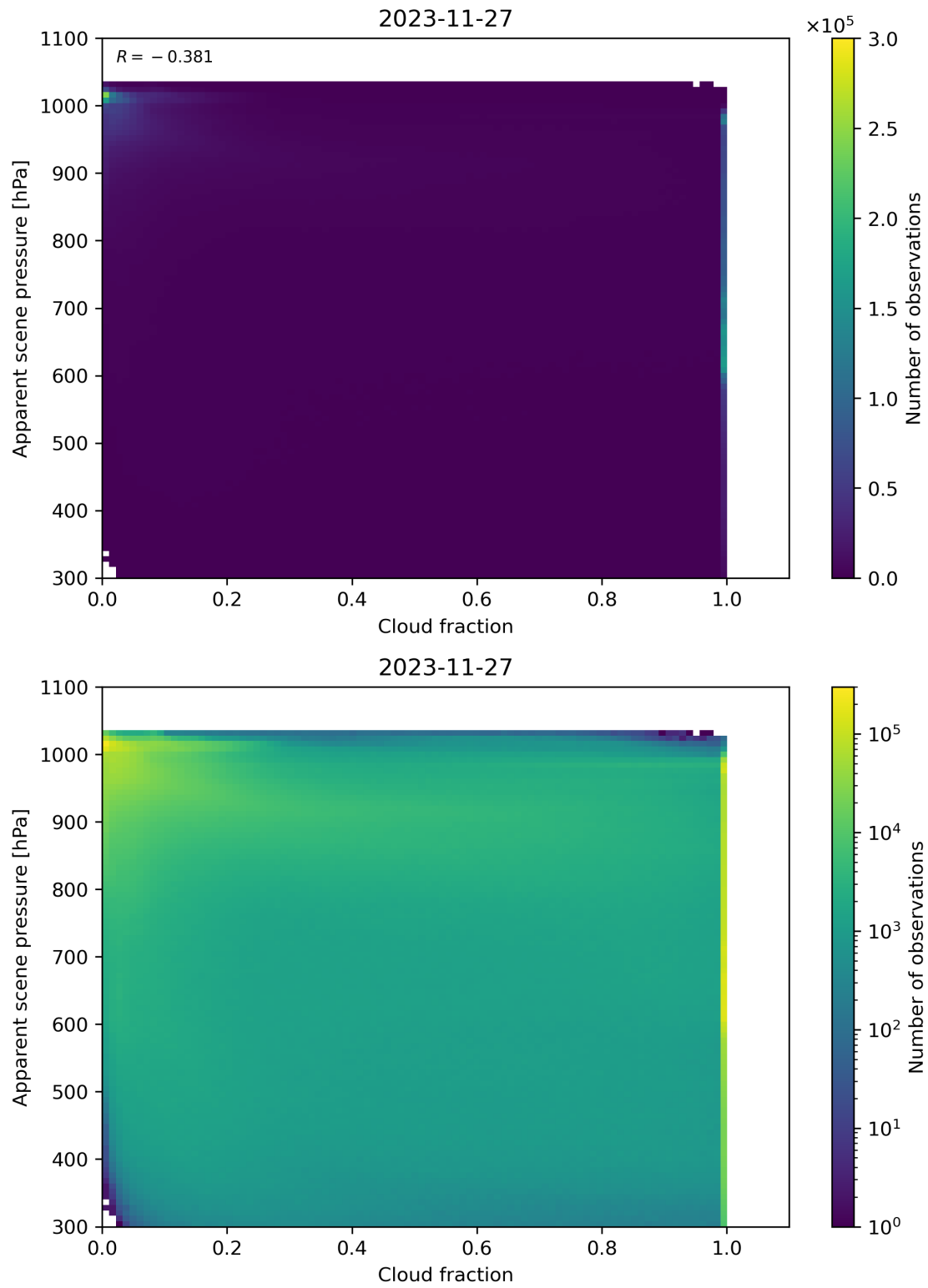
Figure 70: Scatter density plot of “Cloud fraction” against “Apparent scene pressure” for 2023-11-26 to 2023-11-28.
