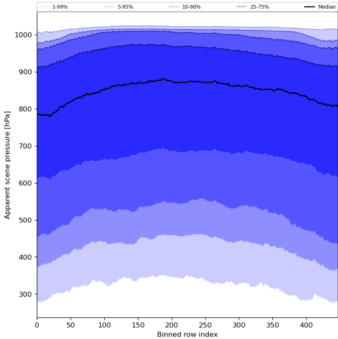
Figure 53: Along track statistics of “Apparent scene pressure” for 2023-11-26 to 2023-11-28
