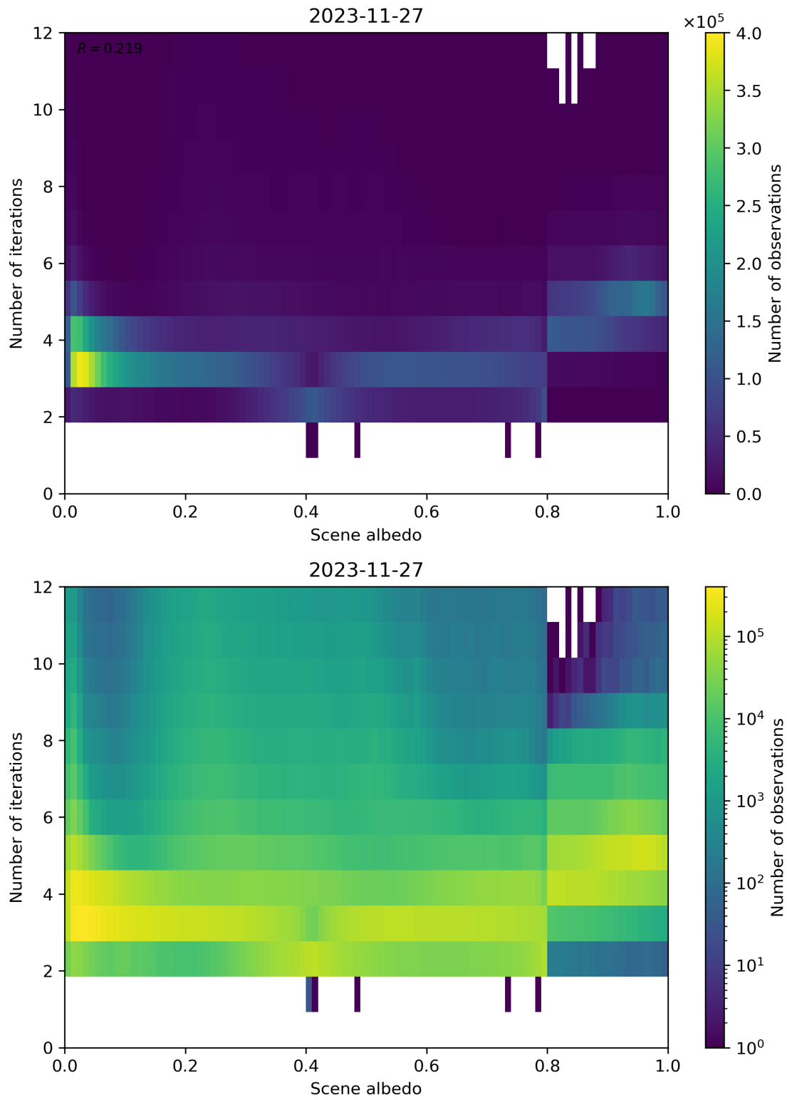
Figure 105: Scatter density plot of “Scene albedo” against “Number of iterations” for 2023-11-26 to 2023-11-28.
