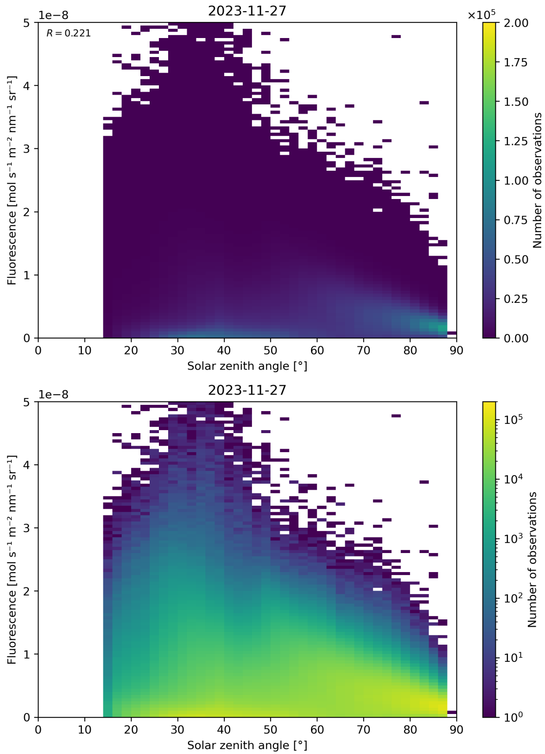
Figure 112: Scatter density plot of “Solar zenith angle” against “Fluorescence” for 2023-11-26 to 2023-11-28.
