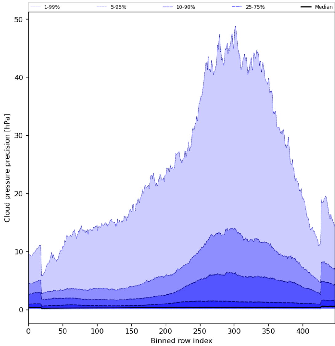
Figure 48: Along track statistics of “Cloud pressure precision” for 2023-11-26 to 2023-11-28
