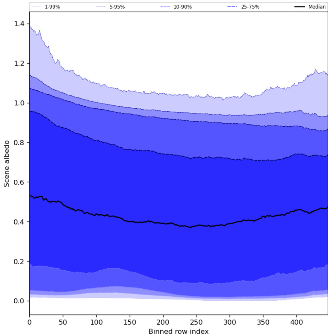
Figure 51: Along track statistics of “Scene albedo” for 2023-11-26 to 2023-11-28
