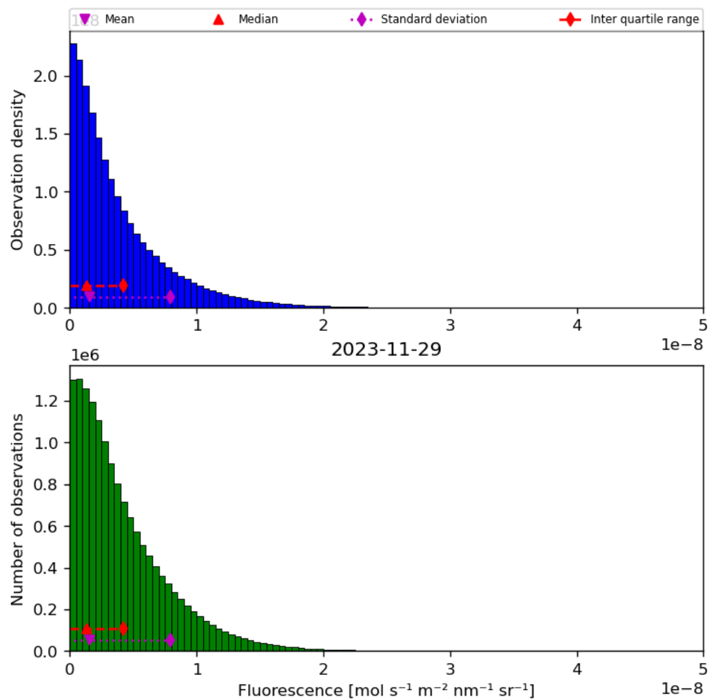
Figure 40: Histogram of “Fluorescence” for 2023-11-28 to 2023-11-30
