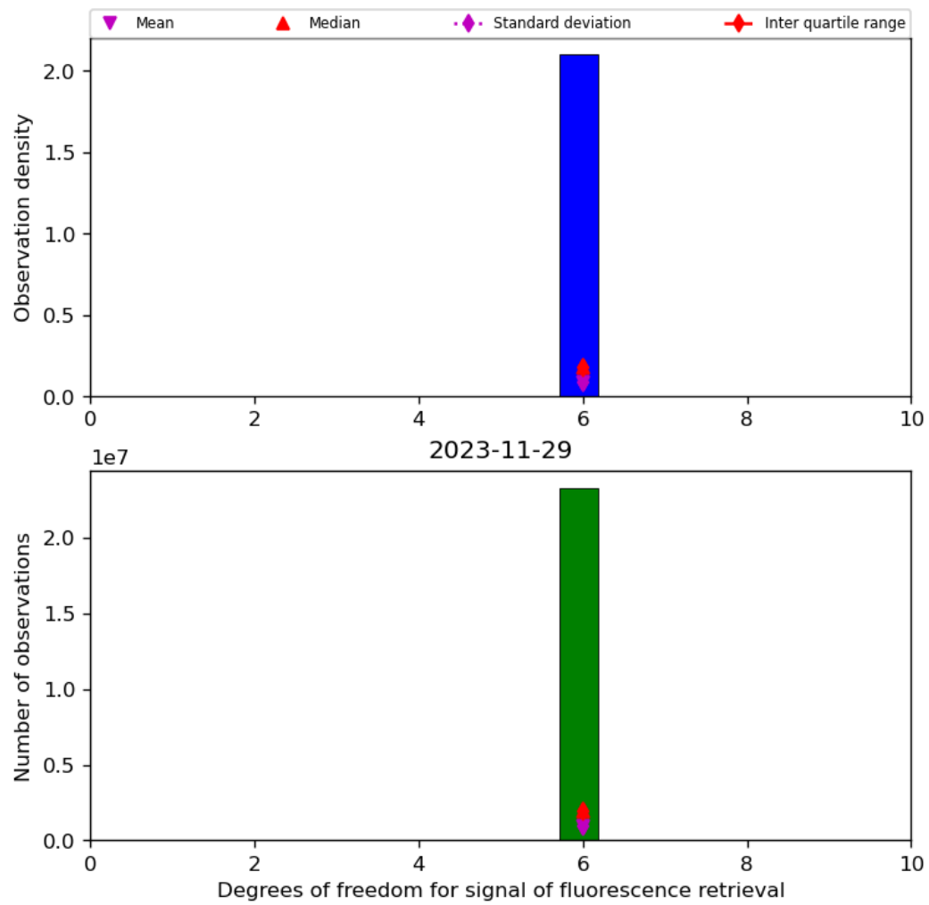
Figure 43: Histogram of “Degrees of freedom for signal of fluorescence retrieval” for 2023-11-28 to 2023-11-30
