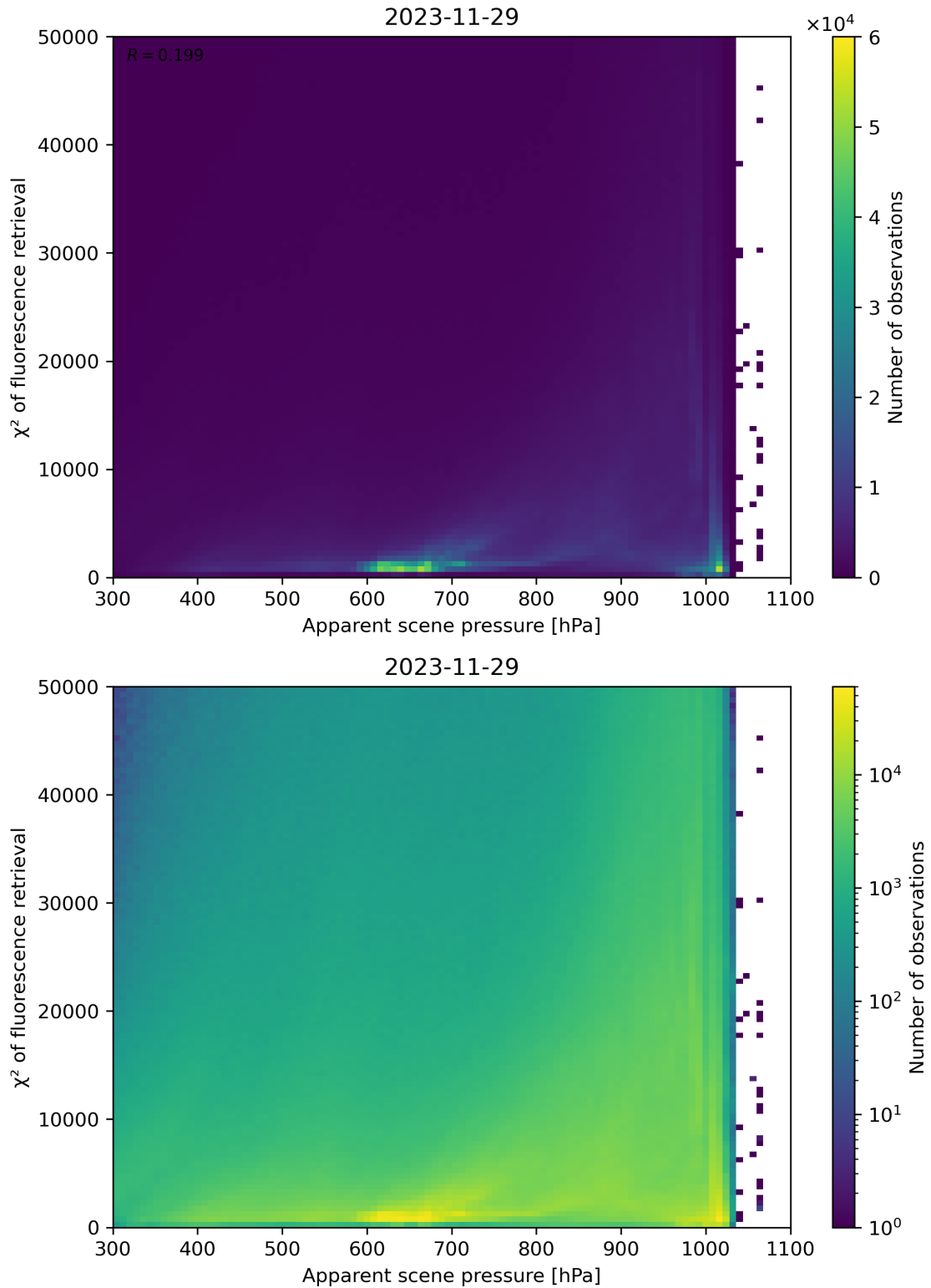
Figure 63: Scatter density plot of “Apparent scene pressure” against “ \chi^2 of fluorescence retrieval” for 2023-11-28 to 2023-11-30.
