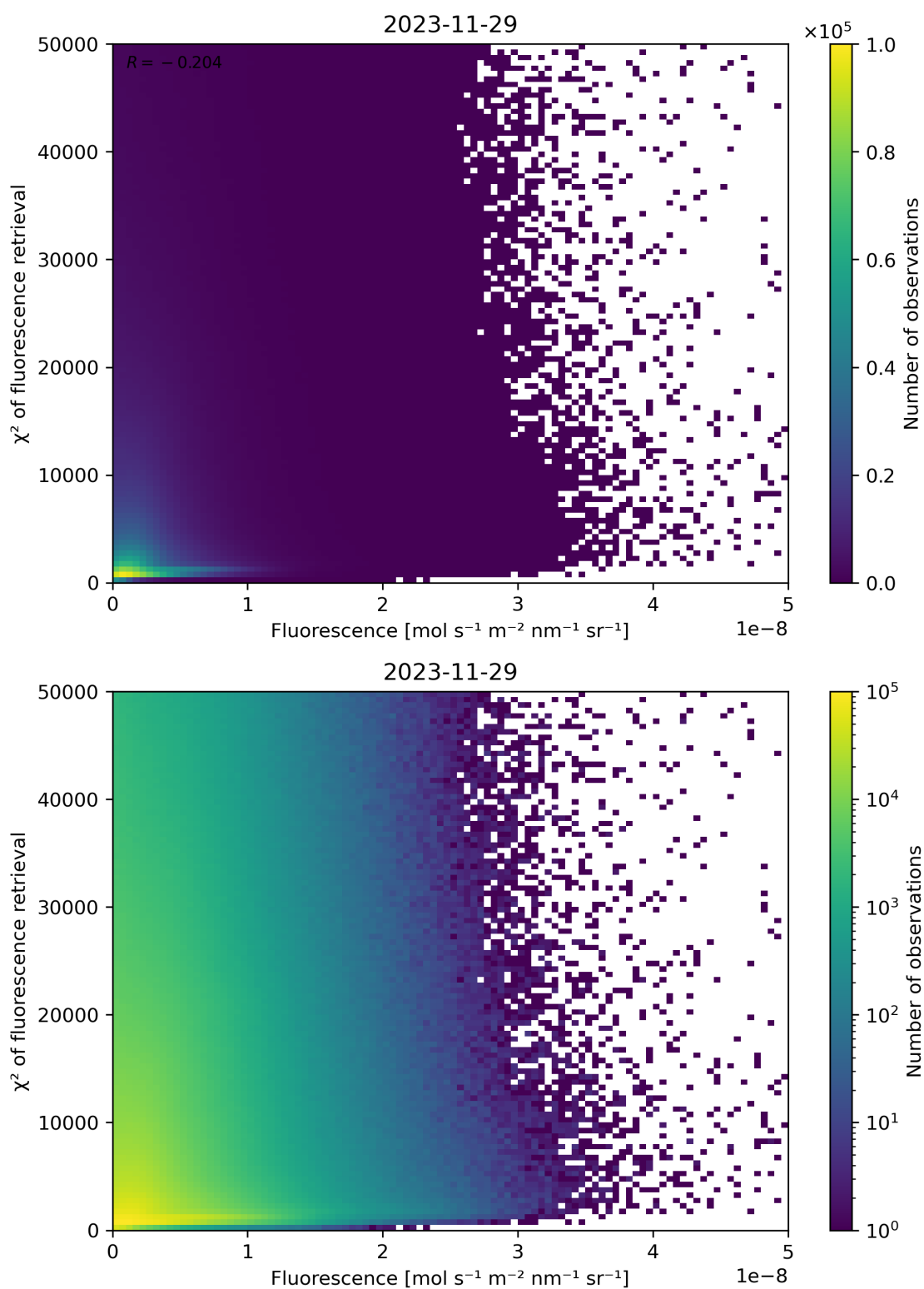
Figure 85: Scatter density plot of “Fluorescence” against “ \chi^2 of fluorescence retrieval” for 2023-11-28 to 2023-11-30.
