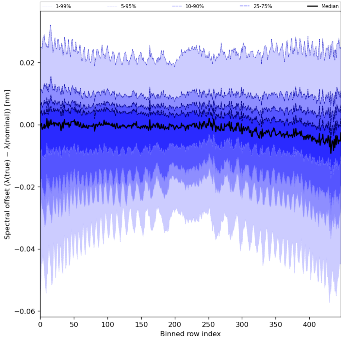
Figure 62: Along track statistics of “Spectral offset ( \lambda(\text{true}) - \lambda(\text{nominal}) )” for 2023-11-28 to 2023-11-30
