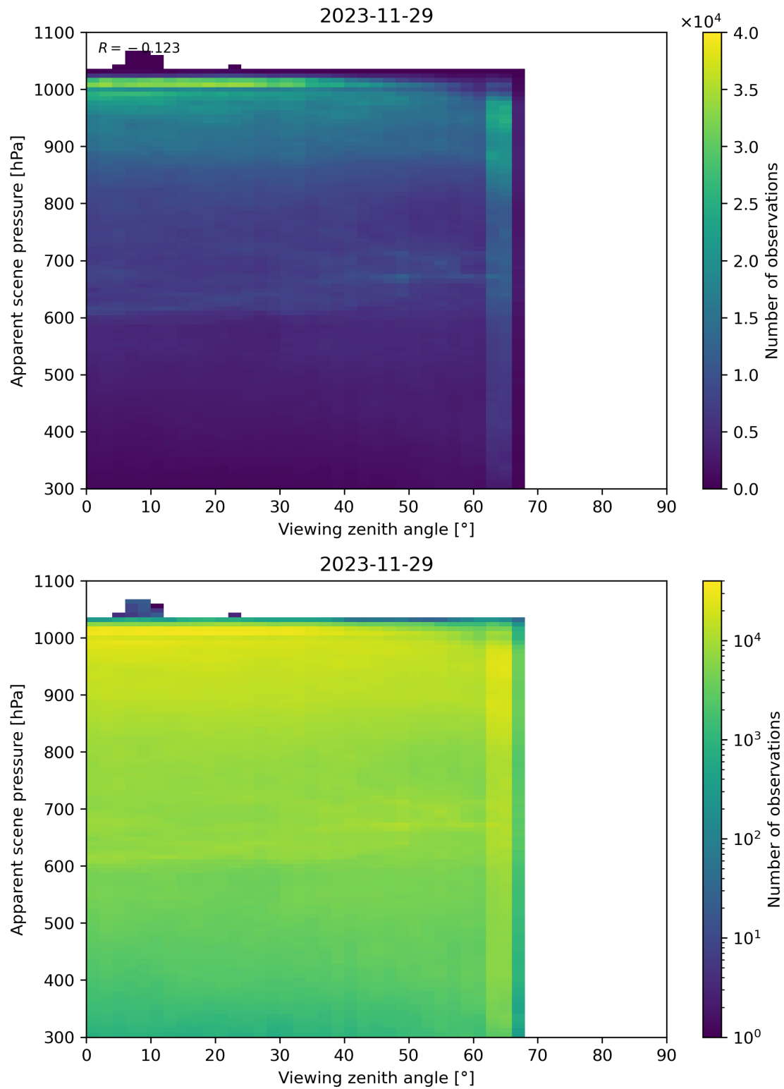
Figure 118: Scatter density plot of “Viewing zenith angle” against “Apparent scene pressure” for 2023-11-28 to 2023-11-30.
