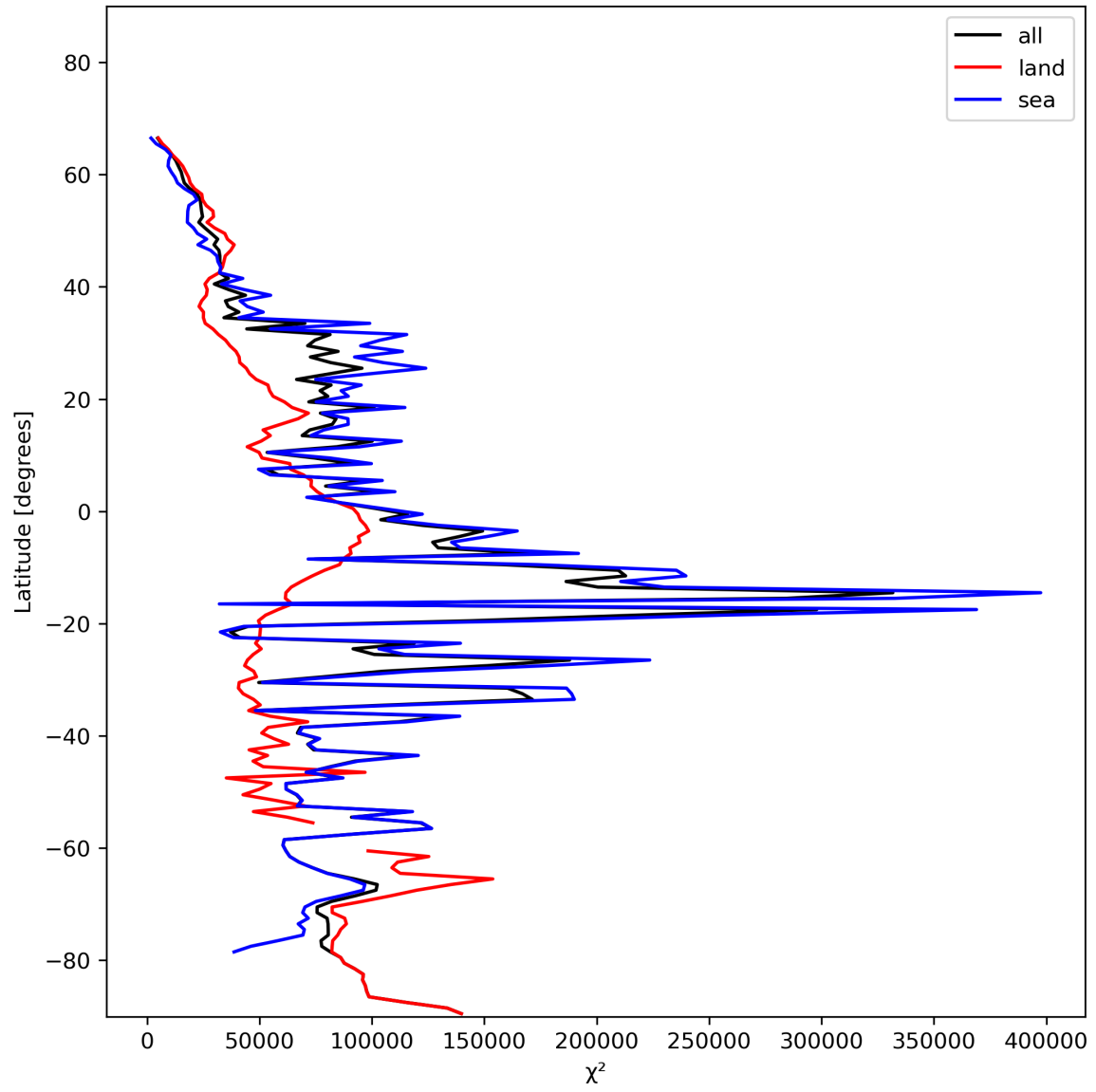
Figure 21: Zonal average of “ \chi^2 ” for 2023-11-28 to 2023-11-30.
