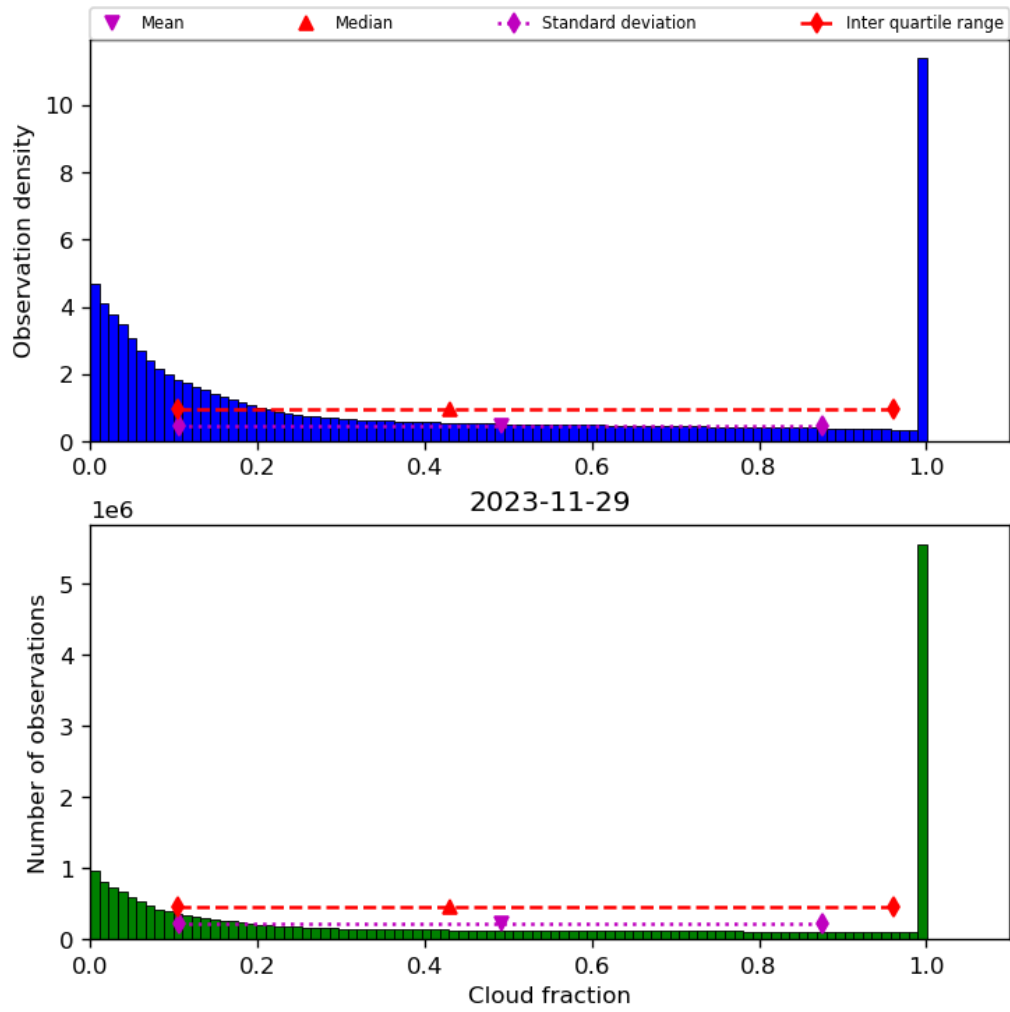
Figure 32: Histogram of “Cloud fraction” for 2023-11-28 to 2023-11-30
