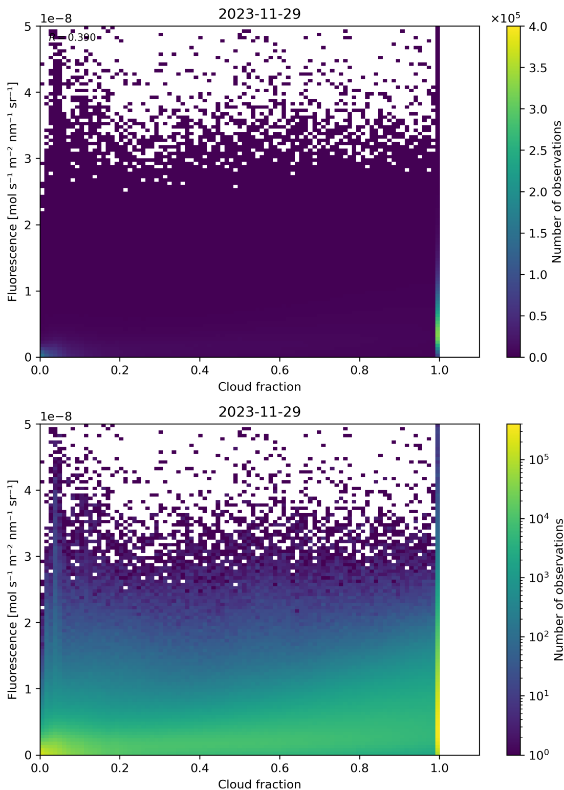
Figure 72: Scatter density plot of “Cloud fraction” against “Fluorescence” for 2023-11-28 to 2023-11-30.
