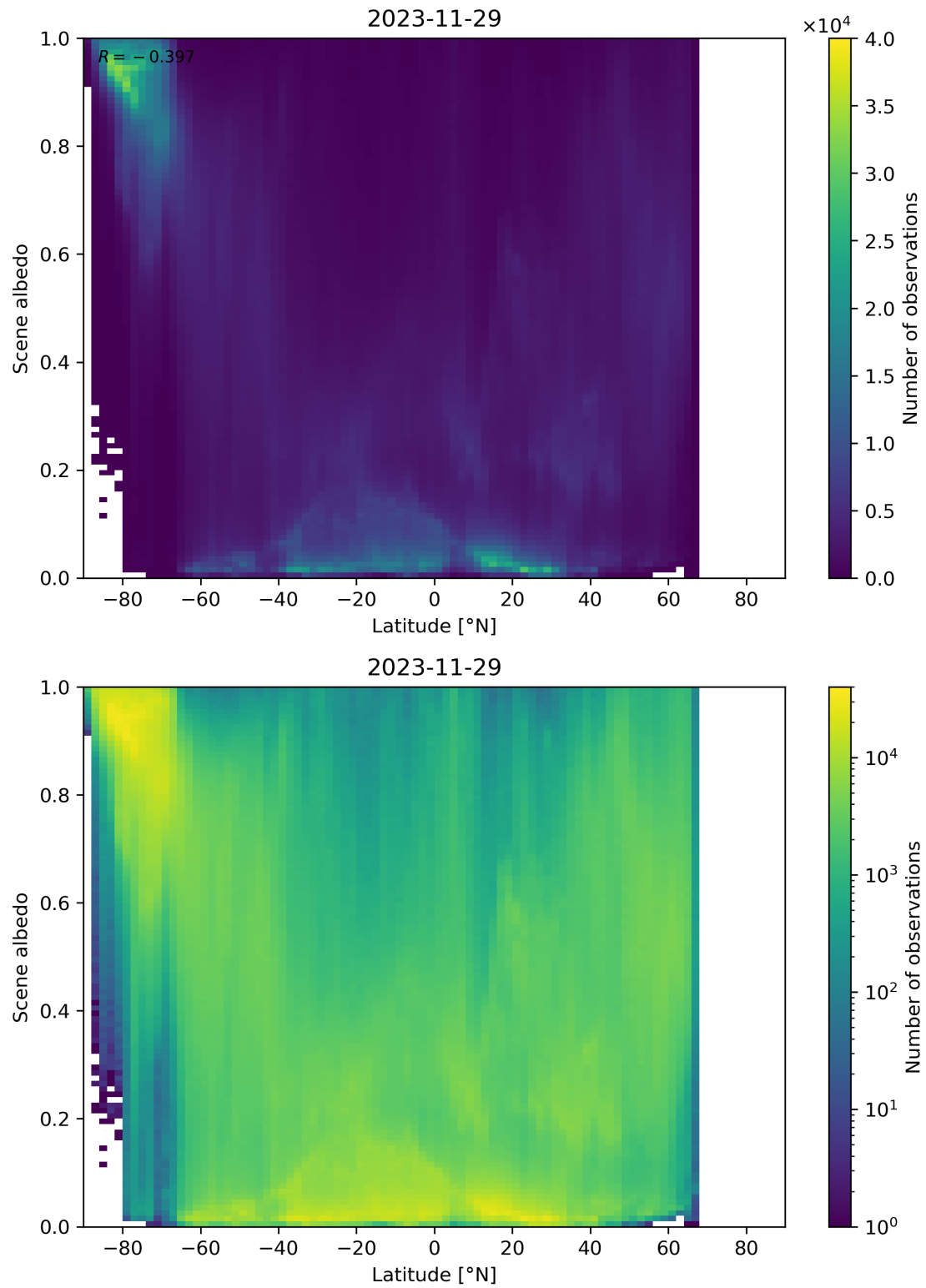
Figure 95: Scatter density plot of “Latitude” against “Scene albedo” for 2023-11-28 to 2023-11-30.
