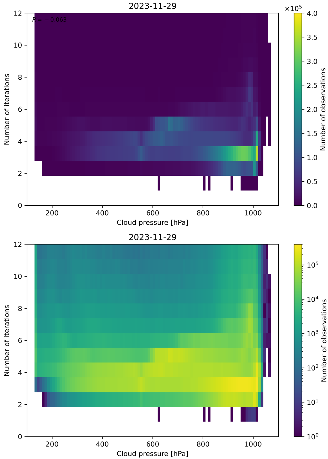
Figure 81: Scatter density plot of “Cloud pressure” against “Number of iterations” for 2023-11-28 to 2023-11-30.
