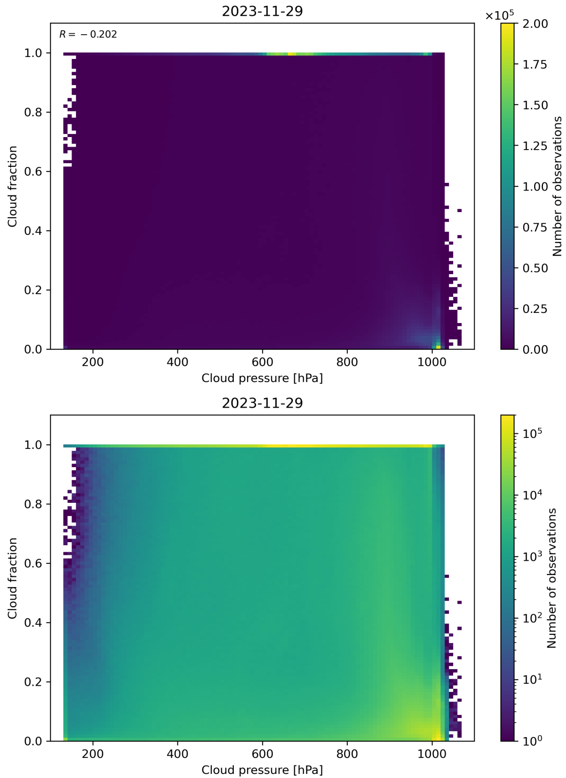
Figure 79: Scatter density plot of “Cloud pressure” against “Cloud fraction” for 2023-11-28 to 2023-11-30.
