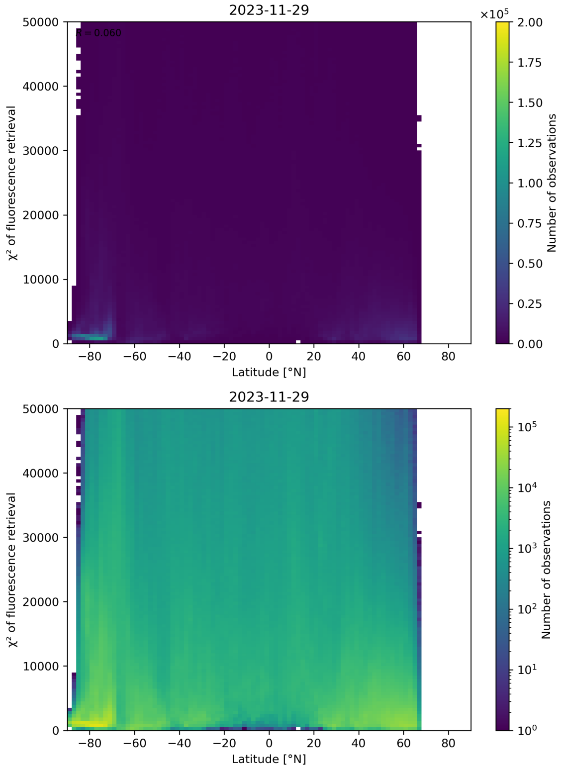
Figure 89: Scatter density plot of “Latitude” against “ \chi^2 of fluorescence retrieval” for 2023-11-28 to 2023-11-30.
