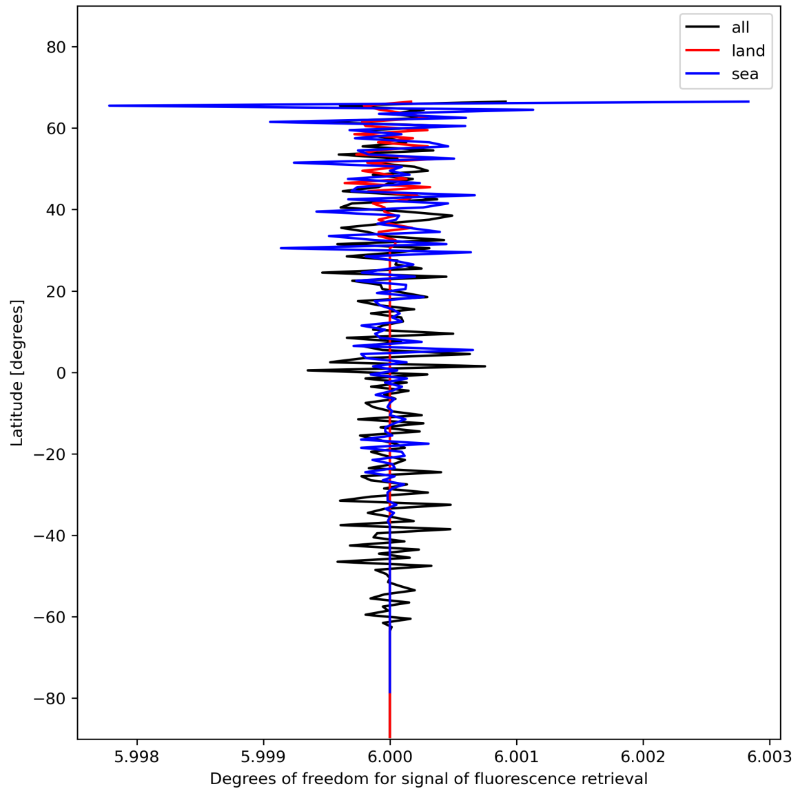
Figure 26: Zonal average of “Degrees of freedom for signal of fluorescence retrieval” for 2023-11-28 to 2023-11-30.
