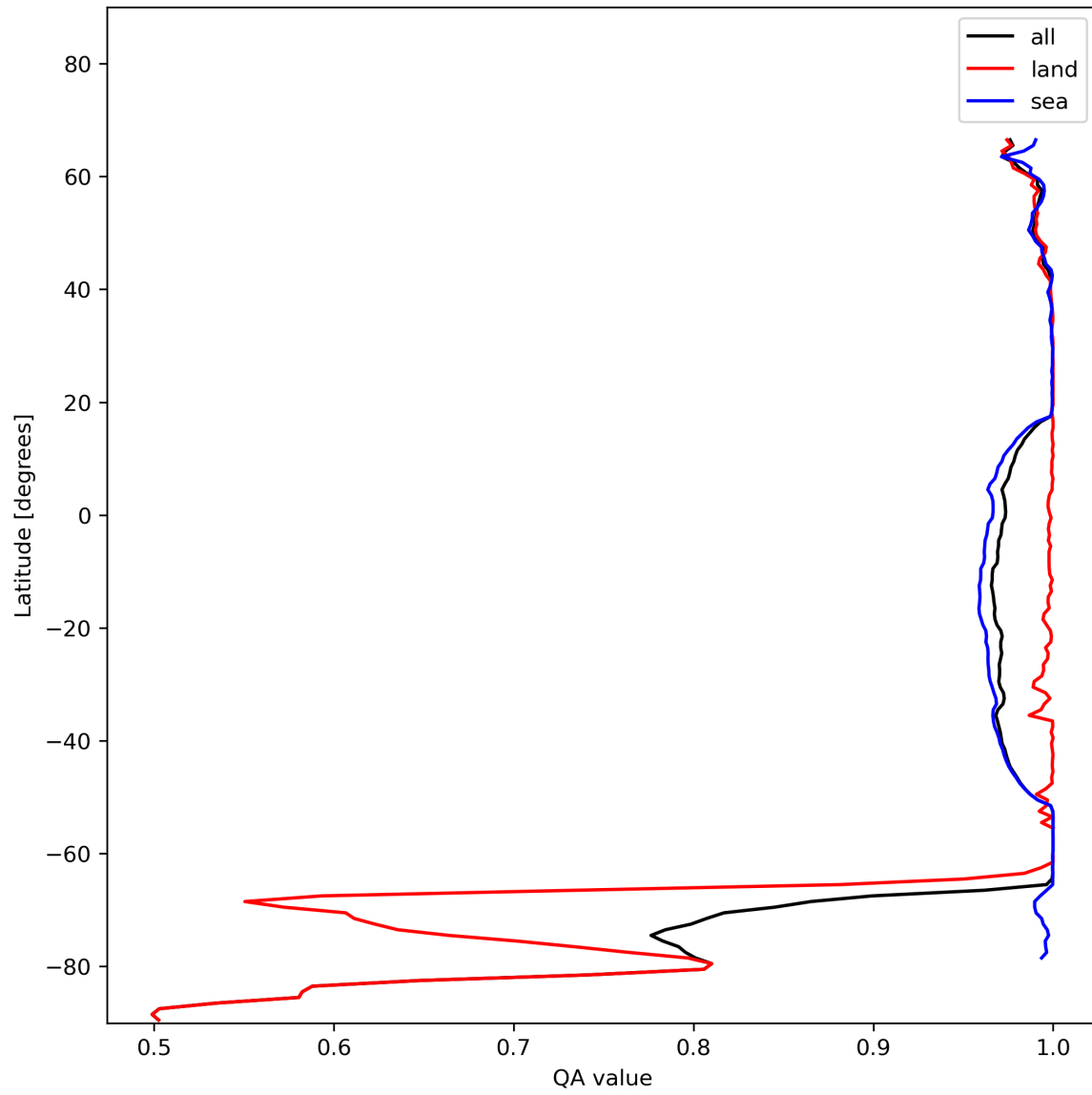
Figure 12: Zonal average of “QA value” for 2023-11-28 to 2023-11-30.
