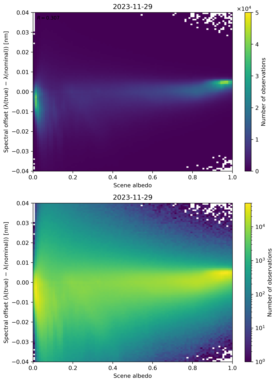
Figure 107: Scatter density plot of “Scene albedo” against “Spectral offset ( \lambda(\text{true}) - \lambda(\text{nominal}) )” for 2023-11-28 to 2023-11-30.
