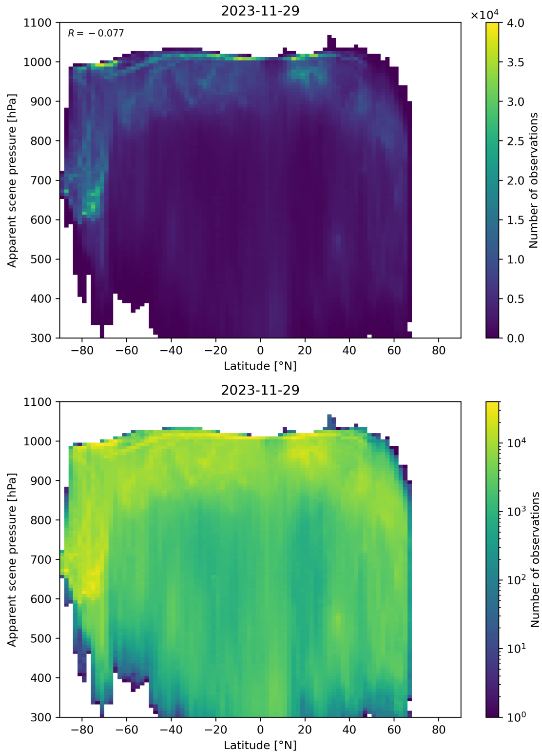
Figure 88: Scatter density plot of “Latitude” against “Apparent scene pressure” for 2023-11-28 to 2023-11-30.
