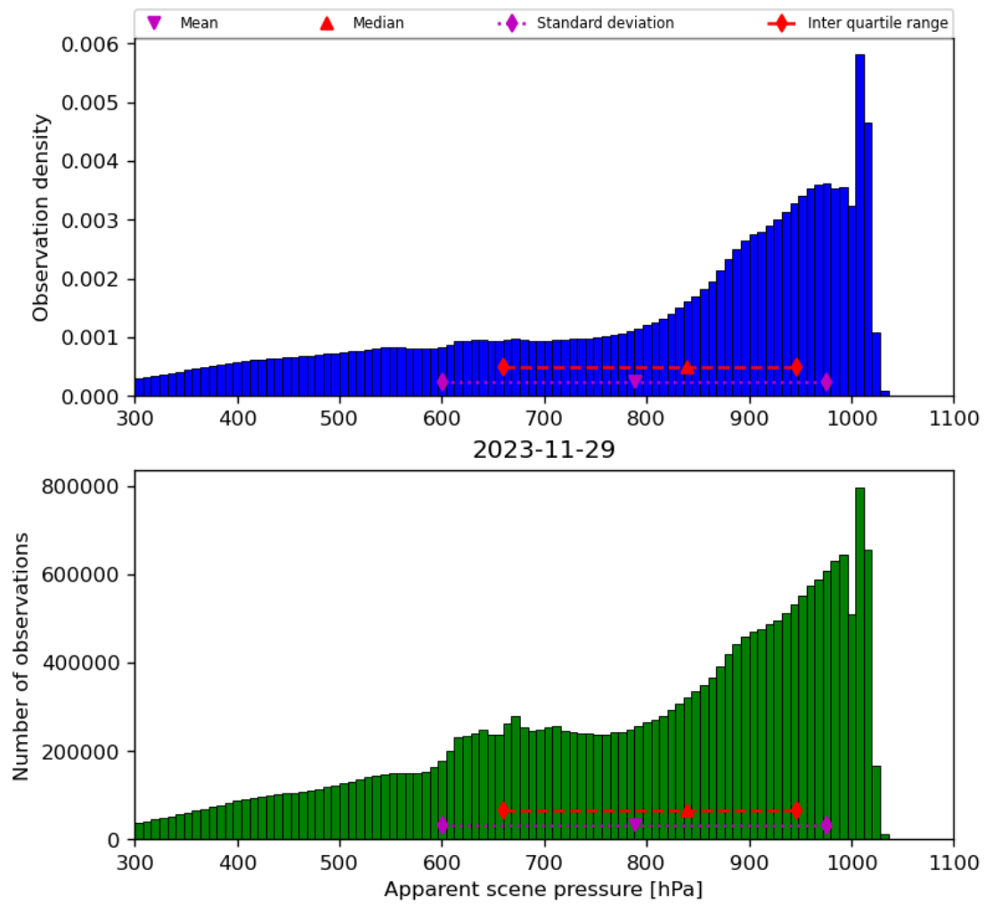
Figure 36: Histogram of “Apparent scene pressure” for 2023-11-28 to 2023-11-30
