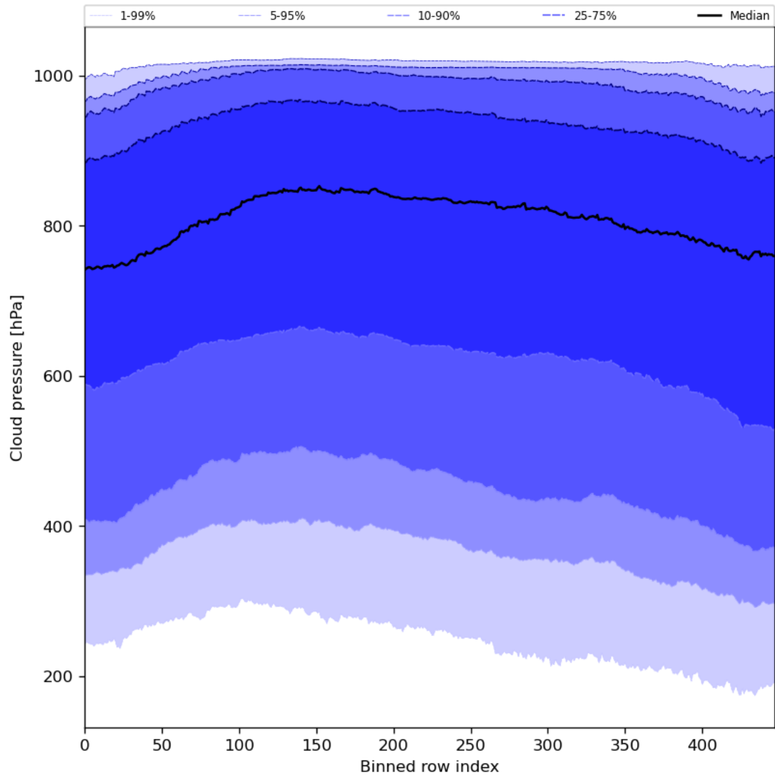
Figure 47: Along track statistics of “Cloud pressure” for 2023-11-28 to 2023-11-30
