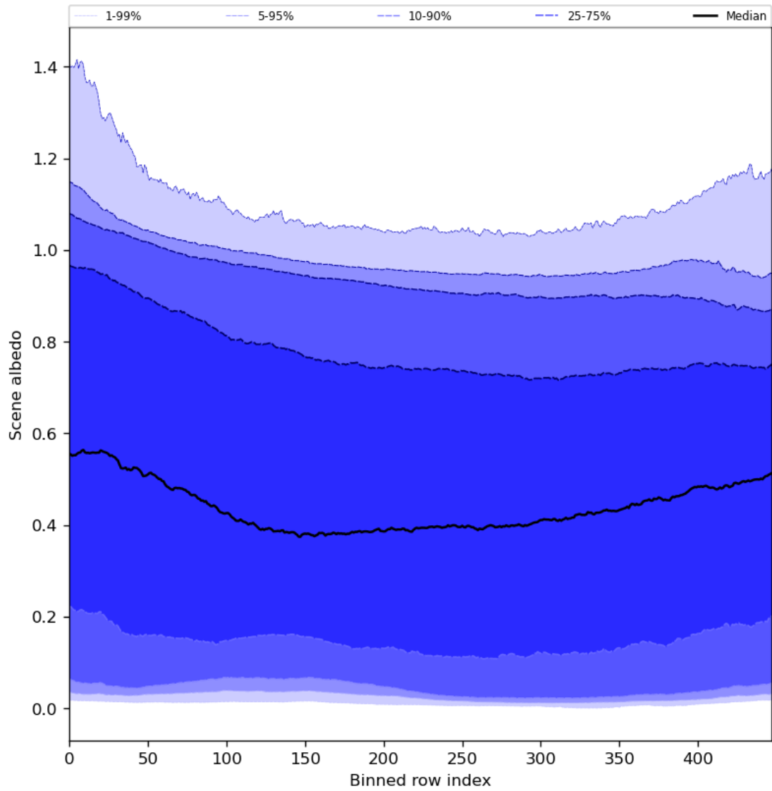
Figure 51: Along track statistics of “Scene albedo” for 2023-11-28 to 2023-11-30
