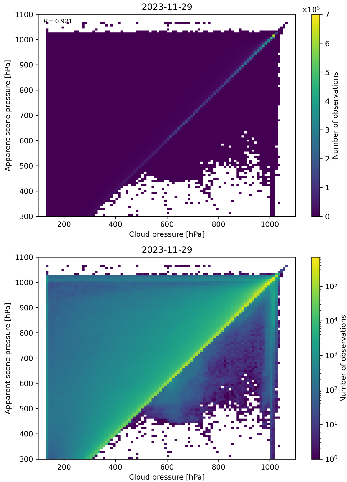
Figure 77: Scatter density plot of “Cloud pressure” against “Apparent scene pressure” for 2023-11-28 to 2023-11-30.
