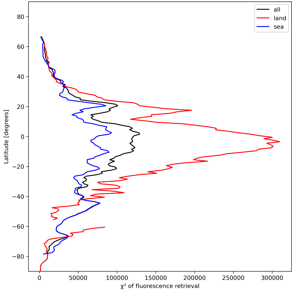
Figure 25: Zonal average of “ \chi^2 of fluorescence retrieval” for 2023-11-28 to 2023-11-30.
