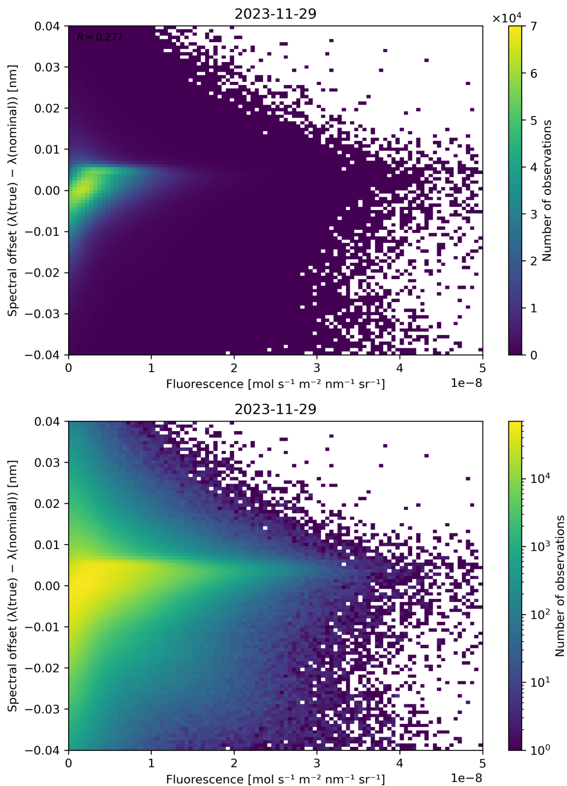
Figure 87: Scatter density plot of “Fluorescence” against “Spectral offset ( \lambda(\text{true}) - \lambda(\text{nominal}) )” for 2023-11-28 to 2023-11-30.
