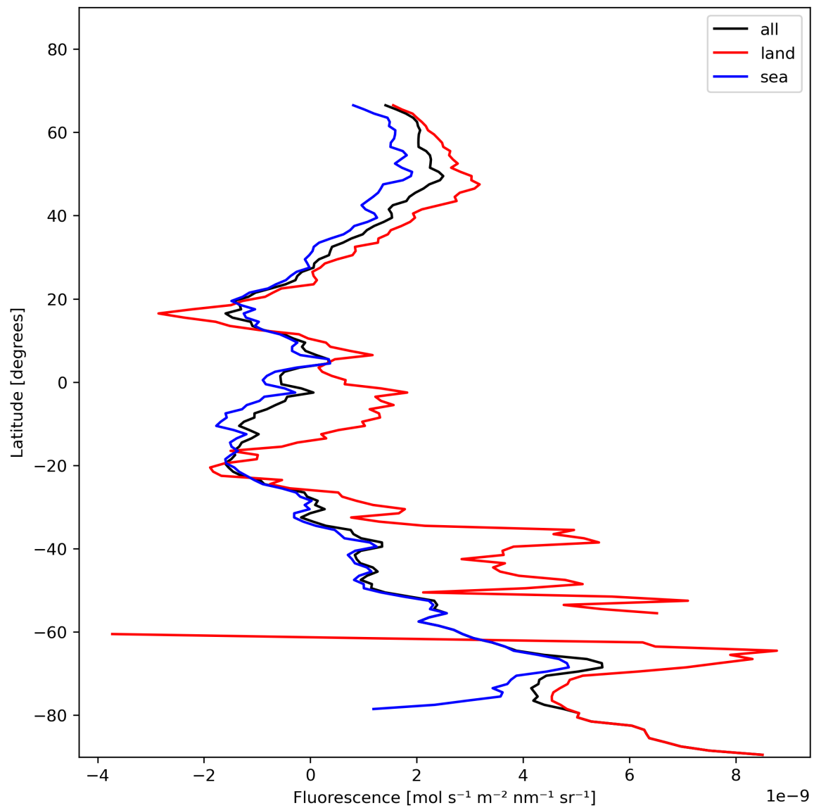
Figure 23: Zonal average of “Fluorescence” for 2023-11-28 to 2023-11-30.
