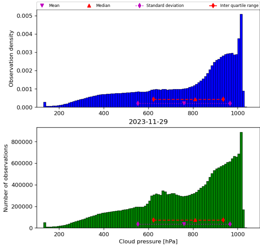
Figure 30: Histogram of “Cloud pressure” for 2023-11-28 to 2023-11-30
