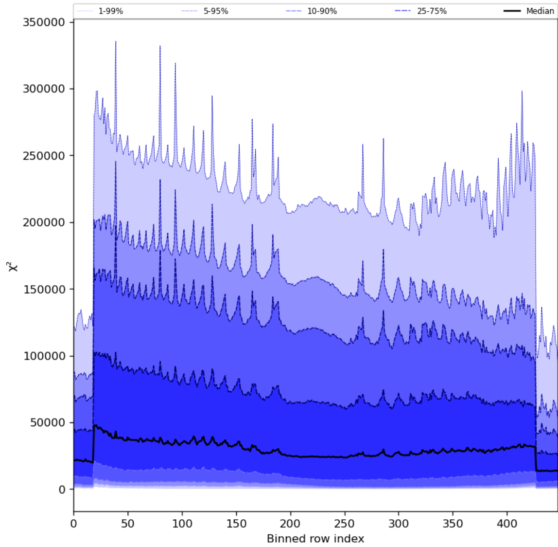
Figure 55: Along track statistics of “ \chi^2 ” for 2023-11-28 to 2023-11-30
