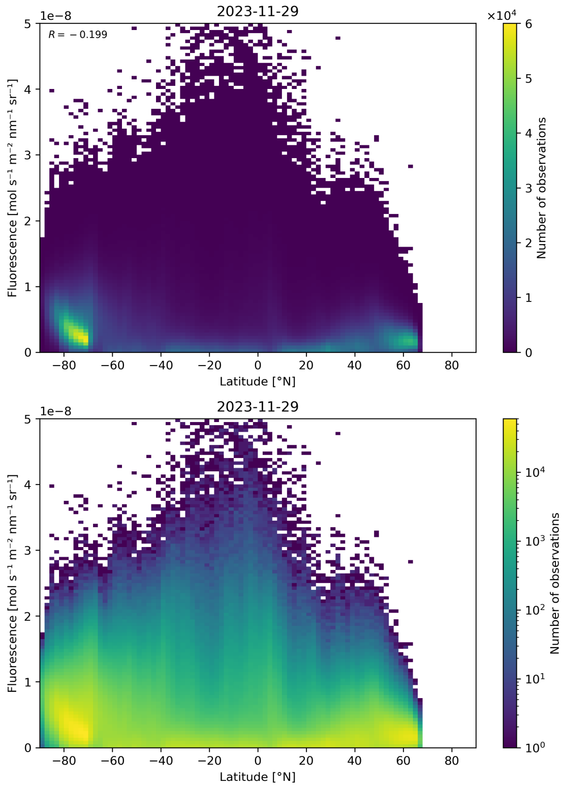
Figure 92: Scatter density plot of “Latitude” against “Fluorescence” for 2023-11-28 to 2023-11-30.
