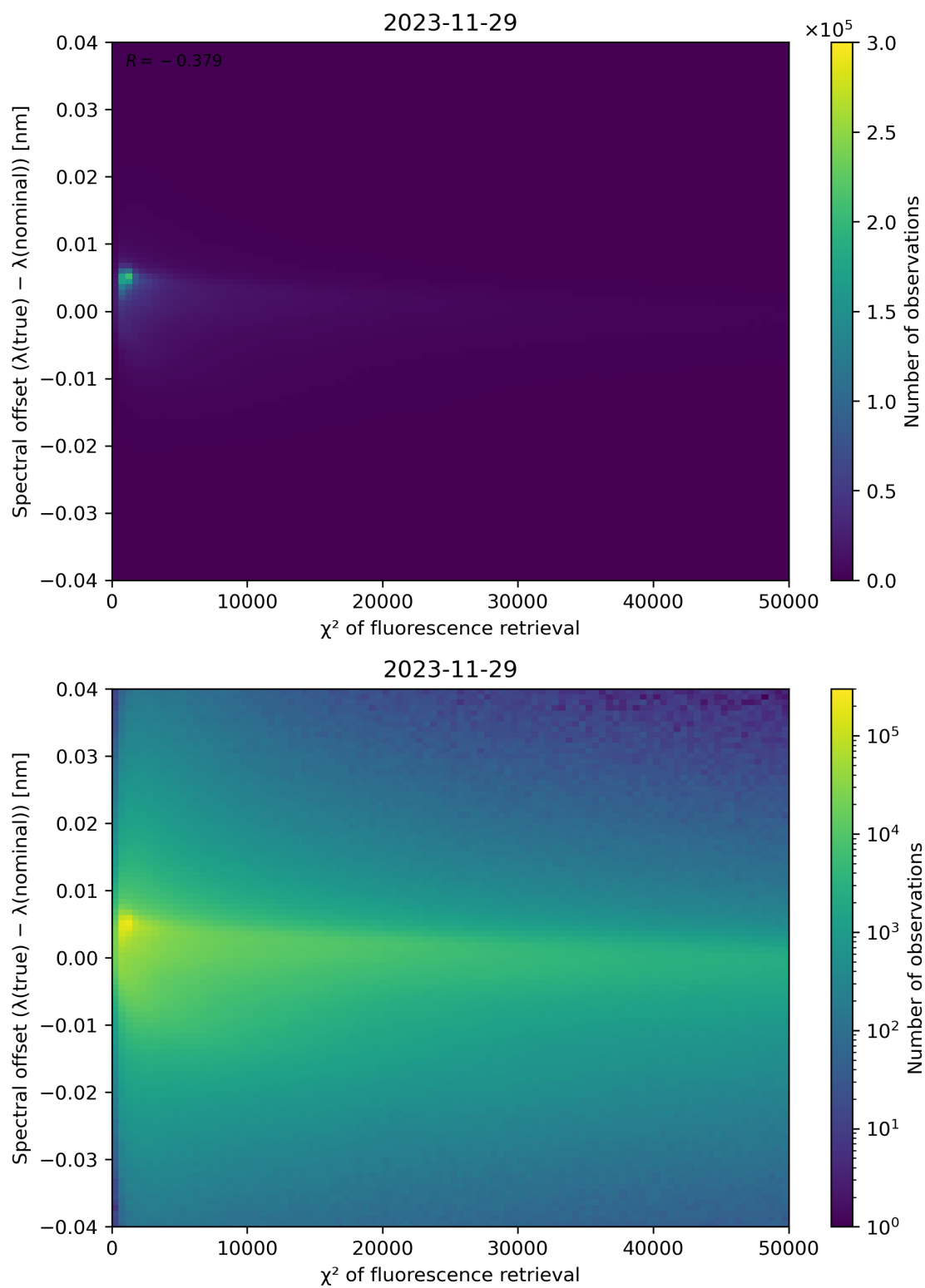
Figure 69: Scatter density plot of " \chi^2 of fluorescence retrieval" against "Spectral offset ( \lambda(\text{true}) - \lambda(\text{nominal}) )" for 2023-11-28 to 2023-11-30.
