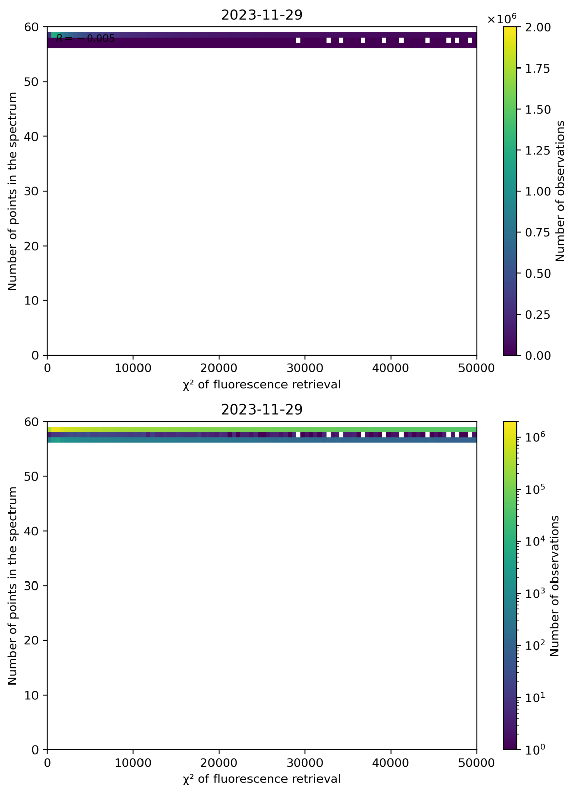
Figure 68: Scatter density plot of " \chi^2 of fluorescence retrieval" against "Number of points in the spectrum" for 2023-11-28 to 2023-11-30.
