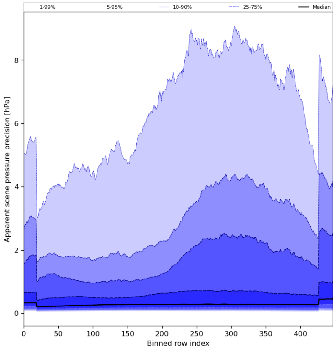
Figure 54: Along track statistics of “Apparent scene pressure precision” for 2023-11-28 to 2023-11-30
