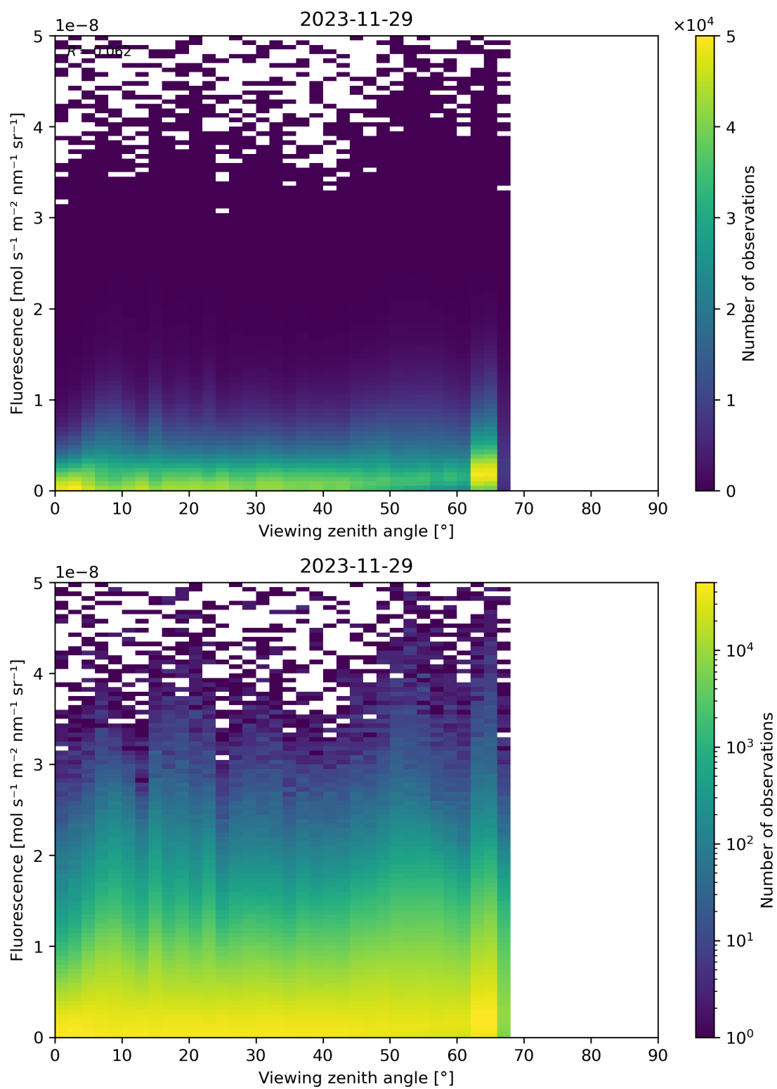
Figure 122: Scatter density plot of “Viewing zenith angle” against “Fluorescence” for 2023-11-28 to 2023-11-30.
