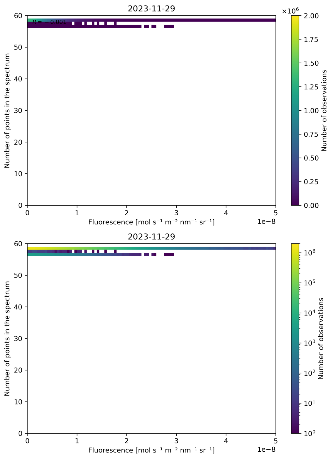
Figure 86: Scatter density plot of “Fluorescence” against “Number of points in the spectrum” for 2023-11-28 to 2023-11-30.
