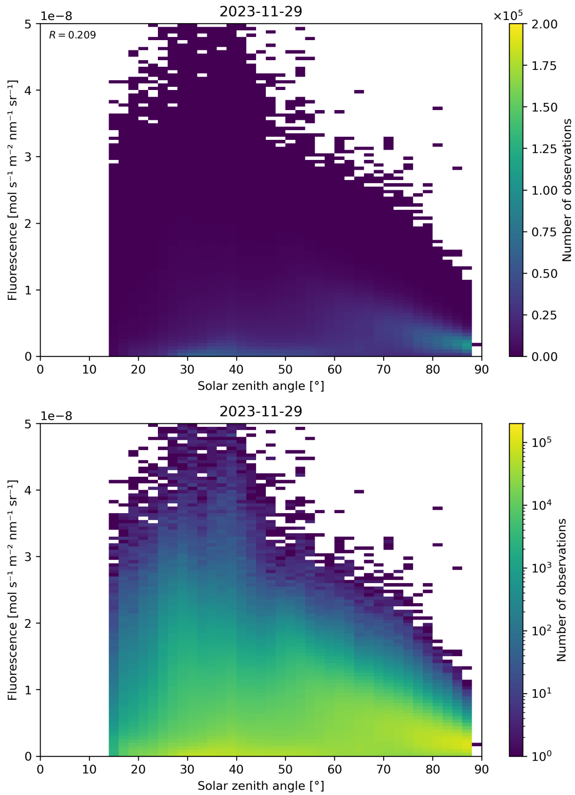
Figure 112: Scatter density plot of “Solar zenith angle” against “Fluorescence” for 2023-11-28 to 2023-11-30.
