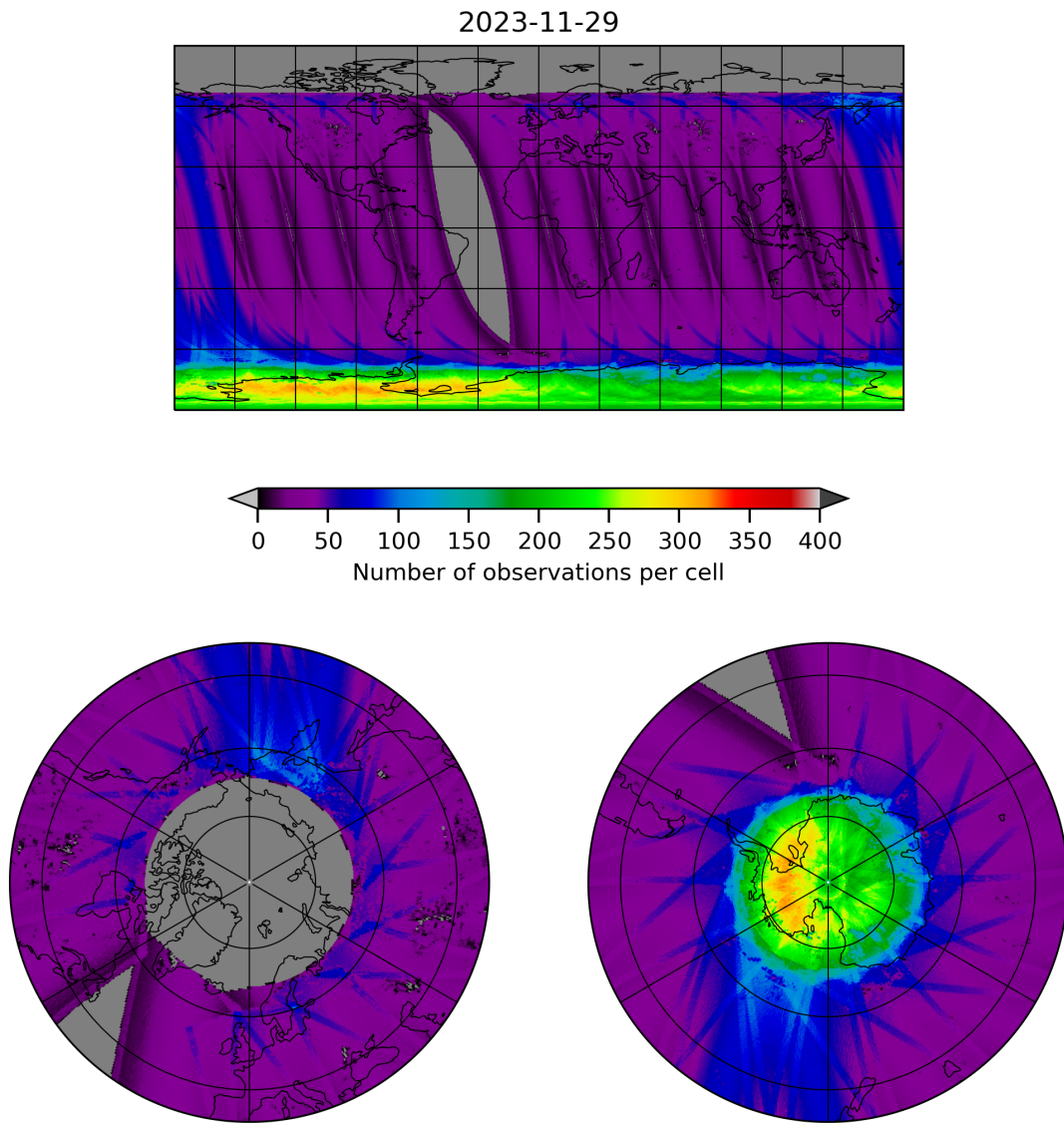
Figure 11: Map of the number of observations for 2023-11-28 to 2023-11-30
