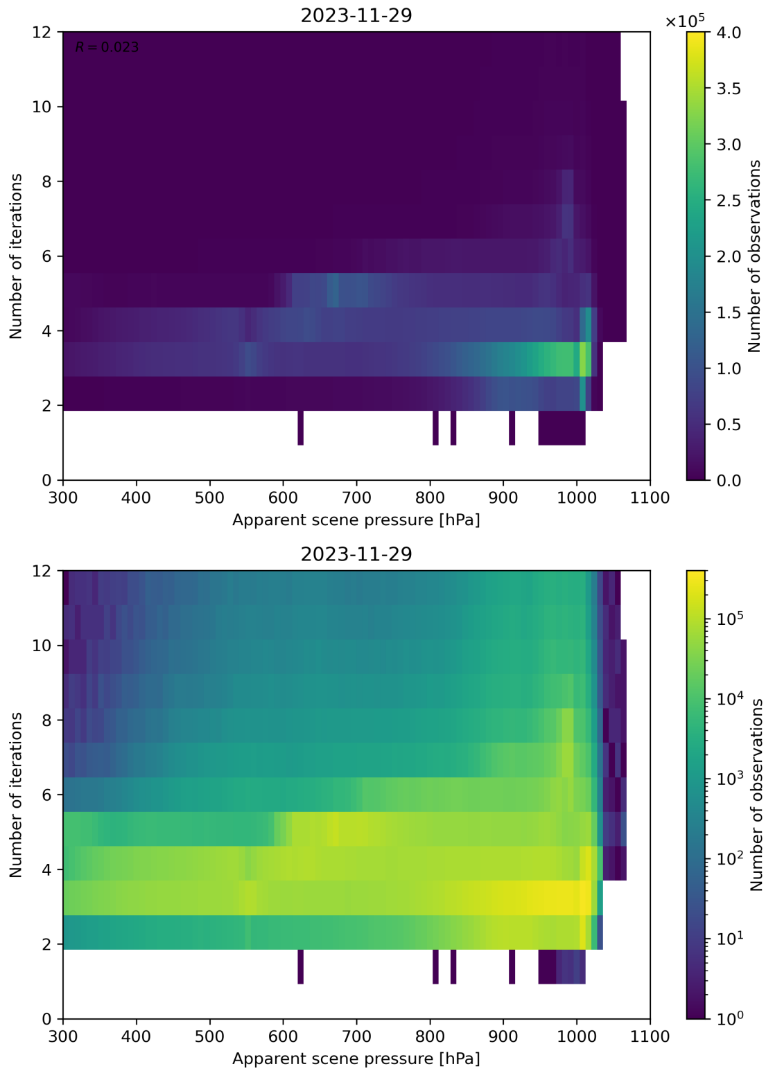
Figure 65: Scatter density plot of “Apparent scene pressure” against “Number of iterations” for 2023-11-28 to 2023-11-30.
