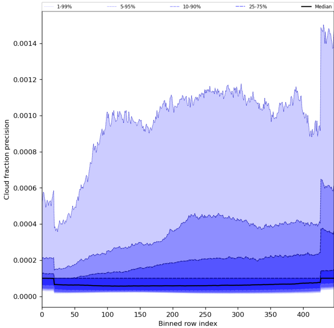
Figure 50: Along track statistics of “Cloud fraction precision” for 2023-11-28 to 2023-11-30
