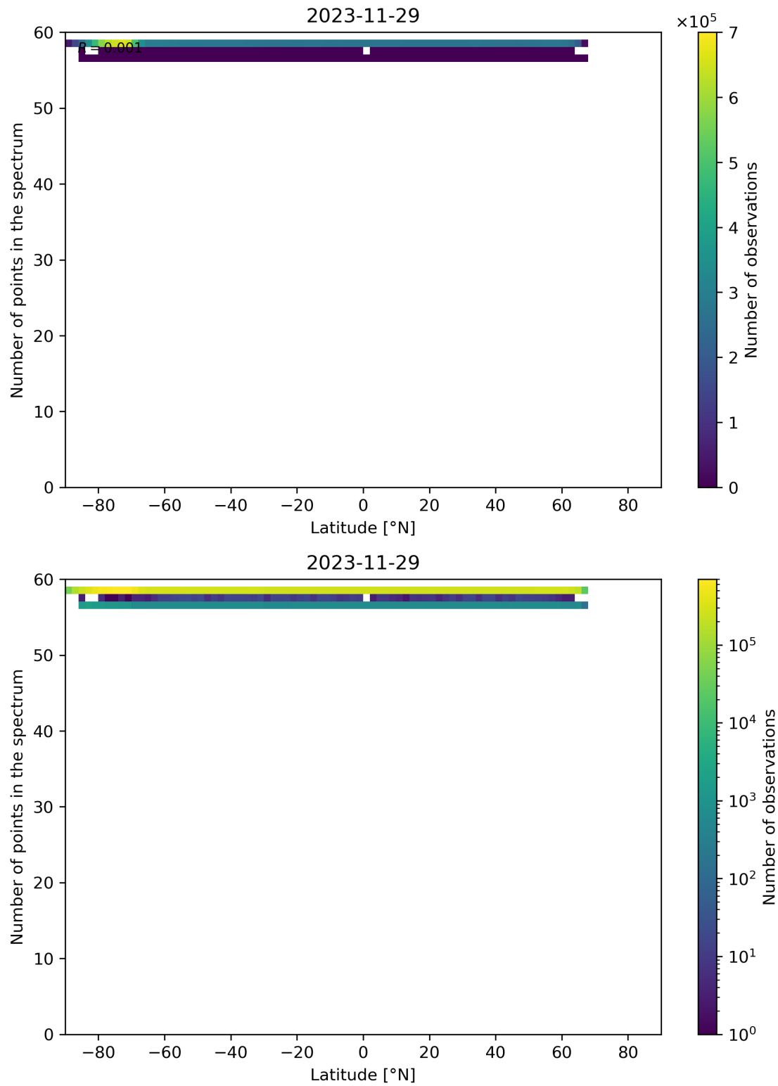
Figure 94: Scatter density plot of “Latitude” against “Number of points in the spectrum” for 2023-11-28 to 2023-11-30.
