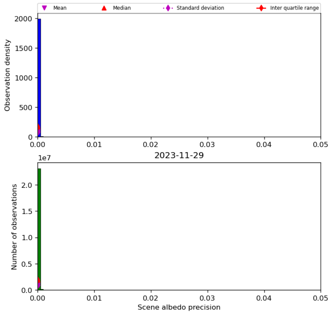
Figure 35: Histogram of “Scene albedo precision” for 2023-11-28 to 2023-11-30
