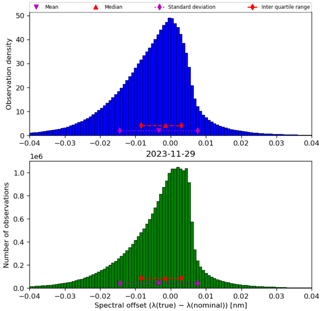
Figure 45: Histogram of “Spectral offset ( \lambda(\text{true}) - \lambda(\text{nominal}) )” for 2023-11-28 to 2023-11-30
