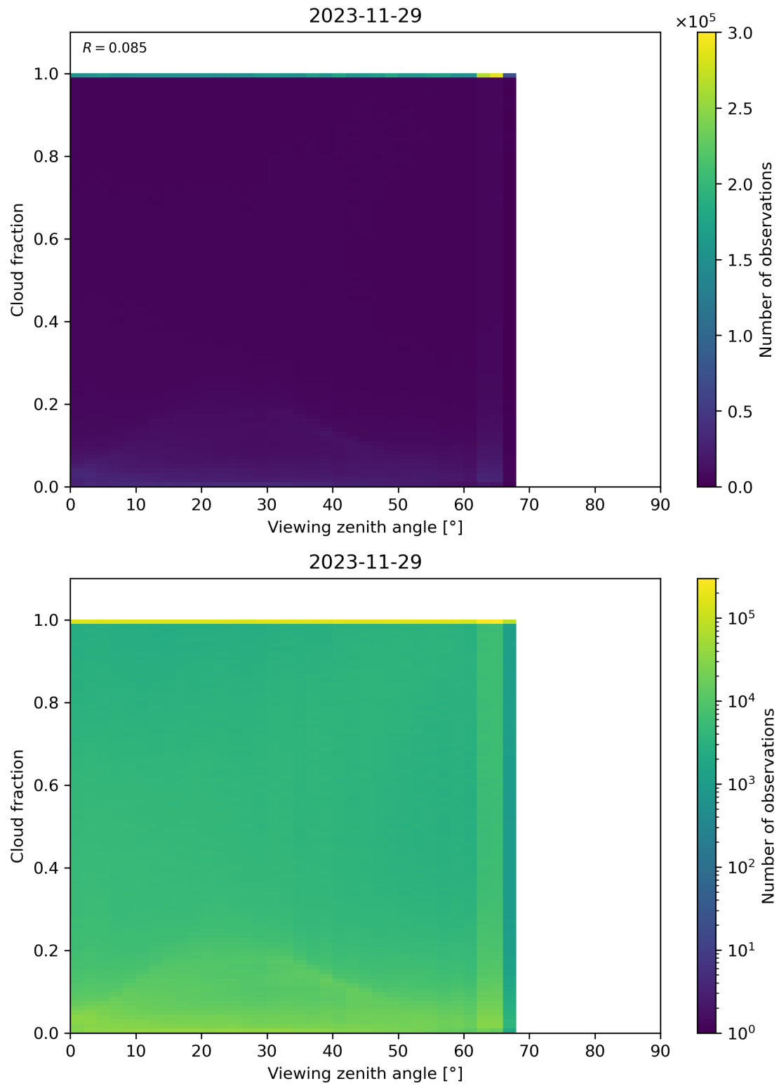
Figure 120: Scatter density plot of “Viewing zenith angle” against “Cloud fraction” for 2023-11-28 to 2023-11-30.
