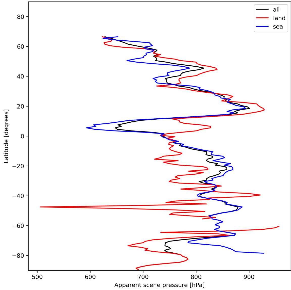
Figure 19: Zonal average of “Apparent scene pressure” for 2023-11-28 to 2023-11-30.
