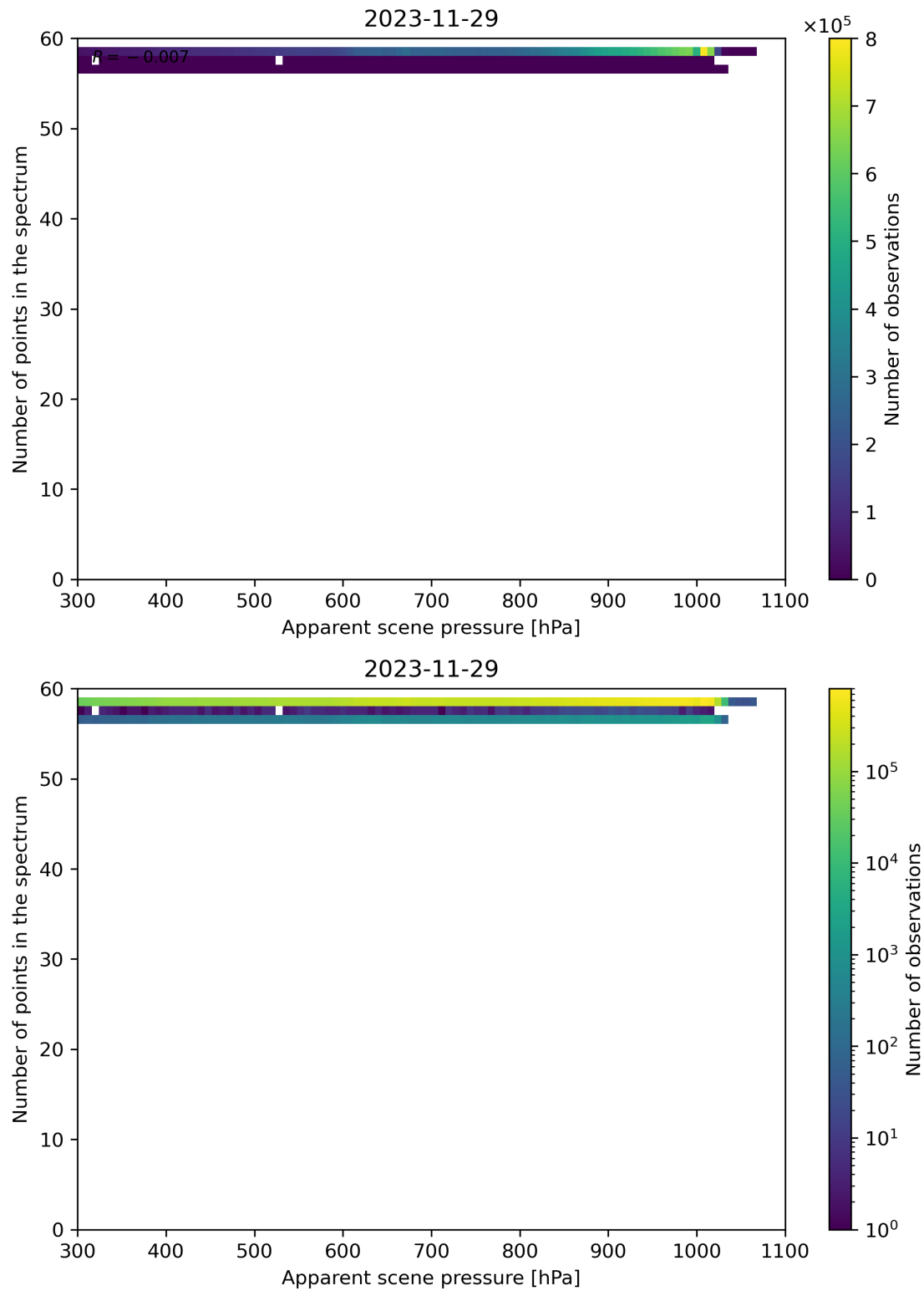
Figure 66: Scatter density plot of “Apparent scene pressure” against “Number of points in the spectrum” for 2023-11-28 to 2023-11-30.
