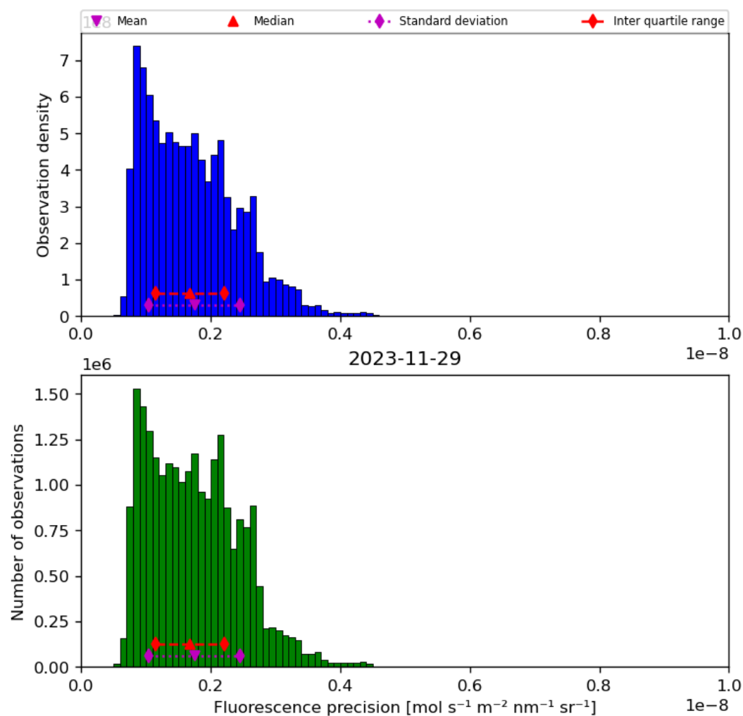
Figure 41: Histogram of “Fluorescence precision” for 2023-11-28 to 2023-11-30
