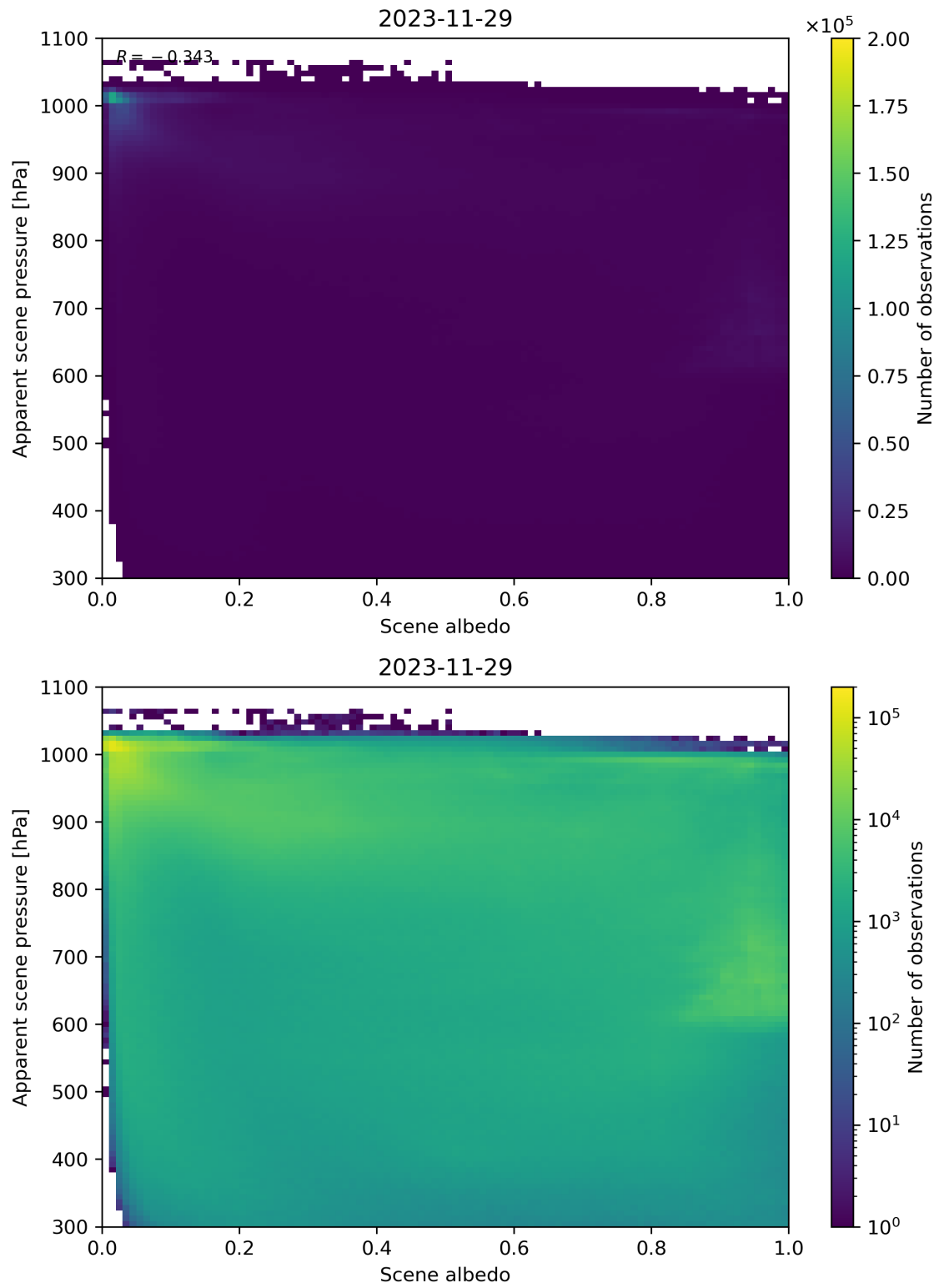
Figure 102: Scatter density plot of “Scene albedo” against “Apparent scene pressure” for 2023-11-28 to 2023-11-30.
