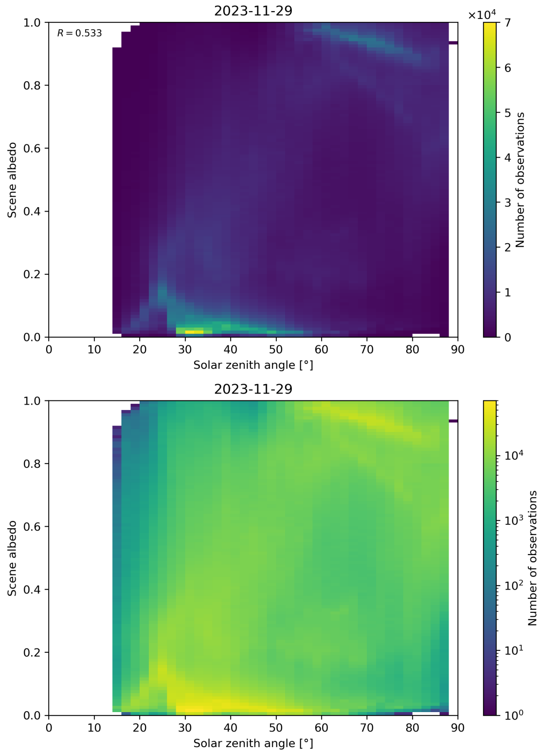
Figure 116: Scatter density plot of “Solar zenith angle” against “Scene albedo” for 2023-11-28 to 2023-11-30.
