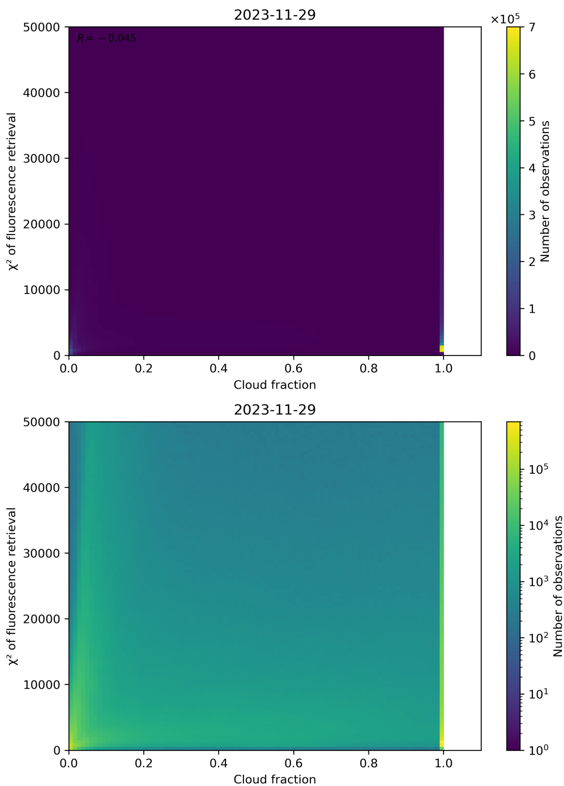
Figure 71: Scatter density plot of “Cloud fraction” against “ \chi^2 of fluorescence retrieval” for 2023-11-28 to 2023-11-30.
