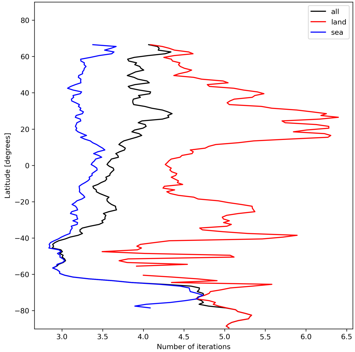
Figure 22: Zonal average of “Number of iterations” for 2023-11-28 to 2023-11-30.
