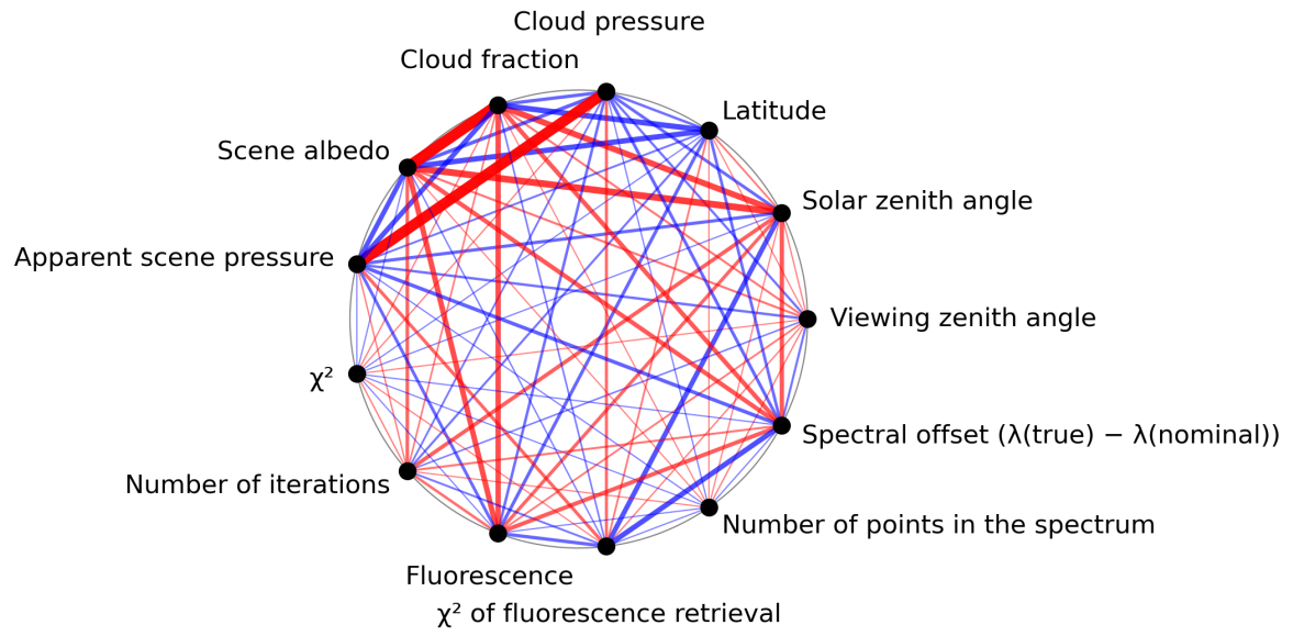
Figure 1: Map of correlation graph for 2023-11-28 to 2023-11-30.
