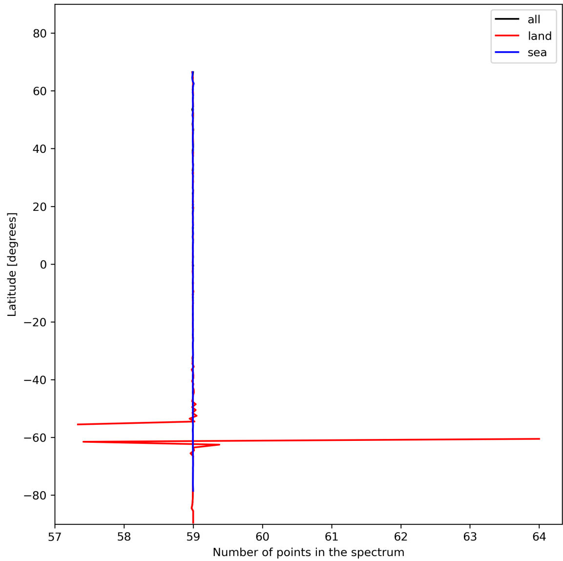
Figure 27: Zonal average of “Number of points in the spectrum” for 2023-11-28 to 2023-11-30.
