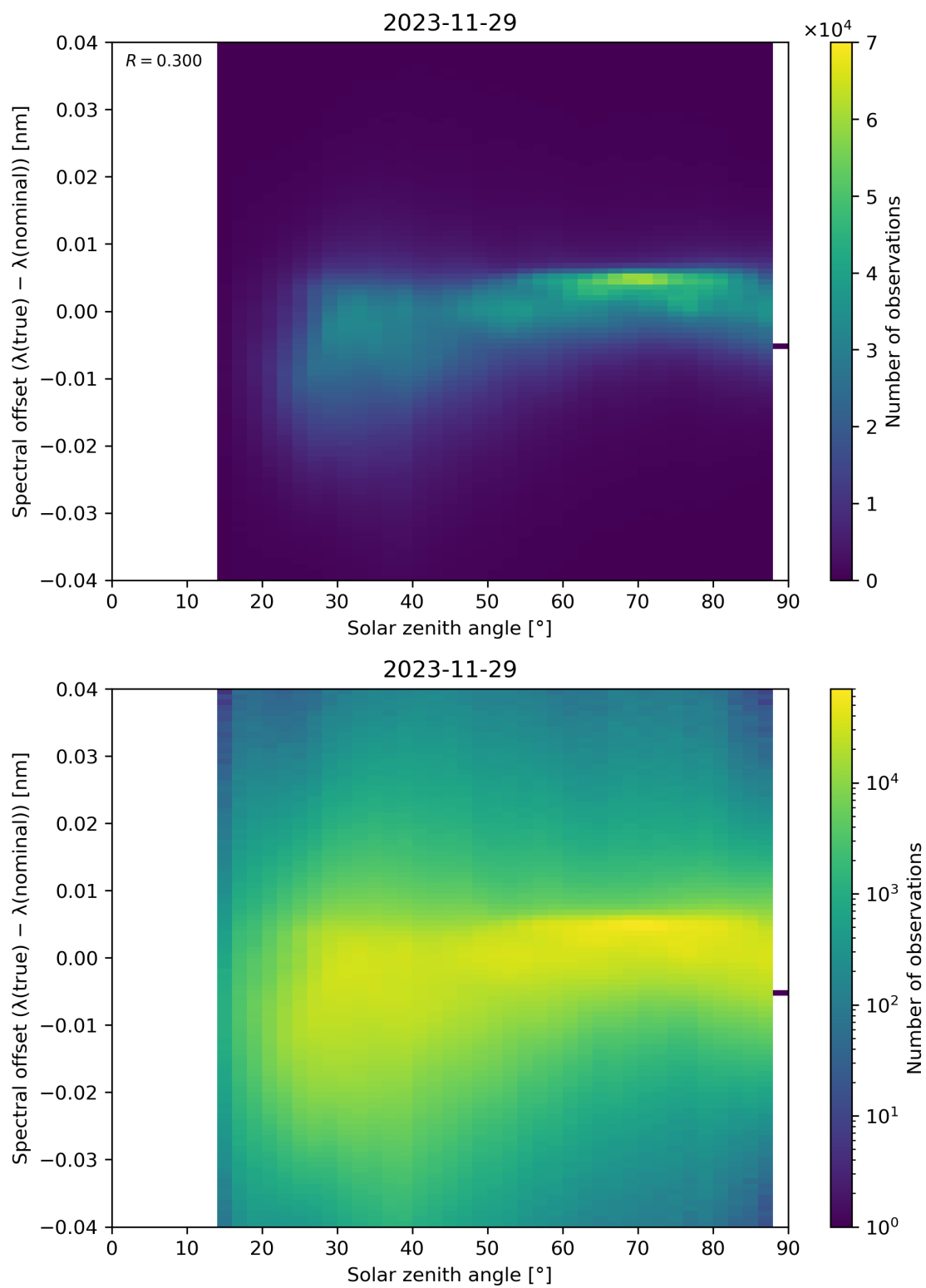
Figure 117: Scatter density plot of “Solar zenith angle” against “Spectral offset ( \lambda(\text{true}) - \lambda(\text{nominal}) )” for 2023-11-28 to 2023-11-30.
