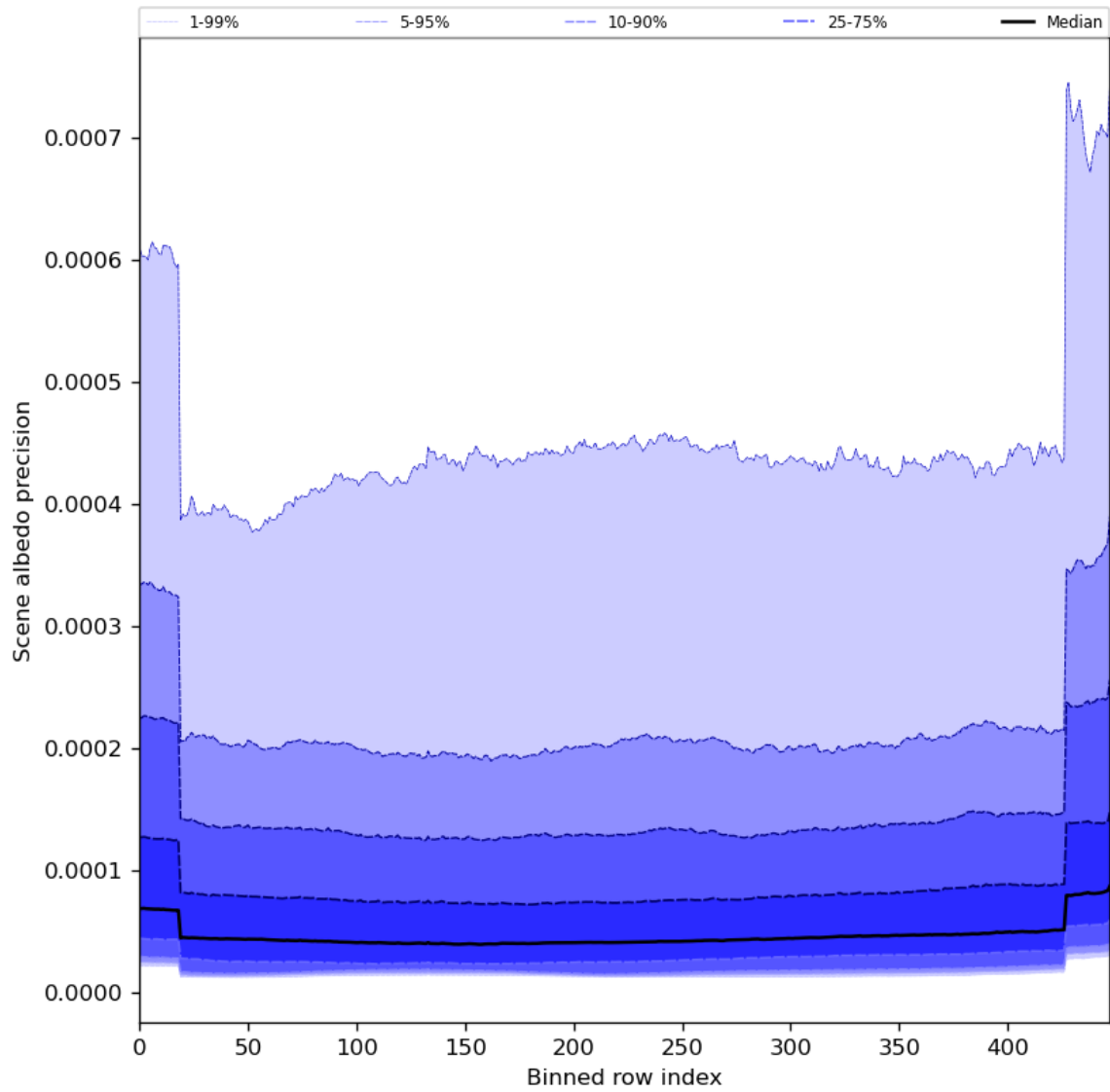
Figure 52: Along track statistics of “Scene albedo precision” for 2023-11-28 to 2023-11-30
