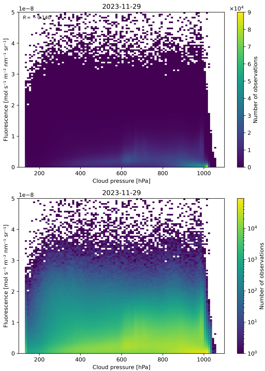
Figure 80: Scatter density plot of “Cloud pressure” against “Fluorescence” for 2023-11-28 to 2023-11-30.
