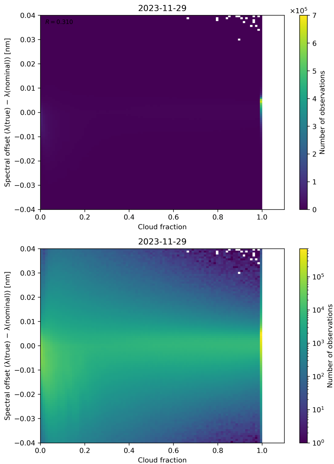
Figure 76: Scatter density plot of “Cloud fraction” against “Spectral offset ( \lambda(\text{true}) - \lambda(\text{nominal}) )” for 2023-11-28 to 2023-11-30.
