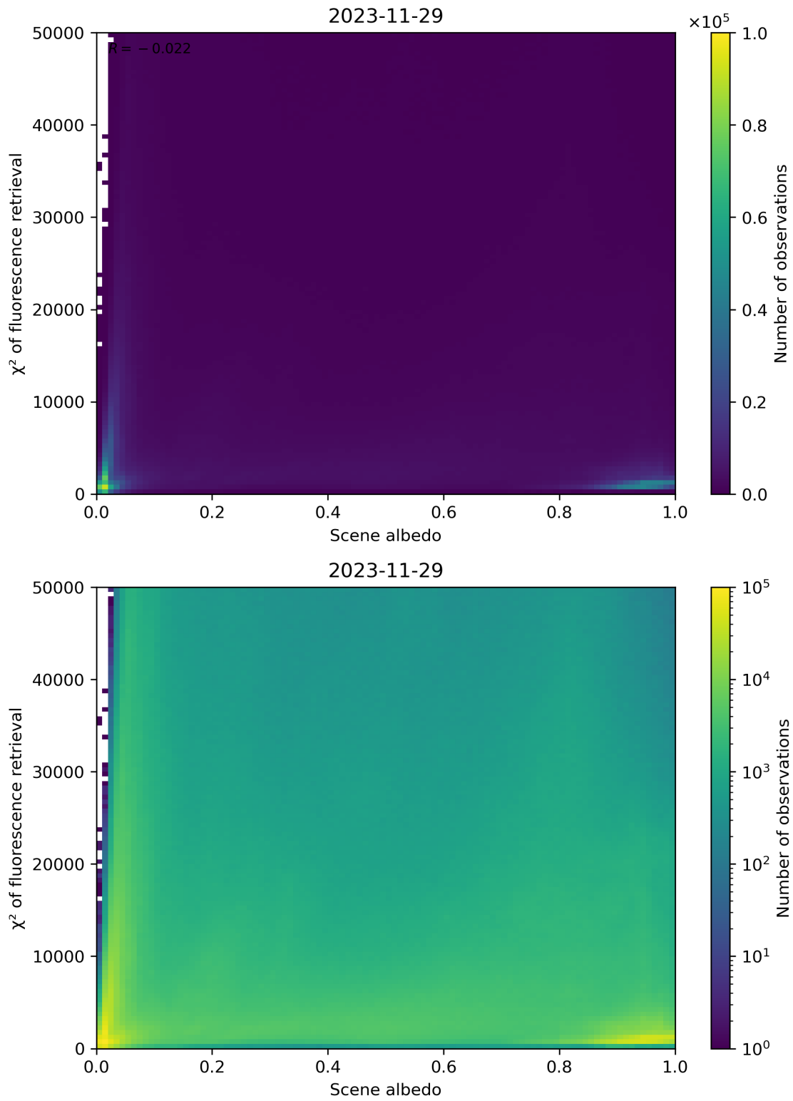
Figure 103: Scatter density plot of “Scene albedo” against “ \chi^2 of fluorescence retrieval” for 2023-11-28 to 2023-11-30.
