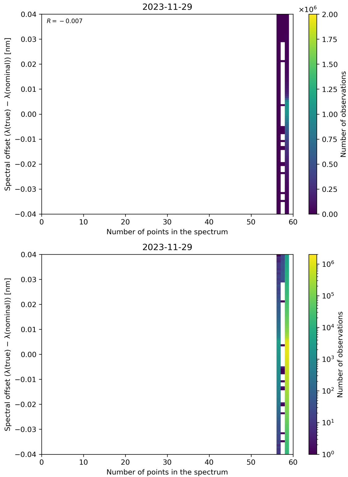
Figure 101: Scatter density plot of “Number of points in the spectrum” against “Spectral offset ( \lambda(\text{true}) - \lambda(\text{nominal}) )” for 2023-11-28 to 2023-11-30.
