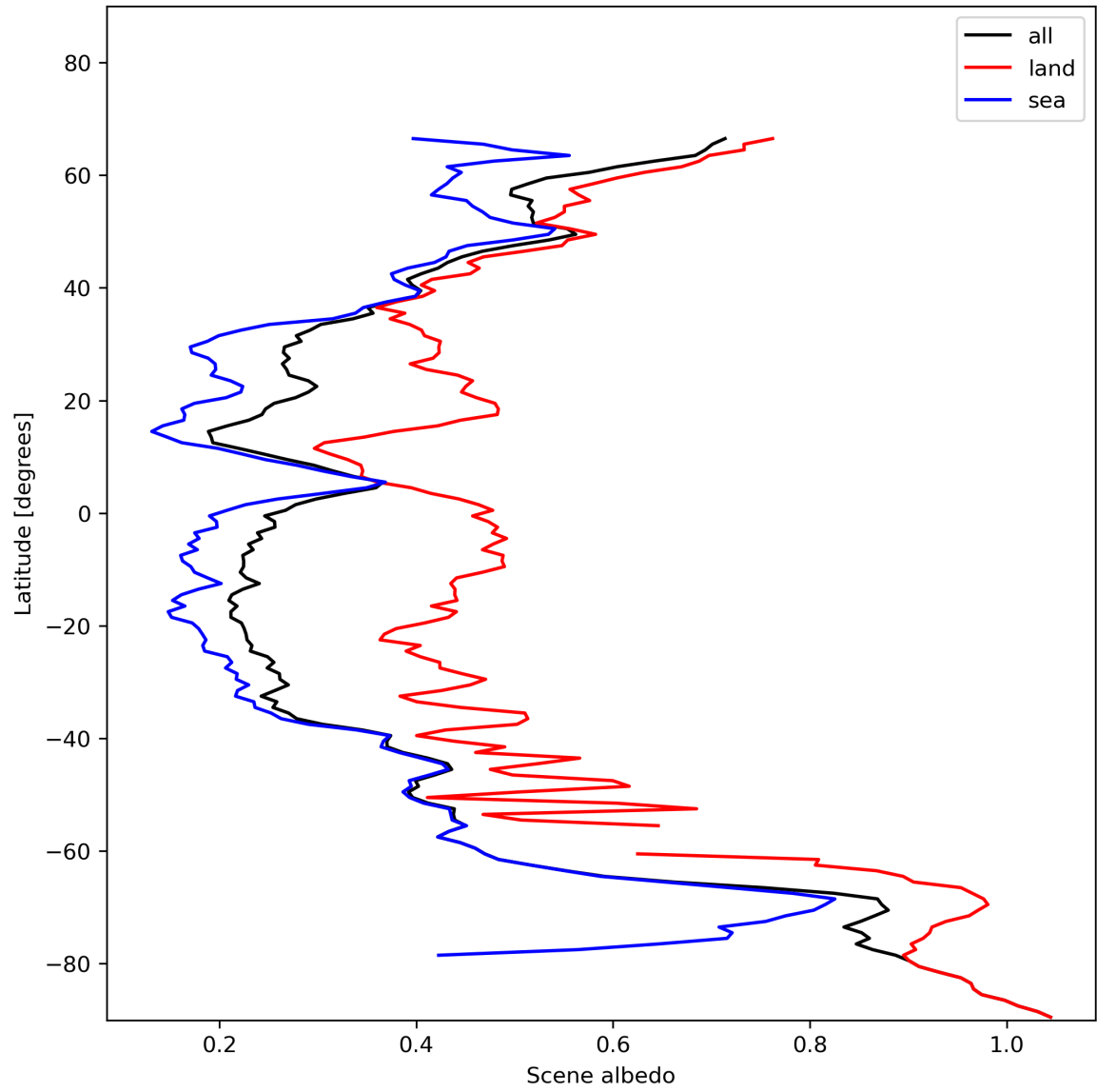
Figure 17: Zonal average of “Scene albedo” for 2023-11-28 to 2023-11-30.
