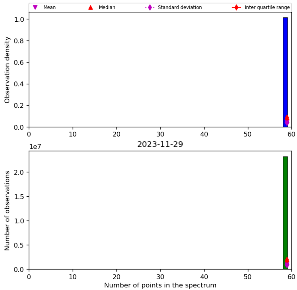
Figure 44: Histogram of “Number of points in the spectrum” for 2023-11-28 to 2023-11-30
