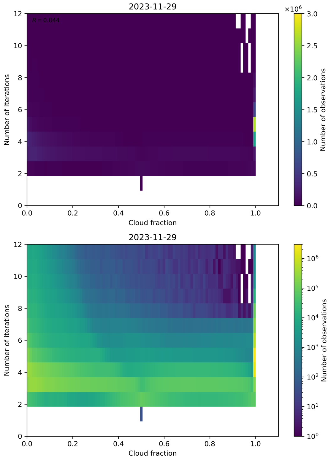
Figure 73: Scatter density plot of “Cloud fraction” against “Number of iterations” for 2023-11-28 to 2023-11-30.
