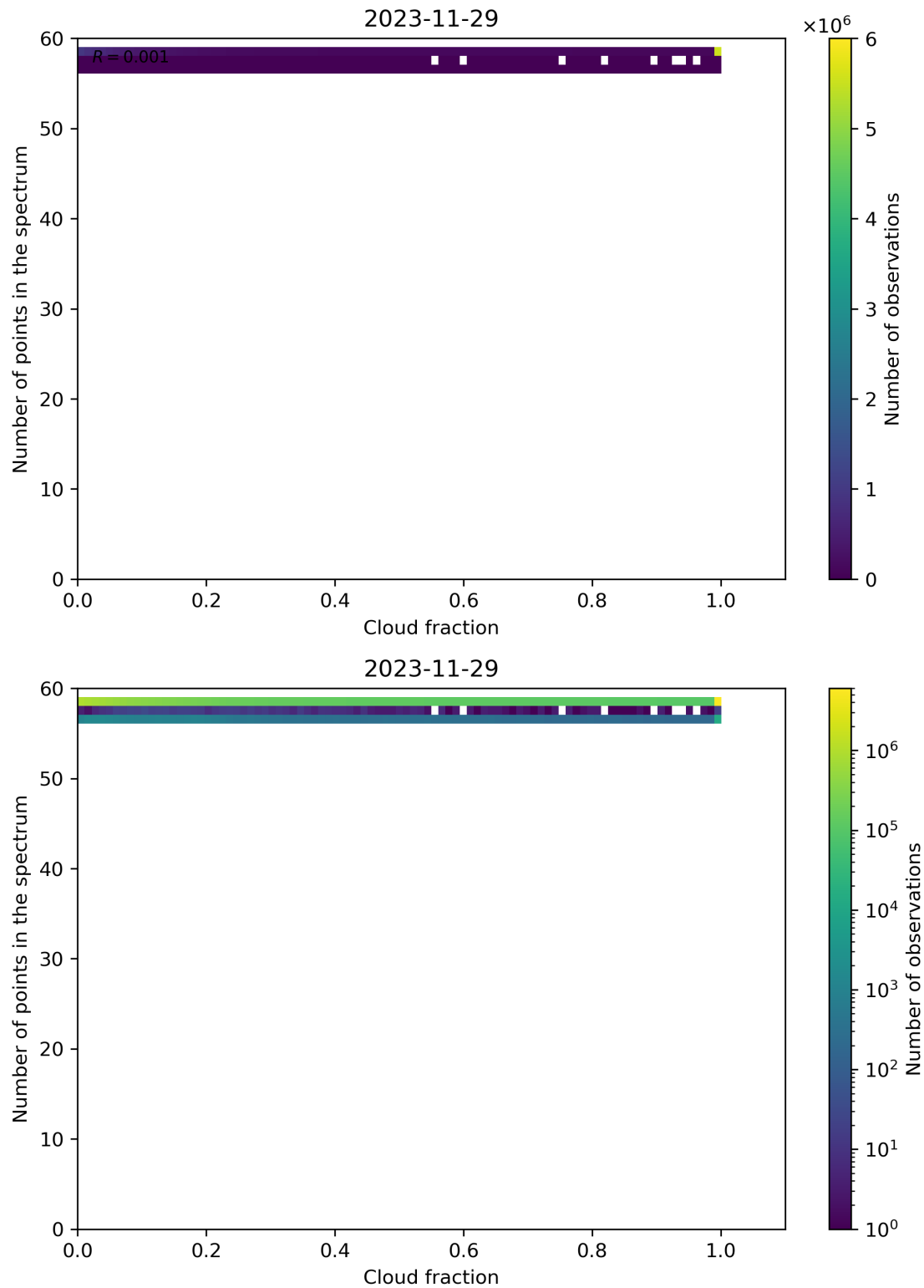
Figure 74: Scatter density plot of “Cloud fraction” against “Number of points in the spectrum” for 2023-11-28 to 2023-11-30.
