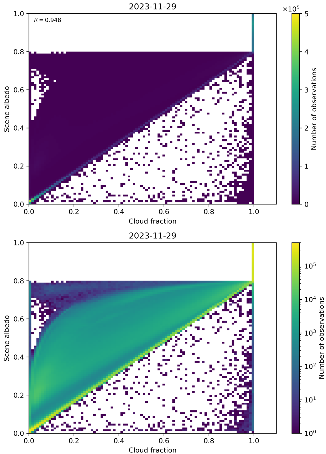
Figure 75: Scatter density plot of “Cloud fraction” against “Scene albedo” for 2023-11-28 to 2023-11-30.
