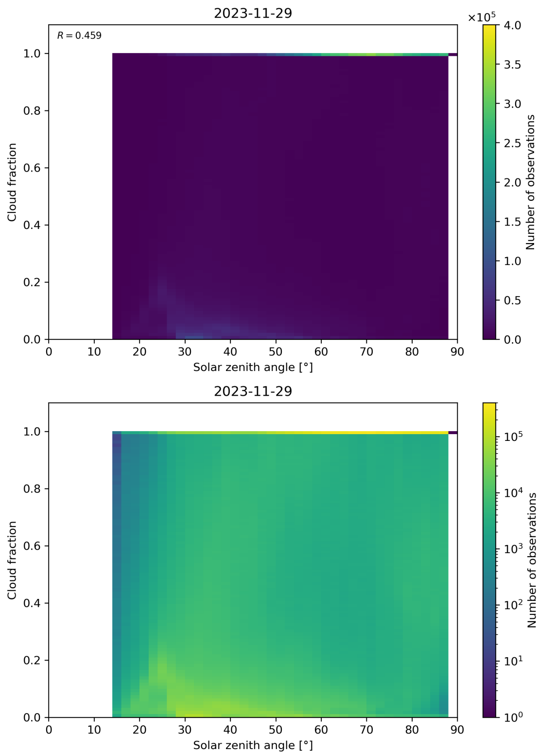
Figure 110: Scatter density plot of “Solar zenith angle” against “Cloud fraction” for 2023-11-28 to 2023-11-30.
