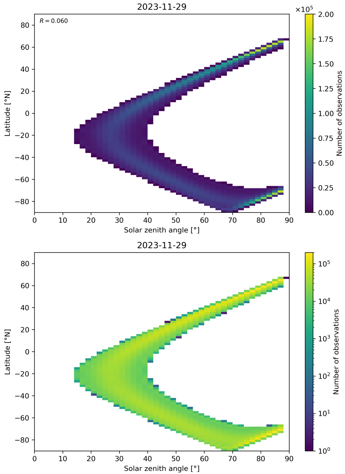
Figure 113: Scatter density plot of “Solar zenith angle” against “Latitude” for 2023-11-28 to 2023-11-30.
