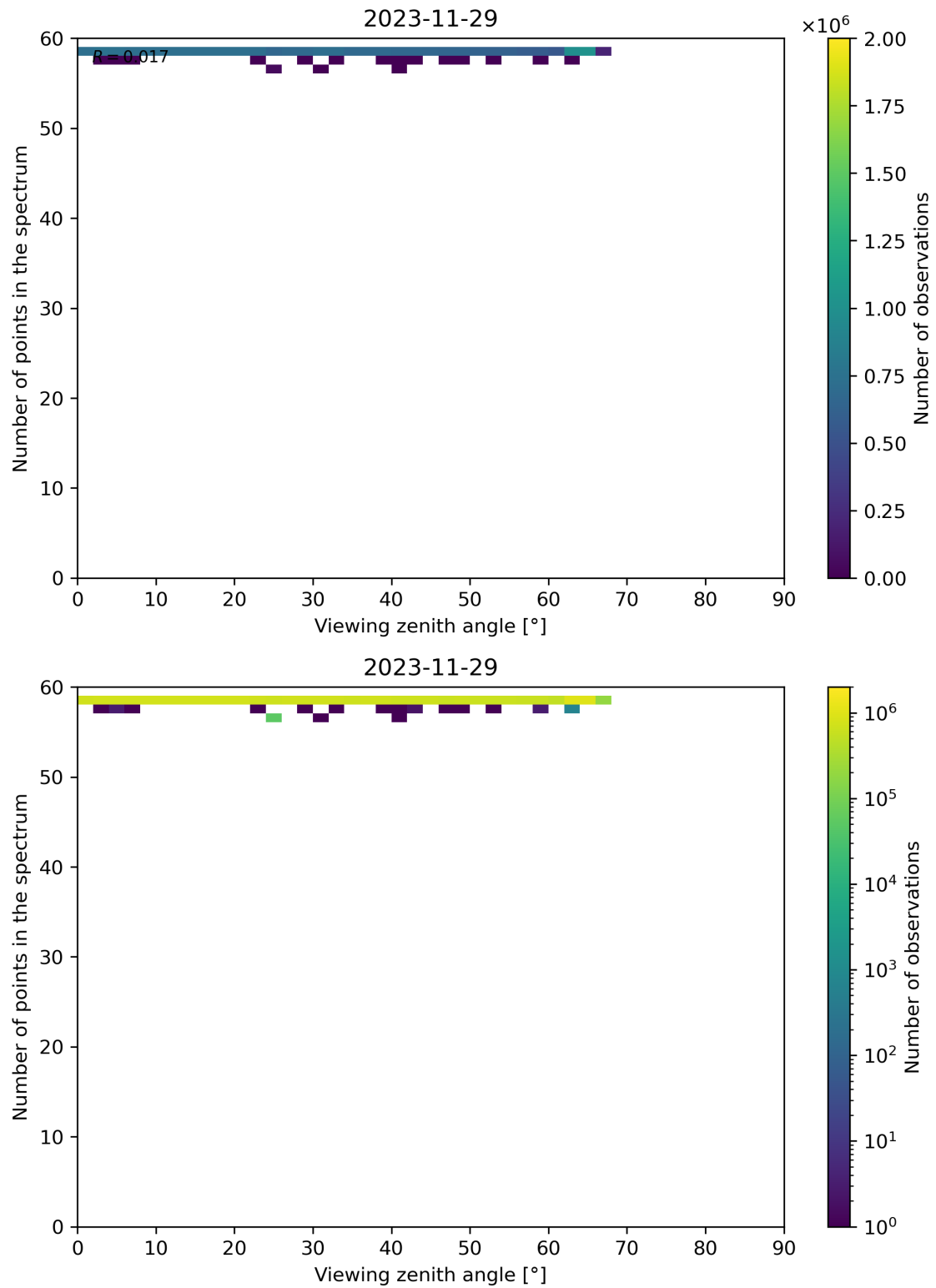
Figure 125: Scatter density plot of “Viewing zenith angle” against “Number of points in the spectrum” for 2023-11-28 to 2023-11-30.
