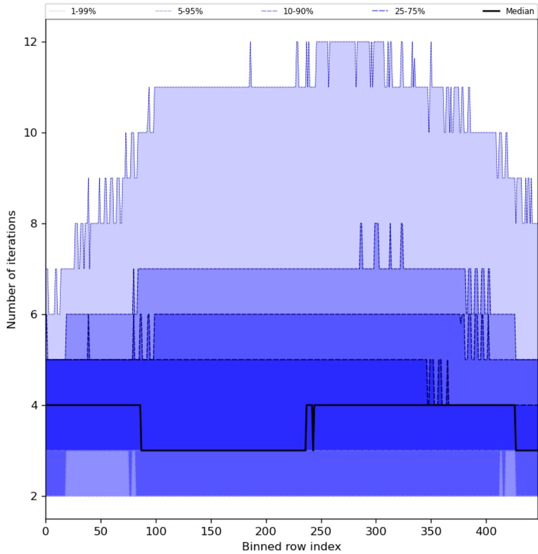
Figure 56: Along track statistics of “Number of iterations” for 2023-11-28 to 2023-11-30
