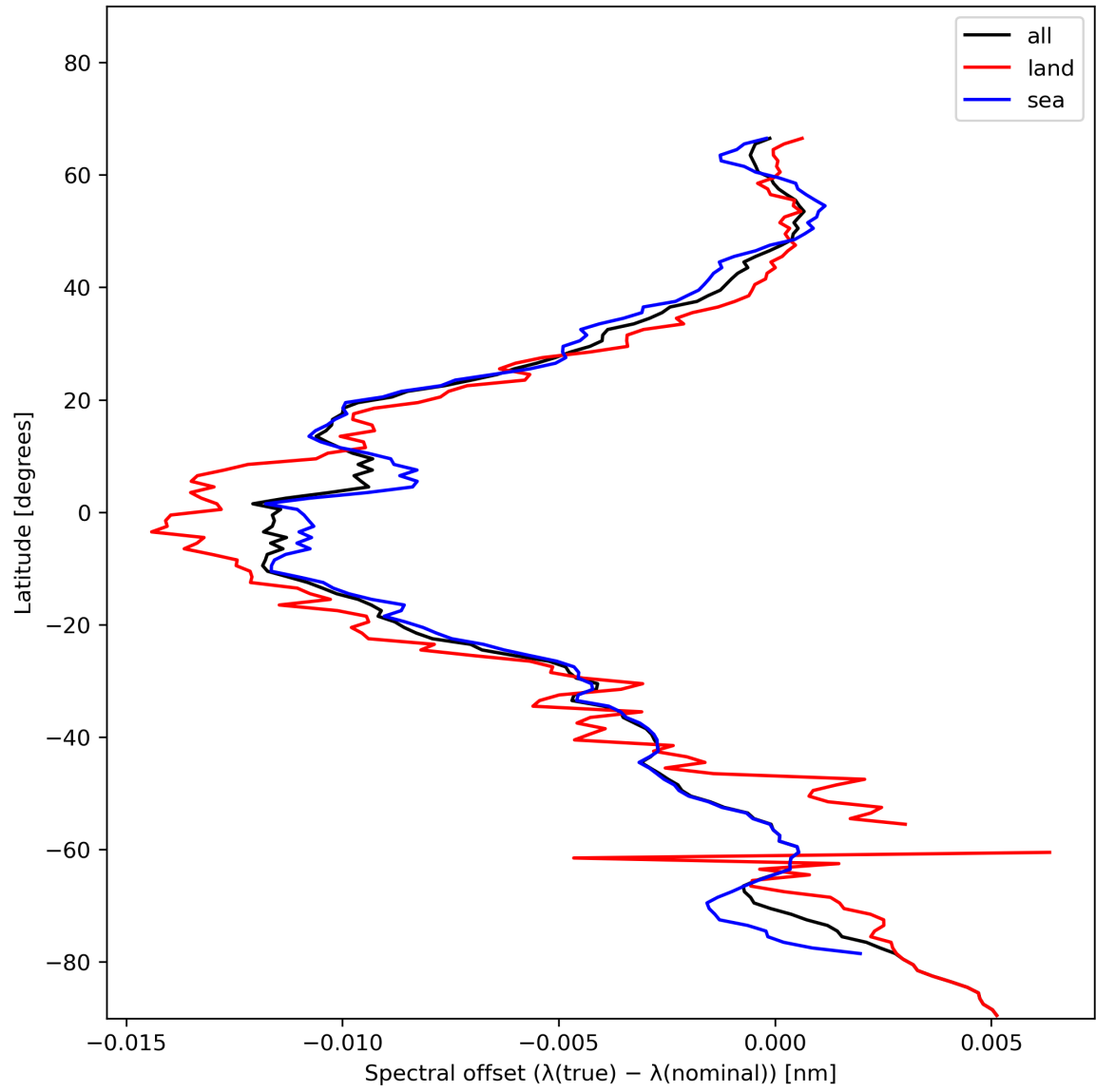
Figure 28: Zonal average of “Spectral offset ( \lambda(\text{true}) - \lambda(\text{nominal}) )” for 2023-11-28 to 2023-11-30.
