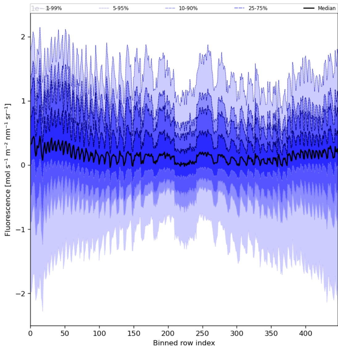
Figure 57: Along track statistics of “Fluorescence” for 2023-11-28 to 2023-11-30
