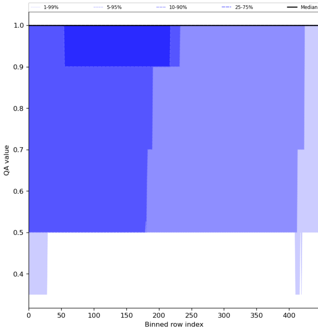
Figure 46: Along track statistics of “QA value” for 2023-11-28 to 2023-11-30
