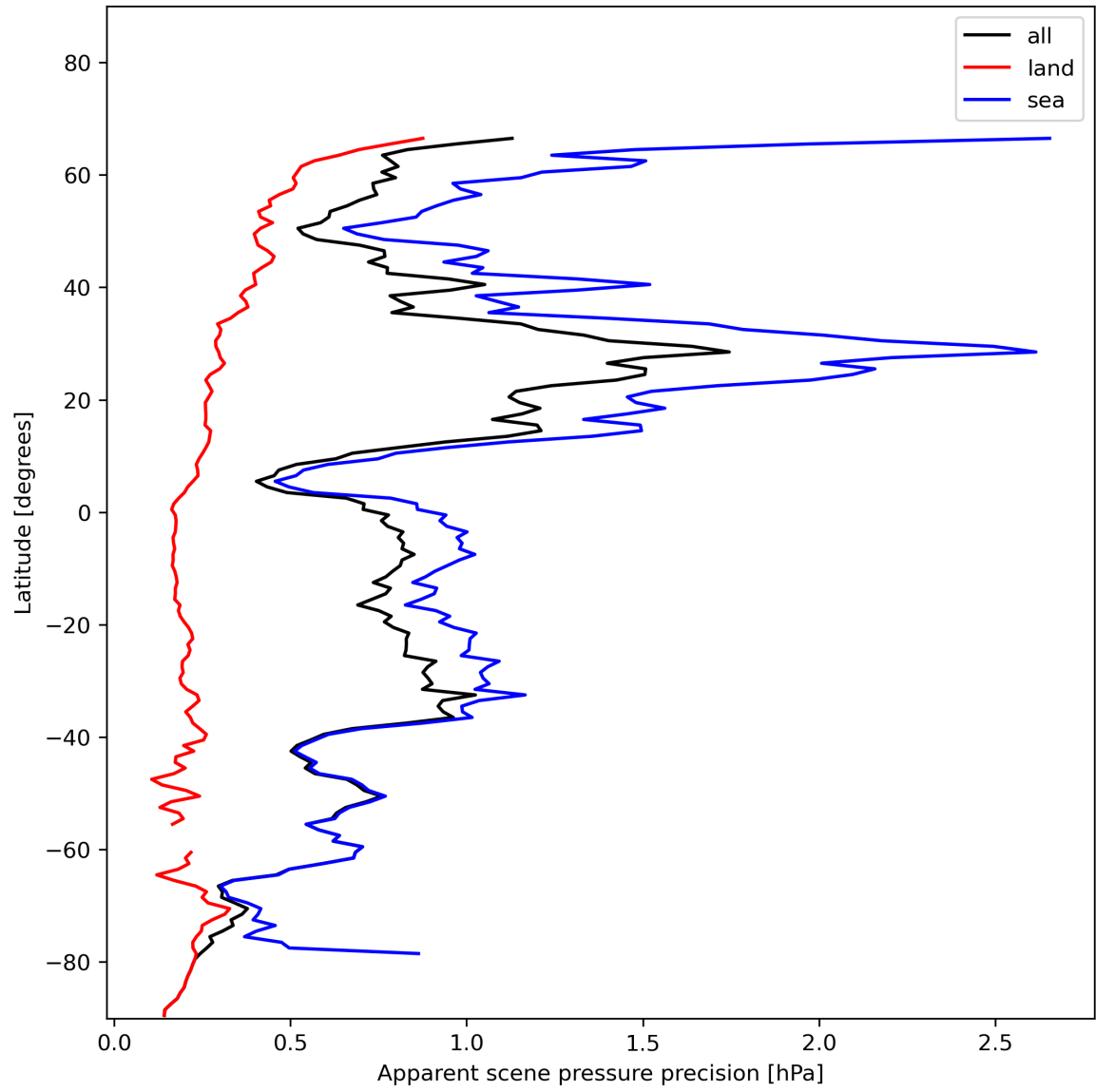
Figure 20: Zonal average of “Apparent scene pressure precision” for 2023-11-28 to 2023-11-30.
