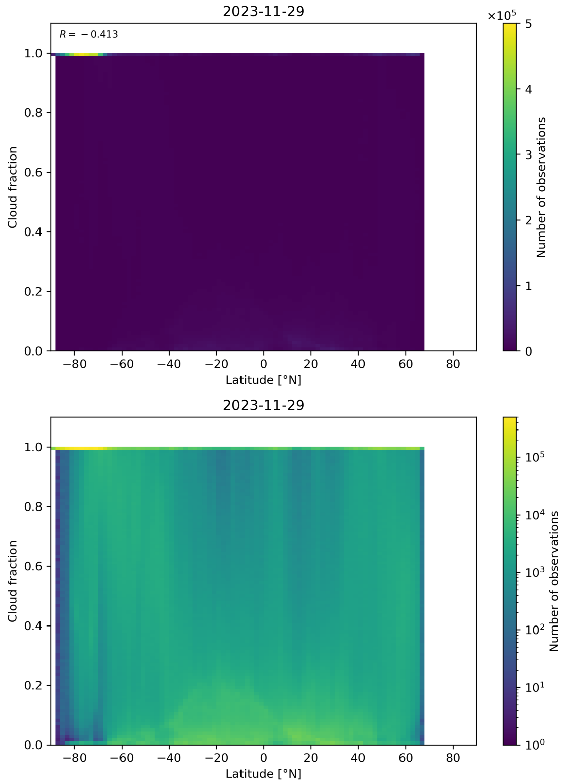
Figure 90: Scatter density plot of “Latitude” against “Cloud fraction” for 2023-11-28 to 2023-11-30.
