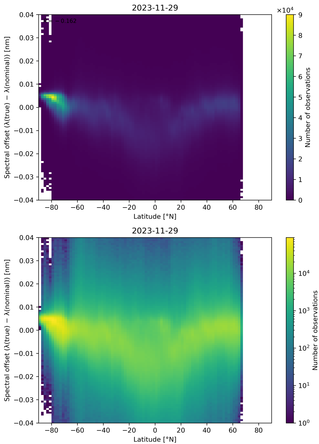
Figure 96: Scatter density plot of “Latitude” against “Spectral offset ( \lambda(\text{true}) - \lambda(\text{nominal}) )” for 2023-11-28 to 2023-11-30.
