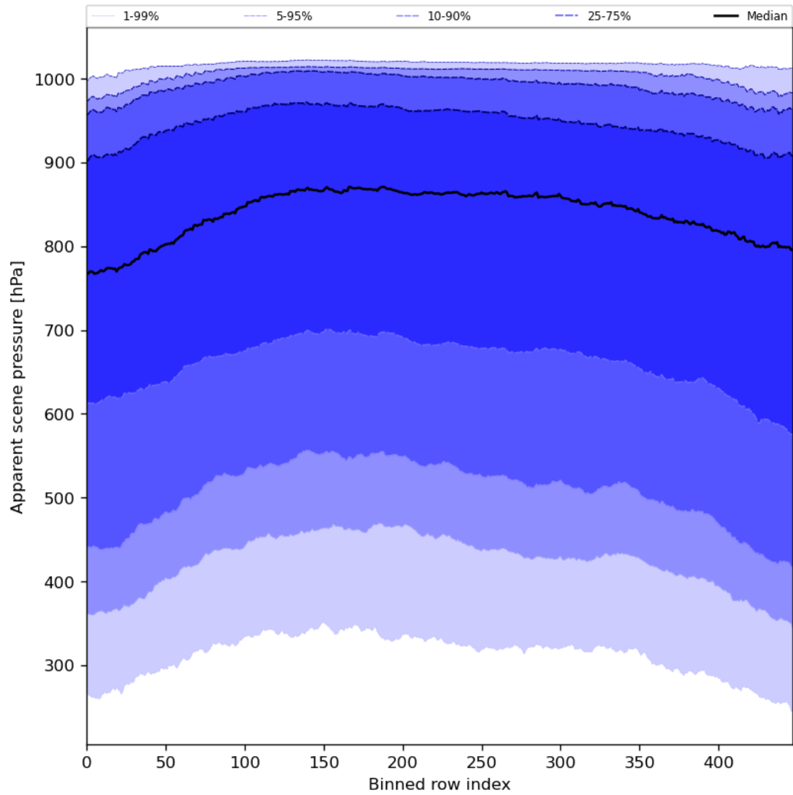
Figure 53: Along track statistics of “Apparent scene pressure” for 2023-11-28 to 2023-11-30
