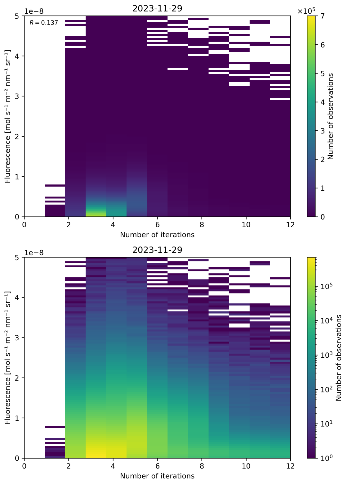
Figure 98: Scatter density plot of “Number of iterations” against “Fluorescence” for 2023-11-28 to 2023-11-30.
