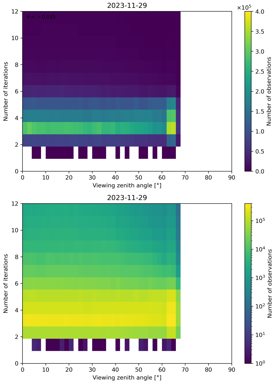
Figure 124: Scatter density plot of “Viewing zenith angle” against “Number of iterations” for 2023-11-28 to 2023-11-30.
