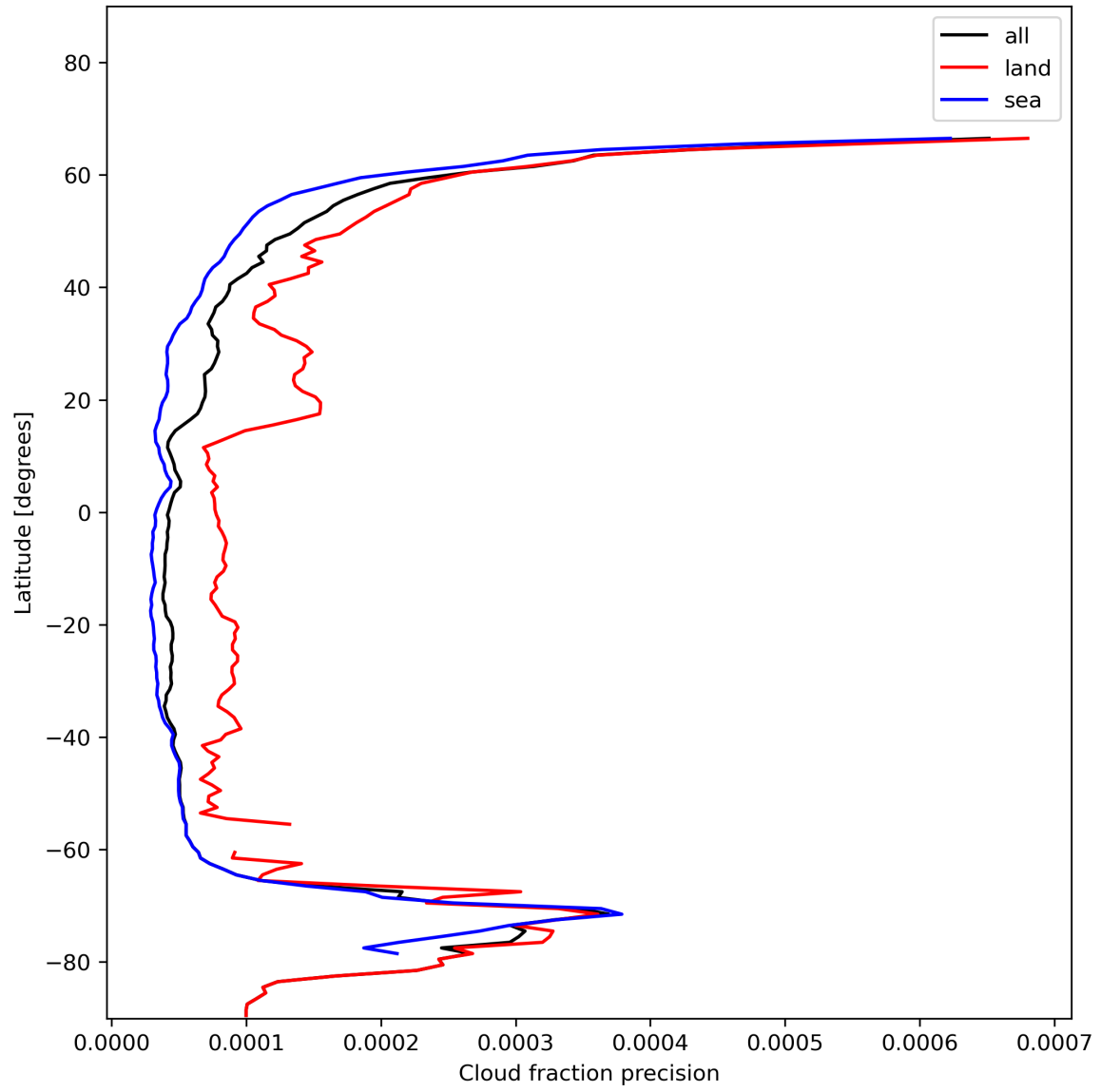
Figure 16: Zonal average of “Cloud fraction precision” for 2023-11-28 to 2023-11-30.
