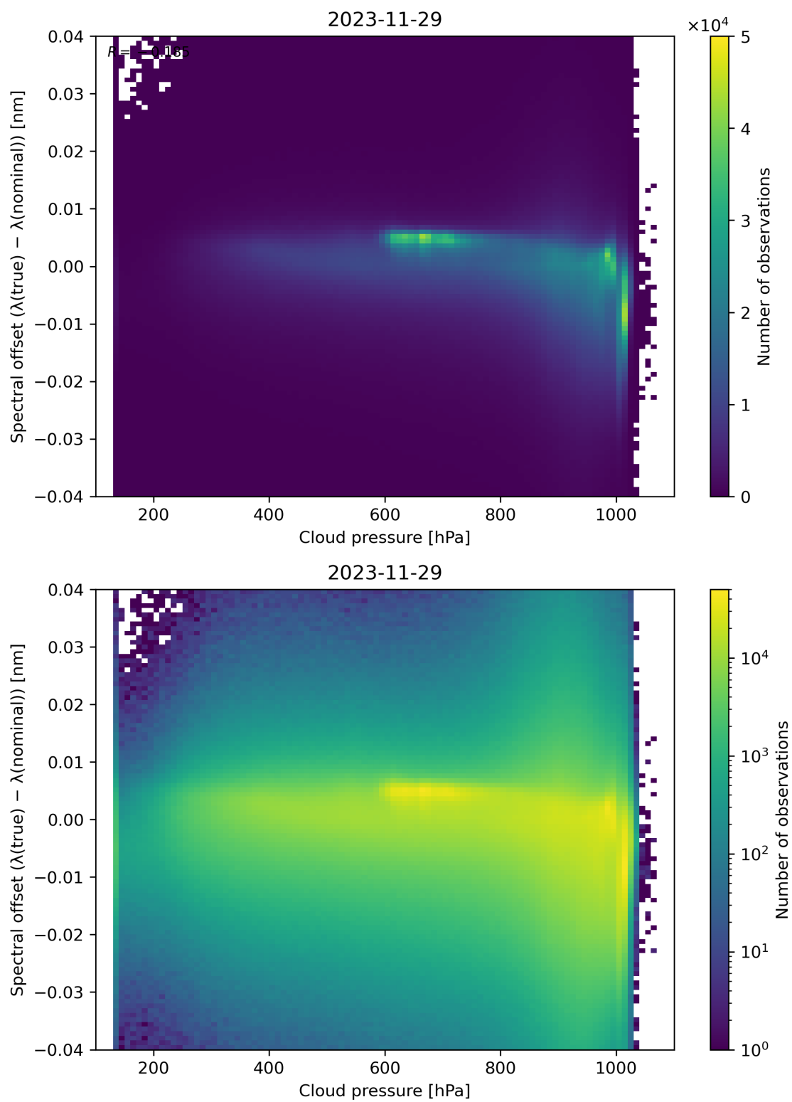
Figure 84: Scatter density plot of “Cloud pressure” against “Spectral offset ( \lambda(\text{true}) - \lambda(\text{nominal}) )” for 2023-11-28 to 2023-11-30.
