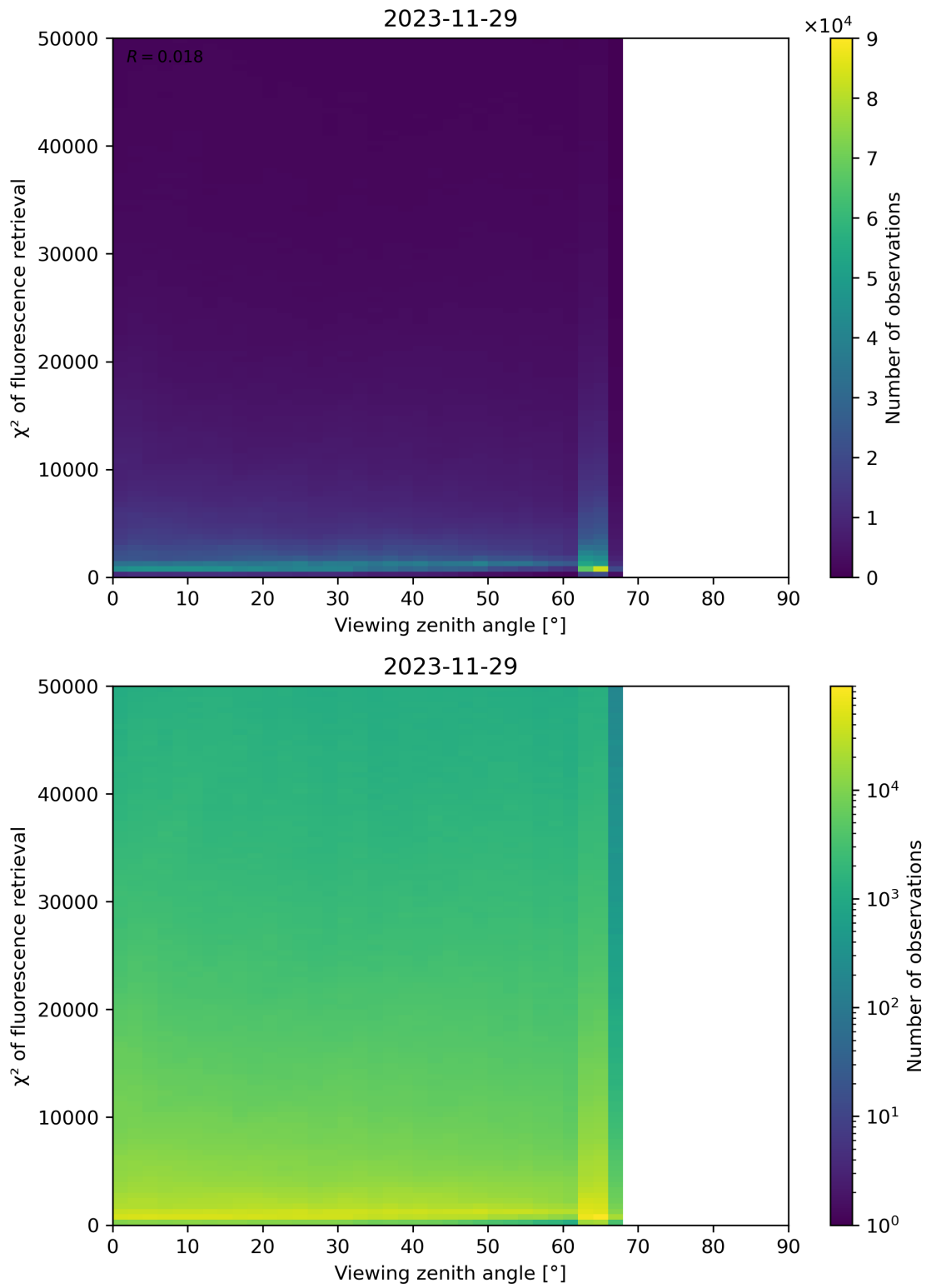
Figure 119: Scatter density plot of “Viewing zenith angle” against “ \chi^2 of fluorescence retrieval” for 2023-11-28 to 2023-11-30.
