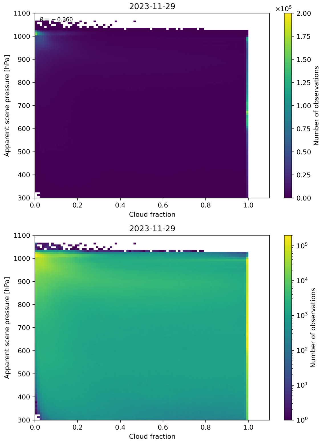
Figure 70: Scatter density plot of “Cloud fraction” against “Apparent scene pressure” for 2023-11-28 to 2023-11-30.
