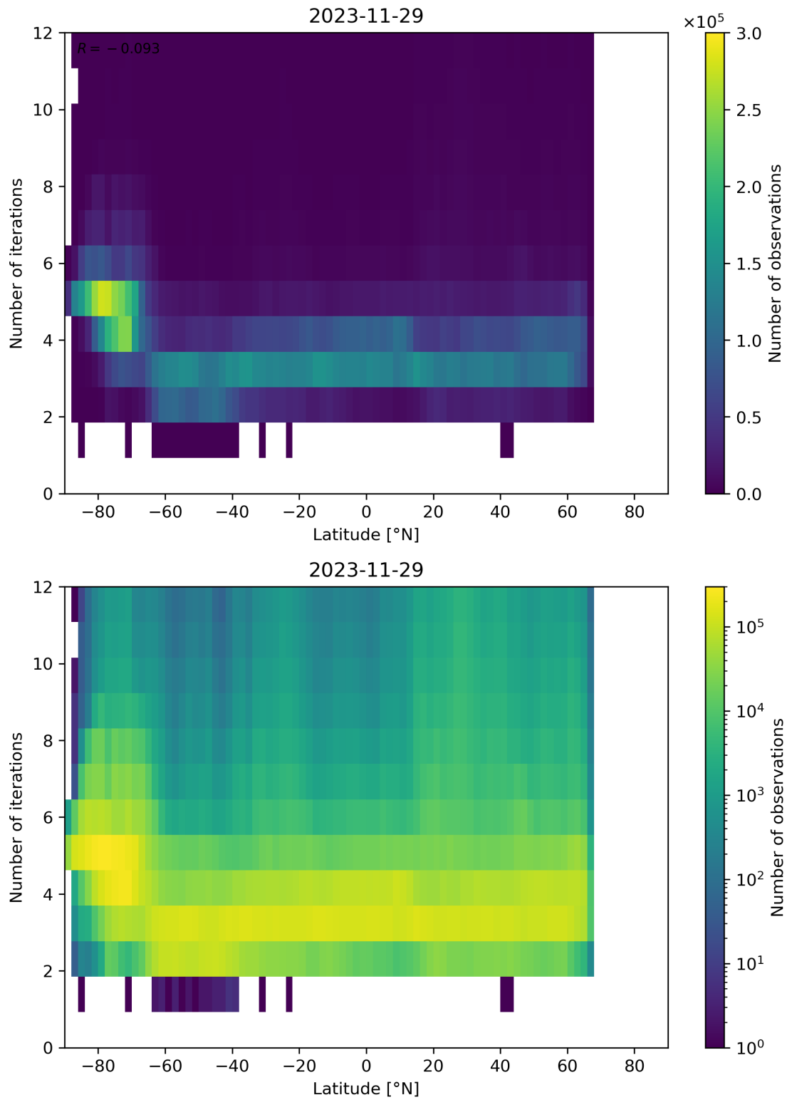
Figure 93: Scatter density plot of “Latitude” against “Number of iterations” for 2023-11-28 to 2023-11-30.
