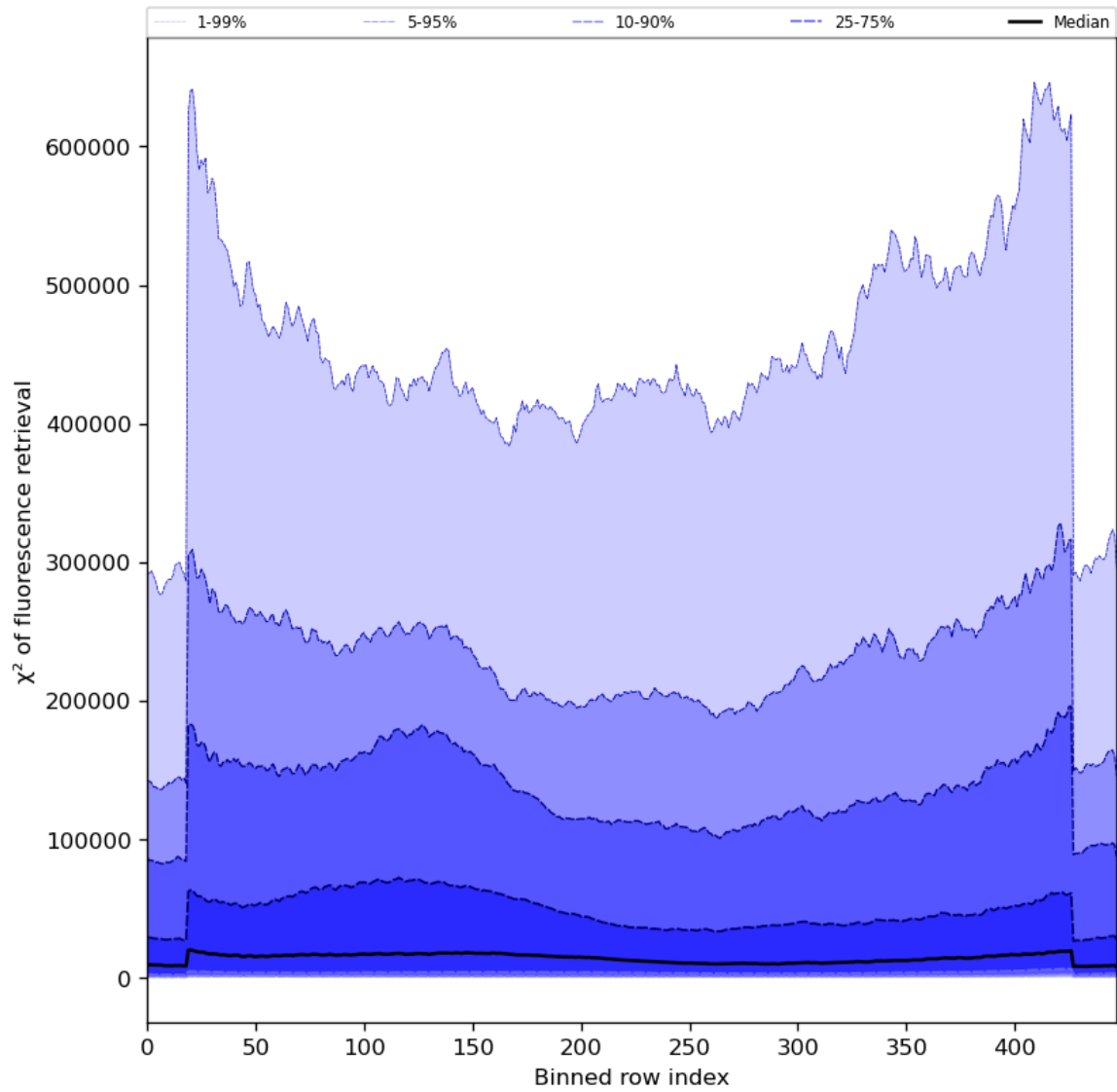
Figure 59: Along track statistics of " \chi^2 of fluorescence retrieval" for 2023-11-28 to 2023-11-30
