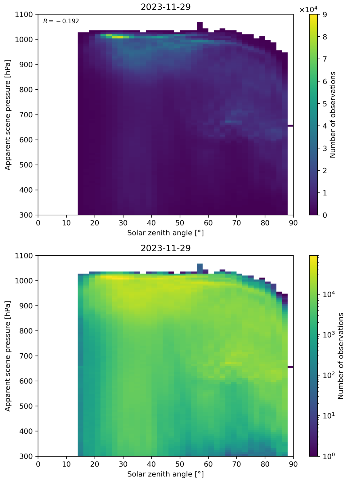
Figure 108: Scatter density plot of “Solar zenith angle” against “Apparent scene pressure” for 2023-11-28 to 2023-11-30.
