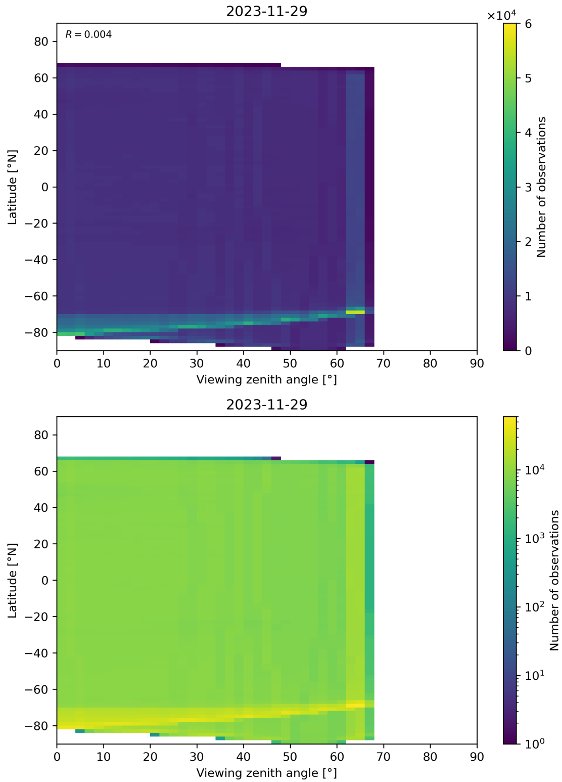
Figure 123: Scatter density plot of “Viewing zenith angle” against “Latitude” for 2023-11-28 to 2023-11-30.
