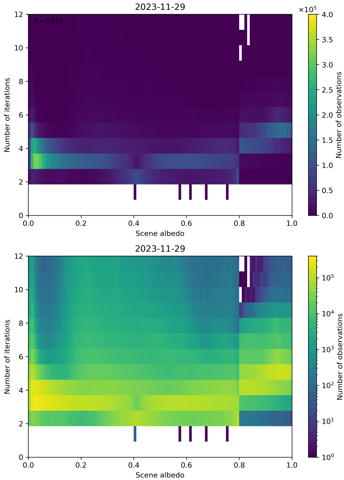
Figure 105: Scatter density plot of “Scene albedo” against “Number of iterations” for 2023-11-28 to 2023-11-30.
