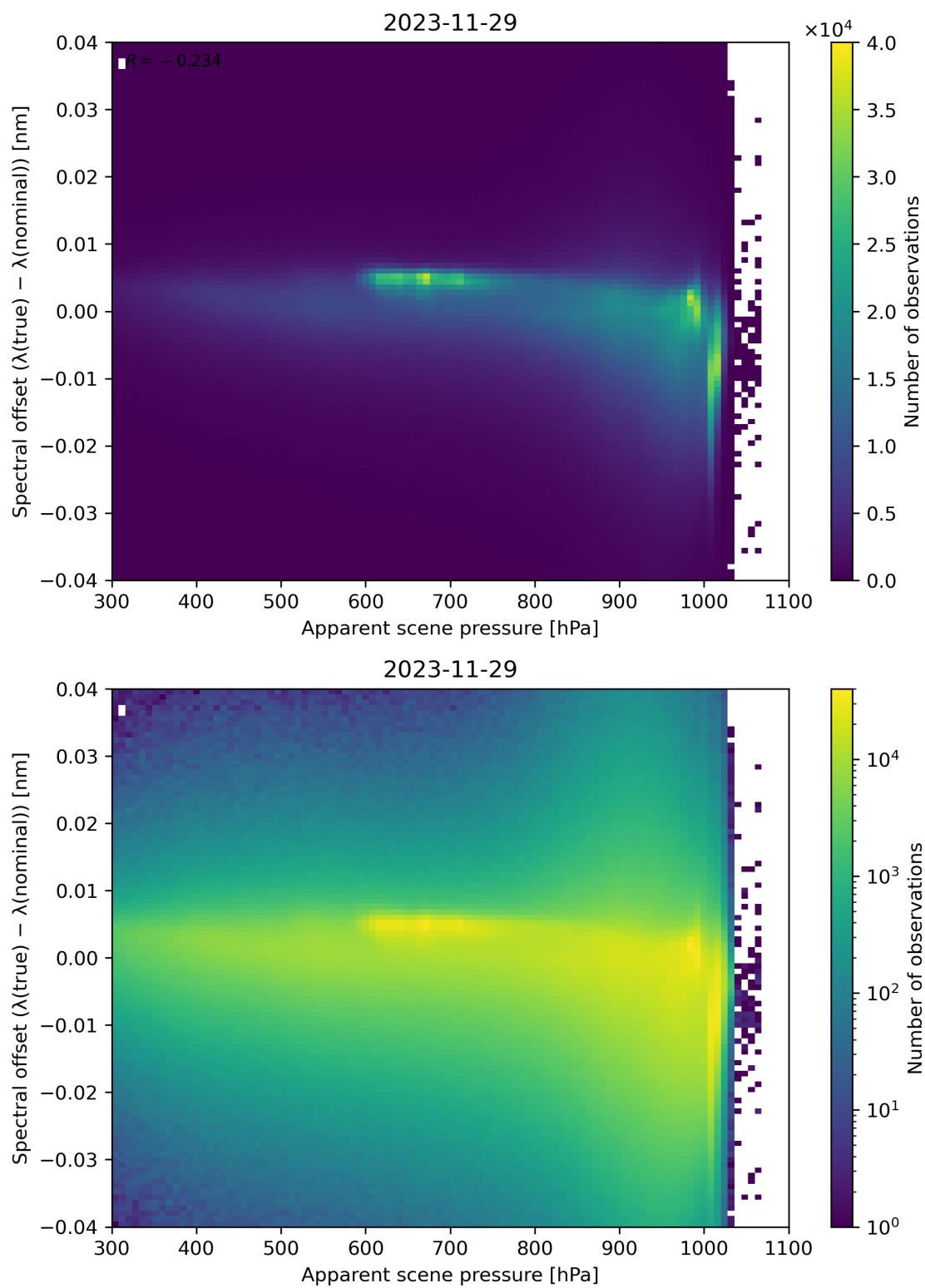
Figure 67: Scatter density plot of “Apparent scene pressure” against “Spectral offset ( \lambda(\text{true}) - \lambda(\text{nominal}) )” for 2023-11-28 to 2023-11-30.
