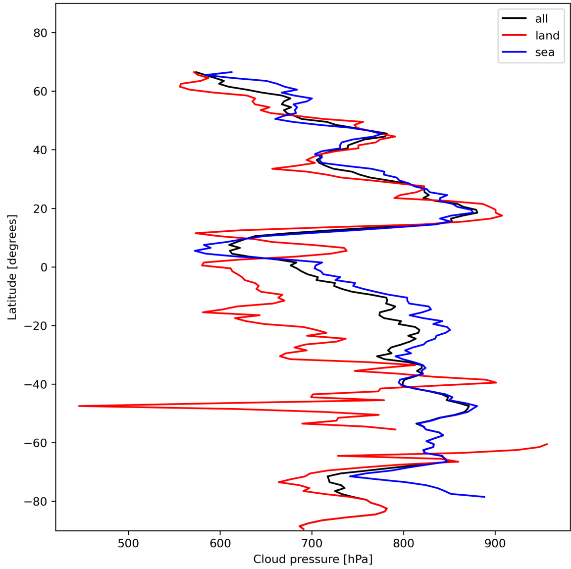
Figure 13: Zonal average of “Cloud pressure” for 2023-11-28 to 2023-11-30.
