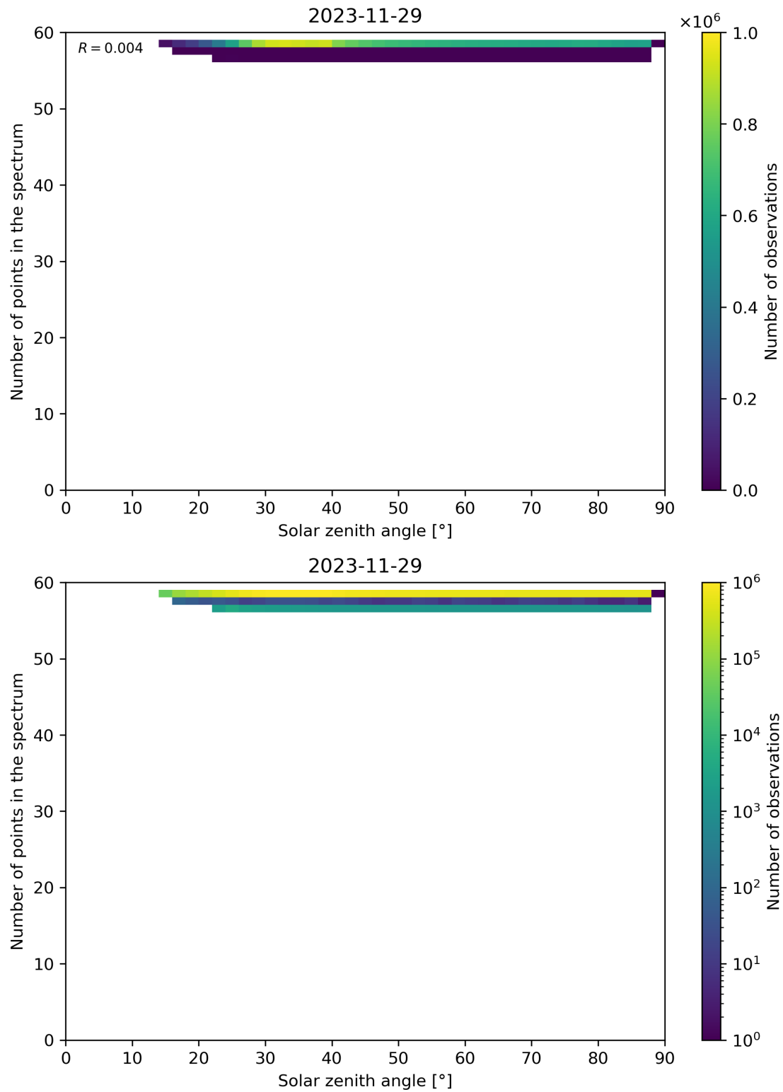
Figure 115: Scatter density plot of “Solar zenith angle” against “Number of points in the spectrum” for 2023-11-28 to 2023-11-30.
