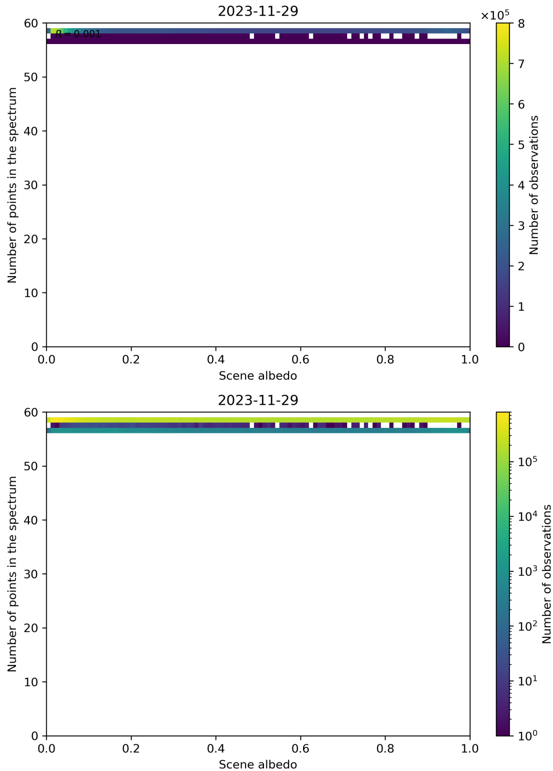
Figure 106: Scatter density plot of “Scene albedo” against “Number of points in the spectrum” for 2023-11-28 to 2023-11-30.
