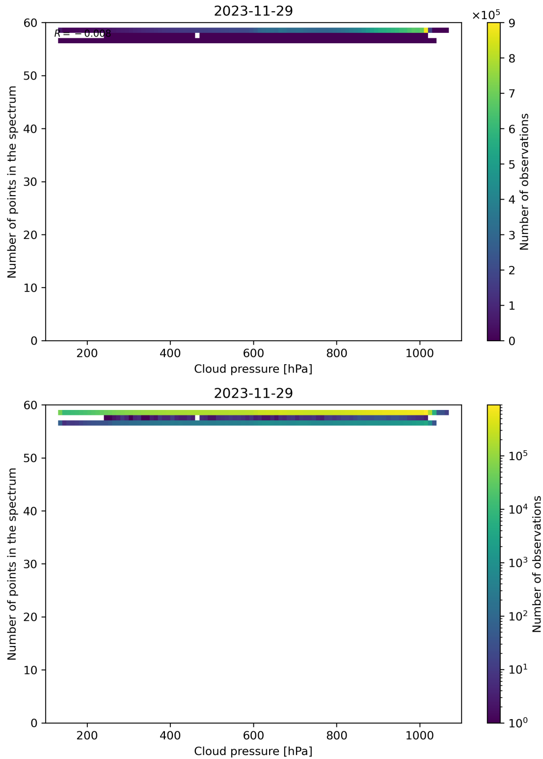
Figure 82: Scatter density plot of “Cloud pressure” against “Number of points in the spectrum” for 2023-11-28 to 2023-11-30.
