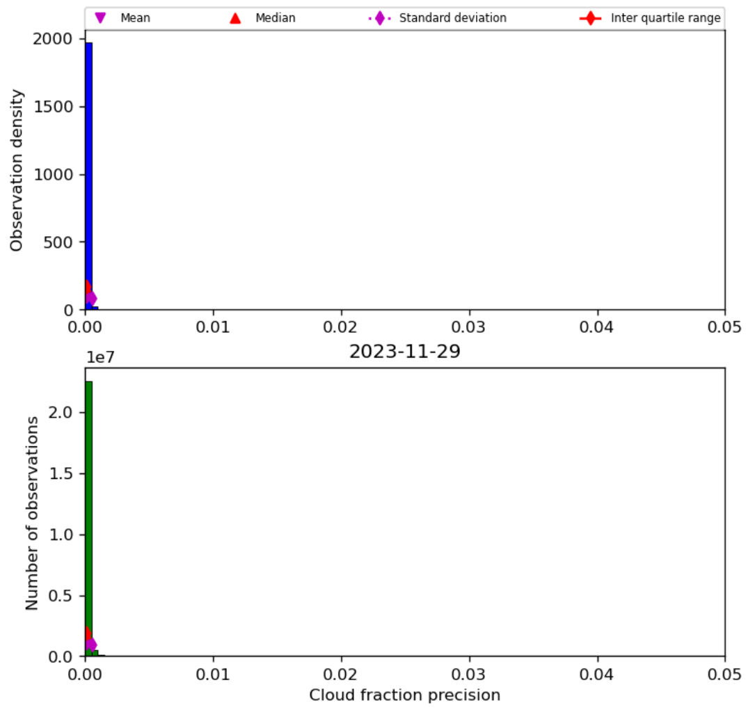
Figure 33: Histogram of “Cloud fraction precision” for 2023-11-28 to 2023-11-30
