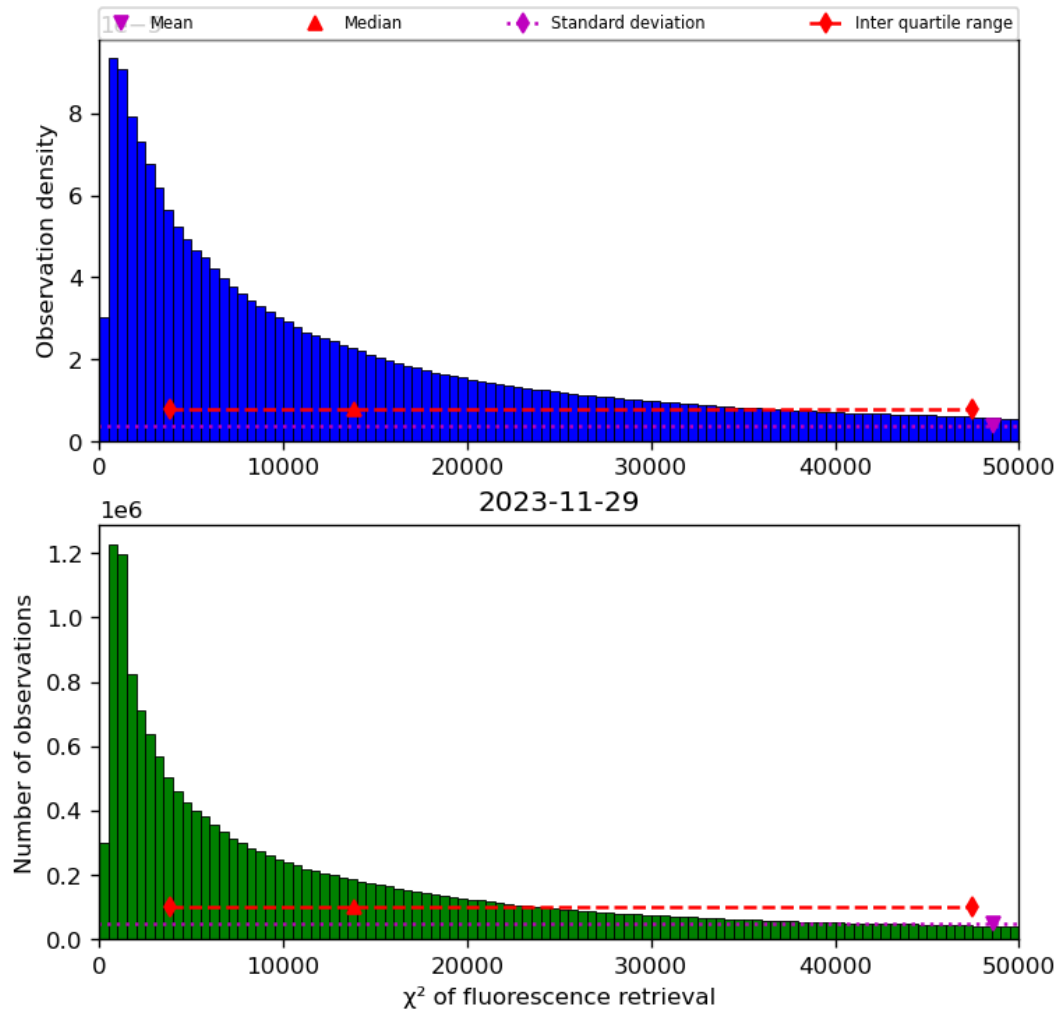
Figure 42: Histogram of “ \chi^2 of fluorescence retrieval” for 2023-11-28 to 2023-11-30
