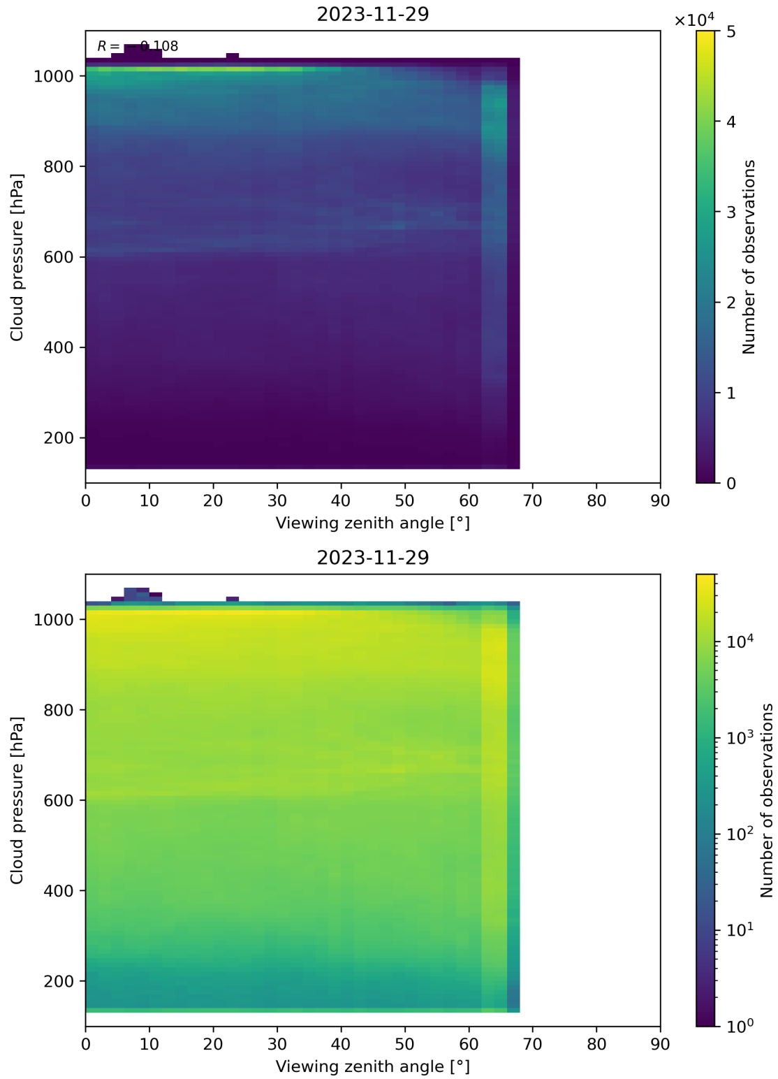
Figure 121: Scatter density plot of “Viewing zenith angle” against “Cloud pressure” for 2023-11-28 to 2023-11-30.
