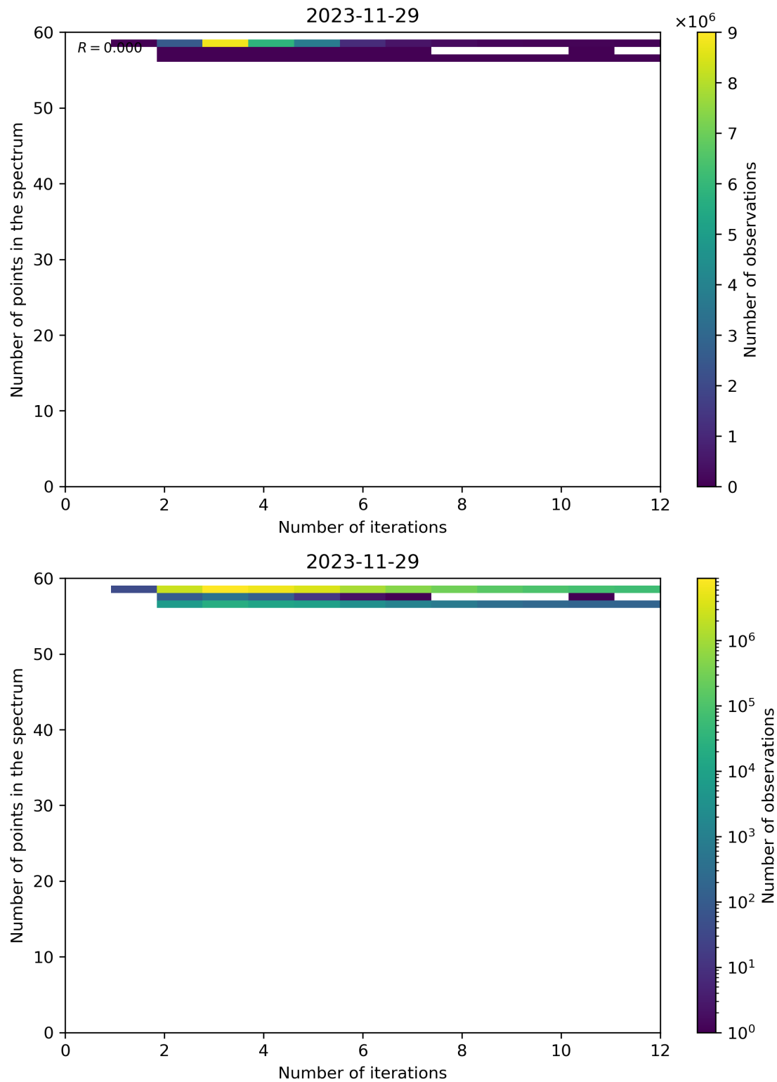
Figure 99: Scatter density plot of “Number of iterations” against “Number of points in the spectrum” for 2023-11-28 to 2023-11-30.
