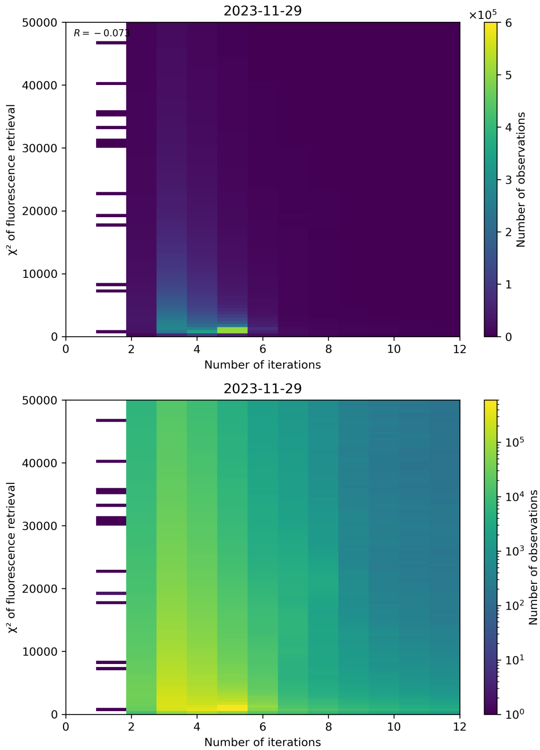
Figure 97: Scatter density plot of “Number of iterations” against “ \chi^2 of fluorescence retrieval” for 2023-11-28 to 2023-11-30.
