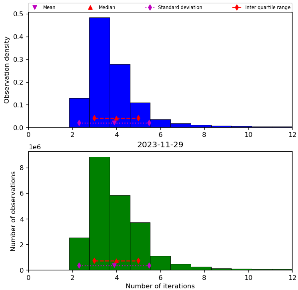
Figure 39: Histogram of “Number of iterations” for 2023-11-28 to 2023-11-30
