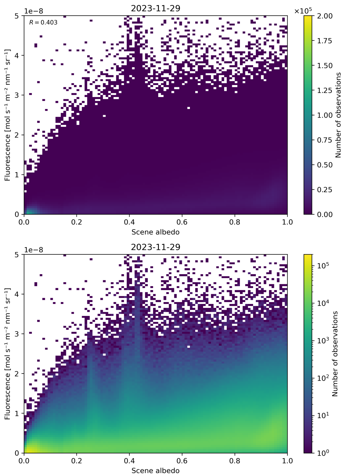
Figure 104: Scatter density plot of “Scene albedo” against “Fluorescence” for 2023-11-28 to 2023-11-30.
