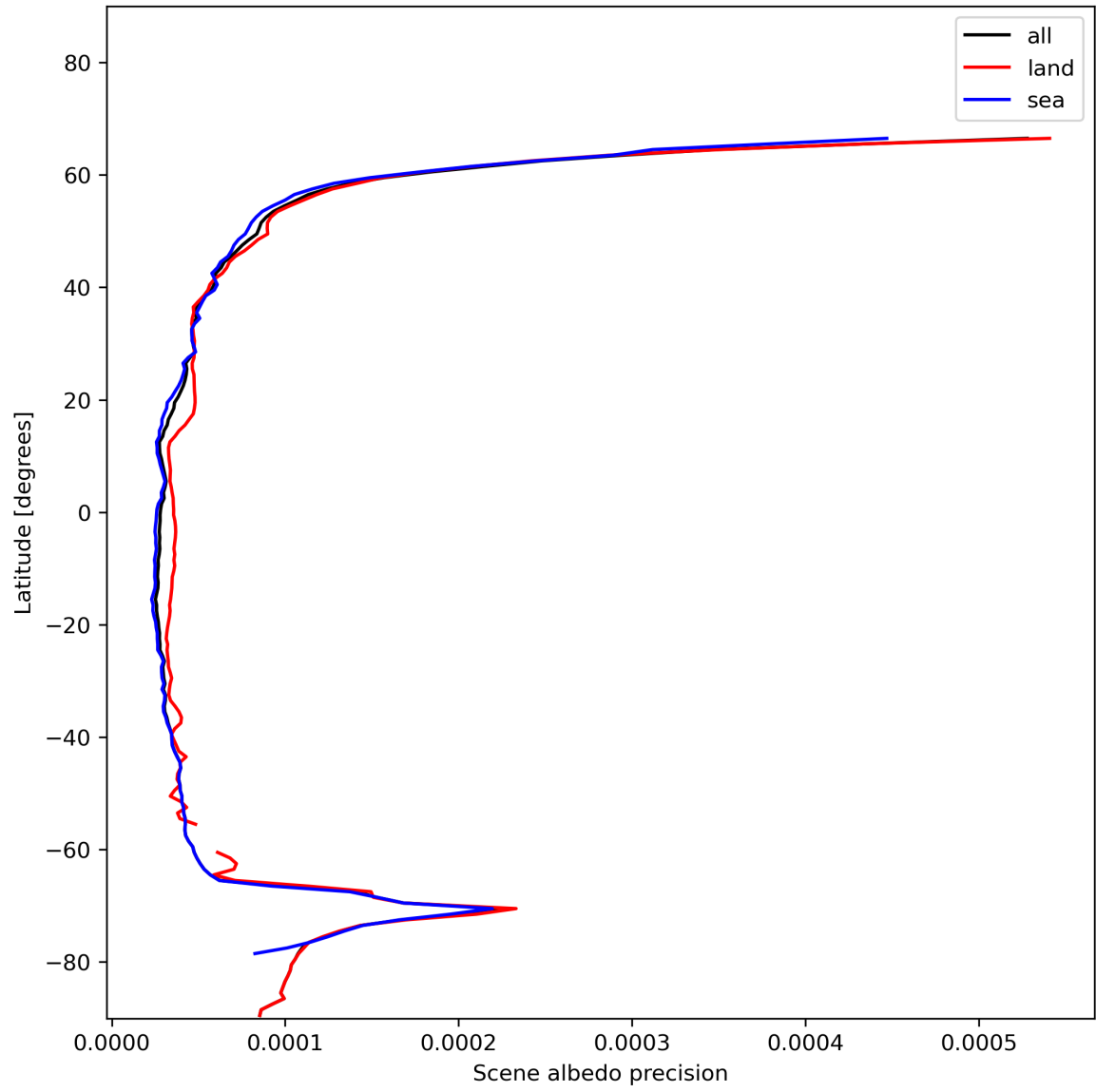
Figure 18: Zonal average of “Scene albedo precision” for 2023-11-28 to 2023-11-30.
