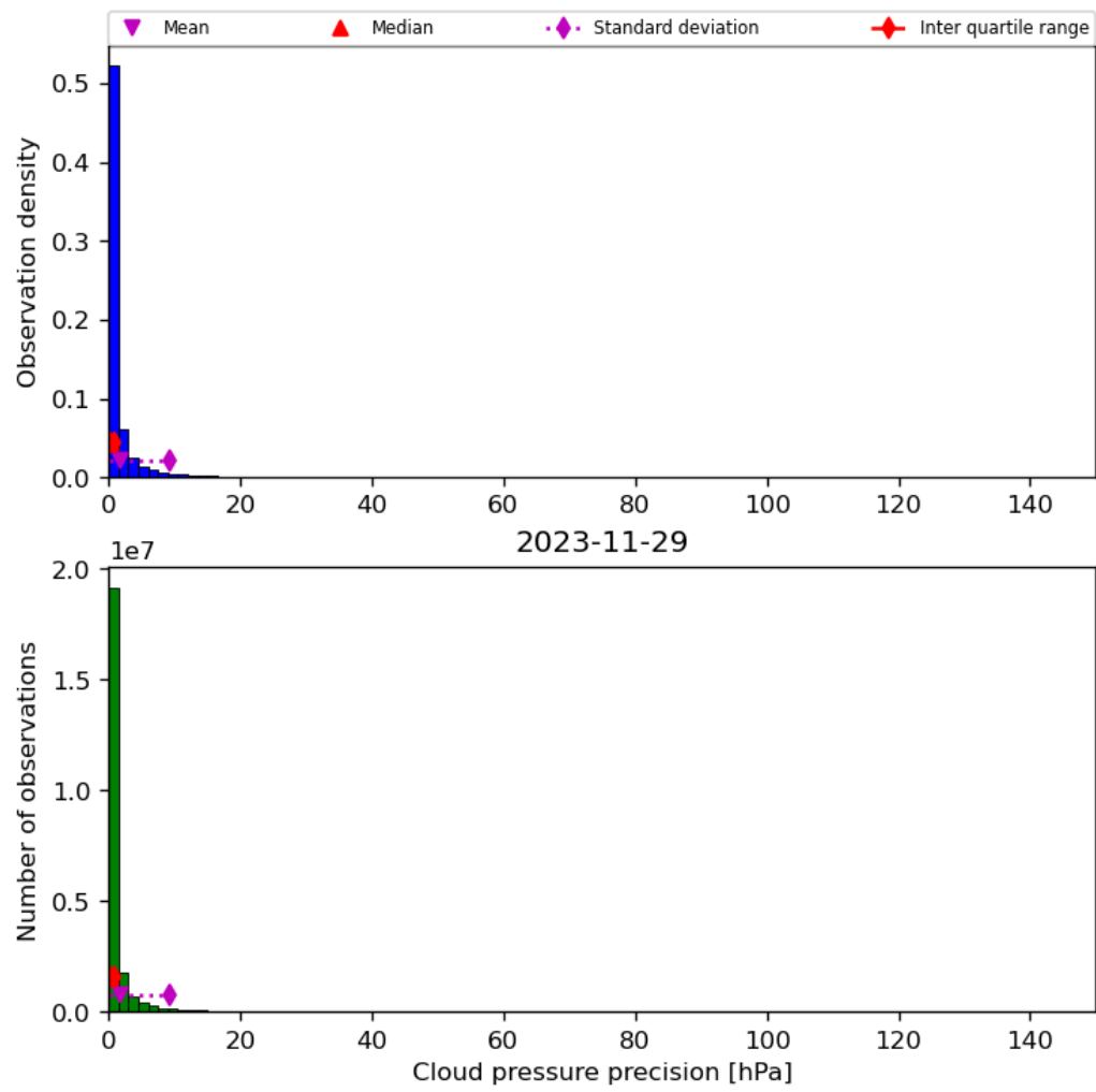
Figure 31: Histogram of “Cloud pressure precision” for 2023-11-28 to 2023-11-30
