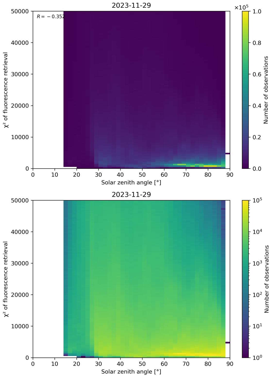
Figure 109: Scatter density plot of “Solar zenith angle” against “ \chi^2 of fluorescence retrieval” for 2023-11-28 to 2023-11-30.
