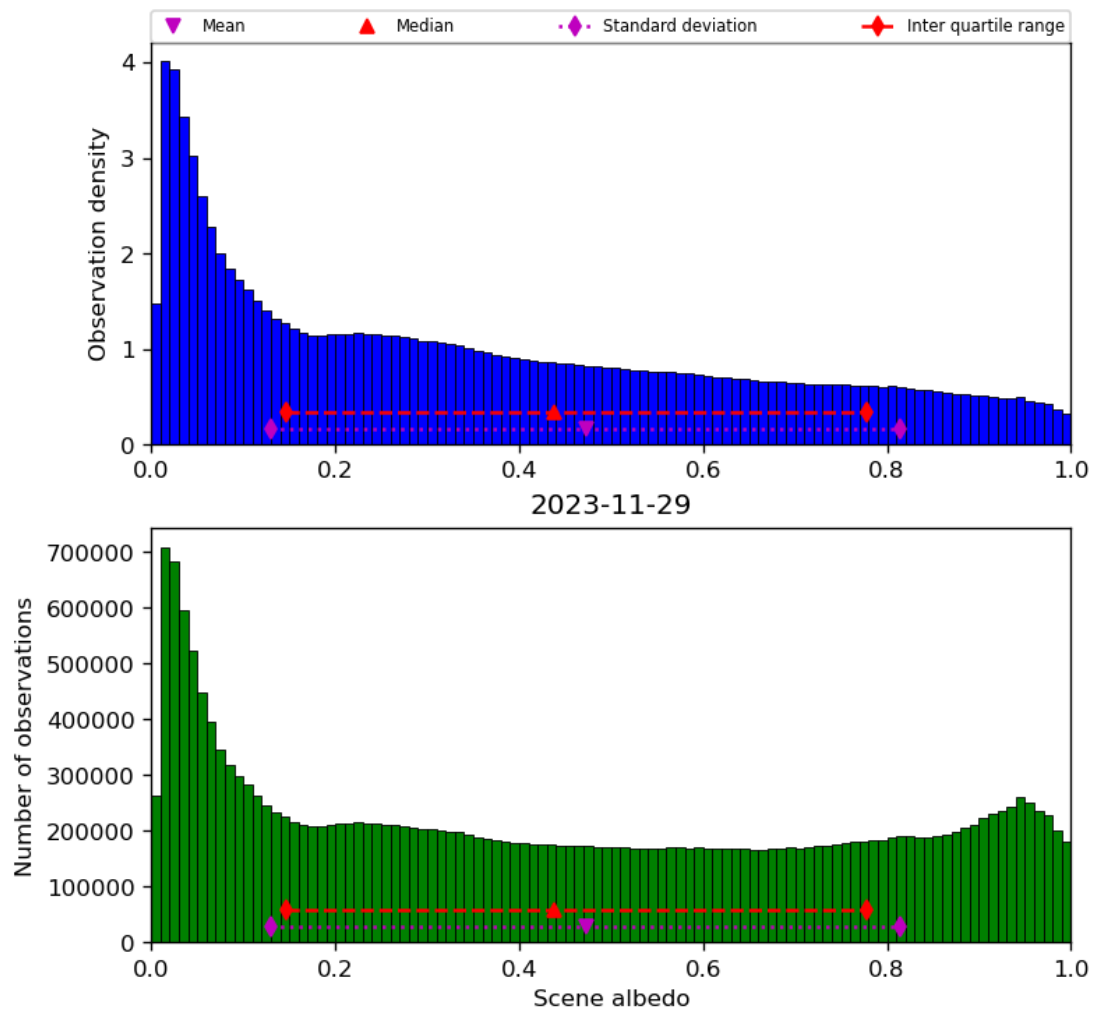
Figure 34: Histogram of “Scene albedo” for 2023-11-28 to 2023-11-30
