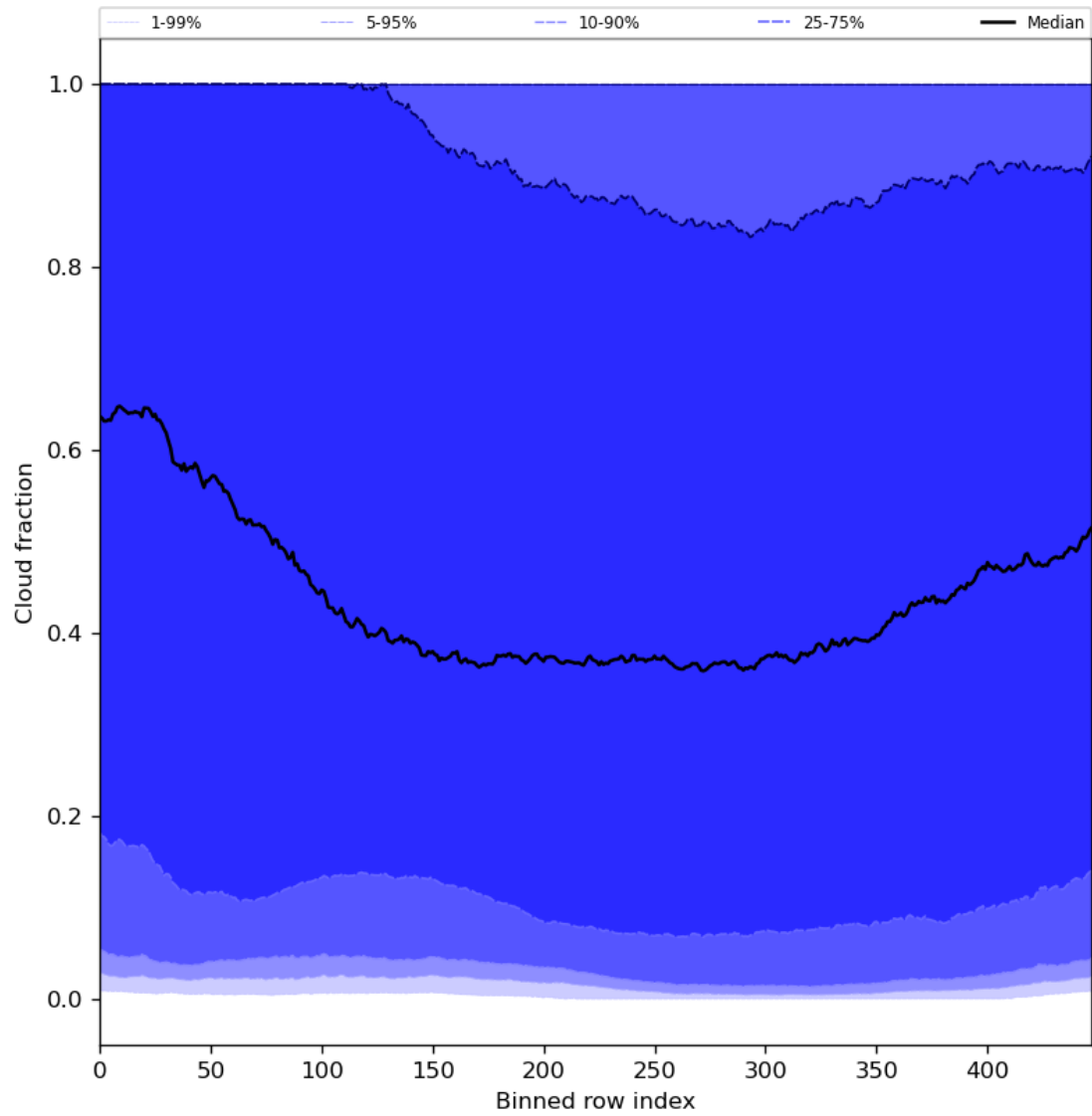
Figure 49: Along track statistics of “Cloud fraction” for 2023-11-28 to 2023-11-30
