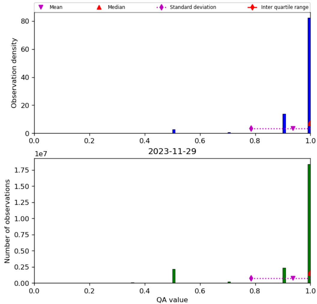
Figure 29: Histogram of “QA value” for 2023-11-28 to 2023-11-30
