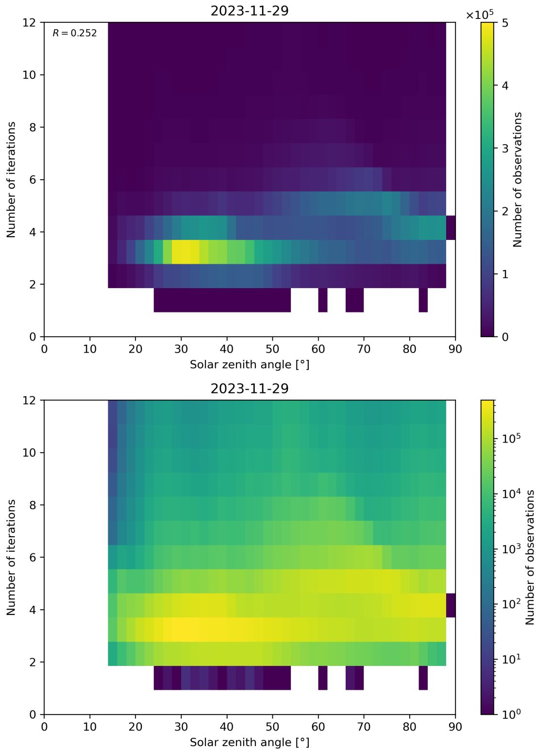
Figure 114: Scatter density plot of “Solar zenith angle” against “Number of iterations” for 2023-11-28 to 2023-11-30.
