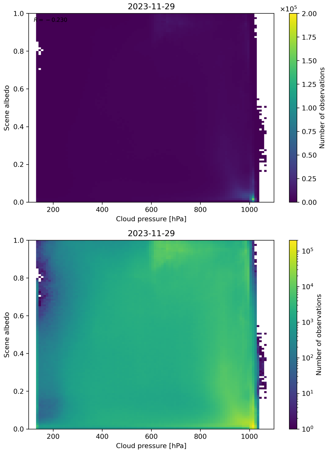
Figure 83: Scatter density plot of “Cloud pressure” against “Scene albedo” for 2023-11-28 to 2023-11-30.
