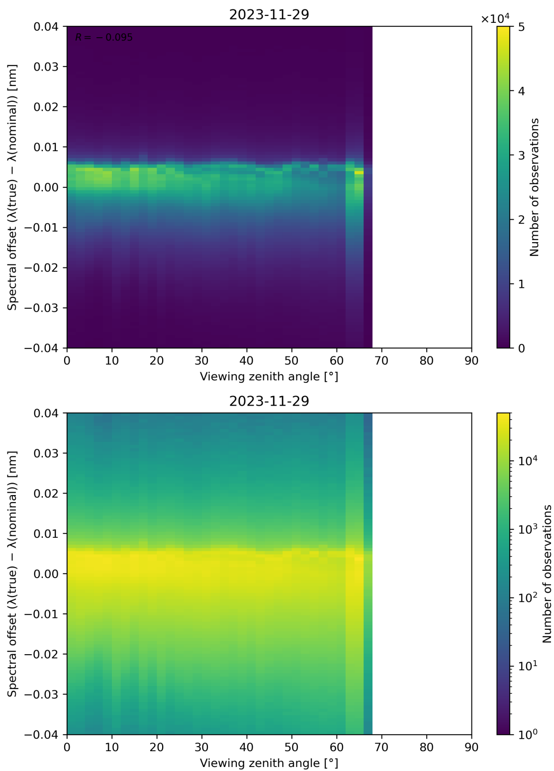
Figure 128: Scatter density plot of “Viewing zenith angle” against “Spectral offset ( \lambda(\text{true}) - \lambda(\text{nominal}) )” for 2023-11-28 to 2023-11-30.
