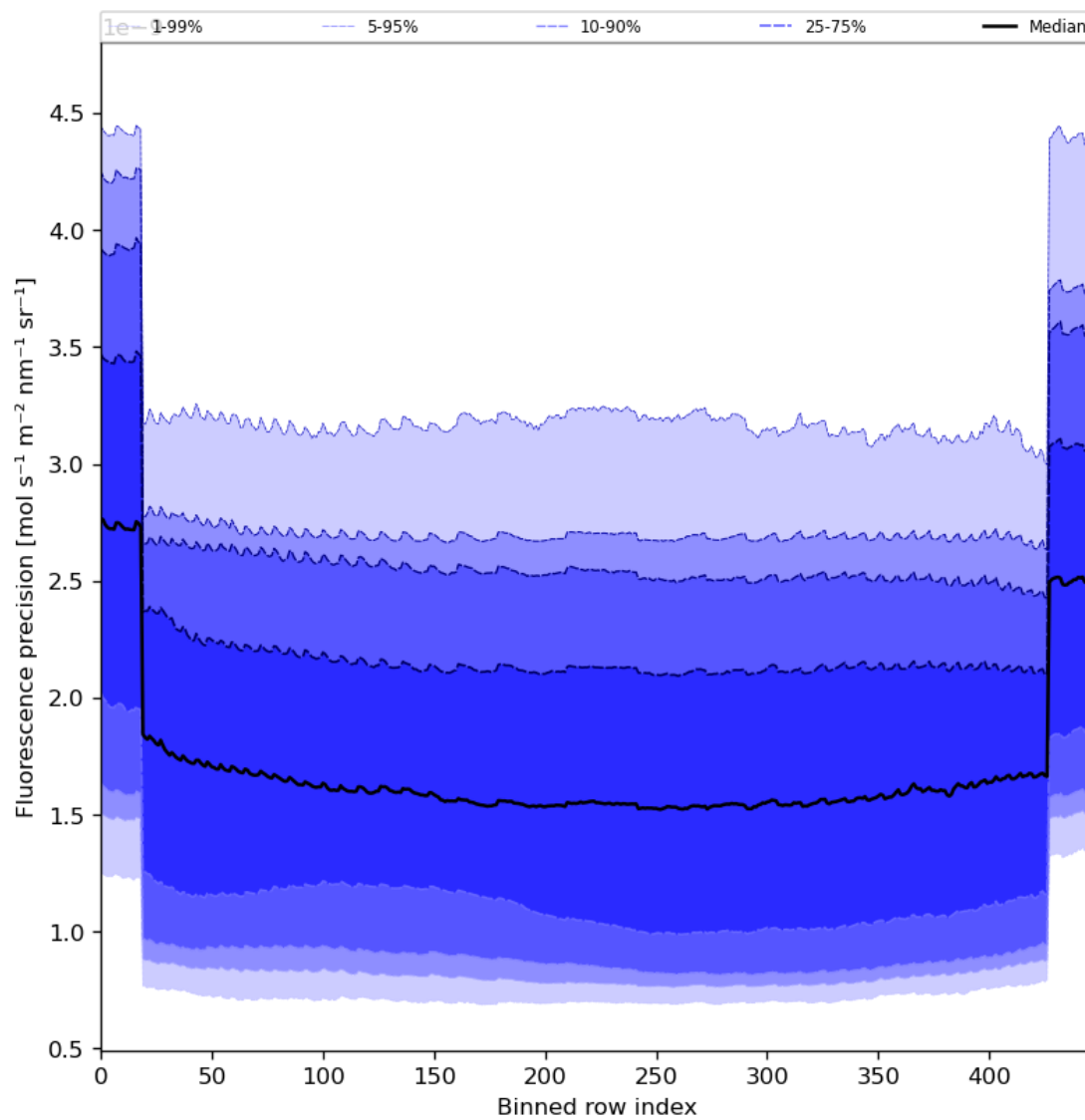
Figure 58: Along track statistics of “Fluorescence precision” for 2023-11-28 to 2023-11-30
