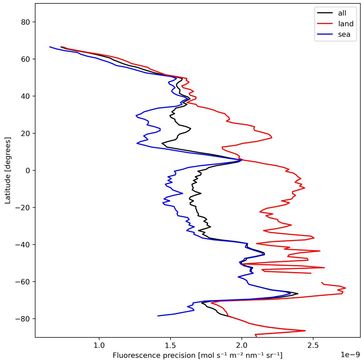
Figure 24: Zonal average of “Fluorescence precision” for 2023-11-28 to 2023-11-30.
