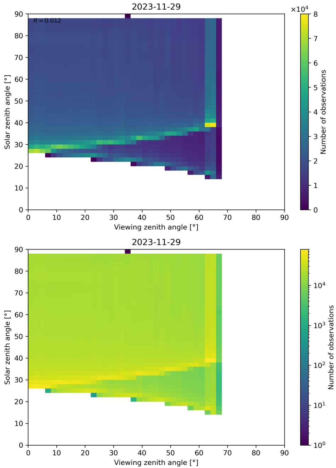
Figure 127: Scatter density plot of “Viewing zenith angle” against “Solar zenith angle” for 2023-11-28 to 2023-11-30.
