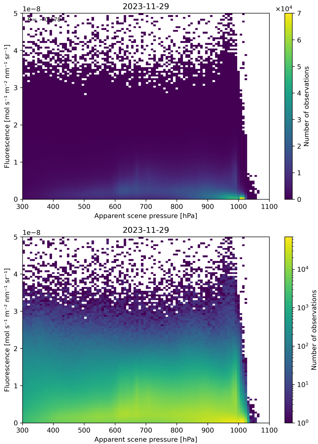
Figure 64: Scatter density plot of “Apparent scene pressure” against “Fluorescence” for 2023-11-28 to 2023-11-30.
