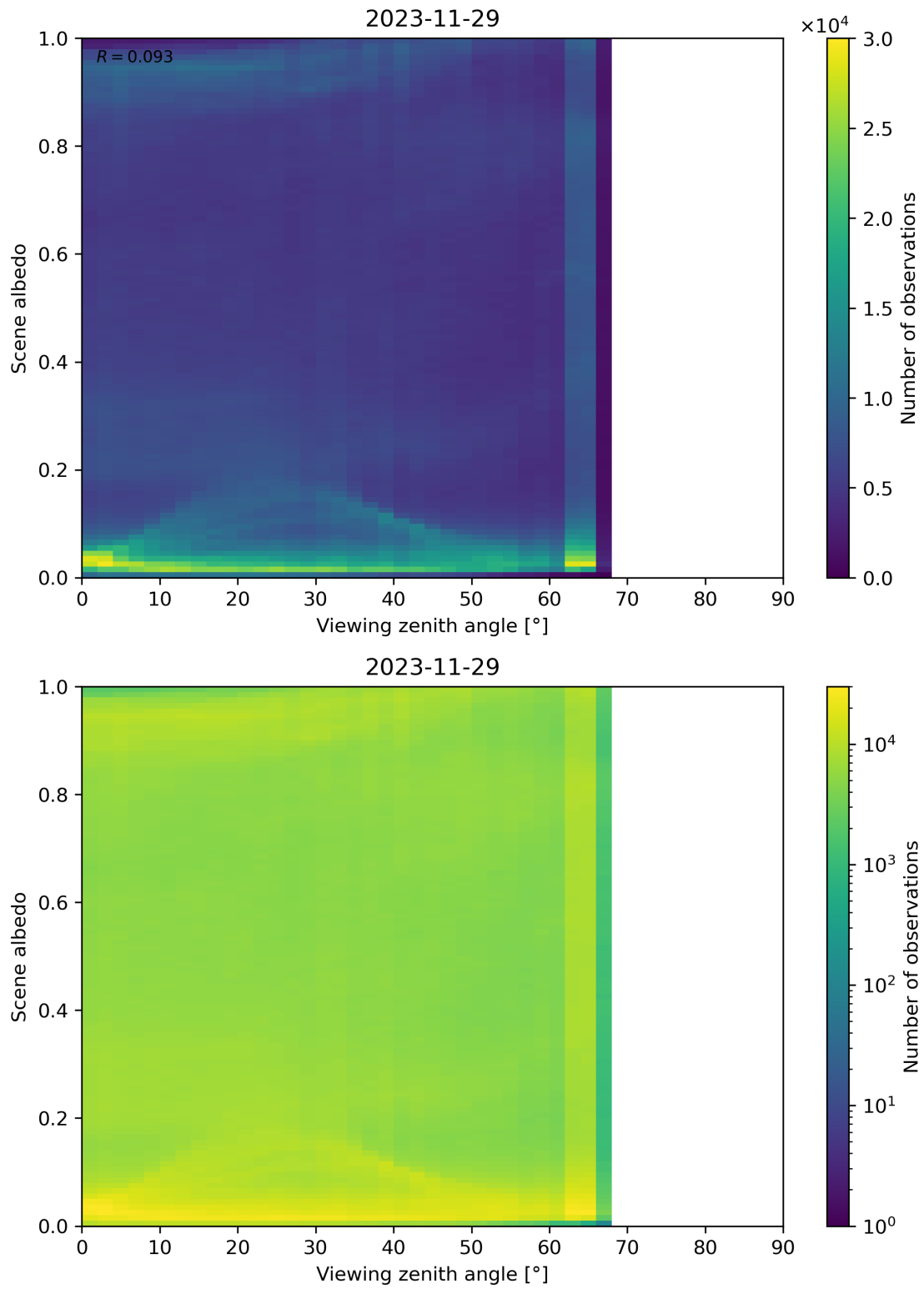
Figure 126: Scatter density plot of “Viewing zenith angle” against “Scene albedo” for 2023-11-28 to 2023-11-30.
