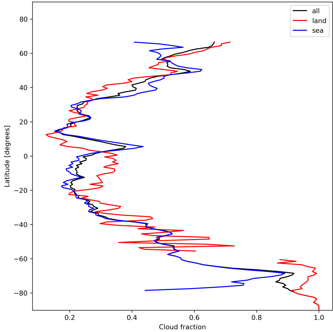
Figure 15: Zonal average of “Cloud fraction” for 2023-11-28 to 2023-11-30.
