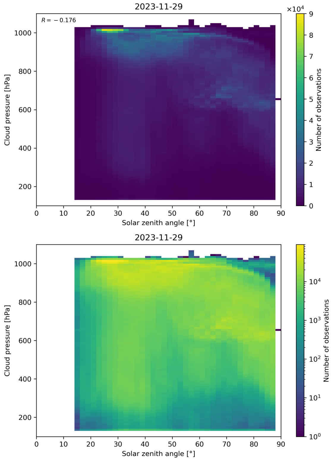
Figure 111: Scatter density plot of “Solar zenith angle” against “Cloud pressure” for 2023-11-28 to 2023-11-30.
