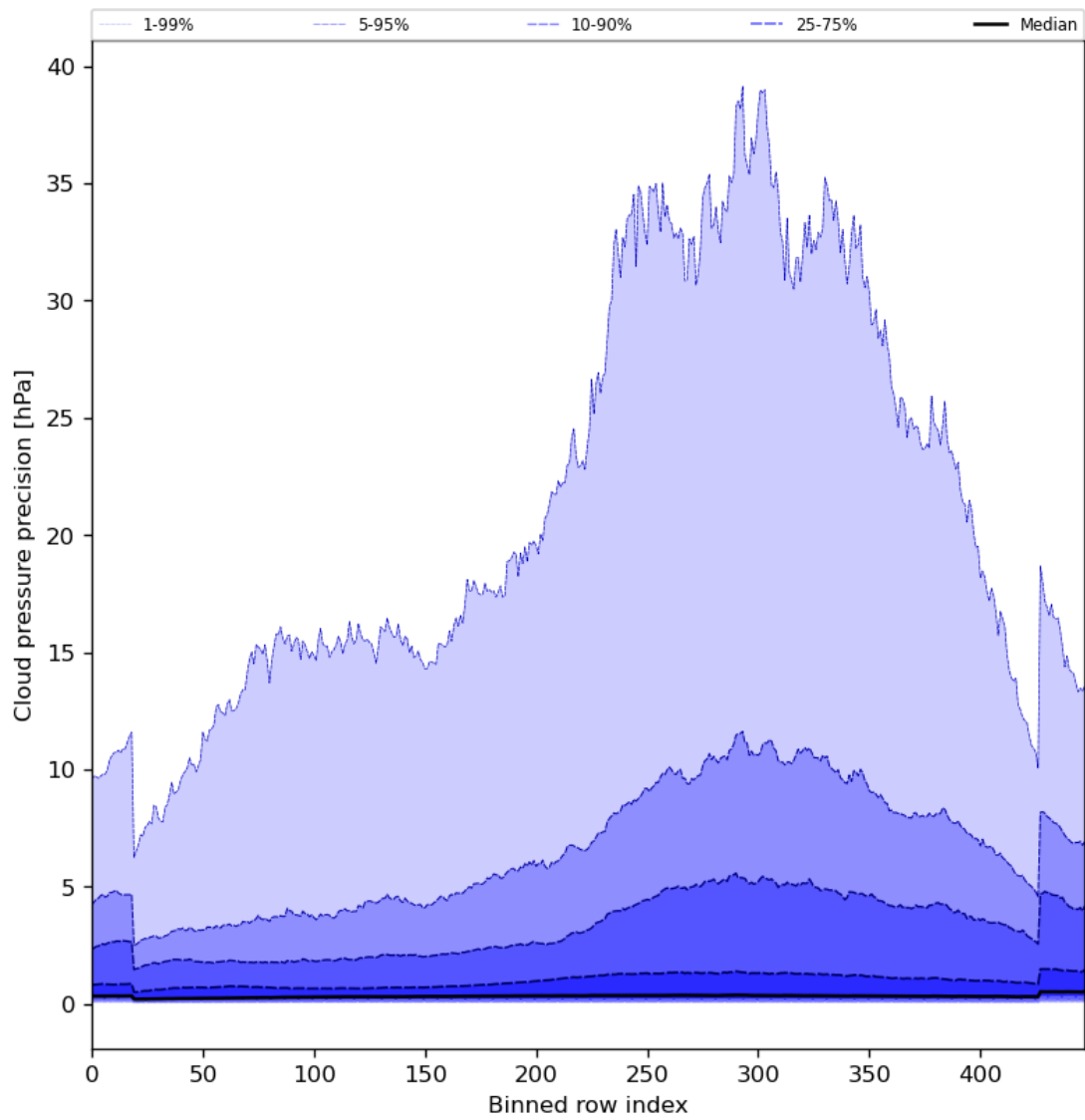
Figure 48: Along track statistics of “Cloud pressure precision” for 2023-11-28 to 2023-11-30
