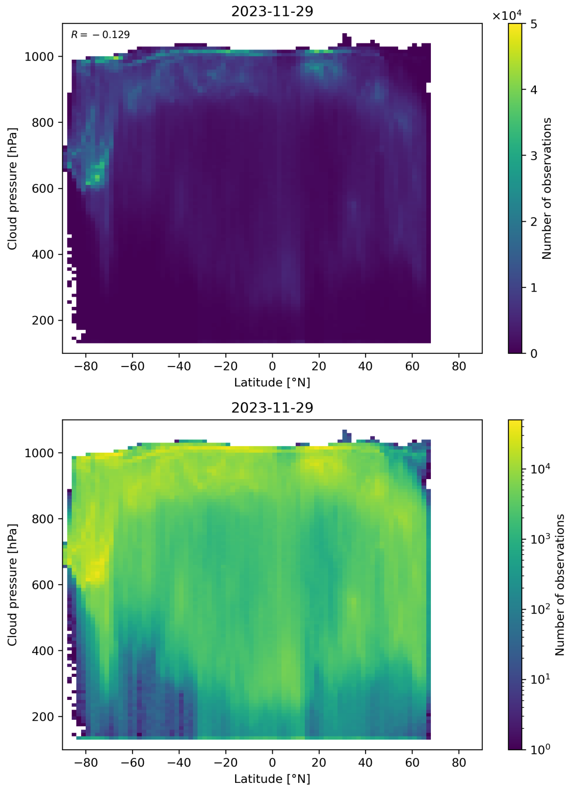
Figure 91: Scatter density plot of “Latitude” against “Cloud pressure” for 2023-11-28 to 2023-11-30.
