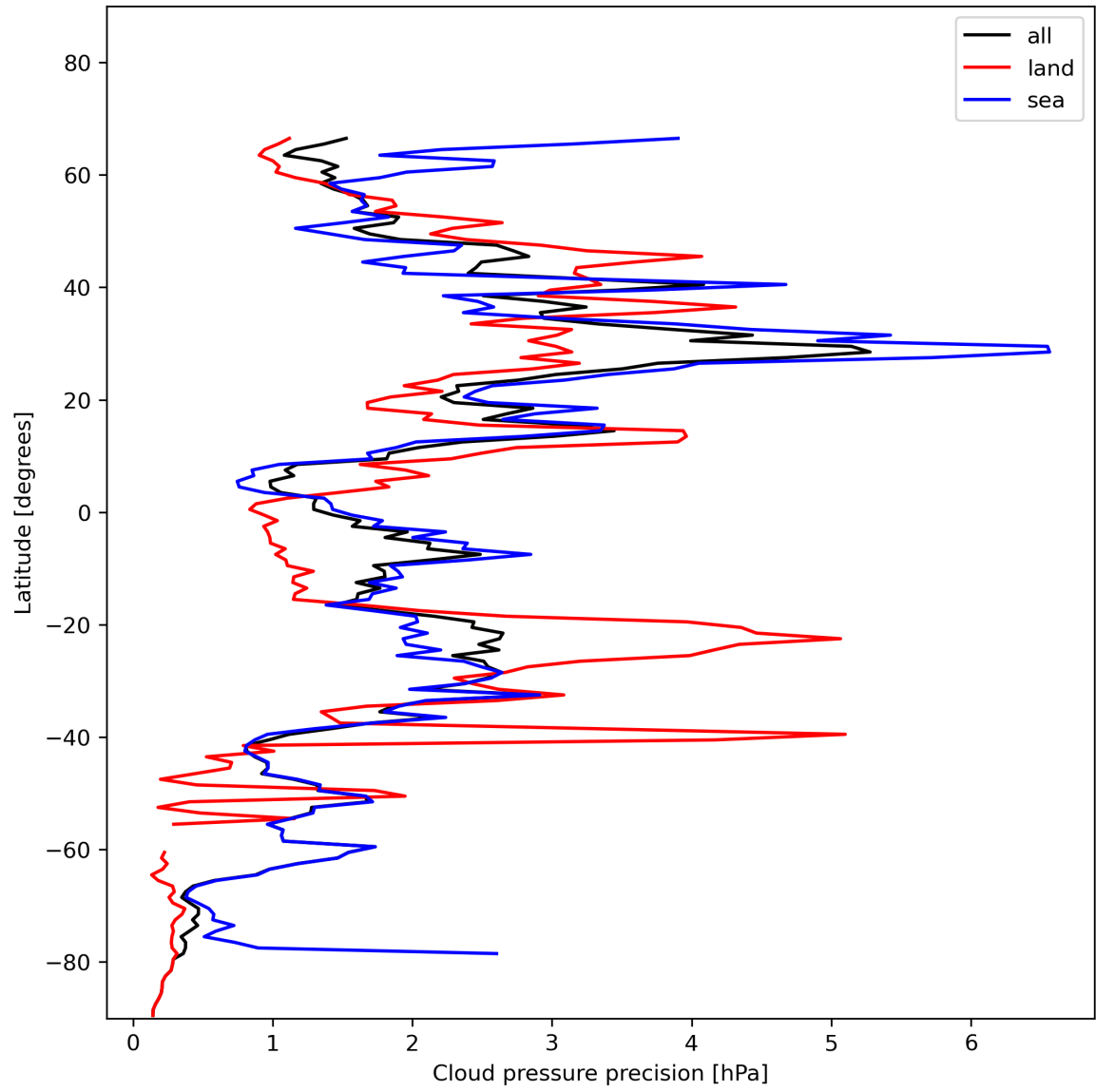
Figure 14: Zonal average of “Cloud pressure precision” for 2023-11-28 to 2023-11-30.
