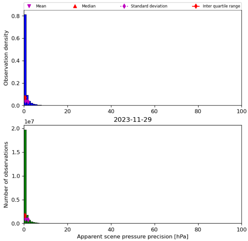
Figure 37: Histogram of “Apparent scene pressure precision” for 2023-11-28 to 2023-11-30
