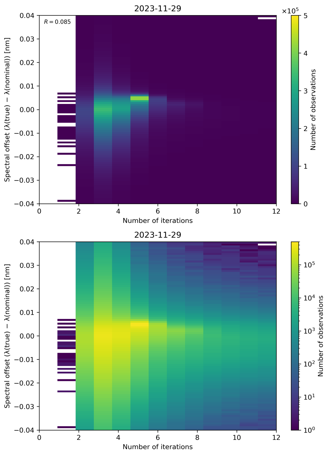
Figure 100: Scatter density plot of “Number of iterations” against “Spectral offset ( \lambda(\text{true}) - \lambda(\text{nominal}) )” for 2023-11-28 to 2023-11-30.
