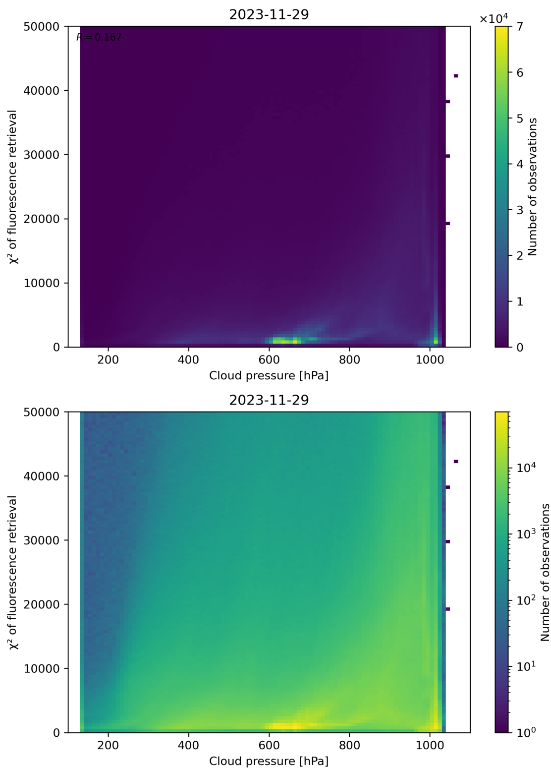
Figure 78: Scatter density plot of “Cloud pressure” against “ \chi^2 of fluorescence retrieval” for 2023-11-28 to 2023-11-30.
