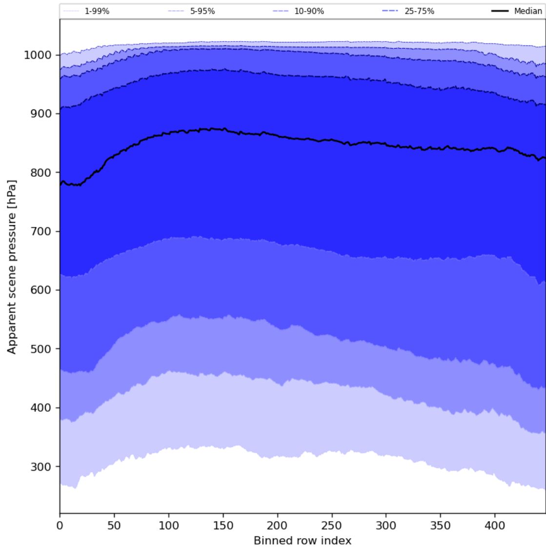
Figure 53: Along track statistics of “Apparent scene pressure” for 2023-11-30 to 2023-12-02
