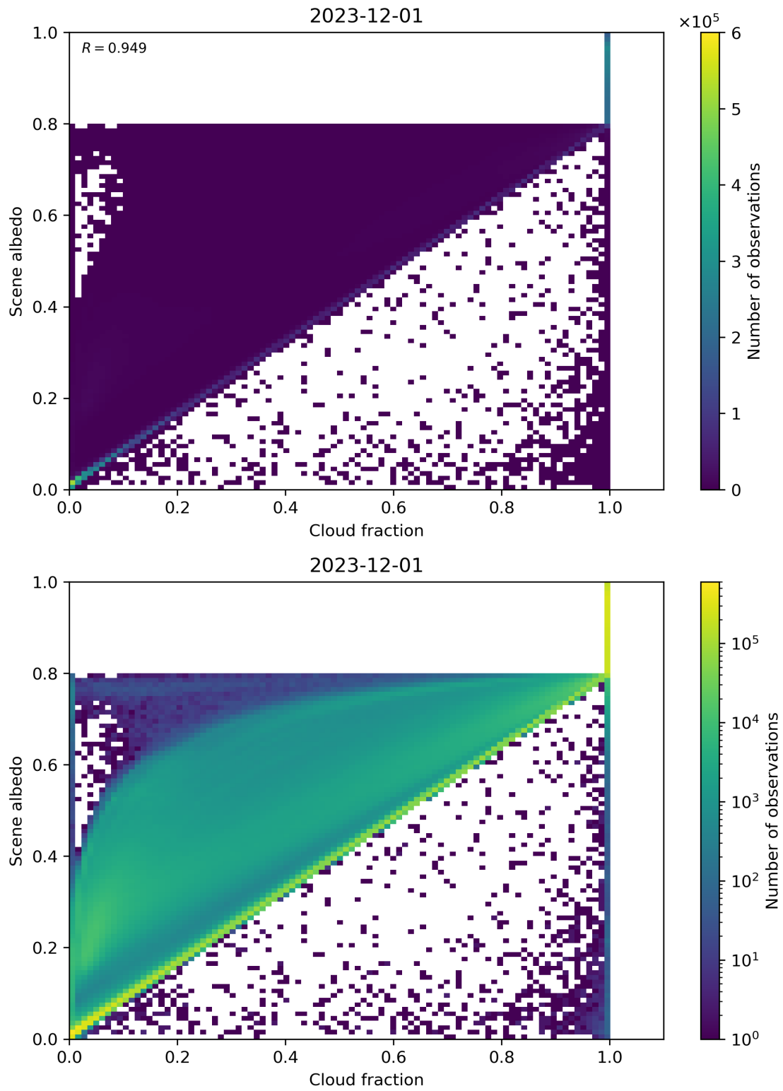
Figure 75: Scatter density plot of “Cloud fraction” against “Scene albedo” for 2023-11-30 to 2023-12-02.
