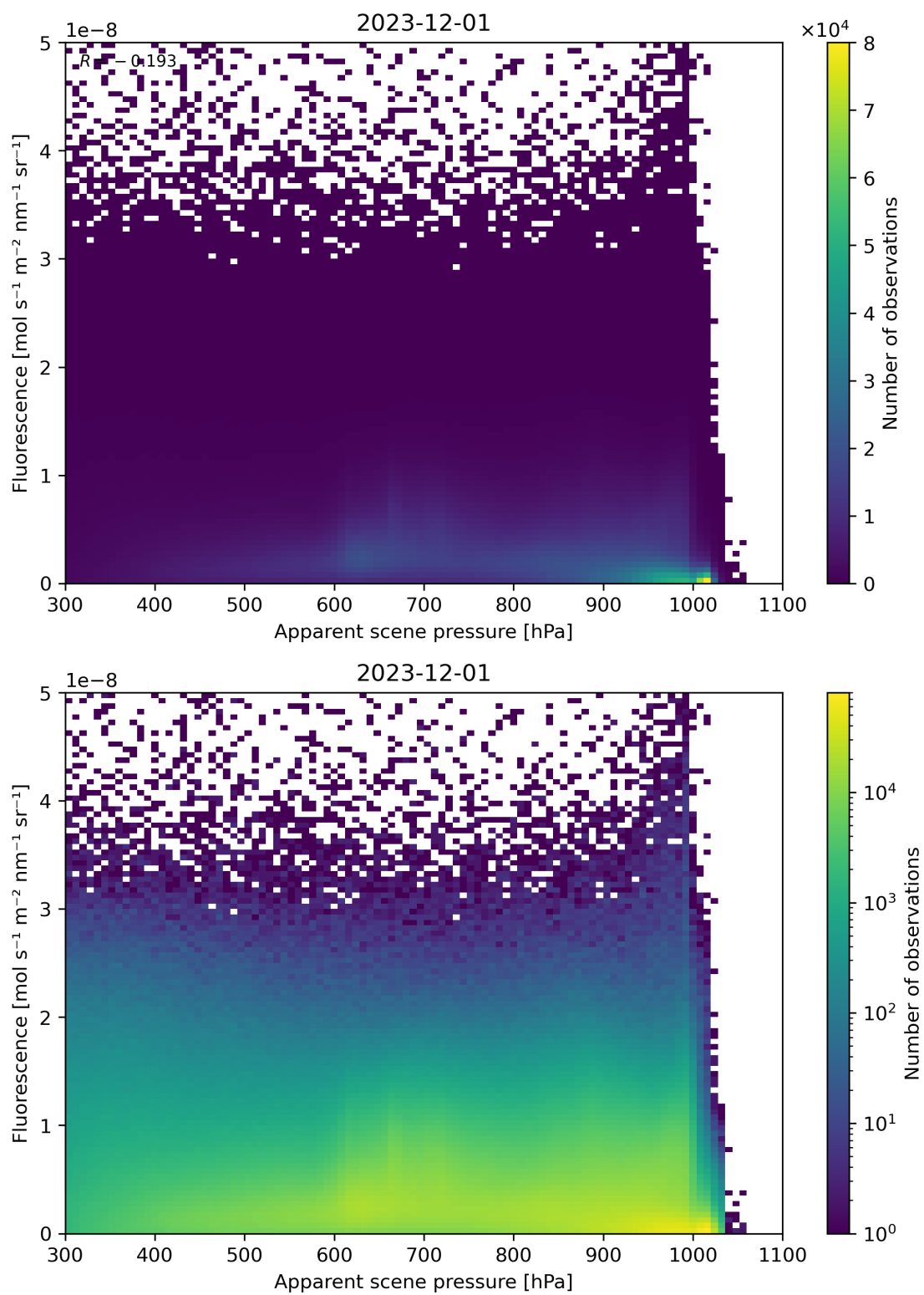
Figure 64: Scatter density plot of “Apparent scene pressure” against “Fluorescence” for 2023-11-30 to 2023-12-02.
