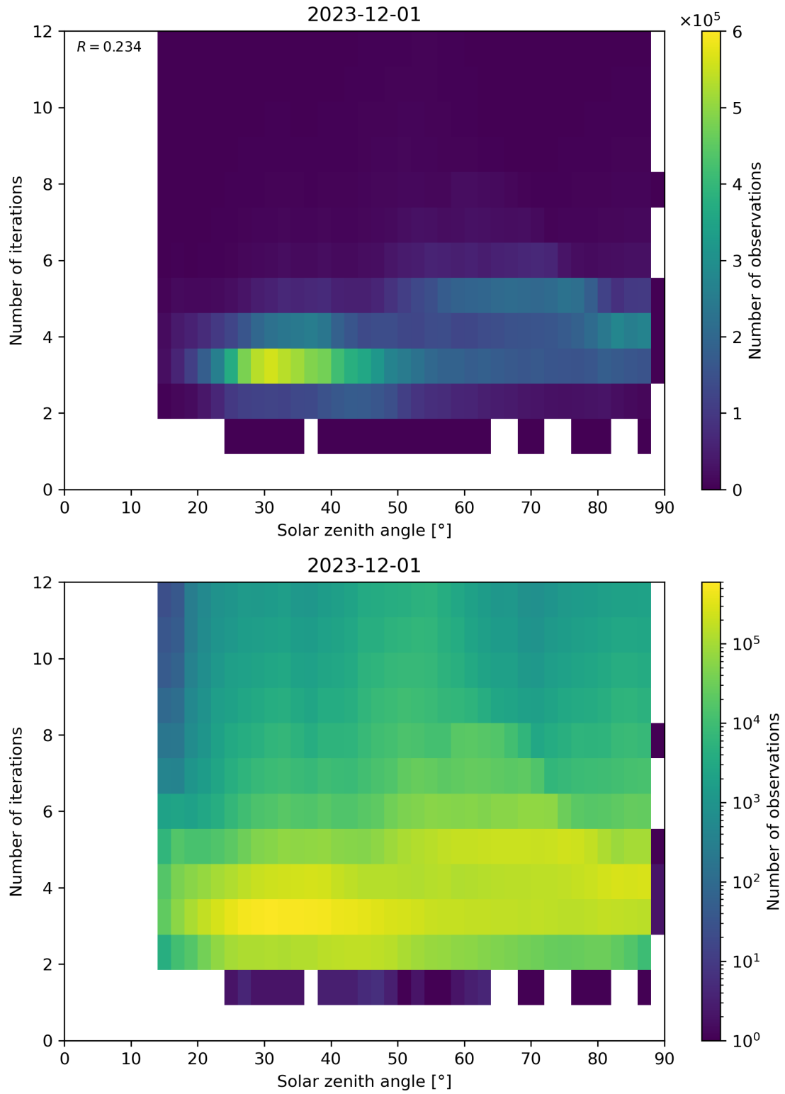
Figure 114: Scatter density plot of “Solar zenith angle” against “Number of iterations” for 2023-11-30 to 2023-12-02.
