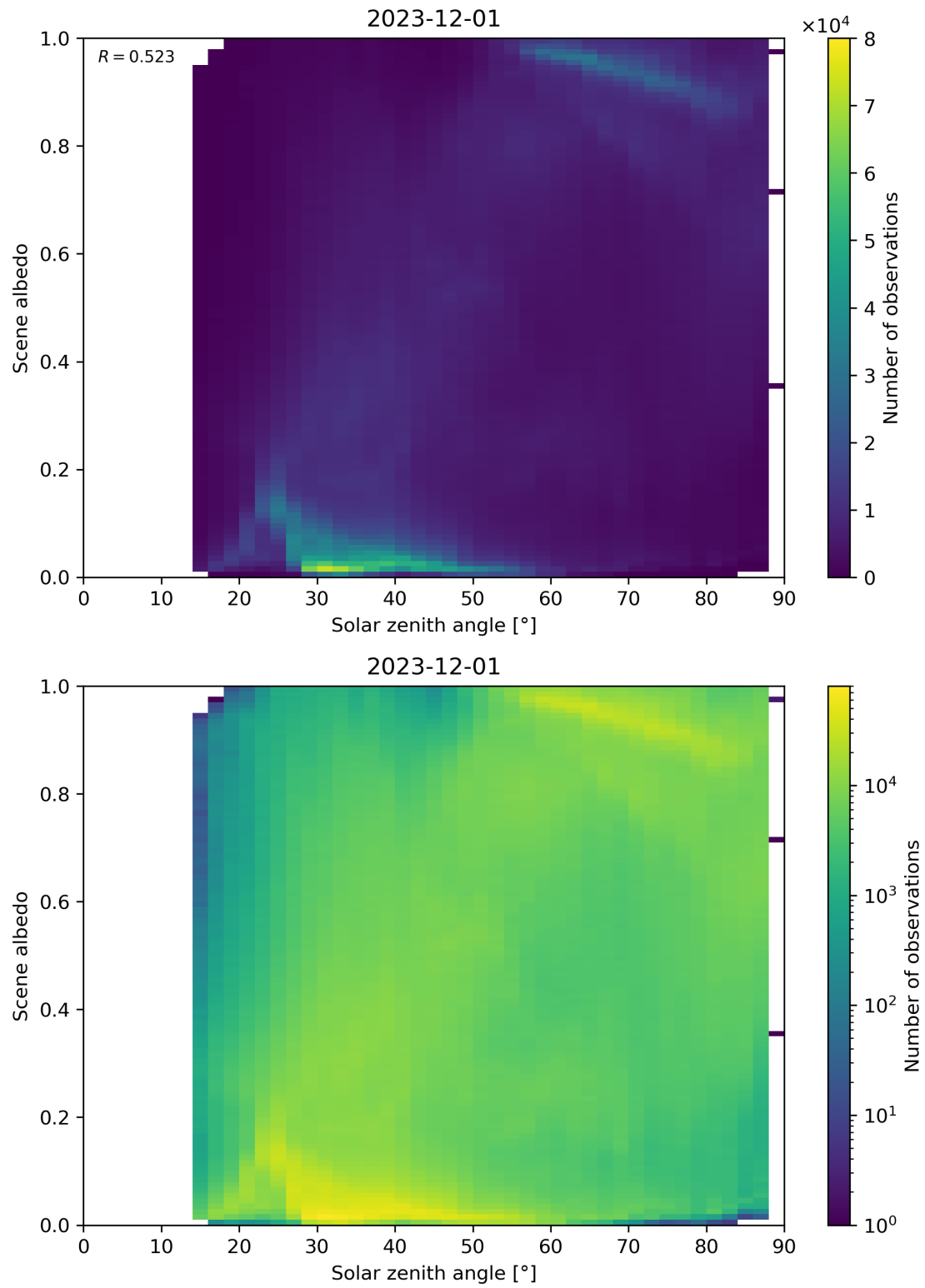
Figure 116: Scatter density plot of “Solar zenith angle” against “Scene albedo” for 2023-11-30 to 2023-12-02.
