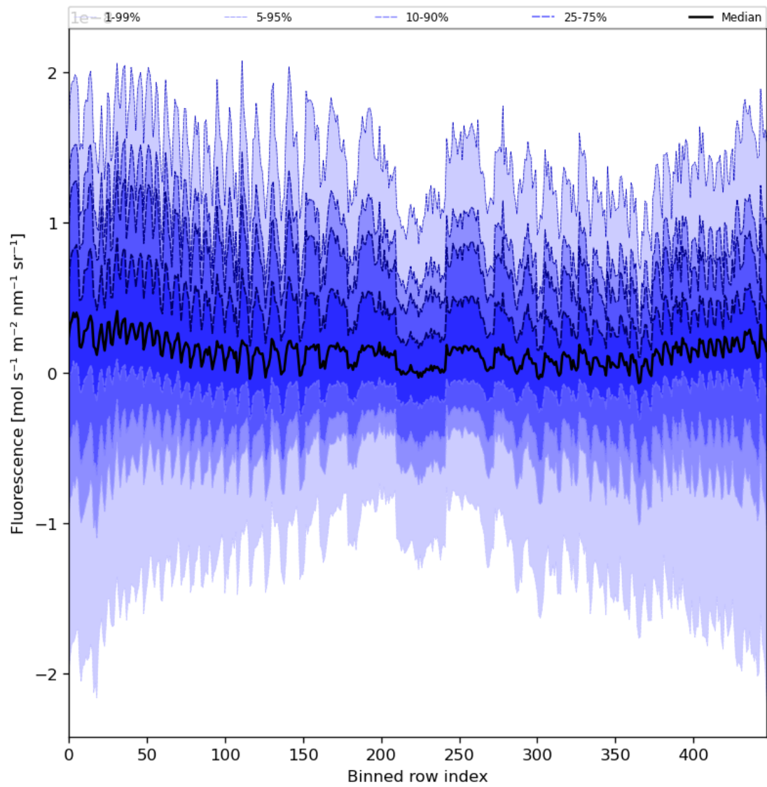
Figure 57: Along track statistics of “Fluorescence” for 2023-11-30 to 2023-12-02
