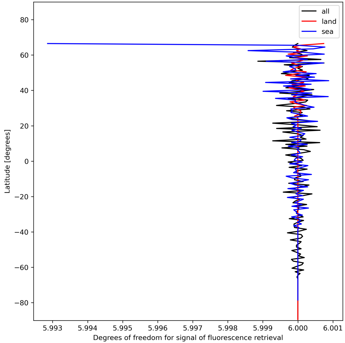
Figure 26: Zonal average of “Degrees of freedom for signal of fluorescence retrieval” for 2023-11-30 to 2023-12-02.
