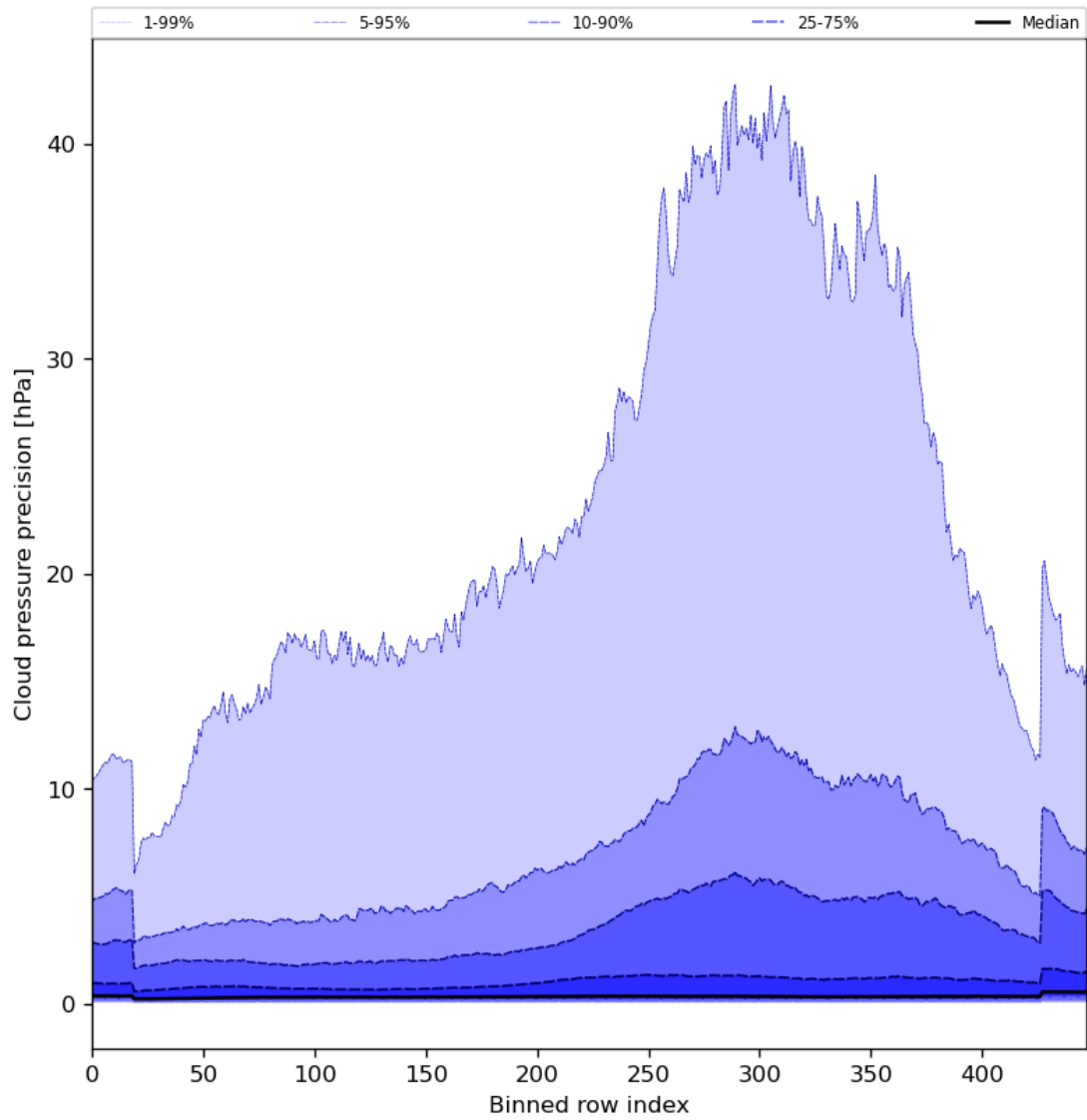
Figure 48: Along track statistics of “Cloud pressure precision” for 2023-11-30 to 2023-12-02
