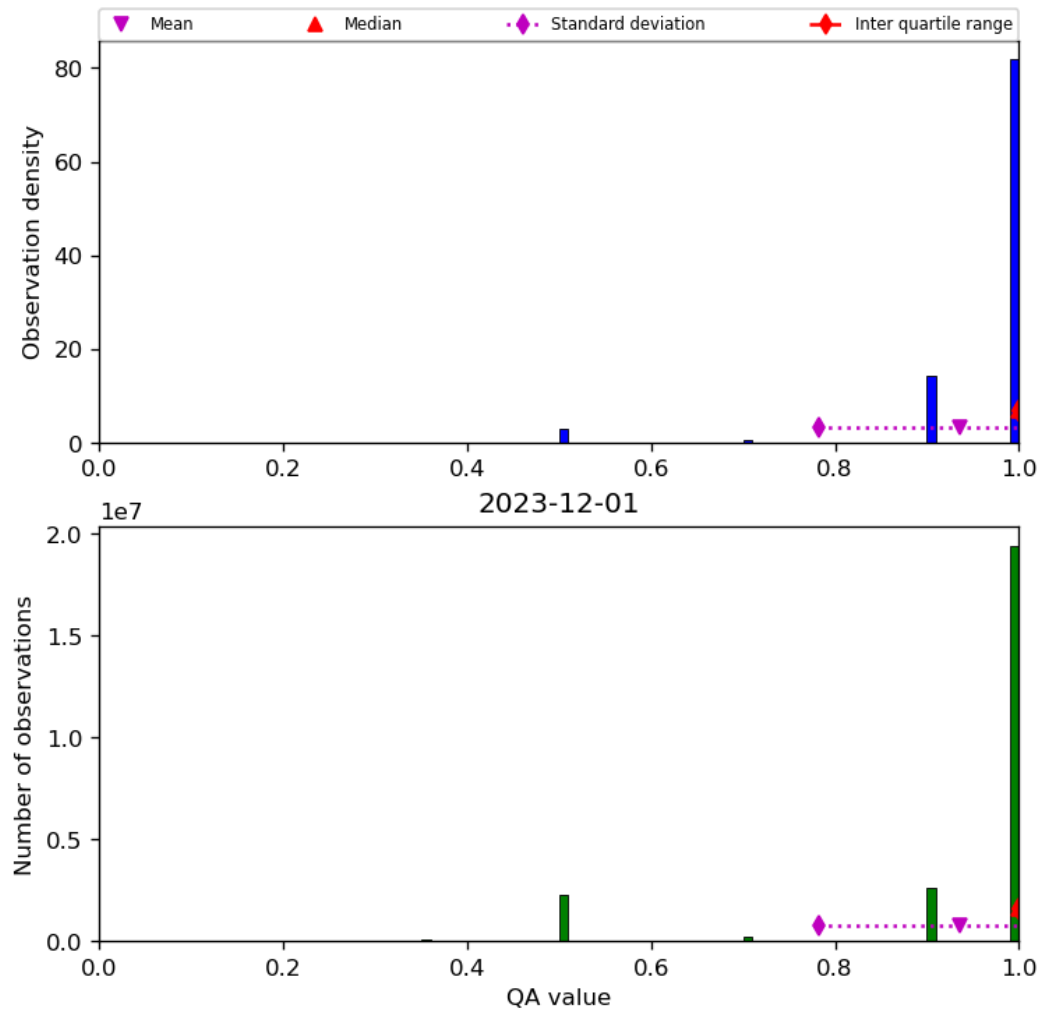
Figure 29: Histogram of “QA value” for 2023-11-30 to 2023-12-02
