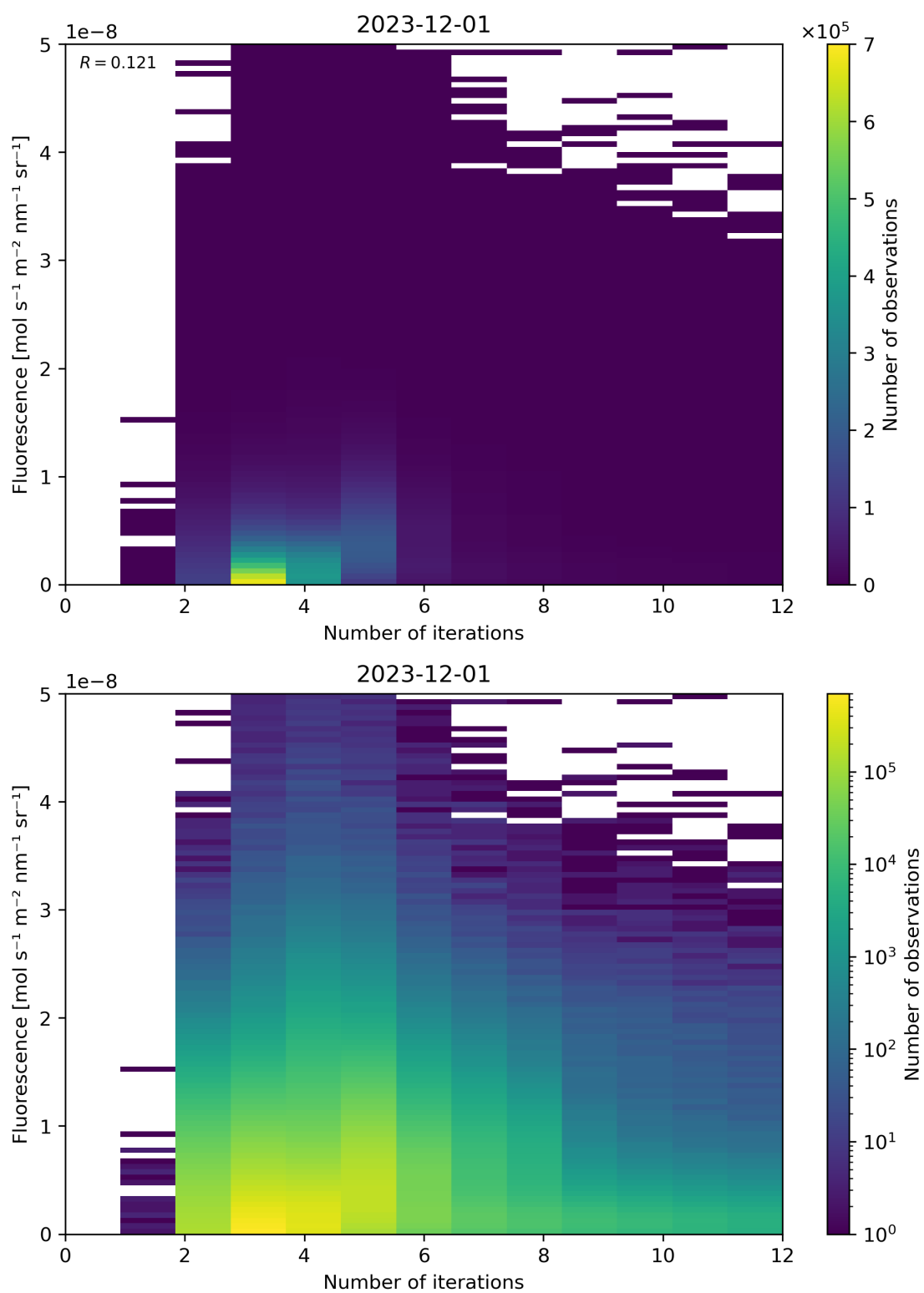
Figure 98: Scatter density plot of “Number of iterations” against “Fluorescence” for 2023-11-30 to 2023-12-02.
