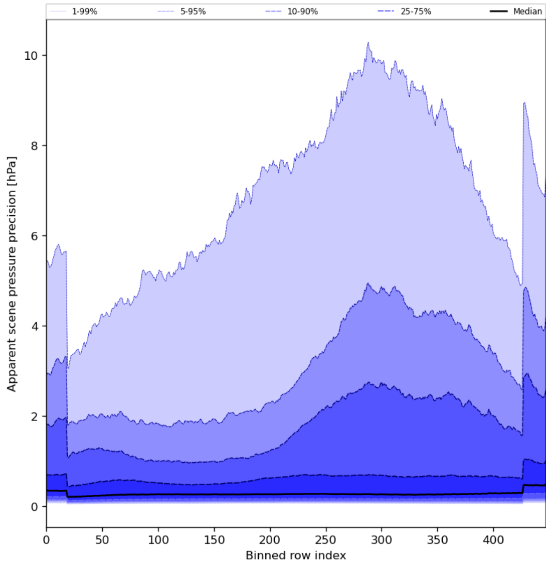
Figure 54: Along track statistics of “Apparent scene pressure precision” for 2023-11-30 to 2023-12-02
