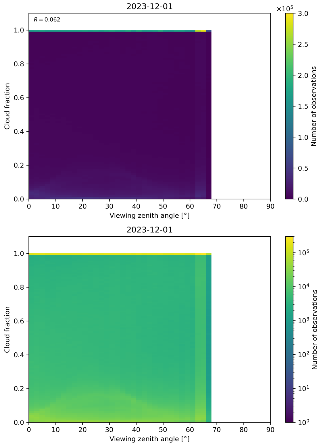
Figure 120: Scatter density plot of “Viewing zenith angle” against “Cloud fraction” for 2023-11-30 to 2023-12-02.
