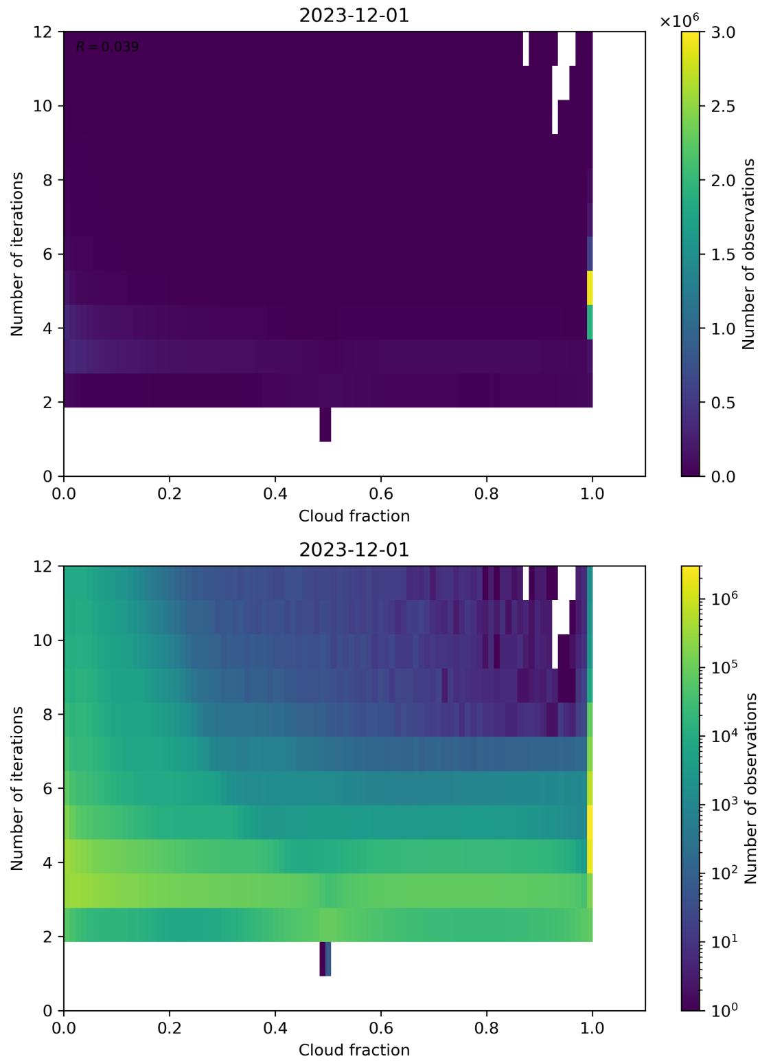
Figure 73: Scatter density plot of “Cloud fraction” against “Number of iterations” for 2023-11-30 to 2023-12-02.
