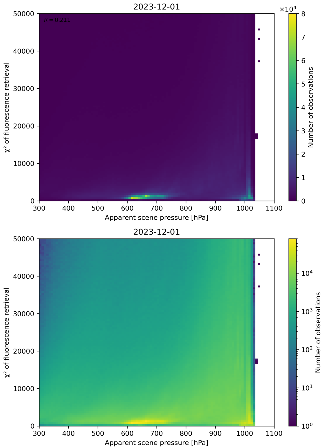
Figure 63: Scatter density plot of “Apparent scene pressure” against “ \chi^2 of fluorescence retrieval” for 2023-11-30 to 2023-12-02.
