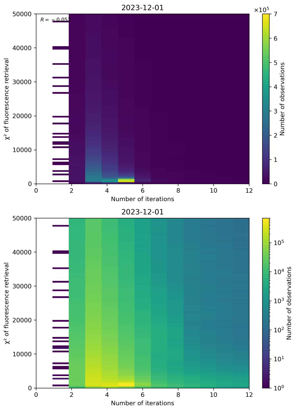
Figure 97: Scatter density plot of “Number of iterations” against “ \chi^2 of fluorescence retrieval” for 2023-11-30 to 2023-12-02.
