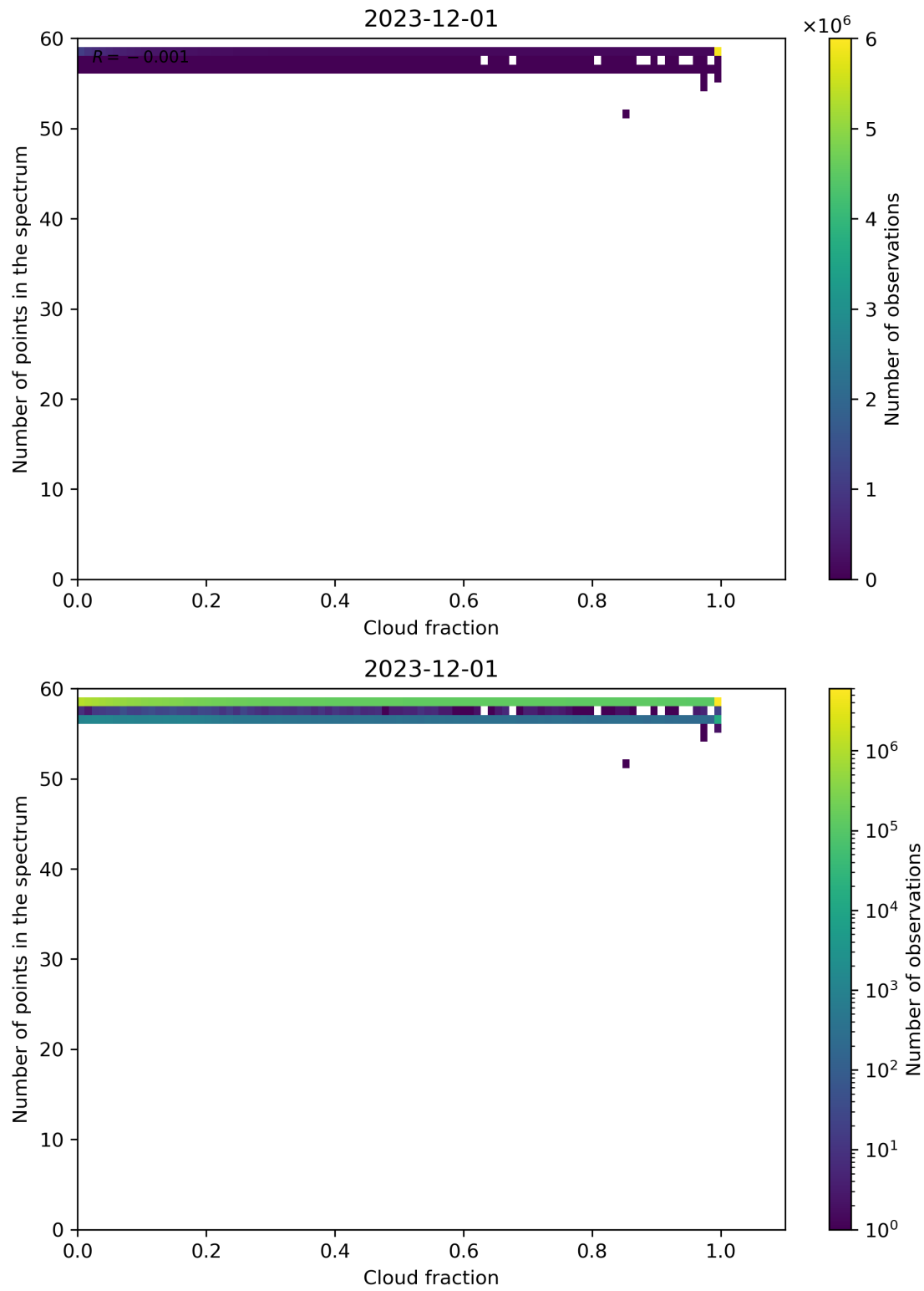
Figure 74: Scatter density plot of “Cloud fraction” against “Number of points in the spectrum” for 2023-11-30 to 2023-12-02.
