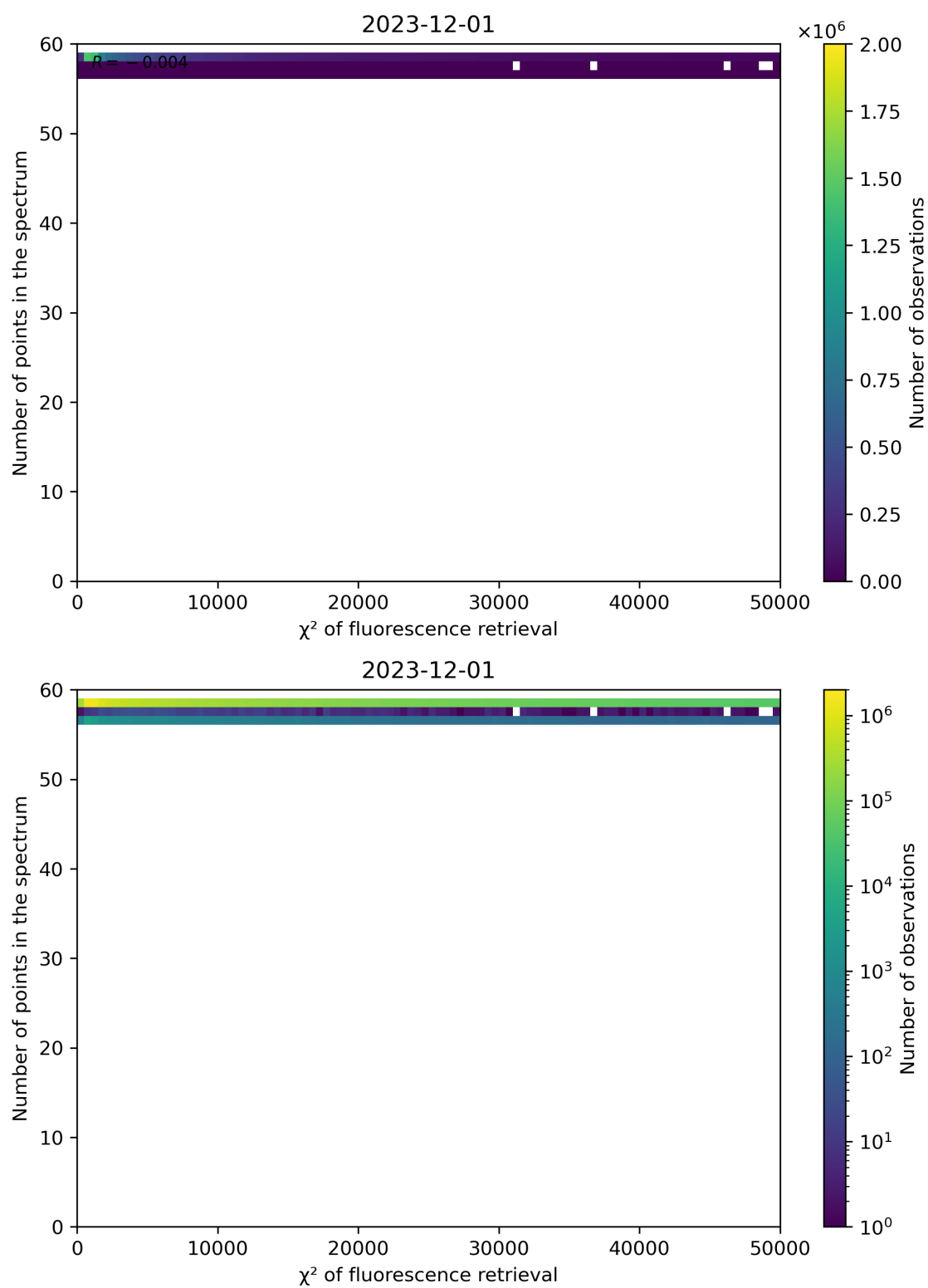
Figure 68: Scatter density plot of “ \chi^2 of fluorescence retrieval” against “Number of points in the spectrum” for 2023-11-30 to 2023-12-02.
