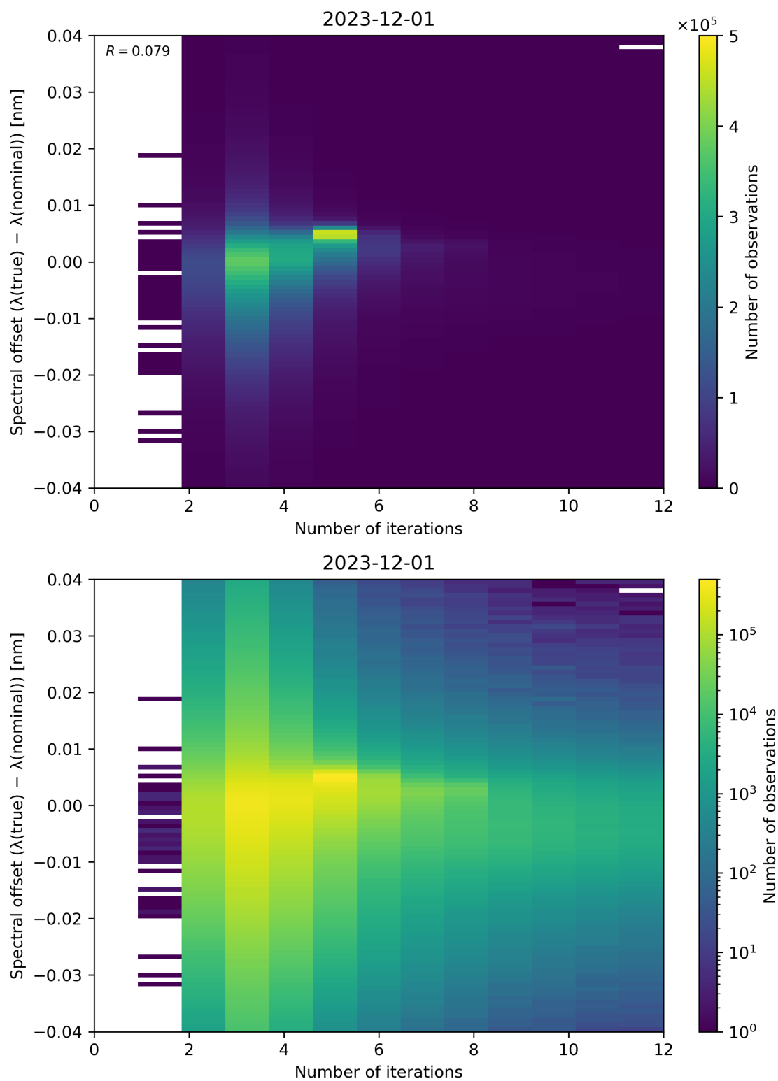
Figure 100: Scatter density plot of “Number of iterations” against “Spectral offset ( \lambda(\text{true}) - \lambda(\text{nominal}) )” for 2023-11-30 to 2023-12-02.
