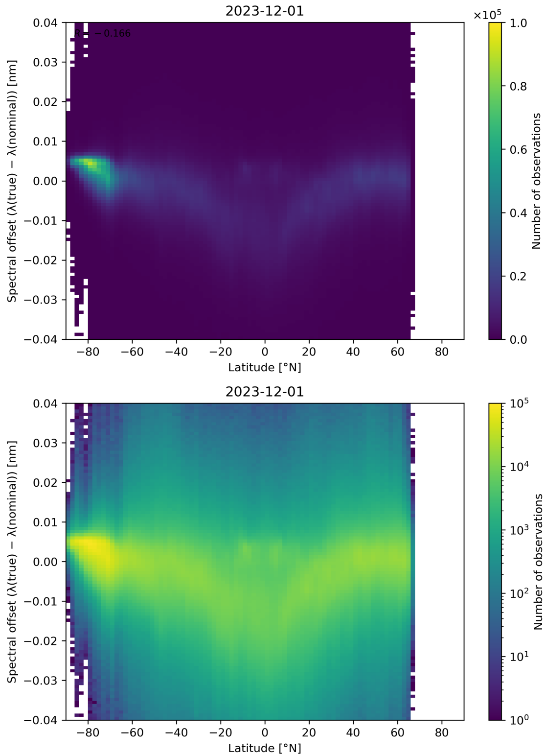
Figure 96: Scatter density plot of “Latitude” against “Spectral offset ( \lambda(\text{true}) - \lambda(\text{nominal}) )” for 2023-11-30 to 2023-12-02.
