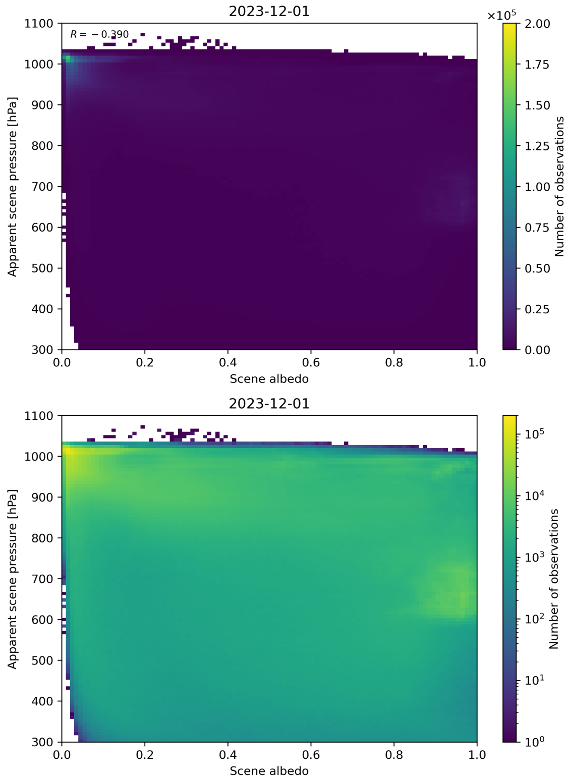
Figure 102: Scatter density plot of “Scene albedo” against “Apparent scene pressure” for 2023-11-30 to 2023-12-02.
