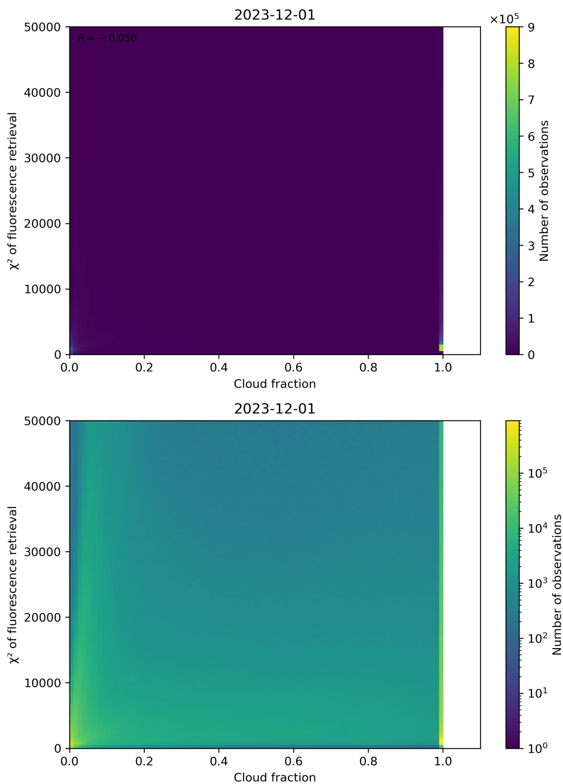
Figure 71: Scatter density plot of “Cloud fraction” against “ \chi^2 of fluorescence retrieval” for 2023-11-30 to 2023-12-02.
