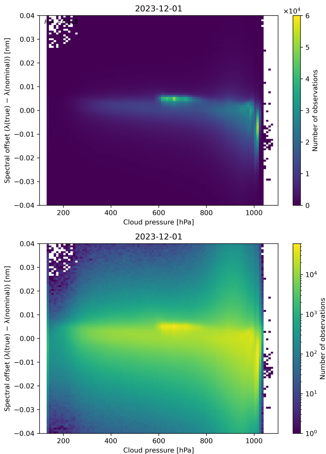
Figure 84: Scatter density plot of “Cloud pressure” against “Spectral offset ( \lambda(\text{true}) - \lambda(\text{nominal}) )” for 2023-11-30 to 2023-12-02.
