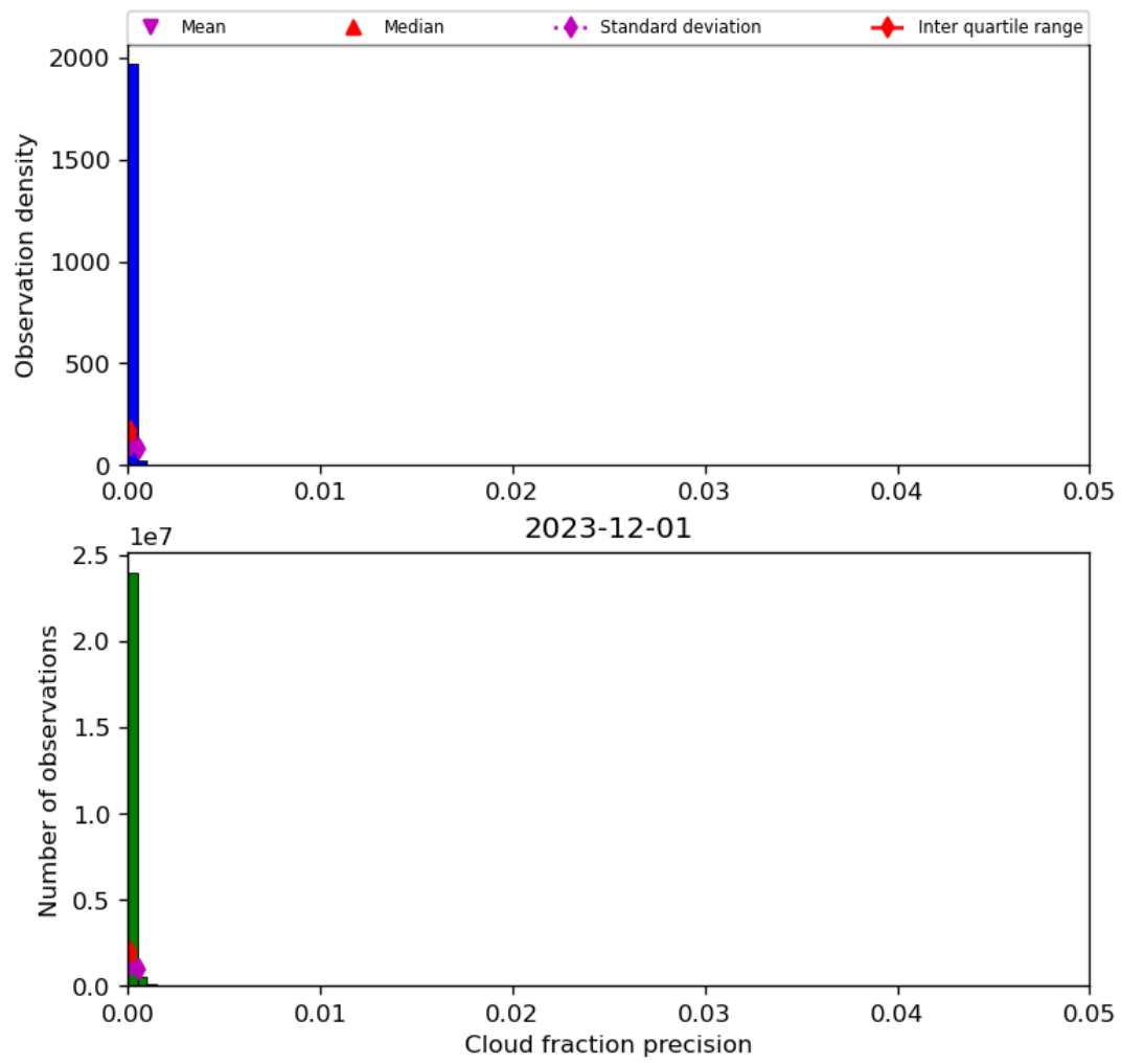
Figure 33: Histogram of “Cloud fraction precision” for 2023-11-30 to 2023-12-02
