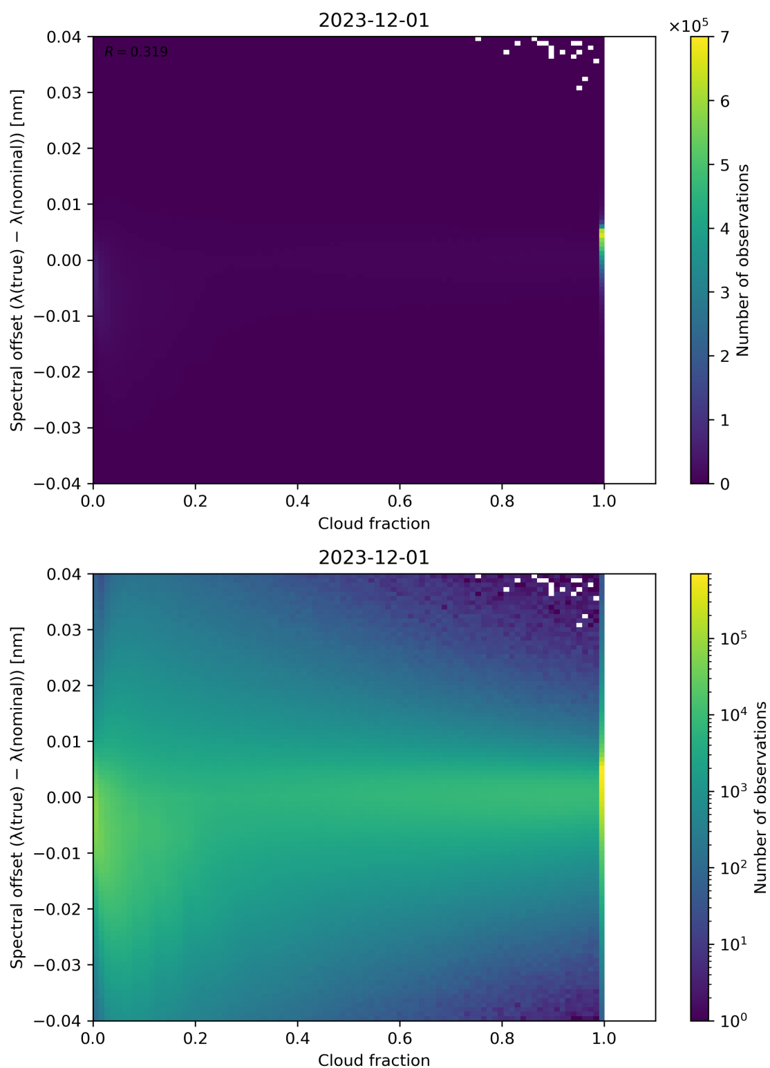
Figure 76: Scatter density plot of “Cloud fraction” against “Spectral offset ( \lambda(\text{true}) - \lambda(\text{nominal}) )” for 2023-11-30 to 2023-12-02.
