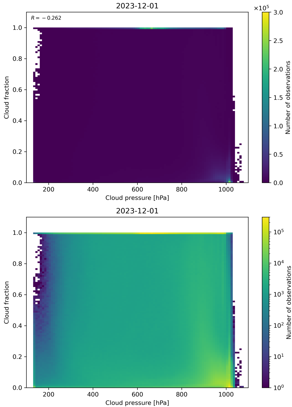
Figure 79: Scatter density plot of “Cloud pressure” against “Cloud fraction” for 2023-11-30 to 2023-12-02.
