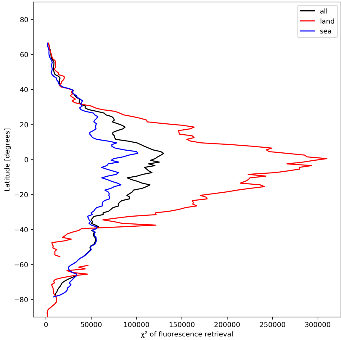
Figure 25: Zonal average of “ \chi^2 of fluorescence retrieval” for 2023-11-30 to 2023-12-02.
