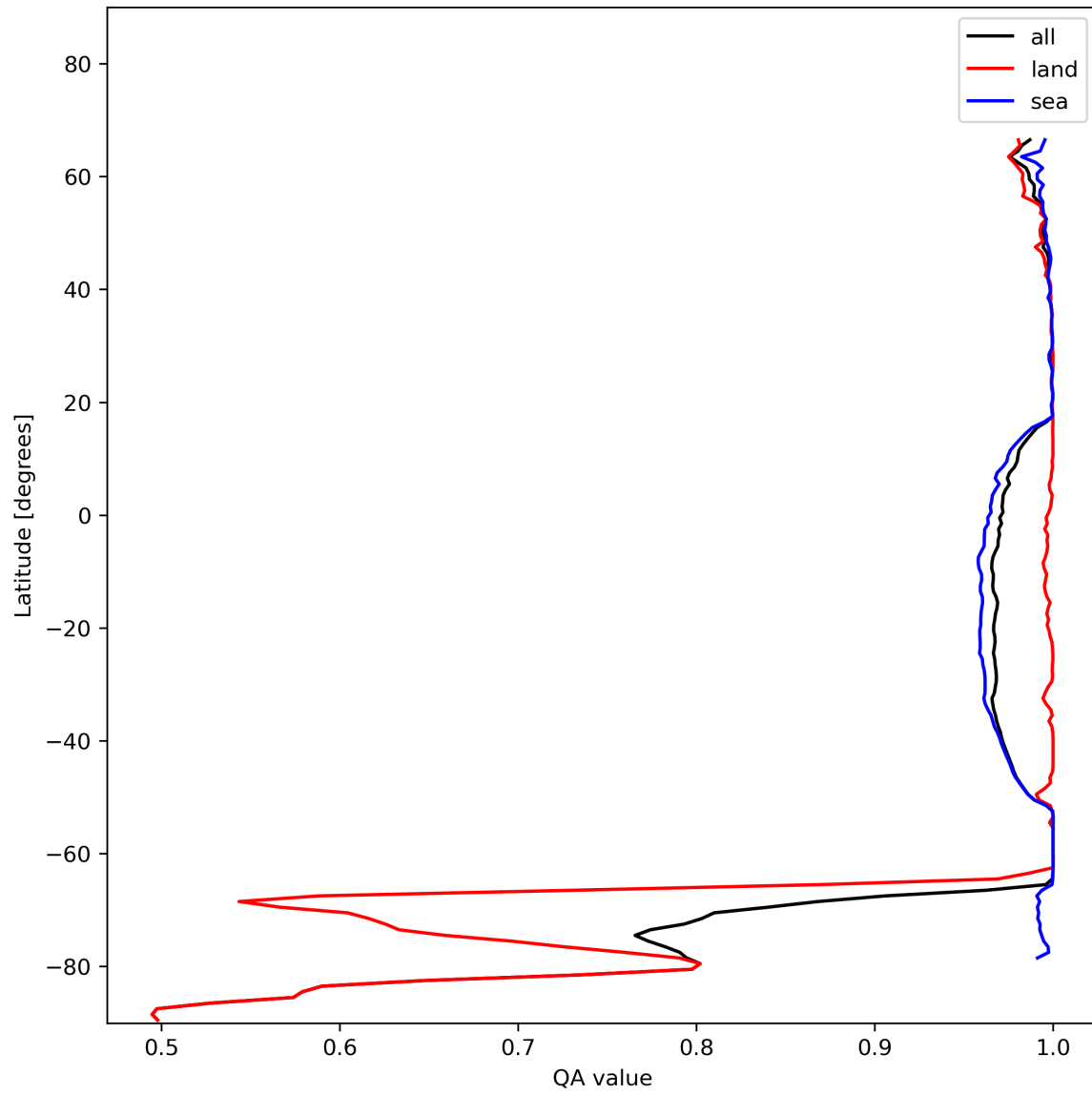
Figure 12: Zonal average of “QA value” for 2023-11-30 to 2023-12-02.
