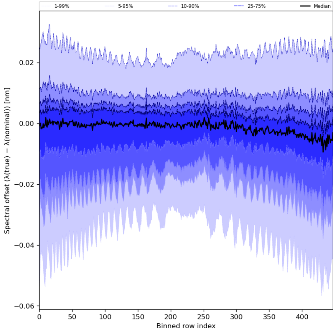
Figure 62: Along track statistics of “Spectral offset ( \lambda(\text{true}) - \lambda(\text{nominal}) )” for 2023-11-30 to 2023-12-02
