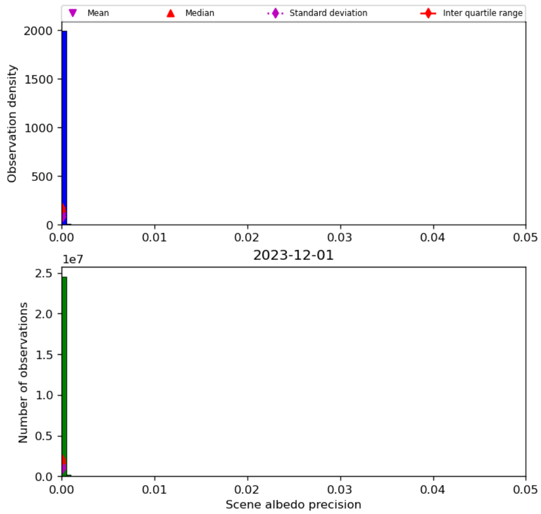
Figure 35: Histogram of “Scene albedo precision” for 2023-11-30 to 2023-12-02
