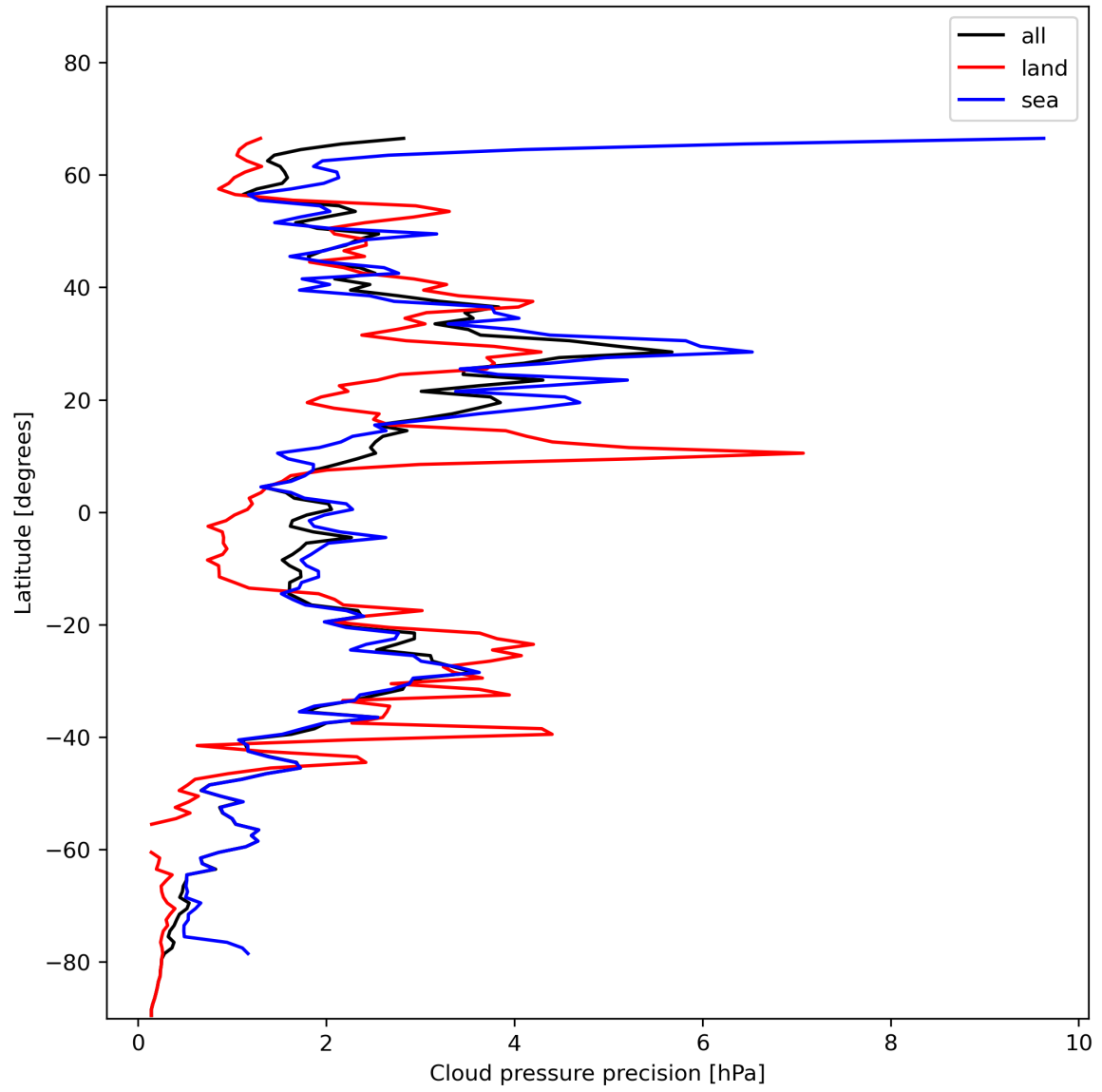
Figure 14: Zonal average of “Cloud pressure precision” for 2023-11-30 to 2023-12-02.
