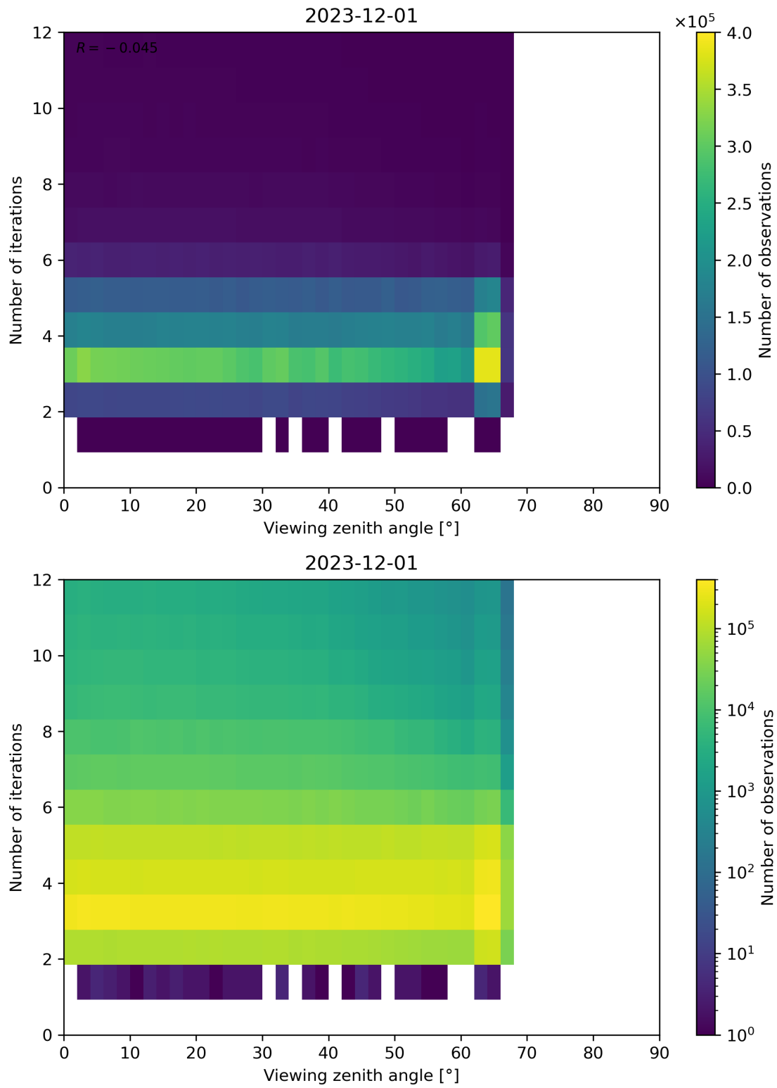
Figure 124: Scatter density plot of “Viewing zenith angle” against “Number of iterations” for 2023-11-30 to 2023-12-02.
