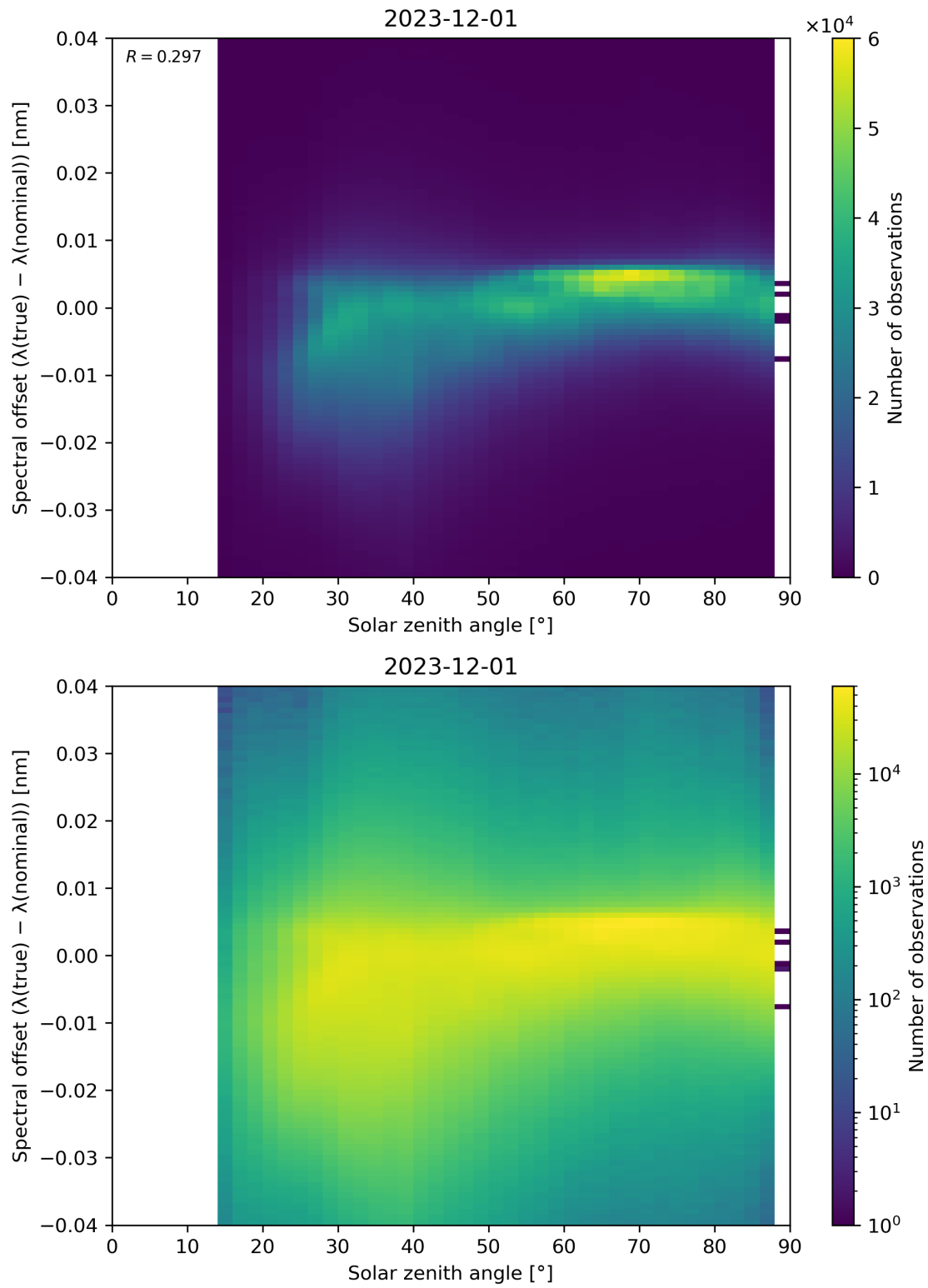
Figure 117: Scatter density plot of “Solar zenith angle” against “Spectral offset ( \lambda(\text{true}) - \lambda(\text{nominal}) )” for 2023-11-30 to 2023-12-02.
