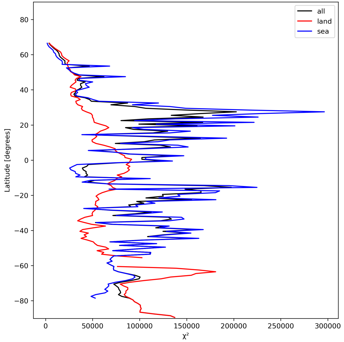
Figure 21: Zonal average of “ \chi^2 ” for 2023-11-30 to 2023-12-02.
