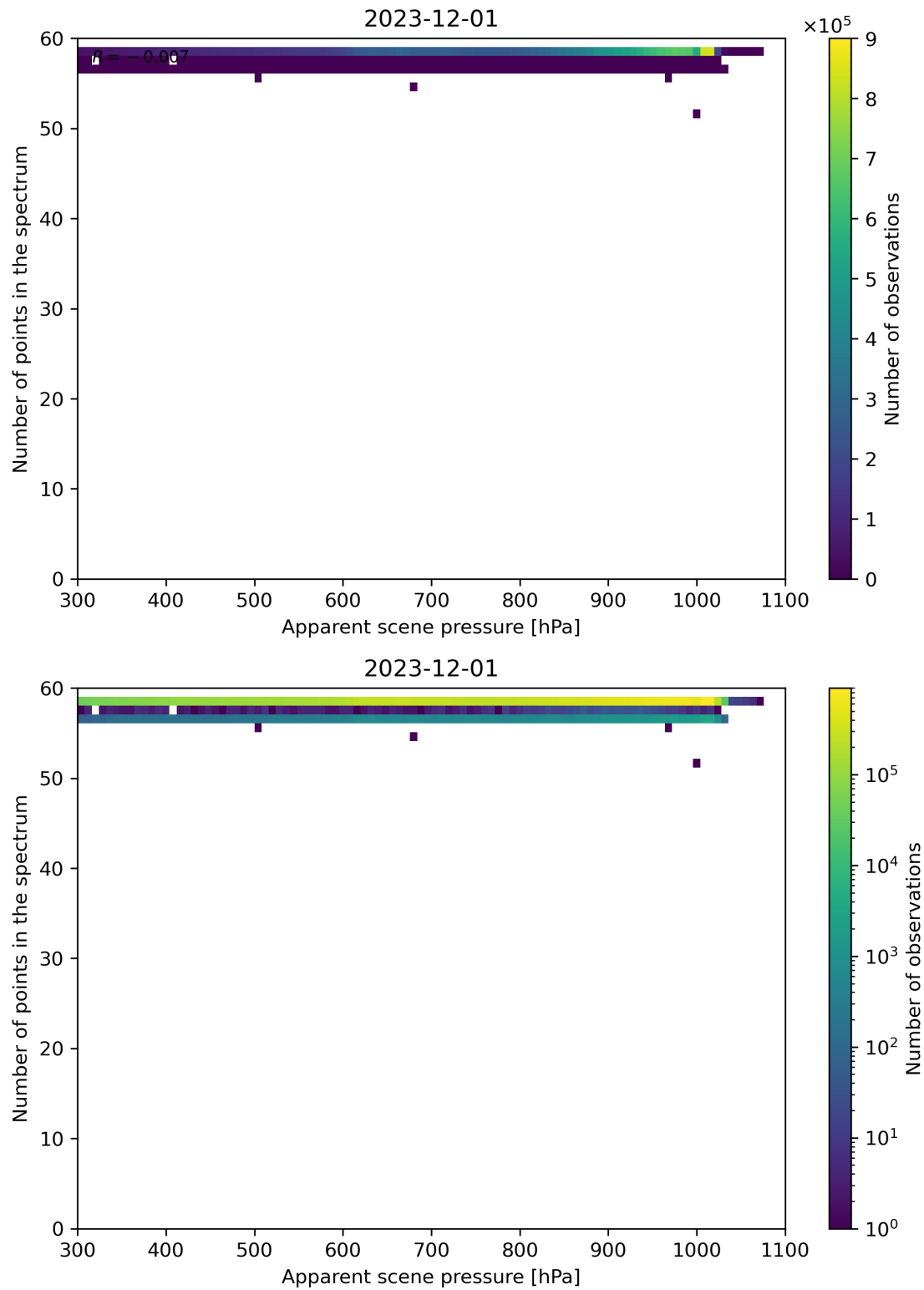
Figure 66: Scatter density plot of “Apparent scene pressure” against “Number of points in the spectrum” for 2023-11-30 to 2023-12-02.
