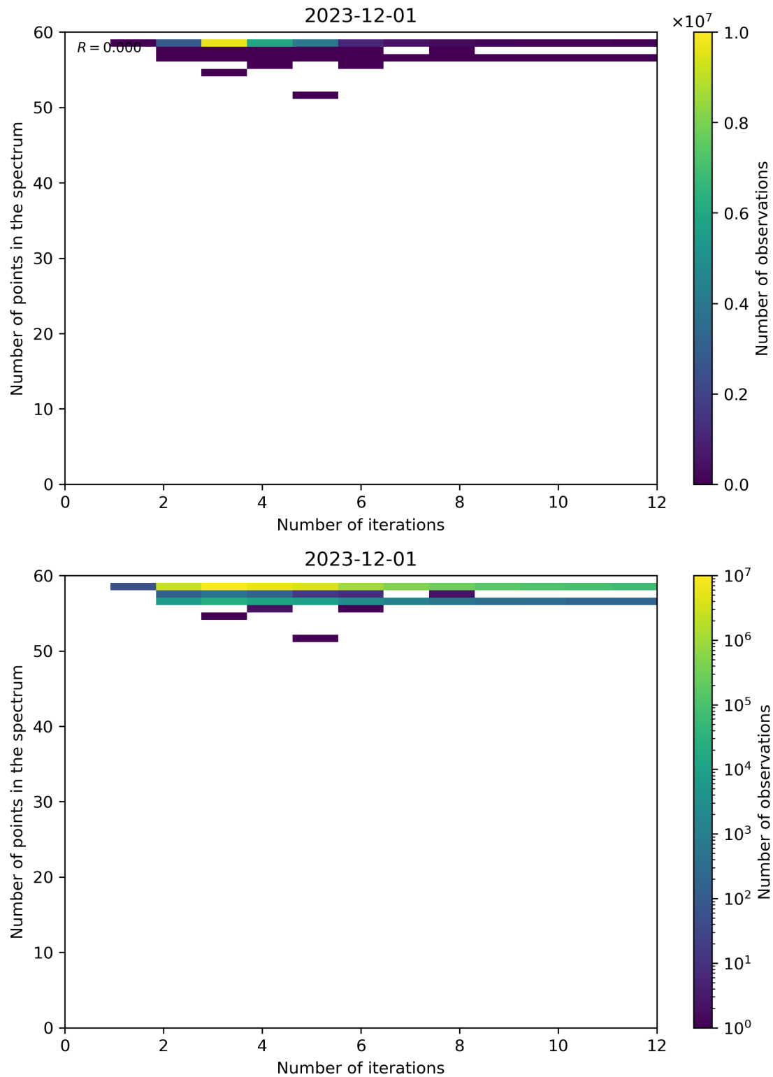
Figure 99: Scatter density plot of “Number of iterations” against “Number of points in the spectrum” for 2023-11-30 to 2023-12-02.
