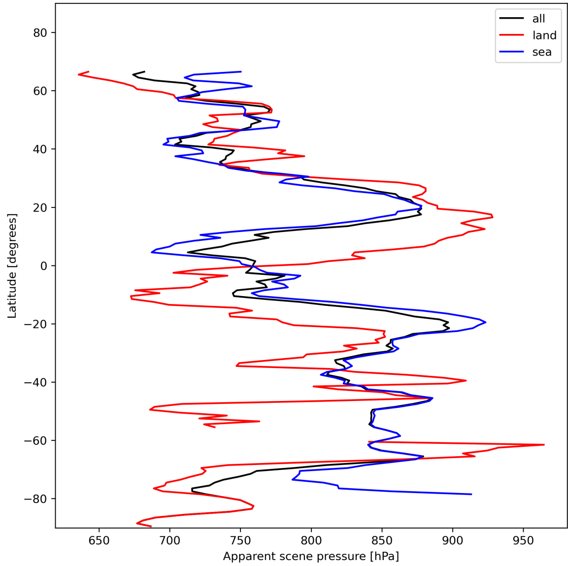
Figure 19: Zonal average of “Apparent scene pressure” for 2023-11-30 to 2023-12-02.
