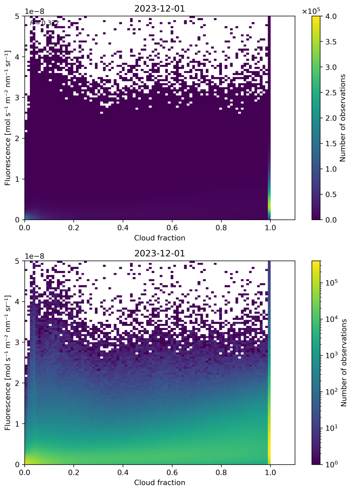
Figure 72: Scatter density plot of “Cloud fraction” against “Fluorescence” for 2023-11-30 to 2023-12-02.
