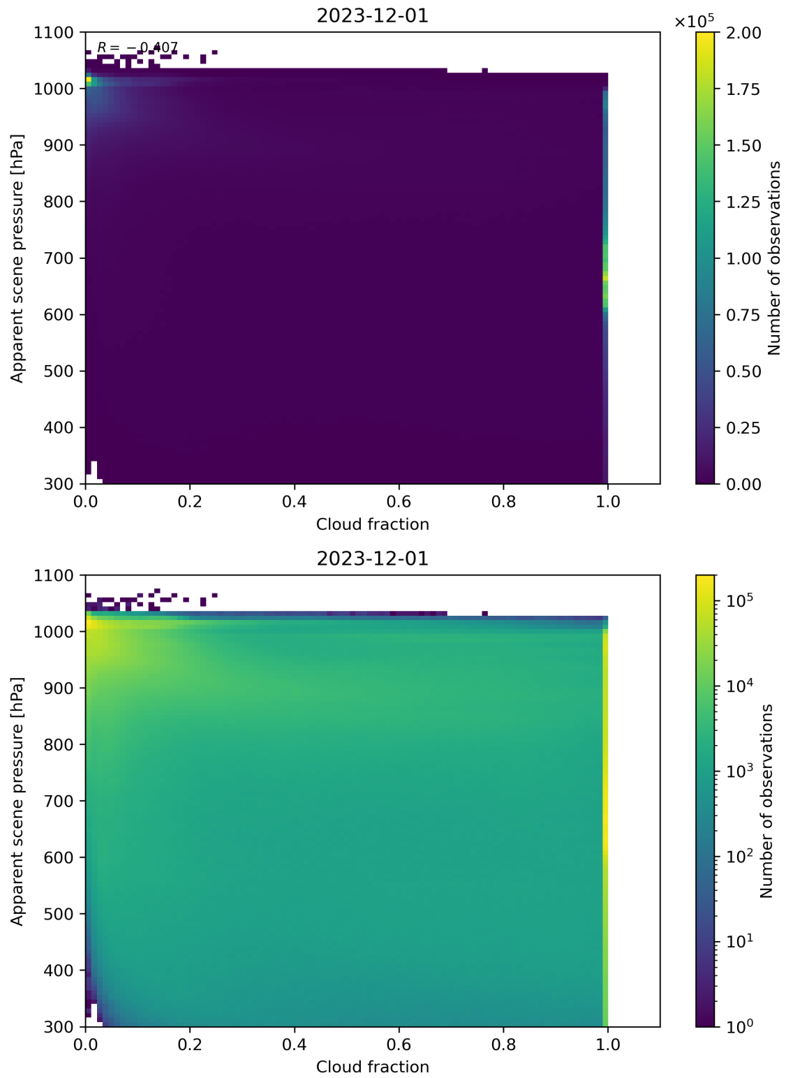
Figure 70: Scatter density plot of “Cloud fraction” against “Apparent scene pressure” for 2023-11-30 to 2023-12-02.
