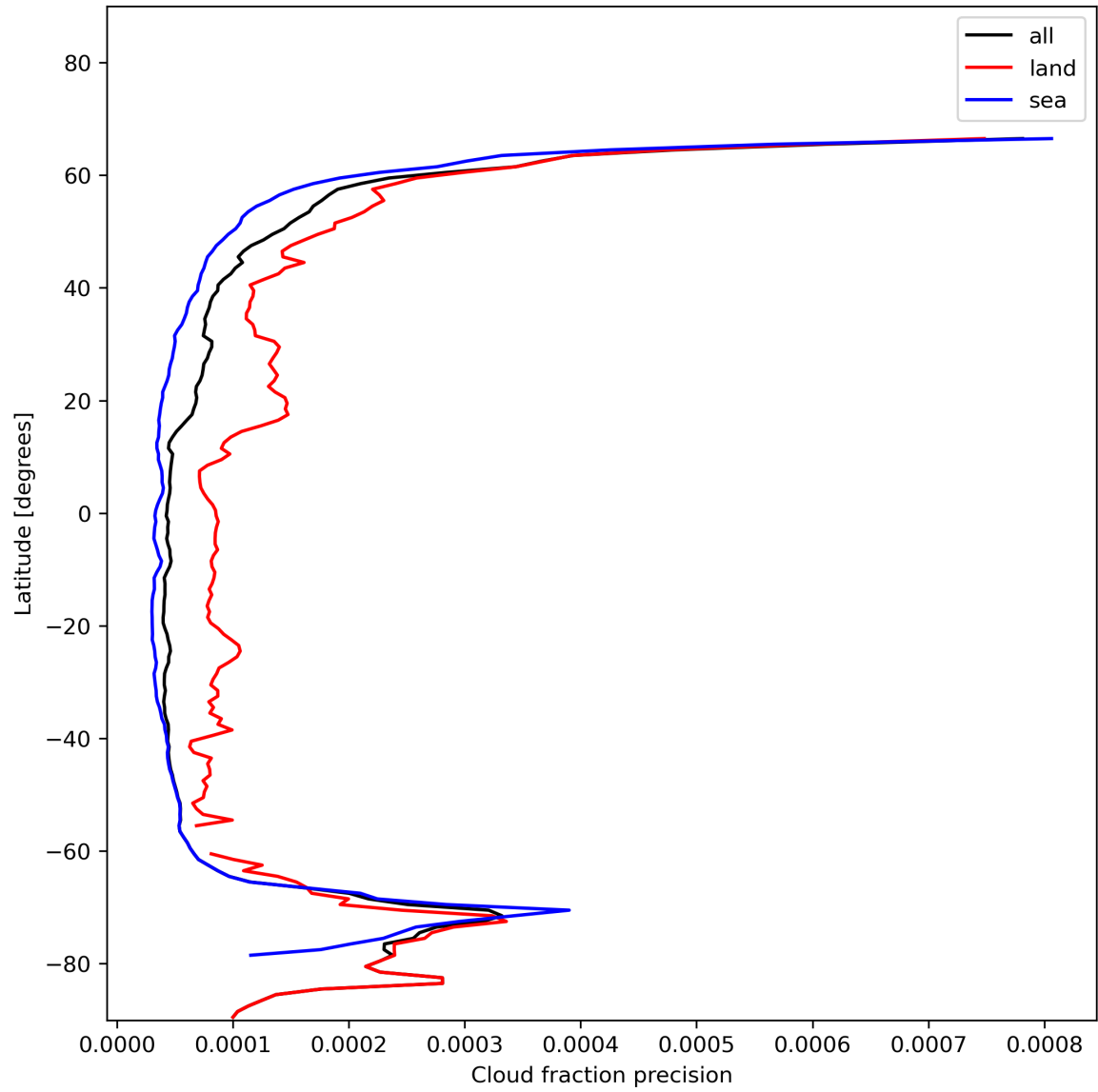
Figure 16: Zonal average of “Cloud fraction precision” for 2023-11-30 to 2023-12-02.
