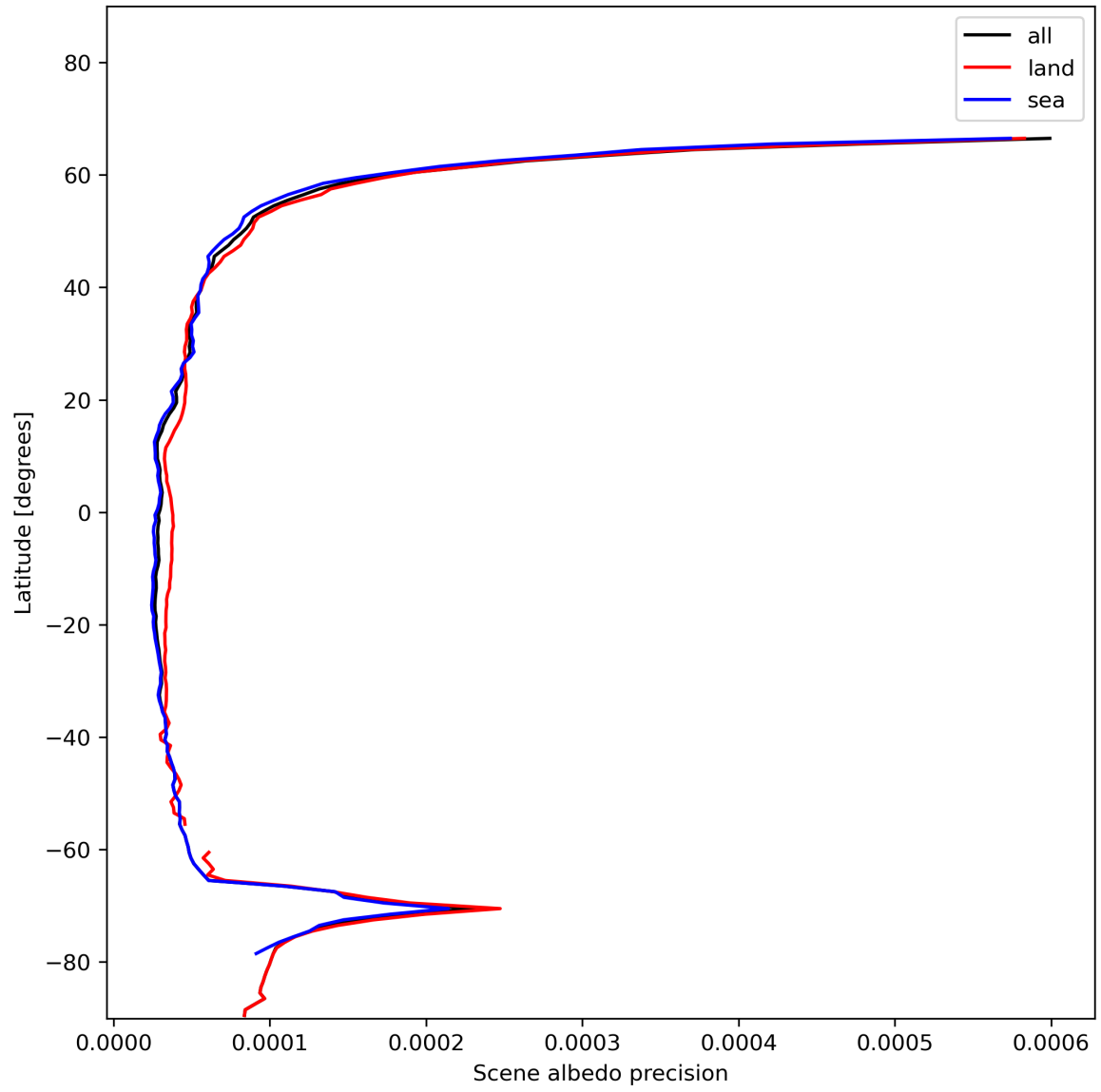
Figure 18: Zonal average of “Scene albedo precision” for 2023-11-30 to 2023-12-02.
