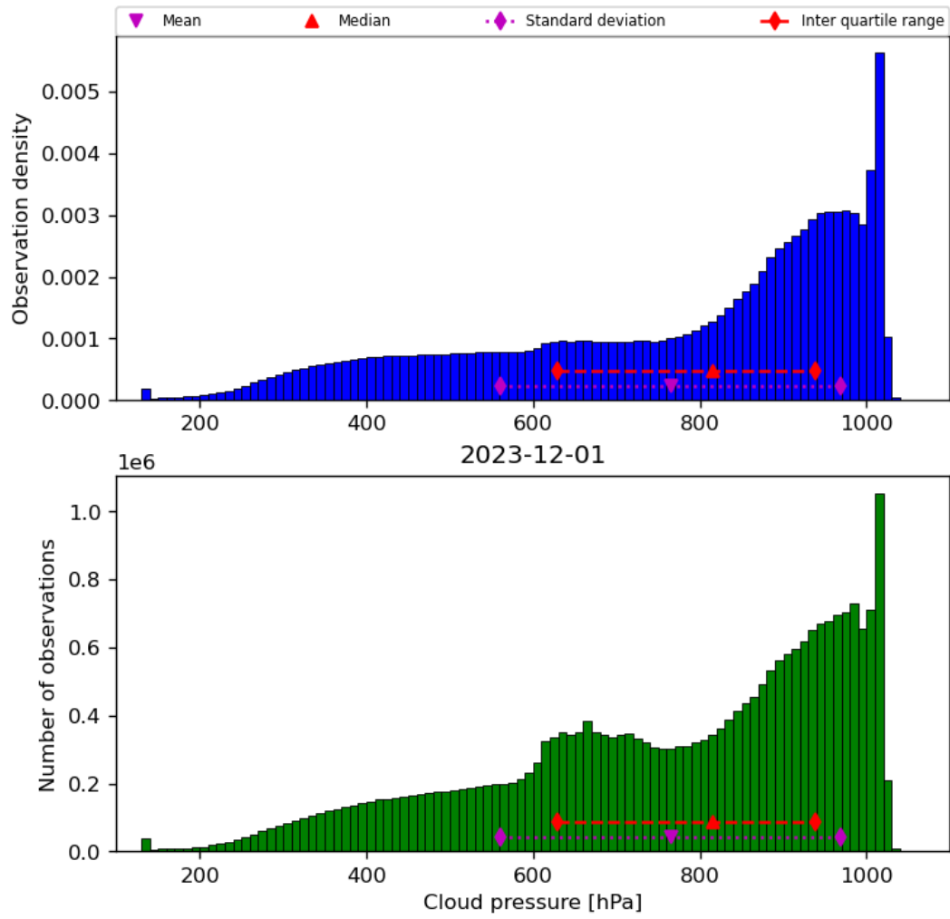
Figure 30: Histogram of “Cloud pressure” for 2023-11-30 to 2023-12-02
