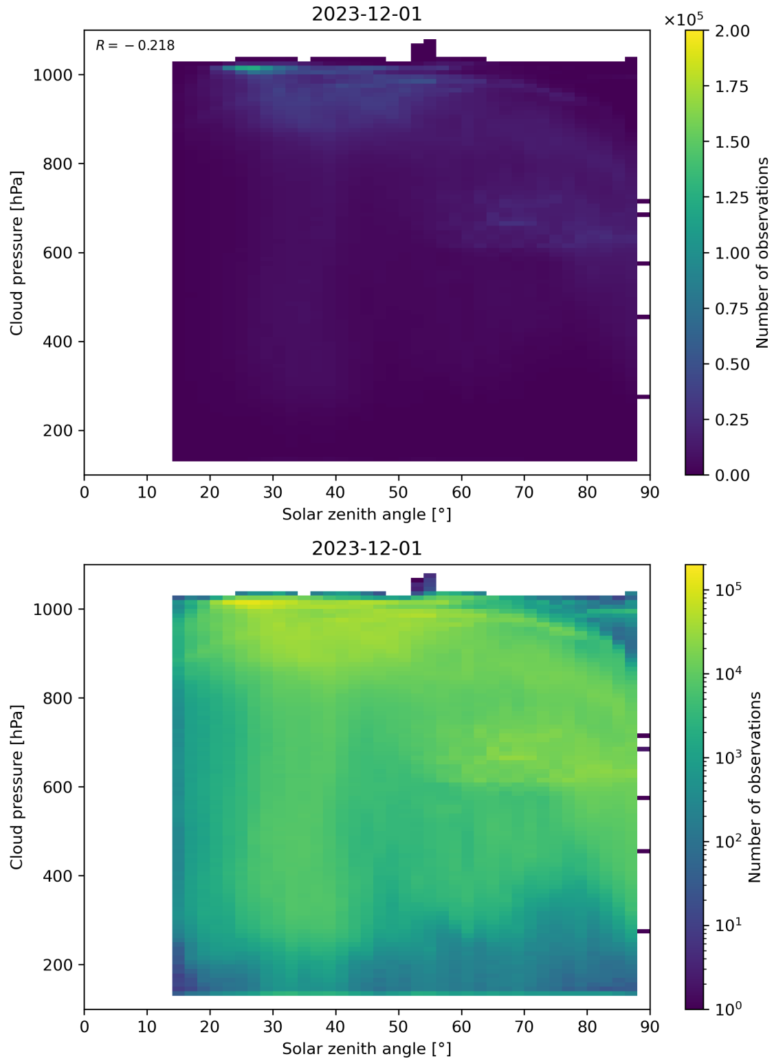
Figure 111: Scatter density plot of “Solar zenith angle” against “Cloud pressure” for 2023-11-30 to 2023-12-02.
