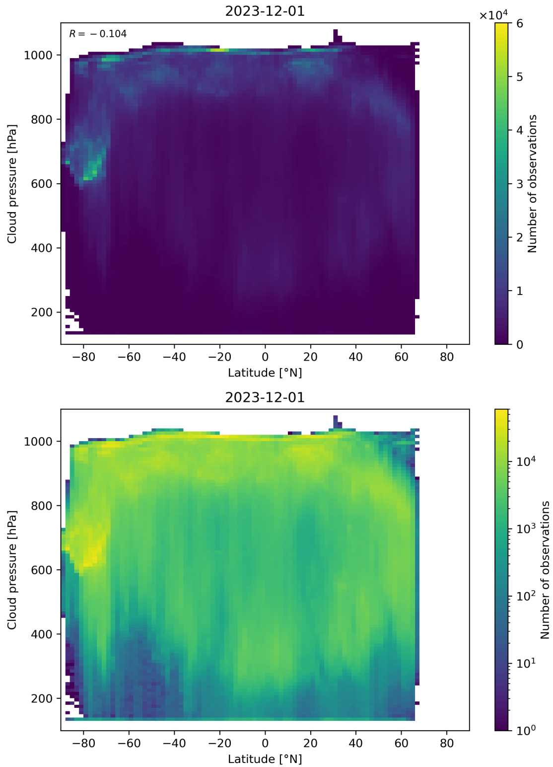
Figure 91: Scatter density plot of “Latitude” against “Cloud pressure” for 2023-11-30 to 2023-12-02.
