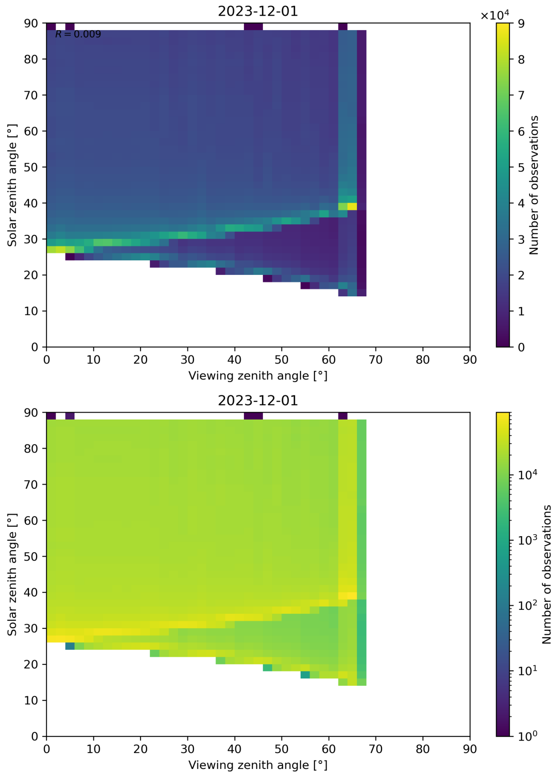
Figure 127: Scatter density plot of “Viewing zenith angle” against “Solar zenith angle” for 2023-11-30 to 2023-12-02.
