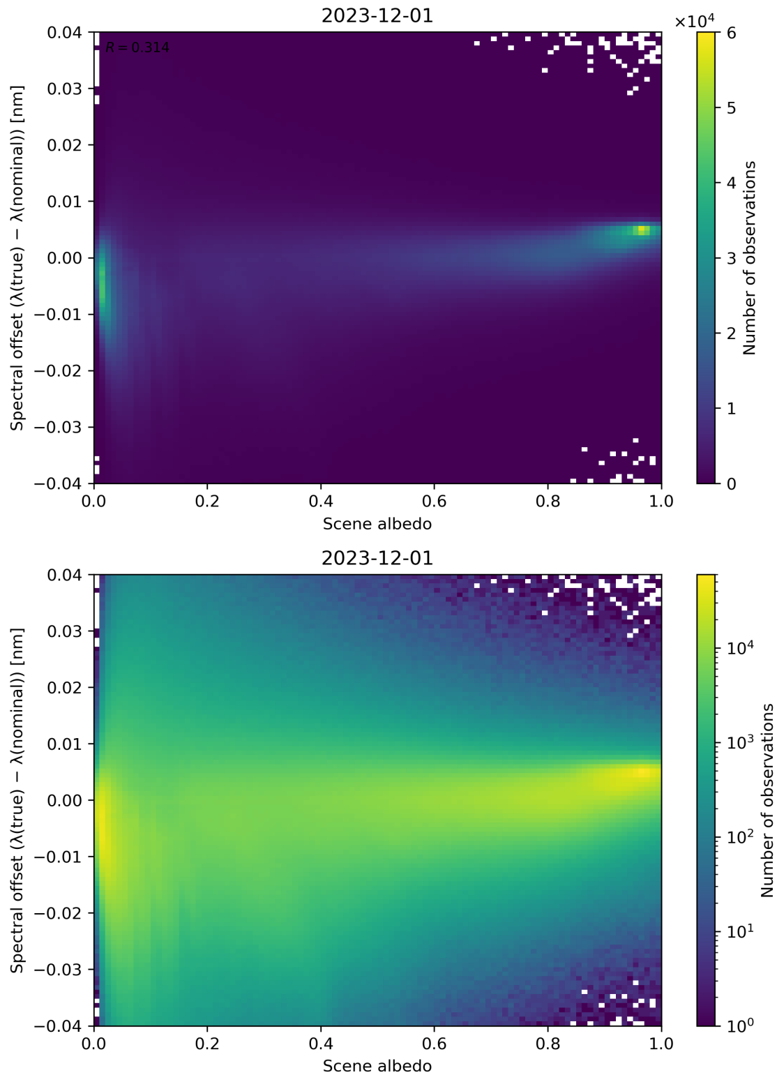
Figure 107: Scatter density plot of “Scene albedo” against “Spectral offset ( \lambda(\text{true}) - \lambda(\text{nominal}) )” for 2023-11-30 to 2023-12-02.
