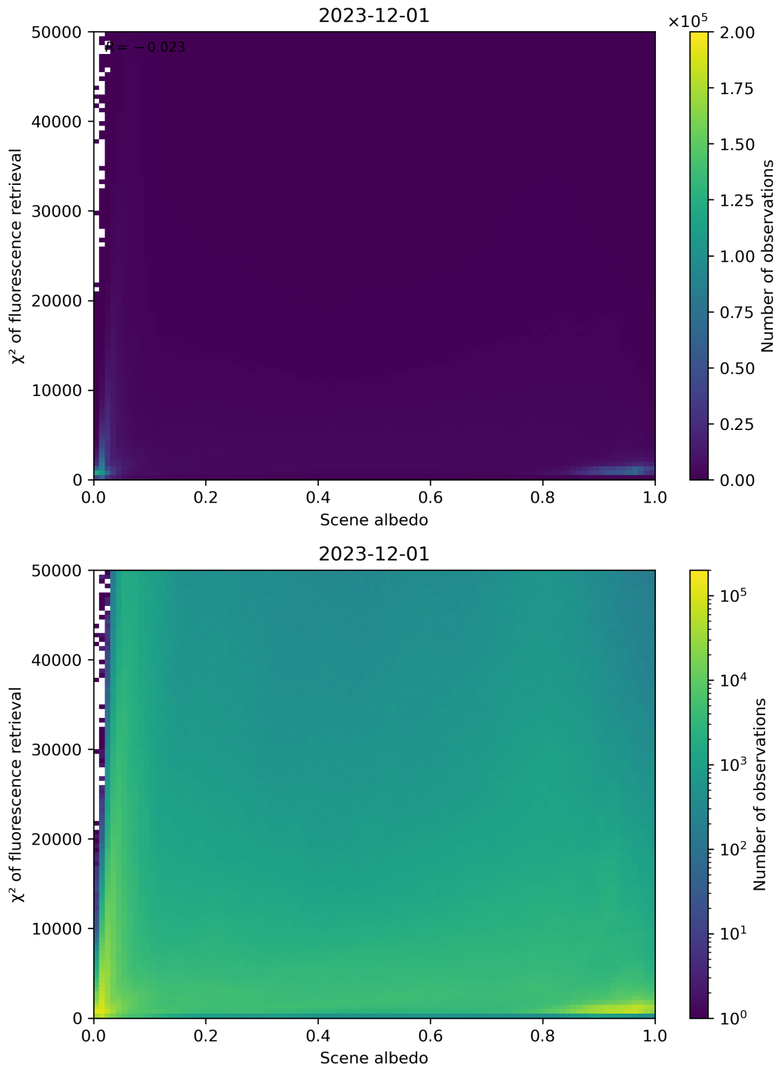
Figure 103: Scatter density plot of “Scene albedo” against “ \chi^2 of fluorescence retrieval” for 2023-11-30 to 2023-12-02.
