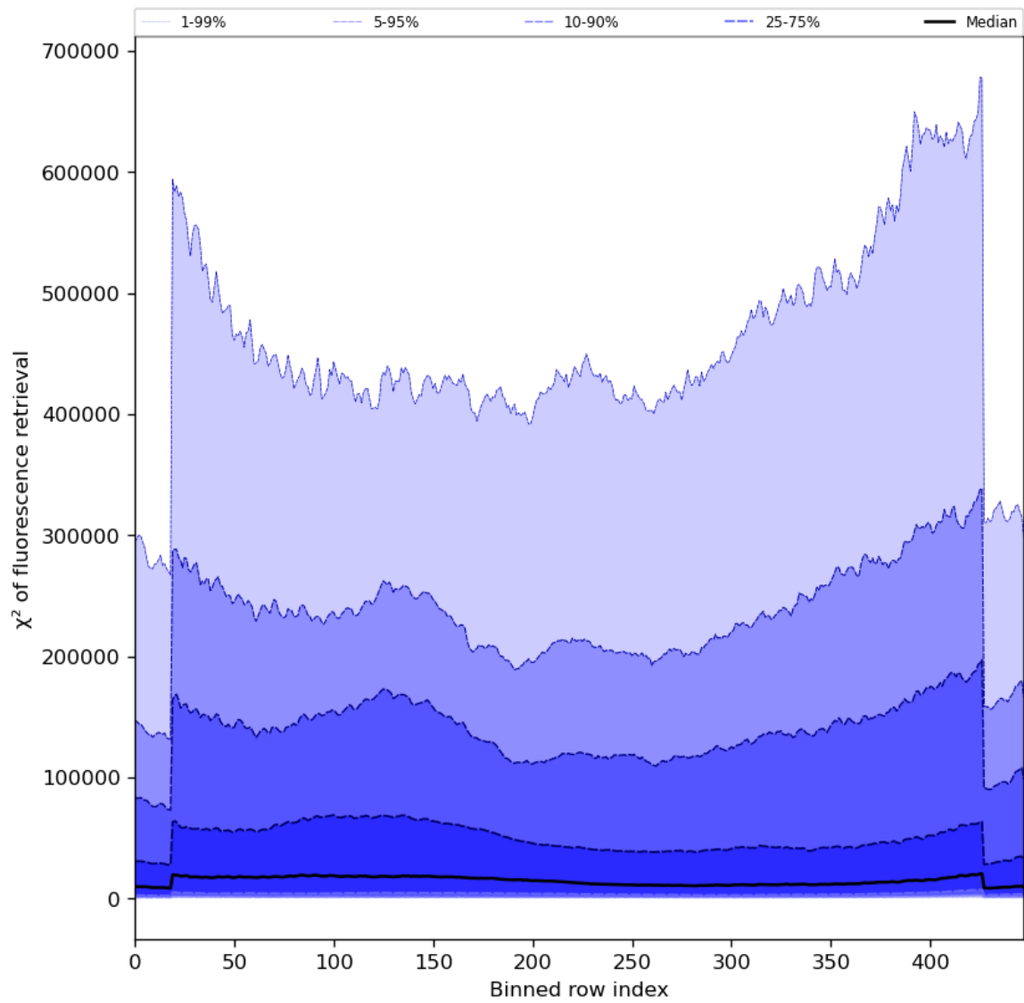
Figure 59: Along track statistics of “ \chi^2 of fluorescence retrieval” for 2023-11-30 to 2023-12-02
