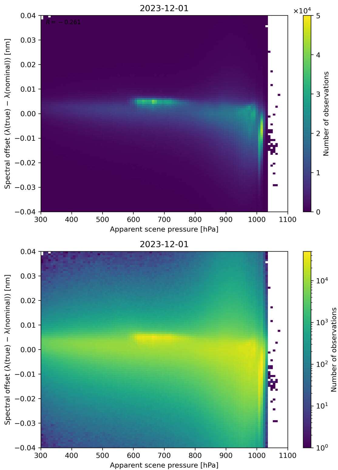
Figure 67: Scatter density plot of “Apparent scene pressure” against “Spectral offset ( \lambda(\text{true}) - \lambda(\text{nominal}) )” for 2023-11-30 to 2023-12-02.
