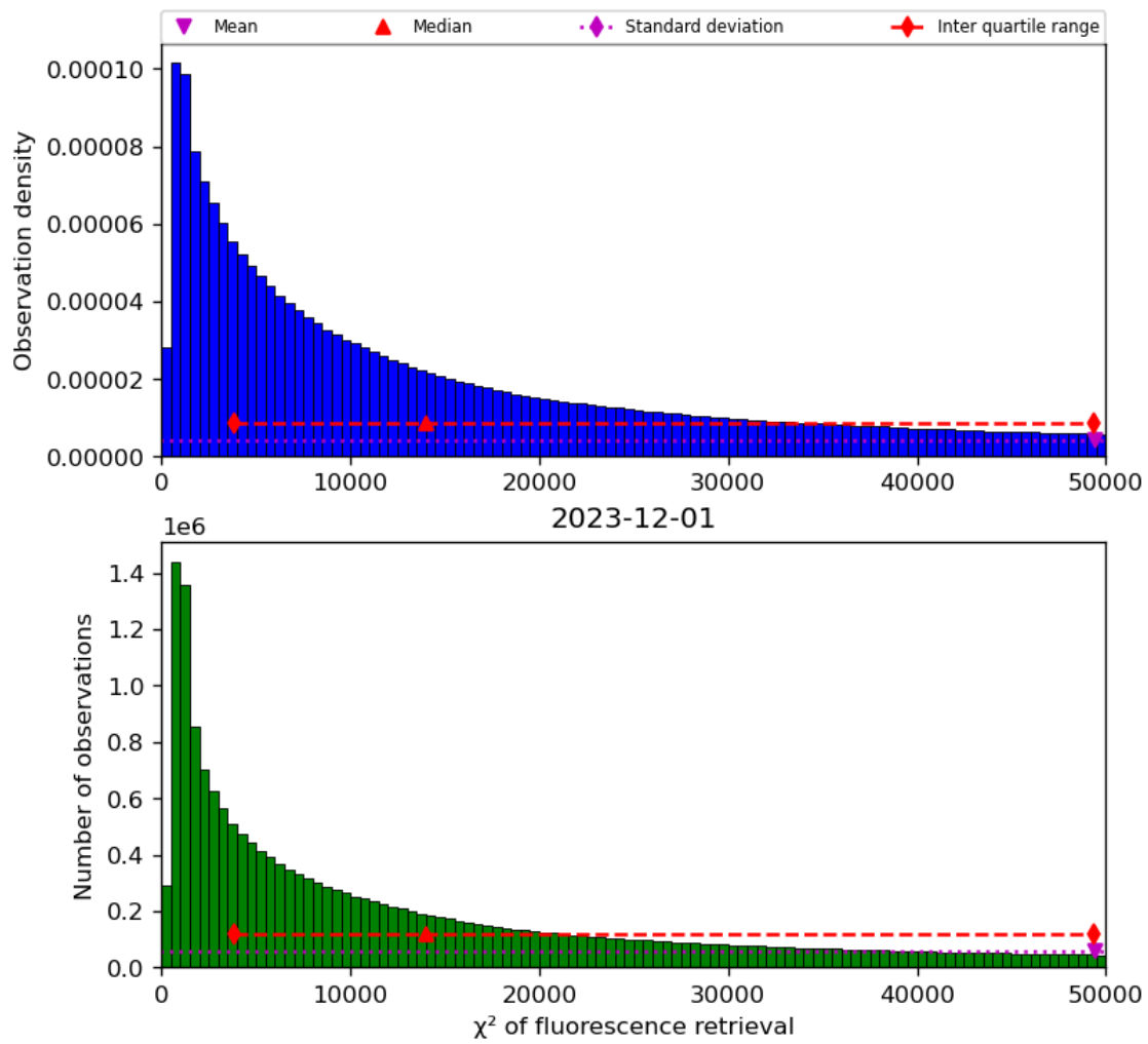
Figure 42: Histogram of “ \chi^2 of fluorescence retrieval” for 2023-11-30 to 2023-12-02
