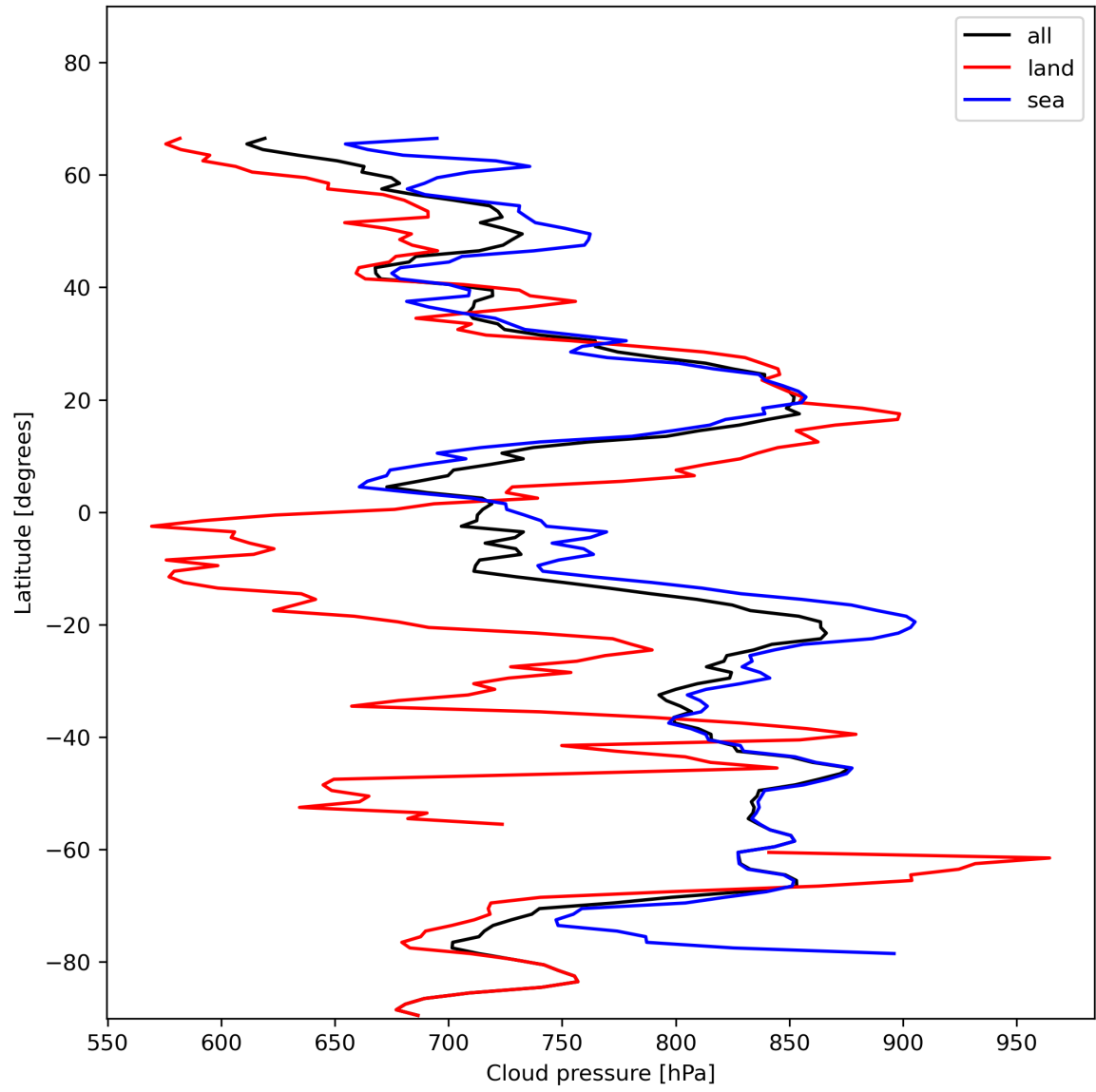
Figure 13: Zonal average of “Cloud pressure” for 2023-11-30 to 2023-12-02.
