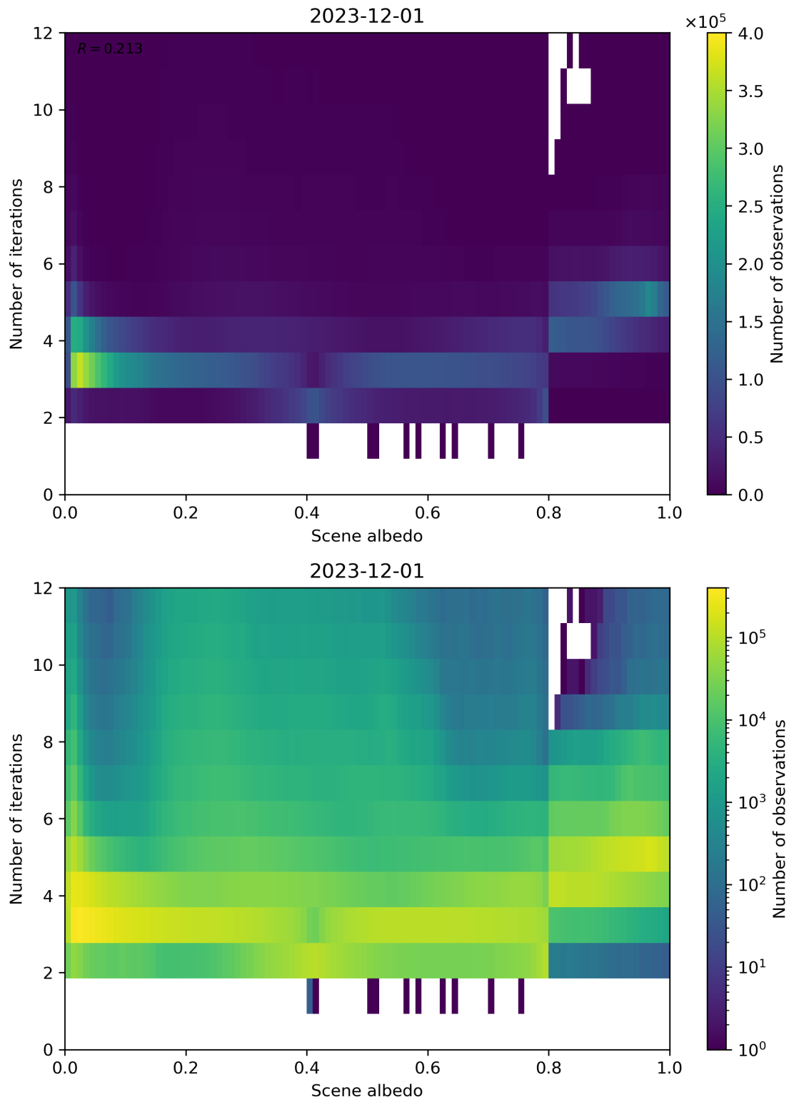
Figure 105: Scatter density plot of “Scene albedo” against “Number of iterations” for 2023-11-30 to 2023-12-02.
