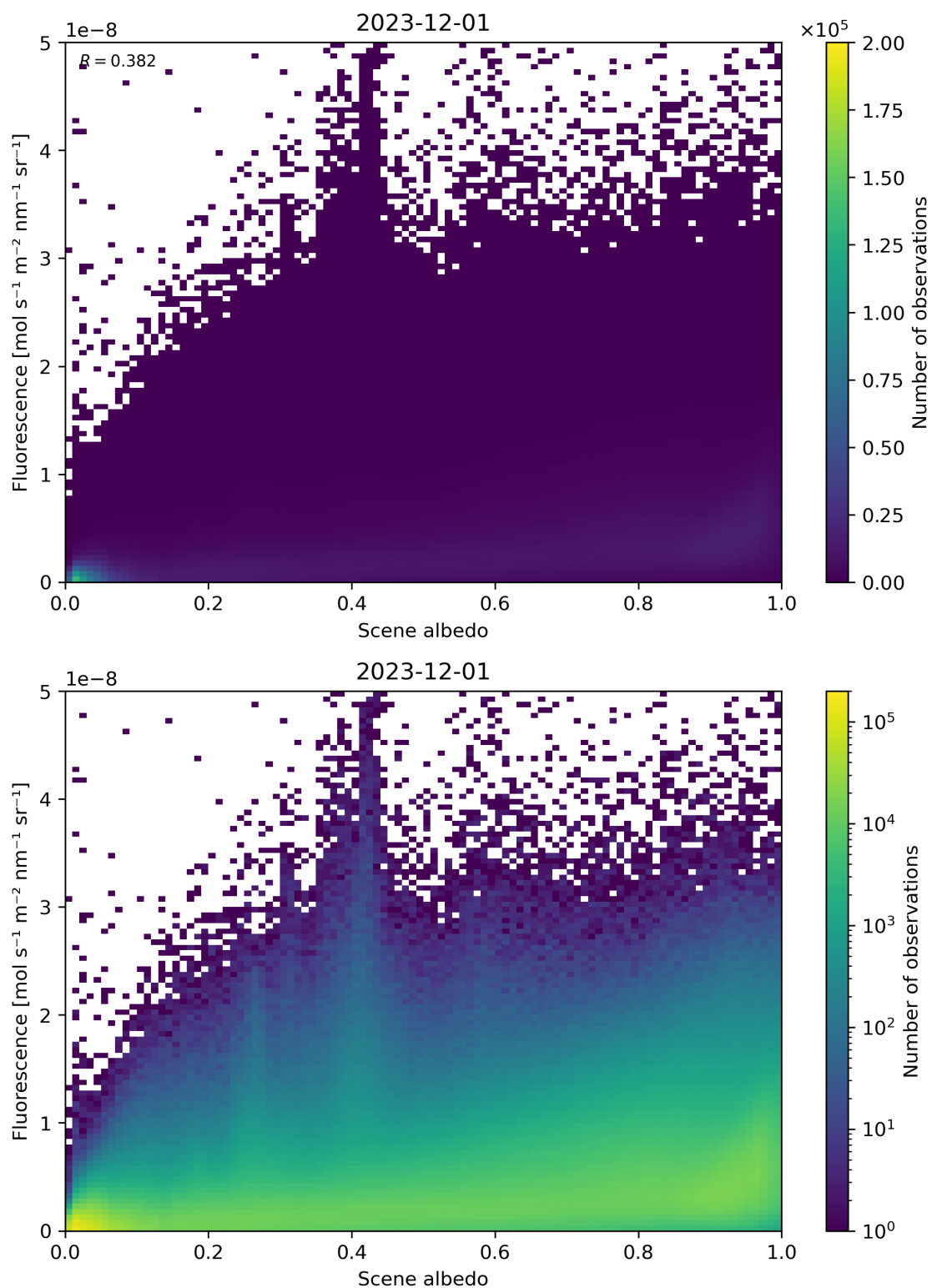
Figure 104: Scatter density plot of “Scene albedo” against “Fluorescence” for 2023-11-30 to 2023-12-02.
