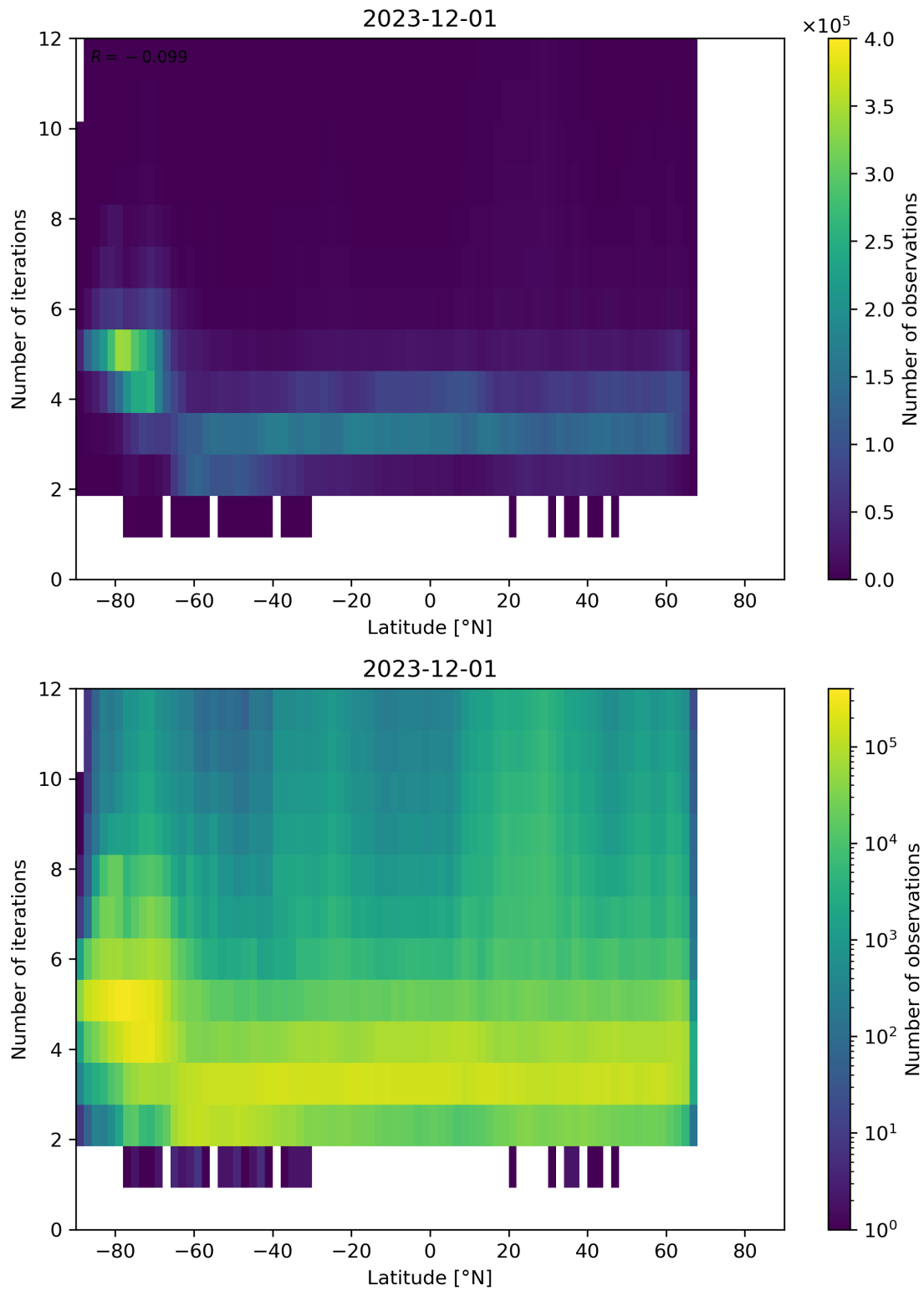
Figure 93: Scatter density plot of “Latitude” against “Number of iterations” for 2023-11-30 to 2023-12-02.
