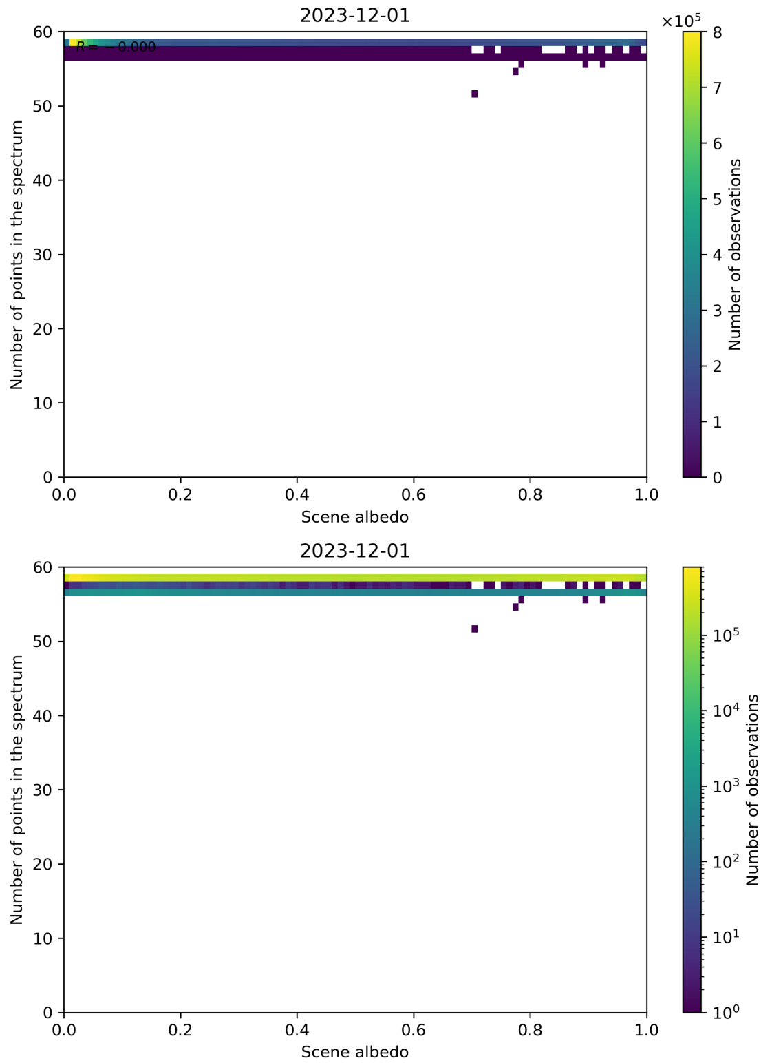
Figure 106: Scatter density plot of “Scene albedo” against “Number of points in the spectrum” for 2023-11-30 to 2023-12-02.
