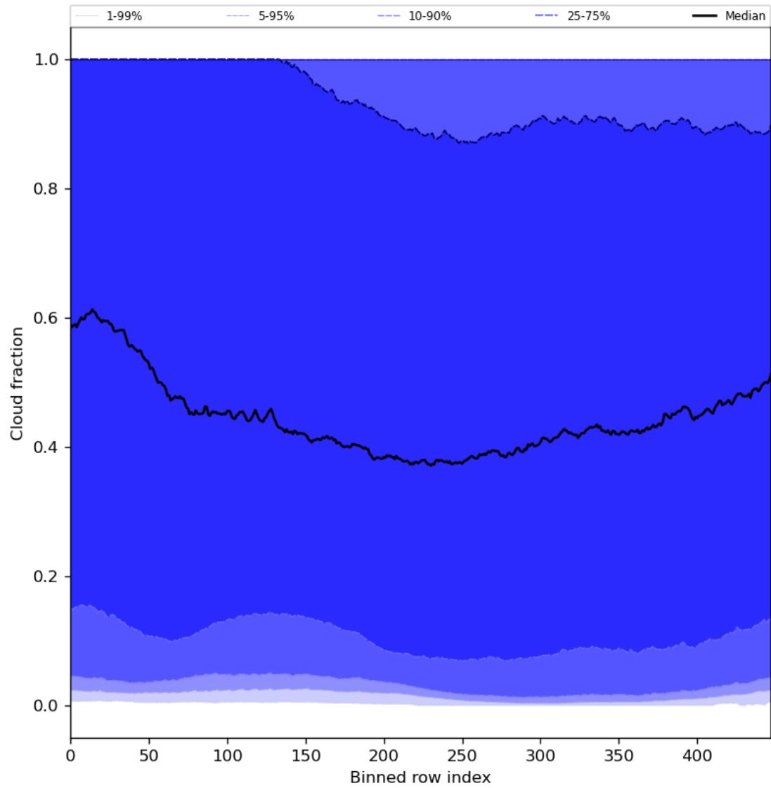
Figure 49: Along track statistics of “Cloud fraction” for 2023-11-30 to 2023-12-02
