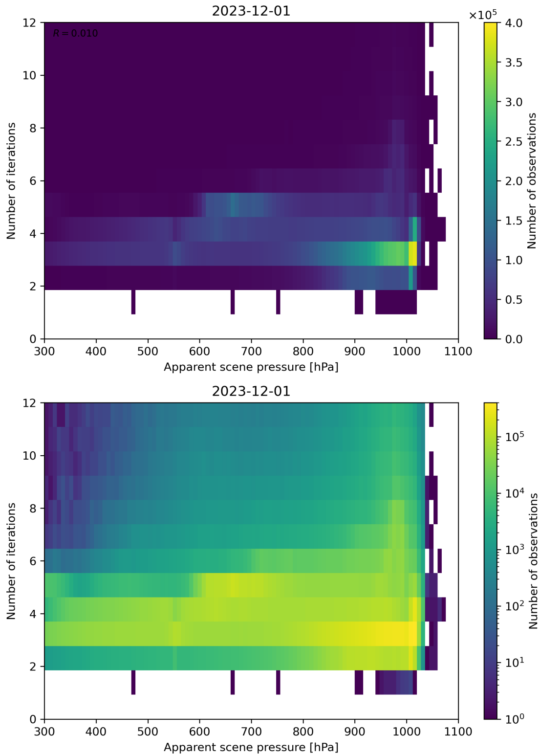
Figure 65: Scatter density plot of “Apparent scene pressure” against “Number of iterations” for 2023-11-30 to 2023-12-02.
