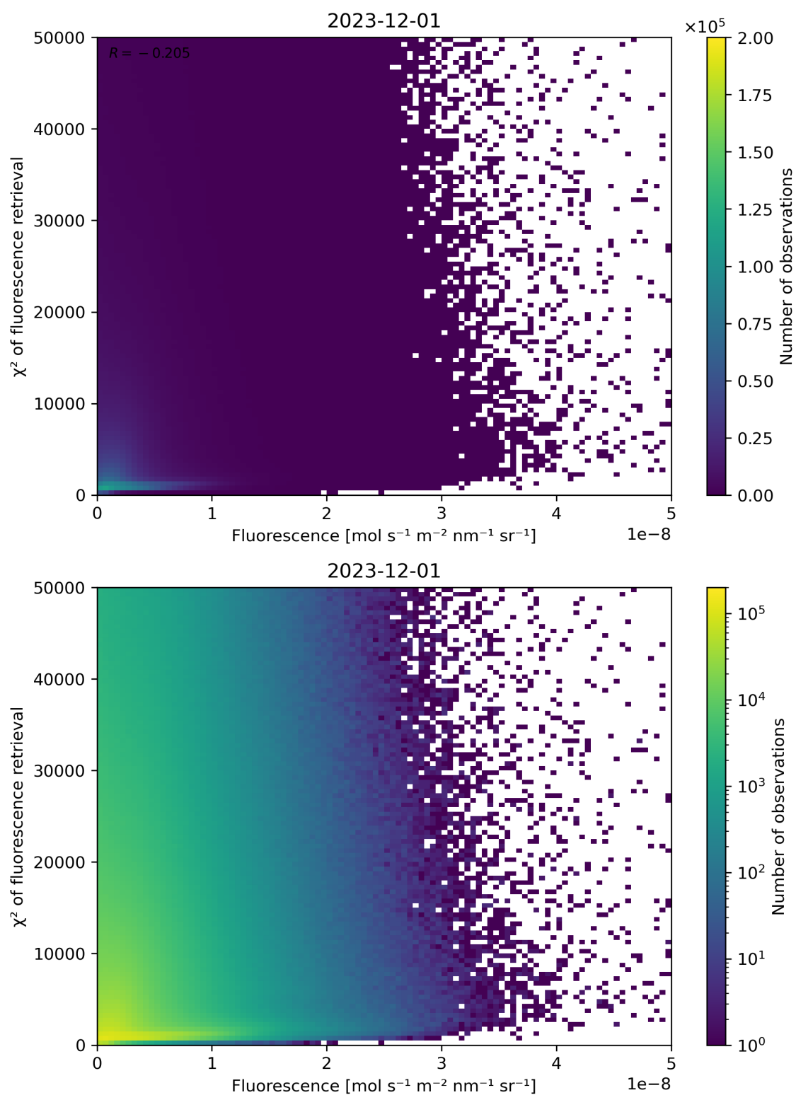
Figure 85: Scatter density plot of “Fluorescence” against “ \chi^2 of fluorescence retrieval” for 2023-11-30 to 2023-12-02.
