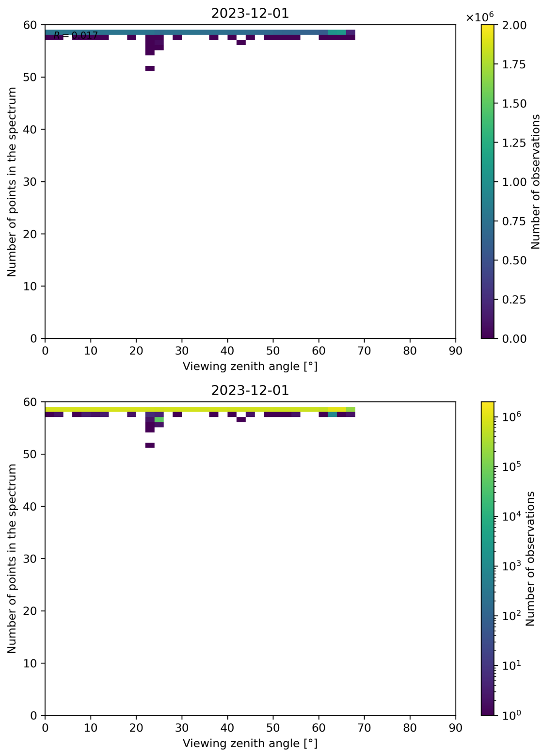
Figure 125: Scatter density plot of “Viewing zenith angle” against “Number of points in the spectrum” for 2023-11-30 to 2023-12-02.
