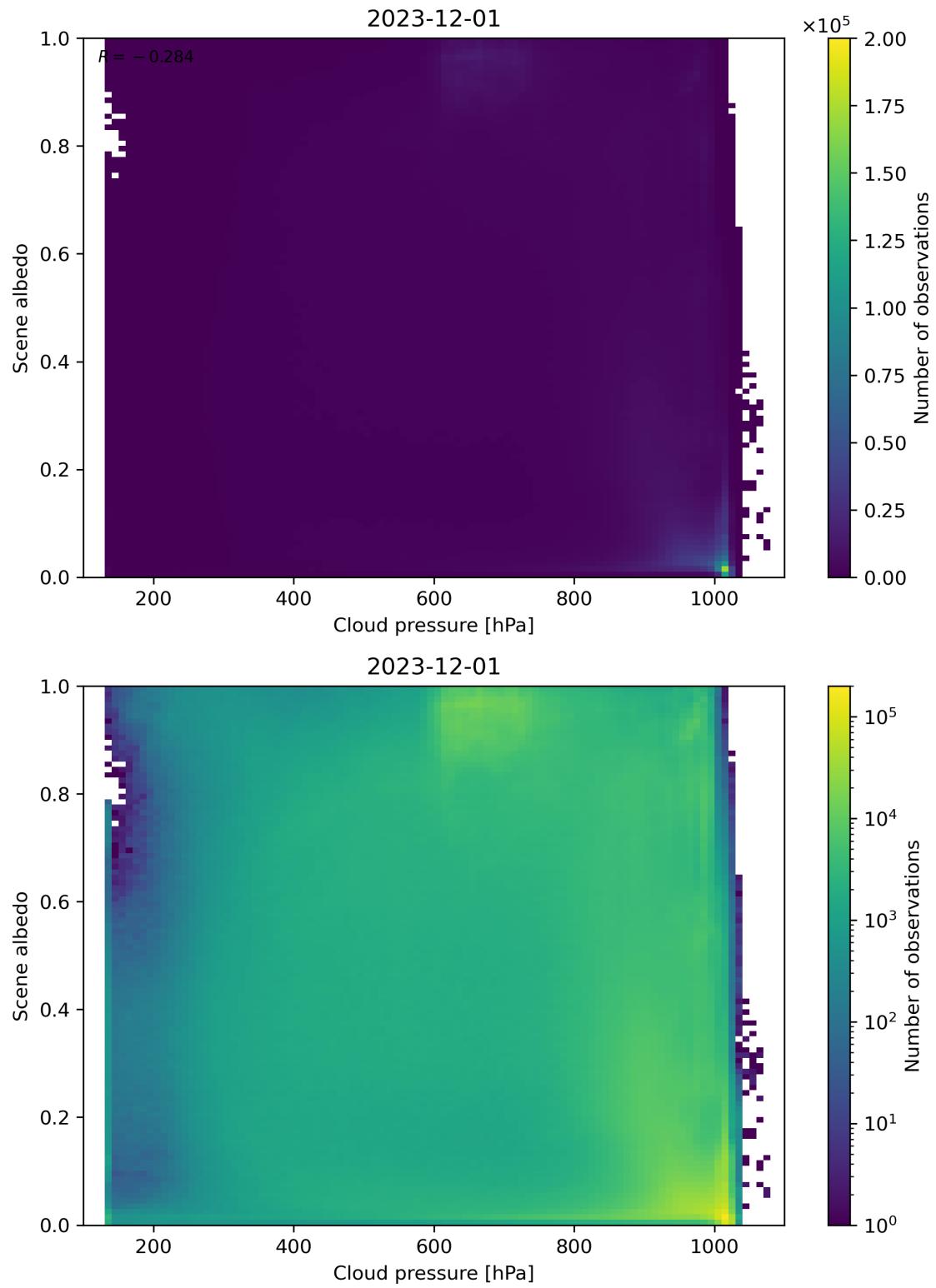
Figure 83: Scatter density plot of “Cloud pressure” against “Scene albedo” for 2023-11-30 to 2023-12-02.
