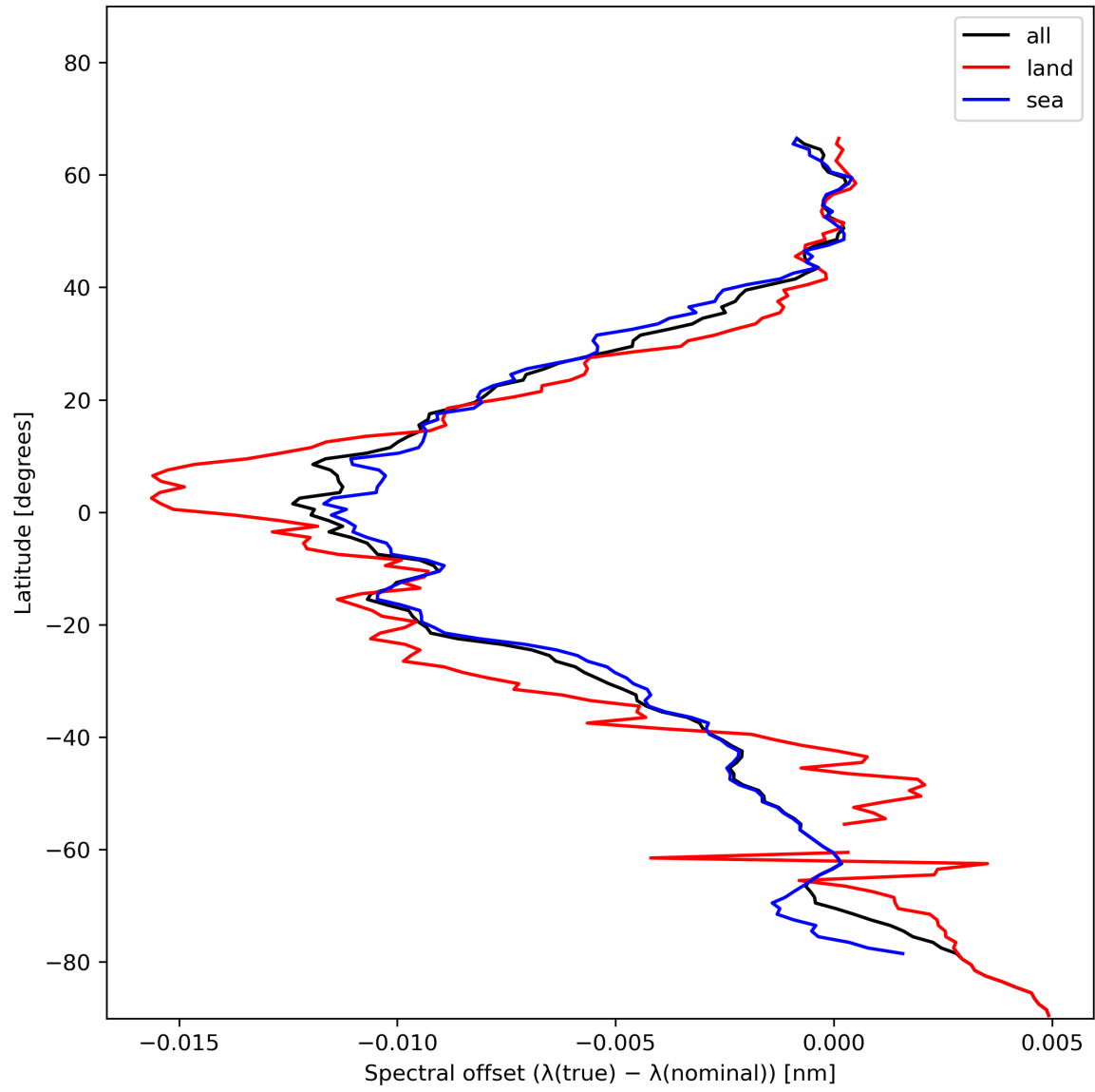
Figure 28: Zonal average of “Spectral offset ( \lambda(\text{true}) - \lambda(\text{nominal}) )” for 2023-11-30 to 2023-12-02.
