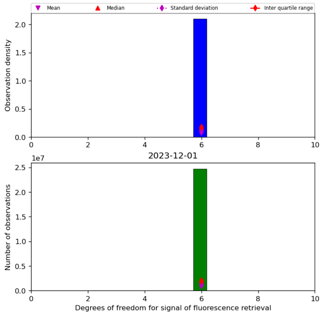
Figure 43: Histogram of “Degrees of freedom for signal of fluorescence retrieval” for 2023-11-30 to 2023-12-02
