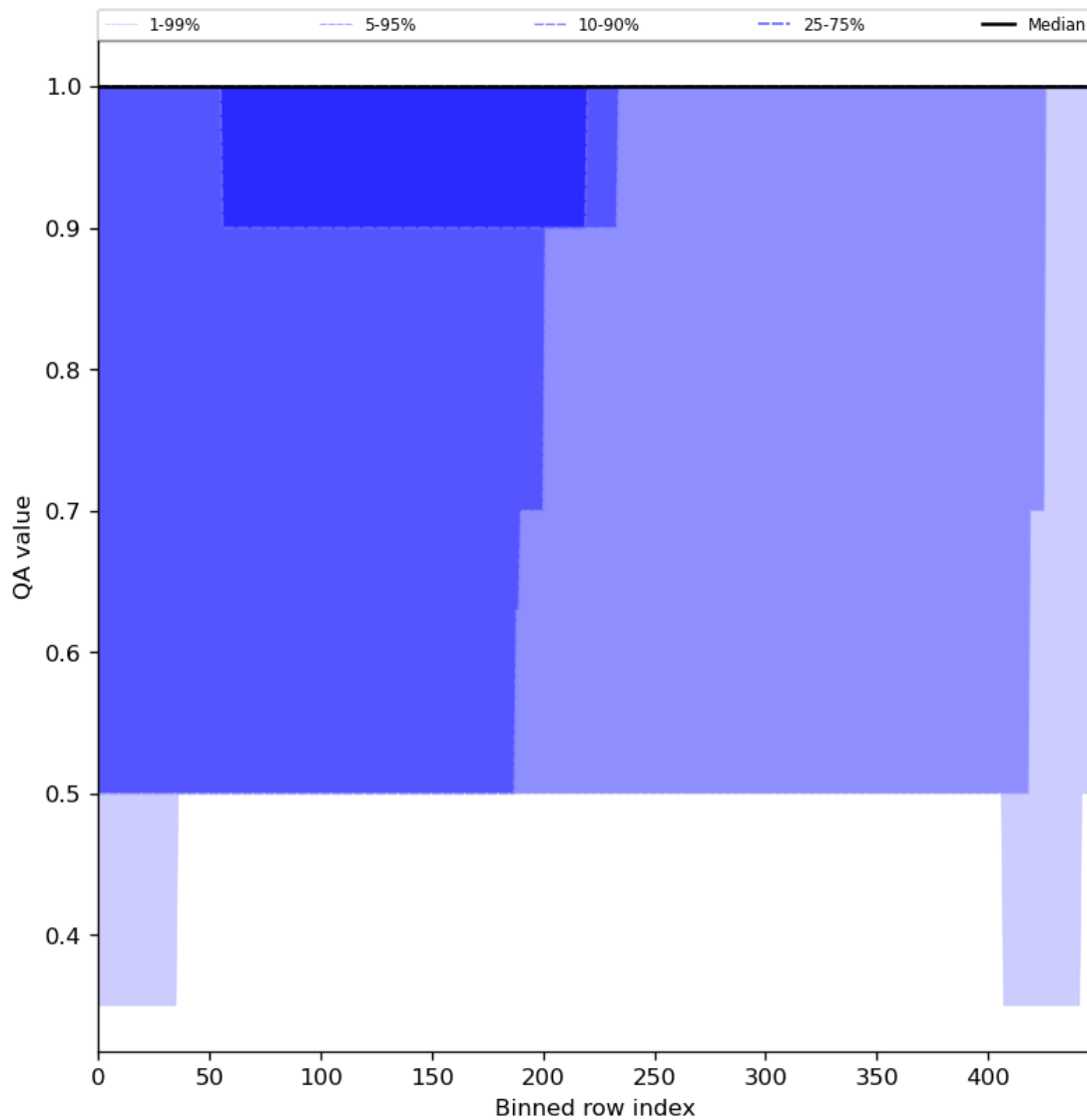
Figure 46: Along track statistics of “QA value” for 2023-11-30 to 2023-12-02
