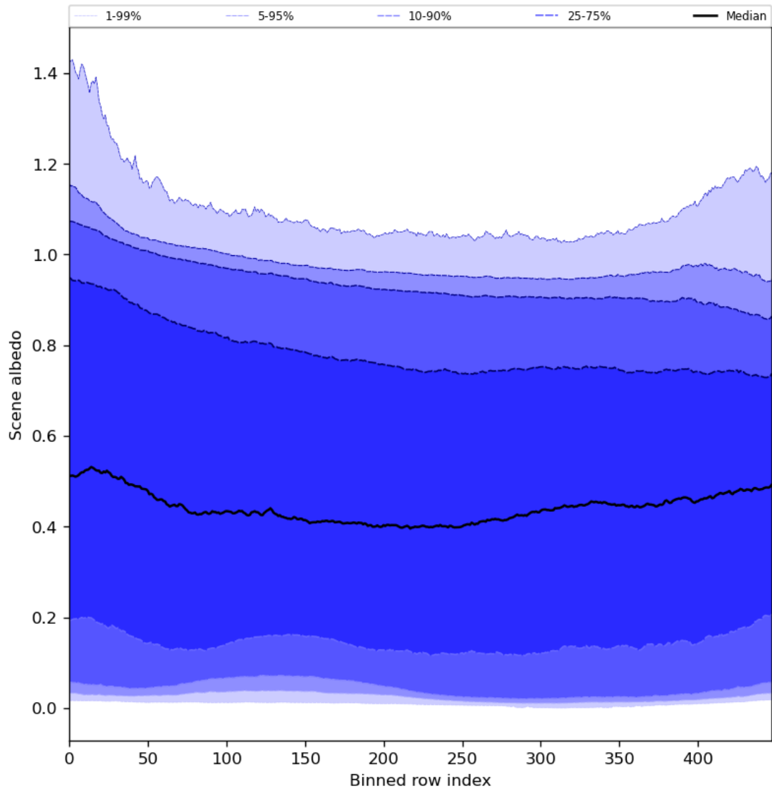
Figure 51: Along track statistics of “Scene albedo” for 2023-11-30 to 2023-12-02
