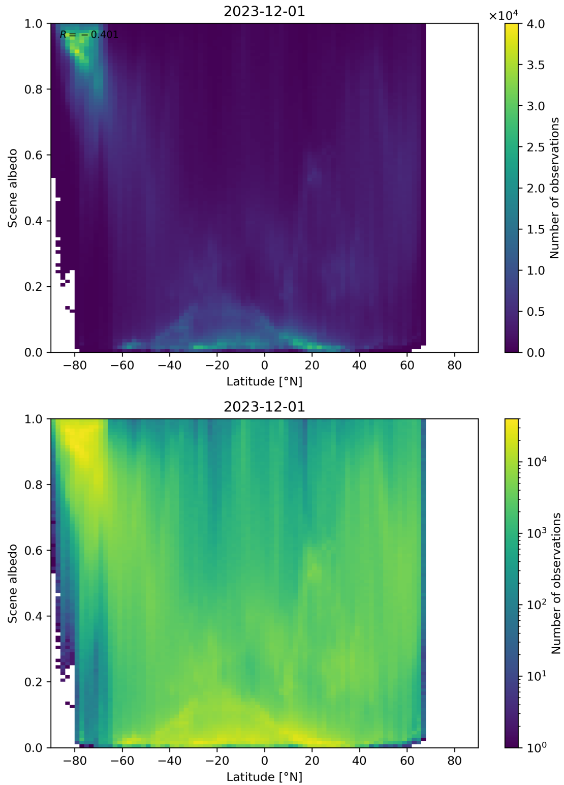
Figure 95: Scatter density plot of “Latitude” against “Scene albedo” for 2023-11-30 to 2023-12-02.
