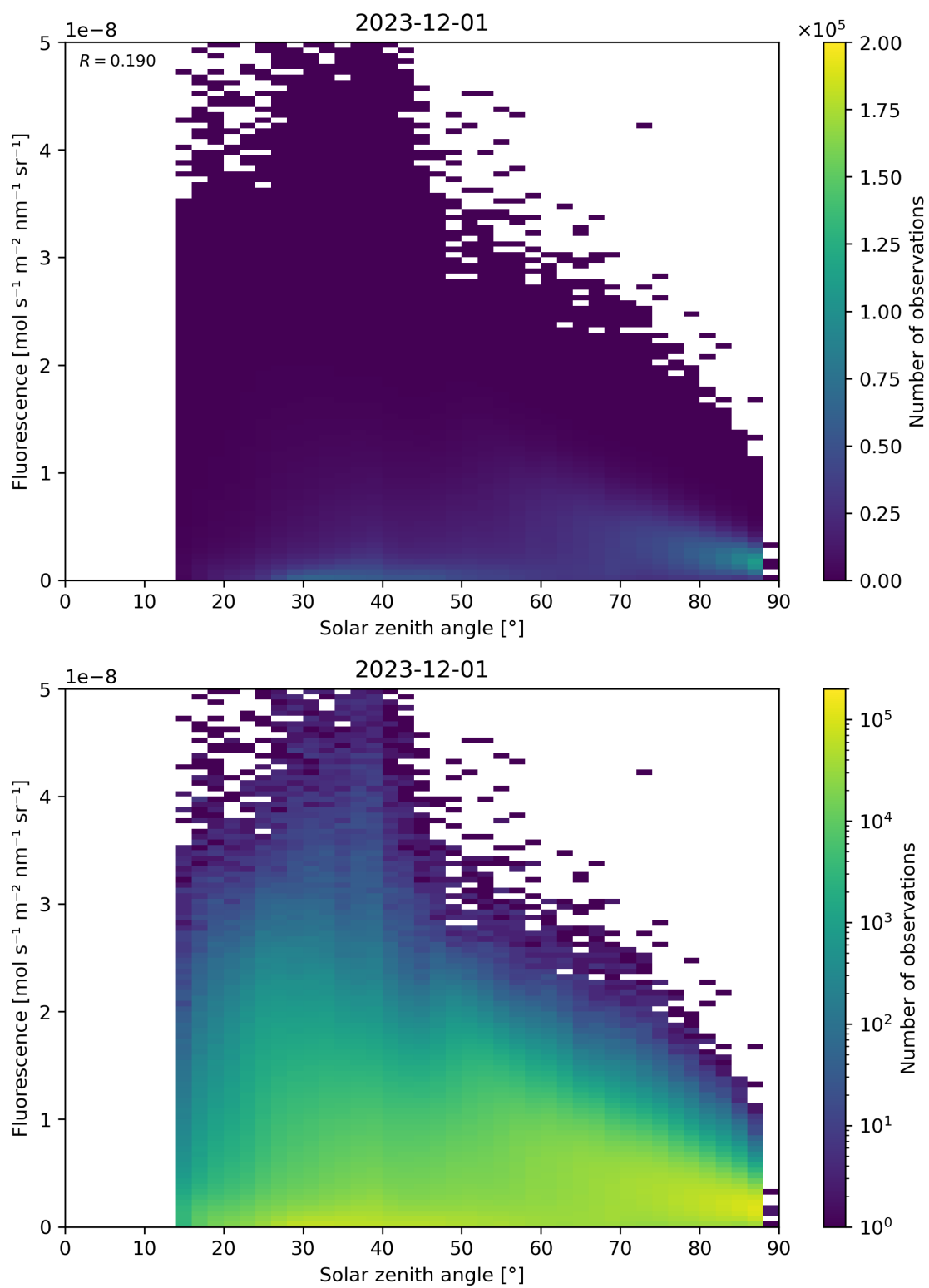
Figure 112: Scatter density plot of “Solar zenith angle” against “Fluorescence” for 2023-11-30 to 2023-12-02.
