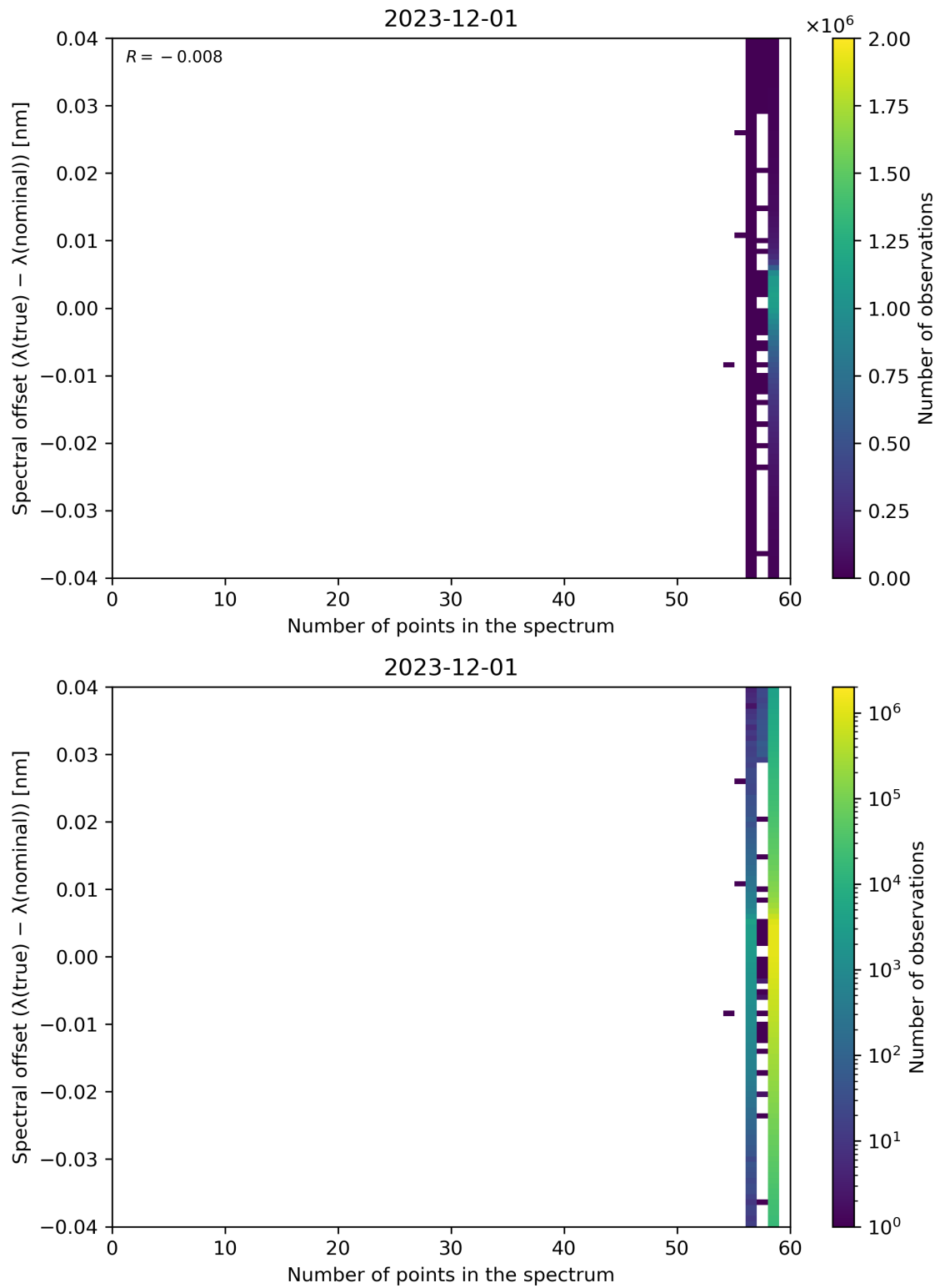
Figure 101: Scatter density plot of “Number of points in the spectrum” against “Spectral offset ( \lambda(\text{true}) - \lambda(\text{nominal}) )” for 2023-11-30 to 2023-12-02.
