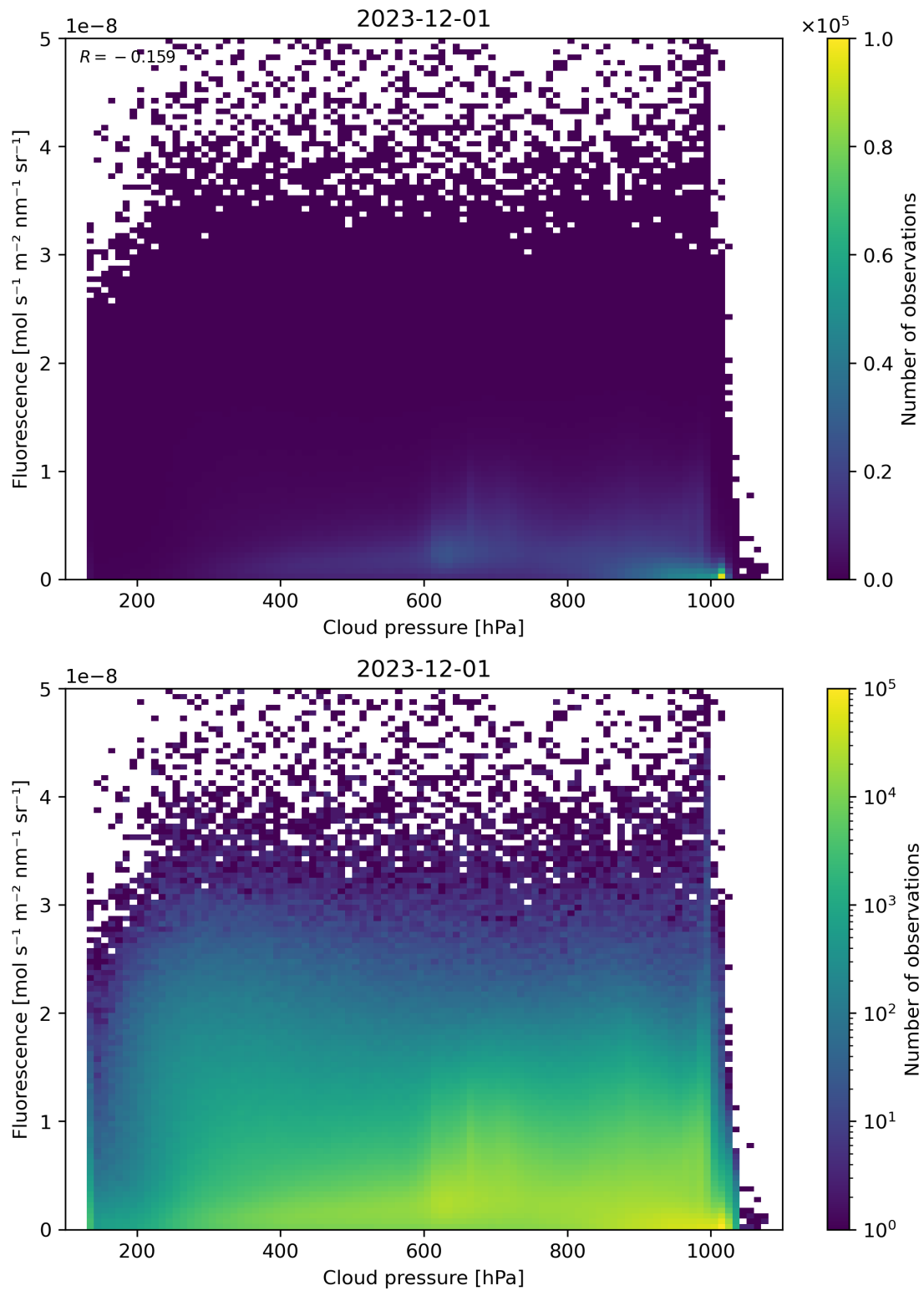
Figure 80: Scatter density plot of “Cloud pressure” against “Fluorescence” for 2023-11-30 to 2023-12-02.
