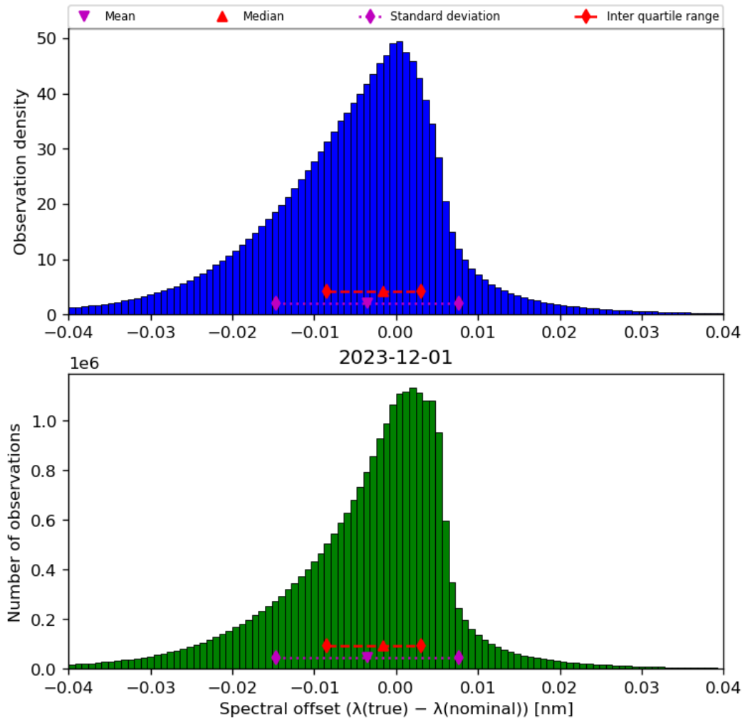
Figure 45: Histogram of “Spectral offset ( \lambda(\text{true}) - \lambda(\text{nominal}) )” for 2023-11-30 to 2023-12-02
