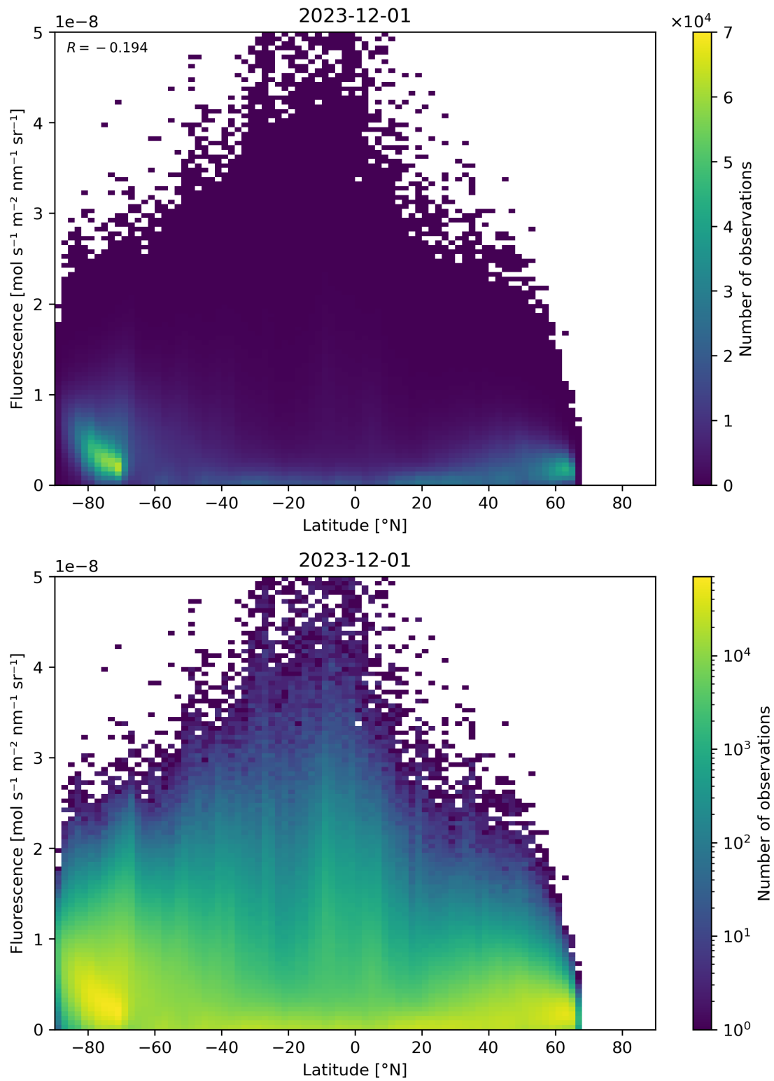
Figure 92: Scatter density plot of “Latitude” against “Fluorescence” for 2023-11-30 to 2023-12-02.
