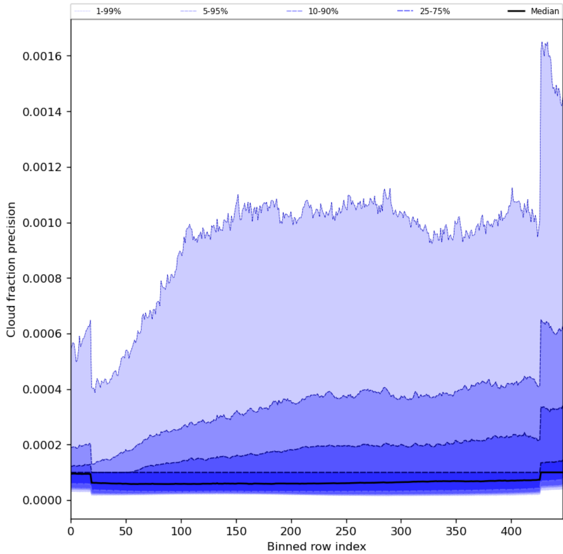
Figure 50: Along track statistics of “Cloud fraction precision” for 2023-11-30 to 2023-12-02
