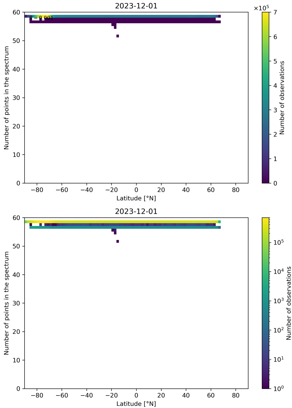
Figure 94: Scatter density plot of “Latitude” against “Number of points in the spectrum” for 2023-11-30 to 2023-12-02.
