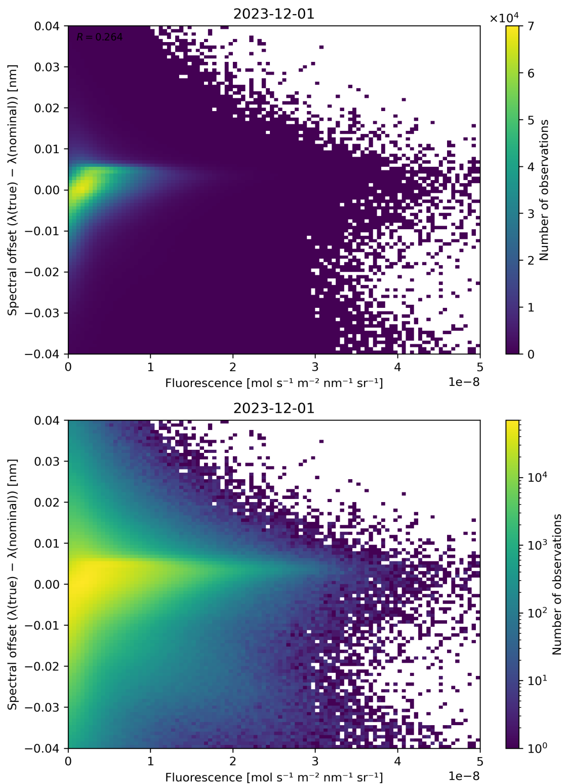
Figure 87: Scatter density plot of “Fluorescence” against “Spectral offset ( \lambda(\text{true}) - \lambda(\text{nominal}) )” for 2023-11-30 to 2023-12-02.
