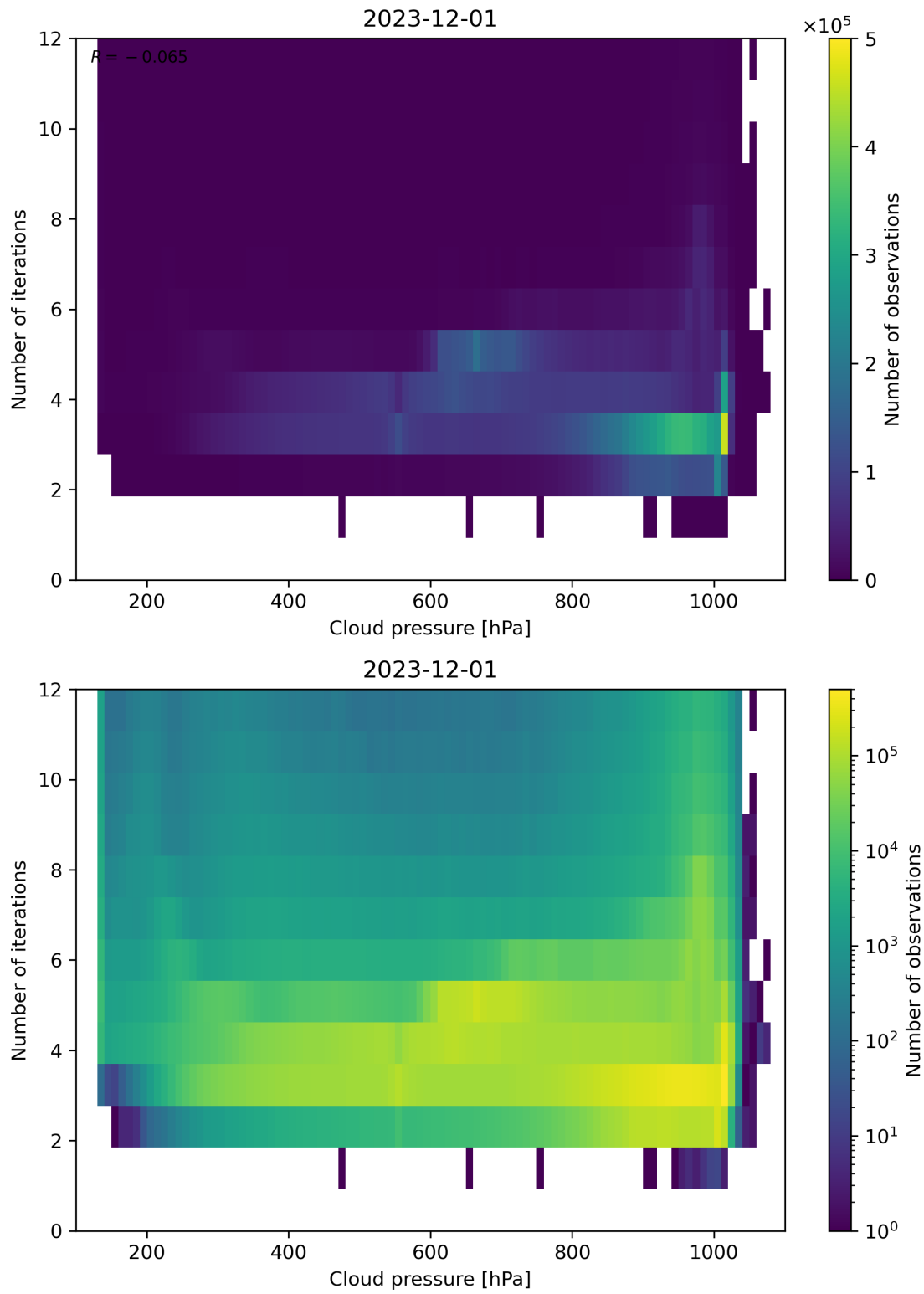
Figure 81: Scatter density plot of “Cloud pressure” against “Number of iterations” for 2023-11-30 to 2023-12-02.
