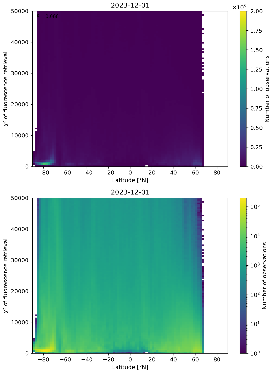
Figure 89: Scatter density plot of “Latitude” against “ \chi^2 of fluorescence retrieval” for 2023-11-30 to 2023-12-02.
