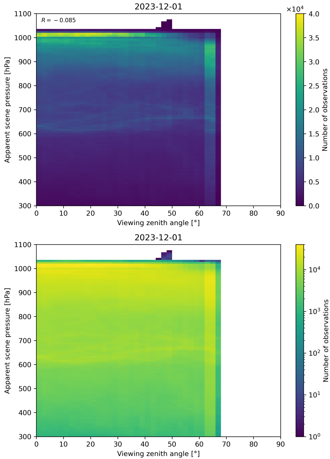
Figure 118: Scatter density plot of “Viewing zenith angle” against “Apparent scene pressure” for 2023-11-30 to 2023-12-02.
