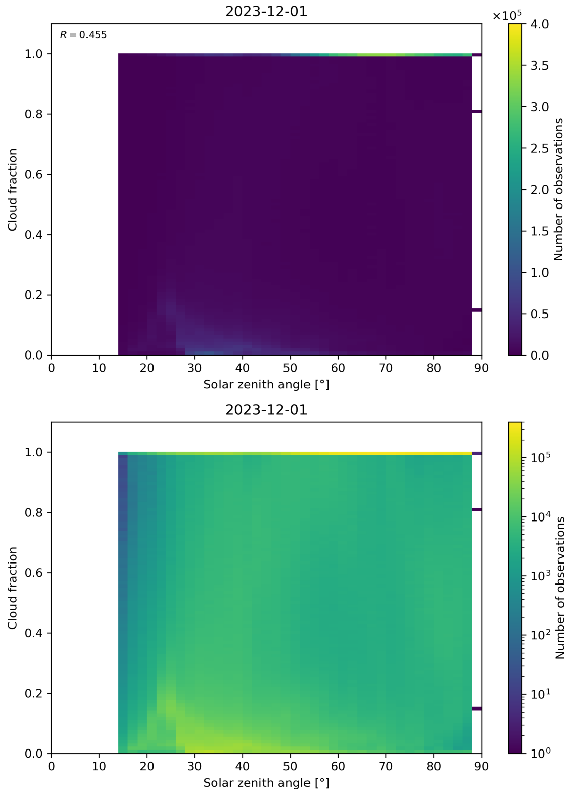
Figure 110: Scatter density plot of “Solar zenith angle” against “Cloud fraction” for 2023-11-30 to 2023-12-02.
