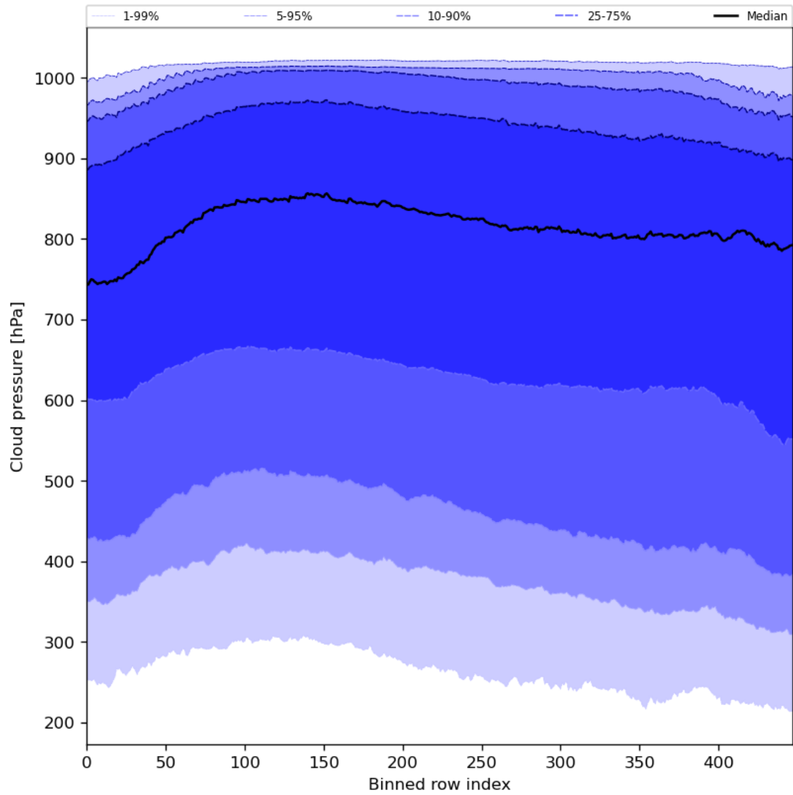
Figure 47: Along track statistics of “Cloud pressure” for 2023-11-30 to 2023-12-02
