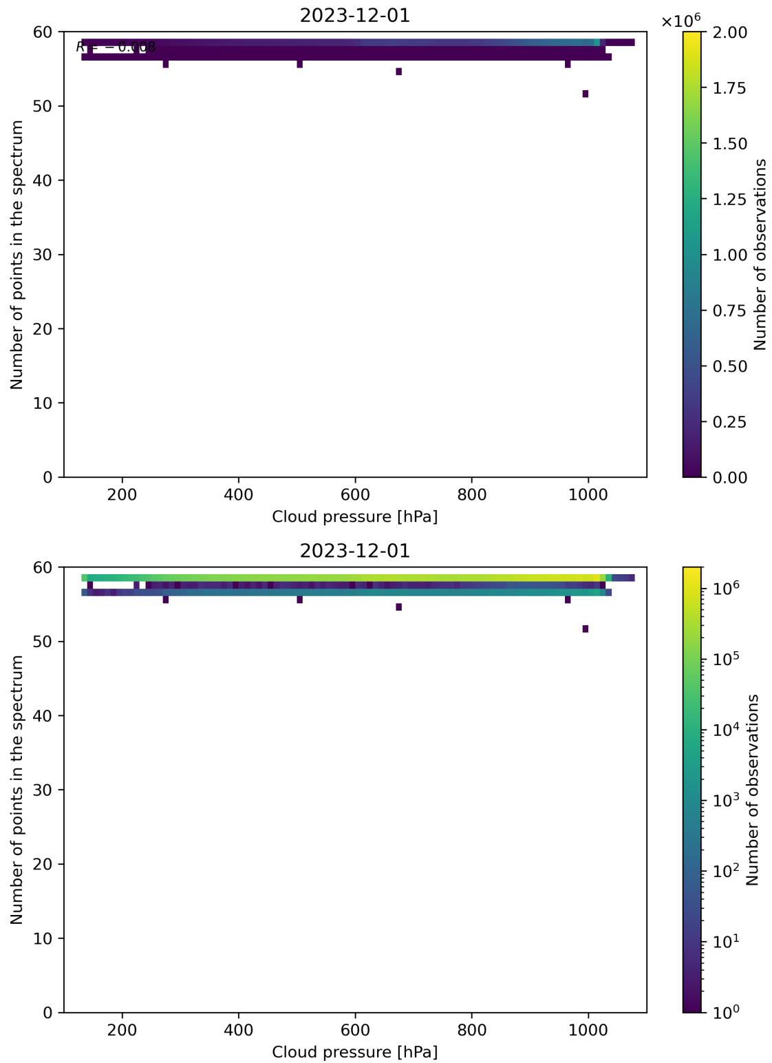
Figure 82: Scatter density plot of “Cloud pressure” against “Number of points in the spectrum” for 2023-11-30 to 2023-12-02.
