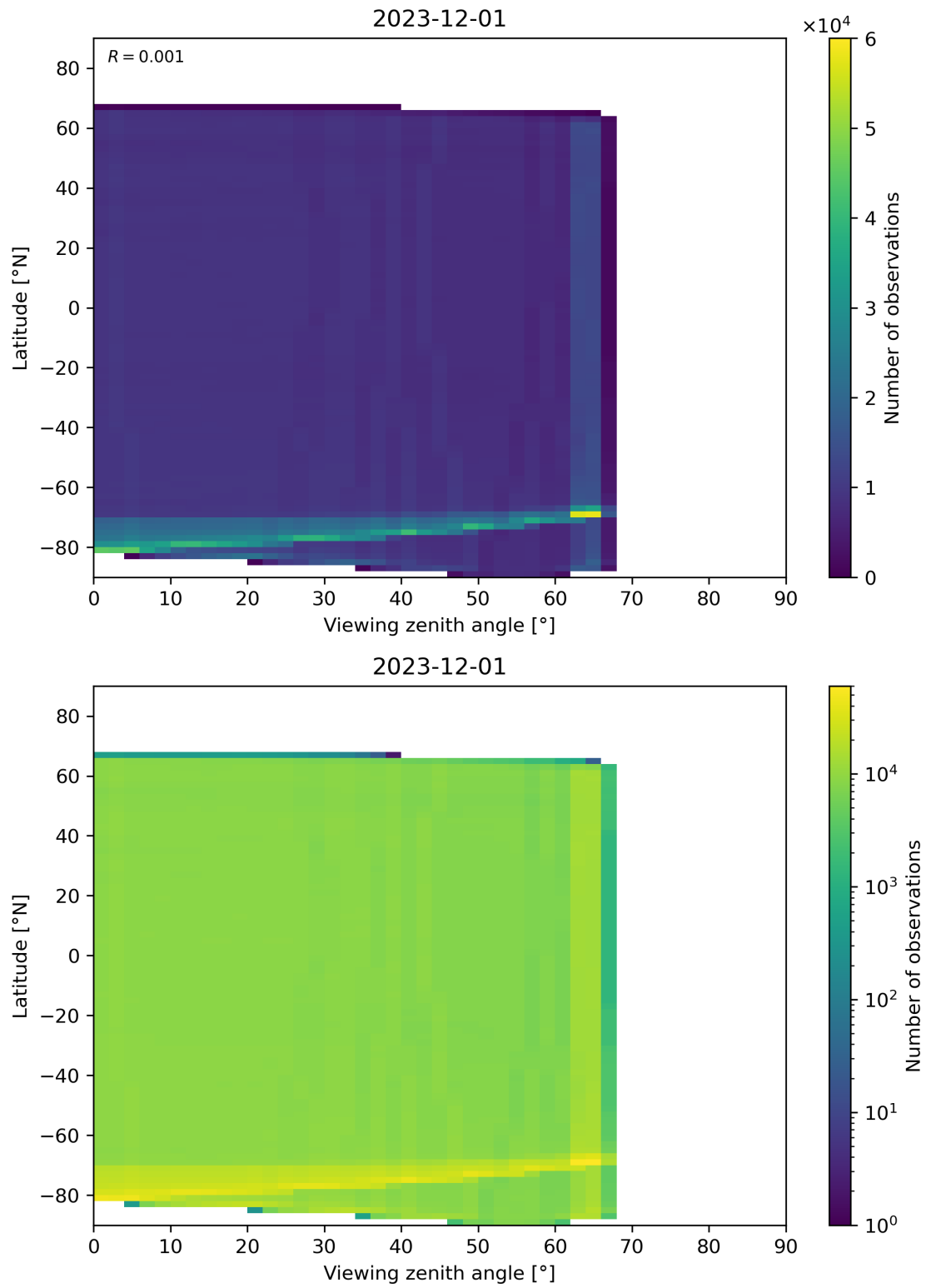
Figure 123: Scatter density plot of “Viewing zenith angle” against “Latitude” for 2023-11-30 to 2023-12-02.
