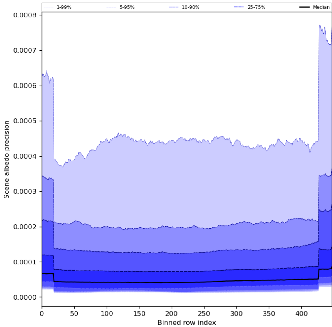
Figure 52: Along track statistics of “Scene albedo precision” for 2023-11-30 to 2023-12-02
