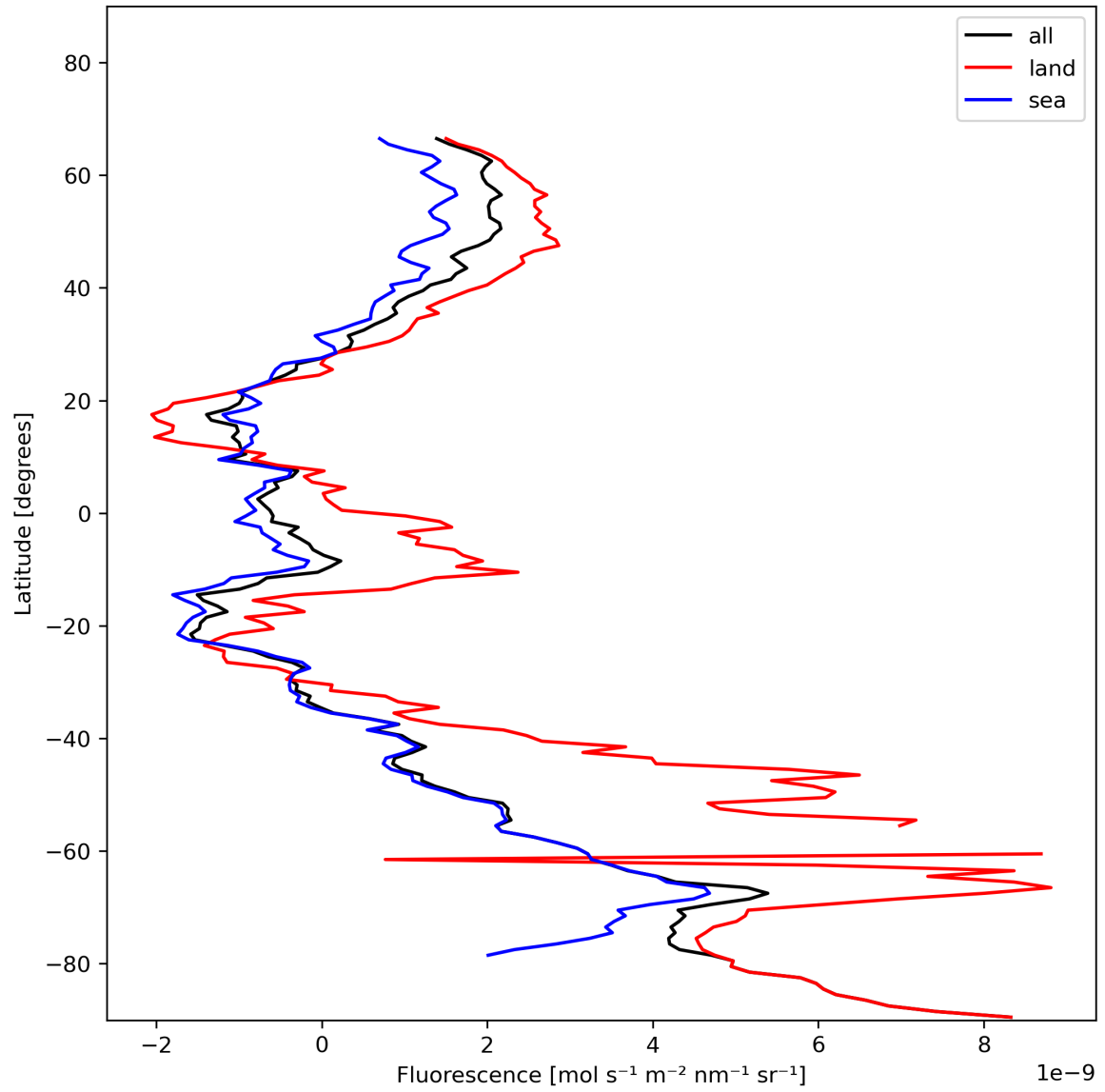
Figure 23: Zonal average of “Fluorescence” for 2023-11-30 to 2023-12-02.
