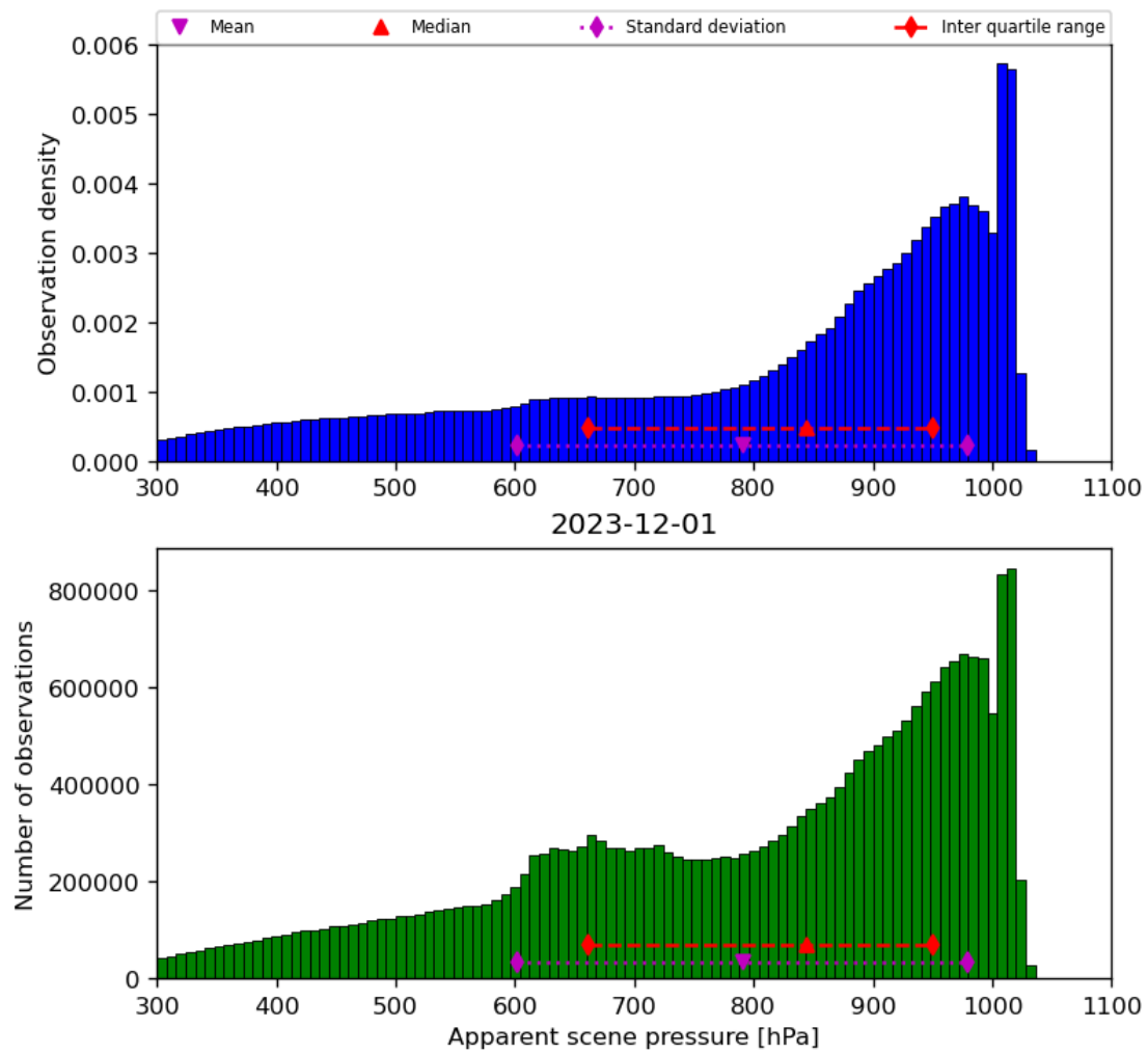
Figure 36: Histogram of “Apparent scene pressure” for 2023-11-30 to 2023-12-02
