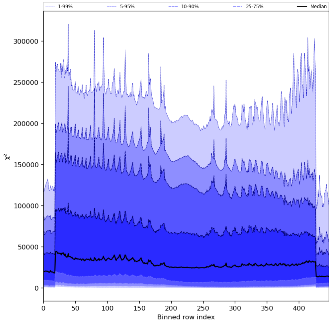
Figure 55: Along track statistics of “ \chi^2 ” for 2023-11-30 to 2023-12-02
