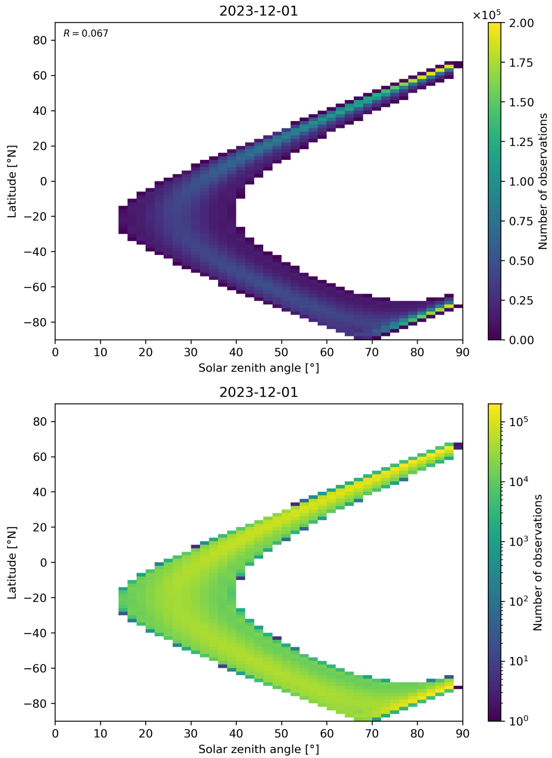
Figure 113: Scatter density plot of “Solar zenith angle” against “Latitude” for 2023-11-30 to 2023-12-02.
