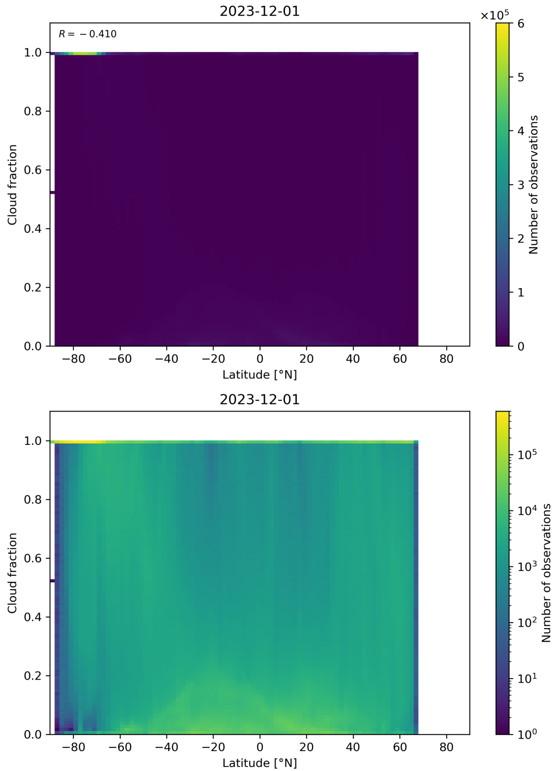
Figure 90: Scatter density plot of “Latitude” against “Cloud fraction” for 2023-11-30 to 2023-12-02.
