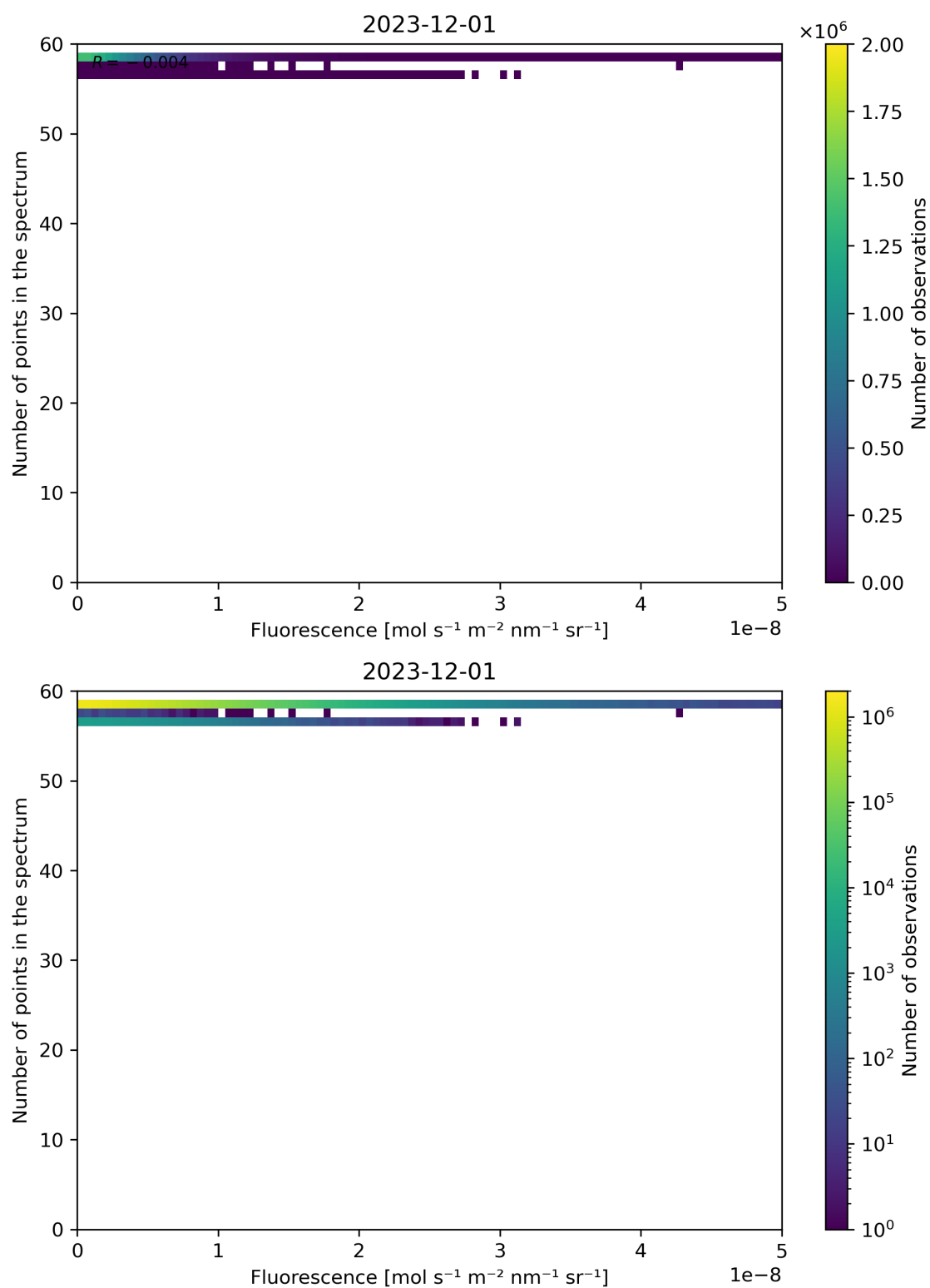
Figure 86: Scatter density plot of “Fluorescence” against “Number of points in the spectrum” for 2023-11-30 to 2023-12-02.
