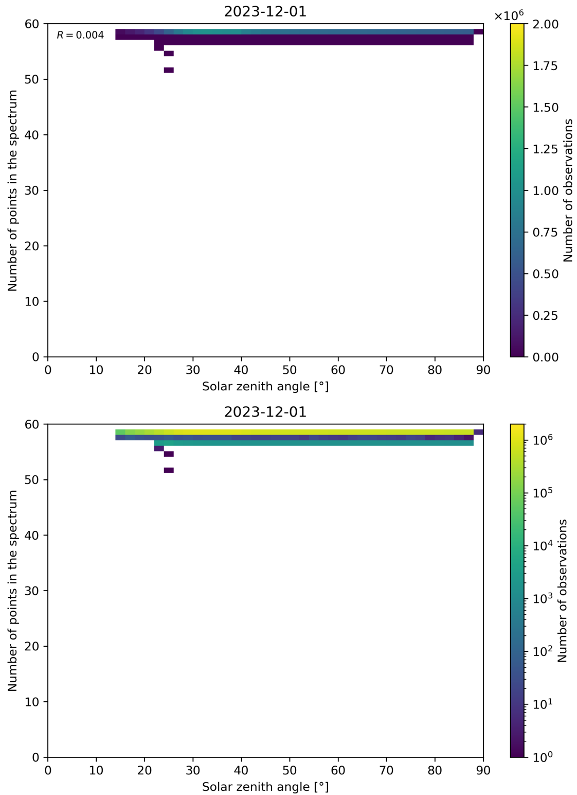
Figure 115: Scatter density plot of “Solar zenith angle” against “Number of points in the spectrum” for 2023-11-30 to 2023-12-02.
