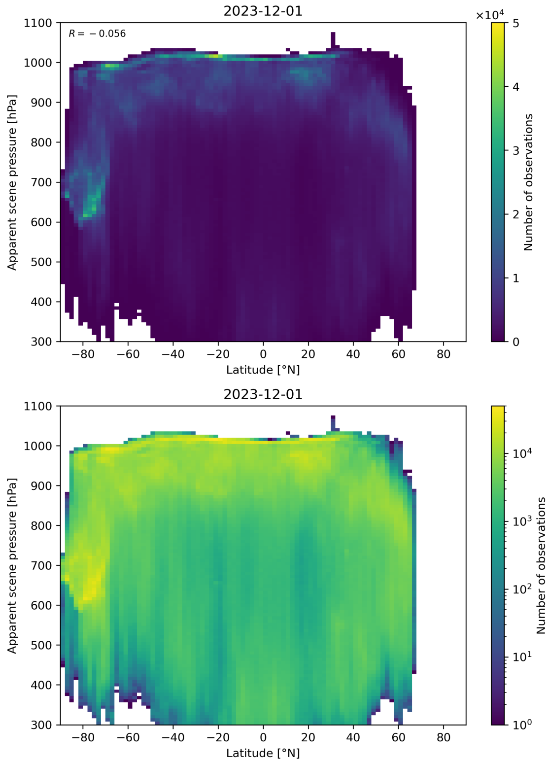
Figure 88: Scatter density plot of “Latitude” against “Apparent scene pressure” for 2023-11-30 to 2023-12-02.
