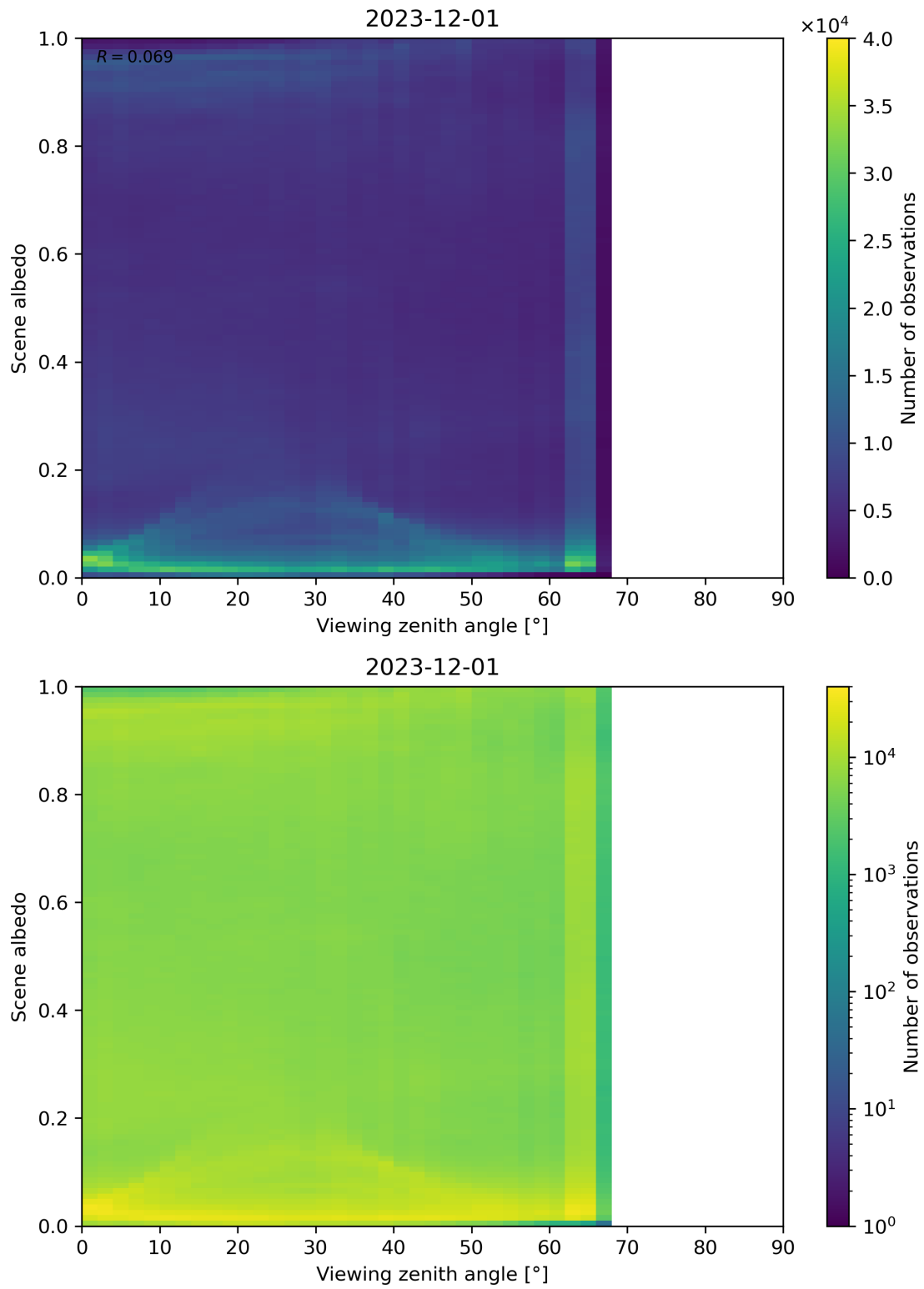
Figure 126: Scatter density plot of “Viewing zenith angle” against “Scene albedo” for 2023-11-30 to 2023-12-02.
