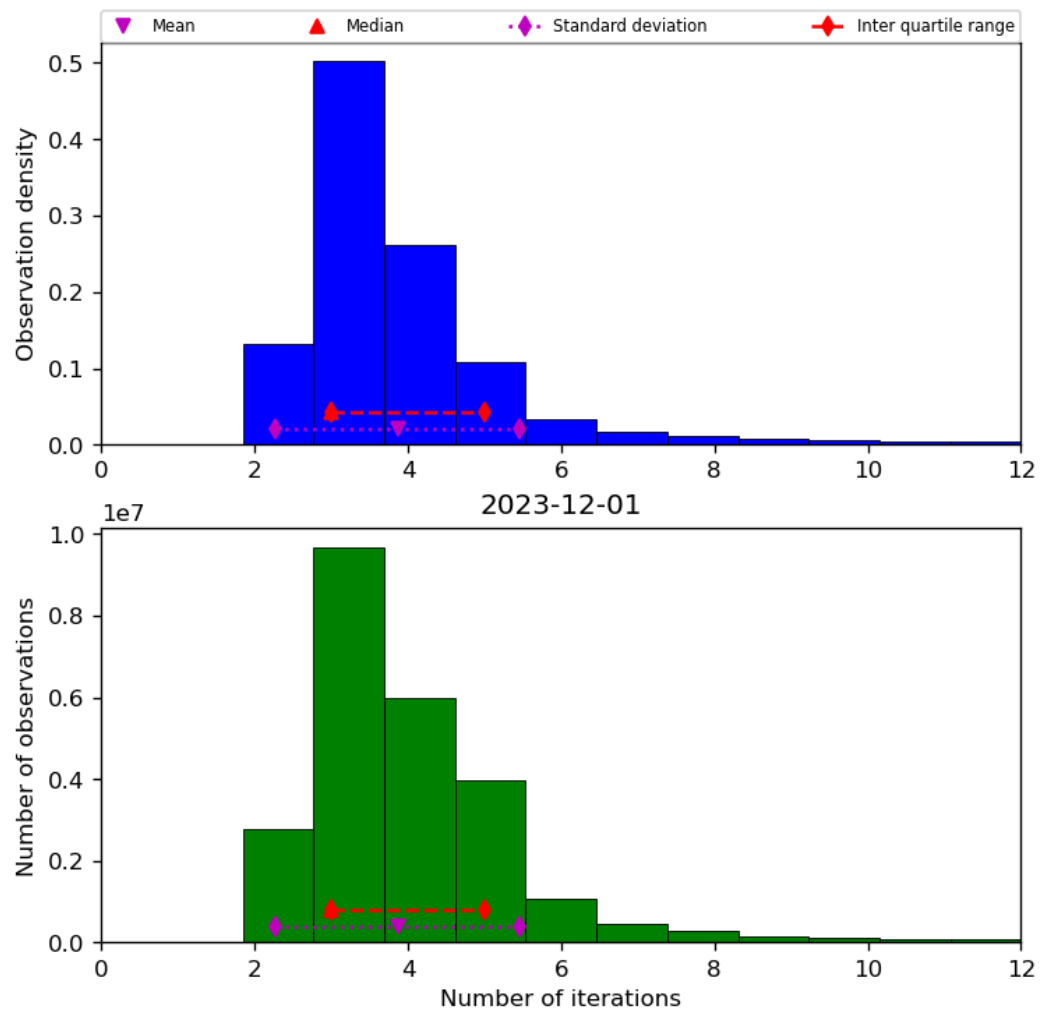
Figure 39: Histogram of “Number of iterations” for 2023-11-30 to 2023-12-02
