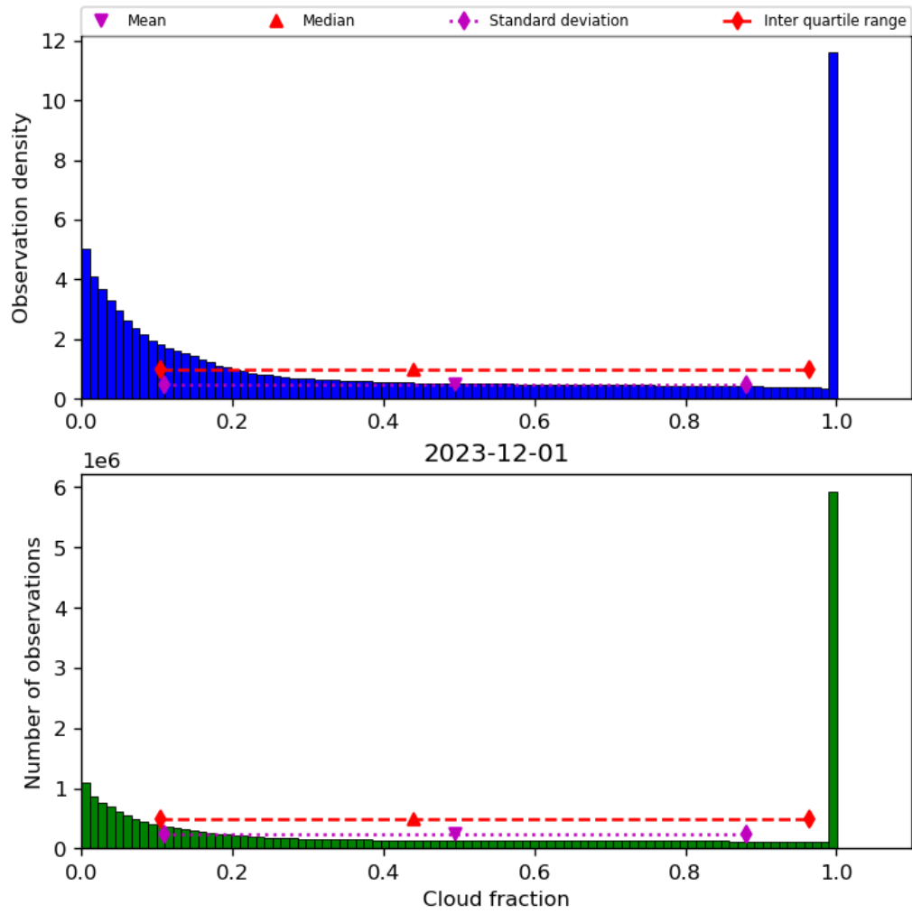
Figure 32: Histogram of “Cloud fraction” for 2023-11-30 to 2023-12-02
