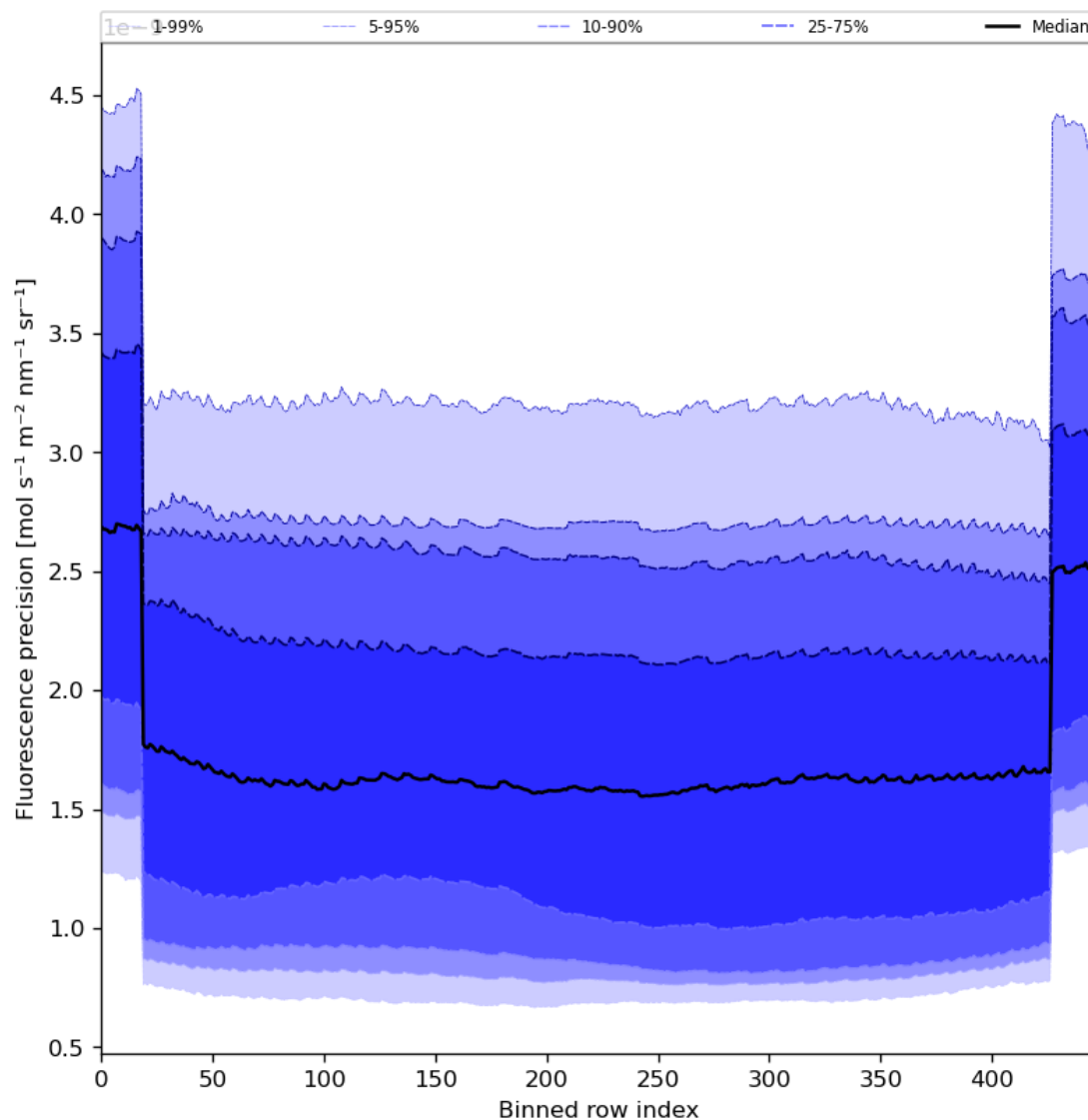
Figure 58: Along track statistics of “Fluorescence precision” for 2023-11-30 to 2023-12-02
