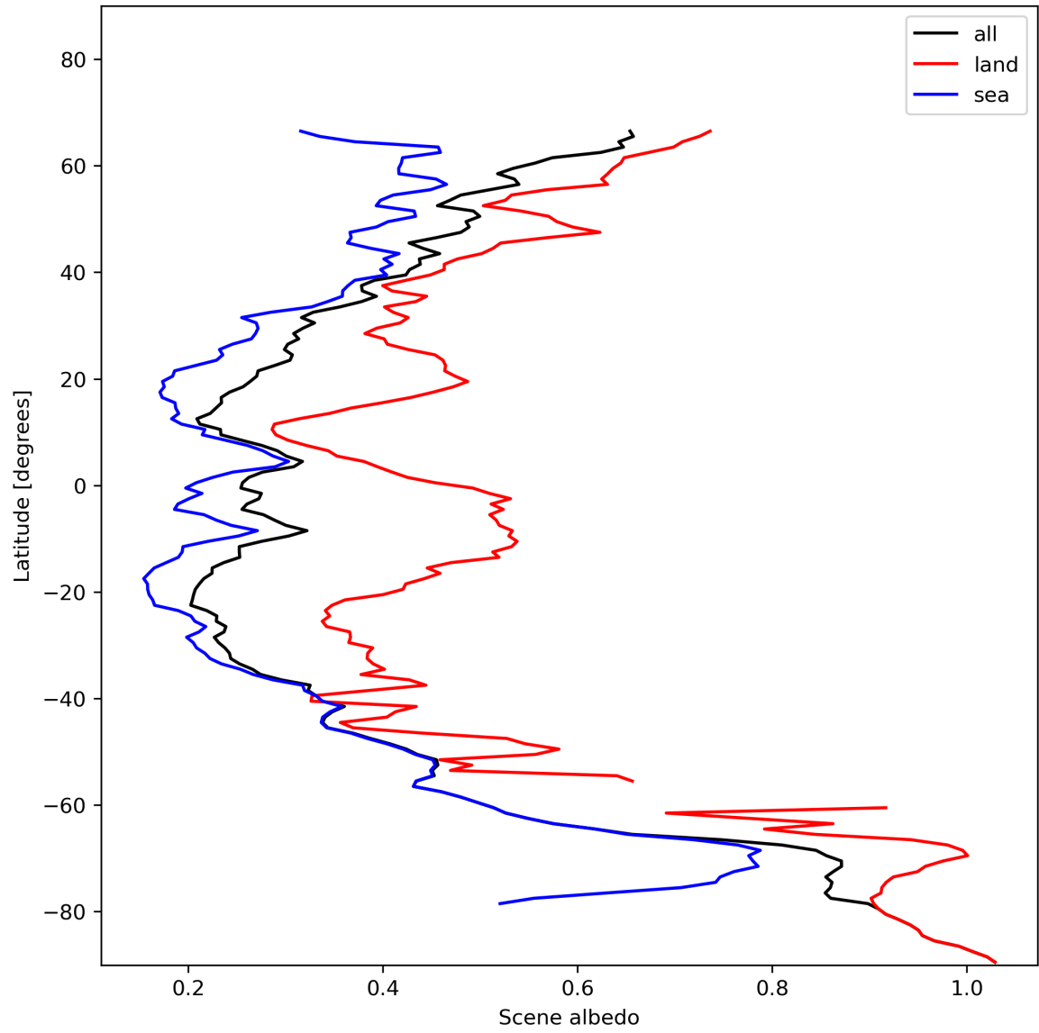
Figure 17: Zonal average of “Scene albedo” for 2023-11-30 to 2023-12-02.
