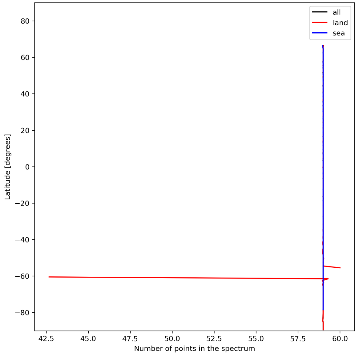
Figure 27: Zonal average of “Number of points in the spectrum” for 2023-11-30 to 2023-12-02.
