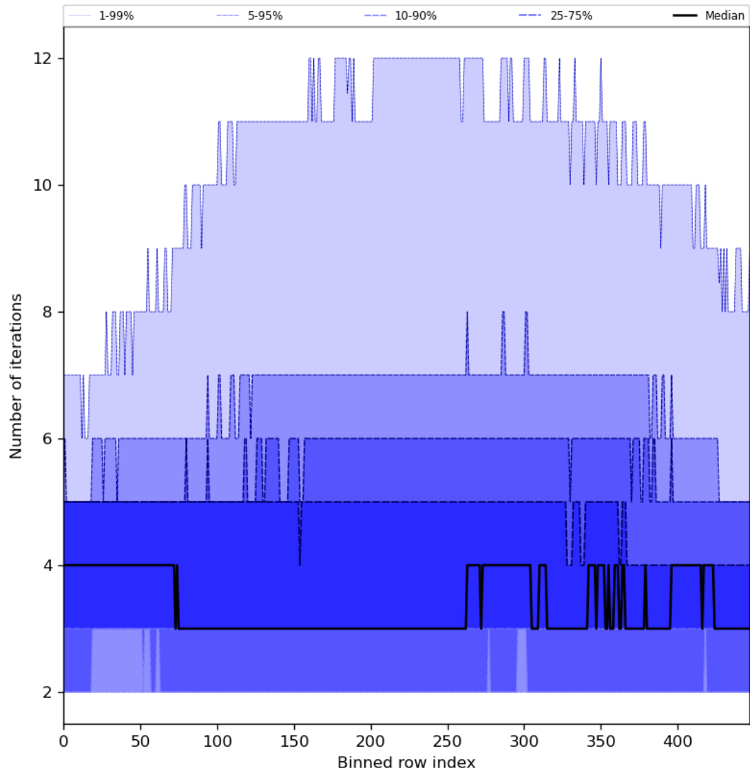
Figure 56: Along track statistics of “Number of iterations” for 2023-11-30 to 2023-12-02
