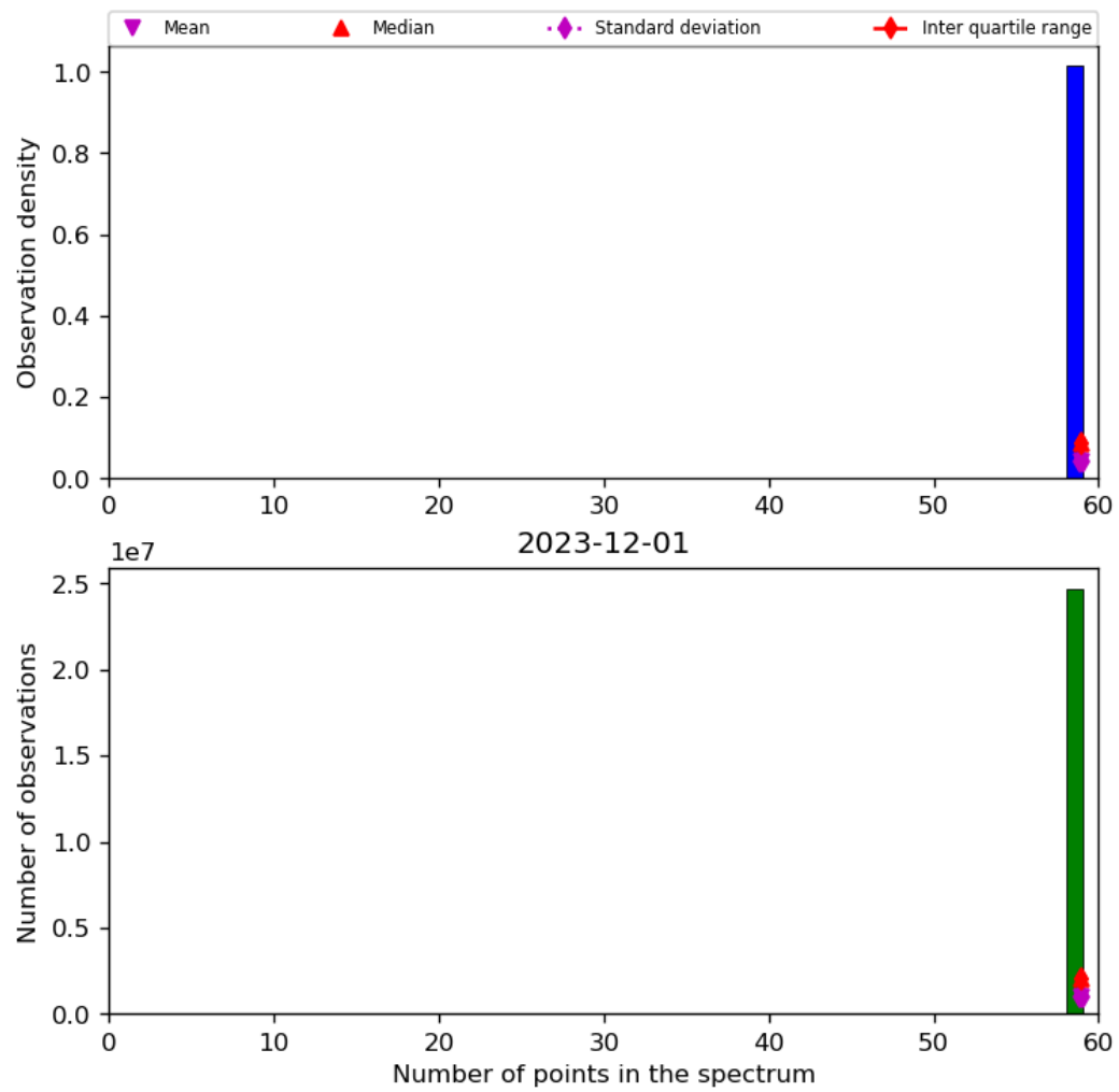
Figure 44: Histogram of "Number of points in the spectrum" for 2023-11-30 to 2023-12-02
