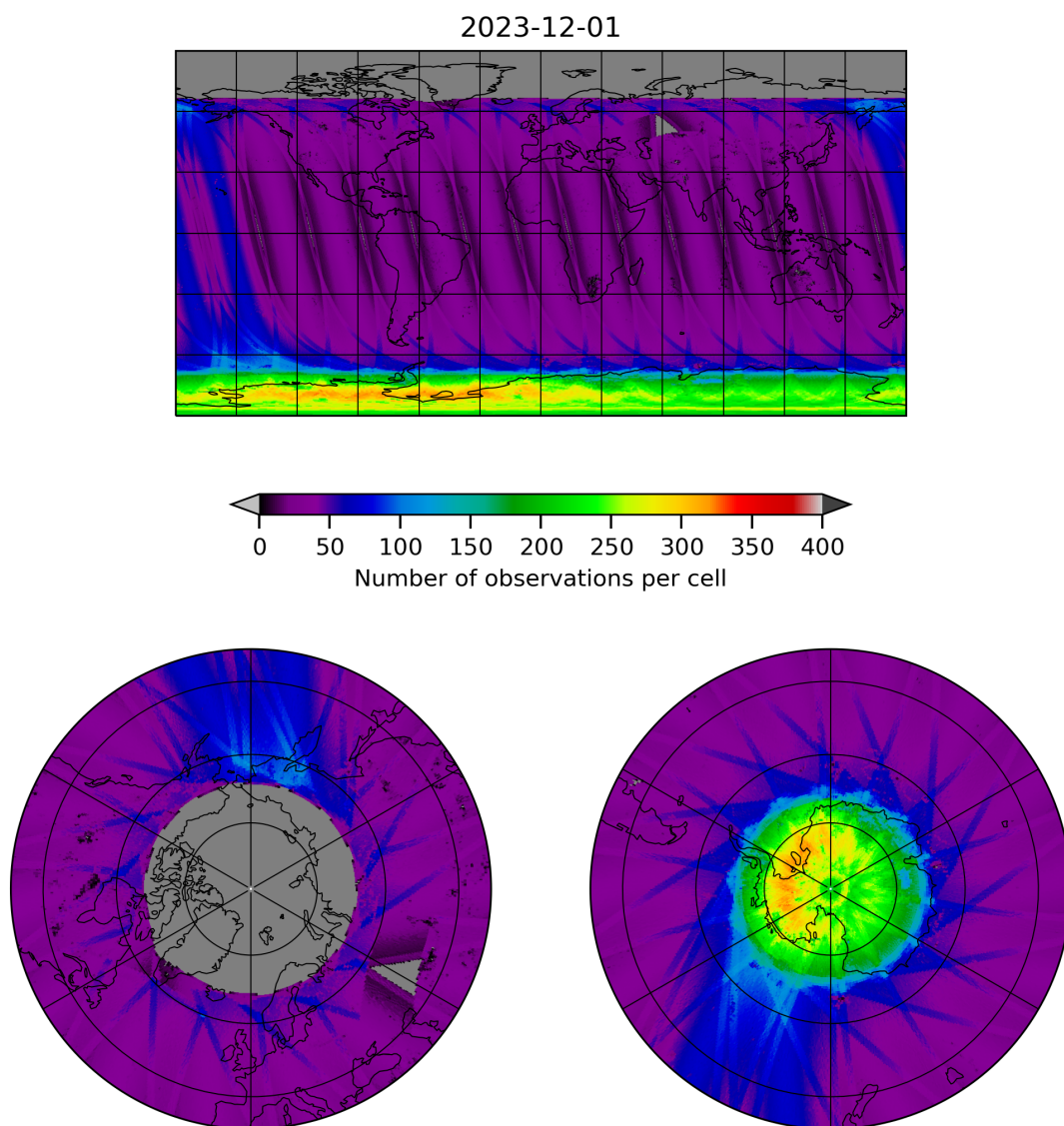
Figure 11: Map of the number of observations for 2023-11-30 to 2023-12-02
