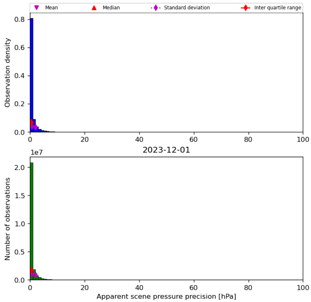
Figure 37: Histogram of “Apparent scene pressure precision” for 2023-11-30 to 2023-12-02
