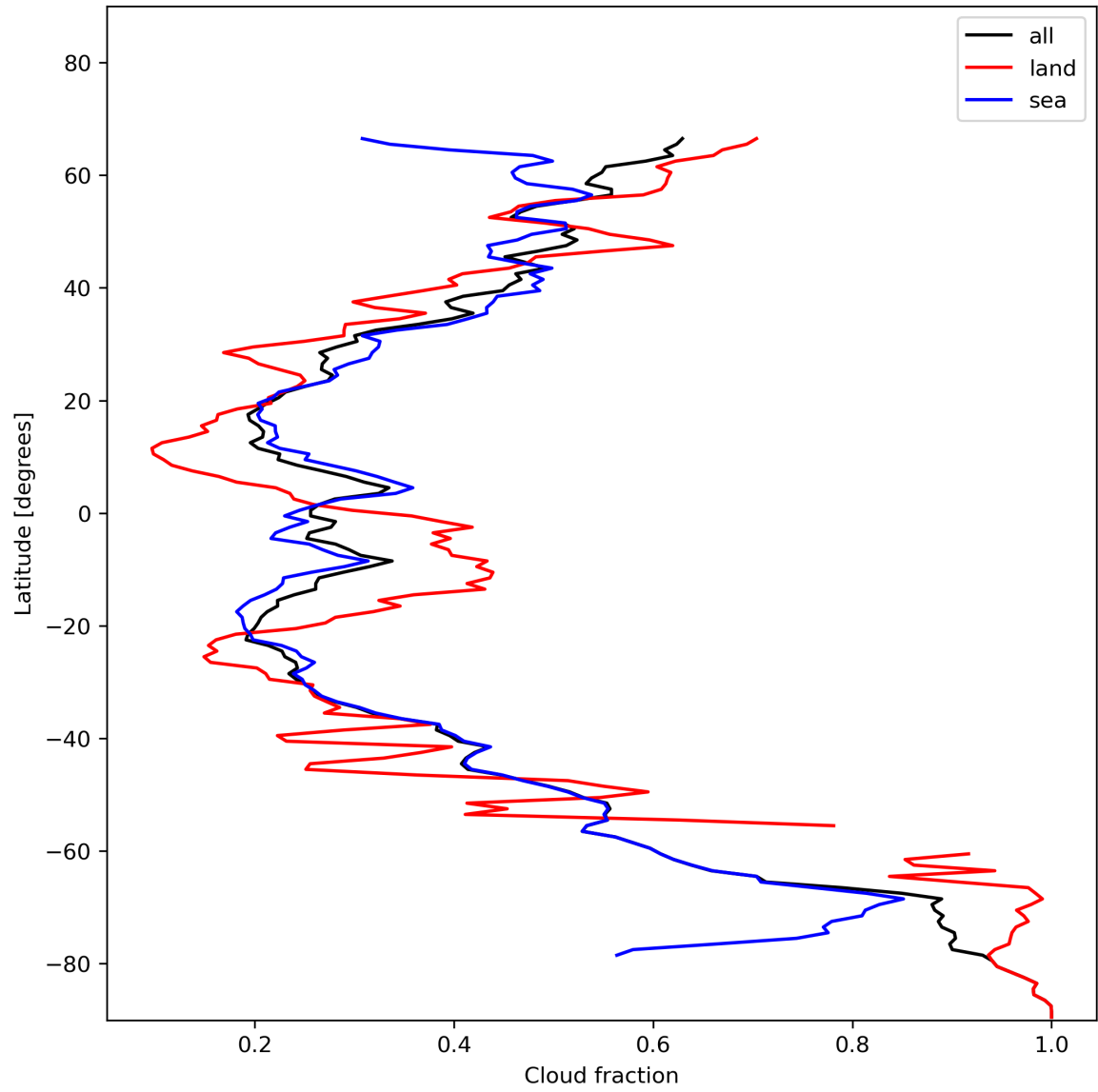
Figure 15: Zonal average of “Cloud fraction” for 2023-11-30 to 2023-12-02.
