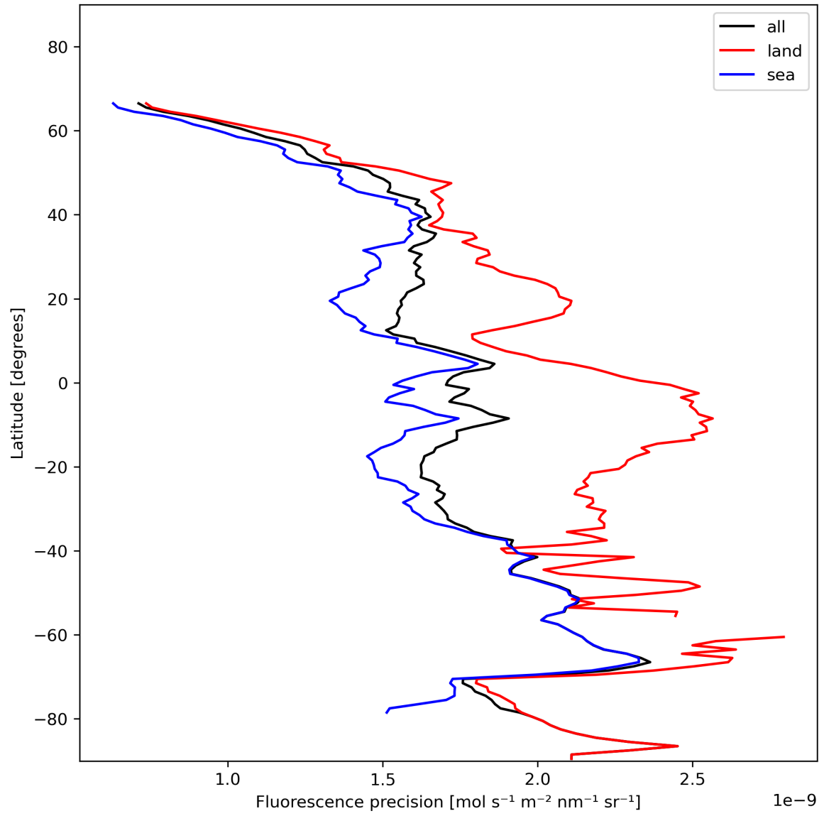
Figure 24: Zonal average of “Fluorescence precision” for 2023-11-30 to 2023-12-02.
