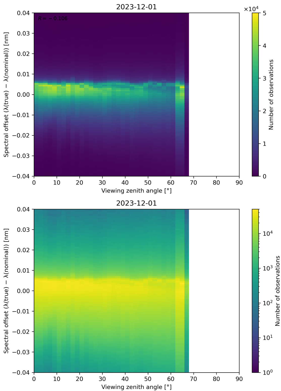
Figure 128: Scatter density plot of “Viewing zenith angle” against “Spectral offset ( \lambda(\text{true}) - \lambda(\text{nominal}) )” for 2023-11-30 to 2023-12-02.
