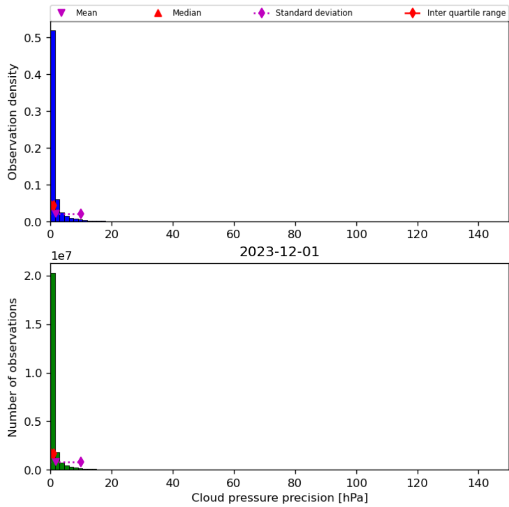
Figure 31: Histogram of “Cloud pressure precision” for 2023-11-30 to 2023-12-02
