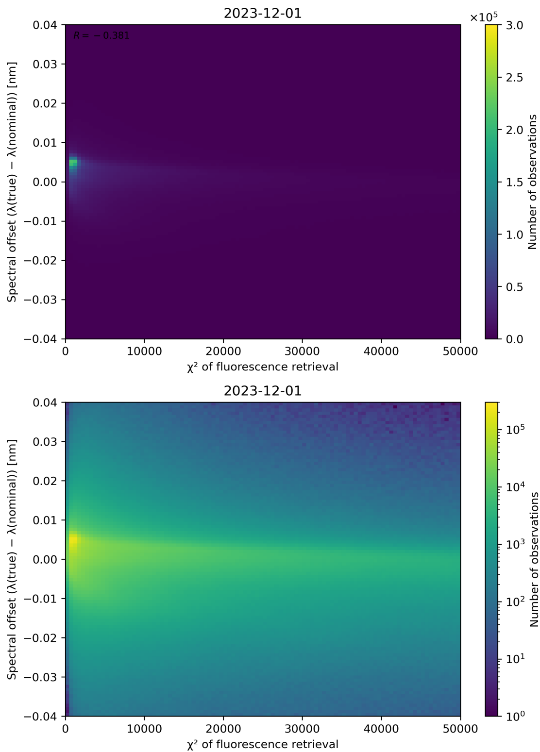
Figure 69: Scatter density plot of " \chi^2 of fluorescence retrieval" against "Spectral offset ( \lambda(\text{true}) - \lambda(\text{nominal}) )" for 2023-11-30 to 2023-12-02.
