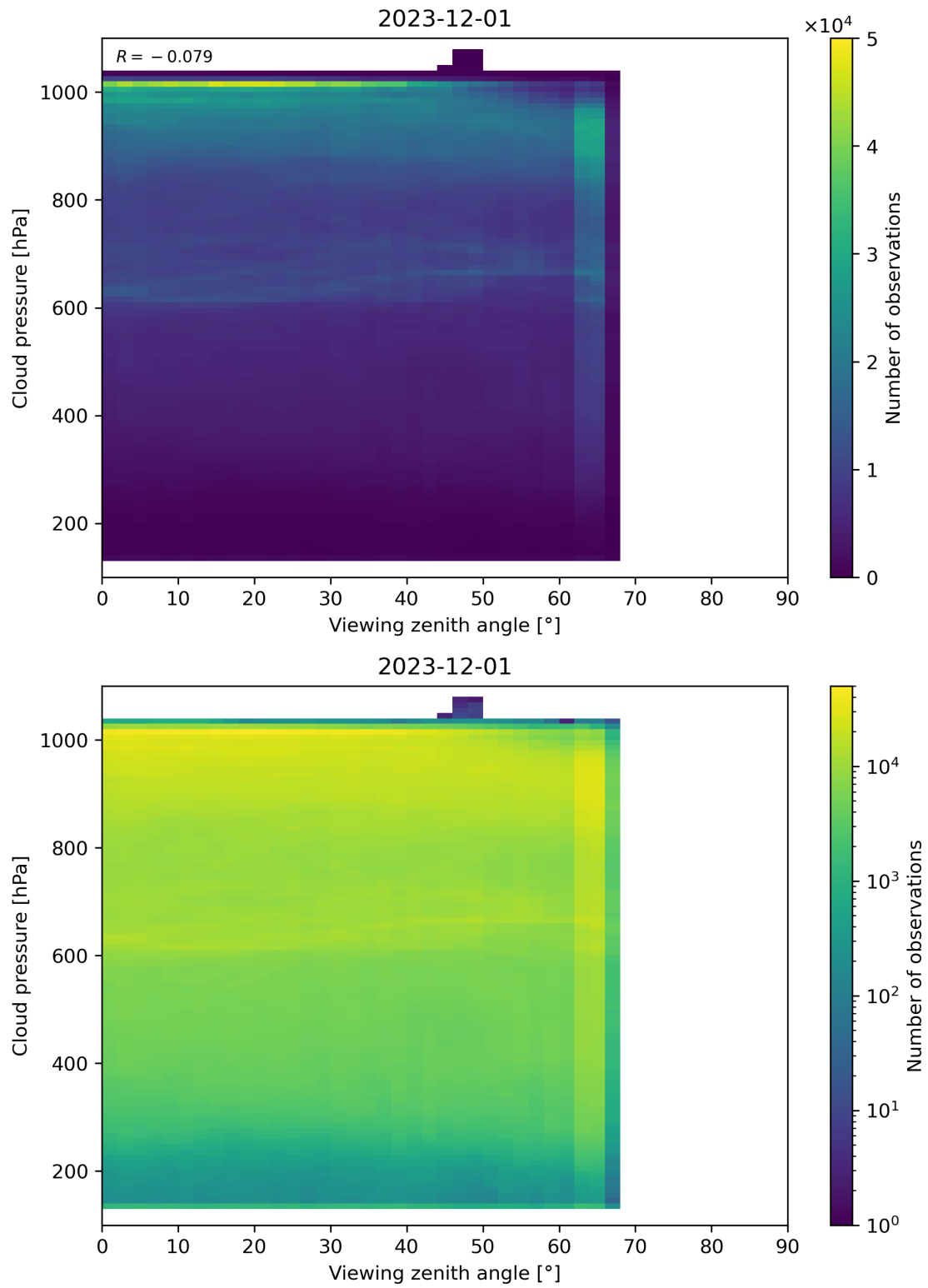
Figure 121: Scatter density plot of “Viewing zenith angle” against “Cloud pressure” for 2023-11-30 to 2023-12-02.
