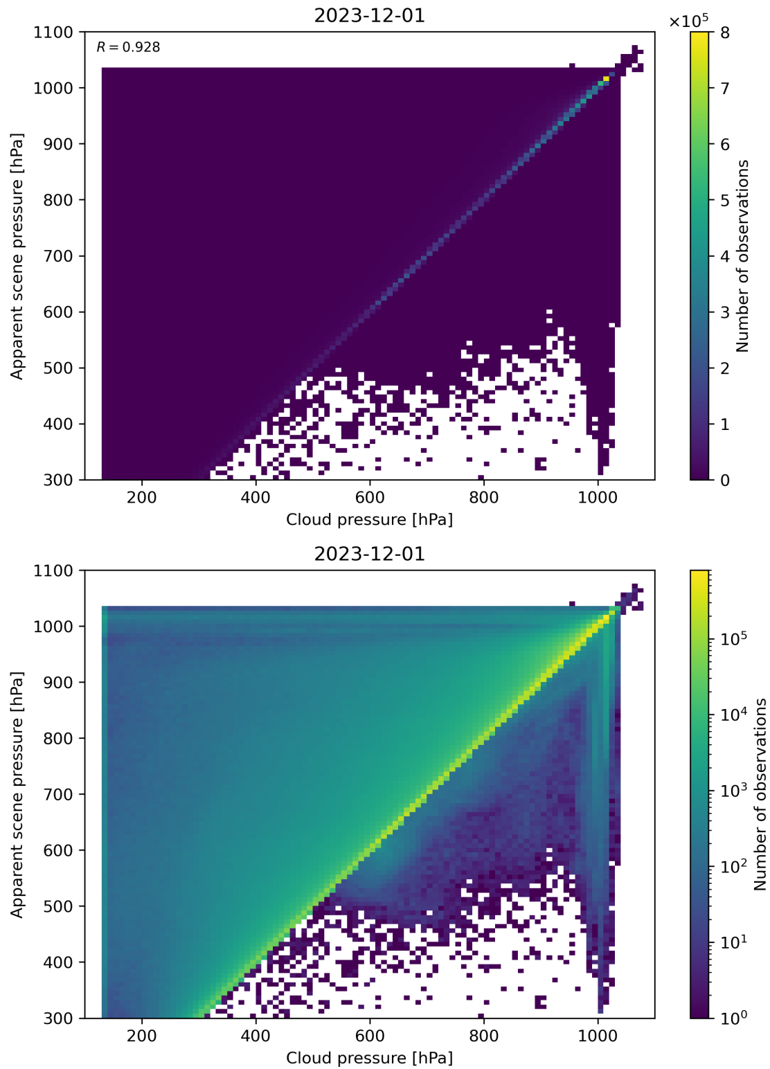
Figure 77: Scatter density plot of “Cloud pressure” against “Apparent scene pressure” for 2023-11-30 to 2023-12-02.
