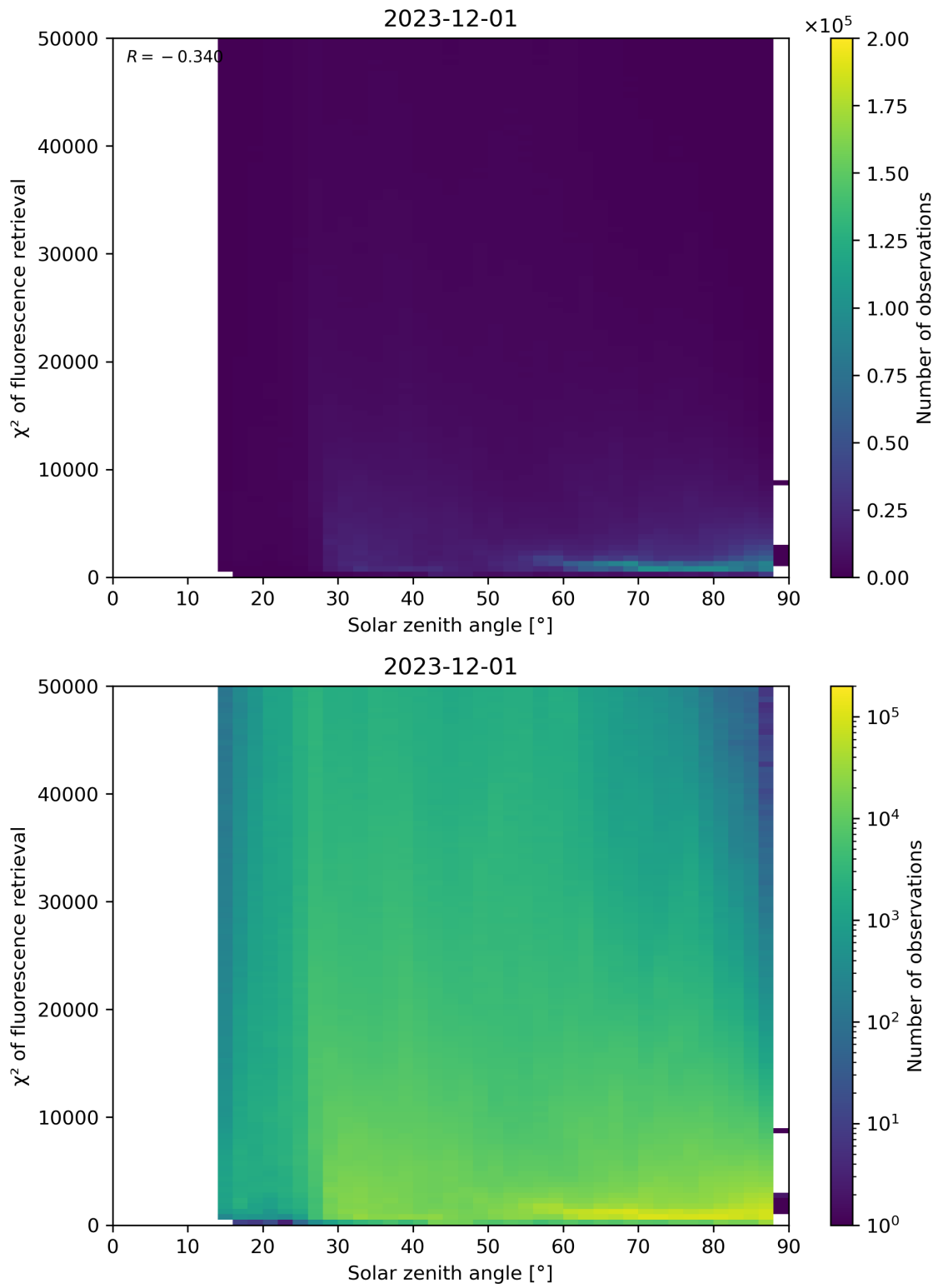
Figure 109: Scatter density plot of “Solar zenith angle” against “ \chi^2 of fluorescence retrieval” for 2023-11-30 to 2023-12-02.
