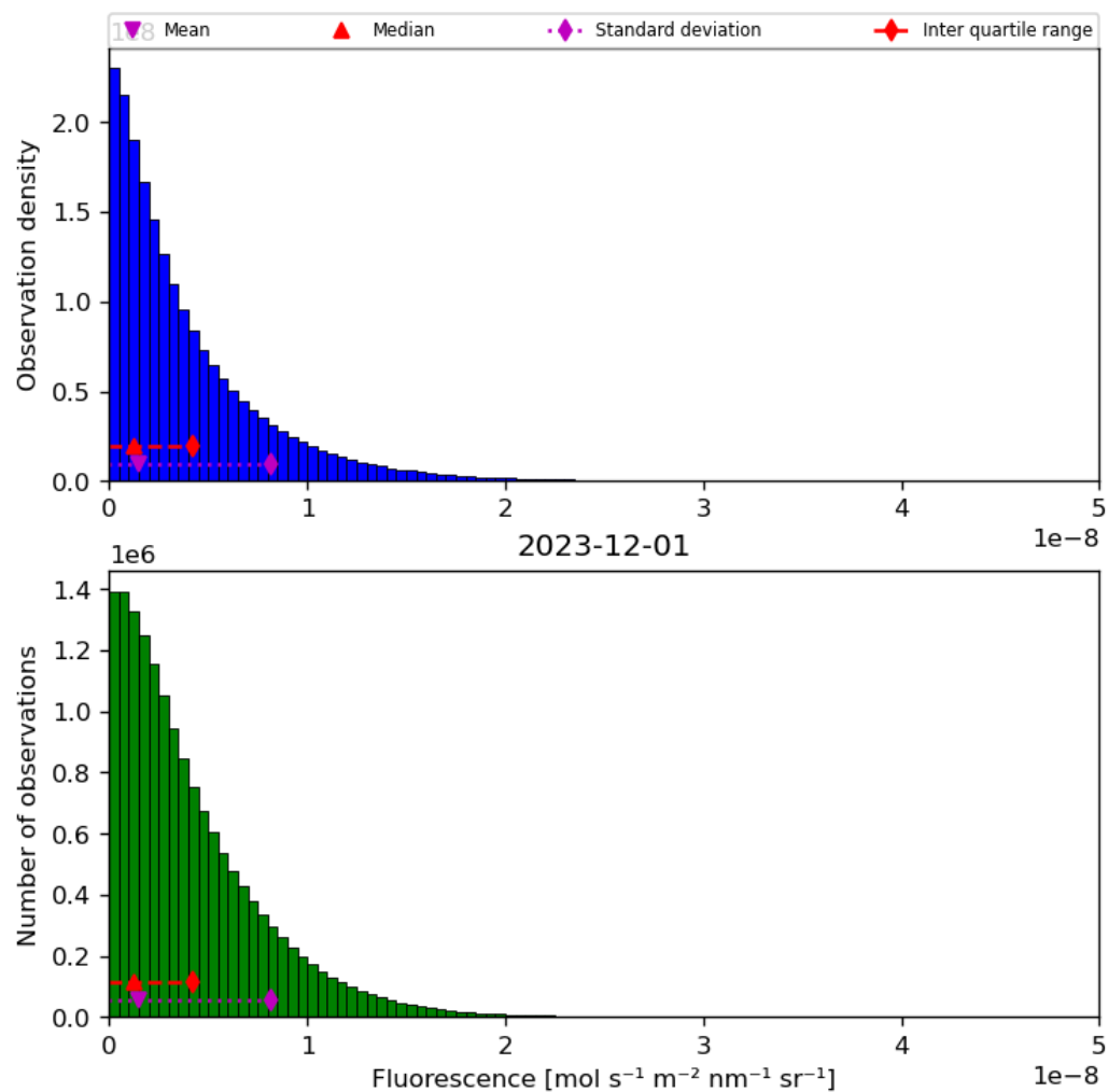
Figure 40: Histogram of “Fluorescence” for 2023-11-30 to 2023-12-02
