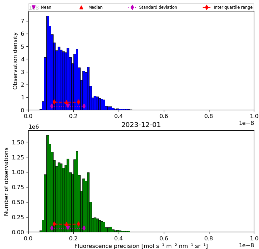
Figure 41: Histogram of “Fluorescence precision” for 2023-11-30 to 2023-12-02
