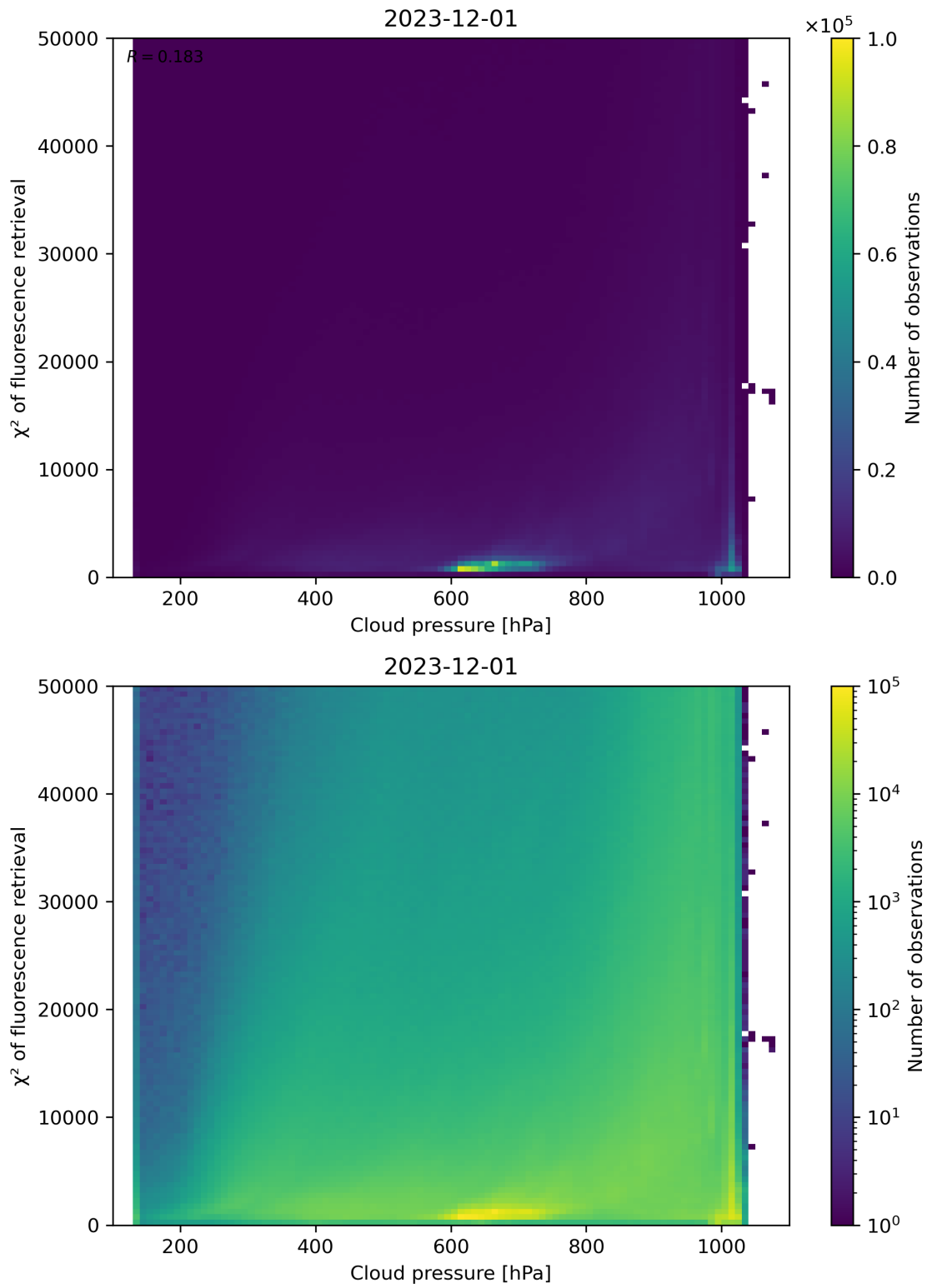
Figure 78: Scatter density plot of “Cloud pressure” against “ \chi^2 of fluorescence retrieval” for 2023-11-30 to 2023-12-02.
