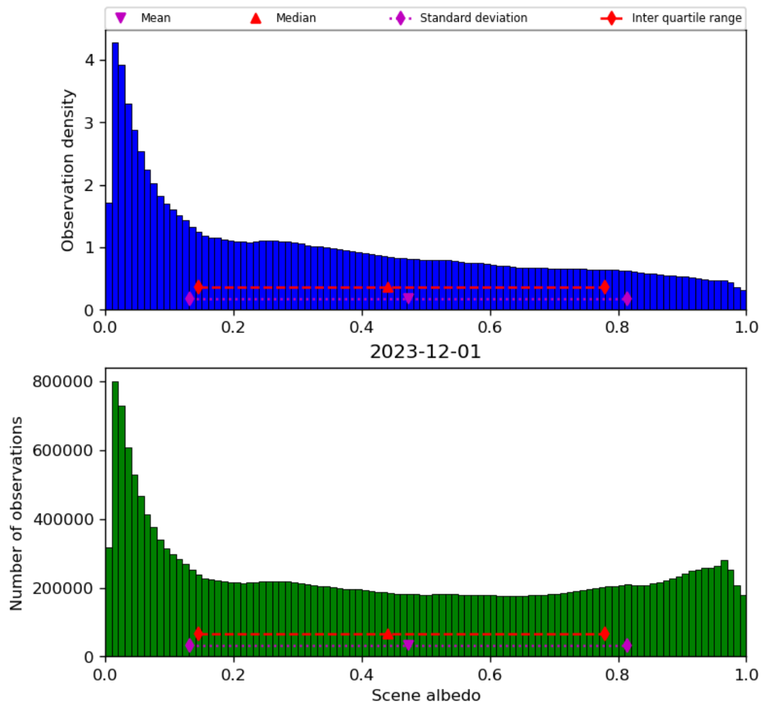
Figure 34: Histogram of “Scene albedo” for 2023-11-30 to 2023-12-02
