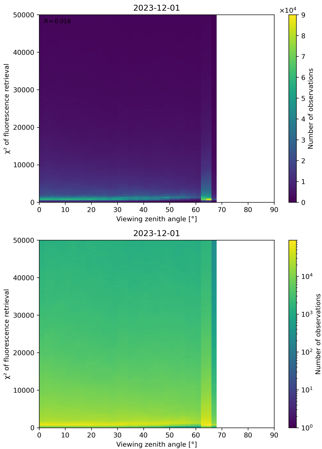
Figure 119: Scatter density plot of “Viewing zenith angle” against “ \chi^2 of fluorescence retrieval” for 2023-11-30 to 2023-12-02.
