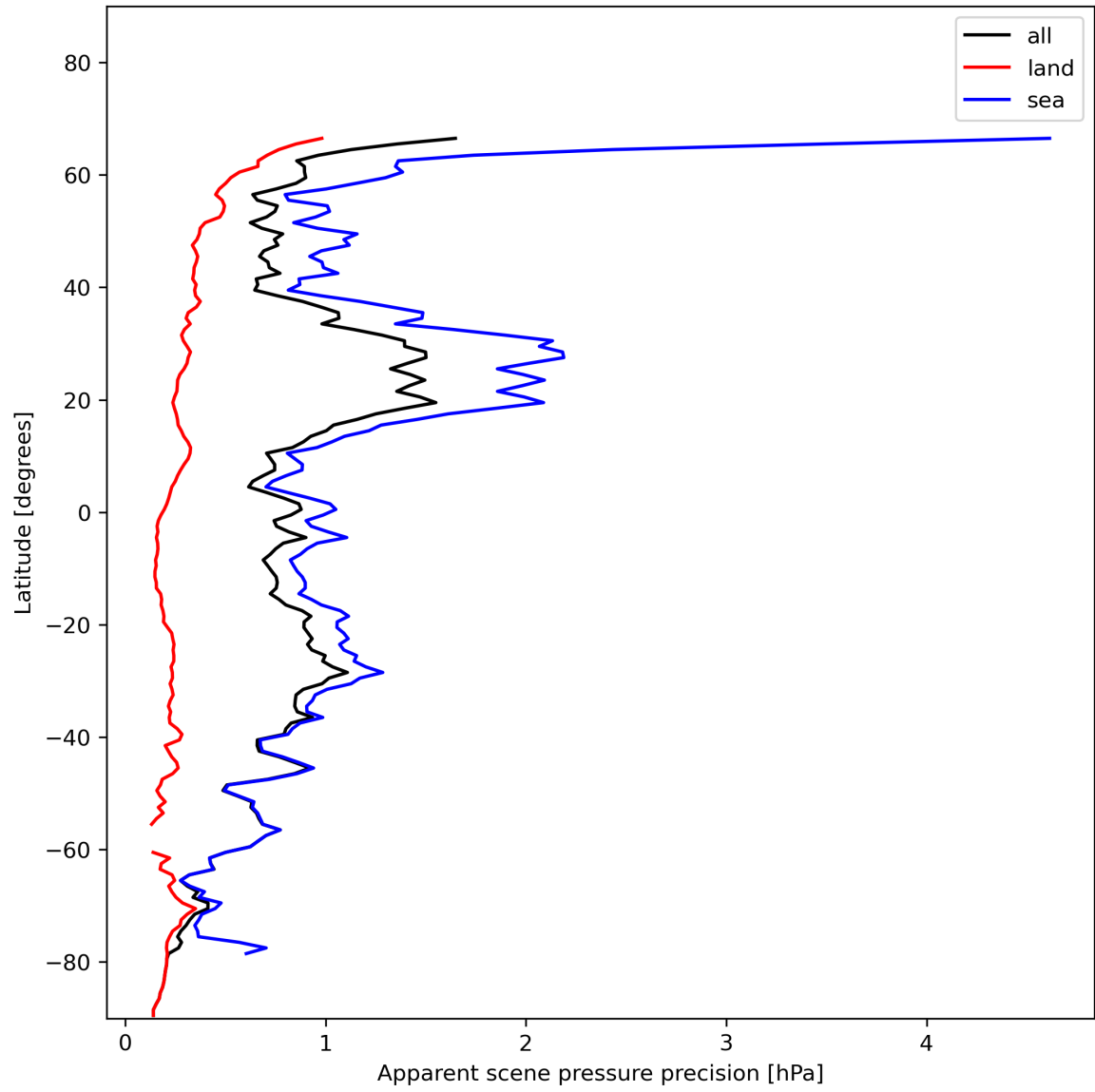
Figure 20: Zonal average of “Apparent scene pressure precision” for 2023-11-30 to 2023-12-02.
