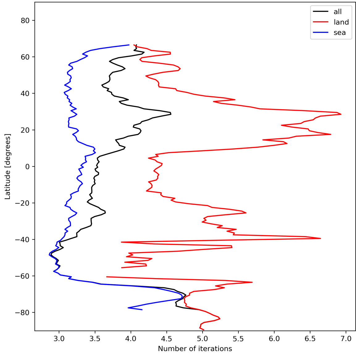
Figure 22: Zonal average of “Number of iterations” for 2023-11-30 to 2023-12-02.
