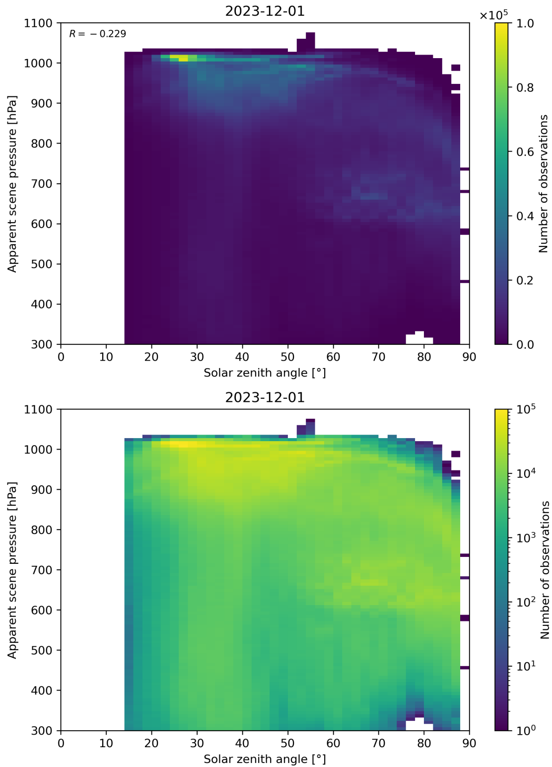
Figure 108: Scatter density plot of “Solar zenith angle” against “Apparent scene pressure” for 2023-11-30 to 2023-12-02.
