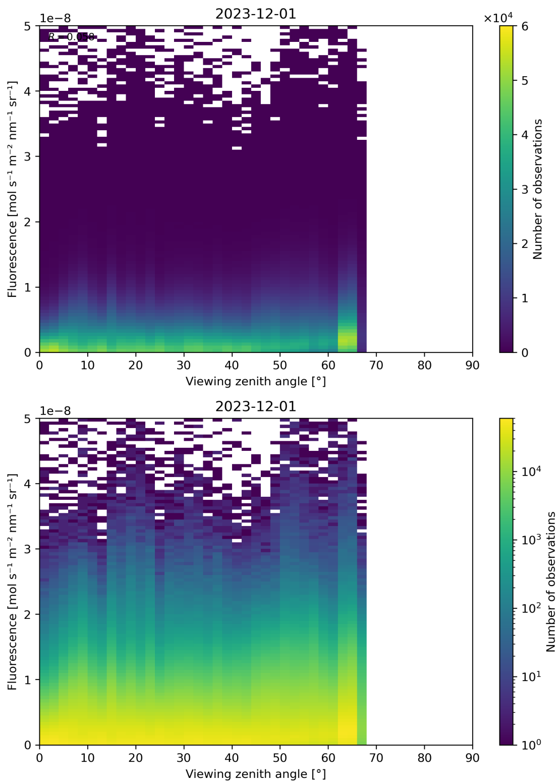
Figure 122: Scatter density plot of “Viewing zenith angle” against “Fluorescence” for 2023-11-30 to 2023-12-02.
