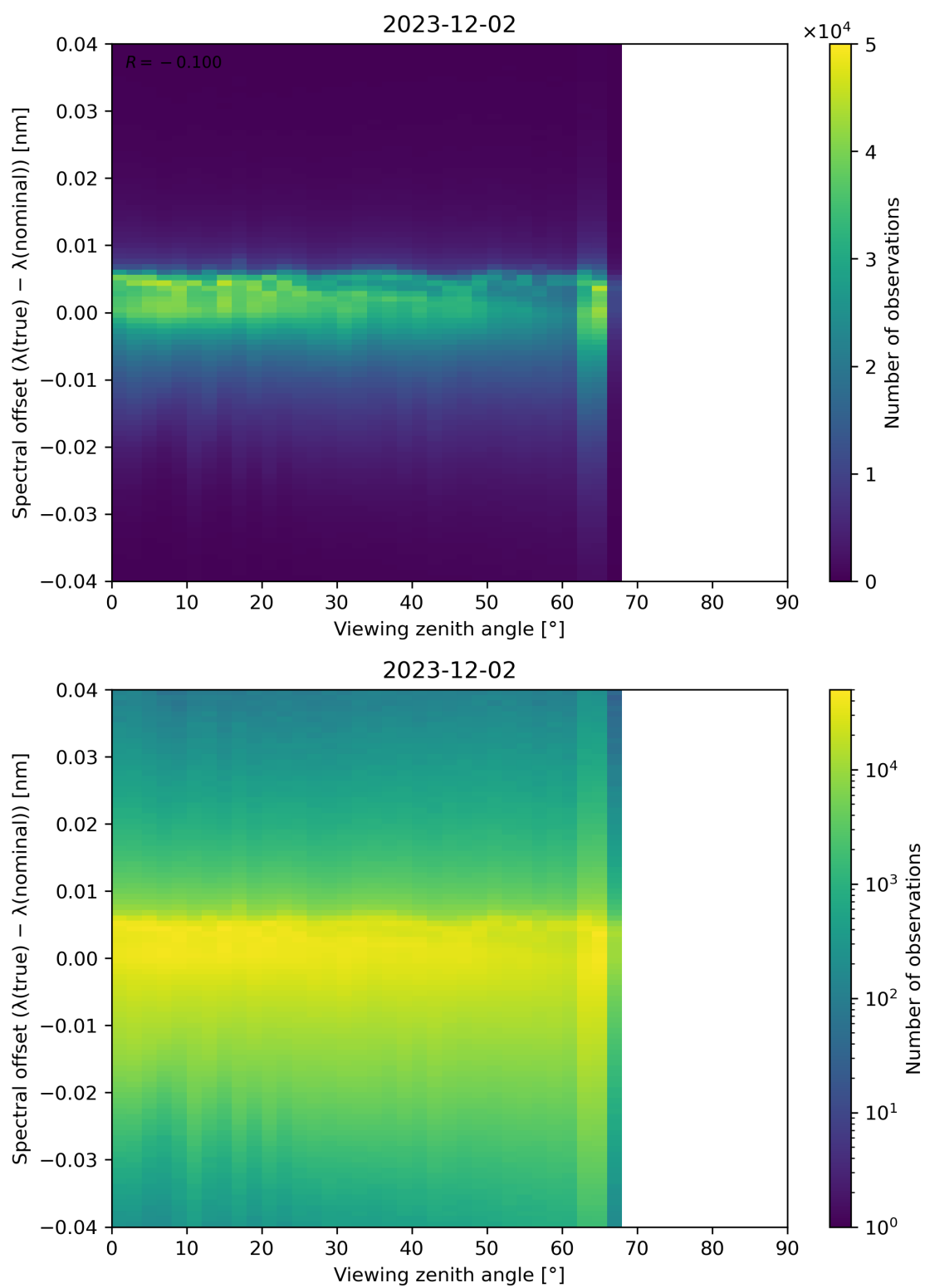
Figure 128: Scatter density plot of “Viewing zenith angle” against “Spectral offset ( \lambda(\text{true}) - \lambda(\text{nominal}) )” for 2023-12-01 to 2023-12-03.
