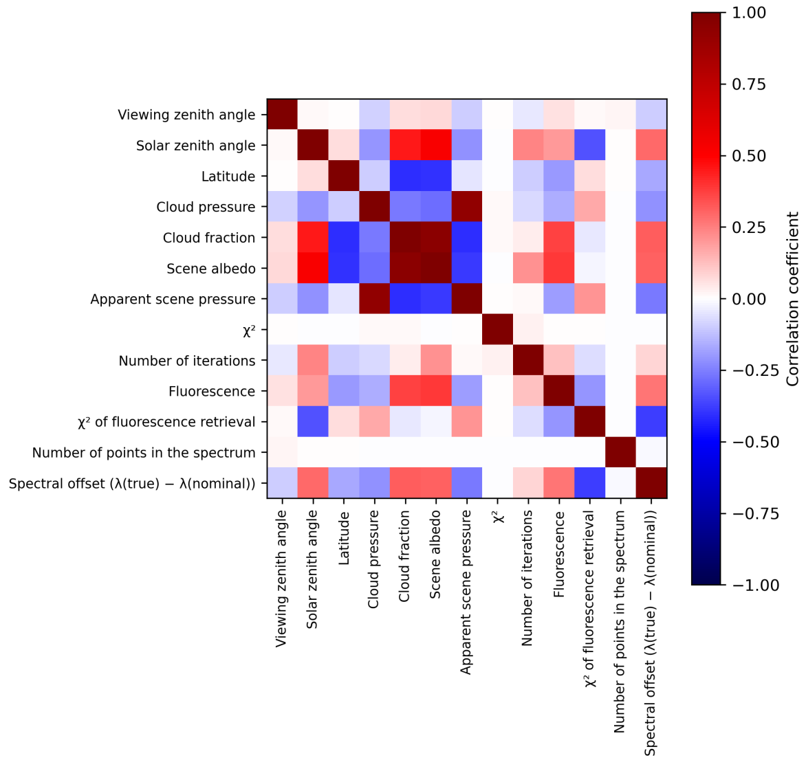
Figure 2: Map of correlation matrix for 2023-12-01 to 2023-12-03.
