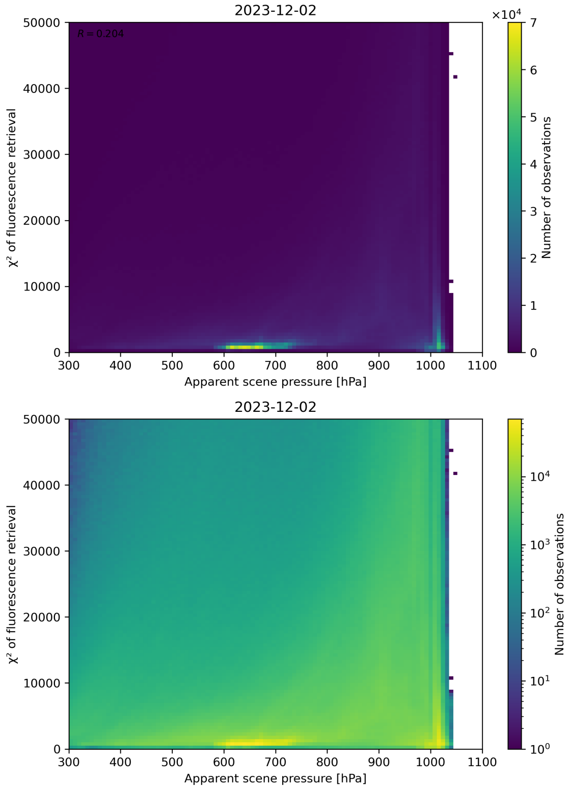
Figure 63: Scatter density plot of “Apparent scene pressure” against “ \chi^2 of fluorescence retrieval” for 2023-12-01 to 2023-12-03.
