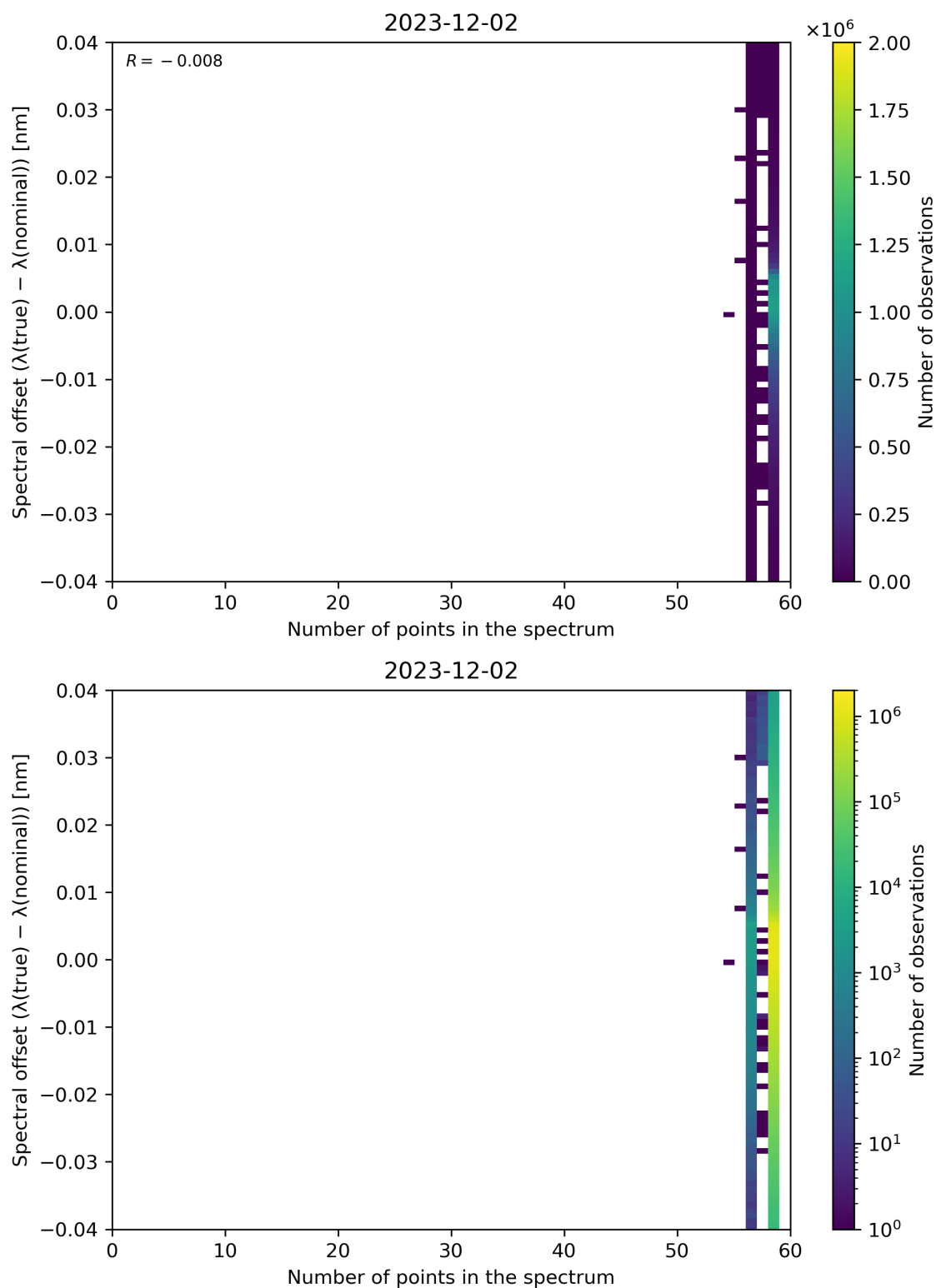
Figure 101: Scatter density plot of “Number of points in the spectrum” against “Spectral offset ( \lambda(\text{true}) - \lambda(\text{nominal})) ” for 2023-12-01 to 2023-12-03.
