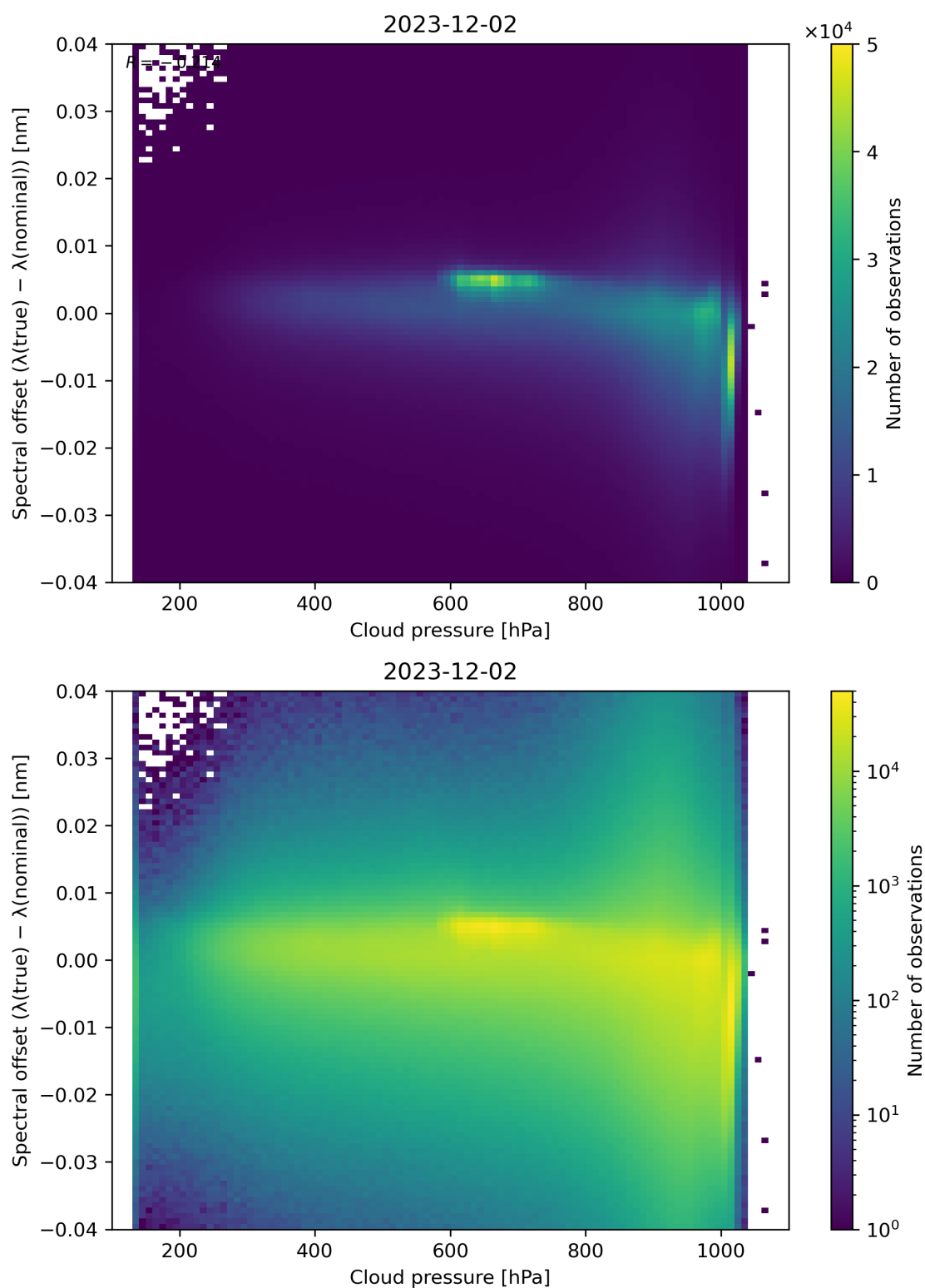
Figure 84: Scatter density plot of “Cloud pressure” against “Spectral offset ( \lambda(\text{true}) - \lambda(\text{nominal}) )” for 2023-12-01 to 2023-12-03.
