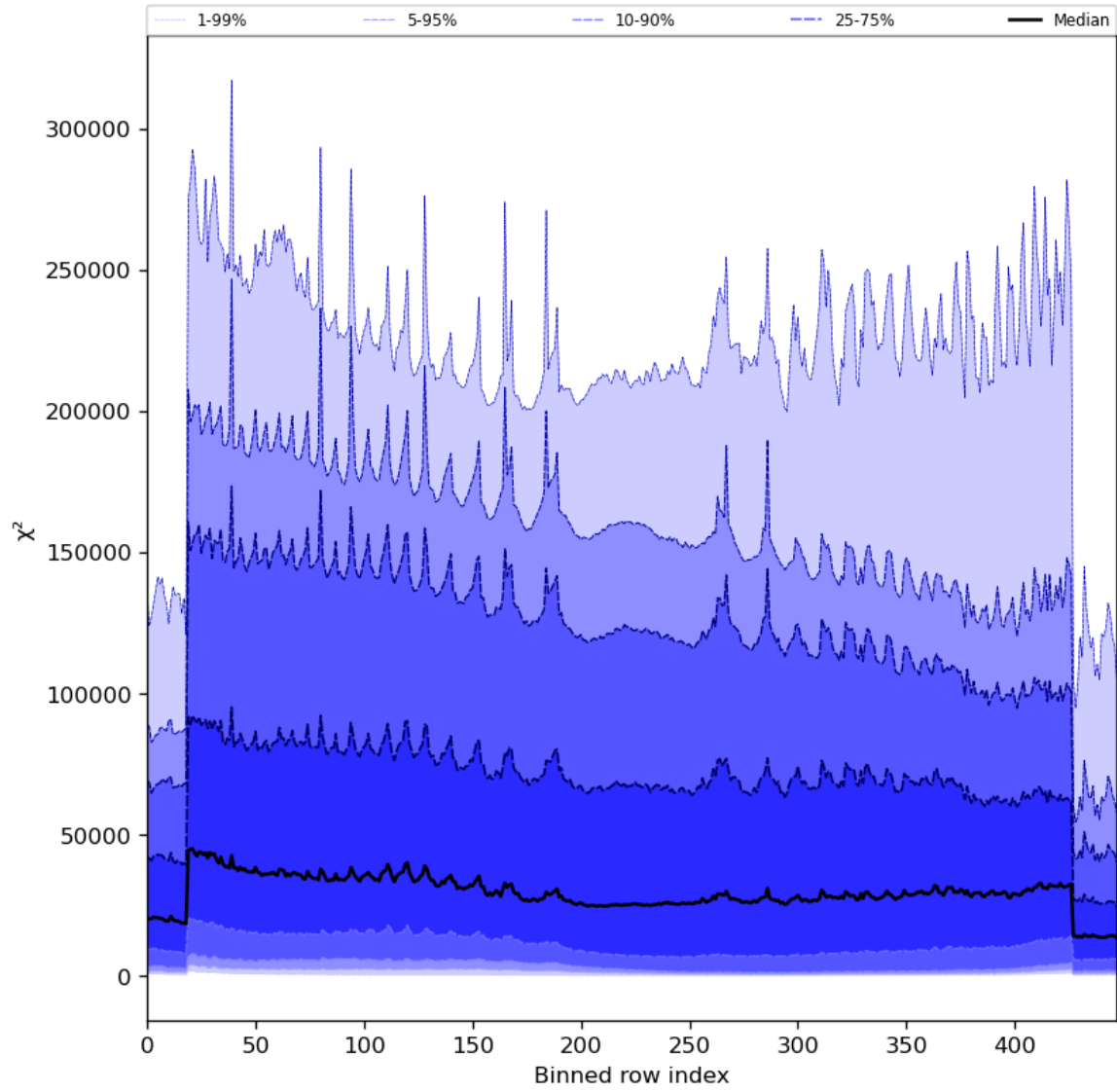
Figure 55: Along track statistics of “ \chi^2 ” for 2023-12-01 to 2023-12-03
