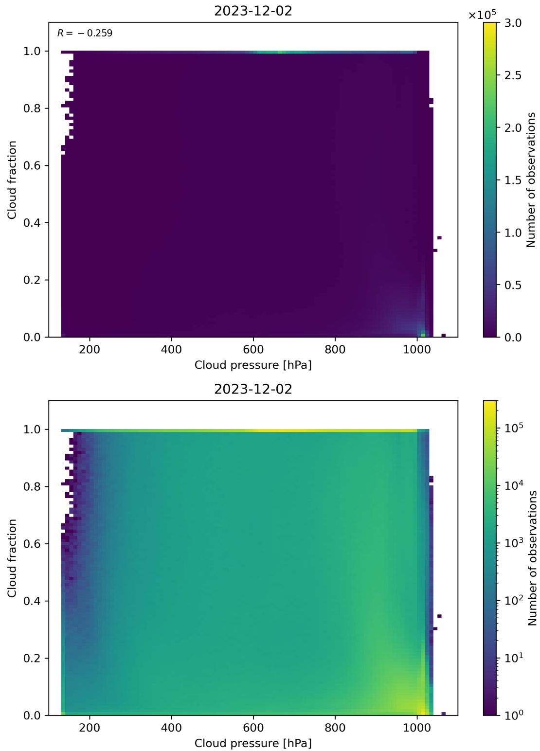
Figure 79: Scatter density plot of “Cloud pressure” against “Cloud fraction” for 2023-12-01 to 2023-12-03.
