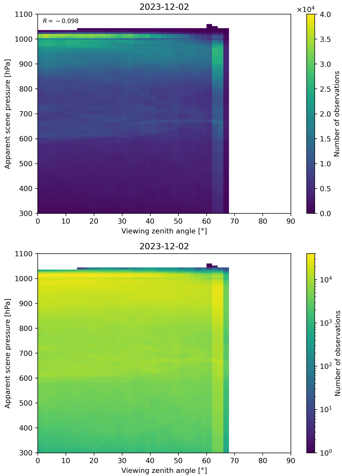
Figure 118: Scatter density plot of “Viewing zenith angle” against “Apparent scene pressure” for 2023-12-01 to 2023-12-03.
