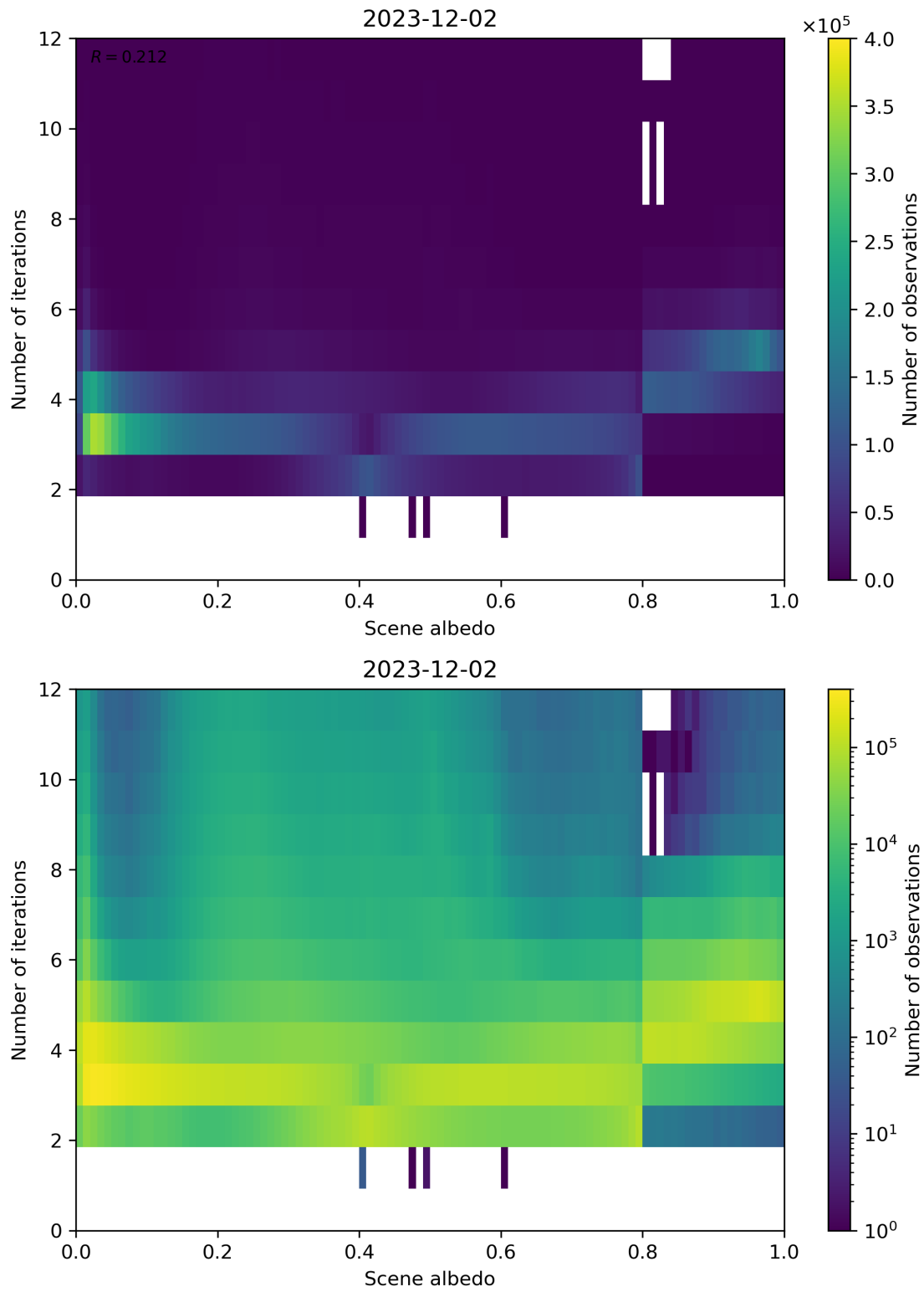
Figure 105: Scatter density plot of “Scene albedo” against “Number of iterations” for 2023-12-01 to 2023-12-03.
