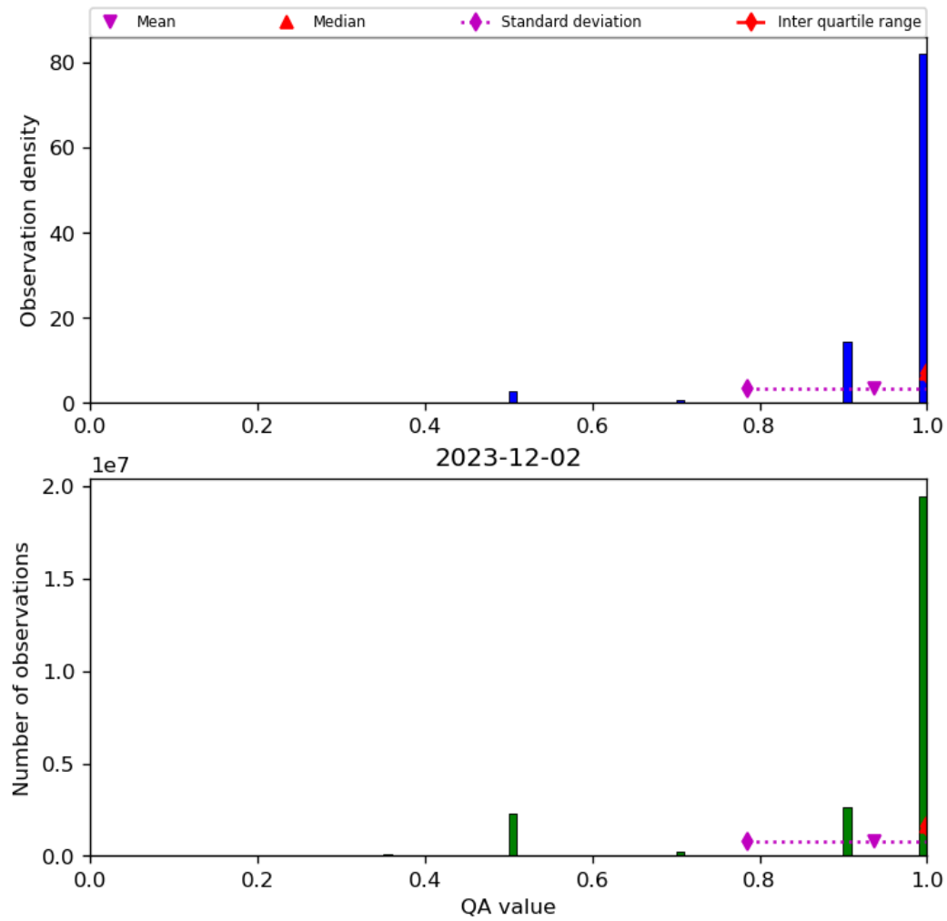
Figure 29: Histogram of “QA value” for 2023-12-01 to 2023-12-03
