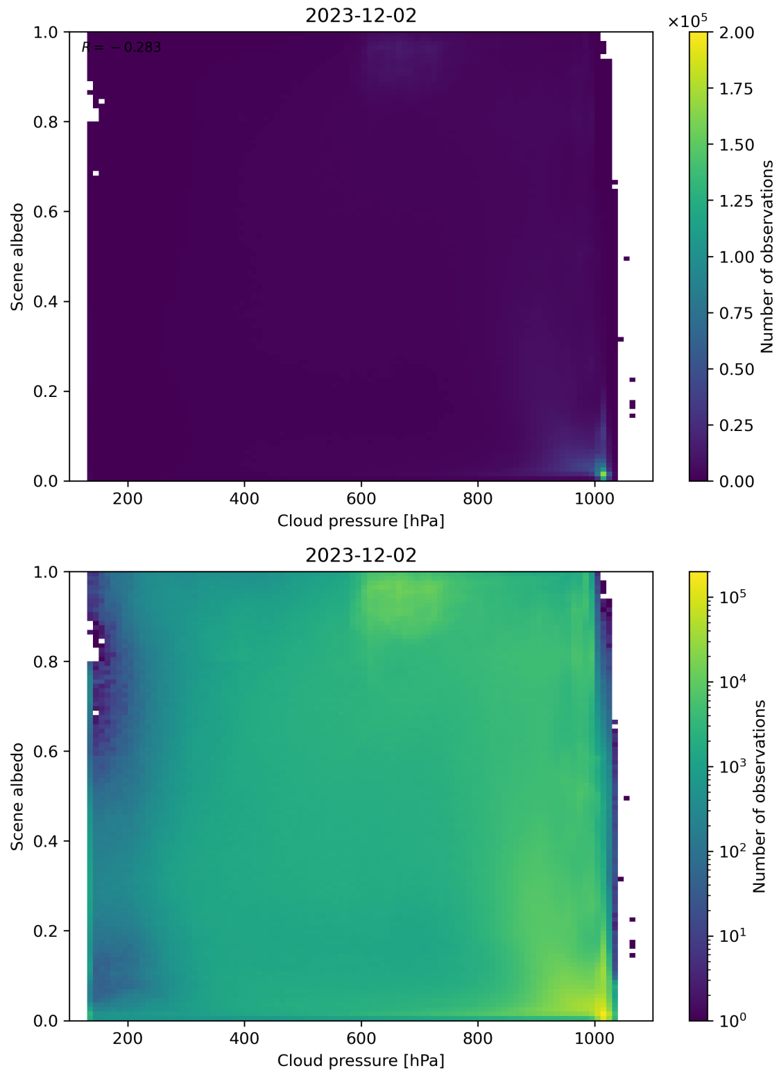
Figure 83: Scatter density plot of “Cloud pressure” against “Scene albedo” for 2023-12-01 to 2023-12-03.
