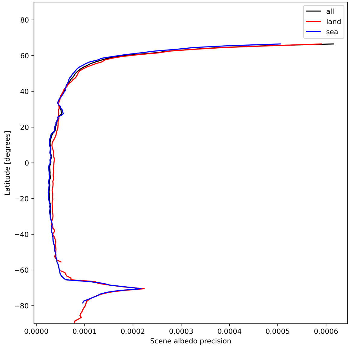
Figure 18: Zonal average of “Scene albedo precision” for 2023-12-01 to 2023-12-03.
