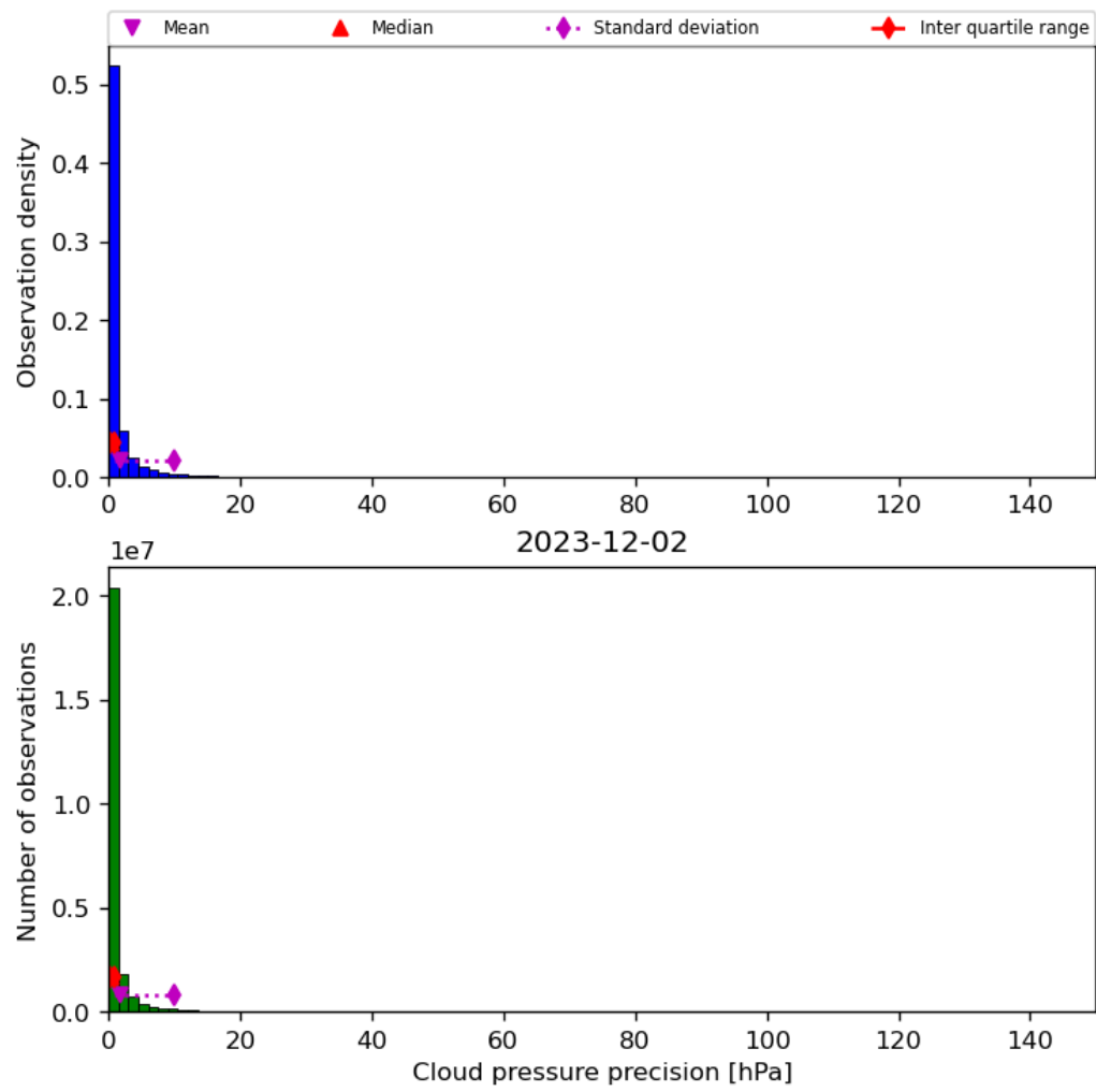
Figure 31: Histogram of “Cloud pressure precision” for 2023-12-01 to 2023-12-03
