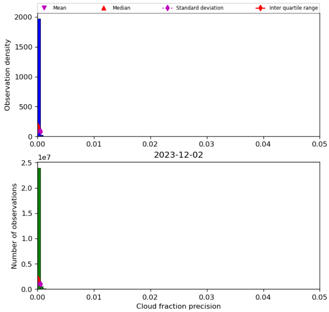
Figure 33: Histogram of “Cloud fraction precision” for 2023-12-01 to 2023-12-03
