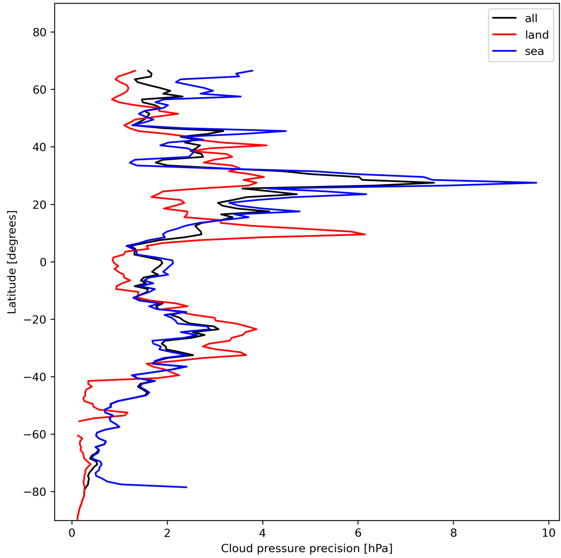
Figure 14: Zonal average of "Cloud pressure precision" for 2023-12-01 to 2023-12-03.
