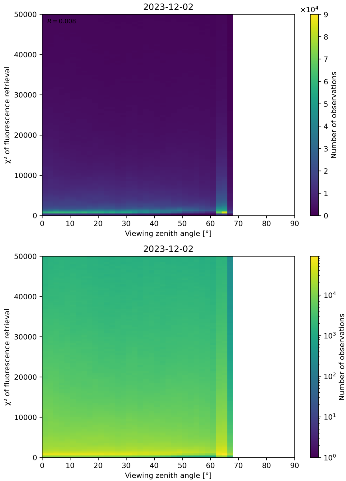
Figure 119: Scatter density plot of “Viewing zenith angle” against “ \chi^2 of fluorescence retrieval” for 2023-12-01 to 2023-12-03.
