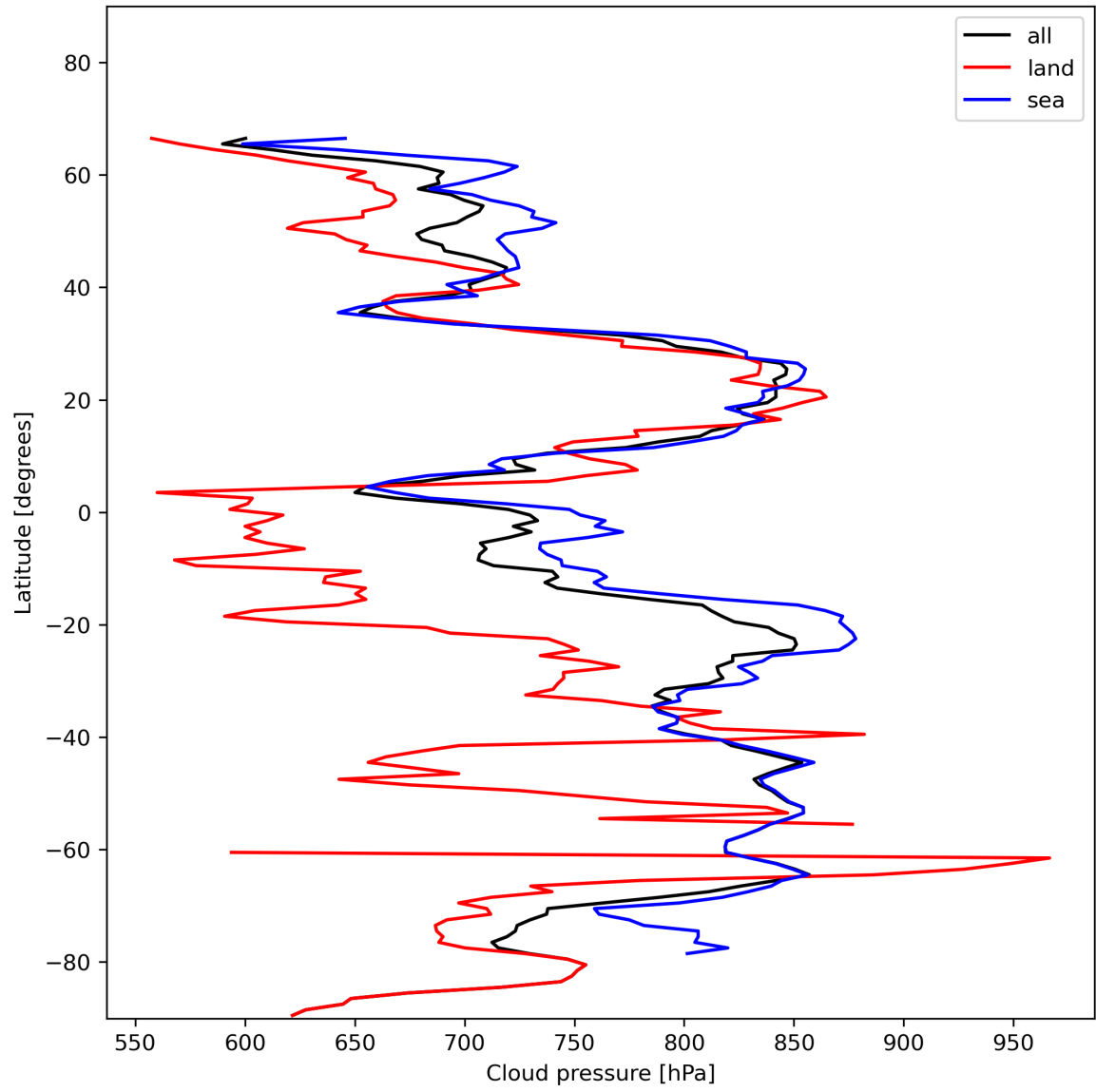
Figure 13: Zonal average of “Cloud pressure” for 2023-12-01 to 2023-12-03.
