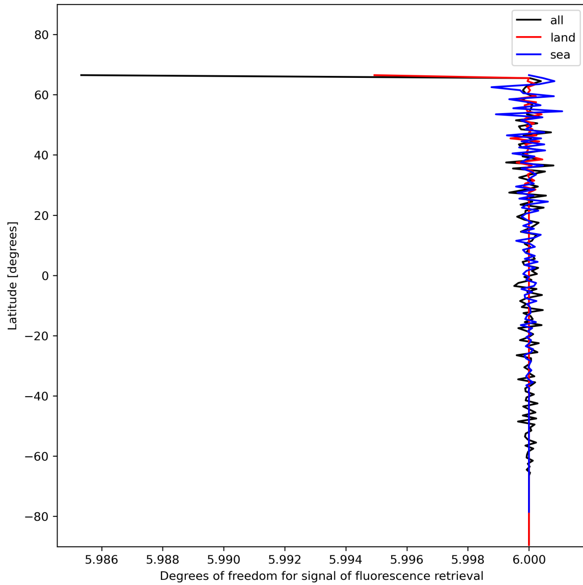
Figure 26: Zonal average of “Degrees of freedom for signal of fluorescence retrieval” for 2023-12-01 to 2023-12-03.
