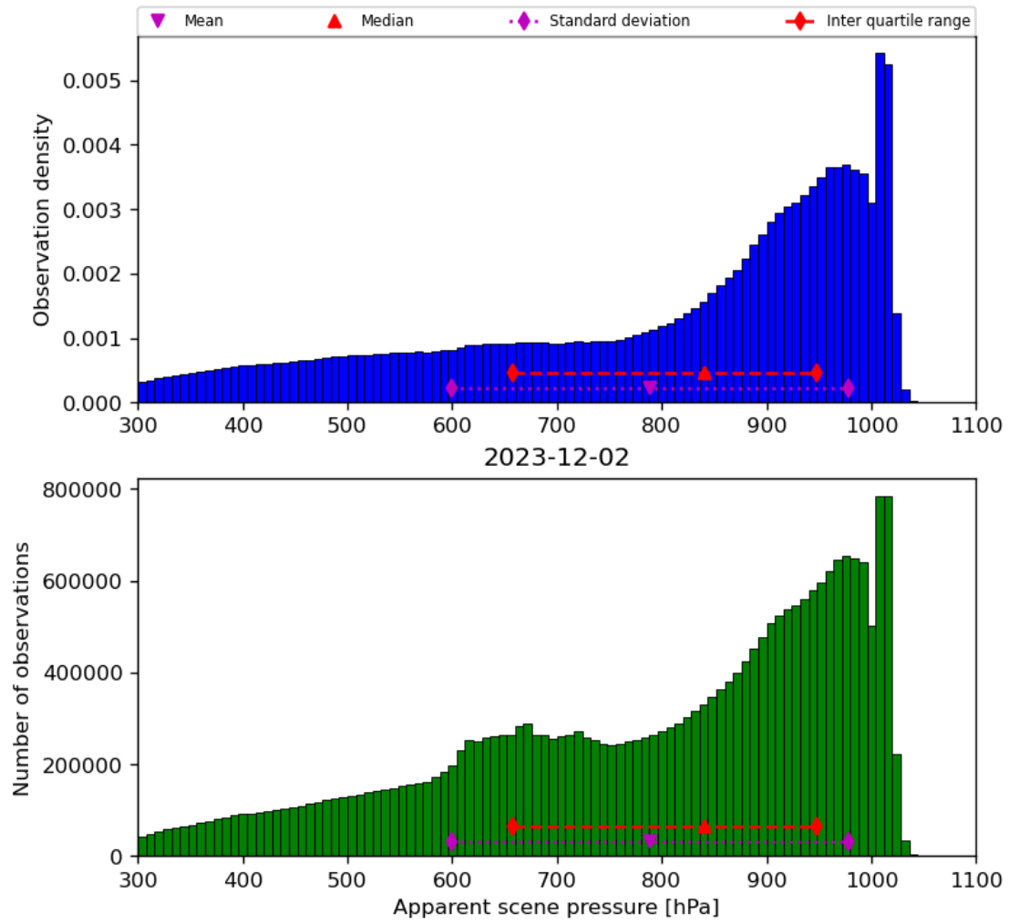
Figure 36: Histogram of “Apparent scene pressure” for 2023-12-01 to 2023-12-03
