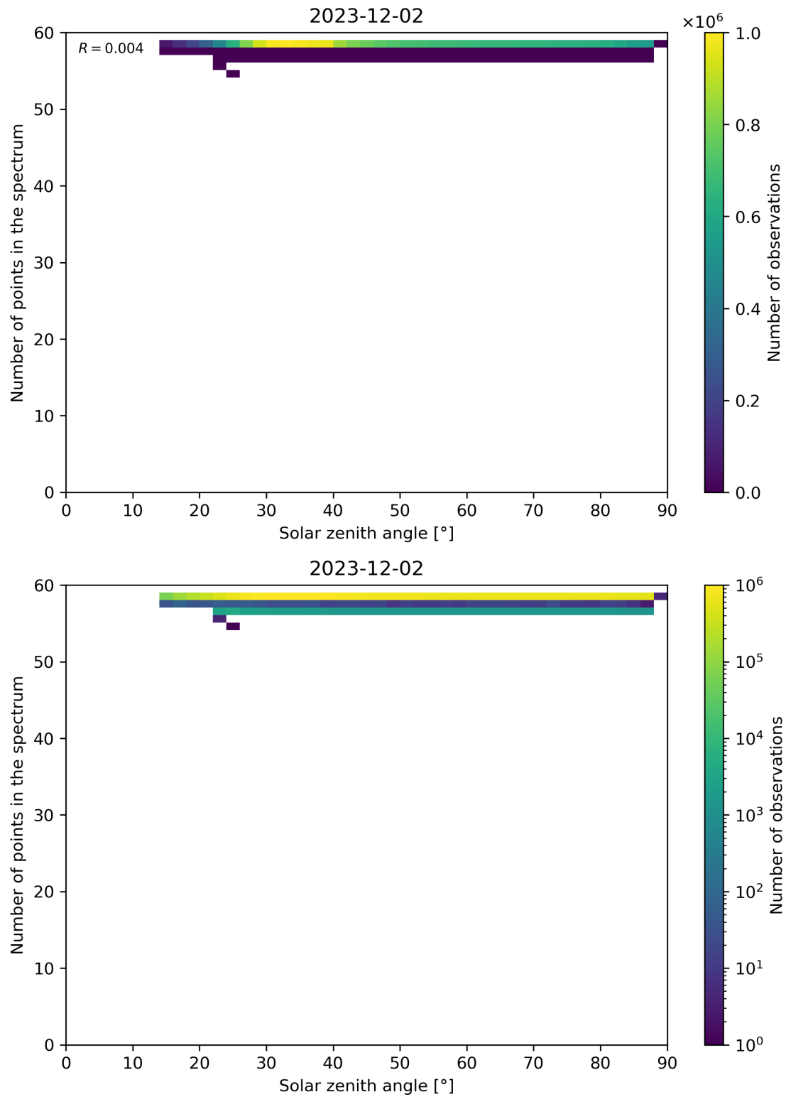
Figure 115: Scatter density plot of “Solar zenith angle” against “Number of points in the spectrum” for 2023-12-01 to 2023-12-03.
