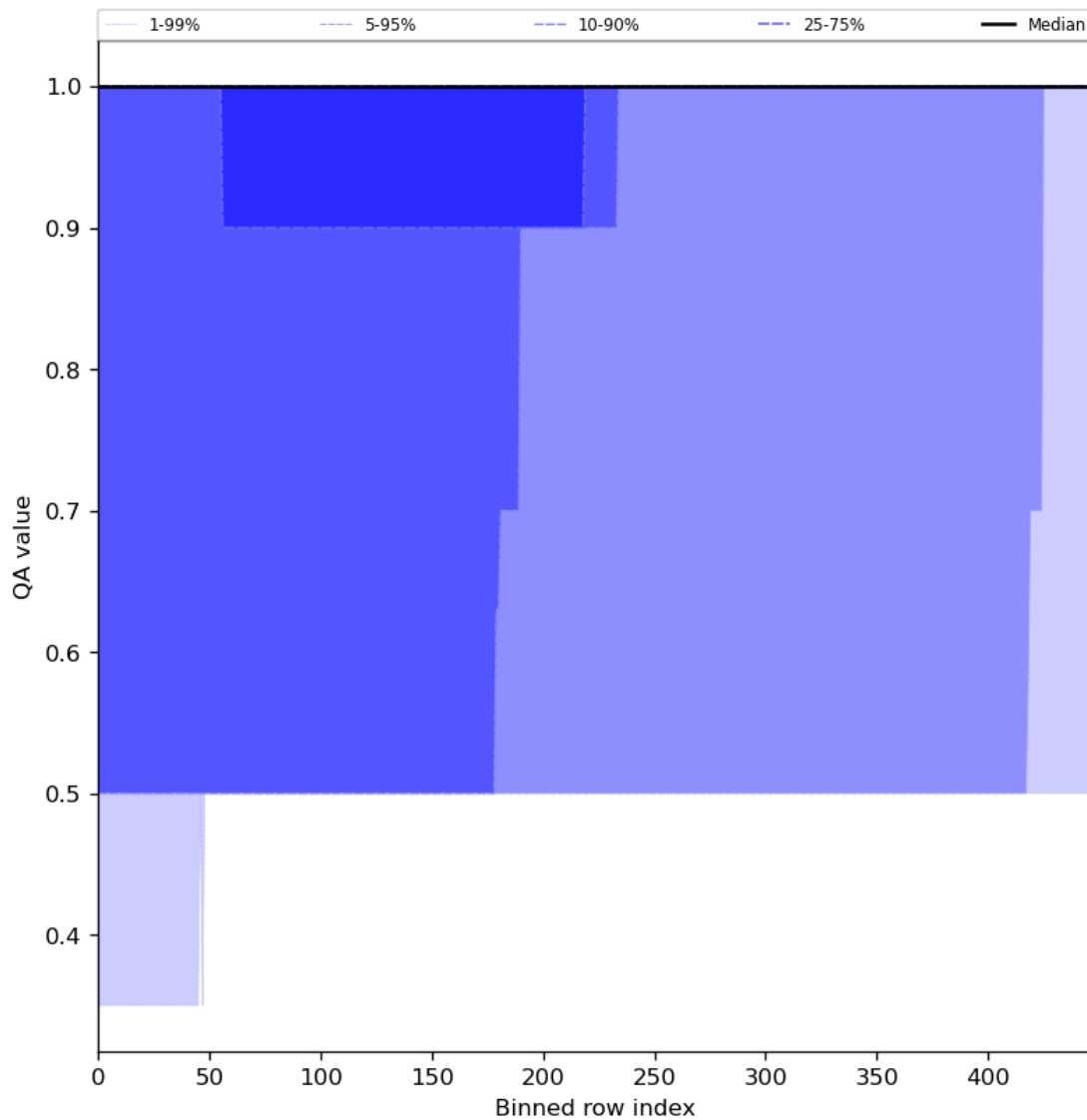
Figure 46: Along track statistics of “QA value” for 2023-12-01 to 2023-12-03
