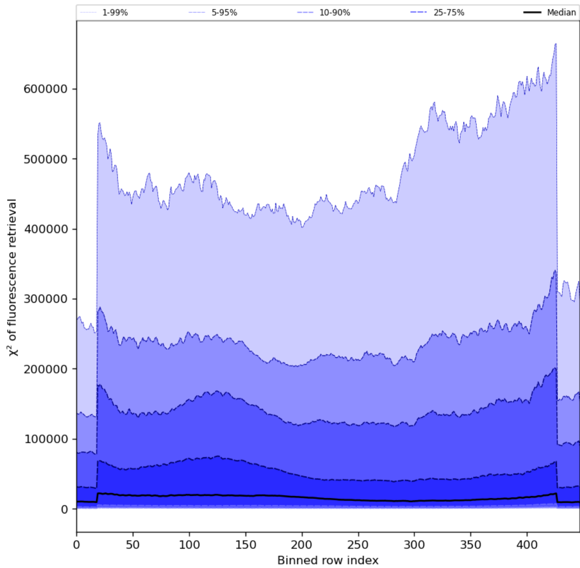
Figure 59: Along track statistics of “ \chi^2 of fluorescence retrieval” for 2023-12-01 to 2023-12-03
