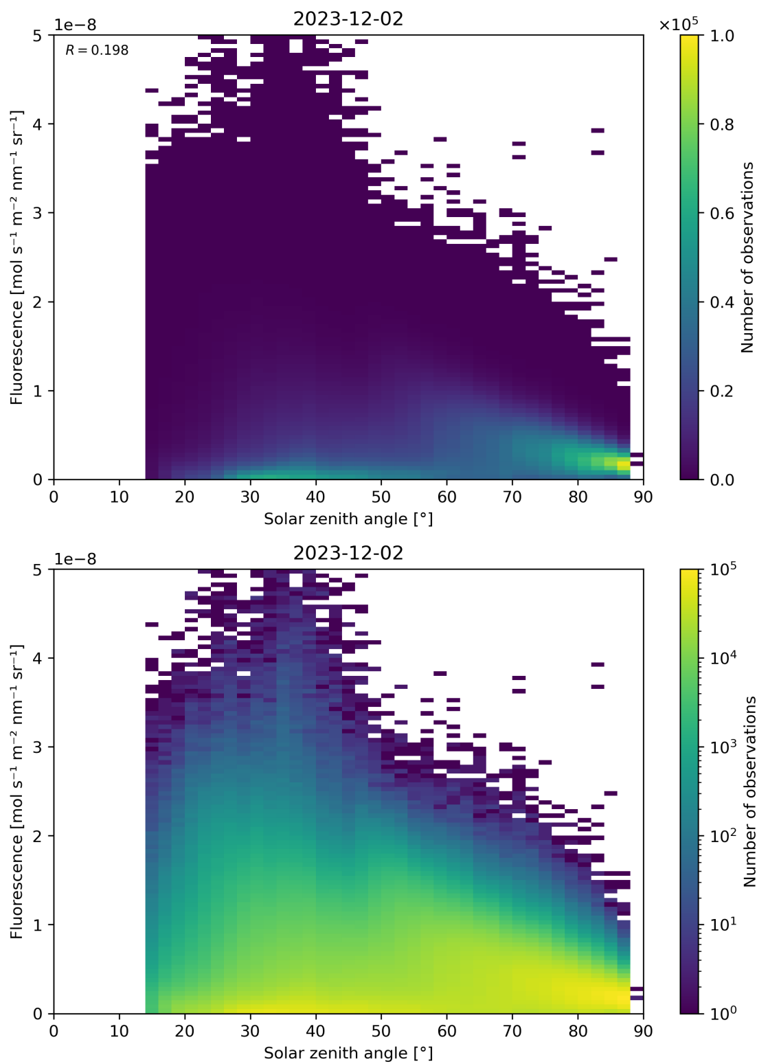
Figure 112: Scatter density plot of “Solar zenith angle” against “Fluorescence” for 2023-12-01 to 2023-12-03.
