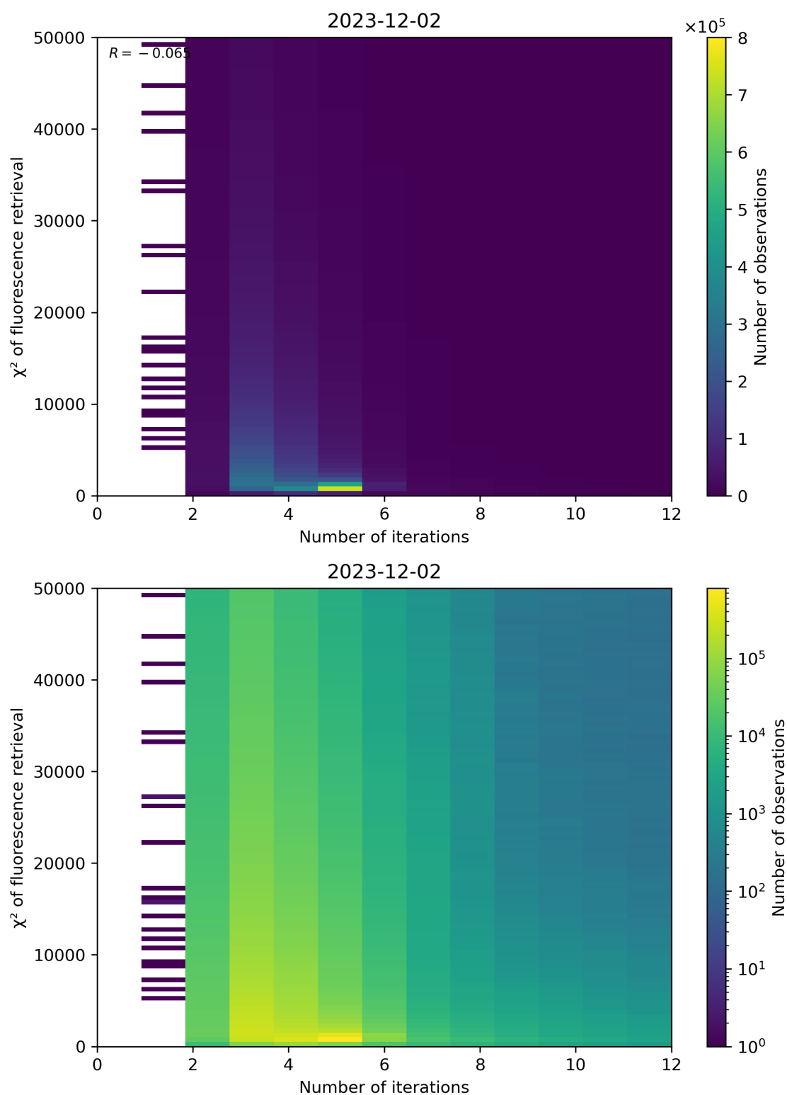
Figure 97: Scatter density plot of “Number of iterations” against “ \chi^2 of fluorescence retrieval” for 2023-12-01 to 2023-12-03.
