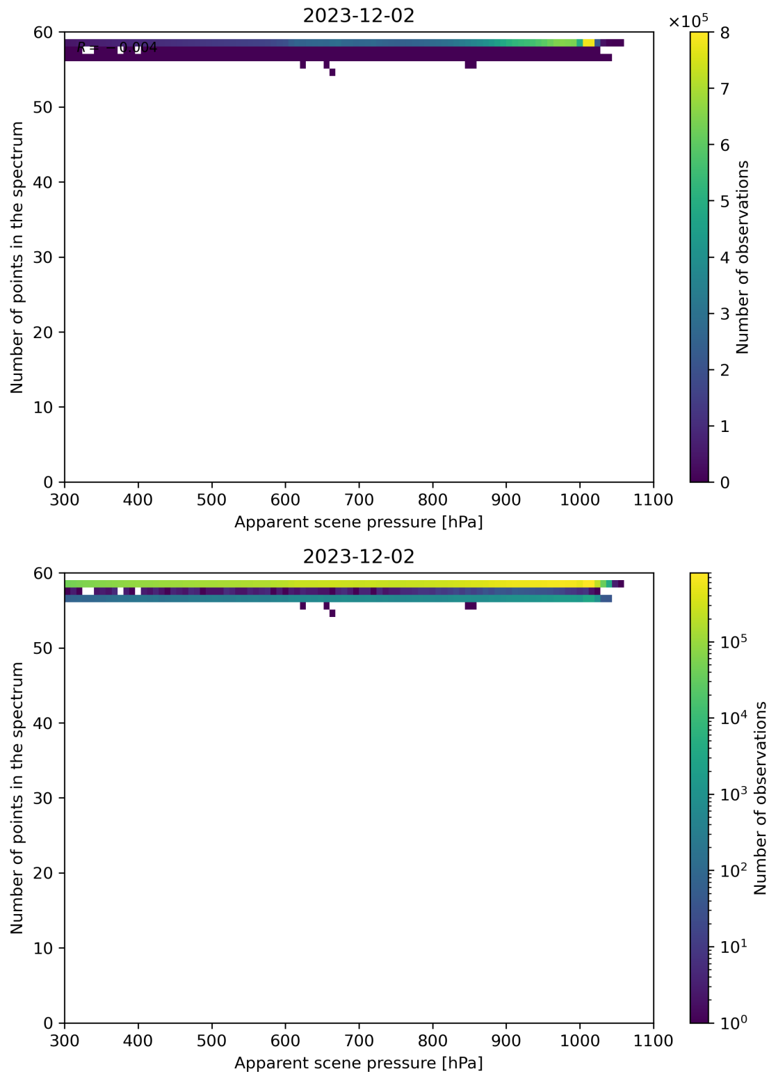
Figure 66: Scatter density plot of “Apparent scene pressure” against “Number of points in the spectrum” for 2023-12-01 to 2023-12-03.
