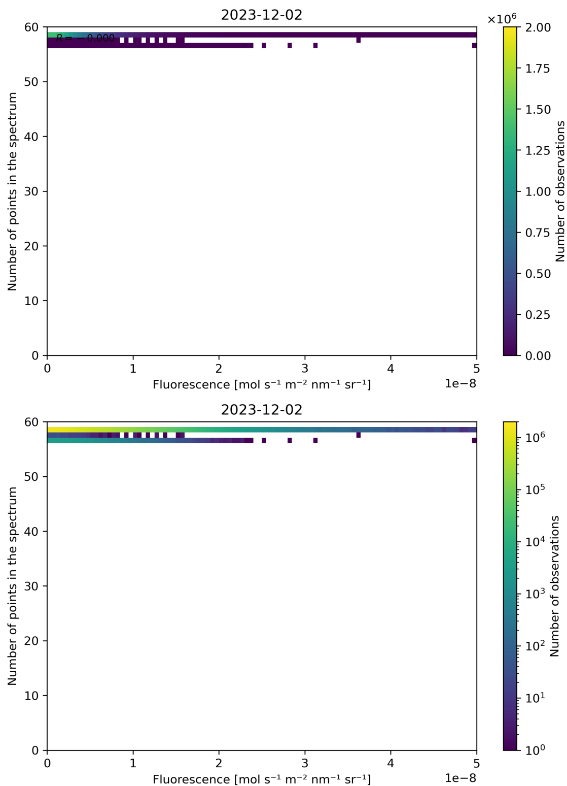
Figure 86: Scatter density plot of “Fluorescence” against “Number of points in the spectrum” for 2023-12-01 to 2023-12-03.
