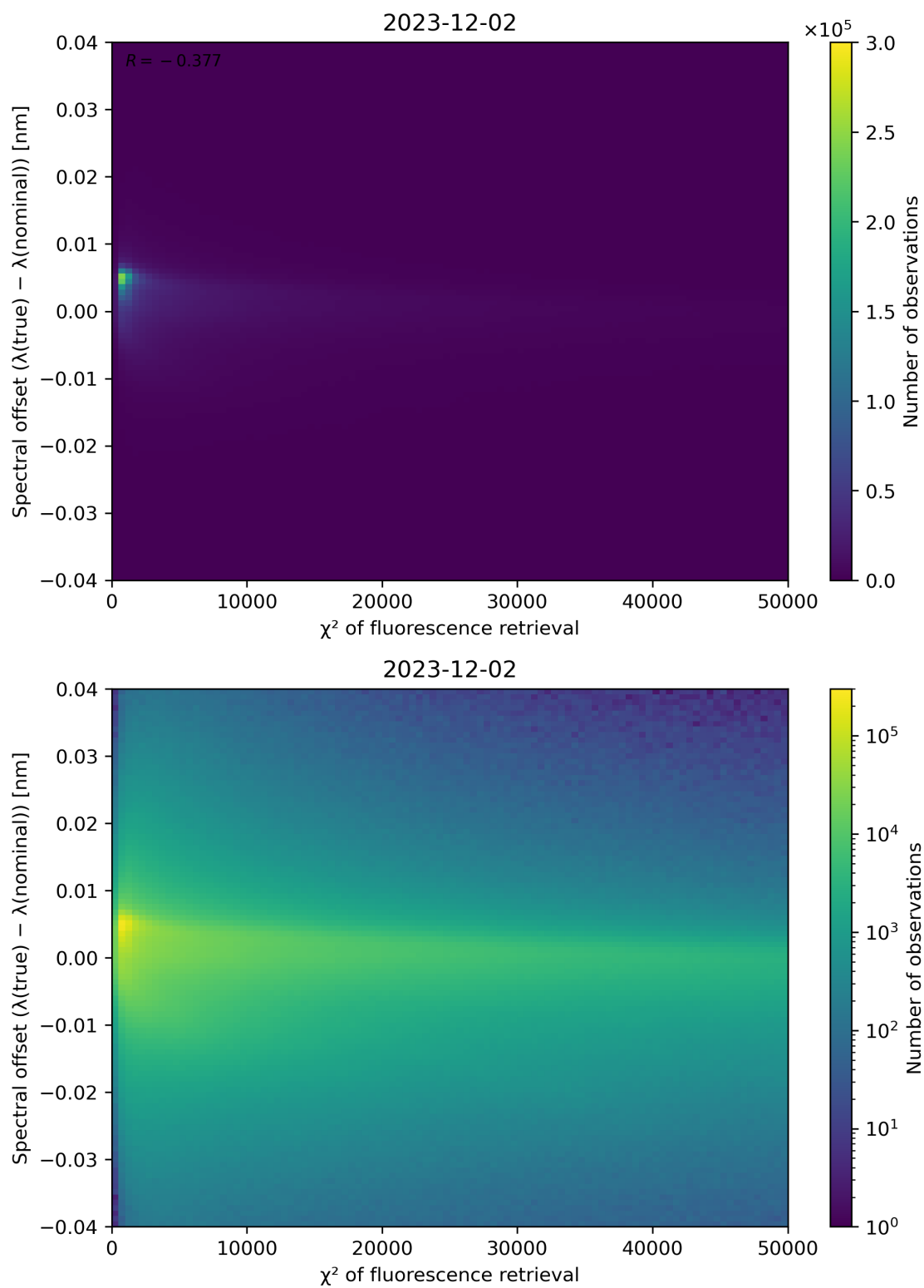
Figure 69: Scatter density plot of " \chi^2 of fluorescence retrieval" against "Spectral offset ( \lambda(\text{true}) - \lambda(\text{nominal}) )" for 2023-12-01 to 2023-12-03.
