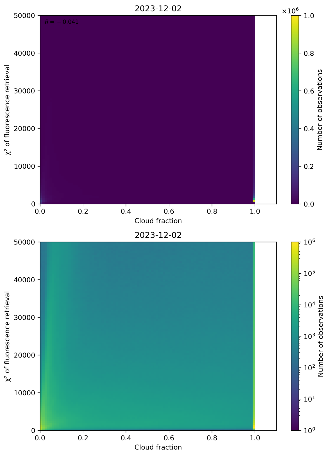
Figure 71: Scatter density plot of “Cloud fraction” against “ \chi^2 of fluorescence retrieval” for 2023-12-01 to 2023-12-03.
