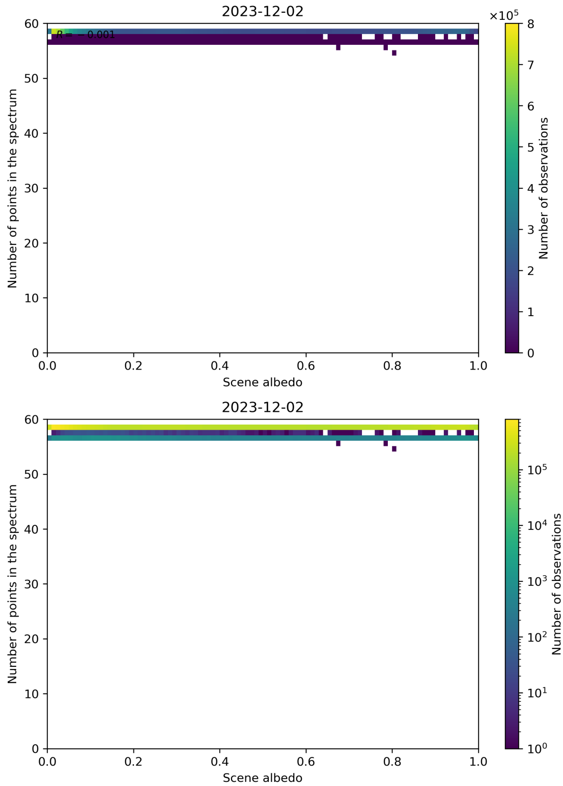
Figure 106: Scatter density plot of “Scene albedo” against “Number of points in the spectrum” for 2023-12-01 to 2023-12-03.
