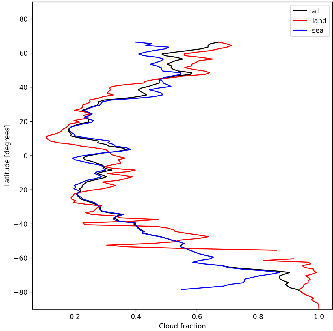
Figure 15: Zonal average of “Cloud fraction” for 2023-12-01 to 2023-12-03.
