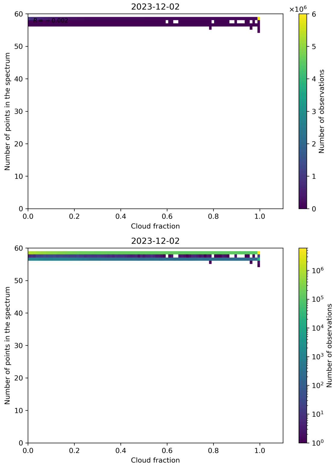
Figure 74: Scatter density plot of “Cloud fraction” against “Number of points in the spectrum” for 2023-12-01 to 2023-12-03.
