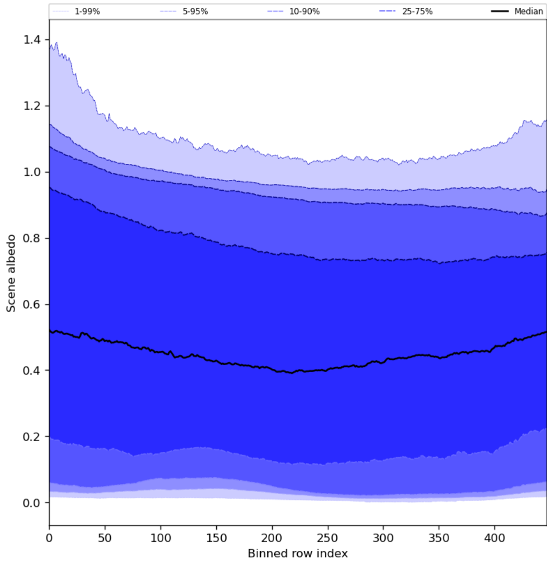
Figure 51: Along track statistics of “Scene albedo” for 2023-12-01 to 2023-12-03
