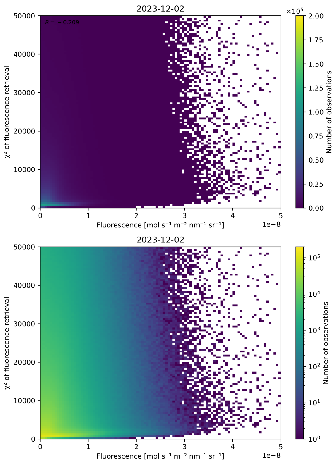
Figure 85: Scatter density plot of “Fluorescence” against “ \chi^2 of fluorescence retrieval” for 2023-12-01 to 2023-12-03.
