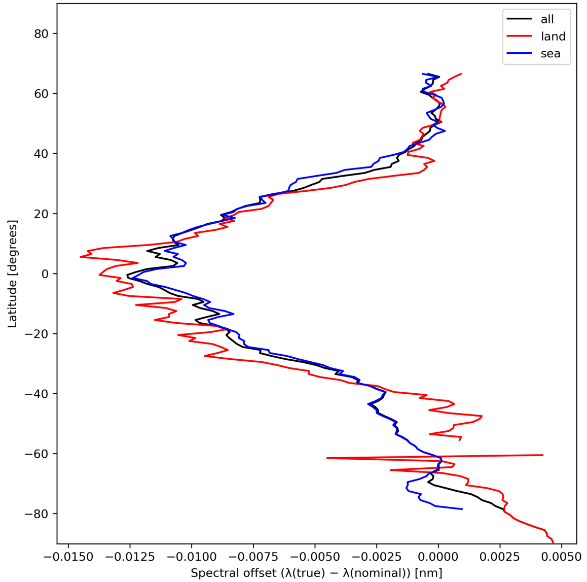
Figure 28: Zonal average of “Spectral offset ( \lambda(\text{true}) - \lambda(\text{nominal}) )” for 2023-12-01 to 2023-12-03.
