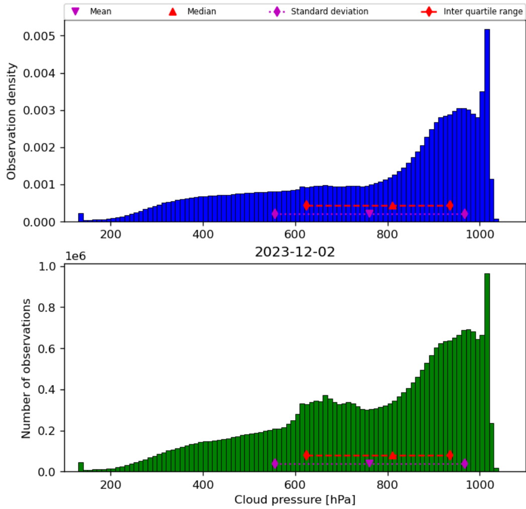
Figure 30: Histogram of “Cloud pressure” for 2023-12-01 to 2023-12-03
