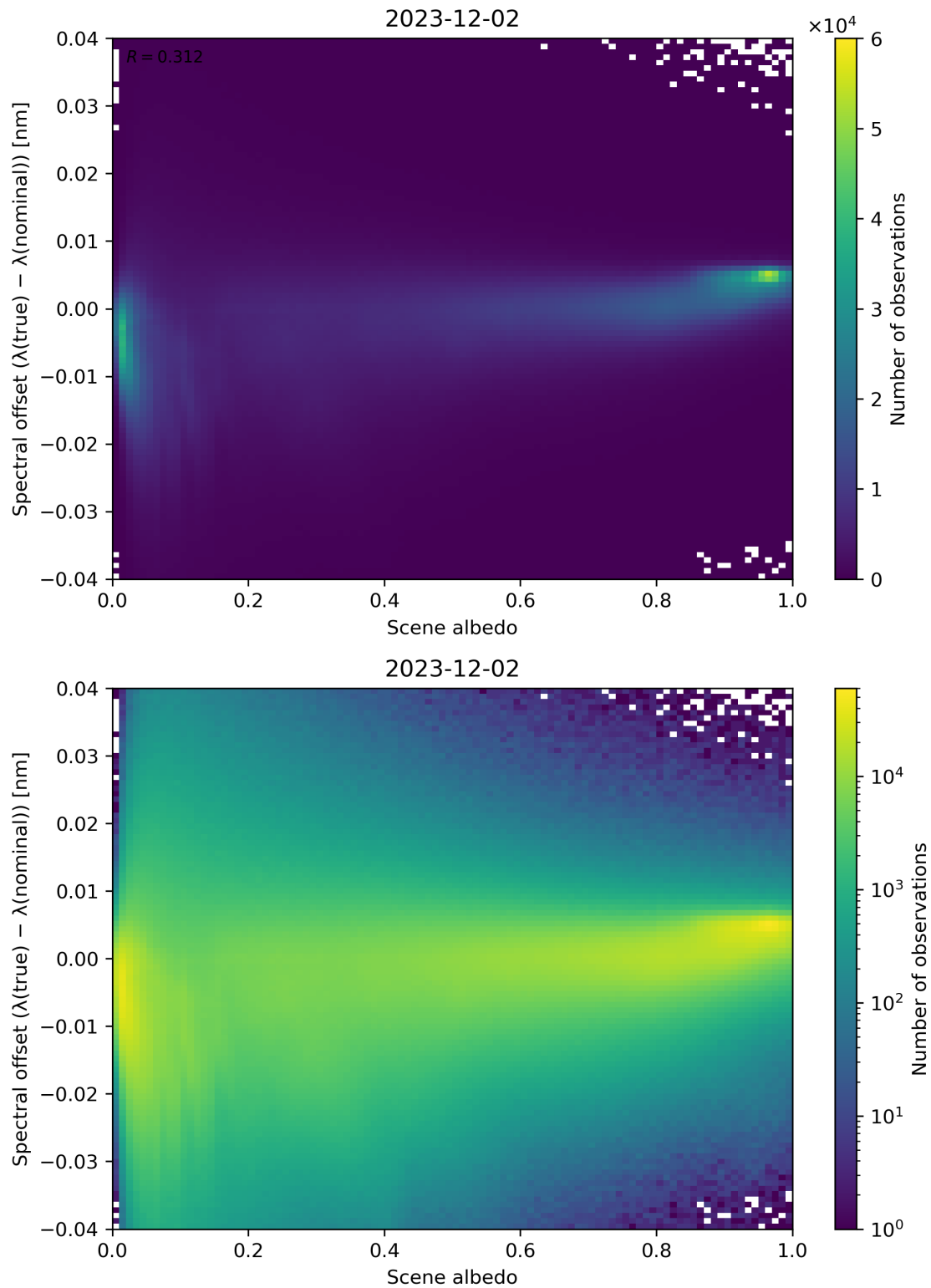
Figure 107: Scatter density plot of “Scene albedo” against “Spectral offset ( \lambda(\text{true}) - \lambda(\text{nominal}) )” for 2023-12-01 to 2023-12-03.
