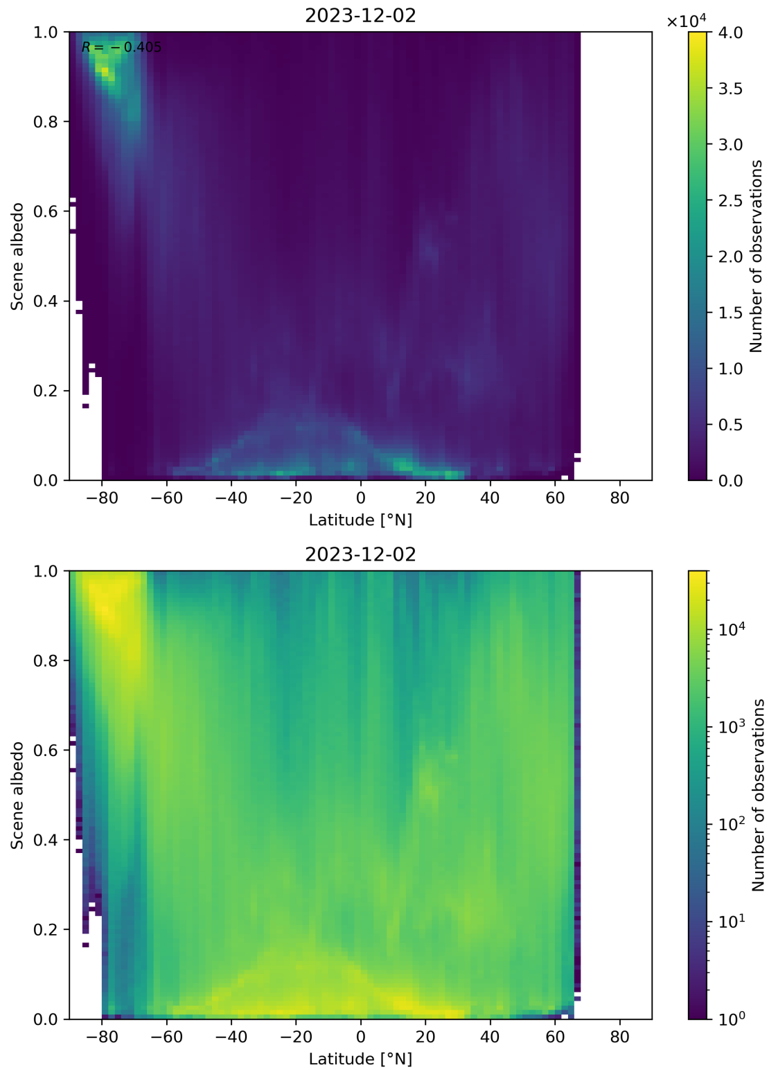
Figure 95: Scatter density plot of “Latitude” against “Scene albedo” for 2023-12-01 to 2023-12-03.
