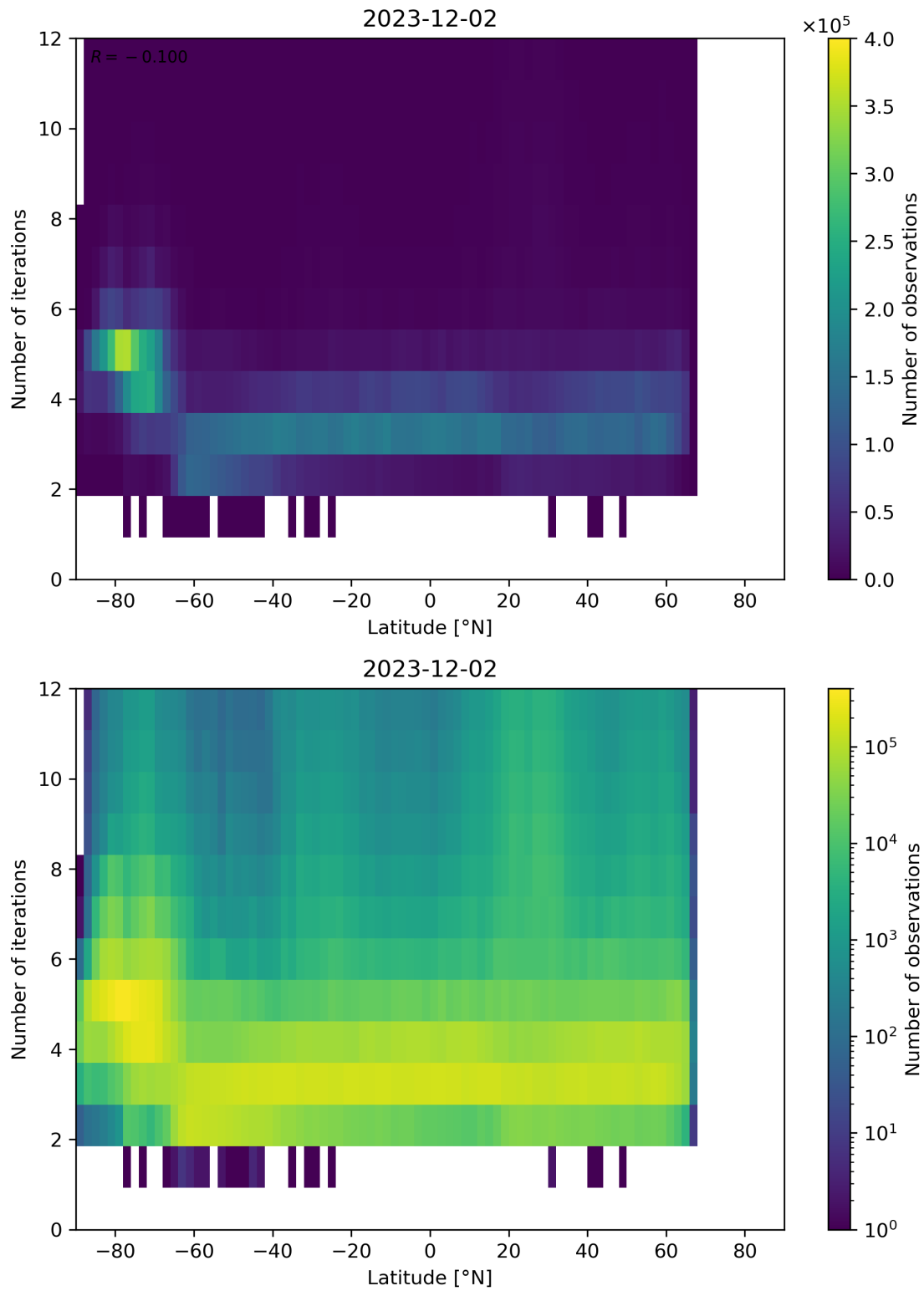
Figure 93: Scatter density plot of “Latitude” against “Number of iterations” for 2023-12-01 to 2023-12-03.
