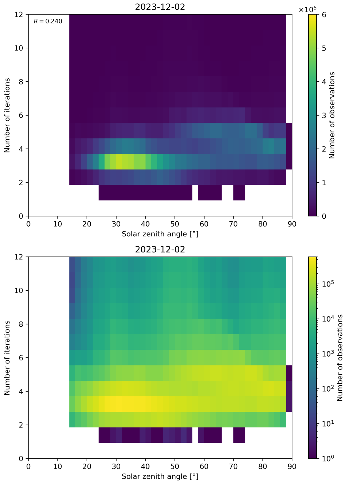
Figure 114: Scatter density plot of “Solar zenith angle” against “Number of iterations” for 2023-12-01 to 2023-12-03.
