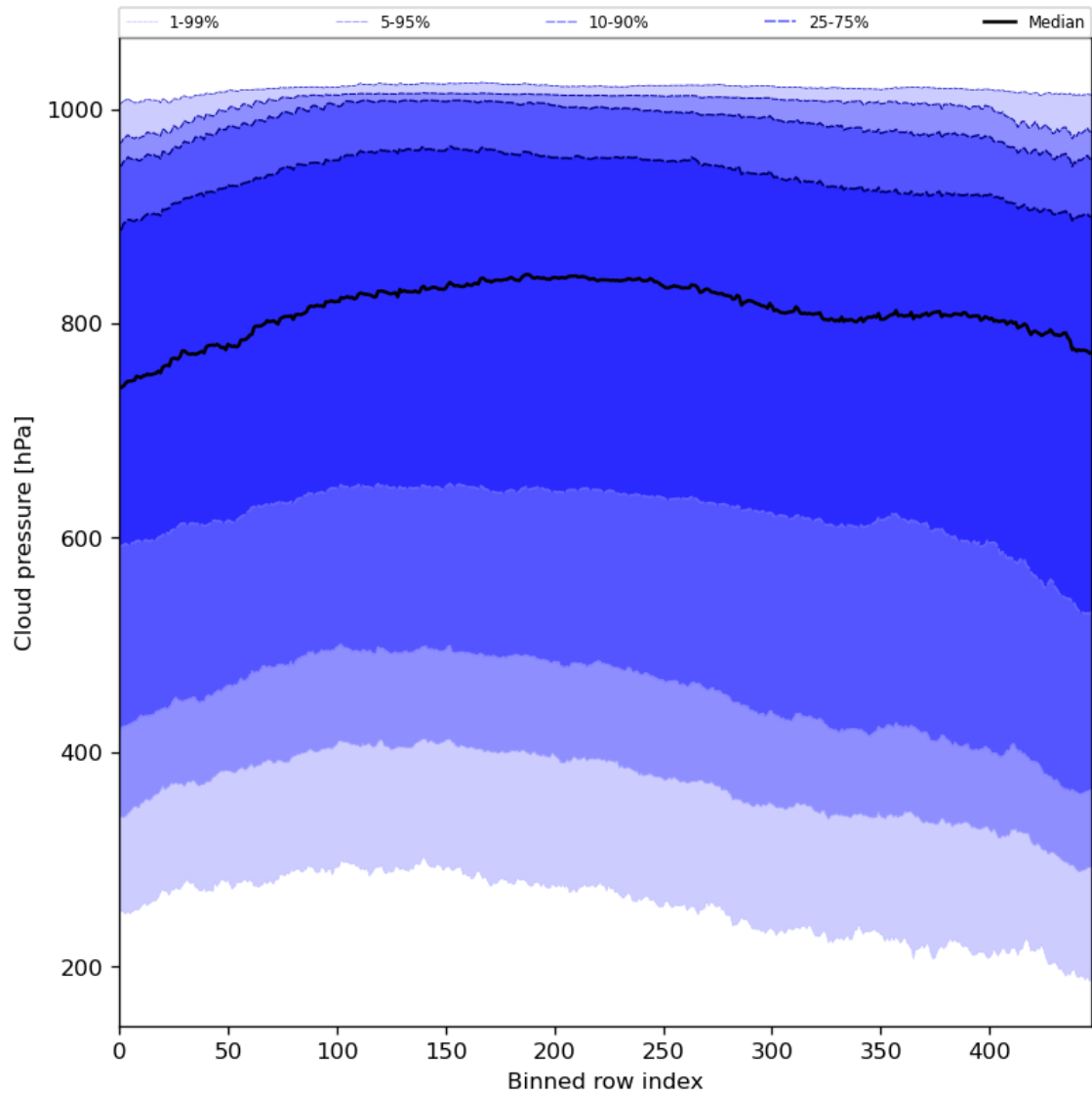
Figure 47: Along track statistics of “Cloud pressure” for 2023-12-01 to 2023-12-03
