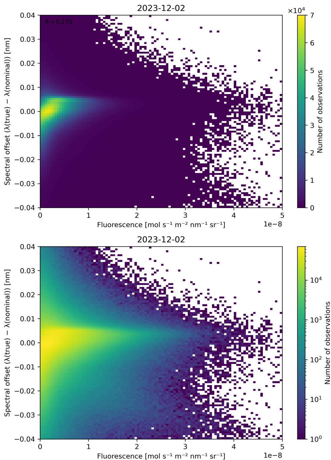
Figure 87: Scatter density plot of “Fluorescence” against “Spectral offset ( \lambda(\text{true}) - \lambda(\text{nominal}) )” for 2023-12-01 to 2023-12-03.
