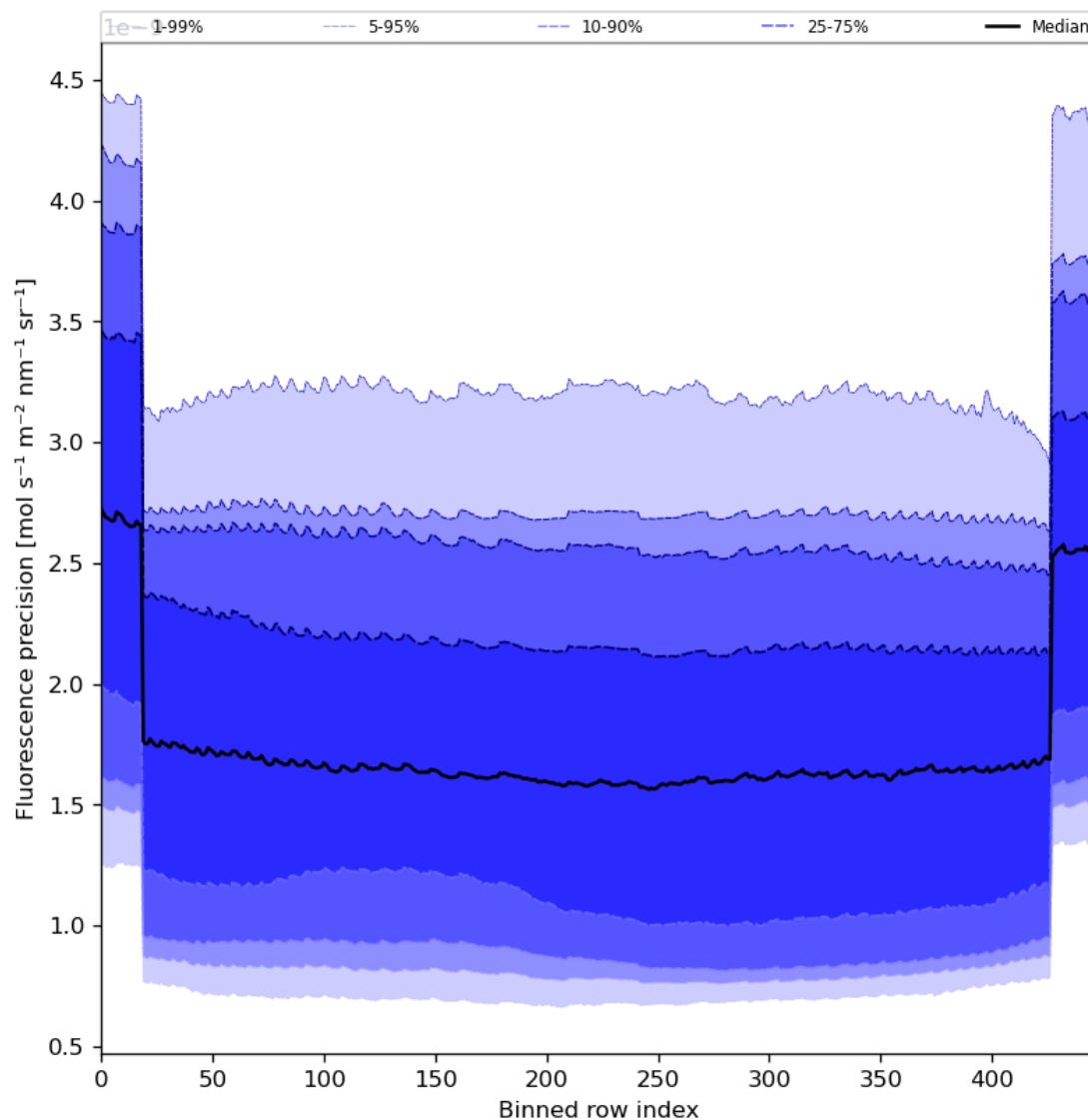
Figure 58: Along track statistics of “Fluorescence precision” for 2023-12-01 to 2023-12-03
