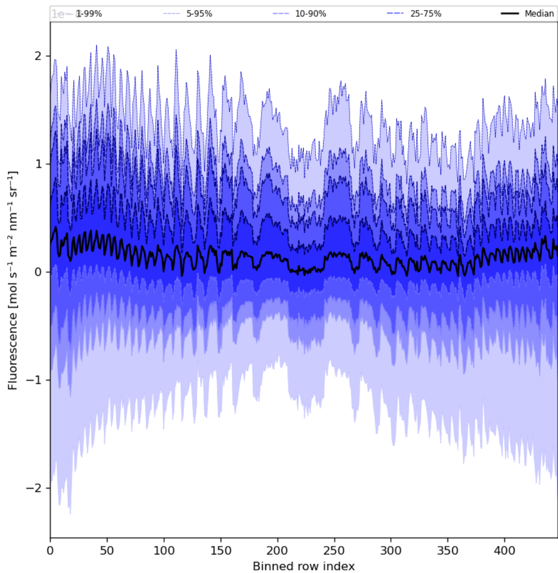
Figure 57: Along track statistics of “Fluorescence” for 2023-12-01 to 2023-12-03
