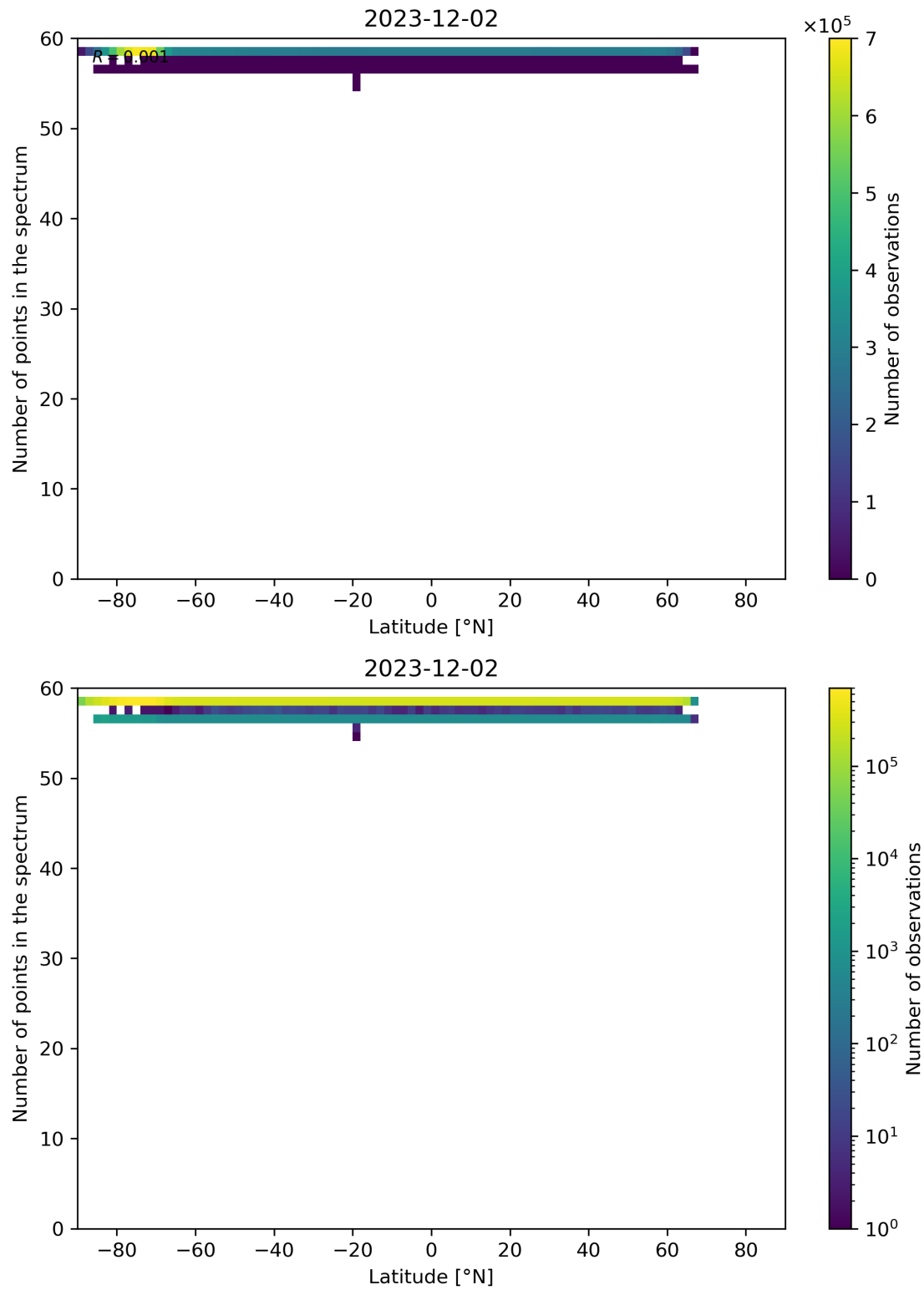
Figure 94: Scatter density plot of “Latitude” against “Number of points in the spectrum” for 2023-12-01 to 2023-12-03.
