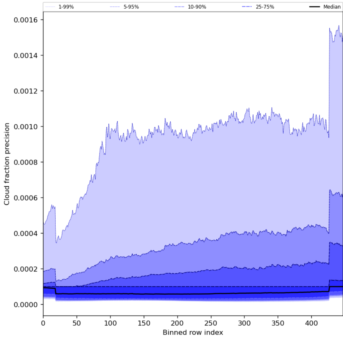
Figure 50: Along track statistics of “Cloud fraction precision” for 2023-12-01 to 2023-12-03
