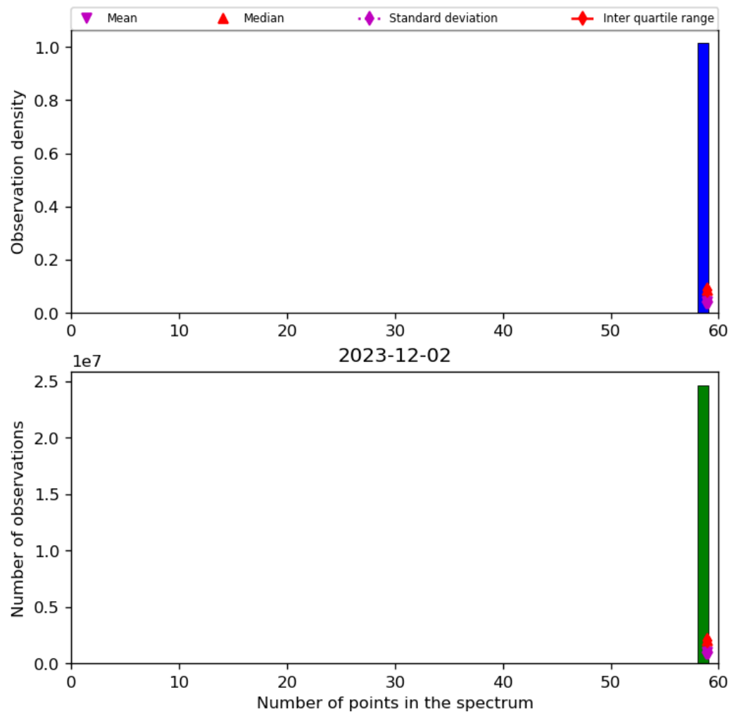
Figure 44: Histogram of “Number of points in the spectrum” for 2023-12-01 to 2023-12-03
