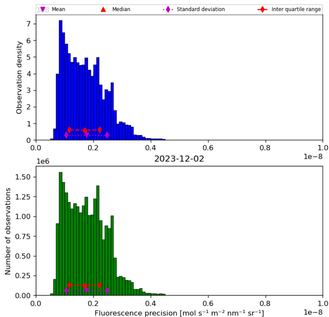
Figure 41: Histogram of “Fluorescence precision” for 2023-12-01 to 2023-12-03
