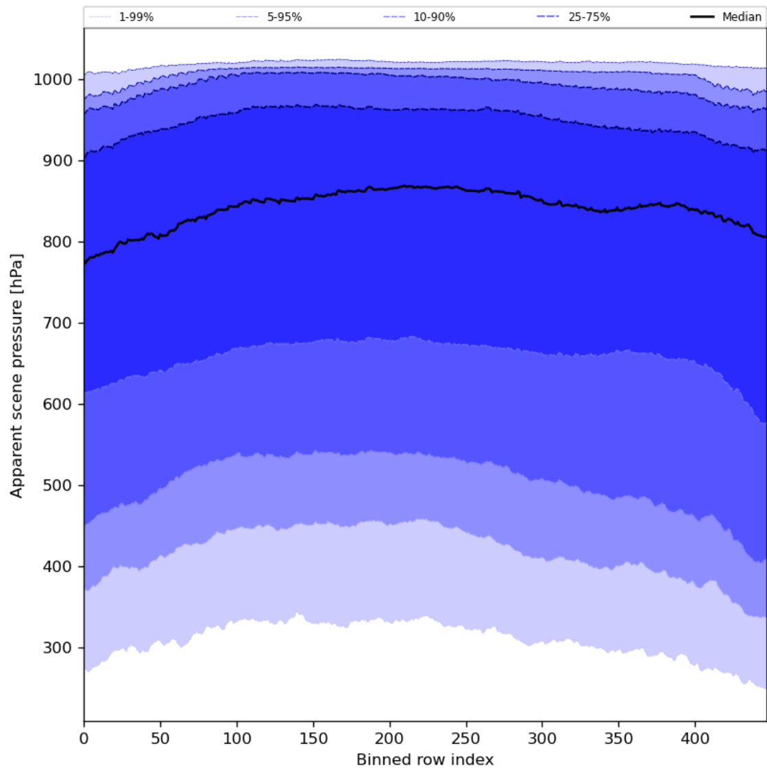
Figure 53: Along track statistics of “Apparent scene pressure” for 2023-12-01 to 2023-12-03
