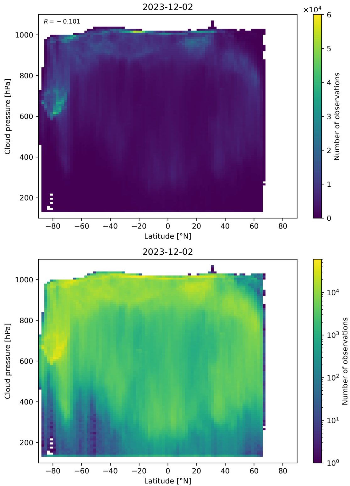
Figure 91: Scatter density plot of “Latitude” against “Cloud pressure” for 2023-12-01 to 2023-12-03.
