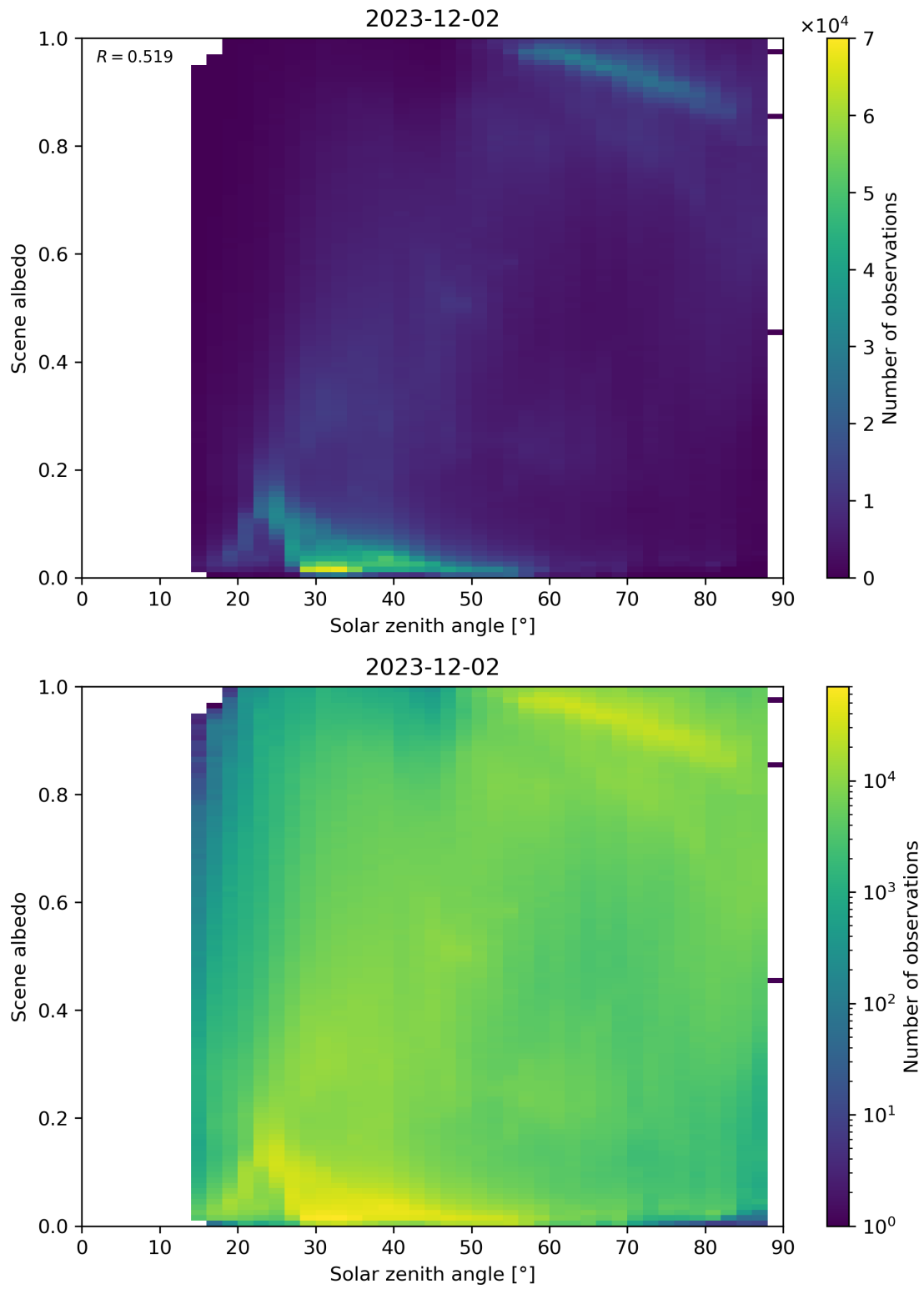
Figure 116: Scatter density plot of “Solar zenith angle” against “Scene albedo” for 2023-12-01 to 2023-12-03.
