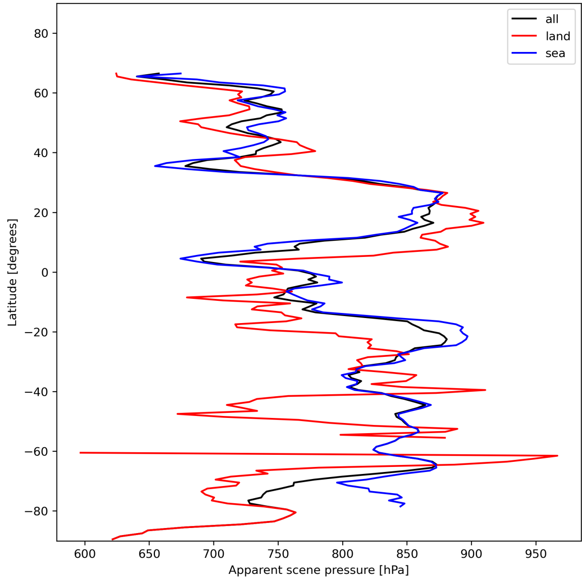
Figure 19: Zonal average of “Apparent scene pressure” for 2023-12-01 to 2023-12-03.
