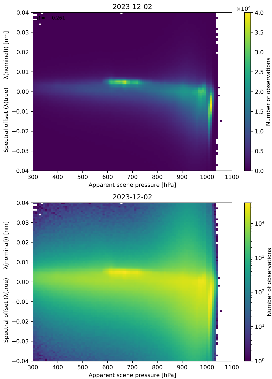
Figure 67: Scatter density plot of “Apparent scene pressure” against “Spectral offset ( \lambda(\text{true}) - \lambda(\text{nominal}) )” for 2023-12-01 to 2023-12-03.
