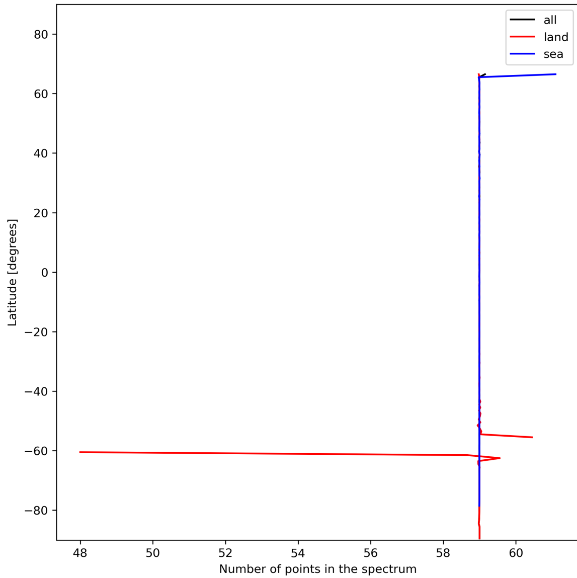
Figure 27: Zonal average of “Number of points in the spectrum” for 2023-12-01 to 2023-12-03.
