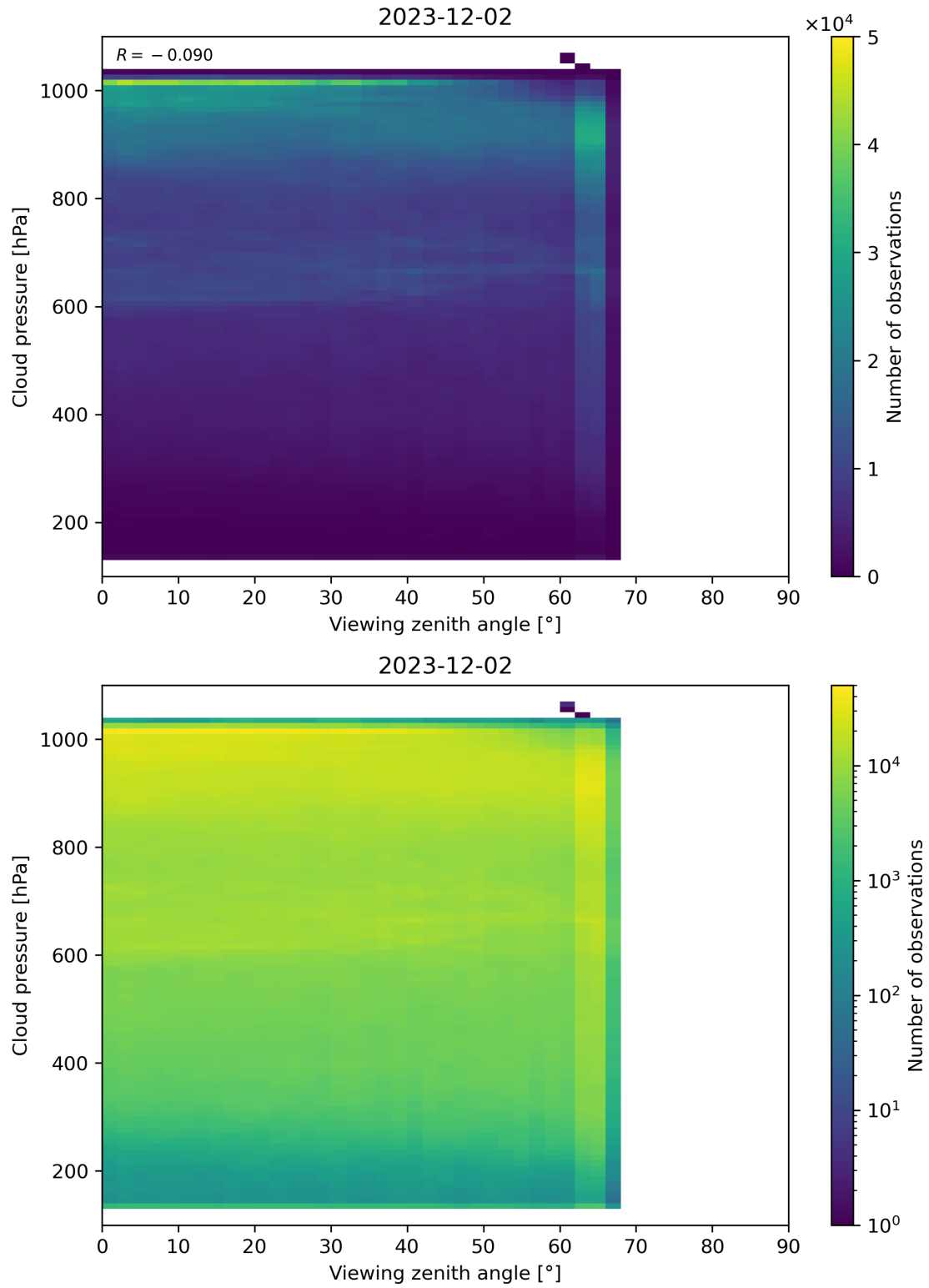
Figure 121: Scatter density plot of “Viewing zenith angle” against “Cloud pressure” for 2023-12-01 to 2023-12-03.
