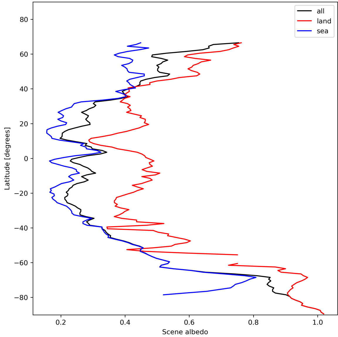
Figure 17: Zonal average of “Scene albedo” for 2023-12-01 to 2023-12-03.
