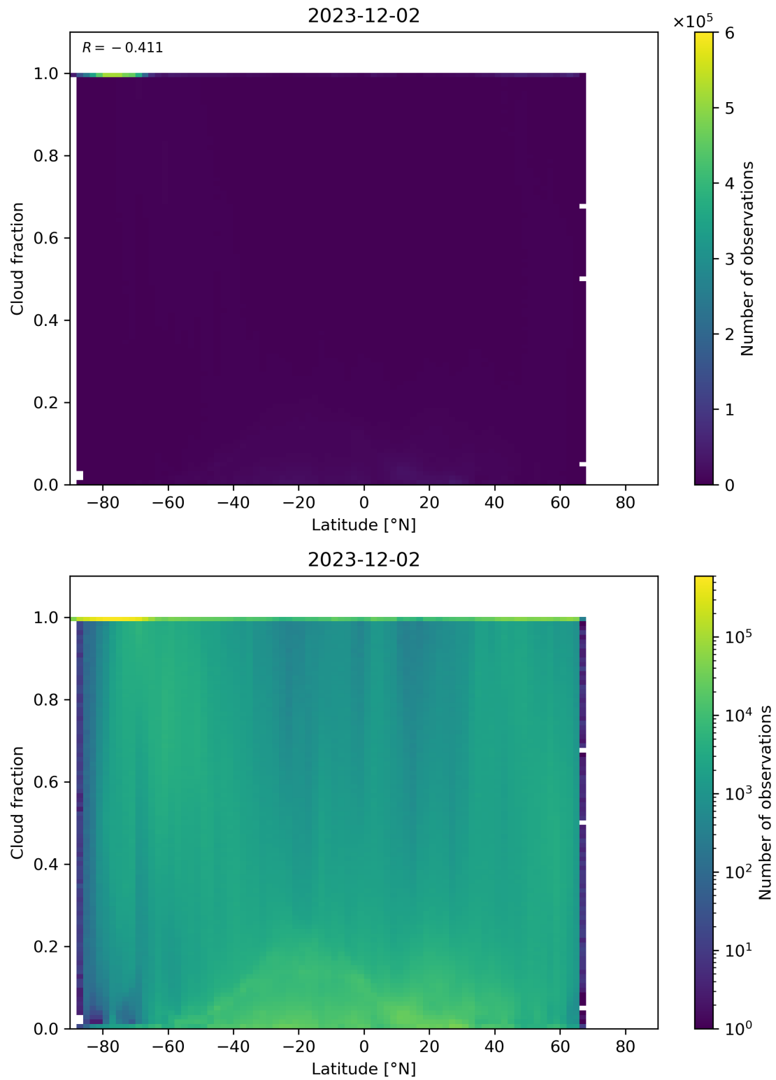
Figure 90: Scatter density plot of “Latitude” against “Cloud fraction” for 2023-12-01 to 2023-12-03.
