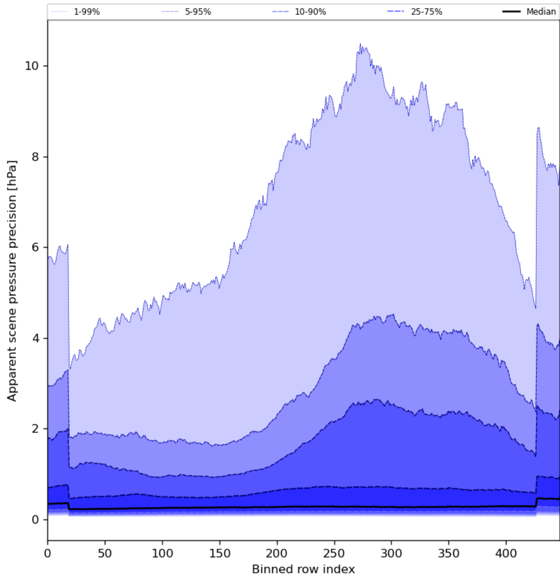
Figure 54: Along track statistics of “Apparent scene pressure precision” for 2023-12-01 to 2023-12-03
