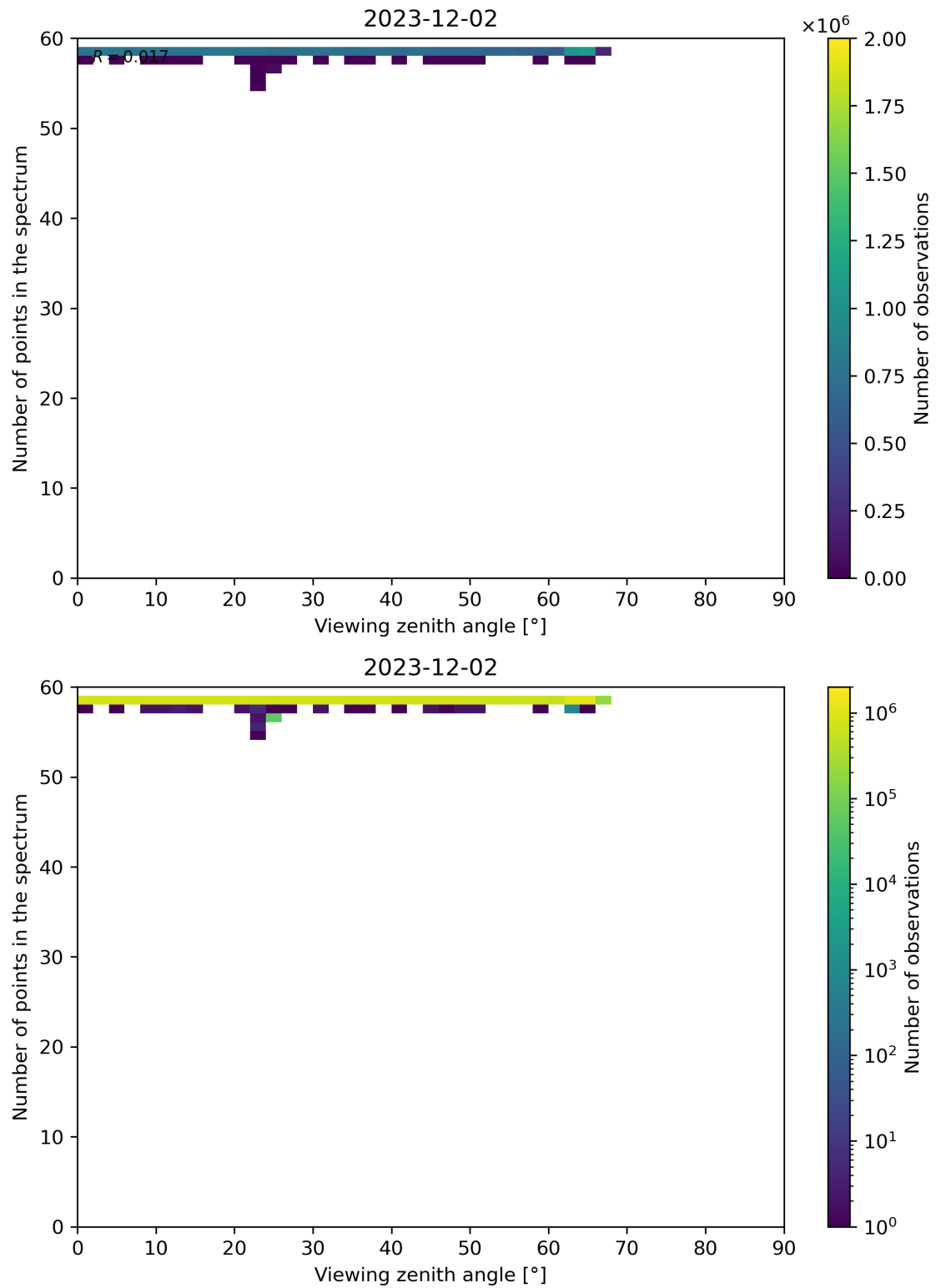
Figure 125: Scatter density plot of “Viewing zenith angle” against “Number of points in the spectrum” for 2023-12-01 to 2023-12-03.
