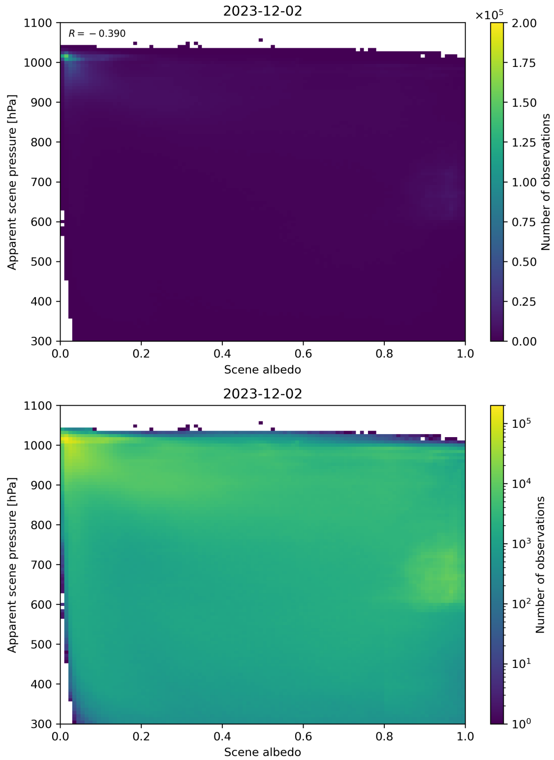
Figure 102: Scatter density plot of “Scene albedo” against “Apparent scene pressure” for 2023-12-01 to 2023-12-03.
