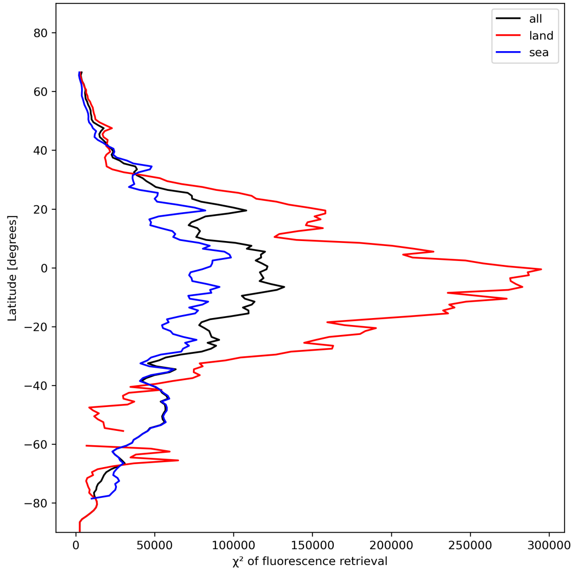
Figure 25: Zonal average of “ \chi^2 of fluorescence retrieval” for 2023-12-01 to 2023-12-03.
