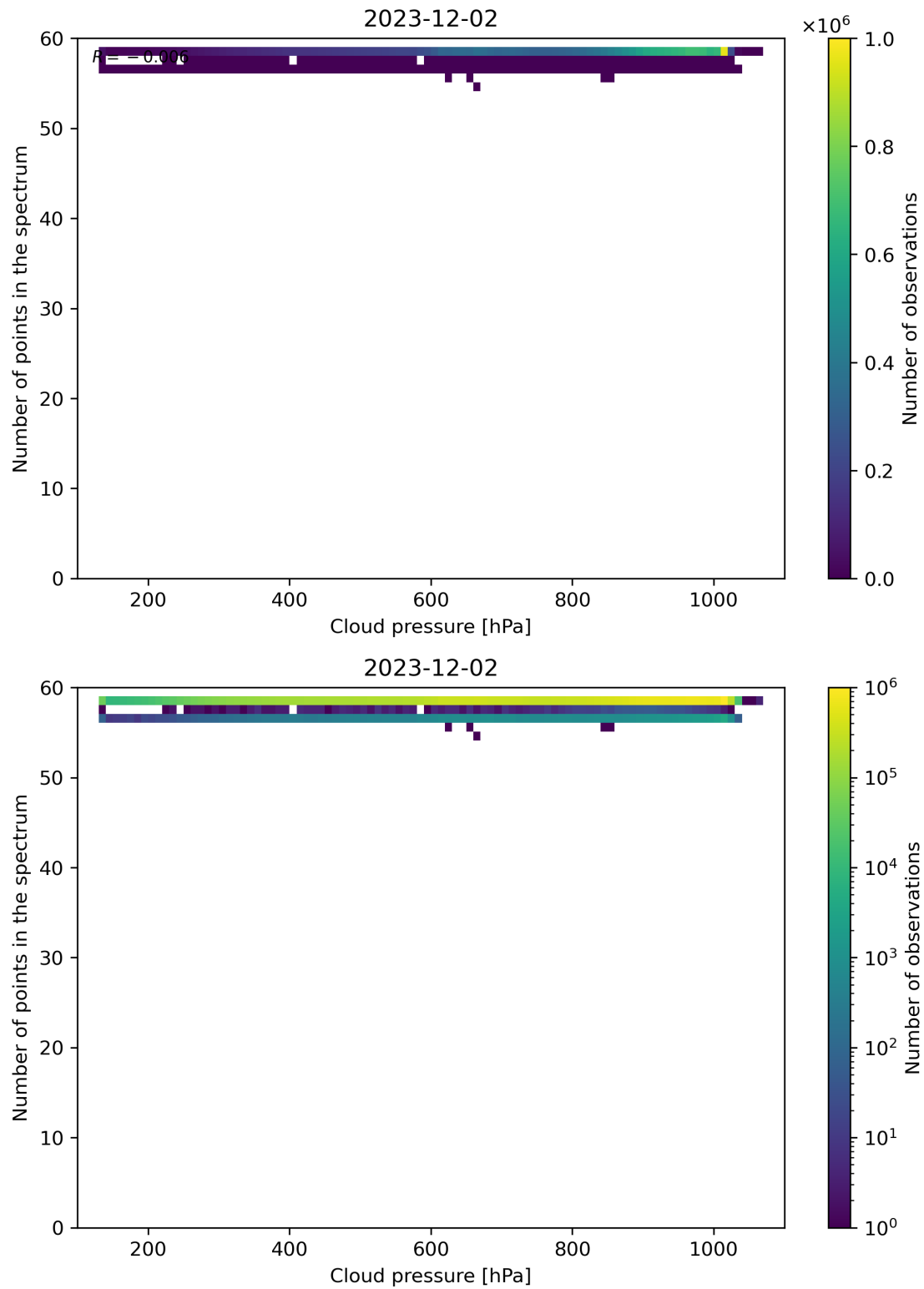
Figure 82: Scatter density plot of “Cloud pressure” against “Number of points in the spectrum” for 2023-12-01 to 2023-12-03.
