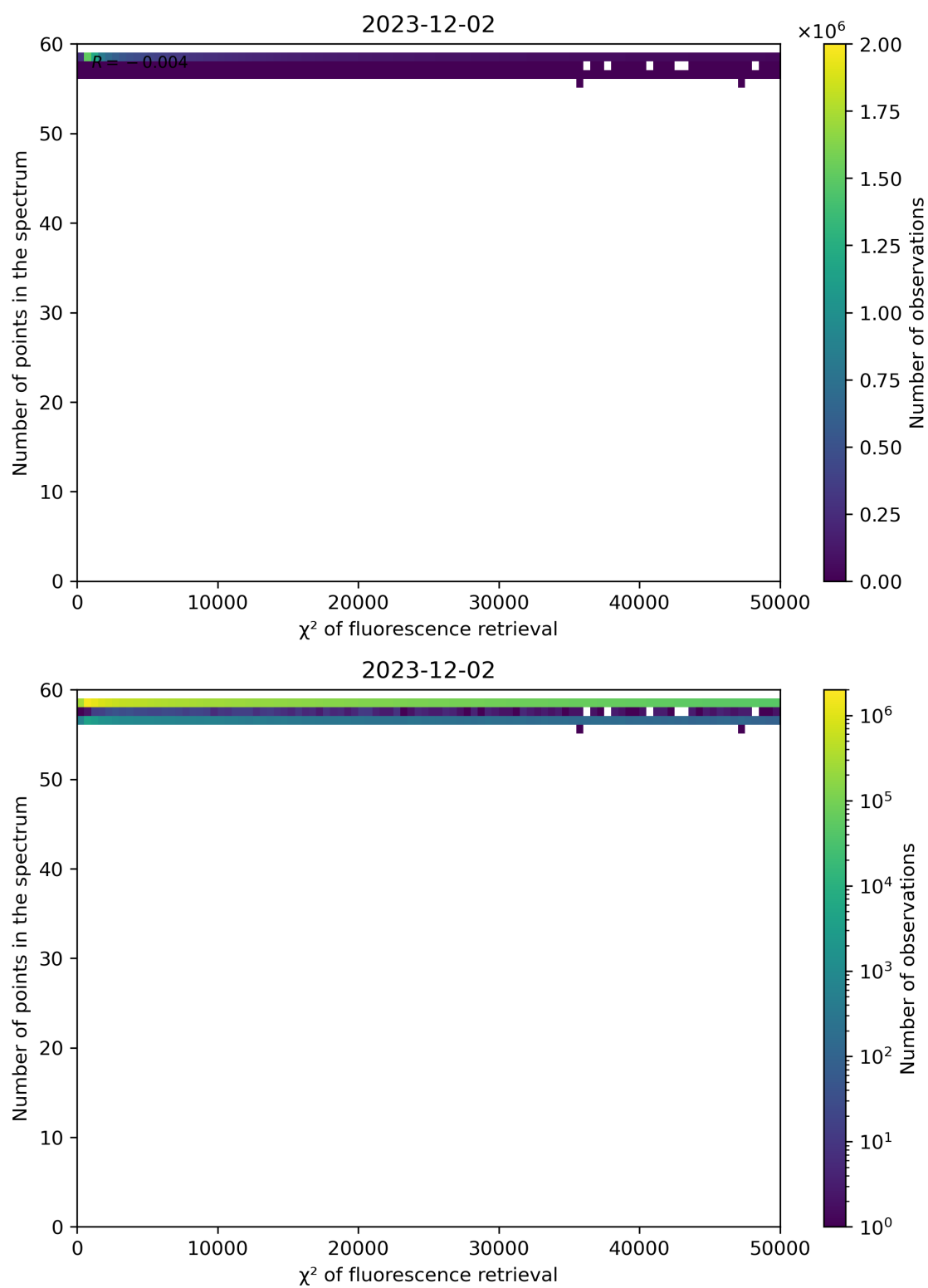
Figure 68: Scatter density plot of “ \chi^2 of fluorescence retrieval” against “Number of points in the spectrum” for 2023-12-01 to 2023-12-03.
