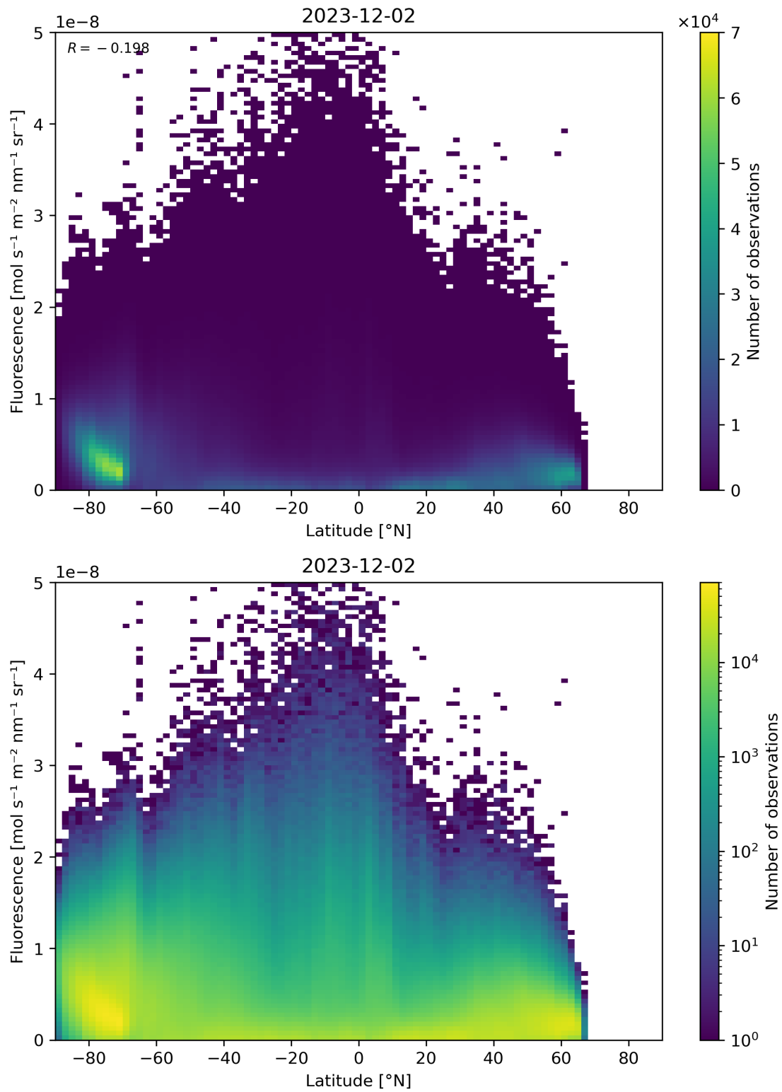
Figure 92: Scatter density plot of “Latitude” against “Fluorescence” for 2023-12-01 to 2023-12-03.
