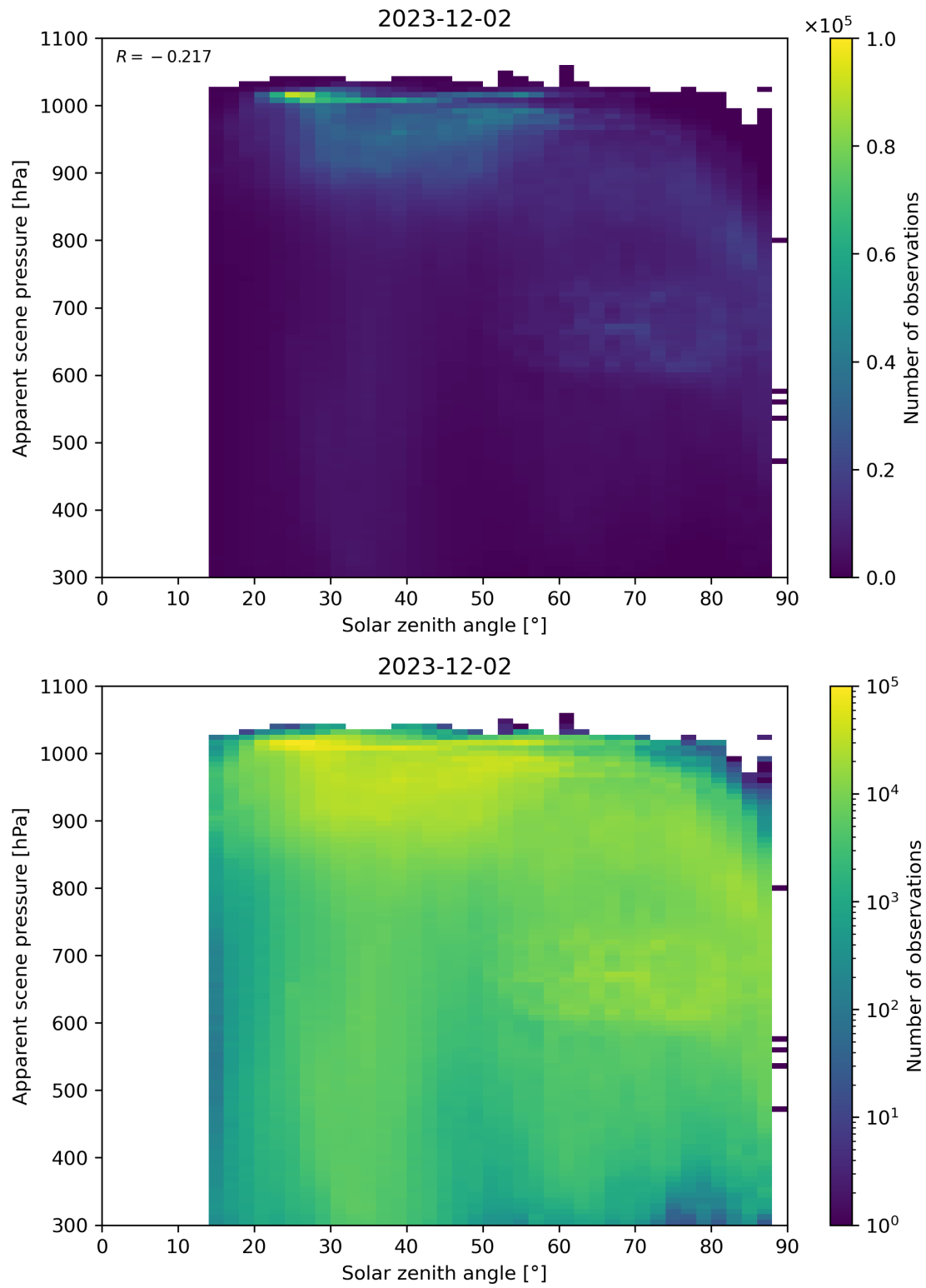
Figure 108: Scatter density plot of “Solar zenith angle” against “Apparent scene pressure” for 2023-12-01 to 2023-12-03.
