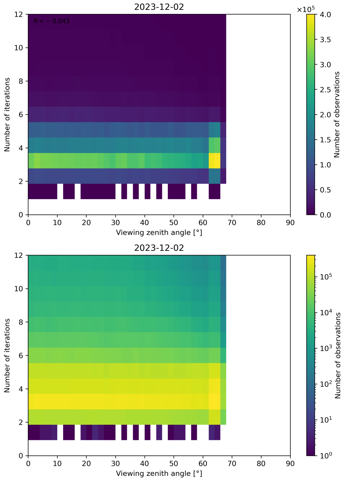
Figure 124: Scatter density plot of “Viewing zenith angle” against “Number of iterations” for 2023-12-01 to 2023-12-03.
