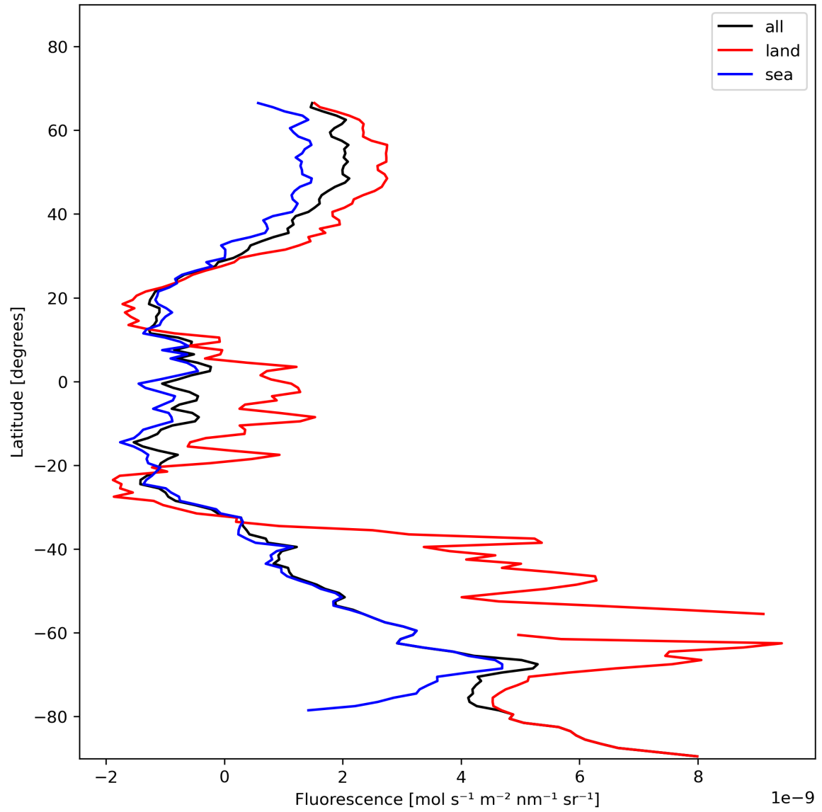
Figure 23: Zonal average of “Fluorescence” for 2023-12-01 to 2023-12-03.
