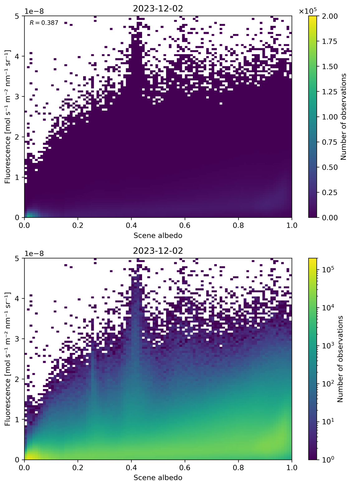
Figure 104: Scatter density plot of “Scene albedo” against “Fluorescence” for 2023-12-01 to 2023-12-03.
