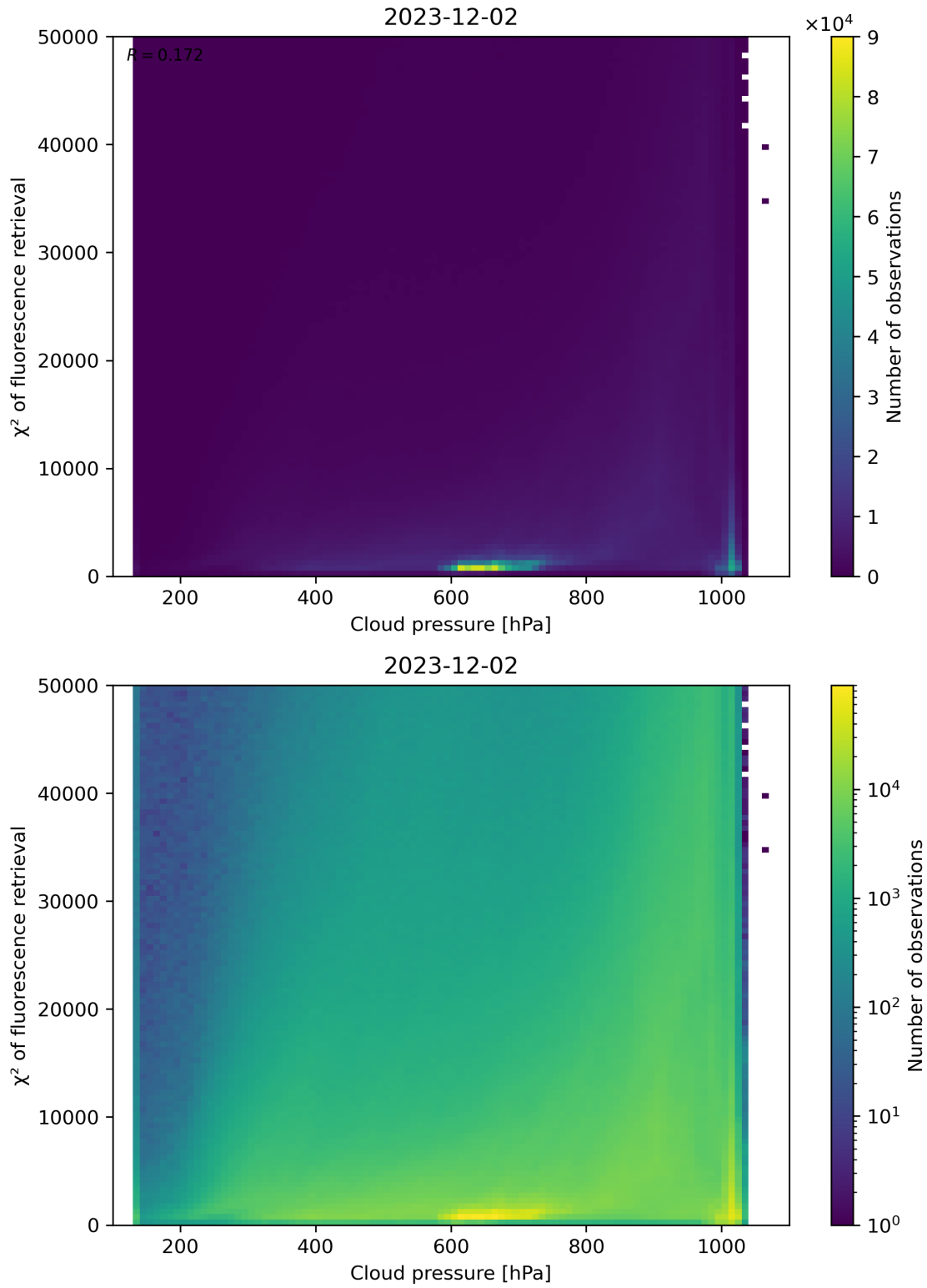
Figure 78: Scatter density plot of “Cloud pressure” against “ \chi^2 of fluorescence retrieval” for 2023-12-01 to 2023-12-03.
