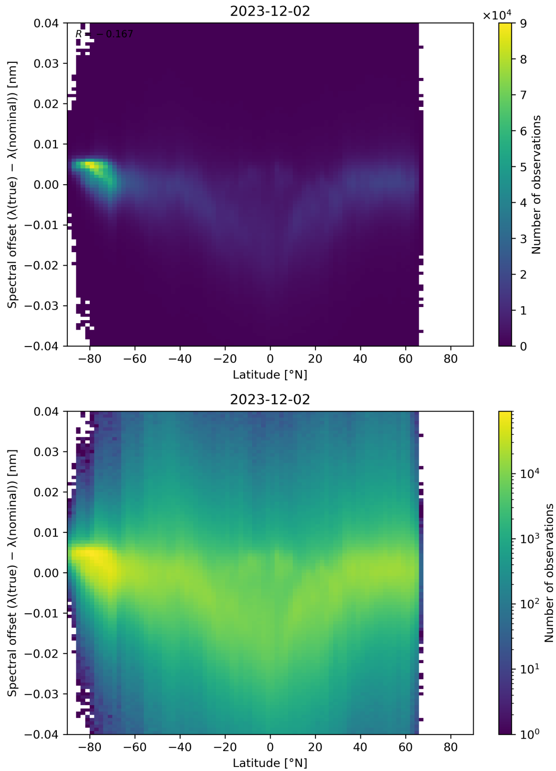
Figure 96: Scatter density plot of “Latitude” against “Spectral offset ( \lambda(\text{true}) - \lambda(\text{nominal}) )” for 2023-12-01 to 2023-12-03.
