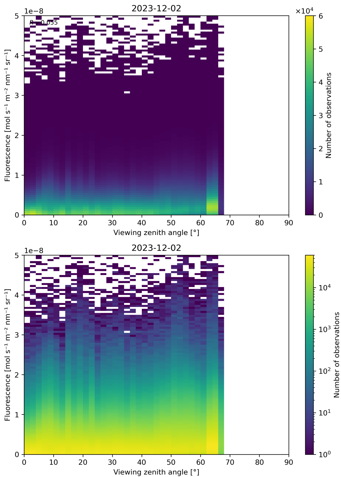
Figure 122: Scatter density plot of “Viewing zenith angle” against “Fluorescence” for 2023-12-01 to 2023-12-03.
