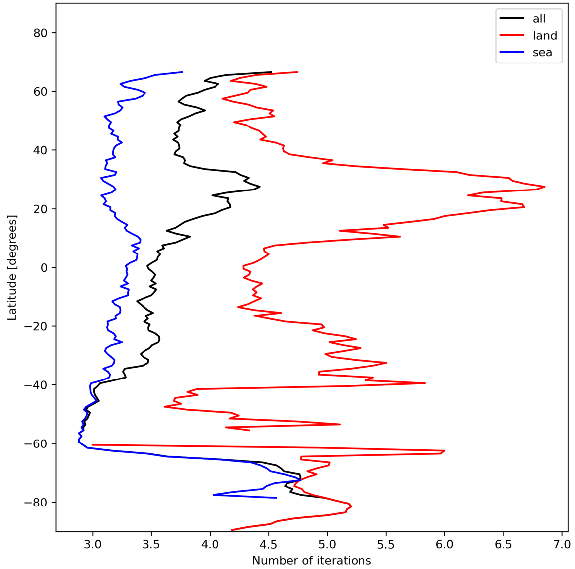
Figure 22: Zonal average of “Number of iterations” for 2023-12-01 to 2023-12-03.
