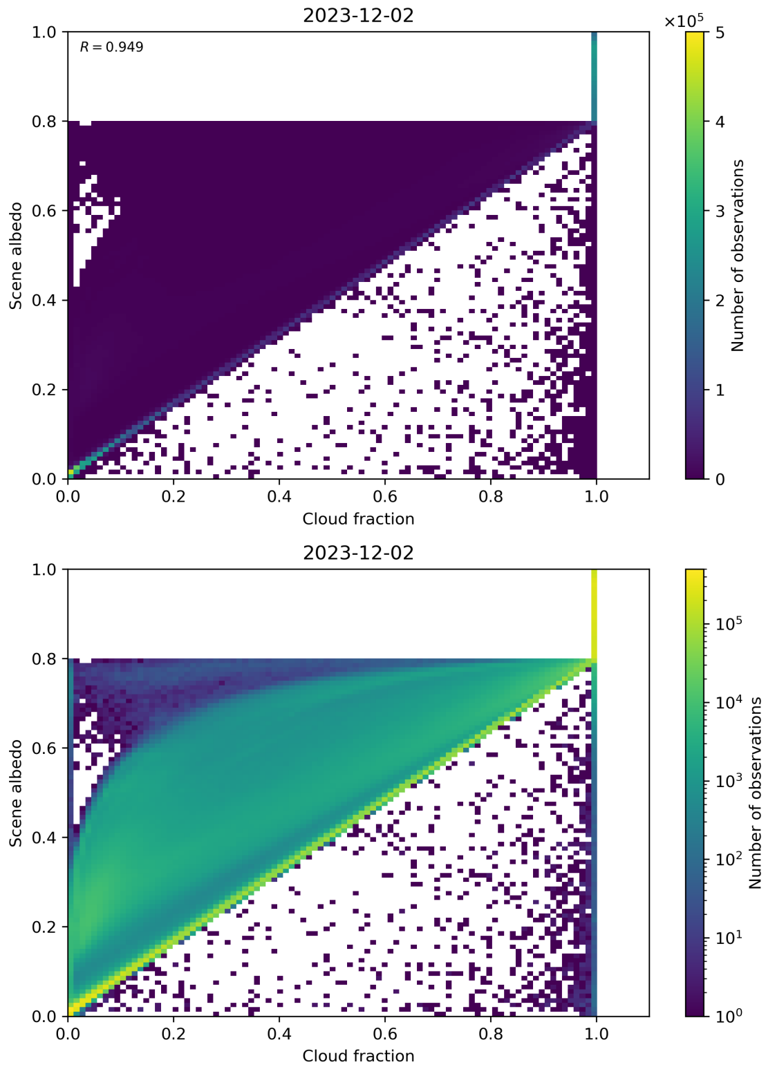
Figure 75: Scatter density plot of “Cloud fraction” against “Scene albedo” for 2023-12-01 to 2023-12-03.
