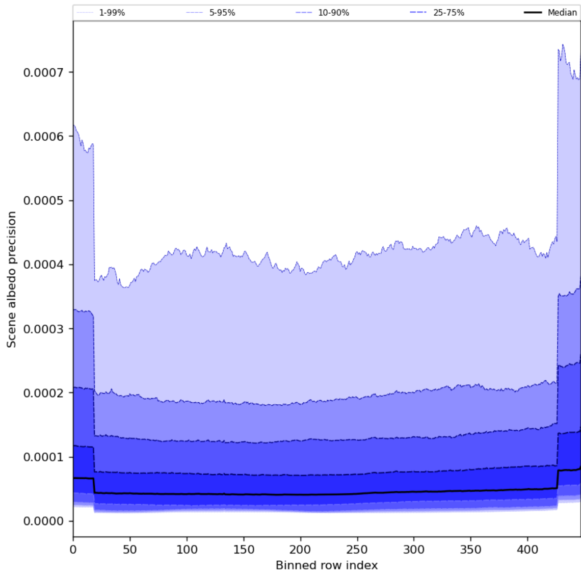
Figure 52: Along track statistics of “Scene albedo precision” for 2023-12-01 to 2023-12-03
