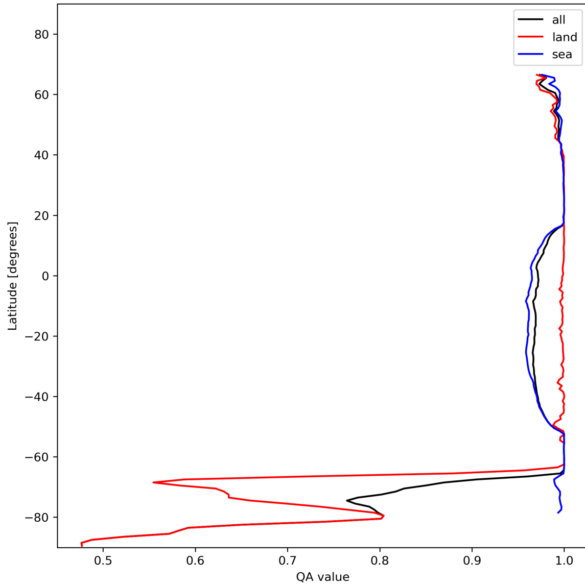
Figure 12: Zonal average of “QA value” for 2023-12-01 to 2023-12-03.
