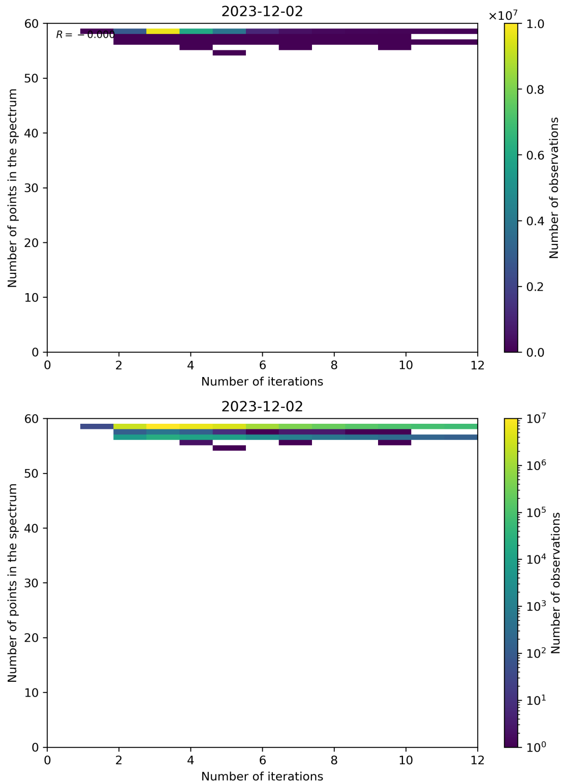
Figure 99: Scatter density plot of “Number of iterations” against “Number of points in the spectrum” for 2023-12-01 to 2023-12-03.
