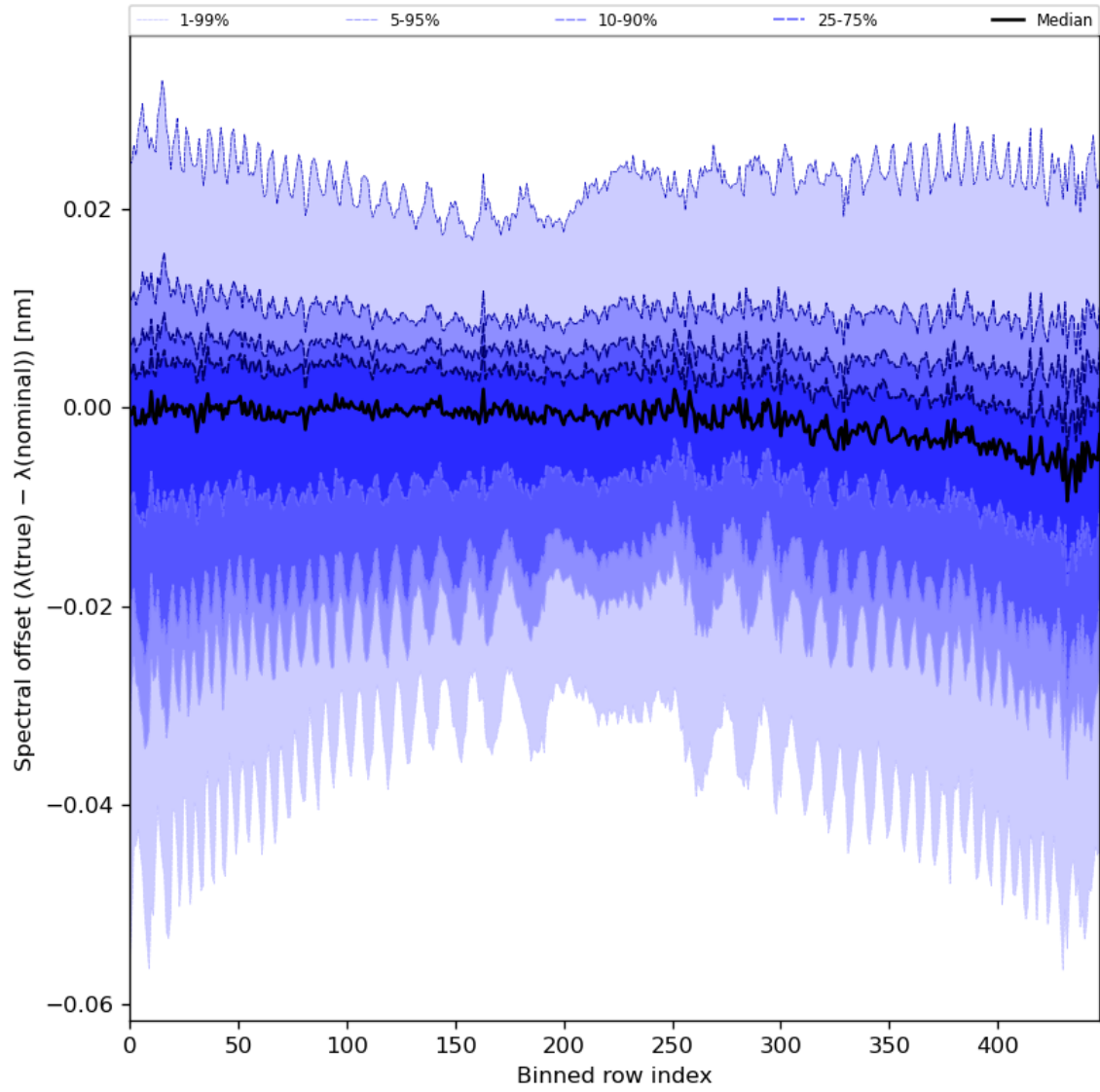
Figure 62: Along track statistics of “Spectral offset ( \lambda(\text{true}) - \lambda(\text{nominal}) )” for 2023-12-01 to 2023-12-03
