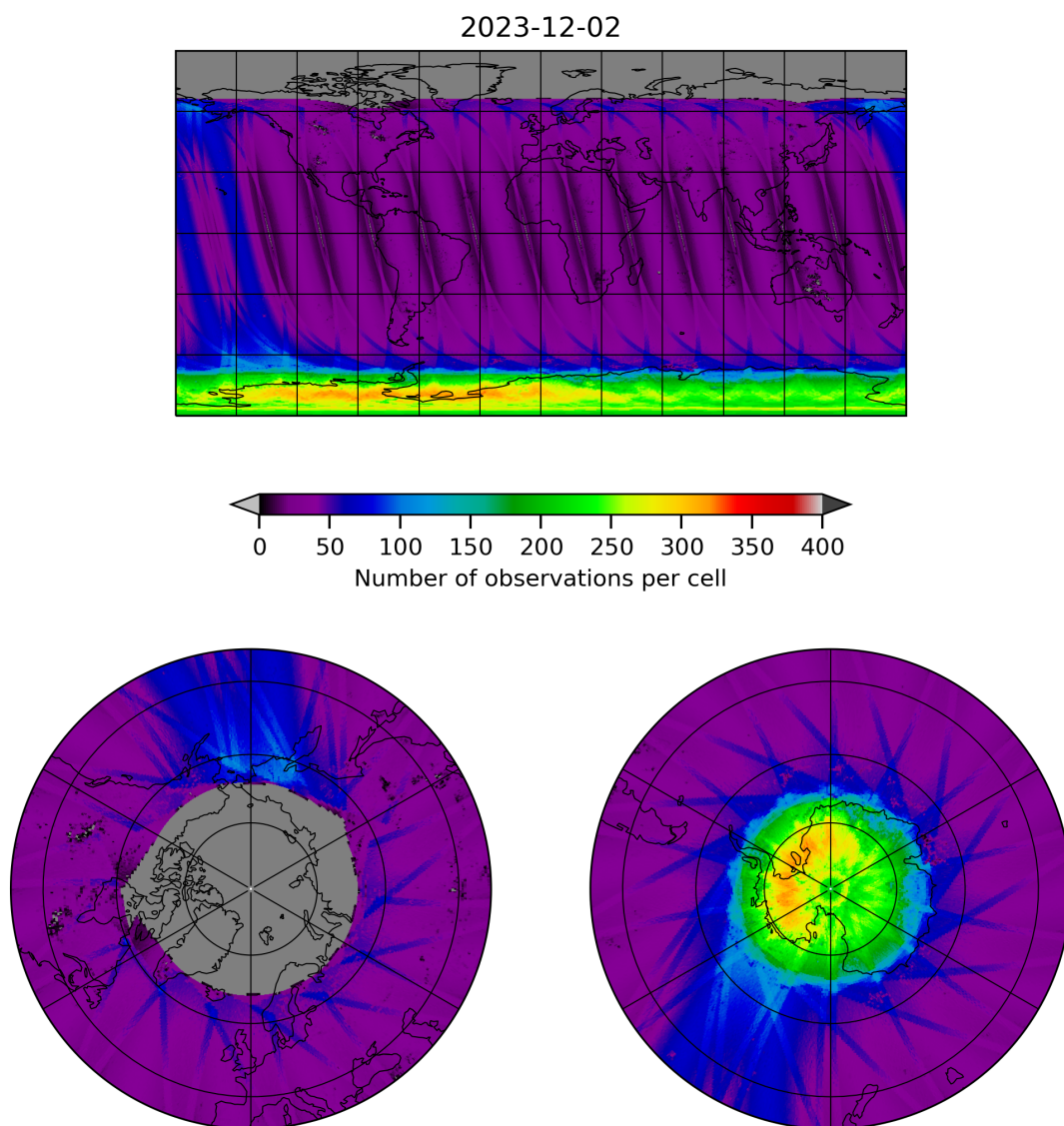
Figure 11: Map of the number of observations for 2023-12-01 to 2023-12-03
