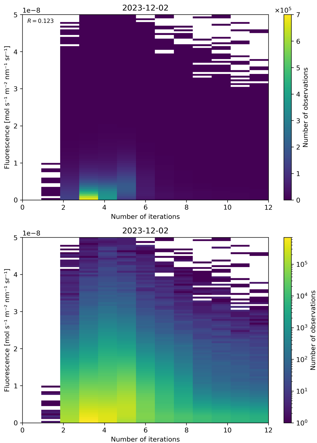
Figure 98: Scatter density plot of “Number of iterations” against “Fluorescence” for 2023-12-01 to 2023-12-03.
