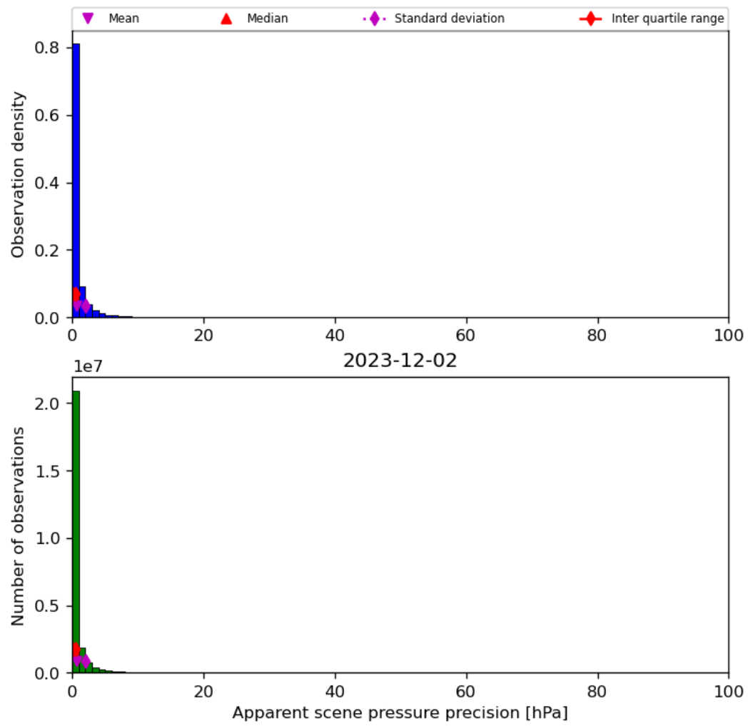
Figure 37: Histogram of “Apparent scene pressure precision” for 2023-12-01 to 2023-12-03
