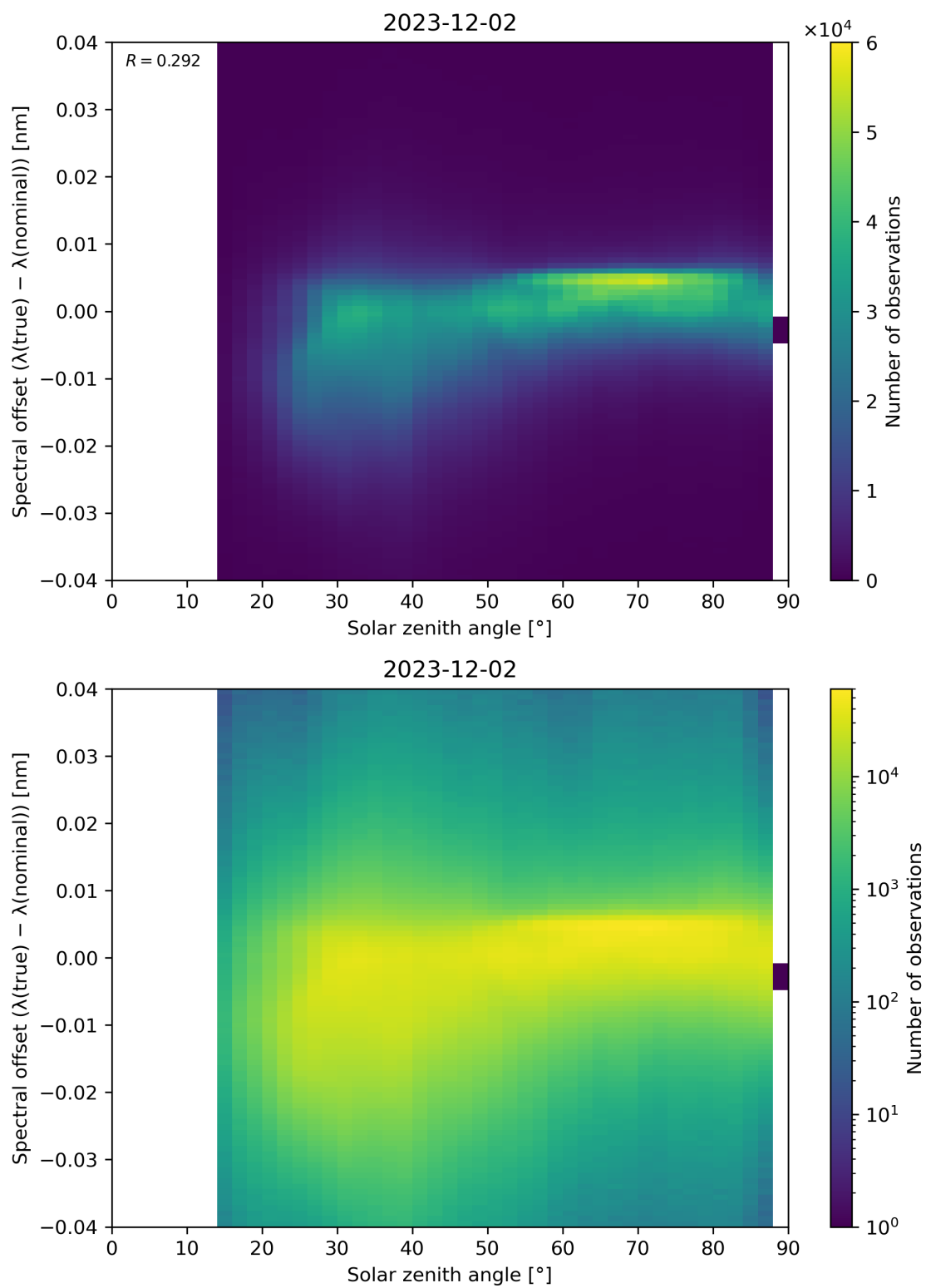
Figure 117: Scatter density plot of “Solar zenith angle” against “Spectral offset ( \lambda(\text{true}) - \lambda(\text{nominal}) )” for 2023-12-01 to 2023-12-03.
