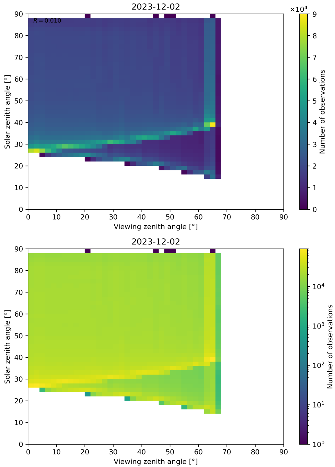
Figure 127: Scatter density plot of “Viewing zenith angle” against “Solar zenith angle” for 2023-12-01 to 2023-12-03.
