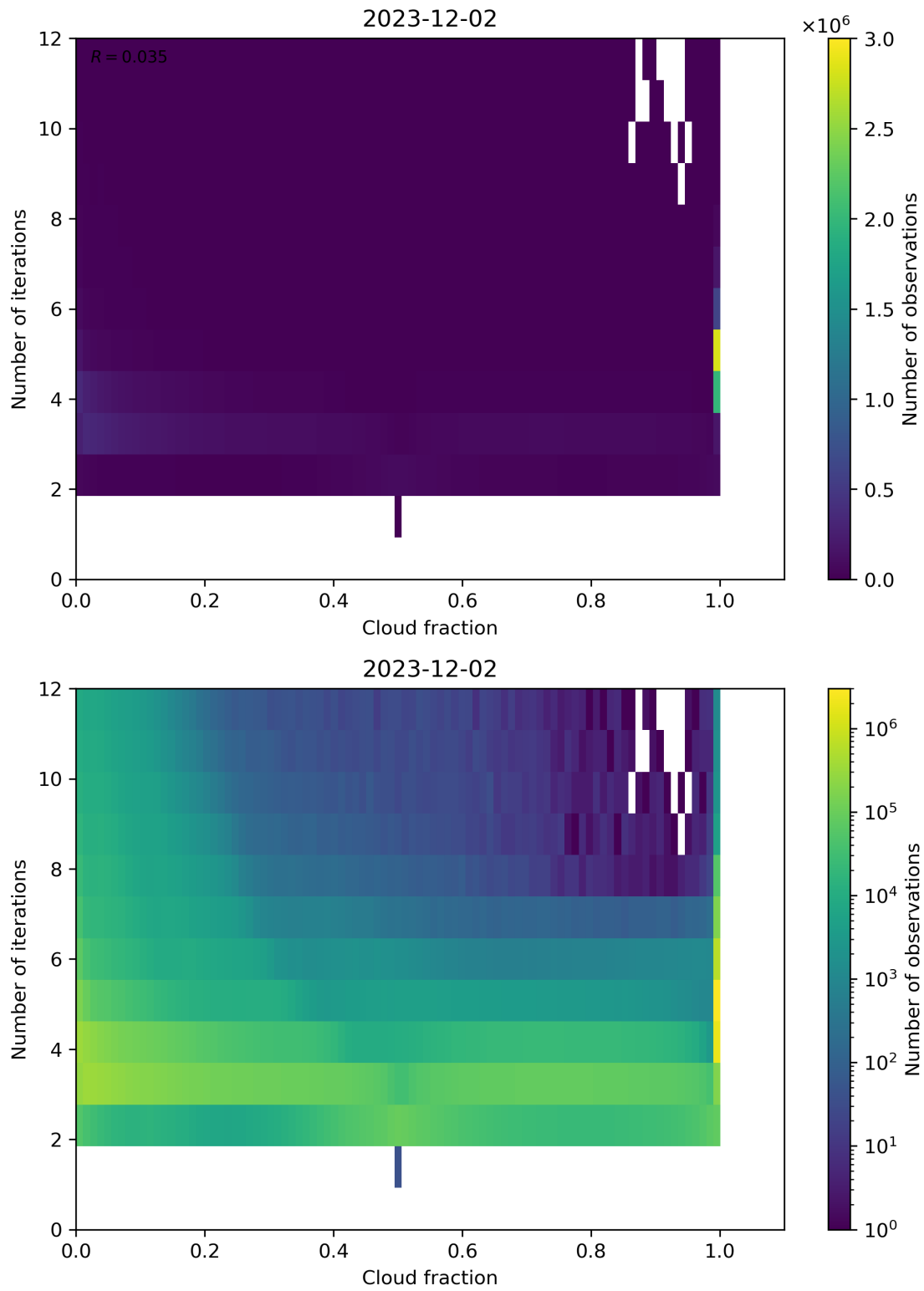
Figure 73: Scatter density plot of “Cloud fraction” against “Number of iterations” for 2023-12-01 to 2023-12-03.
