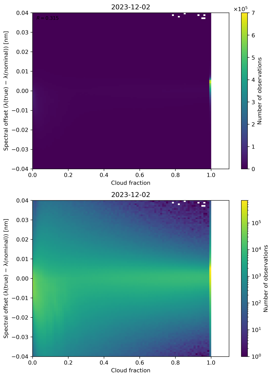
Figure 76: Scatter density plot of “Cloud fraction” against “Spectral offset ( \lambda(\text{true}) - \lambda(\text{nominal}) )” for 2023-12-01 to 2023-12-03.
