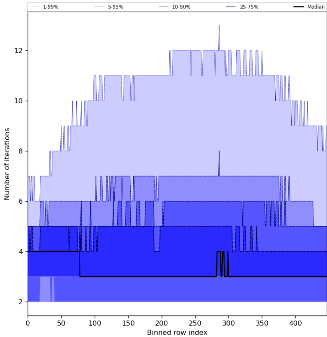
Figure 56: Along track statistics of “Number of iterations” for 2023-12-01 to 2023-12-03
