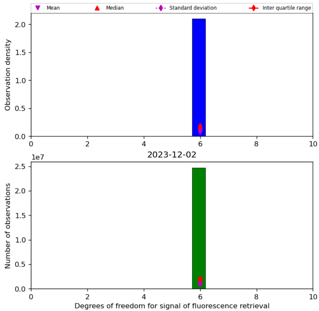
Figure 43: Histogram of “Degrees of freedom for signal of fluorescence retrieval” for 2023-12-01 to 2023-12-03
