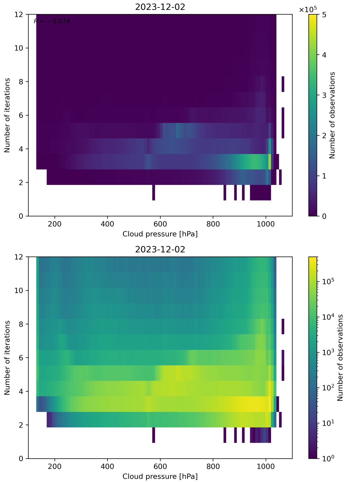
Figure 81: Scatter density plot of “Cloud pressure” against “Number of iterations” for 2023-12-01 to 2023-12-03.
