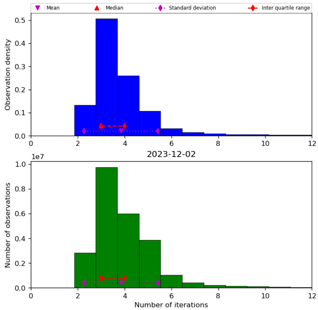
Figure 39: Histogram of “Number of iterations” for 2023-12-01 to 2023-12-03
