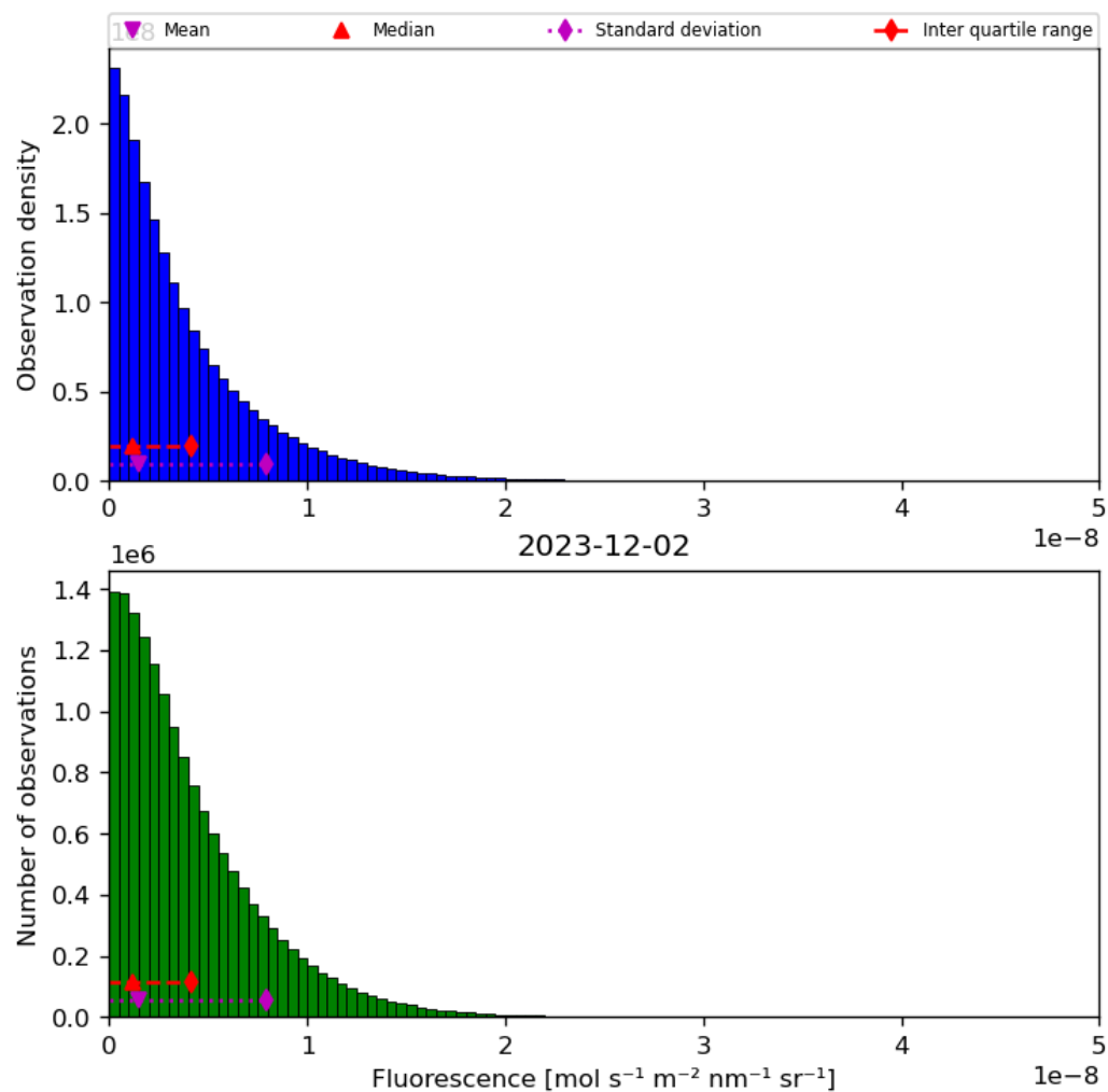
Figure 40: Histogram of “Fluorescence” for 2023-12-01 to 2023-12-03
