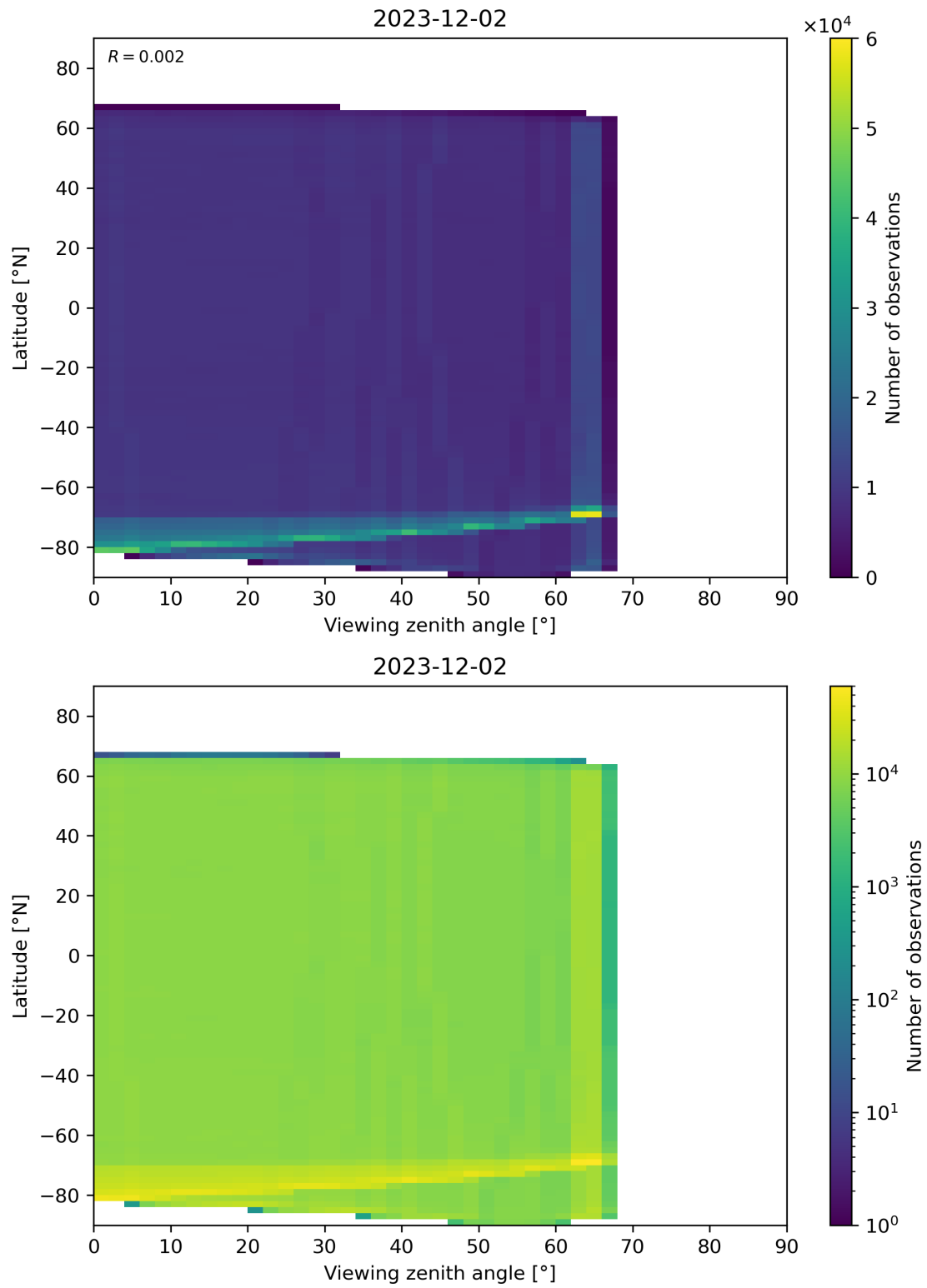
Figure 123: Scatter density plot of “Viewing zenith angle” against “Latitude” for 2023-12-01 to 2023-12-03.
