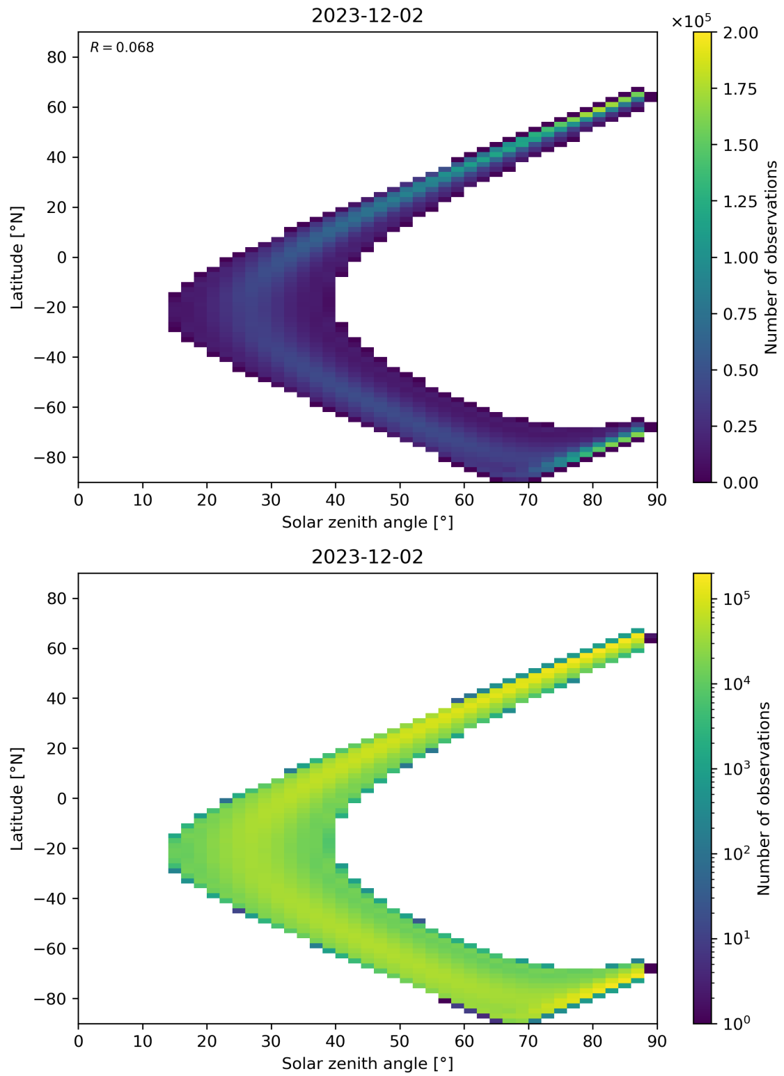
Figure 113: Scatter density plot of “Solar zenith angle” against “Latitude” for 2023-12-01 to 2023-12-03.
