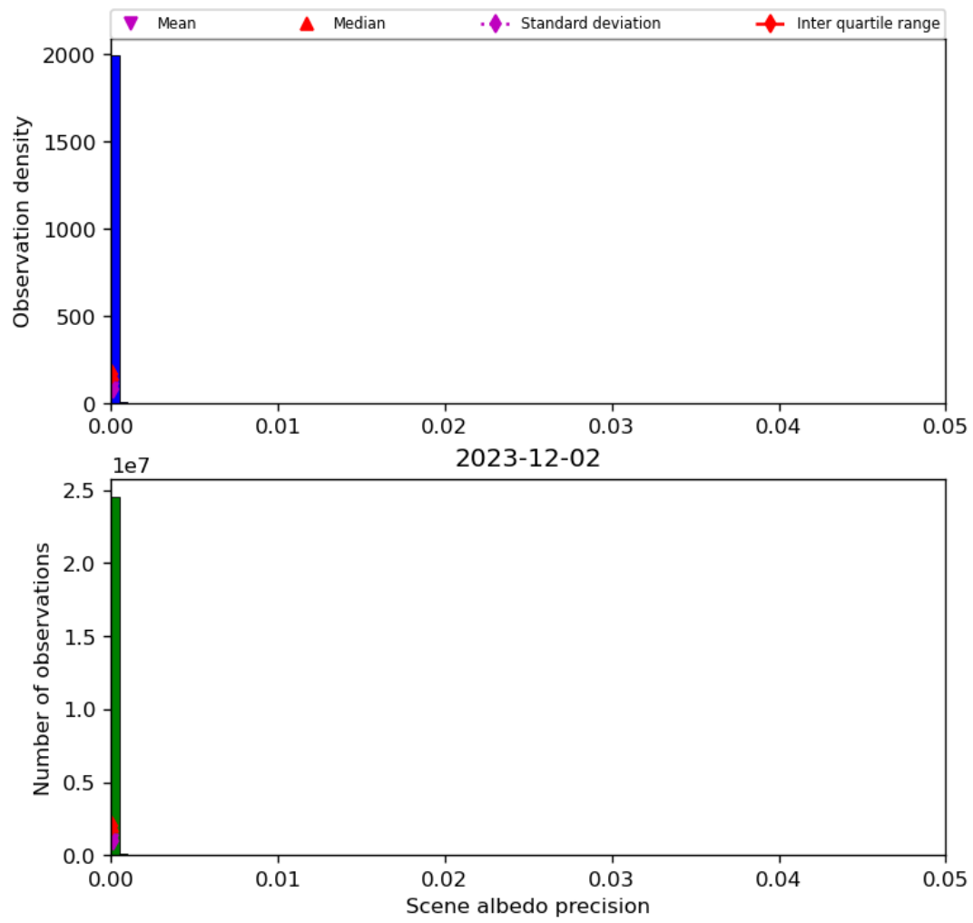
Figure 35: Histogram of “Scene albedo precision” for 2023-12-01 to 2023-12-03
