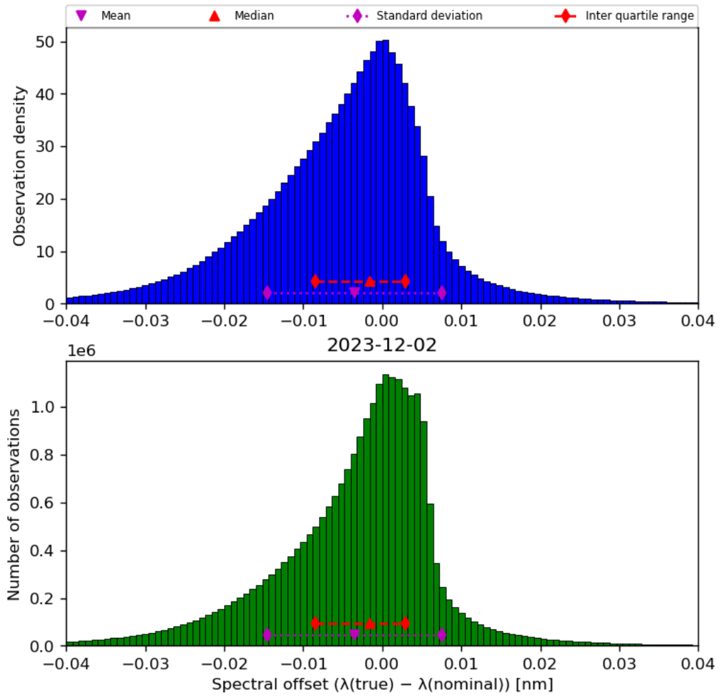
Figure 45: Histogram of “Spectral offset ( \lambda(\text{true}) - \lambda(\text{nominal}) )” for 2023-12-01 to 2023-12-03
