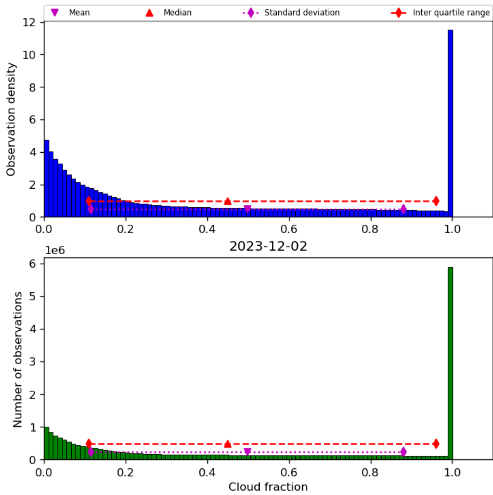
Figure 32: Histogram of “Cloud fraction” for 2023-12-01 to 2023-12-03
