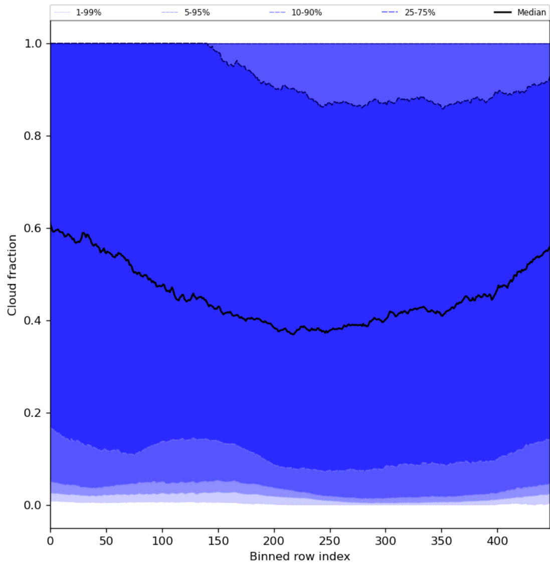
Figure 49: Along track statistics of “Cloud fraction” for 2023-12-01 to 2023-12-03
