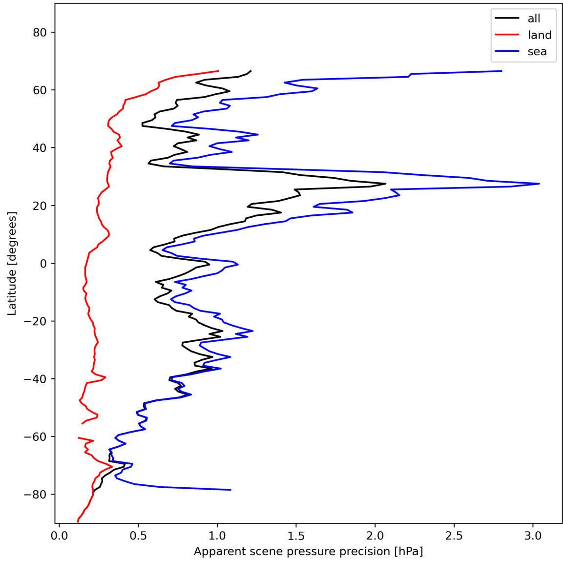
Figure 20: Zonal average of “Apparent scene pressure precision” for 2023-12-01 to 2023-12-03.
