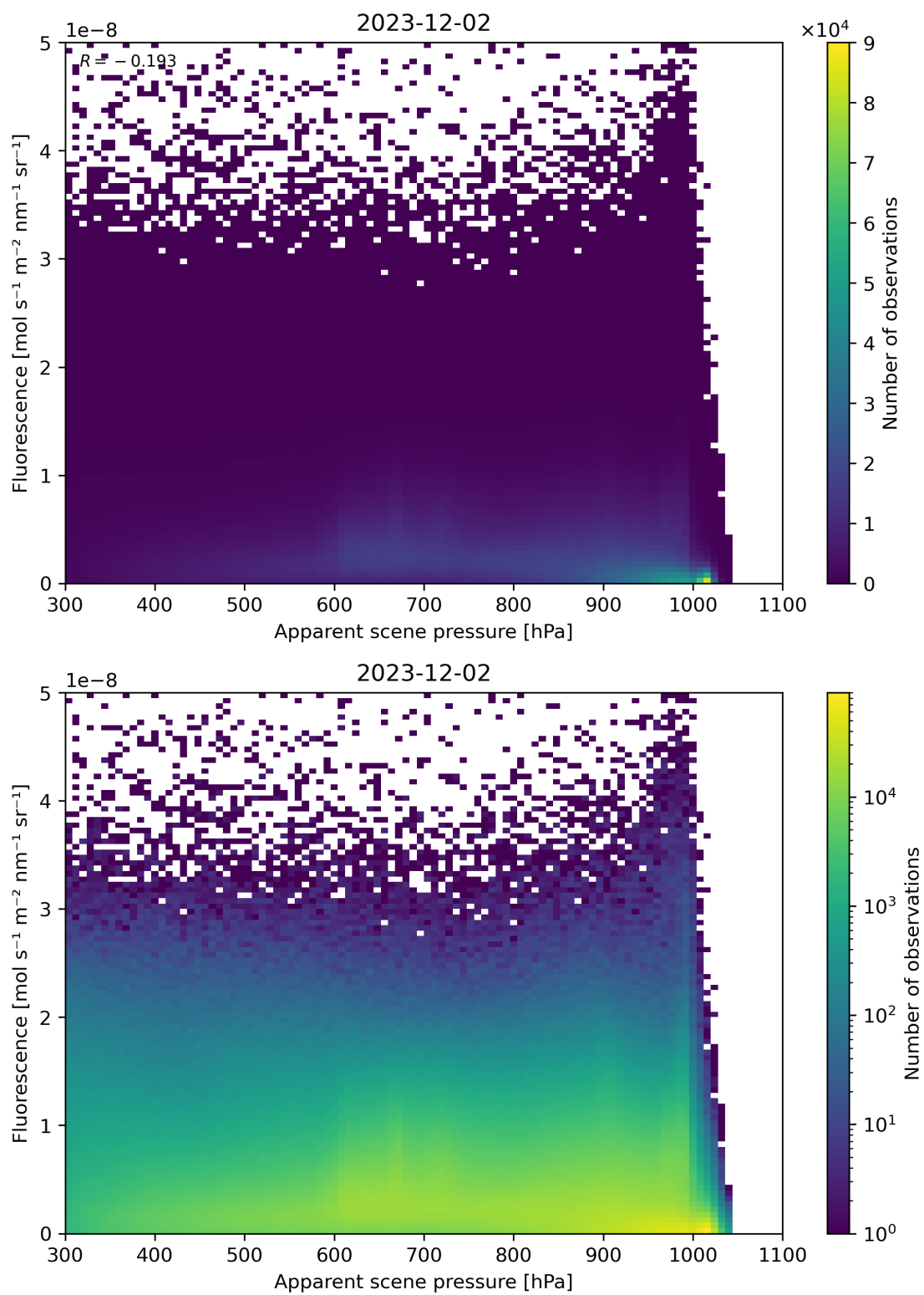
Figure 64: Scatter density plot of “Apparent scene pressure” against “Fluorescence” for 2023-12-01 to 2023-12-03.
