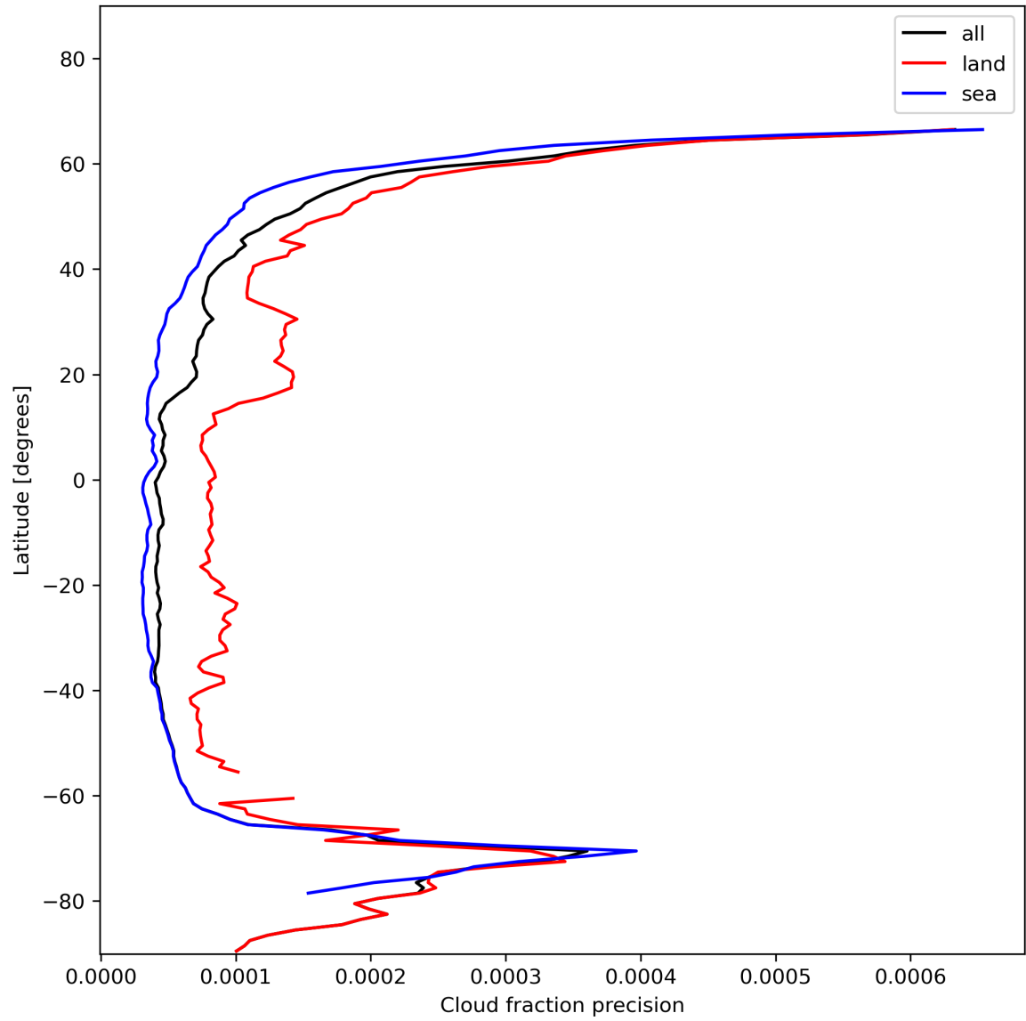
Figure 16: Zonal average of “Cloud fraction precision” for 2023-12-01 to 2023-12-03.
