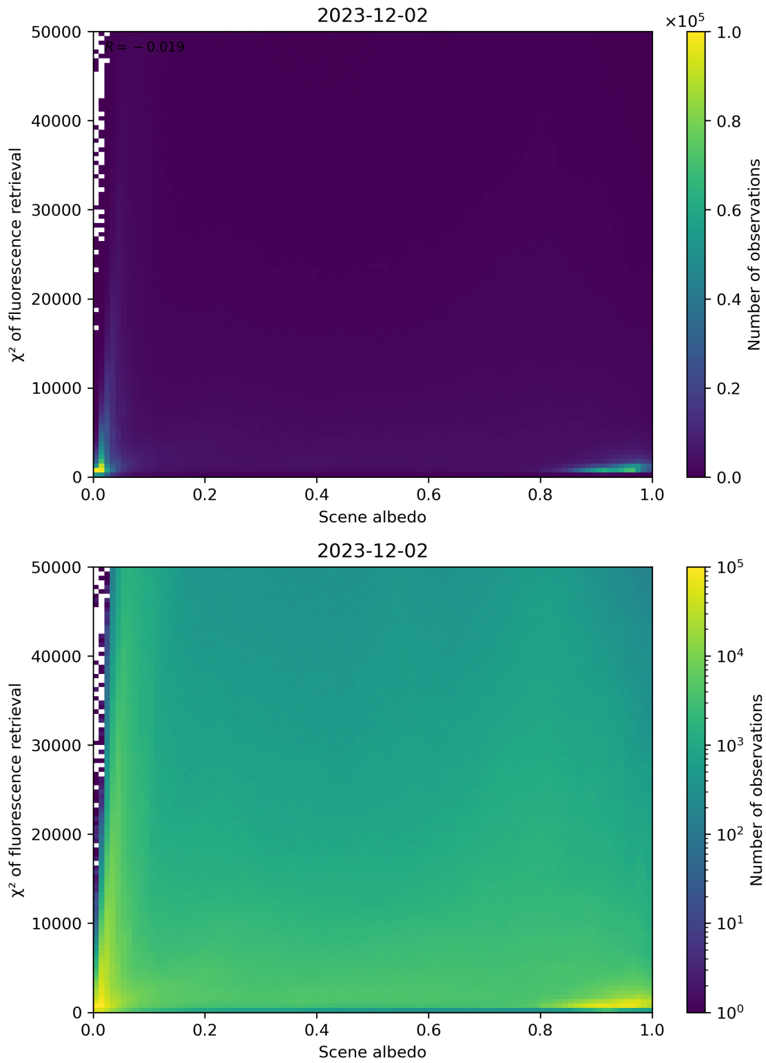
Figure 103: Scatter density plot of “Scene albedo” against “ \chi^2 of fluorescence retrieval” for 2023-12-01 to 2023-12-03.
