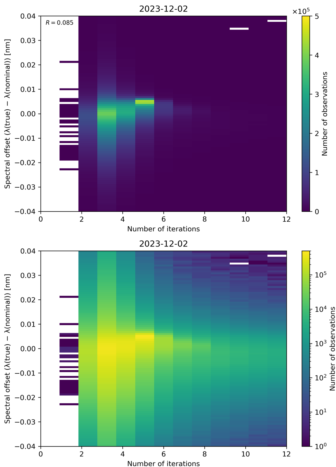
Figure 100: Scatter density plot of “Number of iterations” against “Spectral offset ( \lambda(\text{true}) - \lambda(\text{nominal}) )” for 2023-12-01 to 2023-12-03.
