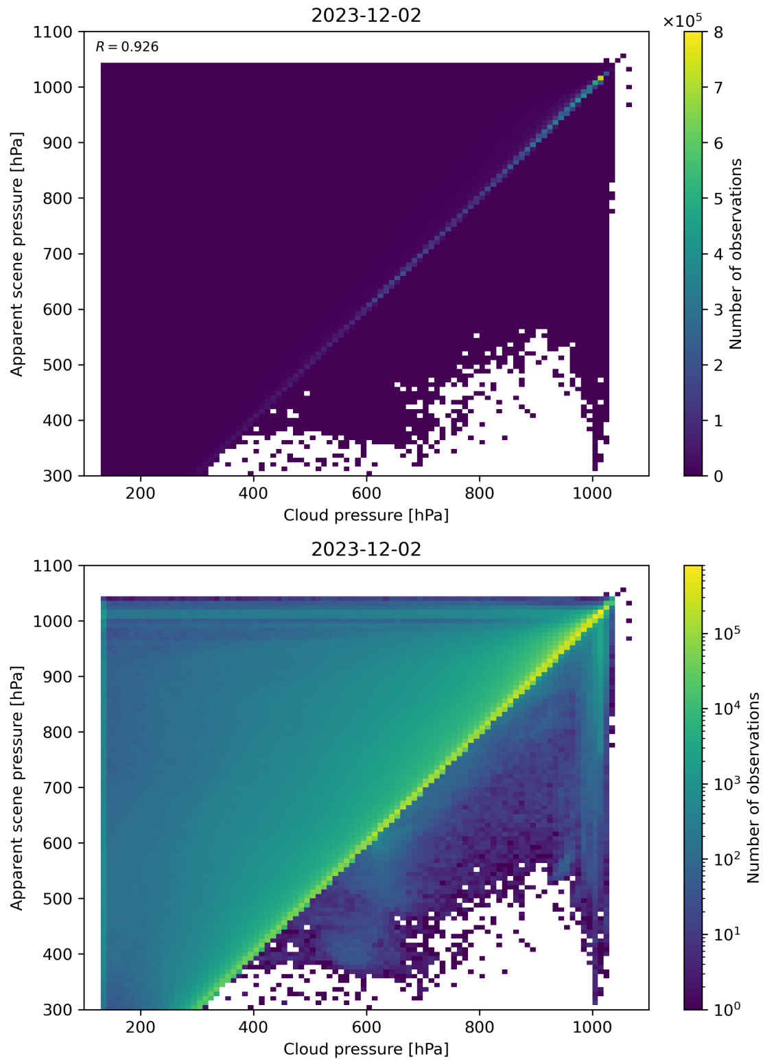
Figure 77: Scatter density plot of “Cloud pressure” against “Apparent scene pressure” for 2023-12-01 to 2023-12-03.
