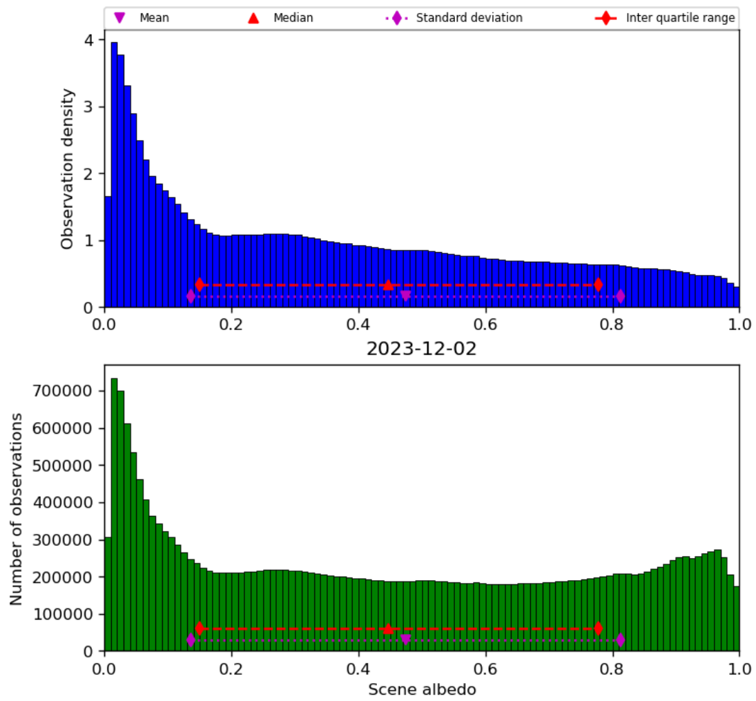
Figure 34: Histogram of “Scene albedo” for 2023-12-01 to 2023-12-03
