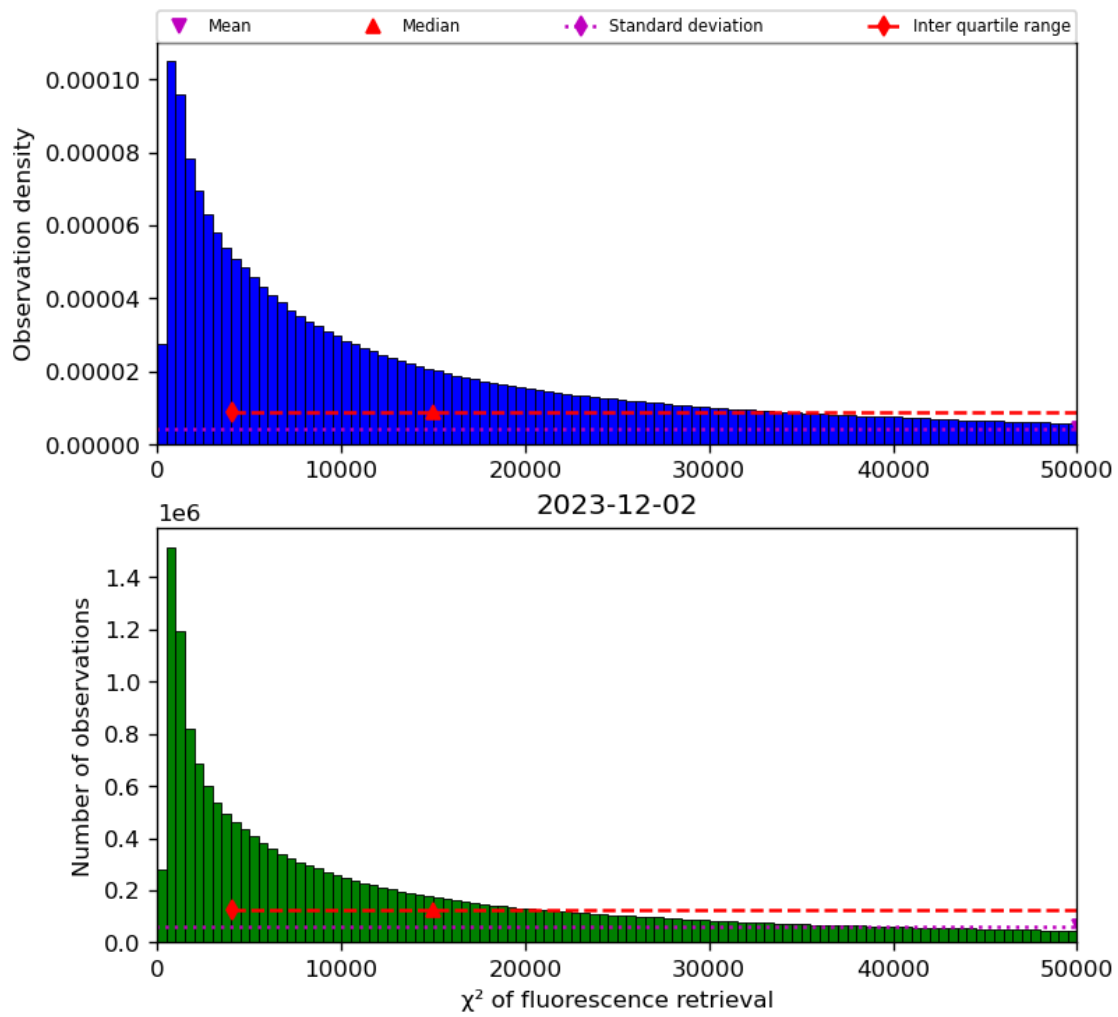
Figure 42: Histogram of “ \chi^2 of fluorescence retrieval” for 2023-12-01 to 2023-12-03
