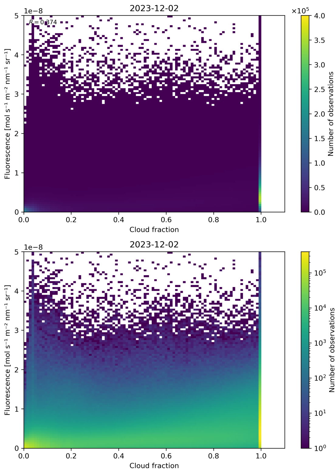
Figure 72: Scatter density plot of “Cloud fraction” against “Fluorescence” for 2023-12-01 to 2023-12-03.
