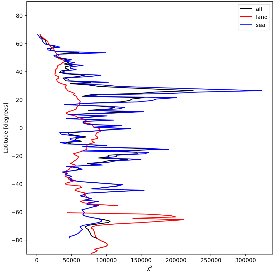
Figure 21: Zonal average of “ \chi^2 ” for 2023-12-01 to 2023-12-03.
