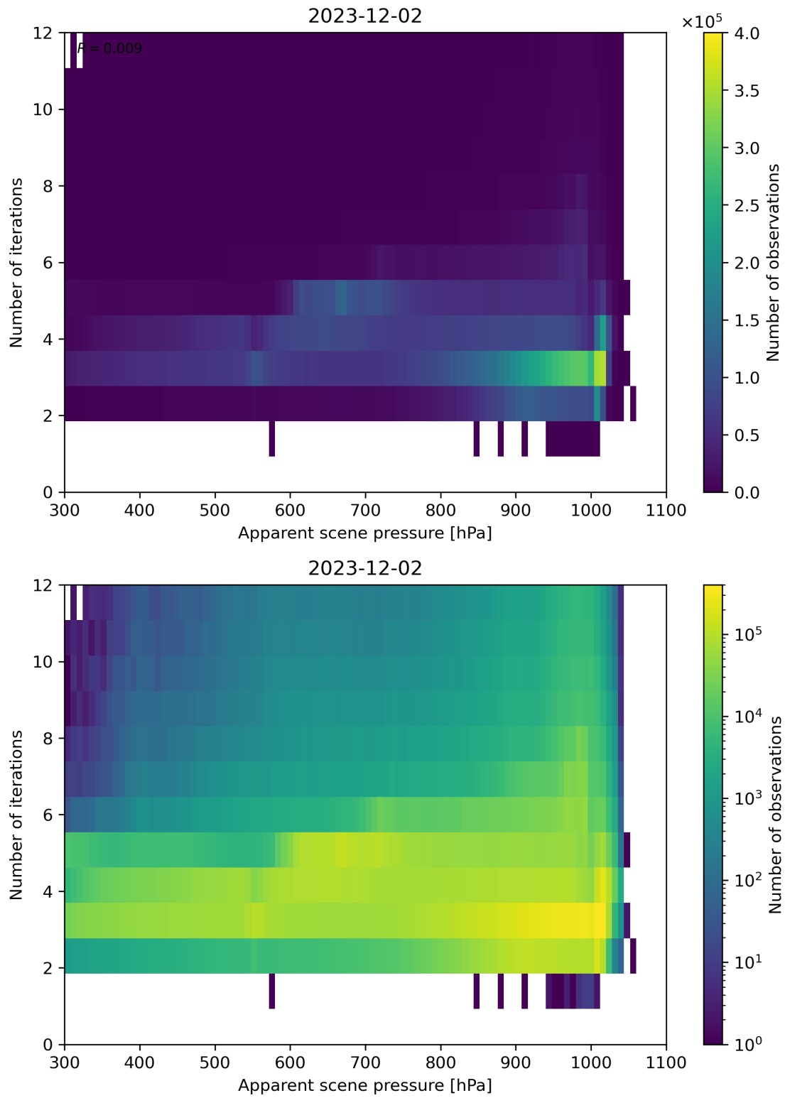
Figure 65: Scatter density plot of “Apparent scene pressure” against “Number of iterations” for 2023-12-01 to 2023-12-03.
