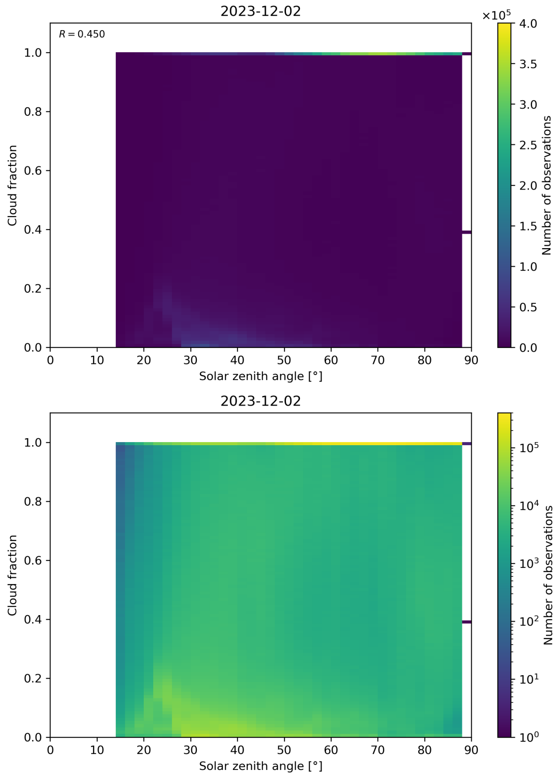
Figure 110: Scatter density plot of “Solar zenith angle” against “Cloud fraction” for 2023-12-01 to 2023-12-03.
