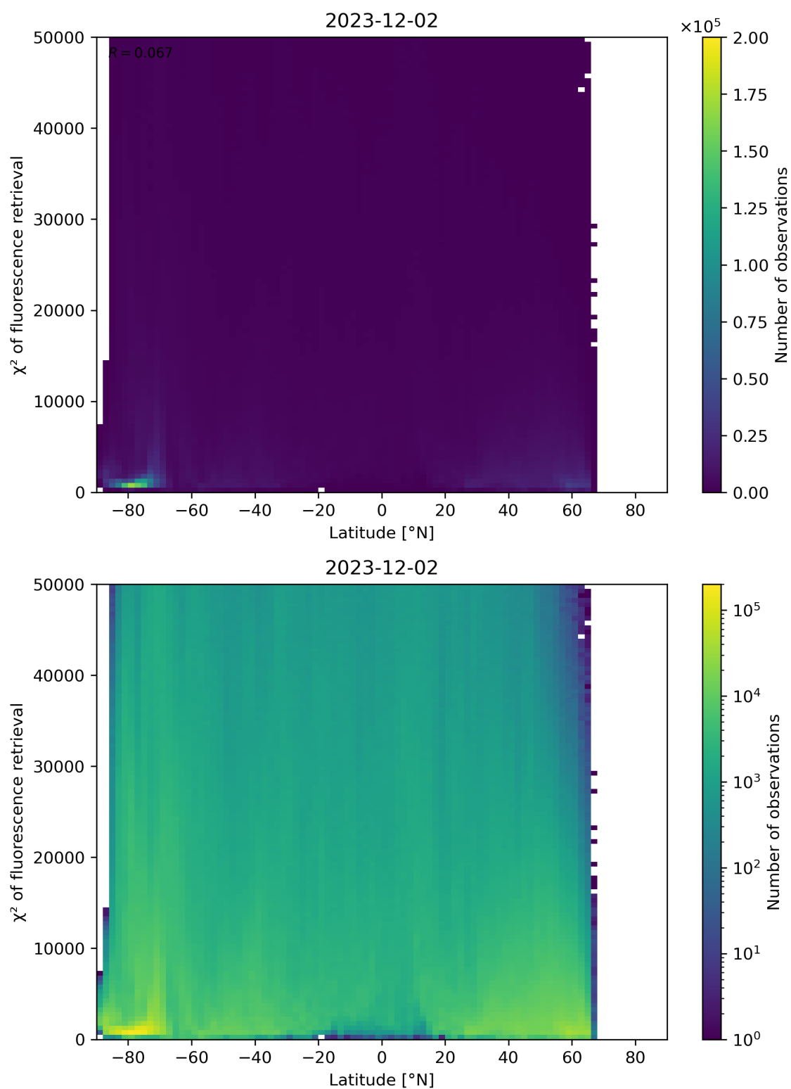
Figure 89: Scatter density plot of “Latitude” against “ \chi^2 of fluorescence retrieval” for 2023-12-01 to 2023-12-03.
