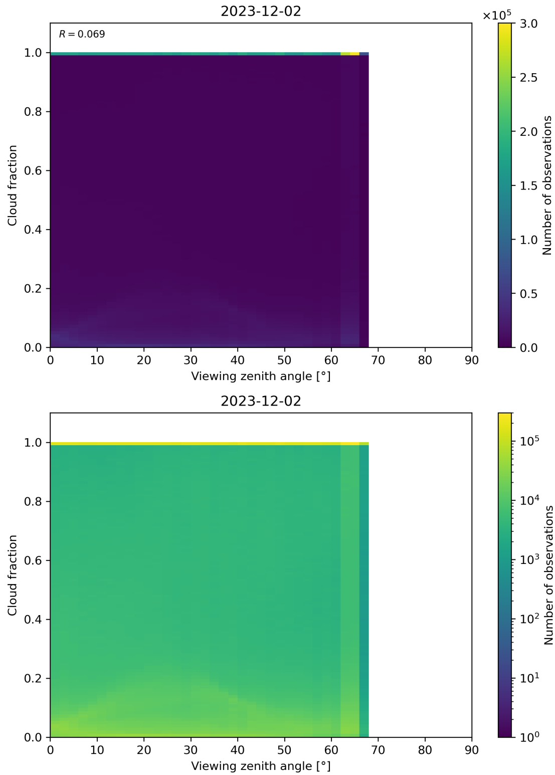
Figure 120: Scatter density plot of “Viewing zenith angle” against “Cloud fraction” for 2023-12-01 to 2023-12-03.
