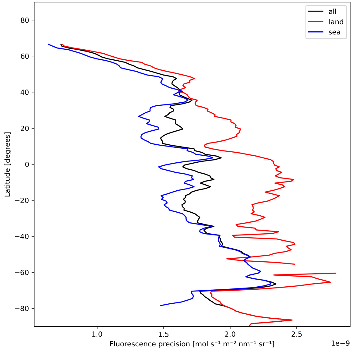
Figure 24: Zonal average of “Fluorescence precision” for 2023-12-01 to 2023-12-03.
