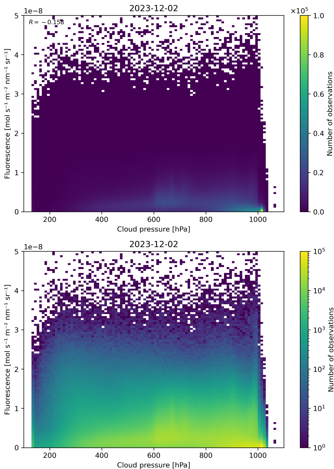
Figure 80: Scatter density plot of “Cloud pressure” against “Fluorescence” for 2023-12-01 to 2023-12-03.
