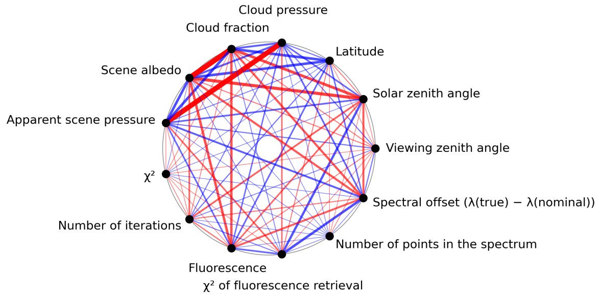
Figure 1: Map of correlation graph for 2023-12-01 to 2023-12-03.
