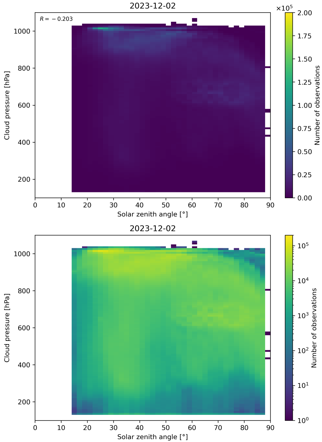
Figure 111: Scatter density plot of “Solar zenith angle” against “Cloud pressure” for 2023-12-01 to 2023-12-03.
