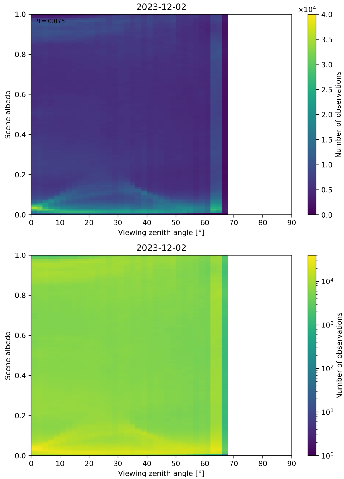
Figure 126: Scatter density plot of “Viewing zenith angle” against “Scene albedo” for 2023-12-01 to 2023-12-03.
