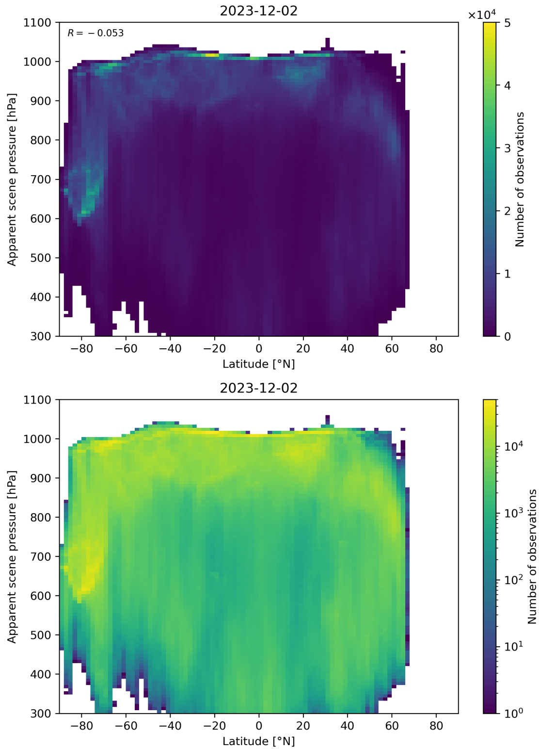
Figure 88: Scatter density plot of “Latitude” against “Apparent scene pressure” for 2023-12-01 to 2023-12-03.
