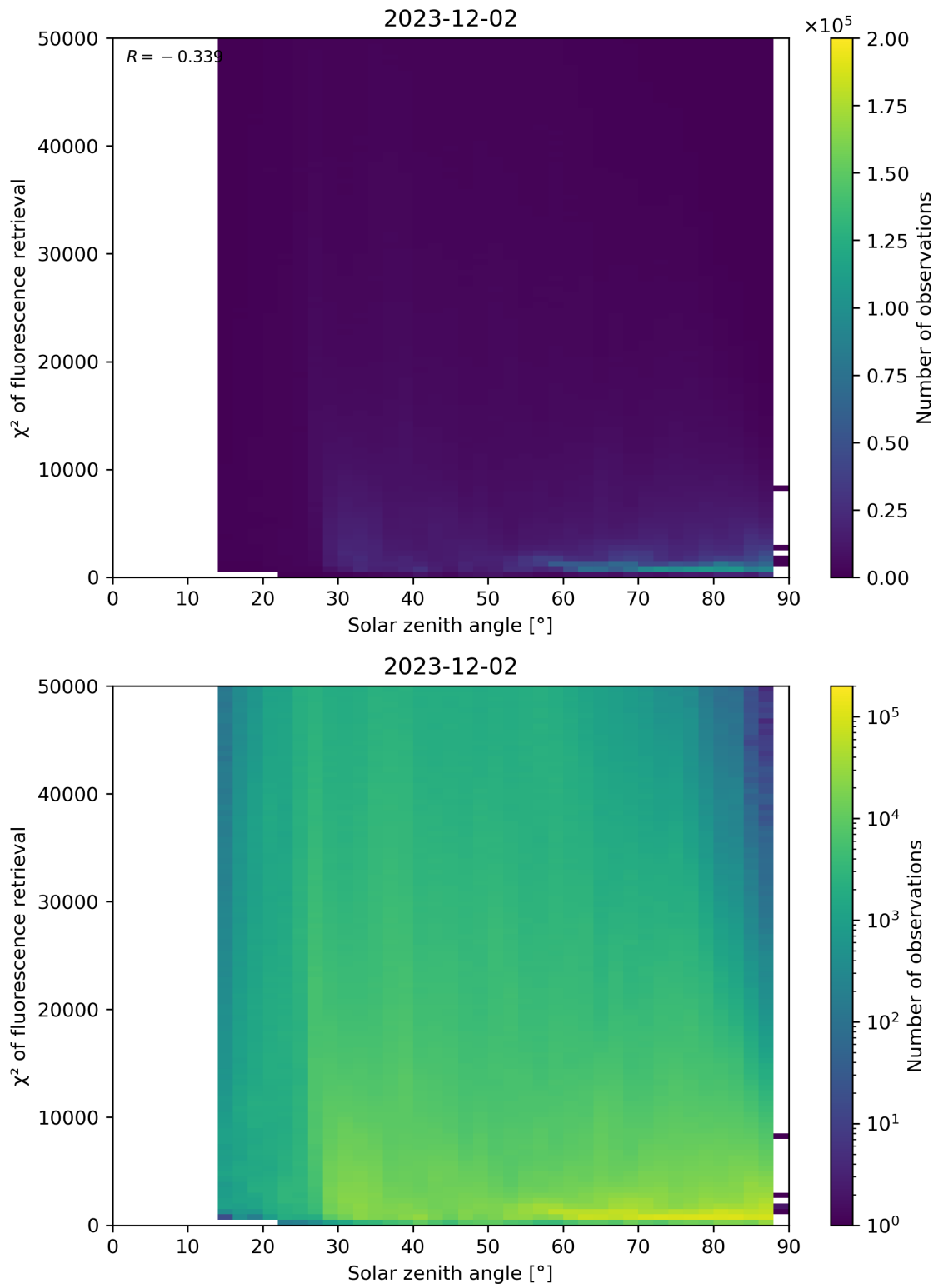
Figure 109: Scatter density plot of “Solar zenith angle” against “ \chi^2 of fluorescence retrieval” for 2023-12-01 to 2023-12-03.
