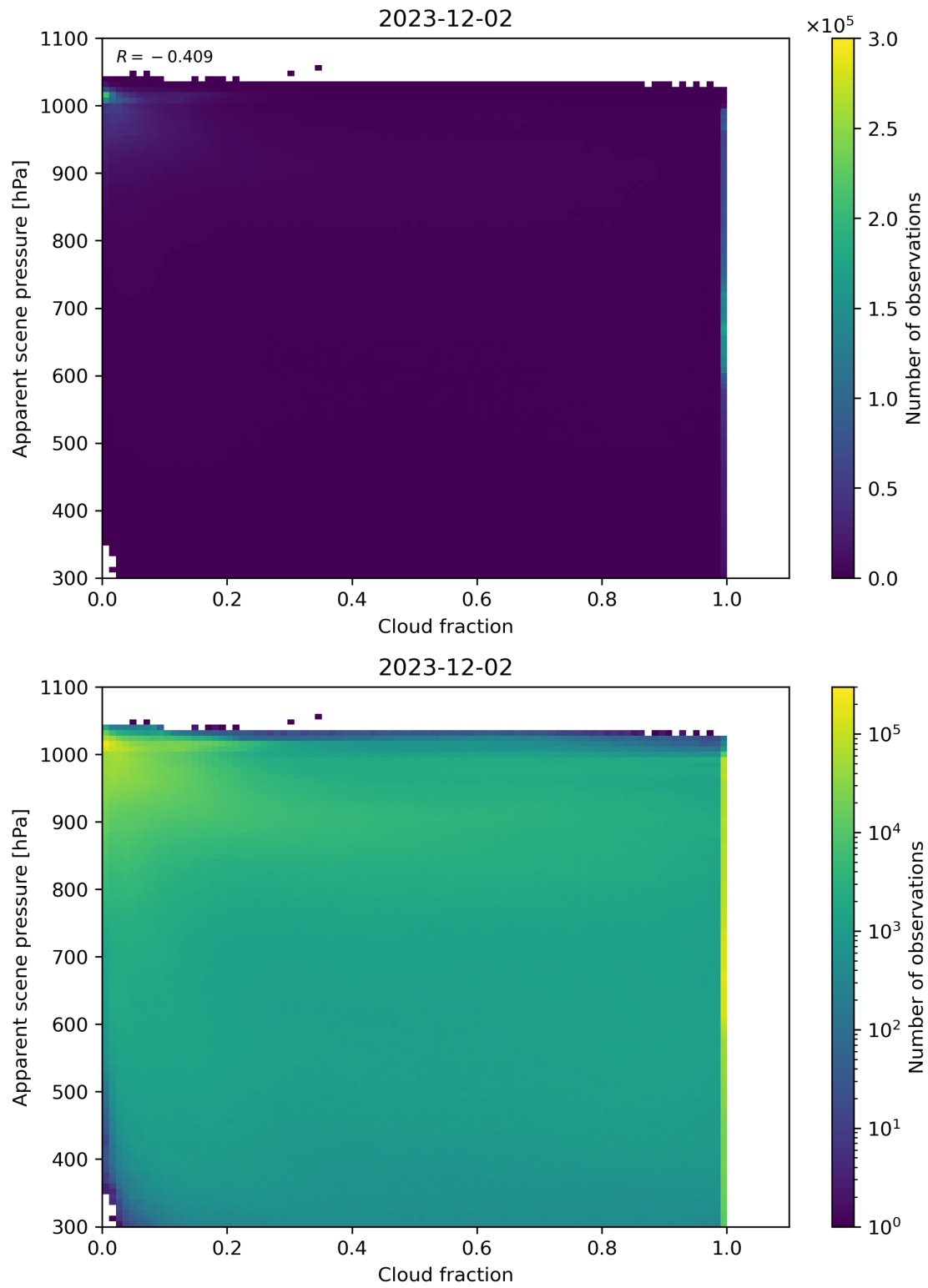
Figure 70: Scatter density plot of “Cloud fraction” against “Apparent scene pressure” for 2023-12-01 to 2023-12-03.
