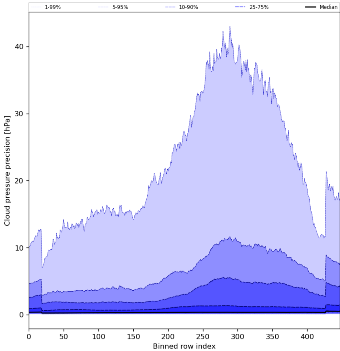
Figure 48: Along track statistics of “Cloud pressure precision” for 2023-12-01 to 2023-12-03
