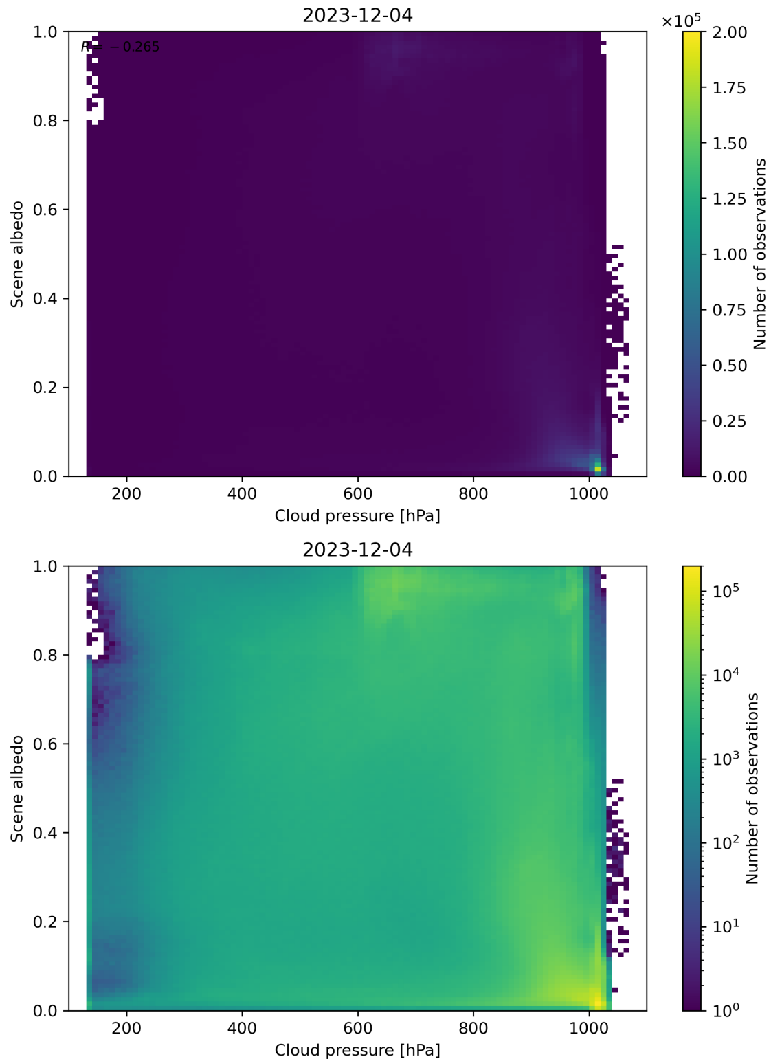
Figure 83: Scatter density plot of “Cloud pressure” against “Scene albedo” for 2023-12-04 to 2023-12-05.
