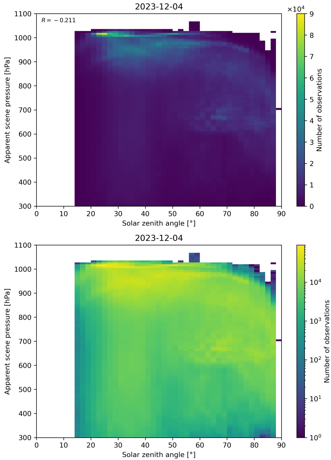
Figure 108: Scatter density plot of “Solar zenith angle” against “Apparent scene pressure” for 2023-12-04 to 2023-12-05.
