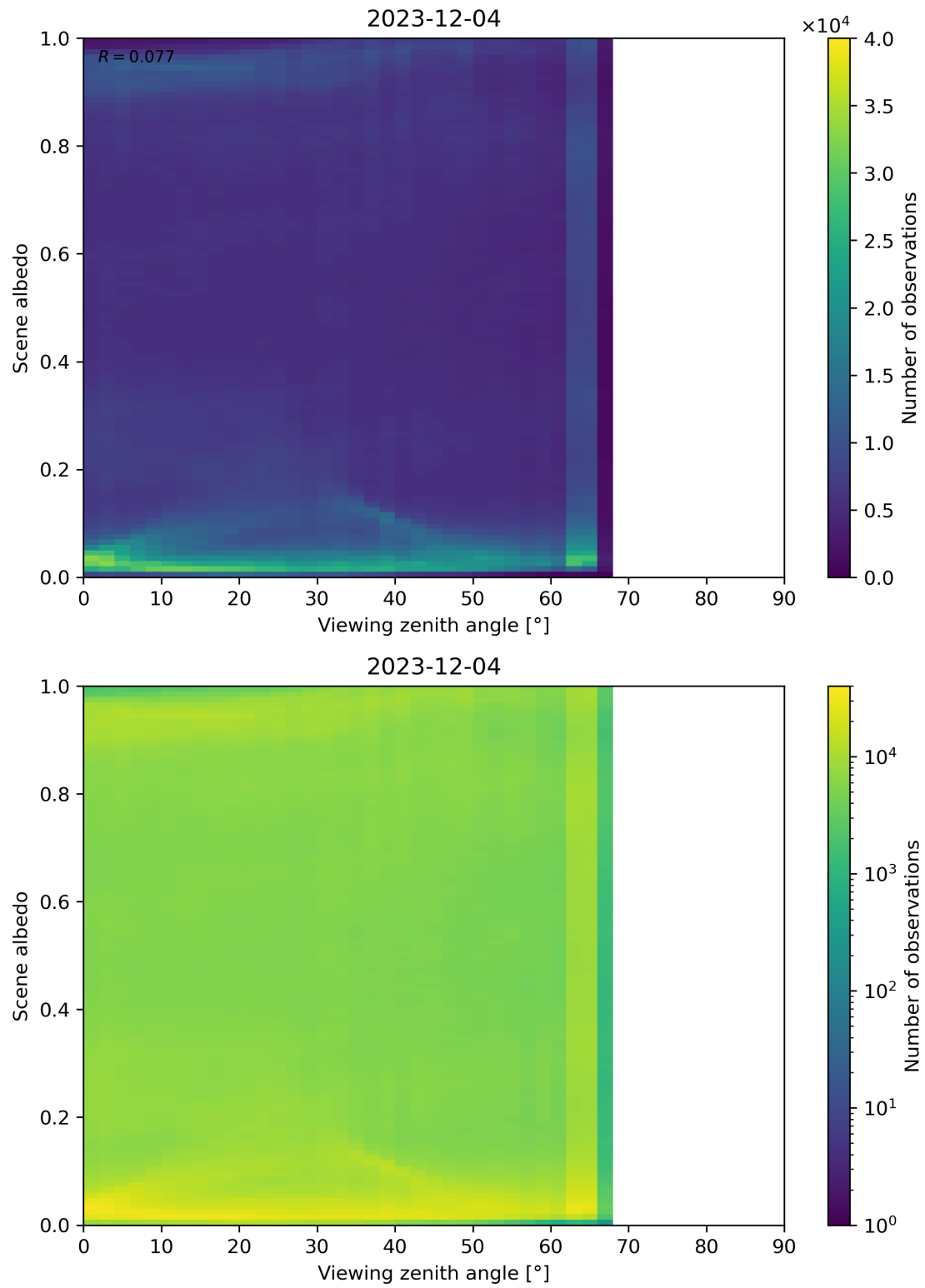
Figure 126: Scatter density plot of “Viewing zenith angle” against “Scene albedo” for 2023-12-04 to 2023-12-05.
