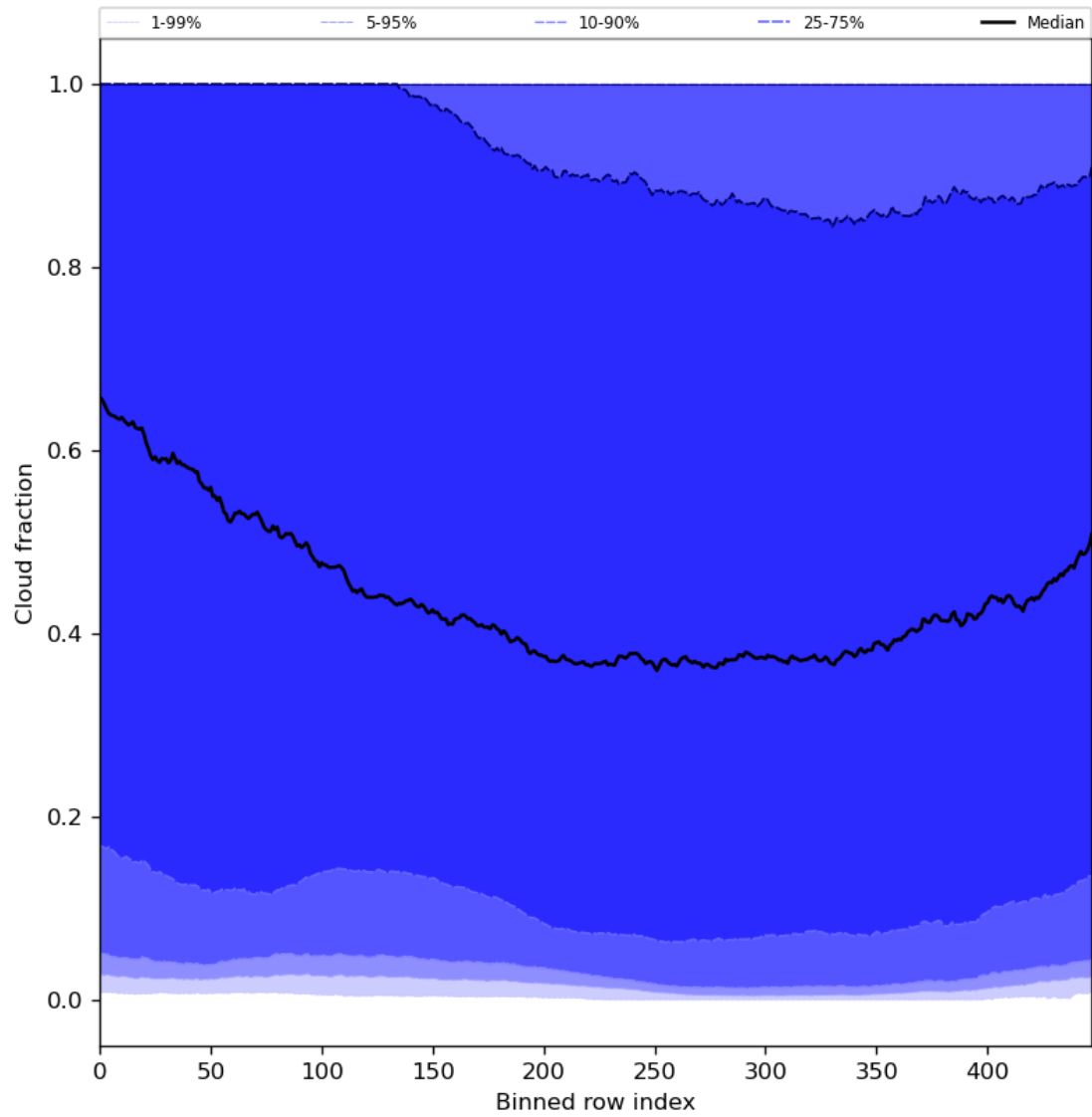
Figure 49: Along track statistics of “Cloud fraction” for 2023-12-04 to 2023-12-05
