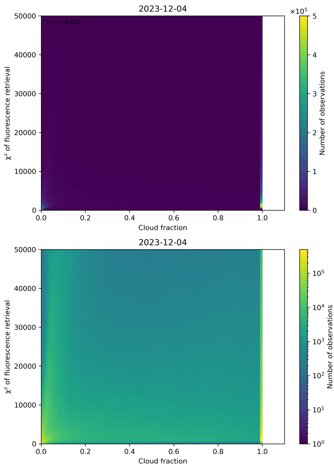
Figure 71: Scatter density plot of “Cloud fraction” against “ \chi^2 of fluorescence retrieval” for 2023-12-04 to 2023-12-05.
