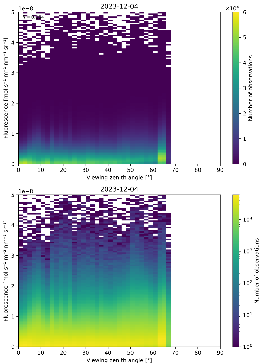
Figure 122: Scatter density plot of “Viewing zenith angle” against “Fluorescence” for 2023-12-04 to 2023-12-05.
