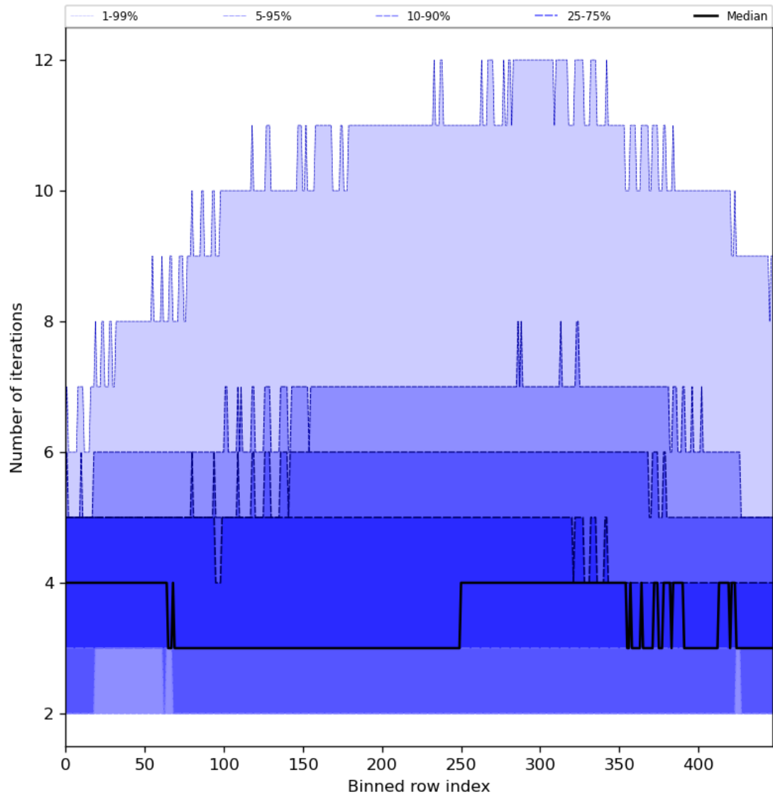
Figure 56: Along track statistics of “Number of iterations” for 2023-12-04 to 2023-12-05
