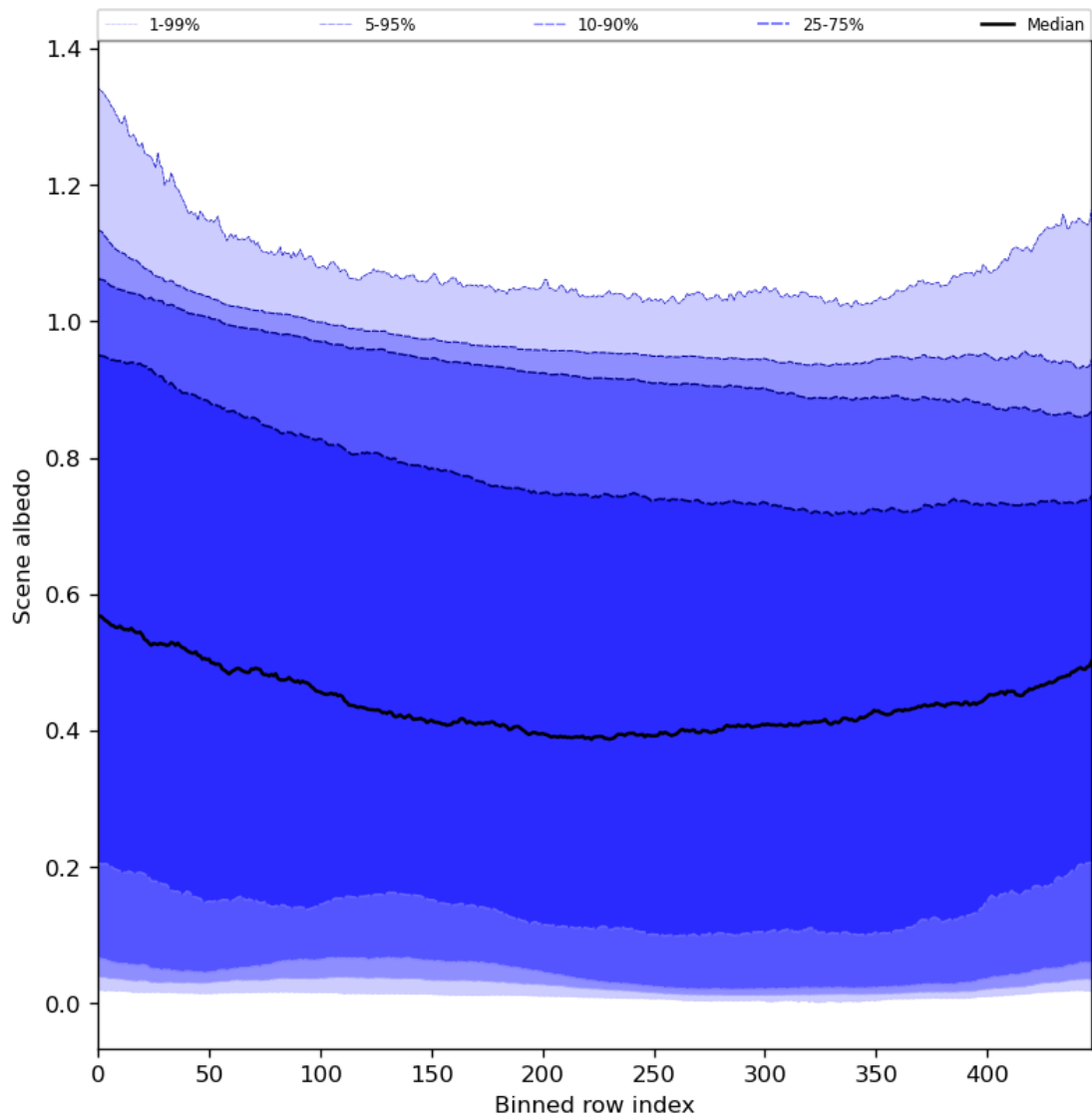
Figure 51: Along track statistics of “Scene albedo” for 2023-12-04 to 2023-12-05
