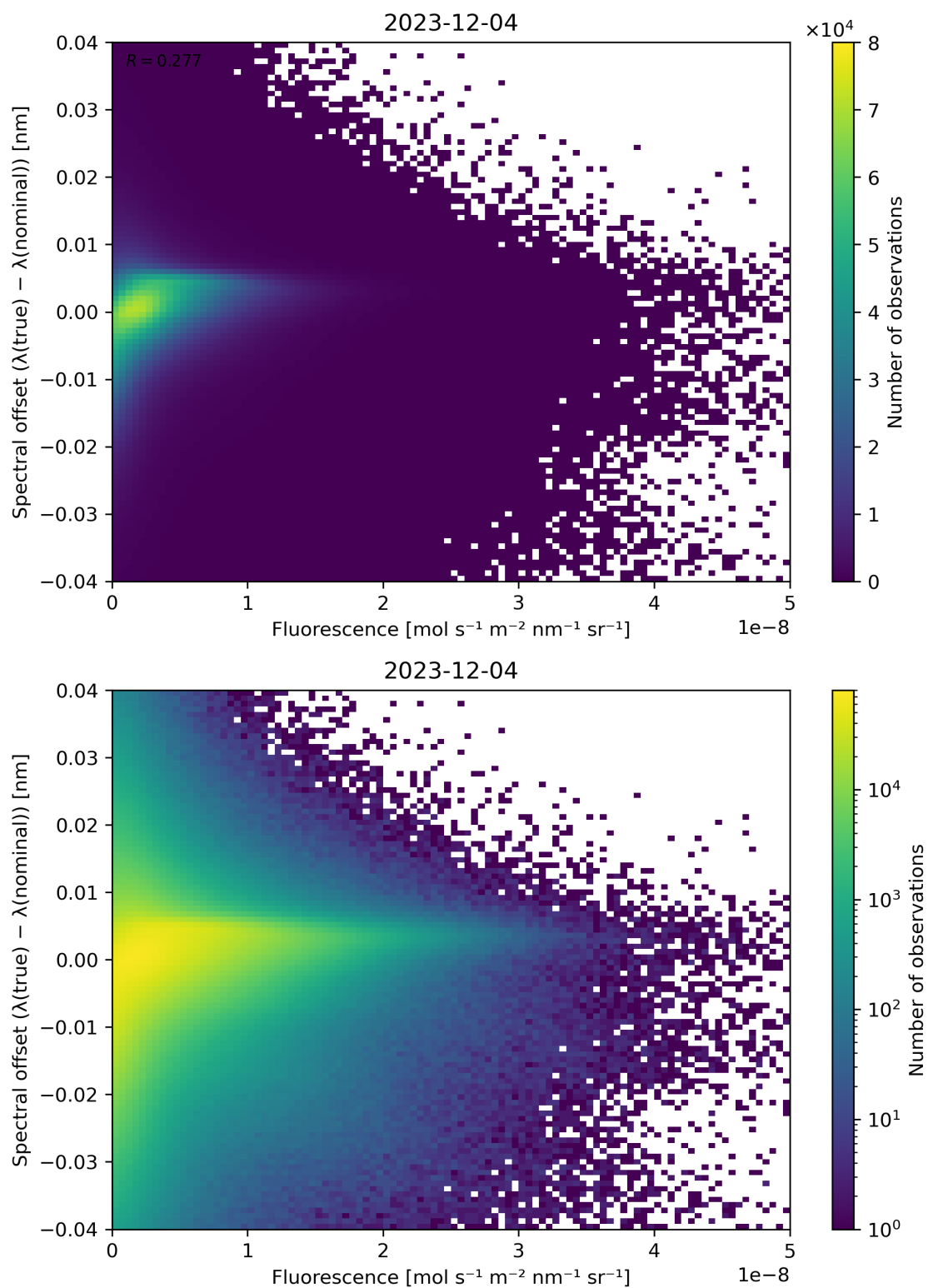
Figure 87: Scatter density plot of “Fluorescence” against “Spectral offset ( \lambda(\text{true}) - \lambda(\text{nominal}) )” for 2023-12-04 to 2023-12-05.
