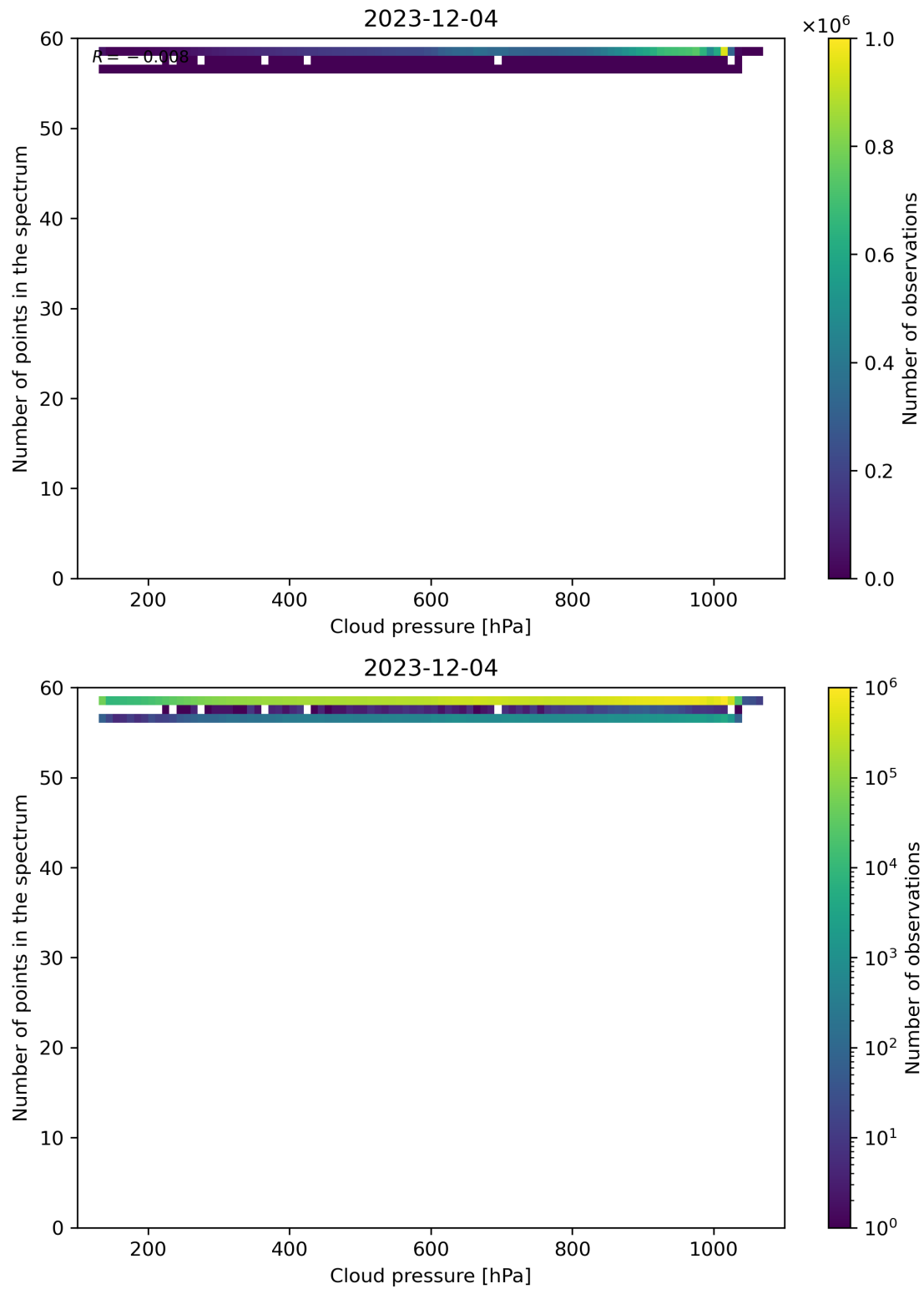
Figure 82: Scatter density plot of “Cloud pressure” against “Number of points in the spectrum” for 2023-12-04 to 2023-12-05.
