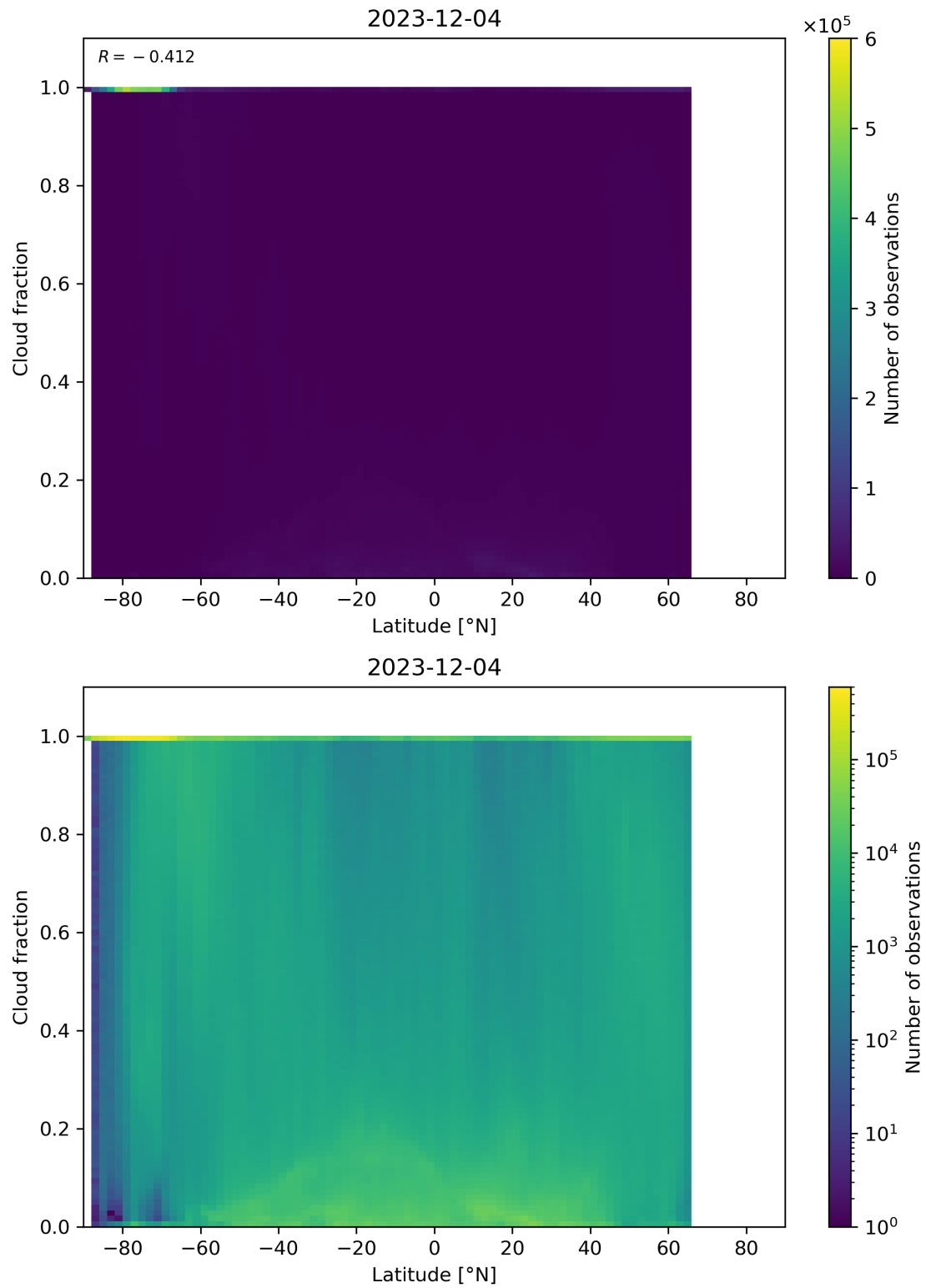
Figure 90: Scatter density plot of “Latitude” against “Cloud fraction” for 2023-12-04 to 2023-12-05.
