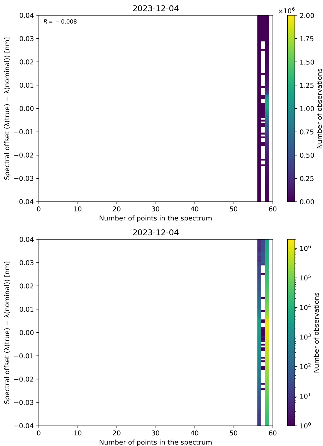
Figure 101: Scatter density plot of “Number of points in the spectrum” against “Spectral offset ( \lambda(\text{true}) - \lambda(\text{nominal}) )” for 2023-12-04 to 2023-12-05.
