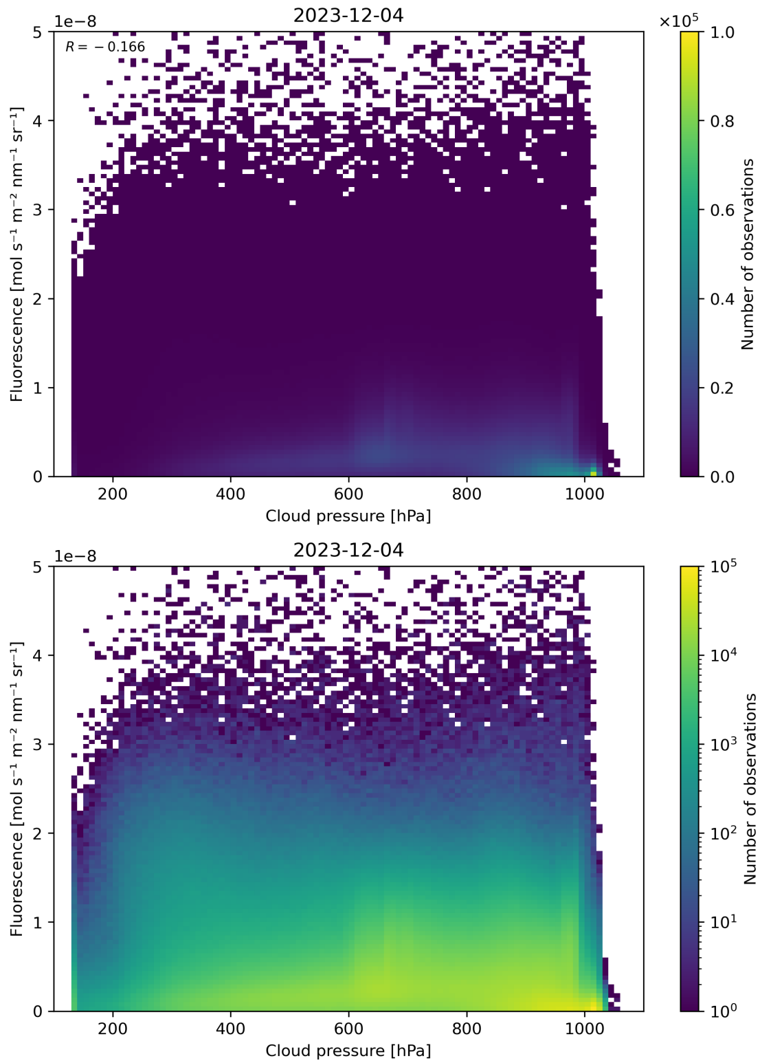
Figure 80: Scatter density plot of “Cloud pressure” against “Fluorescence” for 2023-12-04 to 2023-12-05.
