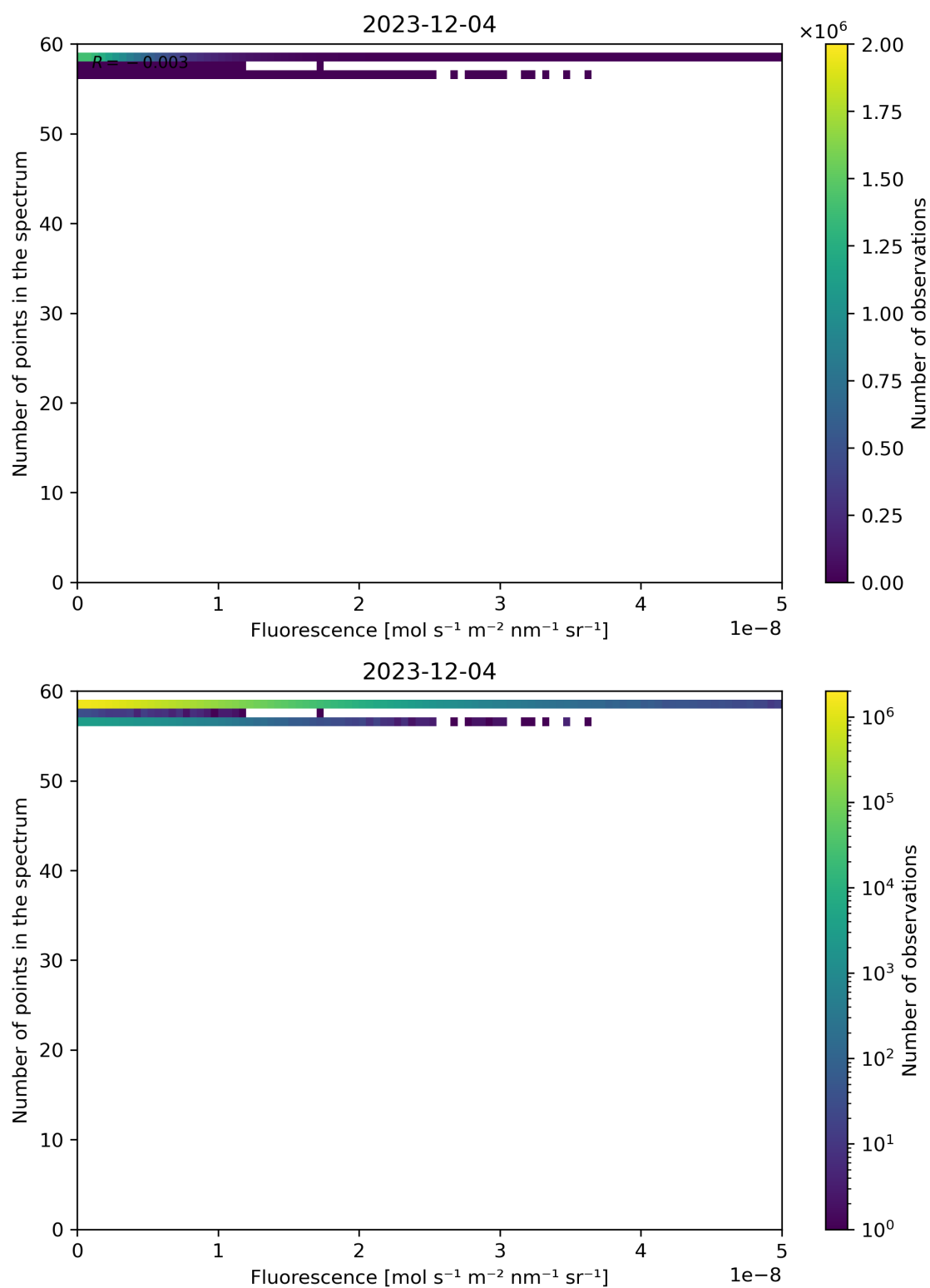
Figure 86: Scatter density plot of “Fluorescence” against “Number of points in the spectrum” for 2023-12-04 to 2023-12-05.
