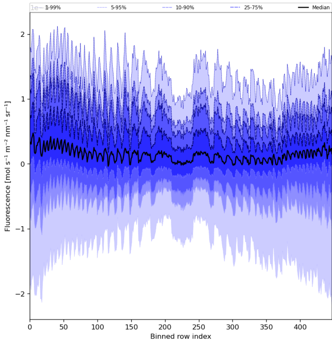
Figure 57: Along track statistics of “Fluorescence” for 2023-12-04 to 2023-12-05
