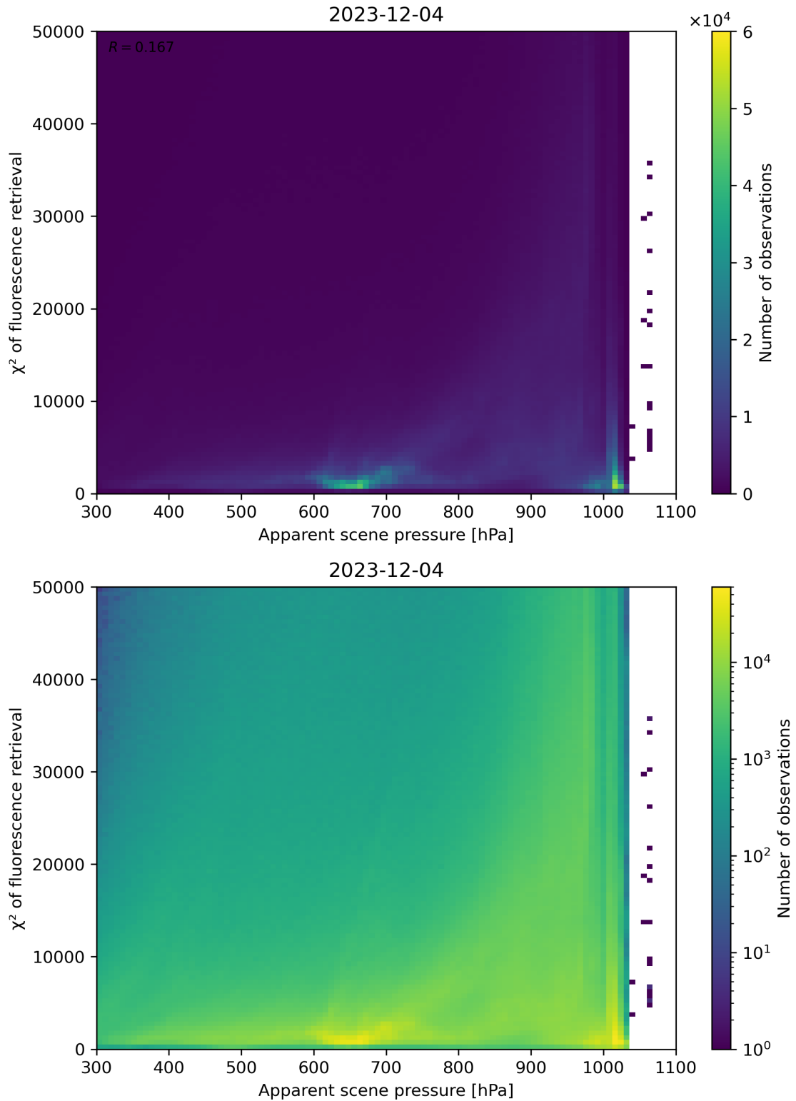
Figure 63: Scatter density plot of “Apparent scene pressure” against “ \chi^2 of fluorescence retrieval” for 2023-12-04 to 2023-12-05.
