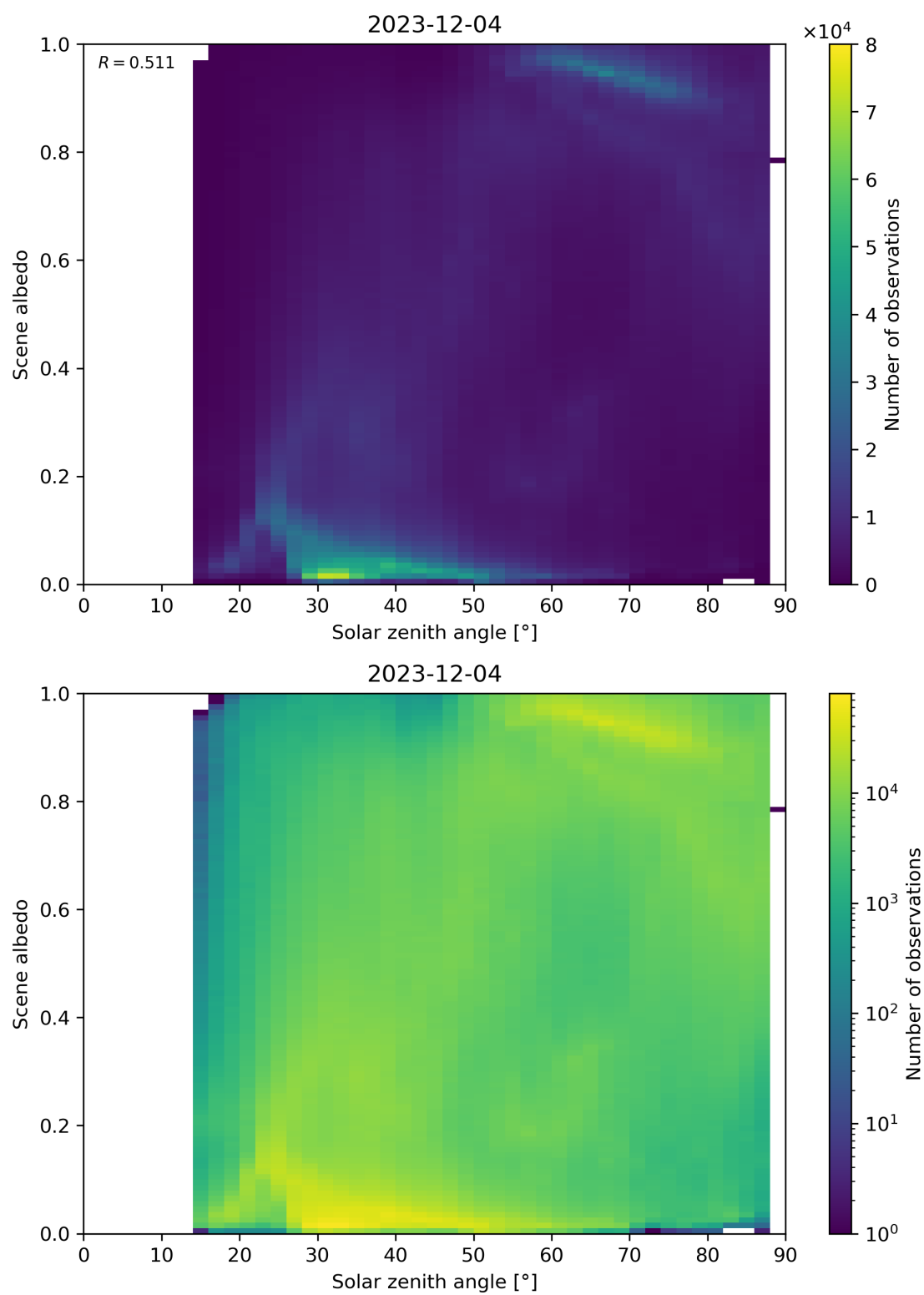
Figure 116: Scatter density plot of “Solar zenith angle” against “Scene albedo” for 2023-12-04 to 2023-12-05.
