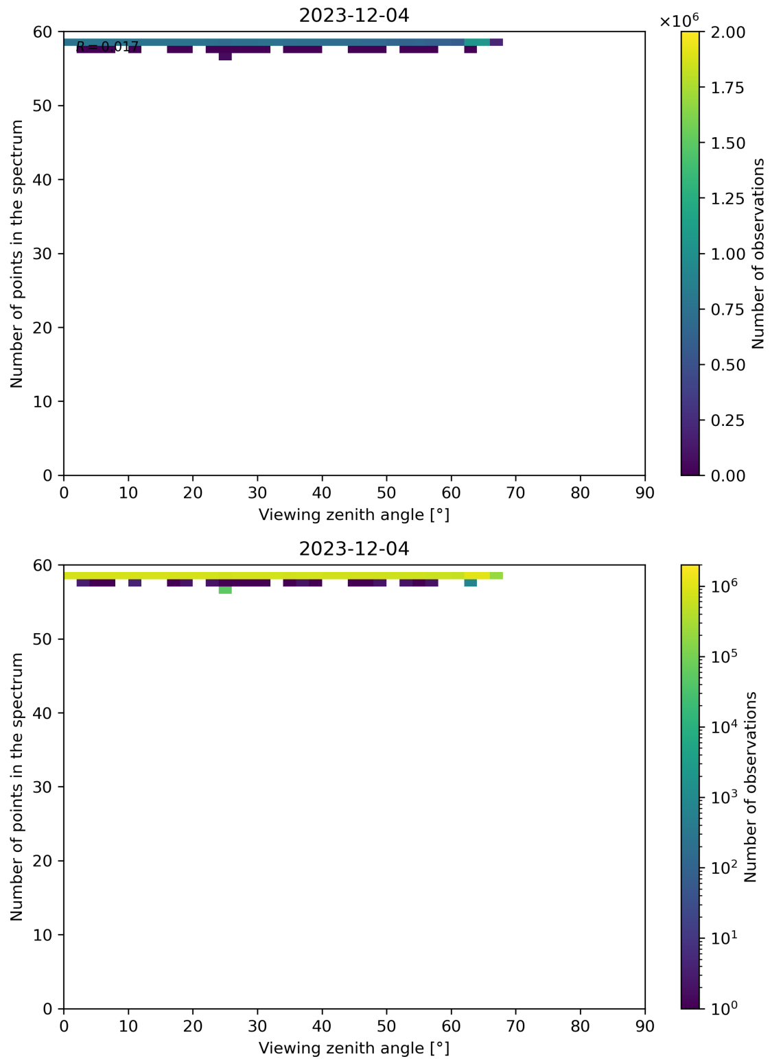
Figure 125: Scatter density plot of “Viewing zenith angle” against “Number of points in the spectrum” for 2023-12-04 to 2023-12-05.
