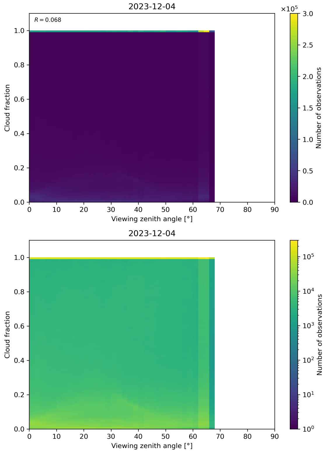
Figure 120: Scatter density plot of “Viewing zenith angle” against “Cloud fraction” for 2023-12-04 to 2023-12-05.
