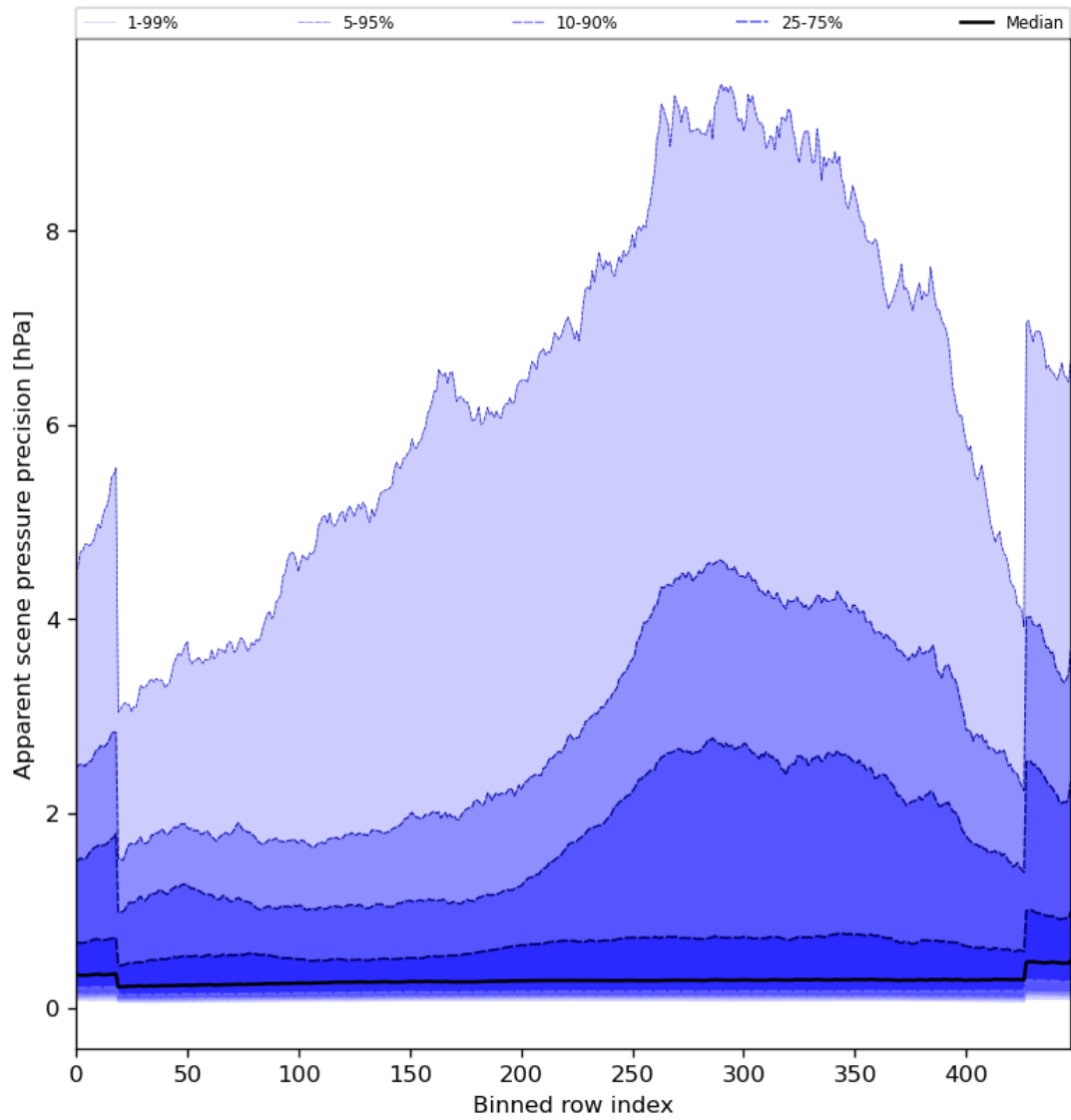
Figure 54: Along track statistics of “Apparent scene pressure precision” for 2023-12-04 to 2023-12-05
