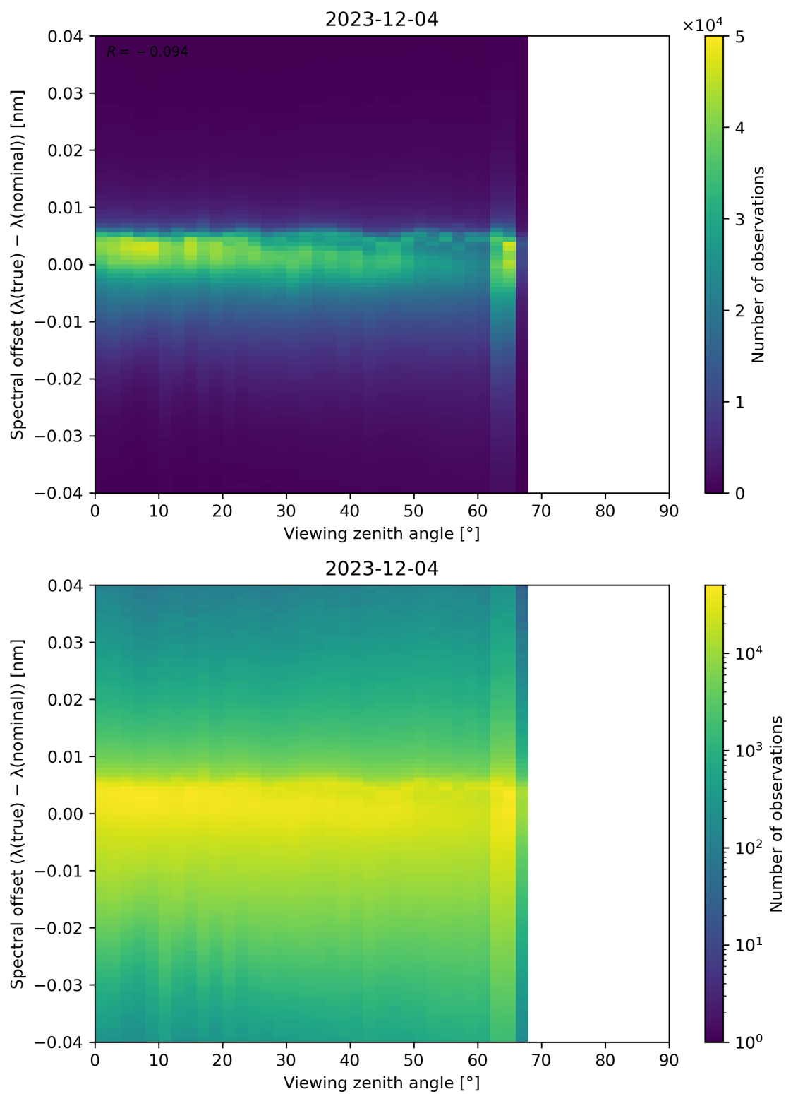
Figure 128: Scatter density plot of “Viewing zenith angle” against “Spectral offset ( \lambda(\text{true}) - \lambda(\text{nominal}) )” for 2023-12-04 to 2023-12-05.
