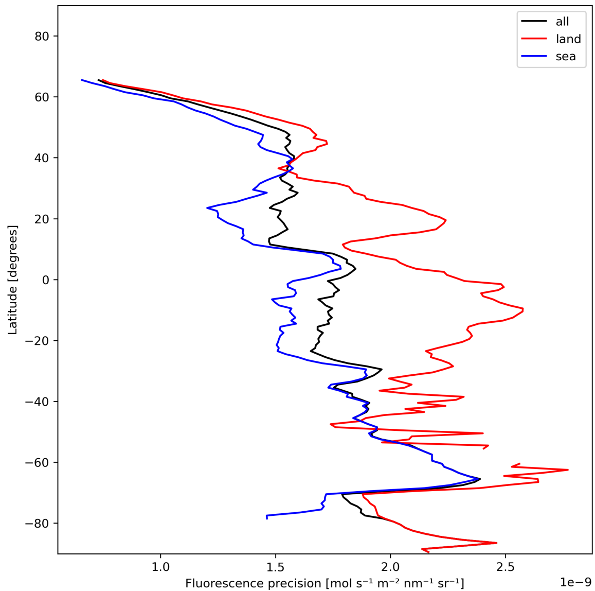
Figure 24: Zonal average of “Fluorescence precision” for 2023-12-04 to 2023-12-05.
