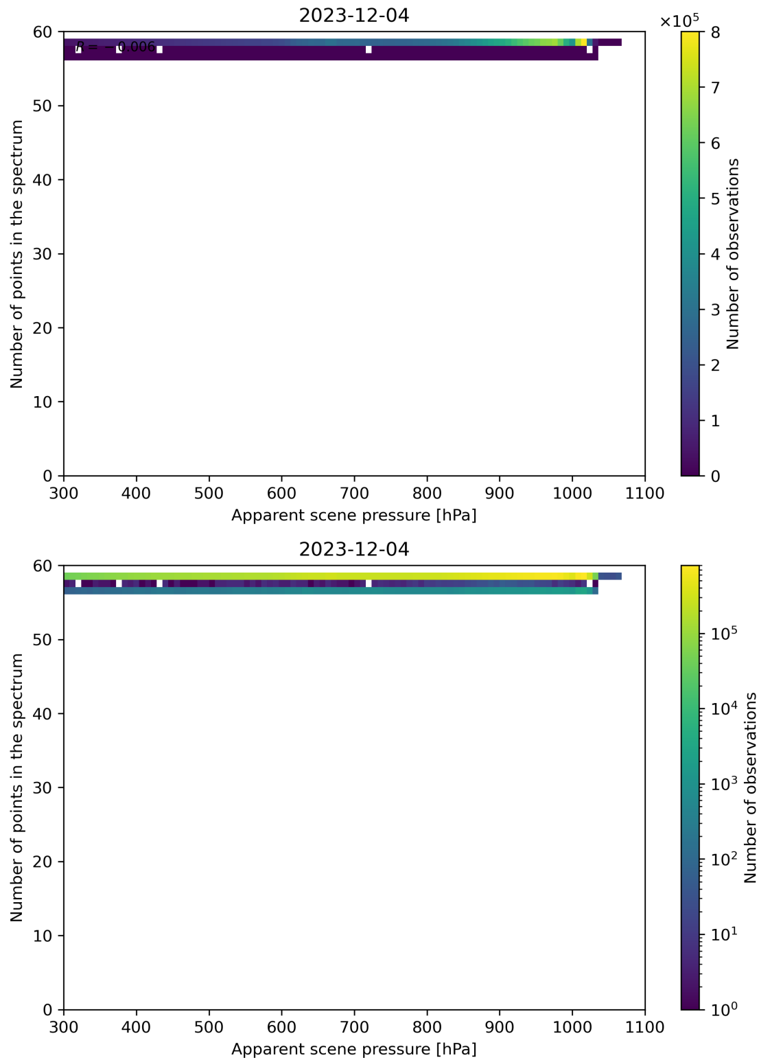
Figure 66: Scatter density plot of “Apparent scene pressure” against “Number of points in the spectrum” for 2023-12-04 to 2023-12-05.
