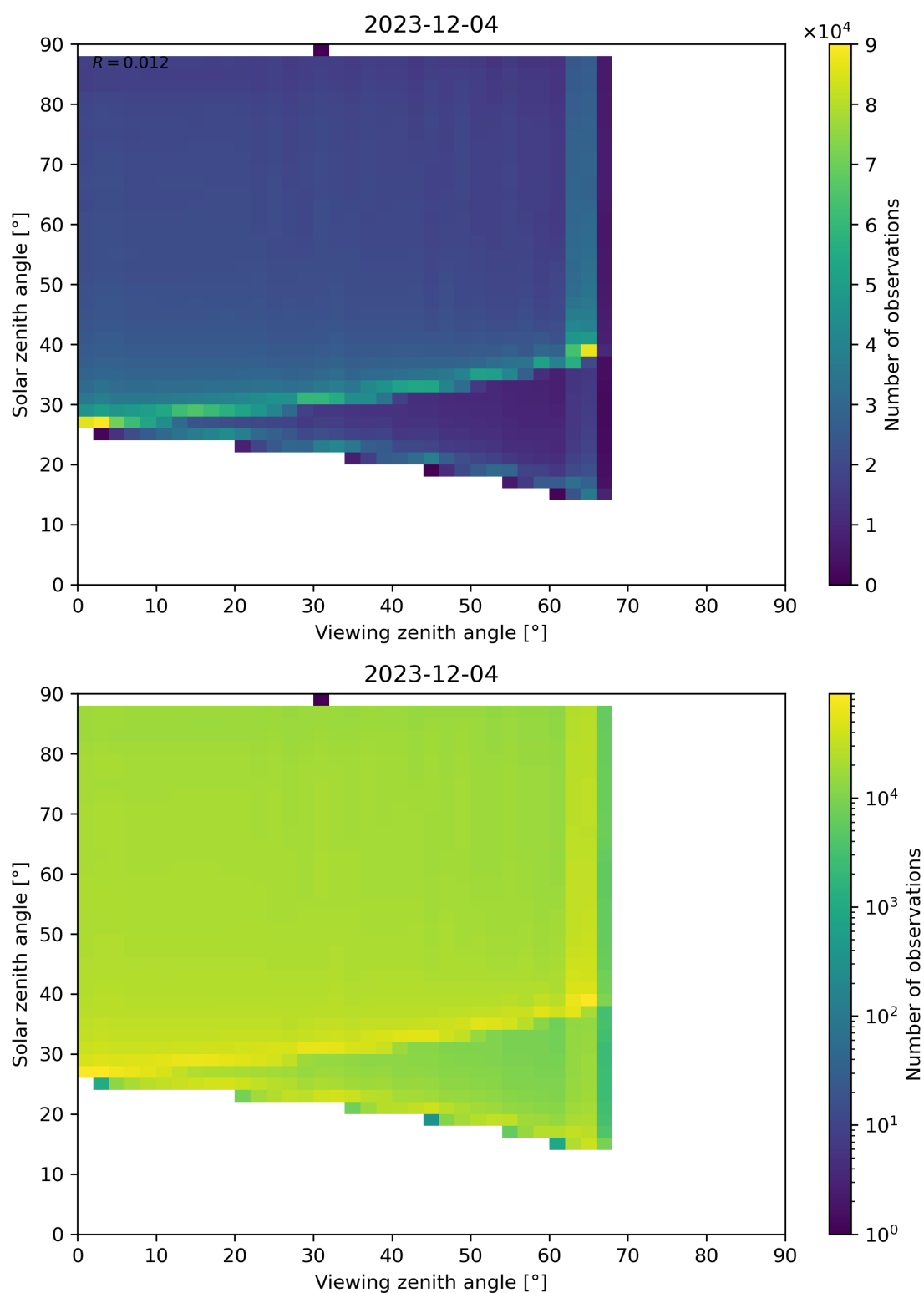
Figure 127: Scatter density plot of “Viewing zenith angle” against “Solar zenith angle” for 2023-12-04 to 2023-12-05.
