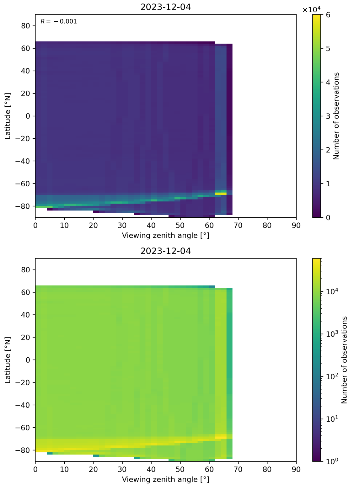
Figure 123: Scatter density plot of “Viewing zenith angle” against “Latitude” for 2023-12-04 to 2023-12-05.
