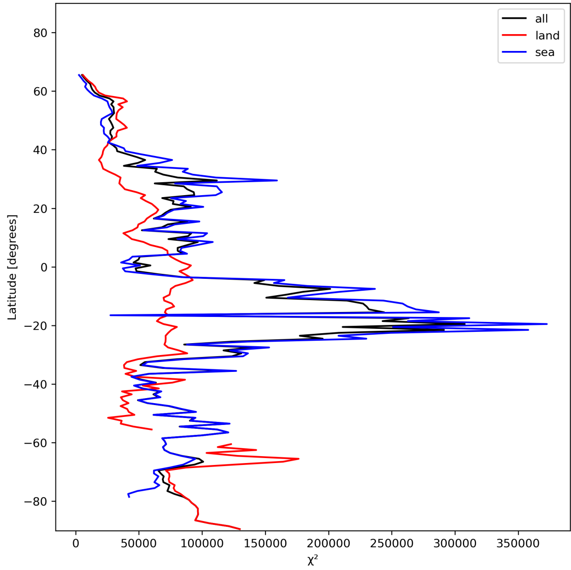
Figure 21: Zonal average of “ \chi^2 ” for 2023-12-04 to 2023-12-05.
