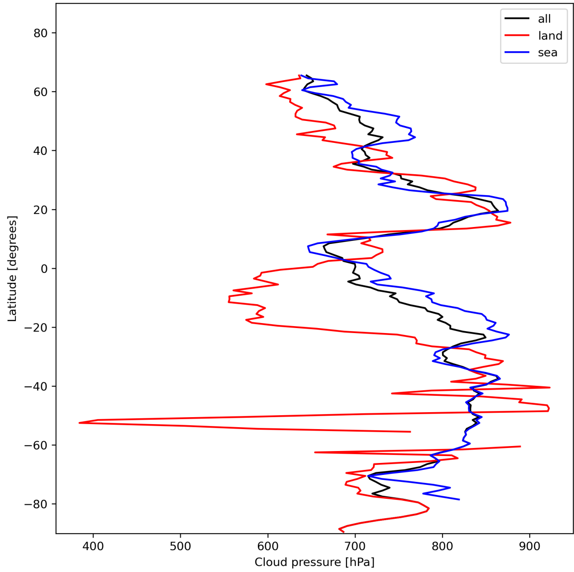
Figure 13: Zonal average of “Cloud pressure” for 2023-12-04 to 2023-12-05.
