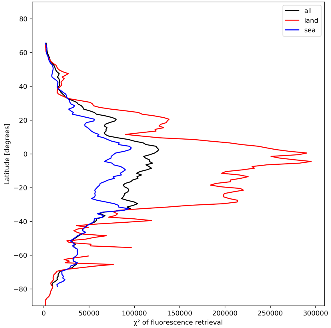
Figure 25: Zonal average of “ \chi^2 of fluorescence retrieval” for 2023-12-04 to 2023-12-05.
