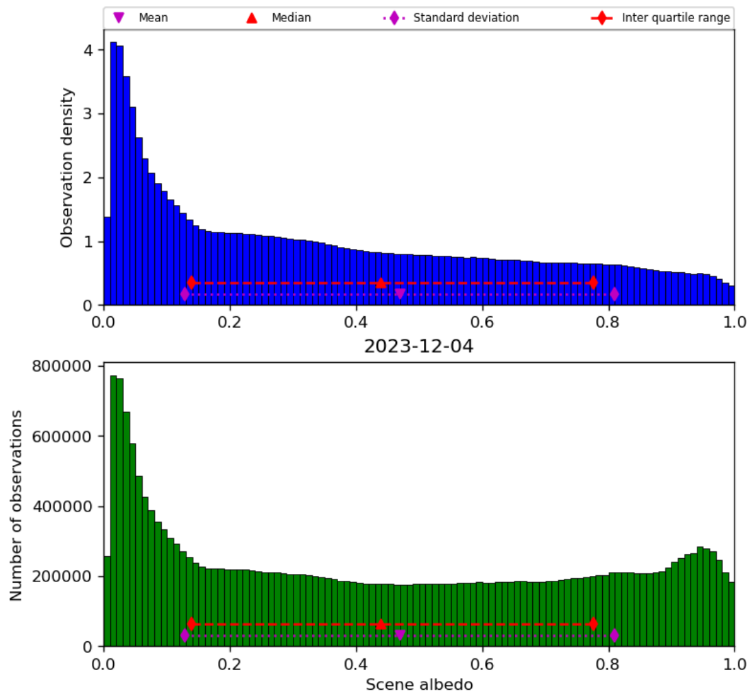
Figure 34: Histogram of “Scene albedo” for 2023-12-04 to 2023-12-05
