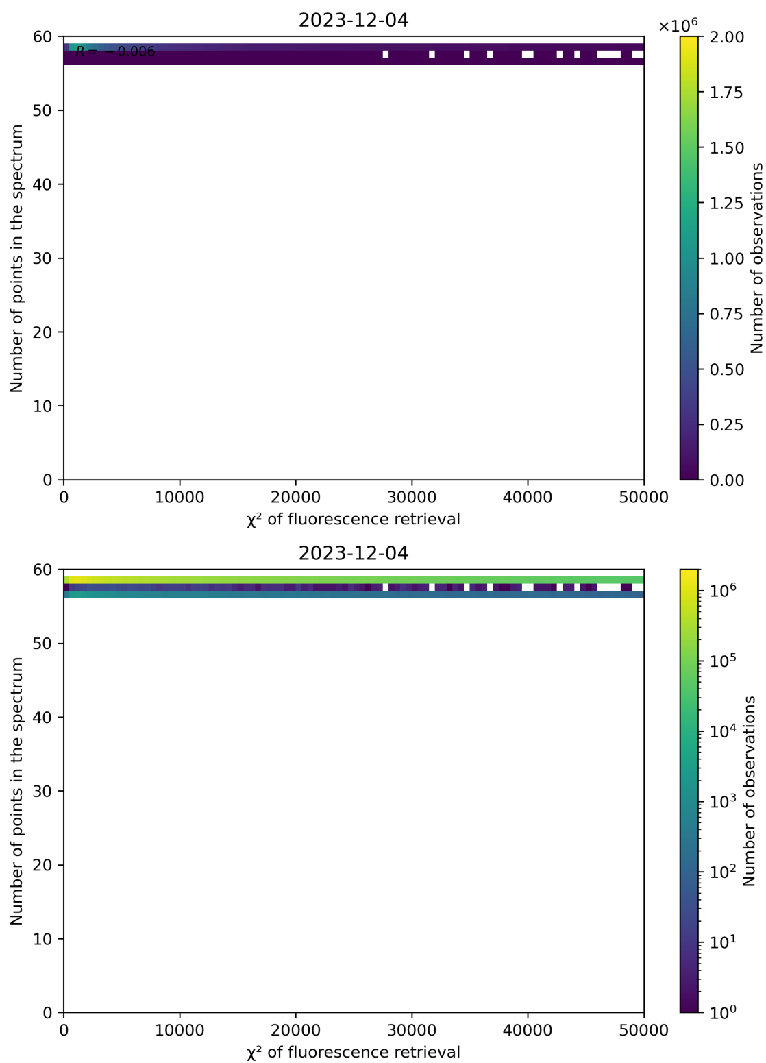
Figure 68: Scatter density plot of " \chi^2 of fluorescence retrieval" against "Number of points in the spectrum" for 2023-12-04 to 2023-12-05.
