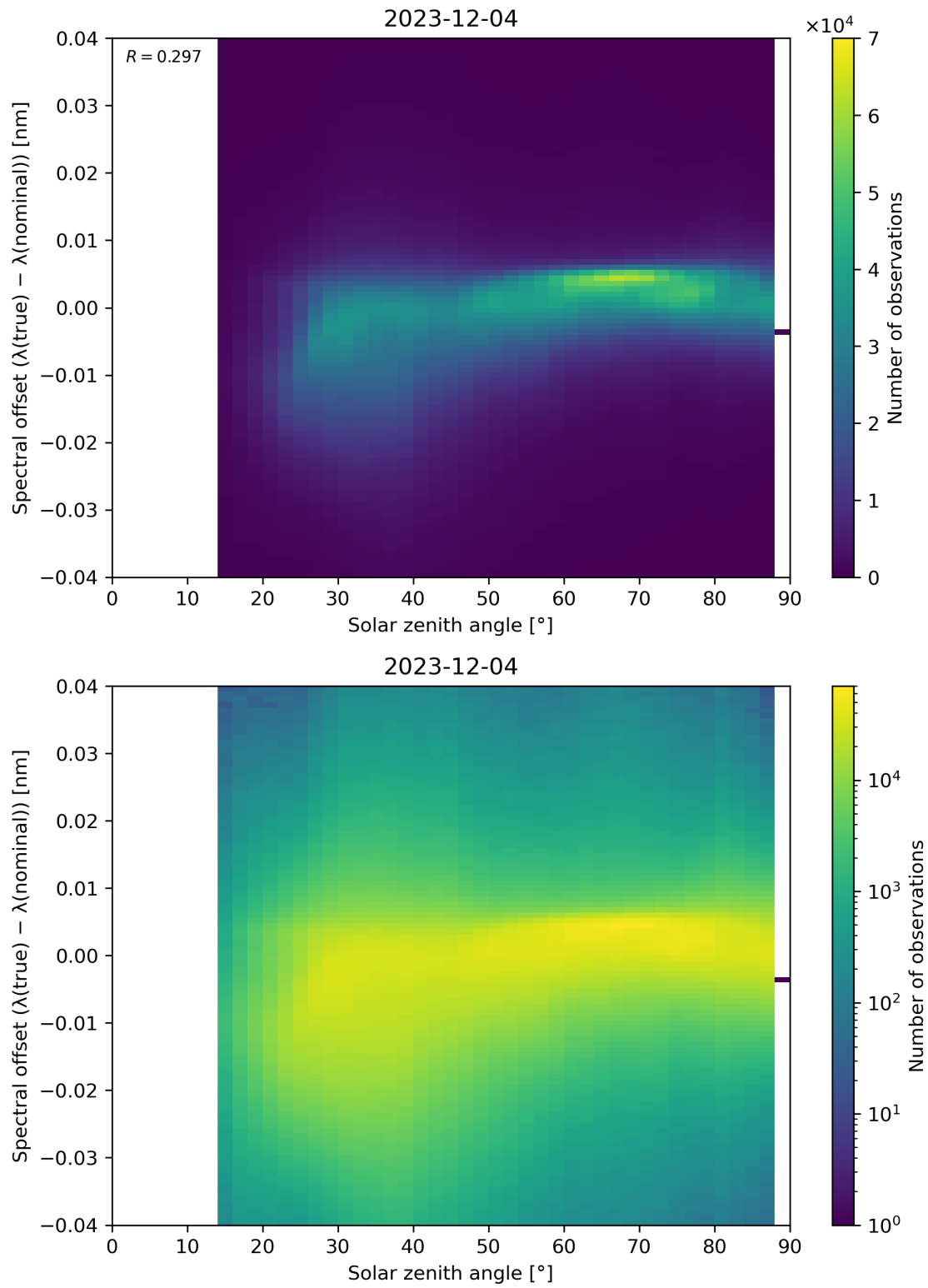
Figure 117: Scatter density plot of “Solar zenith angle” against “Spectral offset ( \lambda(\text{true}) - \lambda(\text{nominal}) )” for 2023-12-04 to 2023-12-05.
