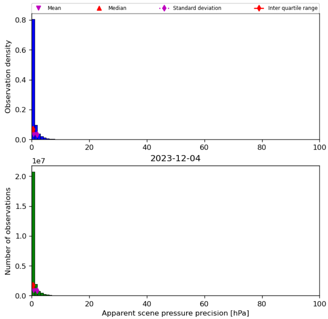
Figure 37: Histogram of “Apparent scene pressure precision” for 2023-12-04 to 2023-12-05
