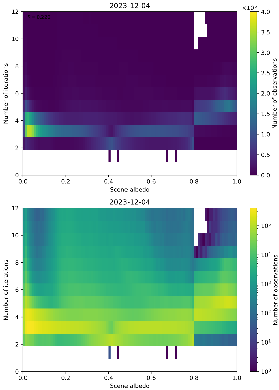
Figure 105: Scatter density plot of “Scene albedo” against “Number of iterations” for 2023-12-04 to 2023-12-05.
