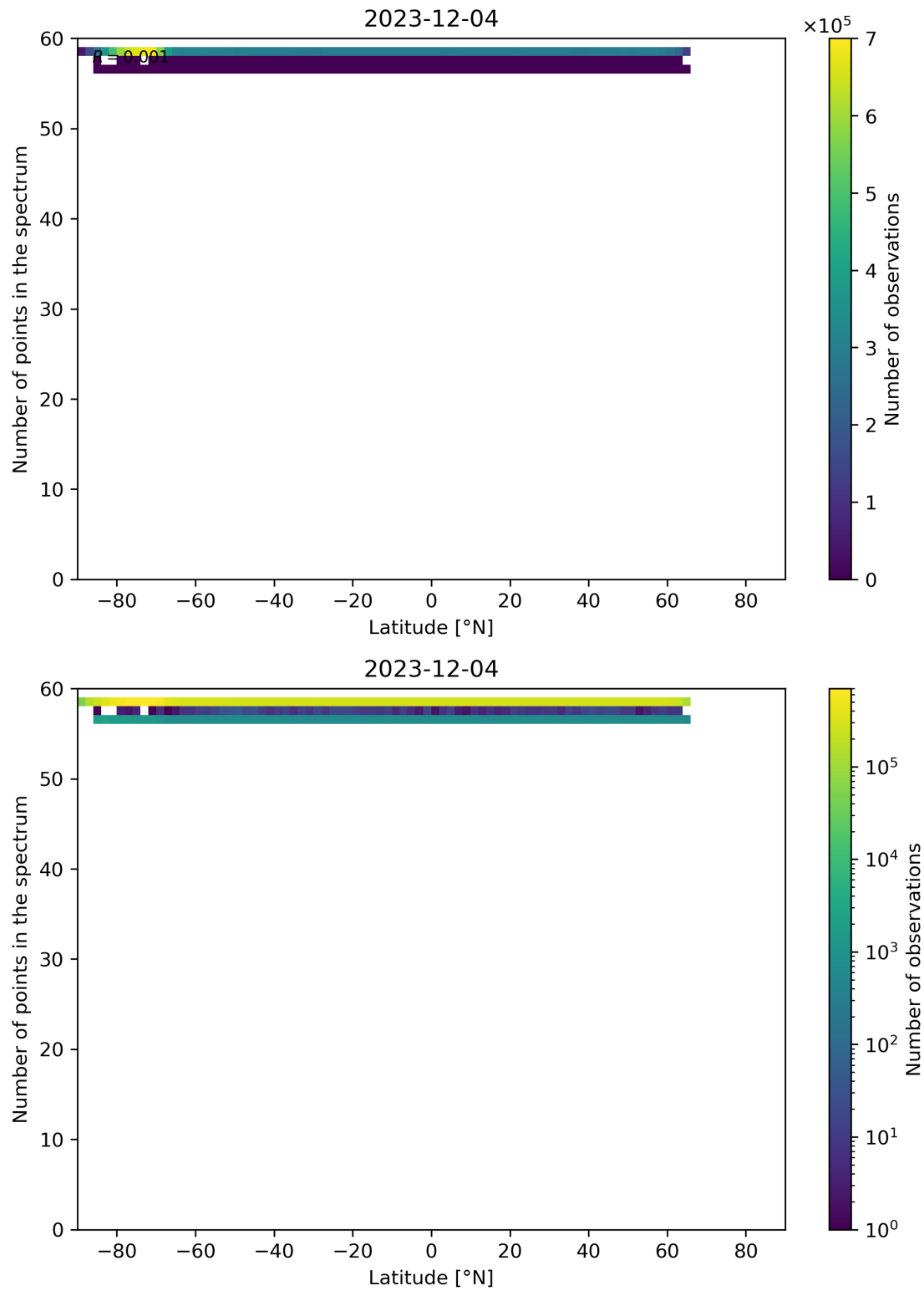
Figure 94: Scatter density plot of “Latitude” against “Number of points in the spectrum” for 2023-12-04 to 2023-12-05.
