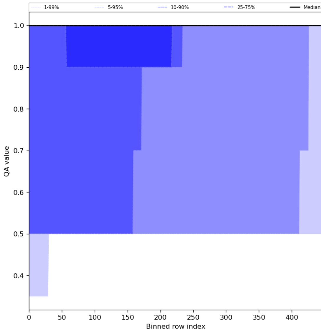
Figure 46: Along track statistics of “QA value” for 2023-12-04 to 2023-12-05
