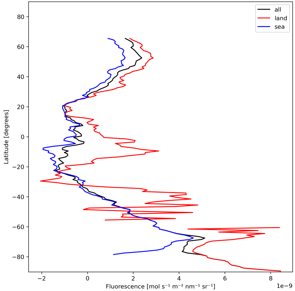
Figure 23: Zonal average of “Fluorescence” for 2023-12-04 to 2023-12-05.
