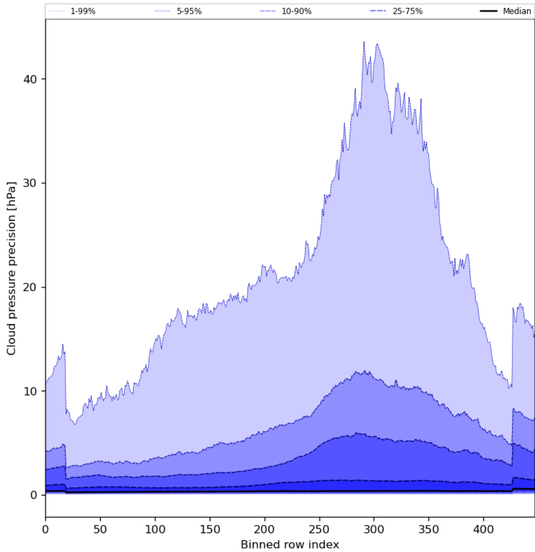
Figure 48: Along track statistics of “Cloud pressure precision” for 2023-12-04 to 2023-12-05
