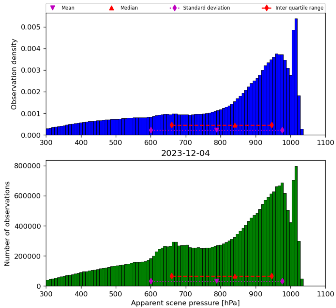
Figure 36: Histogram of “Apparent scene pressure” for 2023-12-04 to 2023-12-05
