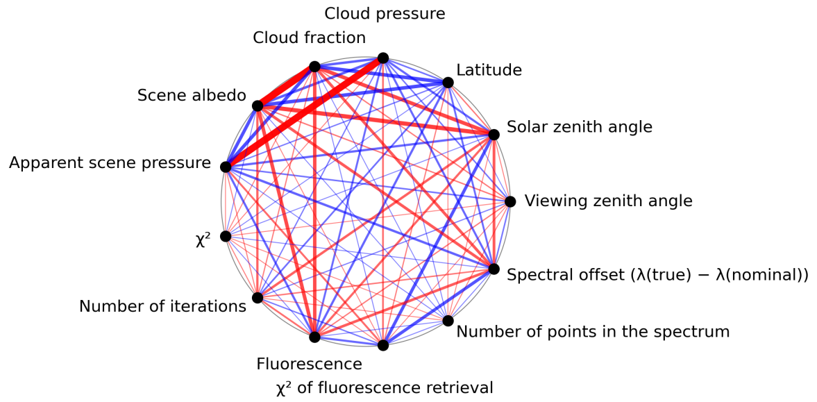
Figure 1: Map of correlation graph for 2023-12-04 to 2023-12-05.
