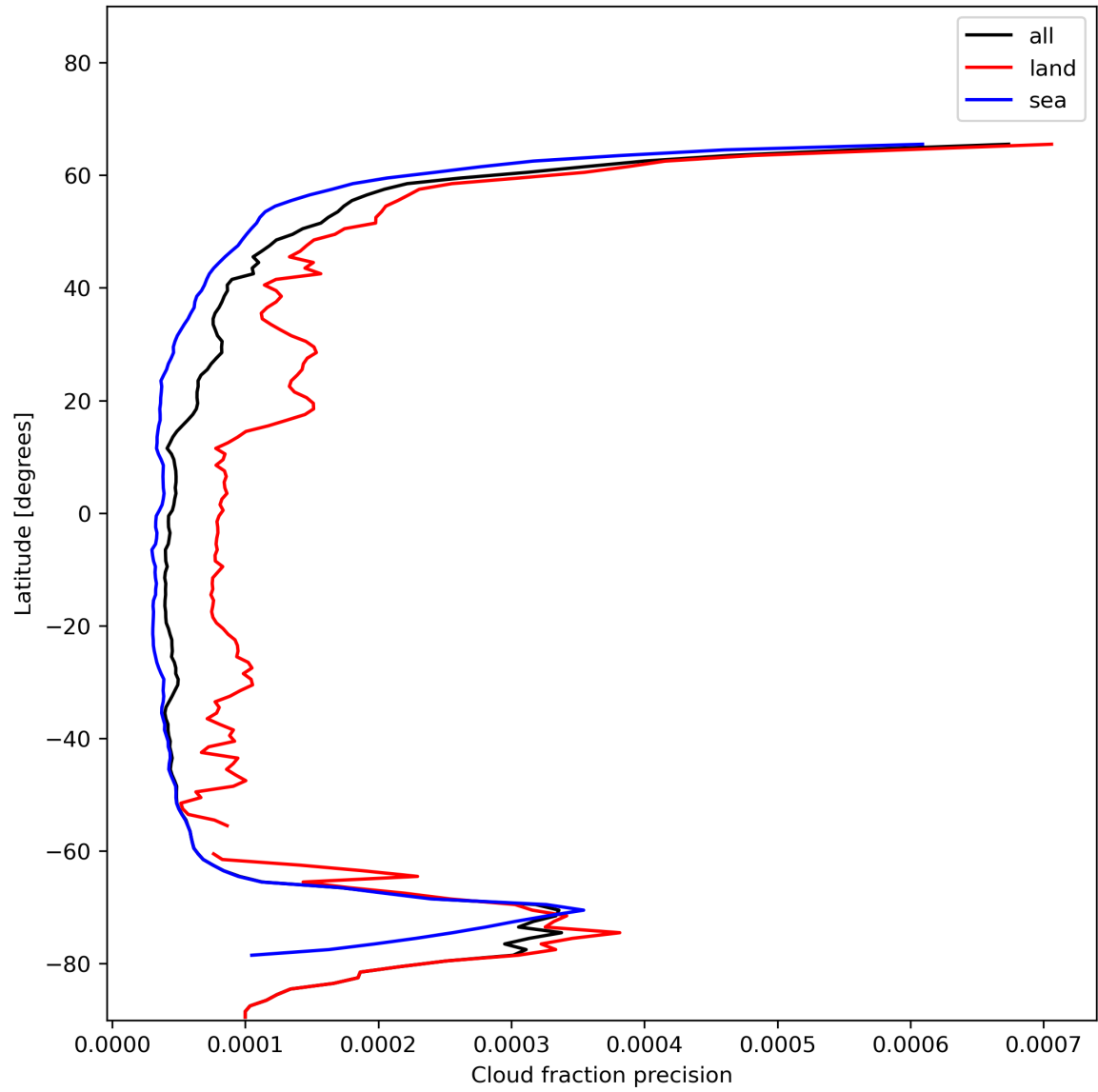
Figure 16: Zonal average of “Cloud fraction precision” for 2023-12-04 to 2023-12-05.
