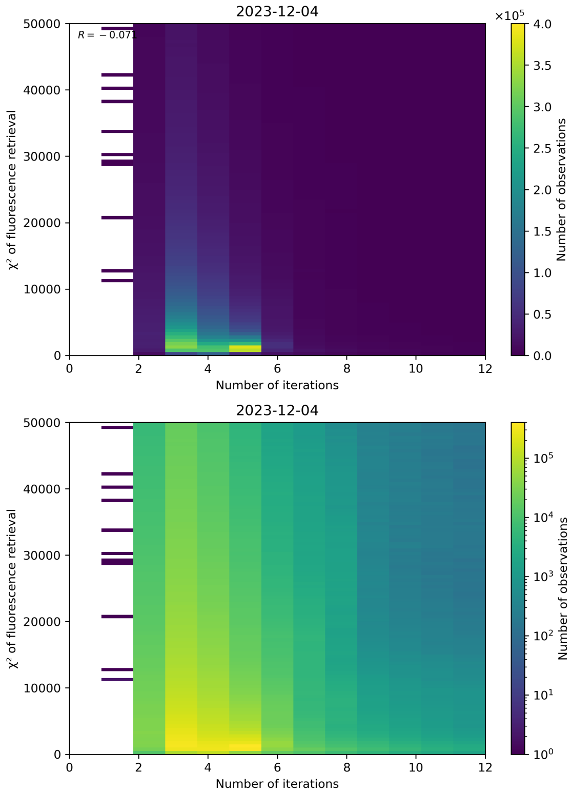
Figure 97: Scatter density plot of “Number of iterations” against “ \chi^2 of fluorescence retrieval” for 2023-12-04 to 2023-12-05.
