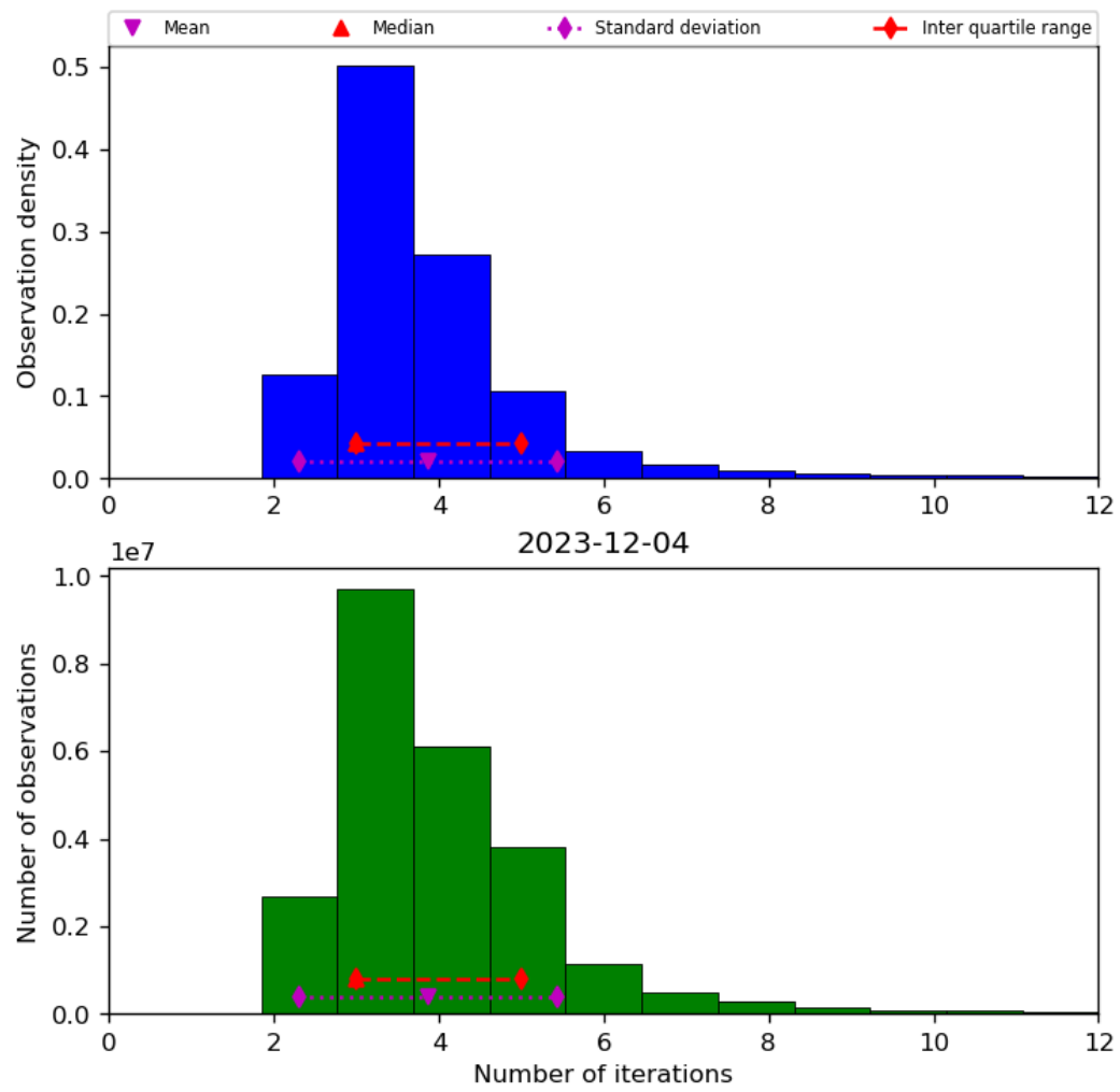
Figure 39: Histogram of “Number of iterations” for 2023-12-04 to 2023-12-05
