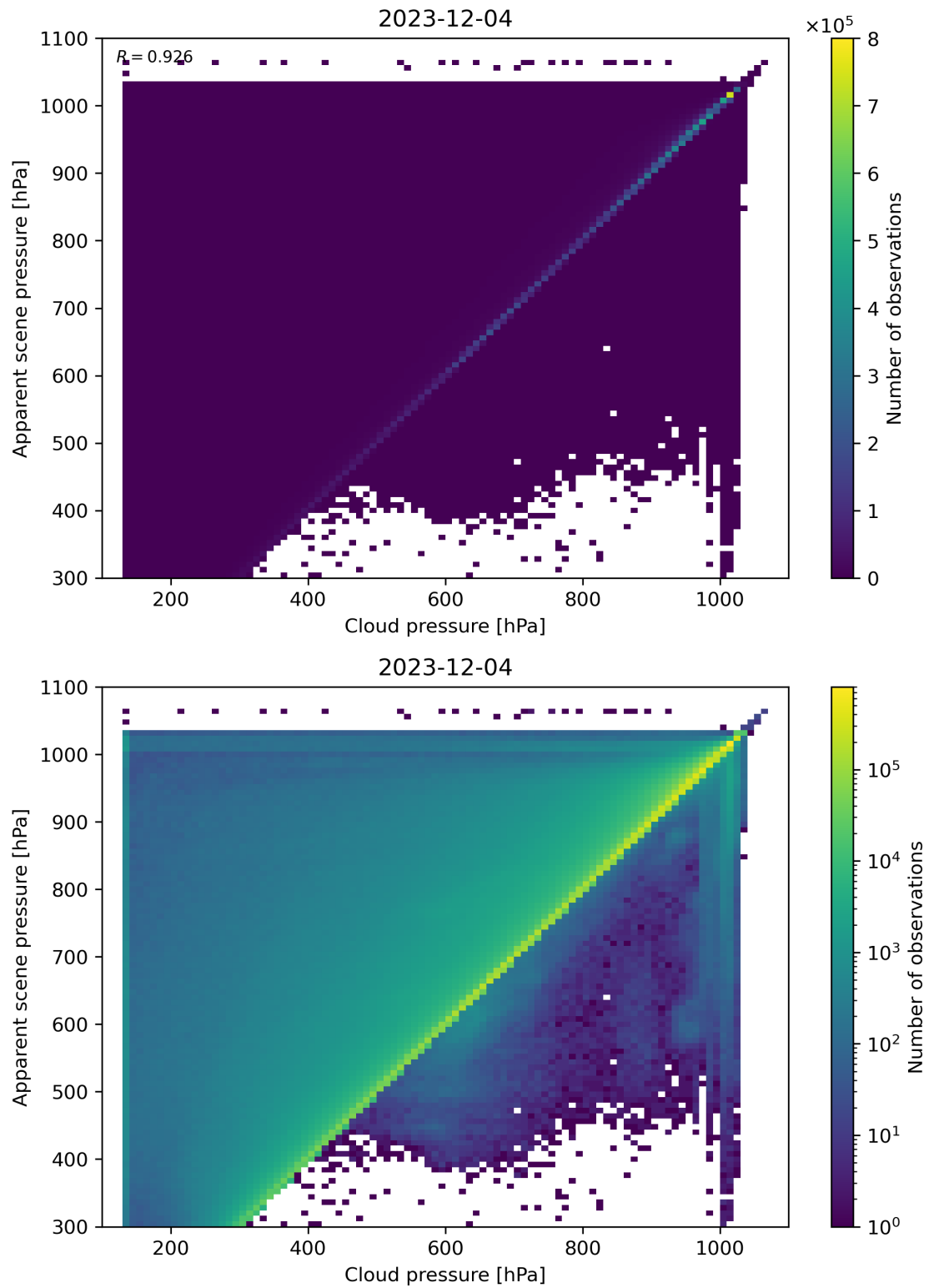
Figure 77: Scatter density plot of “Cloud pressure” against “Apparent scene pressure” for 2023-12-04 to 2023-12-05.
