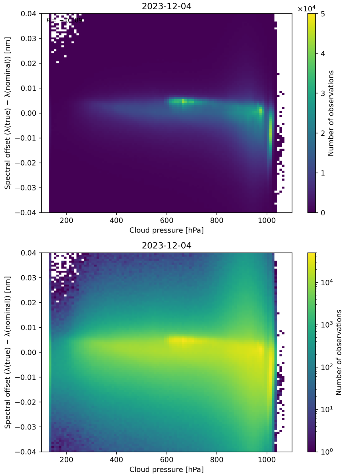
Figure 84: Scatter density plot of “Cloud pressure” against “Spectral offset ( \lambda(\text{true}) - \lambda(\text{nominal}) )” for 2023-12-04 to 2023-12-05.
