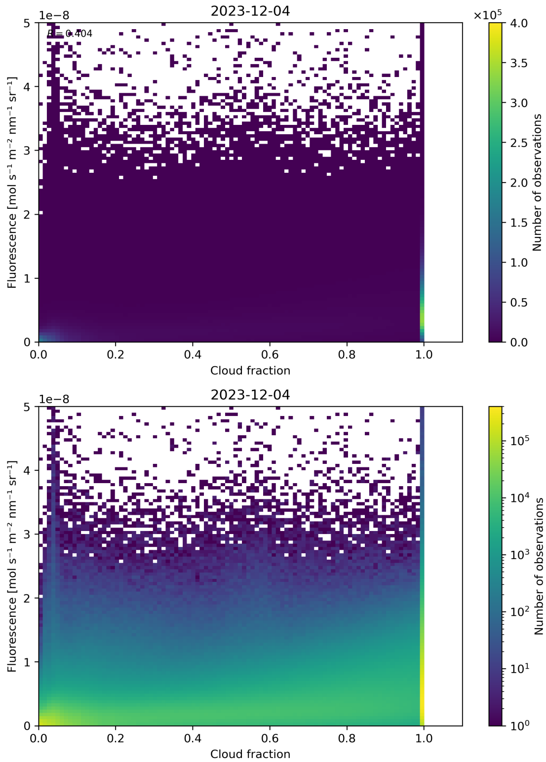
Figure 72: Scatter density plot of “Cloud fraction” against “Fluorescence” for 2023-12-04 to 2023-12-05.
