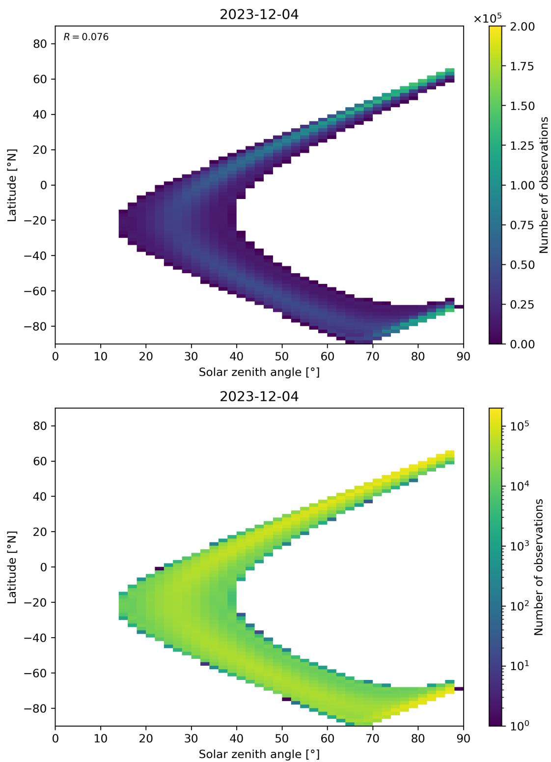
Figure 113: Scatter density plot of “Solar zenith angle” against “Latitude” for 2023-12-04 to 2023-12-05.
