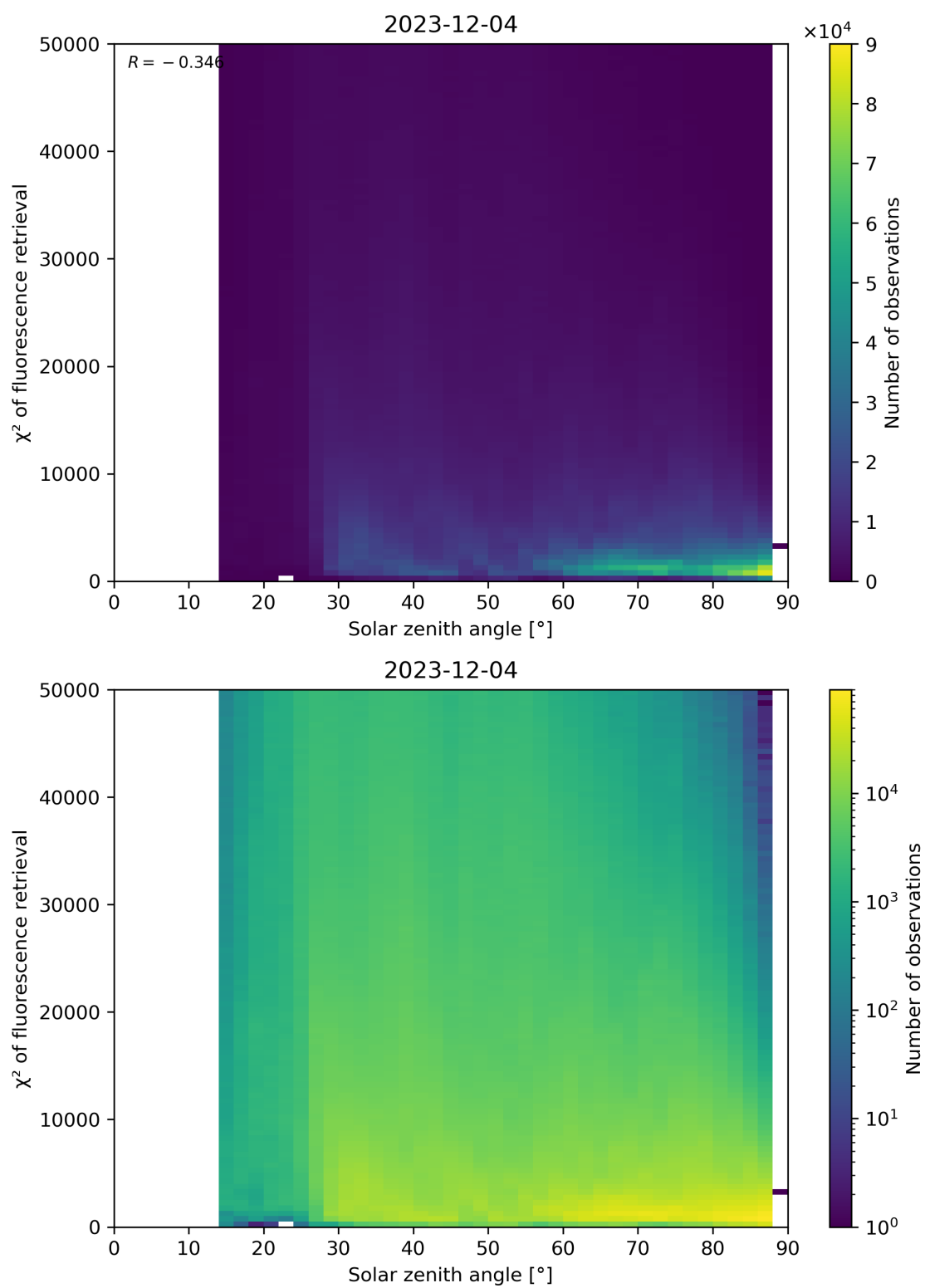
Figure 109: Scatter density plot of “Solar zenith angle” against “ \chi^2 of fluorescence retrieval” for 2023-12-04 to 2023-12-05.
