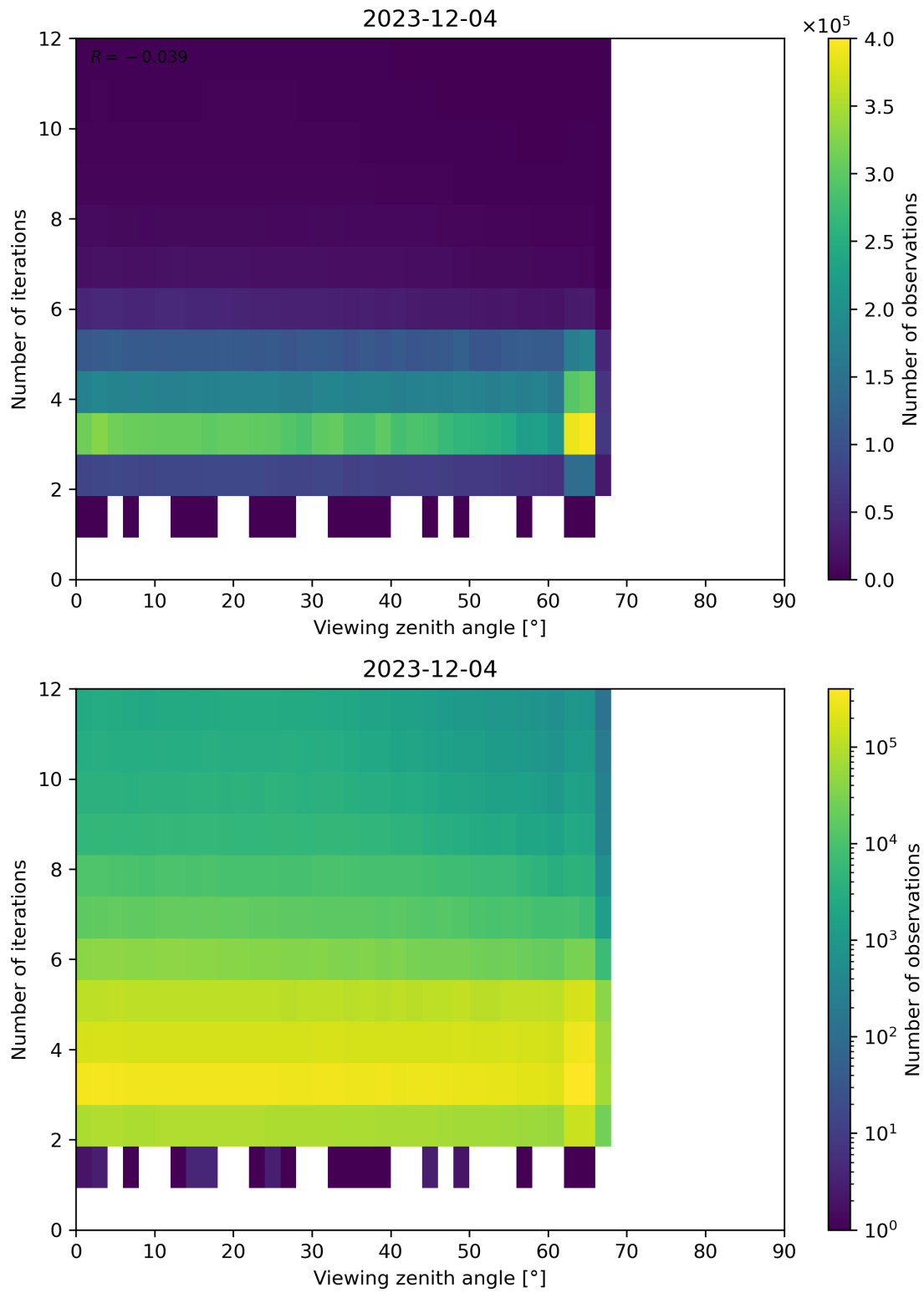
Figure 124: Scatter density plot of “Viewing zenith angle” against “Number of iterations” for 2023-12-04 to 2023-12-05.
