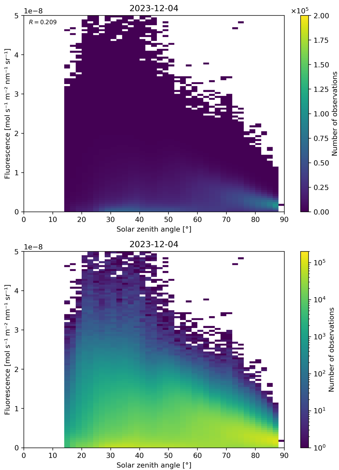
Figure 112: Scatter density plot of “Solar zenith angle” against “Fluorescence” for 2023-12-04 to 2023-12-05.
