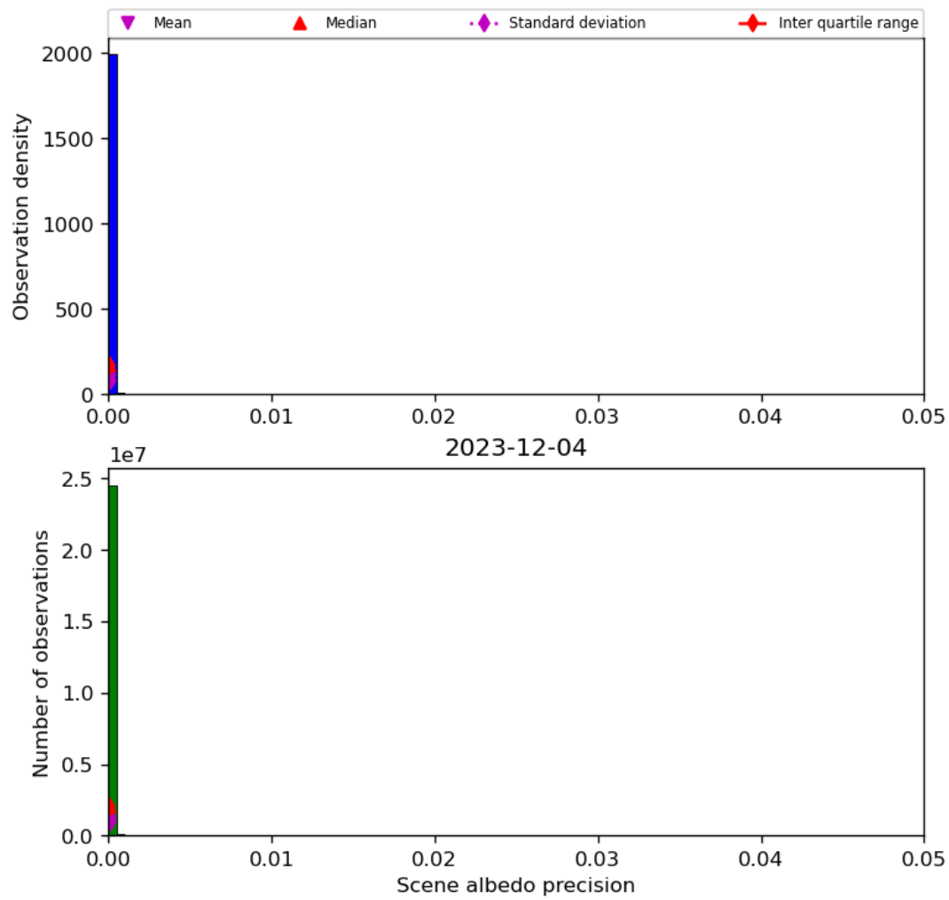
Figure 35: Histogram of “Scene albedo precision” for 2023-12-04 to 2023-12-05
