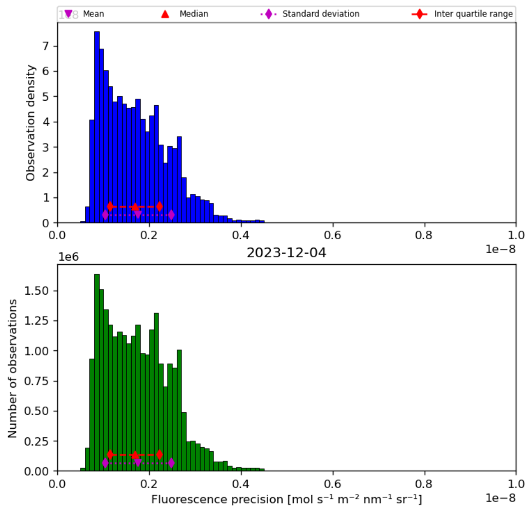
Figure 41: Histogram of “Fluorescence precision” for 2023-12-04 to 2023-12-05
