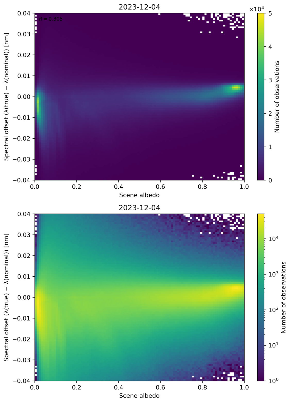
Figure 107: Scatter density plot of “Scene albedo” against “Spectral offset ( \lambda(\text{true}) - \lambda(\text{nominal}) )” for 2023-12-04 to 2023-12-05.
