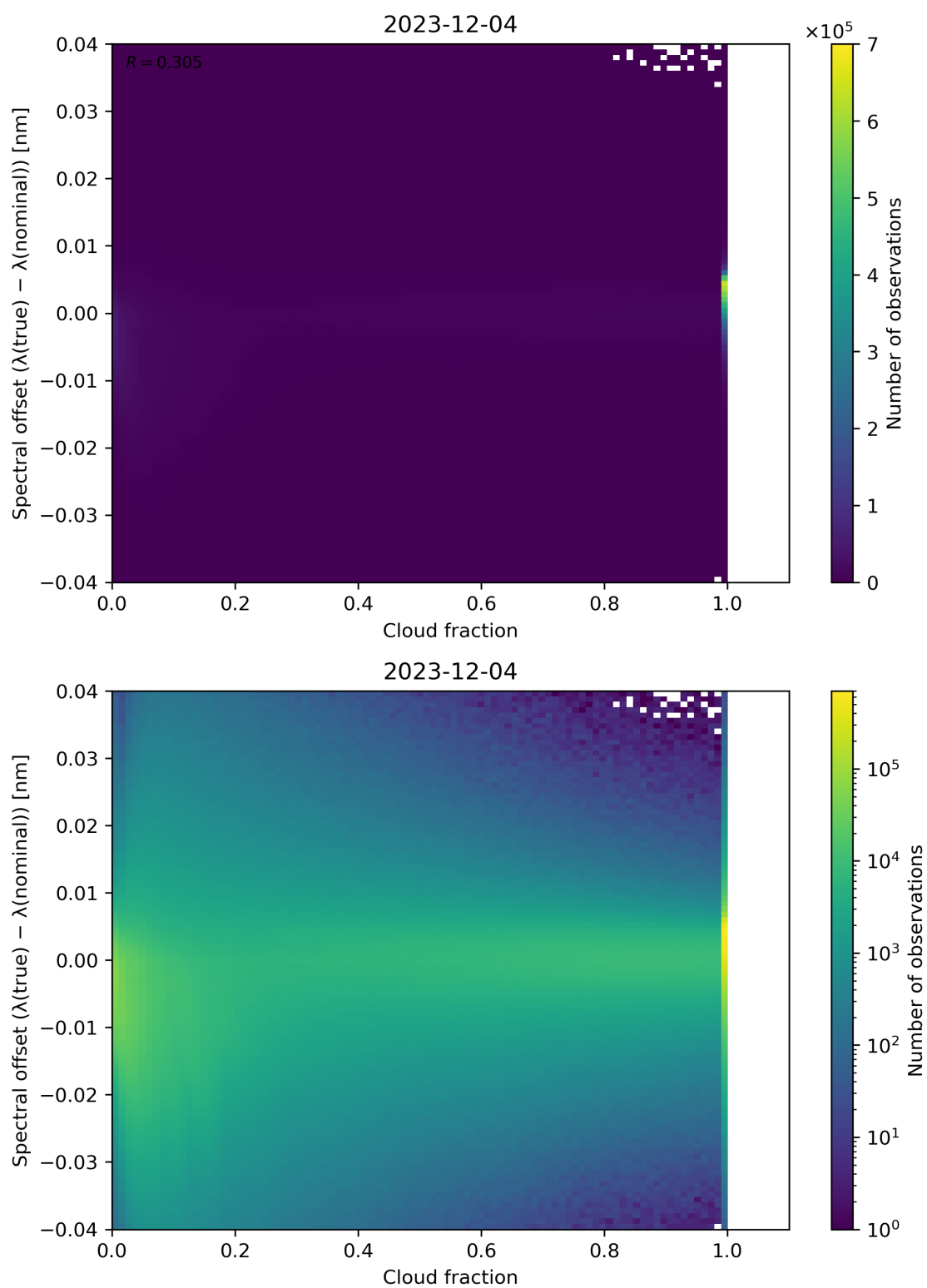
Figure 76: Scatter density plot of “Cloud fraction” against “Spectral offset ( \lambda(\text{true}) - \lambda(\text{nominal}) )” for 2023-12-04 to 2023-12-05.
