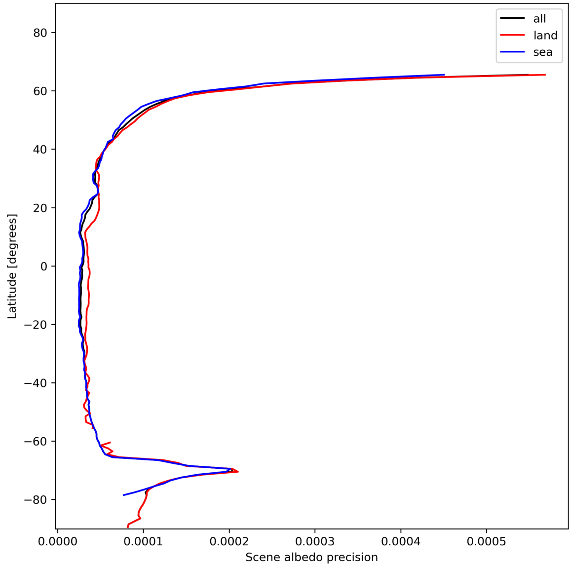
Figure 18: Zonal average of “Scene albedo precision” for 2023-12-04 to 2023-12-05.
