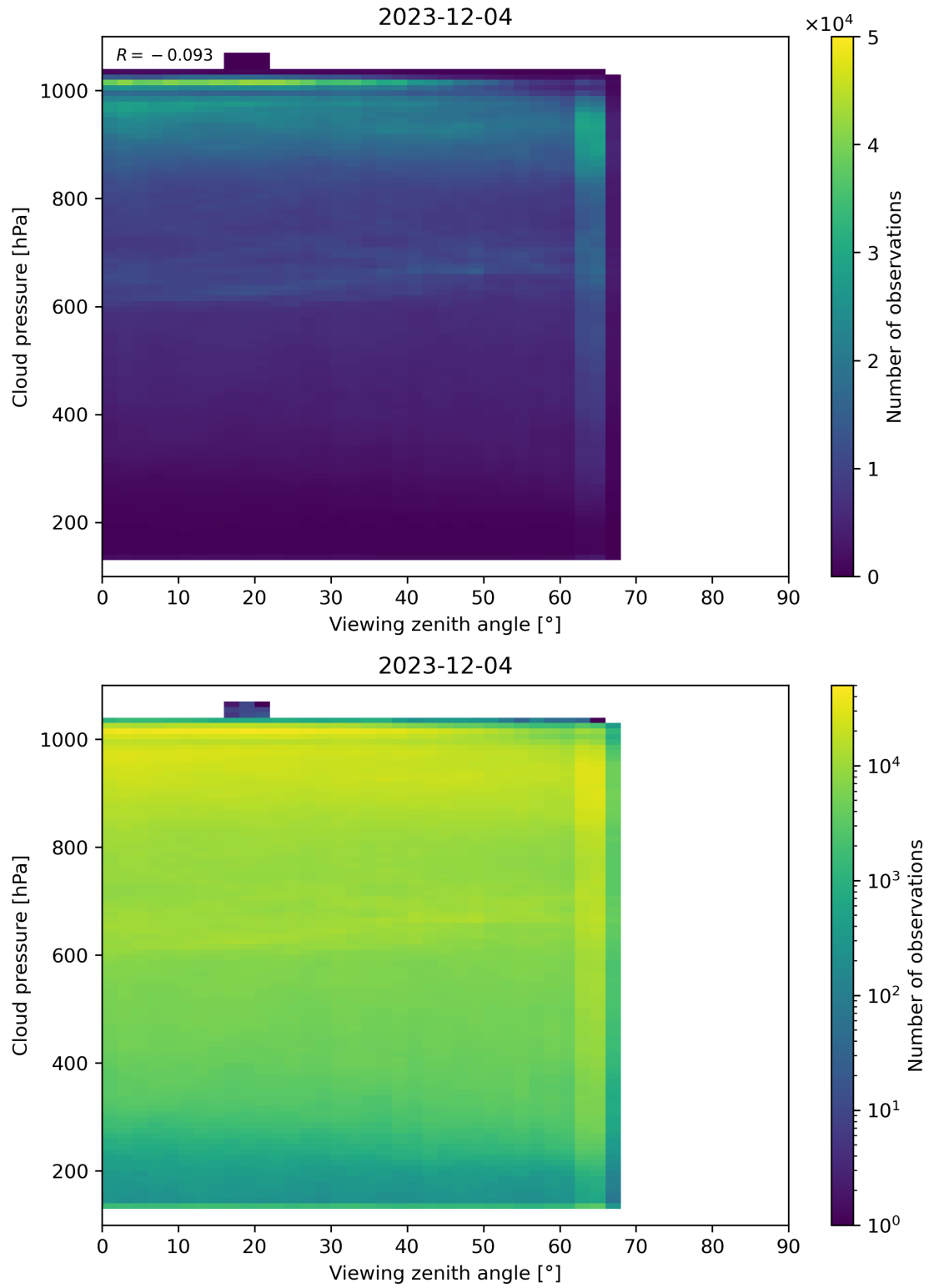
Figure 121: Scatter density plot of “Viewing zenith angle” against “Cloud pressure” for 2023-12-04 to 2023-12-05.
