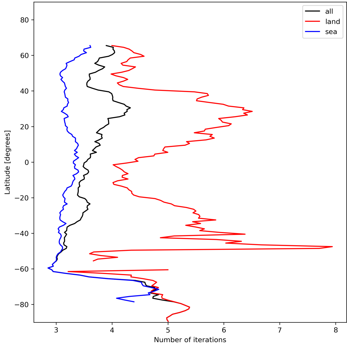
Figure 22: Zonal average of “Number of iterations” for 2023-12-04 to 2023-12-05.
