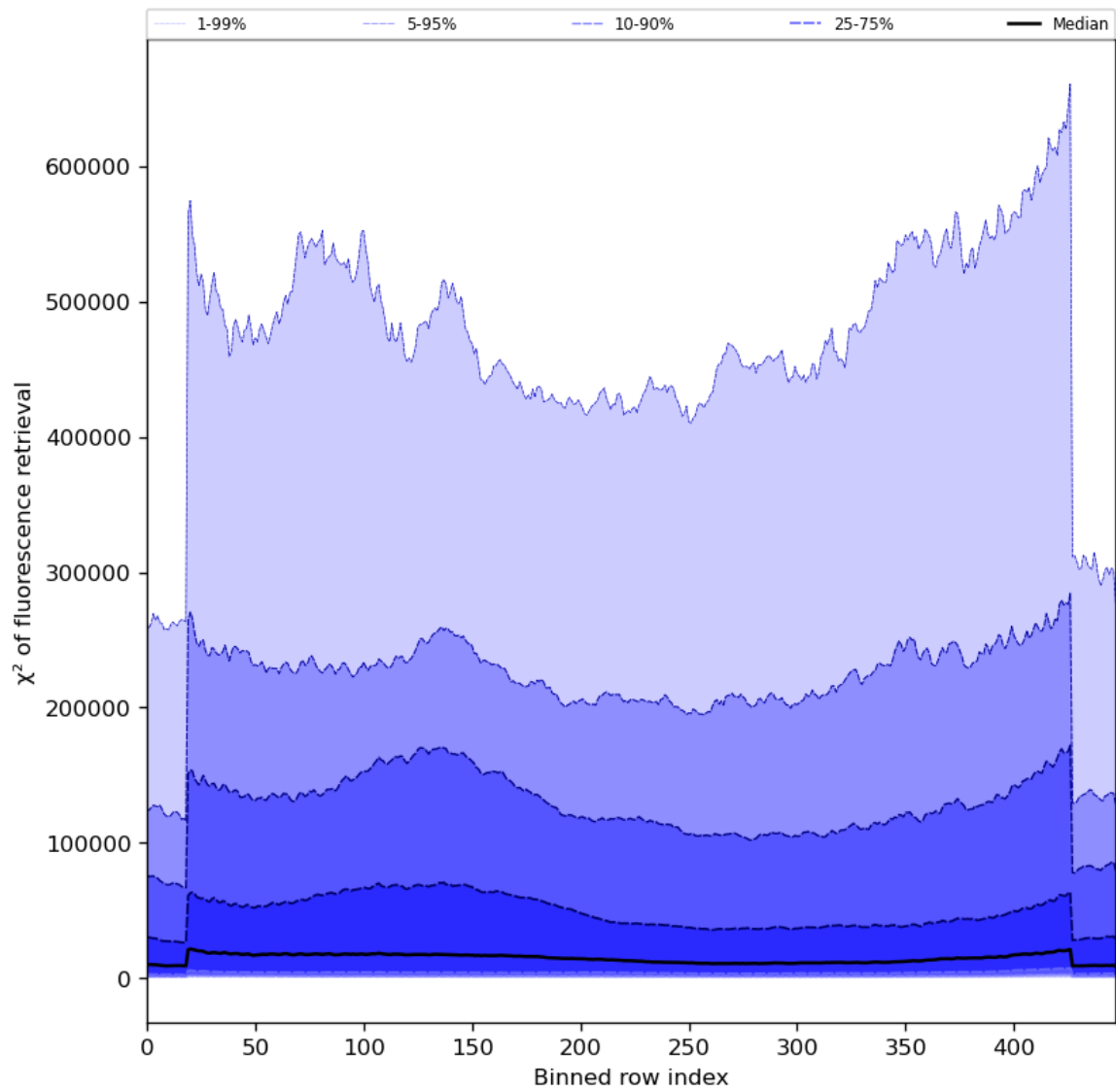
Figure 59: Along track statistics of “ \chi^2 of fluorescence retrieval” for 2023-12-04 to 2023-12-05
