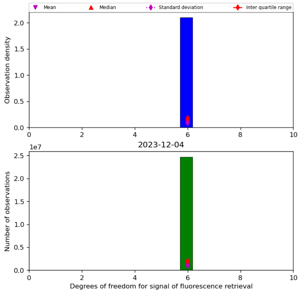
Figure 43: Histogram of “Degrees of freedom for signal of fluorescence retrieval” for 2023-12-04 to 2023-12-05
