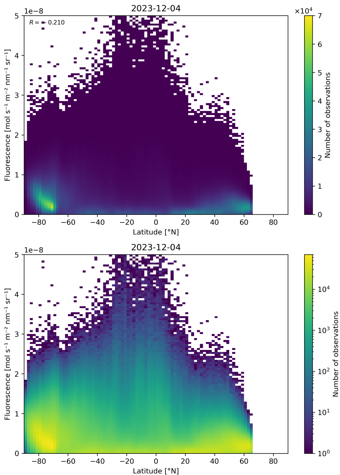
Figure 92: Scatter density plot of “Latitude” against “Fluorescence” for 2023-12-04 to 2023-12-05.
