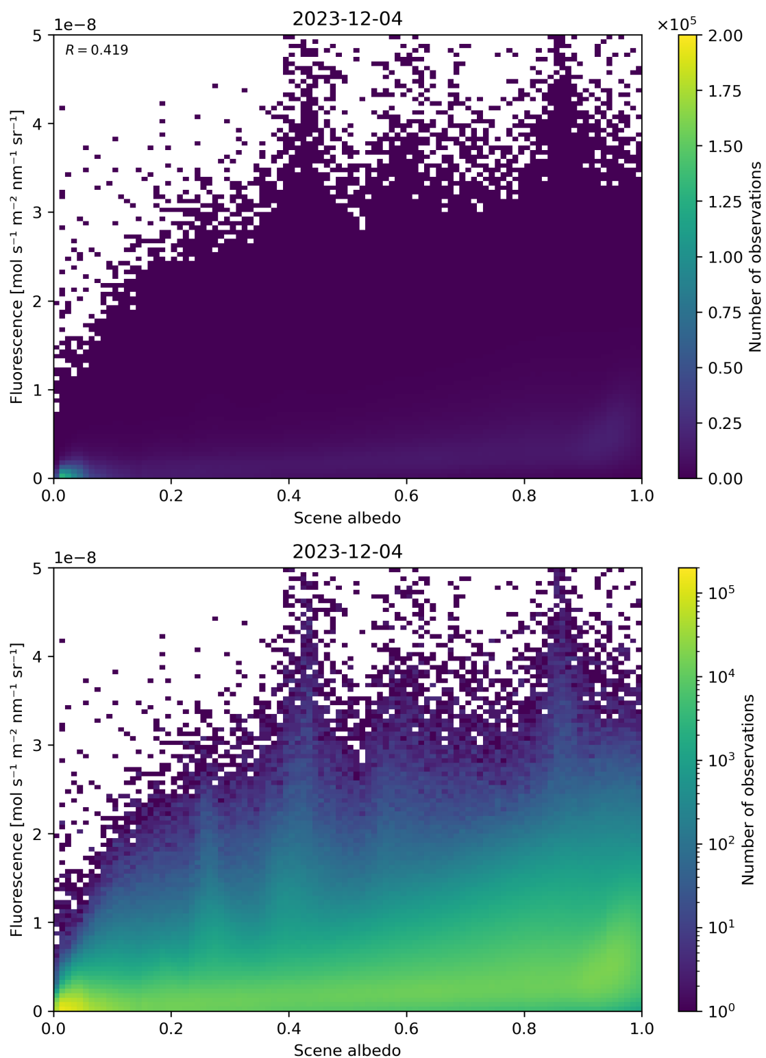
Figure 104: Scatter density plot of “Scene albedo” against “Fluorescence” for 2023-12-04 to 2023-12-05.
