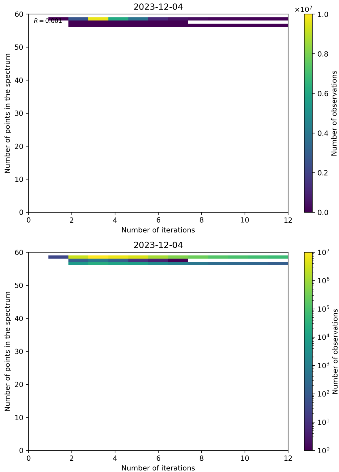
Figure 99: Scatter density plot of “Number of iterations” against “Number of points in the spectrum” for 2023-12-04 to 2023-12-05.
