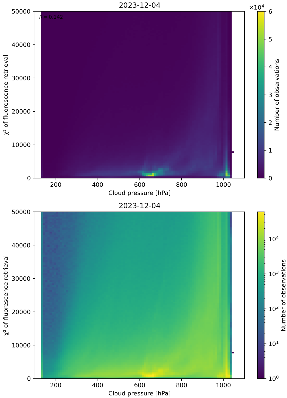
Figure 78: Scatter density plot of “Cloud pressure” against “ \chi^2 of fluorescence retrieval” for 2023-12-04 to 2023-12-05.
