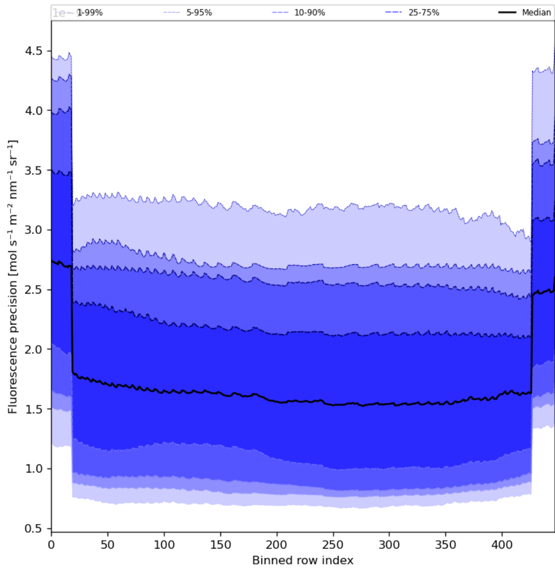
Figure 58: Along track statistics of “Fluorescence precision” for 2023-12-04 to 2023-12-05
