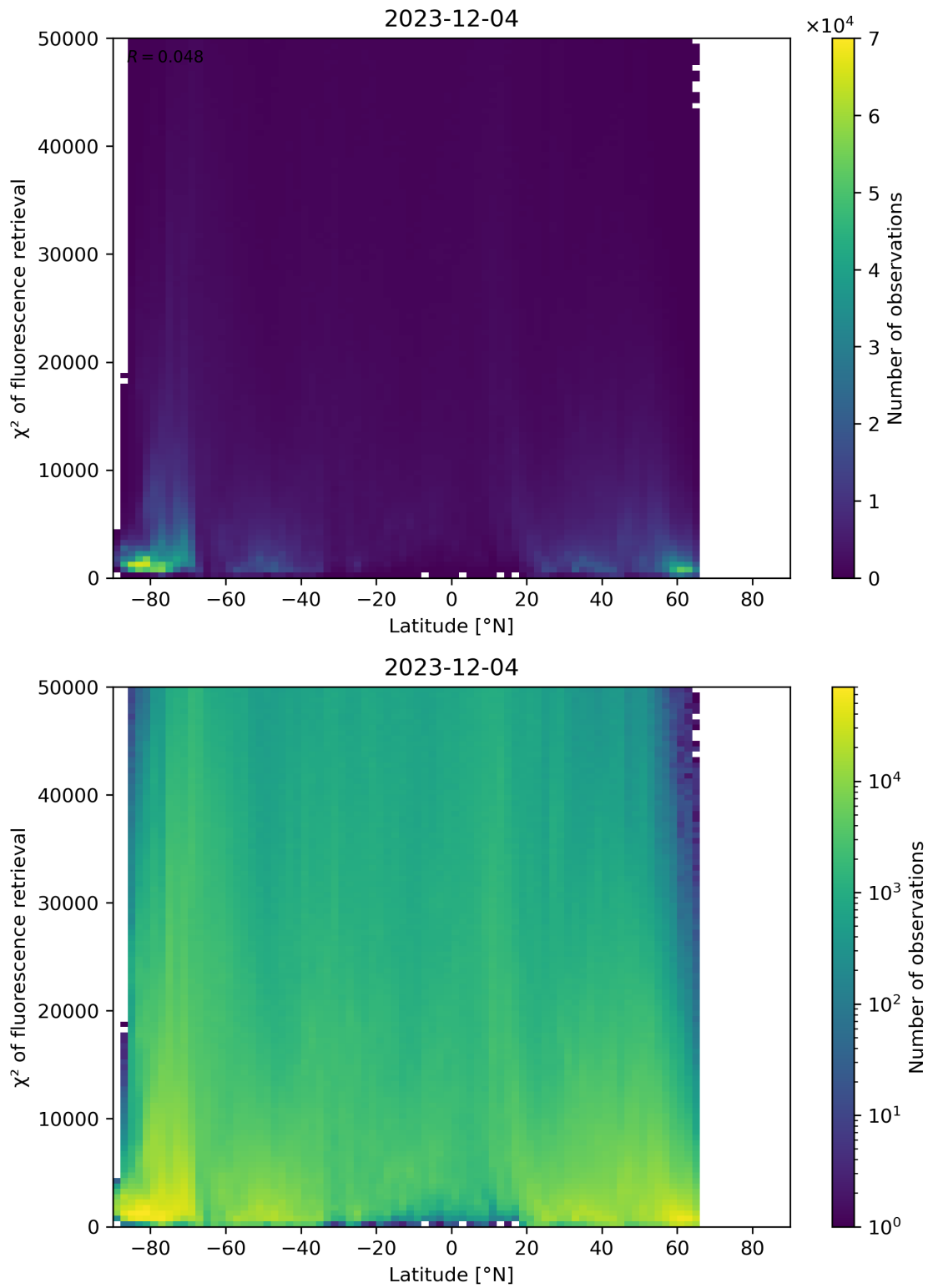
Figure 89: Scatter density plot of “Latitude” against “ \chi^2 of fluorescence retrieval” for 2023-12-04 to 2023-12-05.
