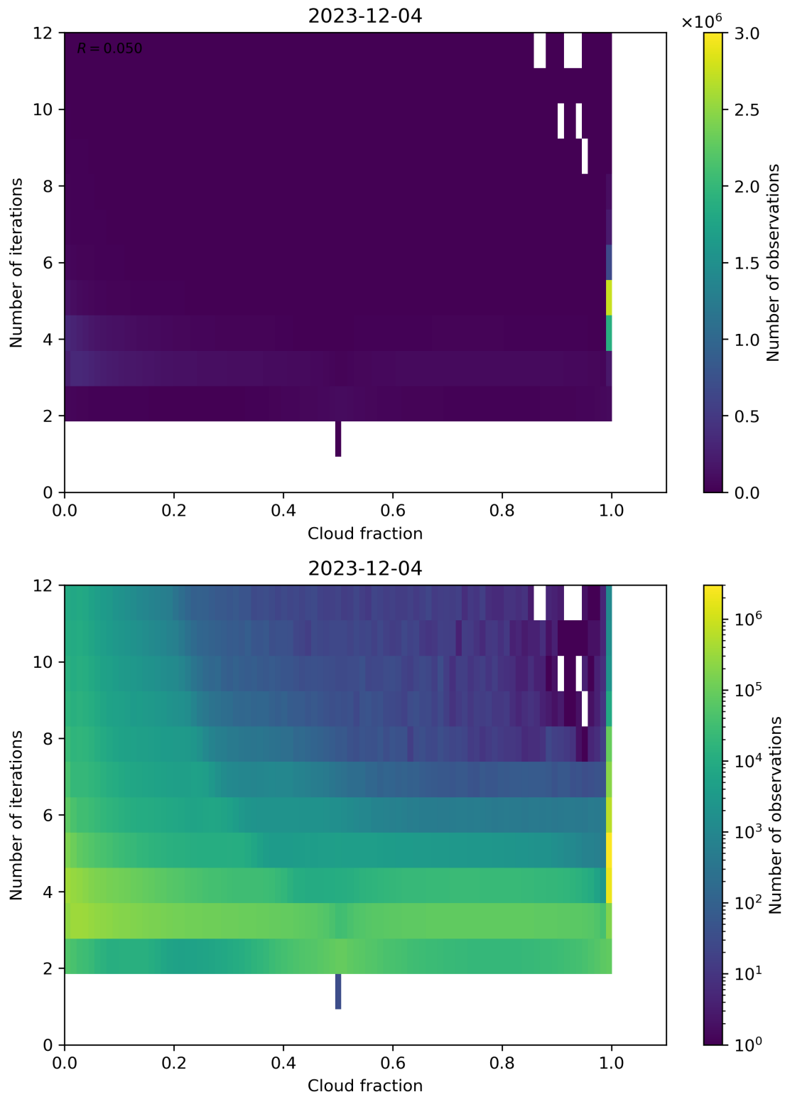
Figure 73: Scatter density plot of “Cloud fraction” against “Number of iterations” for 2023-12-04 to 2023-12-05.
