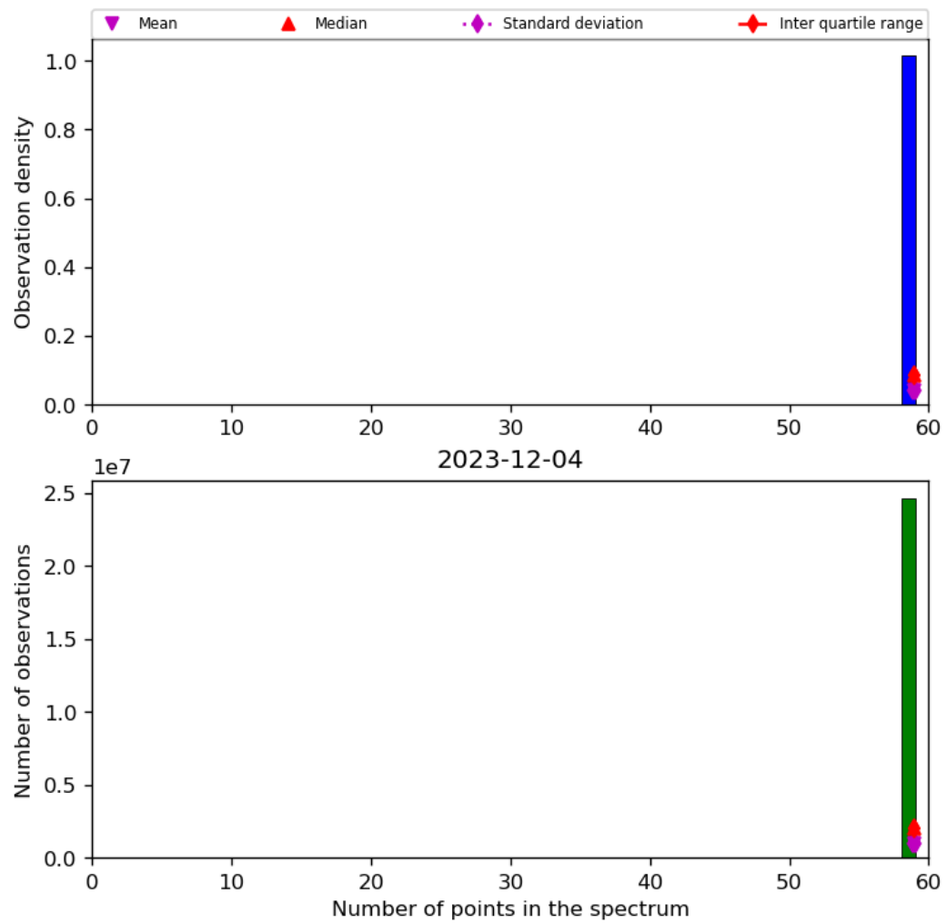
Figure 44: Histogram of “Number of points in the spectrum” for 2023-12-04 to 2023-12-05
