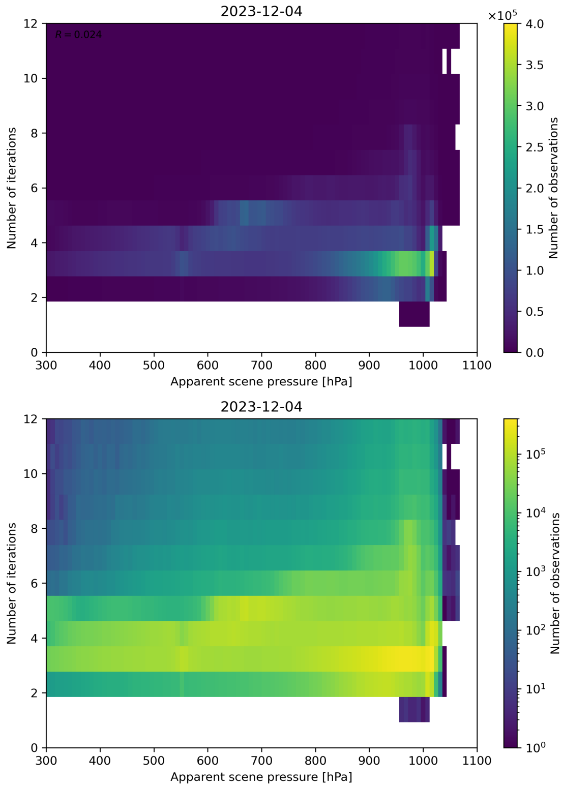
Figure 65: Scatter density plot of “Apparent scene pressure” against “Number of iterations” for 2023-12-04 to 2023-12-05.
