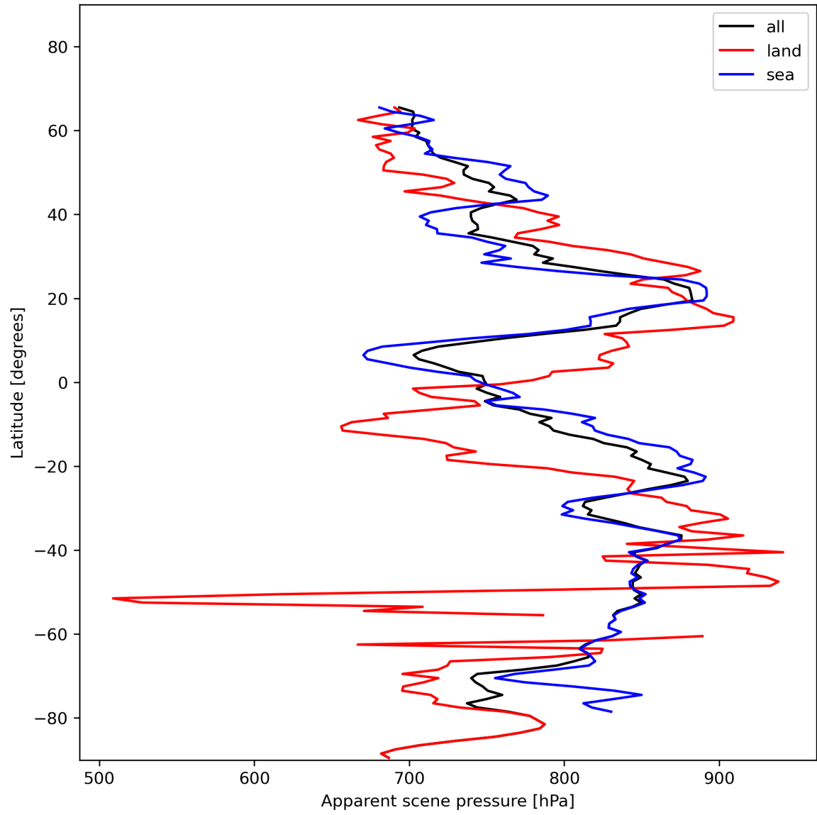
Figure 19: Zonal average of “Apparent scene pressure” for 2023-12-04 to 2023-12-05.
