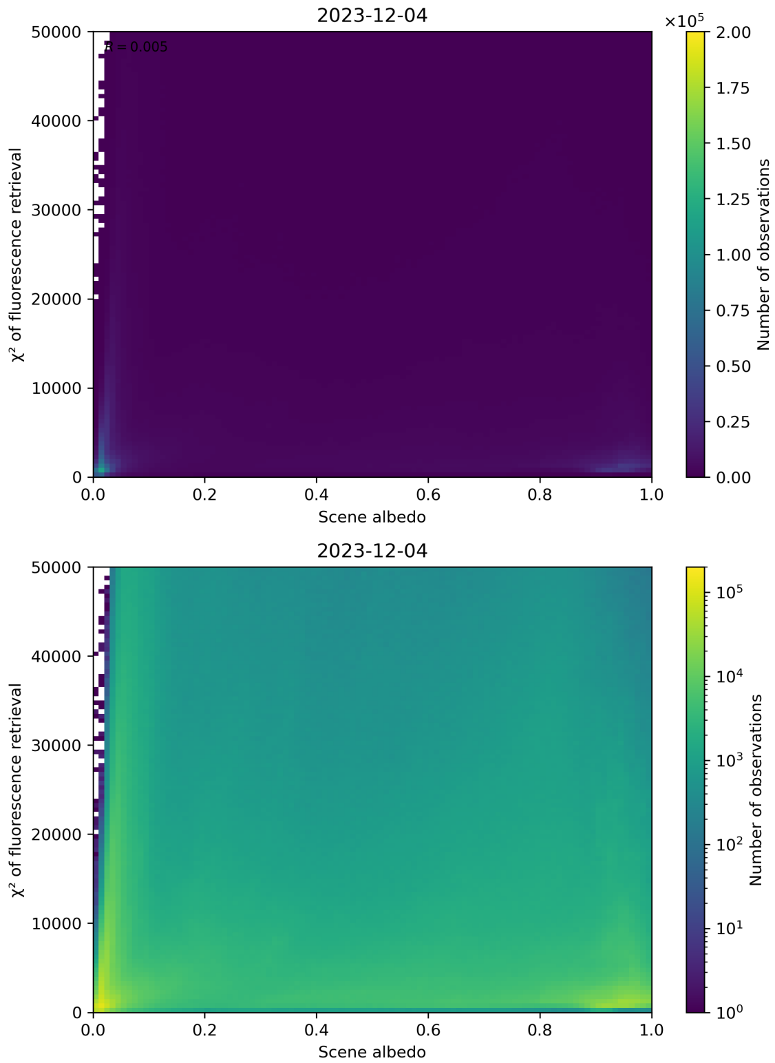
Figure 103: Scatter density plot of “Scene albedo” against “ \chi^2 of fluorescence retrieval” for 2023-12-04 to 2023-12-05.
