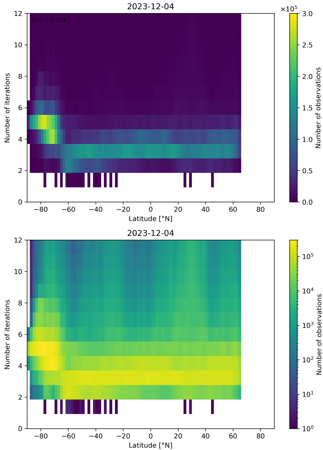
Figure 93: Scatter density plot of “Latitude” against “Number of iterations” for 2023-12-04 to 2023-12-05.
