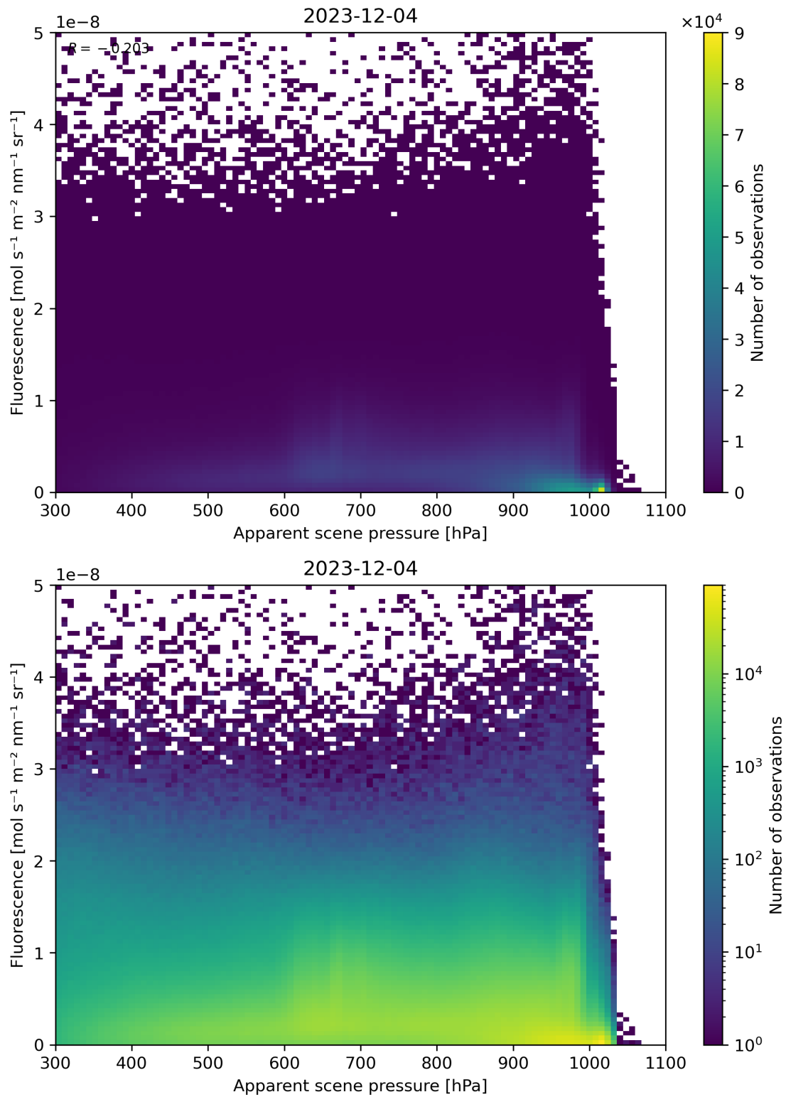
Figure 64: Scatter density plot of “Apparent scene pressure” against “Fluorescence” for 2023-12-04 to 2023-12-05.
