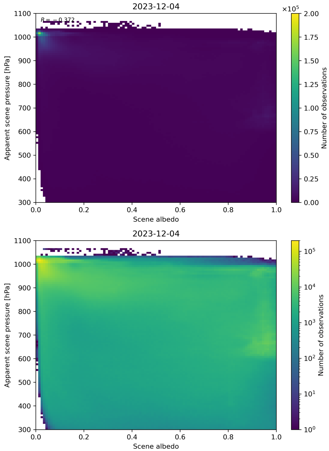
Figure 102: Scatter density plot of “Scene albedo” against “Apparent scene pressure” for 2023-12-04 to 2023-12-05.
