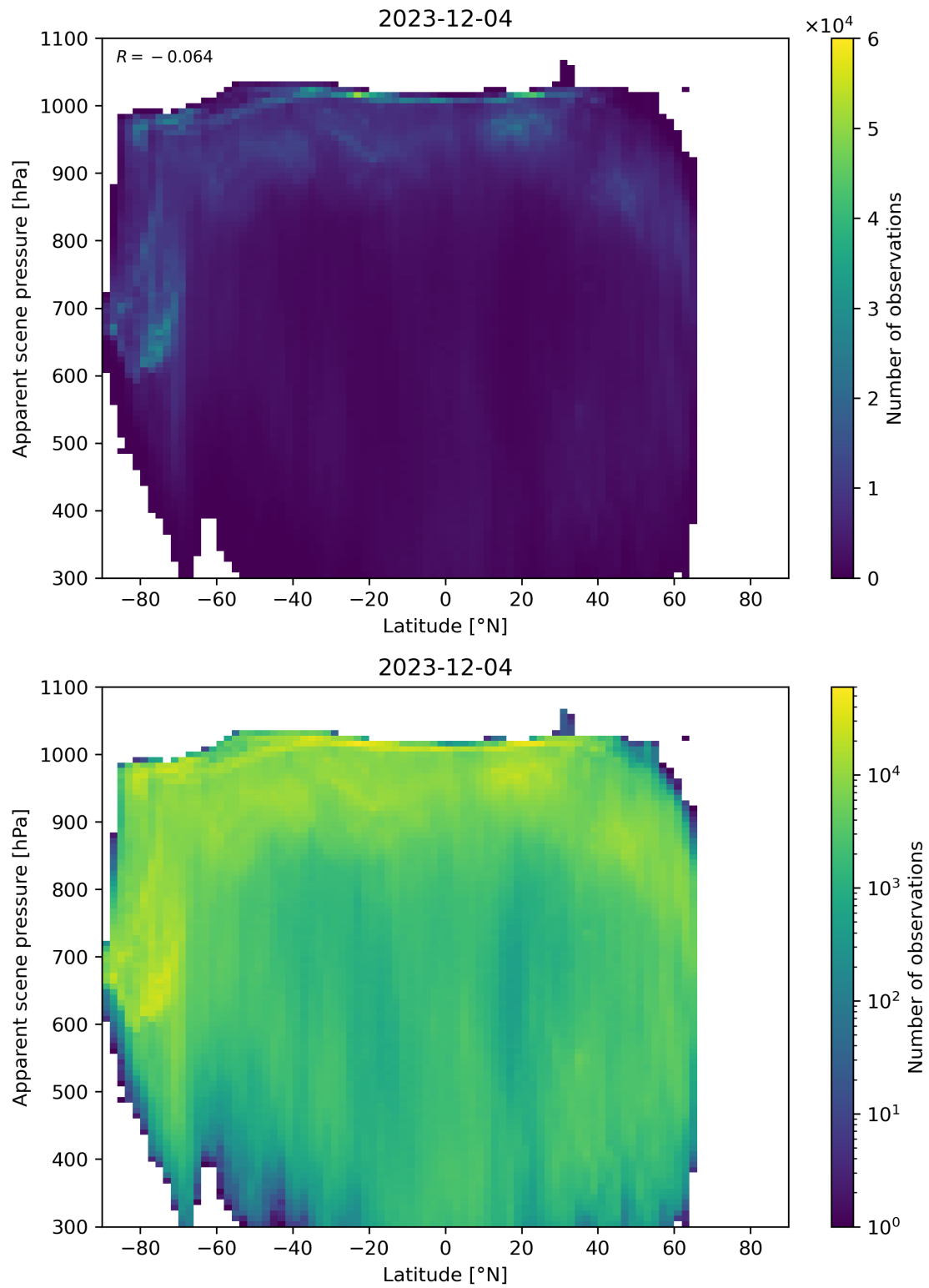
Figure 88: Scatter density plot of “Latitude” against “Apparent scene pressure” for 2023-12-04 to 2023-12-05.
