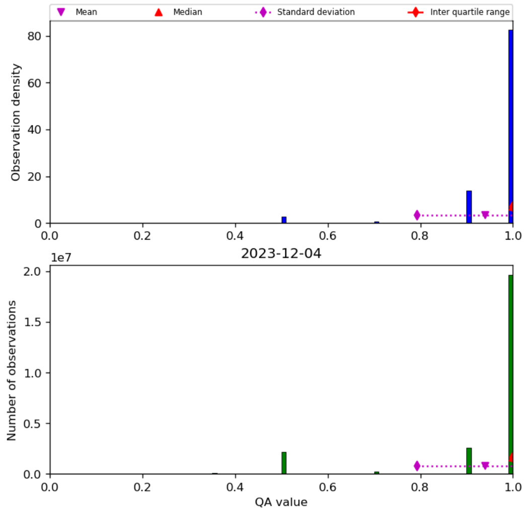
Figure 29: Histogram of “QA value” for 2023-12-04 to 2023-12-05
