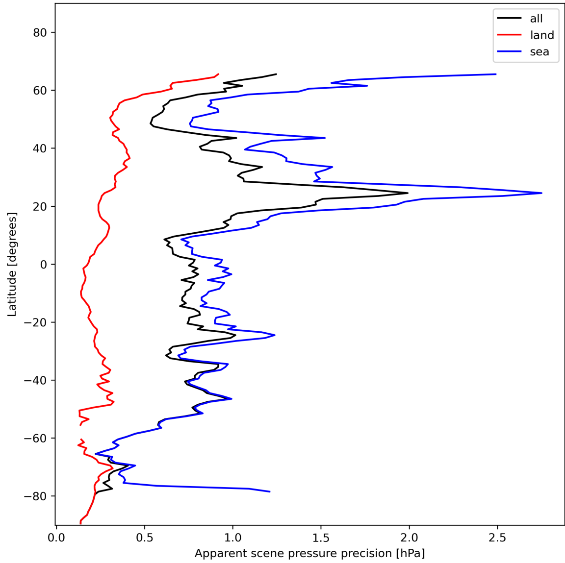
Figure 20: Zonal average of “Apparent scene pressure precision” for 2023-12-04 to 2023-12-05.
