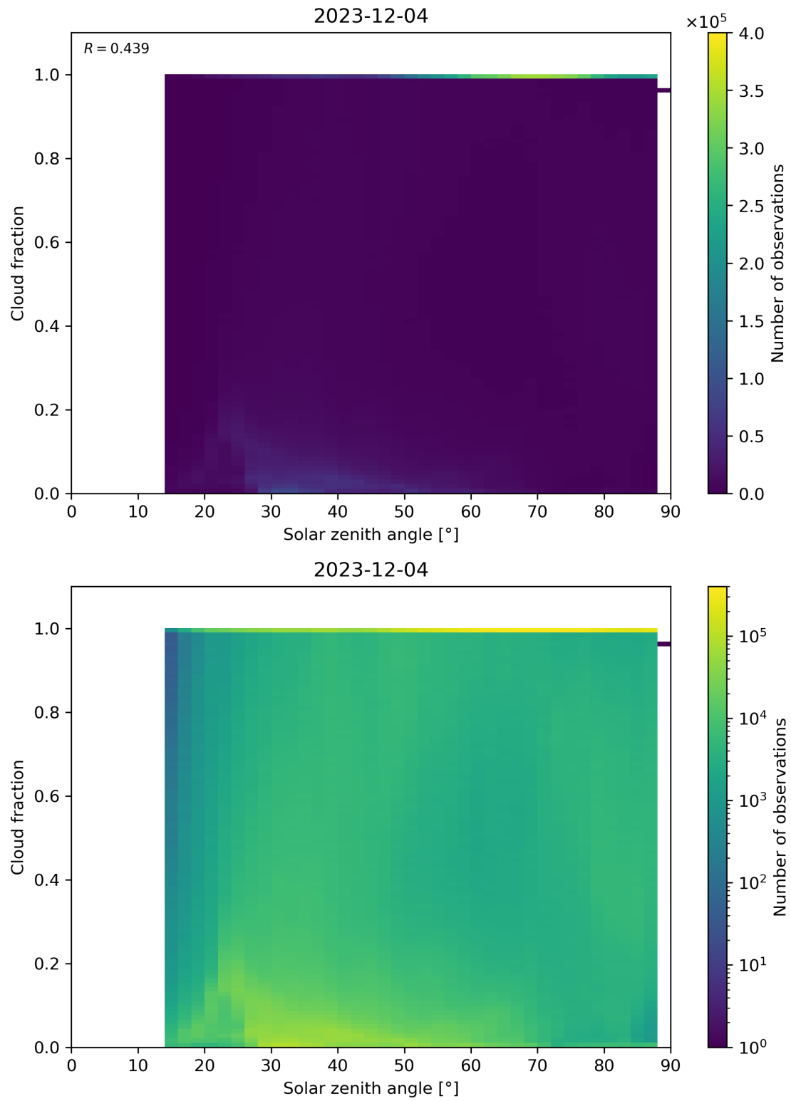
Figure 110: Scatter density plot of “Solar zenith angle” against “Cloud fraction” for 2023-12-04 to 2023-12-05.
