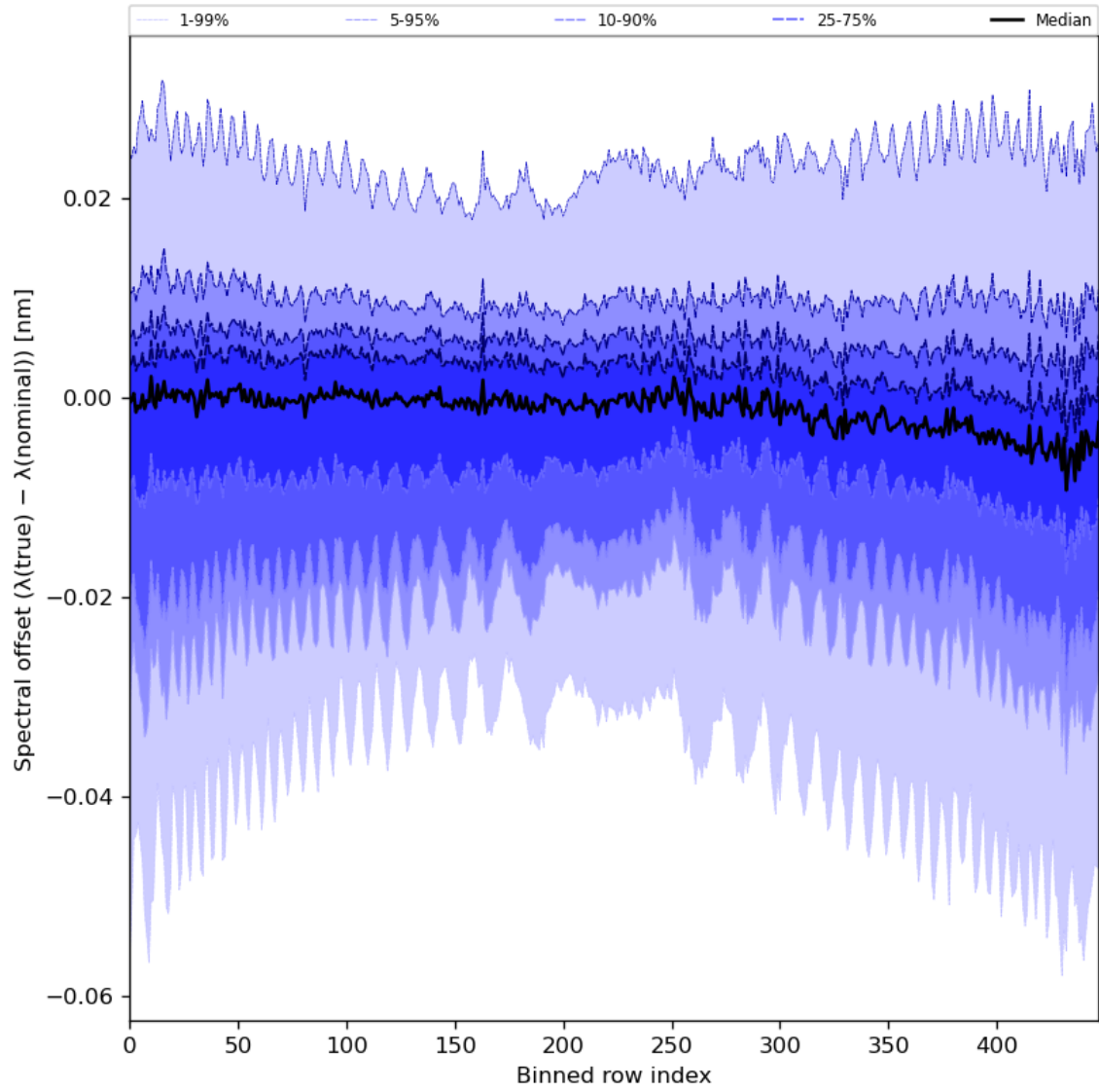
Figure 62: Along track statistics of “Spectral offset ( \lambda(\text{true}) - \lambda(\text{nominal}) )” for 2023-12-04 to 2023-12-05
