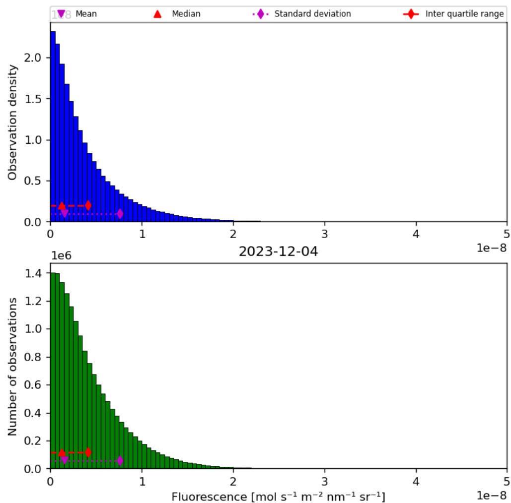
Figure 40: Histogram of “Fluorescence” for 2023-12-04 to 2023-12-05
