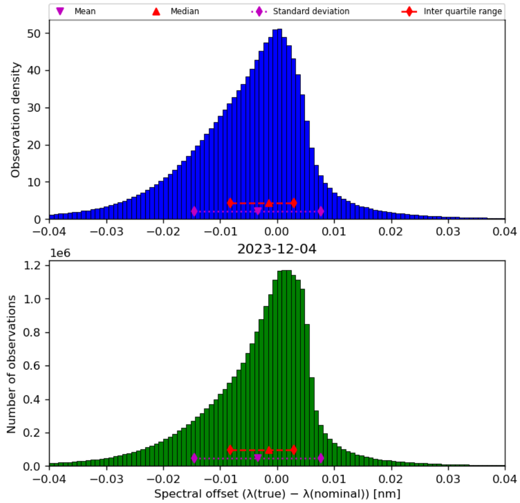
Figure 45: Histogram of “Spectral offset ( \lambda(\text{true}) - \lambda(\text{nominal}) )” for 2023-12-04 to 2023-12-05
