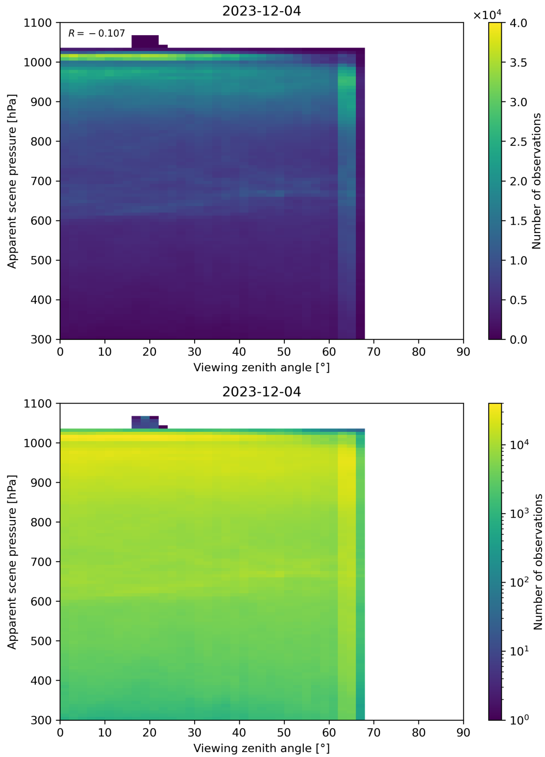
Figure 118: Scatter density plot of “Viewing zenith angle” against “Apparent scene pressure” for 2023-12-04 to 2023-12-05.
