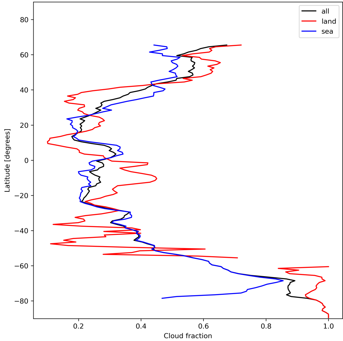
Figure 15: Zonal average of “Cloud fraction” for 2023-12-04 to 2023-12-05.
