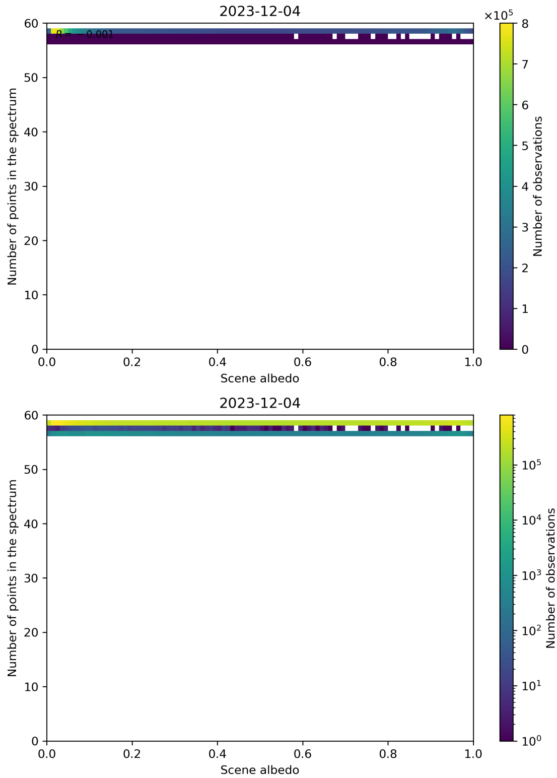
Figure 106: Scatter density plot of “Scene albedo” against “Number of points in the spectrum” for 2023-12-04 to 2023-12-05.
