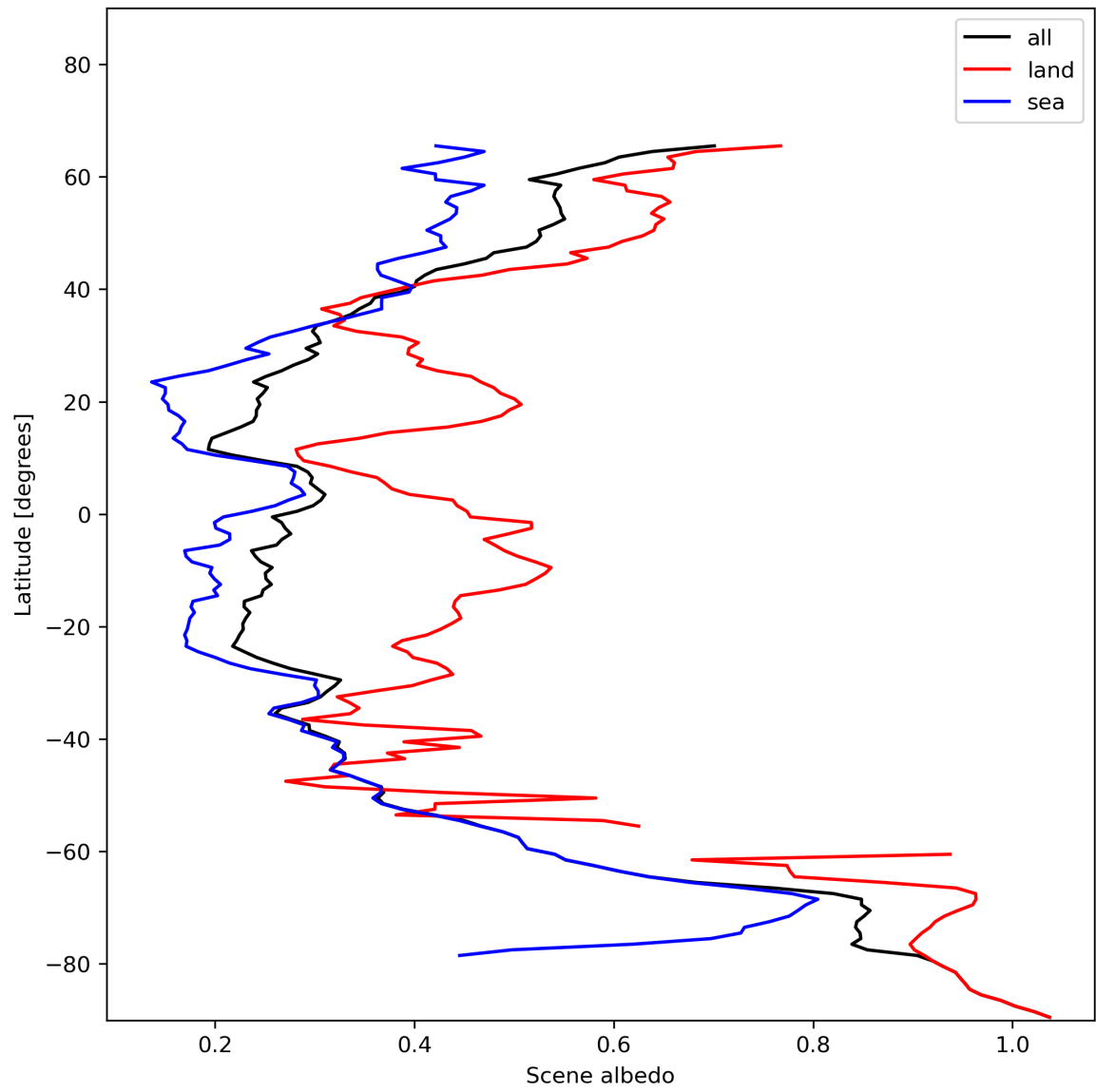
Figure 17: Zonal average of “Scene albedo” for 2023-12-04 to 2023-12-05.
