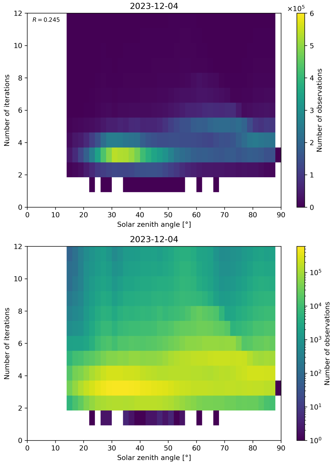
Figure 114: Scatter density plot of “Solar zenith angle” against “Number of iterations” for 2023-12-04 to 2023-12-05.
