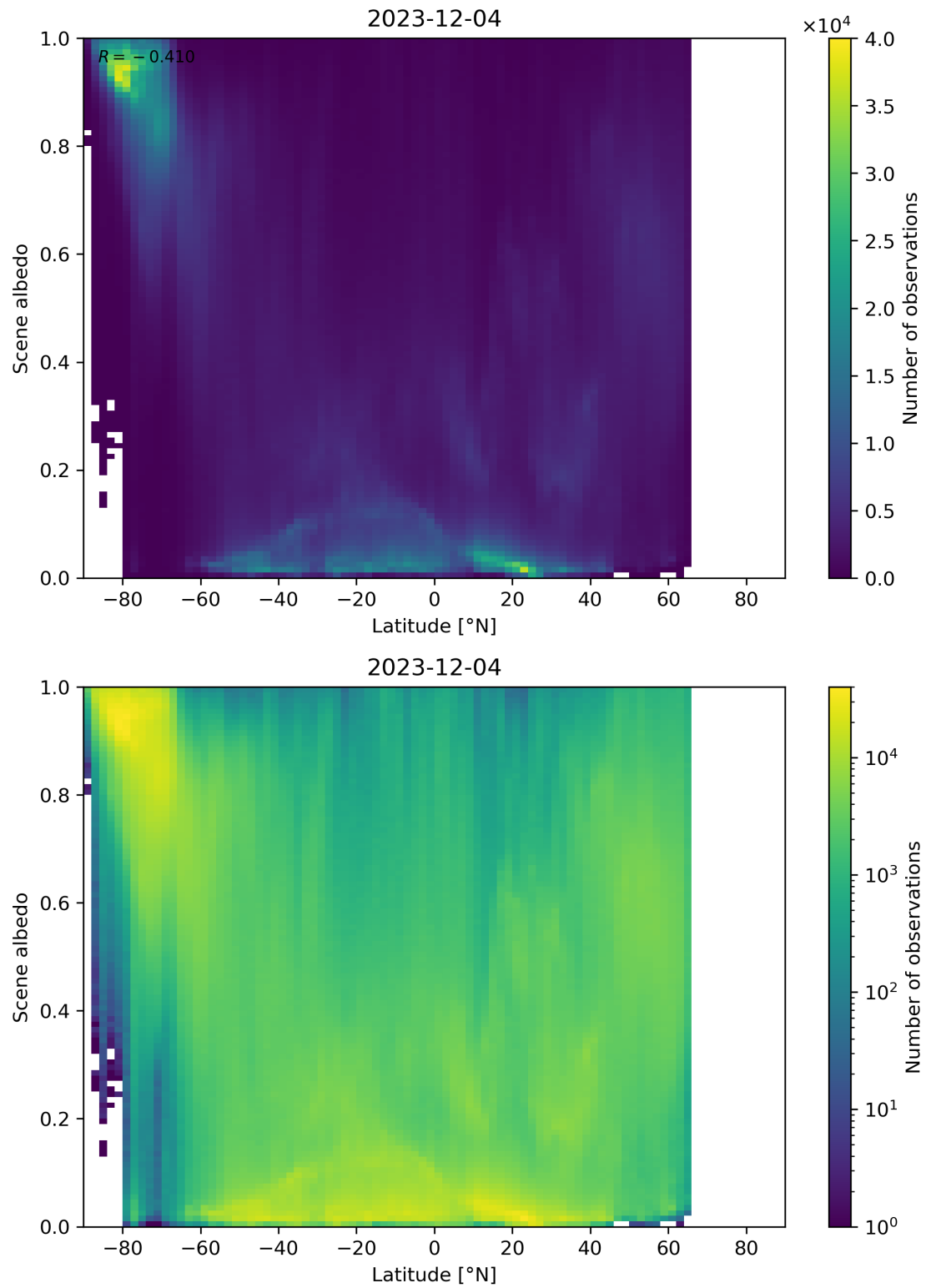
Figure 95: Scatter density plot of “Latitude” against “Scene albedo” for 2023-12-04 to 2023-12-05.
