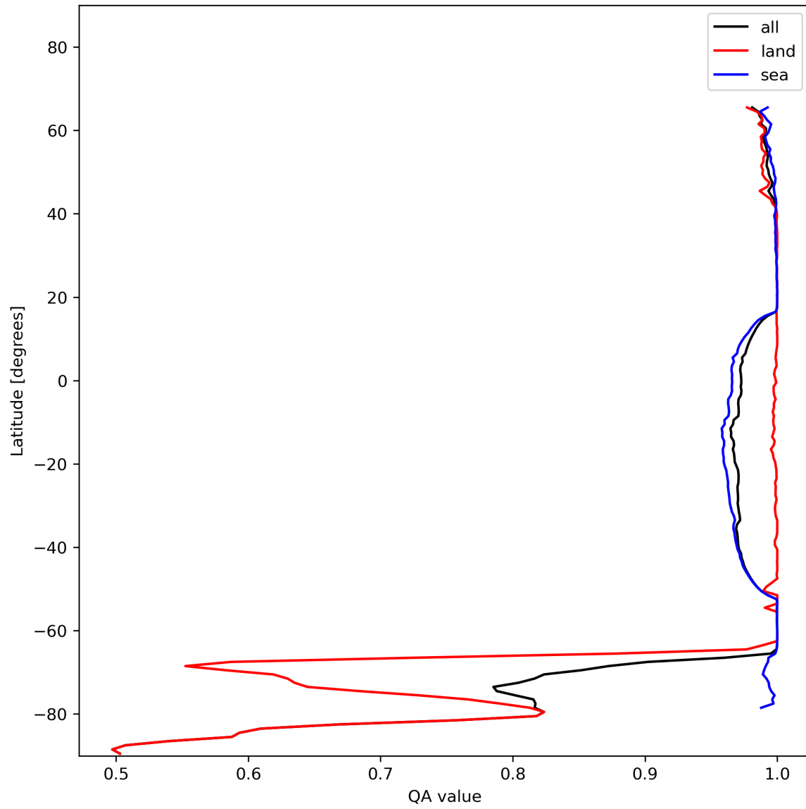
Figure 12: Zonal average of “QA value” for 2023-12-04 to 2023-12-05.
