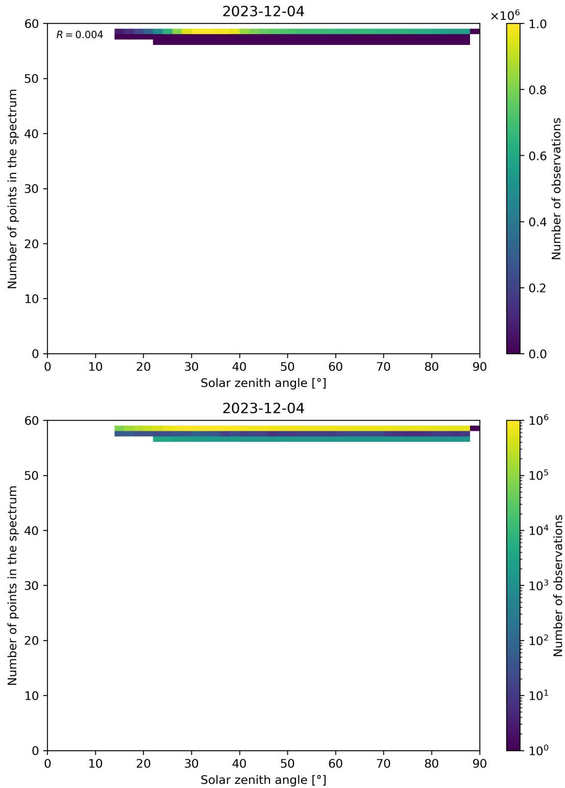
Figure 115: Scatter density plot of “Solar zenith angle” against “Number of points in the spectrum” for 2023-12-04 to 2023-12-05.
