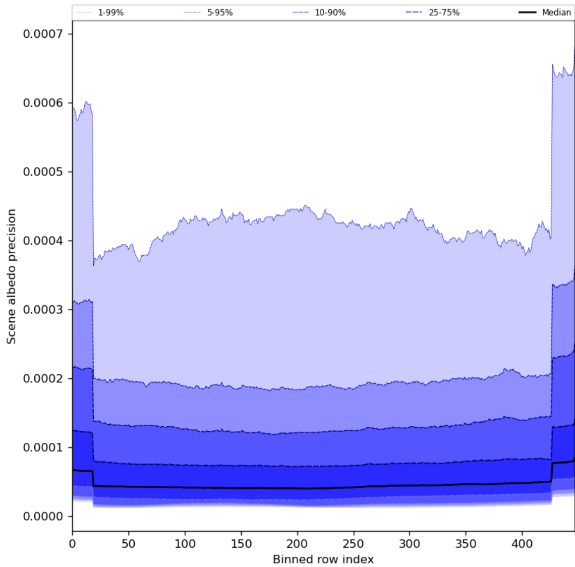
Figure 52: Along track statistics of “Scene albedo precision” for 2023-12-04 to 2023-12-05
