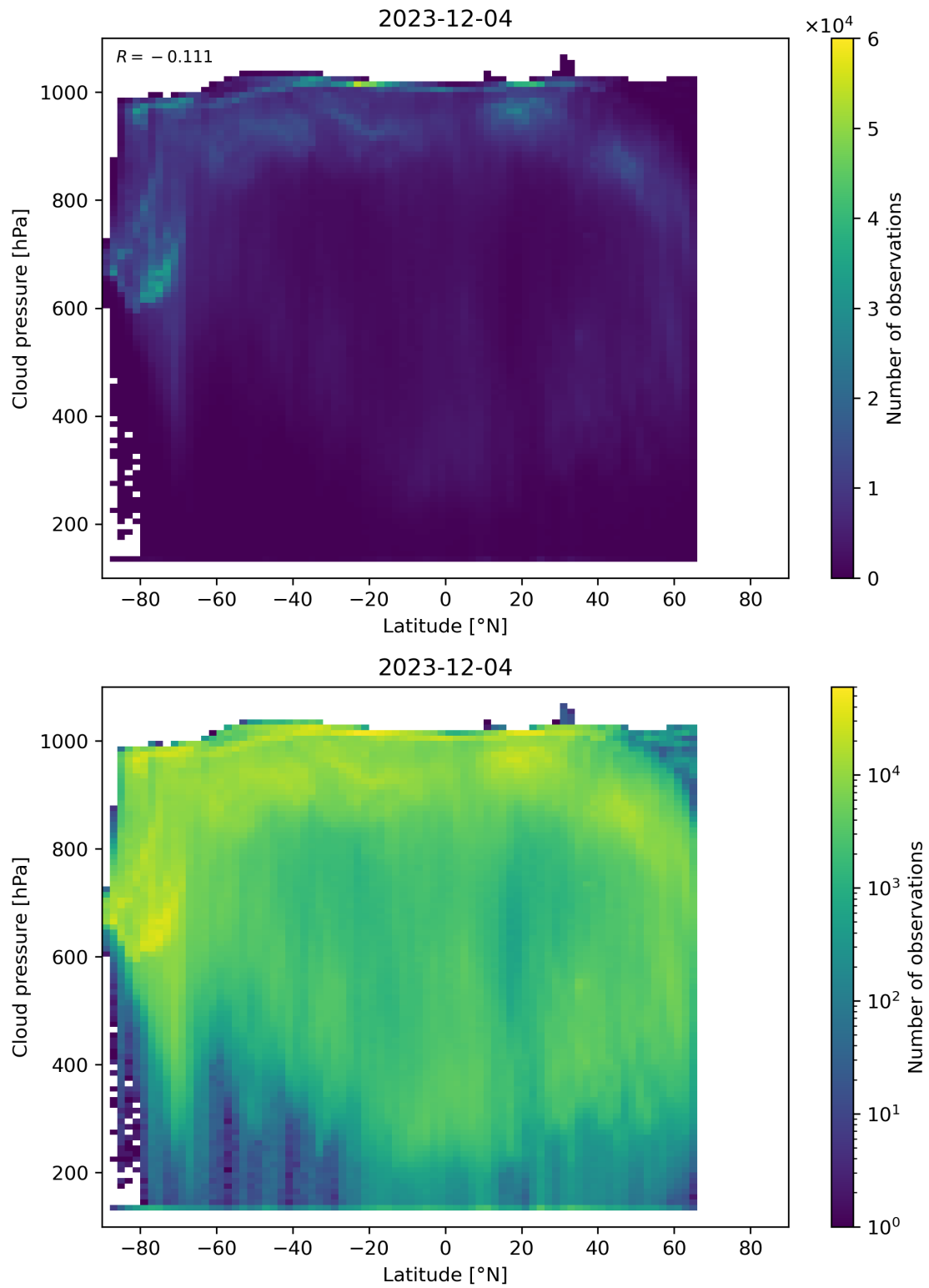
Figure 91: Scatter density plot of “Latitude” against “Cloud pressure” for 2023-12-04 to 2023-12-05.
