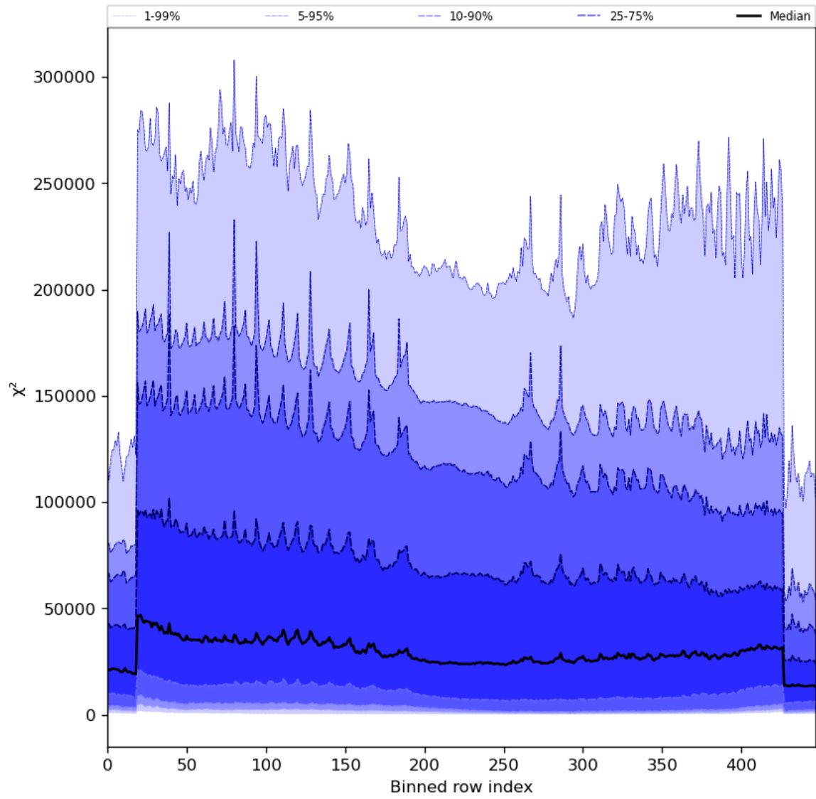
Figure 55: Along track statistics of “ \chi^2 ” for 2023-12-04 to 2023-12-05
