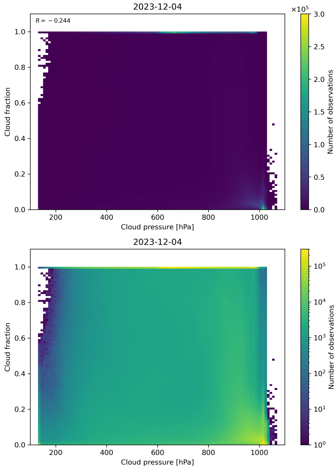
Figure 79: Scatter density plot of “Cloud pressure” against “Cloud fraction” for 2023-12-04 to 2023-12-05.
