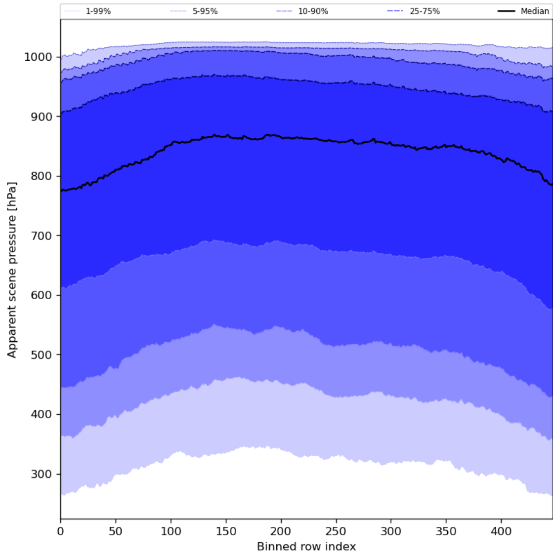
Figure 53: Along track statistics of “Apparent scene pressure” for 2023-12-04 to 2023-12-05
