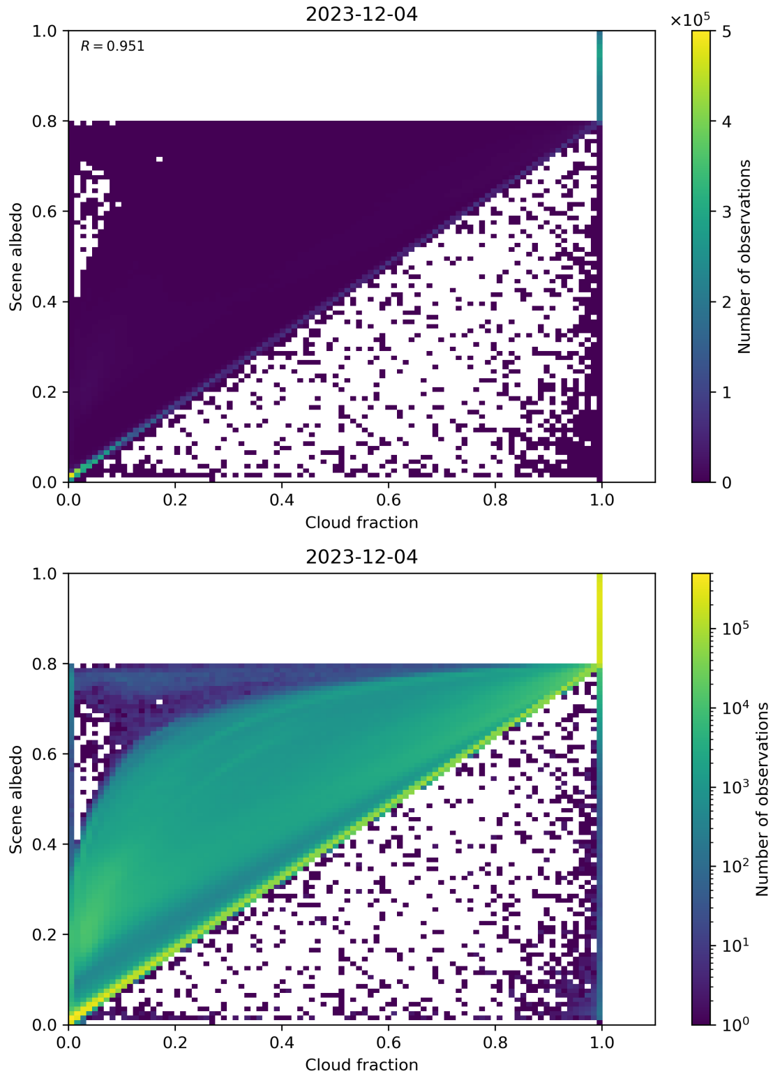
Figure 75: Scatter density plot of “Cloud fraction” against “Scene albedo” for 2023-12-04 to 2023-12-05.
