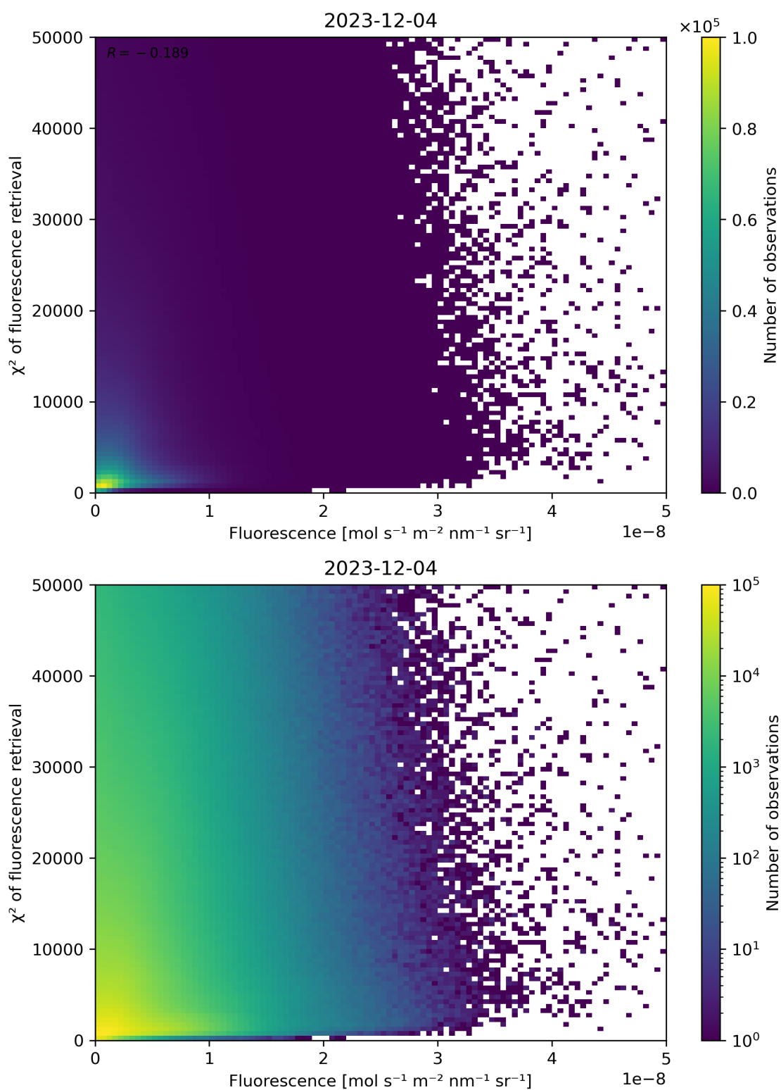
Figure 85: Scatter density plot of “Fluorescence” against “ \chi^2 of fluorescence retrieval” for 2023-12-04 to 2023-12-05.
