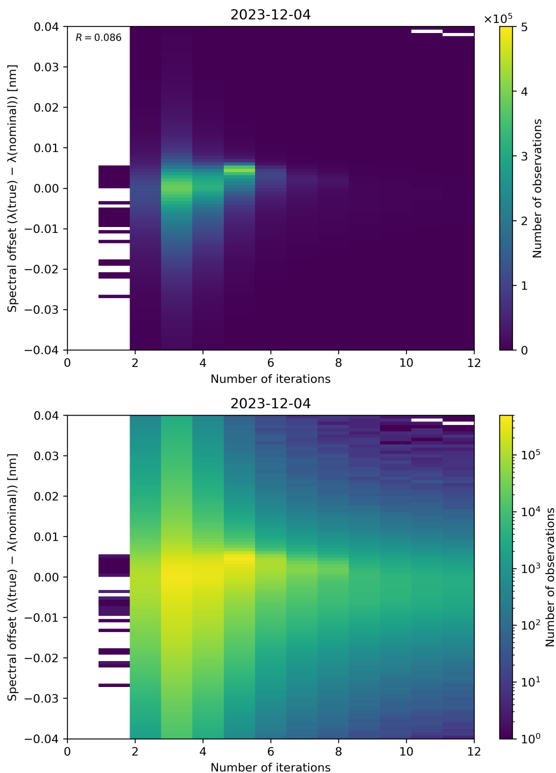
Figure 100: Scatter density plot of “Number of iterations” against “Spectral offset ( \lambda(\text{true}) - \lambda(\text{nominal}) )” for 2023-12-04 to 2023-12-05.
