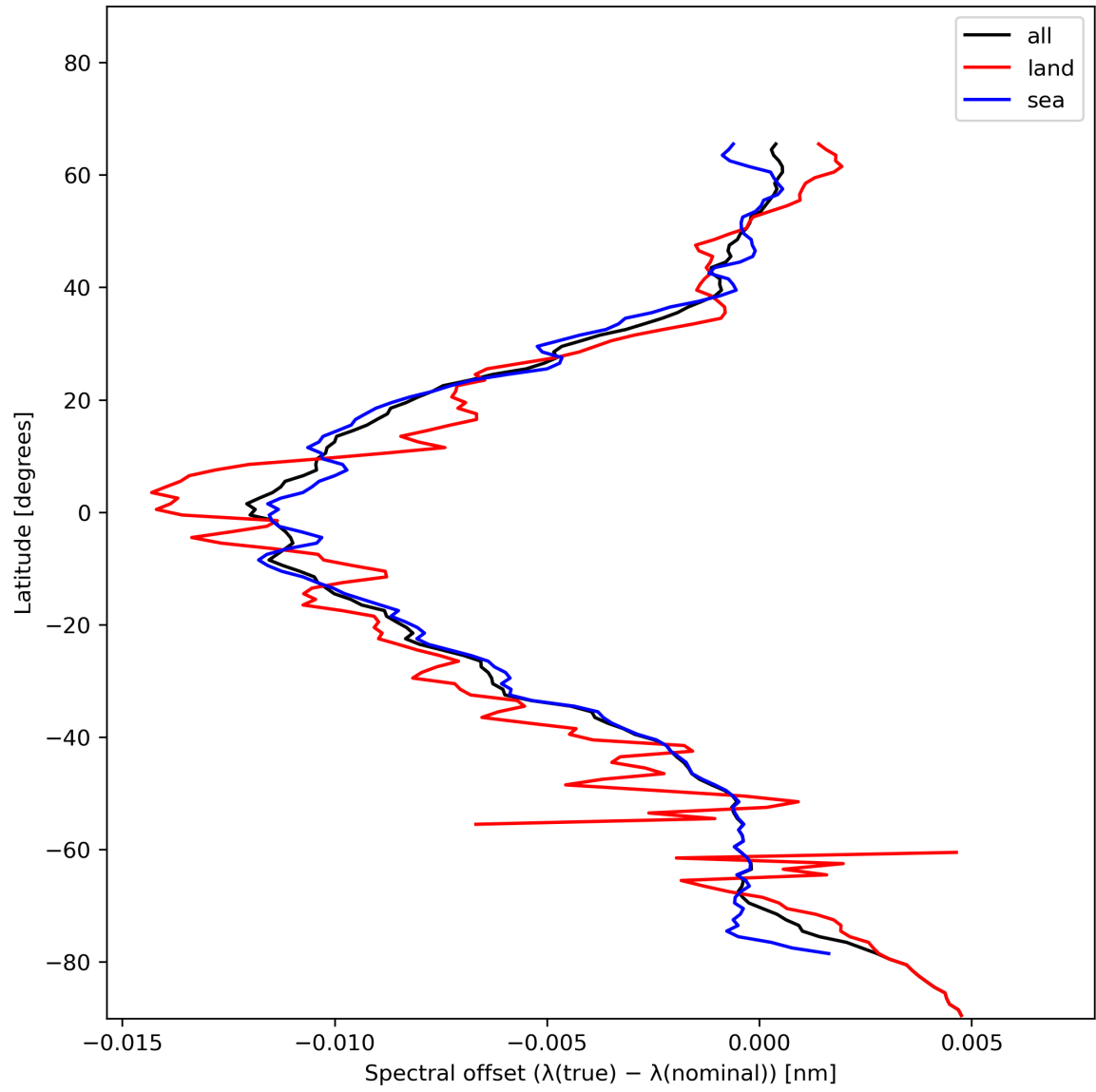
Figure 28: Zonal average of “Spectral offset ( \lambda(\text{true}) - \lambda(\text{nominal}) )” for 2023-12-04 to 2023-12-05.
