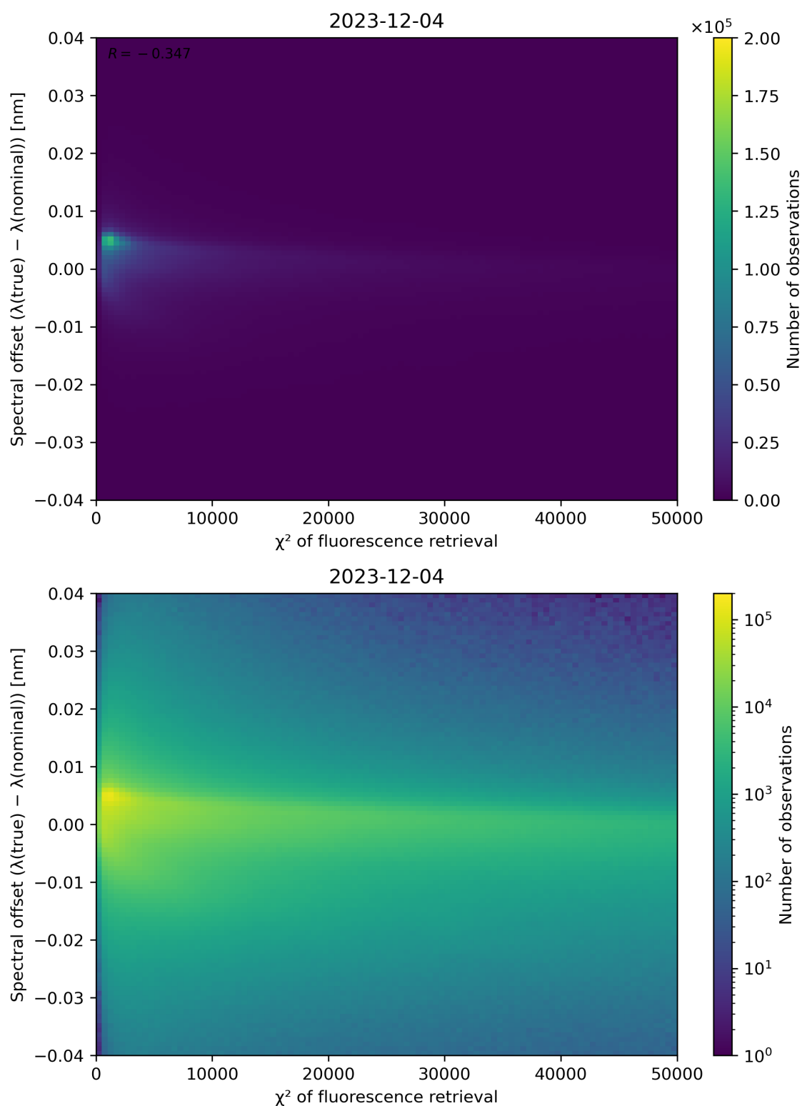
Figure 69: Scatter density plot of " \chi^2 of fluorescence retrieval" against "Spectral offset ( \lambda(\text{true}) - \lambda(\text{nominal}) )" for 2023-12-04 to 2023-12-05.
