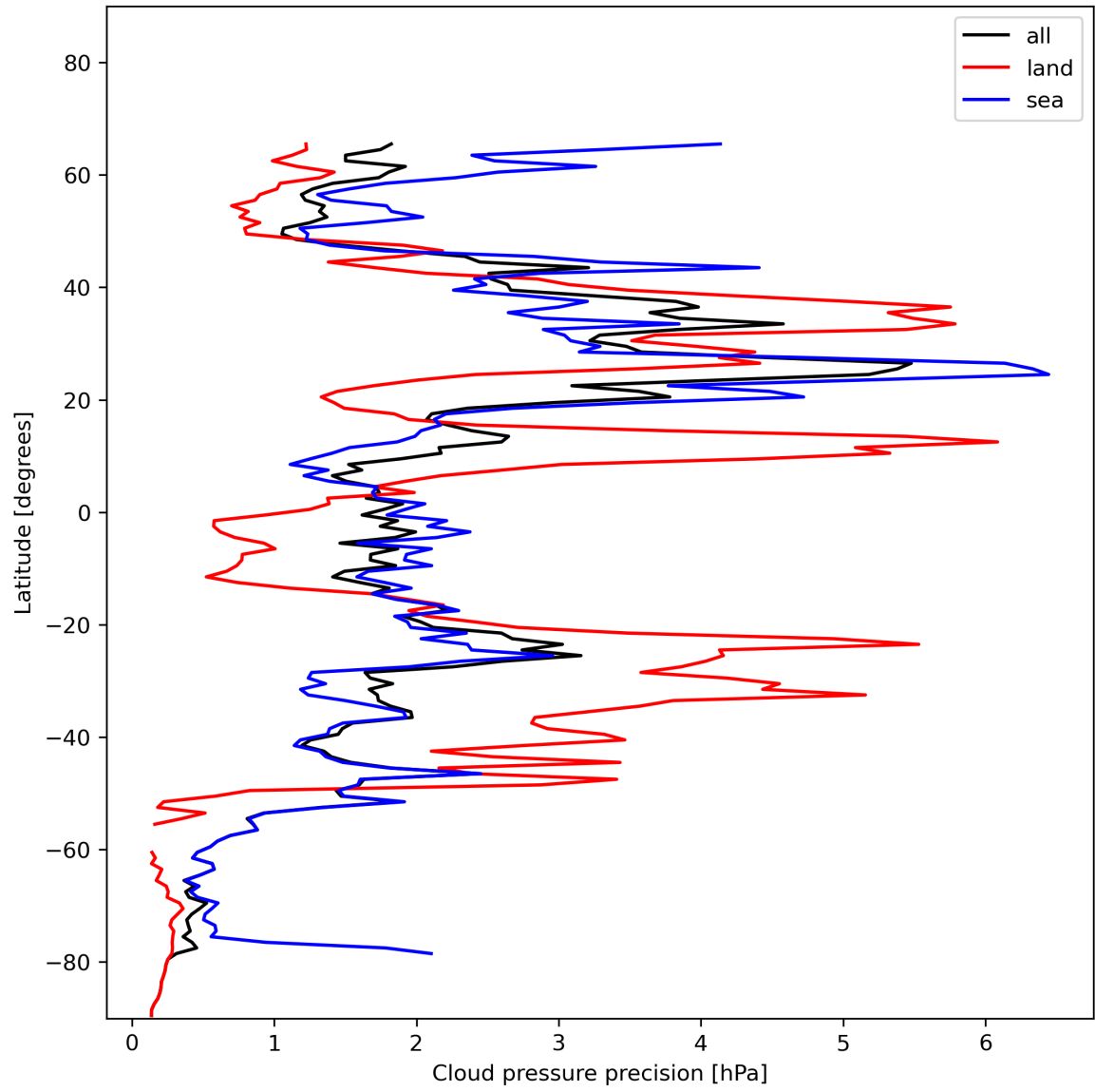
Figure 14: Zonal average of “Cloud pressure precision” for 2023-12-04 to 2023-12-05.
