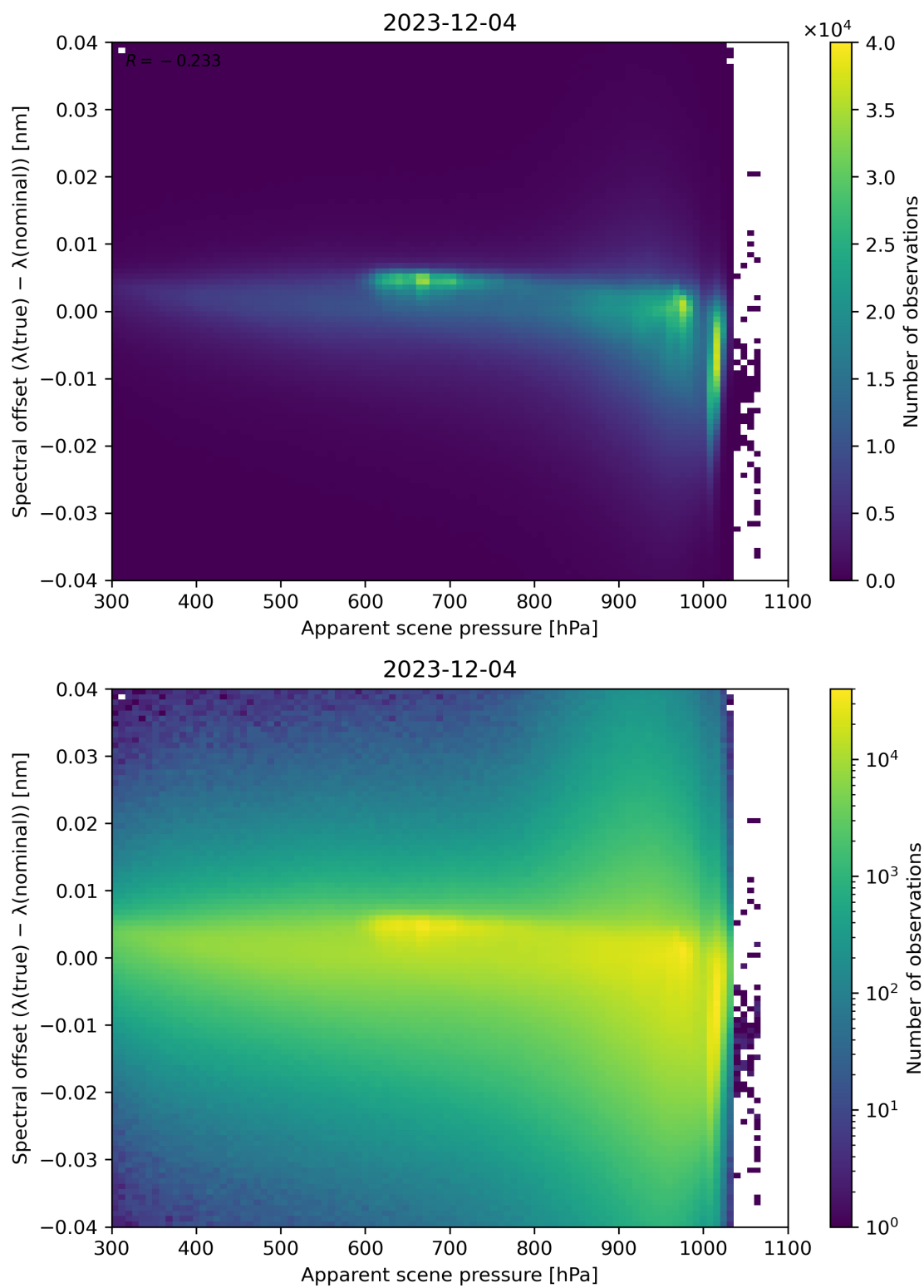
Figure 67: Scatter density plot of “Apparent scene pressure” against “Spectral offset ( \lambda(\text{true}) - \lambda(\text{nominal}) )” for 2023-12-04 to 2023-12-05.
