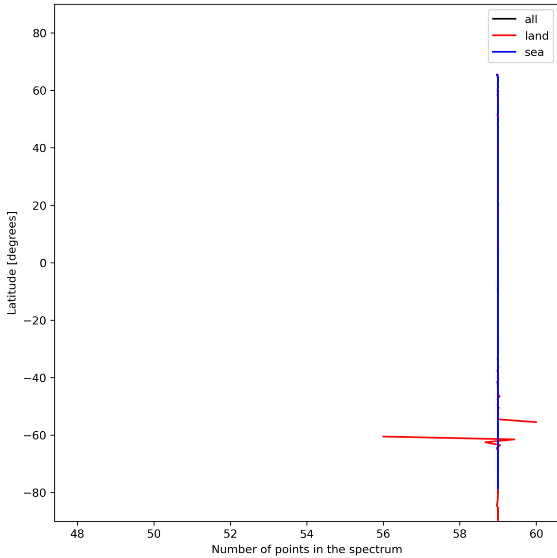
Figure 27: Zonal average of “Number of points in the spectrum” for 2023-12-04 to 2023-12-05.
