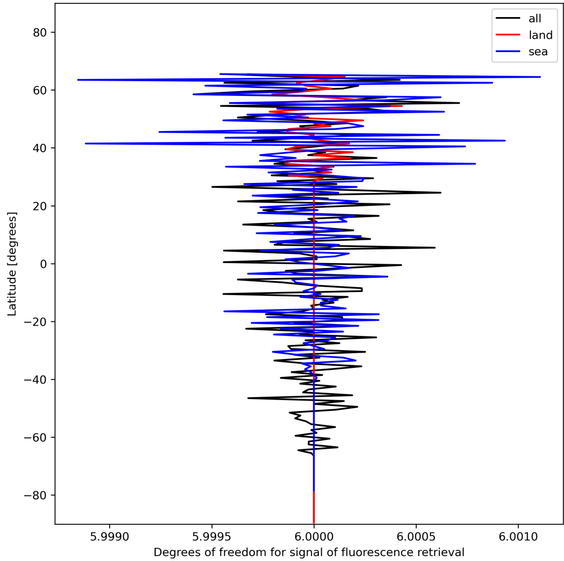
Figure 26: Zonal average of “Degrees of freedom for signal of fluorescence retrieval” for 2023-12-04 to 2023-12-05.
