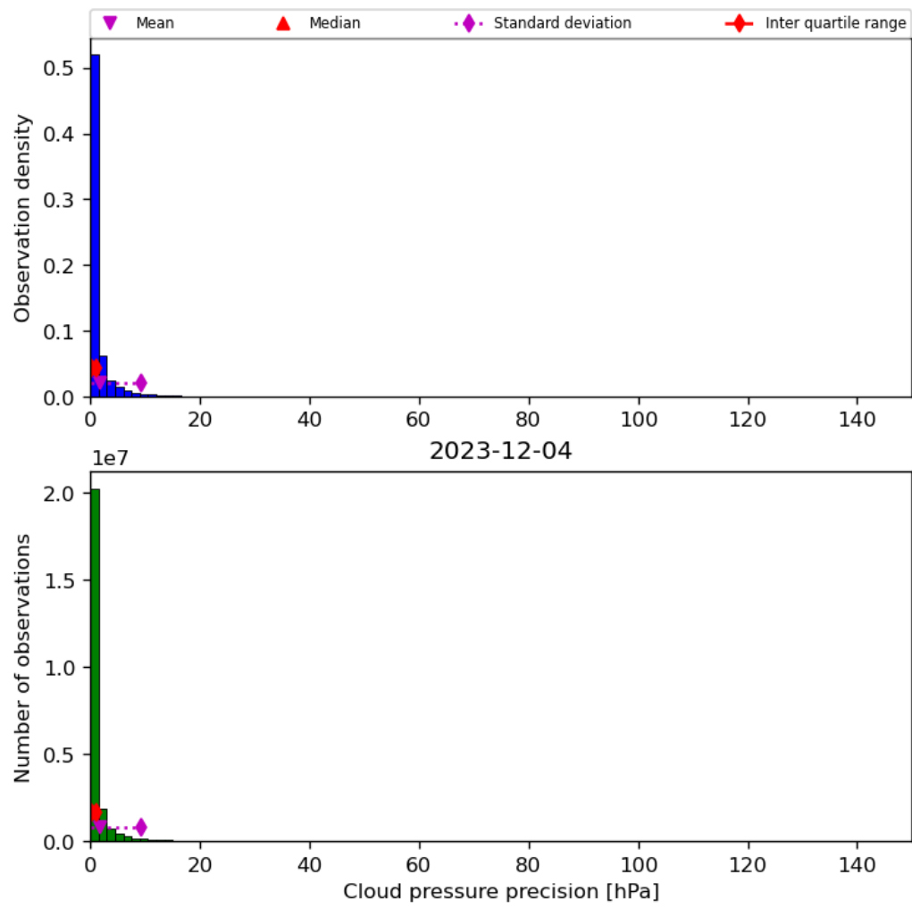
Figure 31: Histogram of “Cloud pressure precision” for 2023-12-04 to 2023-12-05
