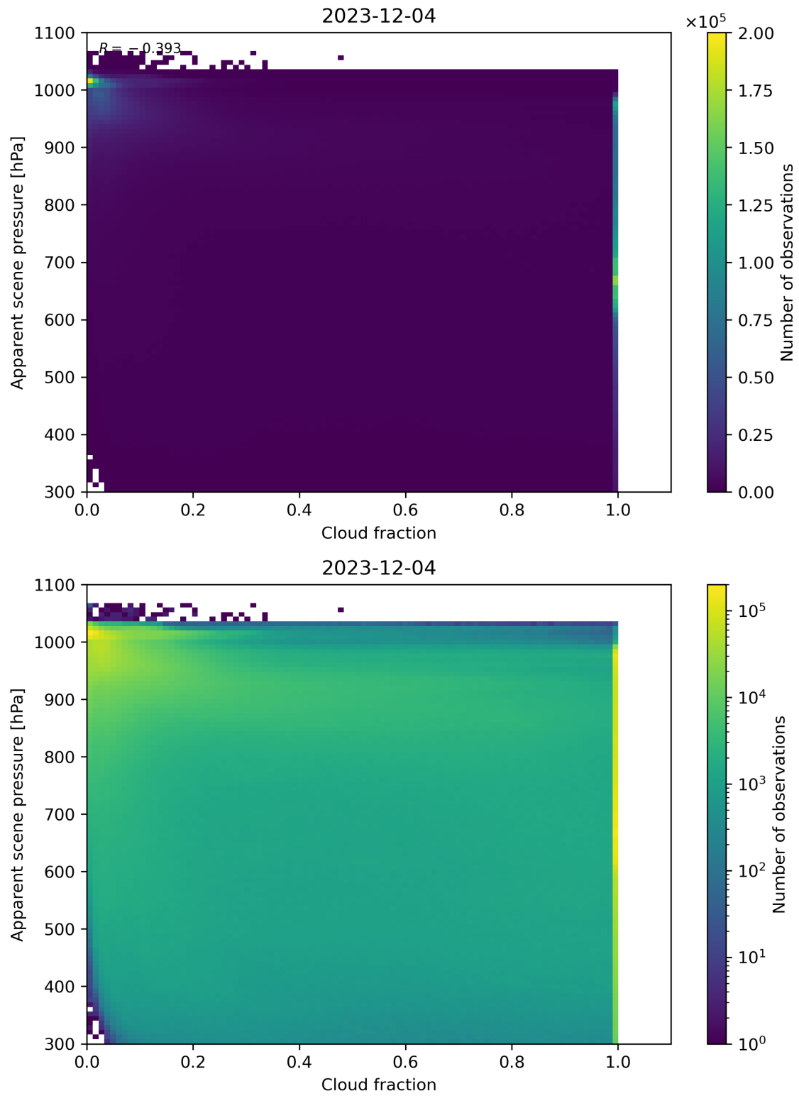
Figure 70: Scatter density plot of “Cloud fraction” against “Apparent scene pressure” for 2023-12-04 to 2023-12-05.
