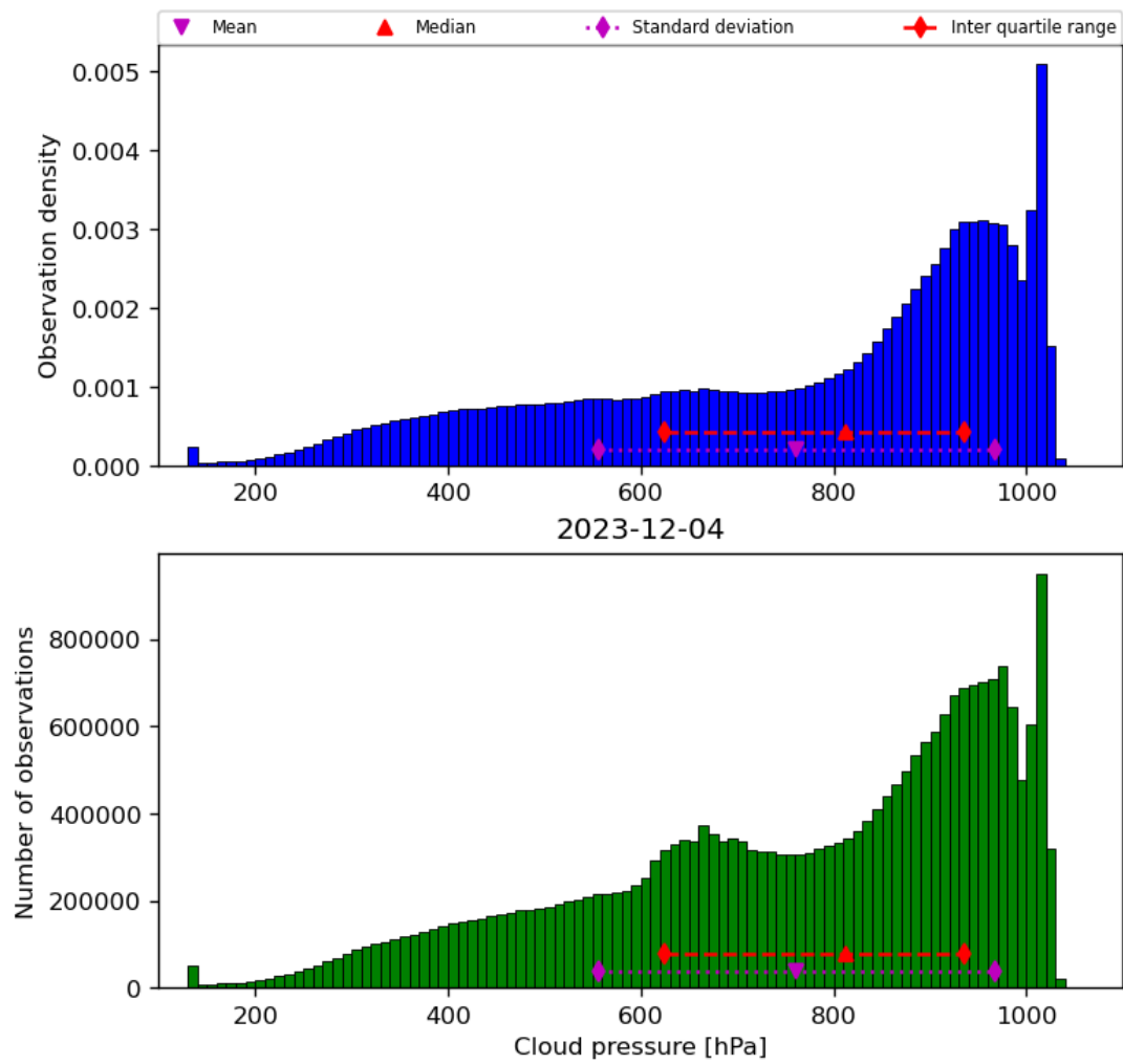
Figure 30: Histogram of “Cloud pressure” for 2023-12-04 to 2023-12-05
