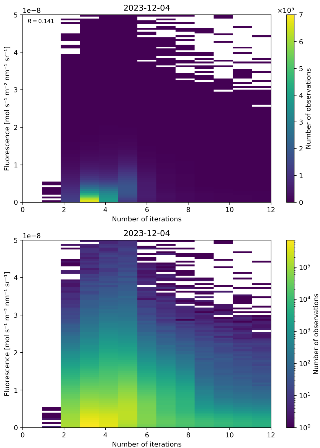
Figure 98: Scatter density plot of “Number of iterations” against “Fluorescence” for 2023-12-04 to 2023-12-05.
