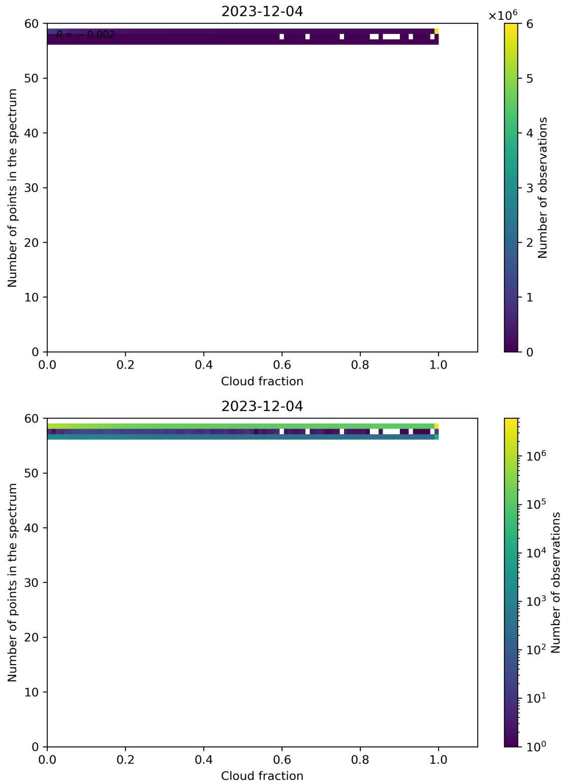
Figure 74: Scatter density plot of “Cloud fraction” against “Number of points in the spectrum” for 2023-12-04 to 2023-12-05.
