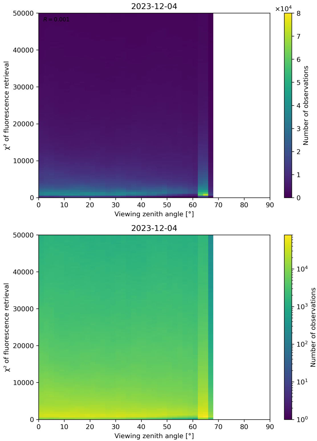
Figure 119: Scatter density plot of “Viewing zenith angle” against “ \chi^2 of fluorescence retrieval” for 2023-12-04 to 2023-12-05.
