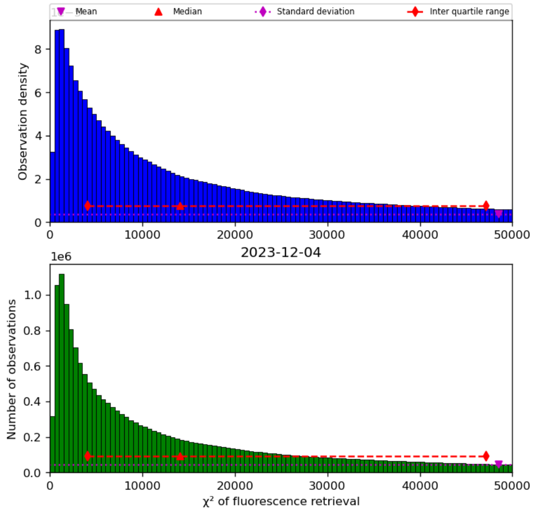
Figure 42: Histogram of “ \chi^2 of fluorescence retrieval” for 2023-12-04 to 2023-12-05
