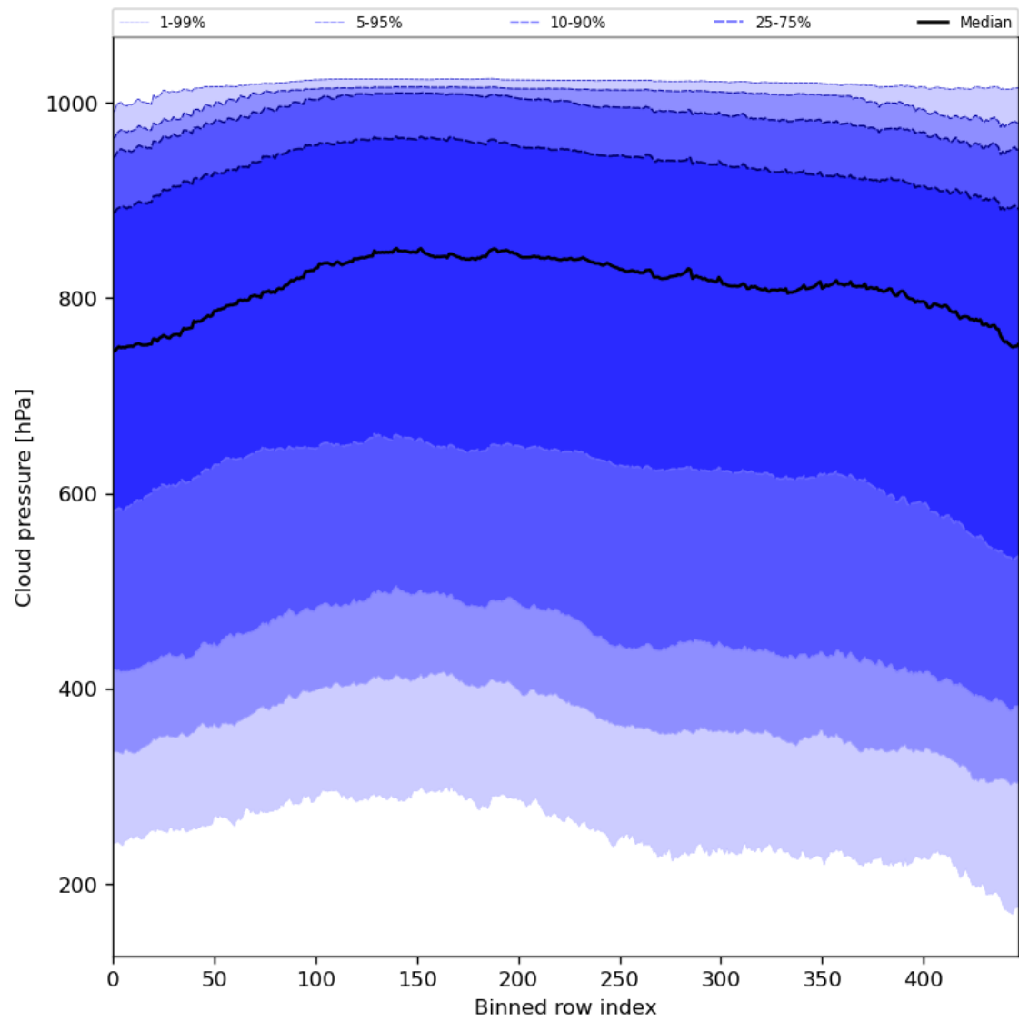
Figure 47: Along track statistics of “Cloud pressure” for 2023-12-04 to 2023-12-05
