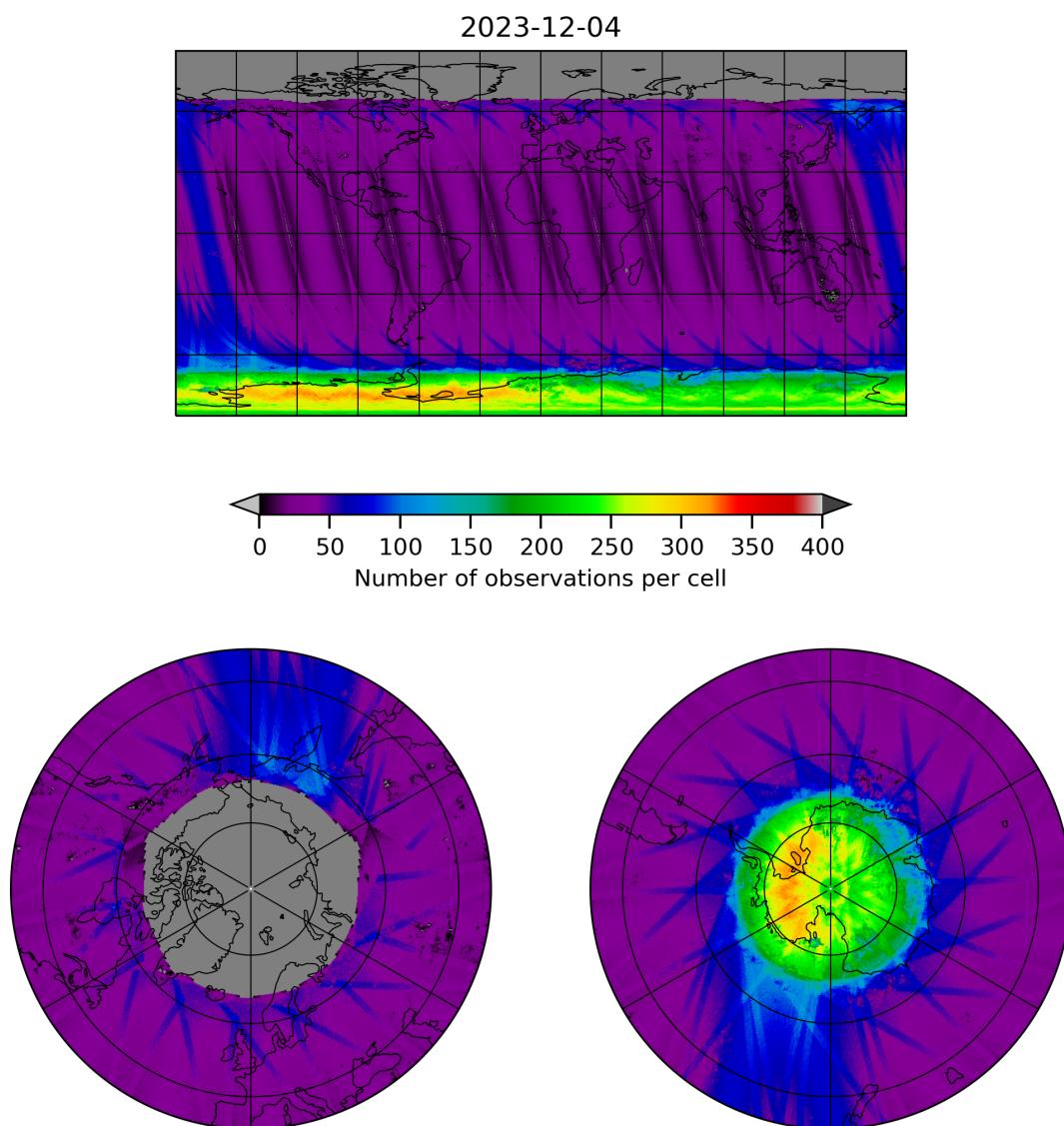
Figure 11: Map of the number of observations for 2023-12-04 to 2023-12-05
