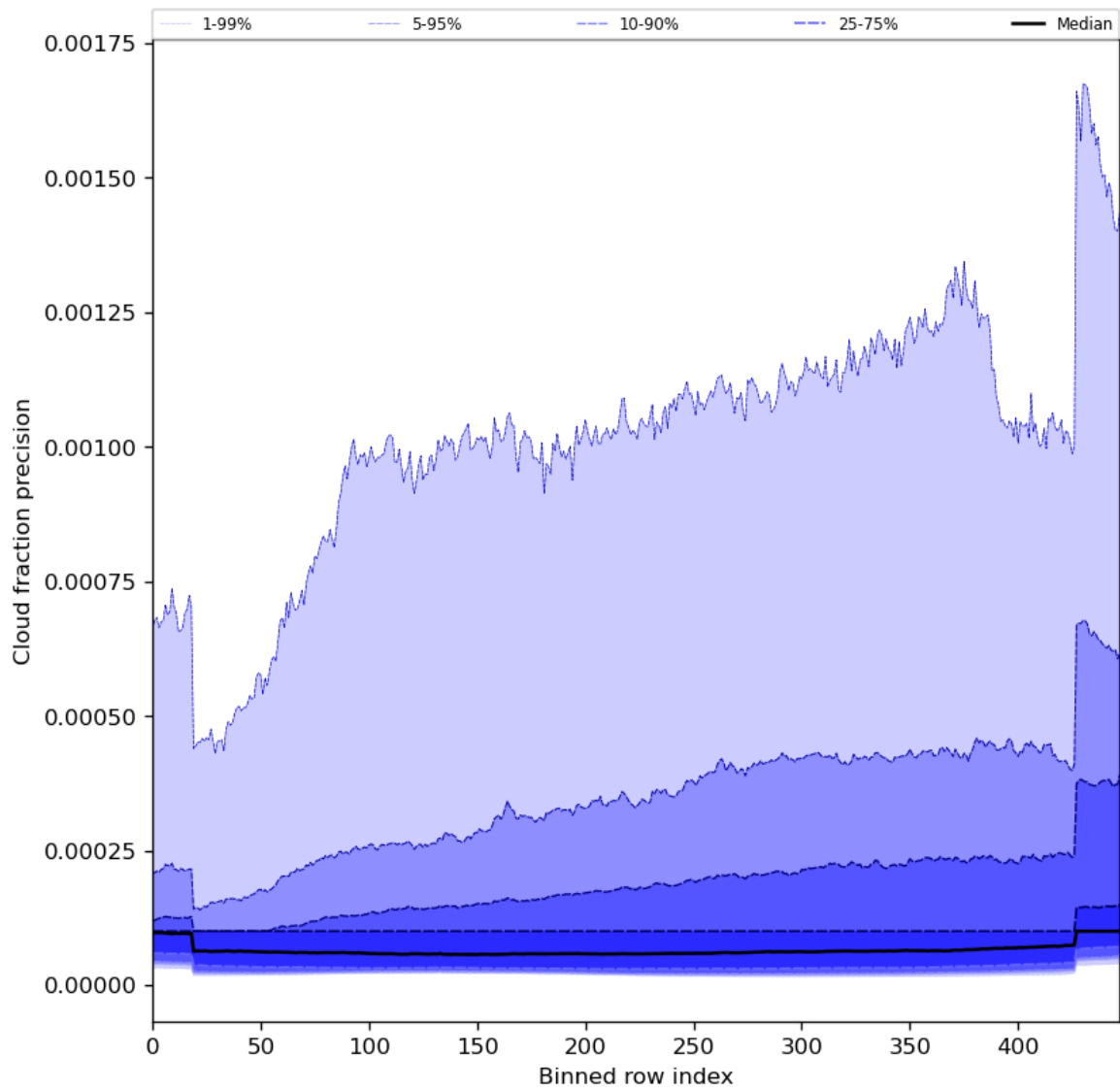
Figure 50: Along track statistics of “Cloud fraction precision” for 2023-12-04 to 2023-12-05
