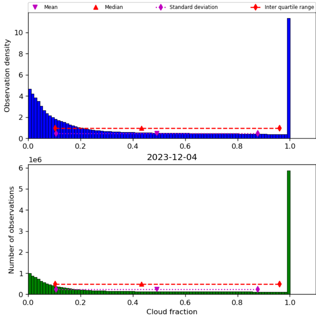
Figure 32: Histogram of “Cloud fraction” for 2023-12-04 to 2023-12-05
