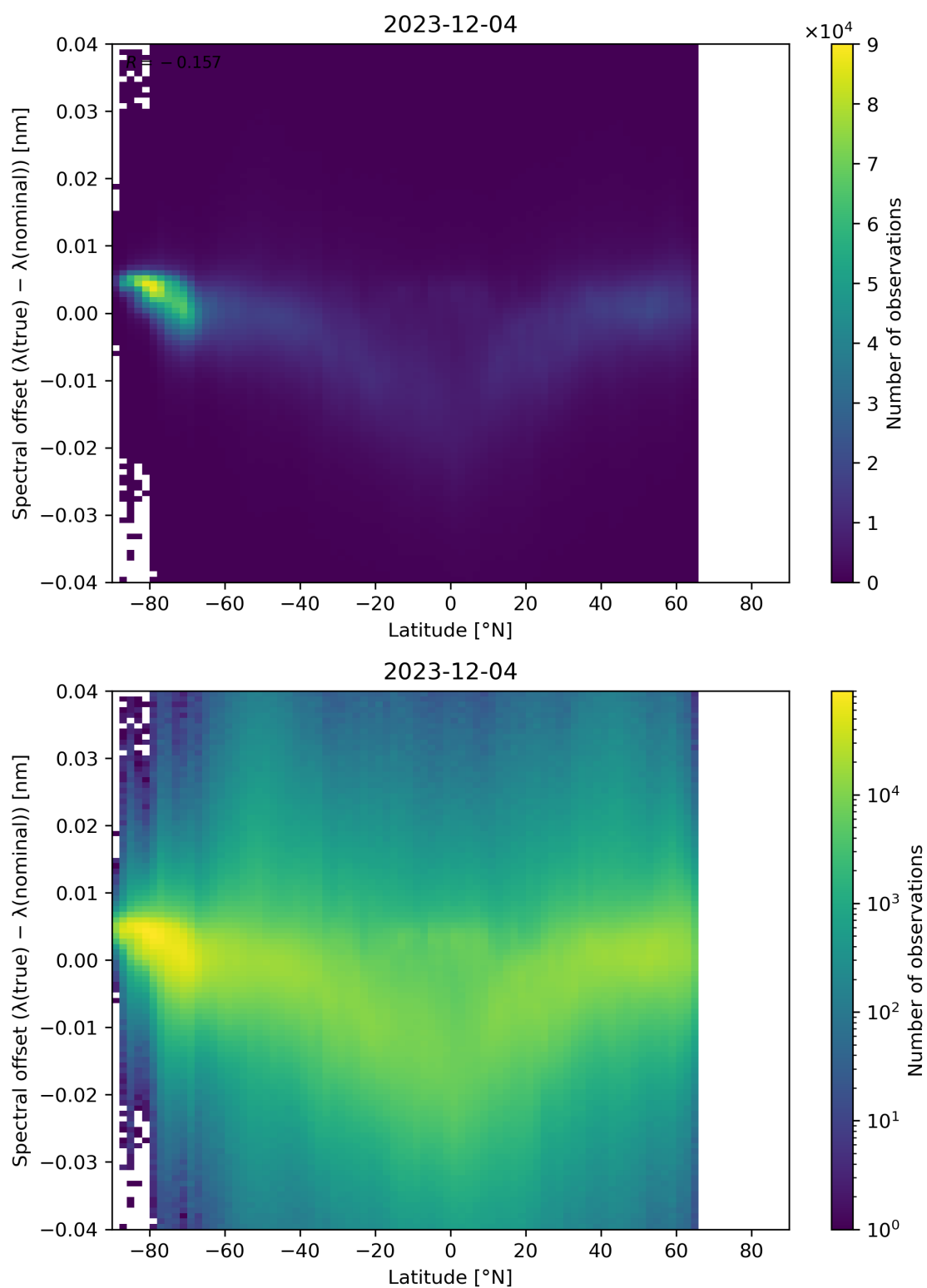
Figure 96: Scatter density plot of “Latitude” against “Spectral offset ( \lambda(\text{true}) - \lambda(\text{nominal}) )” for 2023-12-04 to 2023-12-05.
