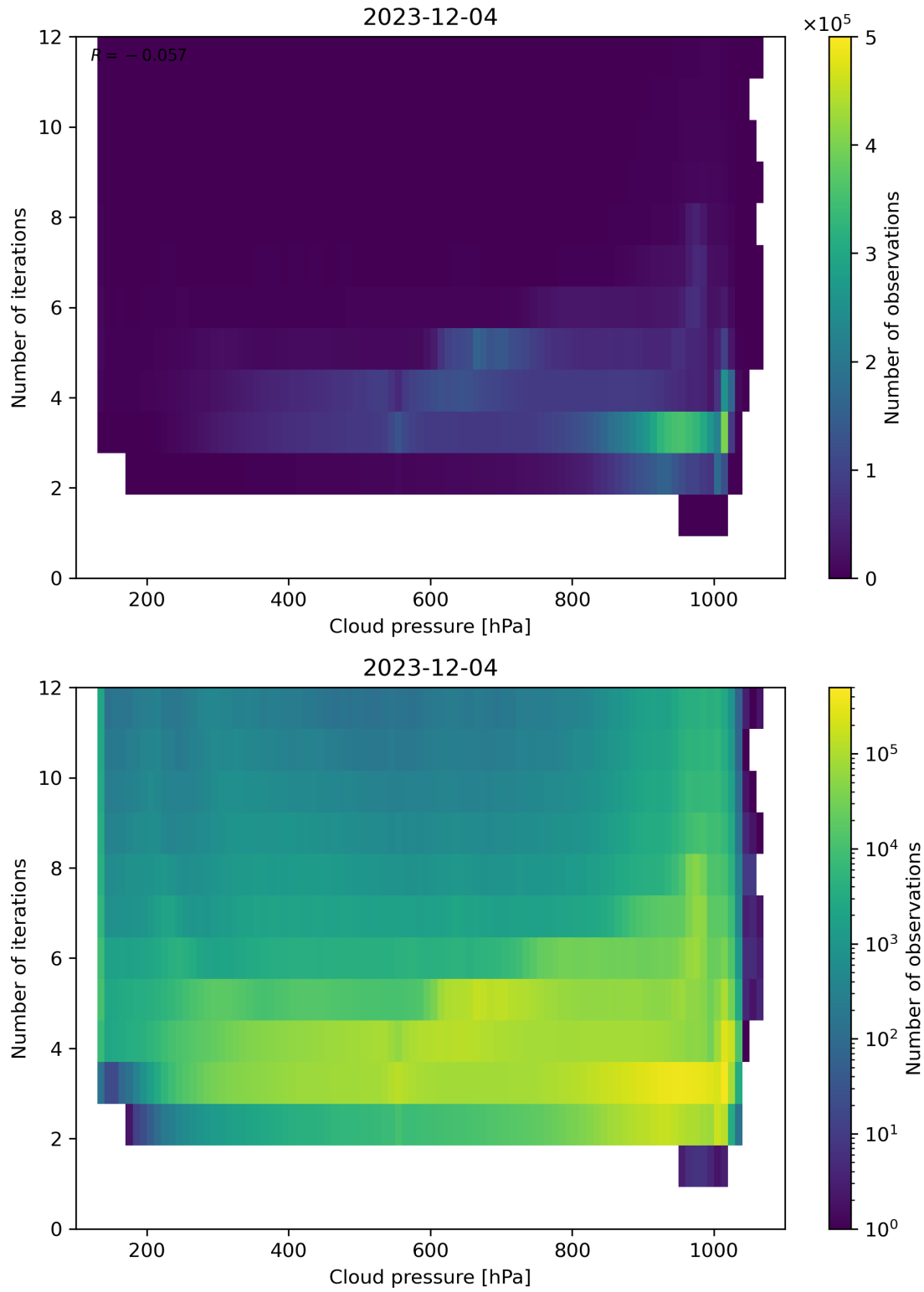
Figure 81: Scatter density plot of “Cloud pressure” against “Number of iterations” for 2023-12-04 to 2023-12-05.
