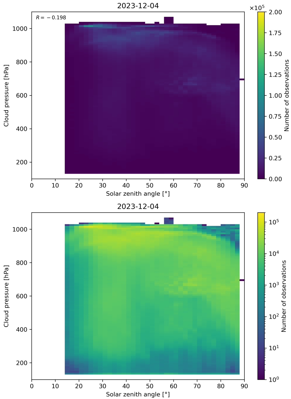
Figure 111: Scatter density plot of “Solar zenith angle” against “Cloud pressure” for 2023-12-04 to 2023-12-05.
