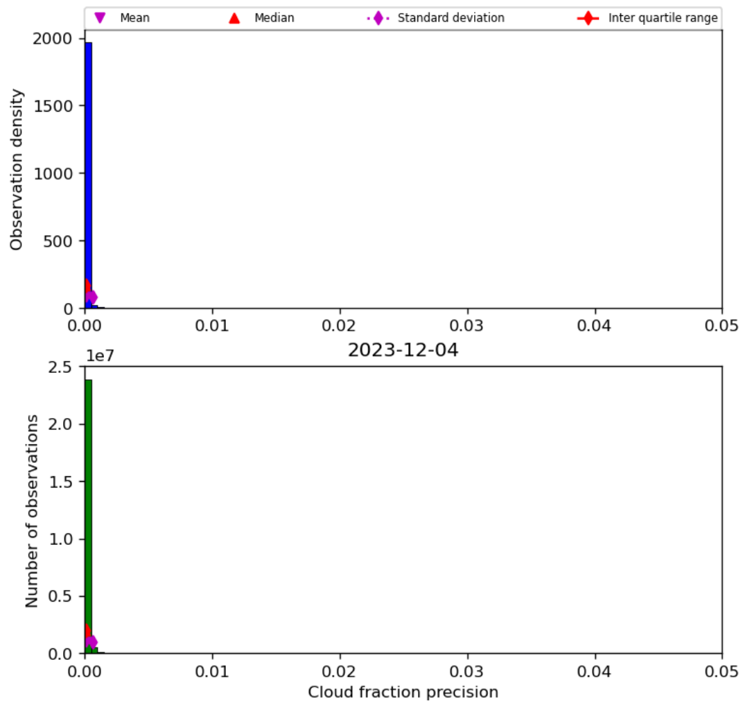
Figure 33: Histogram of “Cloud fraction precision” for 2023-12-04 to 2023-12-05
