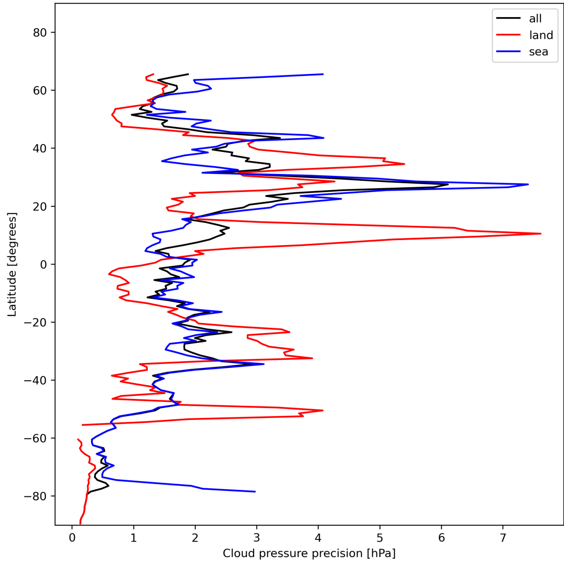
Figure 14: Zonal average of “Cloud pressure precision” for 2023-12-04 to 2023-12-06.
