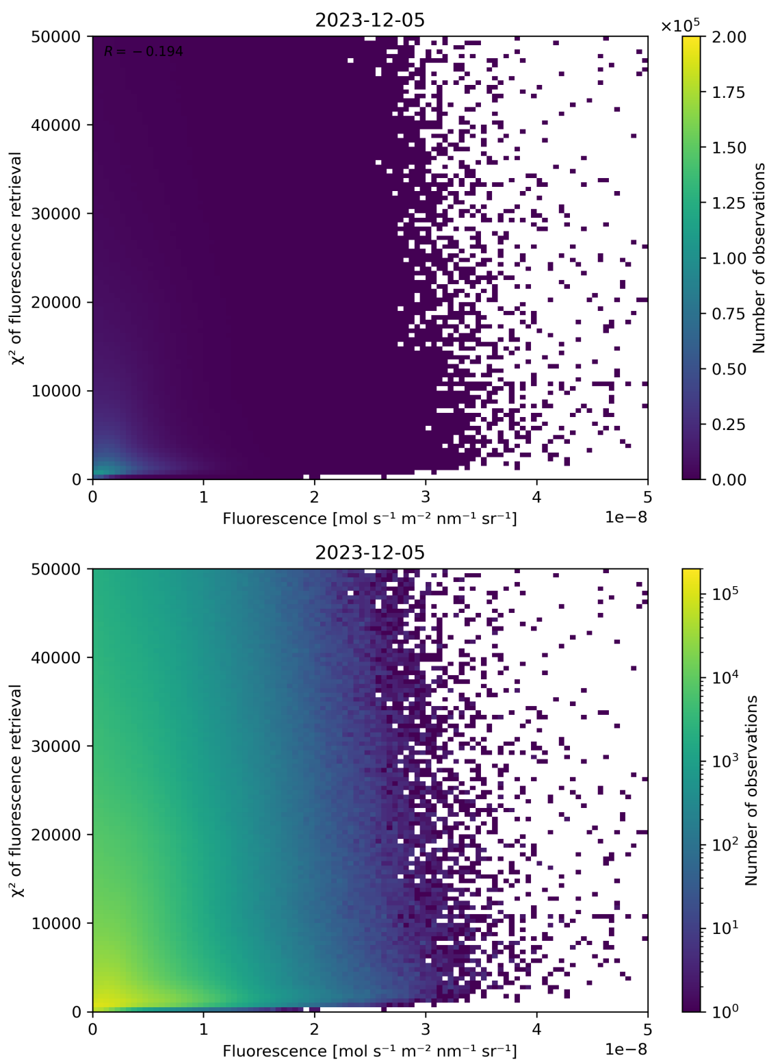
Figure 85: Scatter density plot of “Fluorescence” against “ \chi^2 of fluorescence retrieval” for 2023-12-04 to 2023-12-06.
