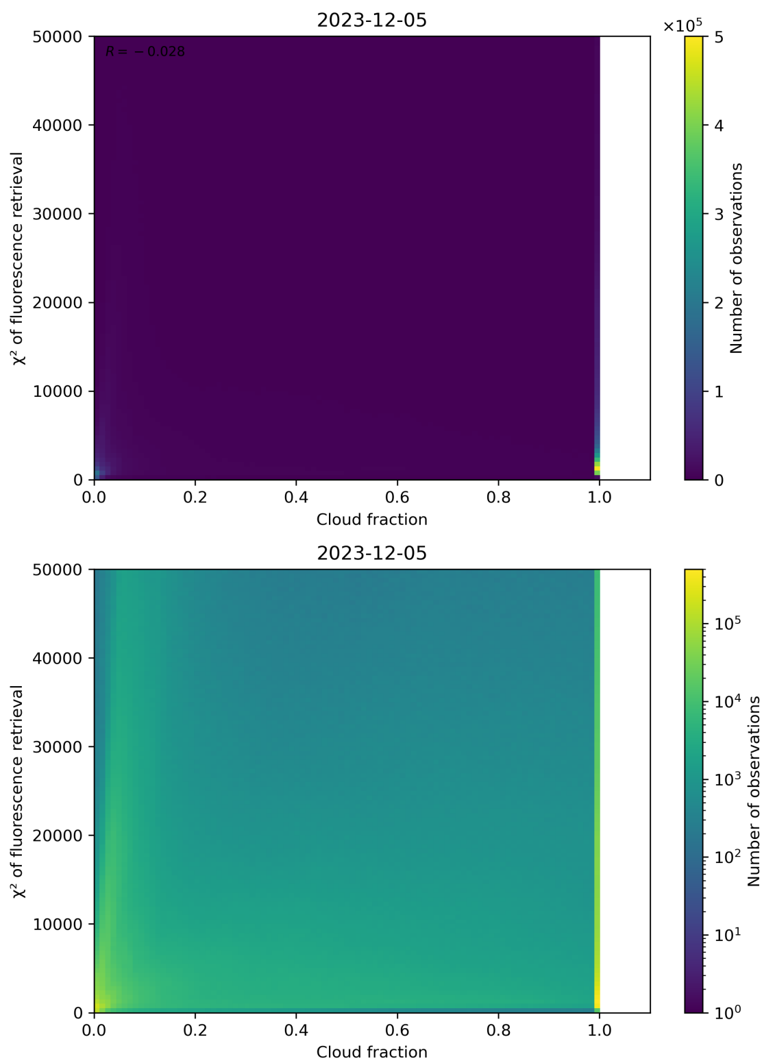
Figure 71: Scatter density plot of “Cloud fraction” against “ \chi^2 of fluorescence retrieval” for 2023-12-04 to 2023-12-06.
