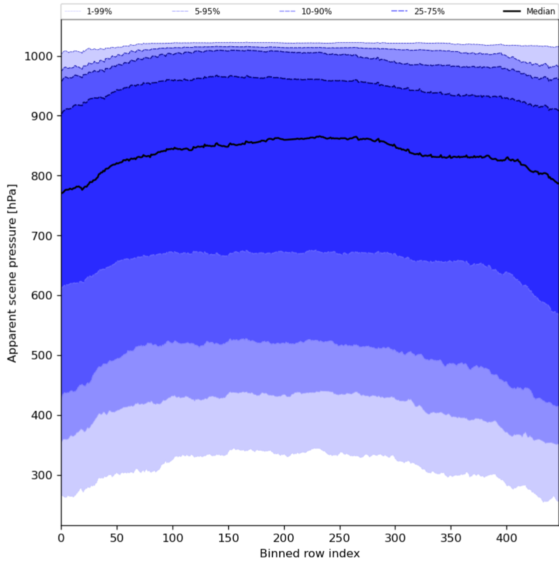
Figure 53: Along track statistics of “Apparent scene pressure” for 2023-12-04 to 2023-12-06
