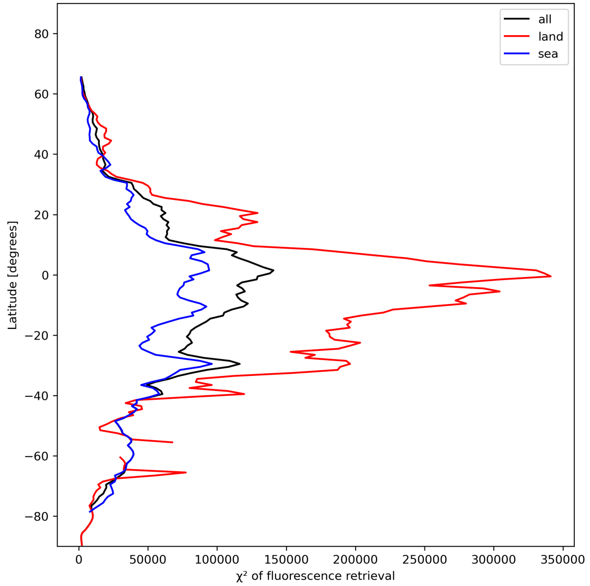
Figure 25: Zonal average of “ \chi^2 of fluorescence retrieval” for 2023-12-04 to 2023-12-06.
