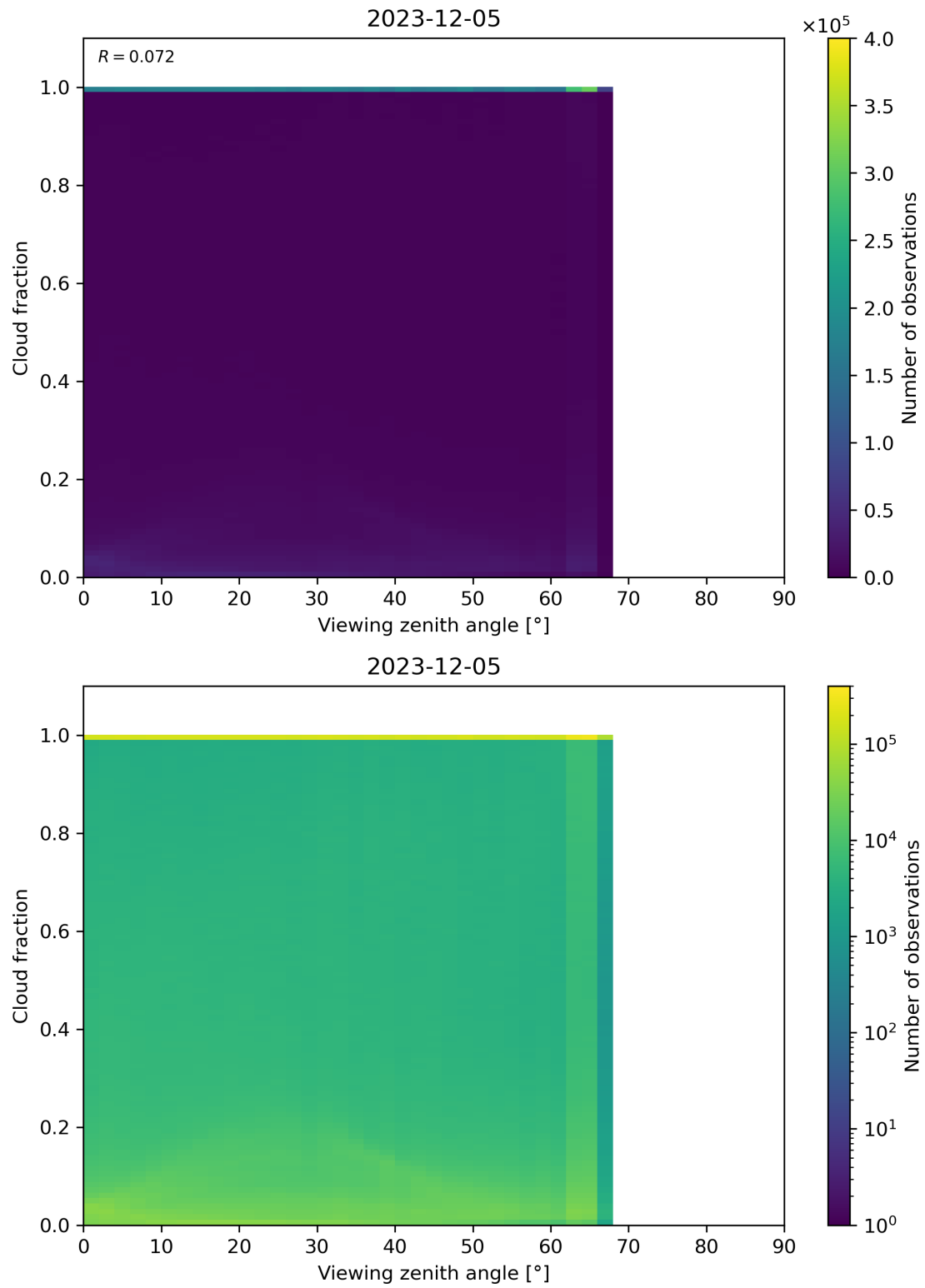
Figure 120: Scatter density plot of “Viewing zenith angle” against “Cloud fraction” for 2023-12-04 to 2023-12-06.
