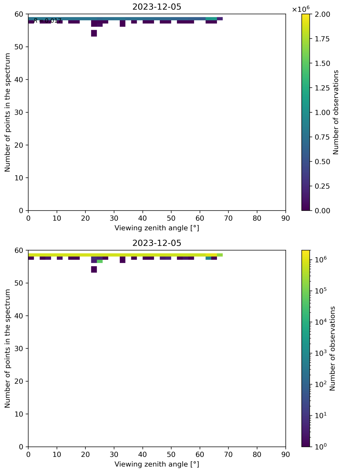
Figure 125: Scatter density plot of “Viewing zenith angle” against “Number of points in the spectrum” for 2023-12-04 to 2023-12-06.
