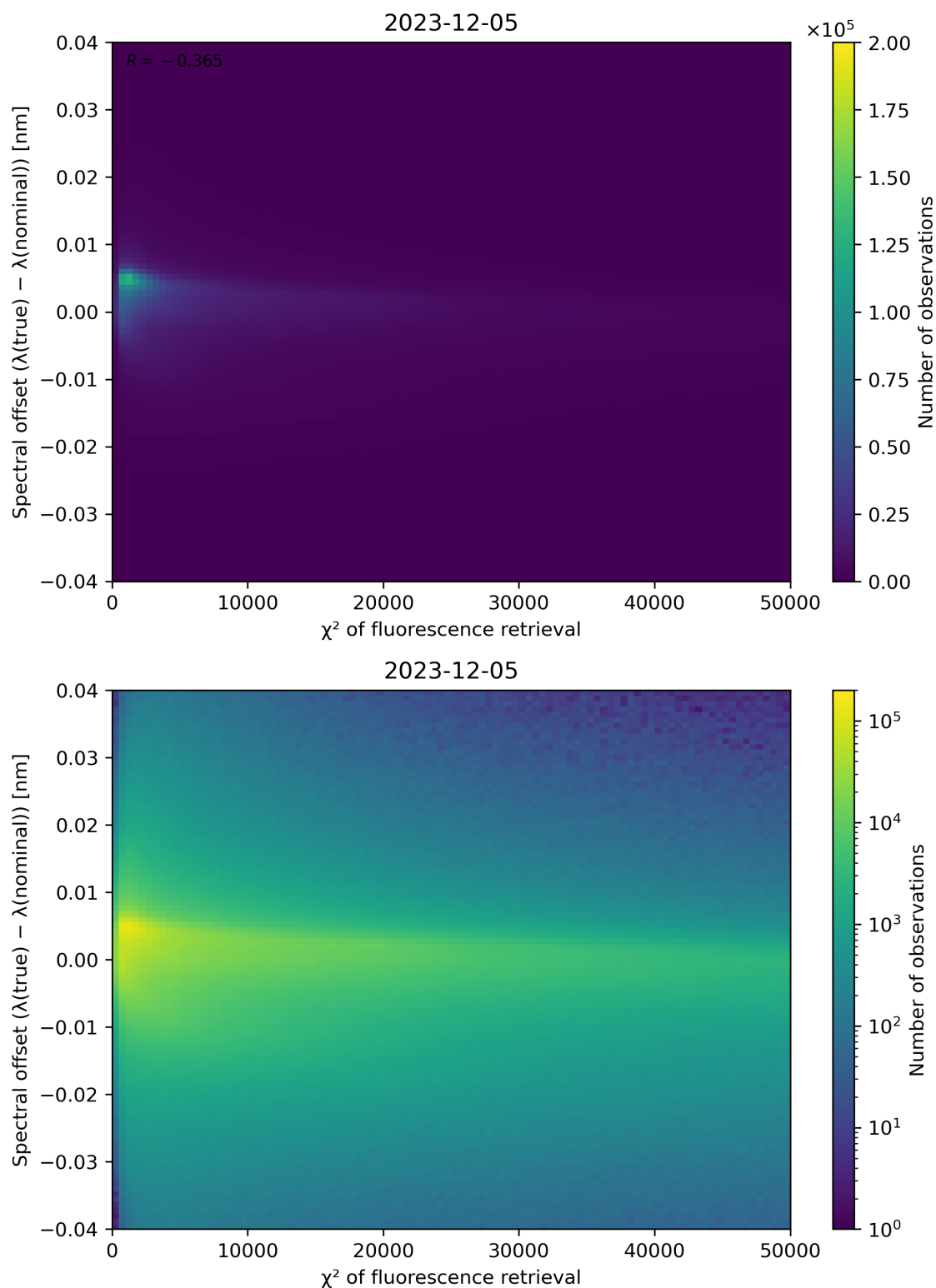
Figure 69: Scatter density plot of " \chi^2 of fluorescence retrieval" against "Spectral offset ( \lambda(\text{true}) - \lambda(\text{nominal}) )" for 2023-12-04 to 2023-12-06.
