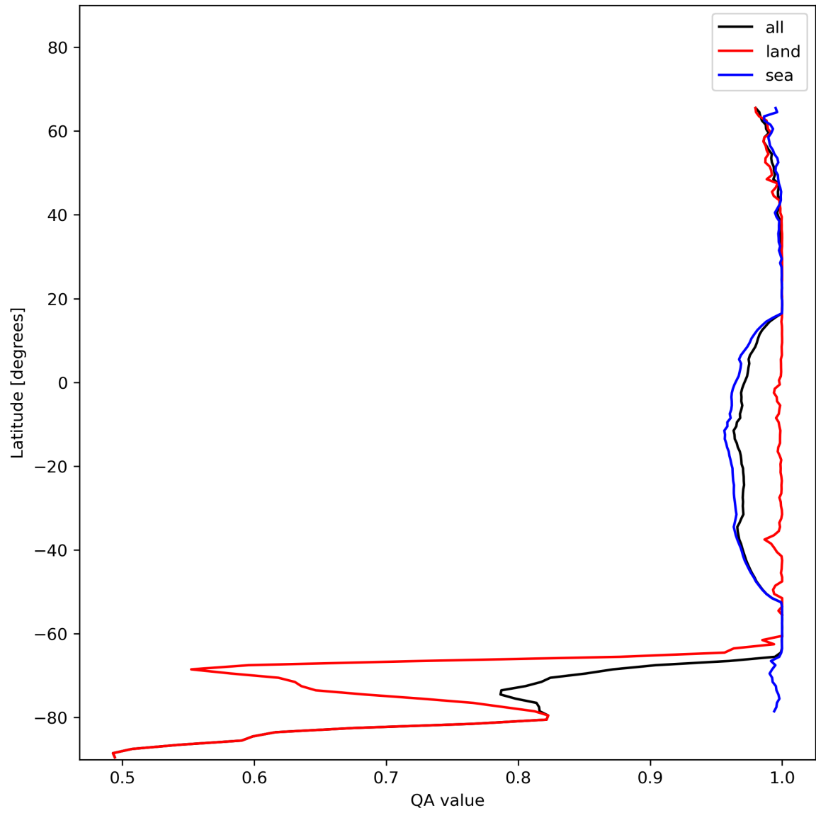
Figure 12: Zonal average of “QA value” for 2023-12-04 to 2023-12-06.
