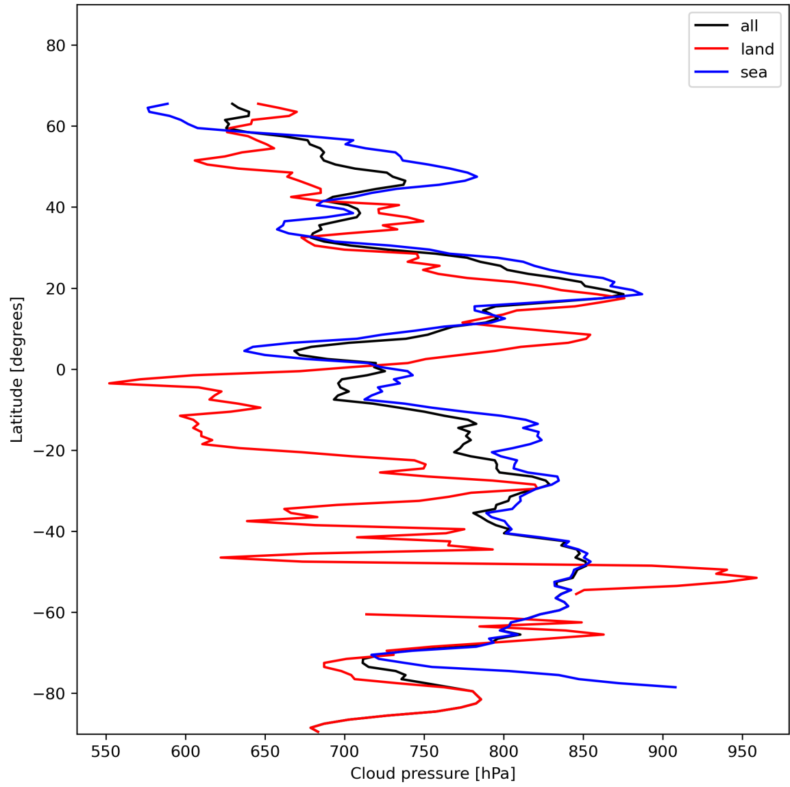
Figure 13: Zonal average of “Cloud pressure” for 2023-12-04 to 2023-12-06.
