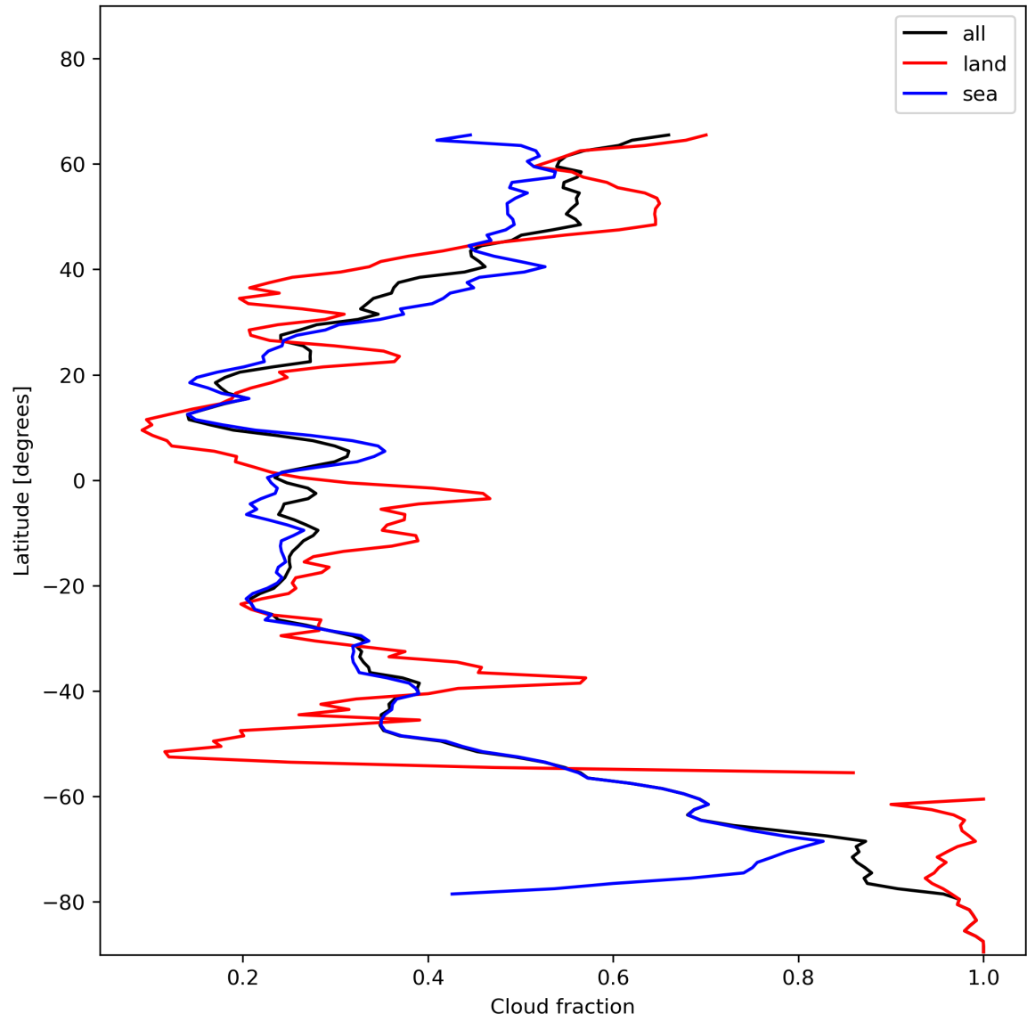
Figure 15: Zonal average of “Cloud fraction” for 2023-12-04 to 2023-12-06.
