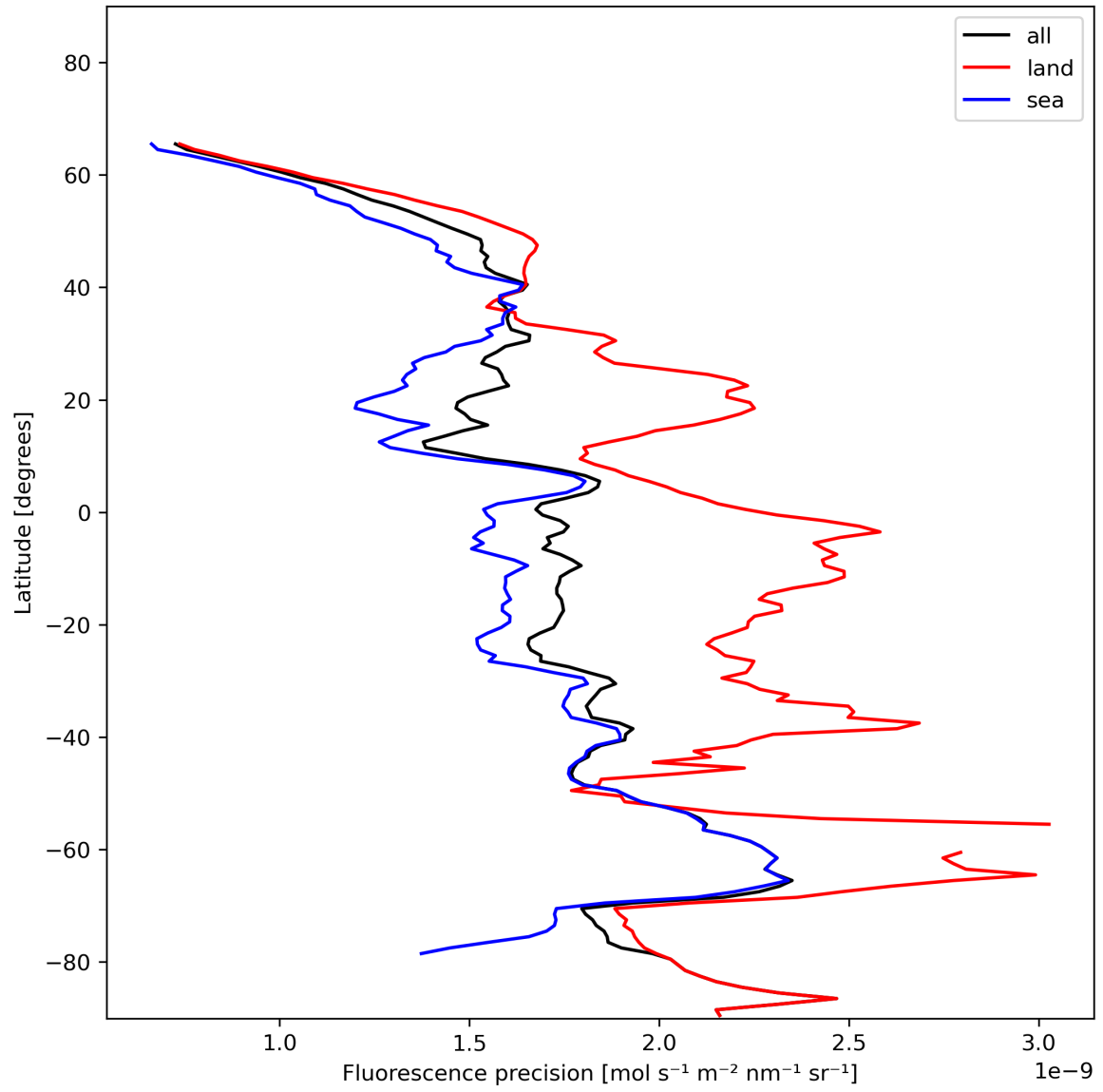
Figure 24: Zonal average of “Fluorescence precision” for 2023-12-04 to 2023-12-06.
