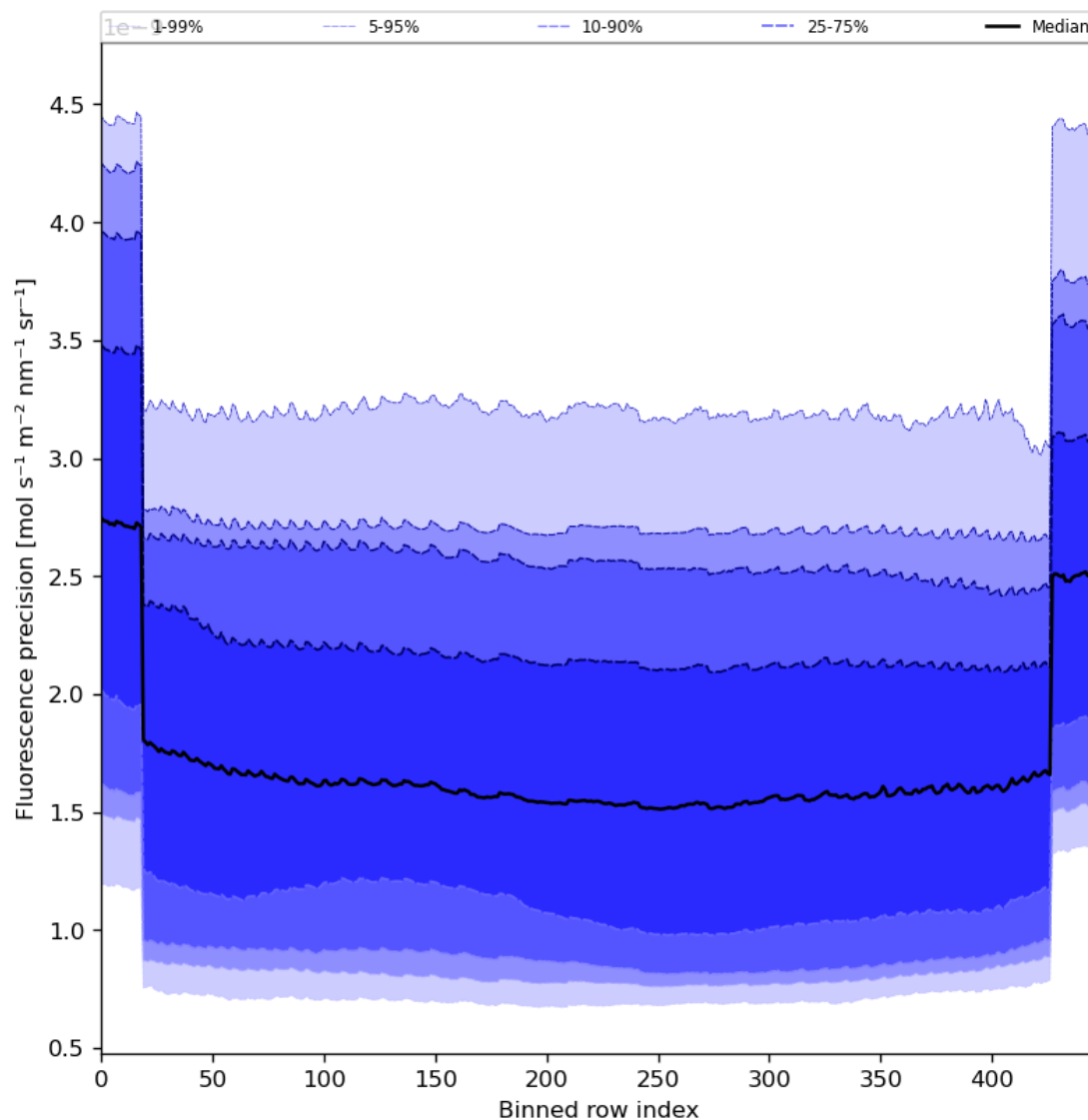
Figure 58: Along track statistics of “Fluorescence precision” for 2023-12-04 to 2023-12-06
