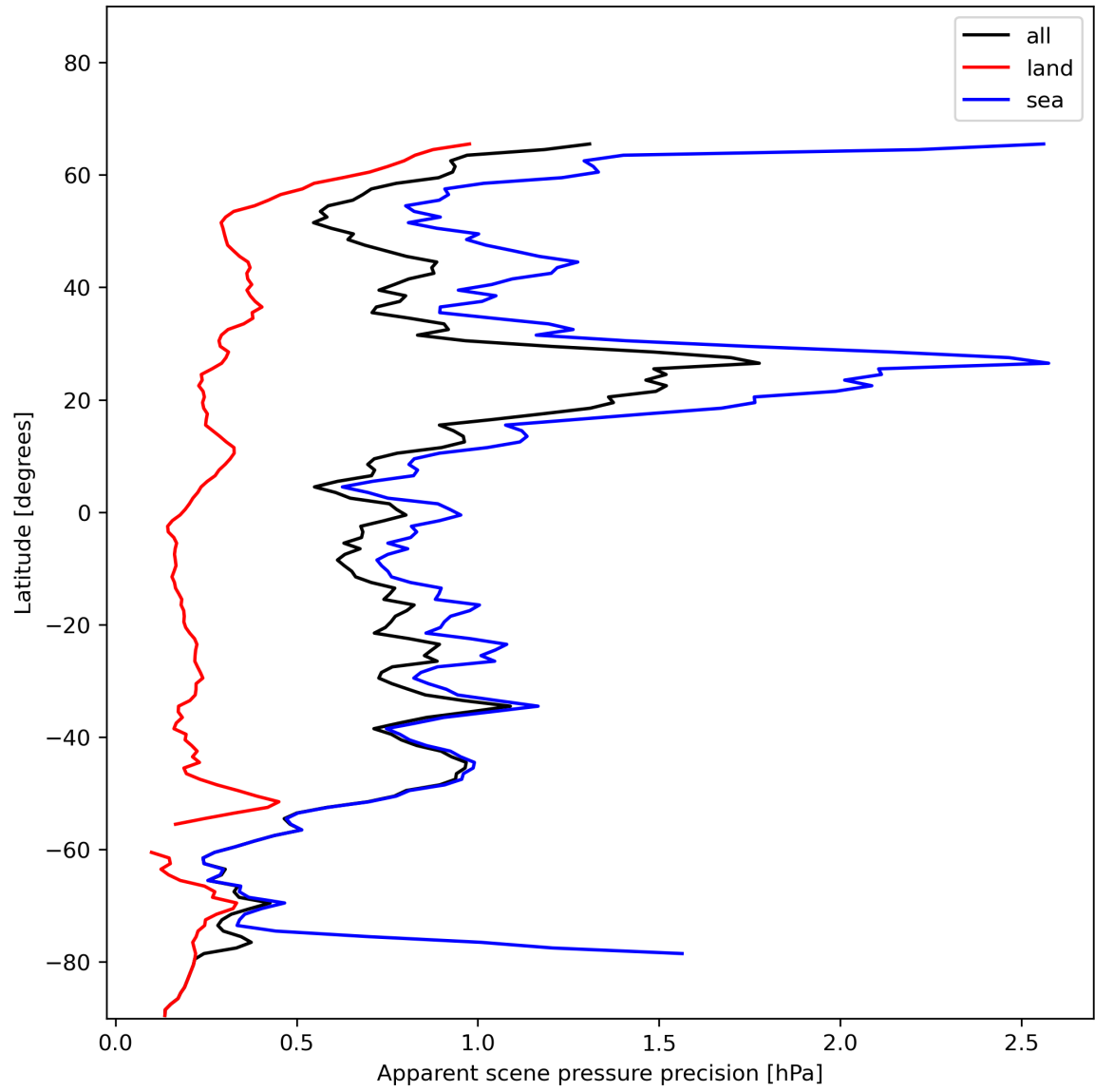
Figure 20: Zonal average of “Apparent scene pressure precision” for 2023-12-04 to 2023-12-06.
