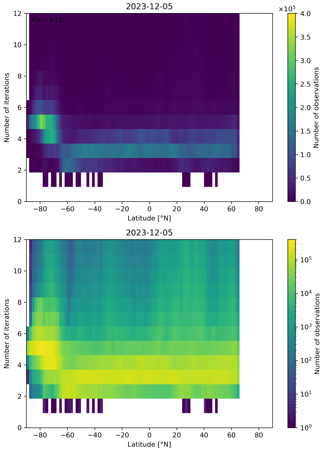
Figure 93: Scatter density plot of “Latitude” against “Number of iterations” for 2023-12-04 to 2023-12-06.
