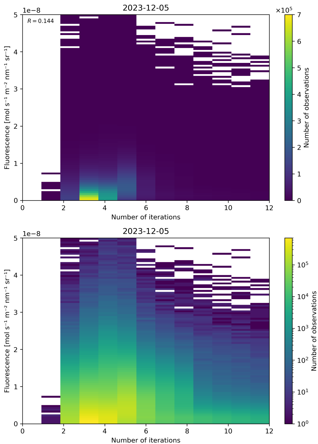
Figure 98: Scatter density plot of “Number of iterations” against “Fluorescence” for 2023-12-04 to 2023-12-06.
