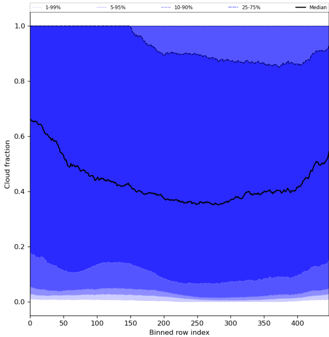
Figure 49: Along track statistics of “Cloud fraction” for 2023-12-04 to 2023-12-06
