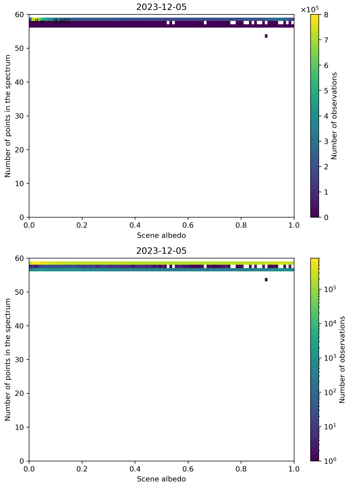
Figure 106: Scatter density plot of “Scene albedo” against “Number of points in the spectrum” for 2023-12-04 to 2023-12-06.
