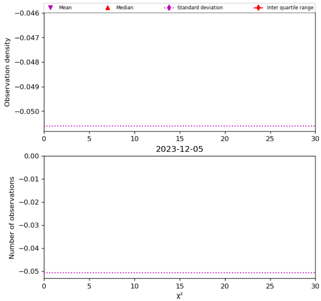
Figure 38: Histogram of “ \chi^2 ” for 2023-12-04 to 2023-12-06
