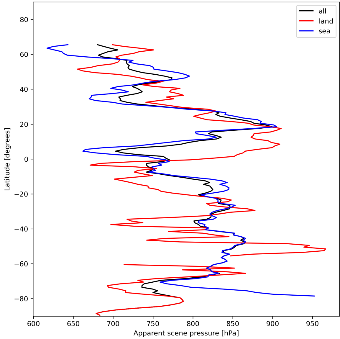
Figure 19: Zonal average of “Apparent scene pressure” for 2023-12-04 to 2023-12-06.
