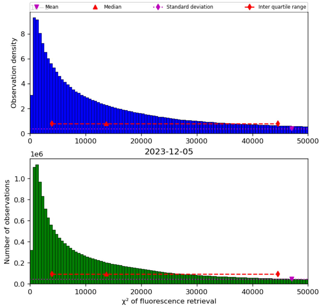
Figure 42: Histogram of “ \chi^2 of fluorescence retrieval” for 2023-12-04 to 2023-12-06
