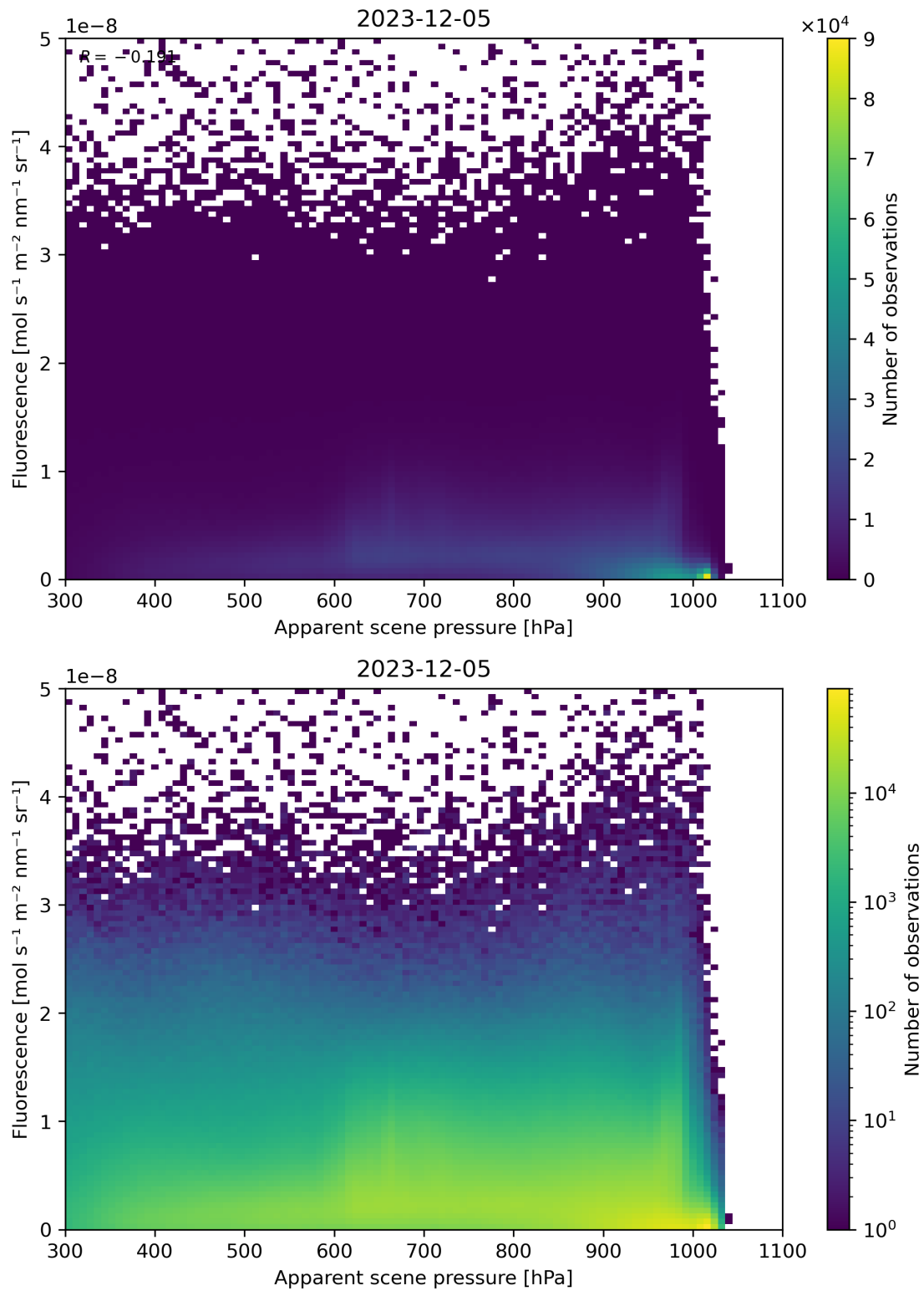
Figure 64: Scatter density plot of “Apparent scene pressure” against “Fluorescence” for 2023-12-04 to 2023-12-06.
