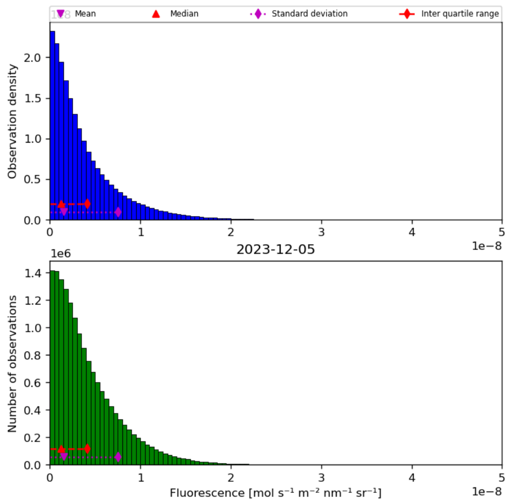
Figure 40: Histogram of “Fluorescence” for 2023-12-04 to 2023-12-06
