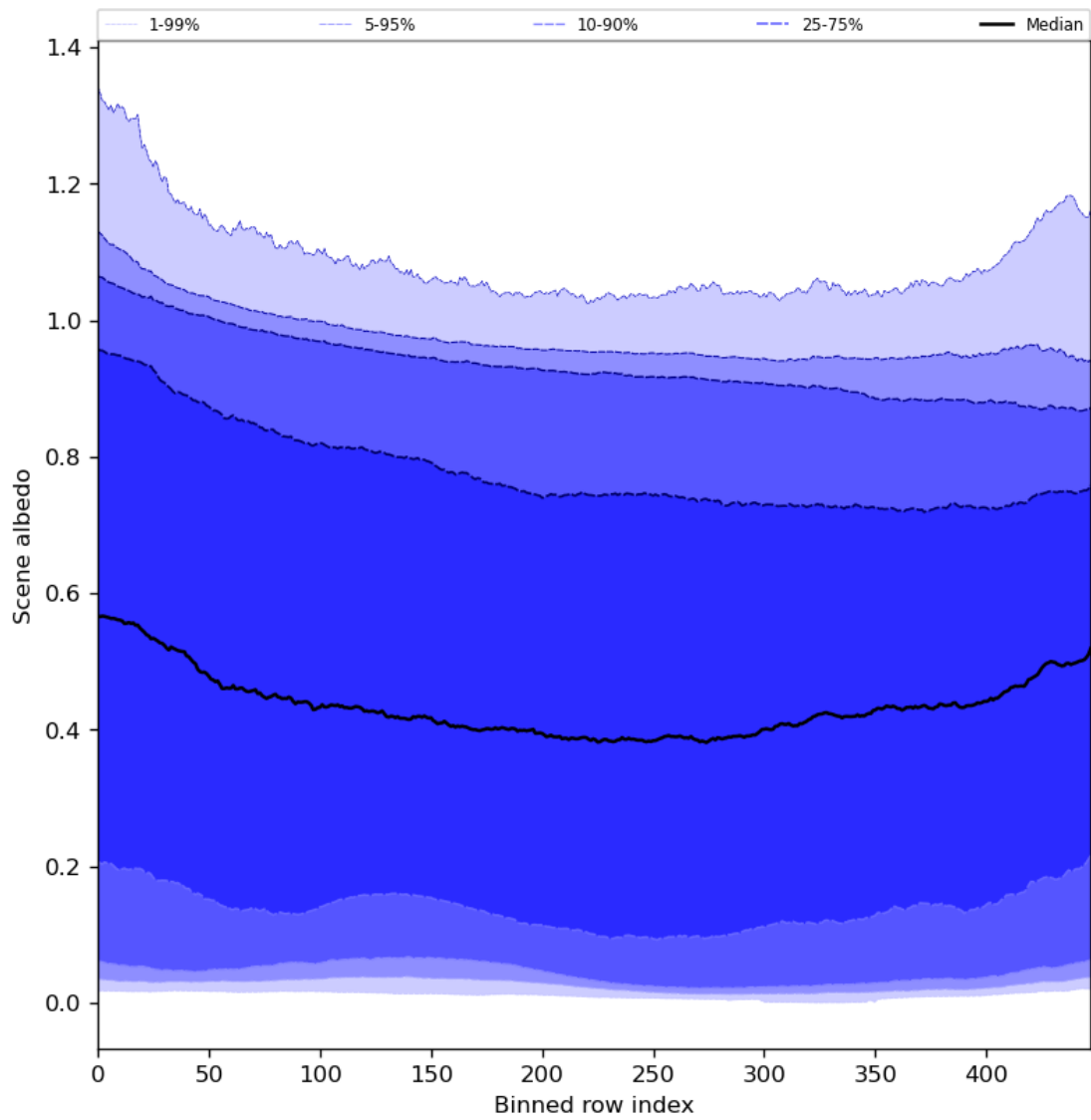
Figure 51: Along track statistics of “Scene albedo” for 2023-12-04 to 2023-12-06
