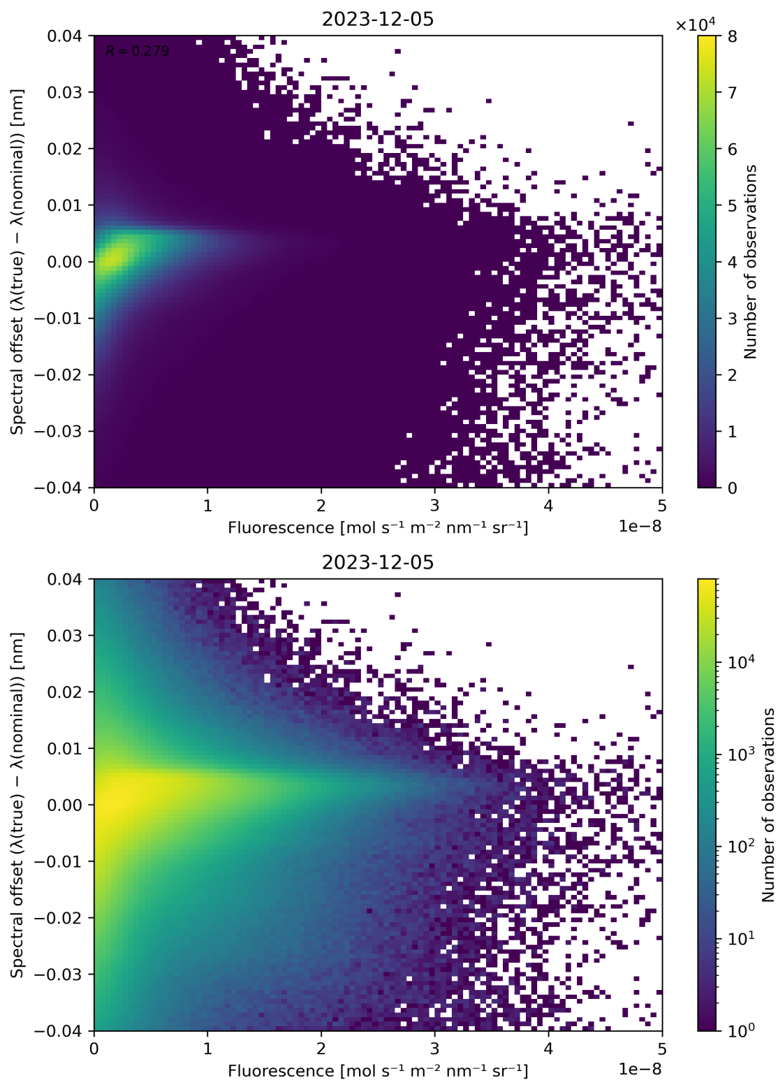
Figure 87: Scatter density plot of “Fluorescence” against “Spectral offset ( \lambda(\text{true}) - \lambda(\text{nominal}) )” for 2023-12-04 to 2023-12-06.
