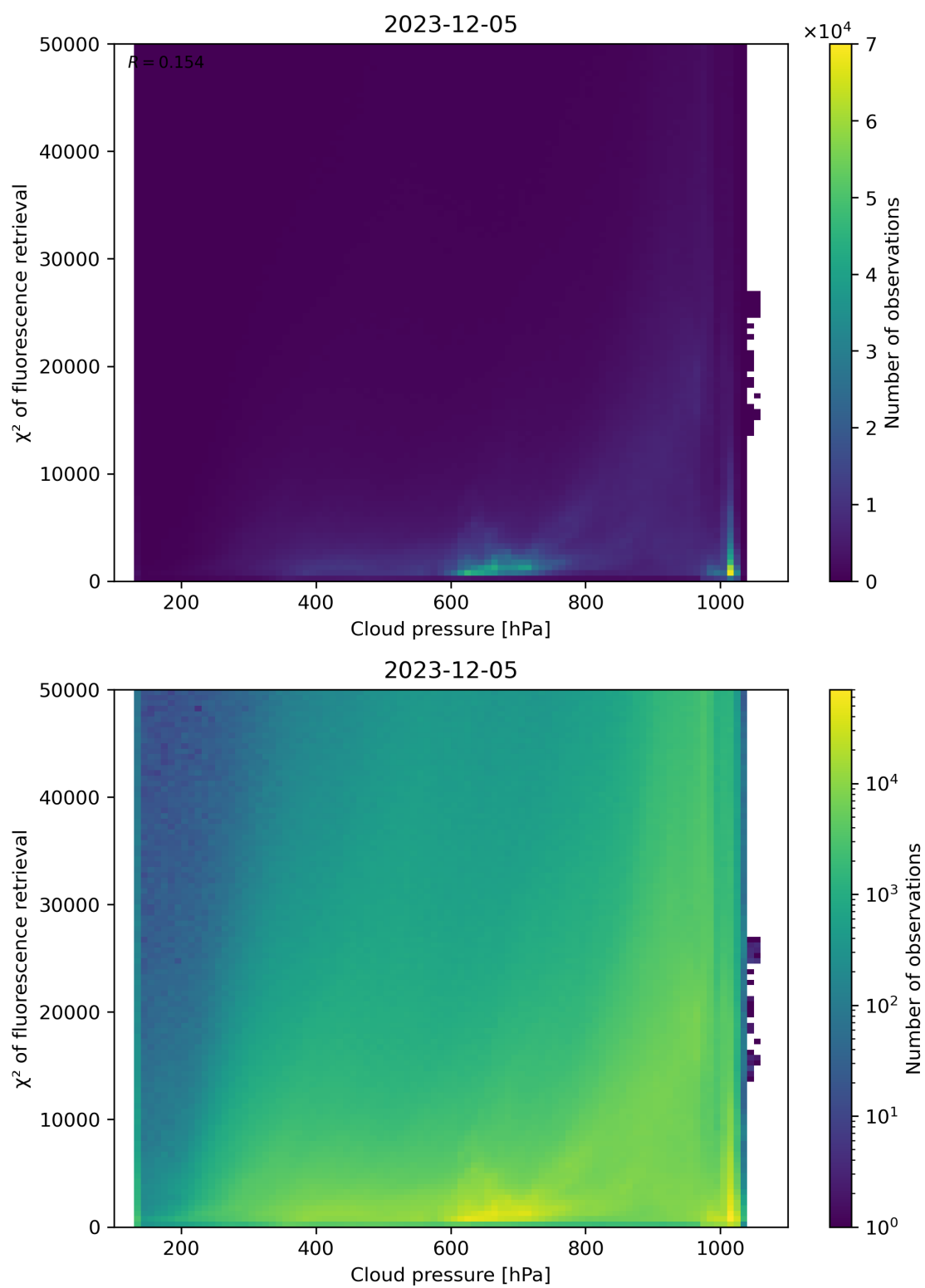
Figure 78: Scatter density plot of “Cloud pressure” against “ \chi^2 of fluorescence retrieval” for 2023-12-04 to 2023-12-06.
