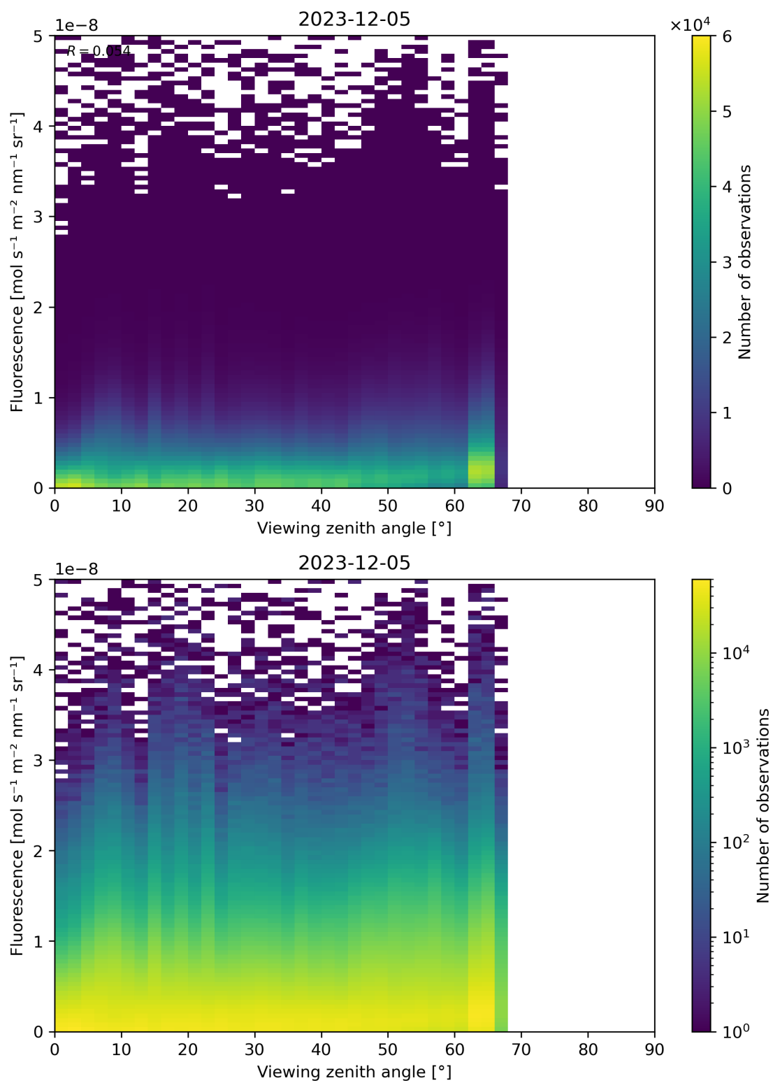
Figure 122: Scatter density plot of “Viewing zenith angle” against “Fluorescence” for 2023-12-04 to 2023-12-06.
