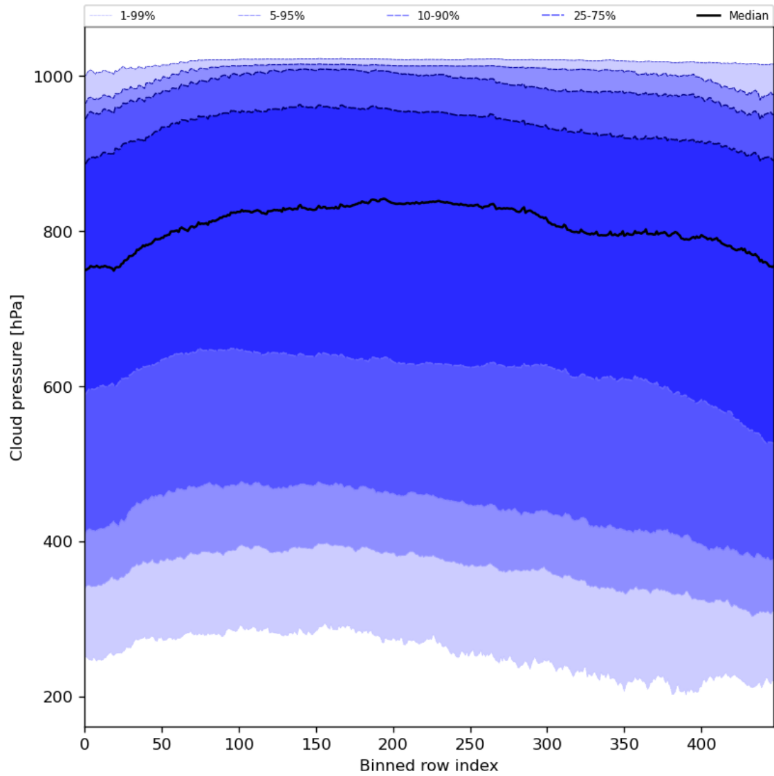
Figure 47: Along track statistics of “Cloud pressure” for 2023-12-04 to 2023-12-06
