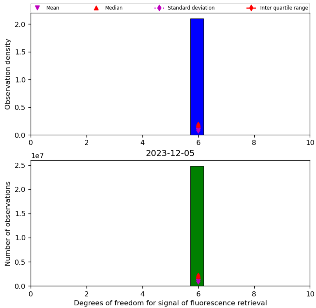
Figure 43: Histogram of “Degrees of freedom for signal of fluorescence retrieval” for 2023-12-04 to 2023-12-06
