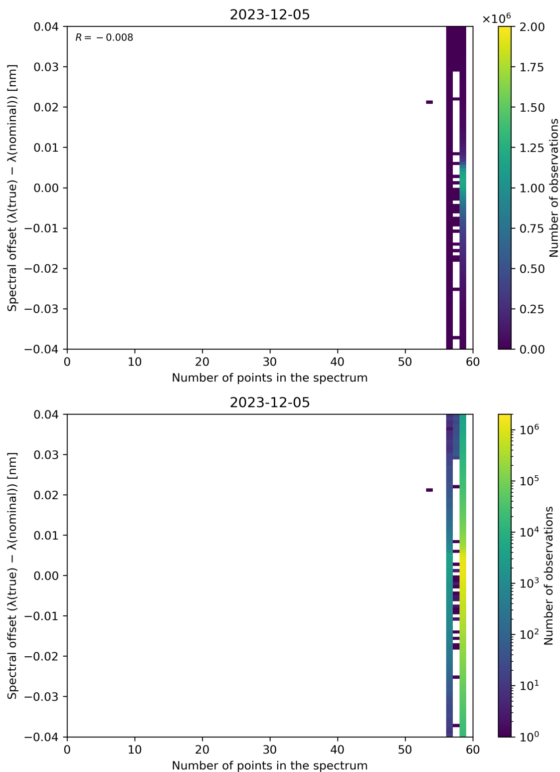
Figure 101: Scatter density plot of “Number of points in the spectrum” against “Spectral offset ( \lambda(\text{true}) - \lambda(\text{nominal}) )” for 2023-12-04 to 2023-12-06.
