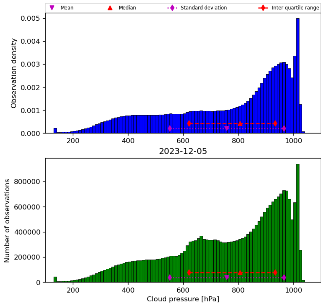
Figure 30: Histogram of “Cloud pressure” for 2023-12-04 to 2023-12-06
