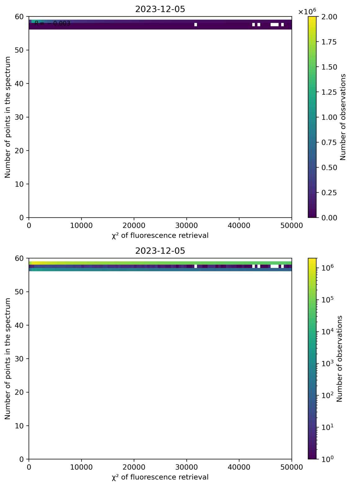
Figure 68: Scatter density plot of " \chi^2 of fluorescence retrieval" against "Number of points in the spectrum" for 2023-12-04 to 2023-12-06.
