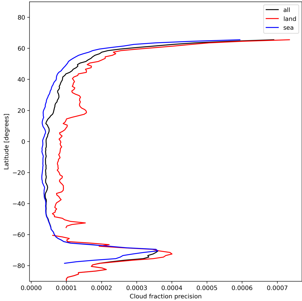
Figure 16: Zonal average of “Cloud fraction precision” for 2023-12-04 to 2023-12-06.
