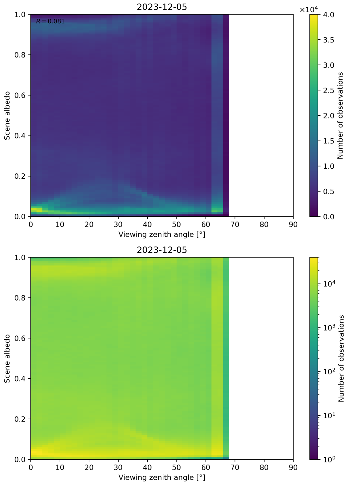
Figure 126: Scatter density plot of “Viewing zenith angle” against “Scene albedo” for 2023-12-04 to 2023-12-06.
