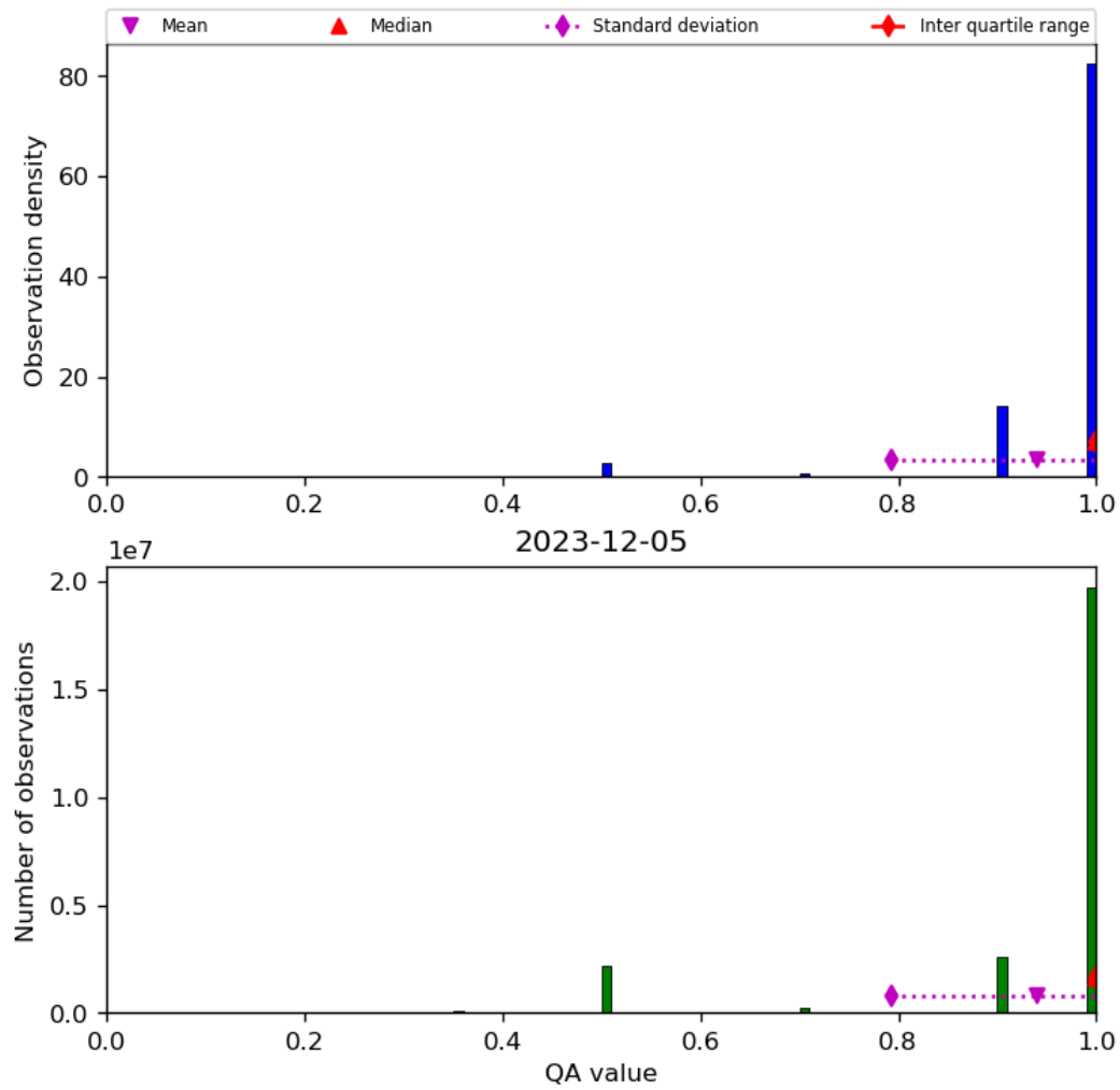
Figure 29: Histogram of “QA value” for 2023-12-04 to 2023-12-06
