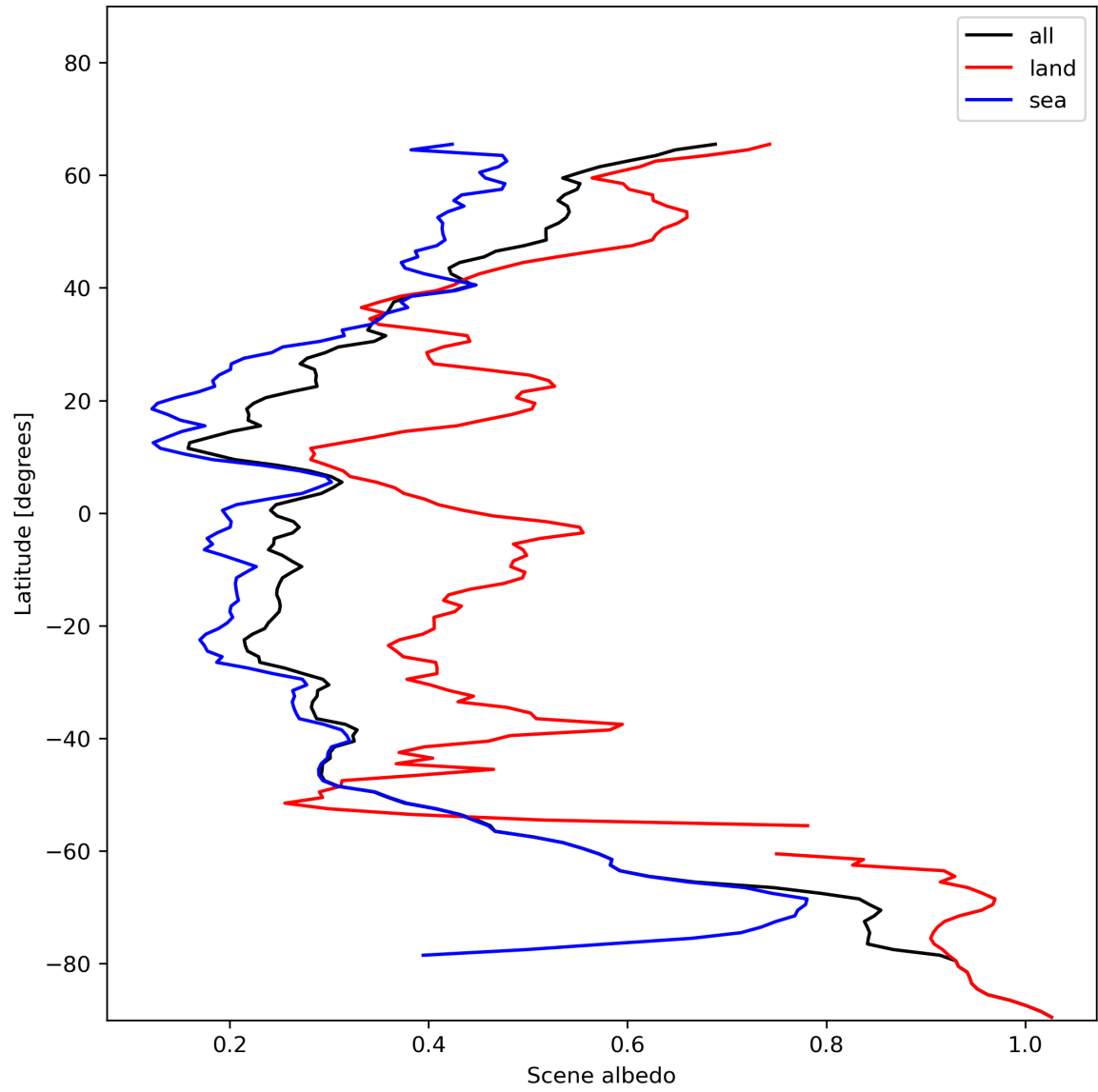
Figure 17: Zonal average of “Scene albedo” for 2023-12-04 to 2023-12-06.
