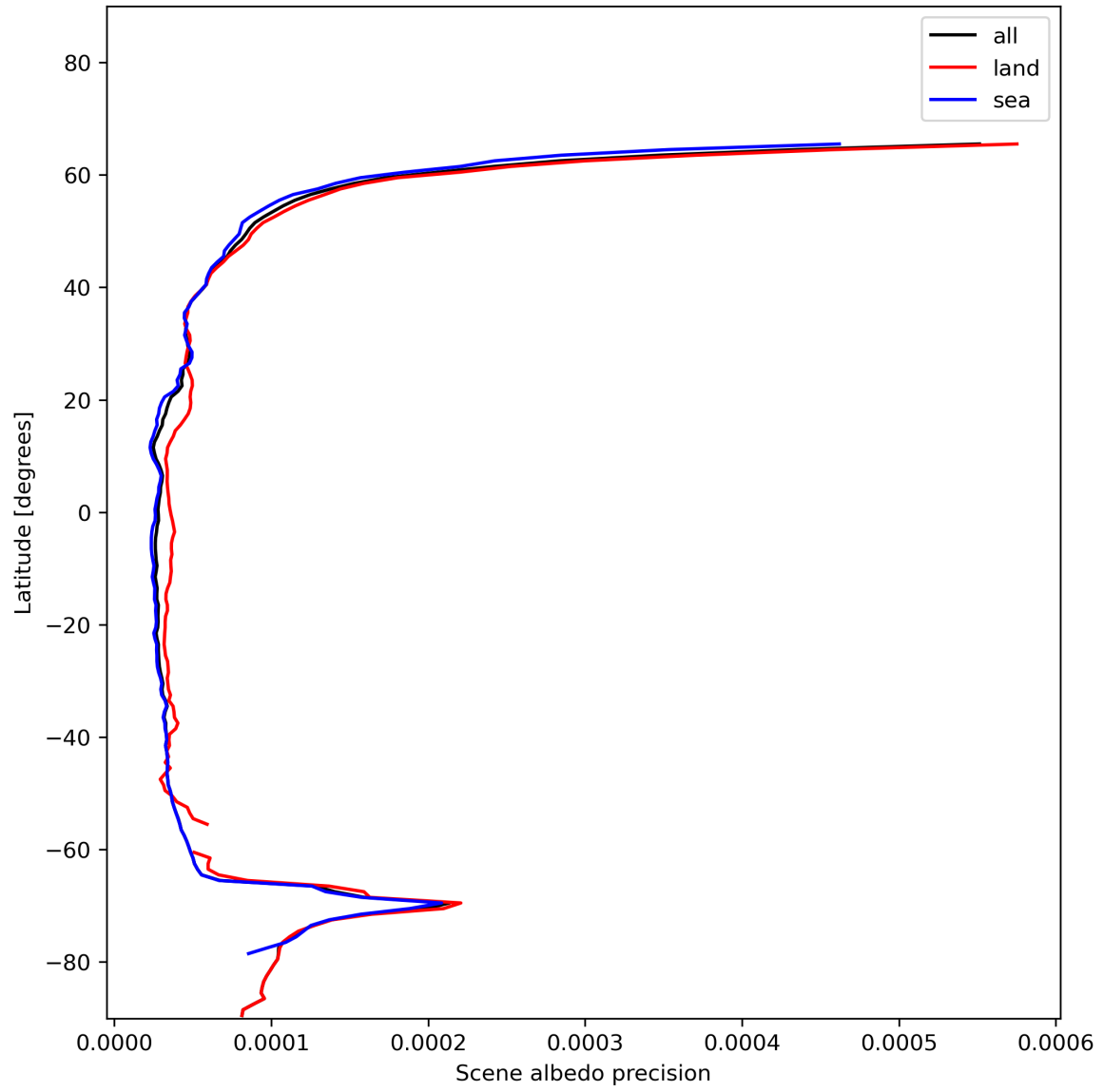
Figure 18: Zonal average of “Scene albedo precision” for 2023-12-04 to 2023-12-06.
