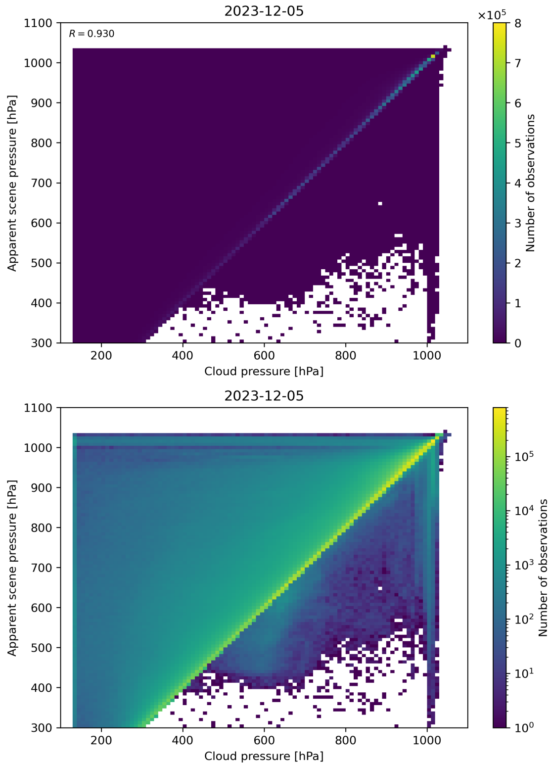
Figure 77: Scatter density plot of “Cloud pressure” against “Apparent scene pressure” for 2023-12-04 to 2023-12-06.
