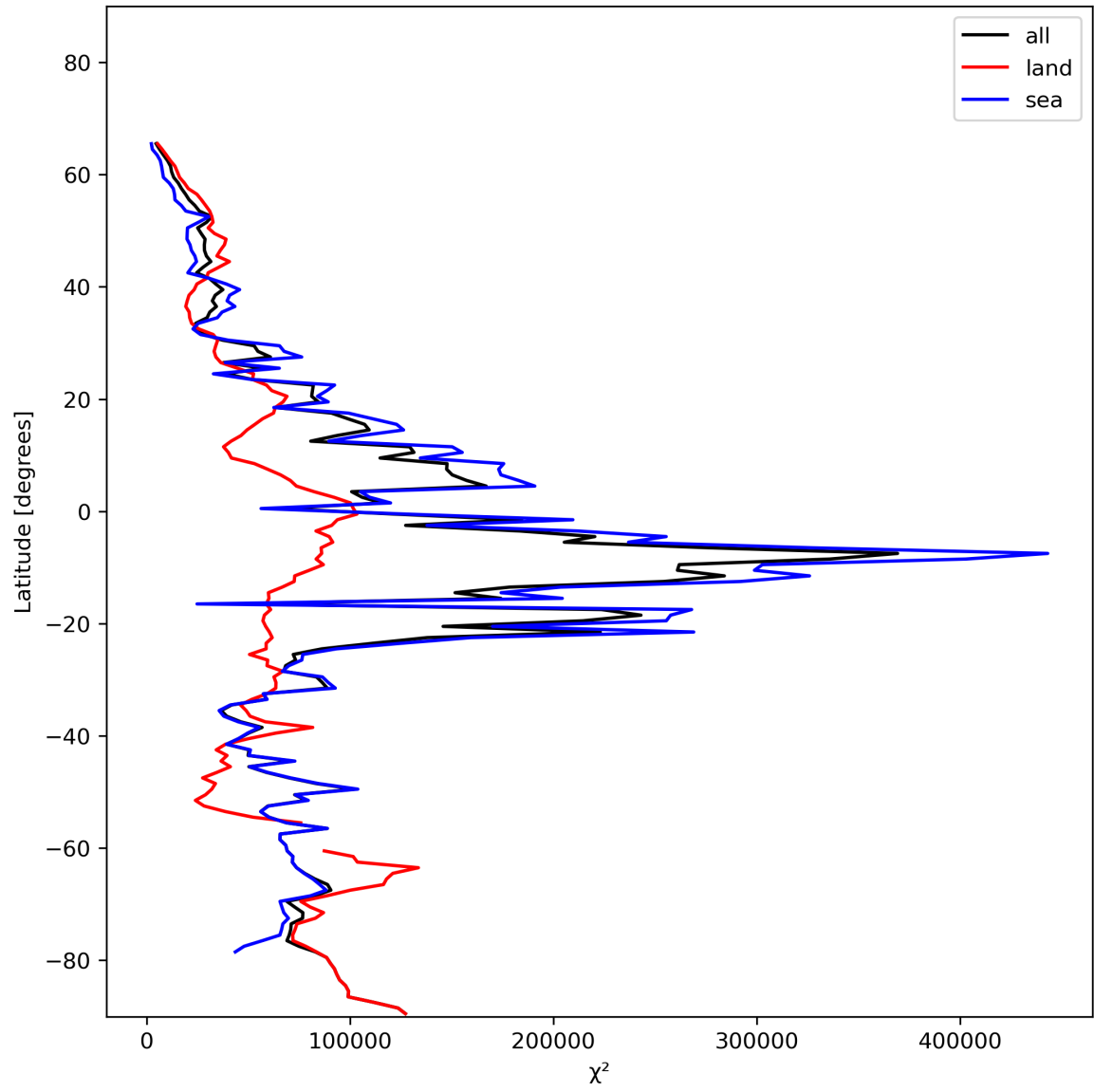
Figure 21: Zonal average of “ \chi^2 ” for 2023-12-04 to 2023-12-06.
