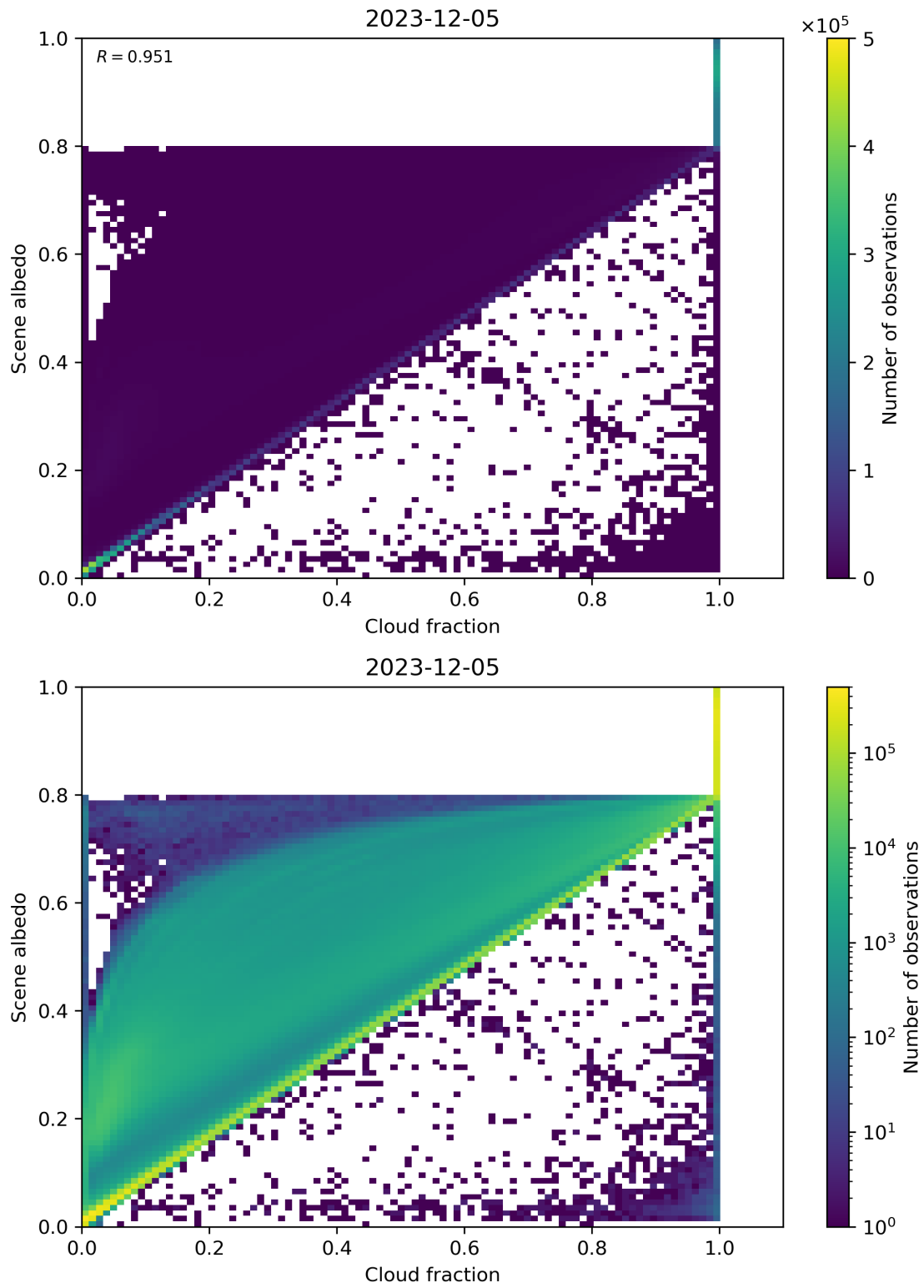
Figure 75: Scatter density plot of “Cloud fraction” against “Scene albedo” for 2023-12-04 to 2023-12-06.
