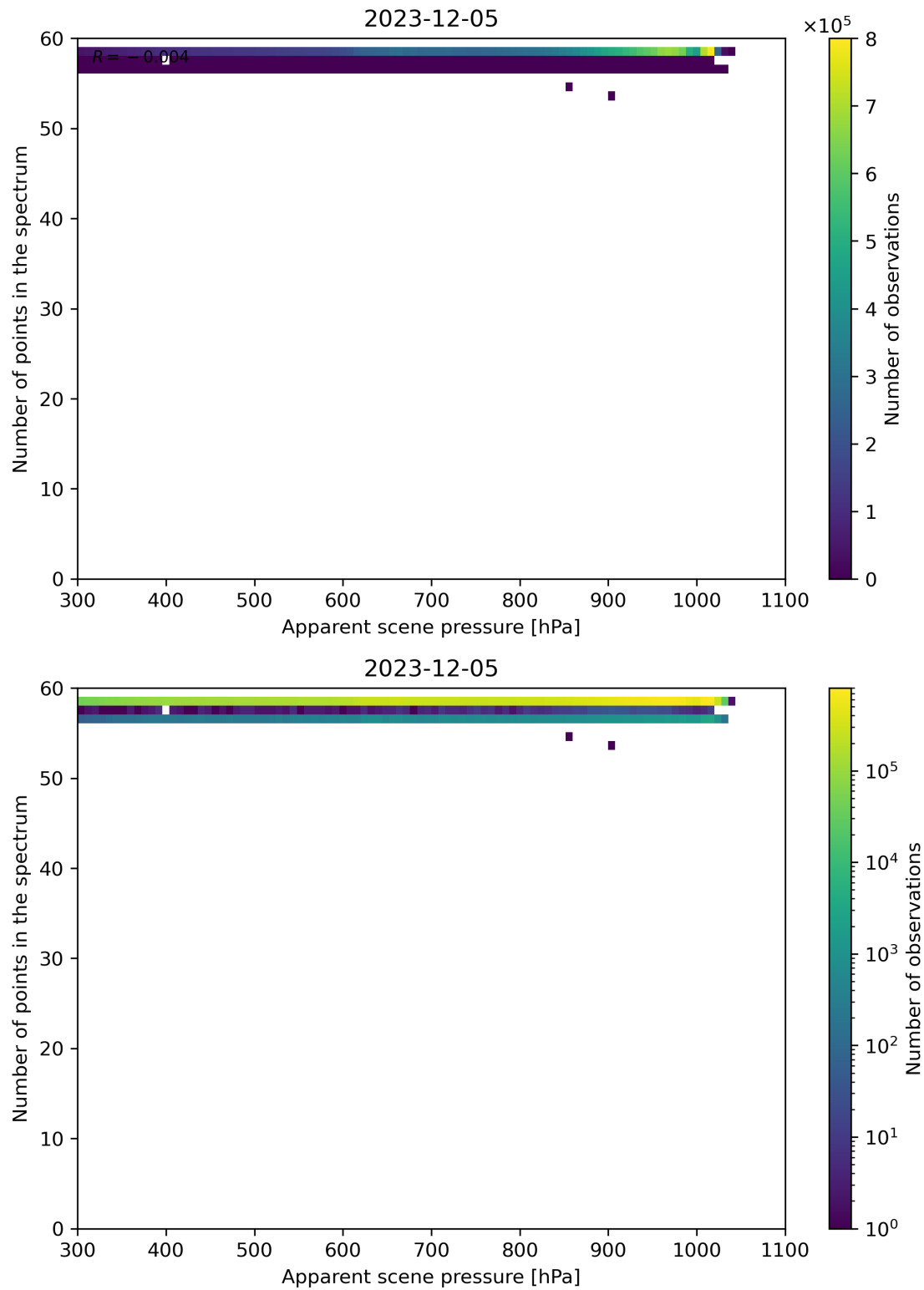
Figure 66: Scatter density plot of “Apparent scene pressure” against “Number of points in the spectrum” for 2023-12-04 to 2023-12-06.
