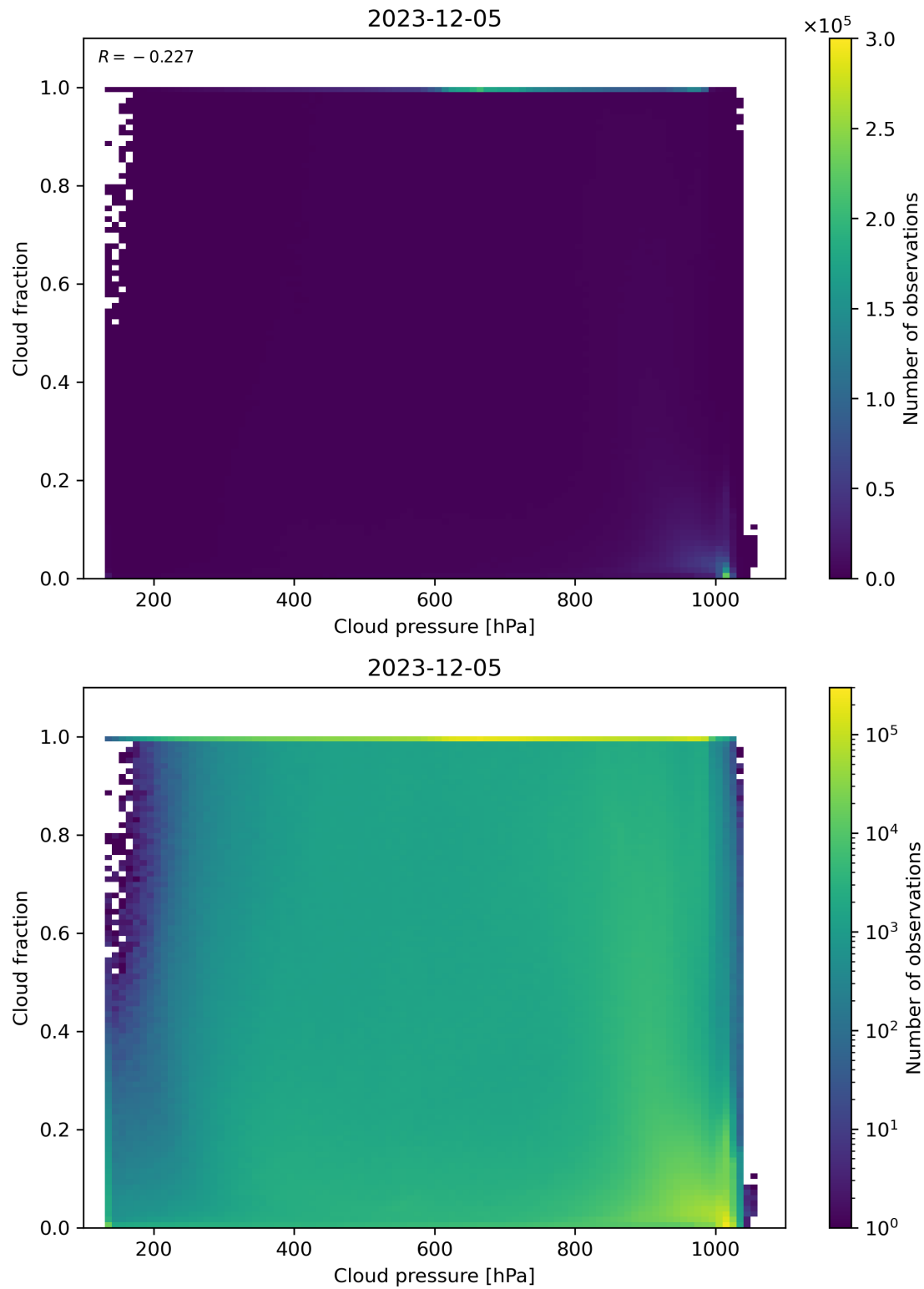
Figure 79: Scatter density plot of “Cloud pressure” against “Cloud fraction” for 2023-12-04 to 2023-12-06.
