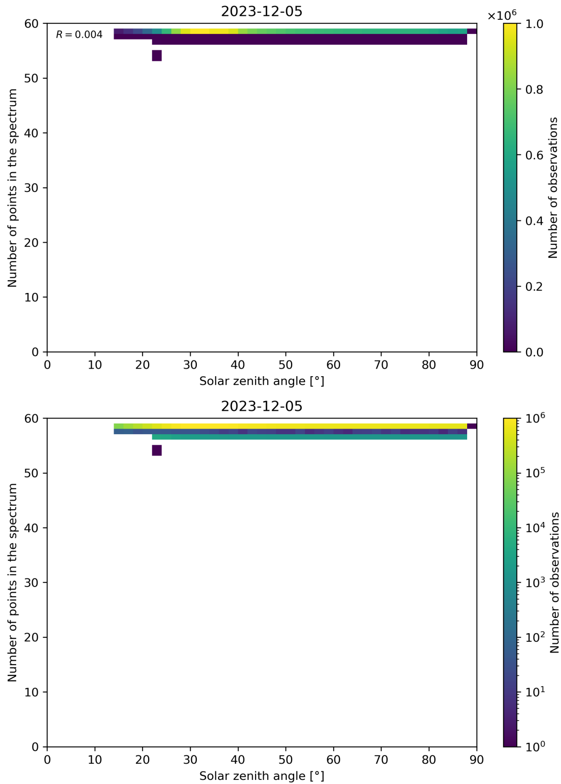
Figure 115: Scatter density plot of “Solar zenith angle” against “Number of points in the spectrum” for 2023-12-04 to 2023-12-06.
