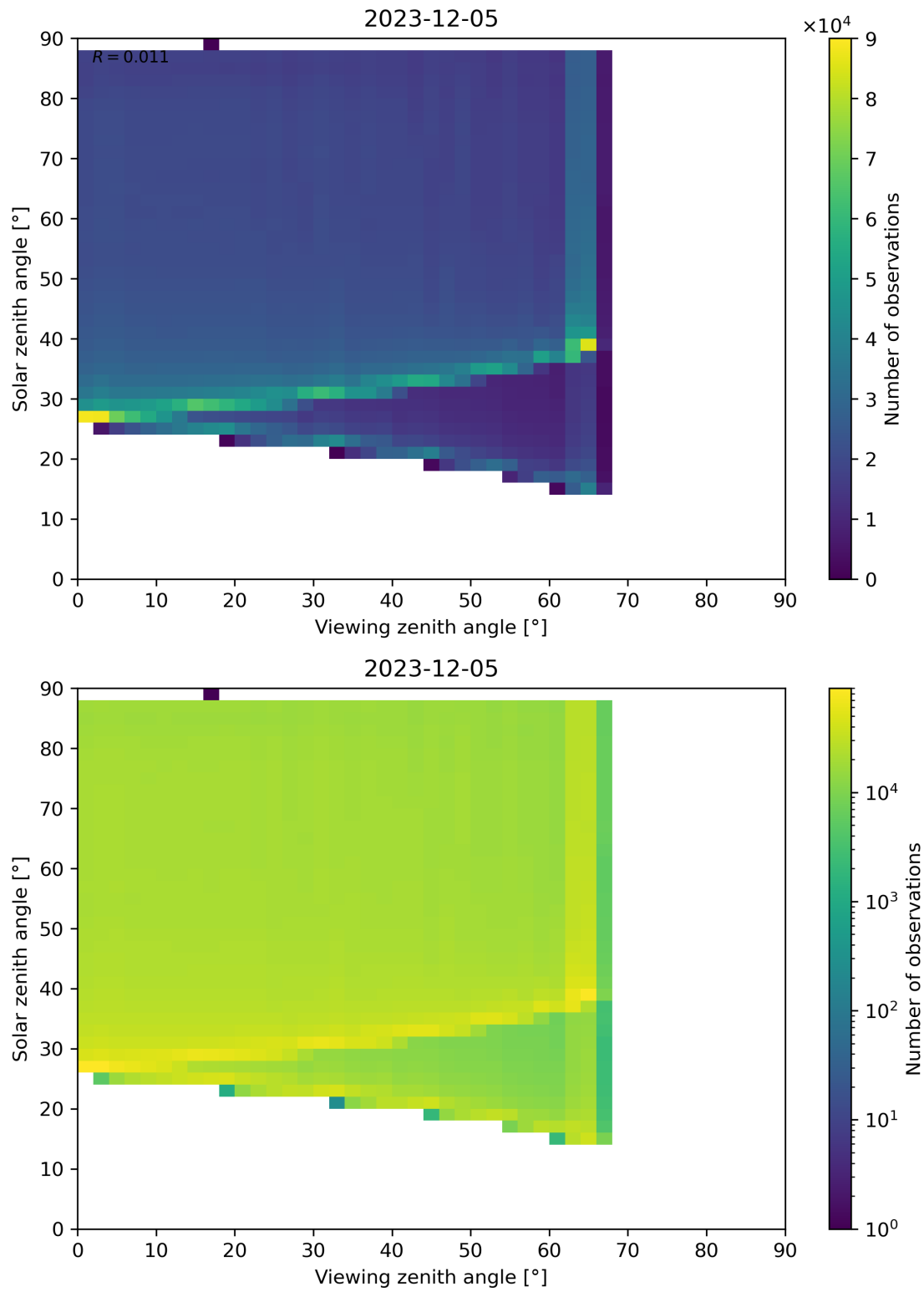
Figure 127: Scatter density plot of “Viewing zenith angle” against “Solar zenith angle” for 2023-12-04 to 2023-12-06.
