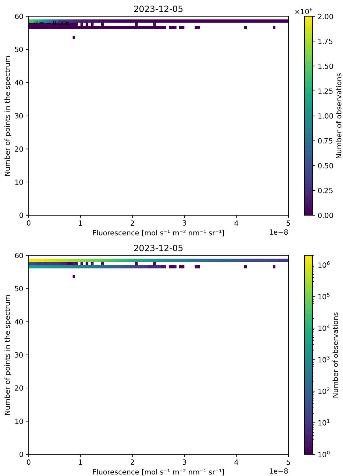
Figure 86: Scatter density plot of “Fluorescence” against “Number of points in the spectrum” for 2023-12-04 to 2023-12-06.
