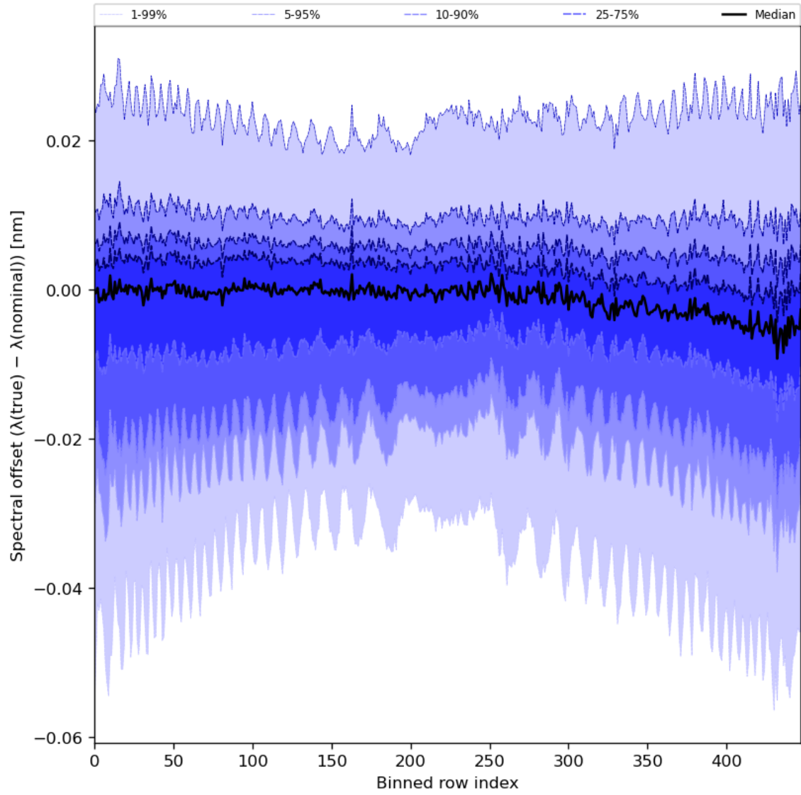
Figure 62: Along track statistics of “Spectral offset ( \lambda(\text{true}) - \lambda(\text{nominal}) )” for 2023-12-04 to 2023-12-06
