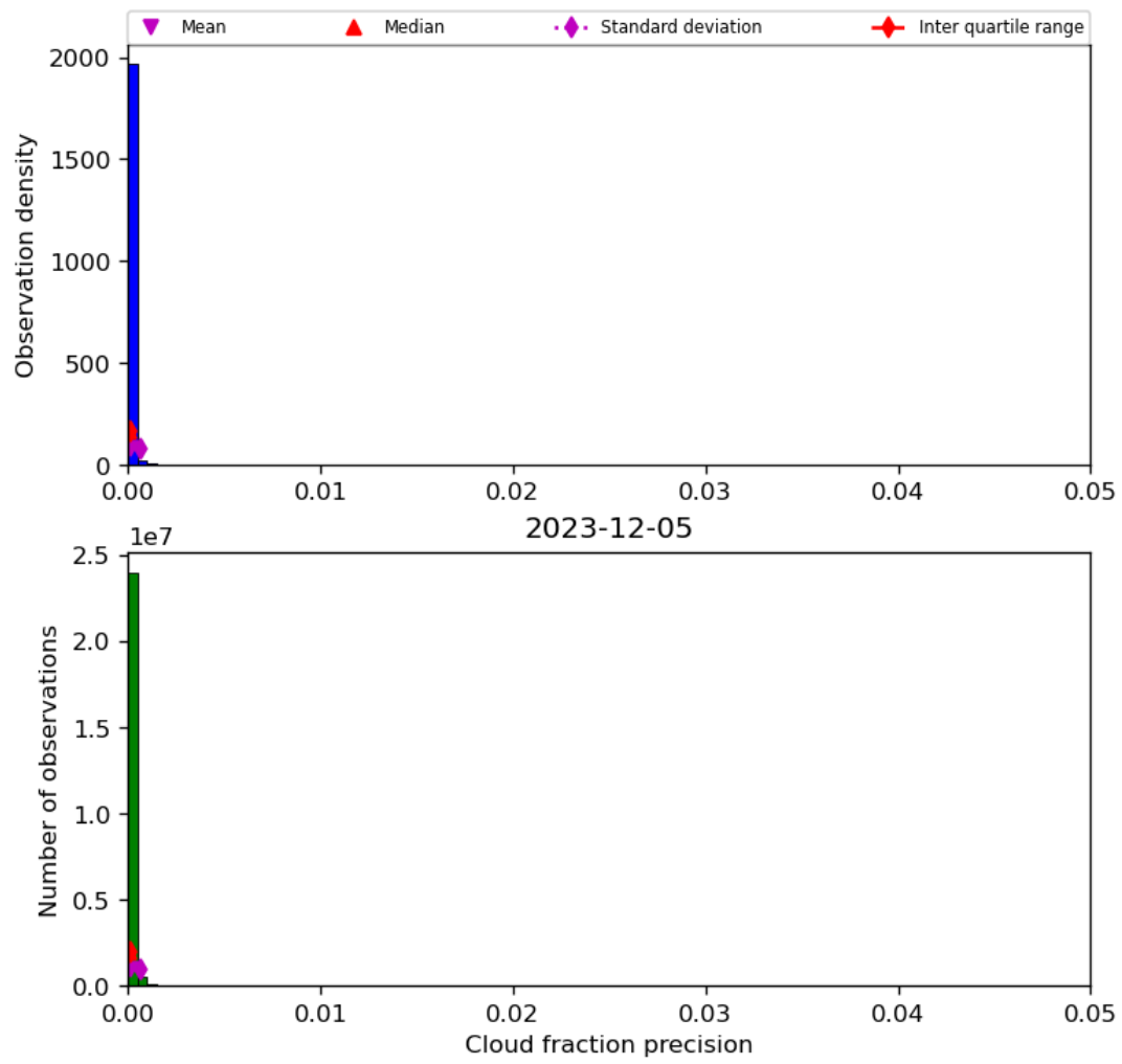
Figure 33: Histogram of “Cloud fraction precision” for 2023-12-04 to 2023-12-06
