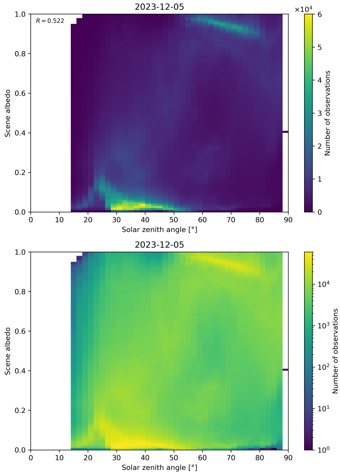
Figure 116: Scatter density plot of “Solar zenith angle” against “Scene albedo” for 2023-12-04 to 2023-12-06.
