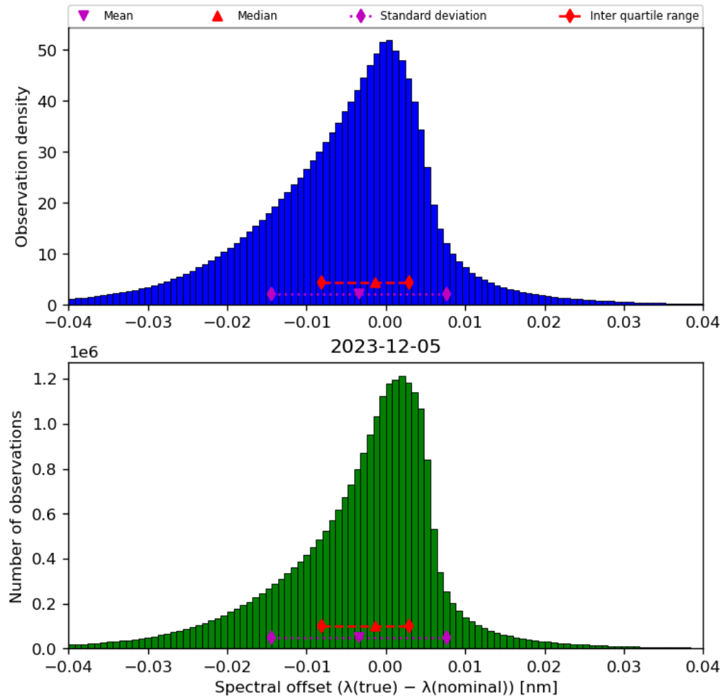
Figure 45: Histogram of “Spectral offset ( \lambda(\text{true}) - \lambda(\text{nominal}) )” for 2023-12-04 to 2023-12-06
