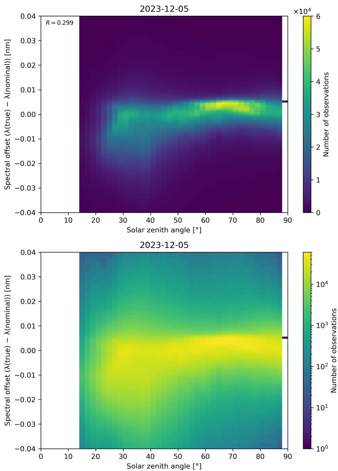
Figure 117: Scatter density plot of “Solar zenith angle” against “Spectral offset ( \lambda(\text{true}) - \lambda(\text{nominal}) )” for 2023-12-04 to 2023-12-06.
