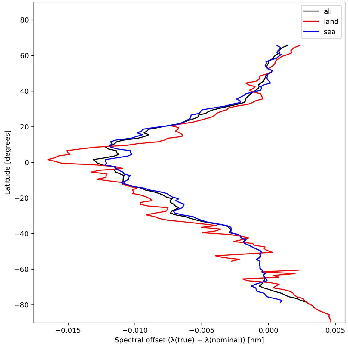
Figure 28: Zonal average of “Spectral offset ( \lambda(\text{true}) - \lambda(\text{nominal}) )” for 2023-12-04 to 2023-12-06.
