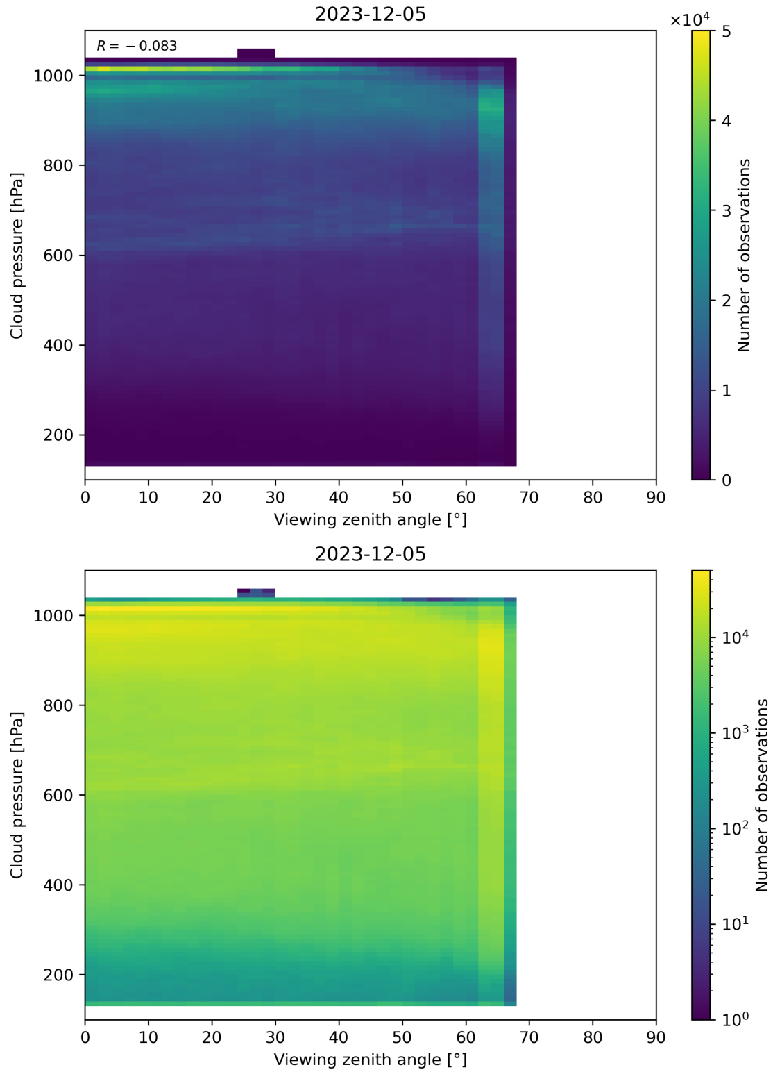
Figure 121: Scatter density plot of “Viewing zenith angle” against “Cloud pressure” for 2023-12-04 to 2023-12-06.
