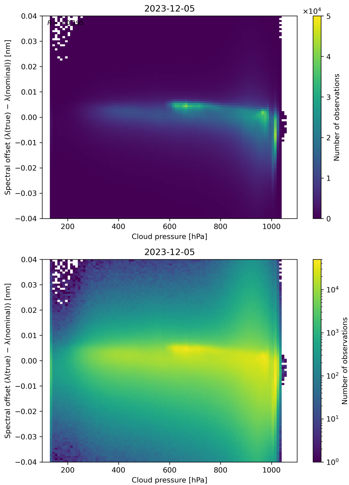
Figure 84: Scatter density plot of “Cloud pressure” against “Spectral offset ( \lambda(\text{true}) - \lambda(\text{nominal}) )” for 2023-12-04 to 2023-12-06.
