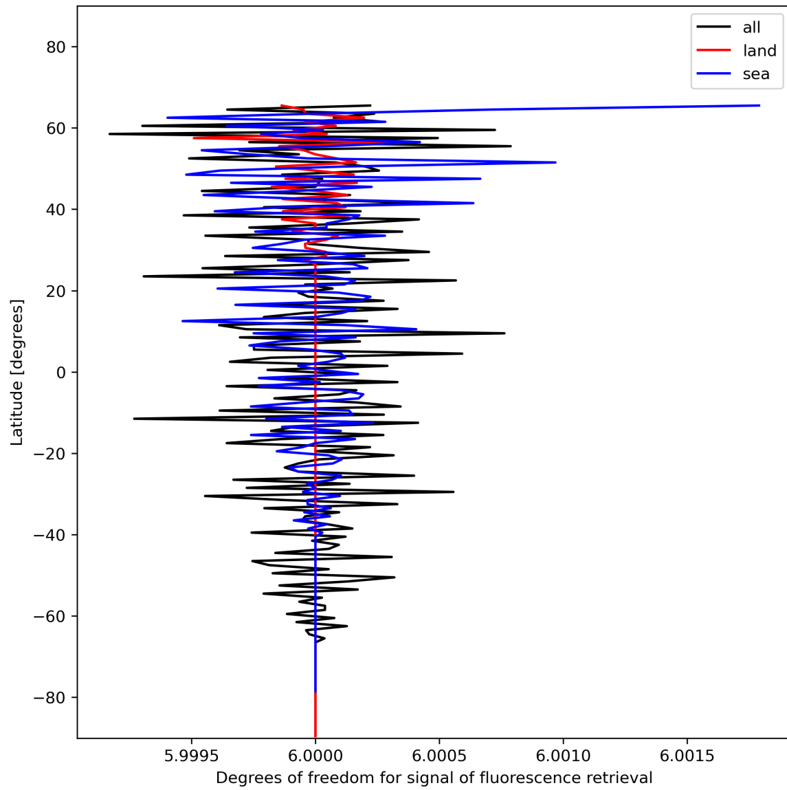
Figure 26: Zonal average of “Degrees of freedom for signal of fluorescence retrieval” for 2023-12-04 to 2023-12-06.
