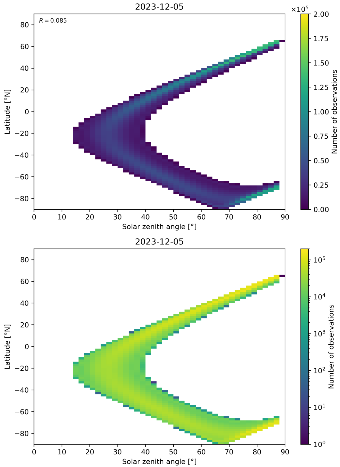
Figure 113: Scatter density plot of “Solar zenith angle” against “Latitude” for 2023-12-04 to 2023-12-06.
