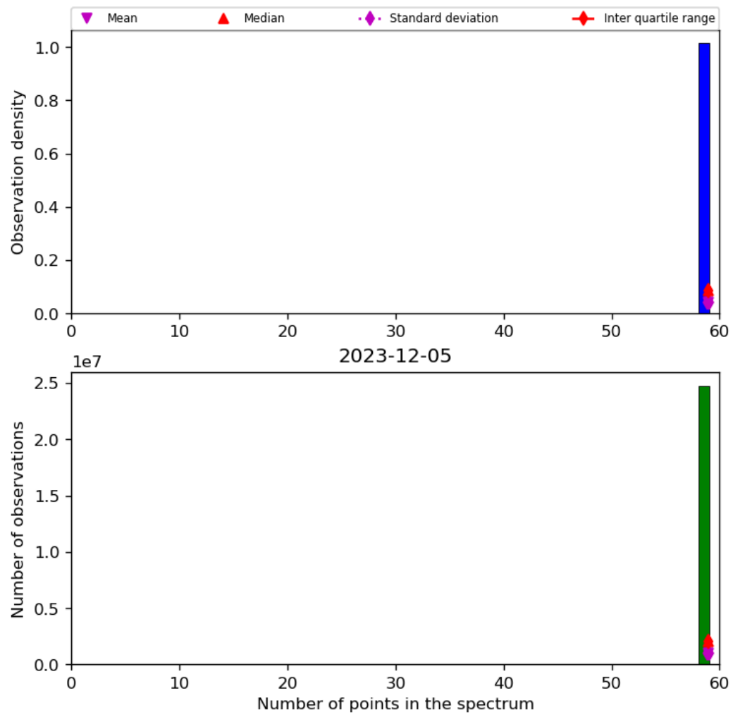
Figure 44: Histogram of “Number of points in the spectrum” for 2023-12-04 to 2023-12-06
