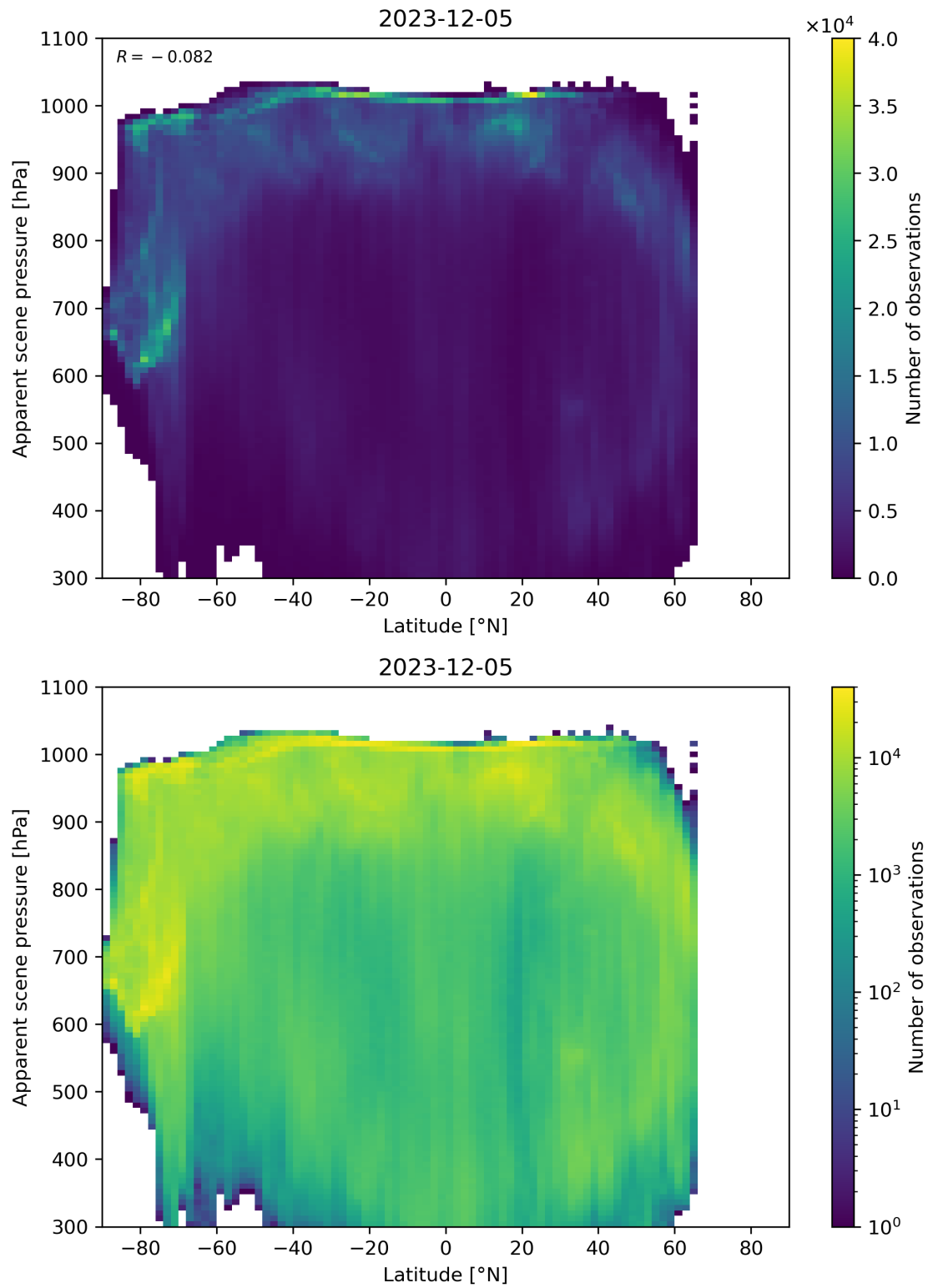
Figure 88: Scatter density plot of “Latitude” against “Apparent scene pressure” for 2023-12-04 to 2023-12-06.
