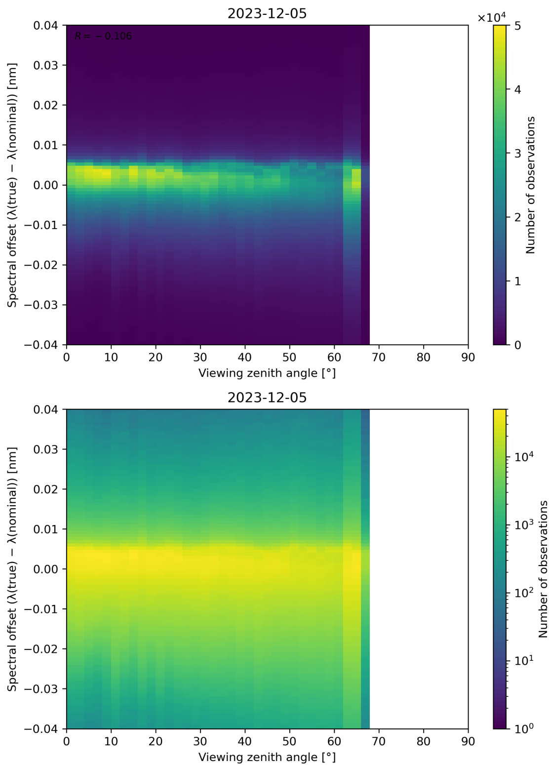
Figure 128: Scatter density plot of “Viewing zenith angle” against “Spectral offset ( \lambda(\text{true}) - \lambda(\text{nominal}) )” for 2023-12-04 to 2023-12-06.
