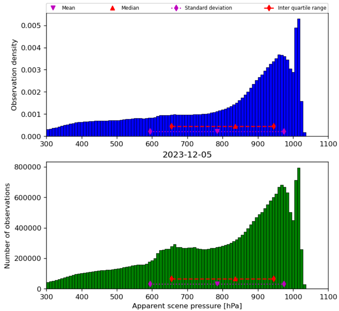
Figure 36: Histogram of “Apparent scene pressure” for 2023-12-04 to 2023-12-06
