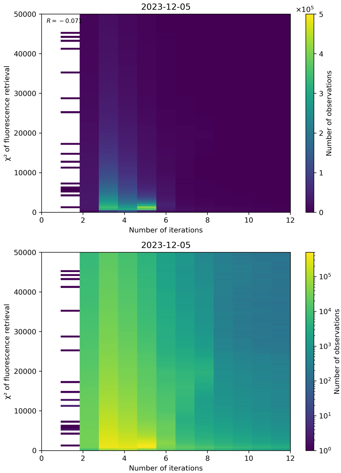
Figure 97: Scatter density plot of “Number of iterations” against “ \chi^2 of fluorescence retrieval” for 2023-12-04 to 2023-12-06.
