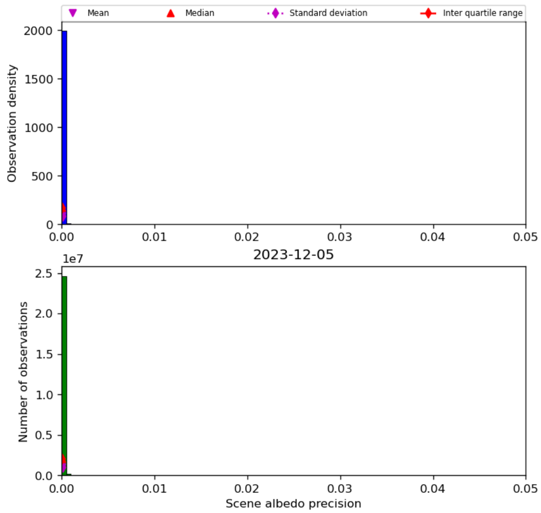
Figure 35: Histogram of “Scene albedo precision” for 2023-12-04 to 2023-12-06
