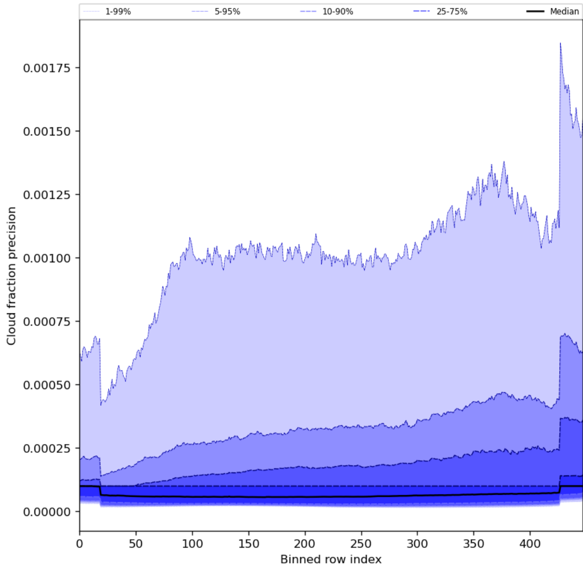
Figure 50: Along track statistics of “Cloud fraction precision” for 2023-12-04 to 2023-12-06
