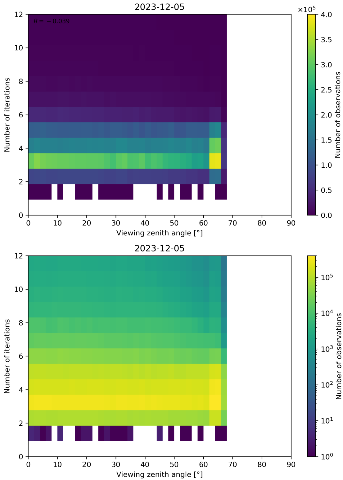
Figure 124: Scatter density plot of “Viewing zenith angle” against “Number of iterations” for 2023-12-04 to 2023-12-06.
