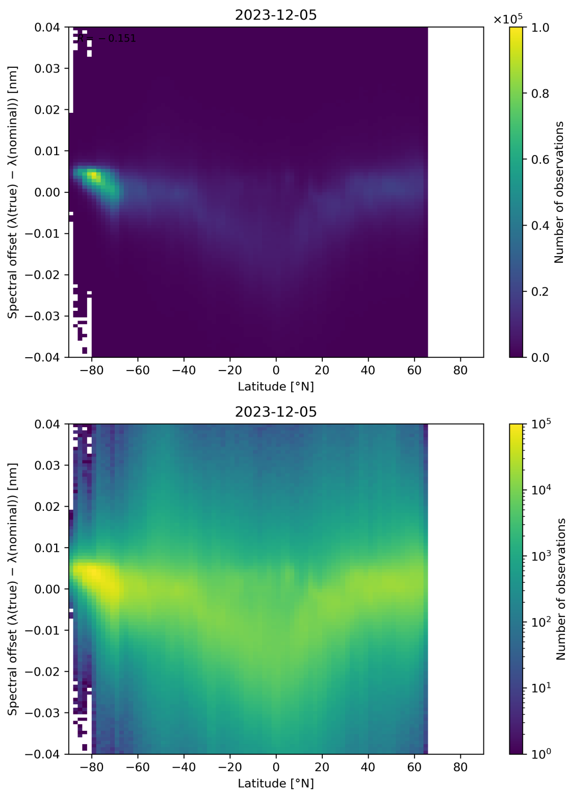
Figure 96: Scatter density plot of “Latitude” against “Spectral offset ( \lambda(\text{true}) - \lambda(\text{nominal}) )” for 2023-12-04 to 2023-12-06.
