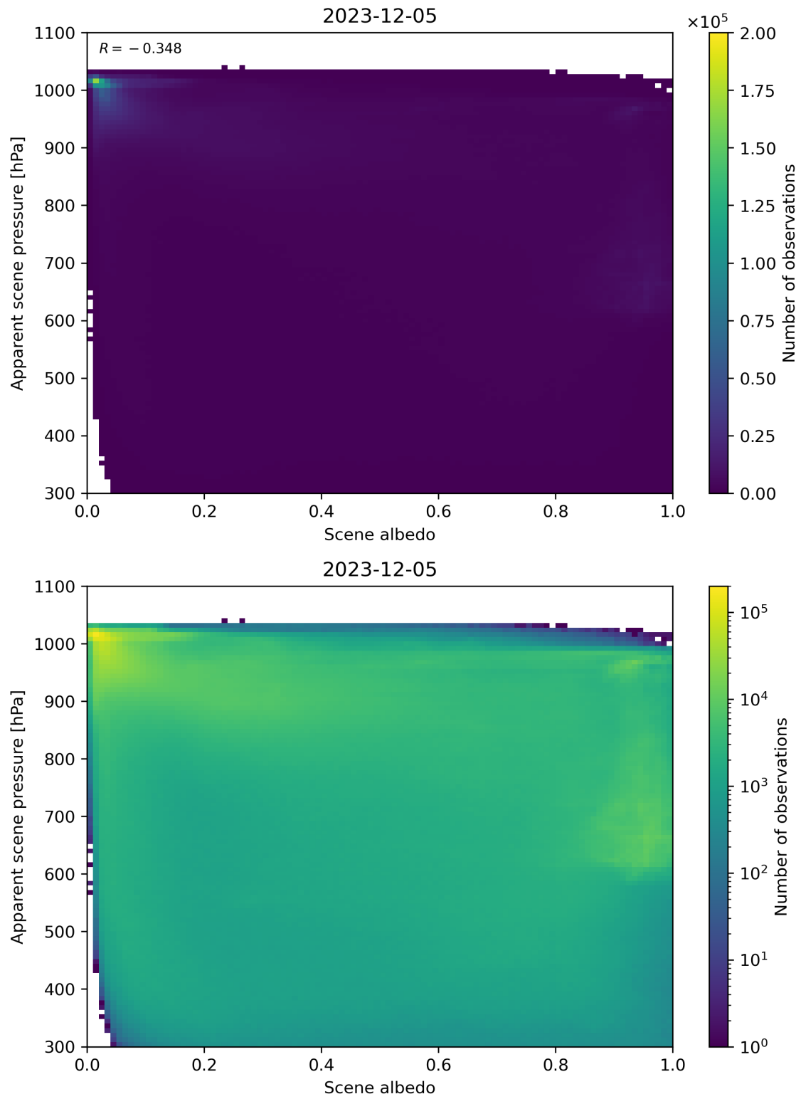
Figure 102: Scatter density plot of “Scene albedo” against “Apparent scene pressure” for 2023-12-04 to 2023-12-06.
