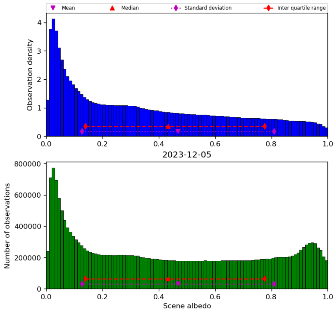
Figure 34: Histogram of “Scene albedo” for 2023-12-04 to 2023-12-06
