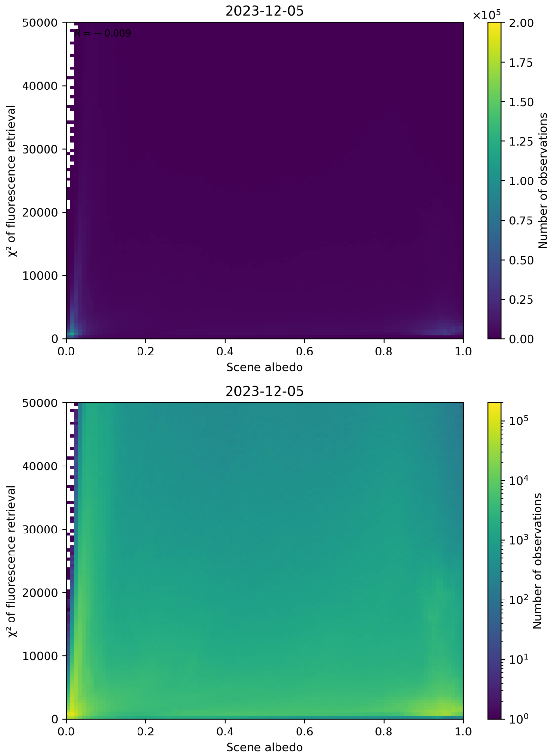
Figure 103: Scatter density plot of “Scene albedo” against “ \chi^2 of fluorescence retrieval” for 2023-12-04 to 2023-12-06.
