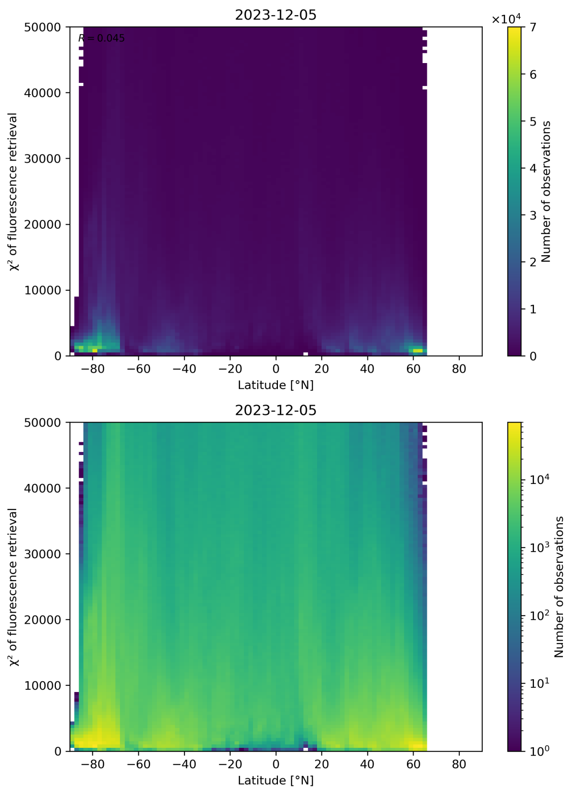
Figure 89: Scatter density plot of “Latitude” against “ \chi^2 of fluorescence retrieval” for 2023-12-04 to 2023-12-06.
