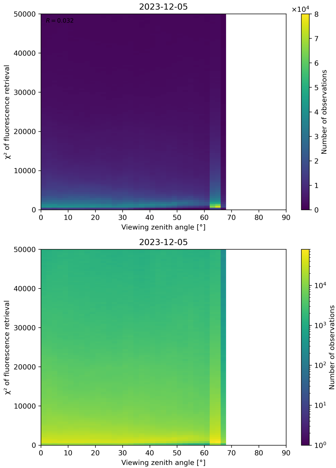
Figure 119: Scatter density plot of “Viewing zenith angle” against “ \chi^2 of fluorescence retrieval” for 2023-12-04 to 2023-12-06.
