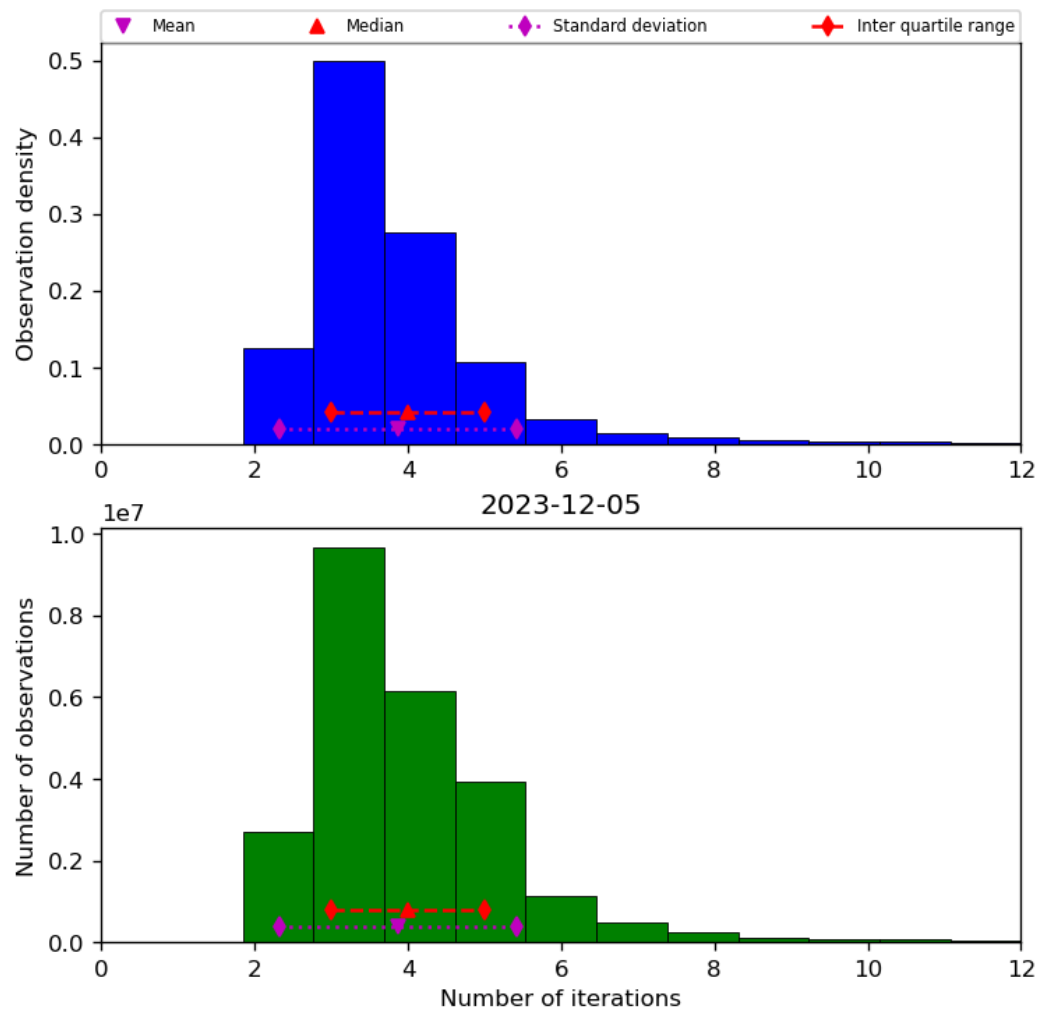
Figure 39: Histogram of “Number of iterations” for 2023-12-04 to 2023-12-06
