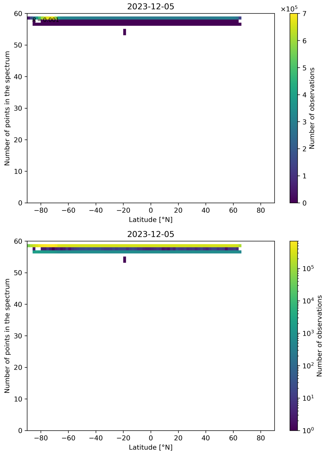
Figure 94: Scatter density plot of “Latitude” against “Number of points in the spectrum” for 2023-12-04 to 2023-12-06.
