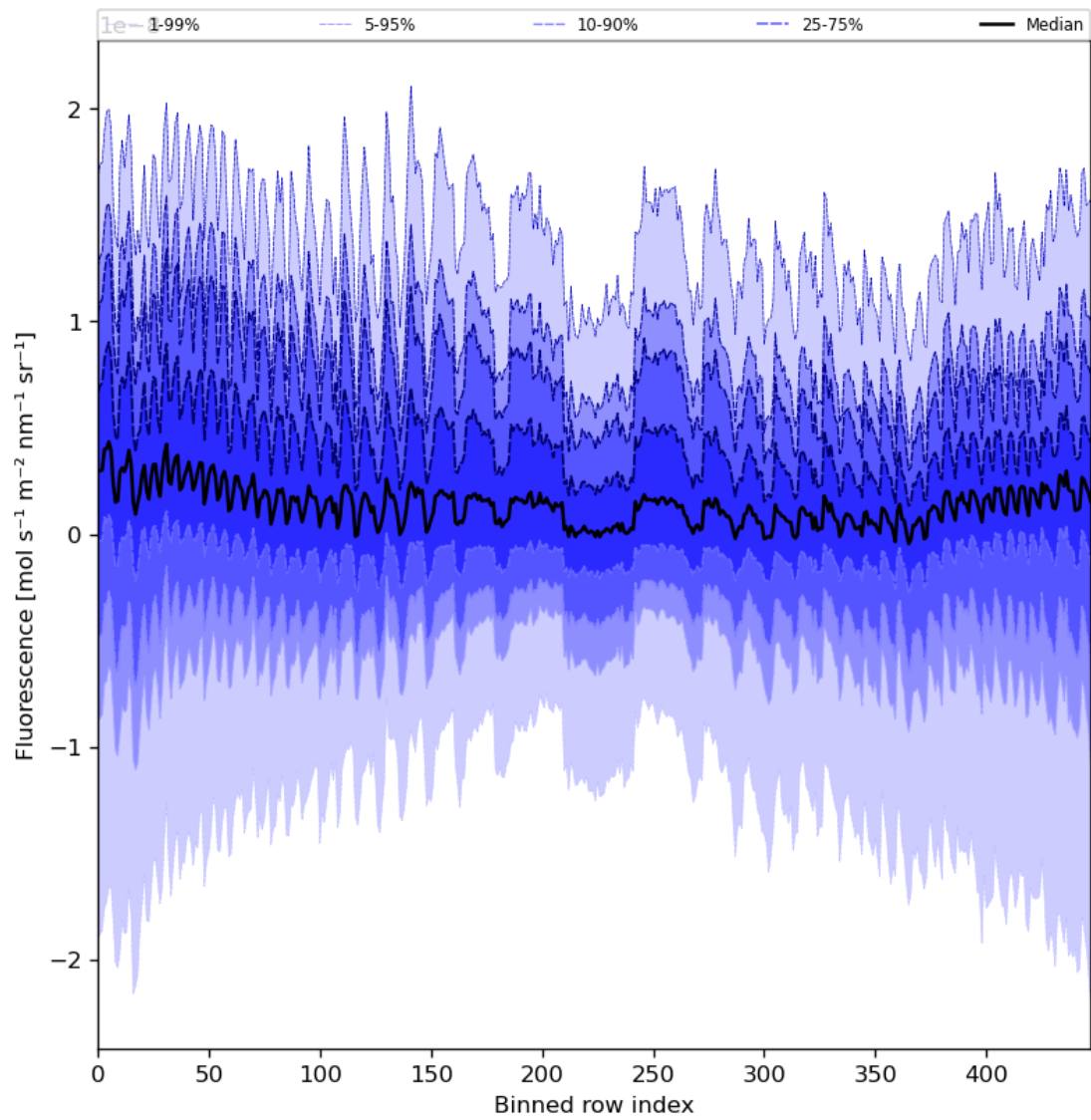
Figure 57: Along track statistics of “Fluorescence” for 2023-12-04 to 2023-12-06
