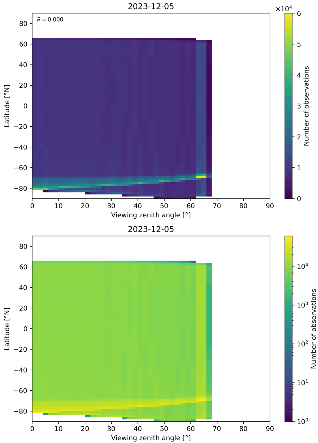
Figure 123: Scatter density plot of “Viewing zenith angle” against “Latitude” for 2023-12-04 to 2023-12-06.
