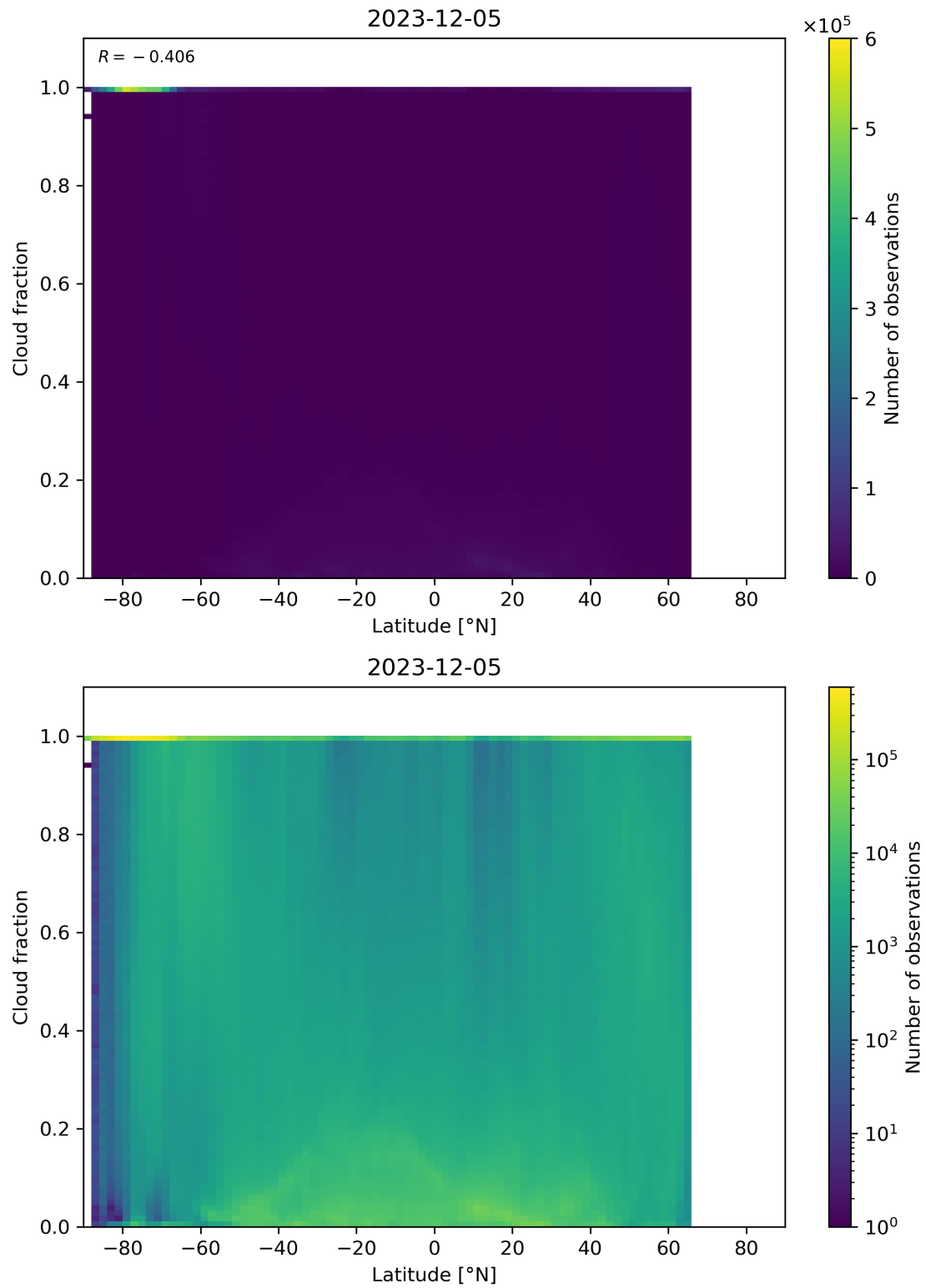
Figure 90: Scatter density plot of “Latitude” against “Cloud fraction” for 2023-12-04 to 2023-12-06.
