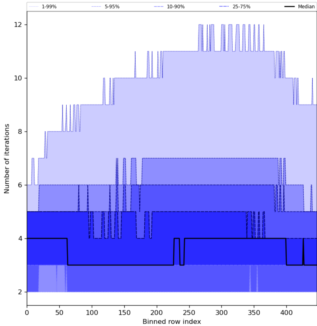
Figure 56: Along track statistics of “Number of iterations” for 2023-12-04 to 2023-12-06
