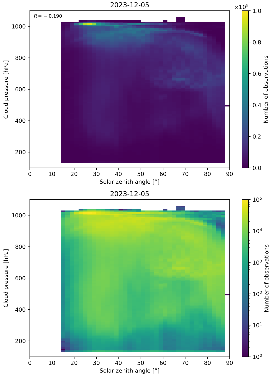
Figure 111: Scatter density plot of “Solar zenith angle” against “Cloud pressure” for 2023-12-04 to 2023-12-06.
