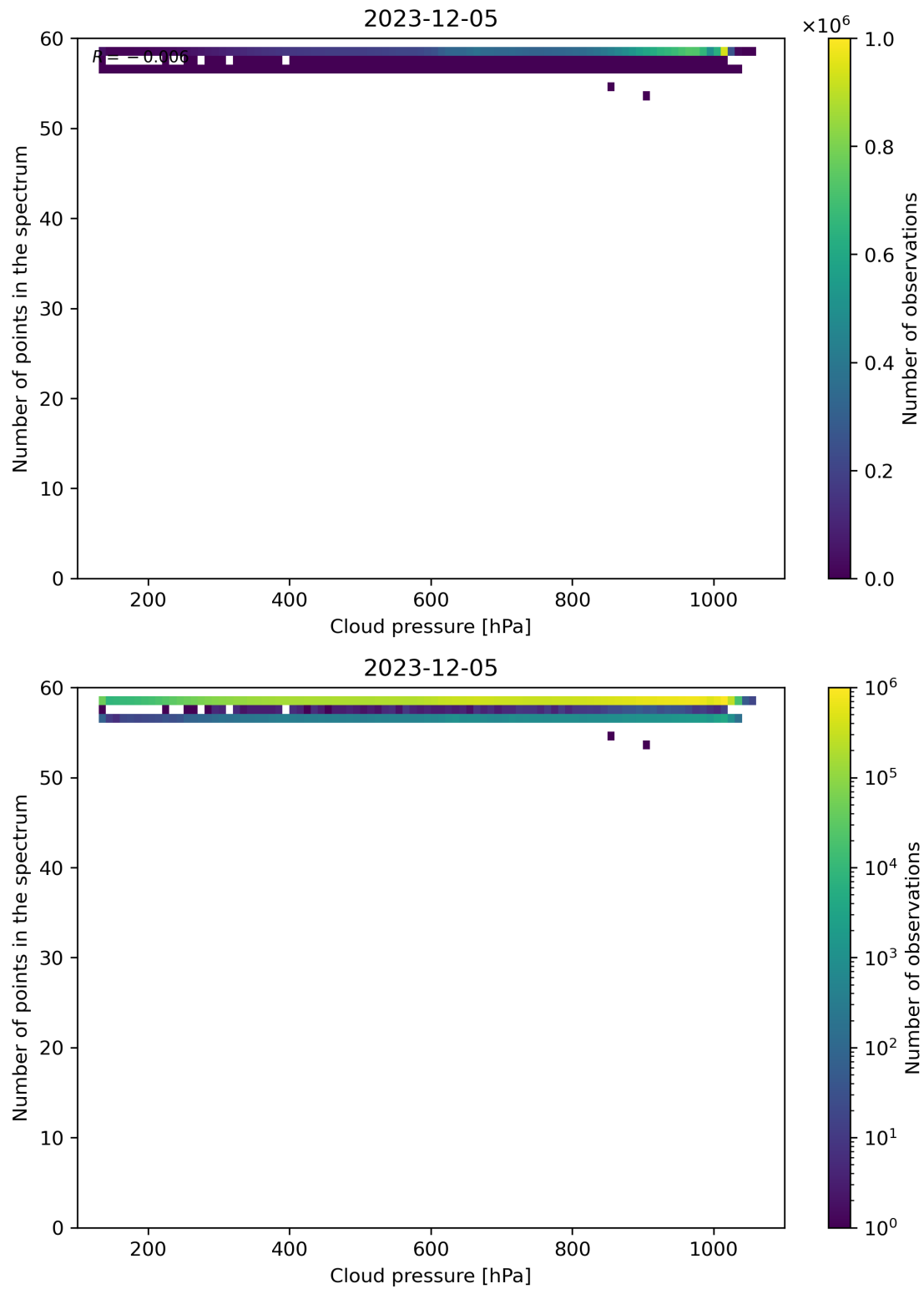
Figure 82: Scatter density plot of “Cloud pressure” against “Number of points in the spectrum” for 2023-12-04 to 2023-12-06.
