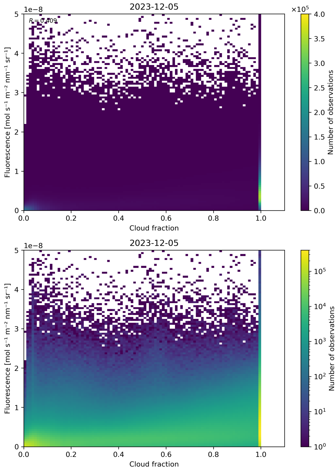
Figure 72: Scatter density plot of “Cloud fraction” against “Fluorescence” for 2023-12-04 to 2023-12-06.
