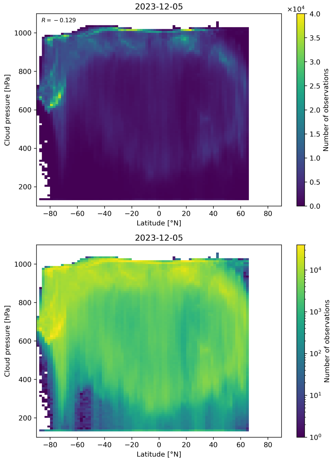
Figure 91: Scatter density plot of “Latitude” against “Cloud pressure” for 2023-12-04 to 2023-12-06.
