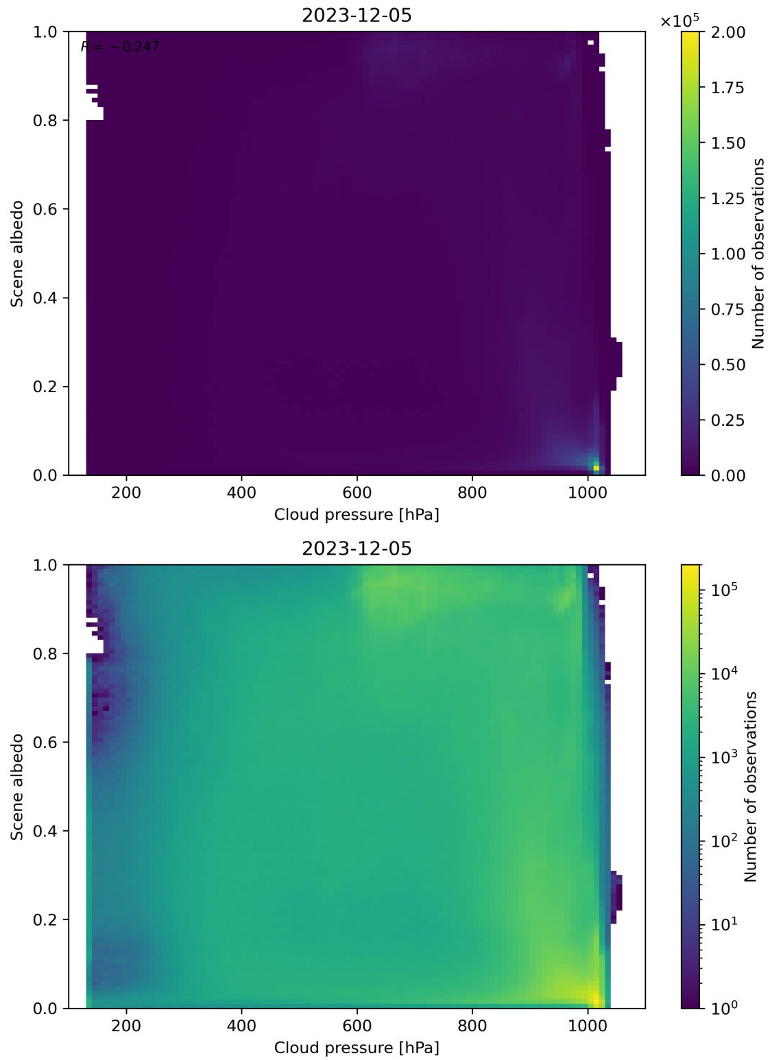
Figure 83: Scatter density plot of “Cloud pressure” against “Scene albedo” for 2023-12-04 to 2023-12-06.
