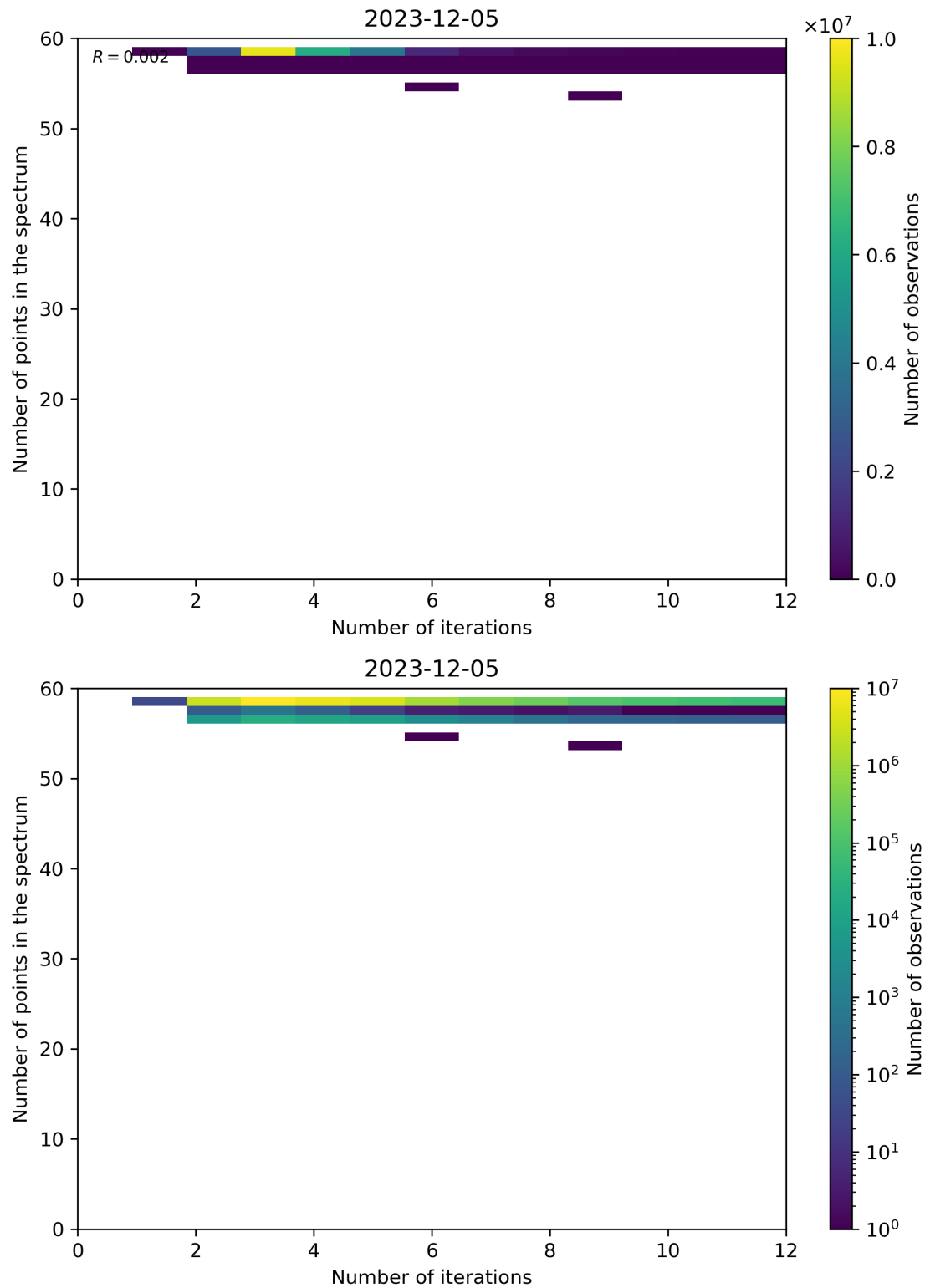
Figure 99: Scatter density plot of “Number of iterations” against “Number of points in the spectrum” for 2023-12-04 to 2023-12-06.
