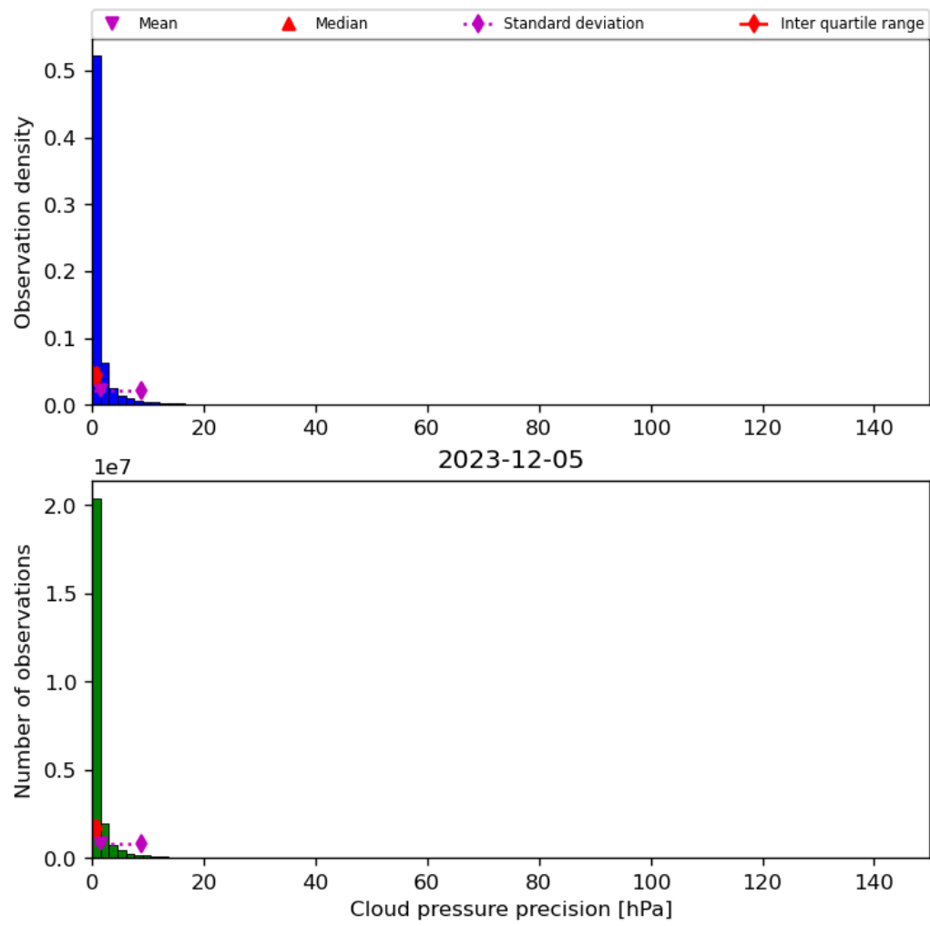
Figure 31: Histogram of “Cloud pressure precision” for 2023-12-04 to 2023-12-06
