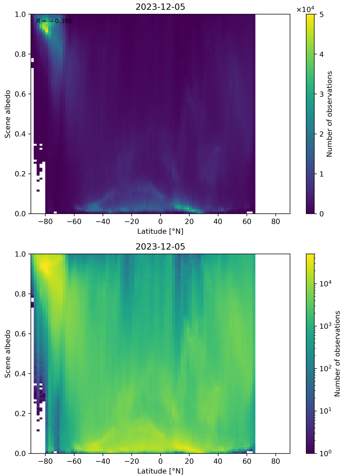
Figure 95: Scatter density plot of “Latitude” against “Scene albedo” for 2023-12-04 to 2023-12-06.
