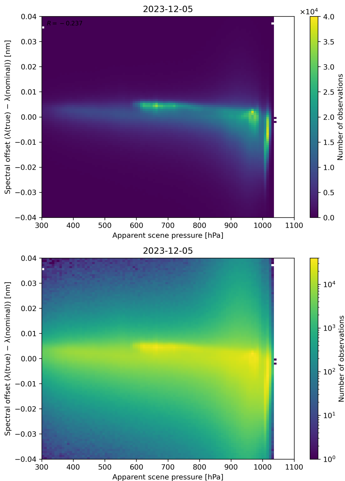
Figure 67: Scatter density plot of “Apparent scene pressure” against “Spectral offset ( \lambda(\text{true}) - \lambda(\text{nominal}) )” for 2023-12-04 to 2023-12-06.
