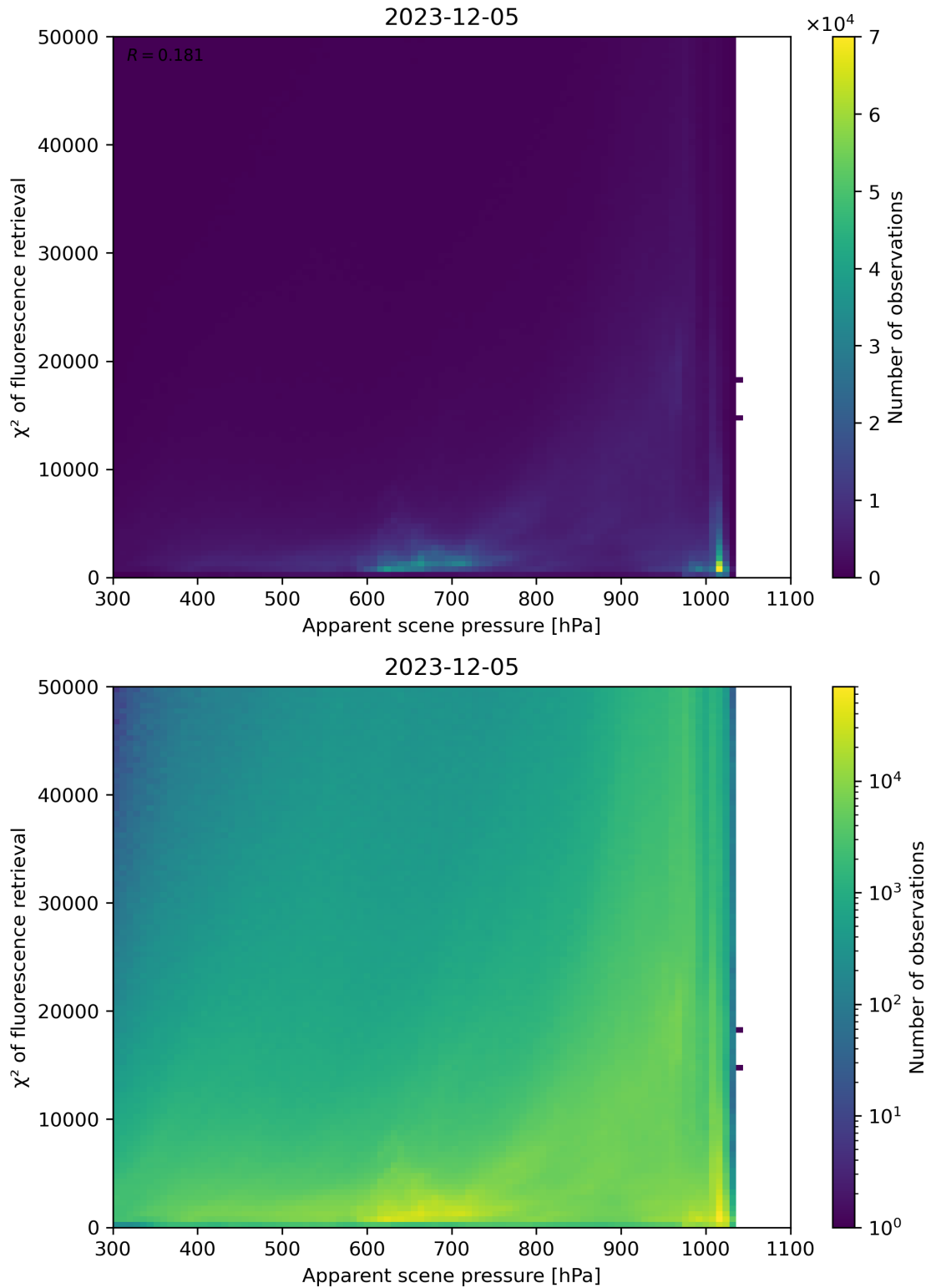
Figure 63: Scatter density plot of “Apparent scene pressure” against “ \chi^2 of fluorescence retrieval” for 2023-12-04 to 2023-12-06.
