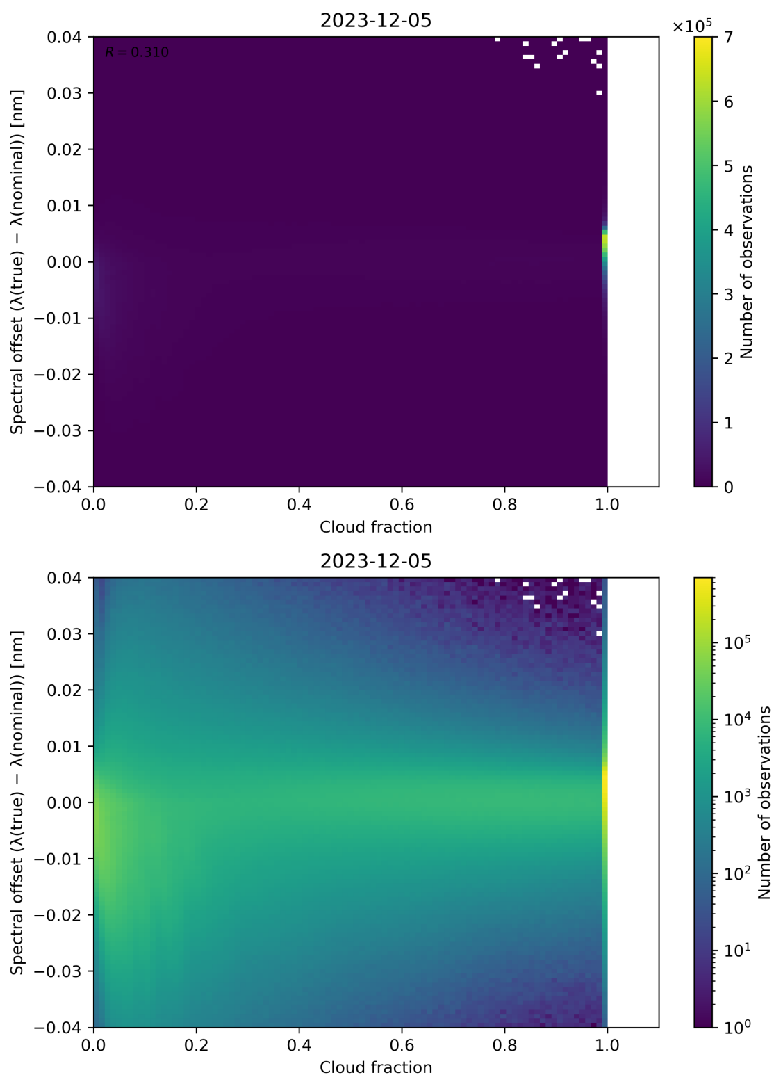
Figure 76: Scatter density plot of “Cloud fraction” against “Spectral offset ( \lambda(\text{true}) - \lambda(\text{nominal}) )” for 2023-12-04 to 2023-12-06.
