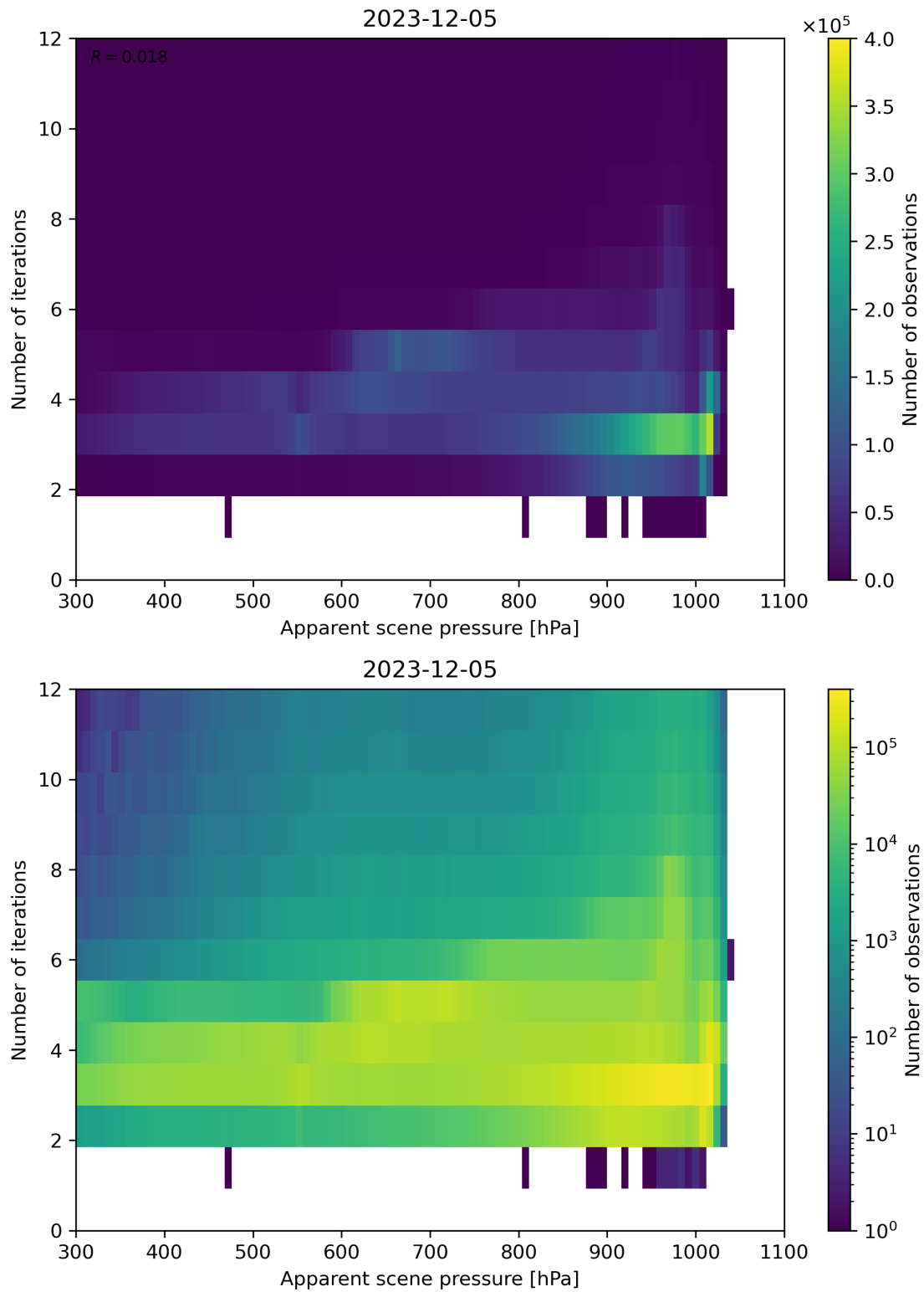
Figure 65: Scatter density plot of “Apparent scene pressure” against “Number of iterations” for 2023-12-04 to 2023-12-06.
