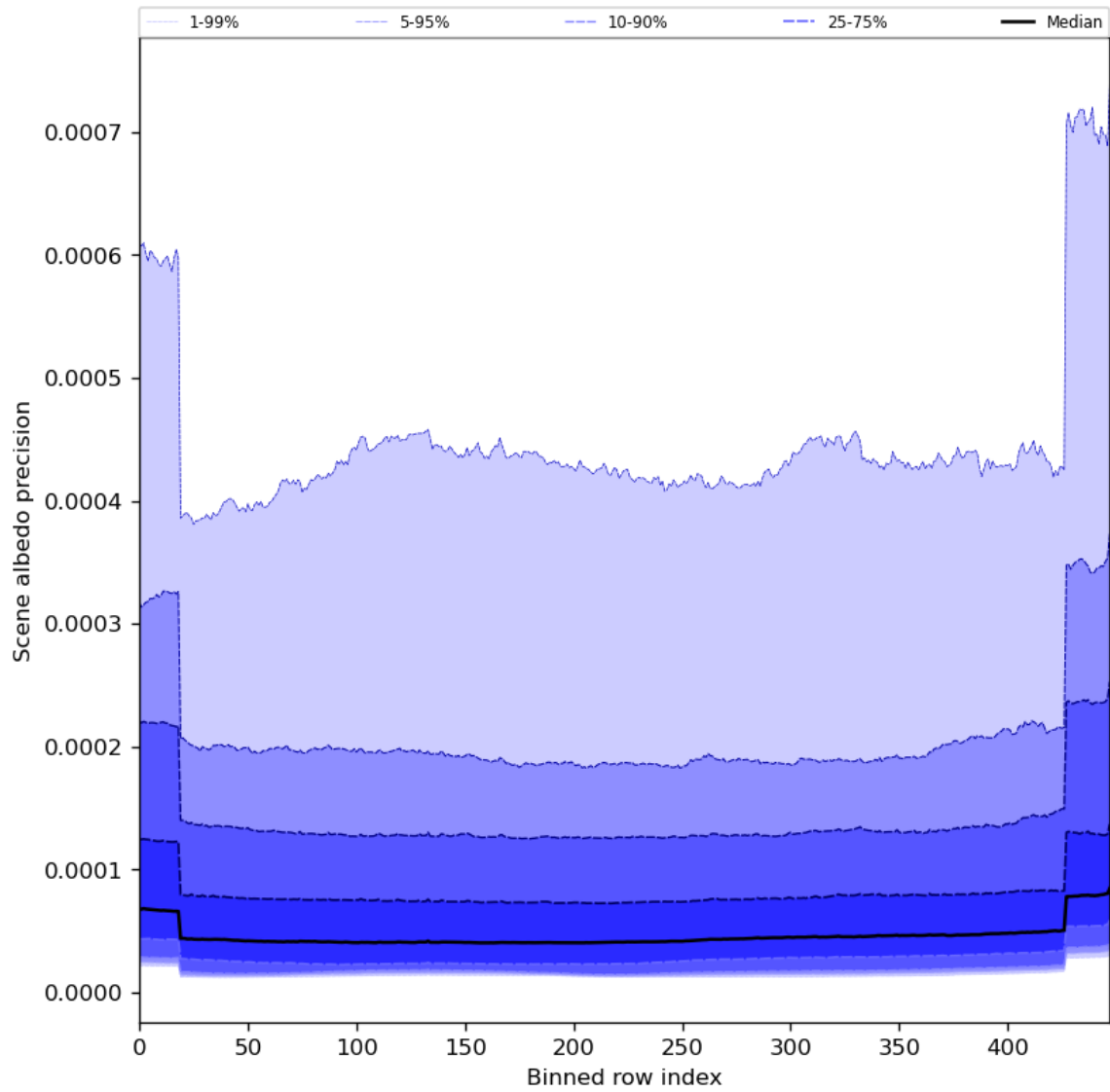
Figure 52: Along track statistics of “Scene albedo precision” for 2023-12-04 to 2023-12-06
