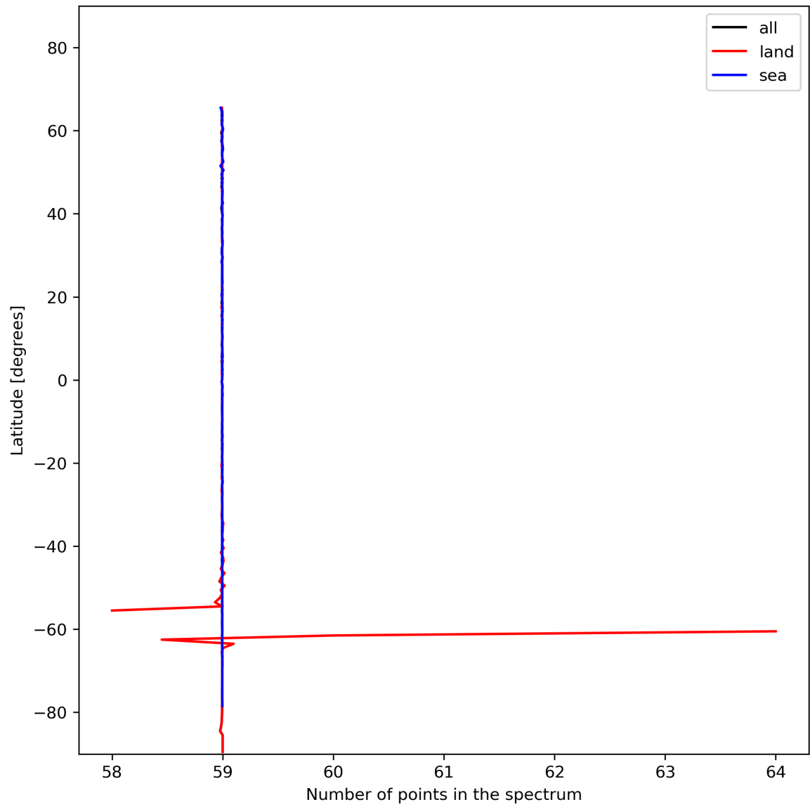
Figure 27: Zonal average of “Number of points in the spectrum” for 2023-12-04 to 2023-12-06.
