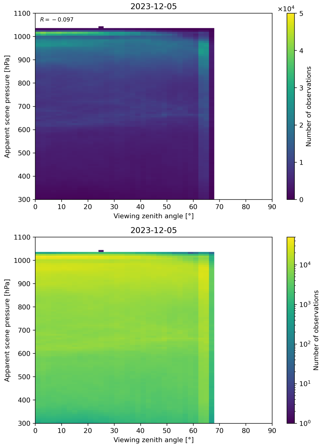
Figure 118: Scatter density plot of “Viewing zenith angle” against “Apparent scene pressure” for 2023-12-04 to 2023-12-06.
