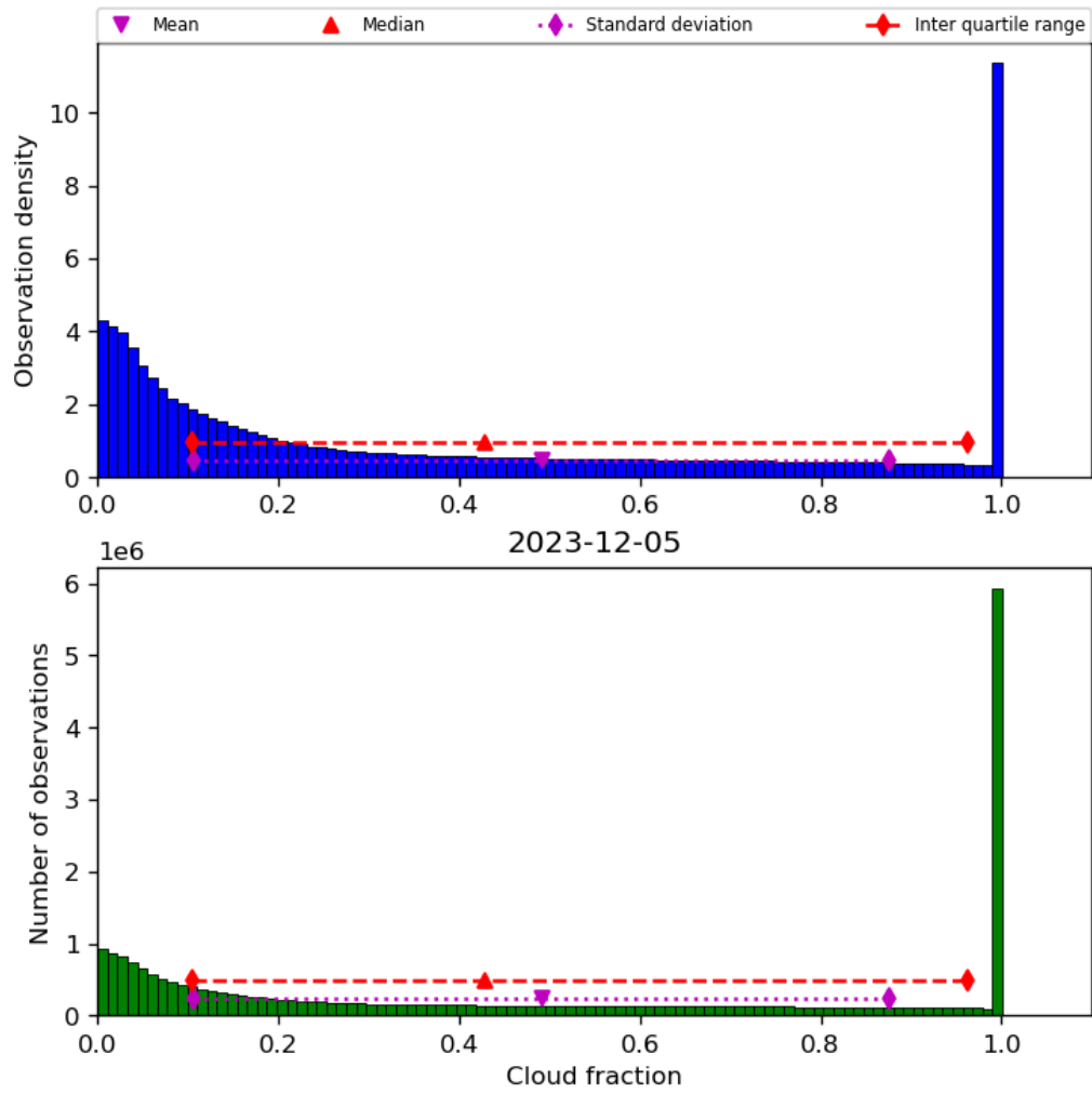
Figure 32: Histogram of “Cloud fraction” for 2023-12-04 to 2023-12-06
