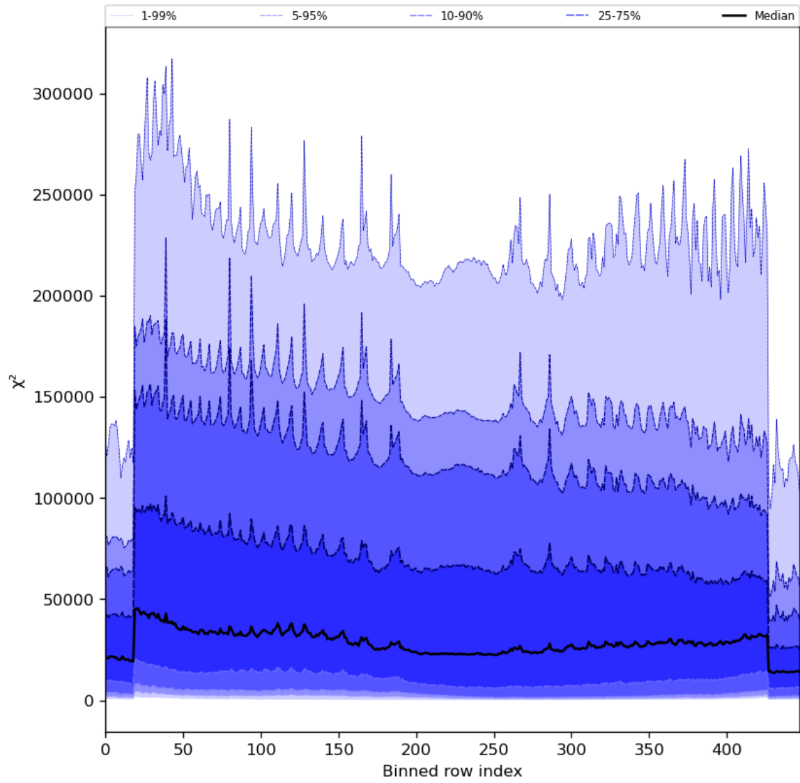
Figure 55: Along track statistics of “ \chi^2 ” for 2023-12-04 to 2023-12-06
