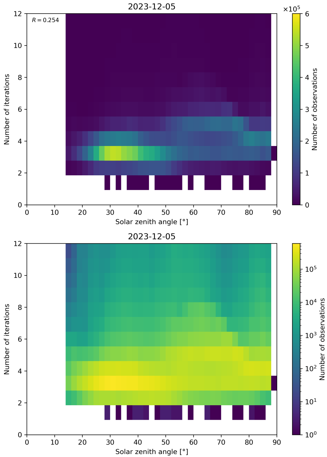
Figure 114: Scatter density plot of “Solar zenith angle” against “Number of iterations” for 2023-12-04 to 2023-12-06.
