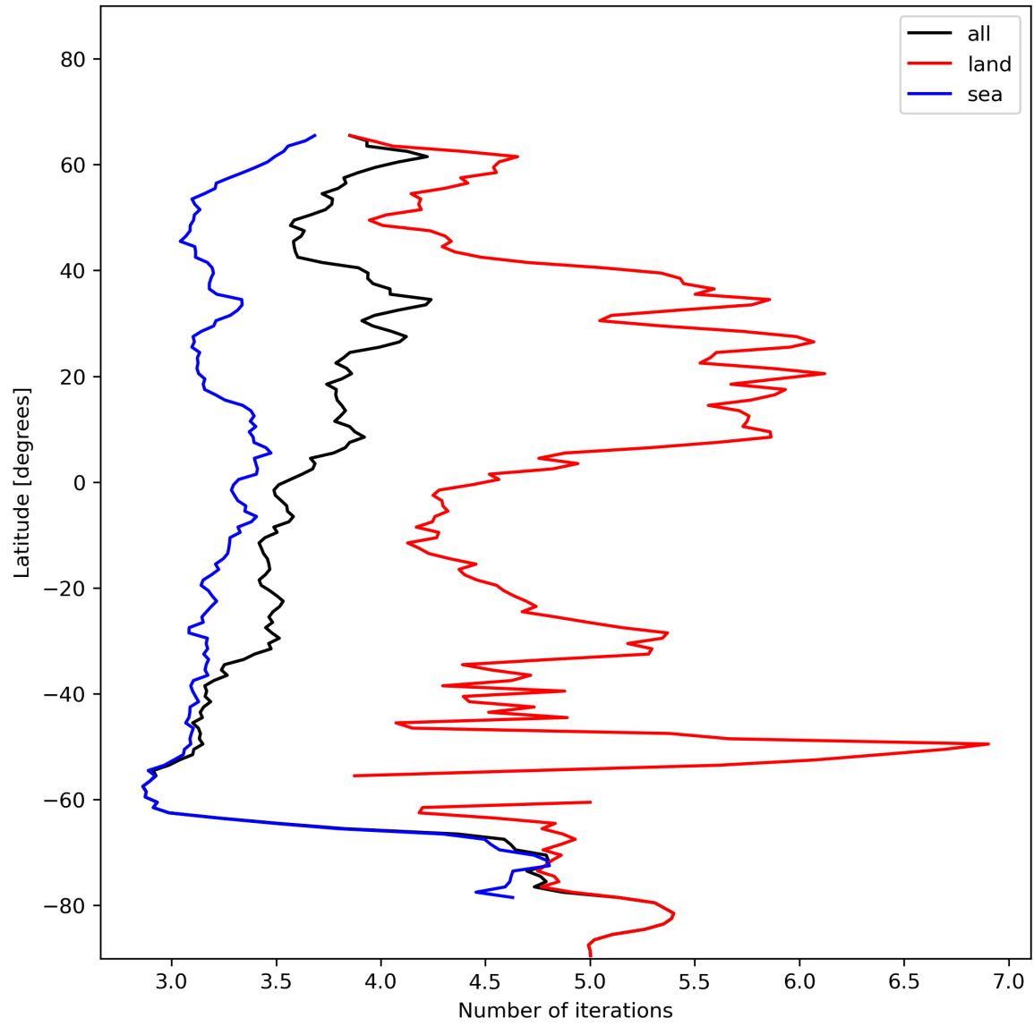
Figure 22: Zonal average of “Number of iterations” for 2023-12-04 to 2023-12-06.
