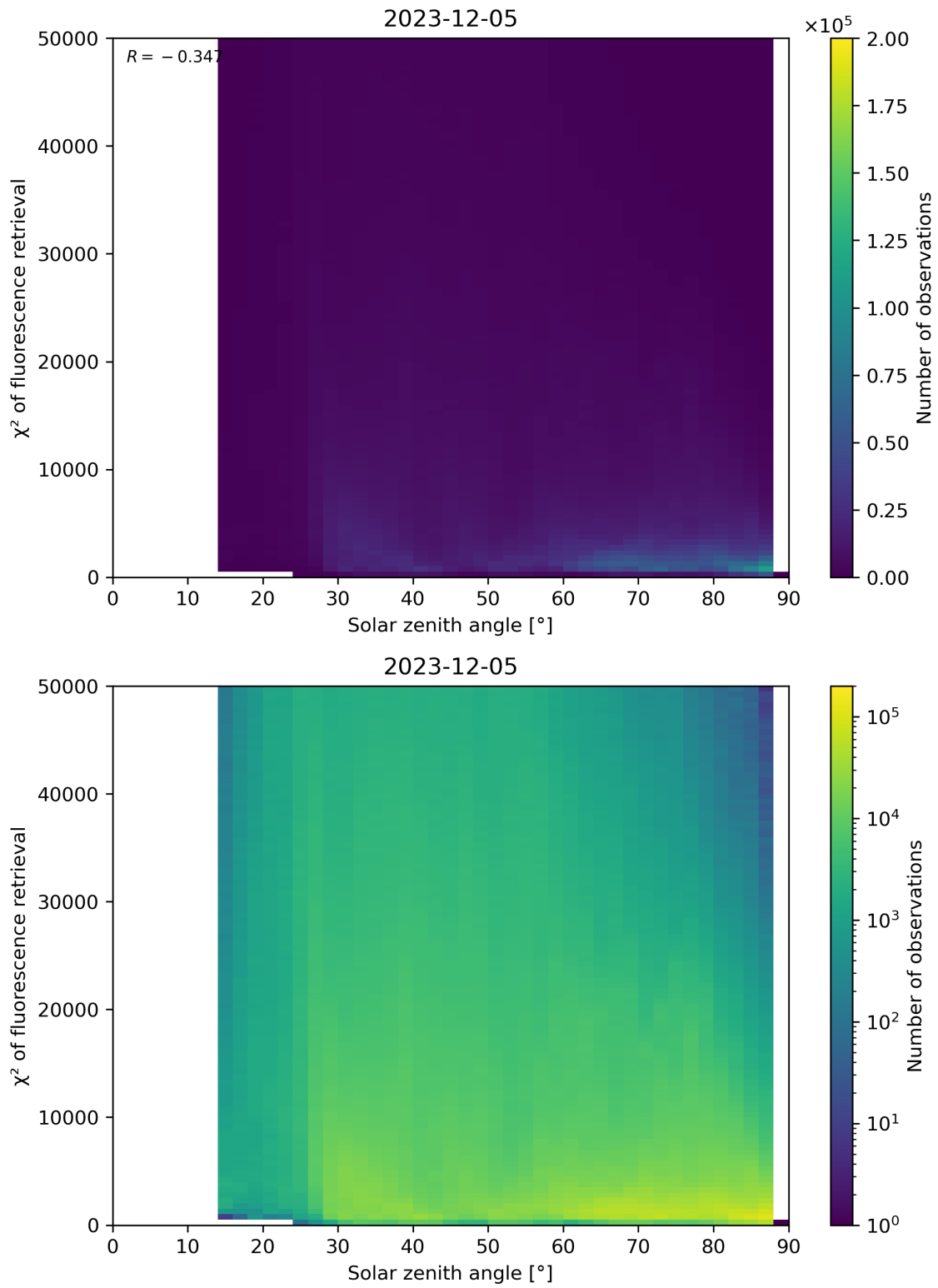
Figure 109: Scatter density plot of “Solar zenith angle” against “ \chi^2 of fluorescence retrieval” for 2023-12-04 to 2023-12-06.
