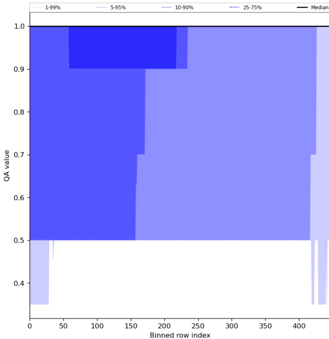
Figure 46: Along track statistics of “QA value” for 2023-12-04 to 2023-12-06
