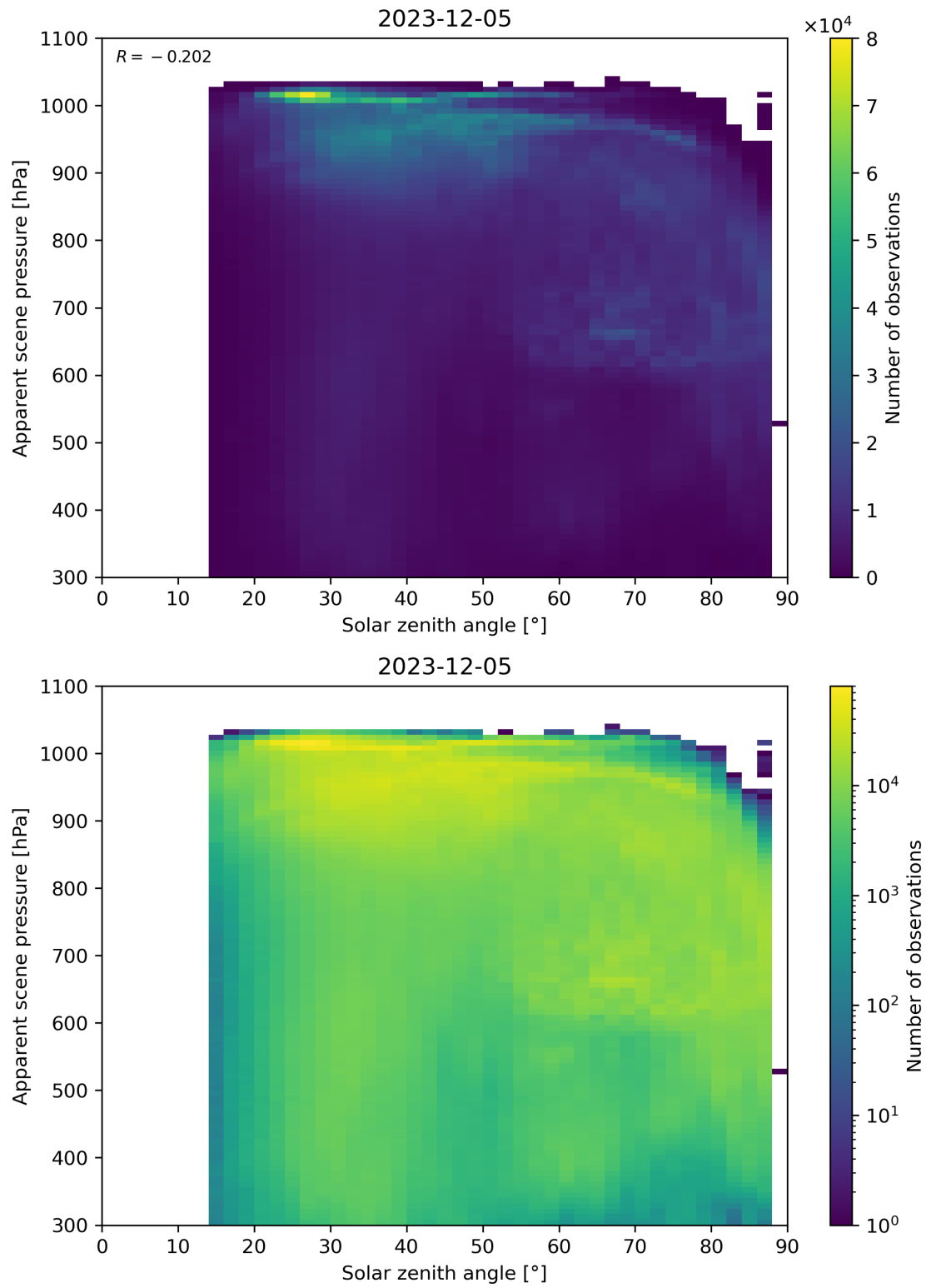
Figure 108: Scatter density plot of “Solar zenith angle” against “Apparent scene pressure” for 2023-12-04 to 2023-12-06.
