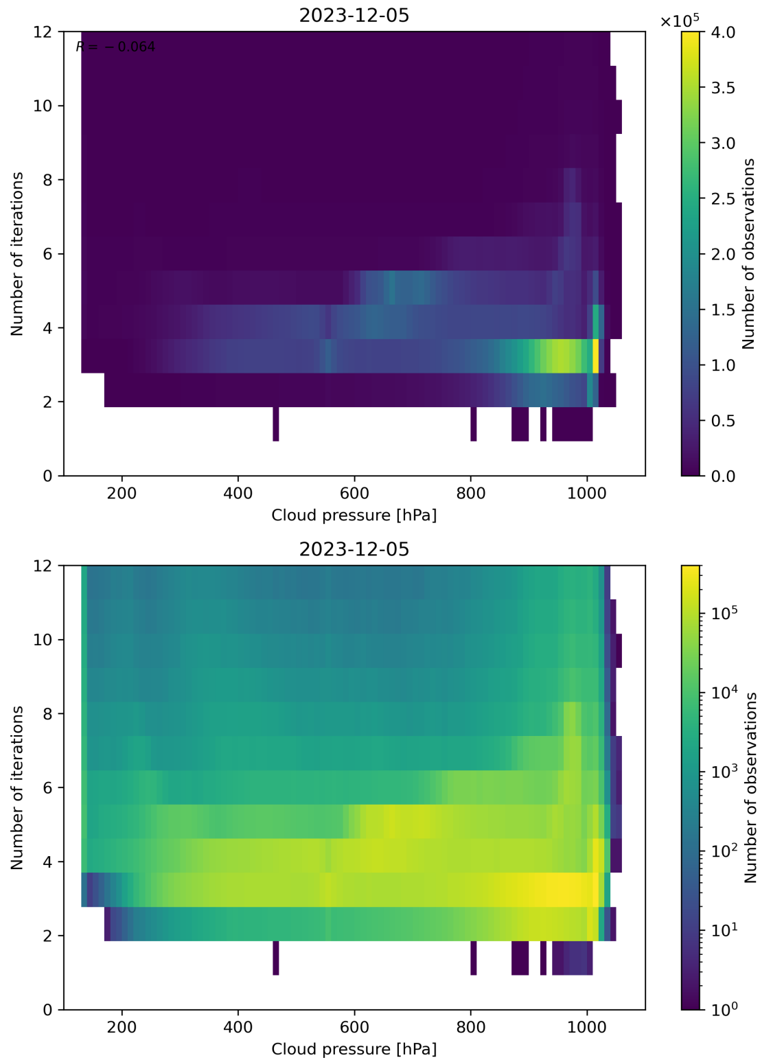
Figure 81: Scatter density plot of “Cloud pressure” against “Number of iterations” for 2023-12-04 to 2023-12-06.
