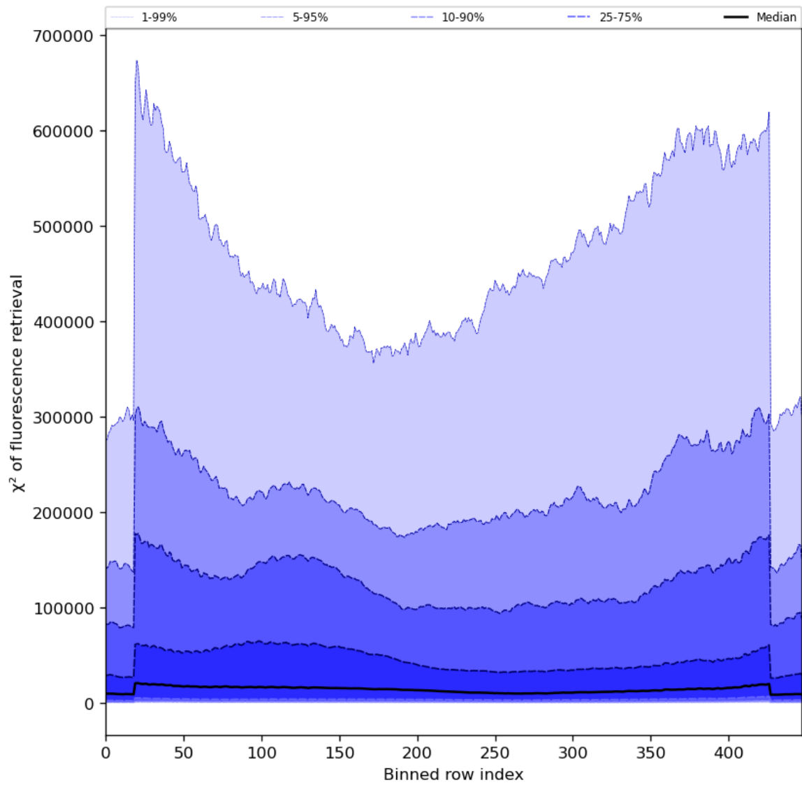
Figure 59: Along track statistics of “ \chi^2 of fluorescence retrieval” for 2023-12-04 to 2023-12-06
