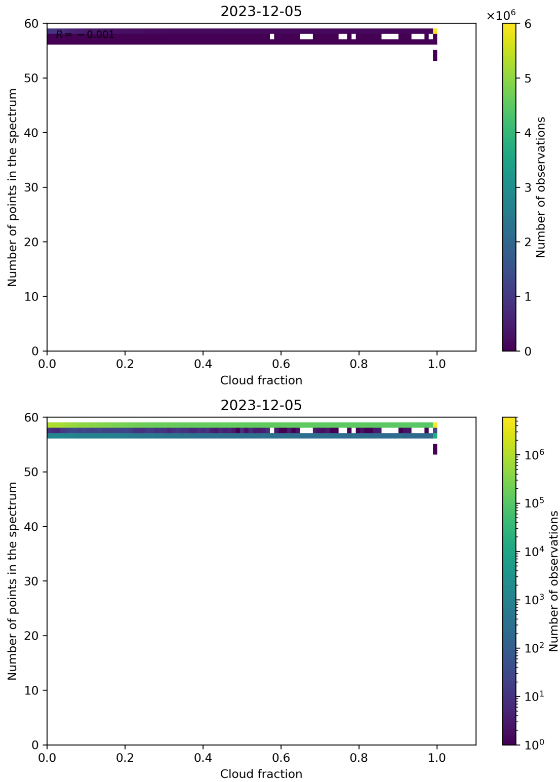
Figure 74: Scatter density plot of “Cloud fraction” against “Number of points in the spectrum” for 2023-12-04 to 2023-12-06.
