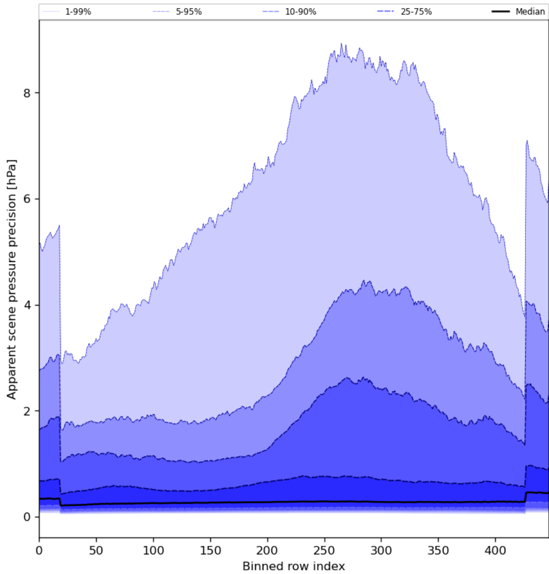
Figure 54: Along track statistics of “Apparent scene pressure precision” for 2023-12-04 to 2023-12-06
