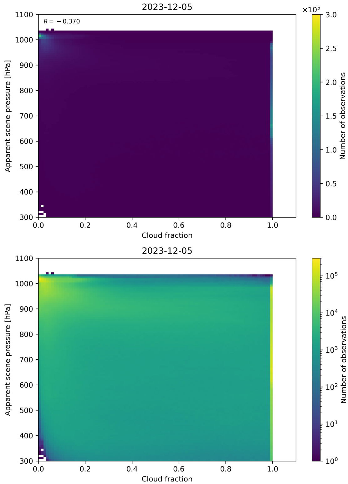
Figure 70: Scatter density plot of “Cloud fraction” against “Apparent scene pressure” for 2023-12-04 to 2023-12-06.
