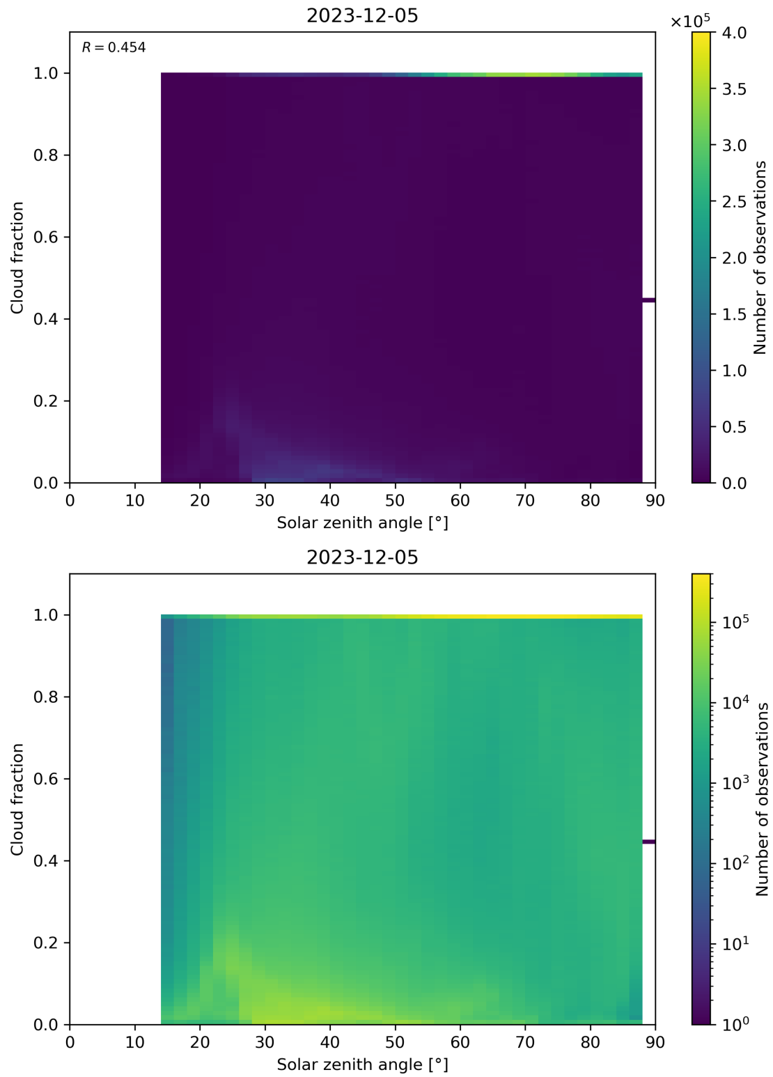
Figure 110: Scatter density plot of “Solar zenith angle” against “Cloud fraction” for 2023-12-04 to 2023-12-06.
