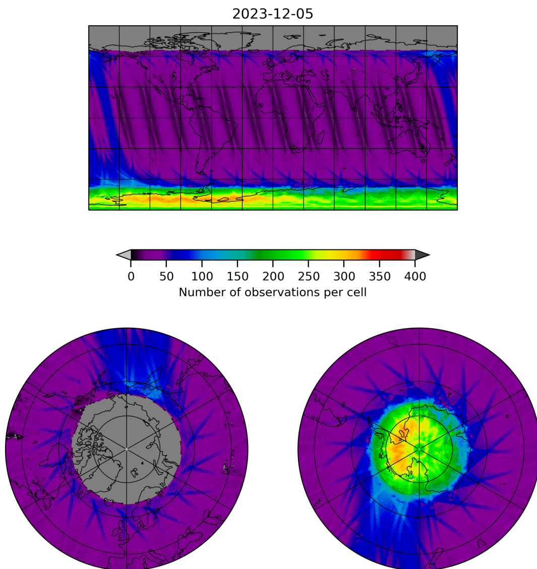
Figure 11: Map of the number of observations for 2023-12-04 to 2023-12-06
