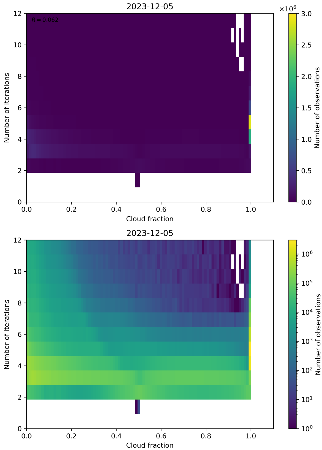
Figure 73: Scatter density plot of “Cloud fraction” against “Number of iterations” for 2023-12-04 to 2023-12-06.
