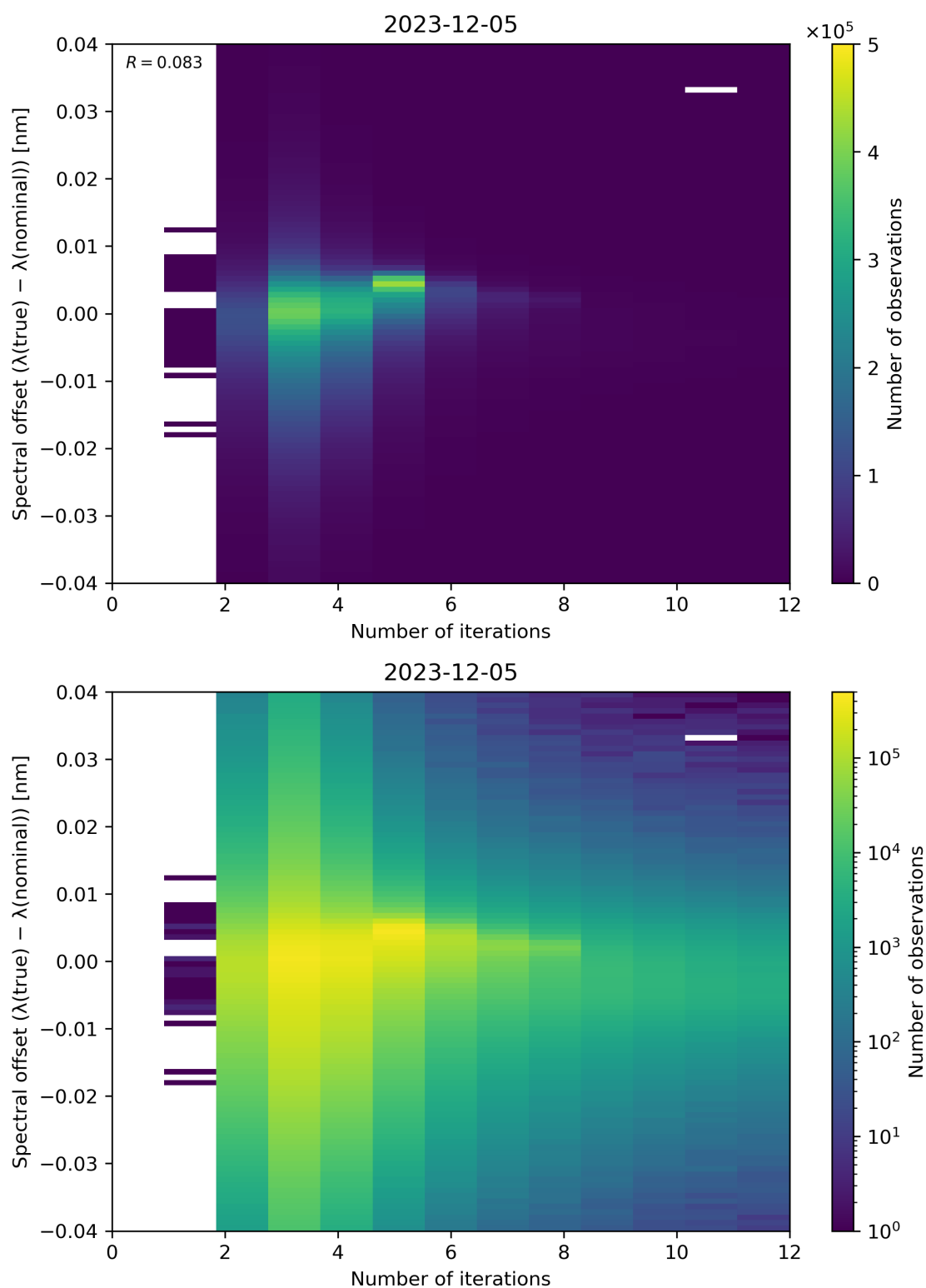
Figure 100: Scatter density plot of “Number of iterations” against “Spectral offset ( \lambda(\text{true}) - \lambda(\text{nominal}) )” for 2023-12-04 to 2023-12-06.
