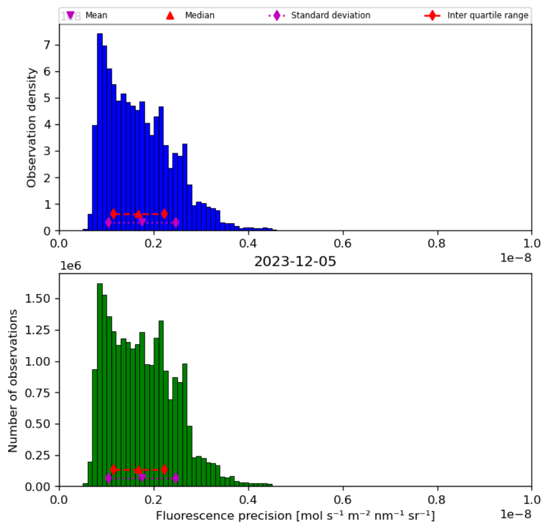
Figure 41: Histogram of “Fluorescence precision” for 2023-12-04 to 2023-12-06
