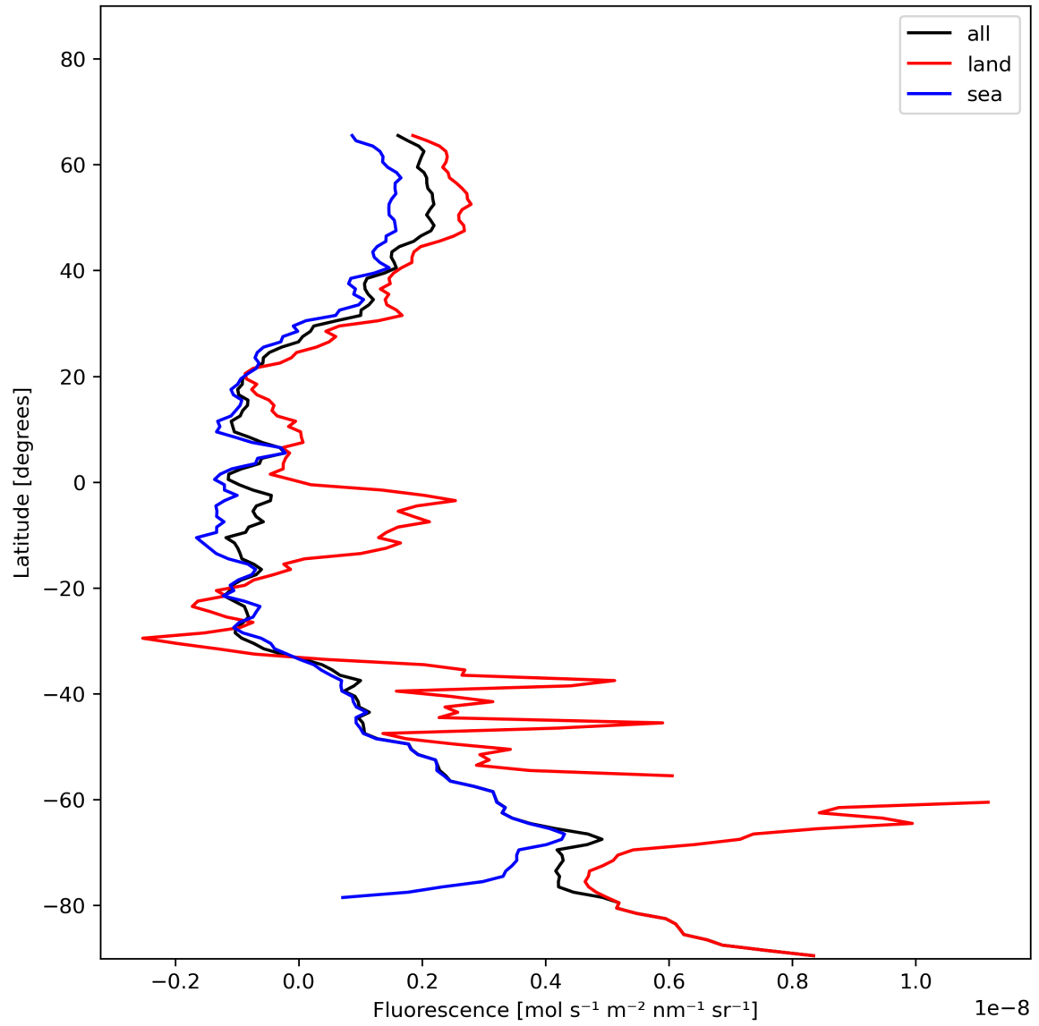
Figure 23: Zonal average of “Fluorescence” for 2023-12-04 to 2023-12-06.
