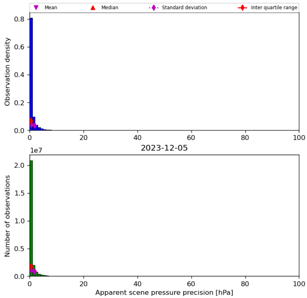
Figure 37: Histogram of “Apparent scene pressure precision” for 2023-12-04 to 2023-12-06
