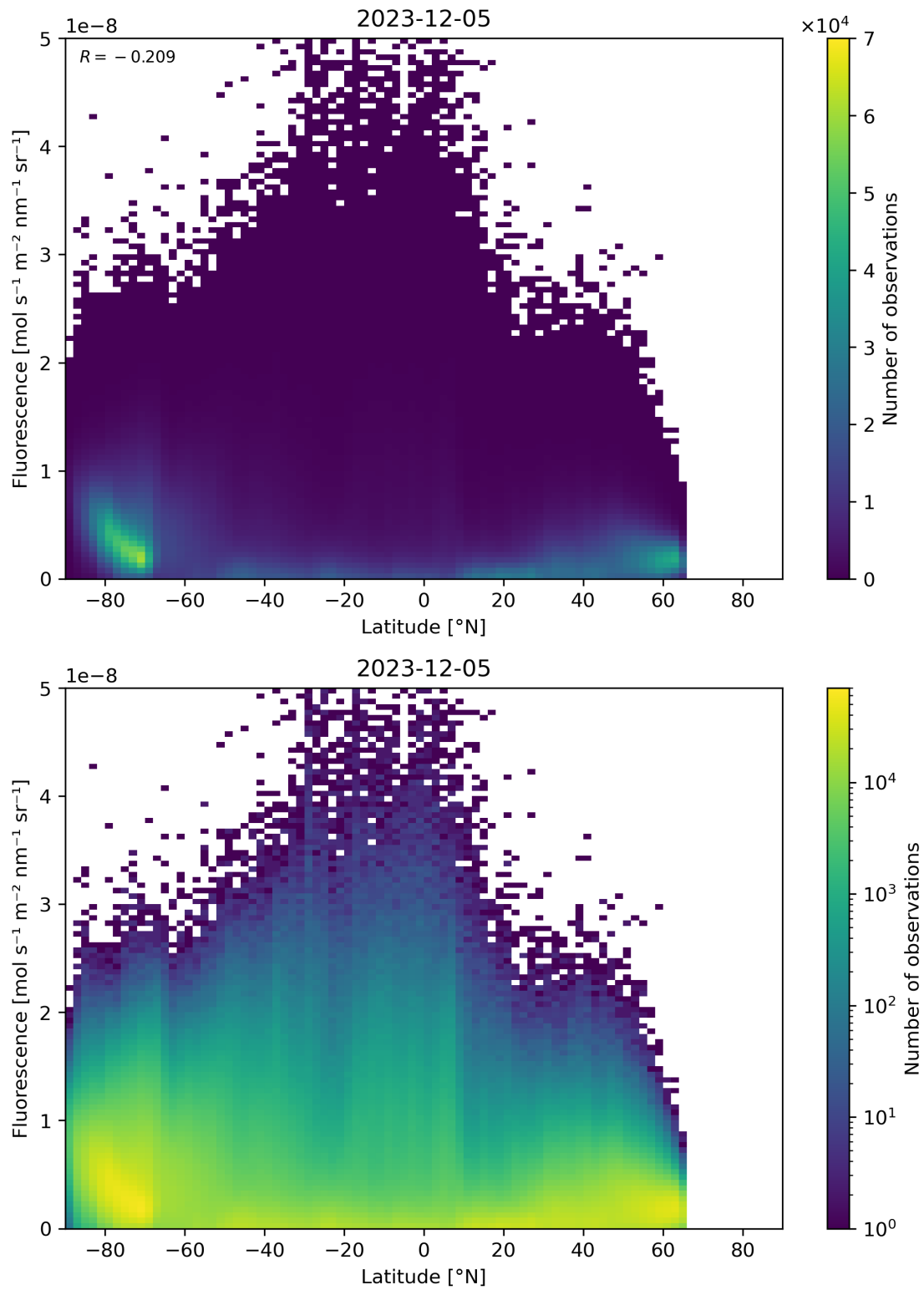
Figure 92: Scatter density plot of “Latitude” against “Fluorescence” for 2023-12-04 to 2023-12-06.
