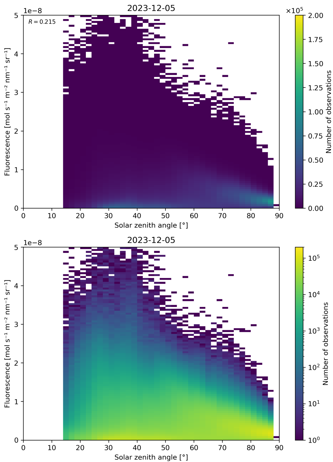
Figure 112: Scatter density plot of “Solar zenith angle” against “Fluorescence” for 2023-12-04 to 2023-12-06.
