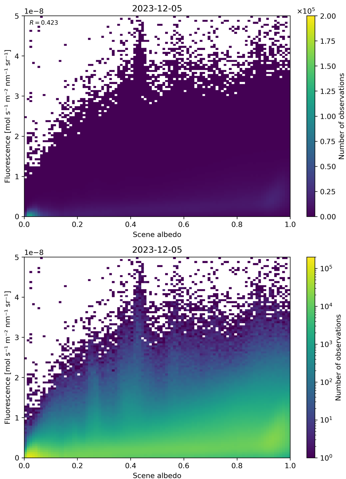
Figure 104: Scatter density plot of “Scene albedo” against “Fluorescence” for 2023-12-04 to 2023-12-06.
