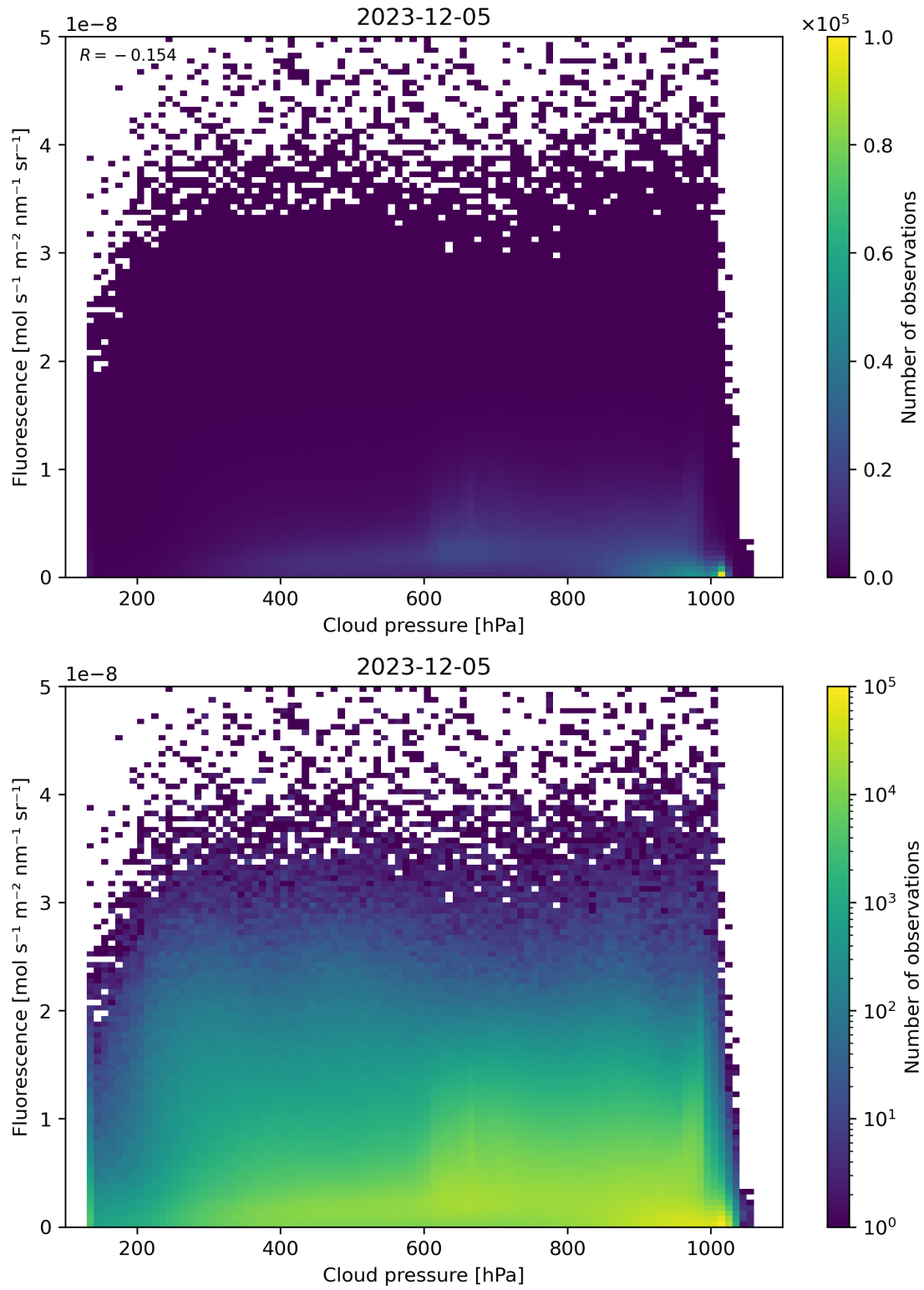
Figure 80: Scatter density plot of “Cloud pressure” against “Fluorescence” for 2023-12-04 to 2023-12-06.
