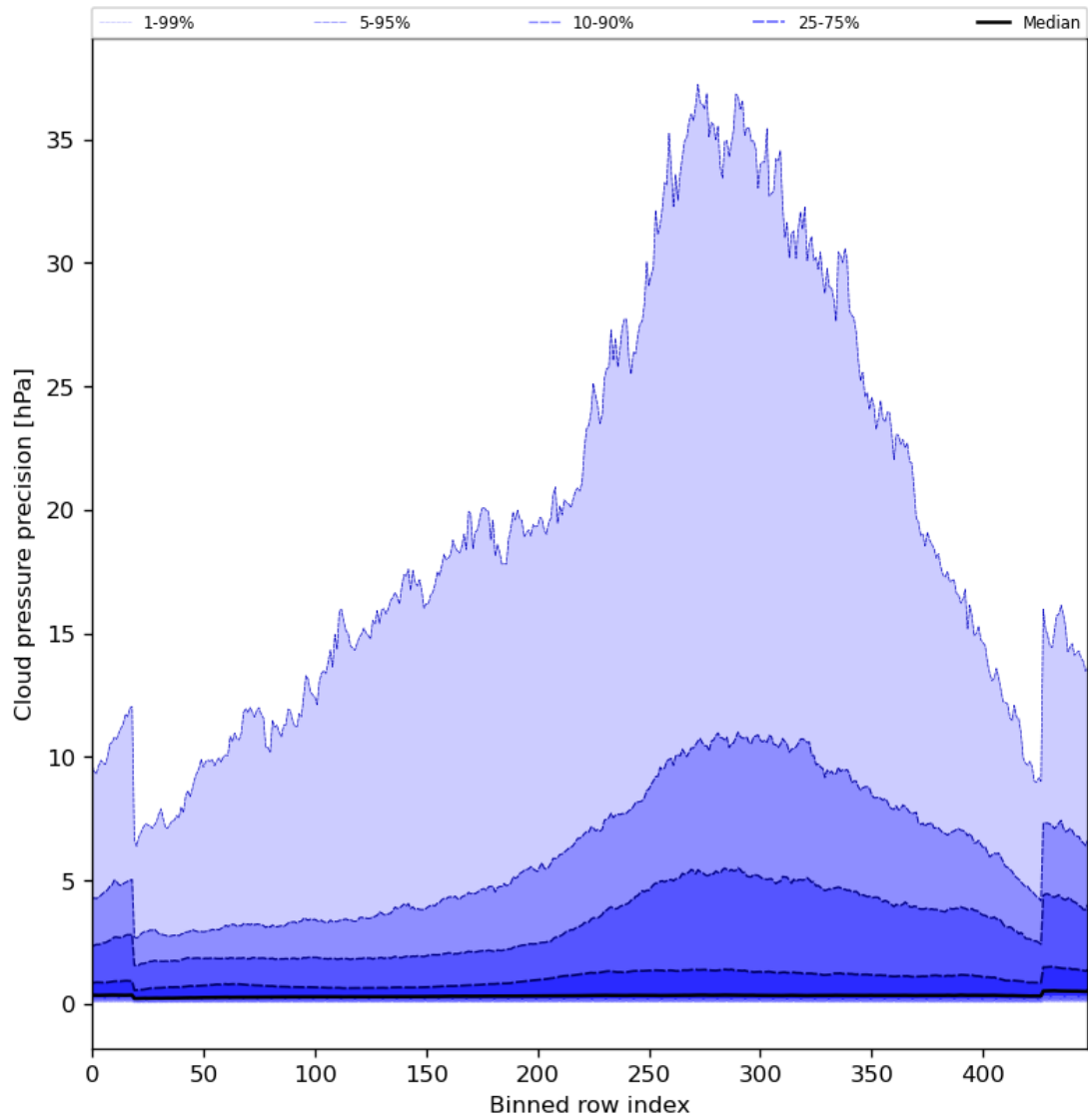
Figure 48: Along track statistics of “Cloud pressure precision” for 2023-12-04 to 2023-12-06
