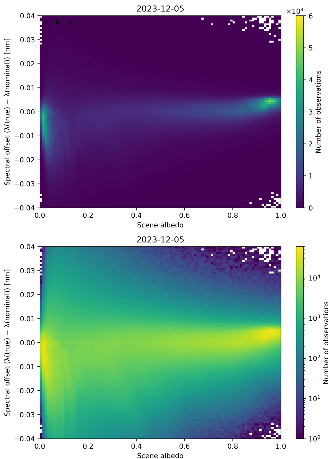
Figure 107: Scatter density plot of “Scene albedo” against “Spectral offset ( \lambda(\text{true}) - \lambda(\text{nominal}) )” for 2023-12-04 to 2023-12-06.
