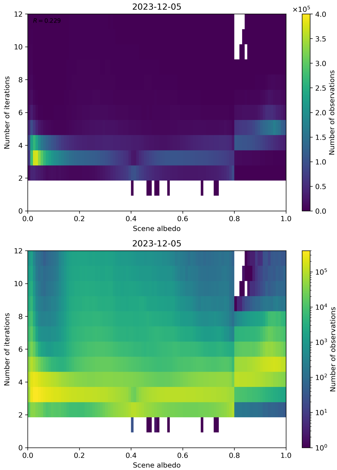
Figure 105: Scatter density plot of “Scene albedo” against “Number of iterations” for 2023-12-04 to 2023-12-06.
