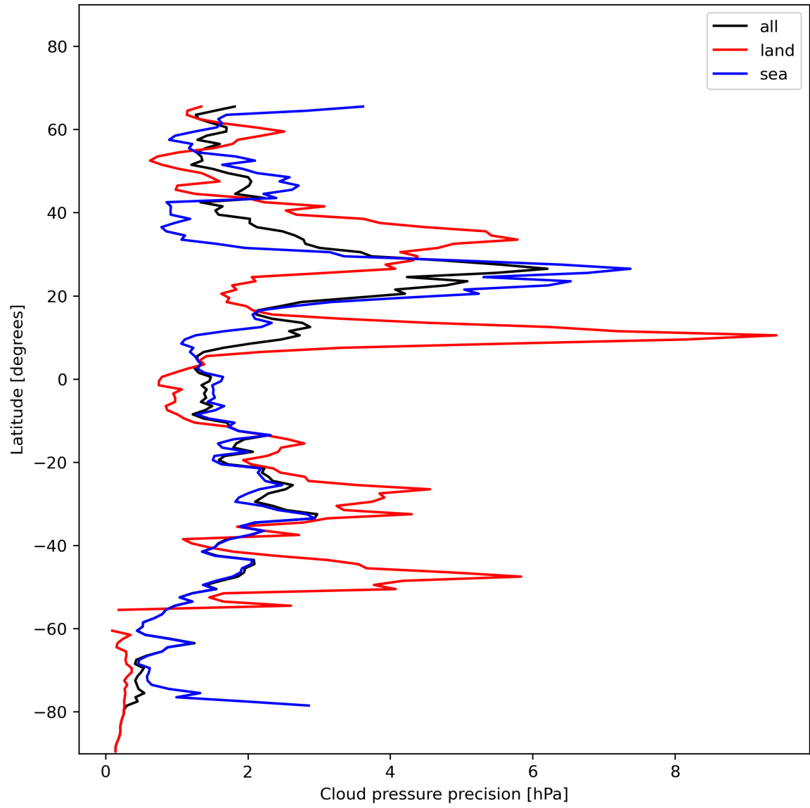
Figure 14: Zonal average of “Cloud pressure precision” for 2023-12-05 to 2023-12-07.
