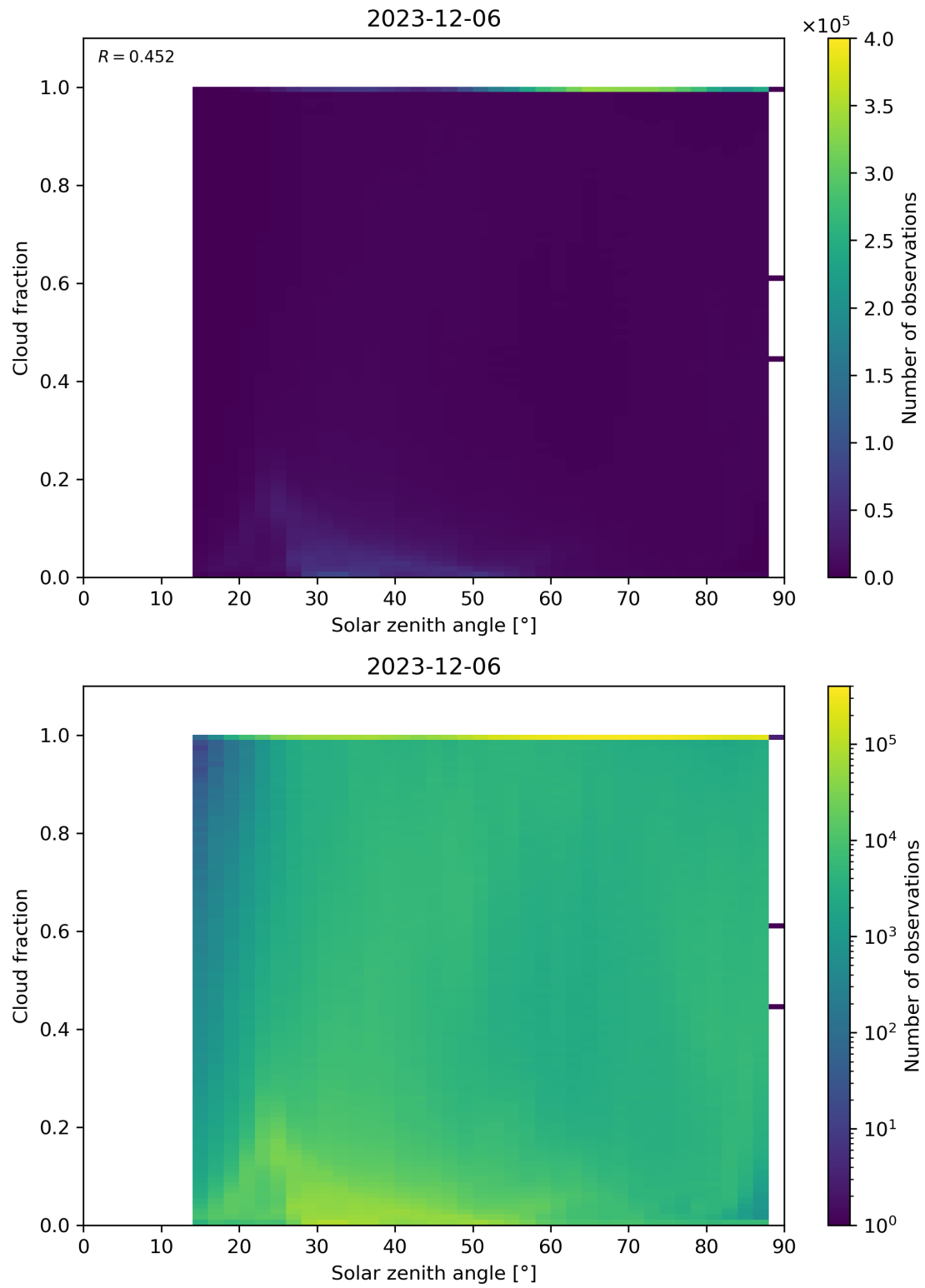
Figure 110: Scatter density plot of “Solar zenith angle” against “Cloud fraction” for 2023-12-05 to 2023-12-07.
