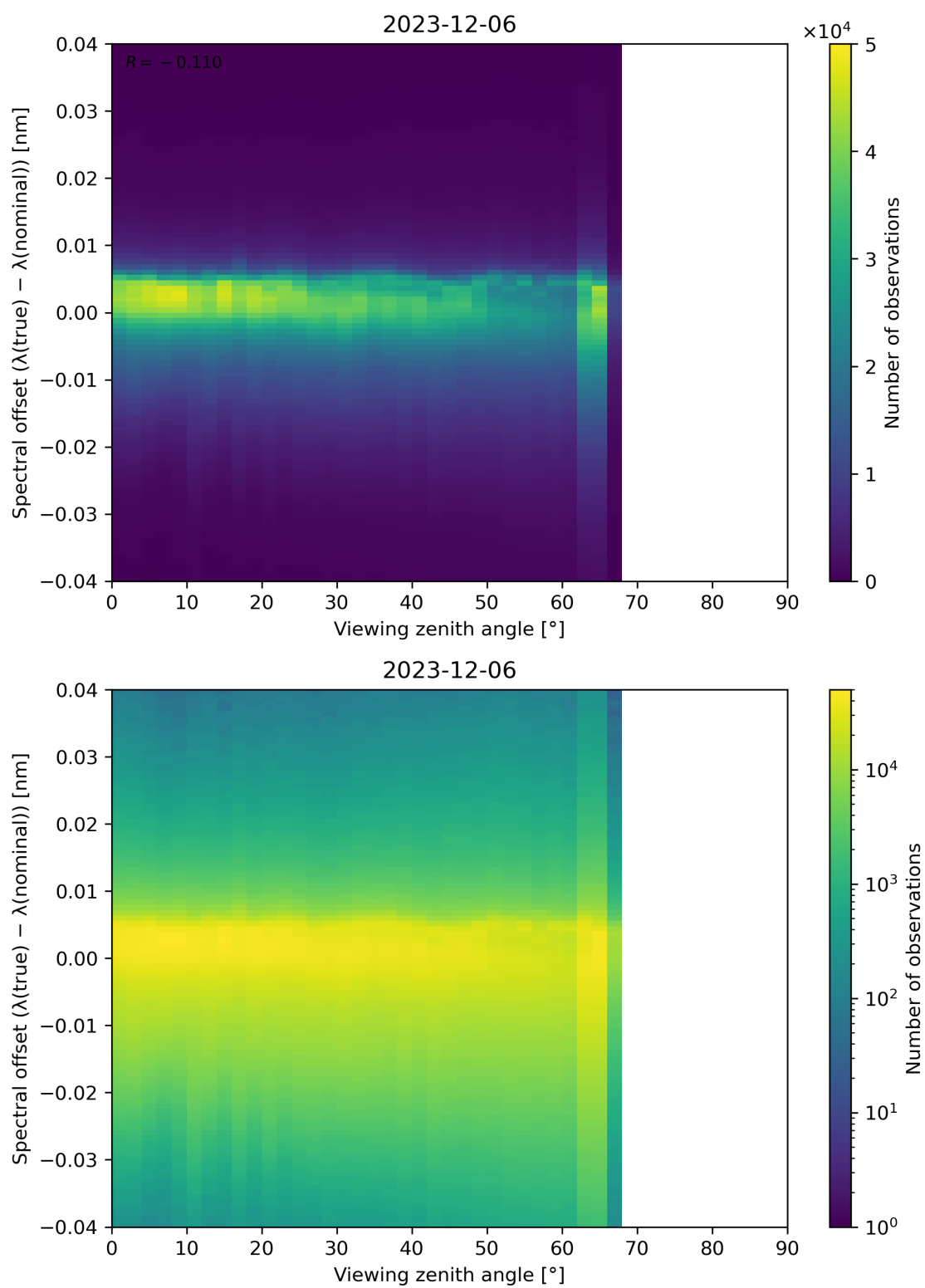
Figure 128: Scatter density plot of “Viewing zenith angle” against “Spectral offset ( \lambda(\text{true}) - \lambda(\text{nominal}) )” for 2023-12-05 to 2023-12-07.
