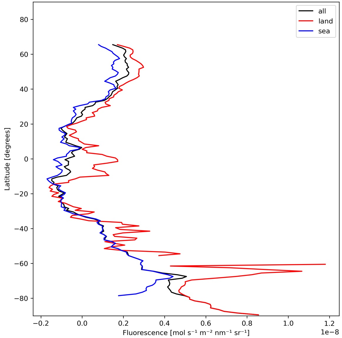
Figure 23: Zonal average of “Fluorescence” for 2023-12-05 to 2023-12-07.
