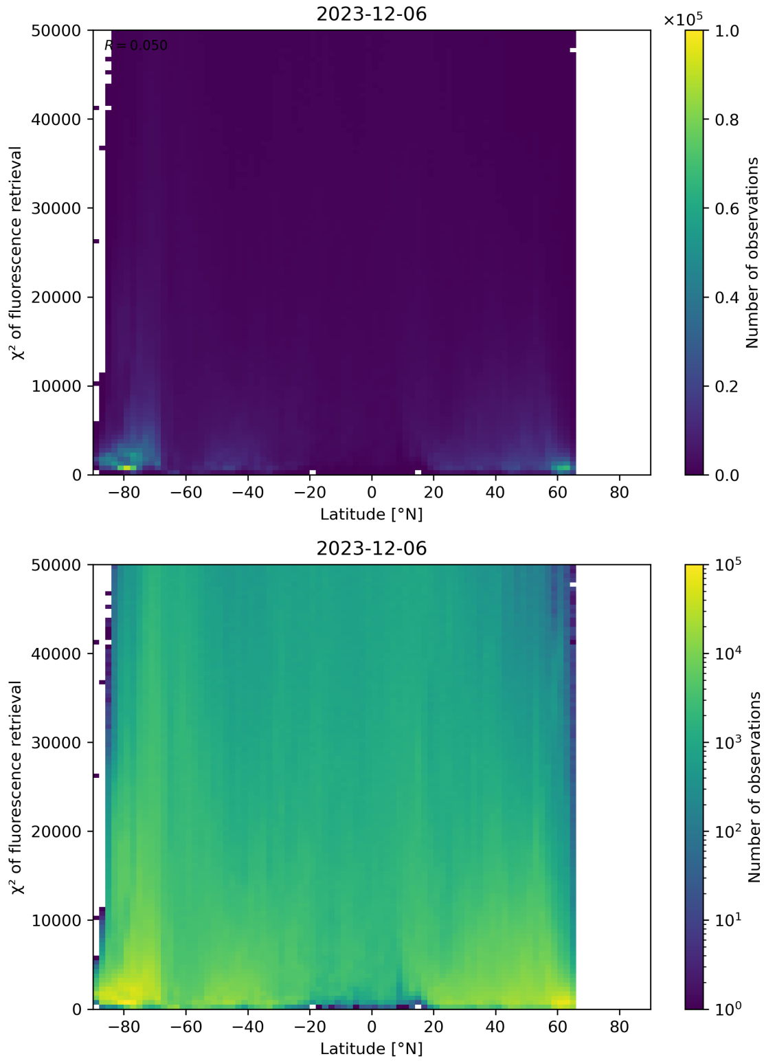
Figure 89: Scatter density plot of “Latitude” against “ \chi^2 of fluorescence retrieval” for 2023-12-05 to 2023-12-07.
