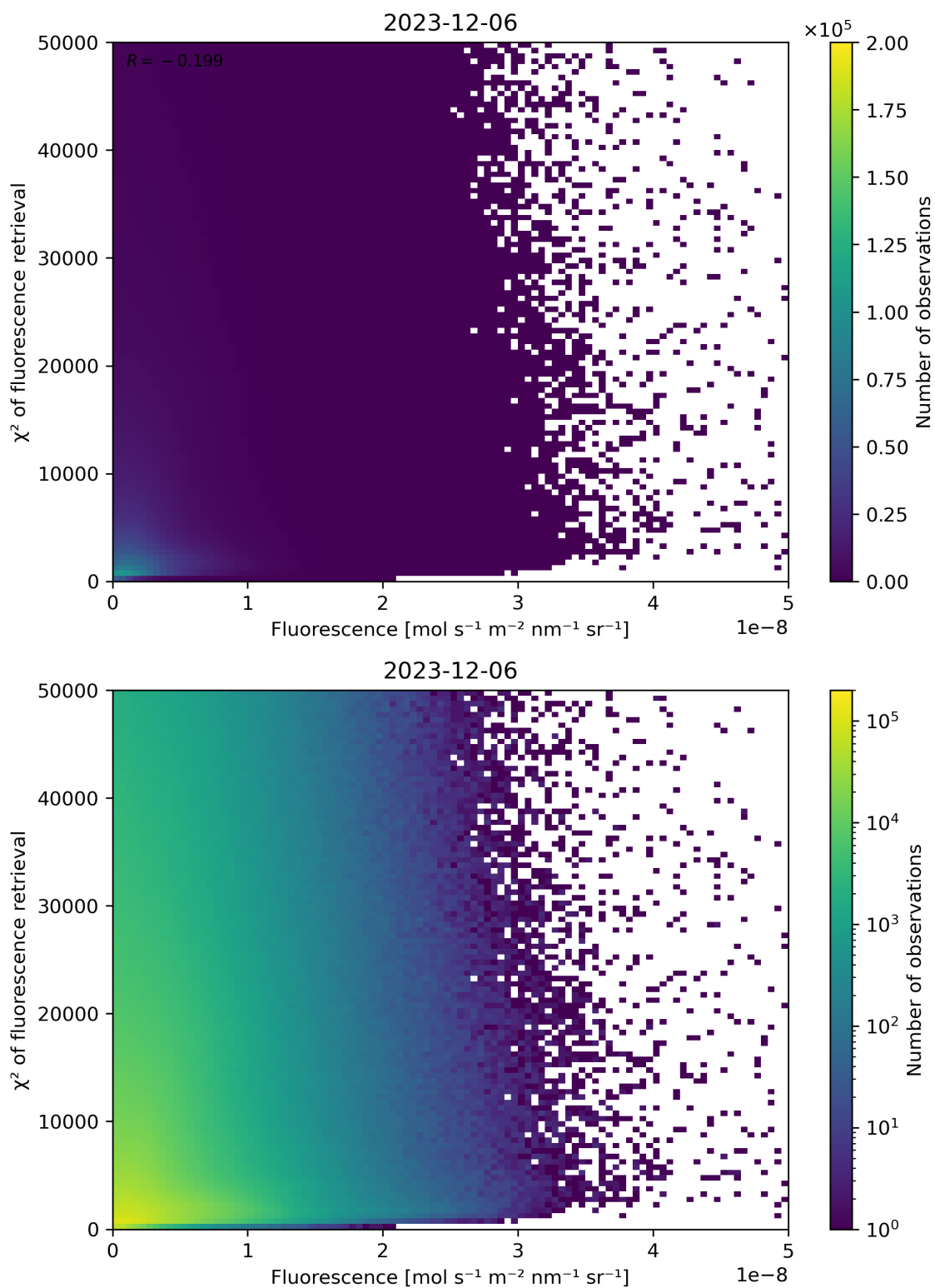
Figure 85: Scatter density plot of “Fluorescence” against “ \chi^2 of fluorescence retrieval” for 2023-12-05 to 2023-12-07.
