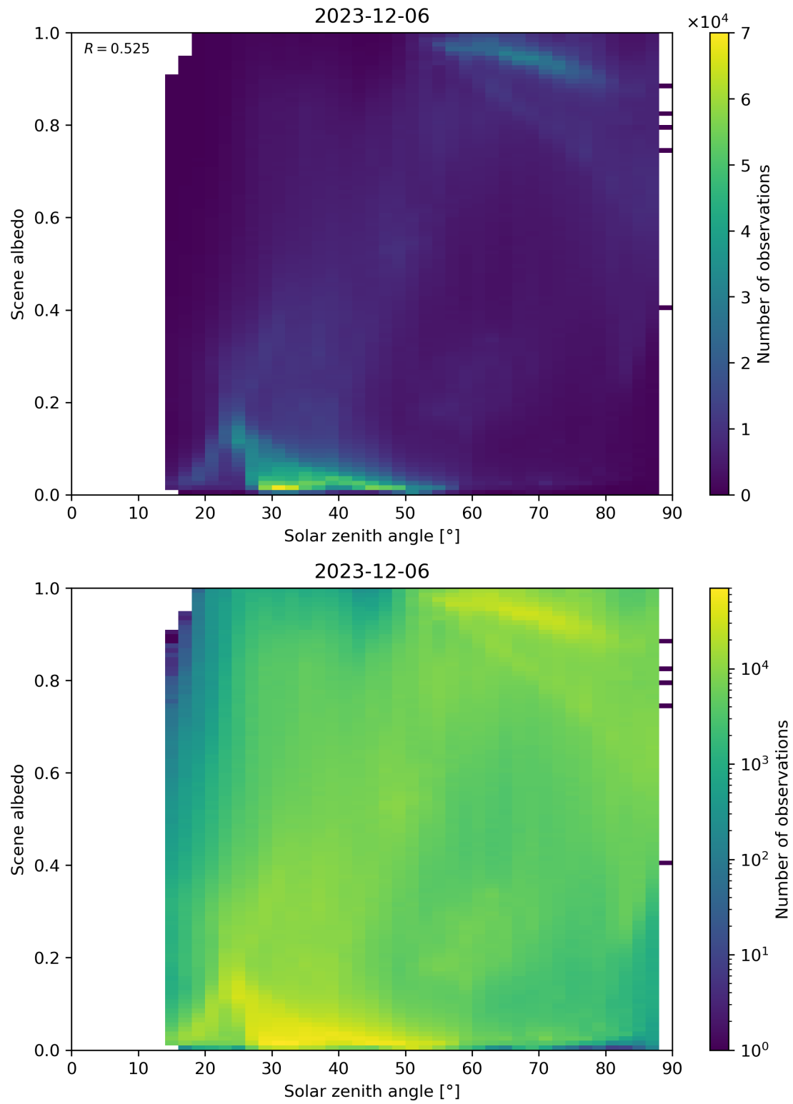
Figure 116: Scatter density plot of “Solar zenith angle” against “Scene albedo” for 2023-12-05 to 2023-12-07.
