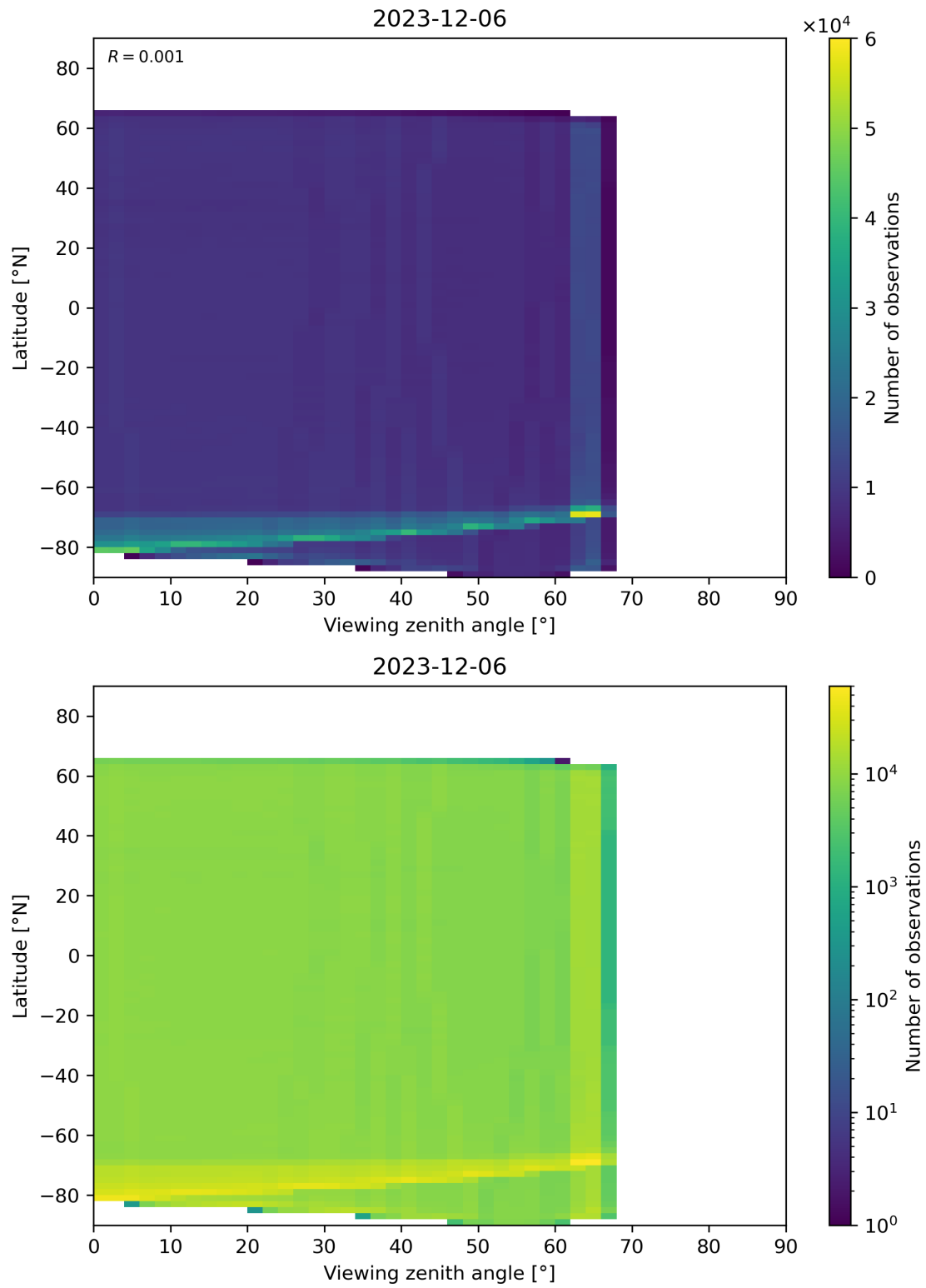
Figure 123: Scatter density plot of “Viewing zenith angle” against “Latitude” for 2023-12-05 to 2023-12-07.
