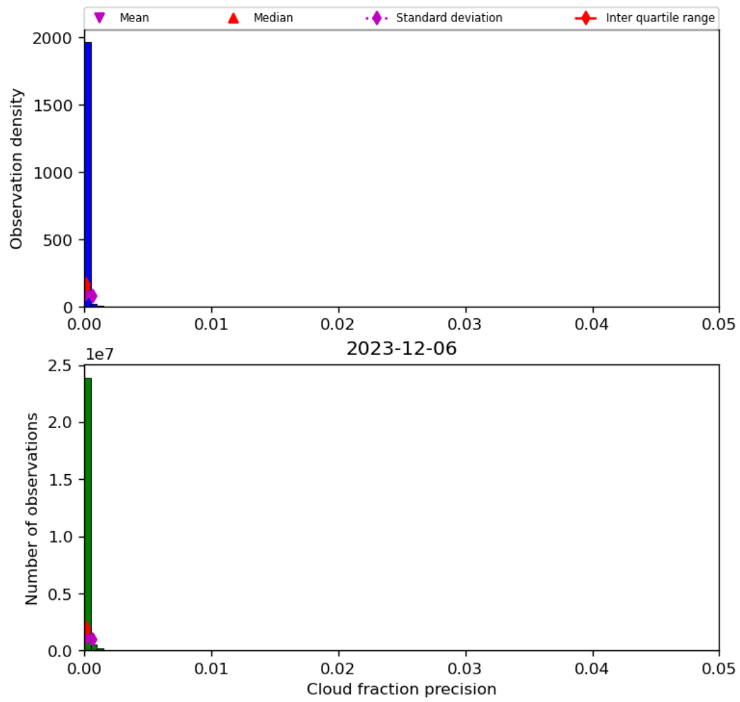
Figure 33: Histogram of “Cloud fraction precision” for 2023-12-05 to 2023-12-07
