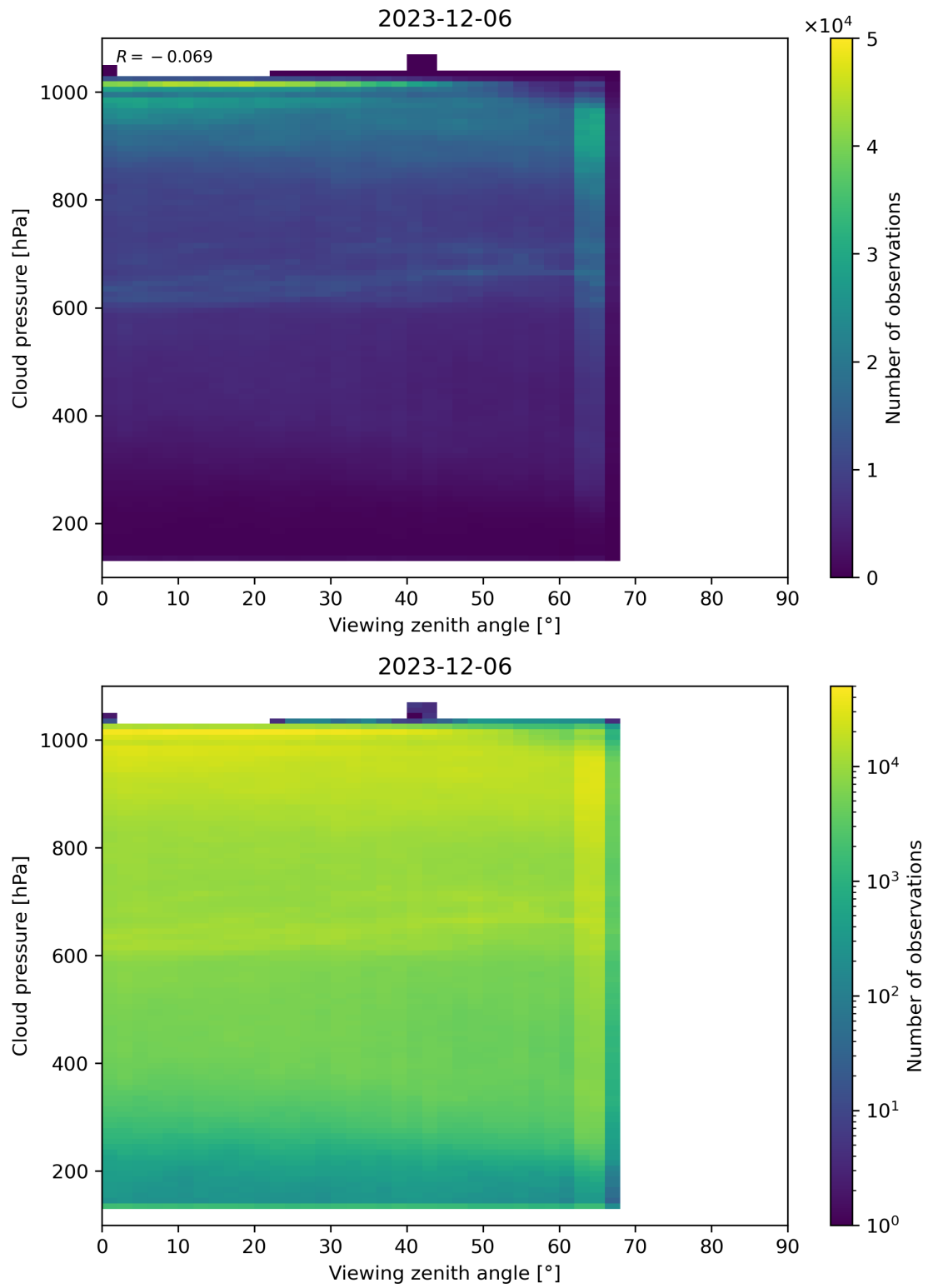
Figure 121: Scatter density plot of “Viewing zenith angle” against “Cloud pressure” for 2023-12-05 to 2023-12-07.
