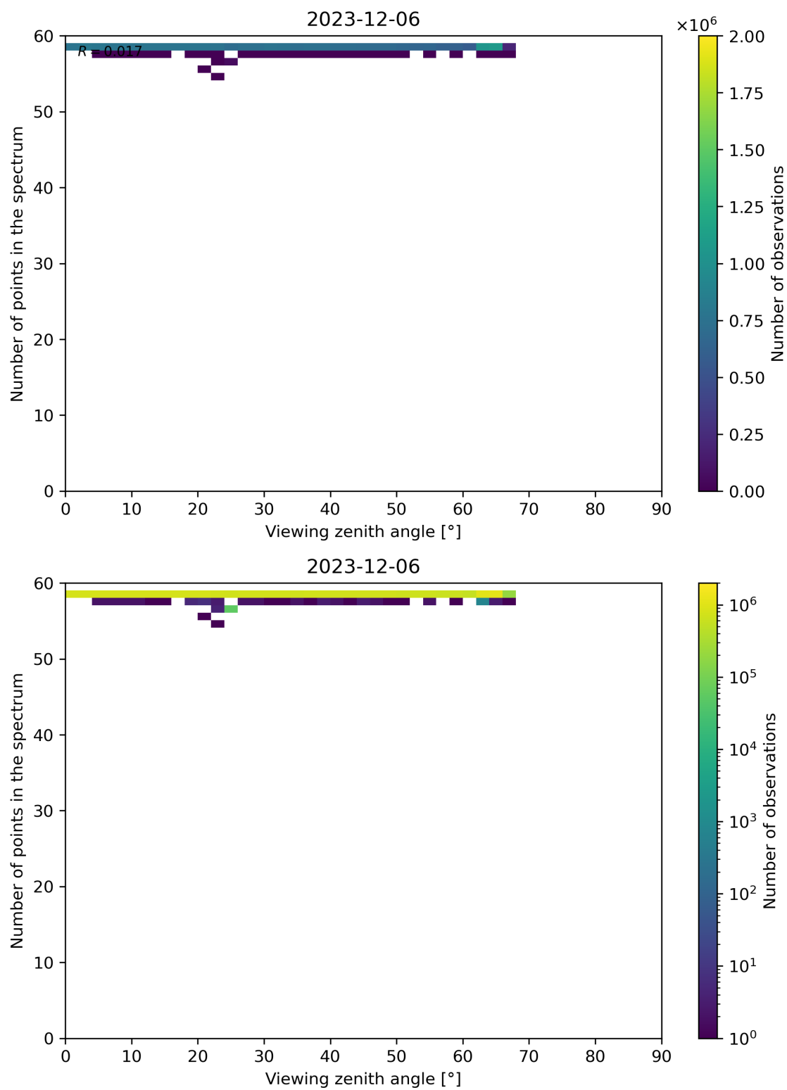
Figure 125: Scatter density plot of “Viewing zenith angle” against “Number of points in the spectrum” for 2023-12-05 to 2023-12-07.
