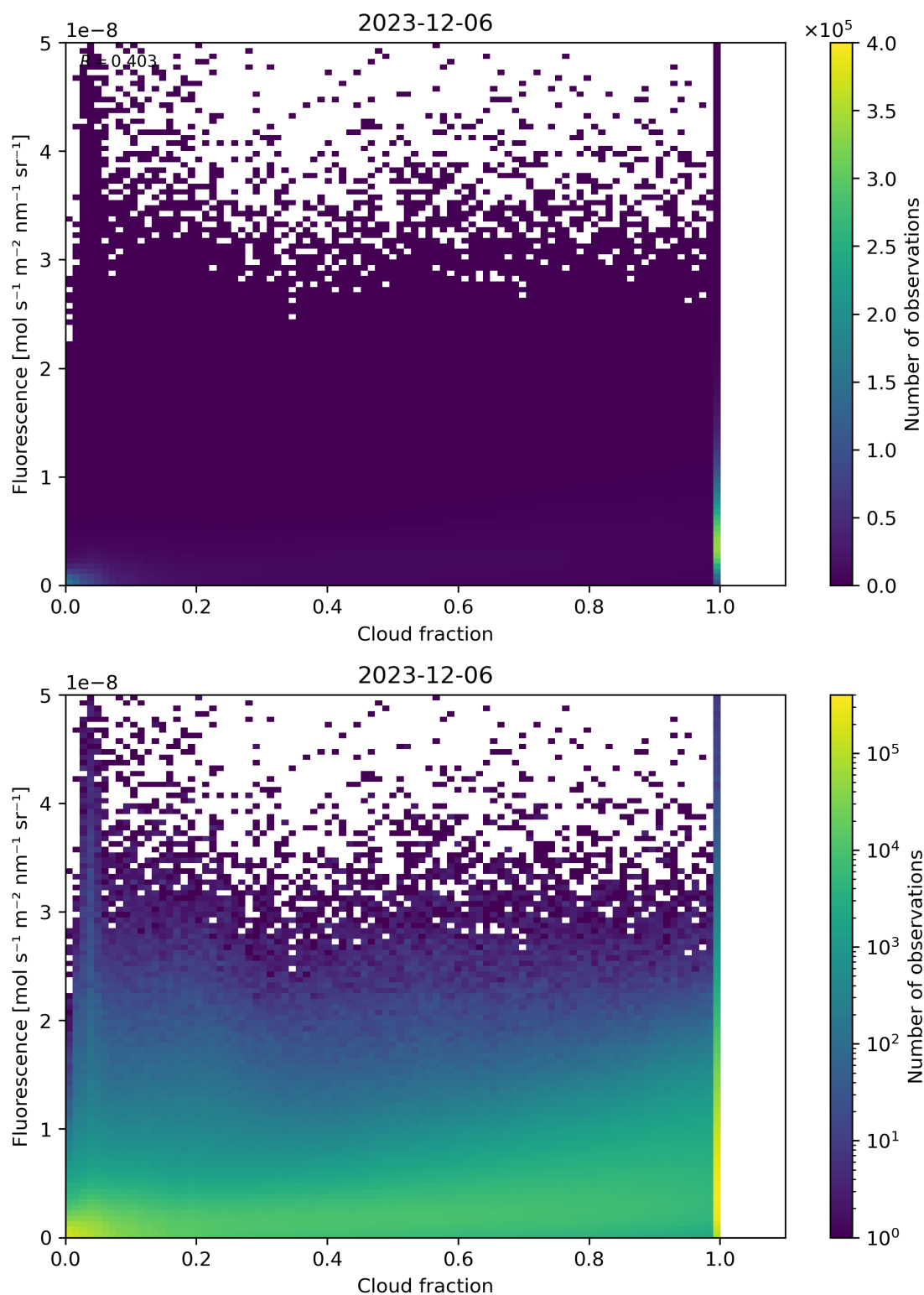
Figure 72: Scatter density plot of “Cloud fraction” against “Fluorescence” for 2023-12-05 to 2023-12-07.
