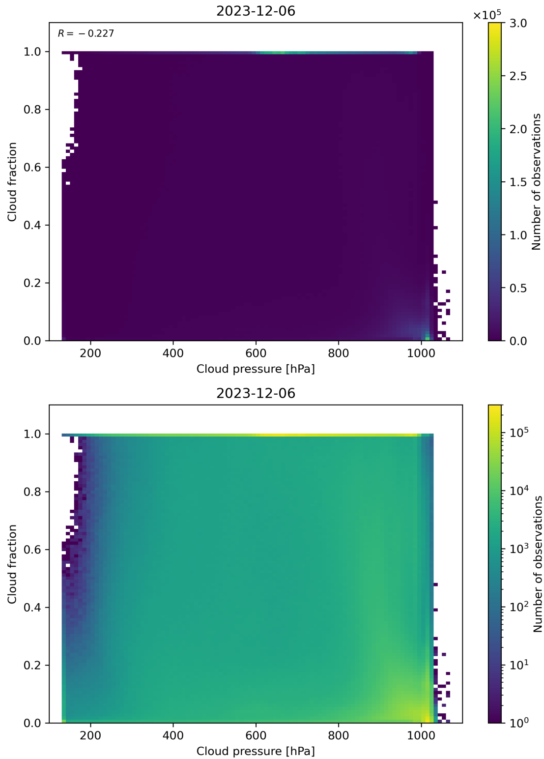
Figure 79: Scatter density plot of “Cloud pressure” against “Cloud fraction” for 2023-12-05 to 2023-12-07.
