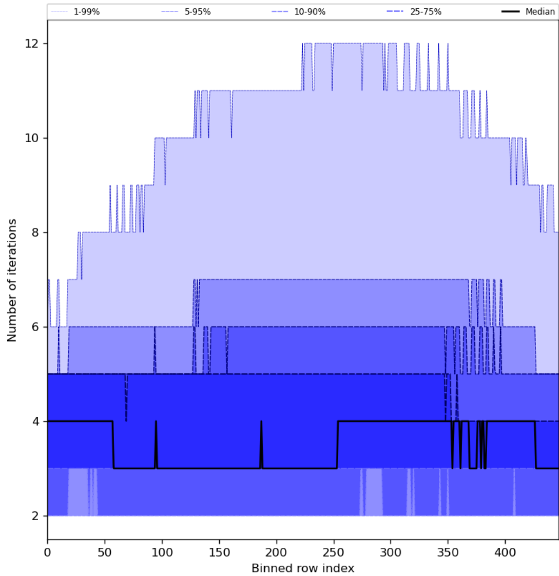
Figure 56: Along track statistics of “Number of iterations” for 2023-12-05 to 2023-12-07
