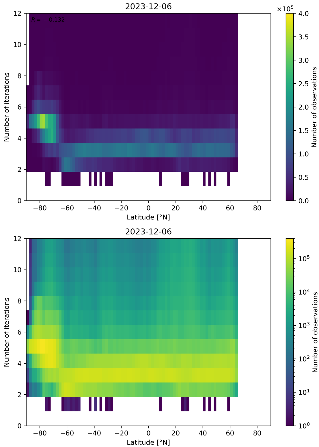
Figure 93: Scatter density plot of “Latitude” against “Number of iterations” for 2023-12-05 to 2023-12-07.
