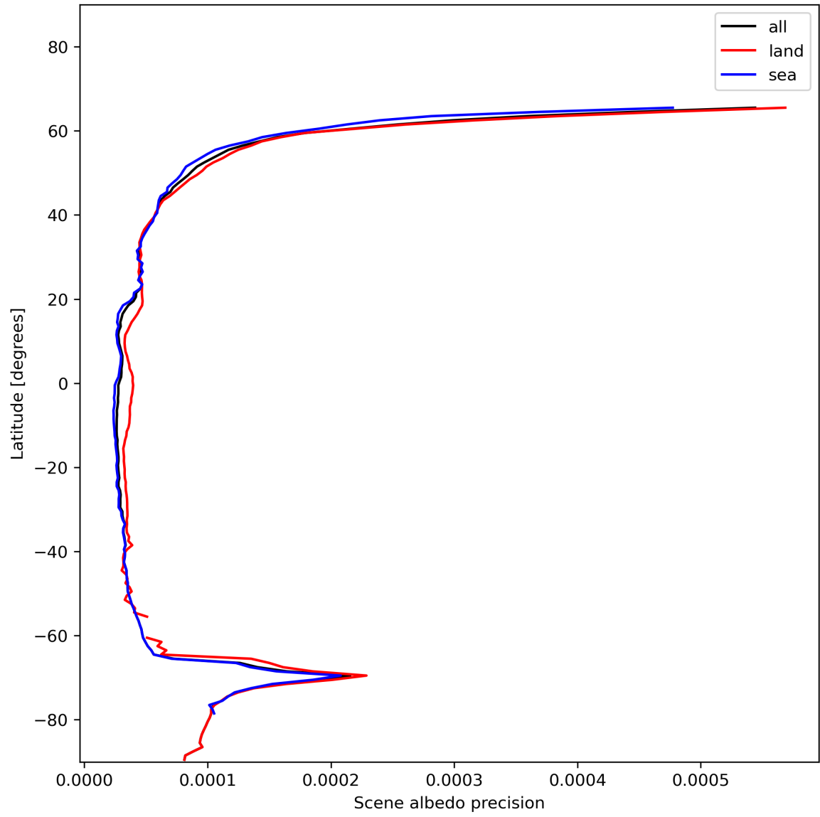
Figure 18: Zonal average of “Scene albedo precision” for 2023-12-05 to 2023-12-07.
