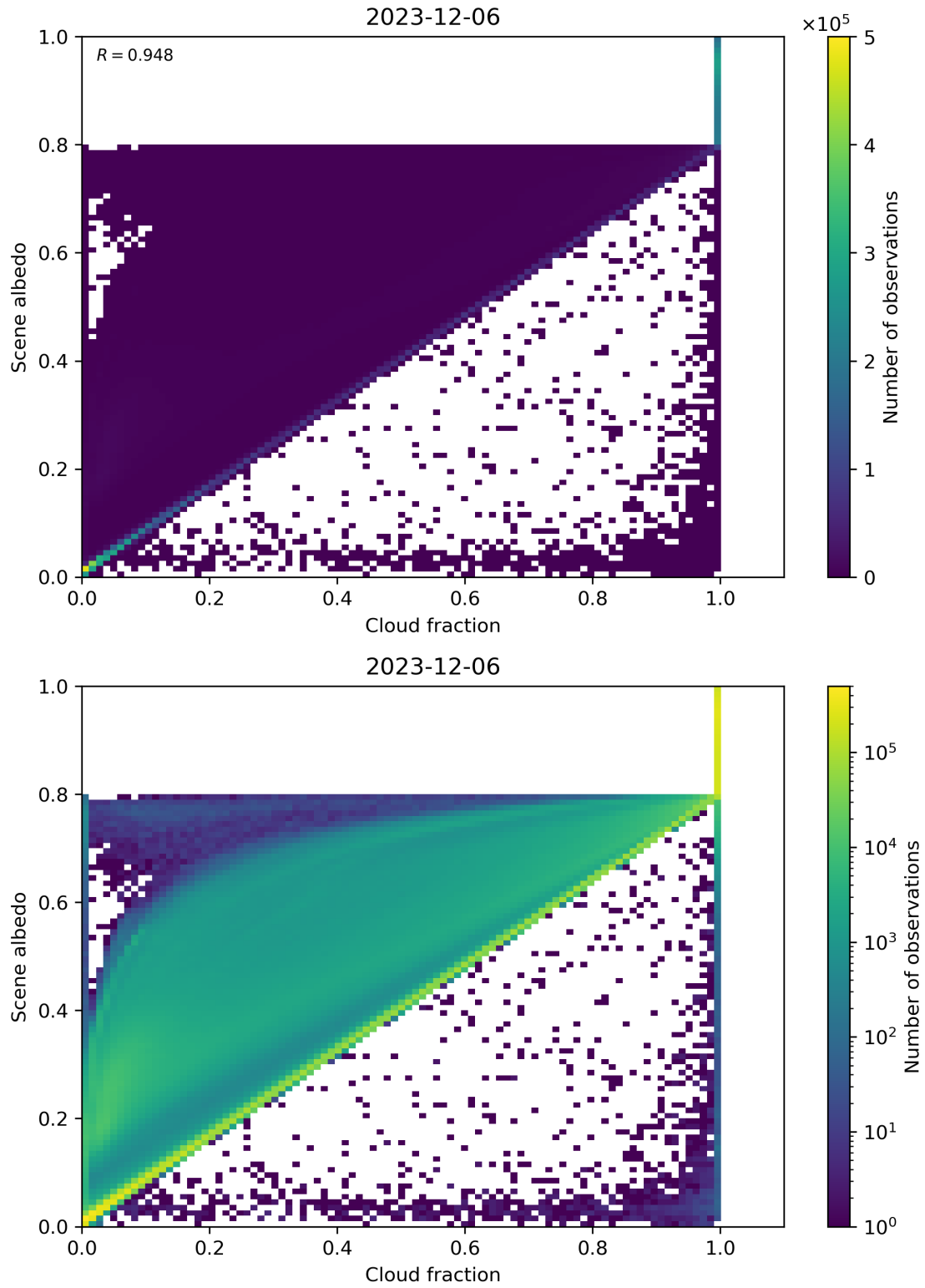
Figure 75: Scatter density plot of “Cloud fraction” against “Scene albedo” for 2023-12-05 to 2023-12-07.
