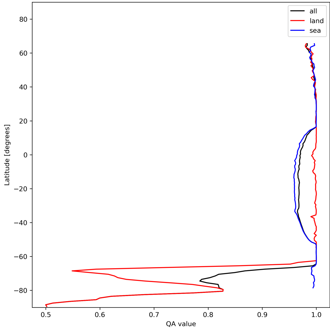
Figure 12: Zonal average of “QA value” for 2023-12-05 to 2023-12-07.
