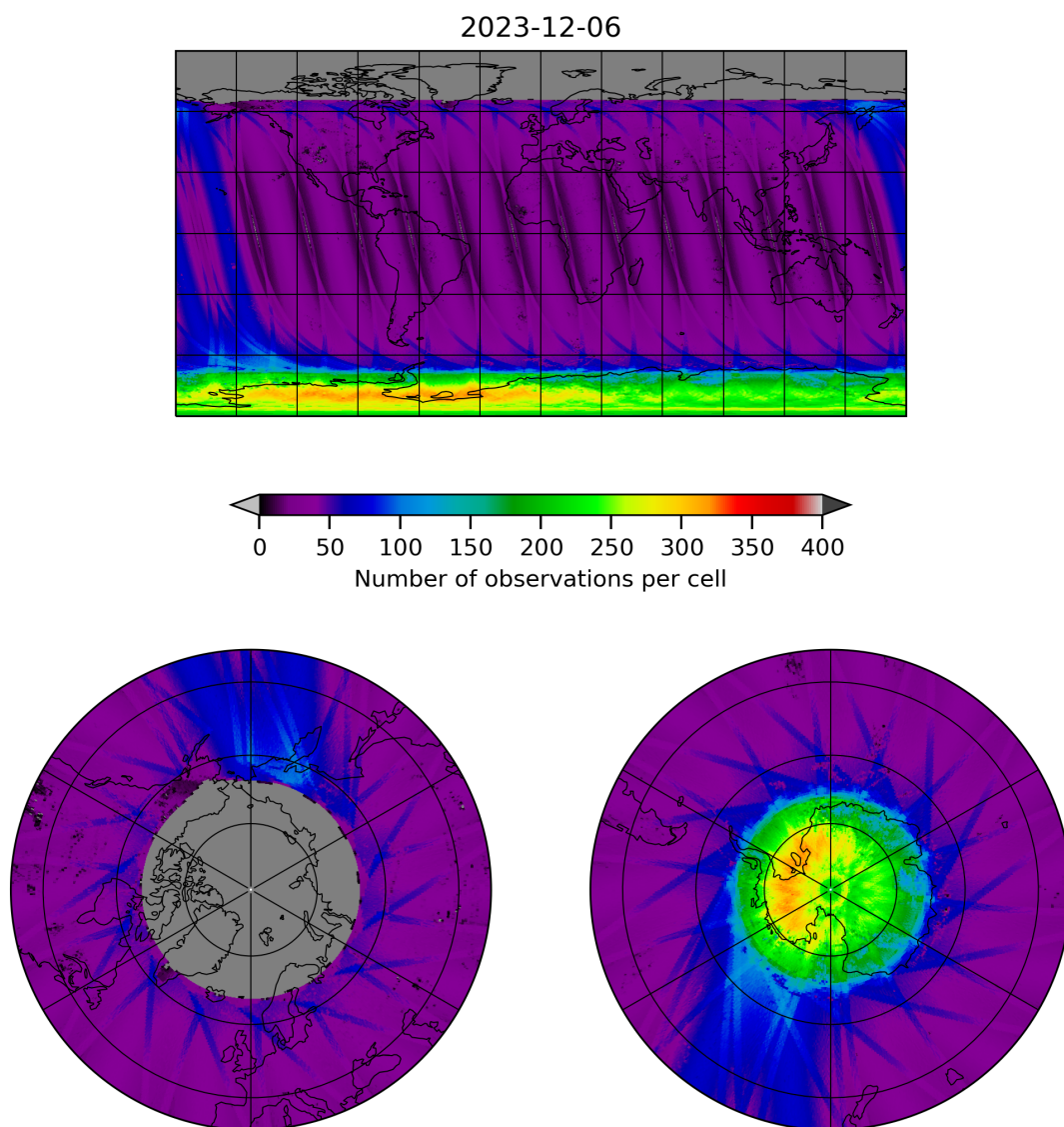
Figure 11: Map of the number of observations for 2023-12-05 to 2023-12-07
