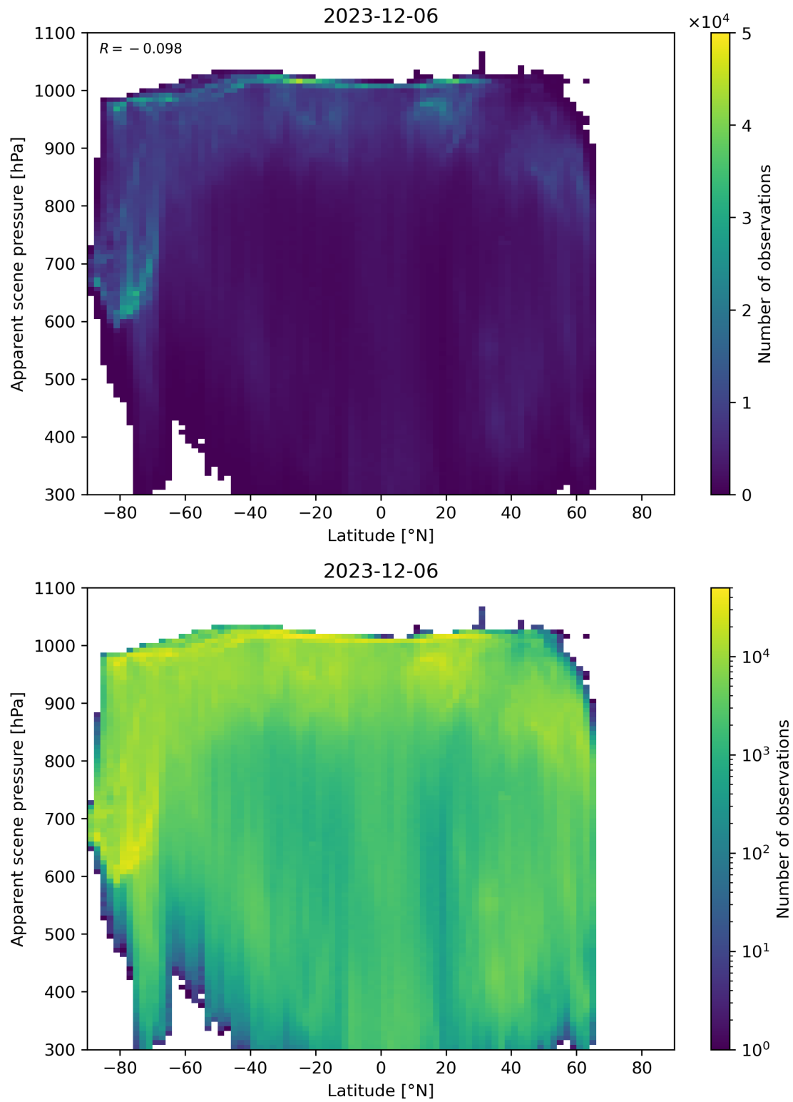
Figure 88: Scatter density plot of “Latitude” against “Apparent scene pressure” for 2023-12-05 to 2023-12-07.
