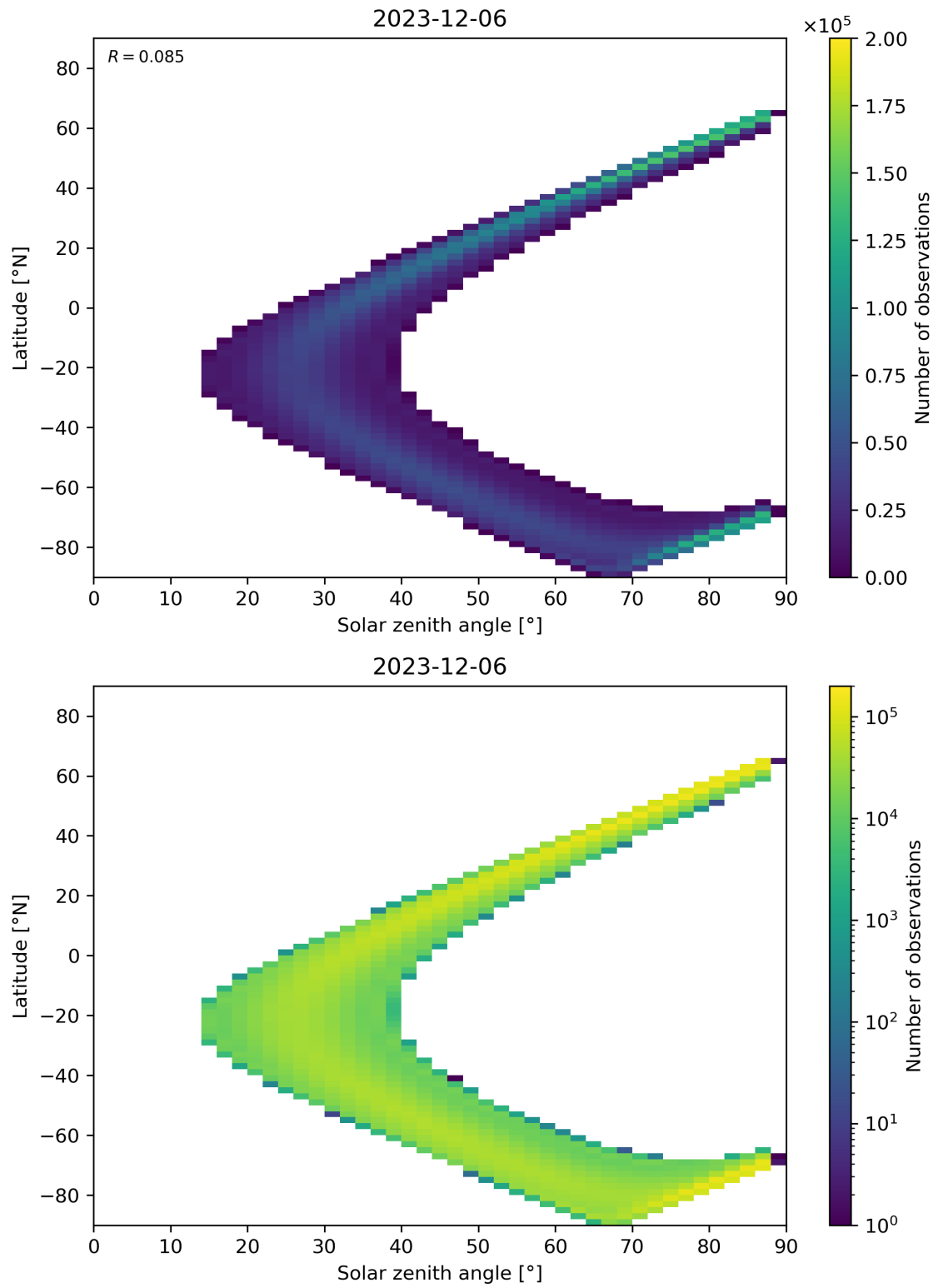
Figure 113: Scatter density plot of “Solar zenith angle” against “Latitude” for 2023-12-05 to 2023-12-07.
