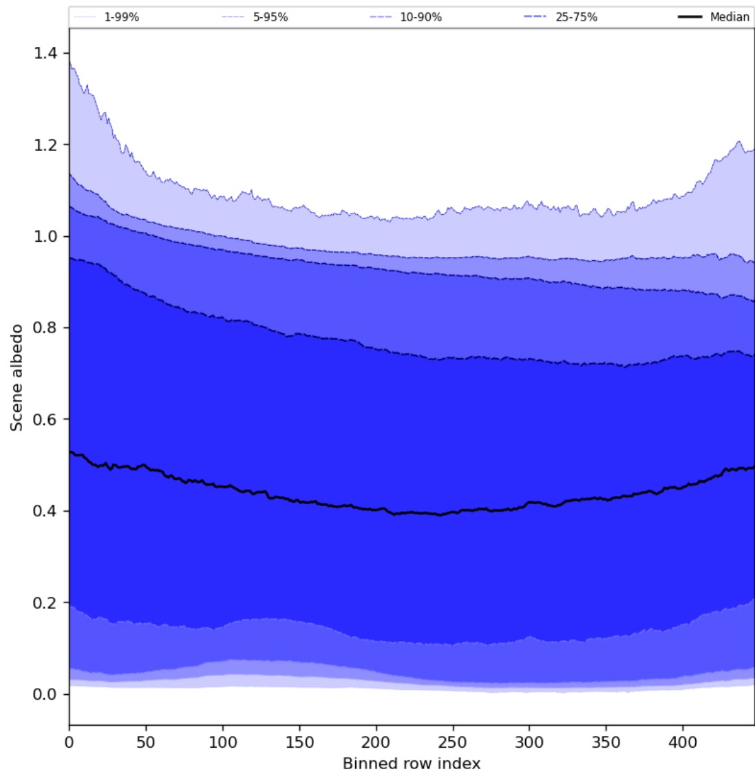
Figure 51: Along track statistics of “Scene albedo” for 2023-12-05 to 2023-12-07
