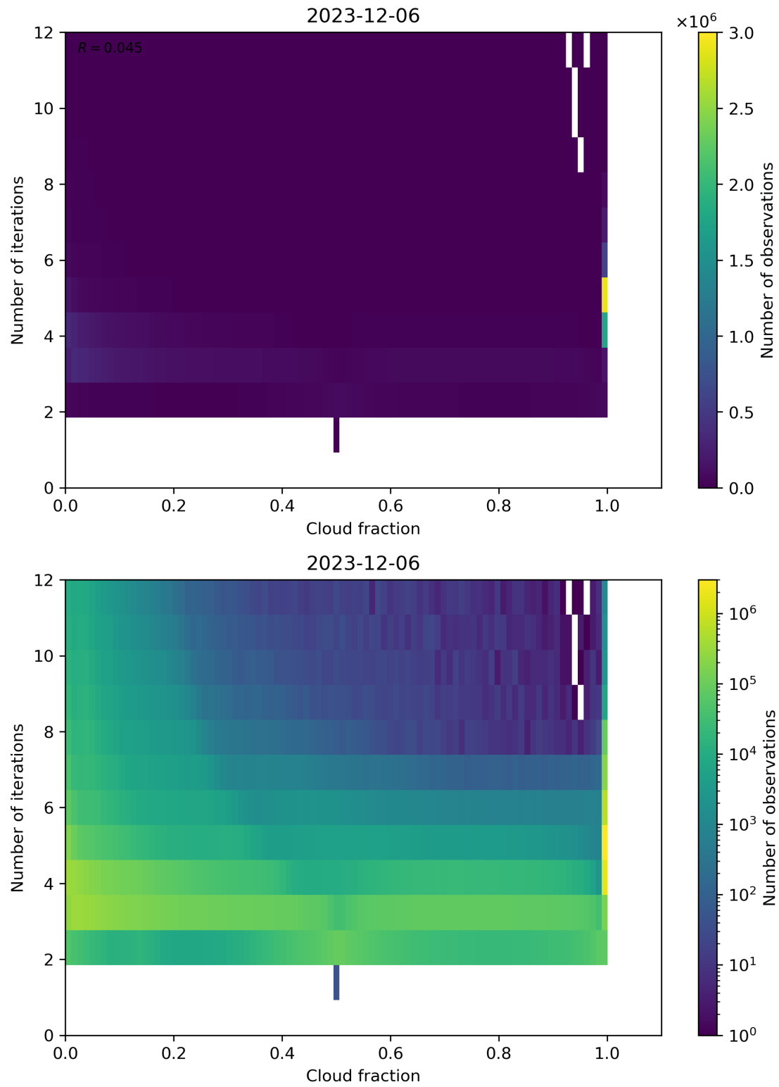
Figure 73: Scatter density plot of “Cloud fraction” against “Number of iterations” for 2023-12-05 to 2023-12-07.
