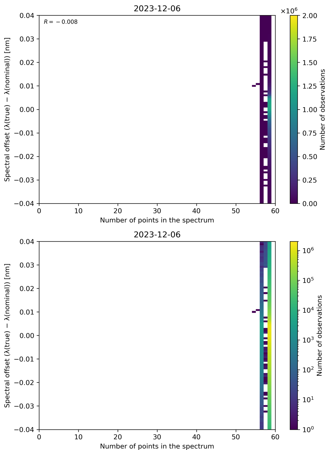
Figure 101: Scatter density plot of “Number of points in the spectrum” against “Spectral offset ( \lambda(\text{true}) - \lambda(\text{nominal}) )” for 2023-12-05 to 2023-12-07.
