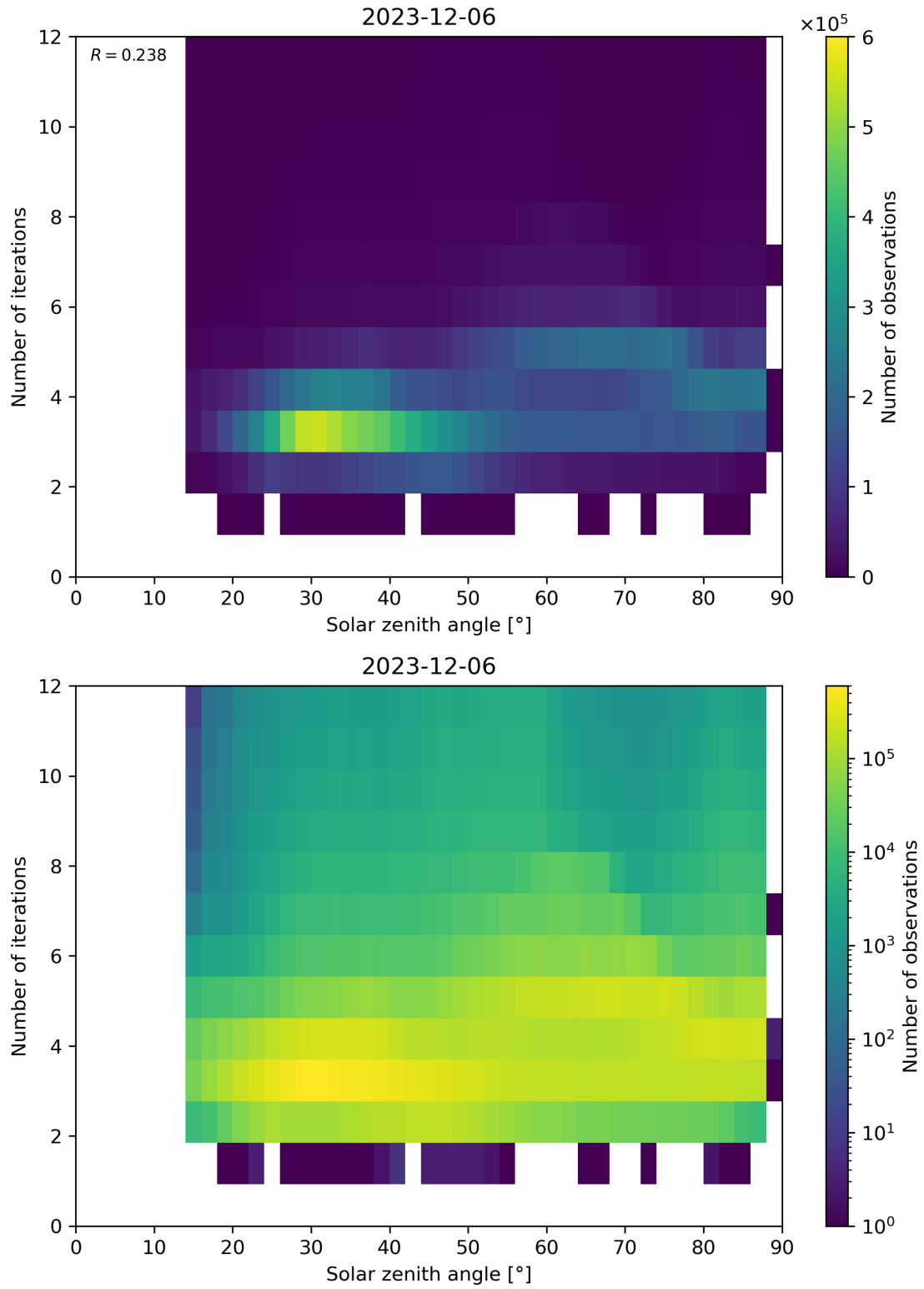
Figure 114: Scatter density plot of “Solar zenith angle” against “Number of iterations” for 2023-12-05 to 2023-12-07.
