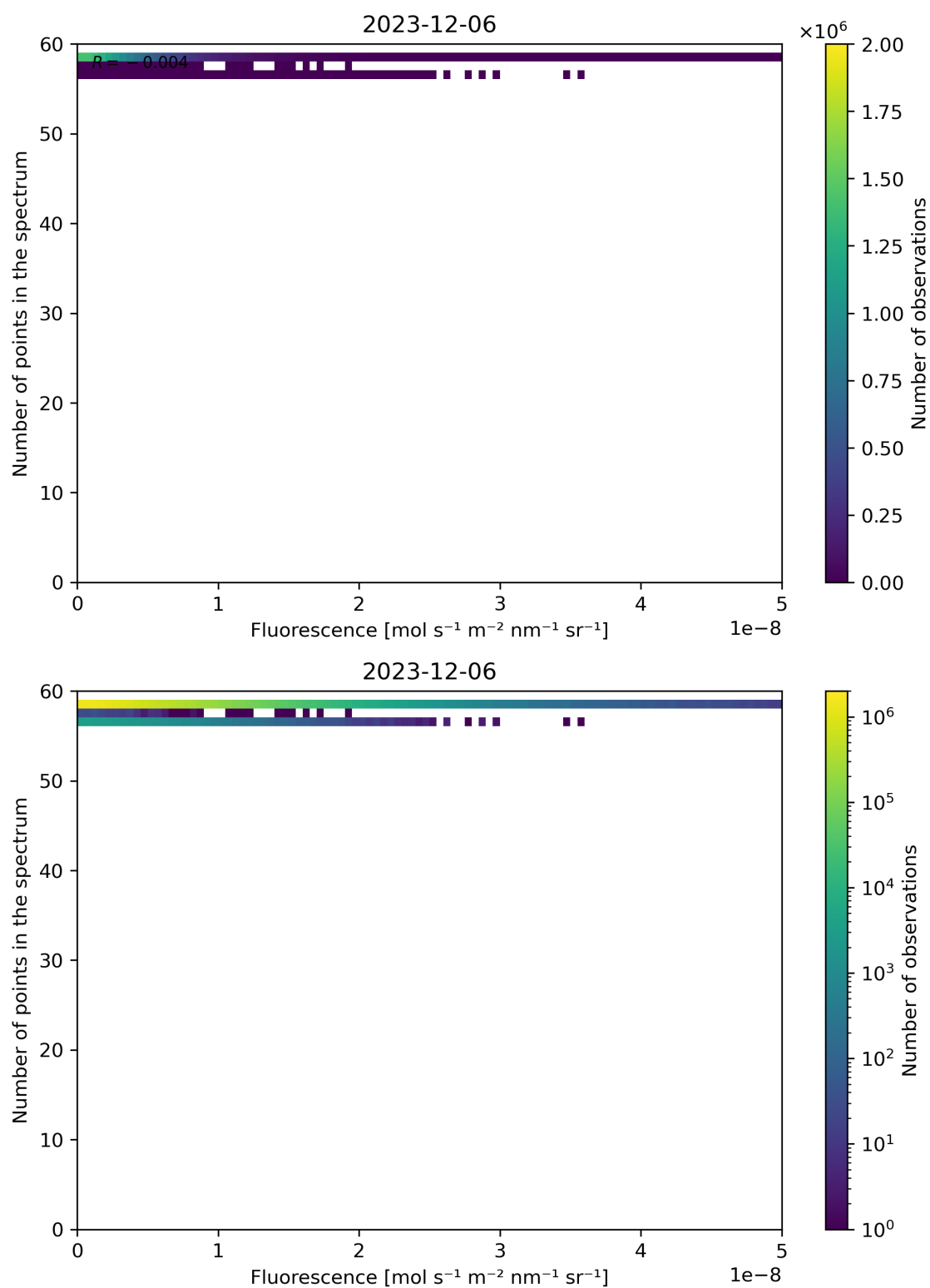
Figure 86: Scatter density plot of “Fluorescence” against “Number of points in the spectrum” for 2023-12-05 to 2023-12-07.
