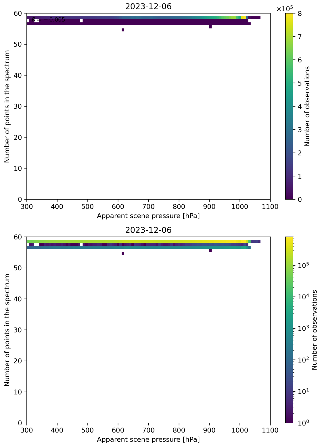
Figure 66: Scatter density plot of “Apparent scene pressure” against “Number of points in the spectrum” for 2023-12-05 to 2023-12-07.
