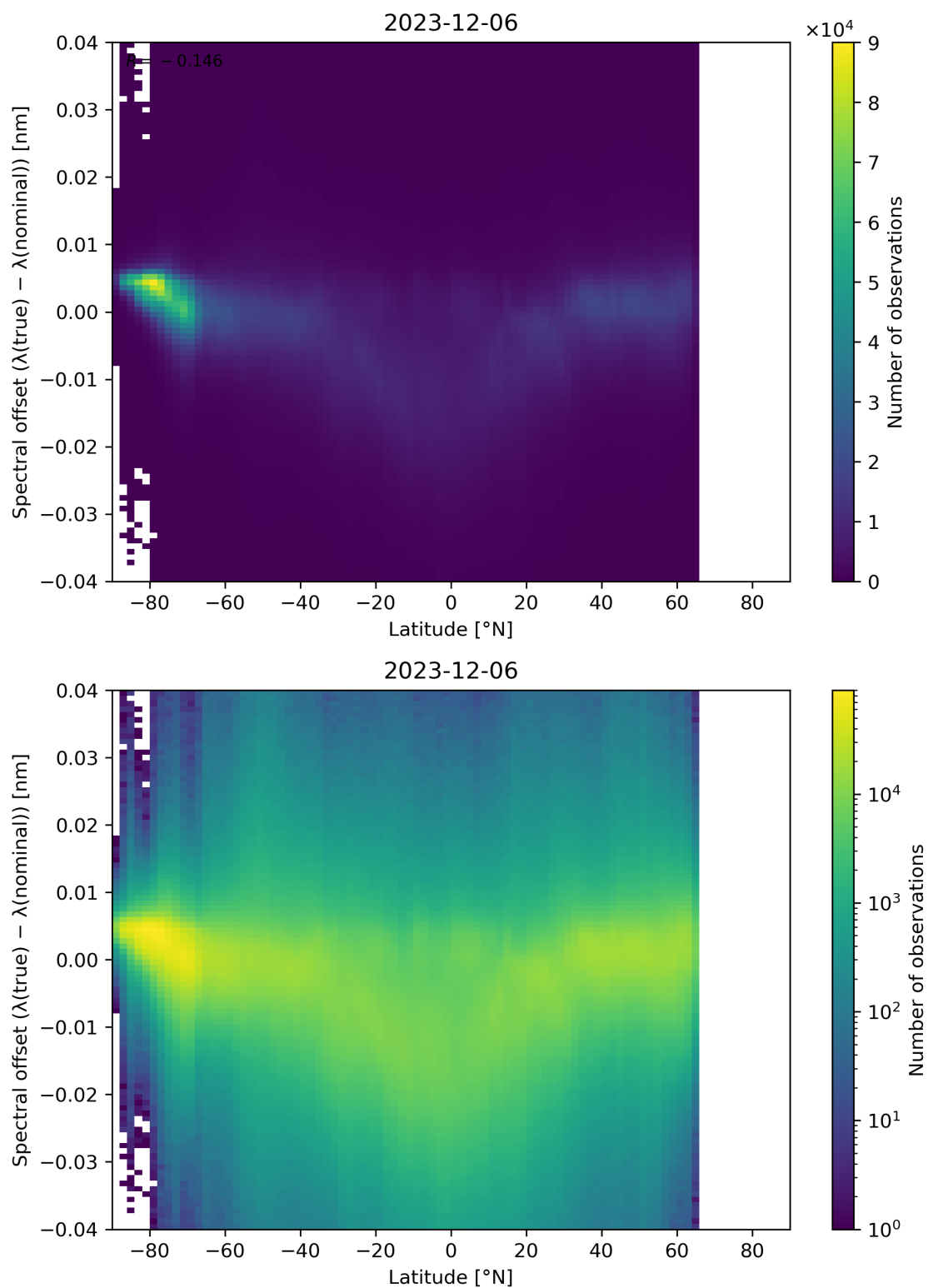
Figure 96: Scatter density plot of “Latitude” against “Spectral offset ( \lambda(\text{true}) - \lambda(\text{nominal}) )” for 2023-12-05 to 2023-12-07.
