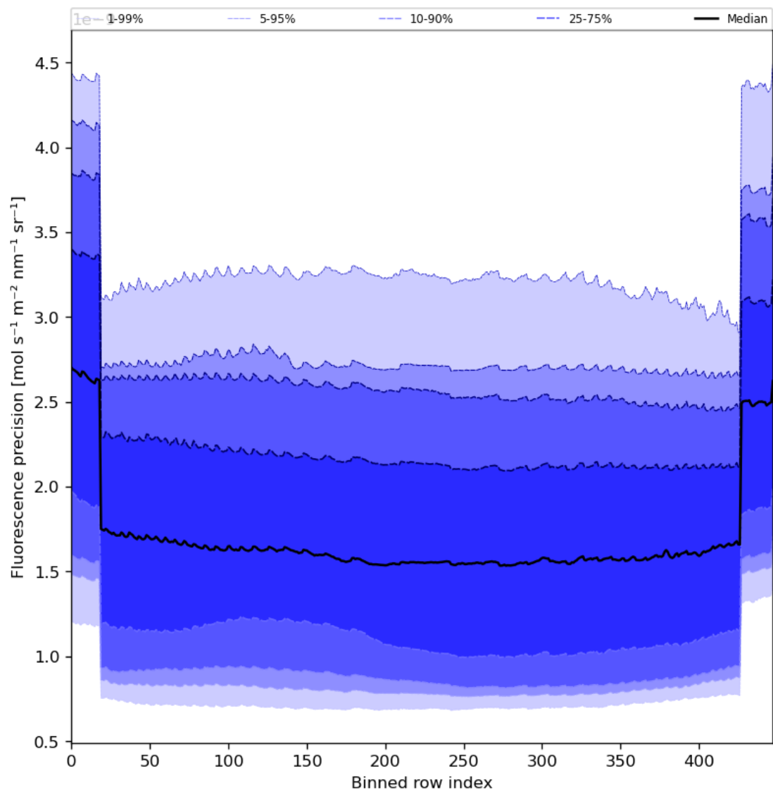
Figure 58: Along track statistics of “Fluorescence precision” for 2023-12-05 to 2023-12-07
