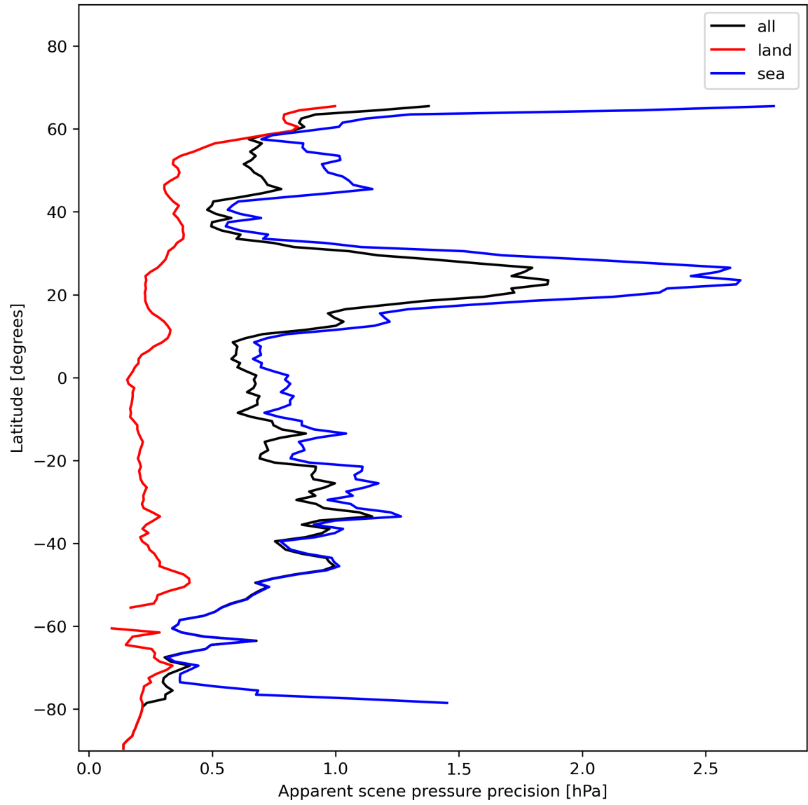
Figure 20: Zonal average of “Apparent scene pressure precision” for 2023-12-05 to 2023-12-07.
