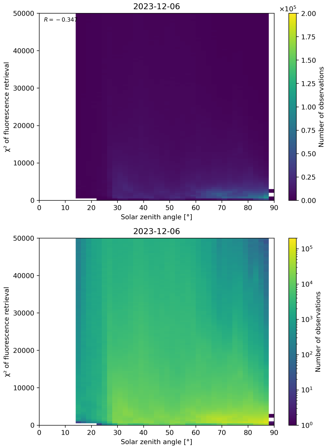
Figure 109: Scatter density plot of “Solar zenith angle” against “ \chi^2 of fluorescence retrieval” for 2023-12-05 to 2023-12-07.
