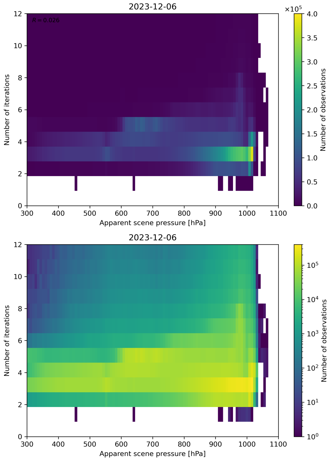
Figure 65: Scatter density plot of “Apparent scene pressure” against “Number of iterations” for 2023-12-05 to 2023-12-07.
