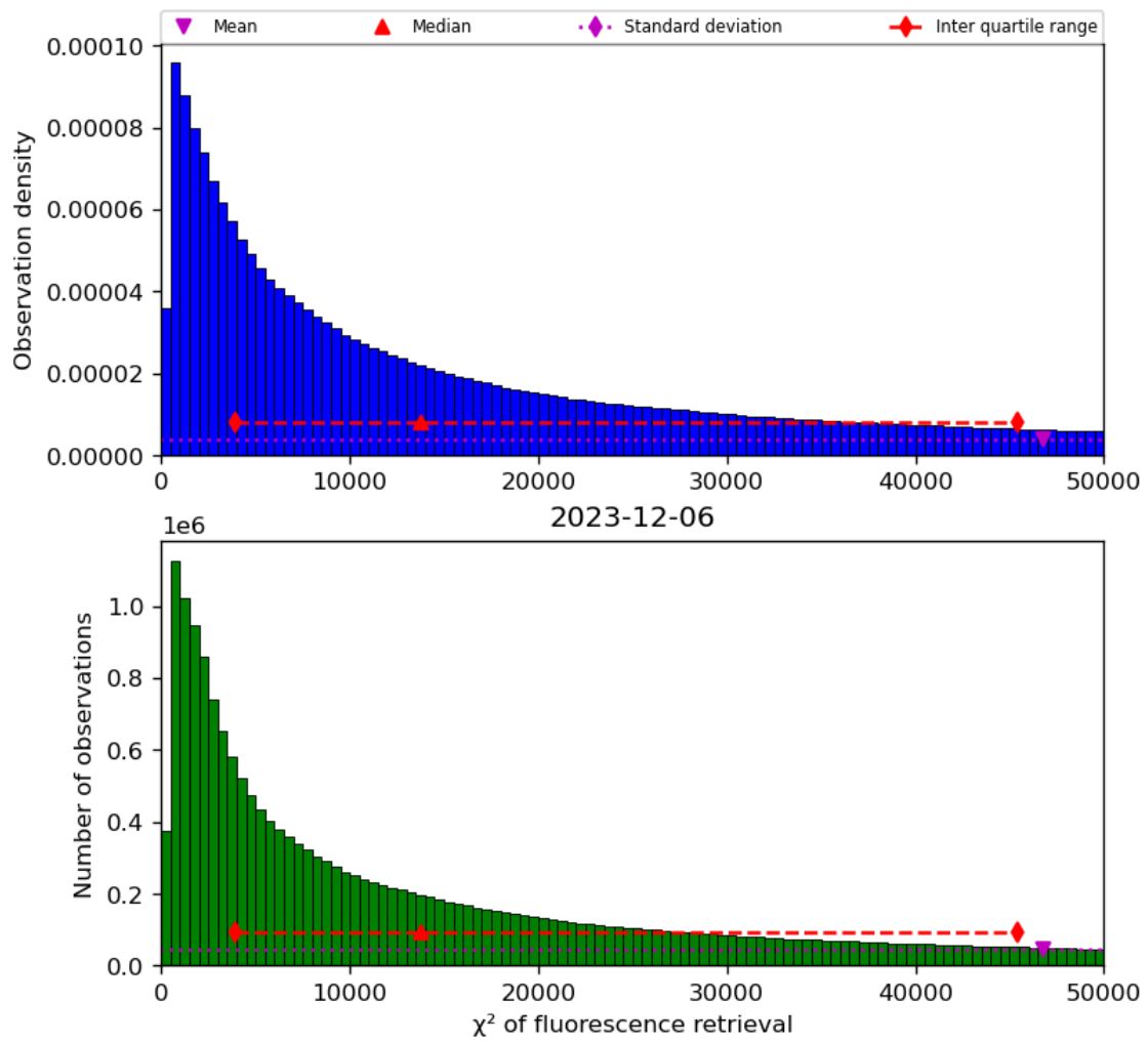
Figure 42: Histogram of “ \chi^2 of fluorescence retrieval” for 2023-12-05 to 2023-12-07
