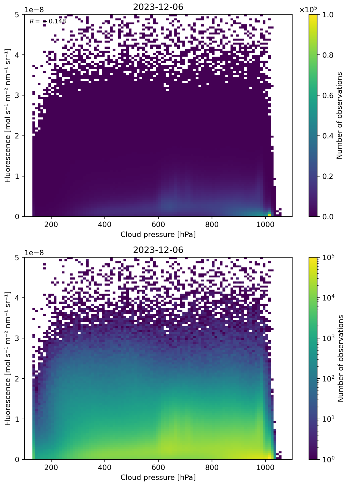
Figure 80: Scatter density plot of “Cloud pressure” against “Fluorescence” for 2023-12-05 to 2023-12-07.
