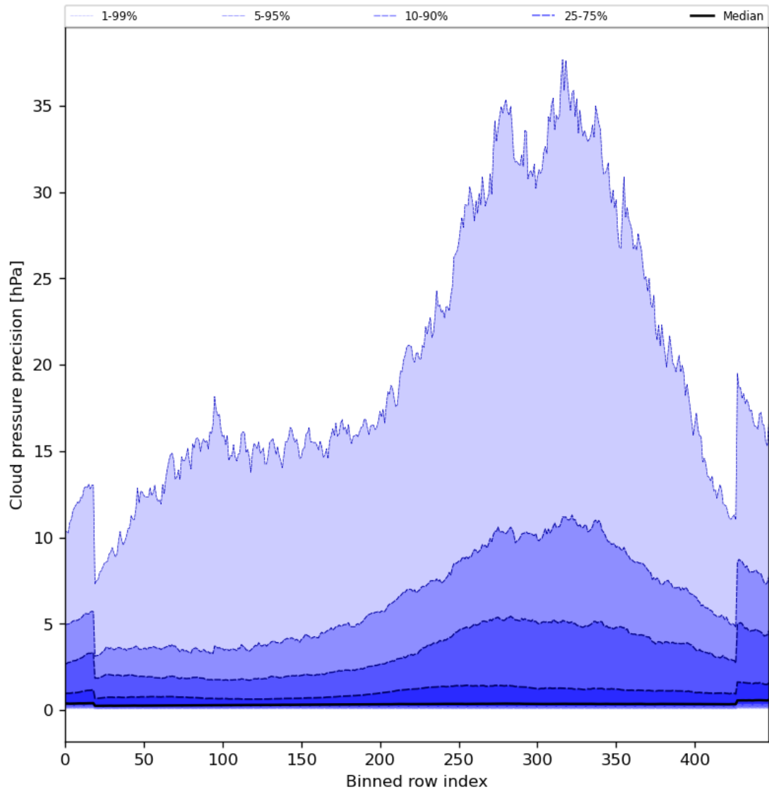
Figure 48: Along track statistics of “Cloud pressure precision” for 2023-12-05 to 2023-12-07
