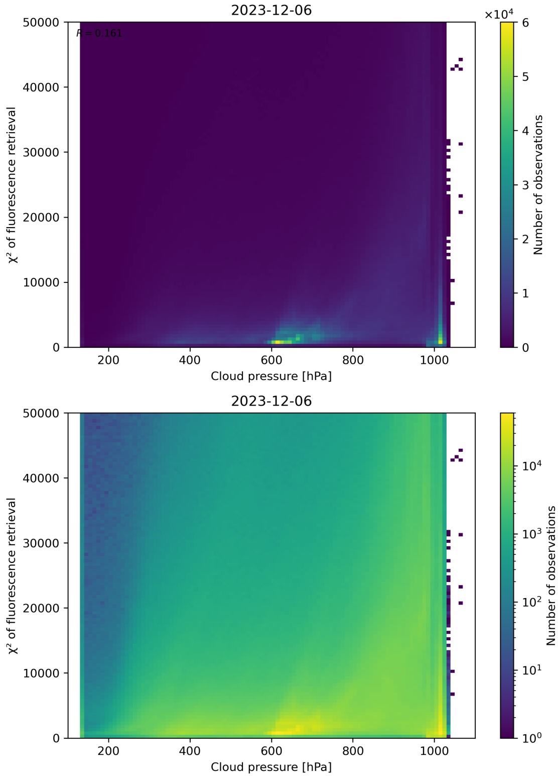
Figure 78: Scatter density plot of “Cloud pressure” against “ \chi^2 of fluorescence retrieval” for 2023-12-05 to 2023-12-07.
