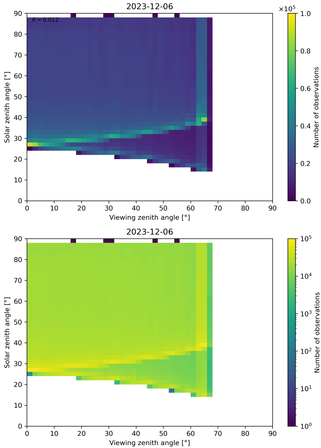
Figure 127: Scatter density plot of “Viewing zenith angle” against “Solar zenith angle” for 2023-12-05 to 2023-12-07.
