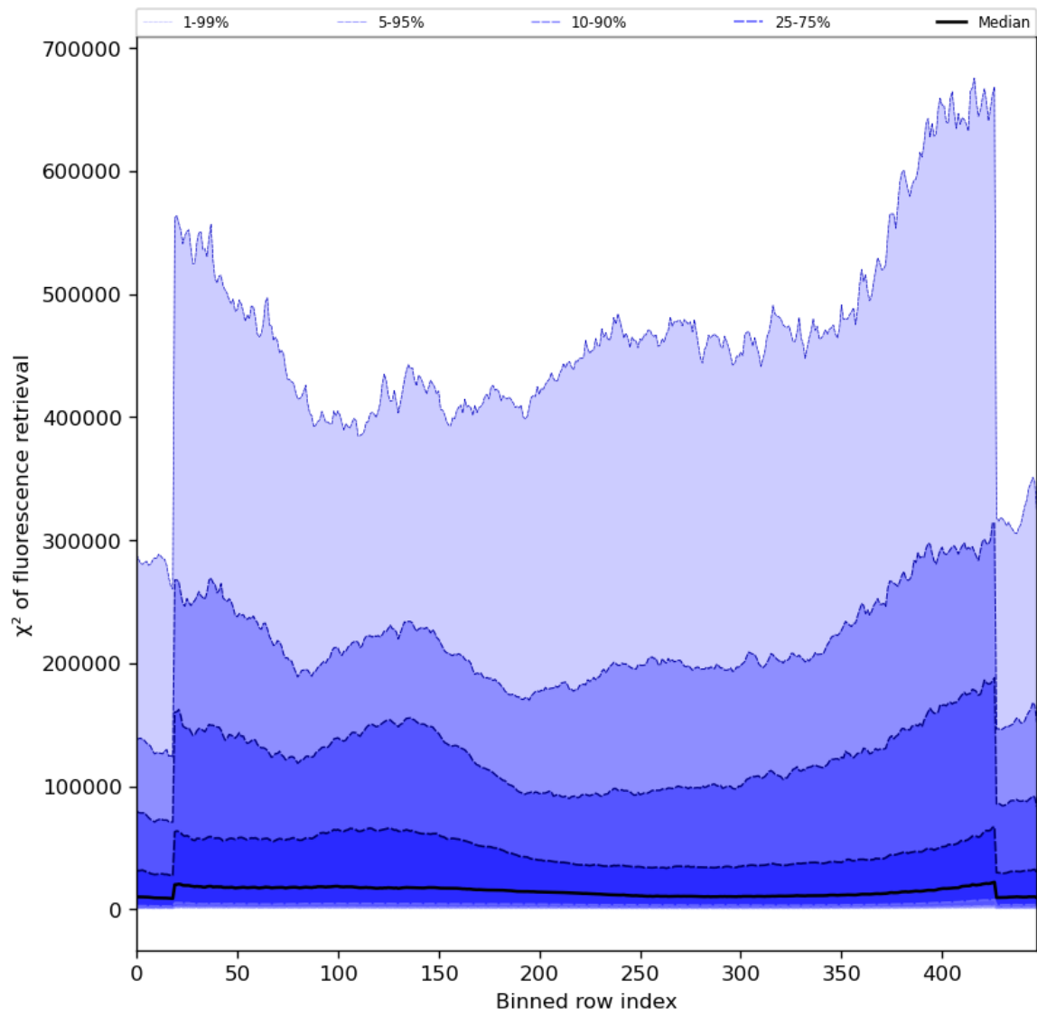
Figure 59: Along track statistics of “ \chi^2 of fluorescence retrieval” for 2023-12-05 to 2023-12-07
