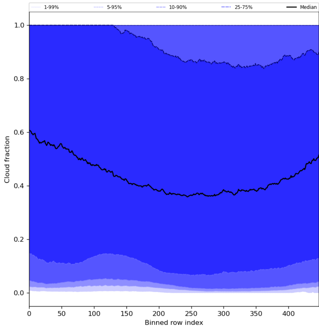
Figure 49: Along track statistics of “Cloud fraction” for 2023-12-05 to 2023-12-07
