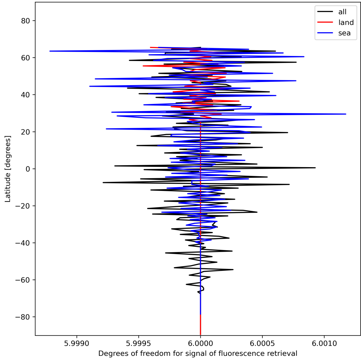
Figure 26: Zonal average of “Degrees of freedom for signal of fluorescence retrieval” for 2023-12-05 to 2023-12-07.
