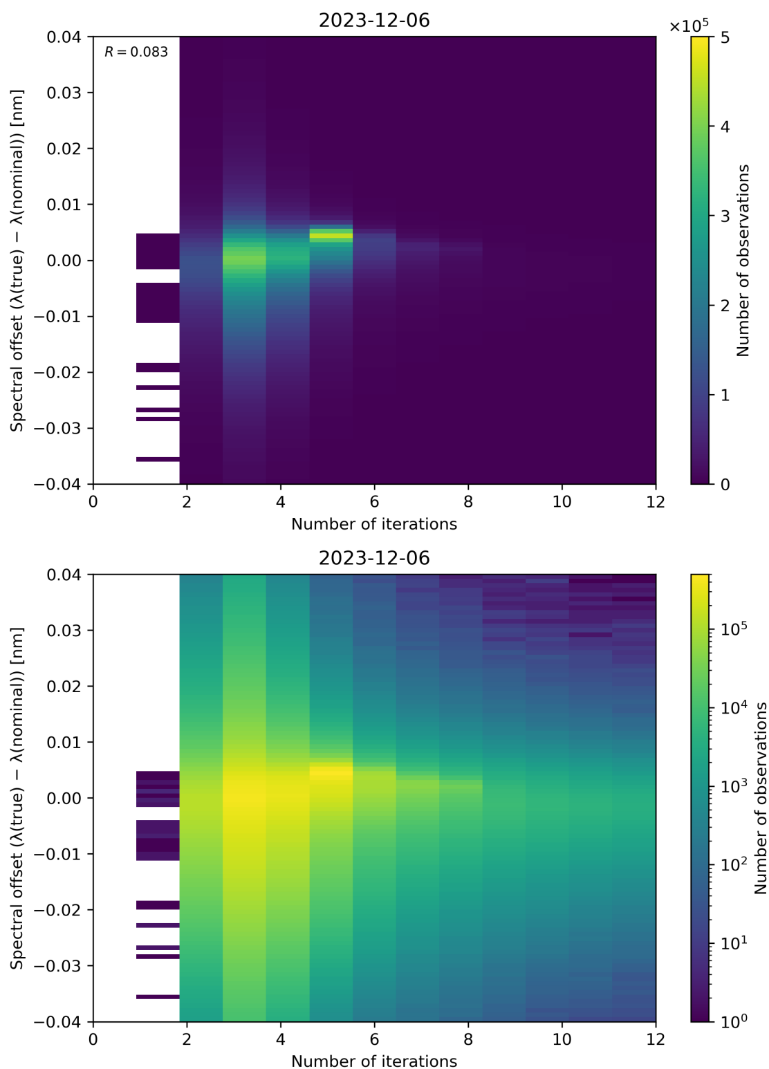
Figure 100: Scatter density plot of “Number of iterations” against “Spectral offset ( \lambda(\text{true}) - \lambda(\text{nominal}) )” for 2023-12-05 to 2023-12-07.
