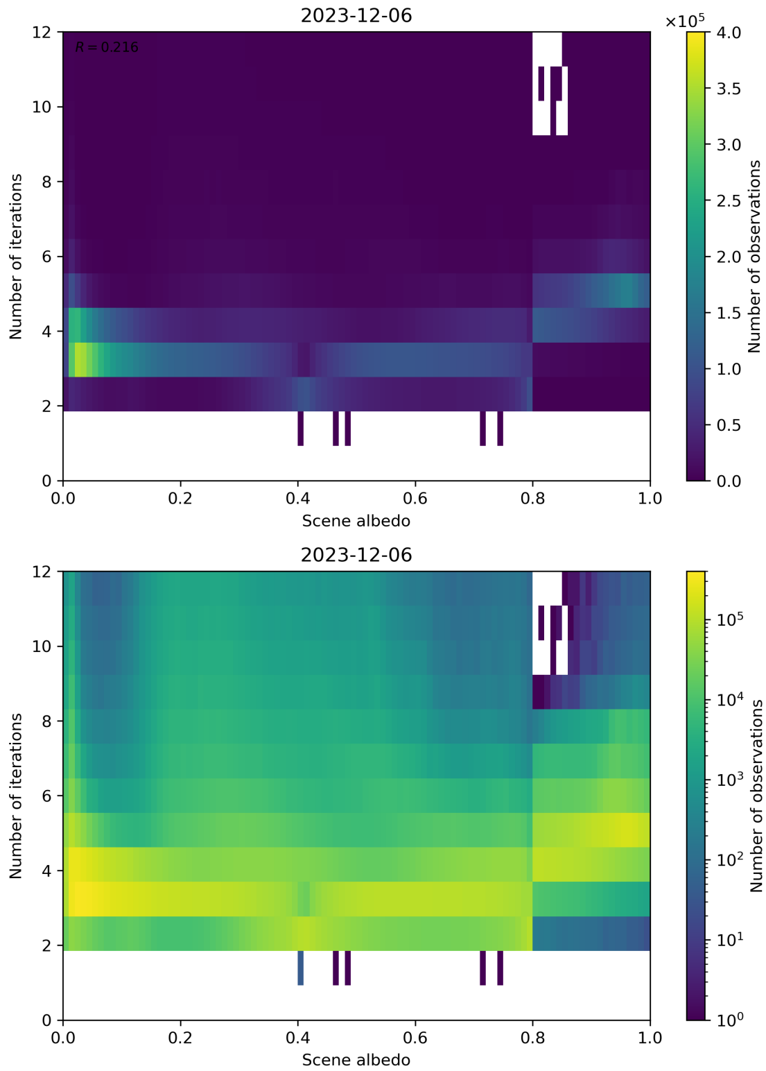
Figure 105: Scatter density plot of “Scene albedo” against “Number of iterations” for 2023-12-05 to 2023-12-07.
