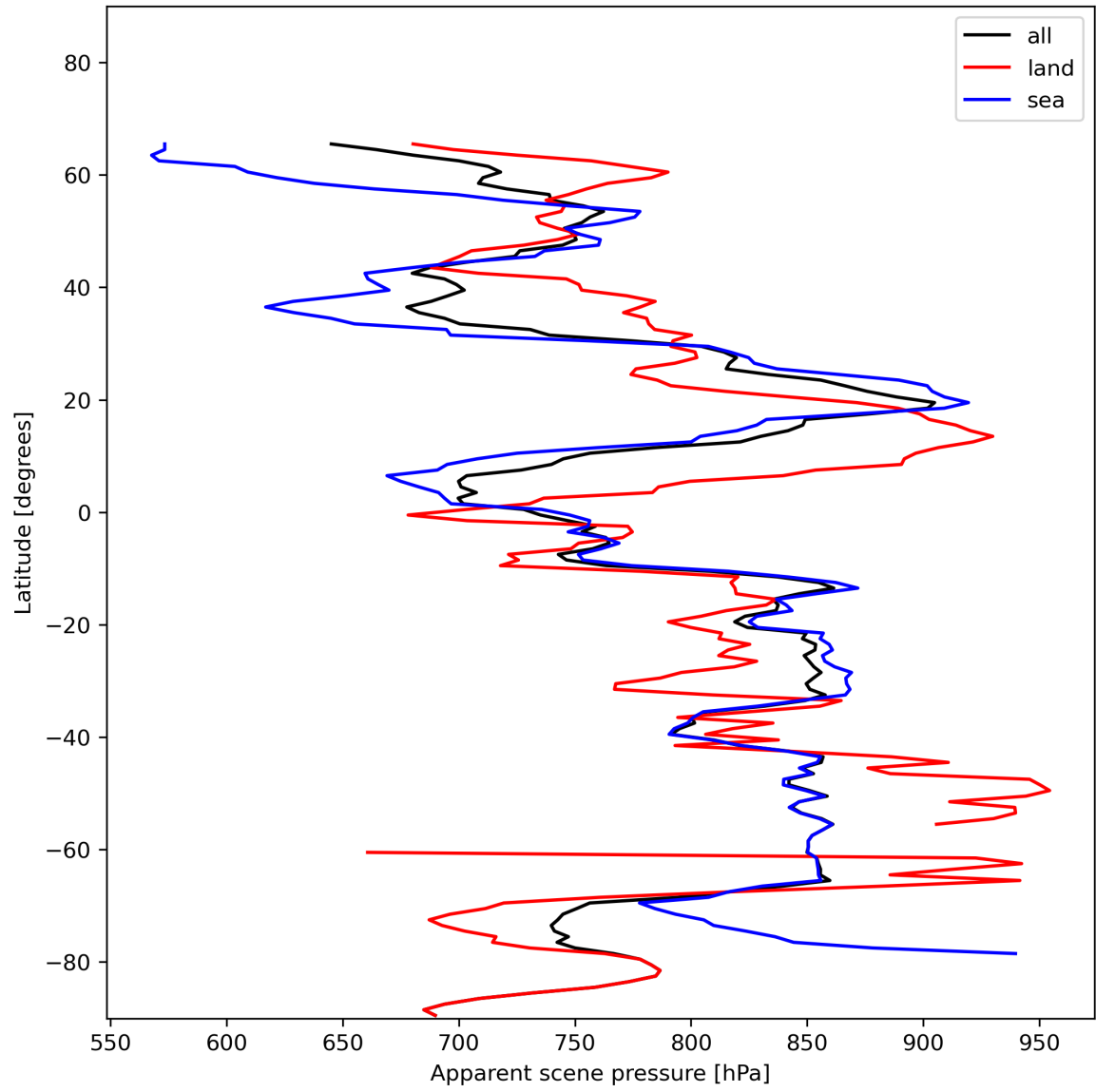
Figure 19: Zonal average of “Apparent scene pressure” for 2023-12-05 to 2023-12-07.
