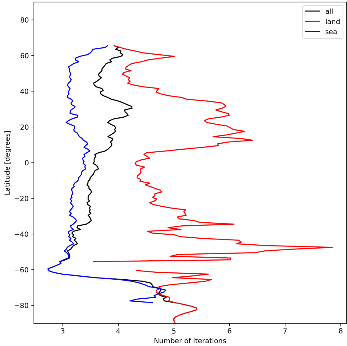
Figure 22: Zonal average of “Number of iterations” for 2023-12-05 to 2023-12-07.
