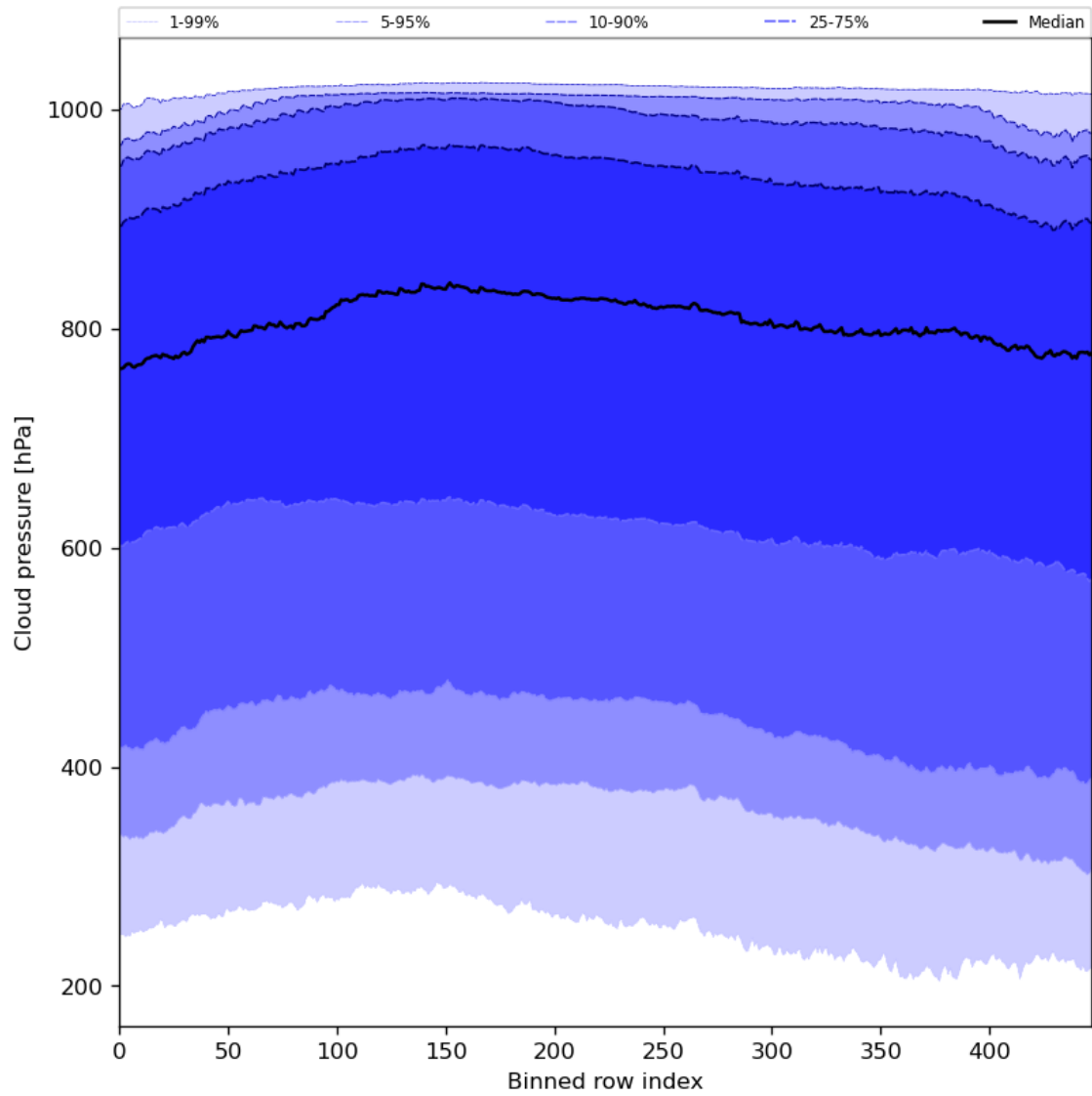
Figure 47: Along track statistics of “Cloud pressure” for 2023-12-05 to 2023-12-07
