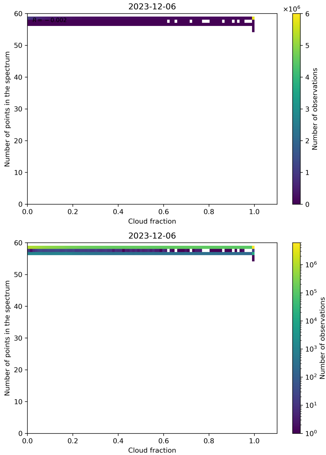
Figure 74: Scatter density plot of “Cloud fraction” against “Number of points in the spectrum” for 2023-12-05 to 2023-12-07.
