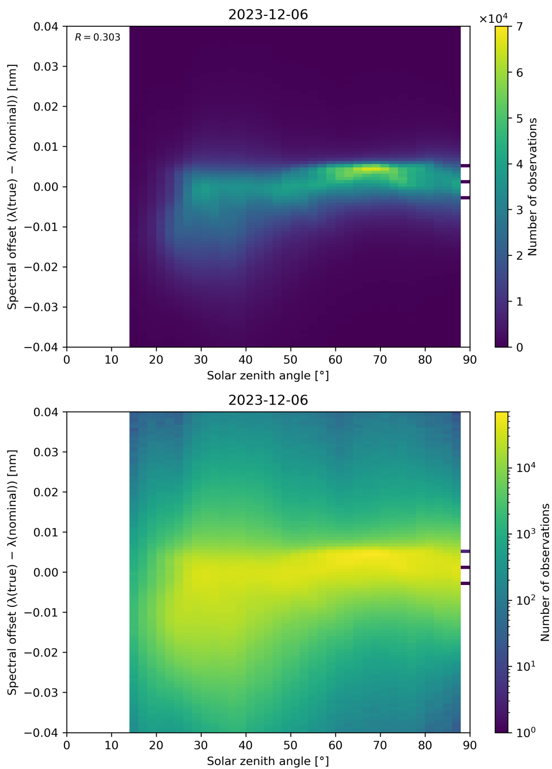
Figure 117: Scatter density plot of “Solar zenith angle” against “Spectral offset ( \lambda(\text{true}) - \lambda(\text{nominal}) )” for 2023-12-05 to 2023-12-07.
