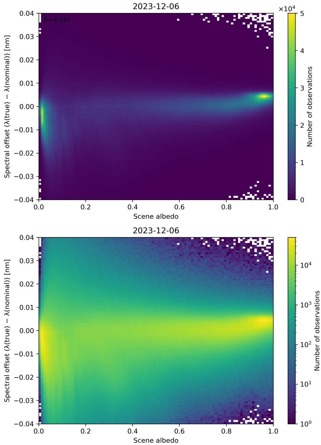
Figure 107: Scatter density plot of “Scene albedo” against “Spectral offset ( \lambda(\text{true}) - \lambda(\text{nominal}) )” for 2023-12-05 to 2023-12-07.
