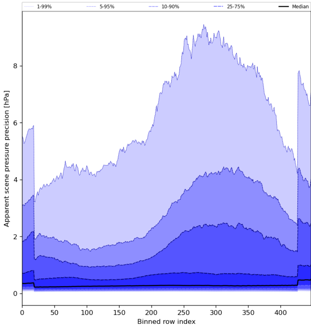
Figure 54: Along track statistics of “Apparent scene pressure precision” for 2023-12-05 to 2023-12-07
