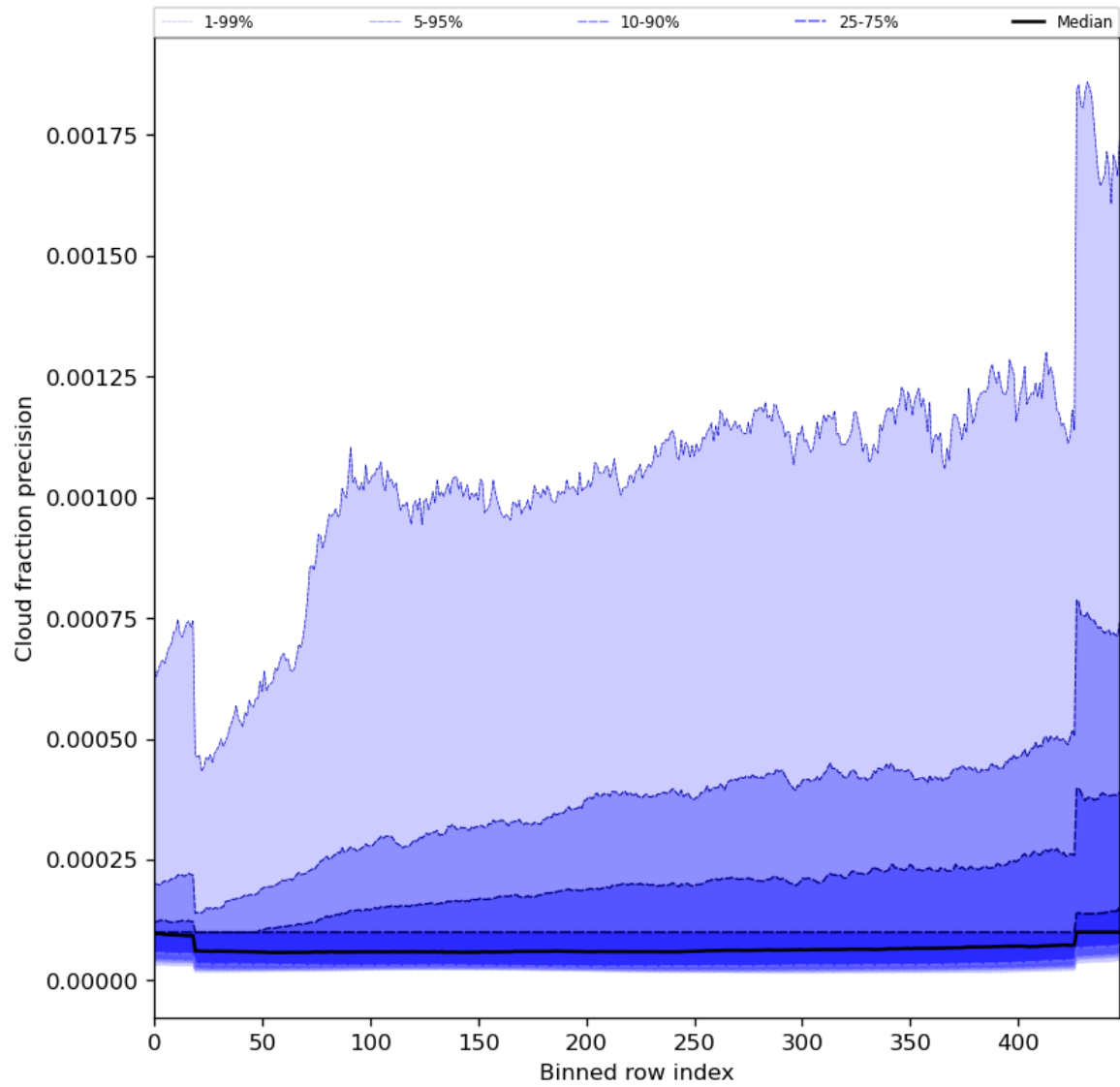
Figure 50: Along track statistics of “Cloud fraction precision” for 2023-12-05 to 2023-12-07
