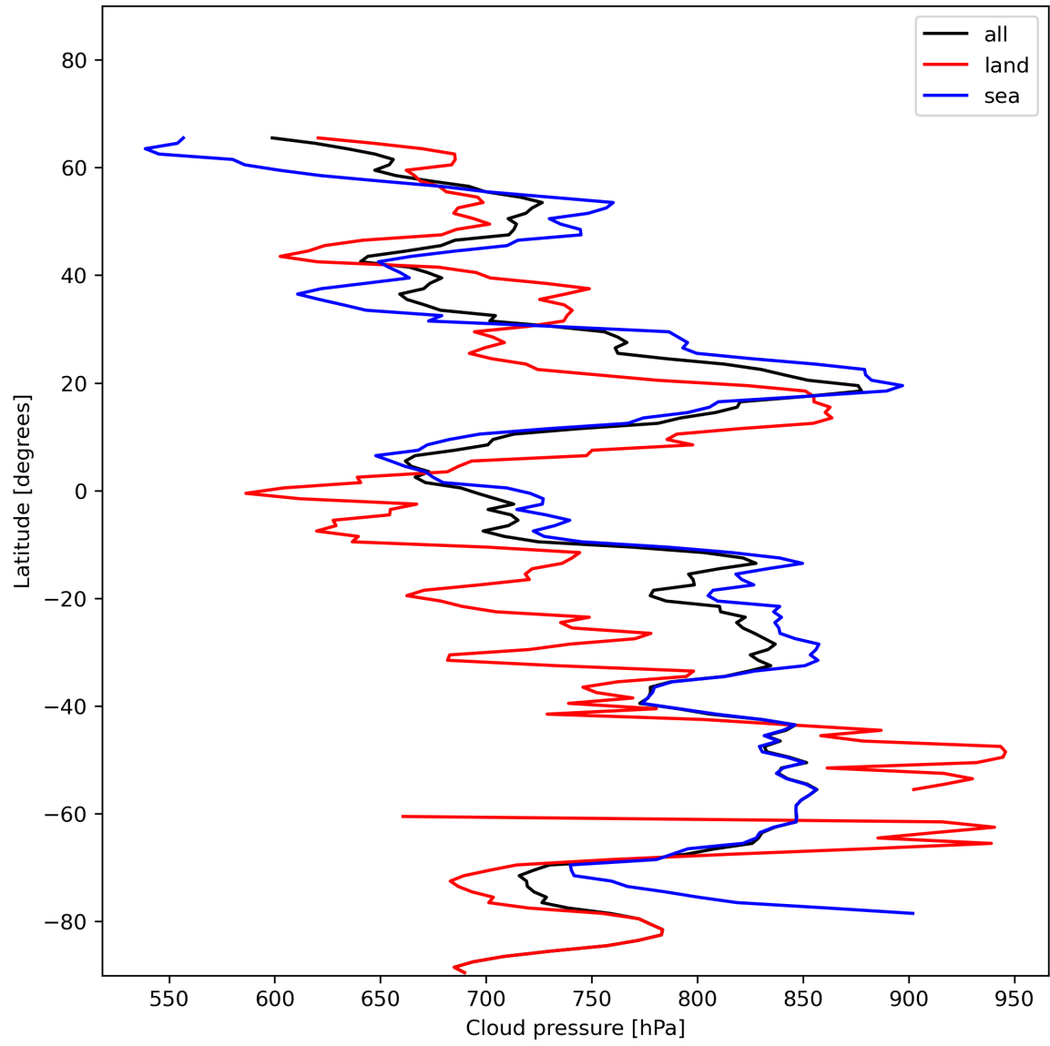
Figure 13: Zonal average of “Cloud pressure” for 2023-12-05 to 2023-12-07.
