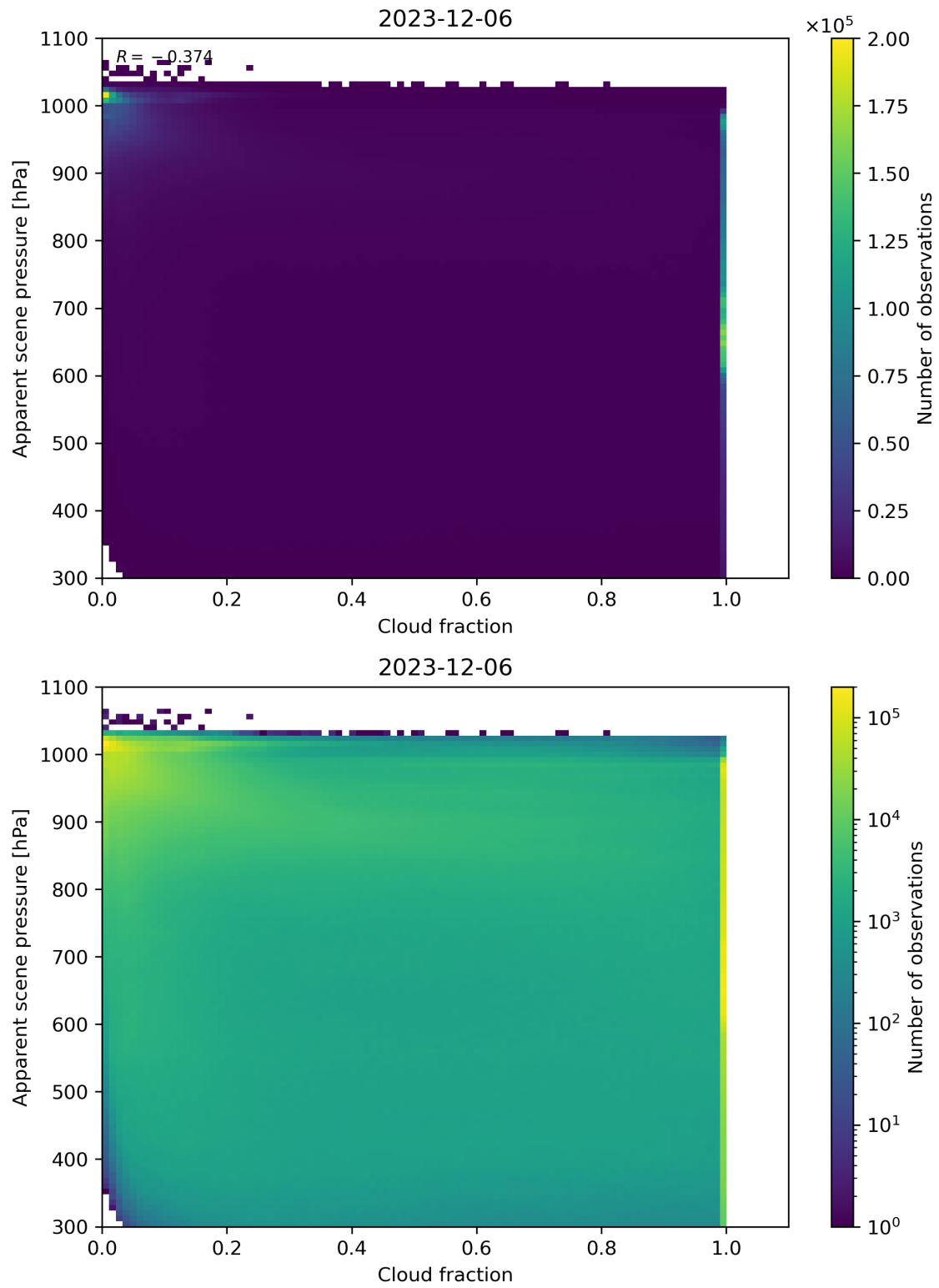
Figure 70: Scatter density plot of “Cloud fraction” against “Apparent scene pressure” for 2023-12-05 to 2023-12-07.
