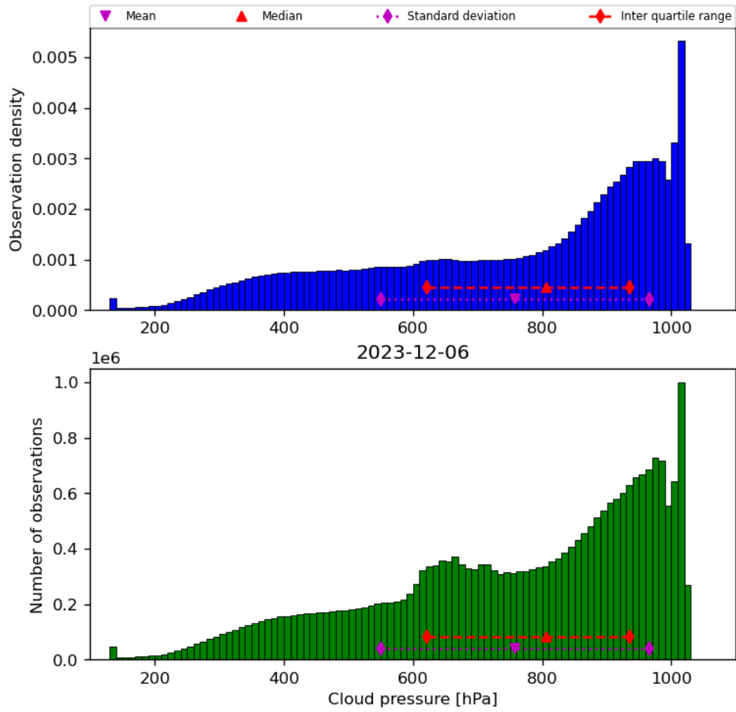
Figure 30: Histogram of “Cloud pressure” for 2023-12-05 to 2023-12-07
