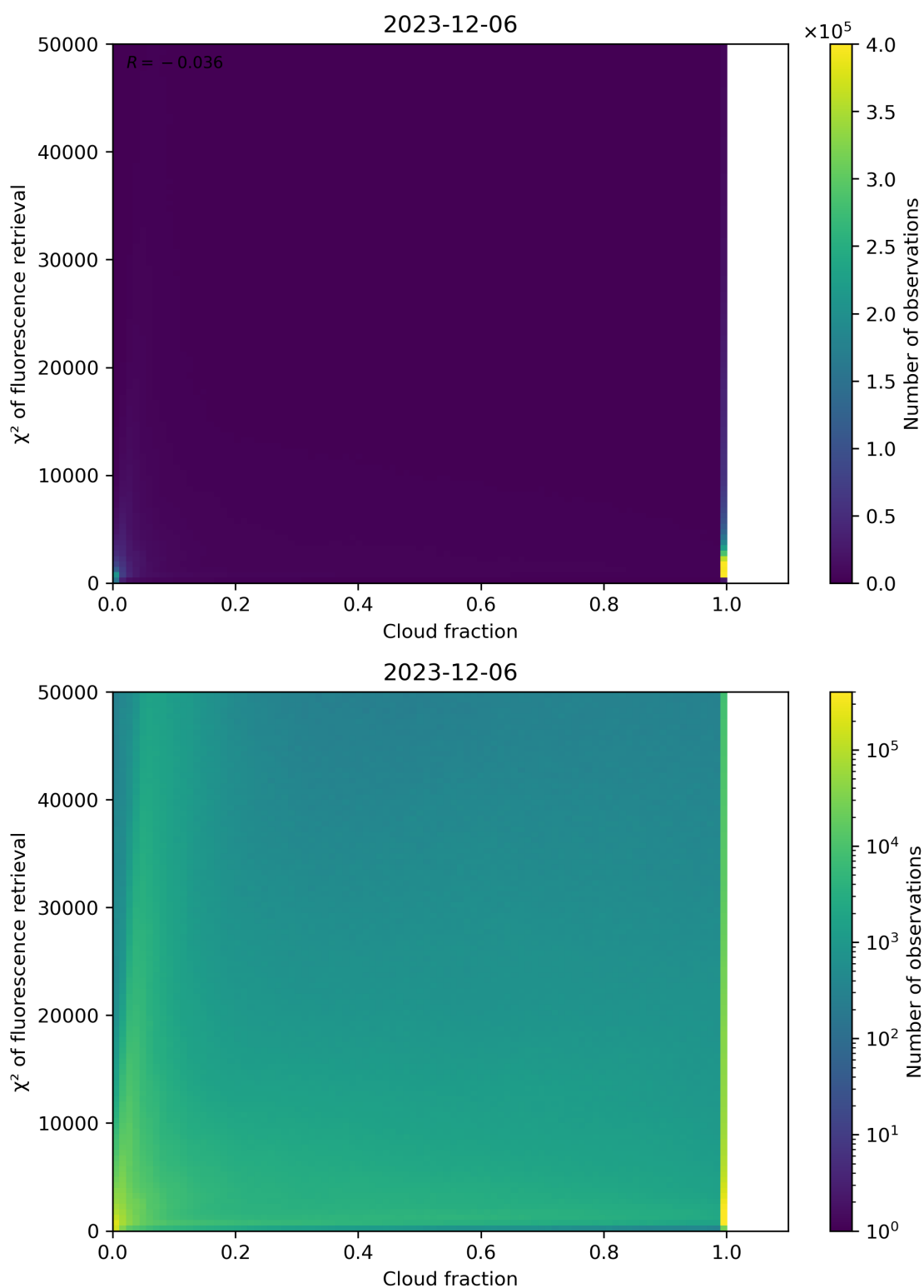
Figure 71: Scatter density plot of “Cloud fraction” against “ \chi^2 of fluorescence retrieval” for 2023-12-05 to 2023-12-07.
