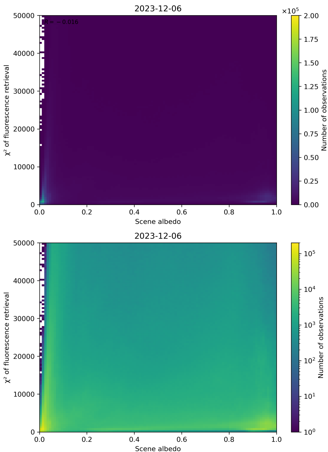
Figure 103: Scatter density plot of “Scene albedo” against “ \chi^2 of fluorescence retrieval” for 2023-12-05 to 2023-12-07.
