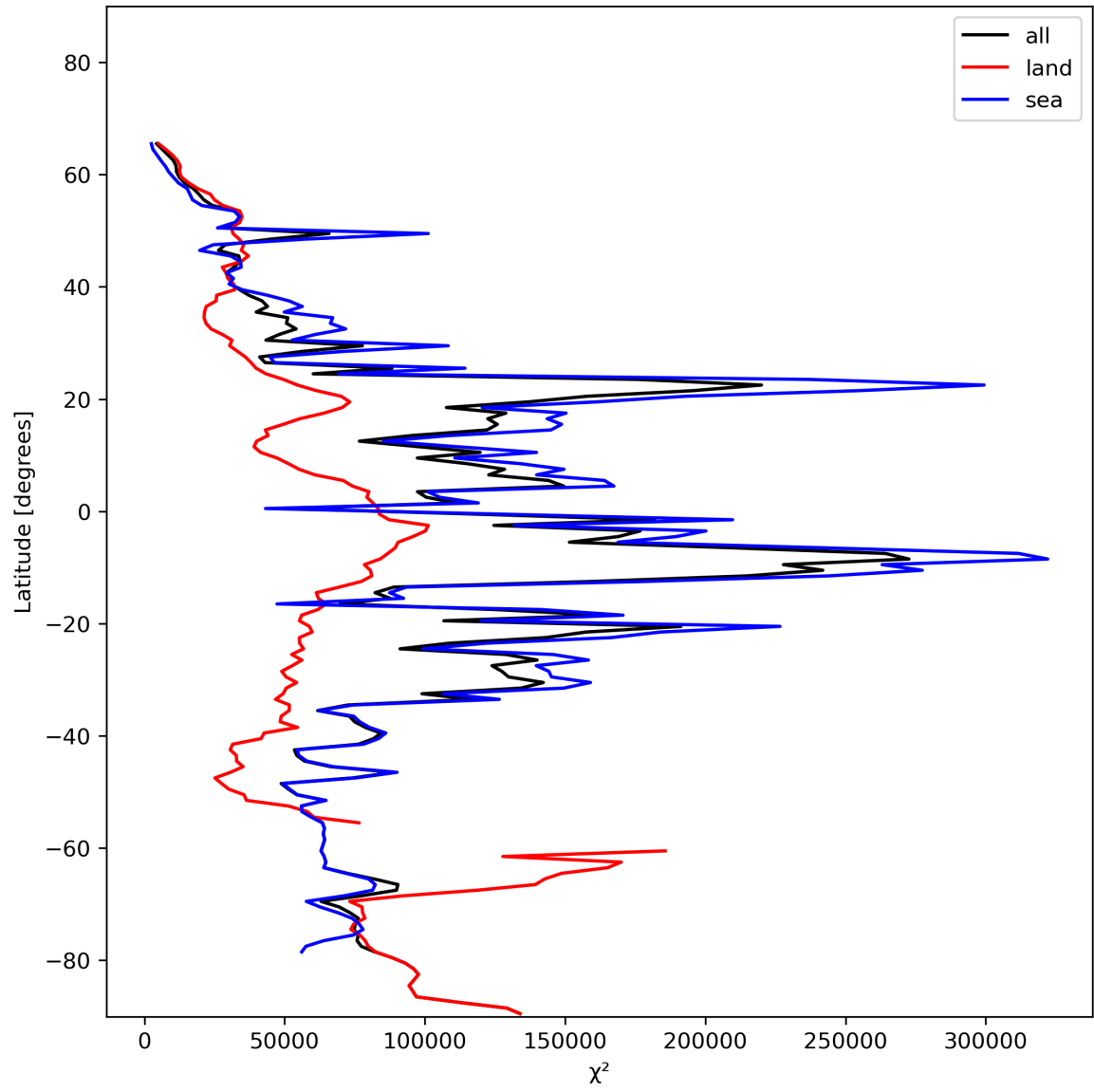
Figure 21: Zonal average of “ \chi^2 ” for 2023-12-05 to 2023-12-07.
