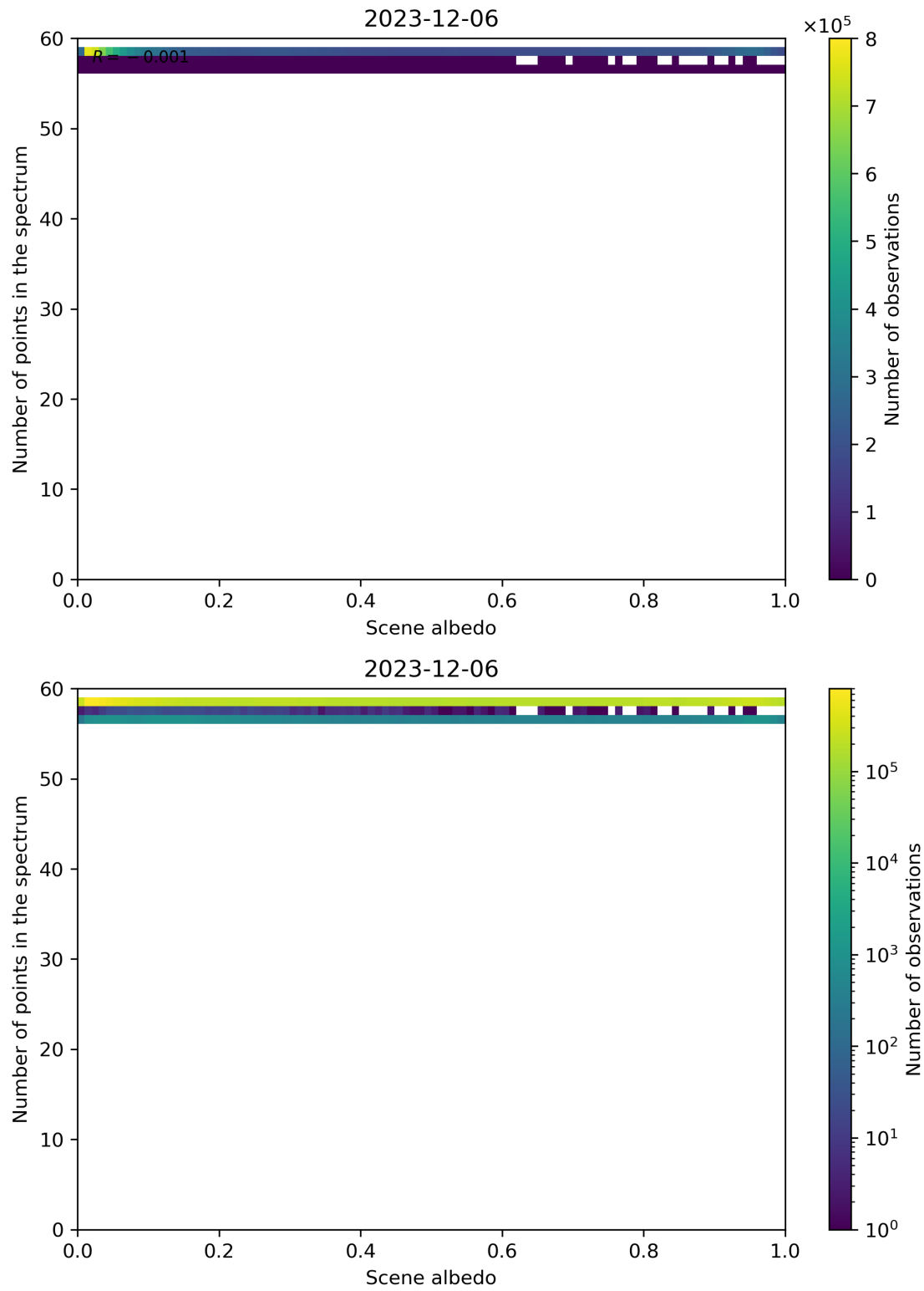
Figure 106: Scatter density plot of “Scene albedo” against “Number of points in the spectrum” for 2023-12-05 to 2023-12-07.
