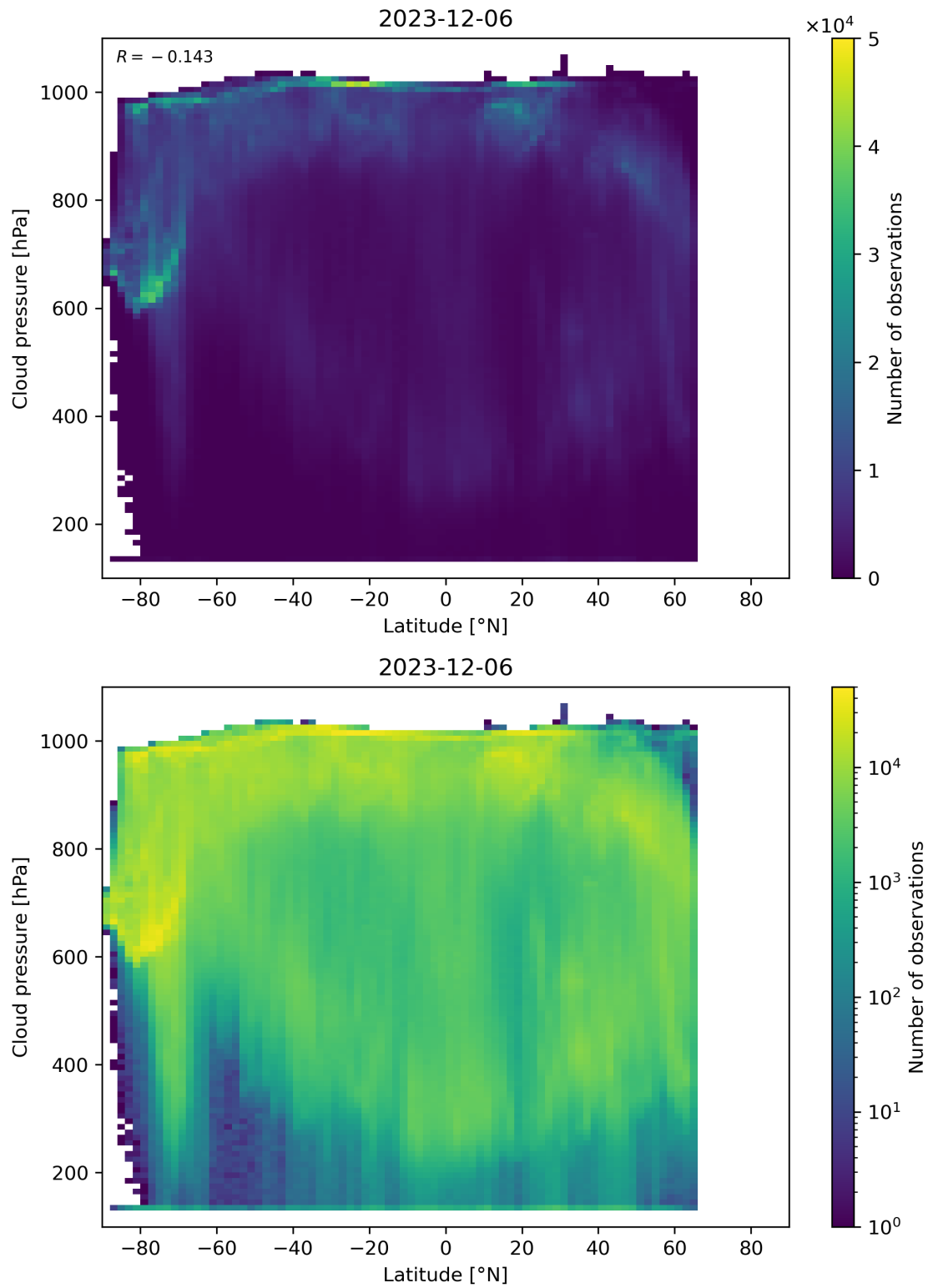
Figure 91: Scatter density plot of “Latitude” against “Cloud pressure” for 2023-12-05 to 2023-12-07.
