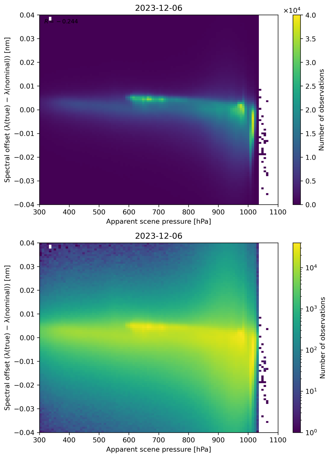
Figure 67: Scatter density plot of “Apparent scene pressure” against “Spectral offset ( \lambda(\text{true}) - \lambda(\text{nominal}) )” for 2023-12-05 to 2023-12-07.
