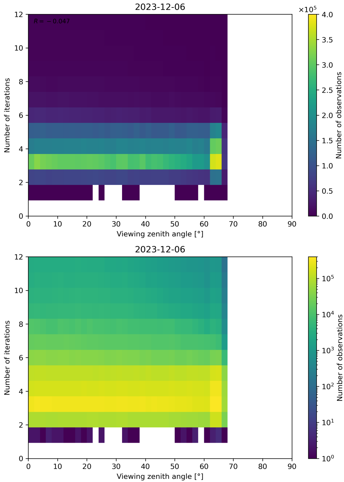
Figure 124: Scatter density plot of “Viewing zenith angle” against “Number of iterations” for 2023-12-05 to 2023-12-07.
