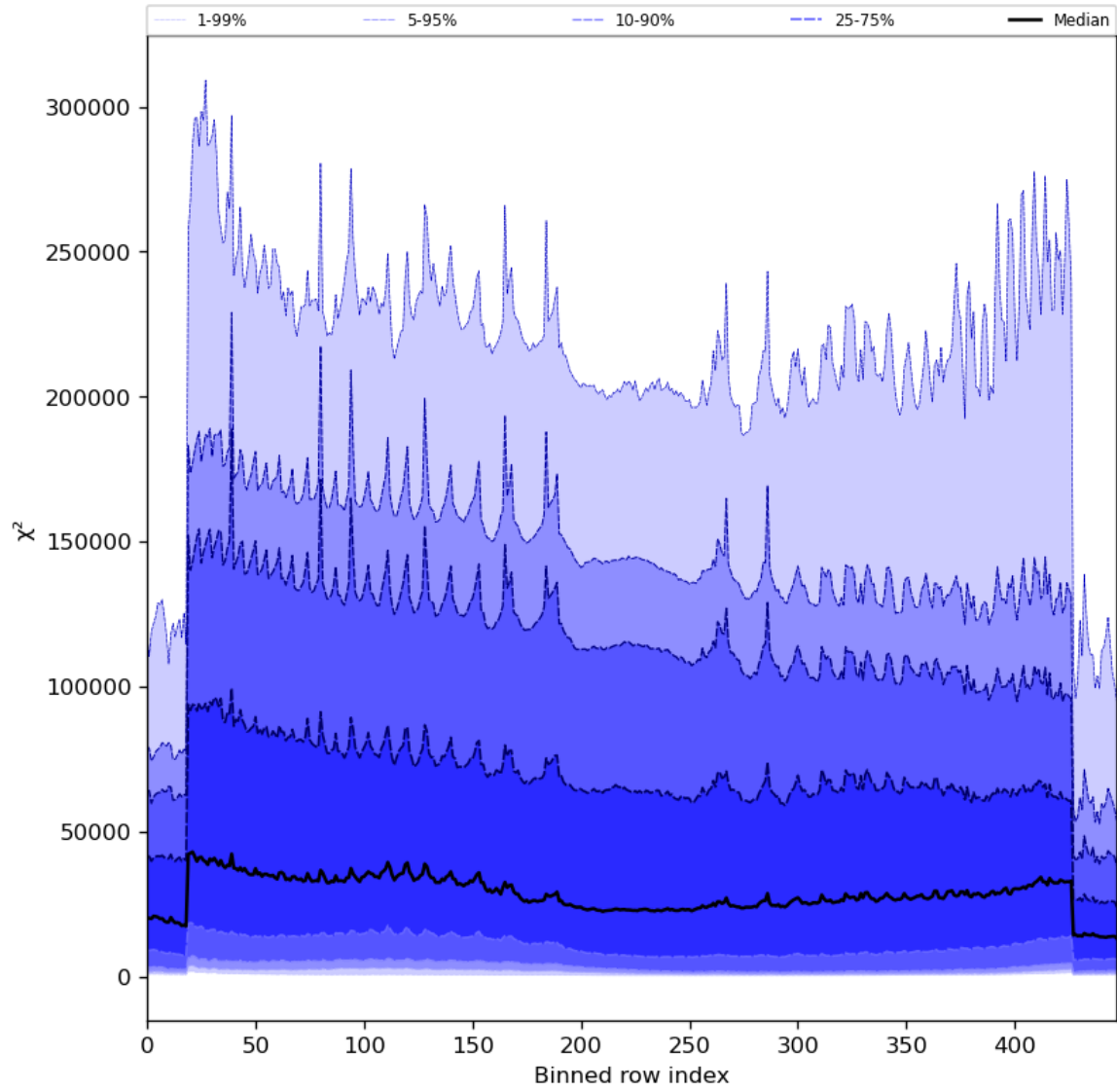
Figure 55: Along track statistics of “ \chi^2 ” for 2023-12-05 to 2023-12-07
