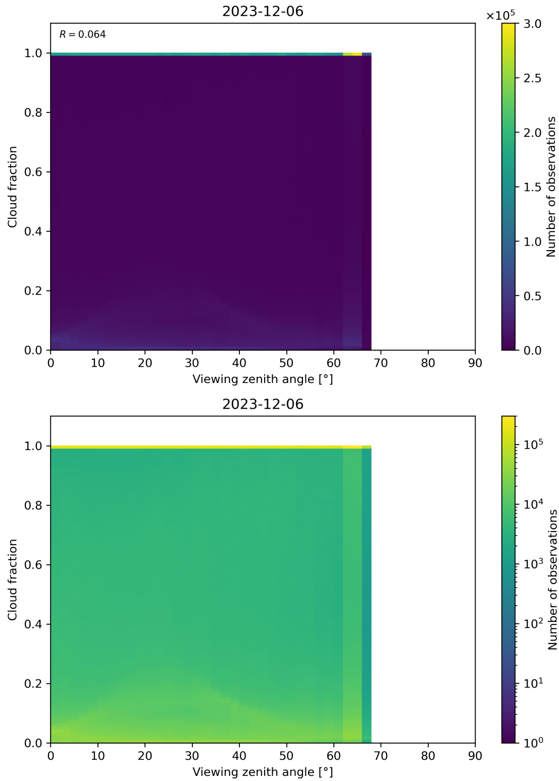
Figure 120: Scatter density plot of “Viewing zenith angle” against “Cloud fraction” for 2023-12-05 to 2023-12-07.
