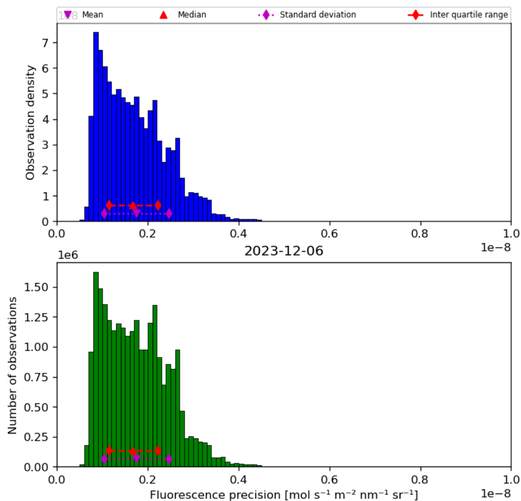
Figure 41: Histogram of “Fluorescence precision” for 2023-12-05 to 2023-12-07
