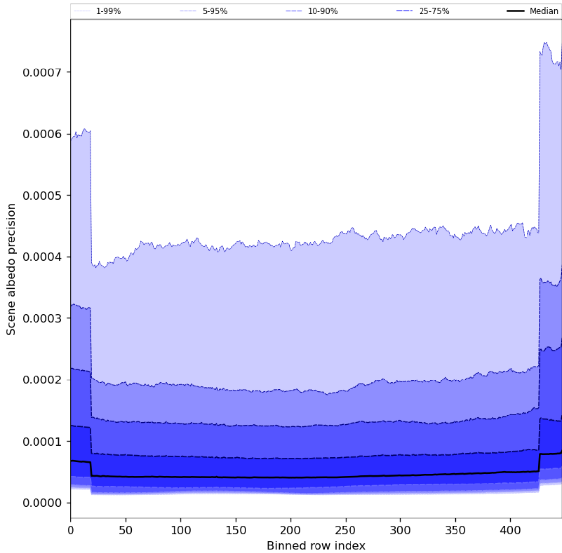
Figure 52: Along track statistics of “Scene albedo precision” for 2023-12-05 to 2023-12-07
