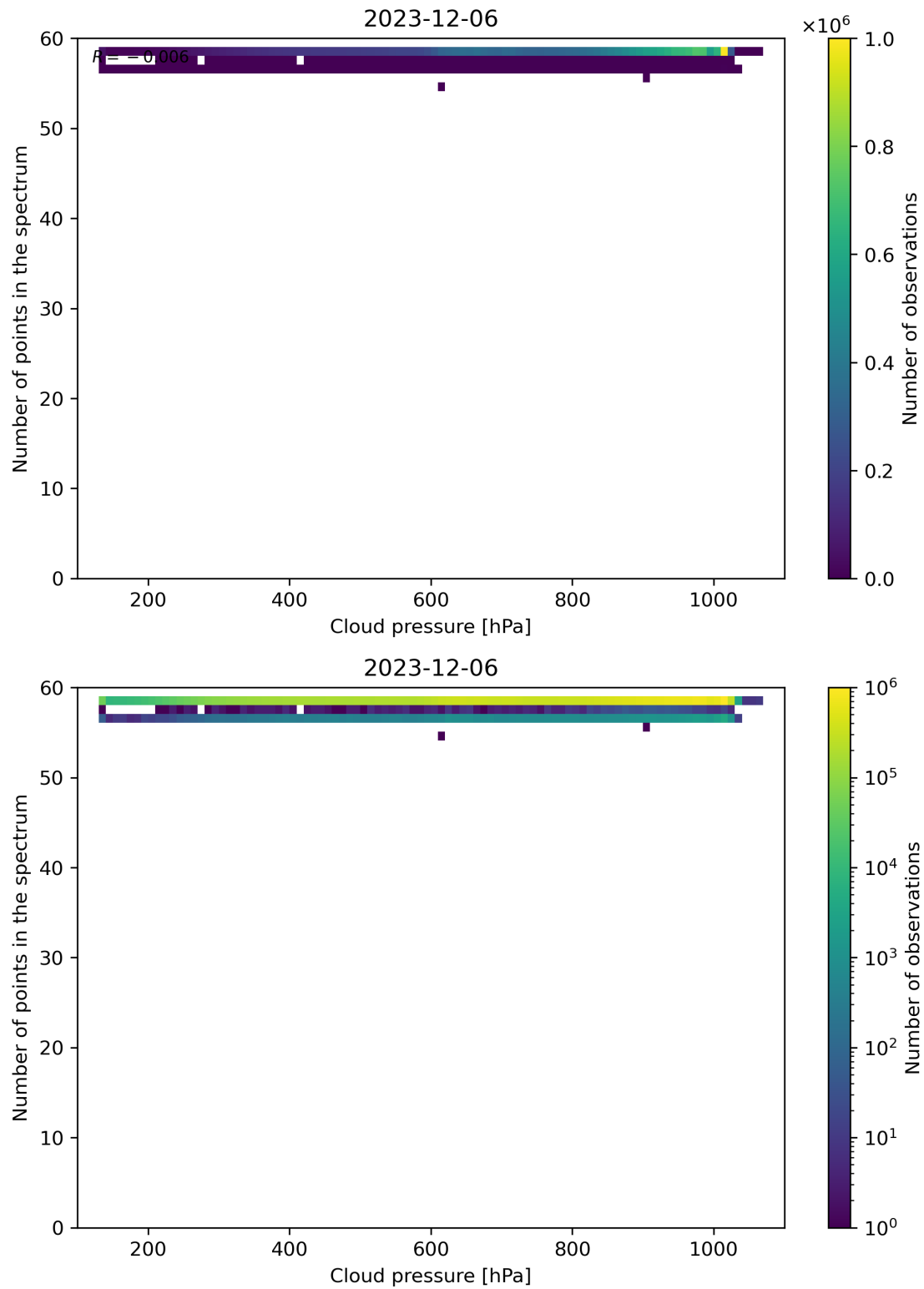
Figure 82: Scatter density plot of “Cloud pressure” against “Number of points in the spectrum” for 2023-12-05 to 2023-12-07.
