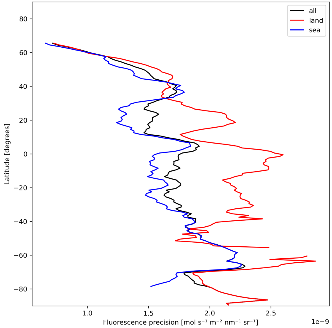
Figure 24: Zonal average of “Fluorescence precision” for 2023-12-05 to 2023-12-07.
