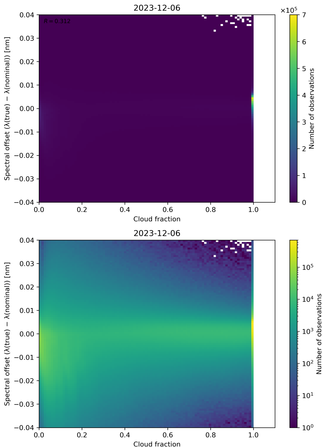
Figure 76: Scatter density plot of “Cloud fraction” against “Spectral offset ( \lambda(\text{true}) - \lambda(\text{nominal}) )” for 2023-12-05 to 2023-12-07.
