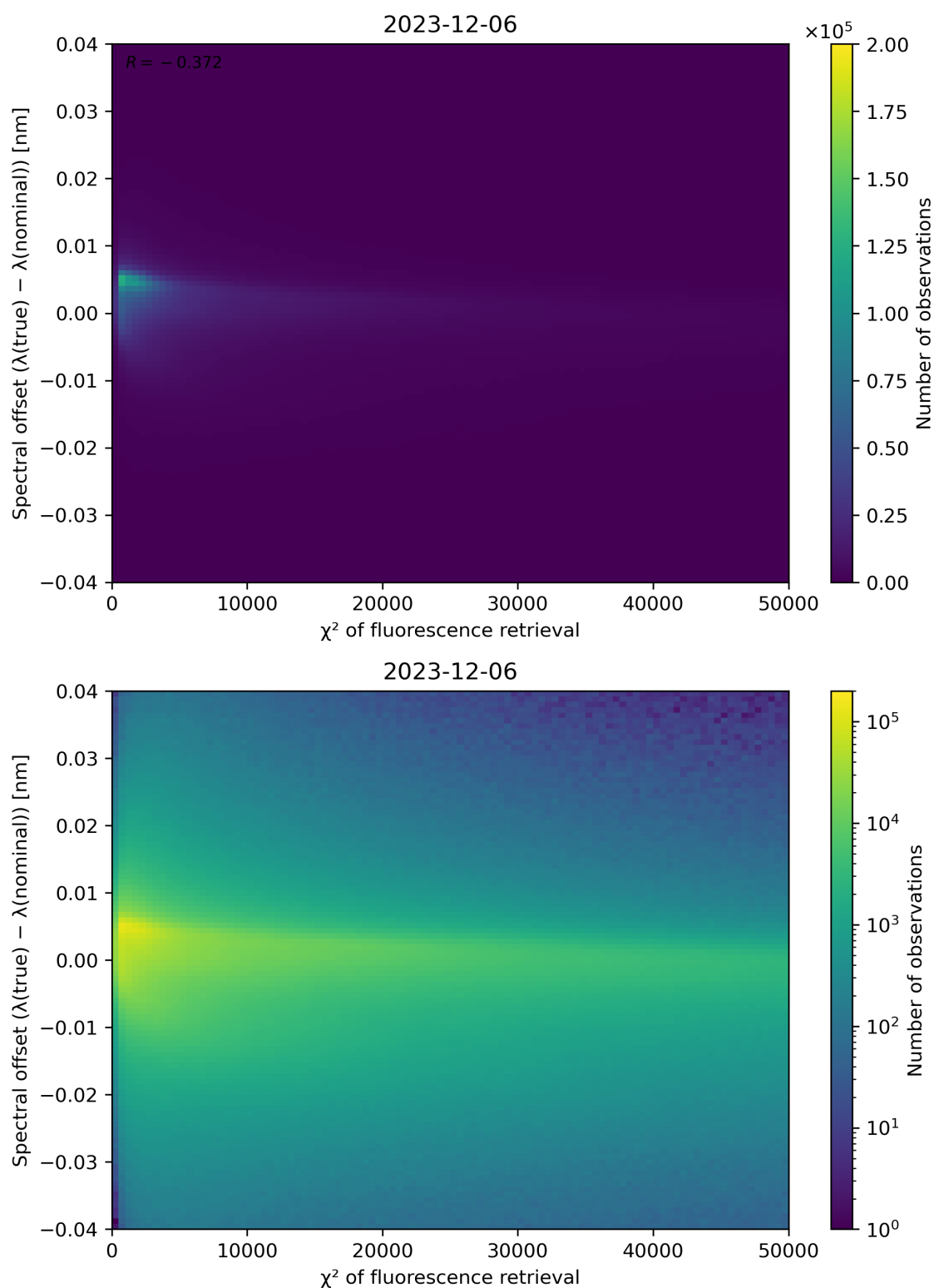
Figure 69: Scatter density plot of " \chi^2 of fluorescence retrieval" against "Spectral offset ( \lambda(\text{true}) - \lambda(\text{nominal})) " for 2023-12-05 to 2023-12-07.
