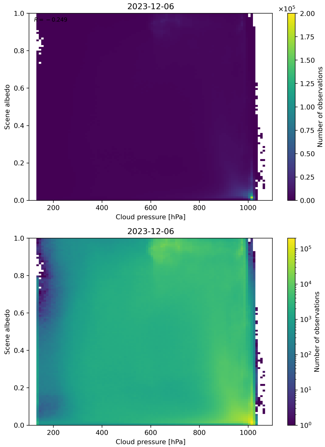
Figure 83: Scatter density plot of “Cloud pressure” against “Scene albedo” for 2023-12-05 to 2023-12-07.
