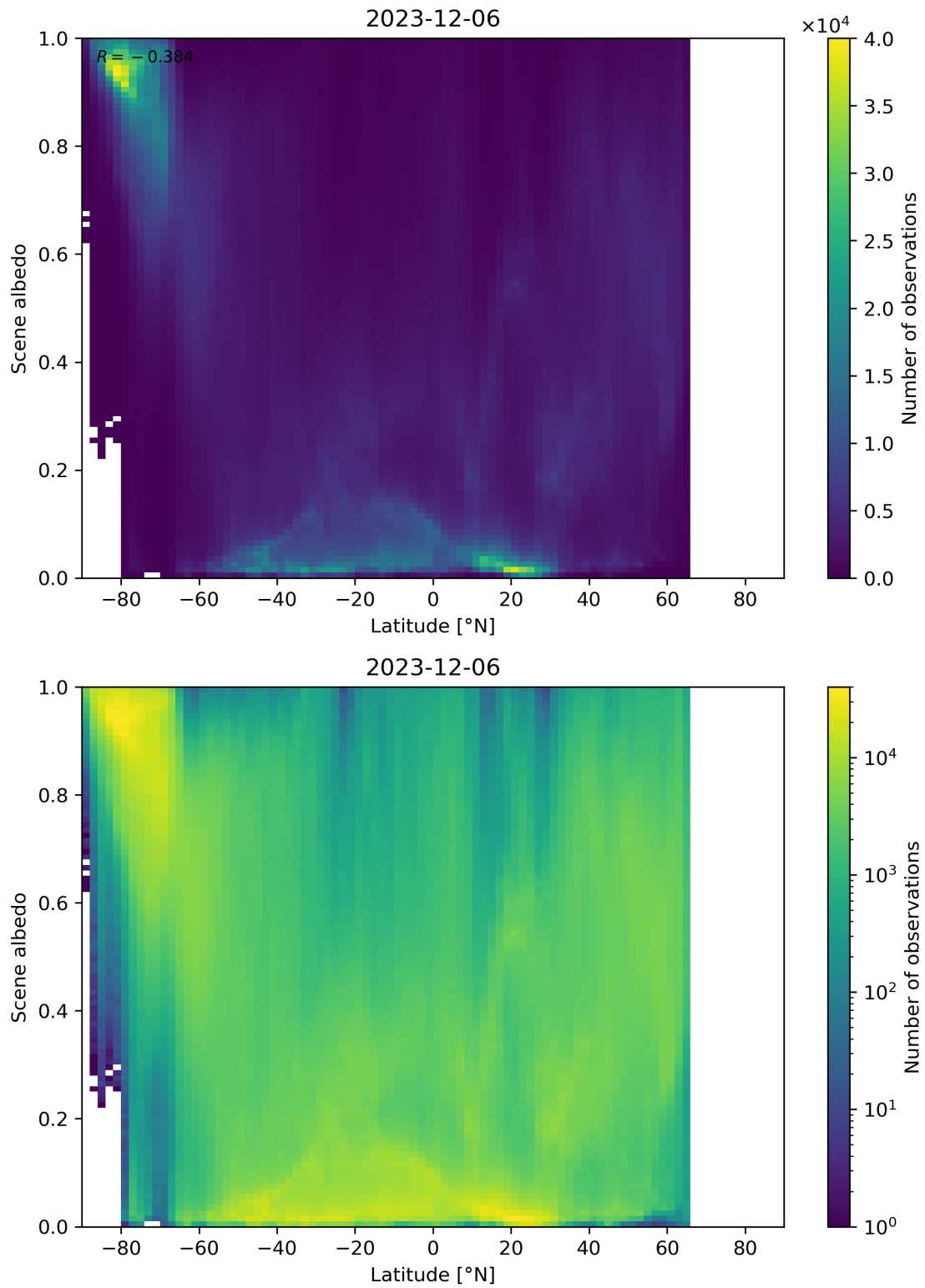
Figure 95: Scatter density plot of “Latitude” against “Scene albedo” for 2023-12-05 to 2023-12-07.
