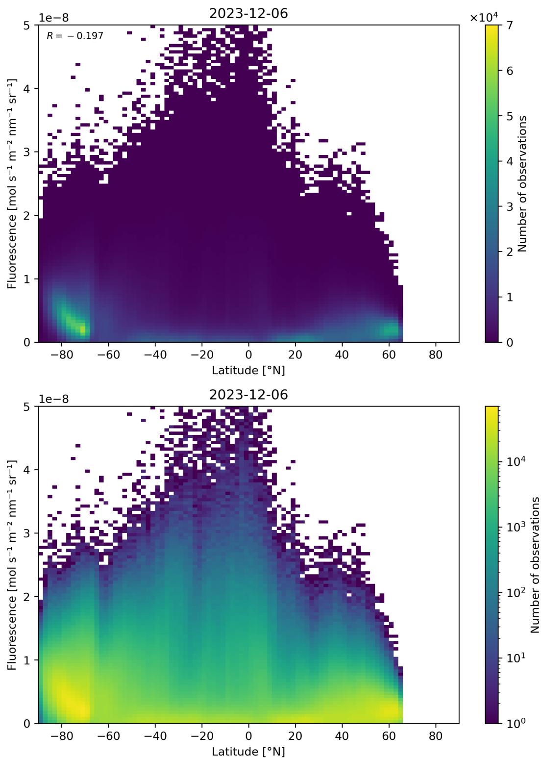
Figure 92: Scatter density plot of “Latitude” against “Fluorescence” for 2023-12-05 to 2023-12-07.
