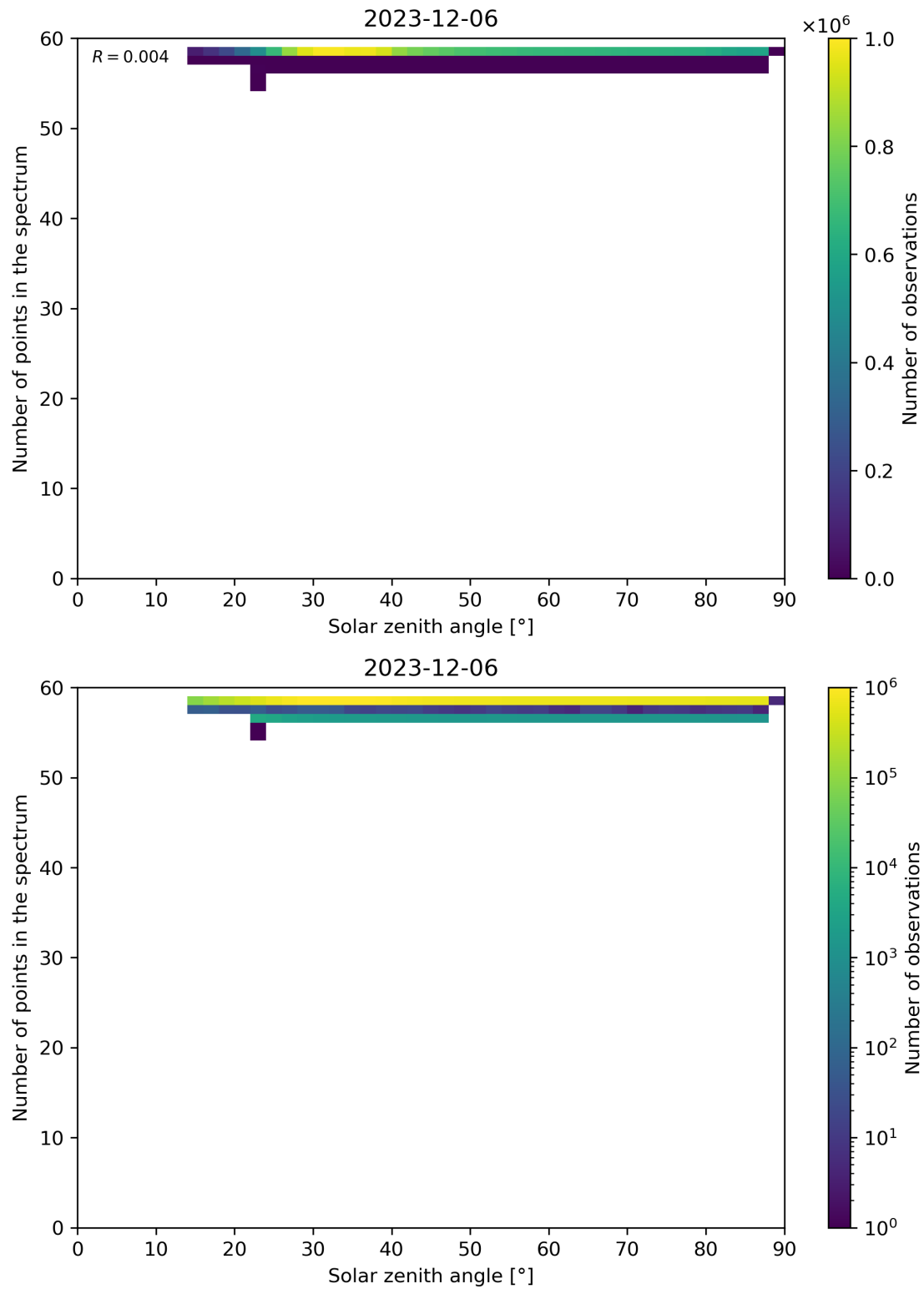
Figure 115: Scatter density plot of “Solar zenith angle” against “Number of points in the spectrum” for 2023-12-05 to 2023-12-07.
