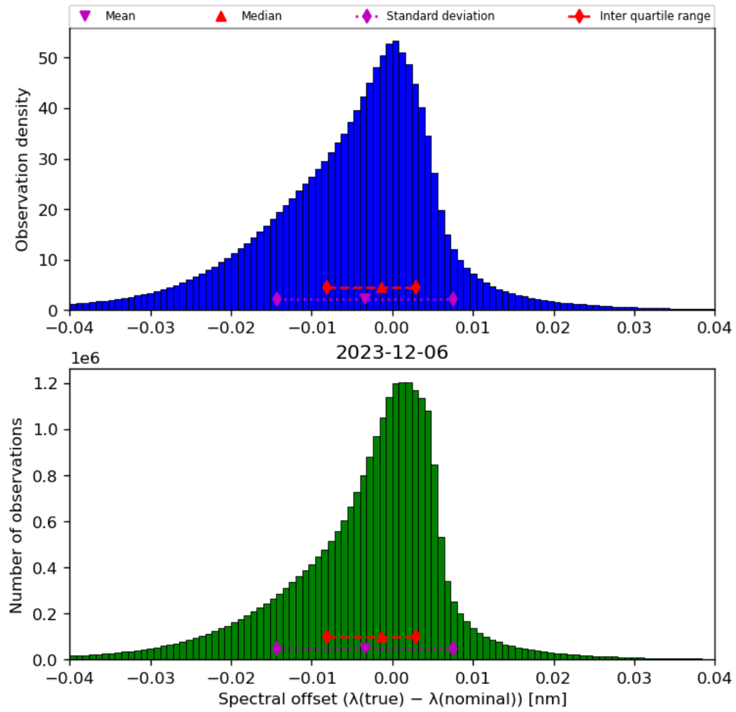
Figure 45: Histogram of “Spectral offset ( \lambda(\text{true}) - \lambda(\text{nominal}) )” for 2023-12-05 to 2023-12-07
