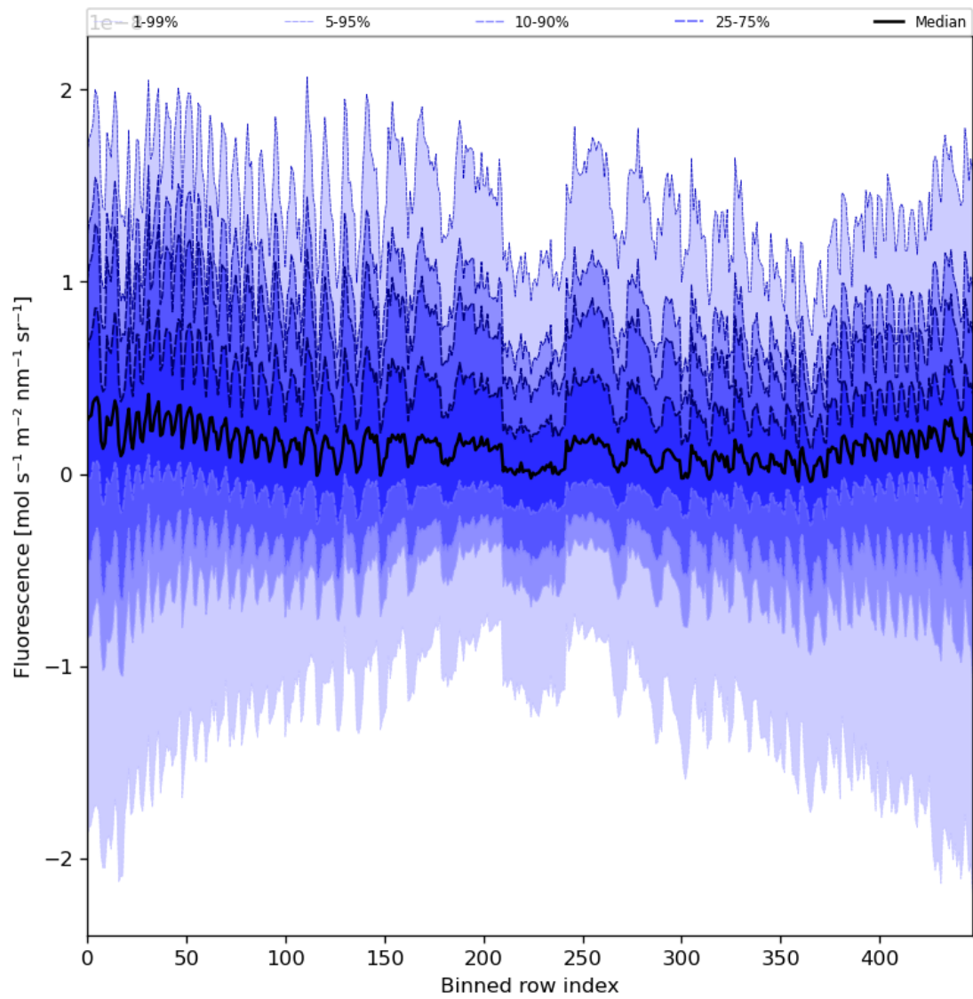
Figure 57: Along track statistics of “Fluorescence” for 2023-12-05 to 2023-12-07
