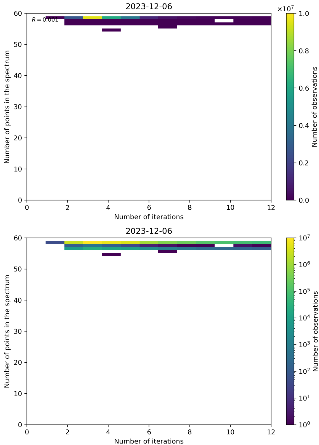
Figure 99: Scatter density plot of “Number of iterations” against “Number of points in the spectrum” for 2023-12-05 to 2023-12-07.
