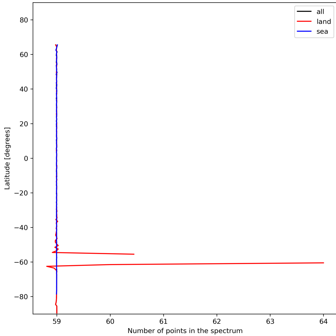
Figure 27: Zonal average of “Number of points in the spectrum” for 2023-12-05 to 2023-12-07.
