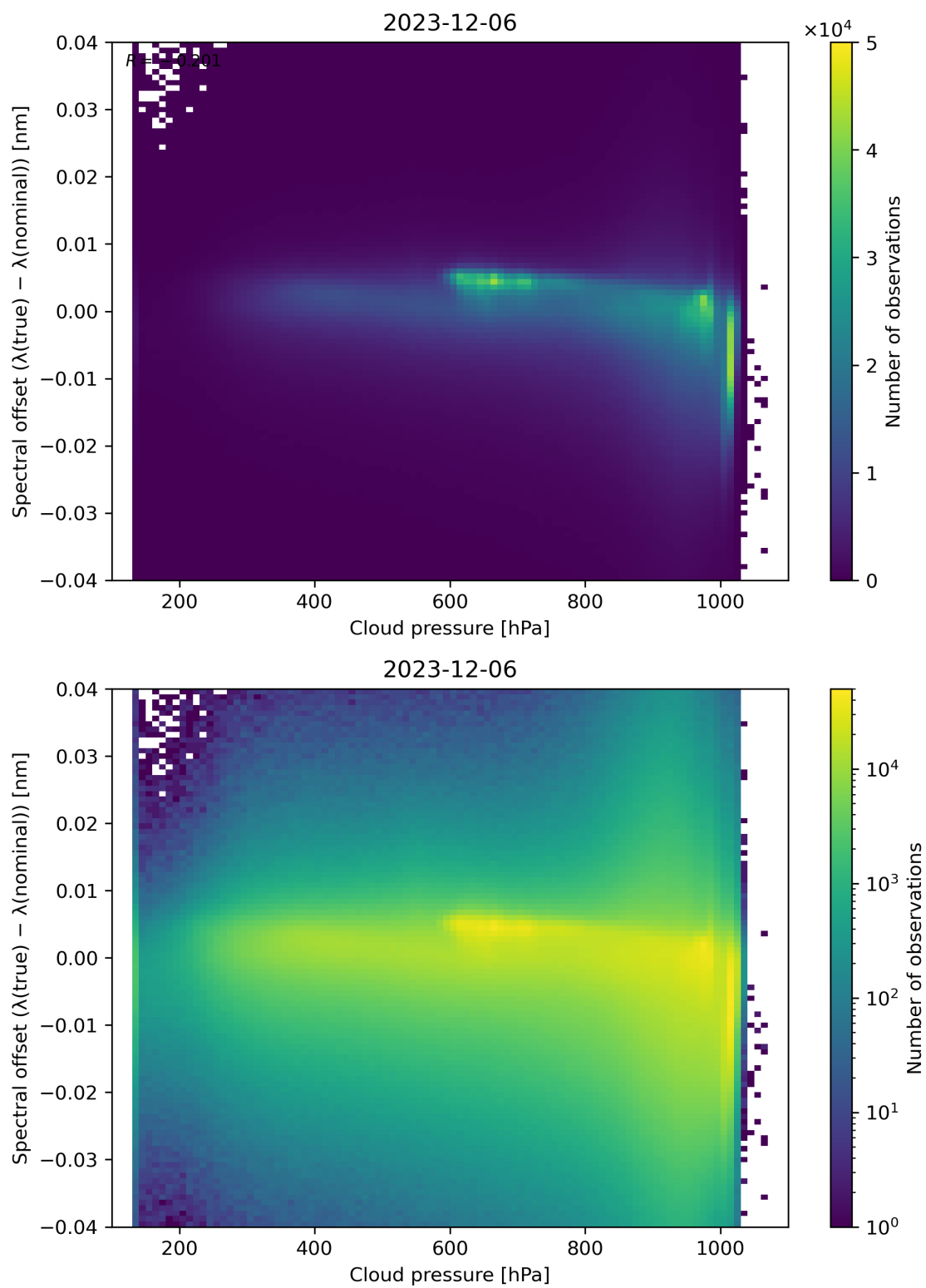
Figure 84: Scatter density plot of “Cloud pressure” against “Spectral offset ( \lambda(\text{true}) - \lambda(\text{nominal}) )” for 2023-12-05 to 2023-12-07.
