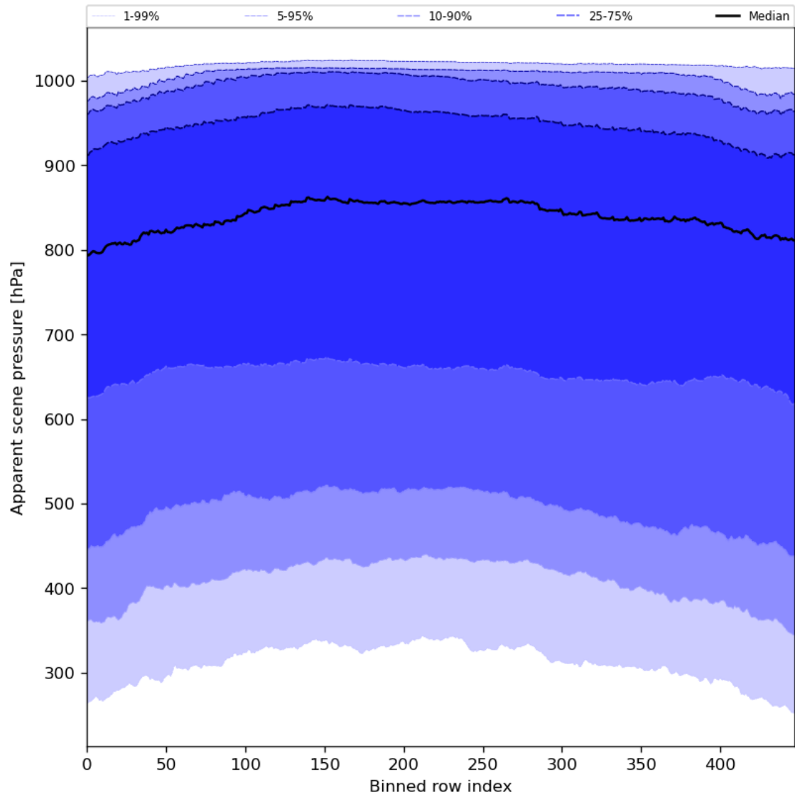
Figure 53: Along track statistics of “Apparent scene pressure” for 2023-12-05 to 2023-12-07
