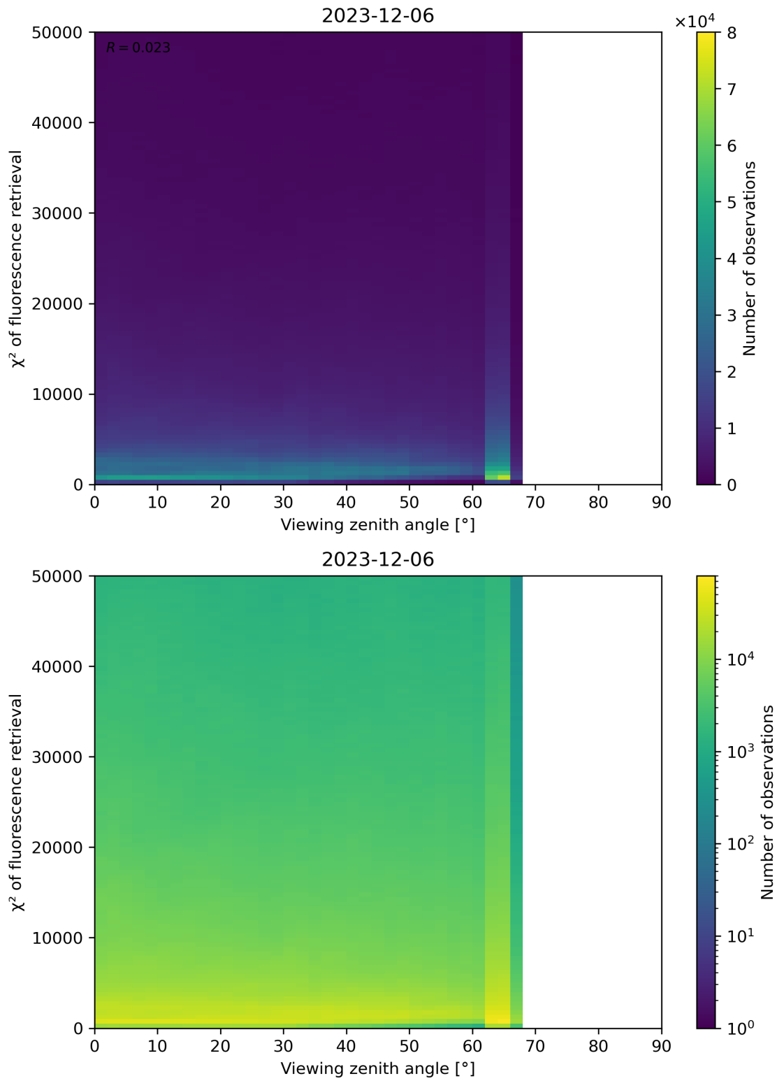
Figure 119: Scatter density plot of “Viewing zenith angle” against “ \chi^2 of fluorescence retrieval” for 2023-12-05 to 2023-12-07.
