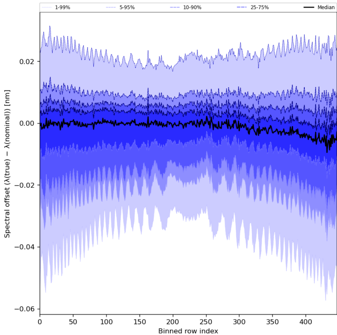
Figure 62: Along track statistics of “Spectral offset ( \lambda(\text{true}) - \lambda(\text{nominal}) )” for 2023-12-05 to 2023-12-07
