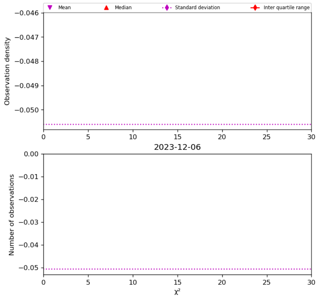
Figure 38: Histogram of “ \chi^2 ” for 2023-12-05 to 2023-12-07
