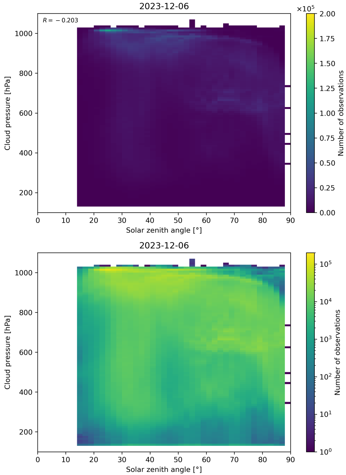
Figure 111: Scatter density plot of “Solar zenith angle” against “Cloud pressure” for 2023-12-05 to 2023-12-07.
