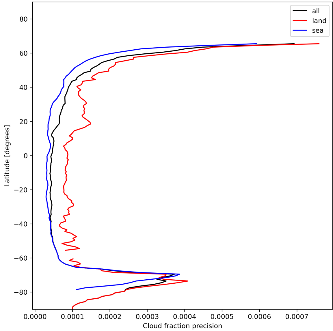
Figure 16: Zonal average of “Cloud fraction precision” for 2023-12-05 to 2023-12-07.
