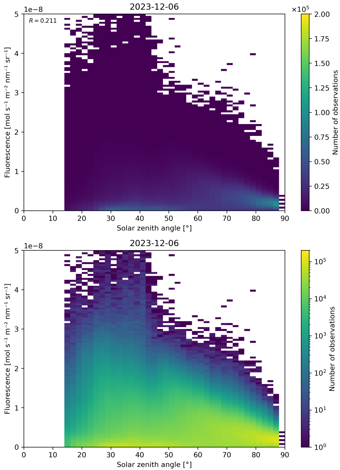
Figure 112: Scatter density plot of “Solar zenith angle” against “Fluorescence” for 2023-12-05 to 2023-12-07.
