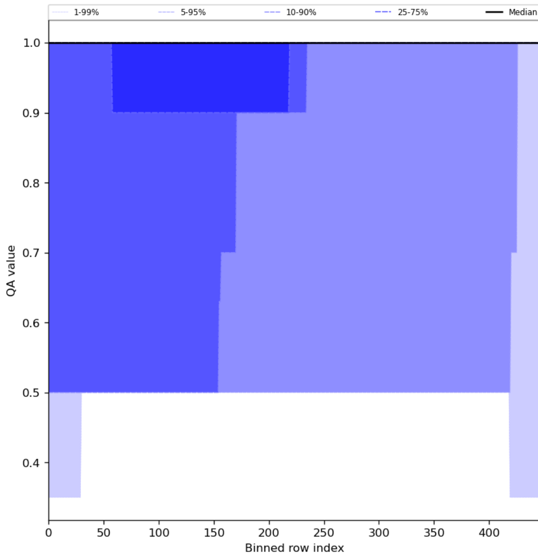
Figure 46: Along track statistics of “QA value” for 2023-12-05 to 2023-12-07
