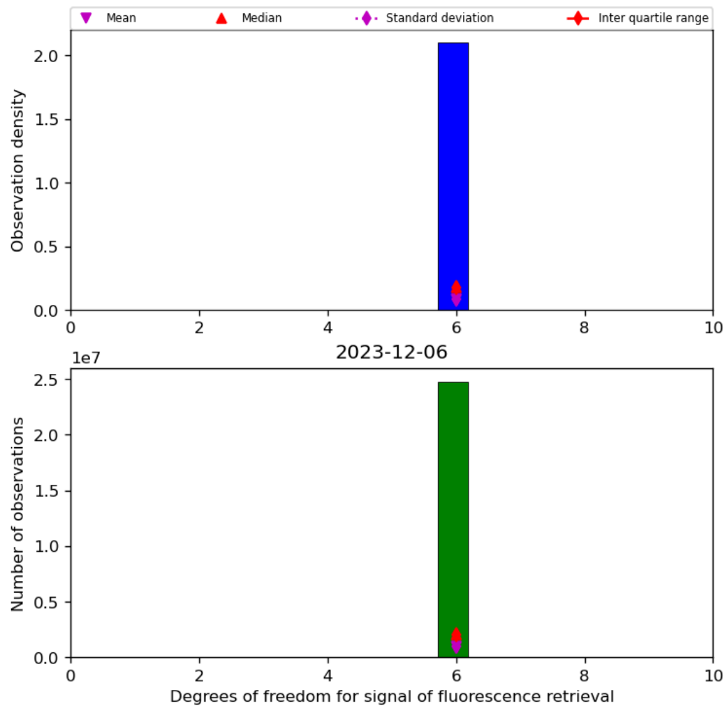
Figure 43: Histogram of “Degrees of freedom for signal of fluorescence retrieval” for 2023-12-05 to 2023-12-07
