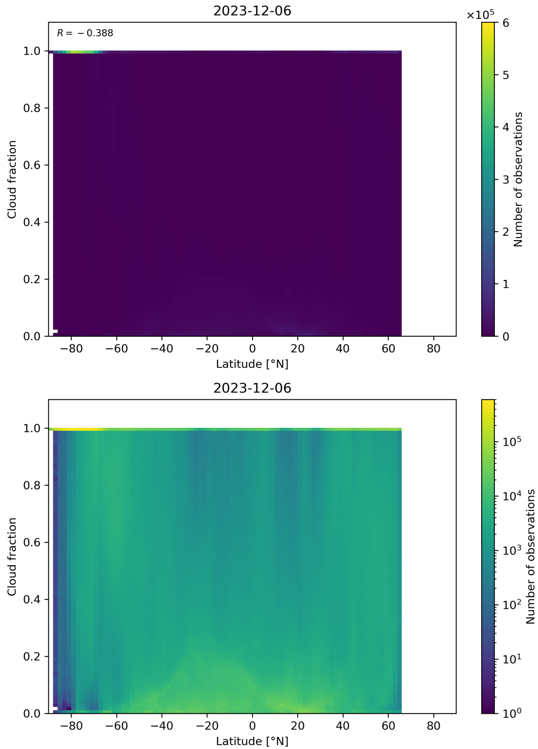
Figure 90: Scatter density plot of “Latitude” against “Cloud fraction” for 2023-12-05 to 2023-12-07.
