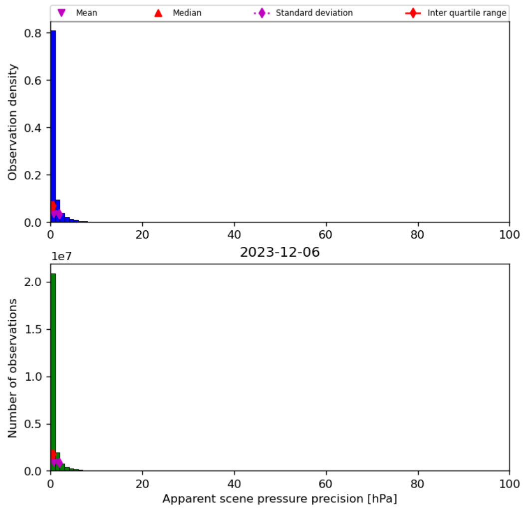
Figure 37: Histogram of “Apparent scene pressure precision” for 2023-12-05 to 2023-12-07
