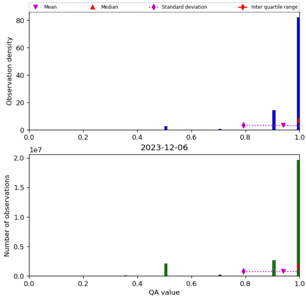
Figure 29: Histogram of “QA value” for 2023-12-05 to 2023-12-07
