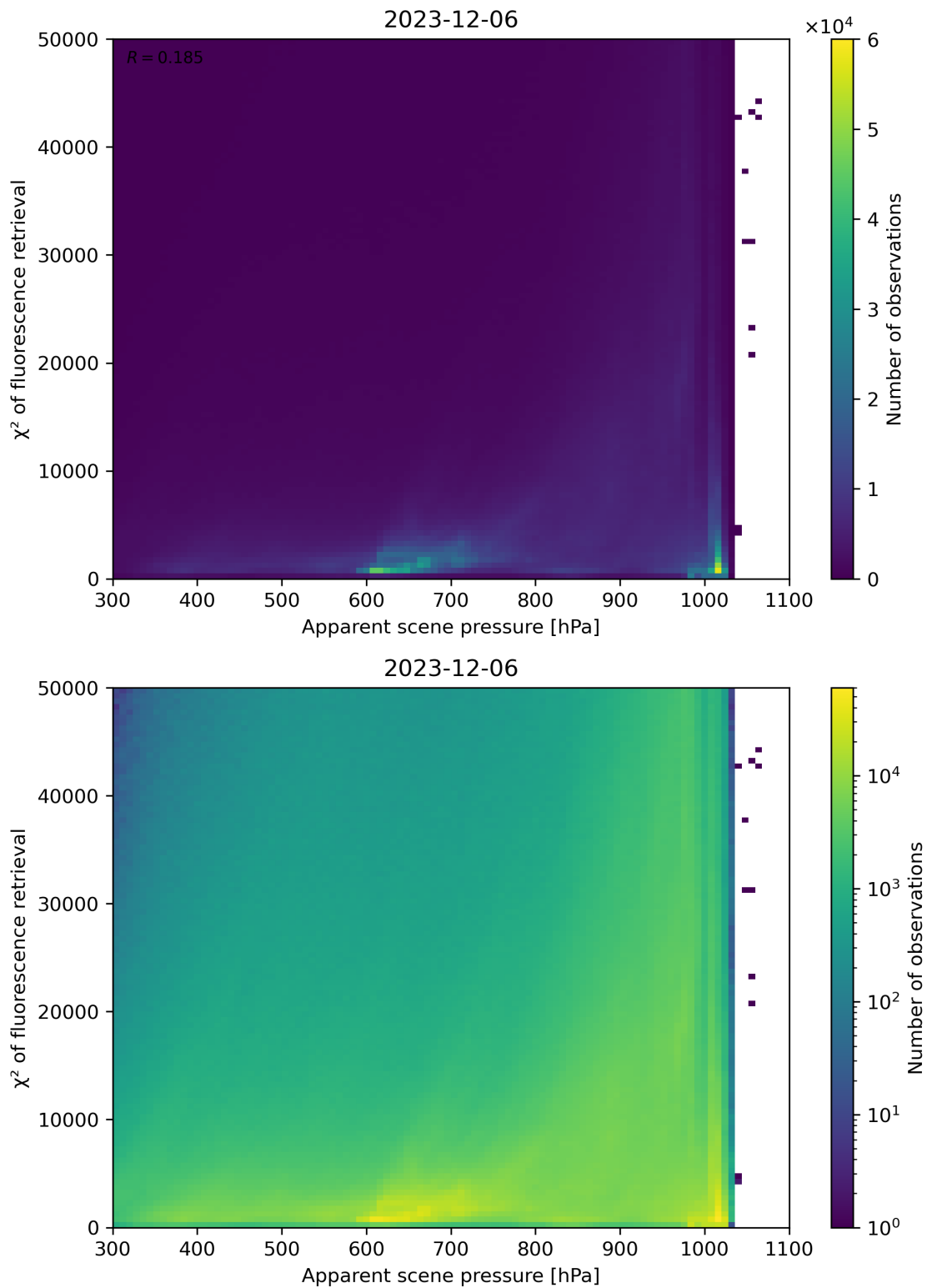
Figure 63: Scatter density plot of “Apparent scene pressure” against “ \chi^2 of fluorescence retrieval” for 2023-12-05 to 2023-12-07.
