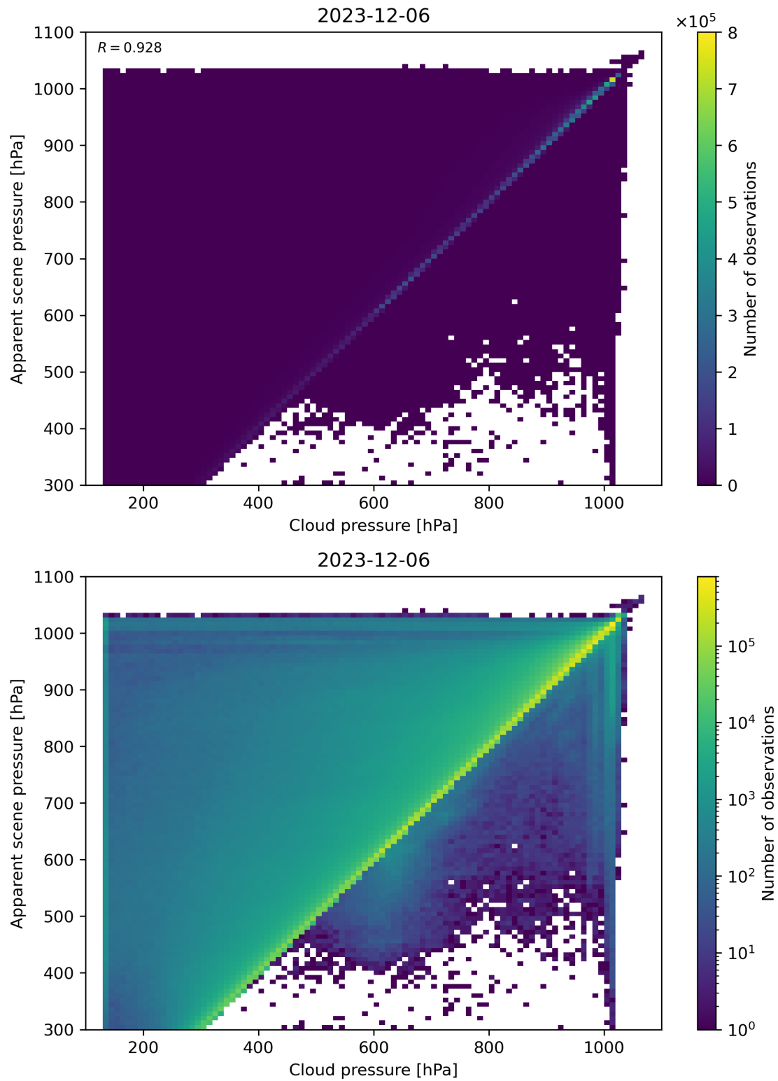
Figure 77: Scatter density plot of “Cloud pressure” against “Apparent scene pressure” for 2023-12-05 to 2023-12-07.
