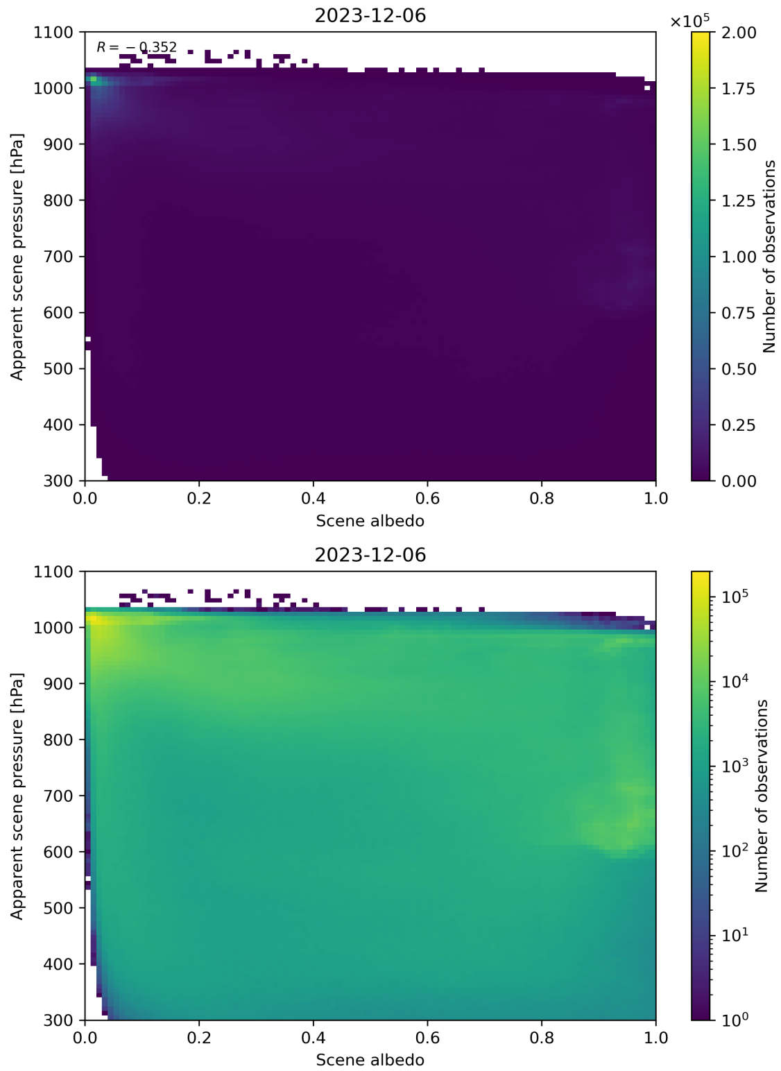
Figure 102: Scatter density plot of “Scene albedo” against “Apparent scene pressure” for 2023-12-05 to 2023-12-07.
