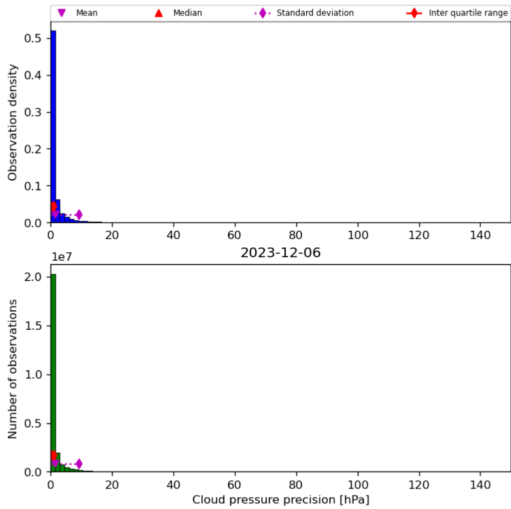
Figure 31: Histogram of “Cloud pressure precision” for 2023-12-05 to 2023-12-07
