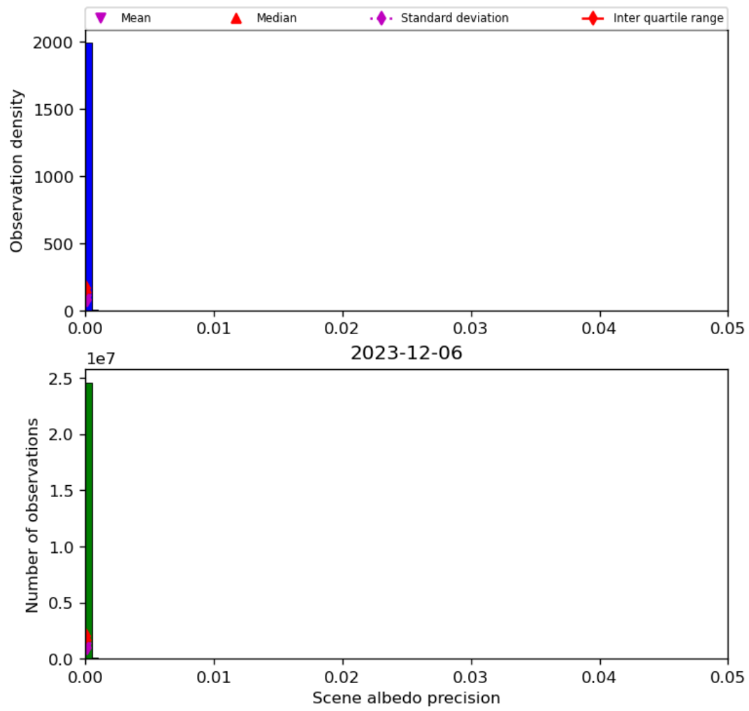
Figure 35: Histogram of “Scene albedo precision” for 2023-12-05 to 2023-12-07
