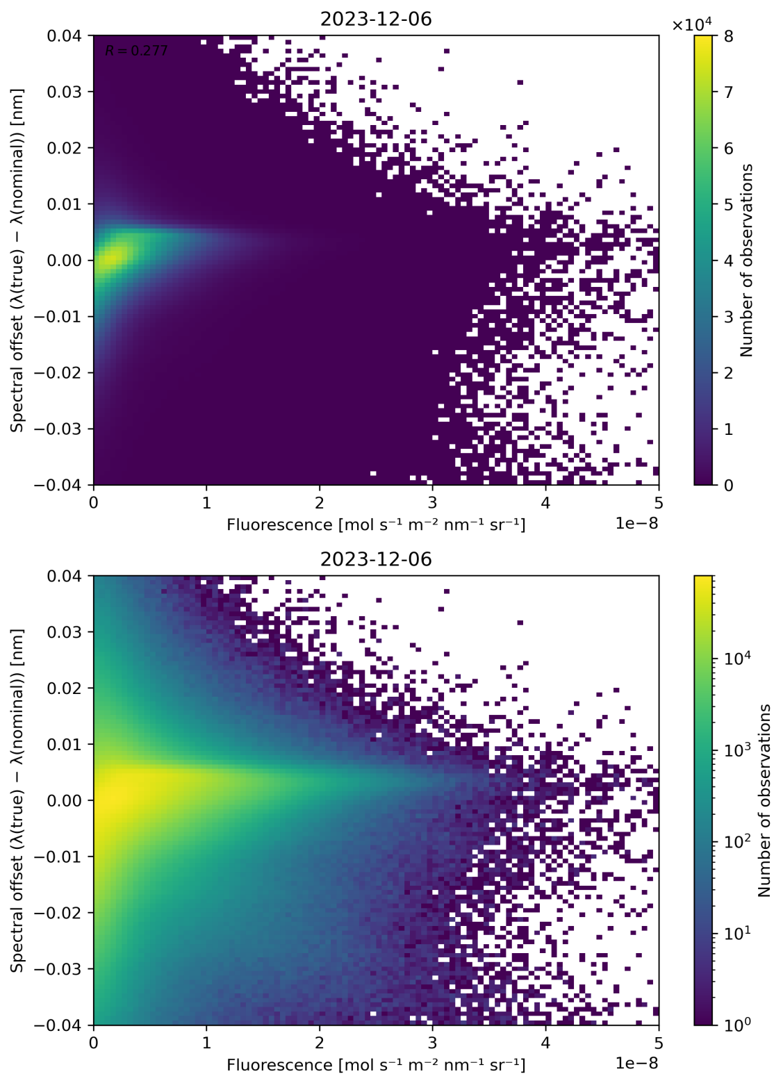
Figure 87: Scatter density plot of “Fluorescence” against “Spectral offset ( \lambda(\text{true}) - \lambda(\text{nominal}) )” for 2023-12-05 to 2023-12-07.
