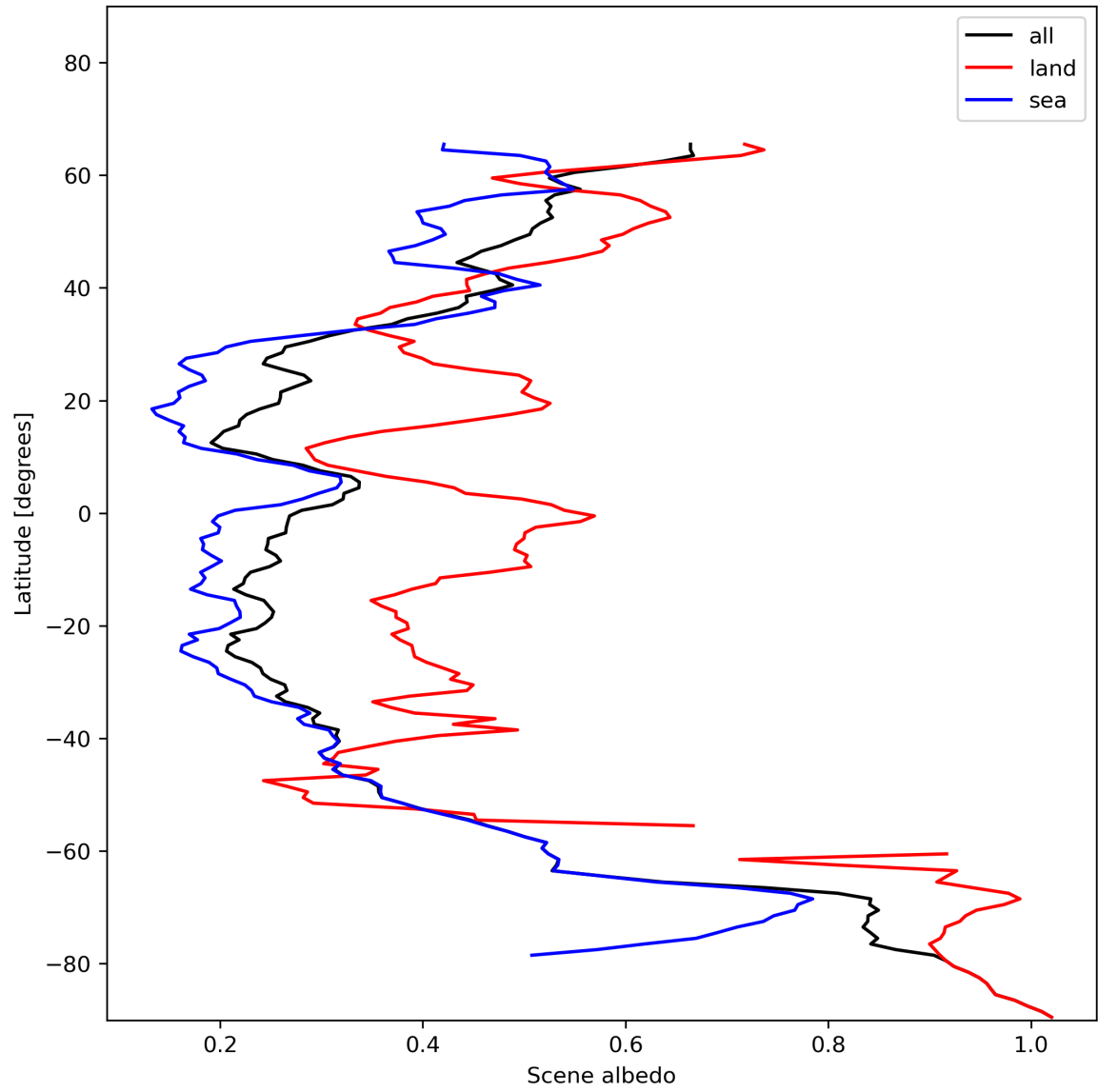
Figure 17: Zonal average of “Scene albedo” for 2023-12-05 to 2023-12-07.
