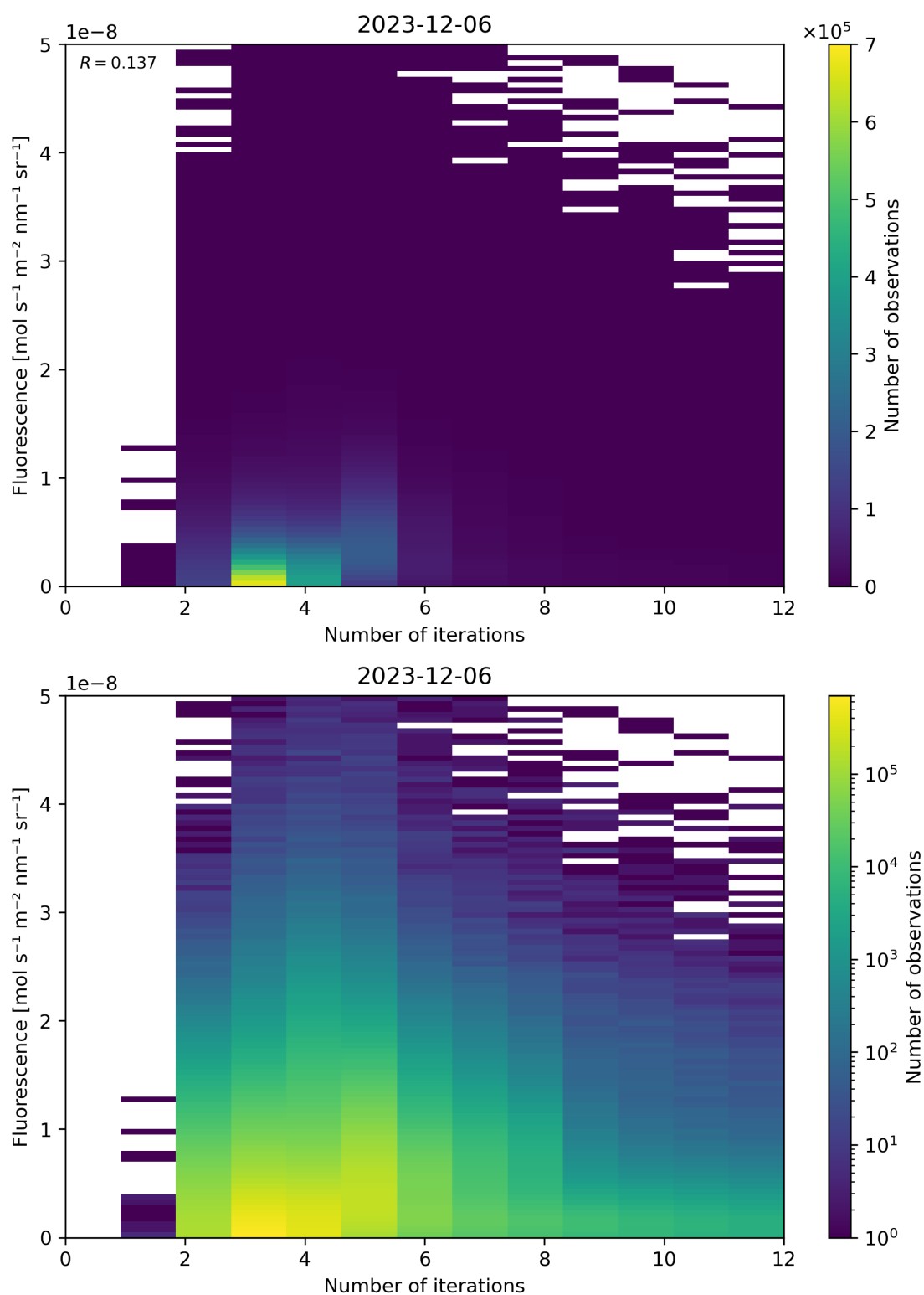
Figure 98: Scatter density plot of “Number of iterations” against “Fluorescence” for 2023-12-05 to 2023-12-07.
