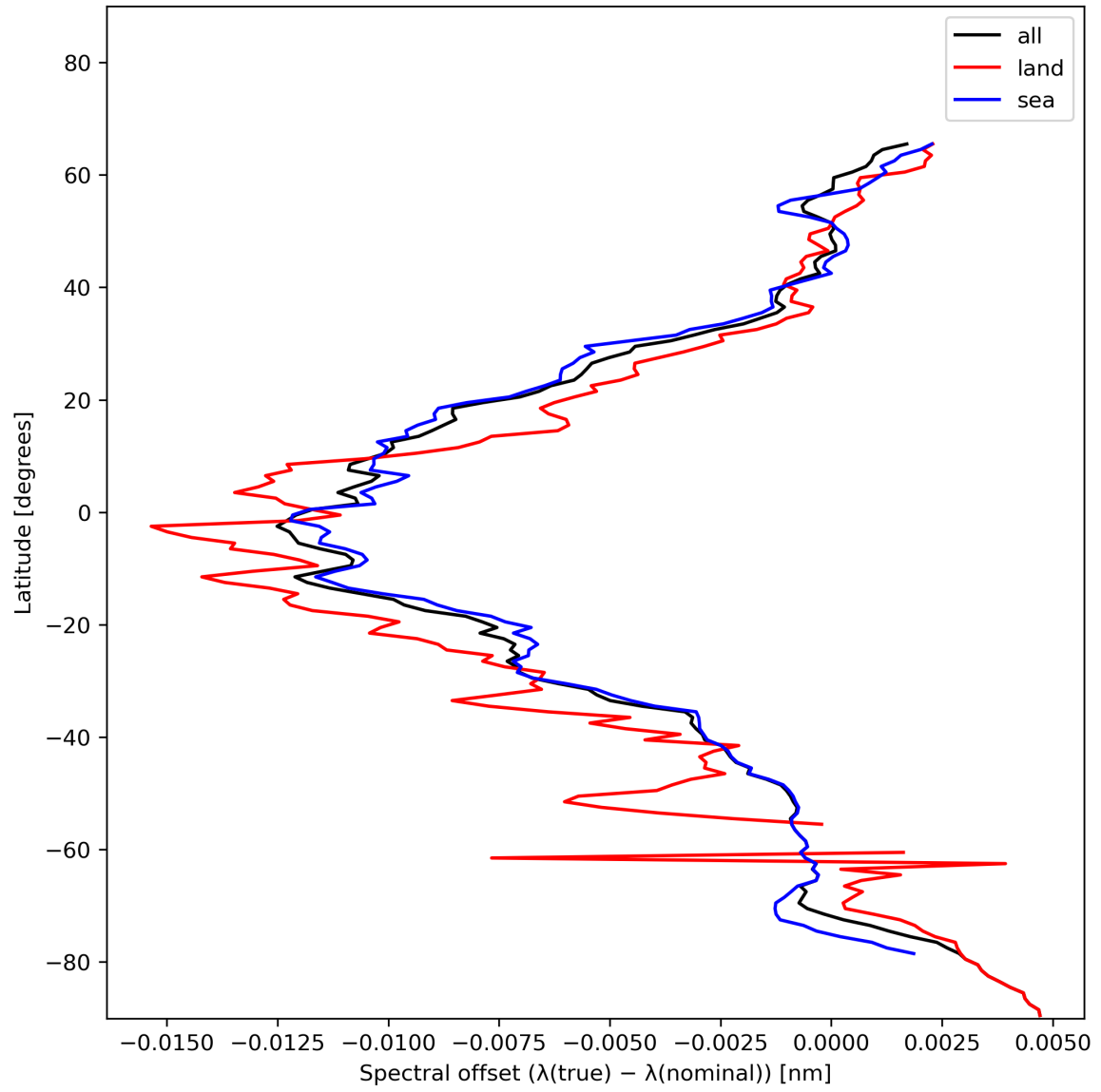
Figure 28: Zonal average of “Spectral offset ( \lambda(\text{true}) - \lambda(\text{nominal}) )” for 2023-12-05 to 2023-12-07.
