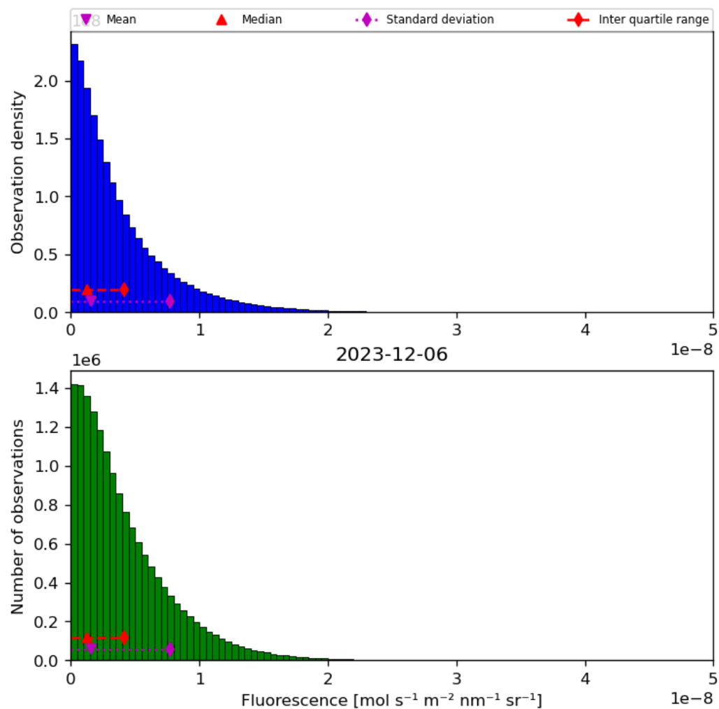
Figure 40: Histogram of “Fluorescence” for 2023-12-05 to 2023-12-07
