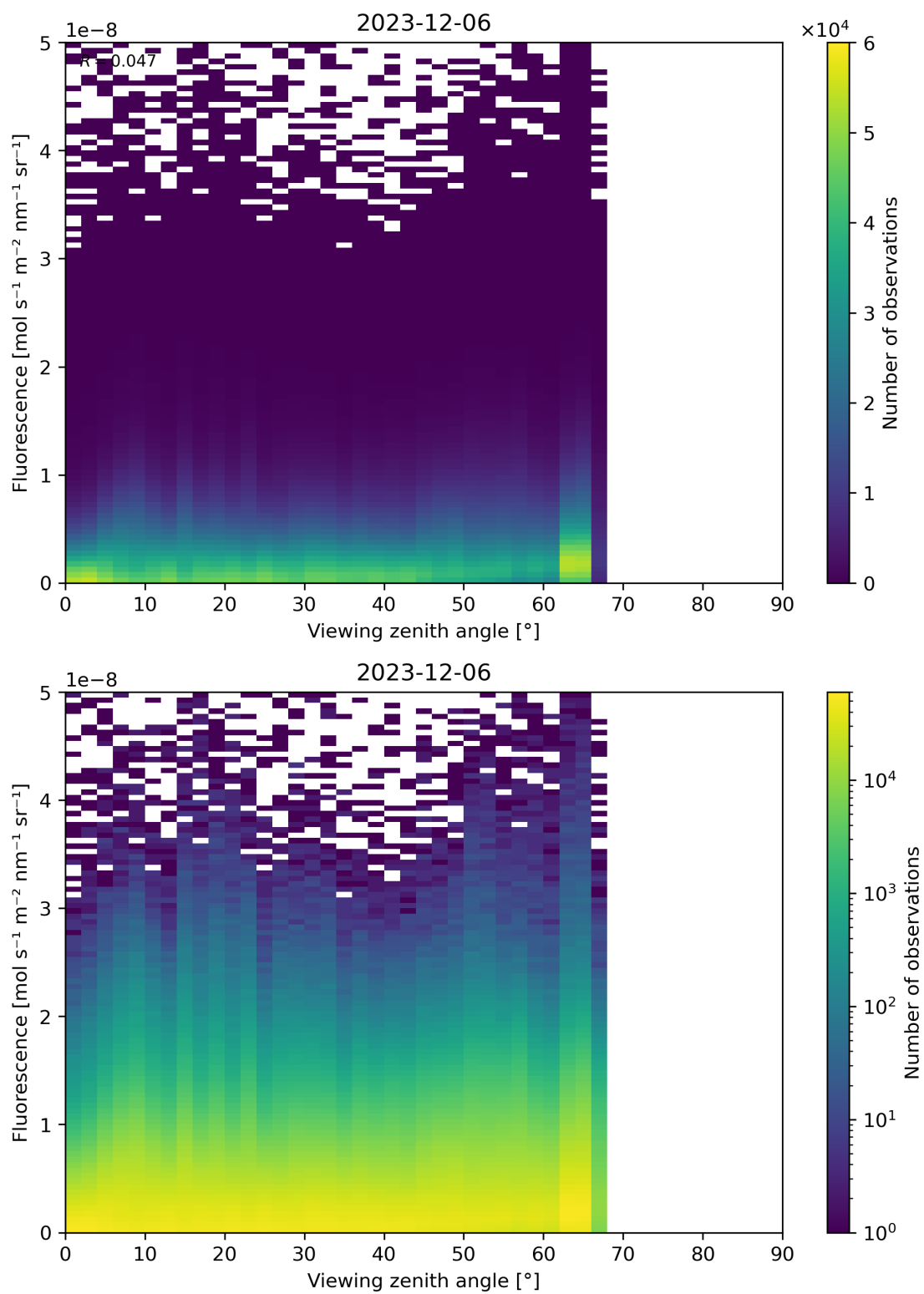
Figure 122: Scatter density plot of “Viewing zenith angle” against “Fluorescence” for 2023-12-05 to 2023-12-07.
