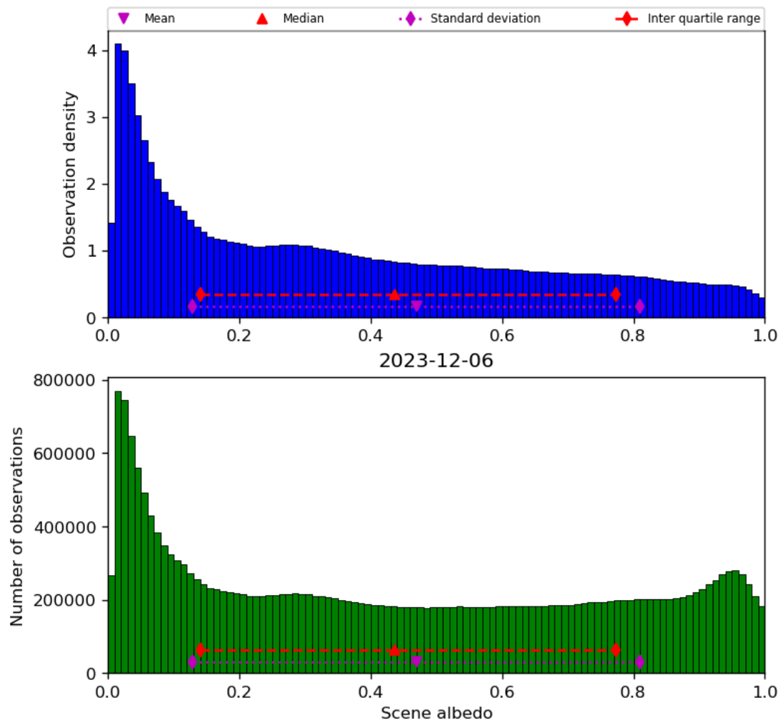
Figure 34: Histogram of “Scene albedo” for 2023-12-05 to 2023-12-07
