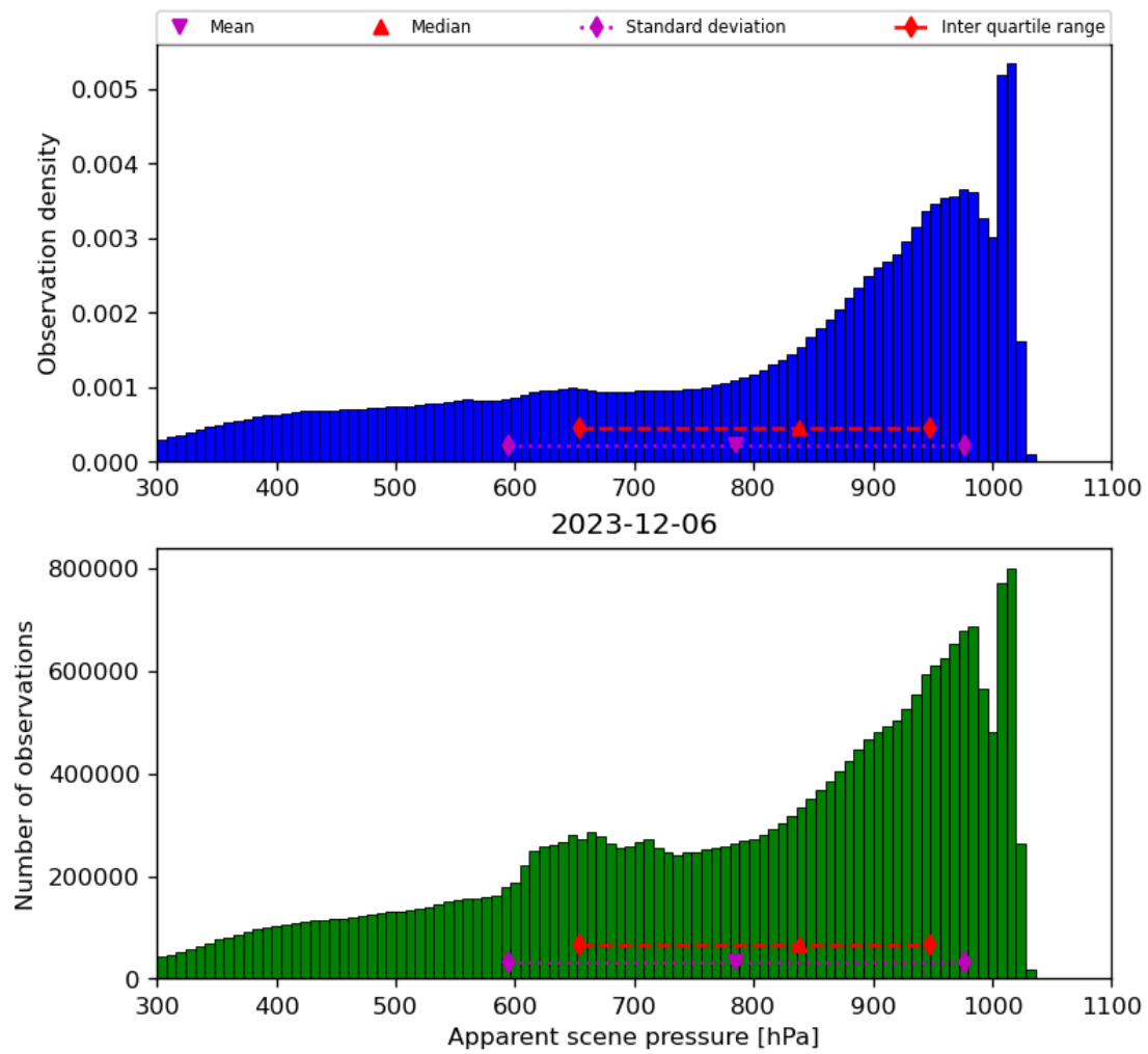
Figure 36: Histogram of “Apparent scene pressure” for 2023-12-05 to 2023-12-07
