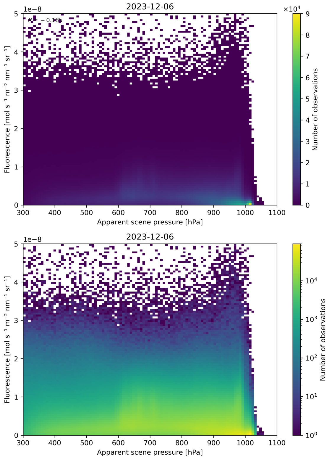
Figure 64: Scatter density plot of “Apparent scene pressure” against “Fluorescence” for 2023-12-05 to 2023-12-07.
