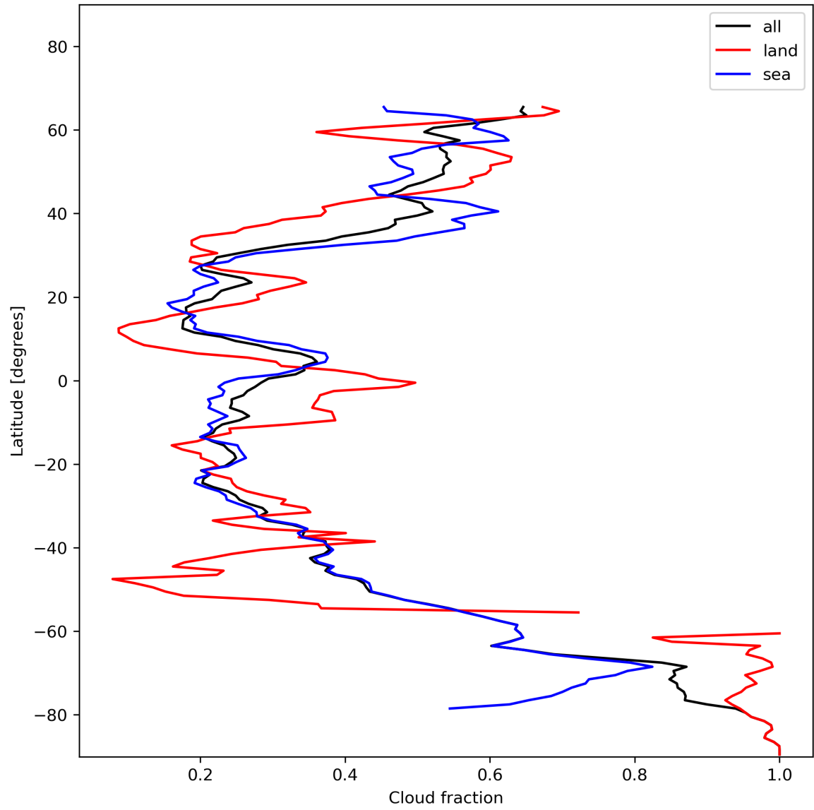
Figure 15: Zonal average of “Cloud fraction” for 2023-12-05 to 2023-12-07.
