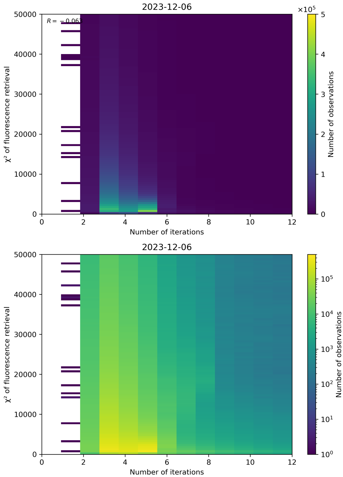
Figure 97: Scatter density plot of “Number of iterations” against “ \chi^2 of fluorescence retrieval” for 2023-12-05 to 2023-12-07.
