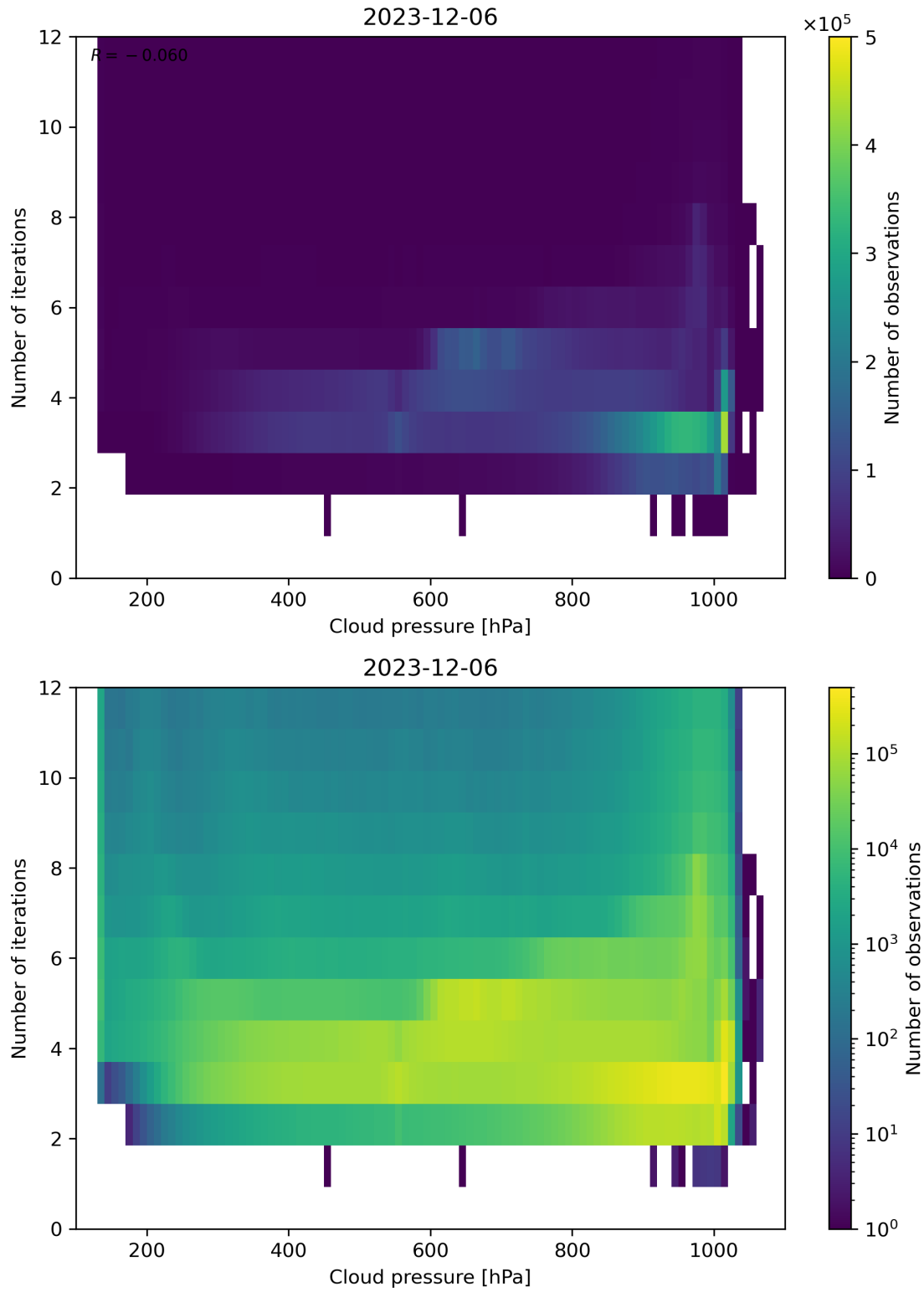
Figure 81: Scatter density plot of “Cloud pressure” against “Number of iterations” for 2023-12-05 to 2023-12-07.
