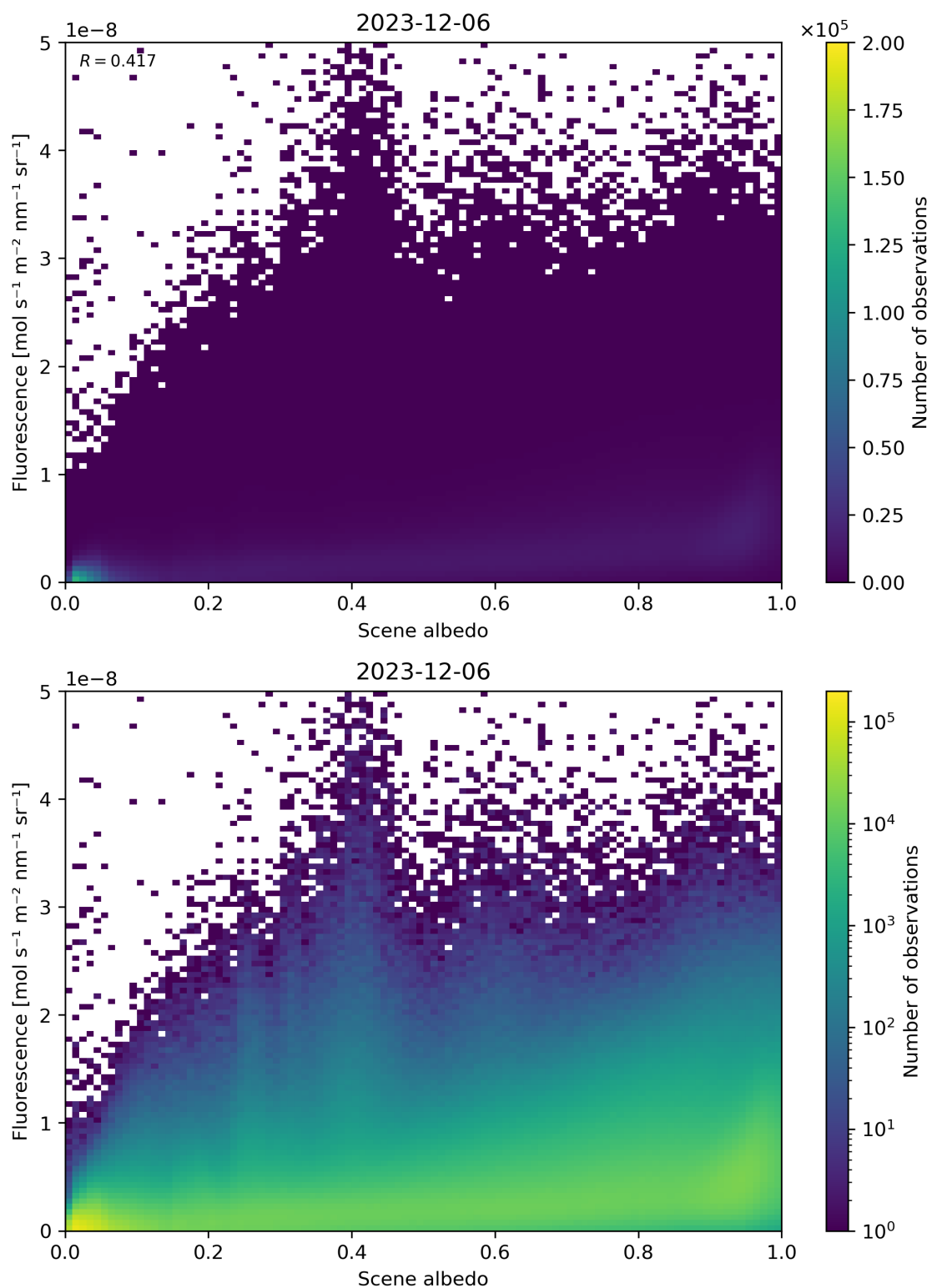
Figure 104: Scatter density plot of “Scene albedo” against “Fluorescence” for 2023-12-05 to 2023-12-07.
