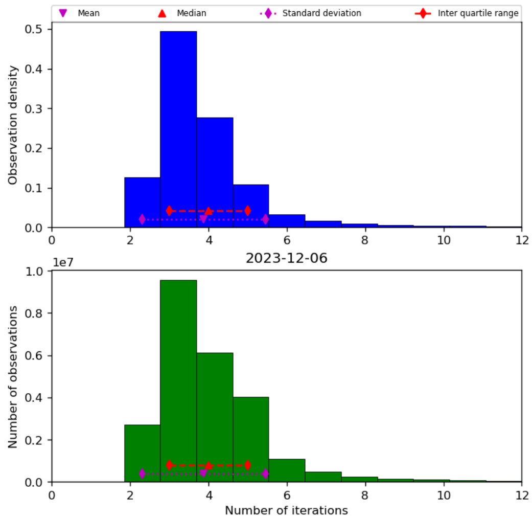
Figure 39: Histogram of “Number of iterations” for 2023-12-05 to 2023-12-07
