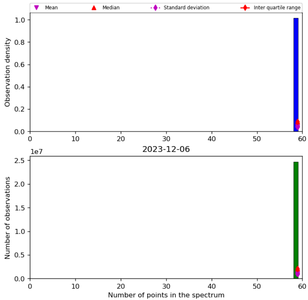
Figure 44: Histogram of “Number of points in the spectrum” for 2023-12-05 to 2023-12-07
