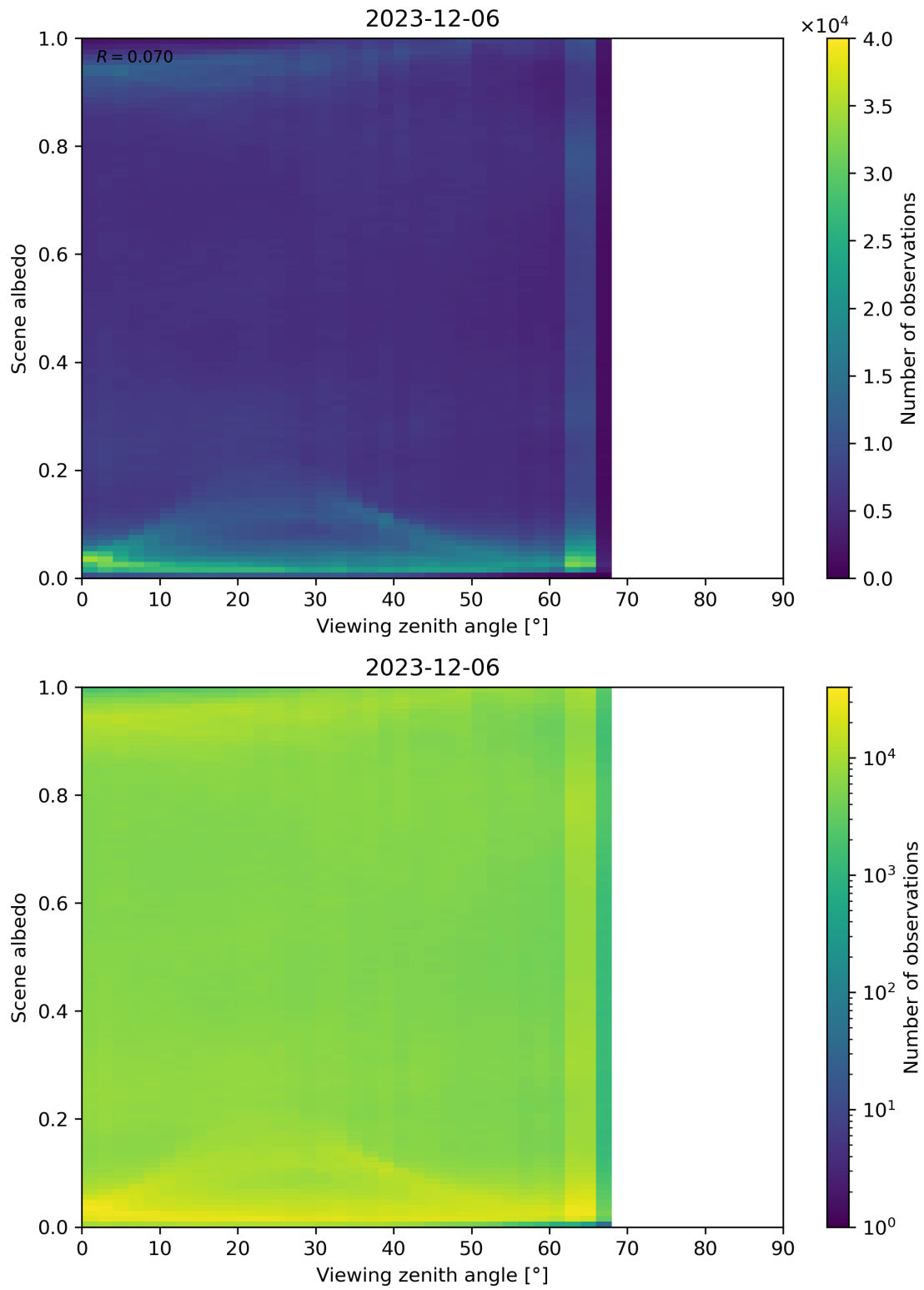
Figure 126: Scatter density plot of “Viewing zenith angle” against “Scene albedo” for 2023-12-05 to 2023-12-07.
