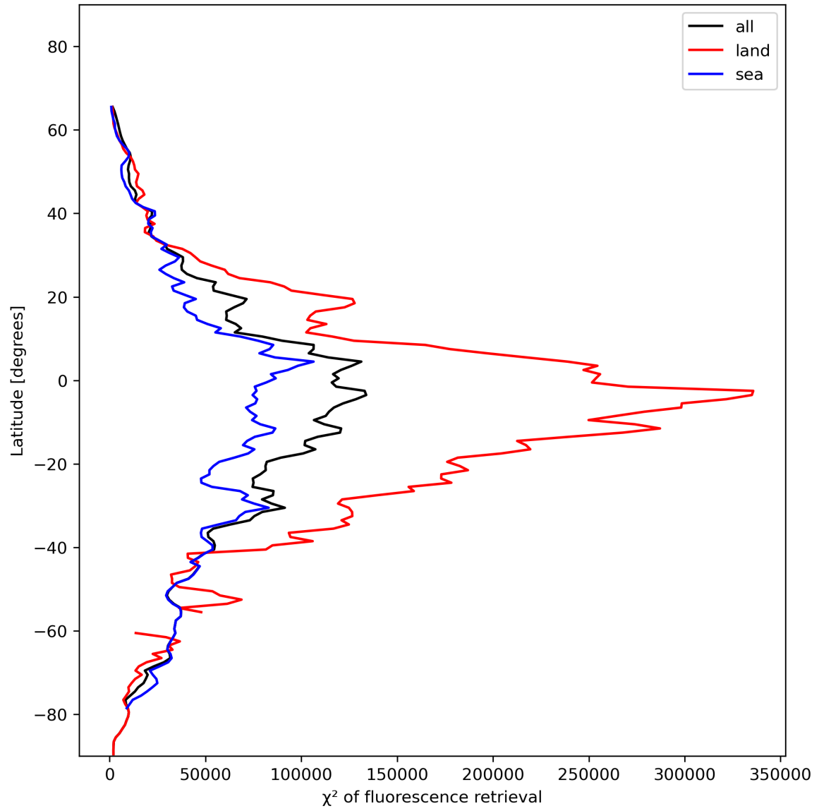
Figure 25: Zonal average of “ \chi^2 of fluorescence retrieval” for 2023-12-05 to 2023-12-07.
