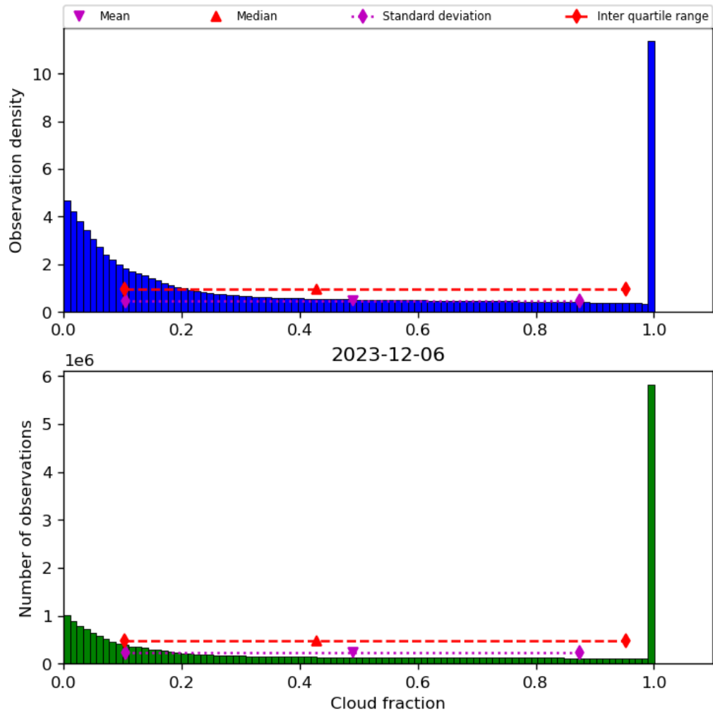
Figure 32: Histogram of “Cloud fraction” for 2023-12-05 to 2023-12-07
