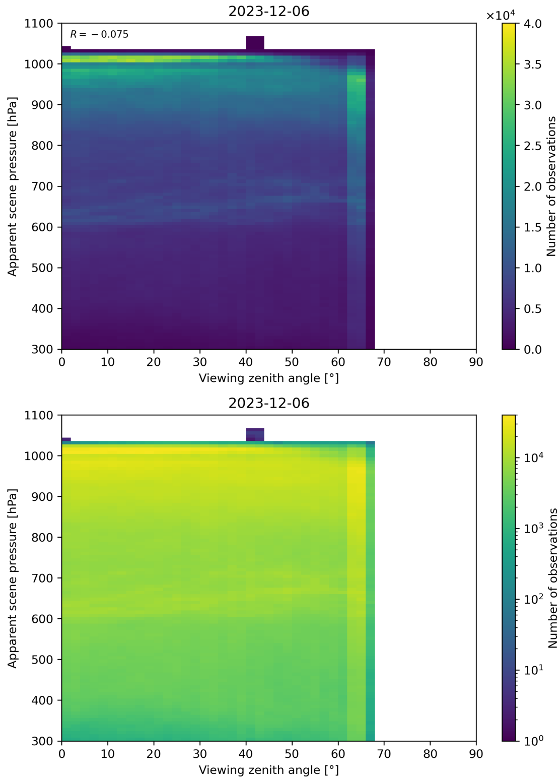
Figure 118: Scatter density plot of “Viewing zenith angle” against “Apparent scene pressure” for 2023-12-05 to 2023-12-07.
