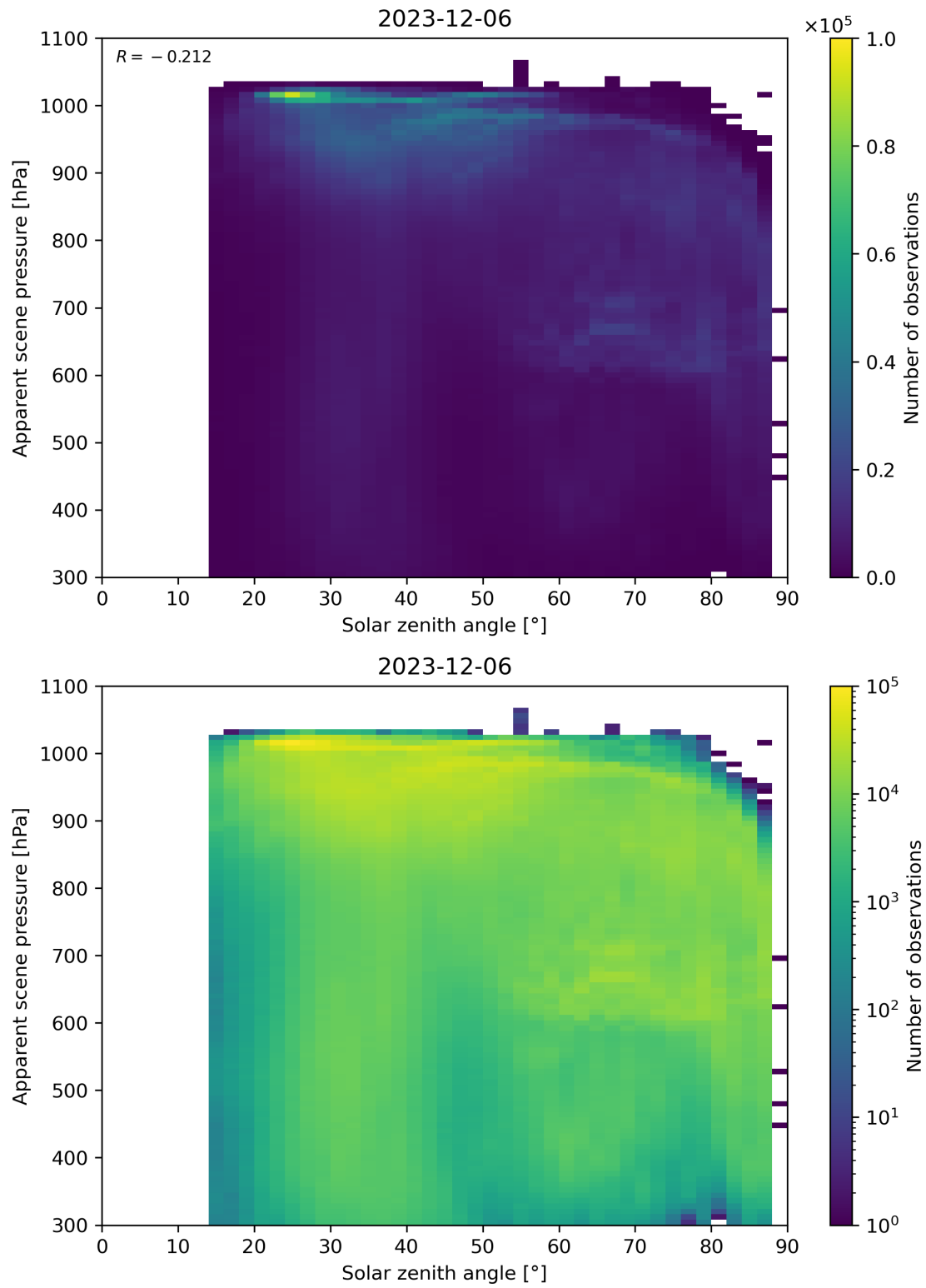
Figure 108: Scatter density plot of “Solar zenith angle” against “Apparent scene pressure” for 2023-12-05 to 2023-12-07.
