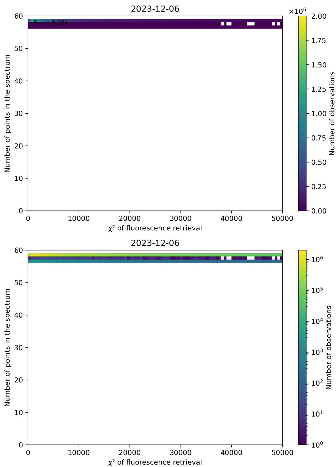
Figure 68: Scatter density plot of “ \chi^2 of fluorescence retrieval” against “Number of points in the spectrum” for 2023-12-05 to 2023-12-07.
