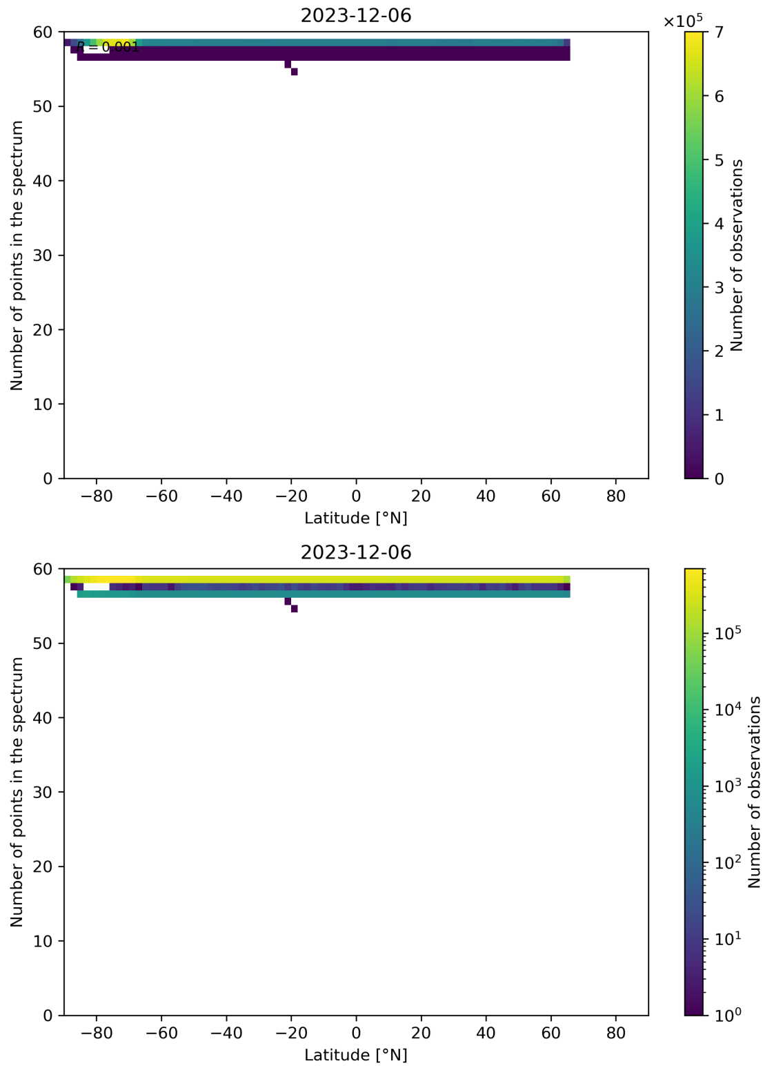
Figure 94: Scatter density plot of “Latitude” against “Number of points in the spectrum” for 2023-12-05 to 2023-12-07.
