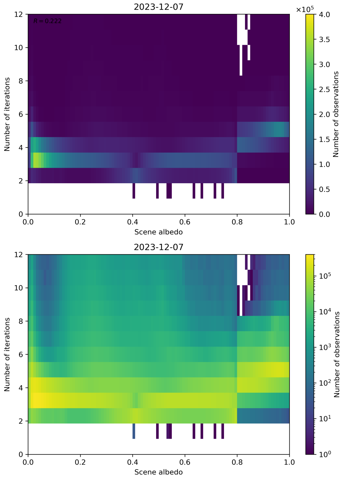
Figure 105: Scatter density plot of “Scene albedo” against “Number of iterations” for 2023-12-06 to 2023-12-08.
