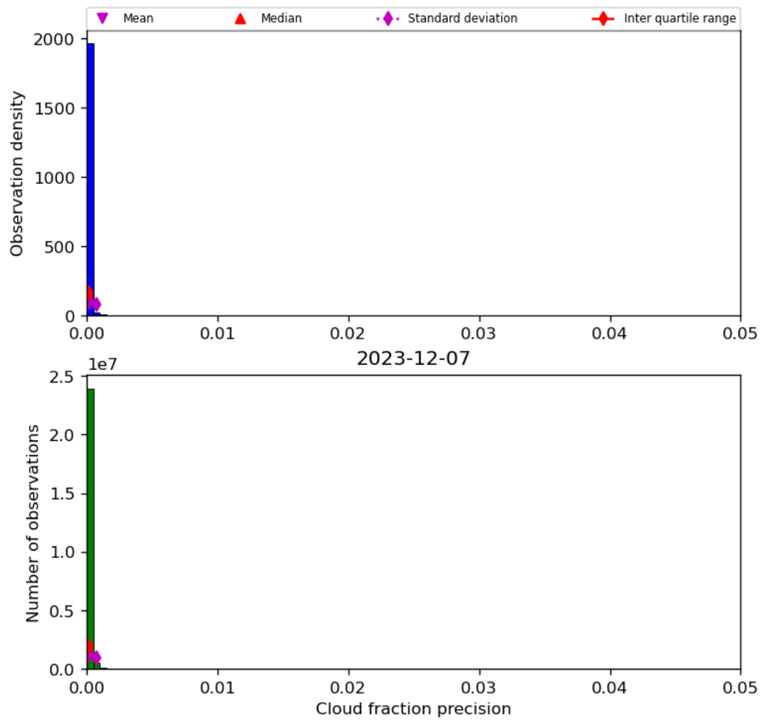
Figure 33: Histogram of “Cloud fraction precision” for 2023-12-06 to 2023-12-08
