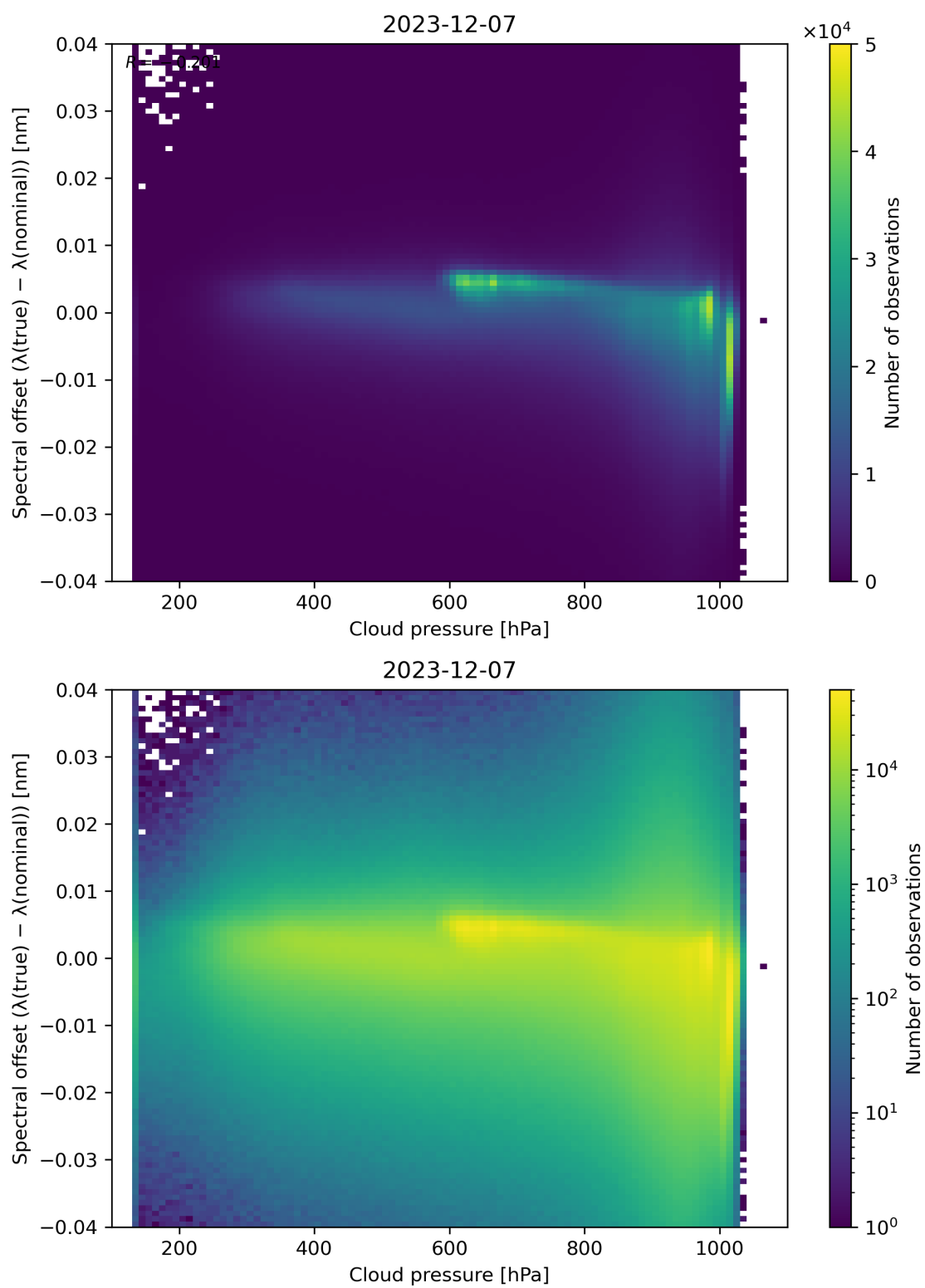
Figure 84: Scatter density plot of “Cloud pressure” against “Spectral offset ( \lambda(\text{true}) - \lambda(\text{nominal}) )” for 2023-12-06 to 2023-12-08.
