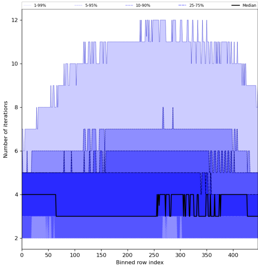
Figure 56: Along track statistics of “Number of iterations” for 2023-12-06 to 2023-12-08
