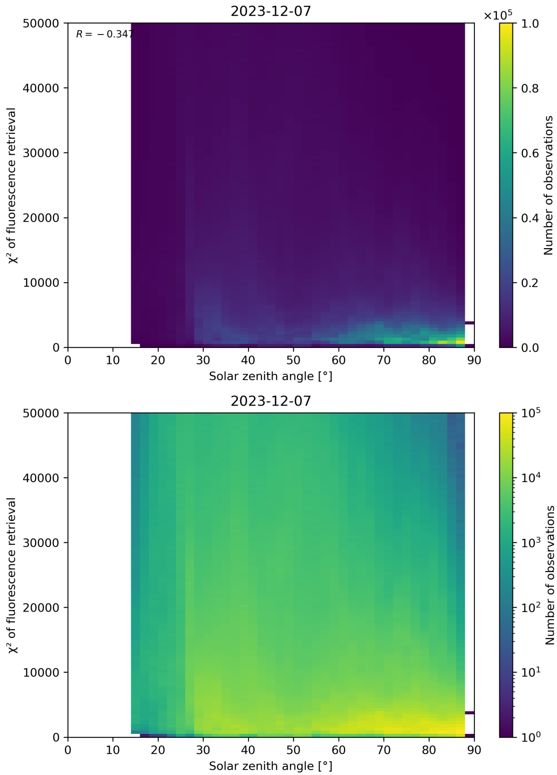
Figure 109: Scatter density plot of “Solar zenith angle” against “ \chi^2 of fluorescence retrieval” for 2023-12-06 to 2023-12-08.
