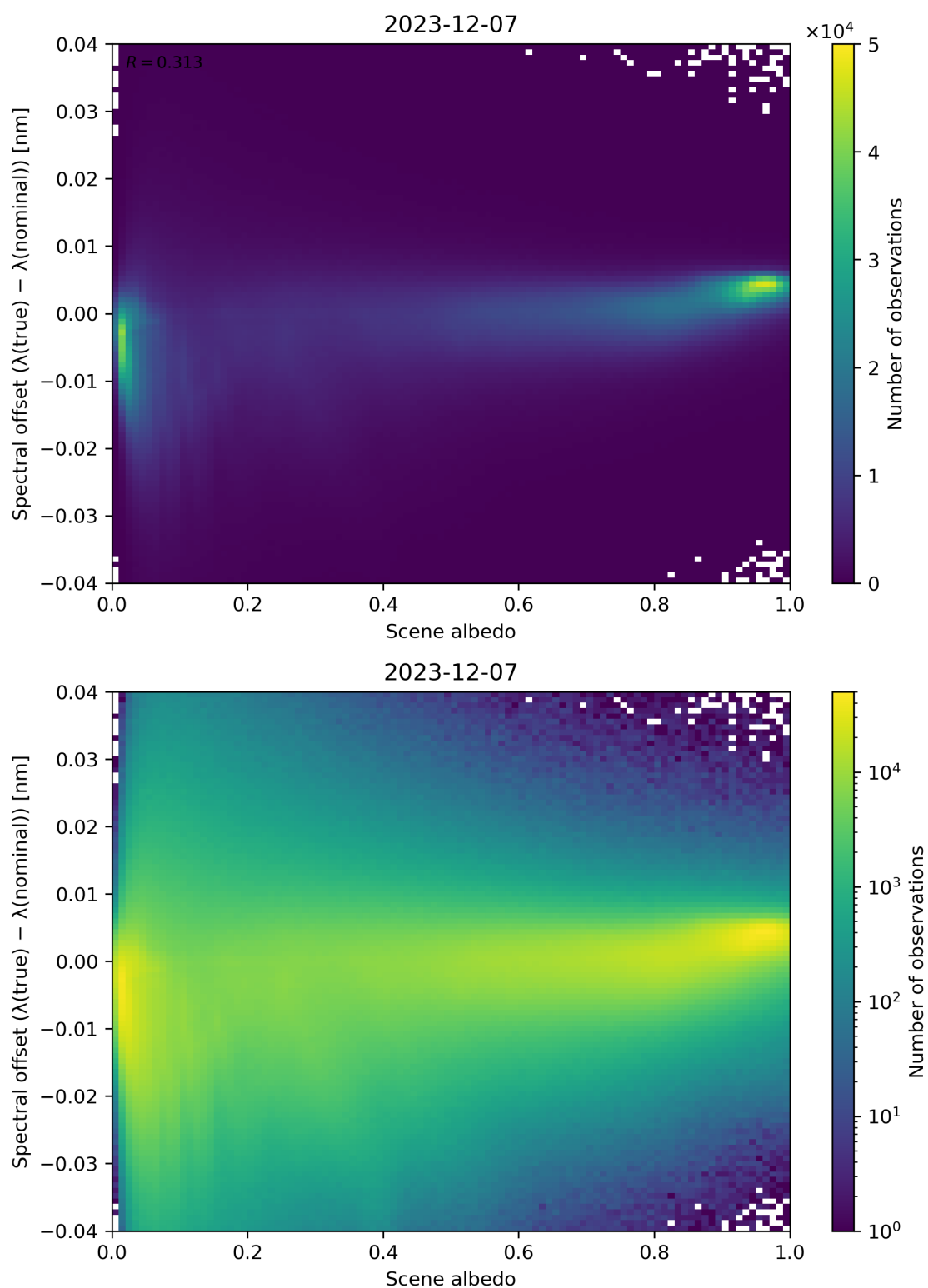
Figure 107: Scatter density plot of “Scene albedo” against “Spectral offset ( \lambda(\text{true}) - \lambda(\text{nominal}) )” for 2023-12-06 to 2023-12-08.
