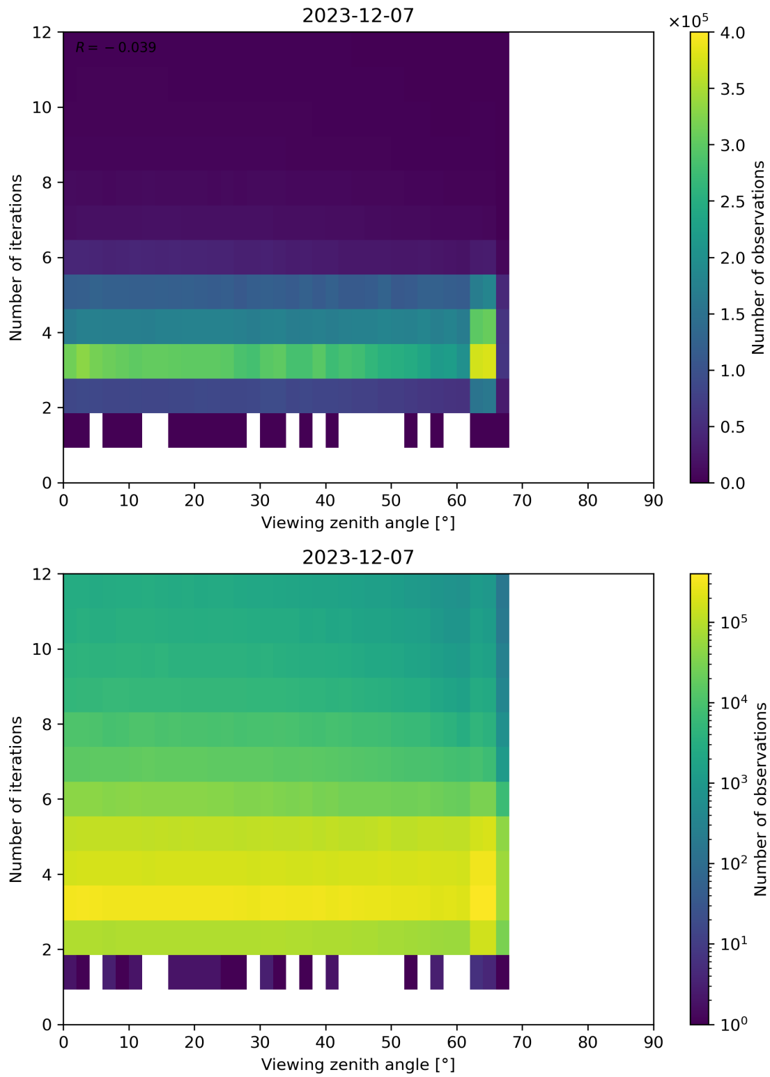
Figure 124: Scatter density plot of “Viewing zenith angle” against “Number of iterations” for 2023-12-06 to 2023-12-08.
