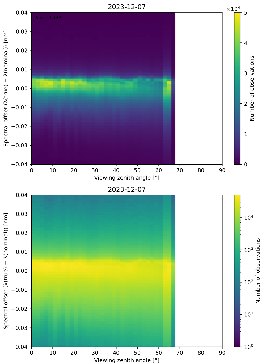
Figure 128: Scatter density plot of “Viewing zenith angle” against “Spectral offset ( \lambda(\text{true}) - \lambda(\text{nominal}) )” for 2023-12-06 to 2023-12-08.
