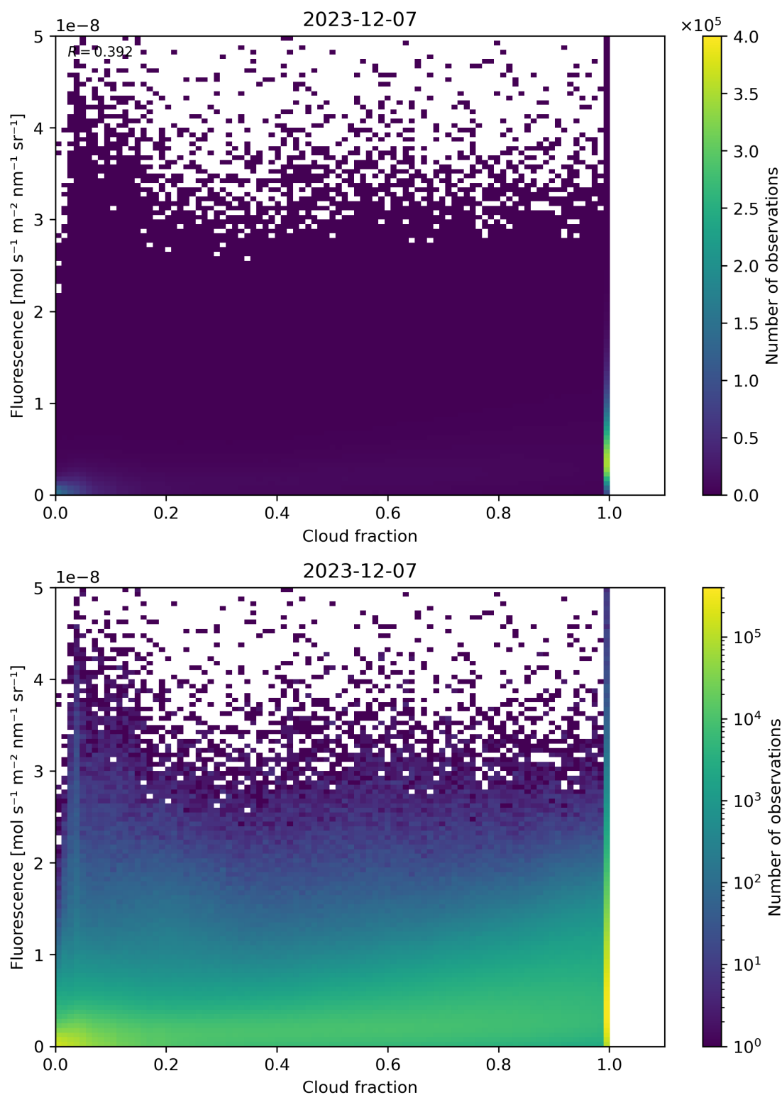
Figure 72: Scatter density plot of “Cloud fraction” against “Fluorescence” for 2023-12-06 to 2023-12-08.
