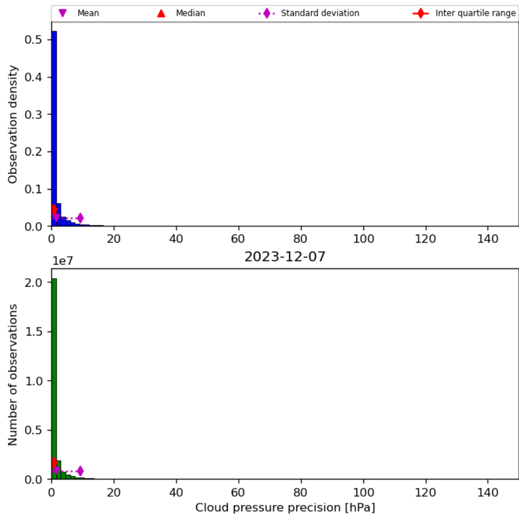
Figure 31: Histogram of “Cloud pressure precision” for 2023-12-06 to 2023-12-08
