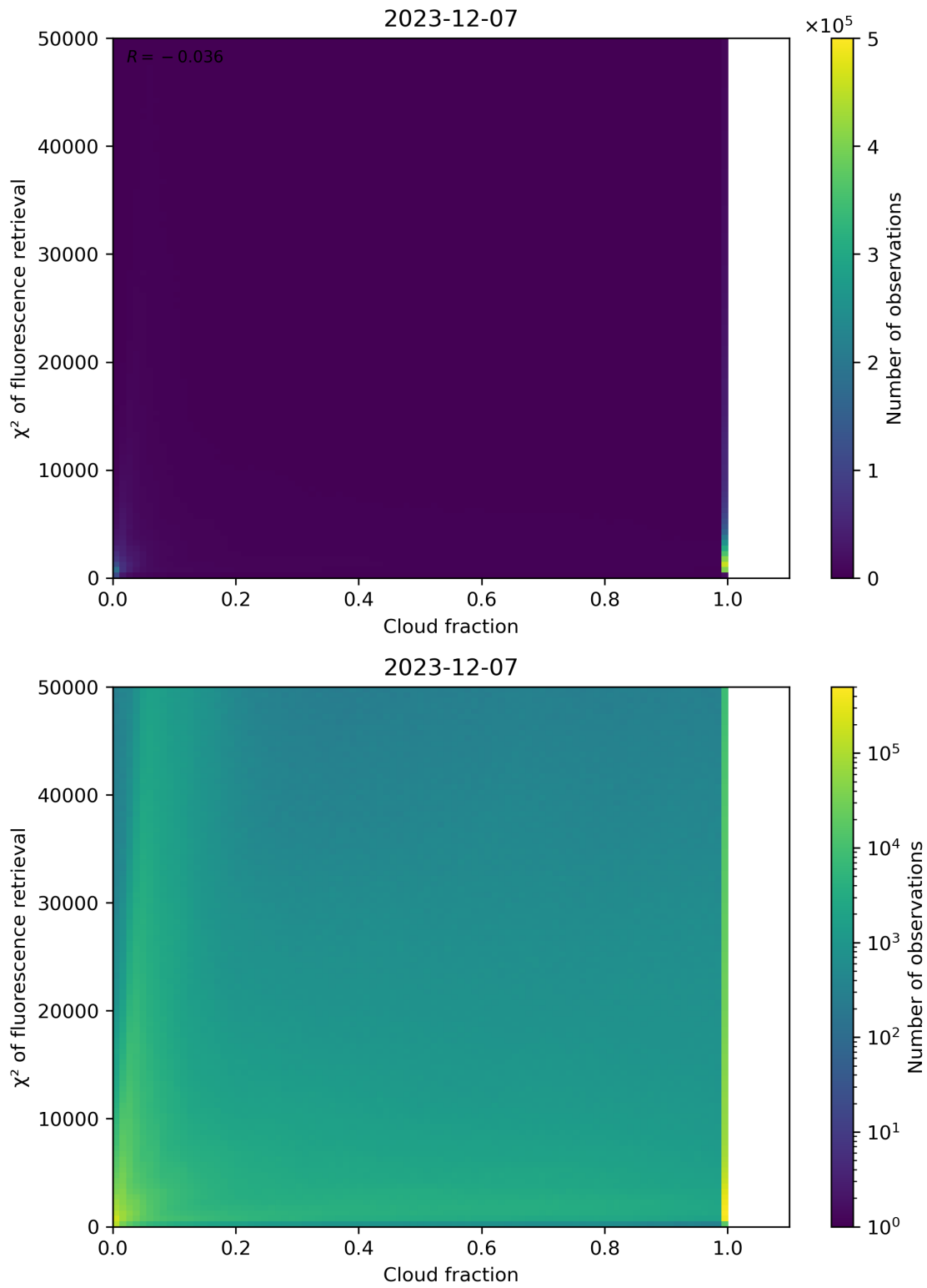
Figure 71: Scatter density plot of “Cloud fraction” against “ \chi^2 of fluorescence retrieval” for 2023-12-06 to 2023-12-08.
