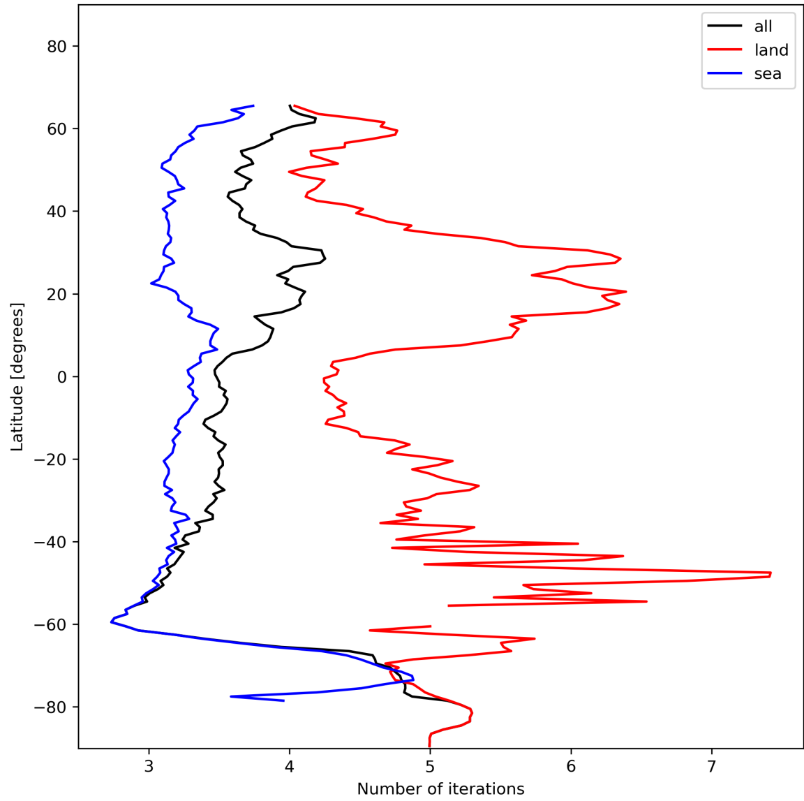
Figure 22: Zonal average of “Number of iterations” for 2023-12-06 to 2023-12-08.
