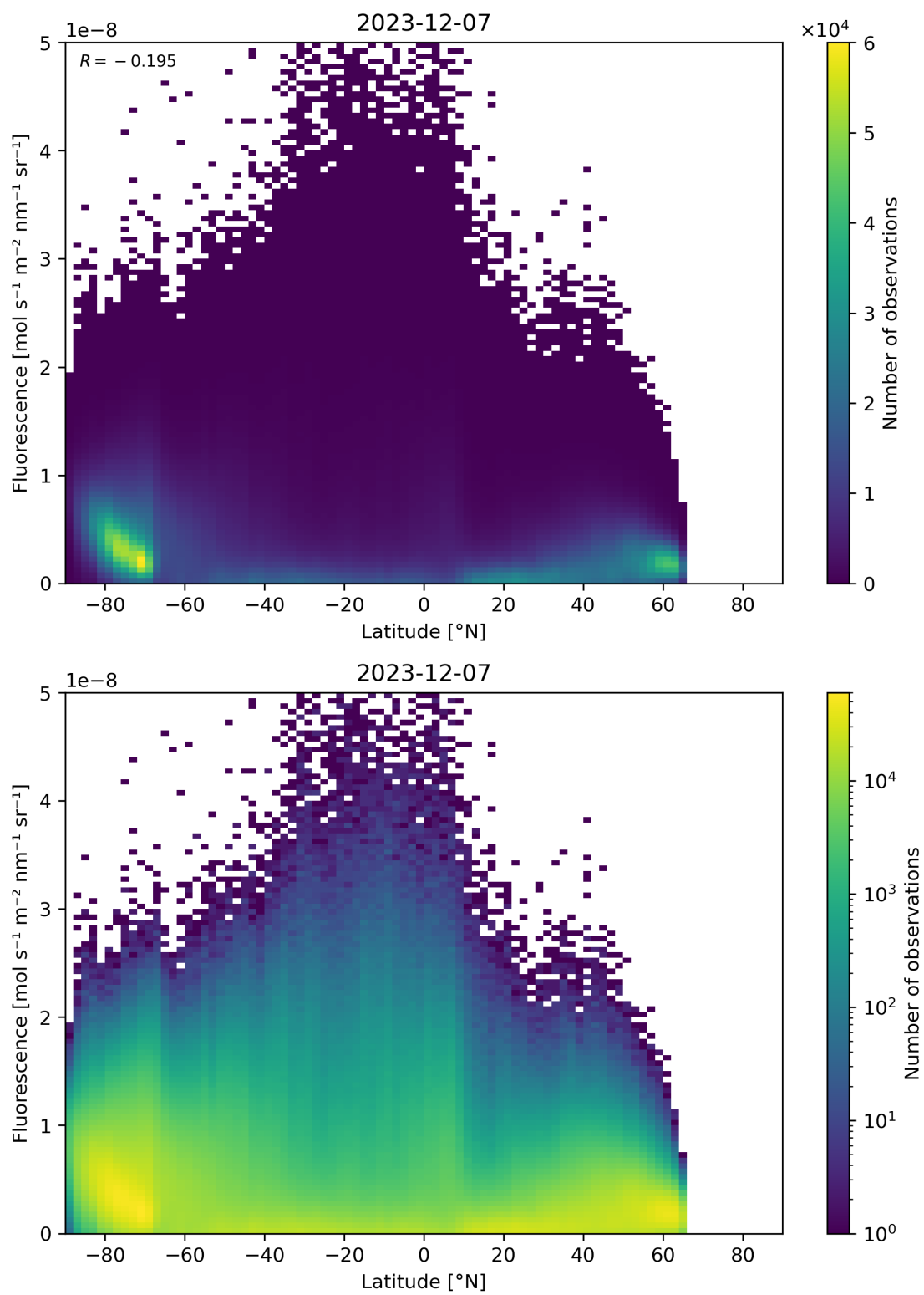
Figure 92: Scatter density plot of “Latitude” against “Fluorescence” for 2023-12-06 to 2023-12-08.
