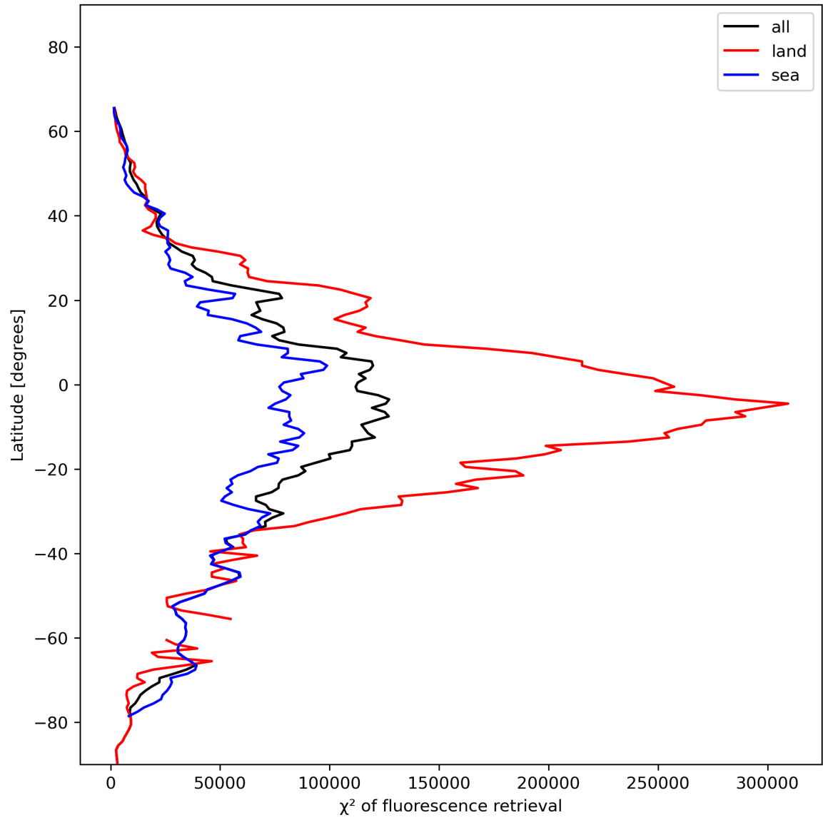
Figure 25: Zonal average of “ \chi^2 of fluorescence retrieval” for 2023-12-06 to 2023-12-08.
