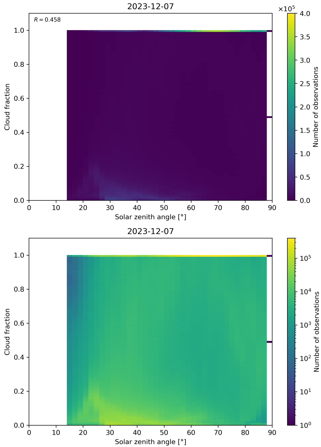
Figure 110: Scatter density plot of “Solar zenith angle” against “Cloud fraction” for 2023-12-06 to 2023-12-08.
