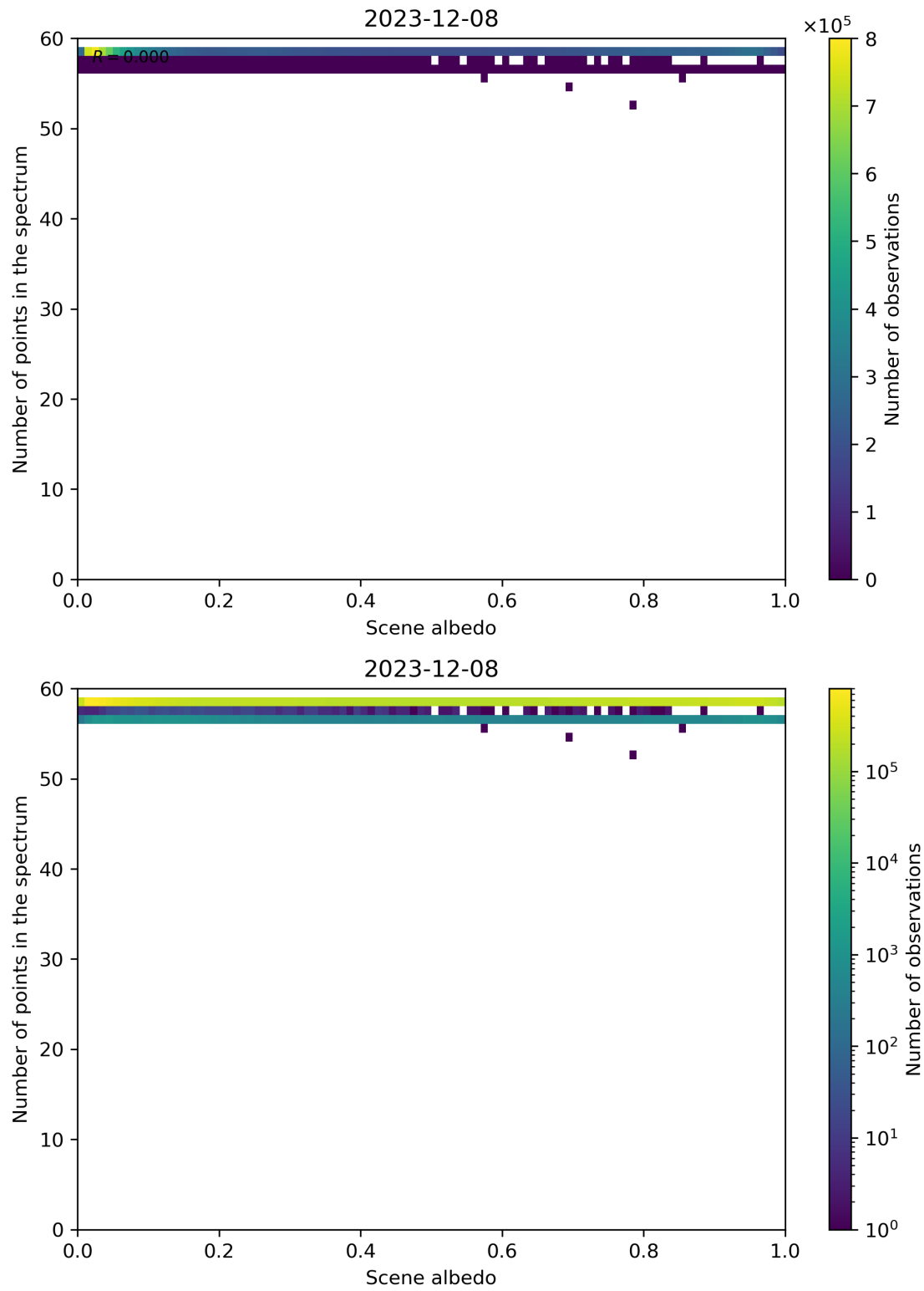
Figure 106: Scatter density plot of “Scene albedo” against “Number of points in the spectrum” for 2023-12-07 to 2023-12-09.
