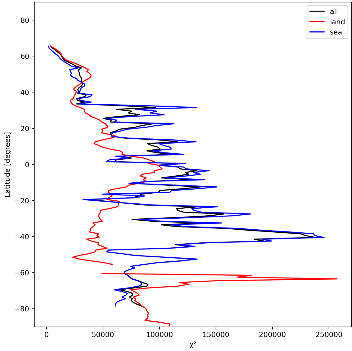
Figure 21: Zonal average of “ \chi^2 ” for 2023-12-07 to 2023-12-09.
