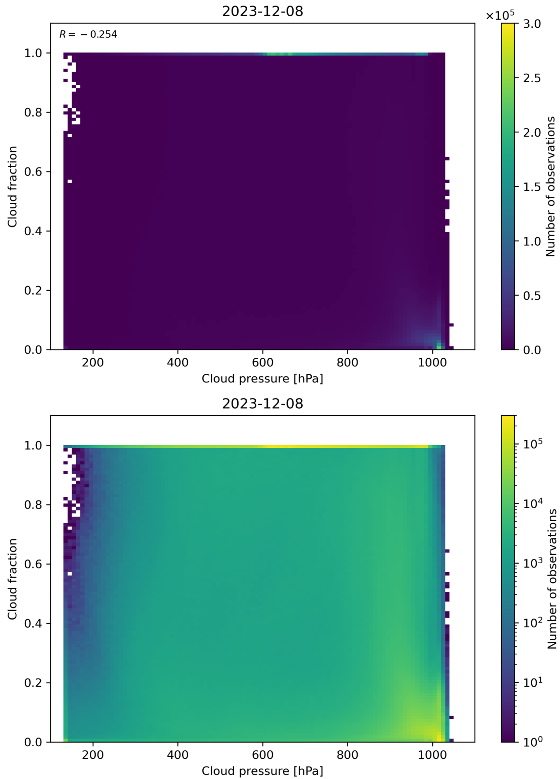
Figure 79: Scatter density plot of “Cloud pressure” against “Cloud fraction” for 2023-12-07 to 2023-12-09.
