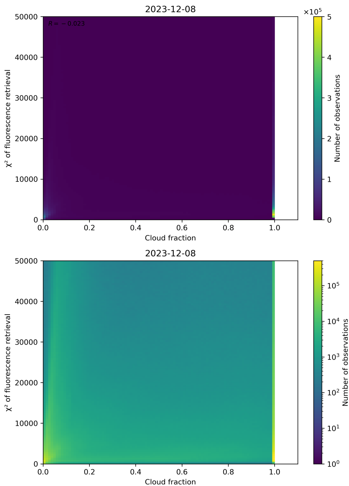
Figure 71: Scatter density plot of “Cloud fraction” against “ \chi^2 of fluorescence retrieval” for 2023-12-07 to 2023-12-09.
