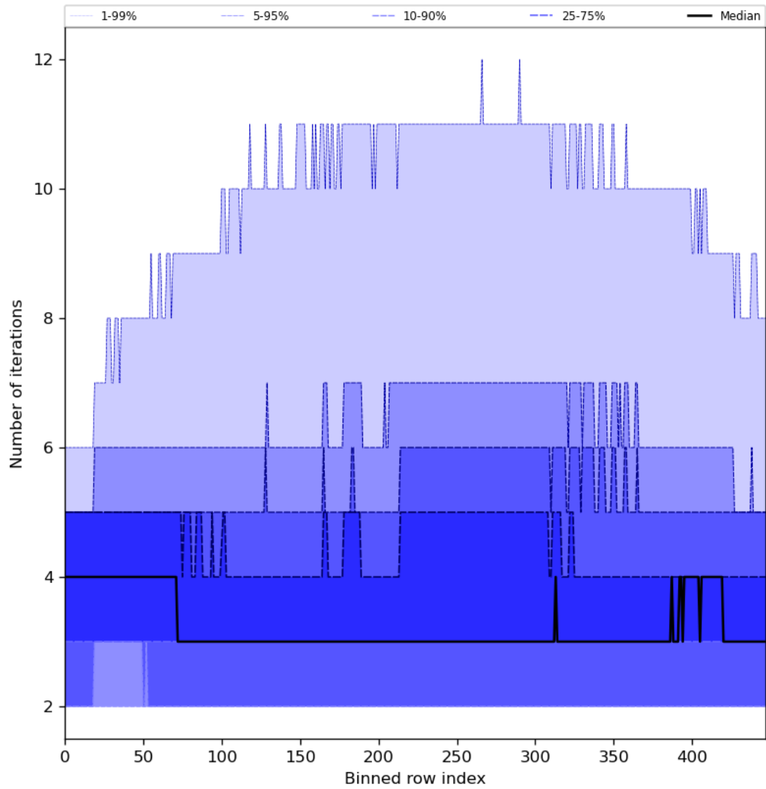
Figure 56: Along track statistics of “Number of iterations” for 2023-12-07 to 2023-12-09
