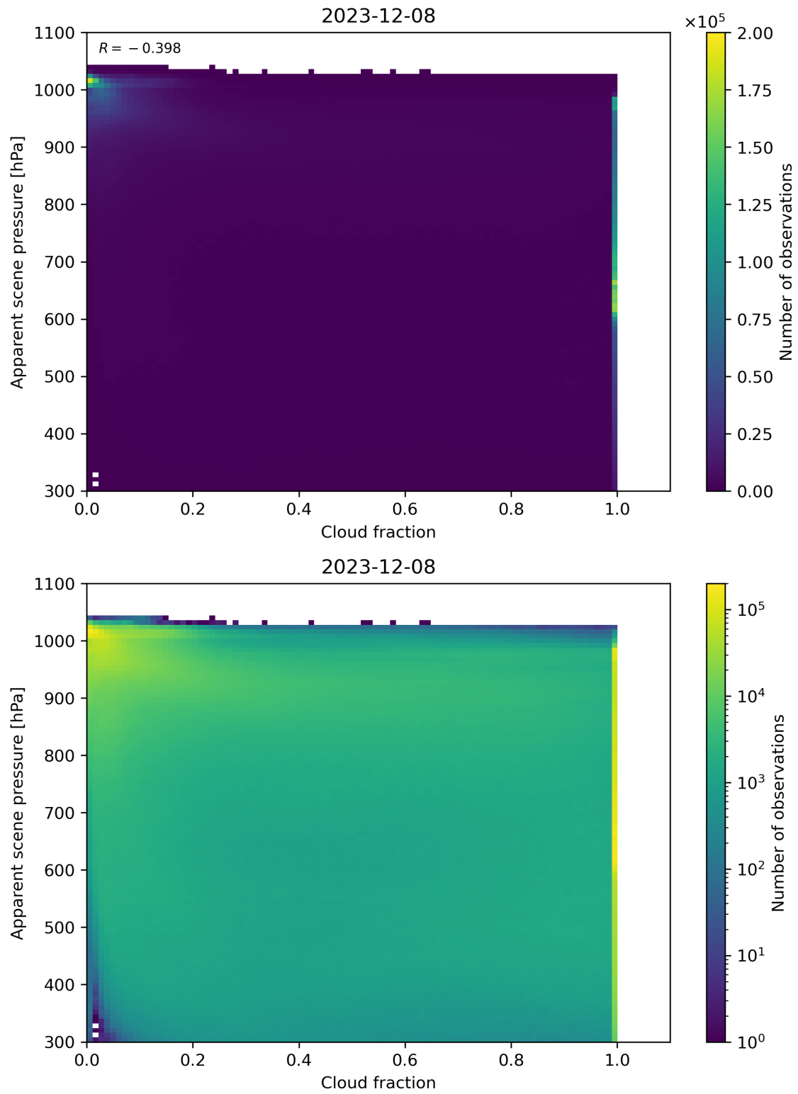
Figure 70: Scatter density plot of “Cloud fraction” against “Apparent scene pressure” for 2023-12-07 to 2023-12-09.
