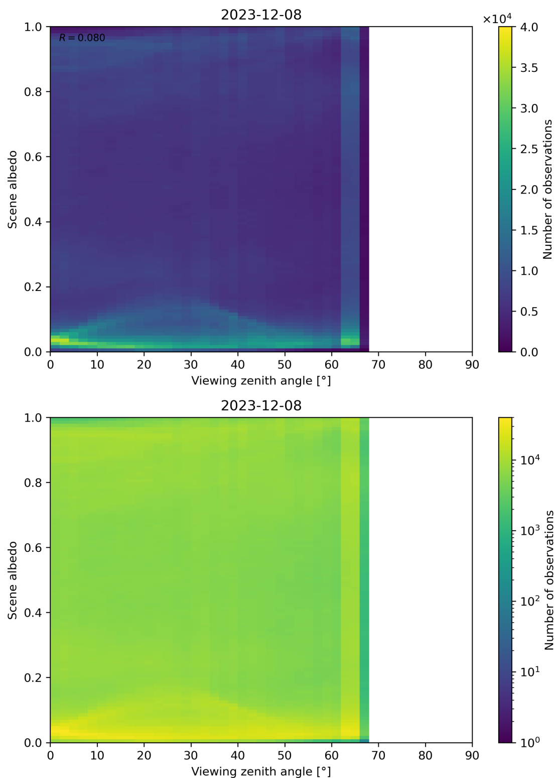
Figure 126: Scatter density plot of “Viewing zenith angle” against “Scene albedo” for 2023-12-07 to 2023-12-09.
