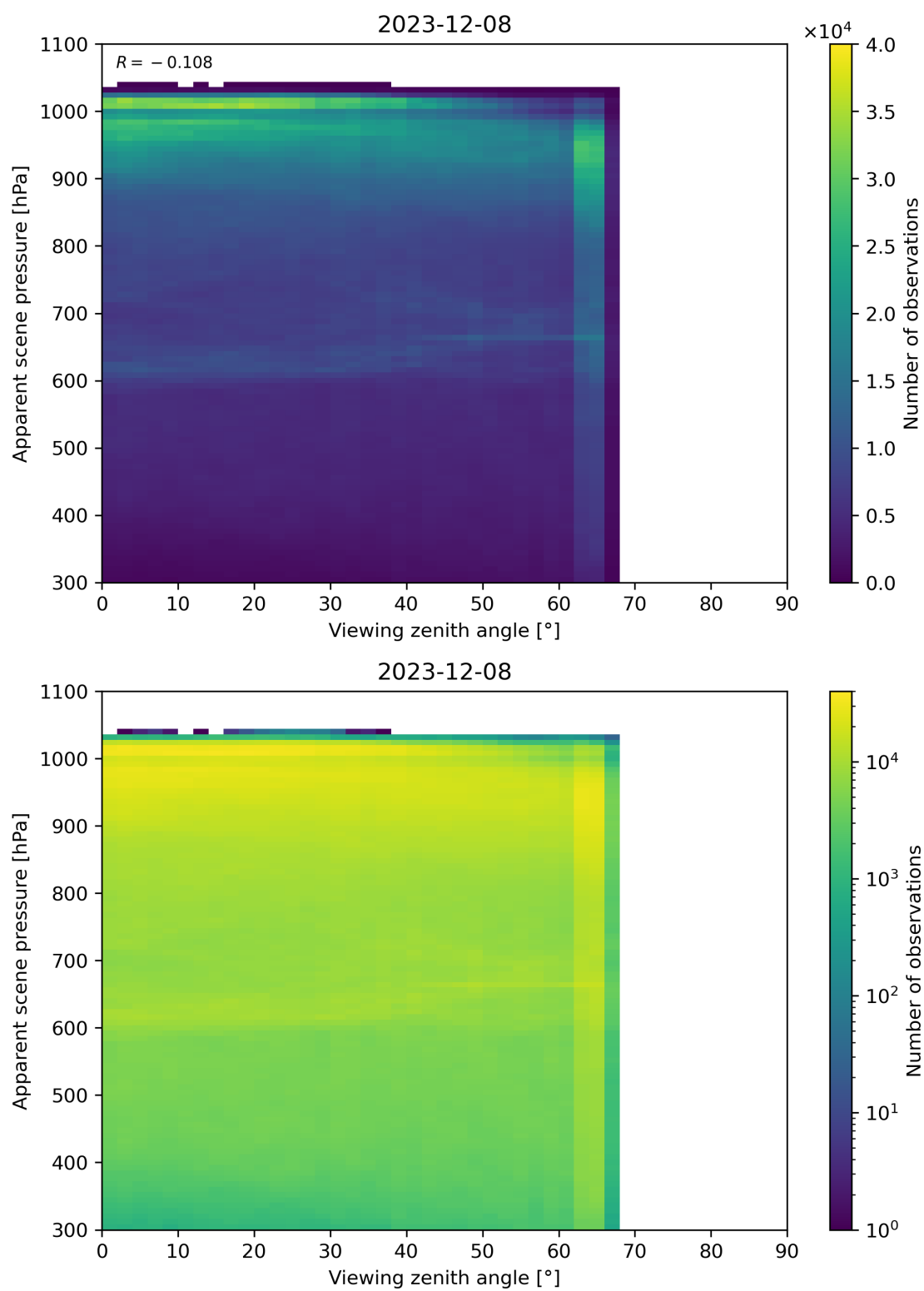
Figure 118: Scatter density plot of “Viewing zenith angle” against “Apparent scene pressure” for 2023-12-07 to 2023-12-09.
