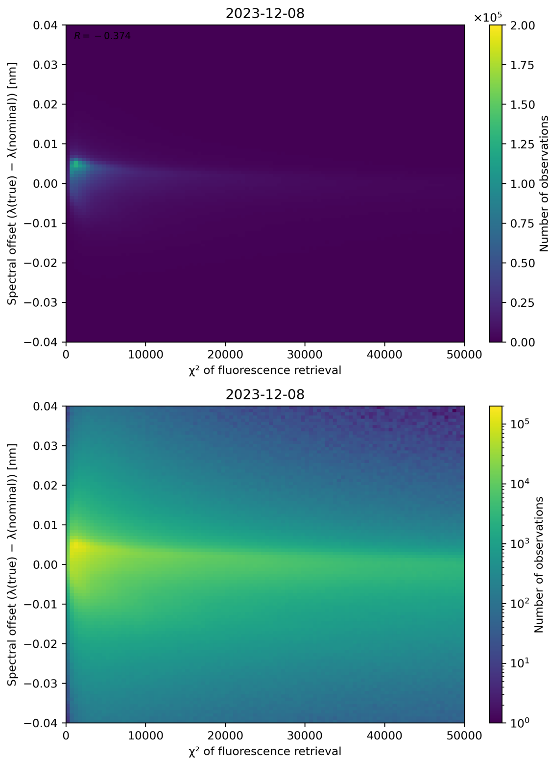
Figure 69: Scatter density plot of " \chi^2 of fluorescence retrieval" against "Spectral offset ( \lambda(\text{true}) - \lambda(\text{nominal}) )" for 2023-12-07 to 2023-12-09.
