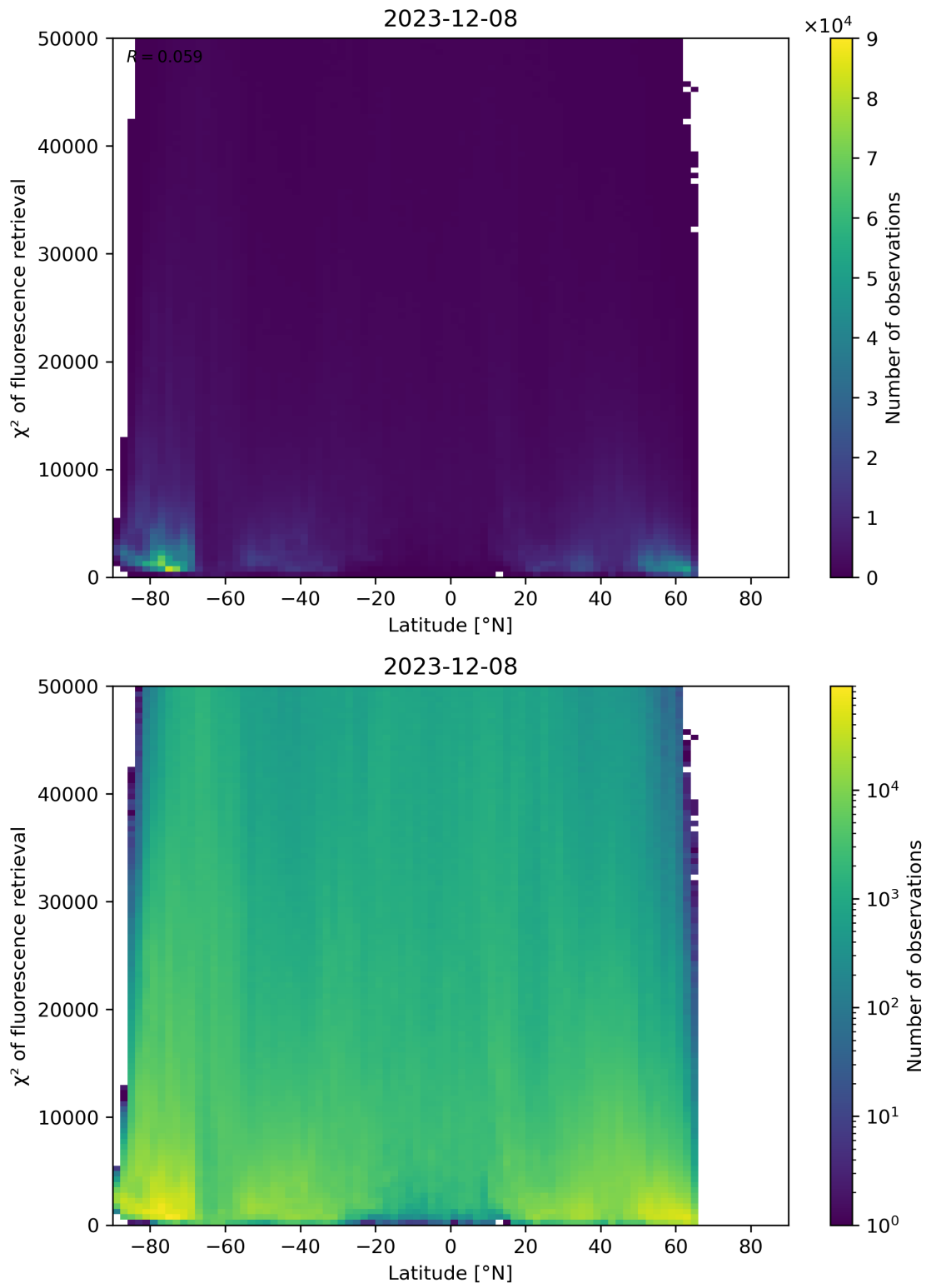
Figure 89: Scatter density plot of “Latitude” against “ \chi^2 of fluorescence retrieval” for 2023-12-07 to 2023-12-09.
