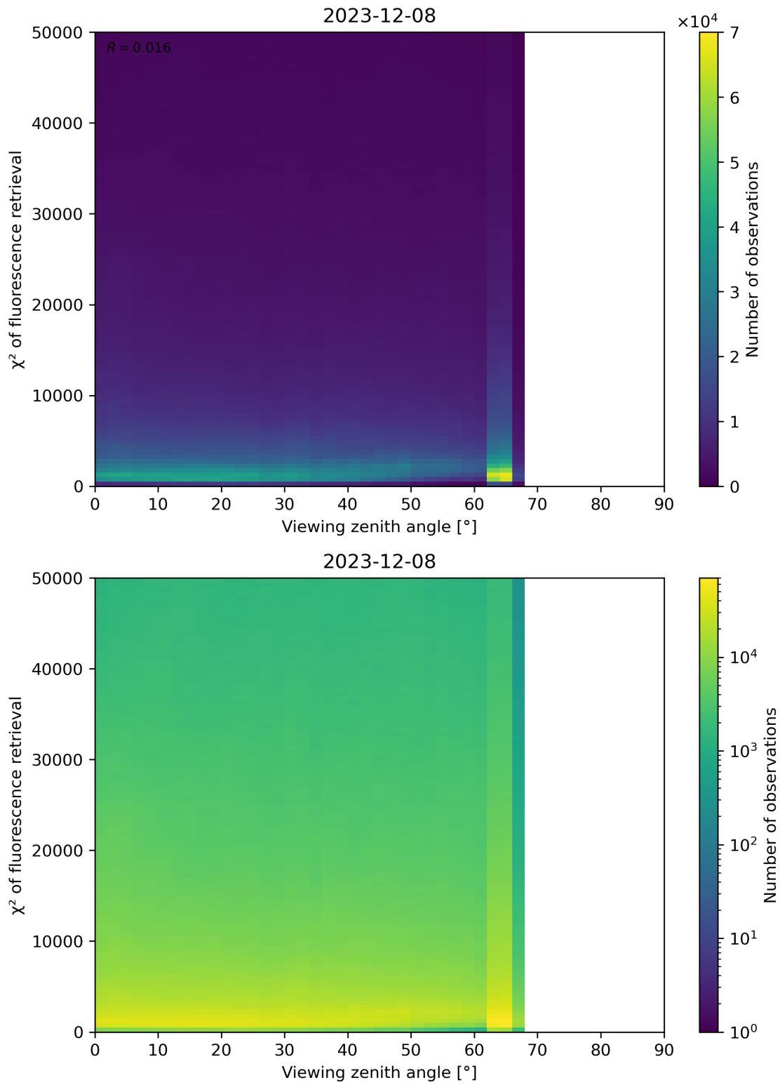
Figure 119: Scatter density plot of “Viewing zenith angle” against “ \chi^2 of fluorescence retrieval” for 2023-12-07 to 2023-12-09.
