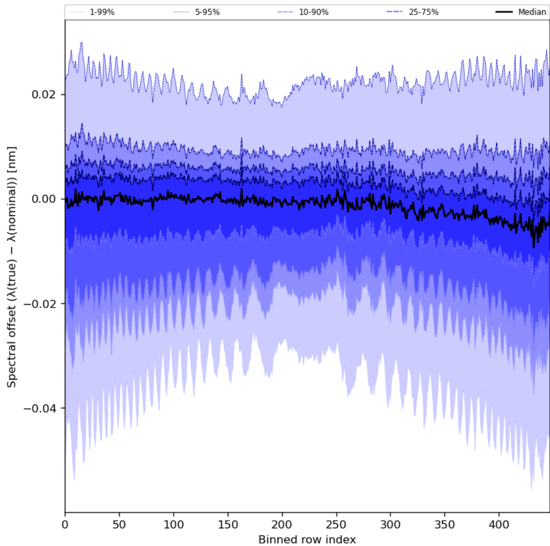
Figure 62: Along track statistics of “Spectral offset ( \lambda(\text{true}) - \lambda(\text{nominal}) )” for 2023-12-07 to 2023-12-09
