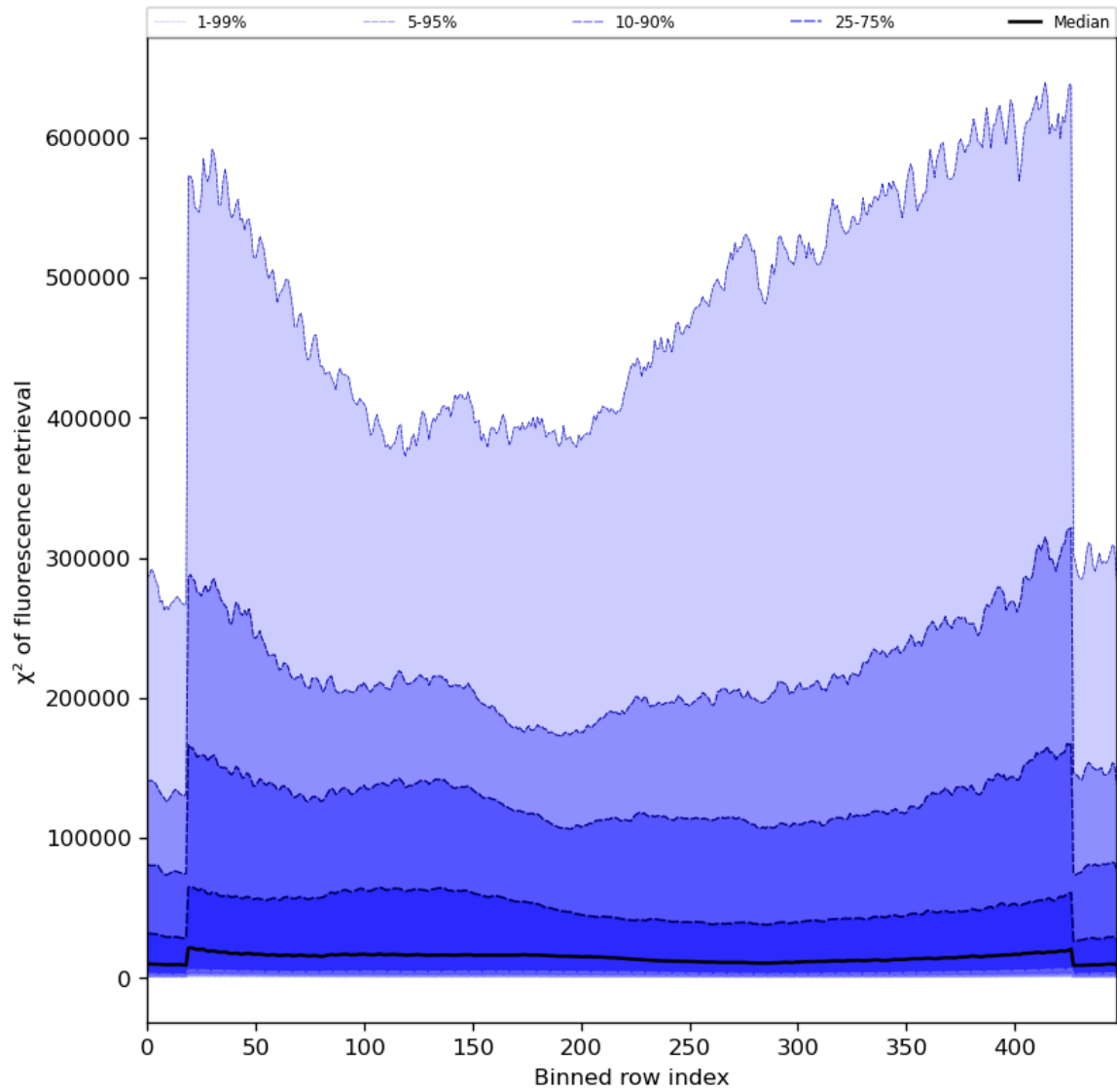
Figure 59: Along track statistics of “ \chi^2 of fluorescence retrieval” for 2023-12-07 to 2023-12-09
