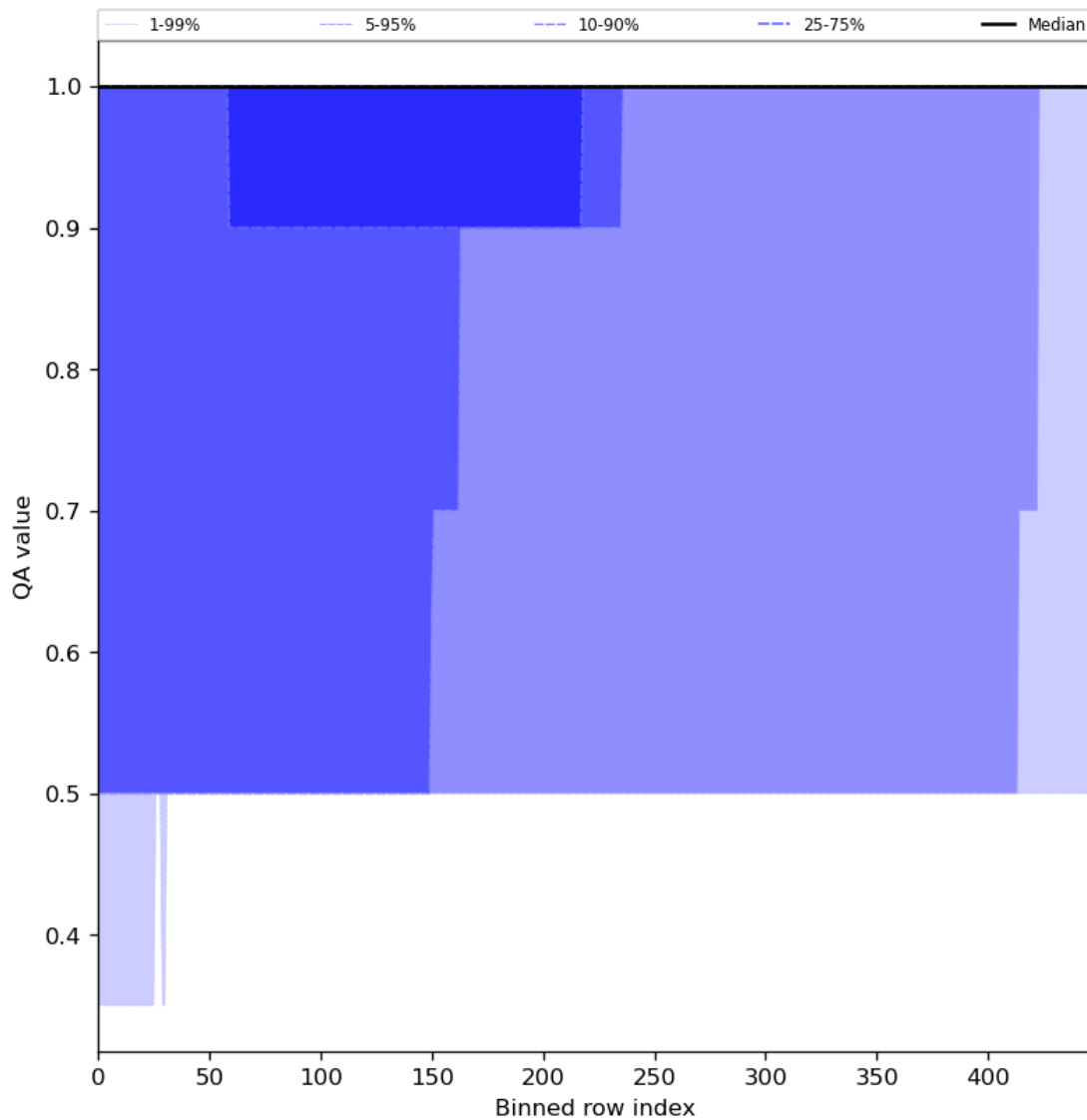
Figure 46: Along track statistics of “QA value” for 2023-12-07 to 2023-12-09
