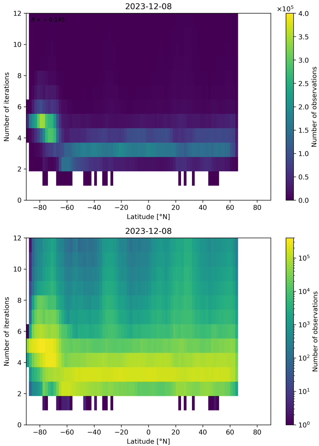
Figure 93: Scatter density plot of “Latitude” against “Number of iterations” for 2023-12-07 to 2023-12-09.
