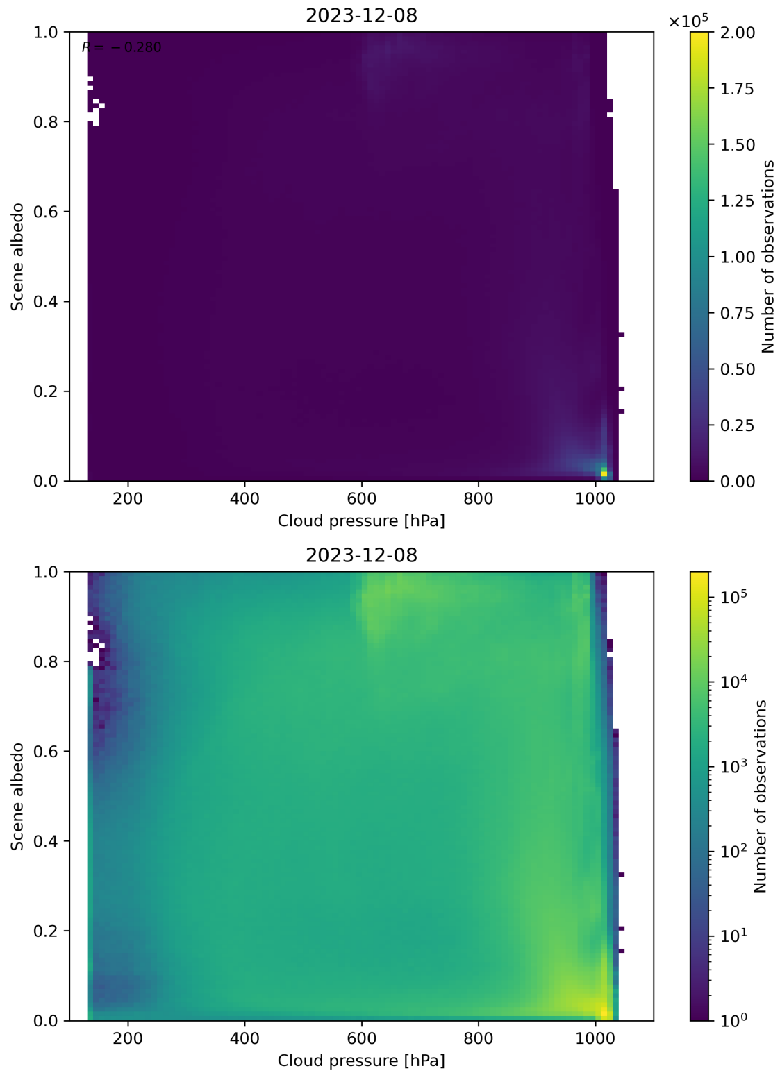
Figure 83: Scatter density plot of “Cloud pressure” against “Scene albedo” for 2023-12-07 to 2023-12-09.
