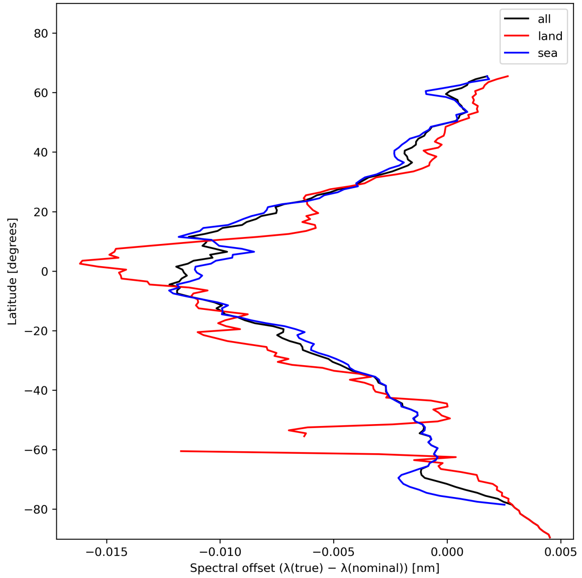
Figure 28: Zonal average of “Spectral offset ( \lambda(\text{true}) - \lambda(\text{nominal}) )” for 2023-12-07 to 2023-12-09.
