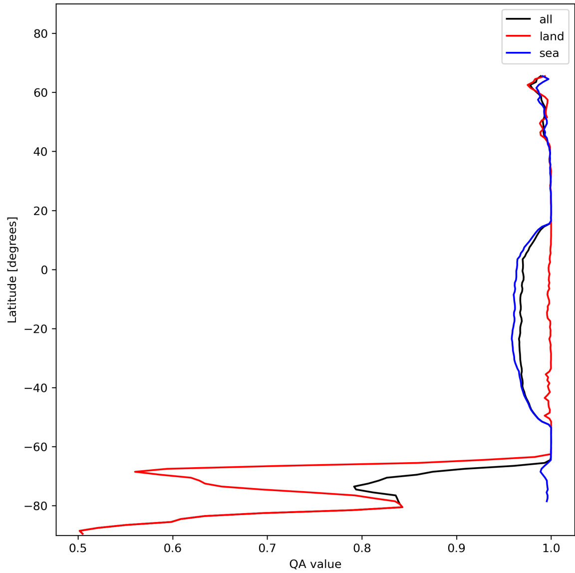
Figure 12: Zonal average of “QA value” for 2023-12-07 to 2023-12-09.
