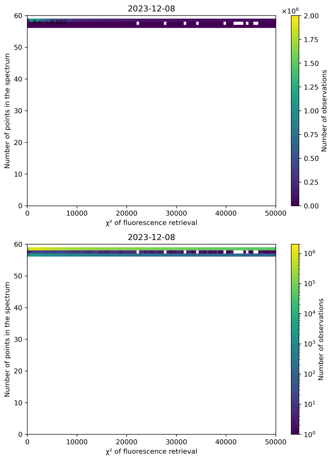
Figure 68: Scatter density plot of " \chi^2 of fluorescence retrieval" against "Number of points in the spectrum" for 2023-12-07 to 2023-12-09.
