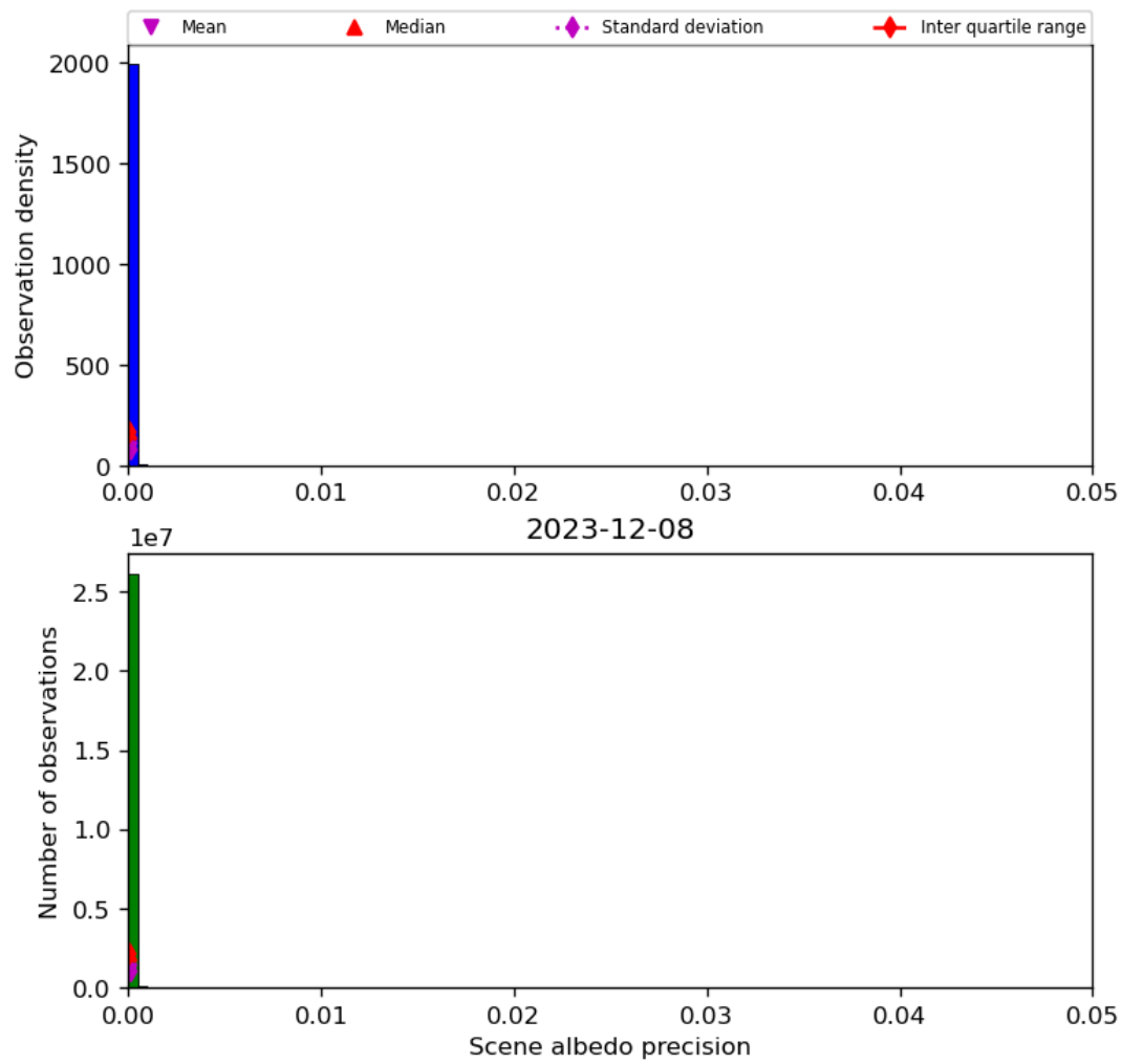
Figure 35: Histogram of “Scene albedo precision” for 2023-12-07 to 2023-12-09
