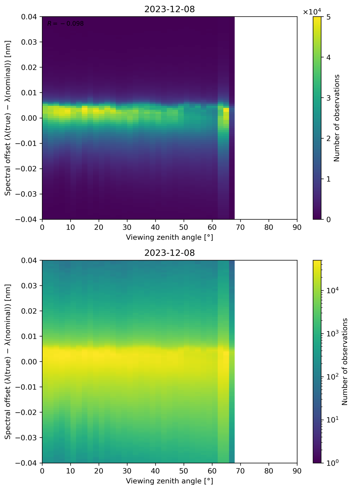
Figure 128: Scatter density plot of “Viewing zenith angle” against “Spectral offset ( \lambda(\text{true}) - \lambda(\text{nominal}) )” for 2023-12-07 to 2023-12-09.
