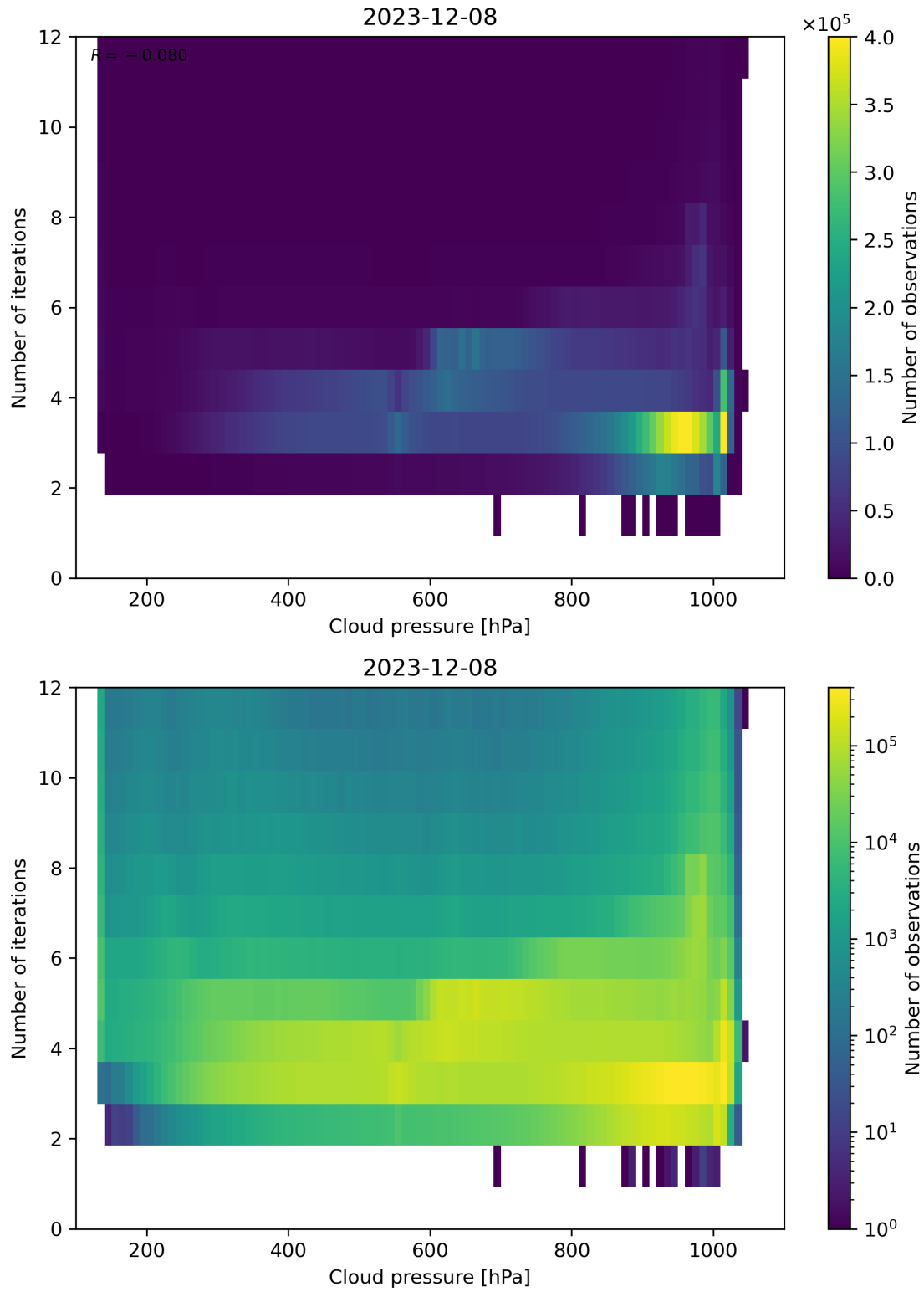
Figure 81: Scatter density plot of “Cloud pressure” against “Number of iterations” for 2023-12-07 to 2023-12-09.
