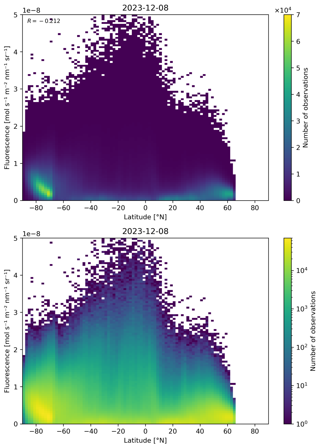
Figure 92: Scatter density plot of “Latitude” against “Fluorescence” for 2023-12-07 to 2023-12-09.
