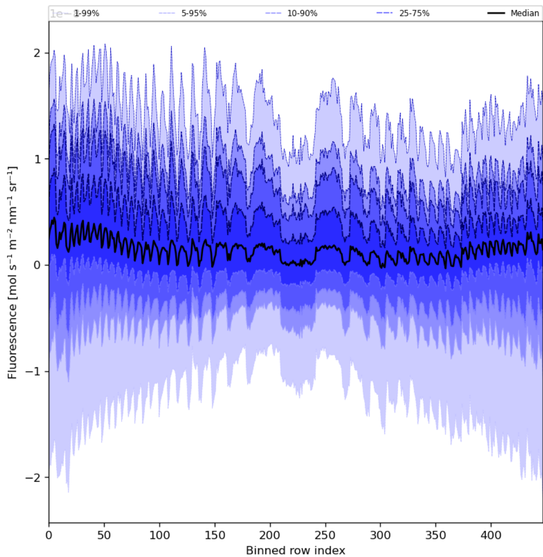
Figure 57: Along track statistics of “Fluorescence” for 2023-12-07 to 2023-12-09
