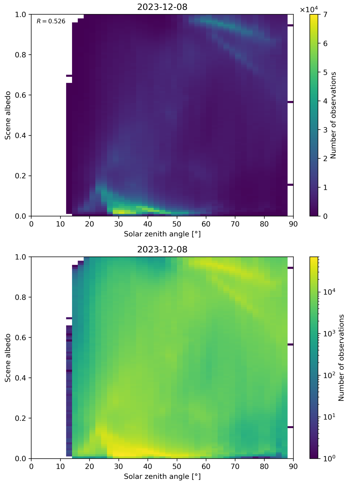
Figure 116: Scatter density plot of “Solar zenith angle” against “Scene albedo” for 2023-12-07 to 2023-12-09.
