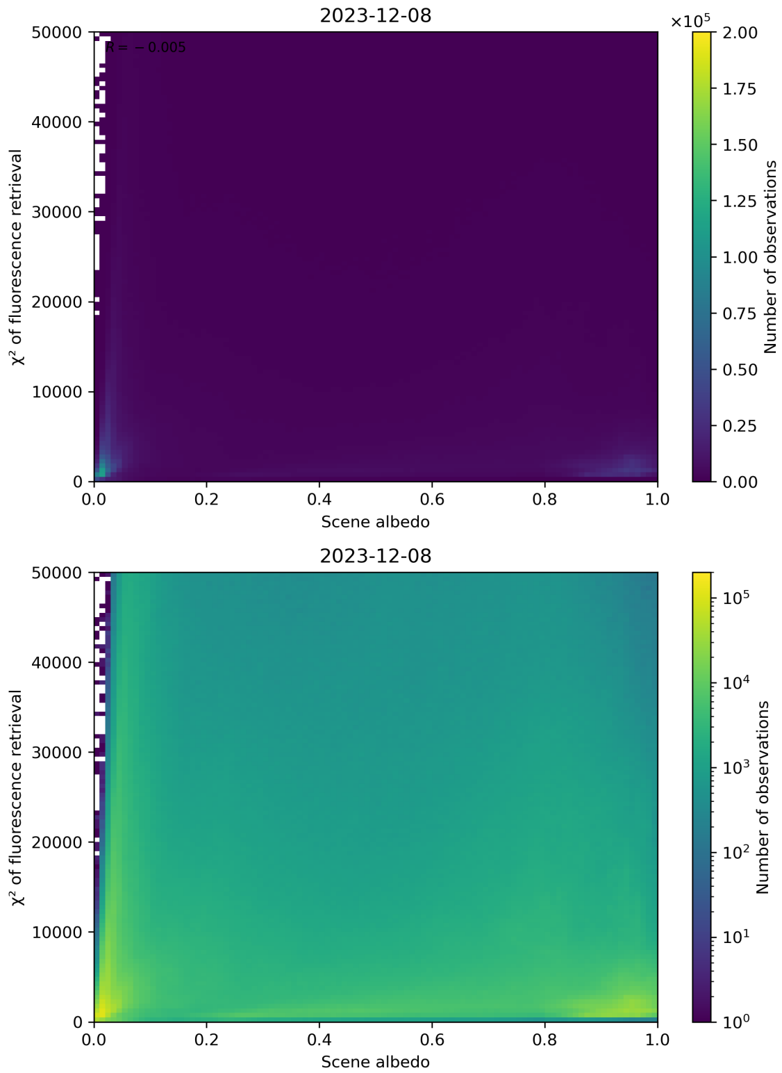
Figure 103: Scatter density plot of “Scene albedo” against “ \chi^2 of fluorescence retrieval” for 2023-12-07 to 2023-12-09.
