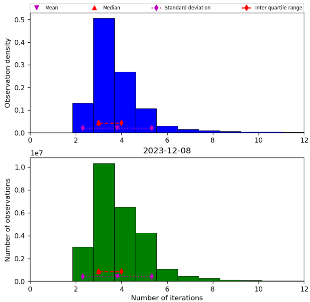
Figure 39: Histogram of “Number of iterations” for 2023-12-07 to 2023-12-09
