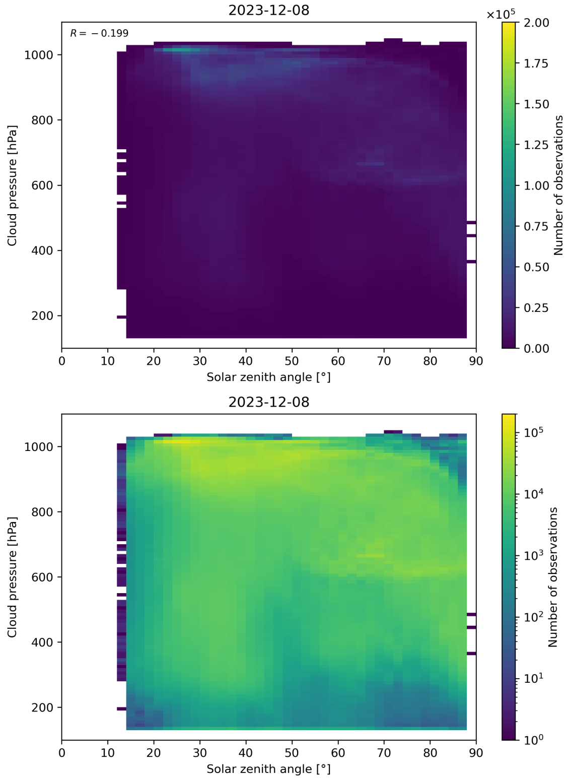
Figure 111: Scatter density plot of “Solar zenith angle” against “Cloud pressure” for 2023-12-07 to 2023-12-09.
