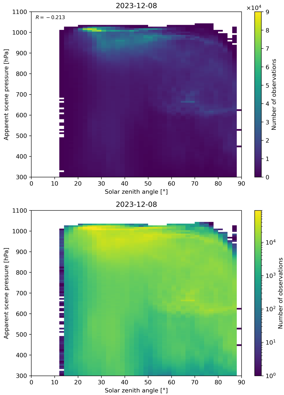
Figure 108: Scatter density plot of “Solar zenith angle” against “Apparent scene pressure” for 2023-12-07 to 2023-12-09.
