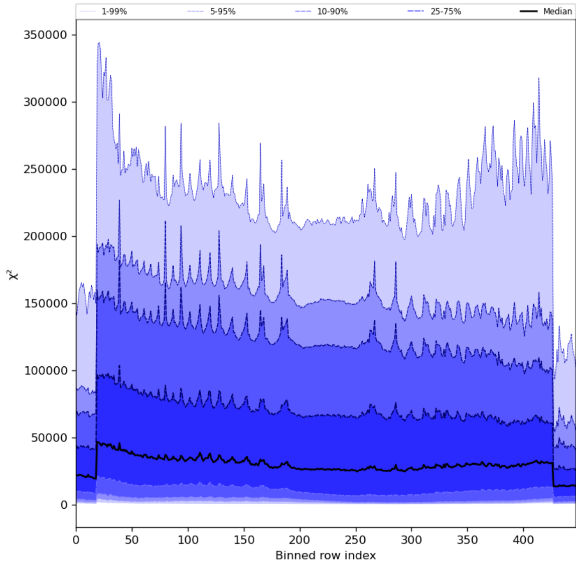
Figure 55: Along track statistics of “ \chi^2 ” for 2023-12-07 to 2023-12-09
