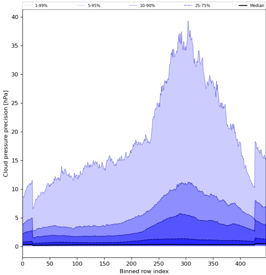
Figure 48: Along track statistics of “Cloud pressure precision” for 2023-12-07 to 2023-12-09
