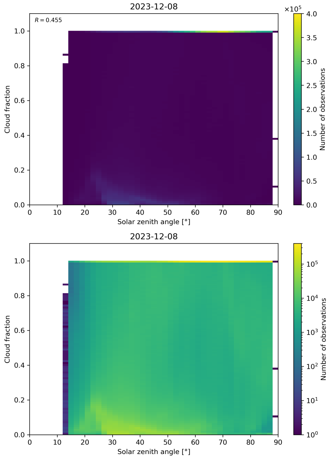
Figure 110: Scatter density plot of “Solar zenith angle” against “Cloud fraction” for 2023-12-07 to 2023-12-09.
