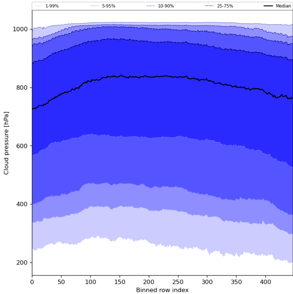
Figure 47: Along track statistics of “Cloud pressure” for 2023-12-07 to 2023-12-09
