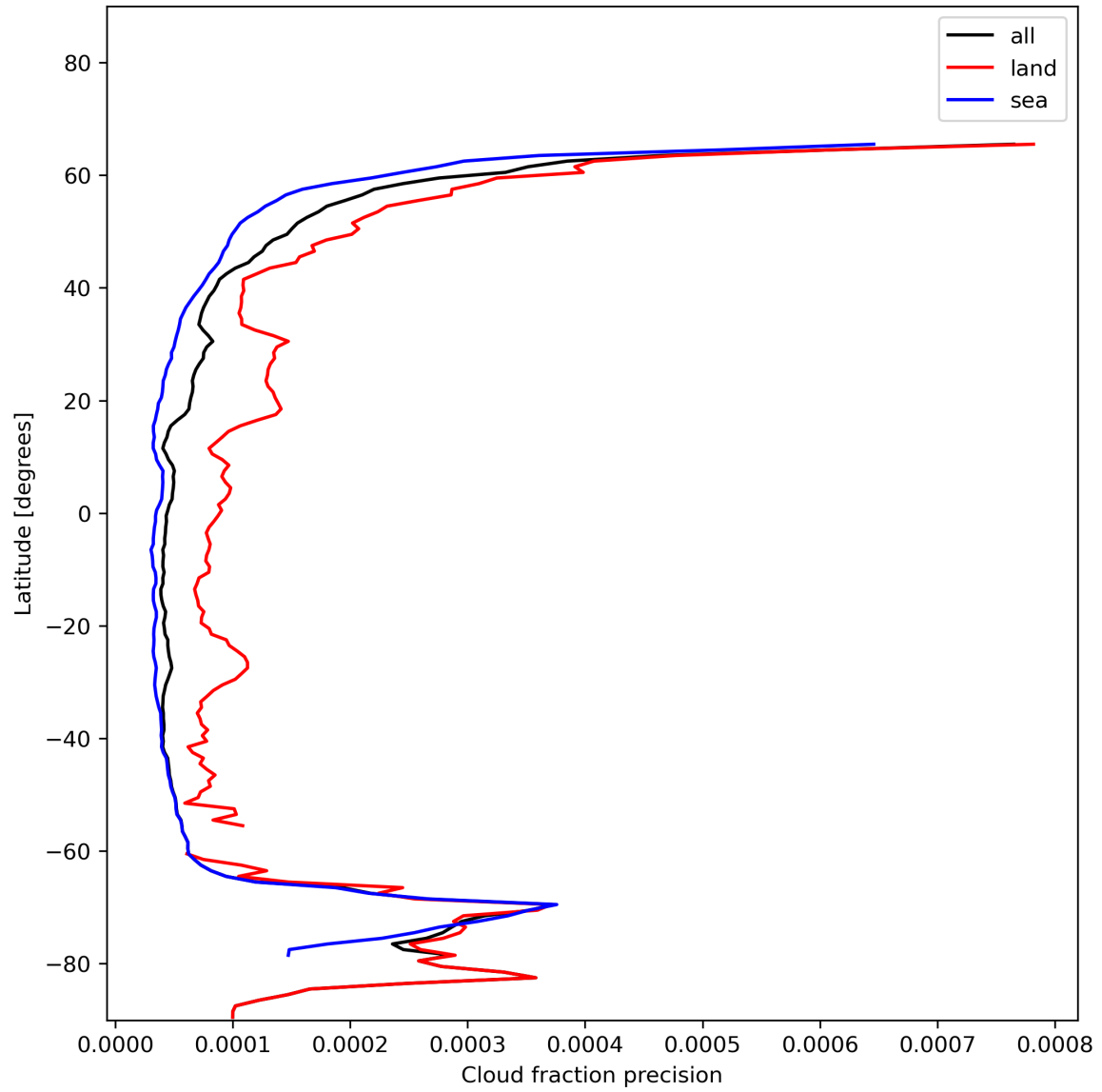
Figure 16: Zonal average of “Cloud fraction precision” for 2023-12-07 to 2023-12-09.
