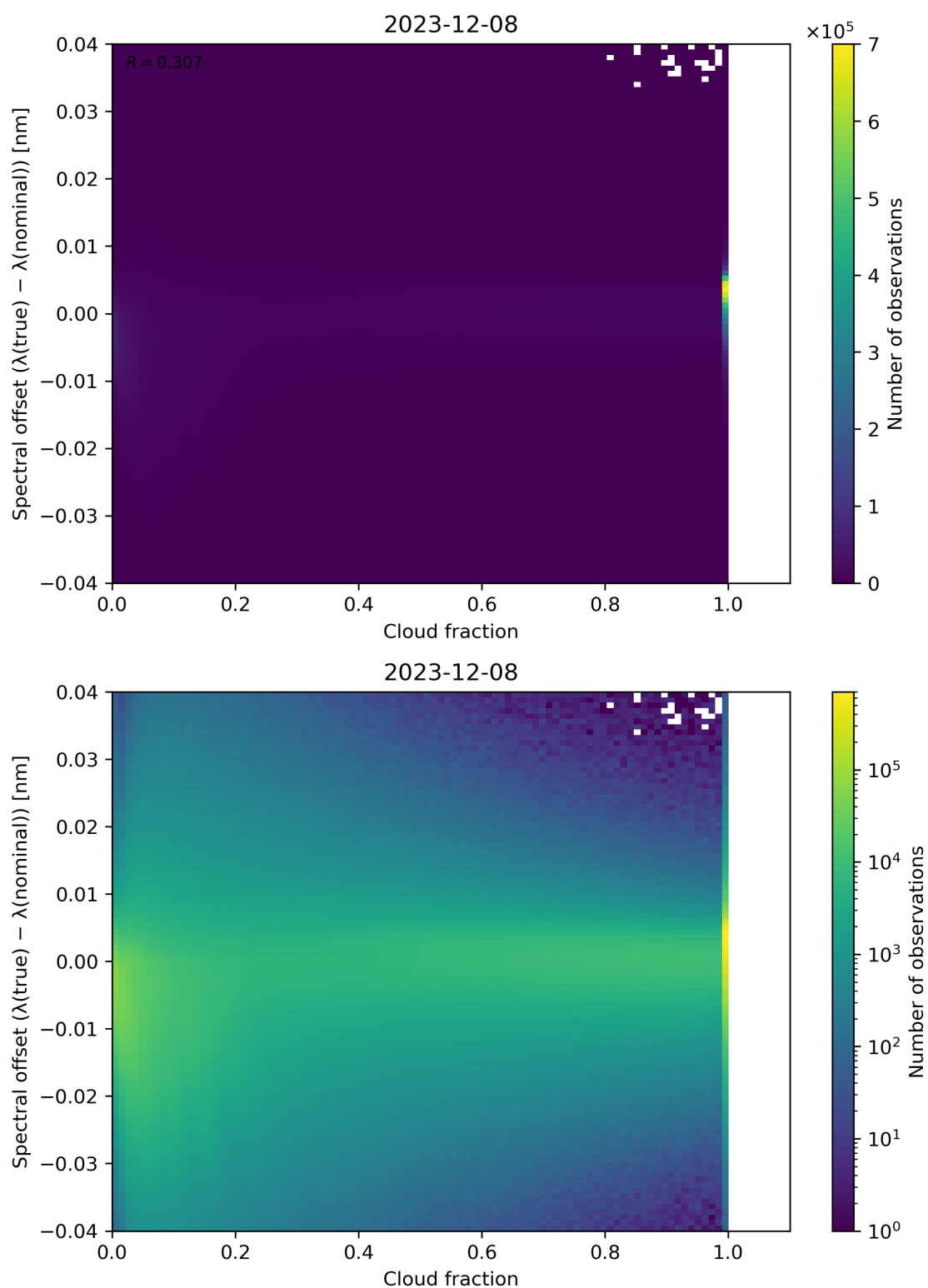
Figure 76: Scatter density plot of “Cloud fraction” against “Spectral offset ( \lambda(\text{true}) - \lambda(\text{nominal}) )” for 2023-12-07 to 2023-12-09.
