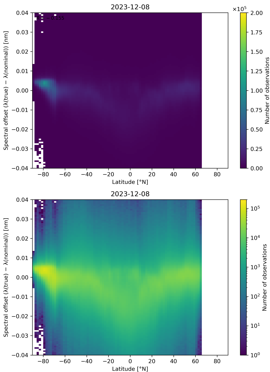
Figure 96: Scatter density plot of “Latitude” against “Spectral offset ( \lambda(\text{true}) - \lambda(\text{nominal}) )” for 2023-12-07 to 2023-12-09.
