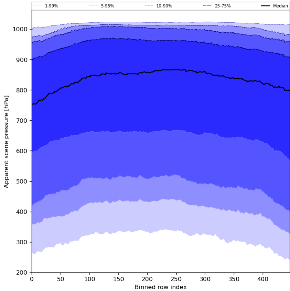
Figure 53: Along track statistics of “Apparent scene pressure” for 2023-12-07 to 2023-12-09
