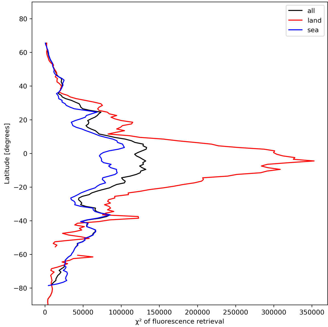
Figure 25: Zonal average of “ \chi^2 of fluorescence retrieval” for 2023-12-09 to 2023-12-11.
