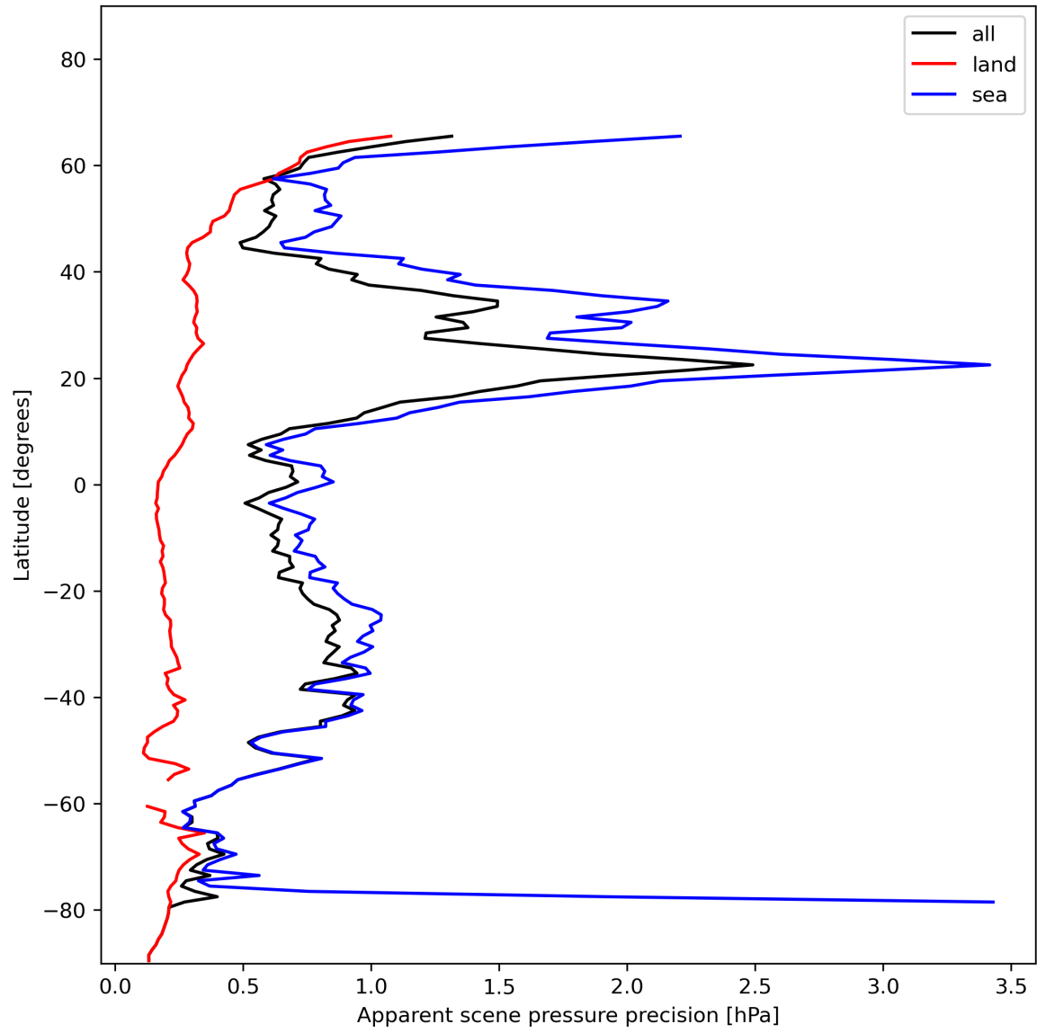
Figure 20: Zonal average of “Apparent scene pressure precision” for 2023-12-09 to 2023-12-11.
