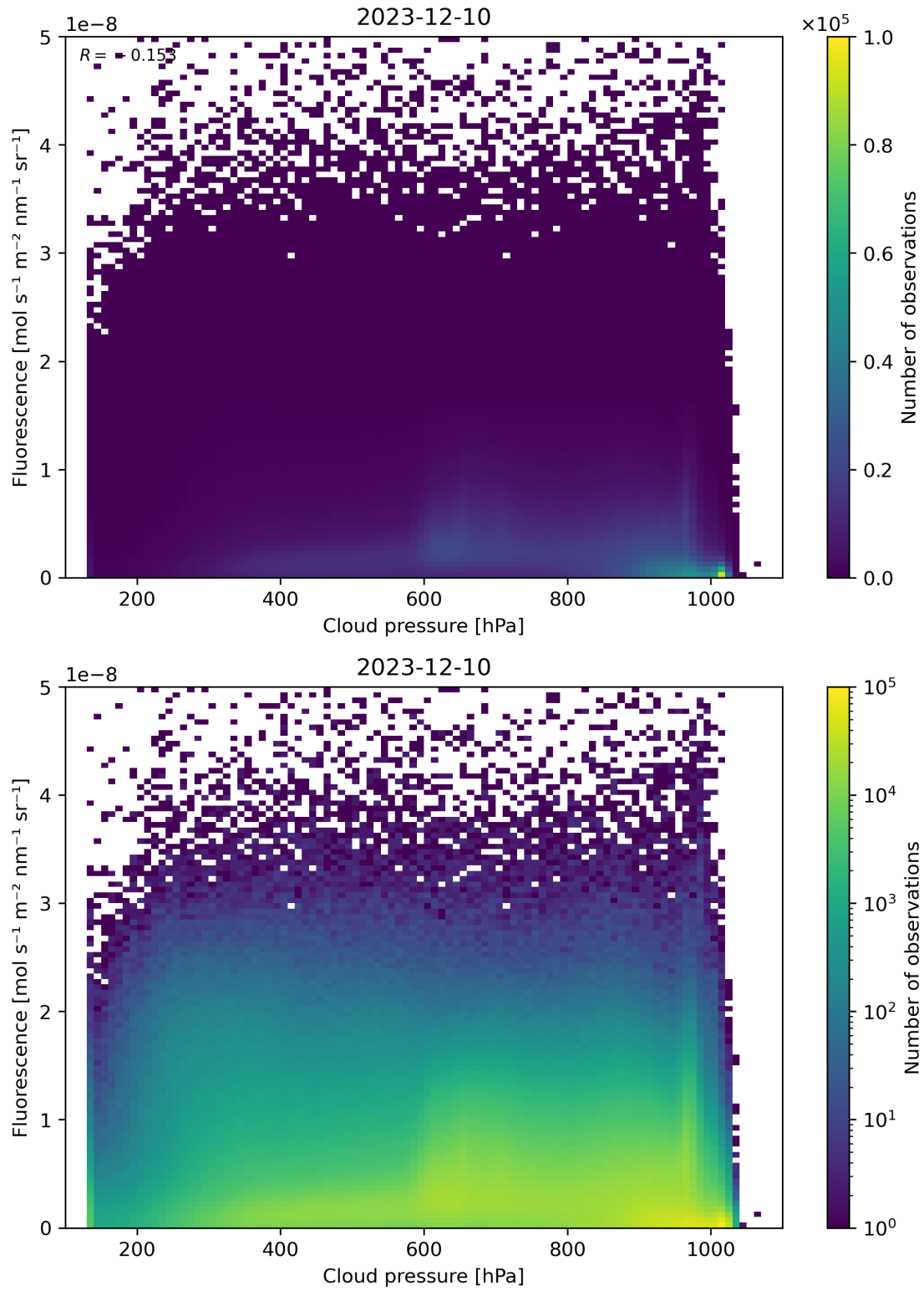
Figure 80: Scatter density plot of “Cloud pressure” against “Fluorescence” for 2023-12-09 to 2023-12-11.
