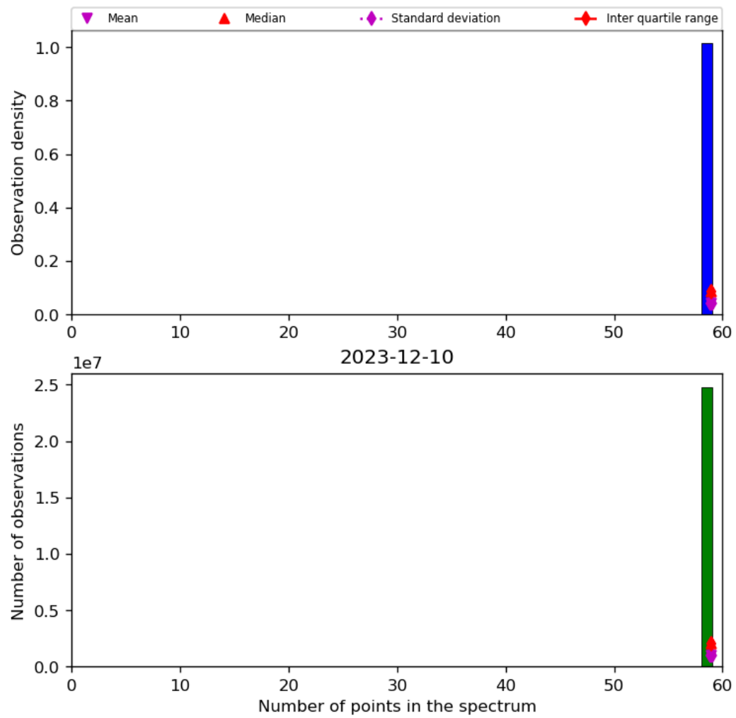
Figure 44: Histogram of “Number of points in the spectrum” for 2023-12-09 to 2023-12-11
