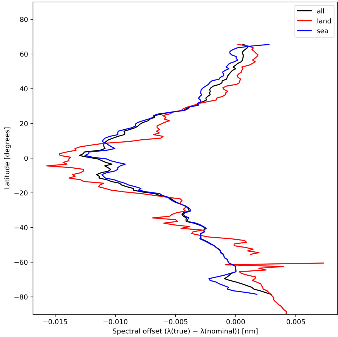
Figure 28: Zonal average of “Spectral offset ( \lambda(\text{true}) - \lambda(\text{nominal}) )” for 2023-12-09 to 2023-12-11.
