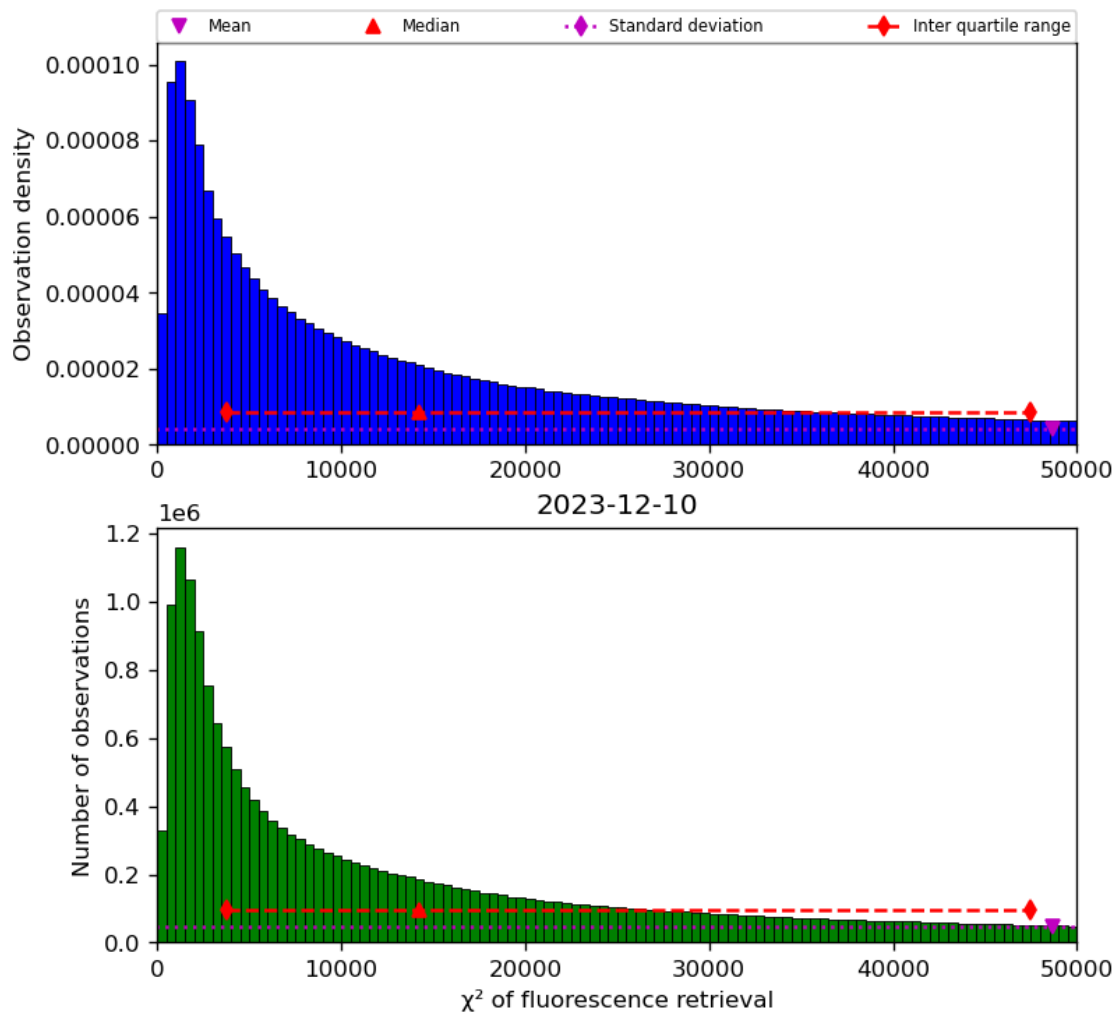
Figure 42: Histogram of “ \chi^2 of fluorescence retrieval” for 2023-12-09 to 2023-12-11
