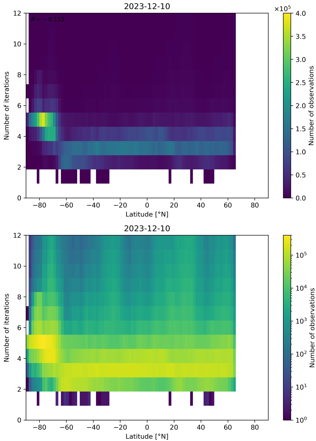
Figure 93: Scatter density plot of “Latitude” against “Number of iterations” for 2023-12-09 to 2023-12-11.
