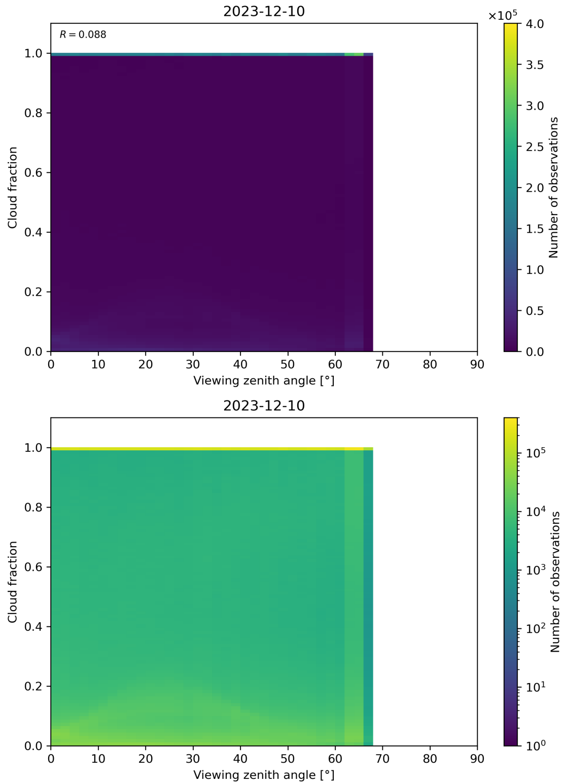
Figure 120: Scatter density plot of “Viewing zenith angle” against “Cloud fraction” for 2023-12-09 to 2023-12-11.
