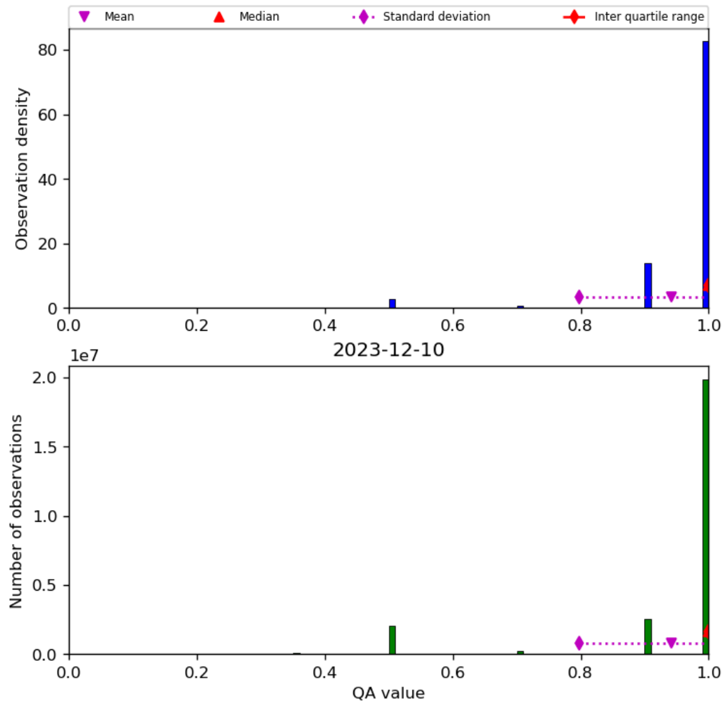
Figure 29: Histogram of “QA value” for 2023-12-09 to 2023-12-11
