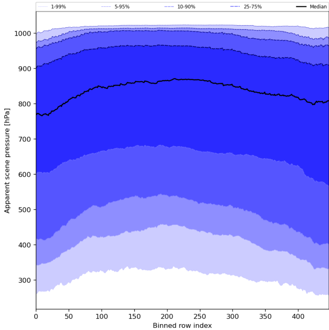
Figure 53: Along track statistics of “Apparent scene pressure” for 2023-12-09 to 2023-12-11
