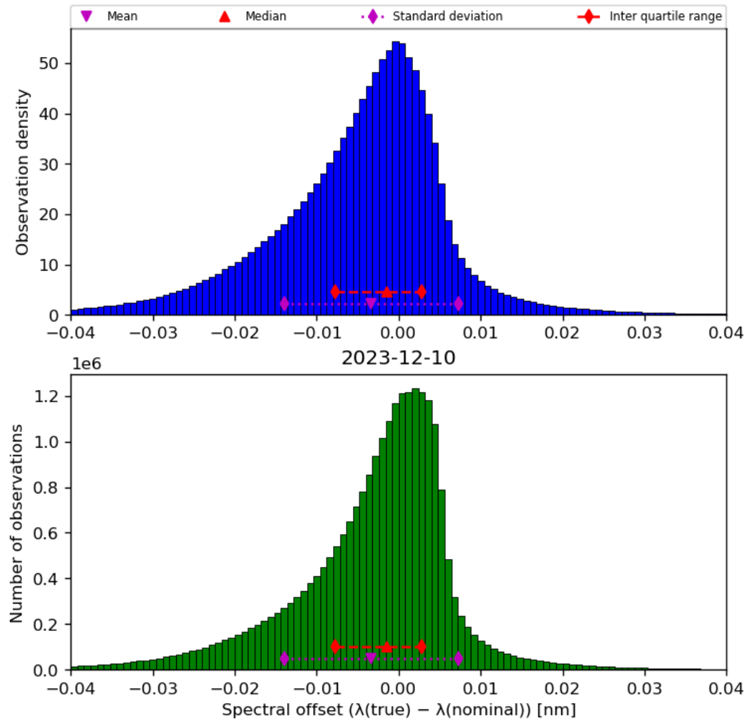
Figure 45: Histogram of “Spectral offset ( \lambda(\text{true}) - \lambda(\text{nominal}) )” for 2023-12-09 to 2023-12-11
