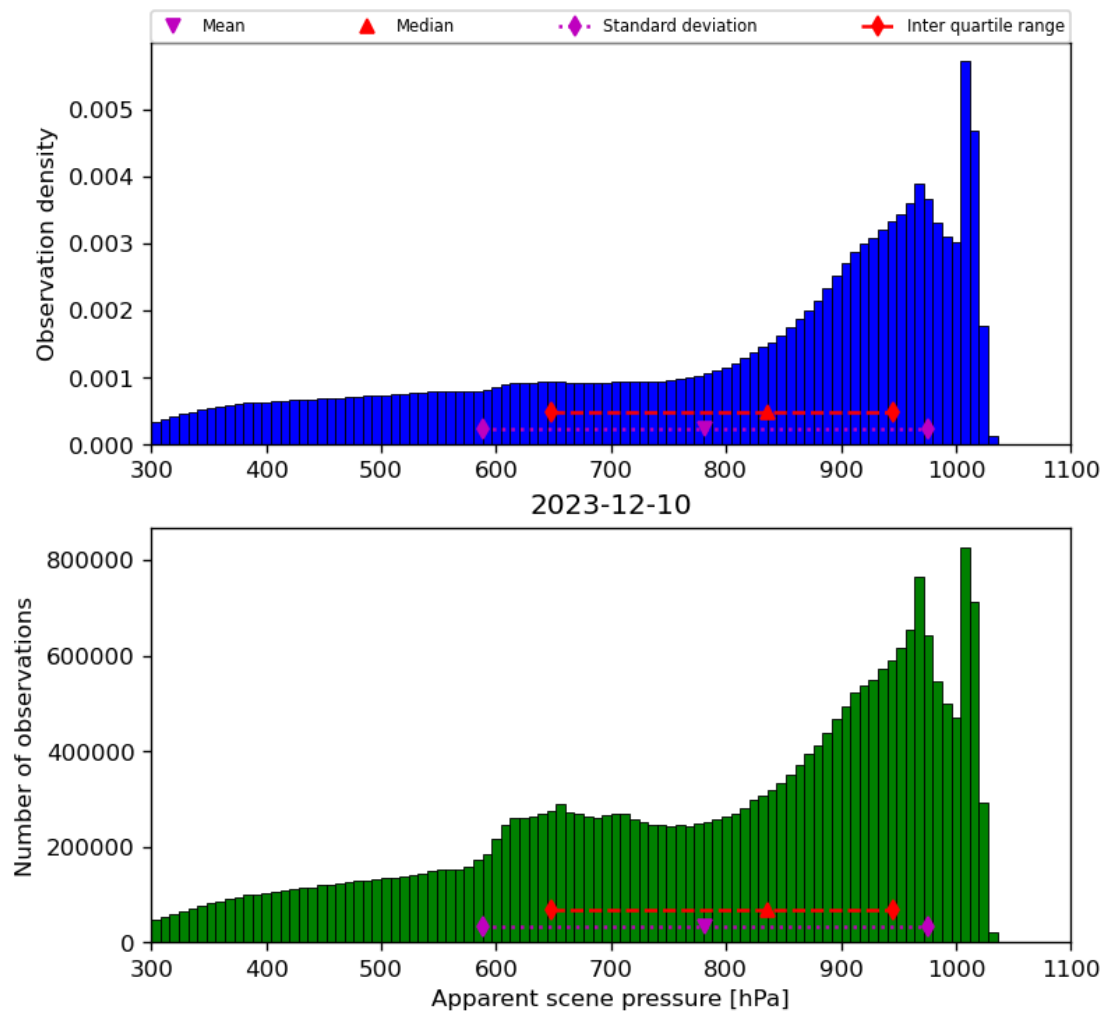
Figure 36: Histogram of “Apparent scene pressure” for 2023-12-09 to 2023-12-11
