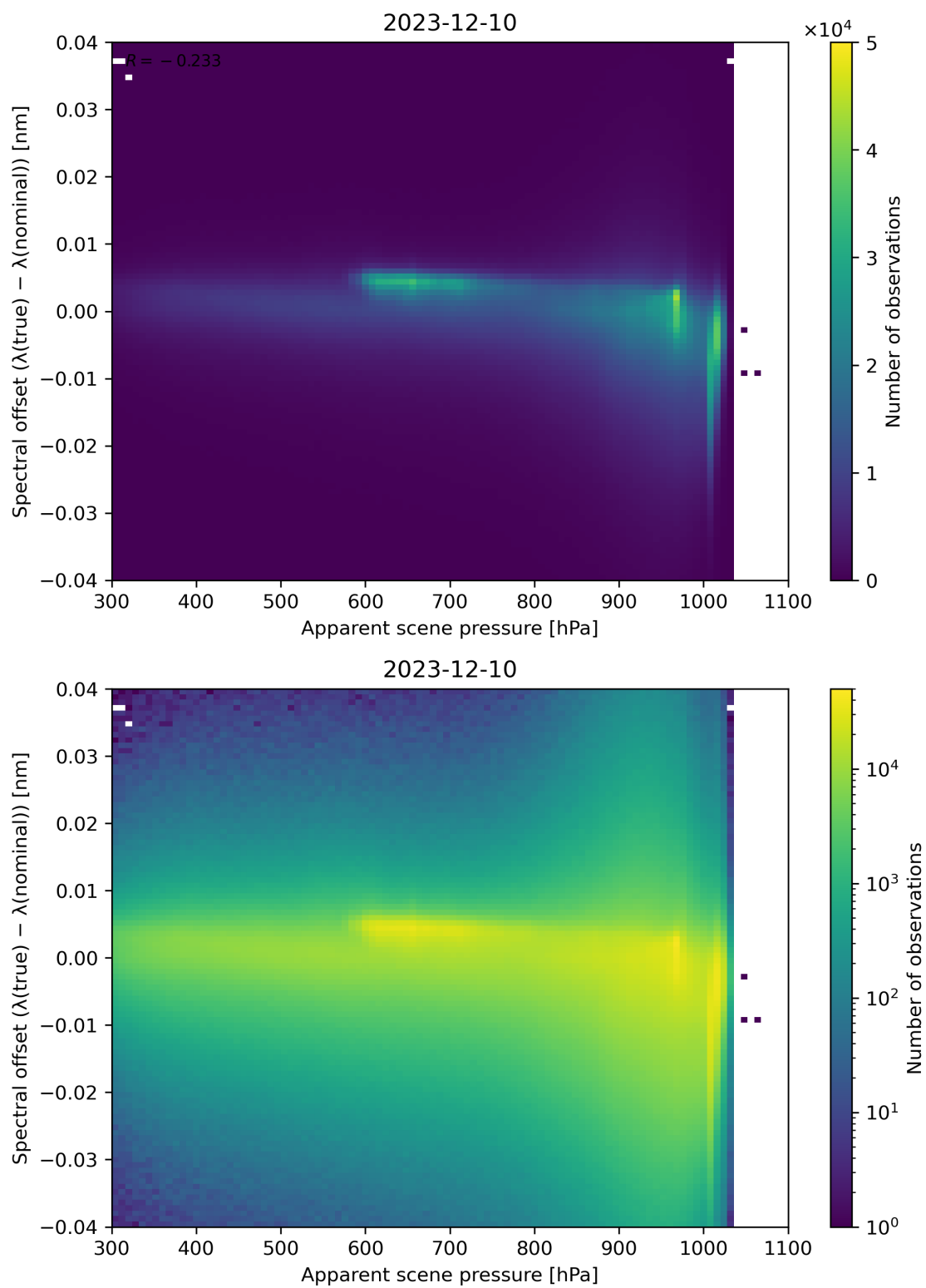
Figure 67: Scatter density plot of “Apparent scene pressure” against “Spectral offset ( \lambda(\text{true}) - \lambda(\text{nominal}) )” for 2023-12-09 to 2023-12-11.
