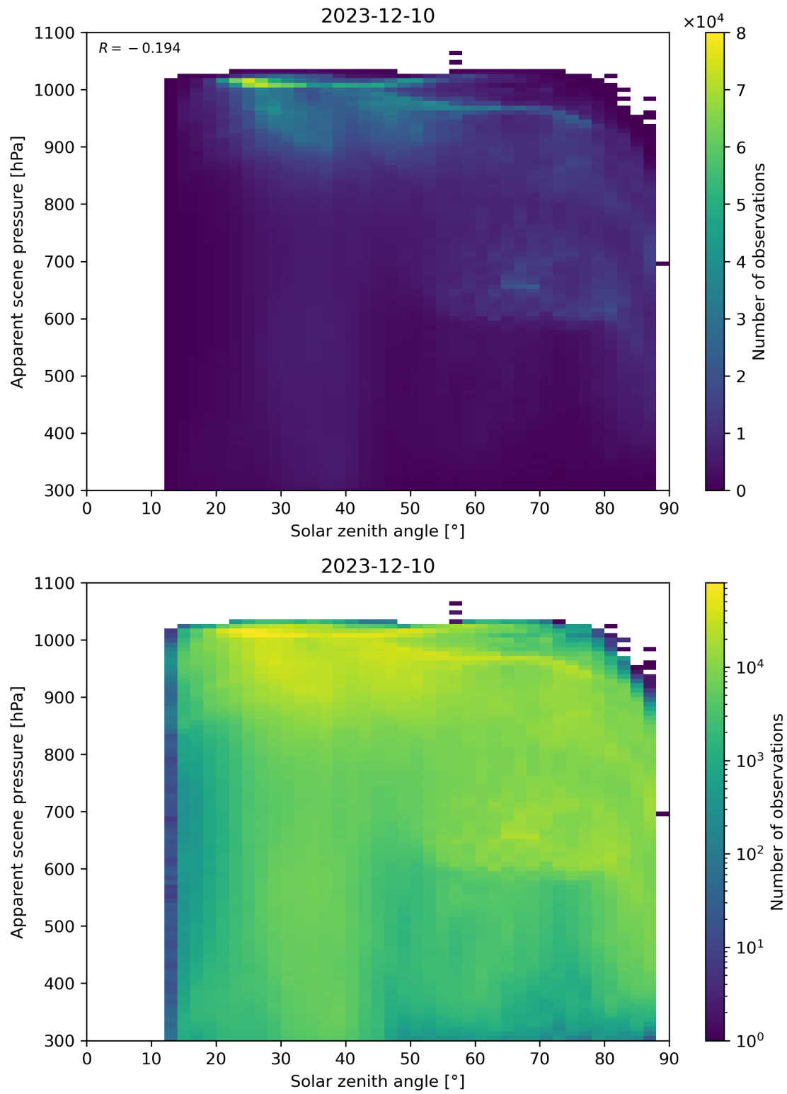
Figure 108: Scatter density plot of “Solar zenith angle” against “Apparent scene pressure” for 2023-12-09 to 2023-12-11.
