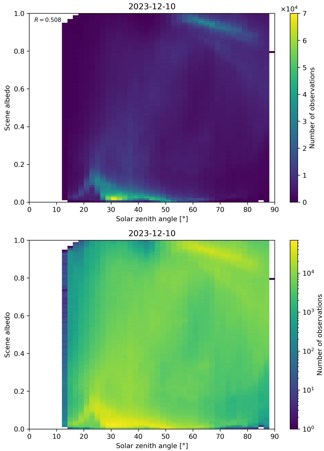
Figure 116: Scatter density plot of “Solar zenith angle” against “Scene albedo” for 2023-12-09 to 2023-12-11.
