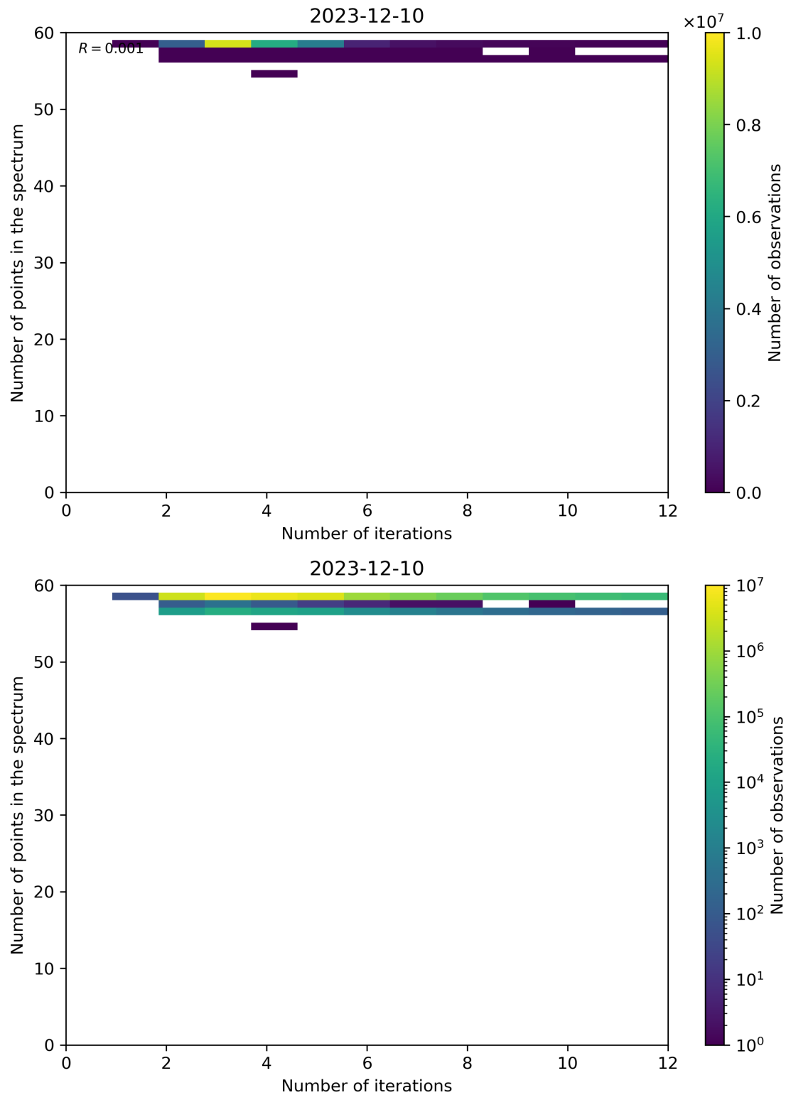
Figure 99: Scatter density plot of “Number of iterations” against “Number of points in the spectrum” for 2023-12-09 to 2023-12-11.
