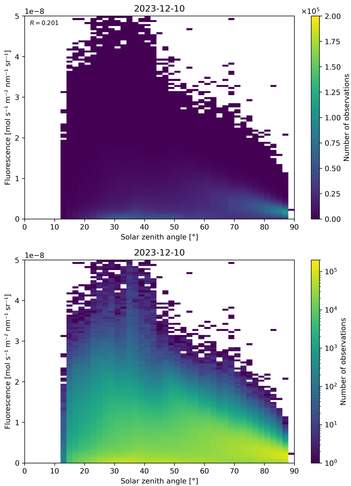
Figure 112: Scatter density plot of “Solar zenith angle” against “Fluorescence” for 2023-12-09 to 2023-12-11.
