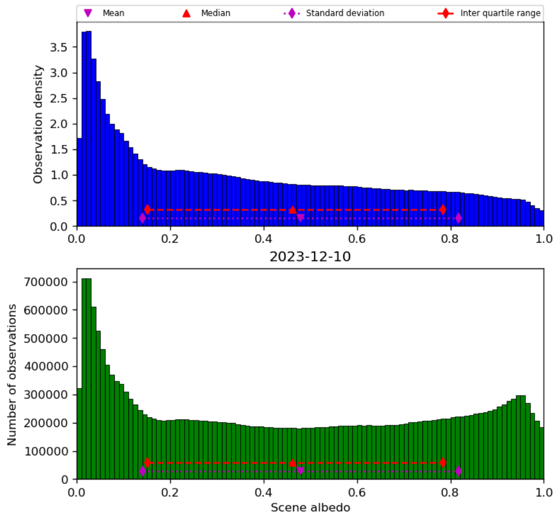
Figure 34: Histogram of “Scene albedo” for 2023-12-09 to 2023-12-11
