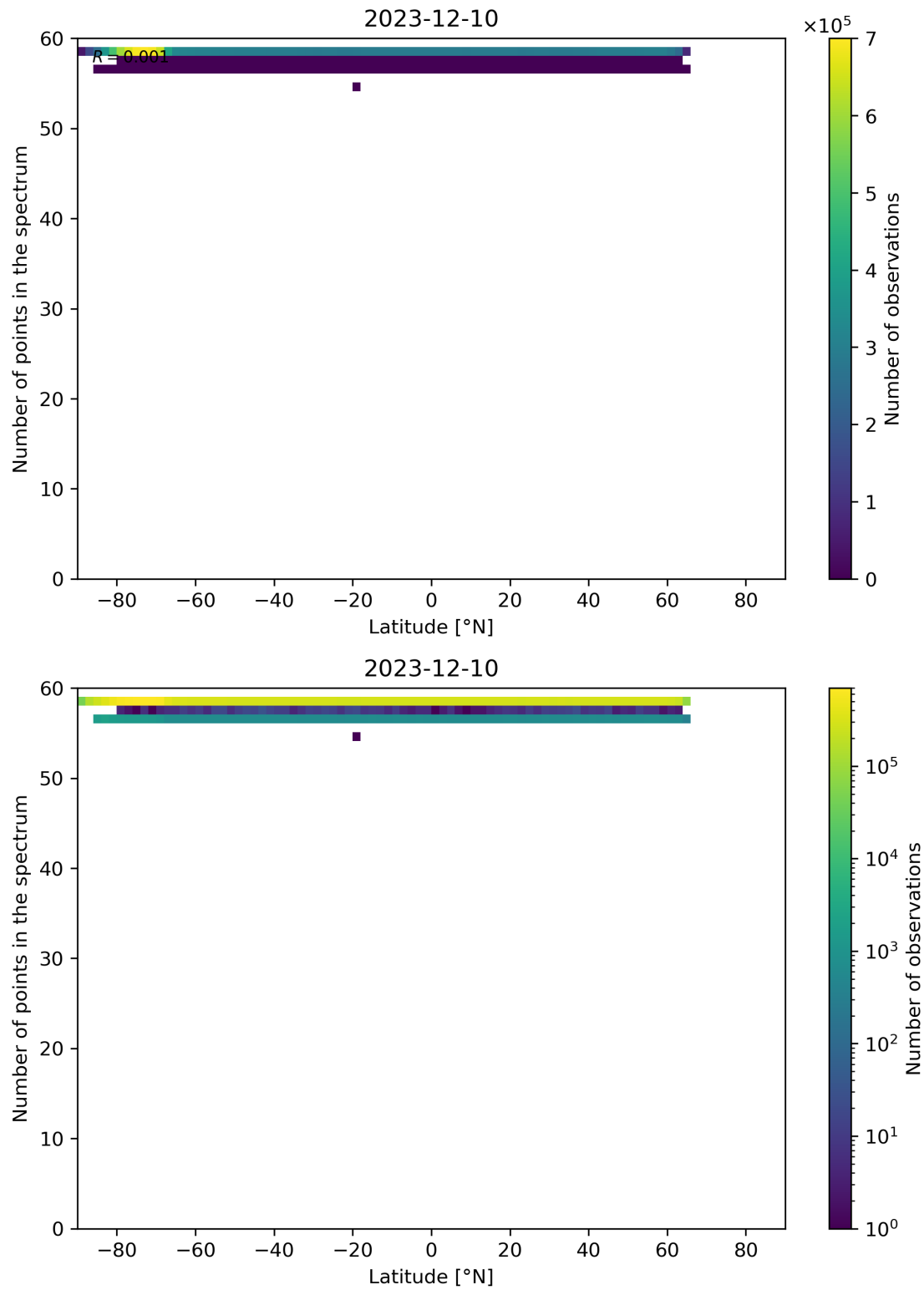
Figure 94: Scatter density plot of “Latitude” against “Number of points in the spectrum” for 2023-12-09 to 2023-12-11.
