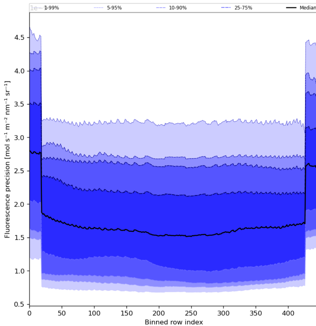
Figure 58: Along track statistics of “Fluorescence precision” for 2023-12-09 to 2023-12-11
