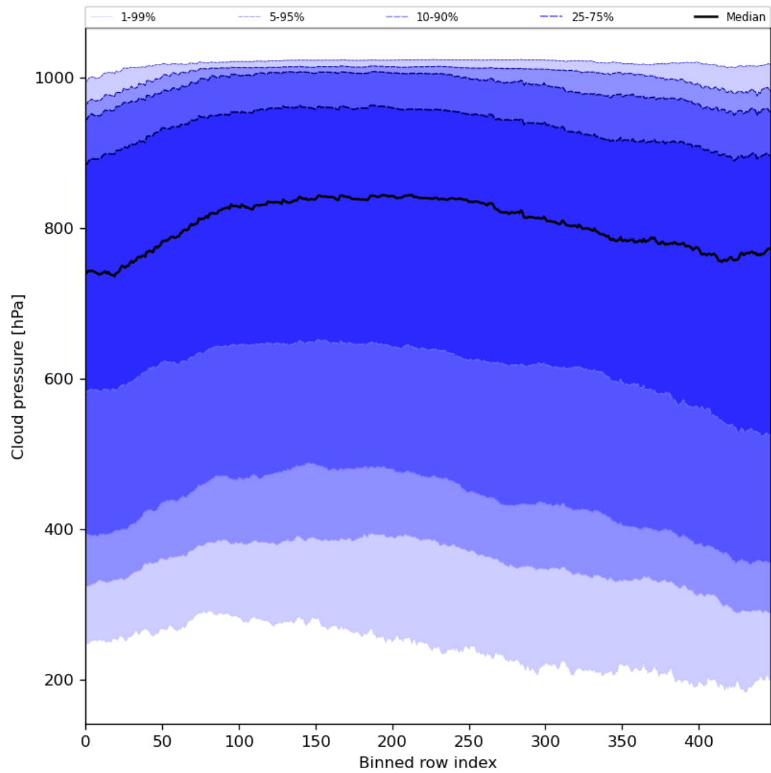
Figure 47: Along track statistics of “Cloud pressure” for 2023-12-09 to 2023-12-11
