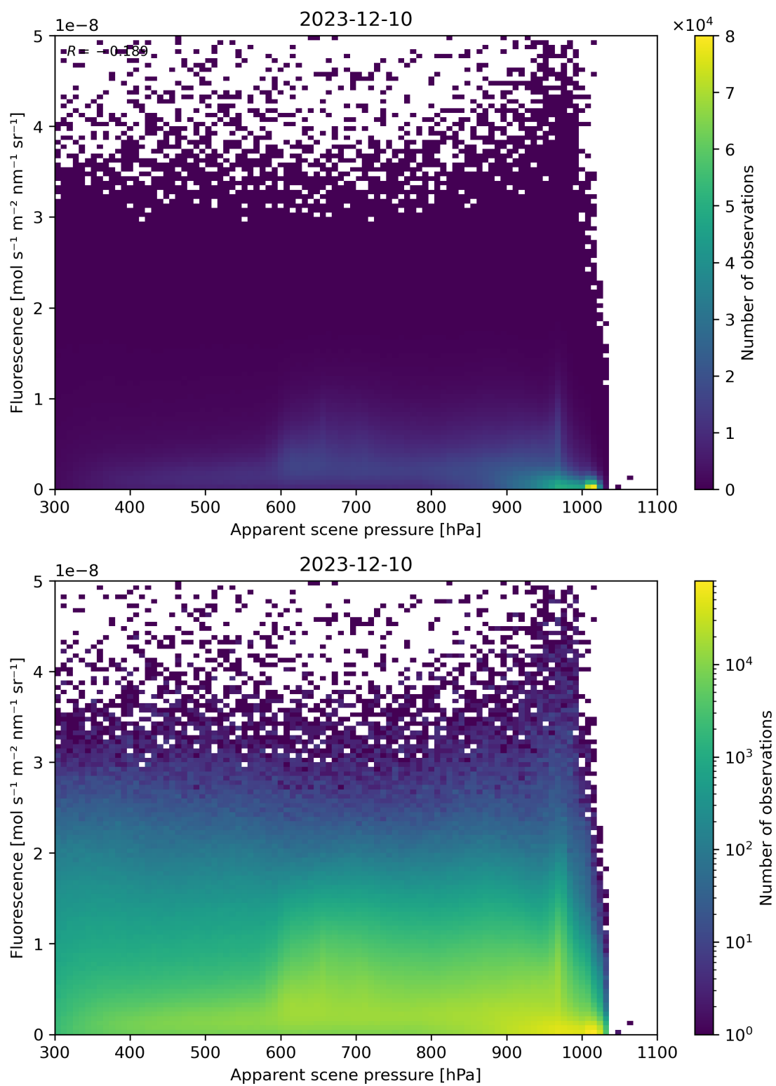
Figure 64: Scatter density plot of “Apparent scene pressure” against “Fluorescence” for 2023-12-09 to 2023-12-11.
