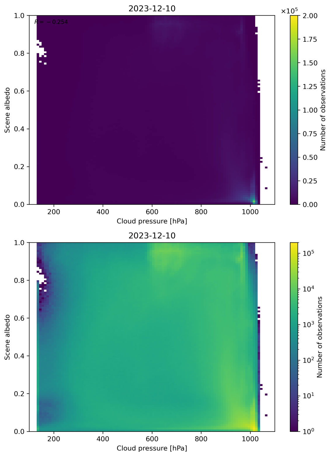
Figure 83: Scatter density plot of “Cloud pressure” against “Scene albedo” for 2023-12-09 to 2023-12-11.
