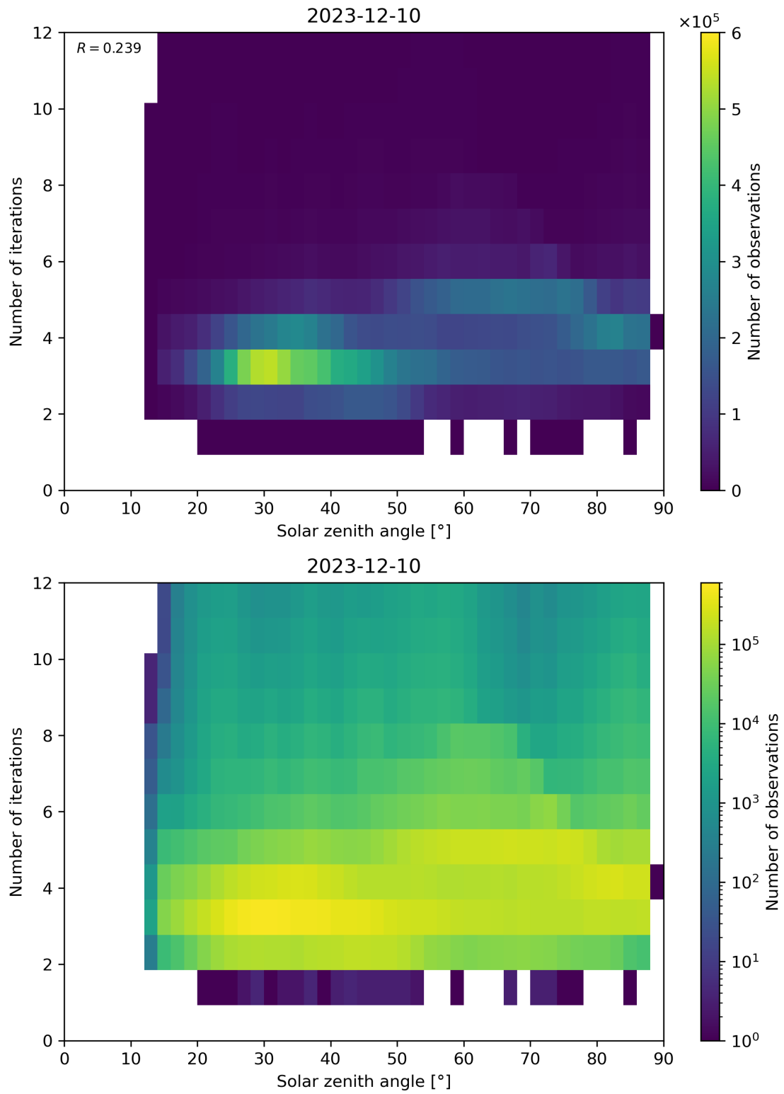
Figure 114: Scatter density plot of “Solar zenith angle” against “Number of iterations” for 2023-12-09 to 2023-12-11.
