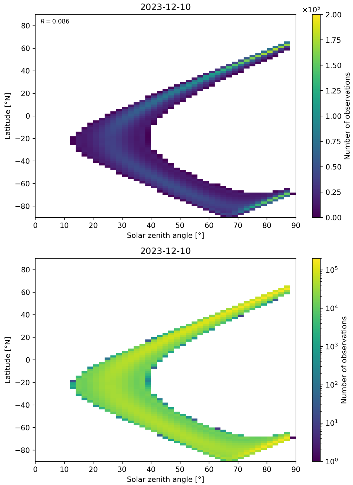
Figure 113: Scatter density plot of “Solar zenith angle” against “Latitude” for 2023-12-09 to 2023-12-11.
