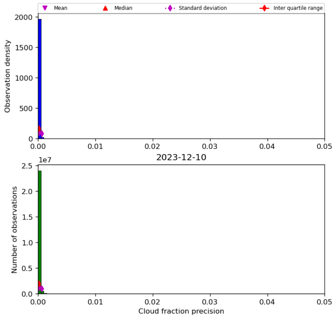
Figure 33: Histogram of “Cloud fraction precision” for 2023-12-09 to 2023-12-11
