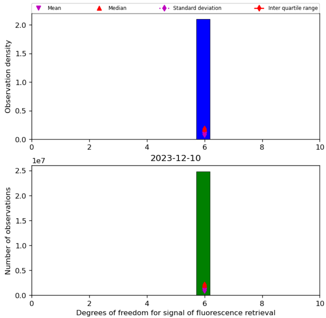
Figure 43: Histogram of “Degrees of freedom for signal of fluorescence retrieval” for 2023-12-09 to 2023-12-11
