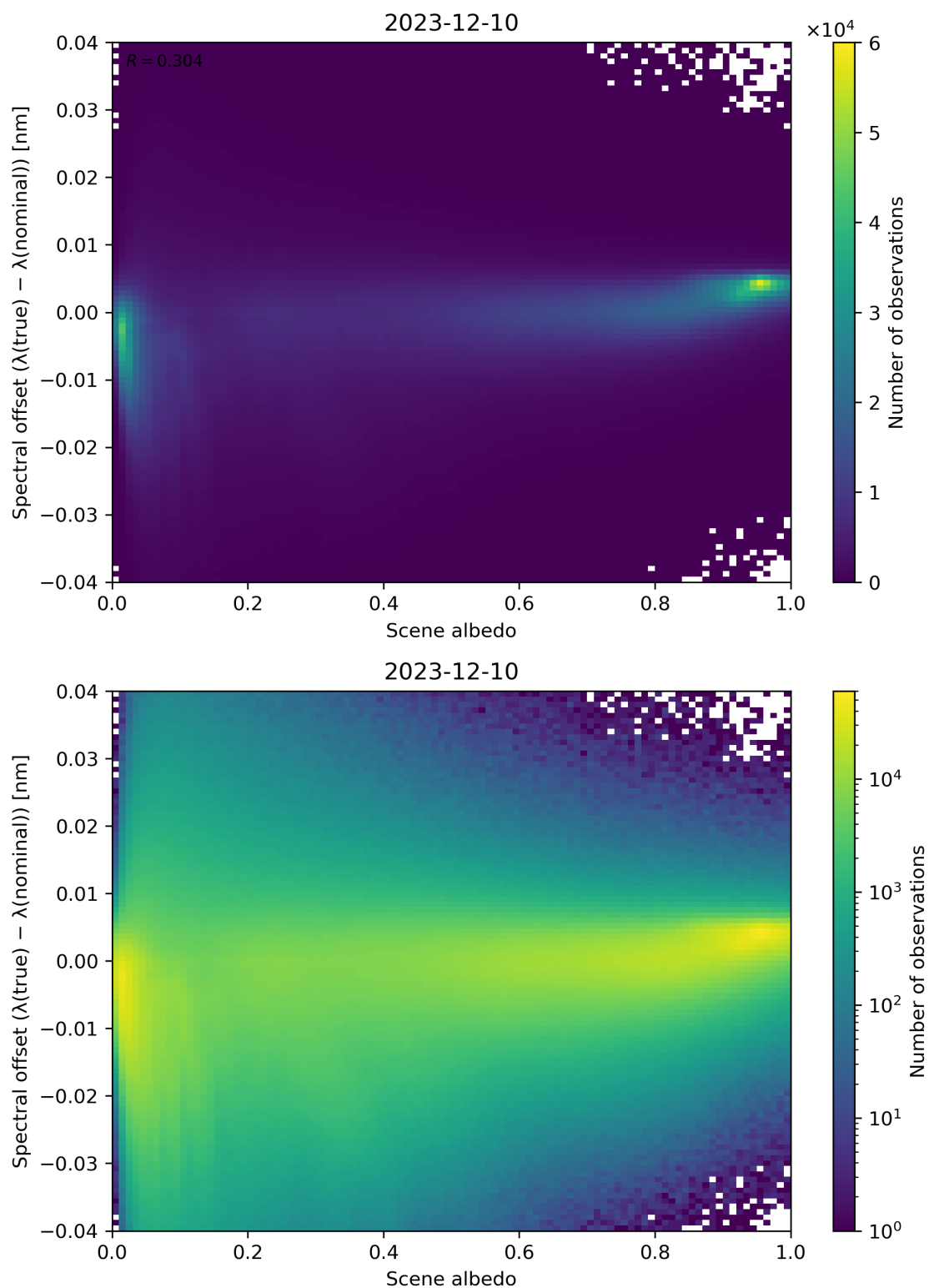
Figure 107: Scatter density plot of “Scene albedo” against “Spectral offset ( \lambda(\text{true}) - \lambda(\text{nominal}) )” for 2023-12-09 to 2023-12-11.
