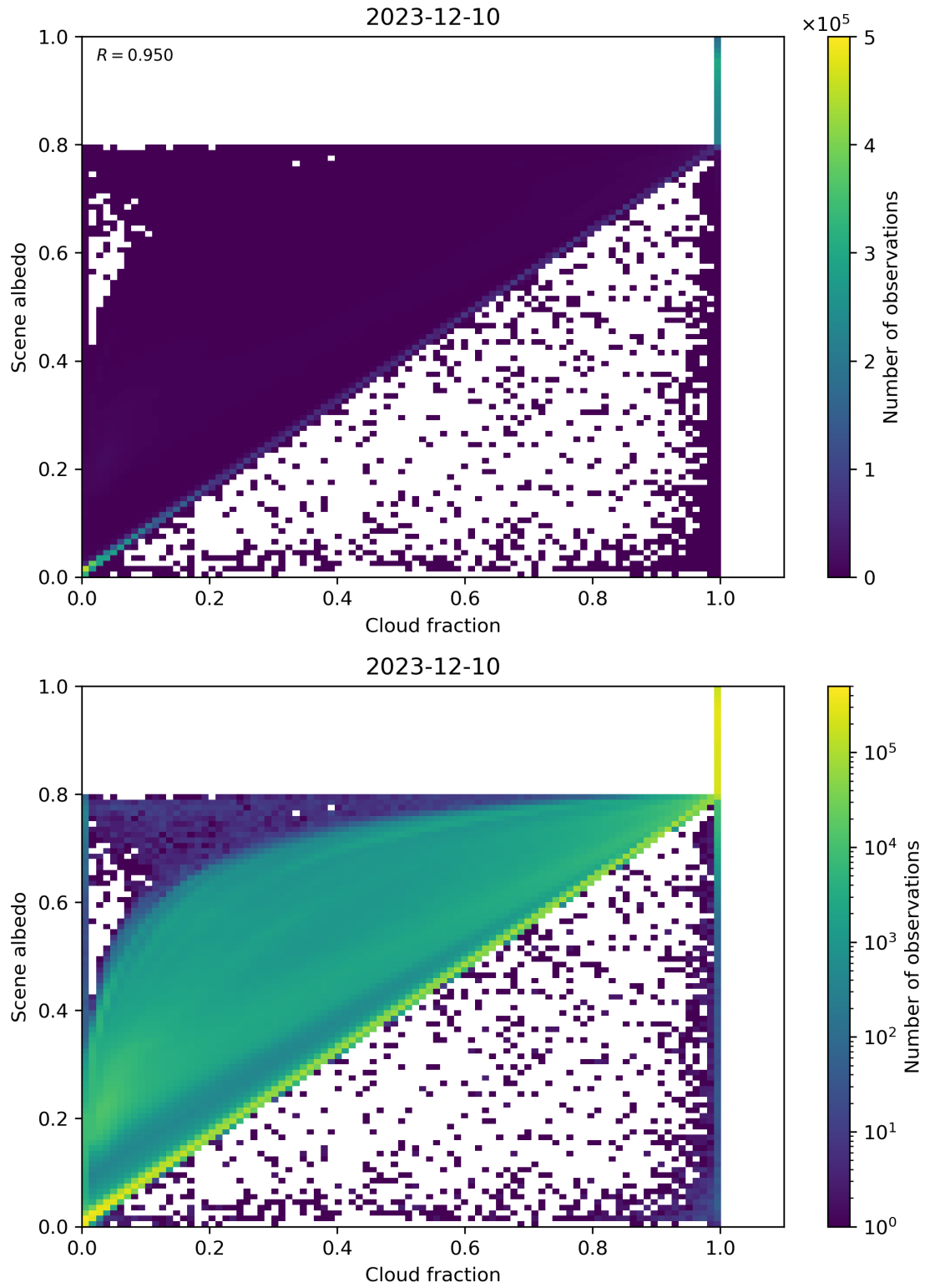
Figure 75: Scatter density plot of “Cloud fraction” against “Scene albedo” for 2023-12-09 to 2023-12-11.
