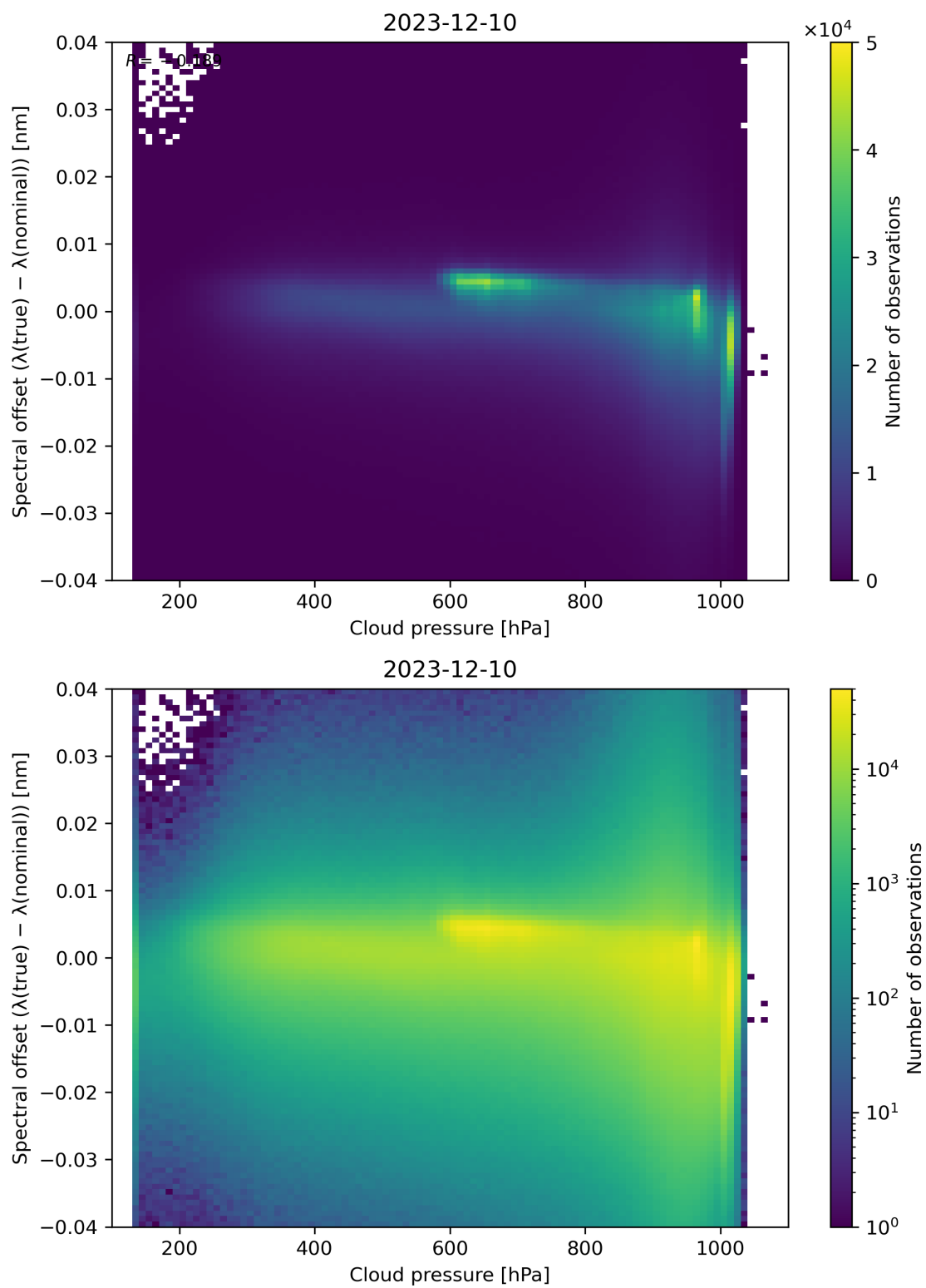
Figure 84: Scatter density plot of “Cloud pressure” against “Spectral offset ( \lambda(\text{true}) - \lambda(\text{nominal}) )” for 2023-12-09 to 2023-12-11.
