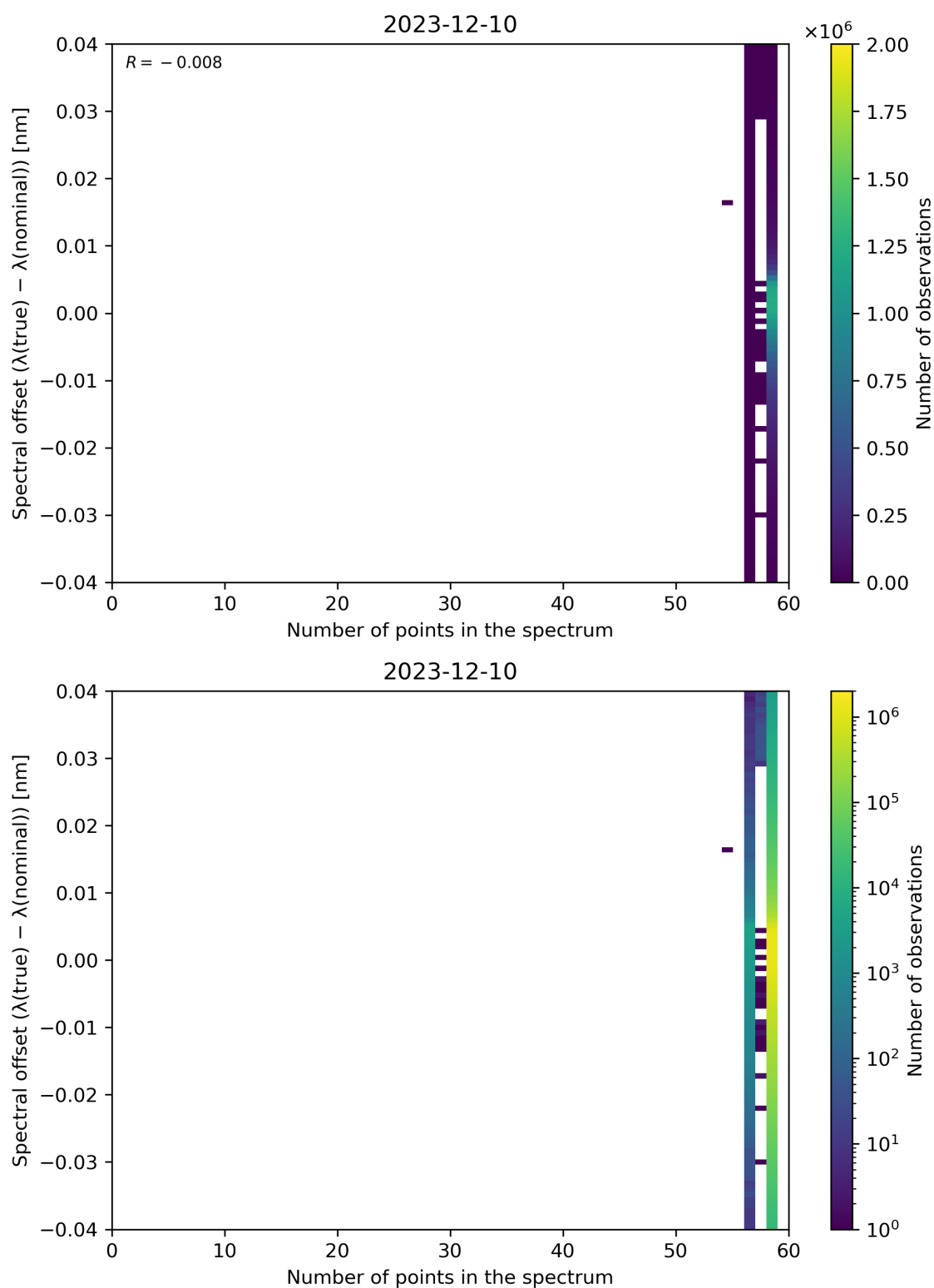
Figure 101: Scatter density plot of “Number of points in the spectrum” against “Spectral offset ( \lambda(\text{true}) - \lambda(\text{nominal}) )” for 2023-12-09 to 2023-12-11.
