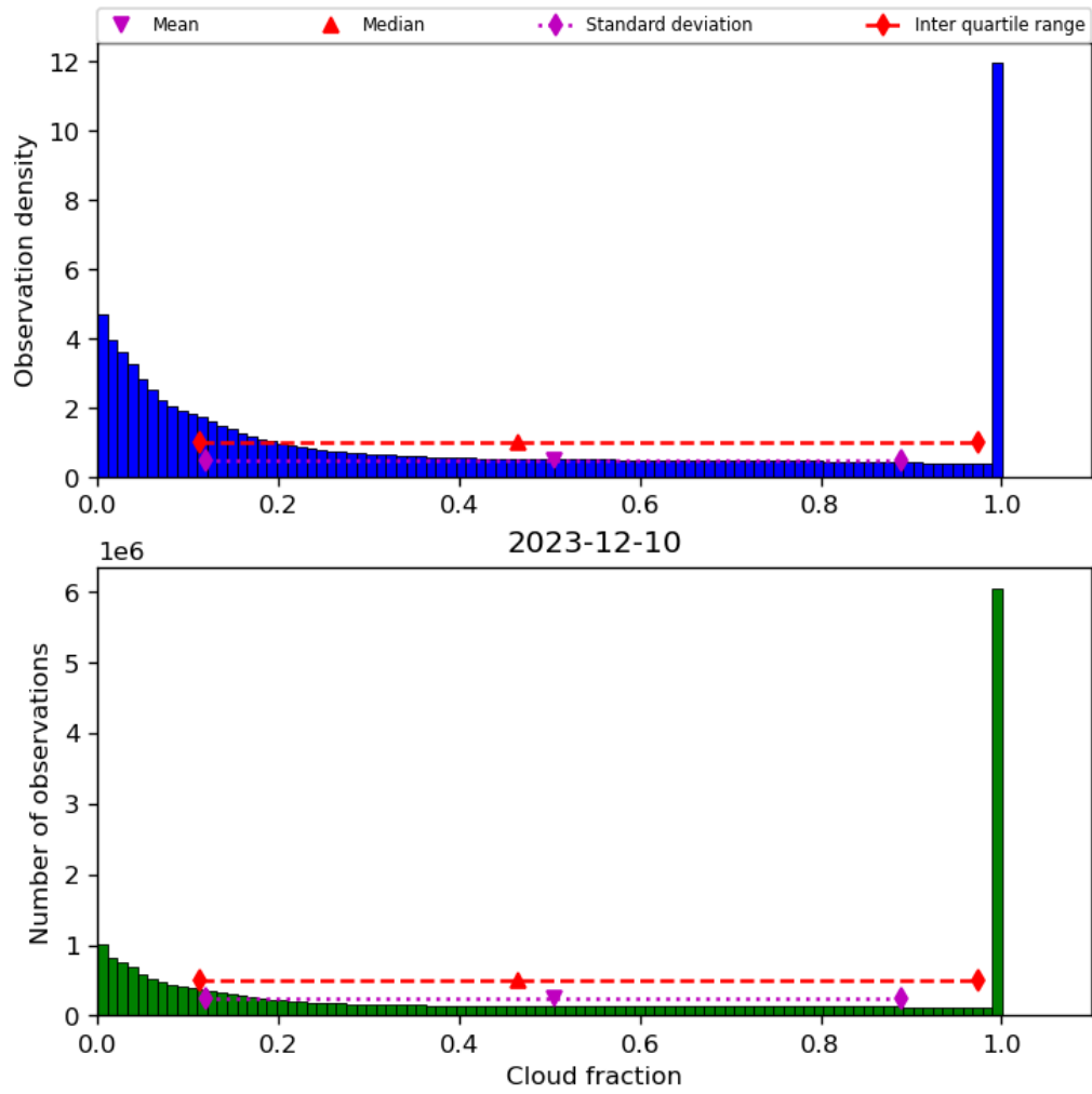
Figure 32: Histogram of “Cloud fraction” for 2023-12-09 to 2023-12-11
