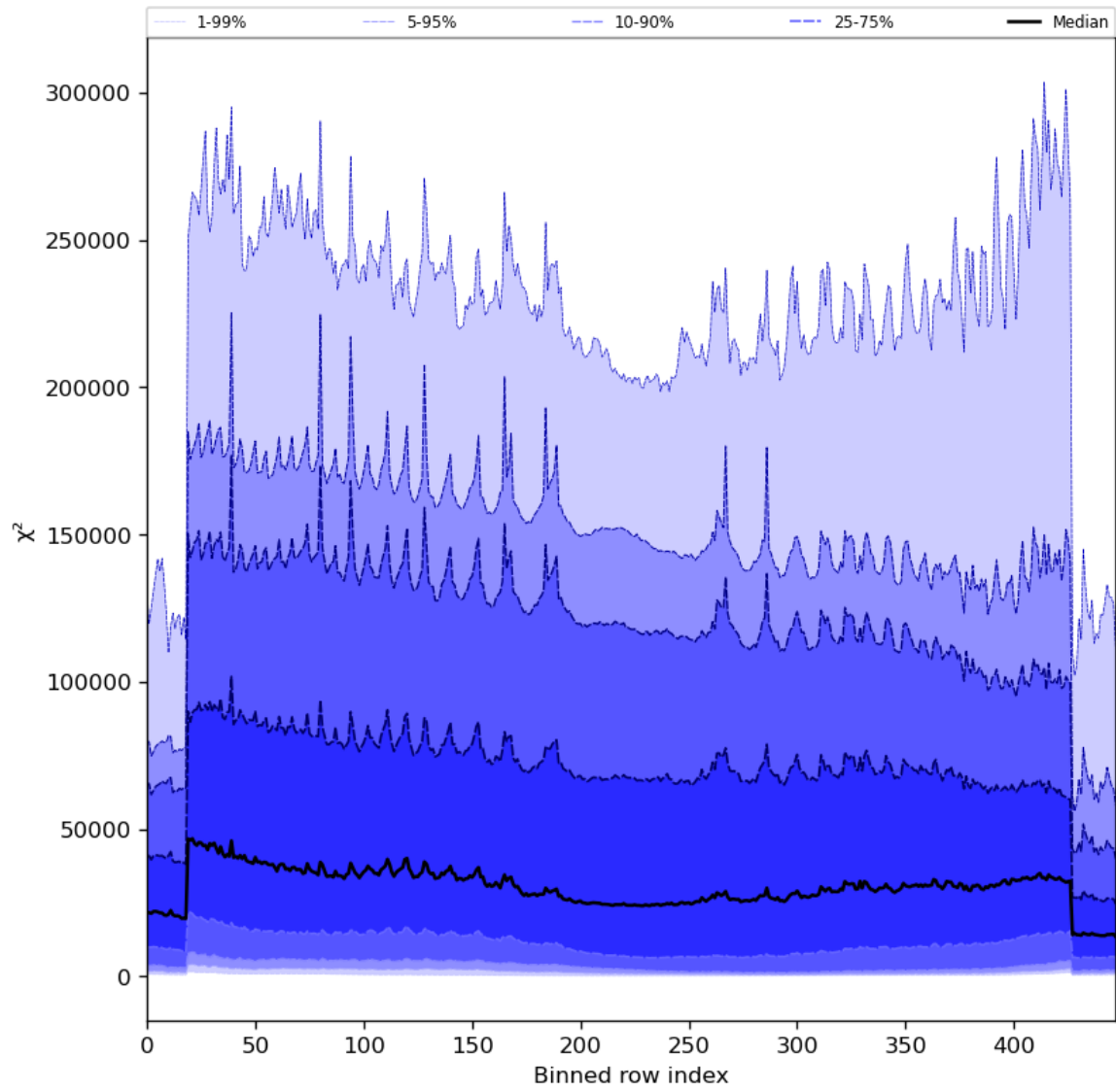
Figure 55: Along track statistics of “ \chi^2 ” for 2023-12-09 to 2023-12-11
