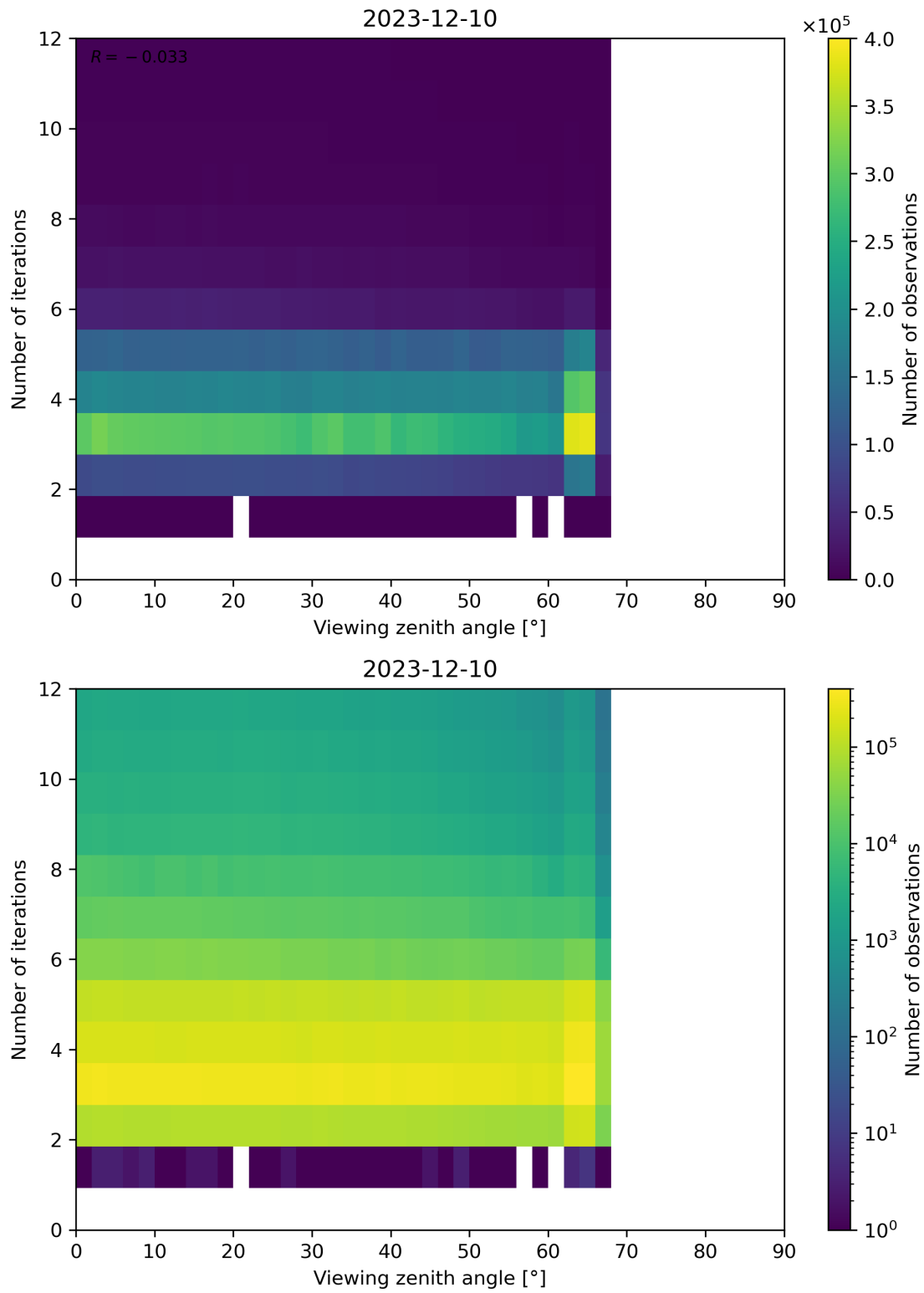
Figure 124: Scatter density plot of “Viewing zenith angle” against “Number of iterations” for 2023-12-09 to 2023-12-11.
