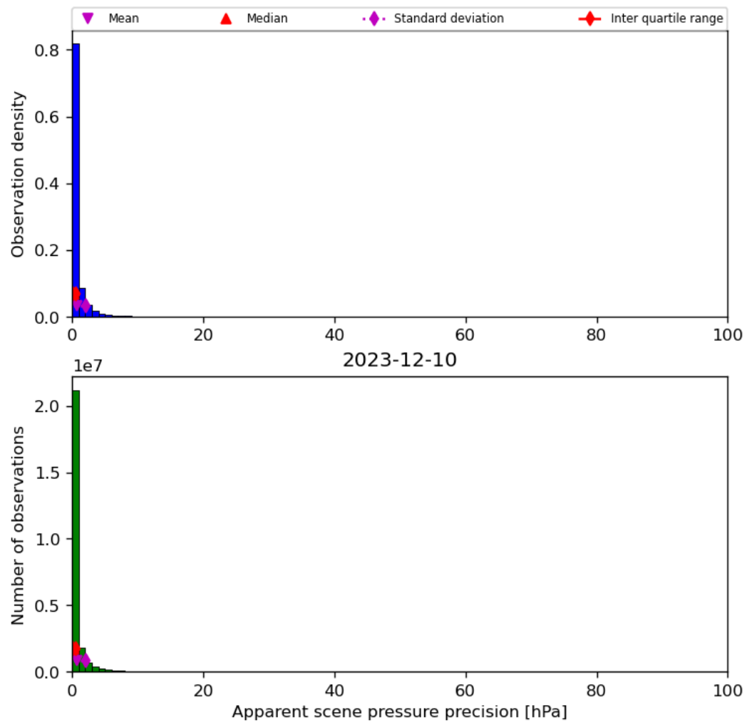
Figure 37: Histogram of “Apparent scene pressure precision” for 2023-12-09 to 2023-12-11
