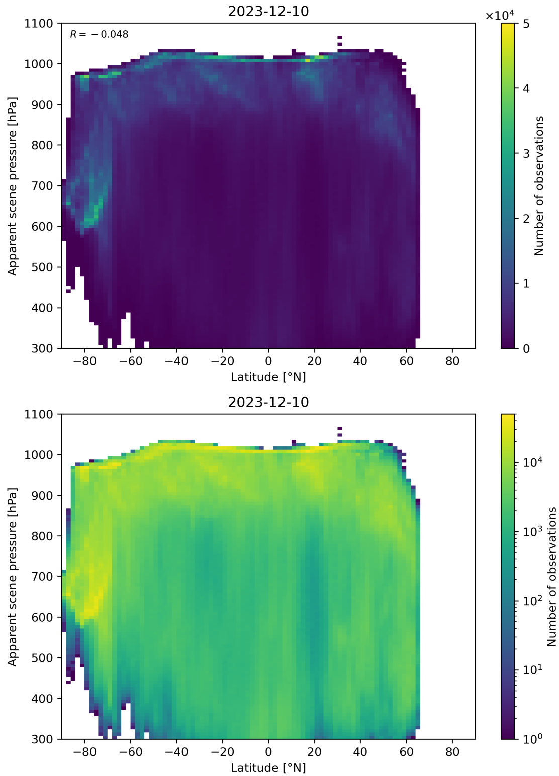
Figure 88: Scatter density plot of “Latitude” against “Apparent scene pressure” for 2023-12-09 to 2023-12-11.
