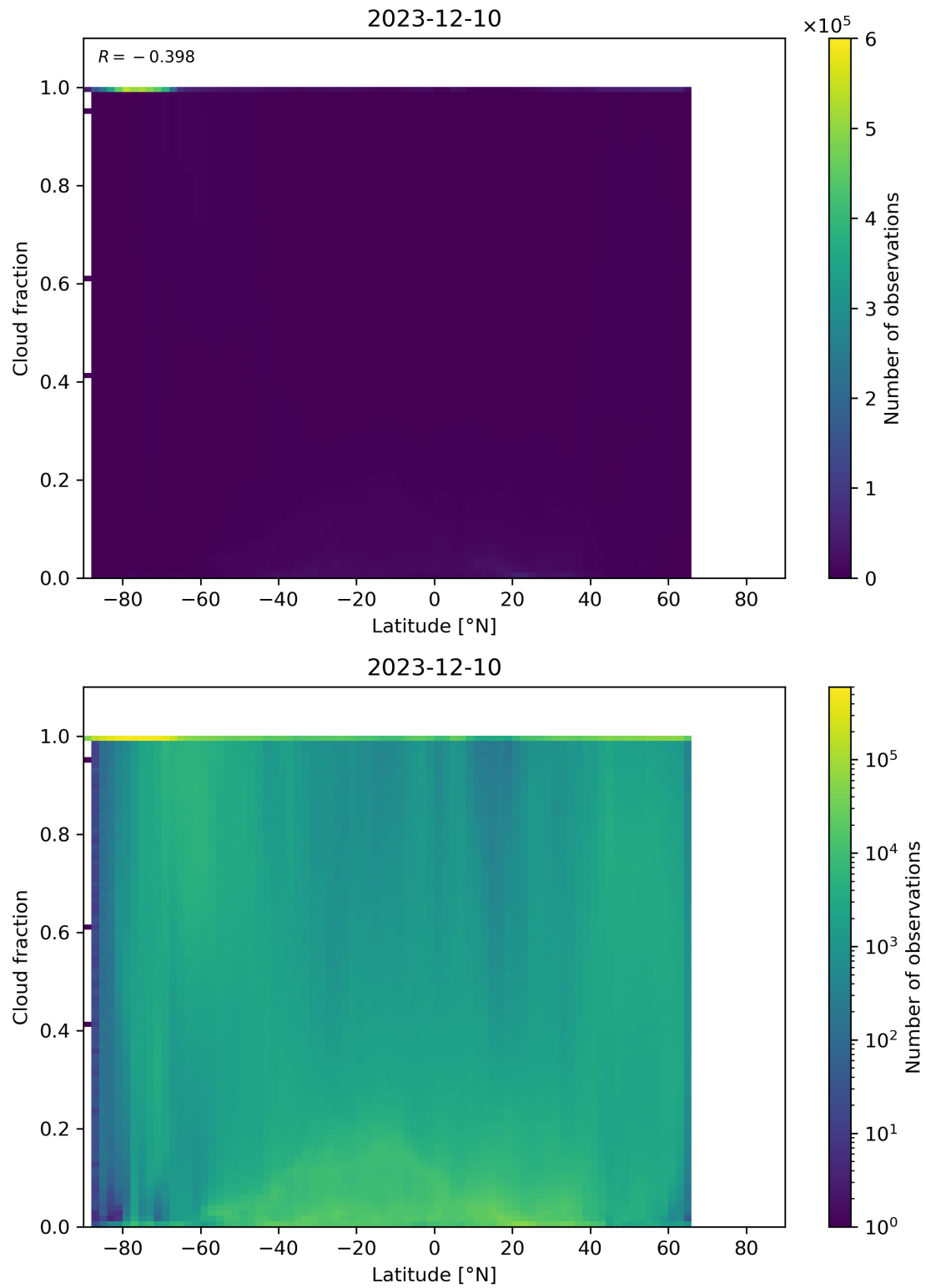
Figure 90: Scatter density plot of “Latitude” against “Cloud fraction” for 2023-12-09 to 2023-12-11.
