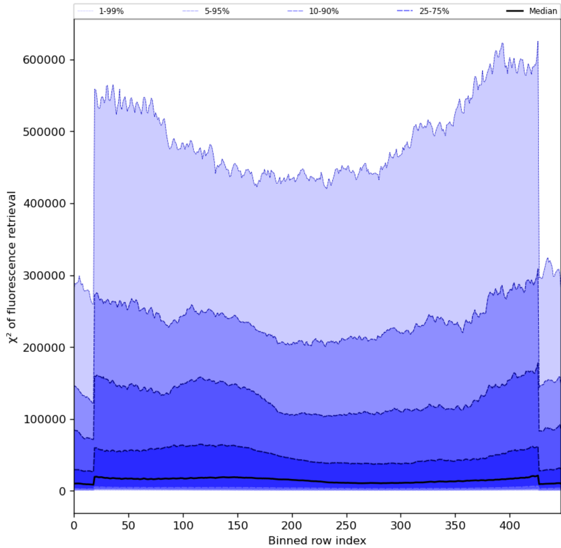
Figure 59: Along track statistics of “ \chi^2 of fluorescence retrieval” for 2023-12-09 to 2023-12-11
