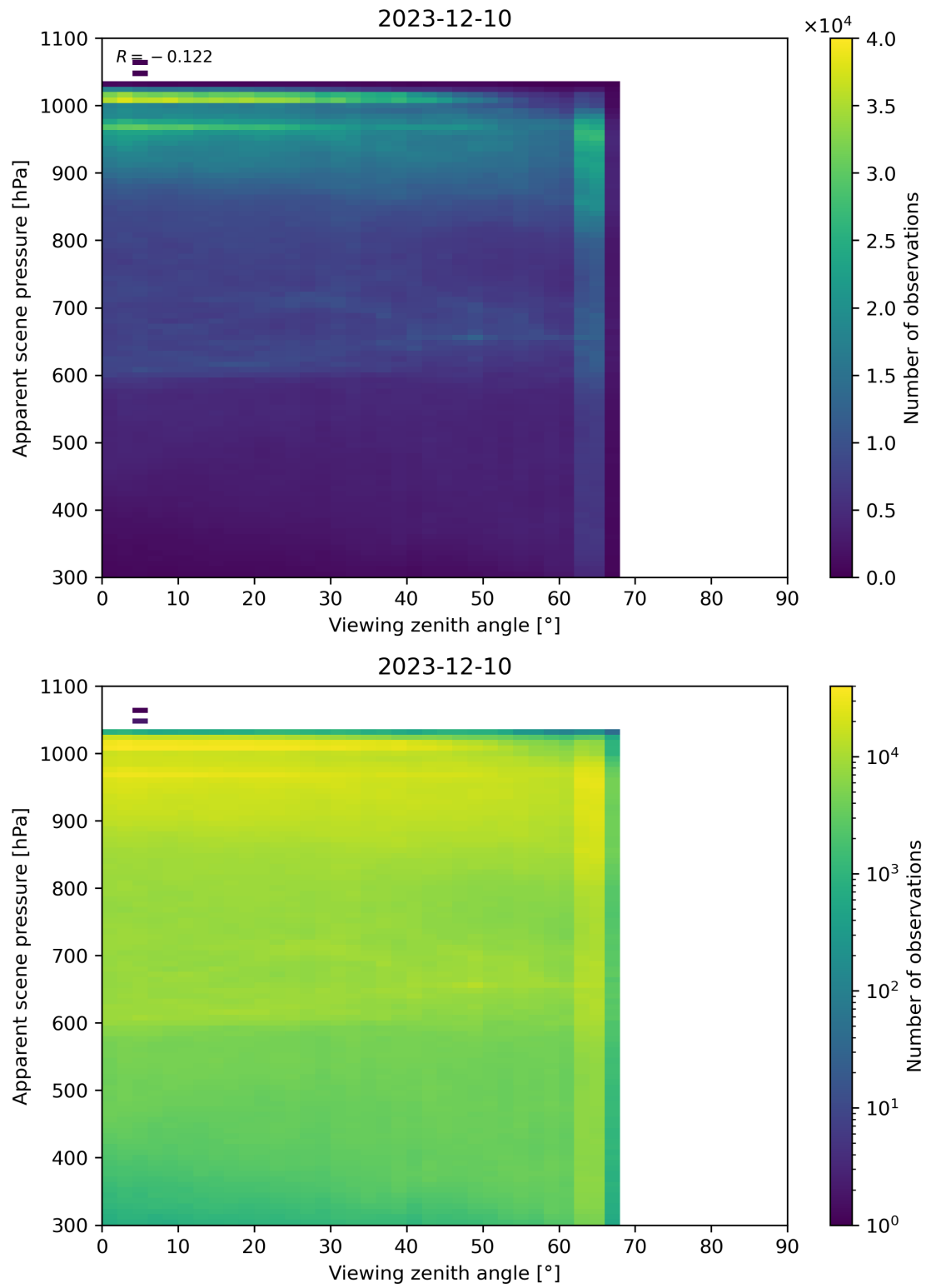
Figure 118: Scatter density plot of “Viewing zenith angle” against “Apparent scene pressure” for 2023-12-09 to 2023-12-11.
