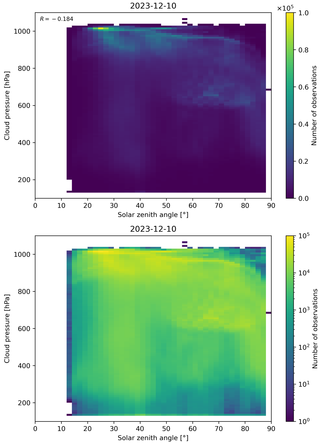
Figure 111: Scatter density plot of “Solar zenith angle” against “Cloud pressure” for 2023-12-09 to 2023-12-11.
