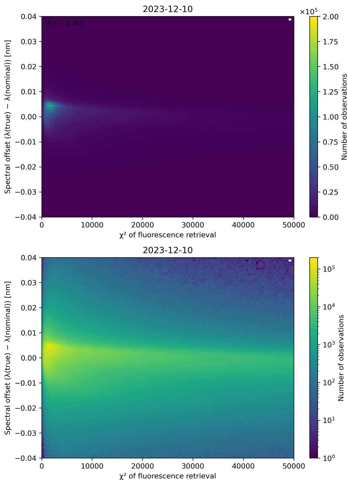
Figure 69: Scatter density plot of " \chi^2 of fluorescence retrieval" against "Spectral offset ( \lambda(\text{true}) - \lambda(\text{nominal}) )" for 2023-12-09 to 2023-12-11.
