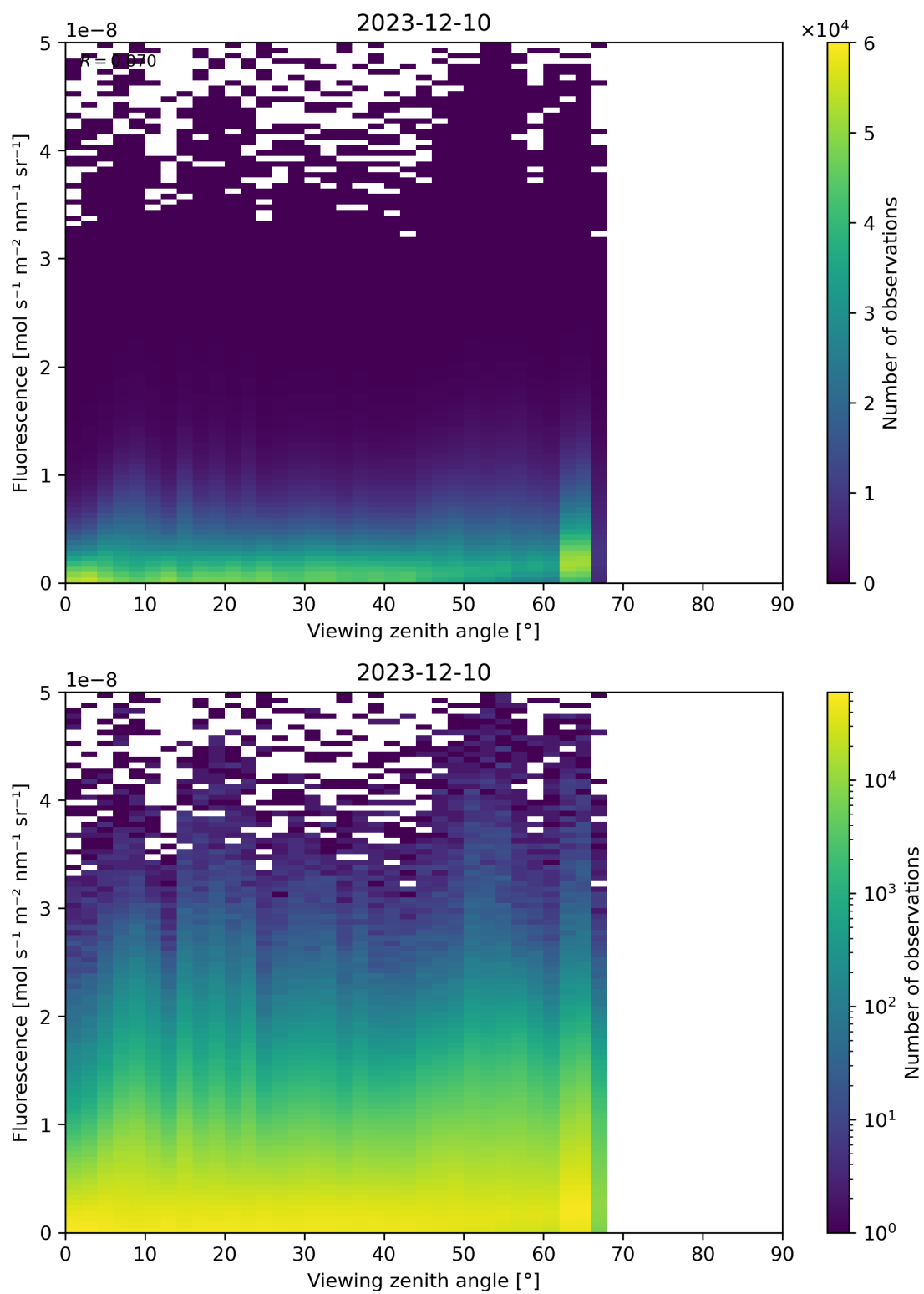
Figure 122: Scatter density plot of “Viewing zenith angle” against “Fluorescence” for 2023-12-09 to 2023-12-11.
