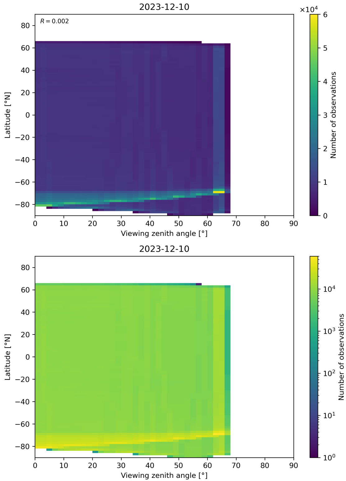
Figure 123: Scatter density plot of “Viewing zenith angle” against “Latitude” for 2023-12-09 to 2023-12-11.
