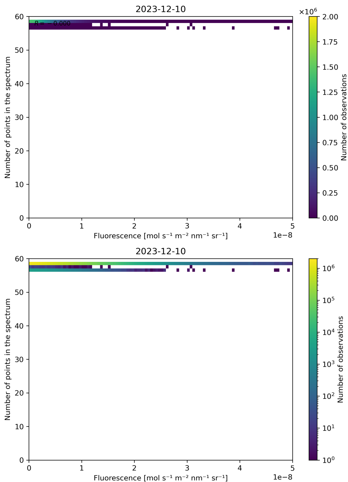
Figure 86: Scatter density plot of “Fluorescence” against “Number of points in the spectrum” for 2023-12-09 to 2023-12-11.
