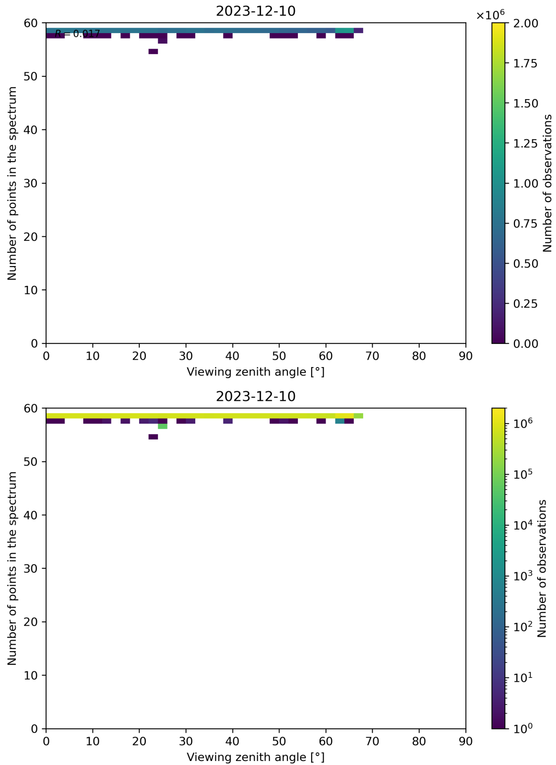
Figure 125: Scatter density plot of “Viewing zenith angle” against “Number of points in the spectrum” for 2023-12-09 to 2023-12-11.
