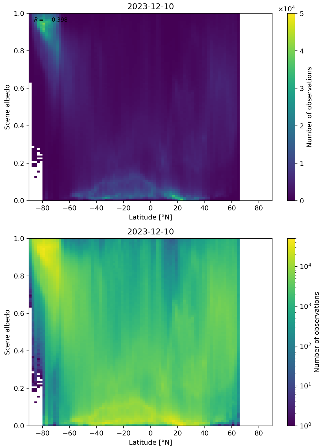
Figure 95: Scatter density plot of “Latitude” against “Scene albedo” for 2023-12-09 to 2023-12-11.
