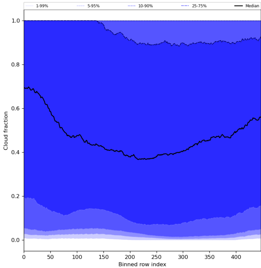
Figure 49: Along track statistics of “Cloud fraction” for 2023-12-09 to 2023-12-11
