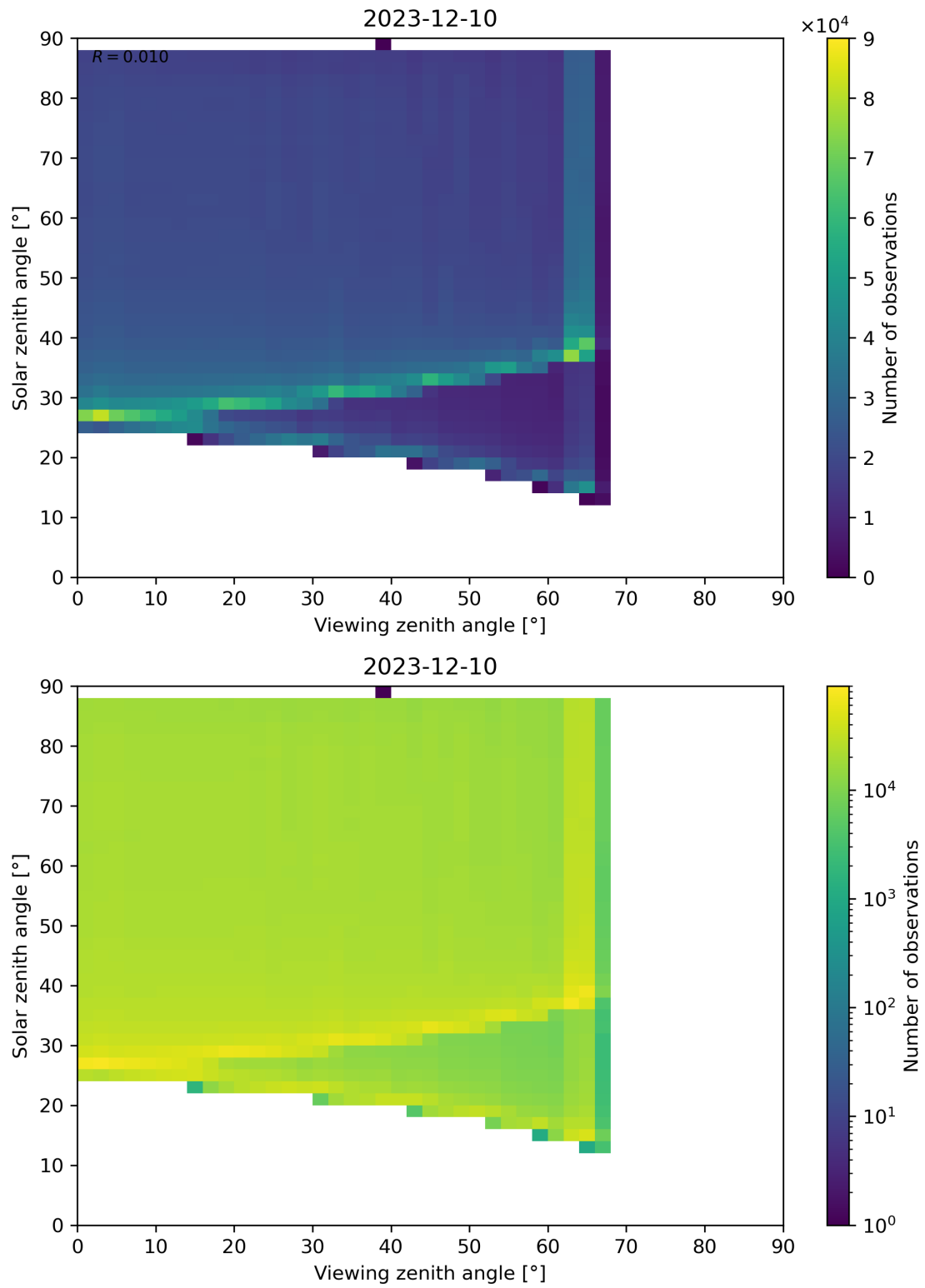
Figure 127: Scatter density plot of “Viewing zenith angle” against “Solar zenith angle” for 2023-12-09 to 2023-12-11.
