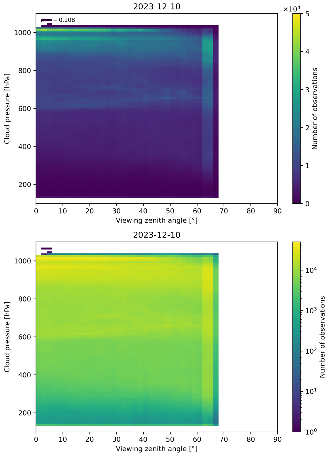
Figure 121: Scatter density plot of “Viewing zenith angle” against “Cloud pressure” for 2023-12-09 to 2023-12-11.
