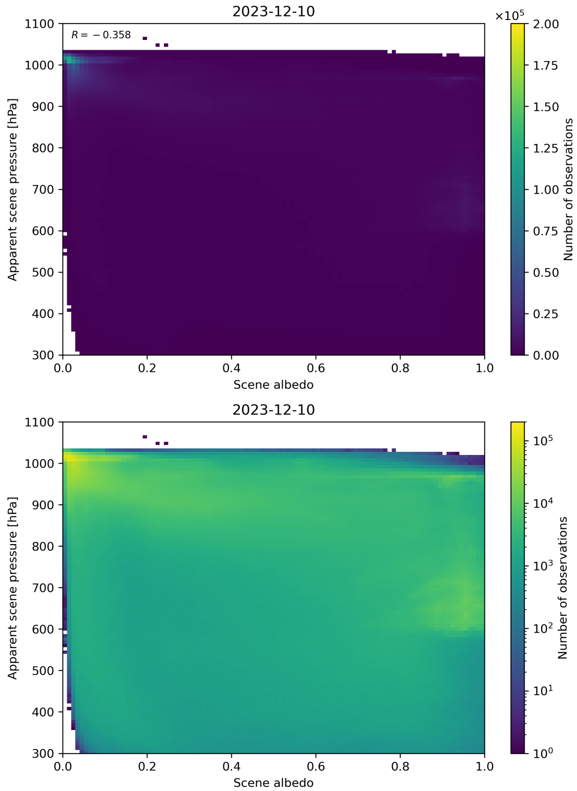
Figure 102: Scatter density plot of “Scene albedo” against “Apparent scene pressure” for 2023-12-09 to 2023-12-11.
