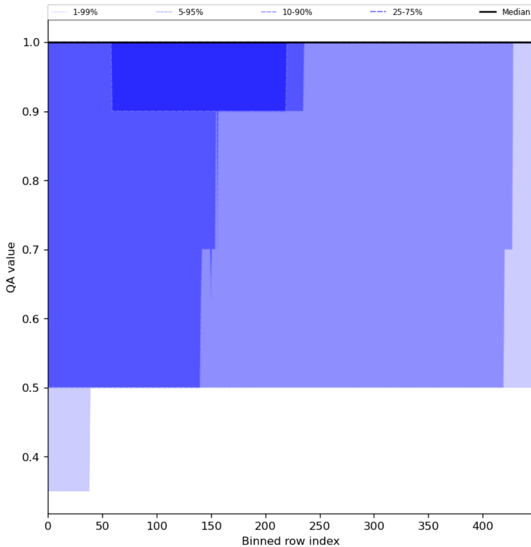
Figure 46: Along track statistics of “QA value” for 2023-12-09 to 2023-12-11
