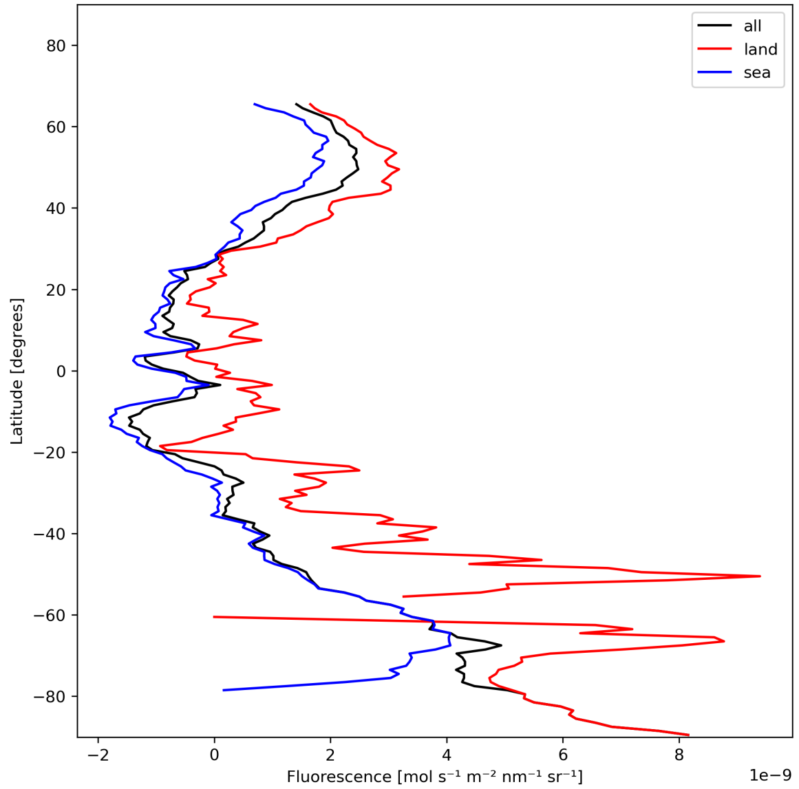
Figure 23: Zonal average of “Fluorescence” for 2023-12-09 to 2023-12-11.
