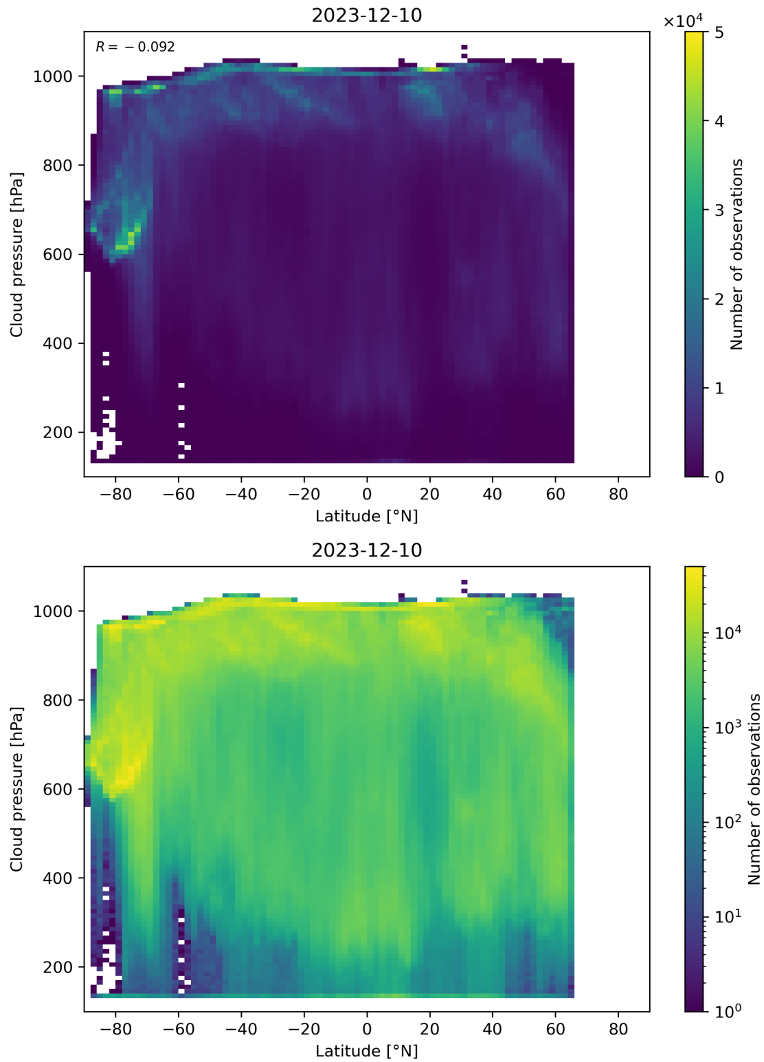
Figure 91: Scatter density plot of “Latitude” against “Cloud pressure” for 2023-12-09 to 2023-12-11.
