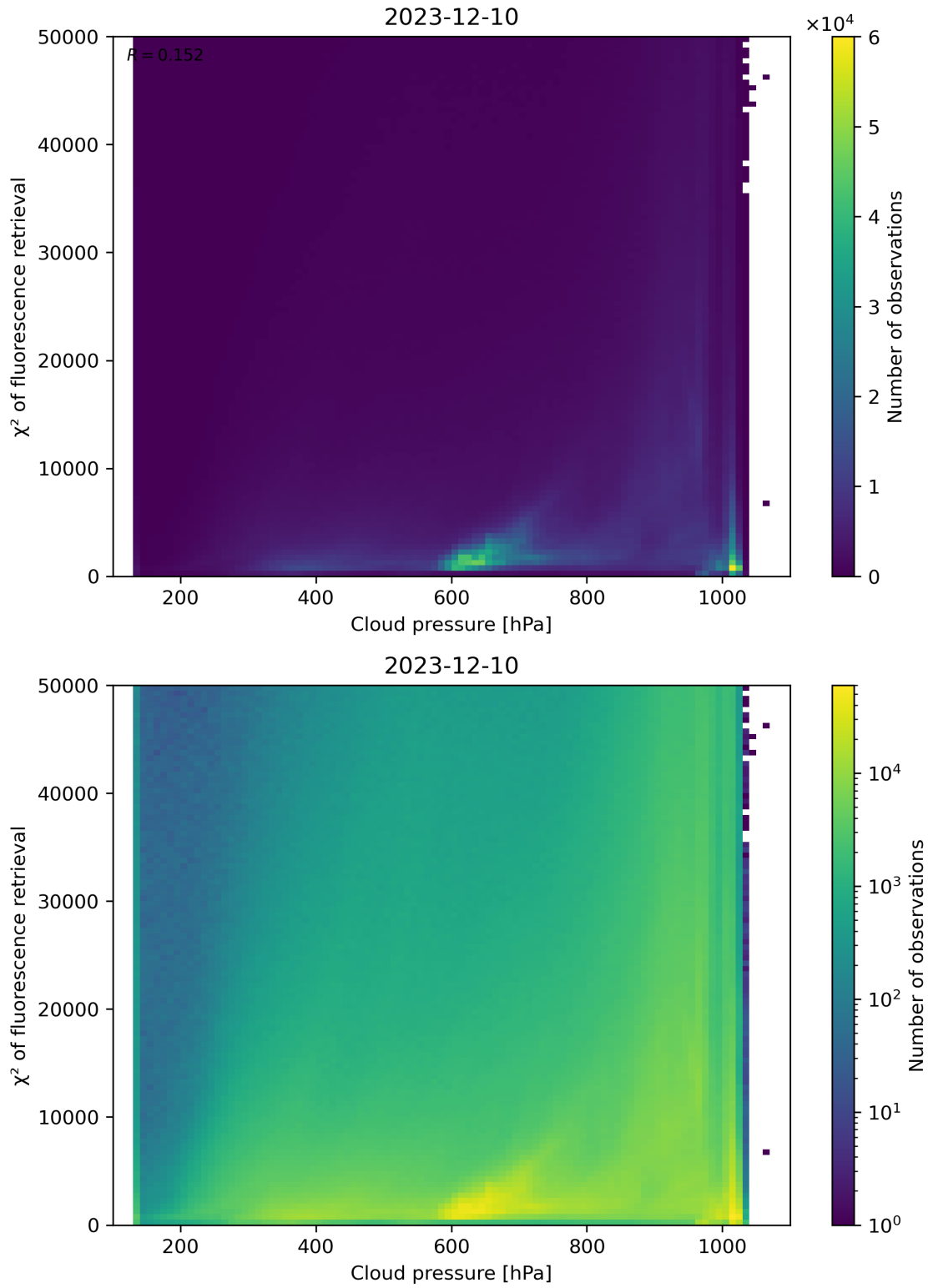
Figure 78: Scatter density plot of “Cloud pressure” against “ \chi^2 of fluorescence retrieval” for 2023-12-09 to 2023-12-11.
