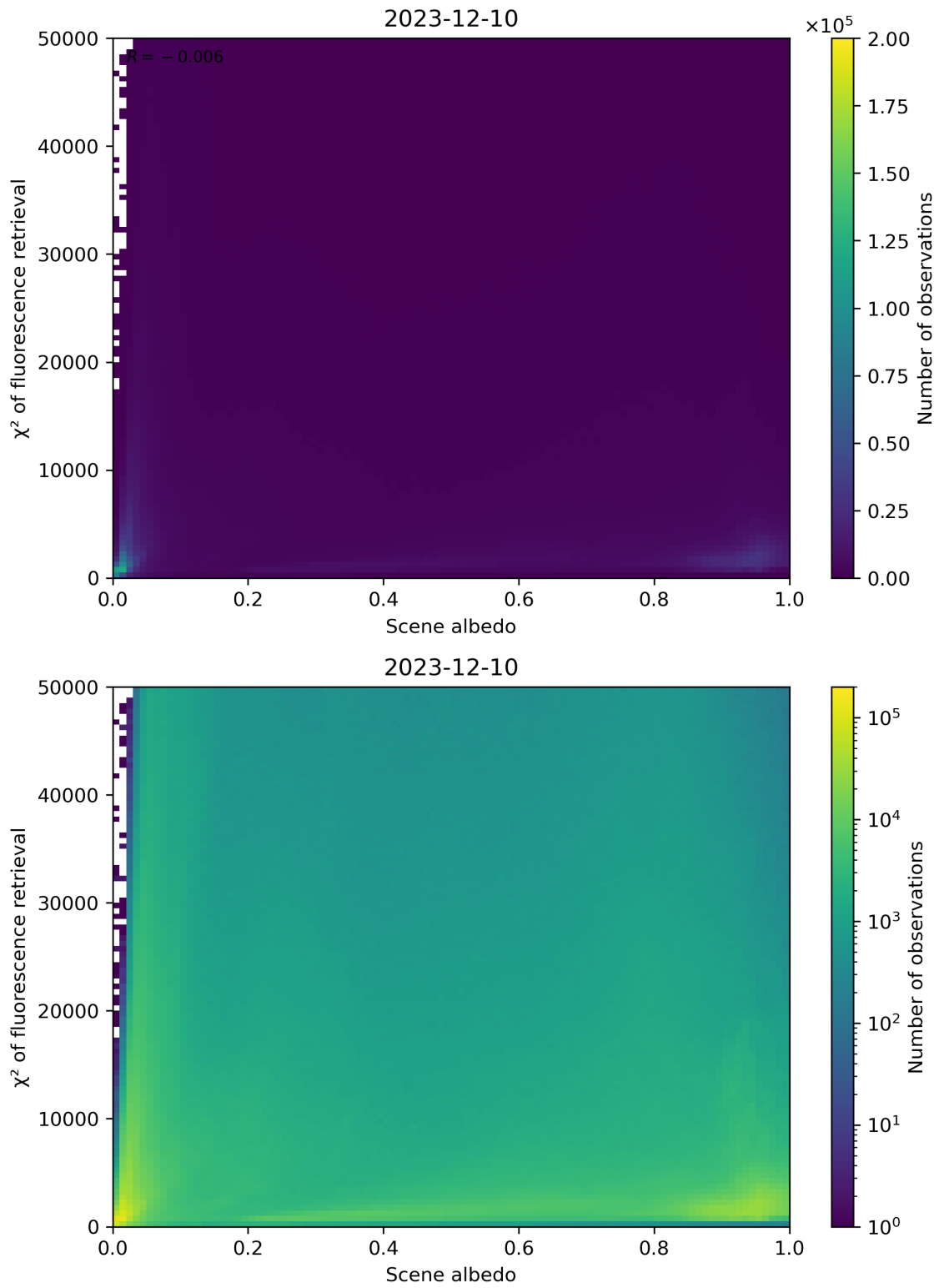
Figure 103: Scatter density plot of “Scene albedo” against “ \chi^2 of fluorescence retrieval” for 2023-12-09 to 2023-12-11.
