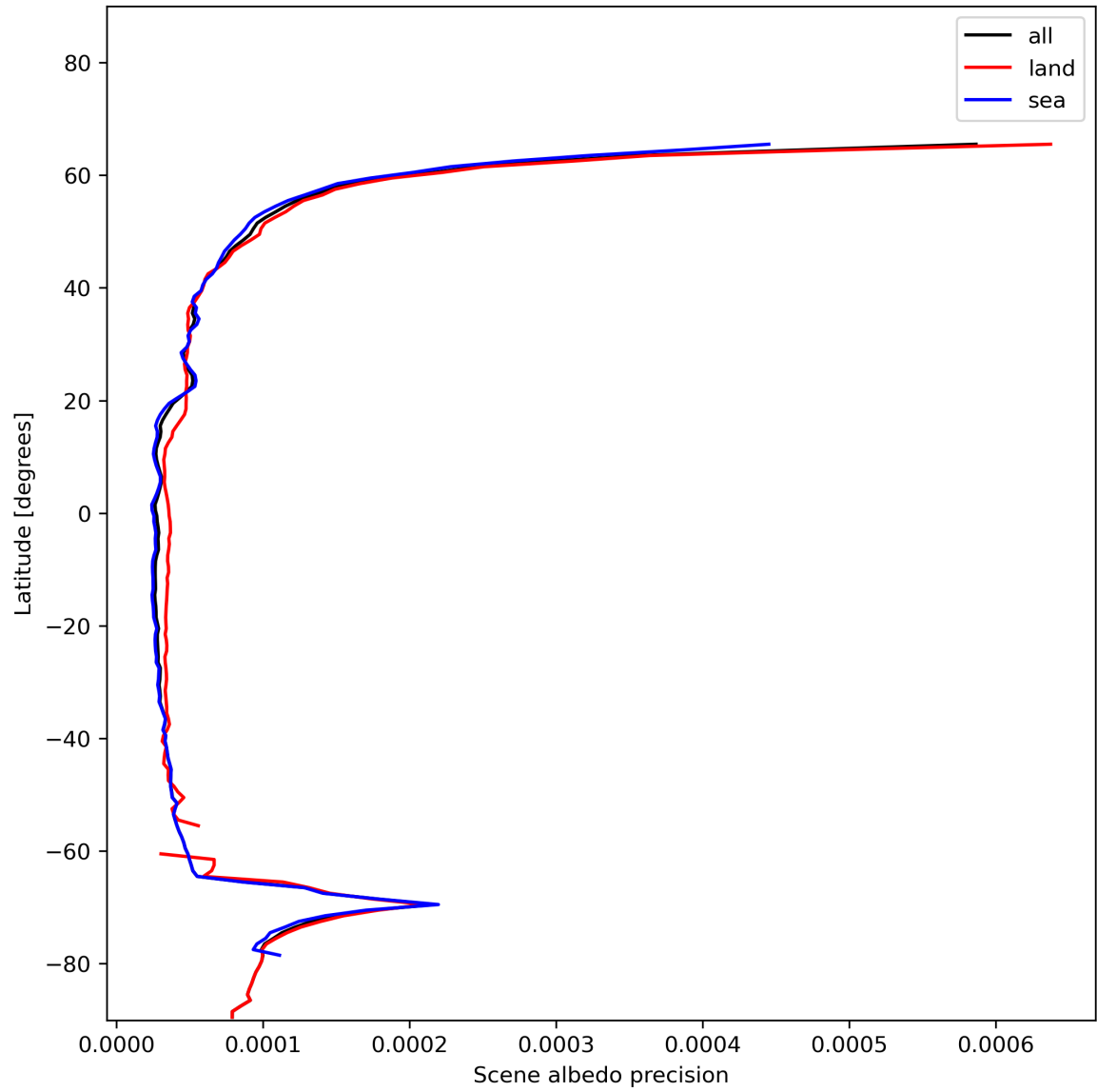
Figure 18: Zonal average of “Scene albedo precision” for 2023-12-09 to 2023-12-11.
