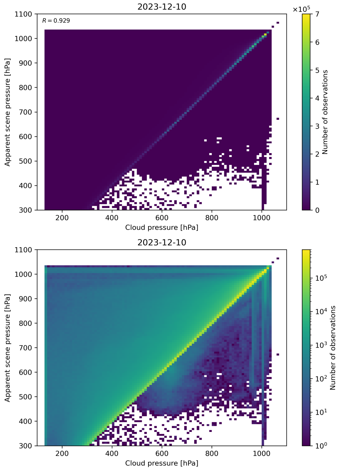
Figure 77: Scatter density plot of “Cloud pressure” against “Apparent scene pressure” for 2023-12-09 to 2023-12-11.
