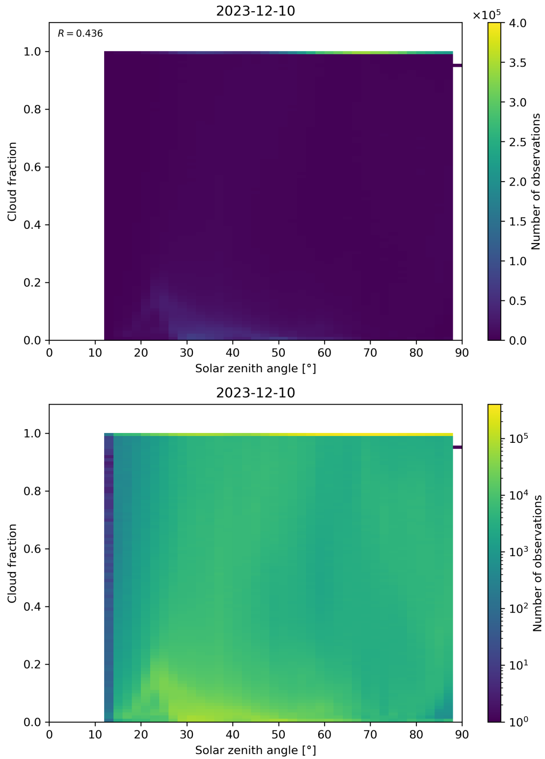
Figure 110: Scatter density plot of “Solar zenith angle” against “Cloud fraction” for 2023-12-09 to 2023-12-11.
