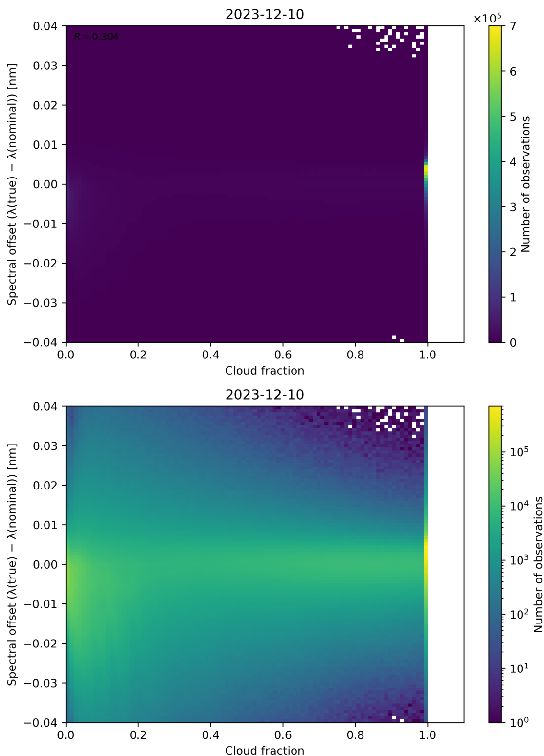
Figure 76: Scatter density plot of “Cloud fraction” against “Spectral offset ( \lambda(\text{true}) - \lambda(\text{nominal}) )” for 2023-12-09 to 2023-12-11.
