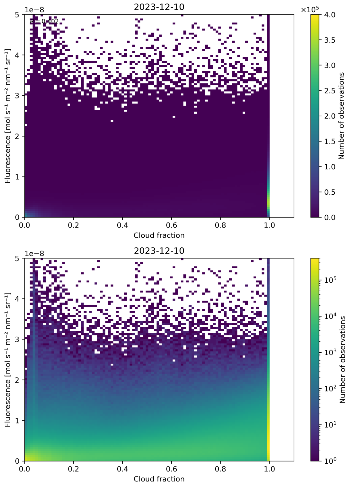
Figure 72: Scatter density plot of “Cloud fraction” against “Fluorescence” for 2023-12-09 to 2023-12-11.
