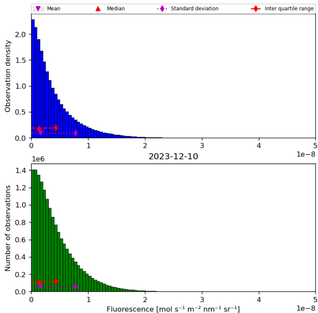
Figure 40: Histogram of “Fluorescence” for 2023-12-09 to 2023-12-11
