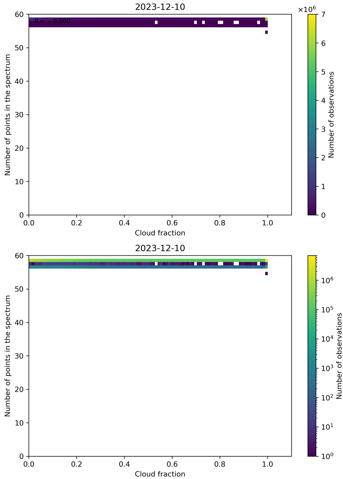
Figure 74: Scatter density plot of “Cloud fraction” against “Number of points in the spectrum” for 2023-12-09 to 2023-12-11.
