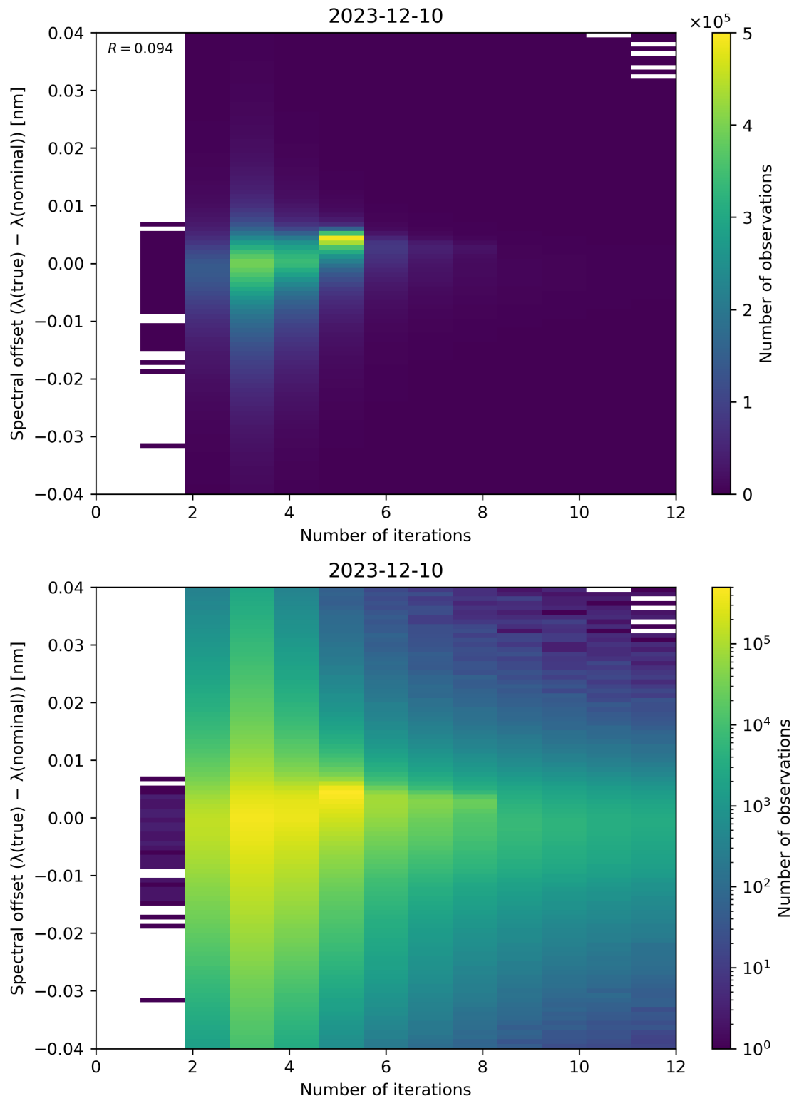
Figure 100: Scatter density plot of “Number of iterations” against “Spectral offset ( \lambda(\text{true}) - \lambda(\text{nominal}) )” for 2023-12-09 to 2023-12-11.
