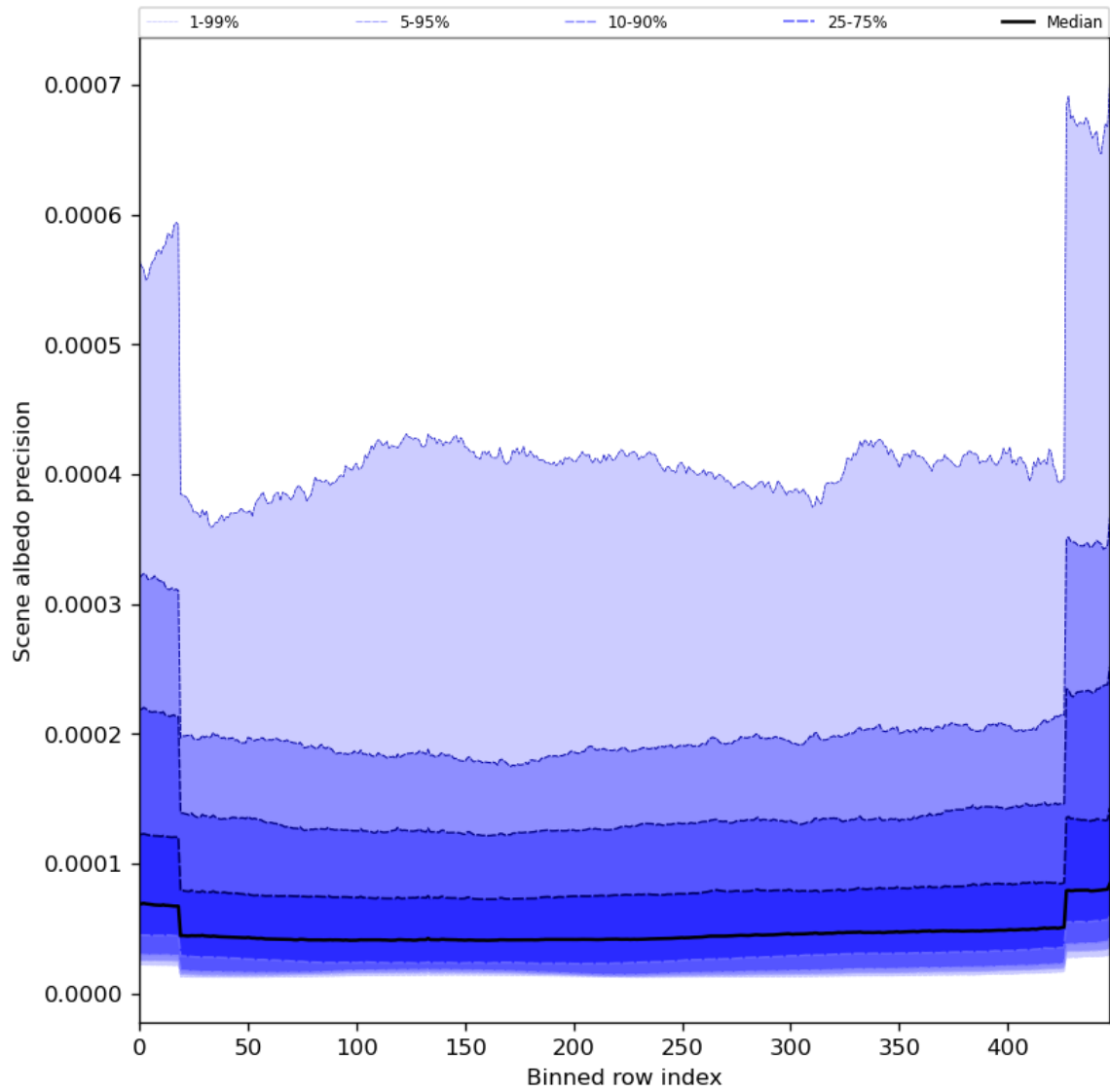
Figure 52: Along track statistics of “Scene albedo precision” for 2023-12-09 to 2023-12-11
