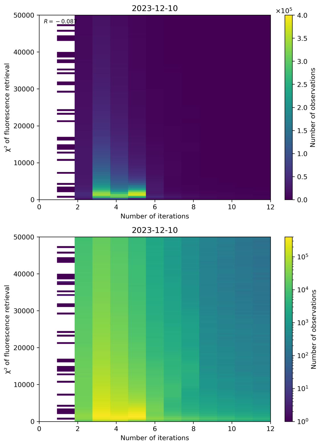
Figure 97: Scatter density plot of “Number of iterations” against “ \chi^2 of fluorescence retrieval” for 2023-12-09 to 2023-12-11.
