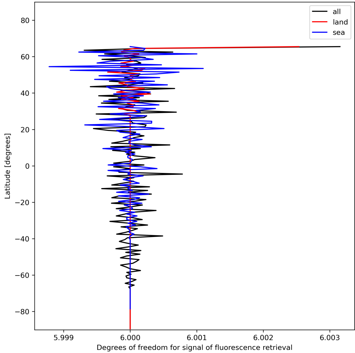
Figure 26: Zonal average of “Degrees of freedom for signal of fluorescence retrieval” for 2023-12-09 to 2023-12-11.
