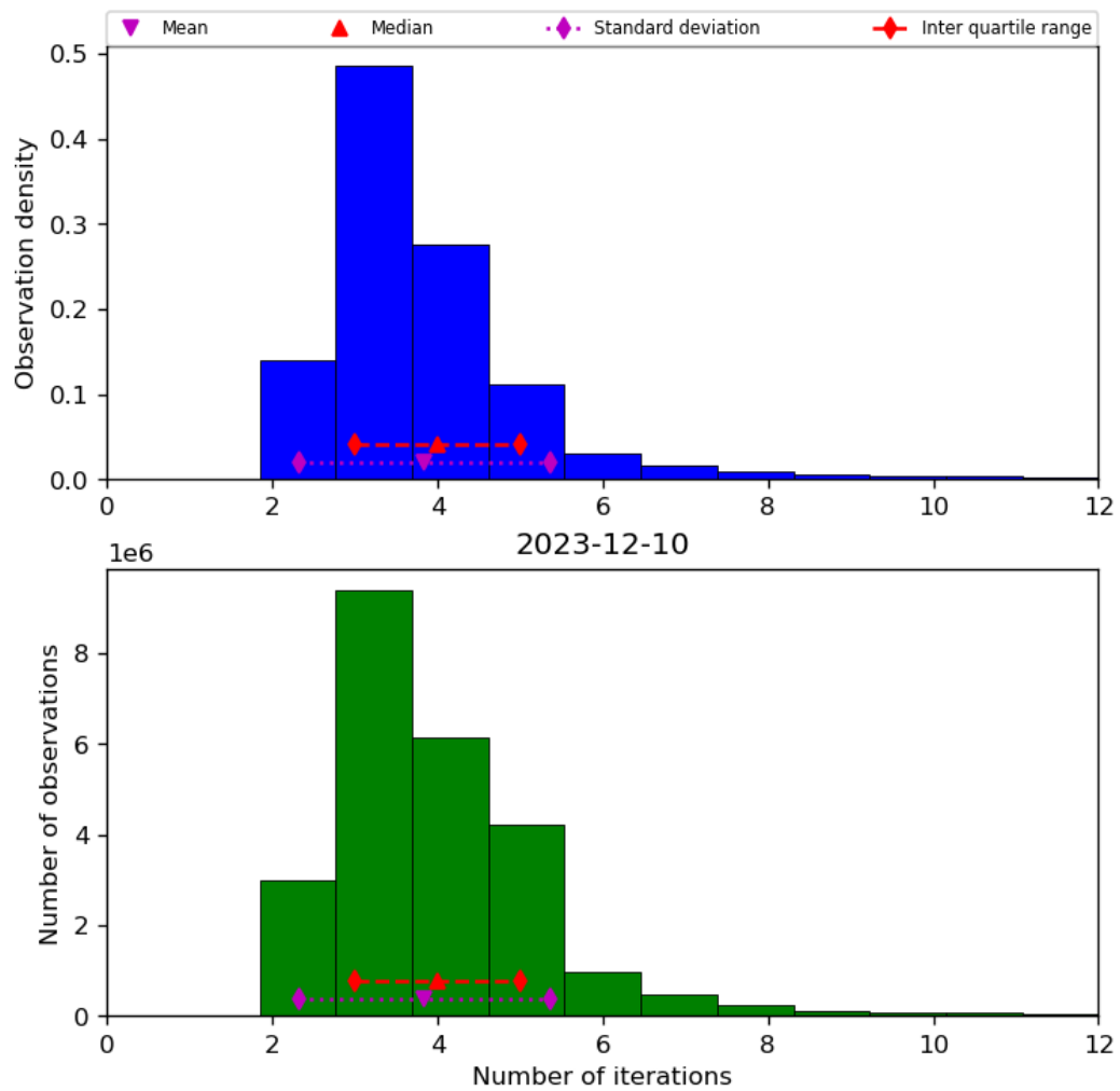
Figure 39: Histogram of “Number of iterations” for 2023-12-09 to 2023-12-11
