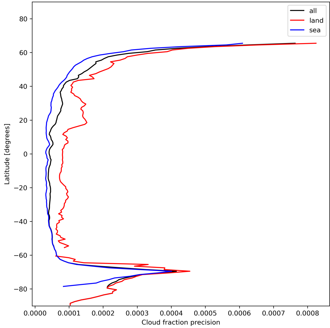
Figure 16: Zonal average of “Cloud fraction precision” for 2023-12-09 to 2023-12-11.
