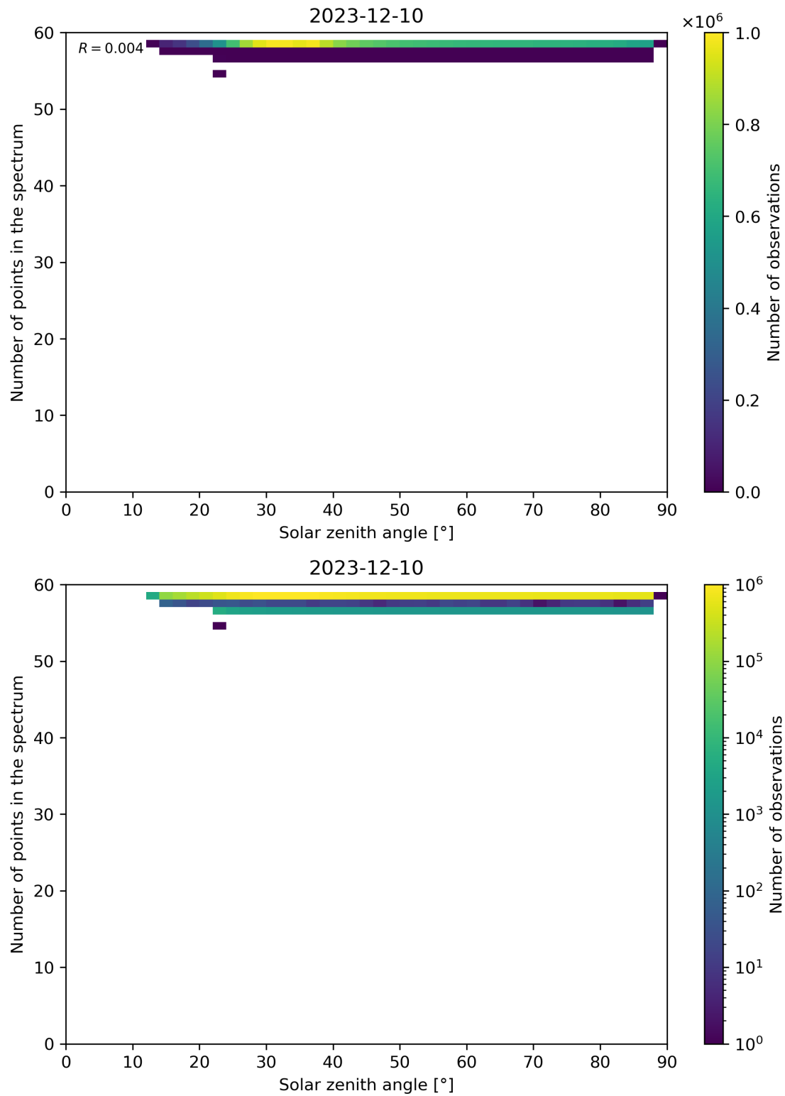
Figure 115: Scatter density plot of “Solar zenith angle” against “Number of points in the spectrum” for 2023-12-09 to 2023-12-11.
