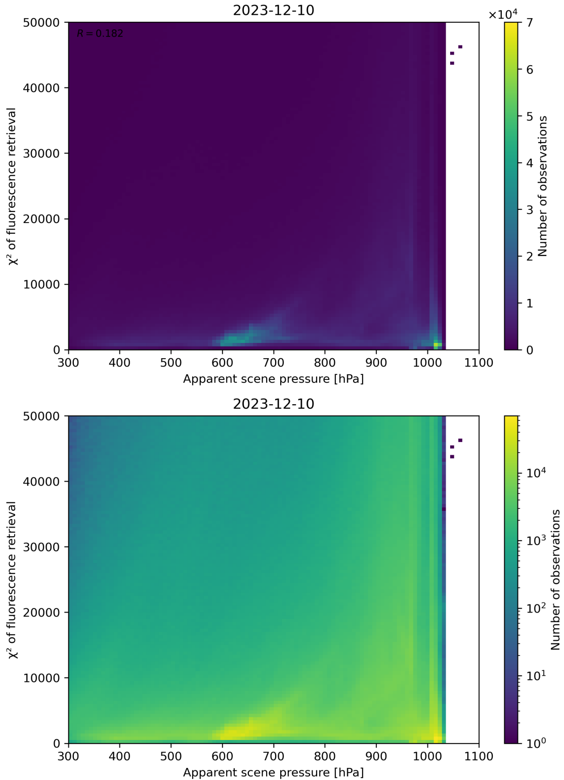
Figure 63: Scatter density plot of “Apparent scene pressure” against “ \chi^2 of fluorescence retrieval” for 2023-12-09 to 2023-12-11.
