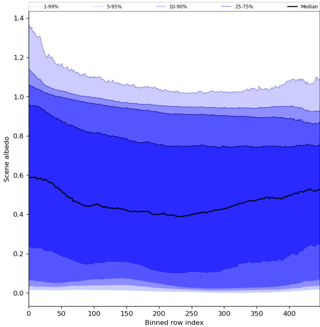
Figure 51: Along track statistics of “Scene albedo” for 2023-12-09 to 2023-12-11
