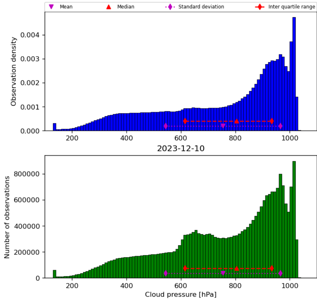
Figure 30: Histogram of “Cloud pressure” for 2023-12-09 to 2023-12-11
