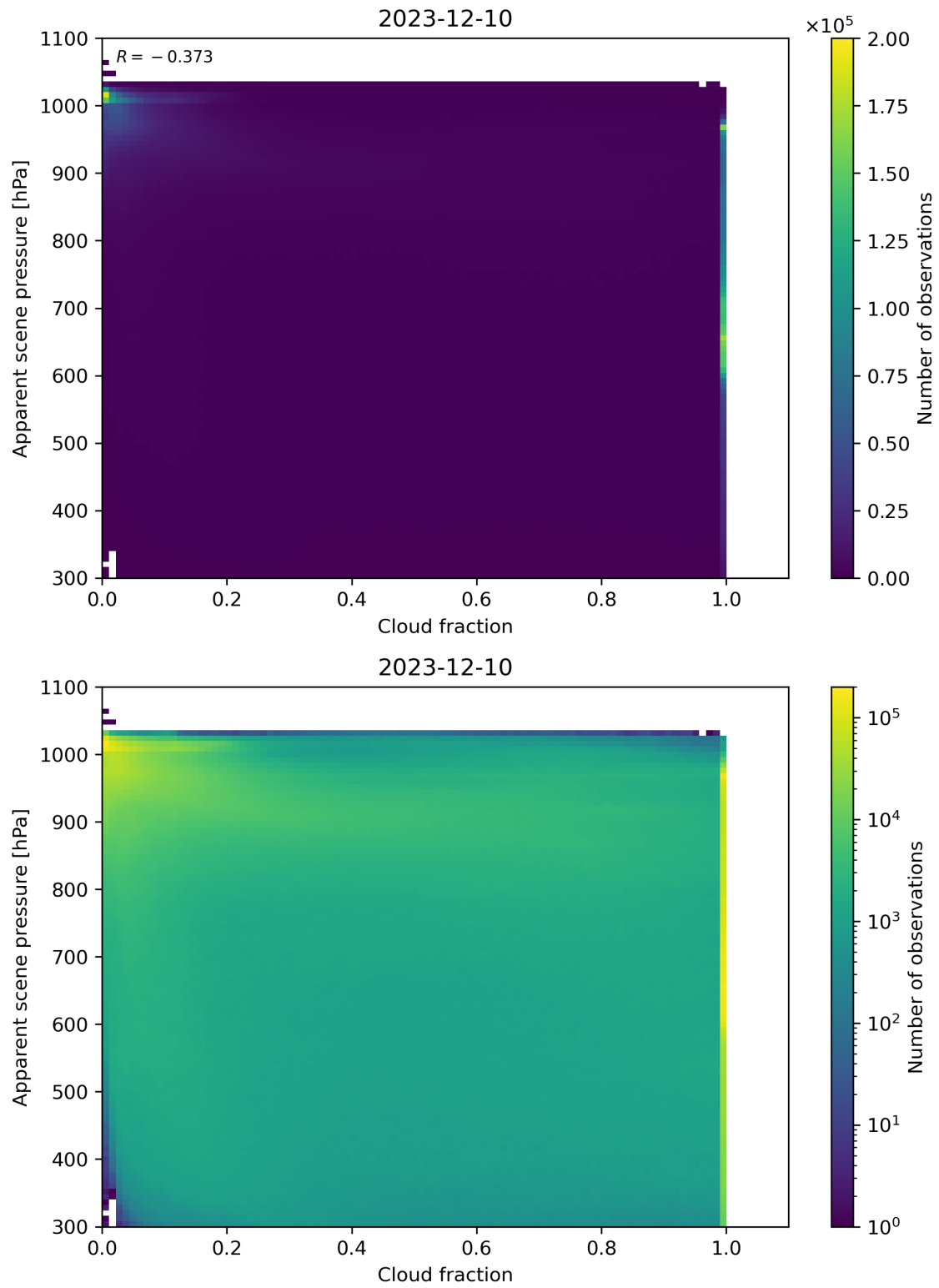
Figure 70: Scatter density plot of “Cloud fraction” against “Apparent scene pressure” for 2023-12-09 to 2023-12-11.
