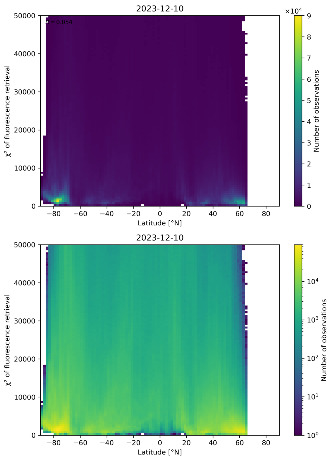
Figure 89: Scatter density plot of “Latitude” against “ \chi^2 of fluorescence retrieval” for 2023-12-09 to 2023-12-11.
