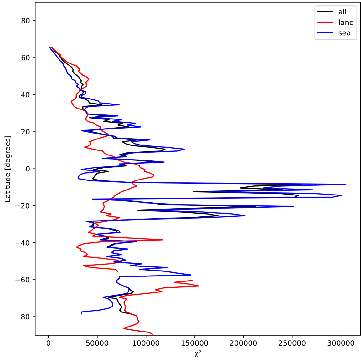
Figure 21: Zonal average of “ \chi^2 ” for 2023-12-09 to 2023-12-11.
