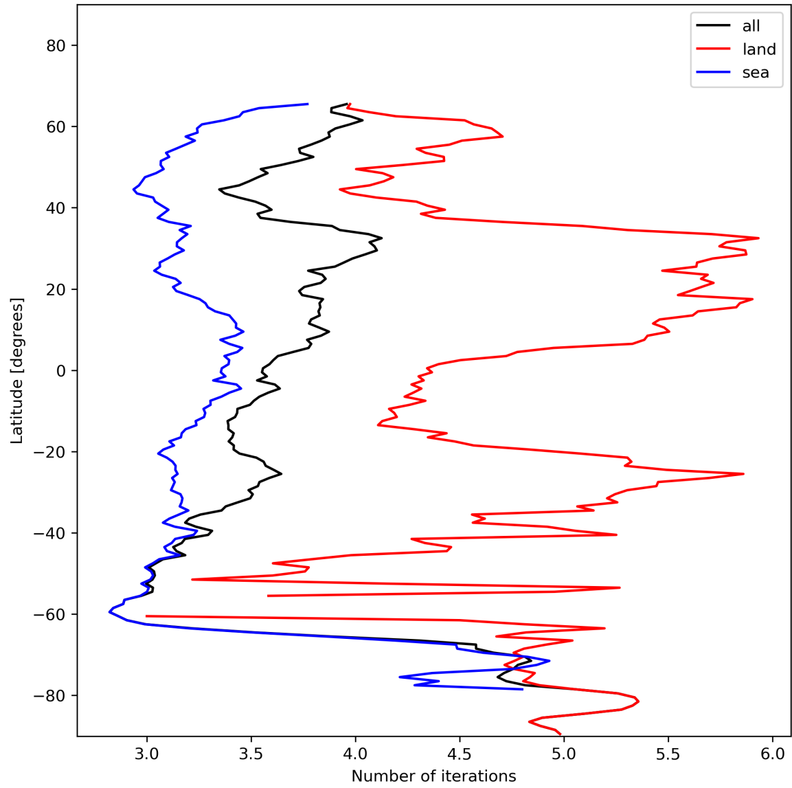
Figure 22: Zonal average of “Number of iterations” for 2023-12-09 to 2023-12-11.
