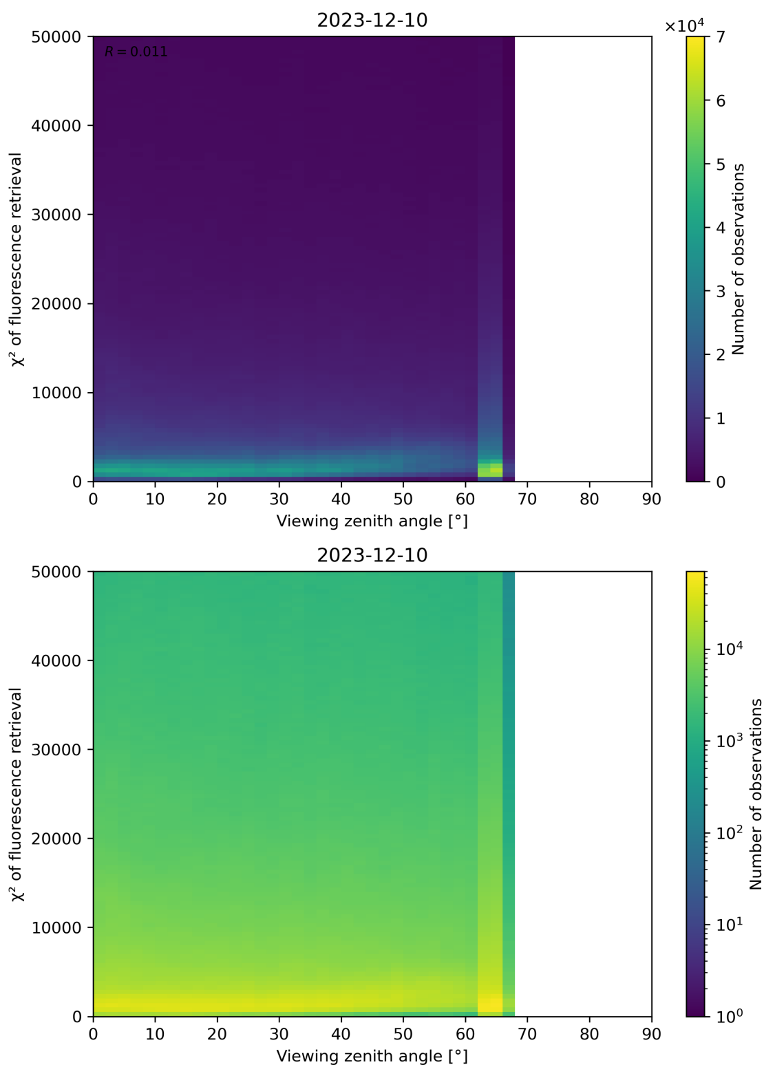
Figure 119: Scatter density plot of “Viewing zenith angle” against “ \chi^2 of fluorescence retrieval” for 2023-12-09 to 2023-12-11.
