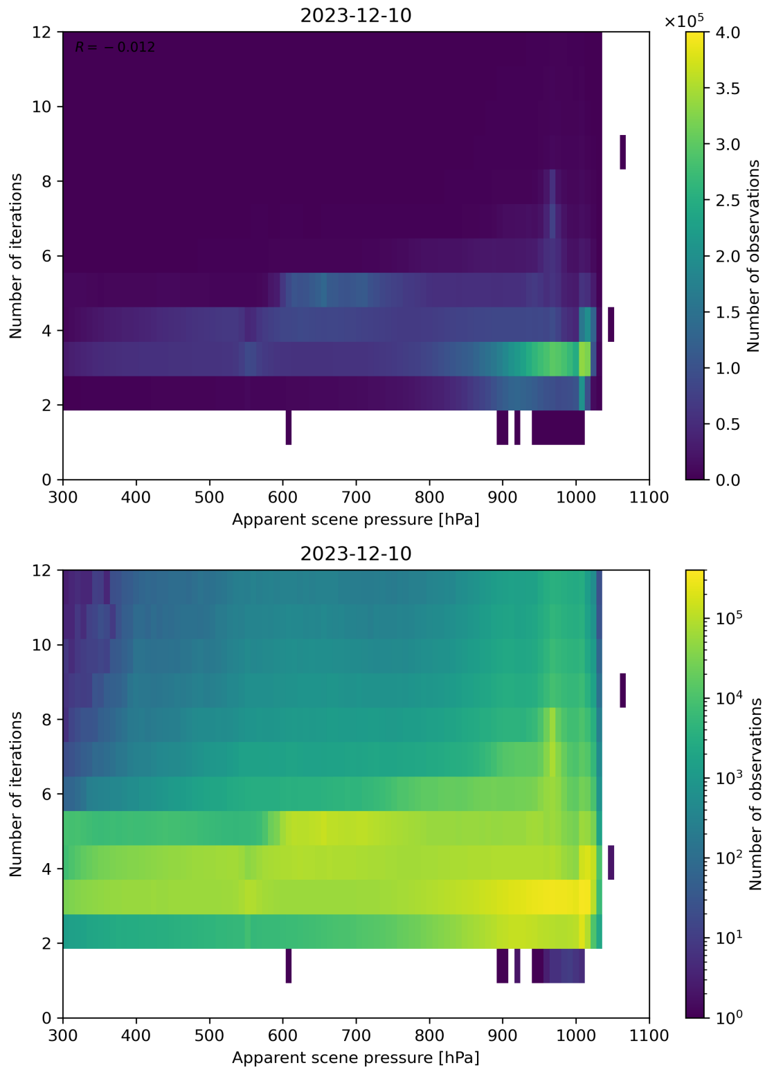
Figure 65: Scatter density plot of “Apparent scene pressure” against “Number of iterations” for 2023-12-09 to 2023-12-11.
