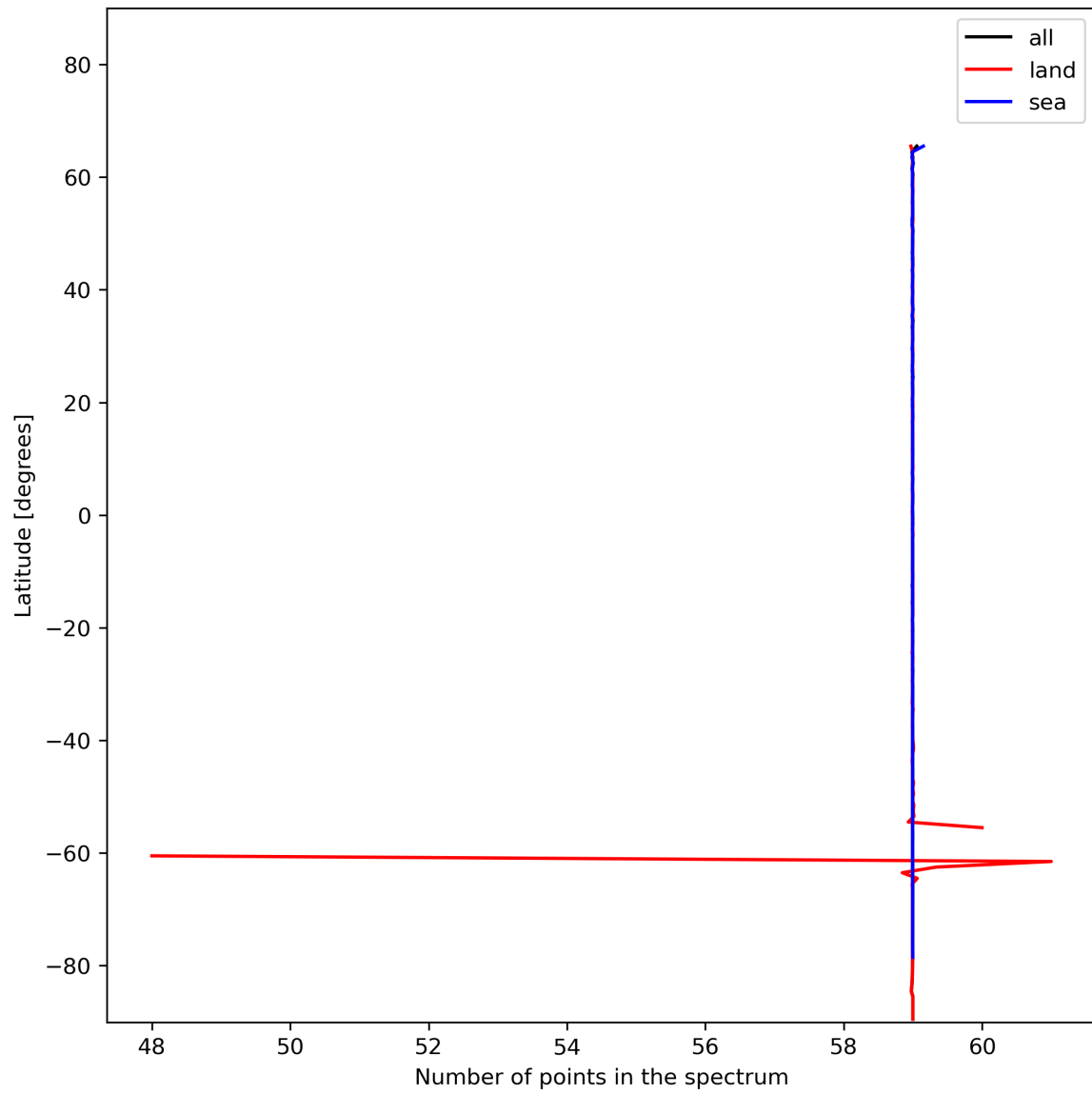
Figure 27: Zonal average of “Number of points in the spectrum” for 2023-12-09 to 2023-12-11.
