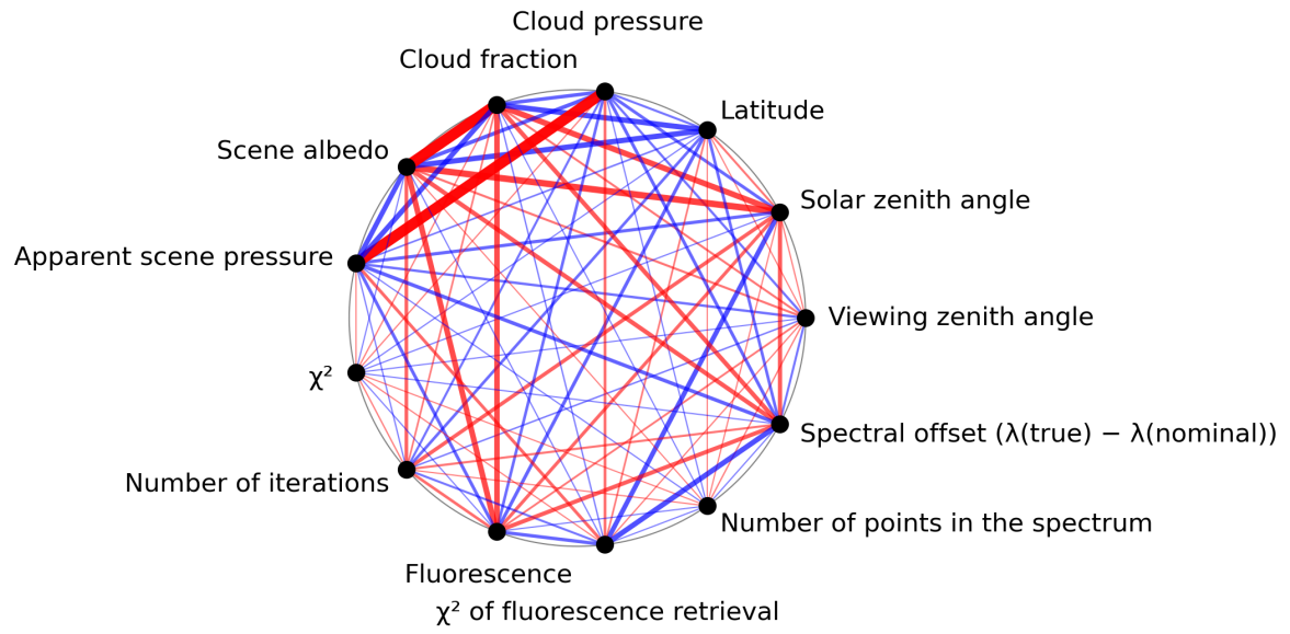
Figure 1: Map of correlation graph for 2023-12-09 to 2023-12-11.
