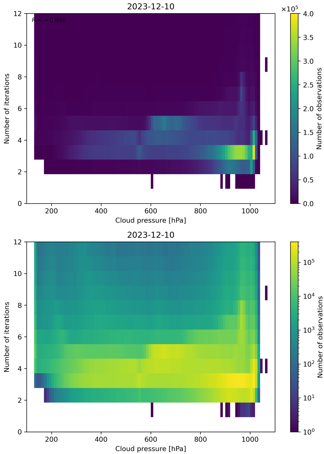
Figure 81: Scatter density plot of “Cloud pressure” against “Number of iterations” for 2023-12-09 to 2023-12-11.
