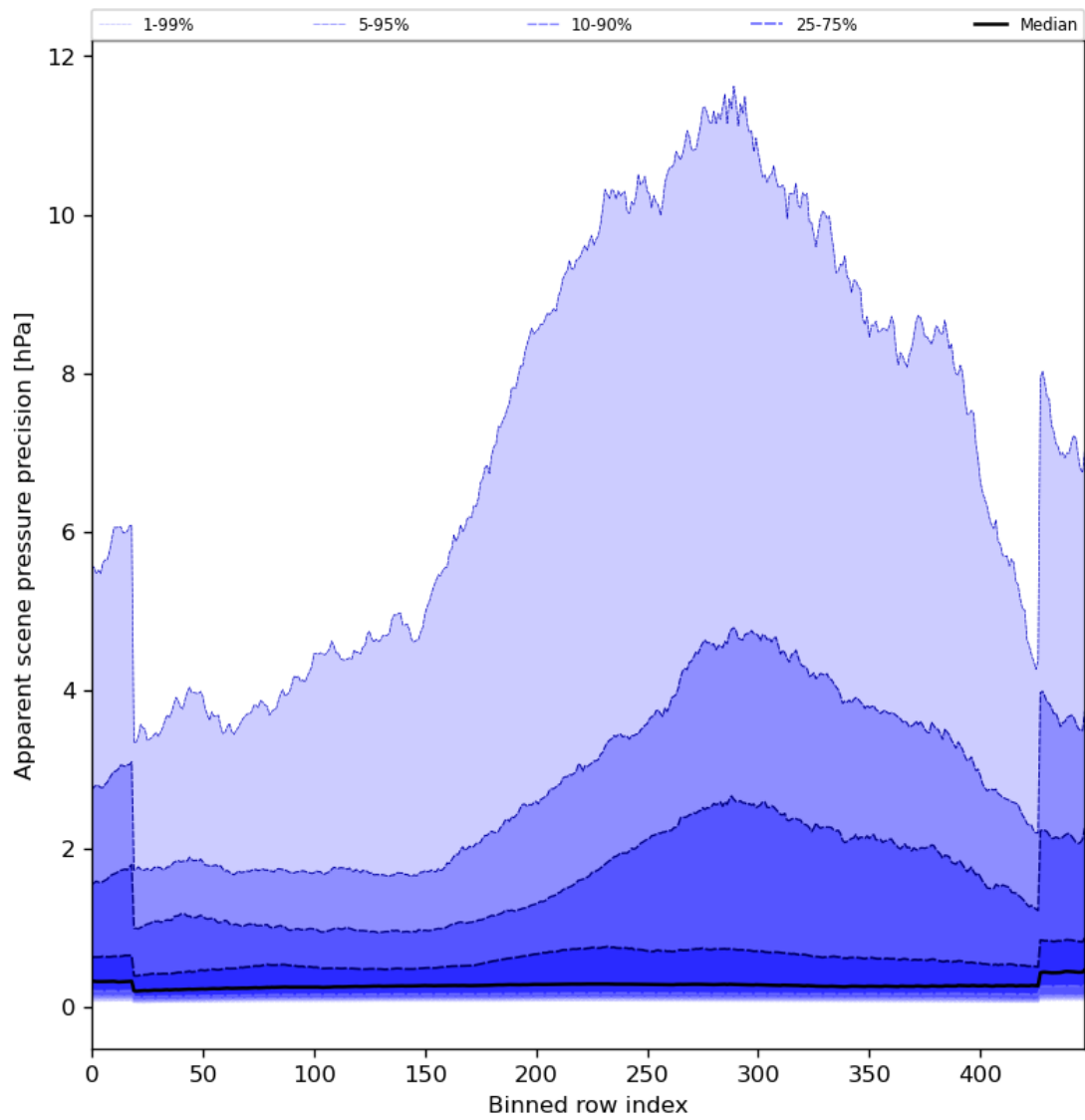
Figure 54: Along track statistics of “Apparent scene pressure precision” for 2023-12-09 to 2023-12-11
