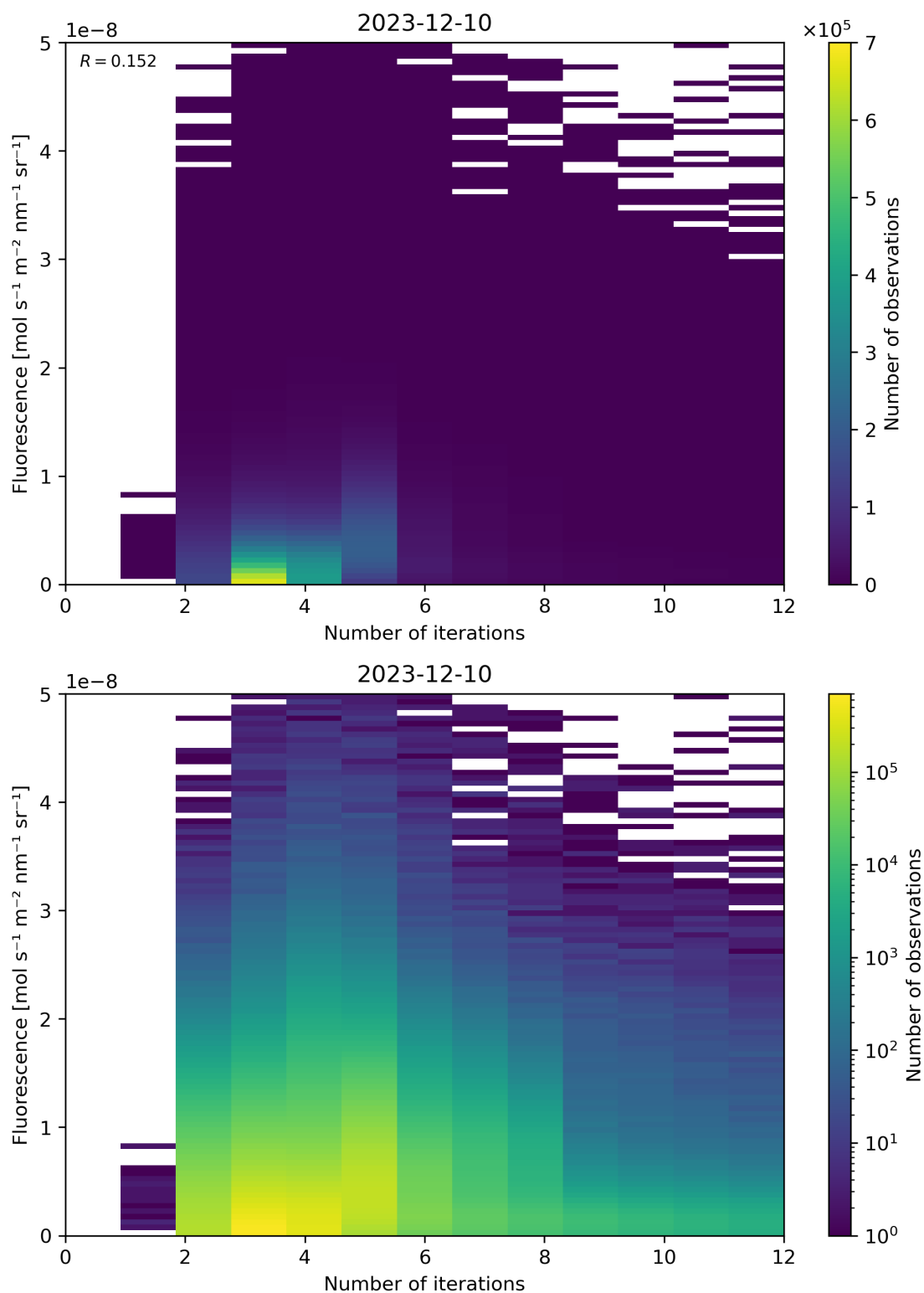
Figure 98: Scatter density plot of “Number of iterations” against “Fluorescence” for 2023-12-09 to 2023-12-11.
