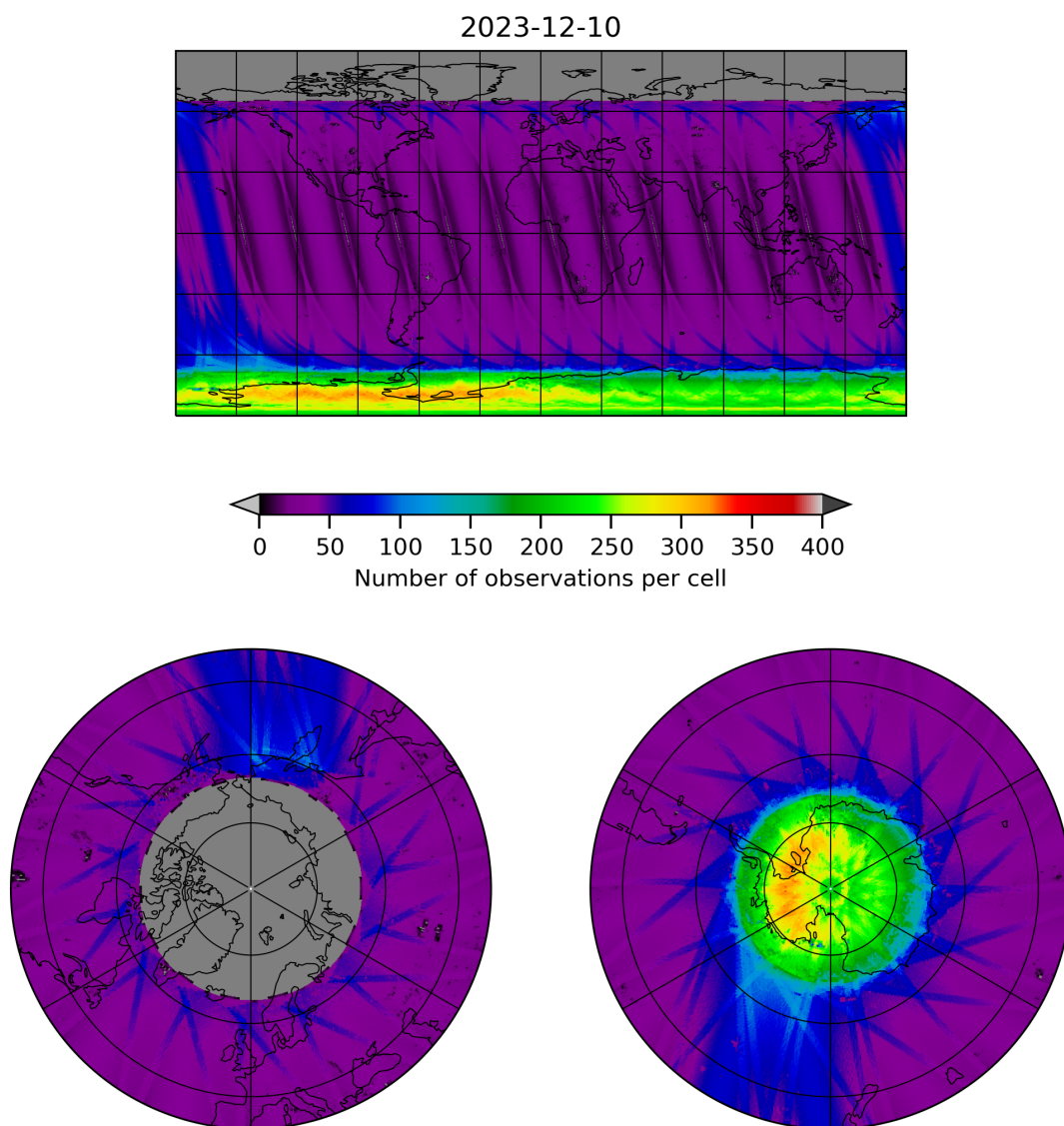
Figure 11: Map of the number of observations for 2023-12-09 to 2023-12-11
