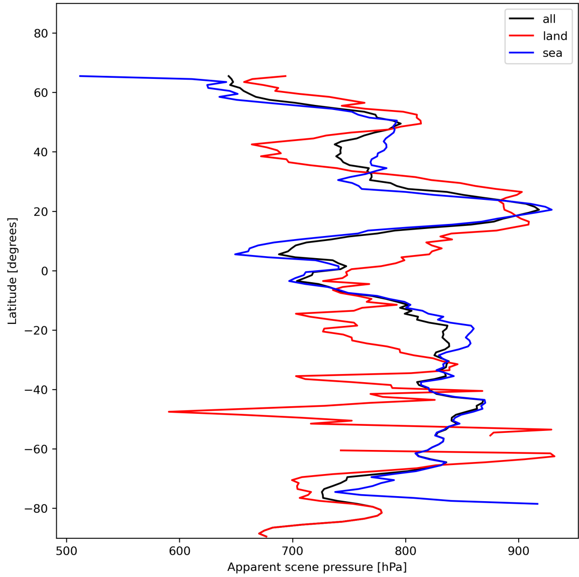
Figure 19: Zonal average of “Apparent scene pressure” for 2023-12-09 to 2023-12-11.
