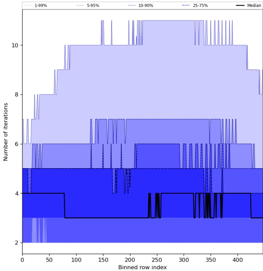
Figure 56: Along track statistics of “Number of iterations” for 2023-12-09 to 2023-12-11
