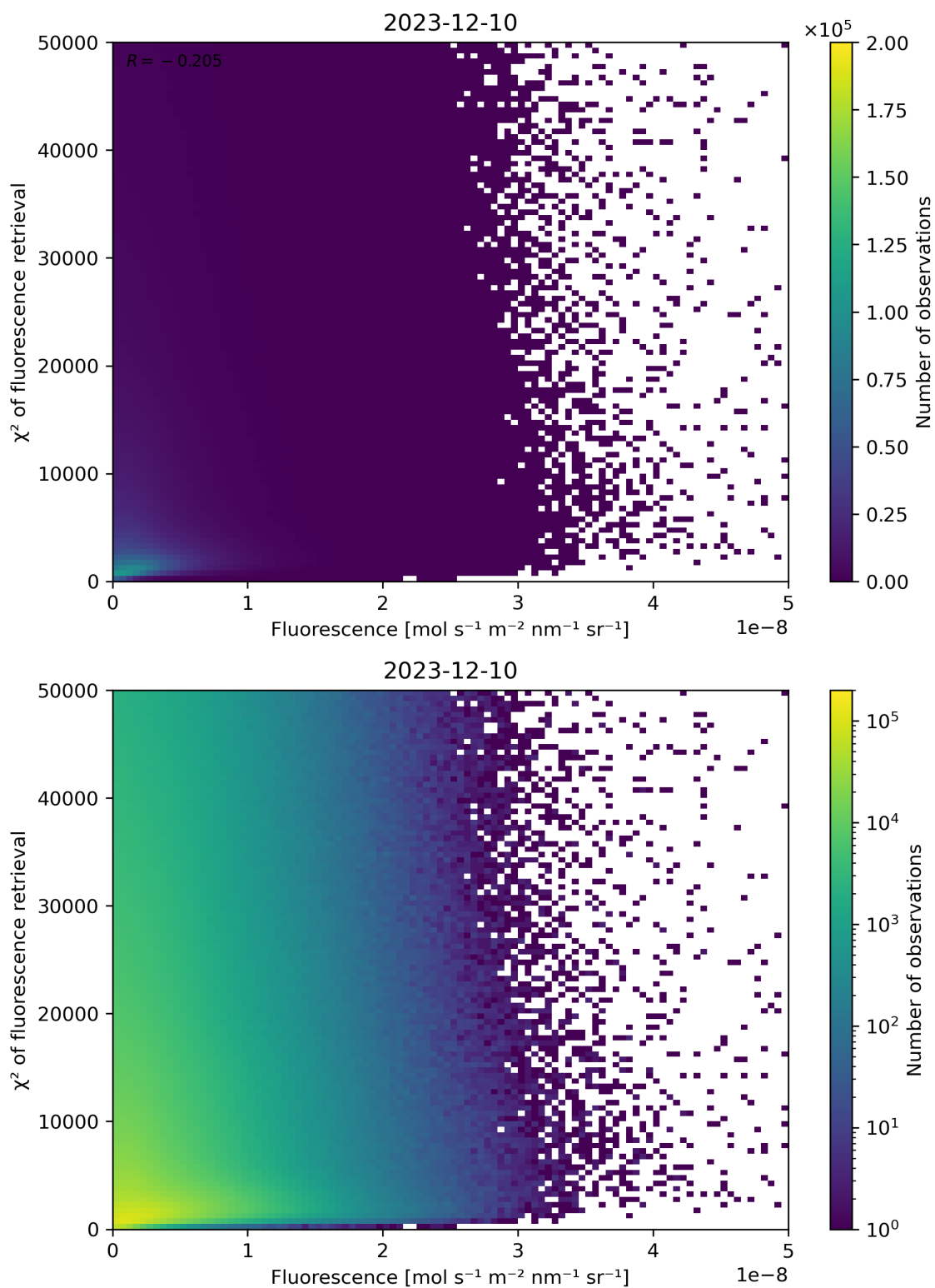
Figure 85: Scatter density plot of “Fluorescence” against “ \chi^2 of fluorescence retrieval” for 2023-12-09 to 2023-12-11.
