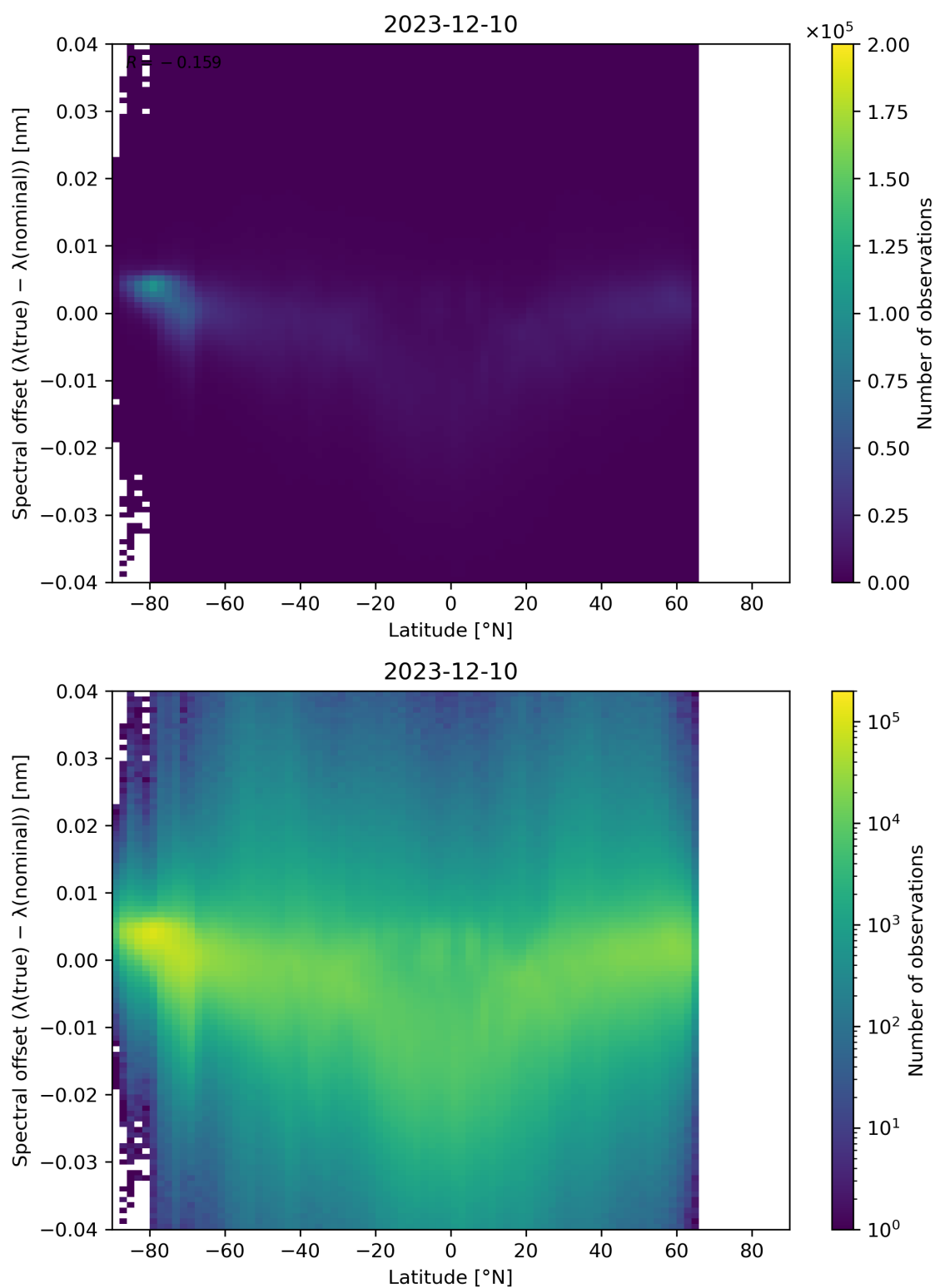
Figure 96: Scatter density plot of “Latitude” against “Spectral offset ( \lambda(\text{true}) - \lambda(\text{nominal}) )” for 2023-12-09 to 2023-12-11.
