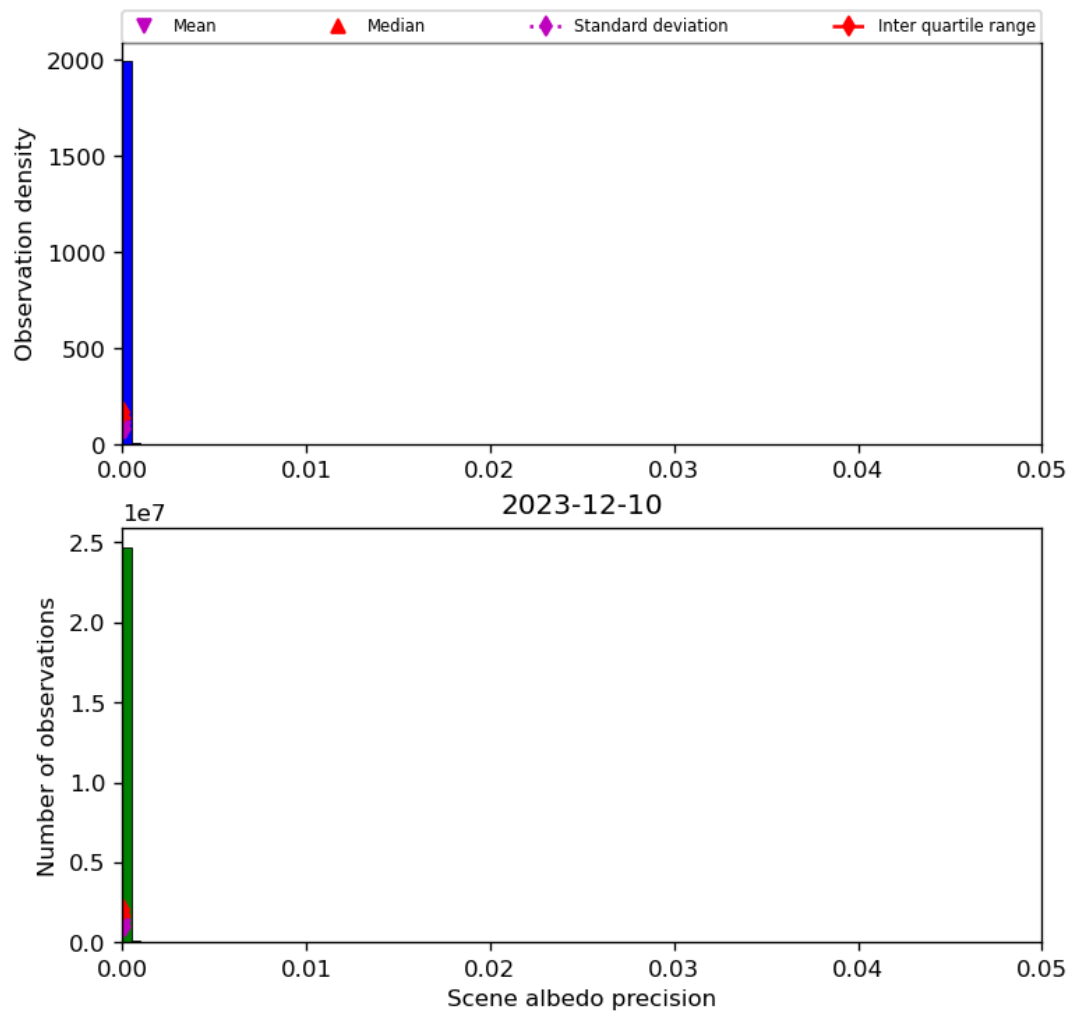
Figure 35: Histogram of “Scene albedo precision” for 2023-12-09 to 2023-12-11
