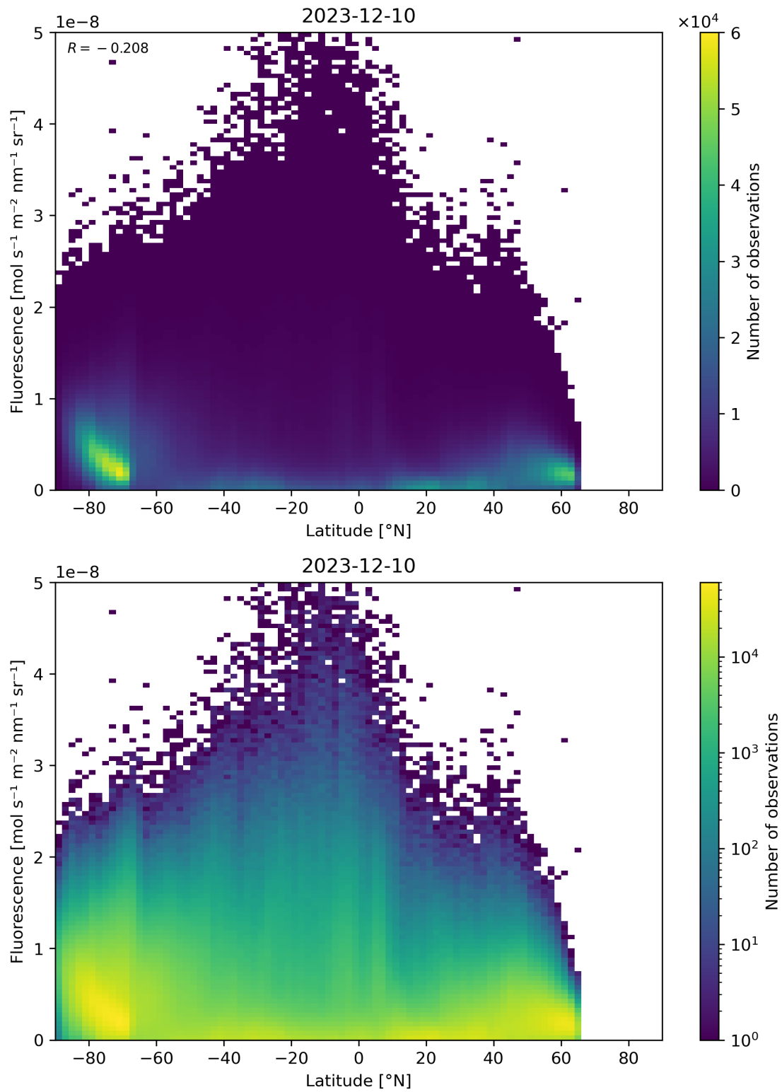
Figure 92: Scatter density plot of “Latitude” against “Fluorescence” for 2023-12-09 to 2023-12-11.
