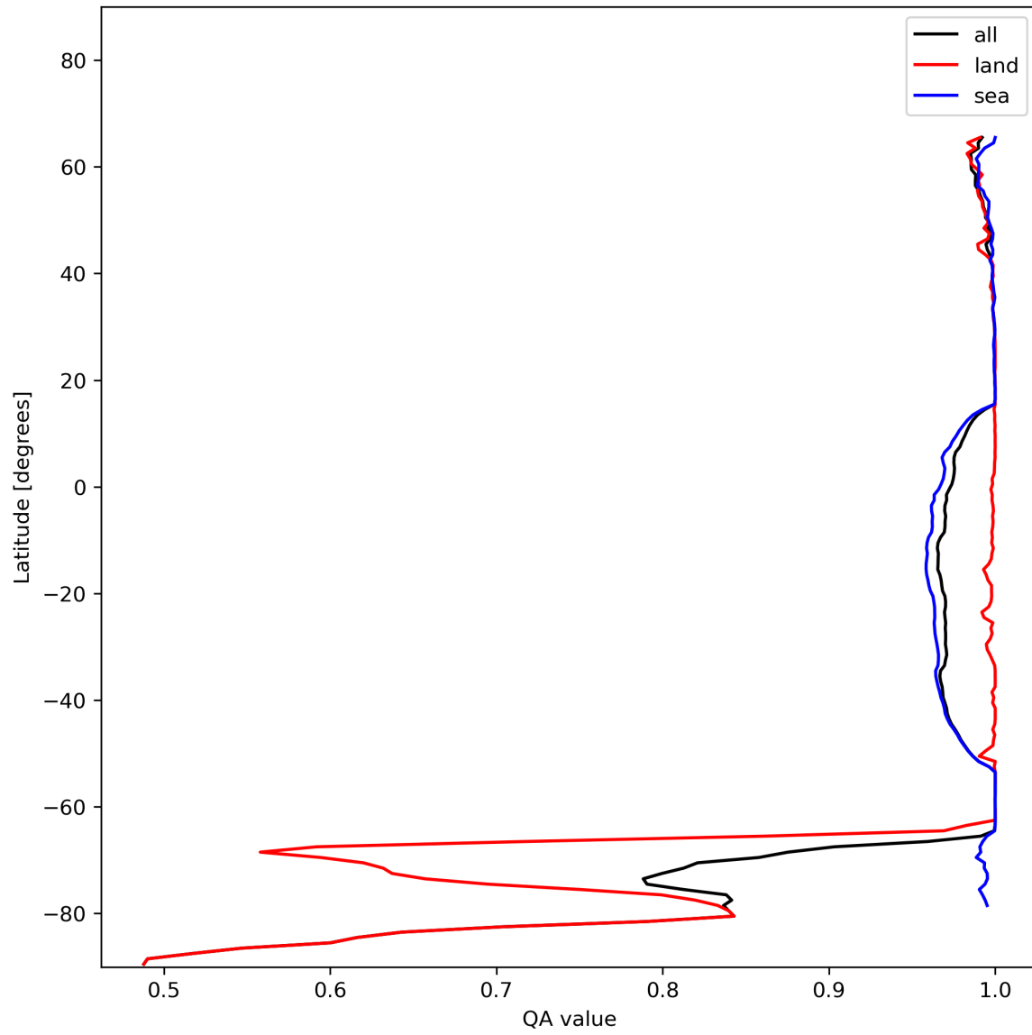
Figure 12: Zonal average of “QA value” for 2023-12-09 to 2023-12-11.
