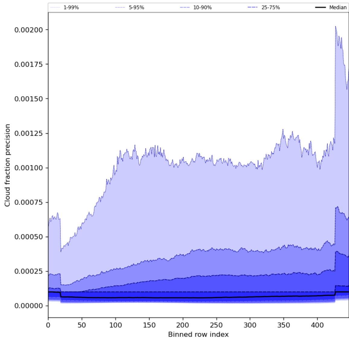
Figure 50: Along track statistics of “Cloud fraction precision” for 2023-12-09 to 2023-12-11
