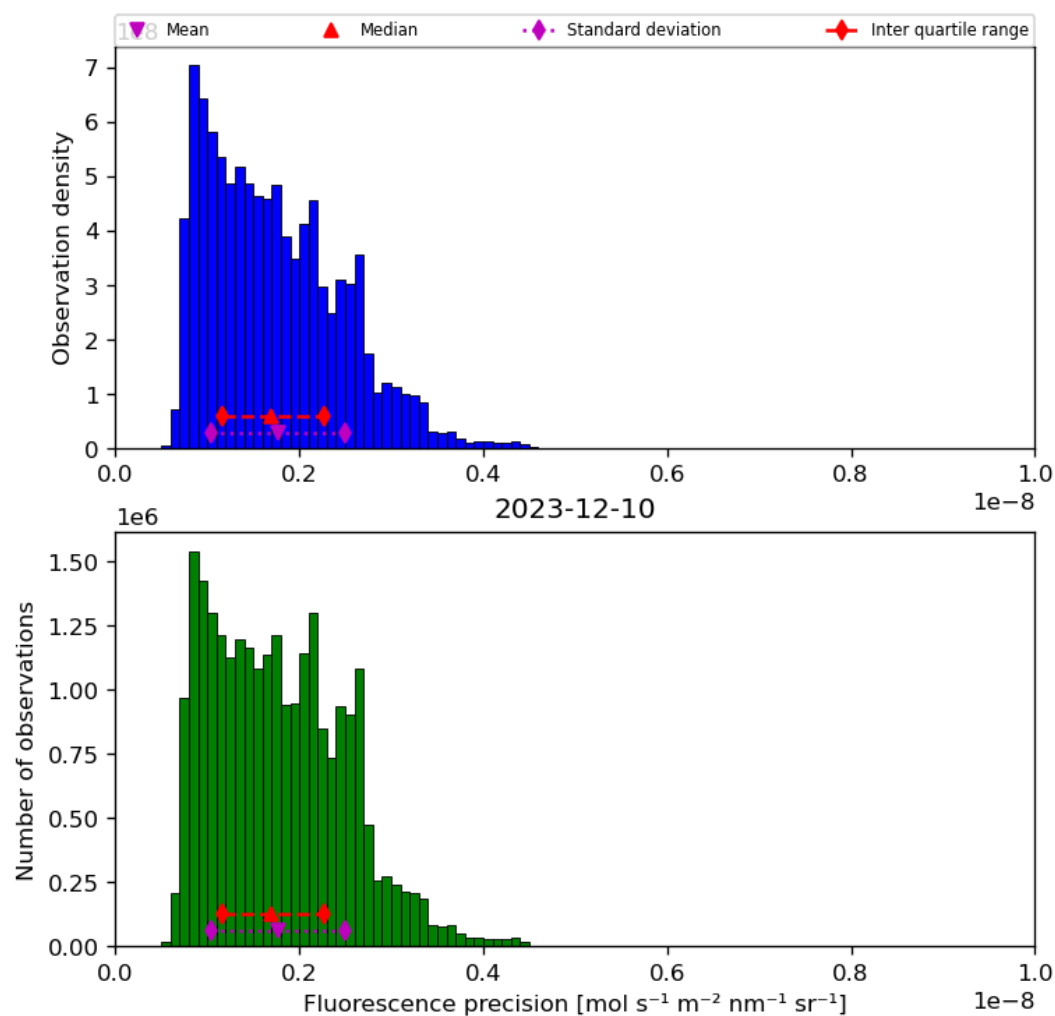
Figure 41: Histogram of “Fluorescence precision” for 2023-12-09 to 2023-12-11
