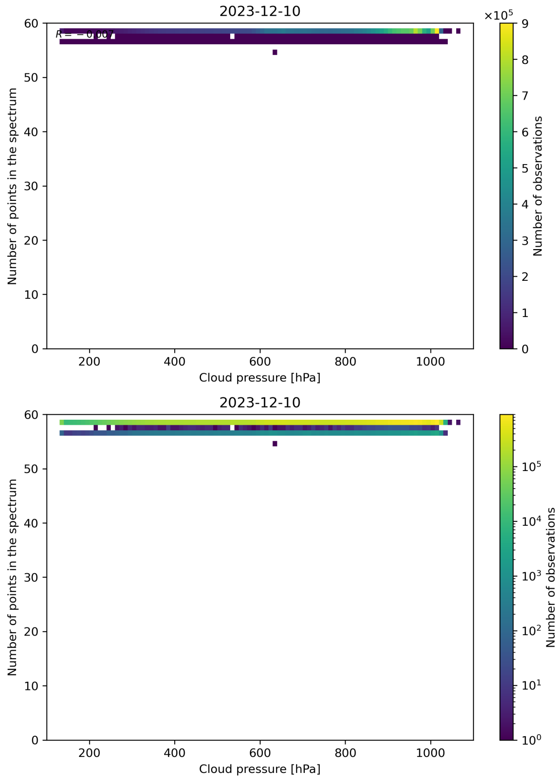
Figure 82: Scatter density plot of “Cloud pressure” against “Number of points in the spectrum” for 2023-12-09 to 2023-12-11.
