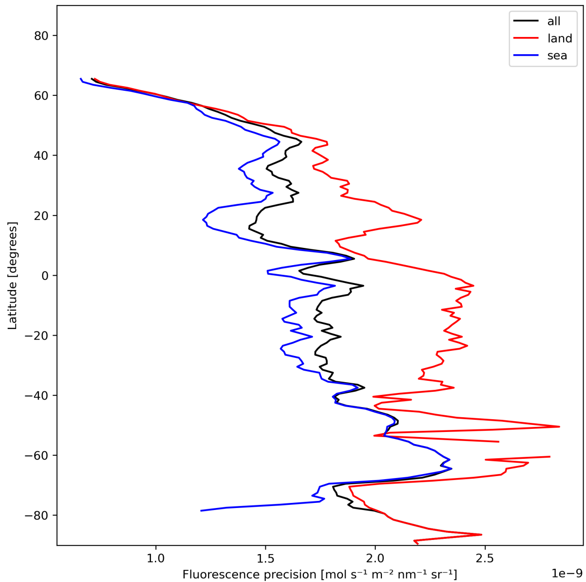
Figure 24: Zonal average of “Fluorescence precision” for 2023-12-09 to 2023-12-11.
