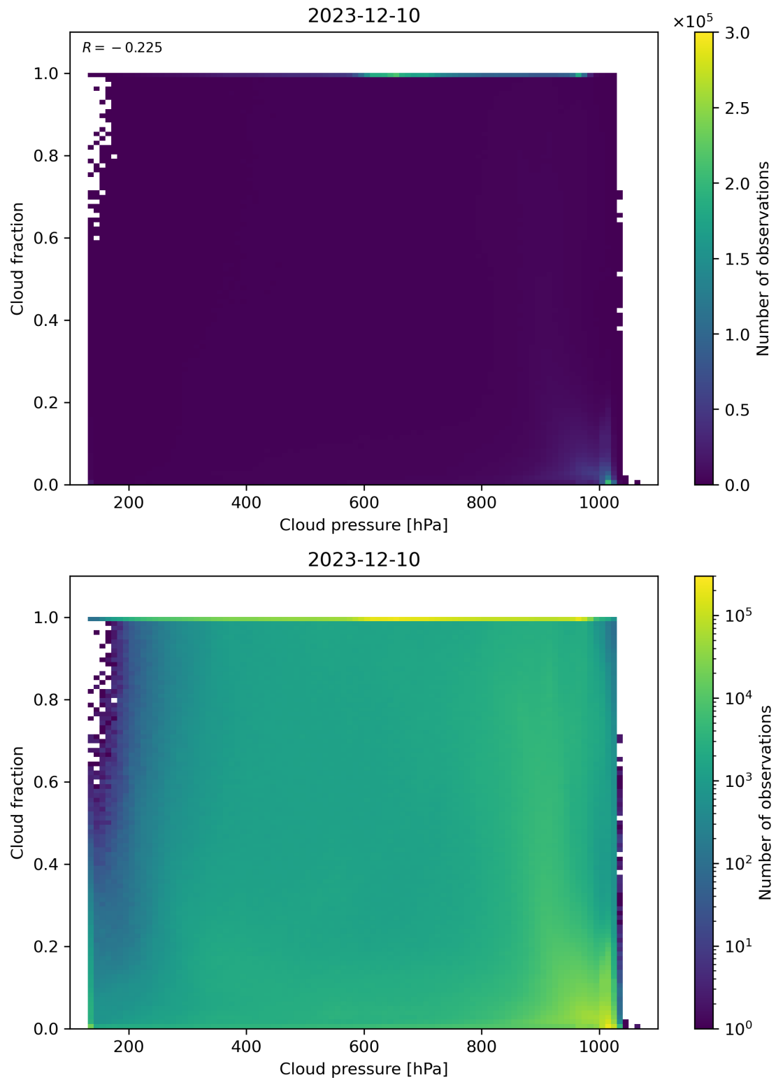
Figure 79: Scatter density plot of “Cloud pressure” against “Cloud fraction” for 2023-12-09 to 2023-12-11.
