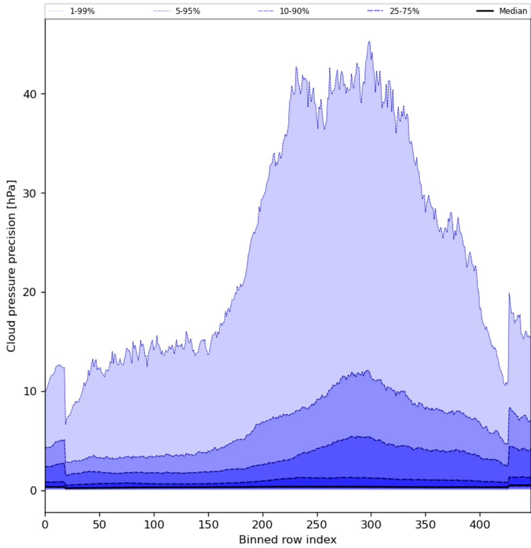
Figure 48: Along track statistics of “Cloud pressure precision” for 2023-12-09 to 2023-12-11
