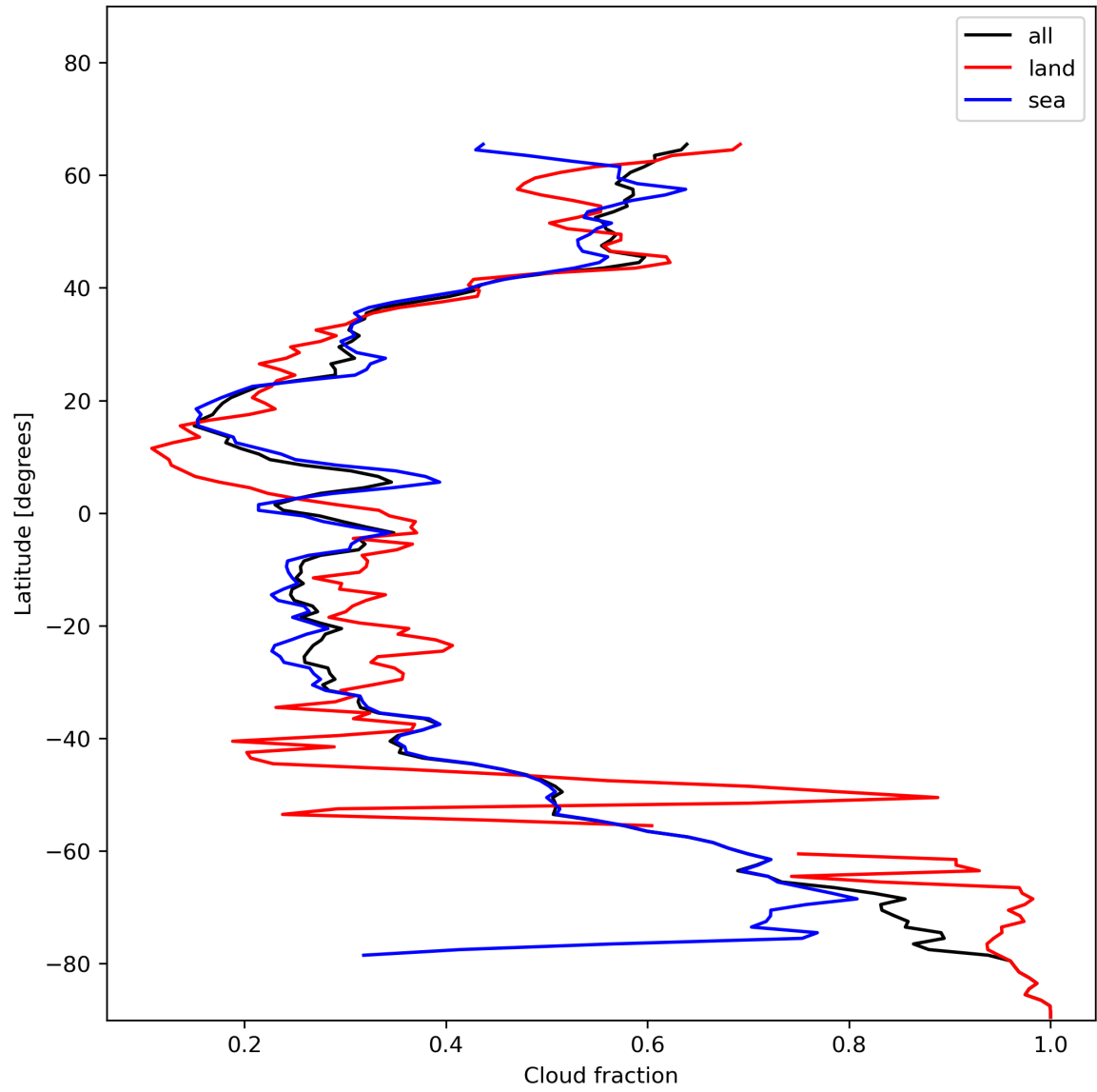
Figure 15: Zonal average of “Cloud fraction” for 2023-12-09 to 2023-12-11.
