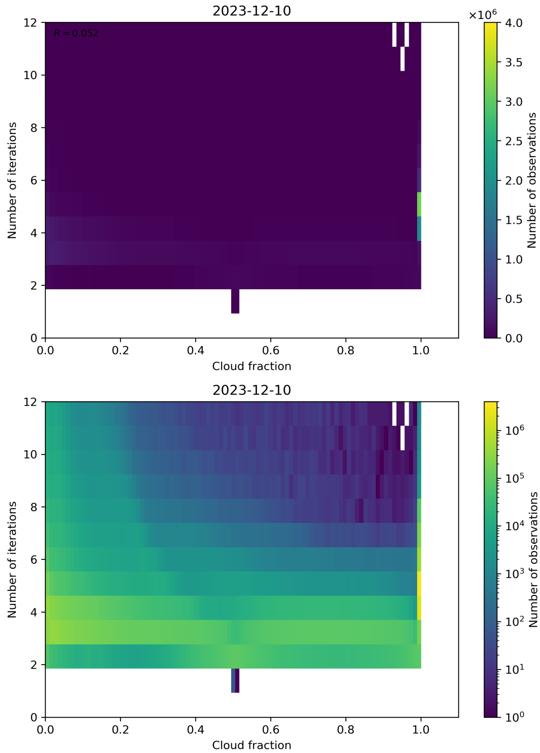
Figure 73: Scatter density plot of “Cloud fraction” against “Number of iterations” for 2023-12-09 to 2023-12-11.
