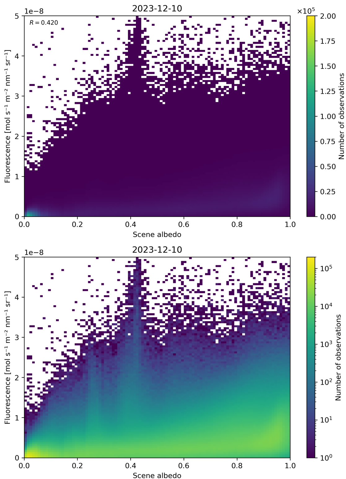
Figure 104: Scatter density plot of “Scene albedo” against “Fluorescence” for 2023-12-09 to 2023-12-11.
