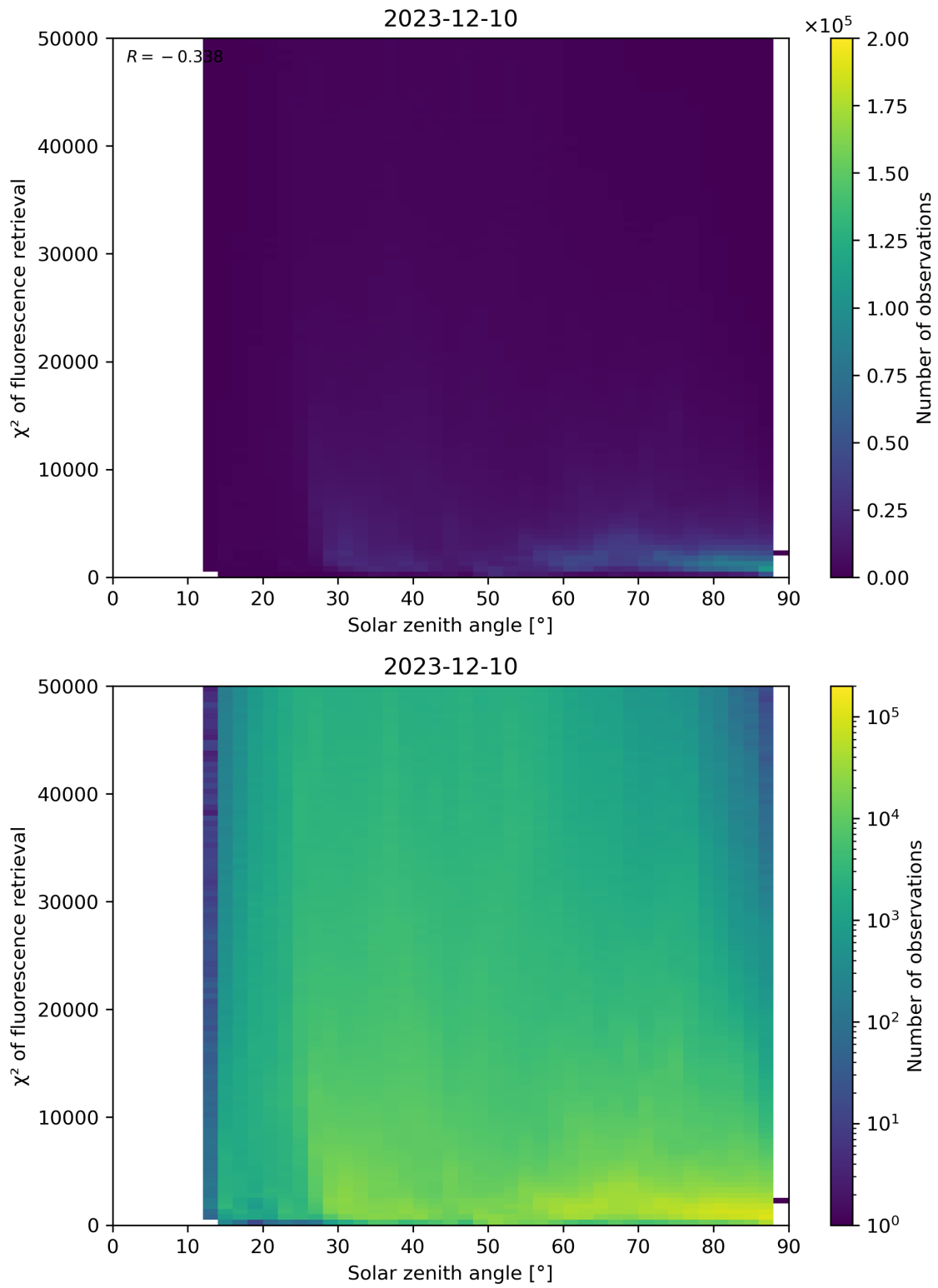
Figure 109: Scatter density plot of “Solar zenith angle” against “ \chi^2 of fluorescence retrieval” for 2023-12-09 to 2023-12-11.
