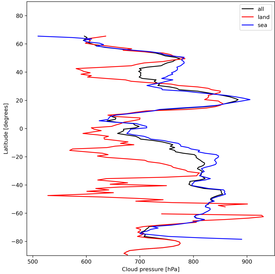
Figure 13: Zonal average of “Cloud pressure” for 2023-12-09 to 2023-12-11.
