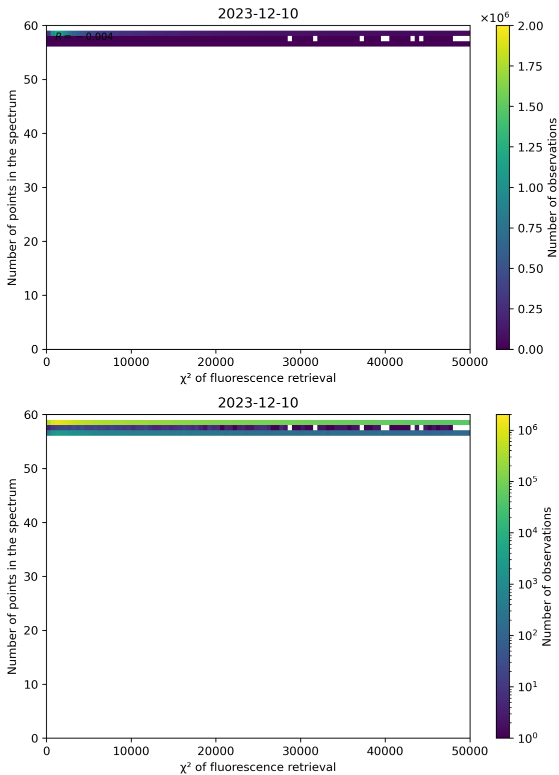
Figure 68: Scatter density plot of " \chi^2 of fluorescence retrieval" against "Number of points in the spectrum" for 2023-12-09 to 2023-12-11.
