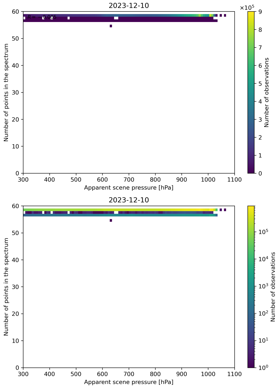
Figure 66: Scatter density plot of “Apparent scene pressure” against “Number of points in the spectrum” for 2023-12-09 to 2023-12-11.
