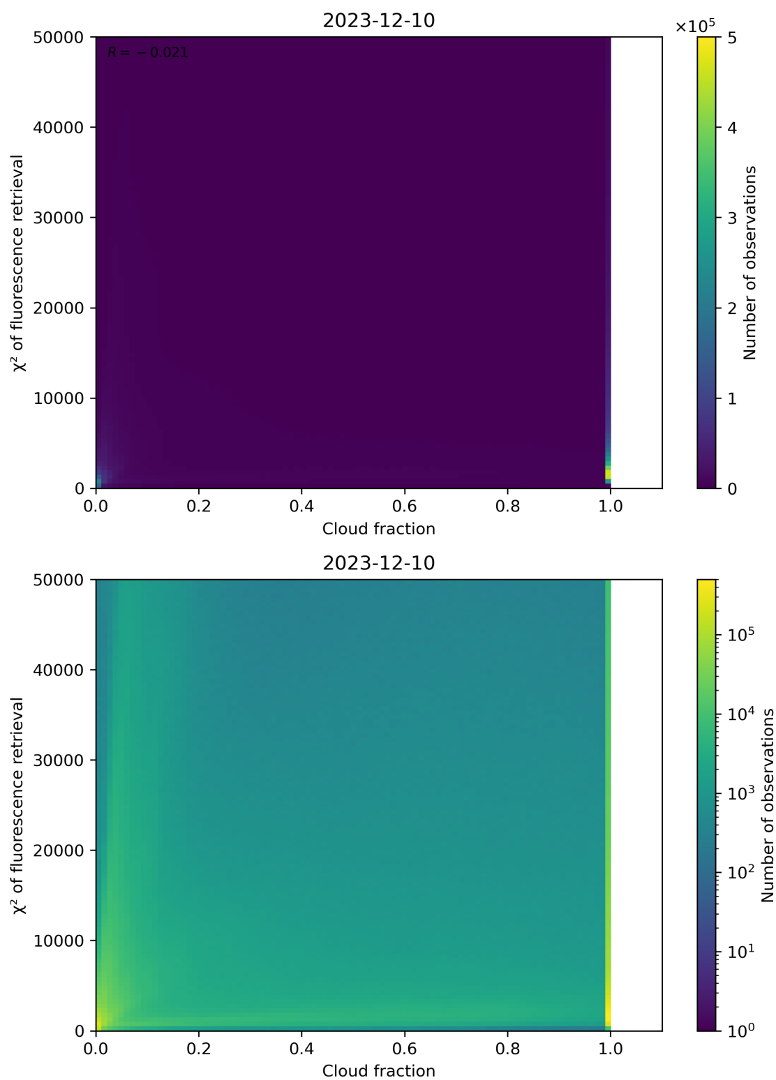
Figure 71: Scatter density plot of “Cloud fraction” against “ \chi^2 of fluorescence retrieval” for 2023-12-09 to 2023-12-11.
