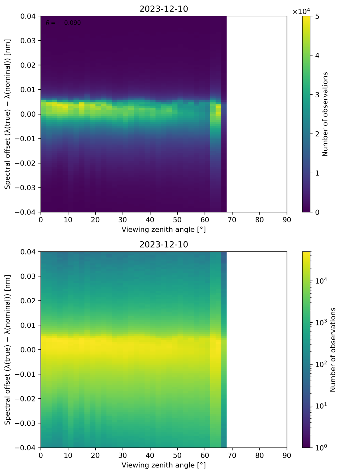
Figure 128: Scatter density plot of “Viewing zenith angle” against “Spectral offset ( \lambda(\text{true}) - \lambda(\text{nominal}) )” for 2023-12-09 to 2023-12-11.
