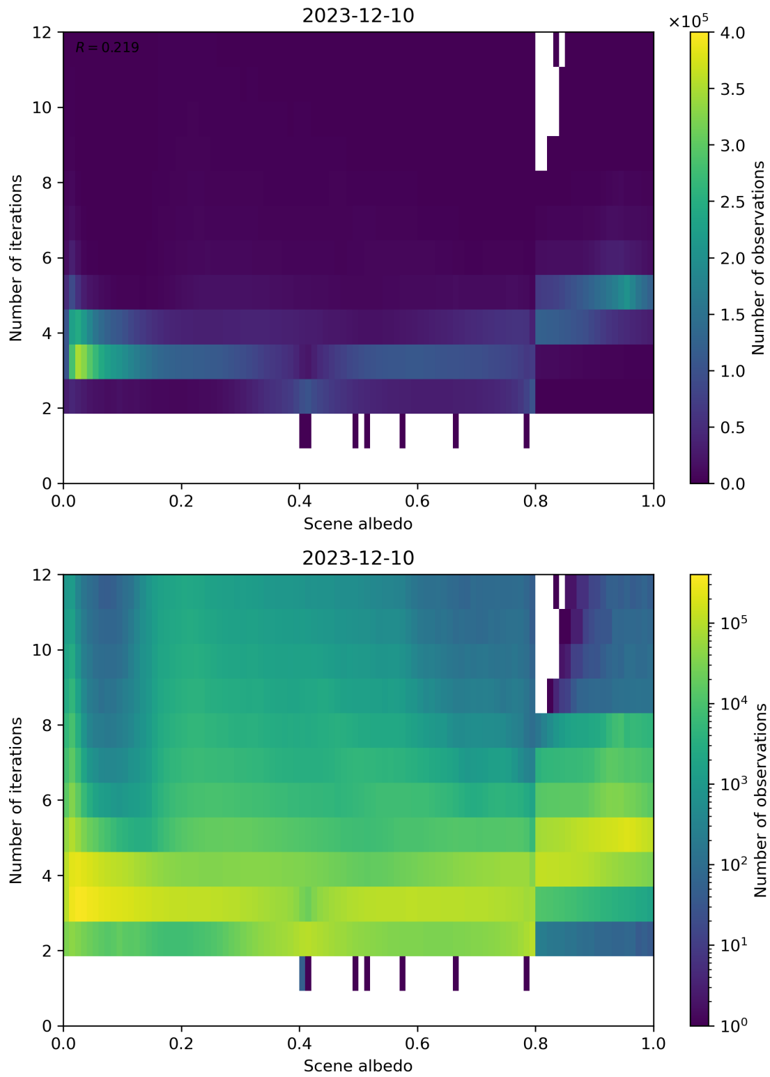
Figure 105: Scatter density plot of “Scene albedo” against “Number of iterations” for 2023-12-09 to 2023-12-11.
