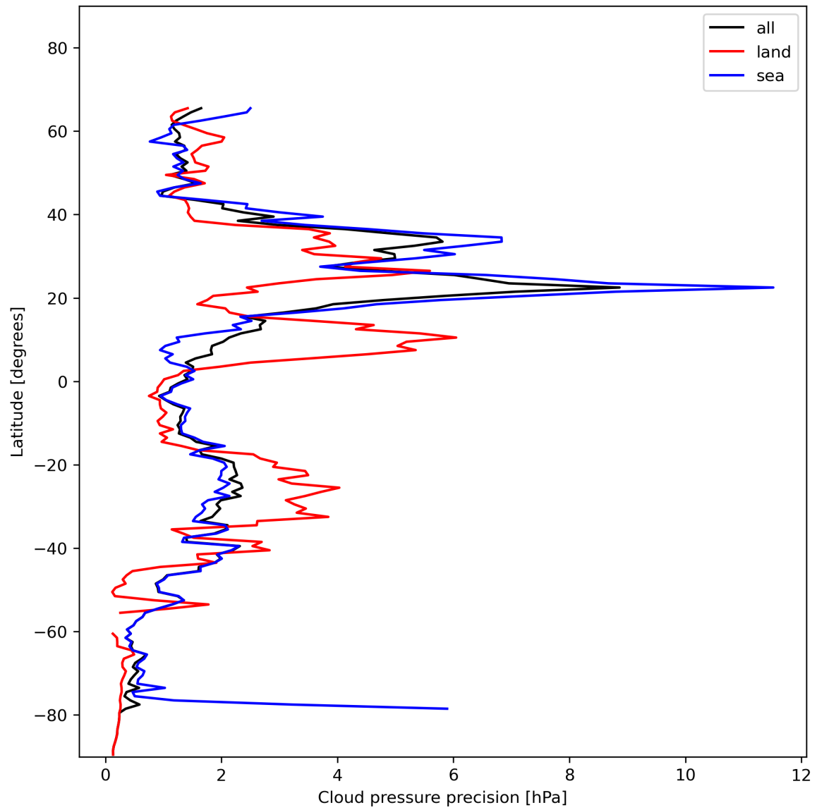
Figure 14: Zonal average of “Cloud pressure precision” for 2023-12-09 to 2023-12-11.
