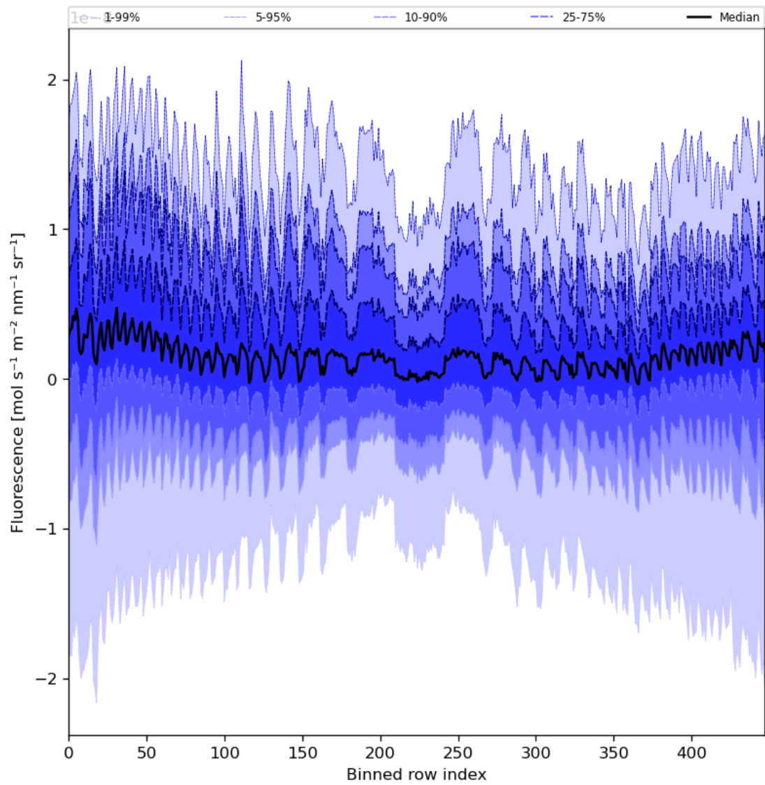
Figure 57: Along track statistics of “Fluorescence” for 2023-12-09 to 2023-12-11
