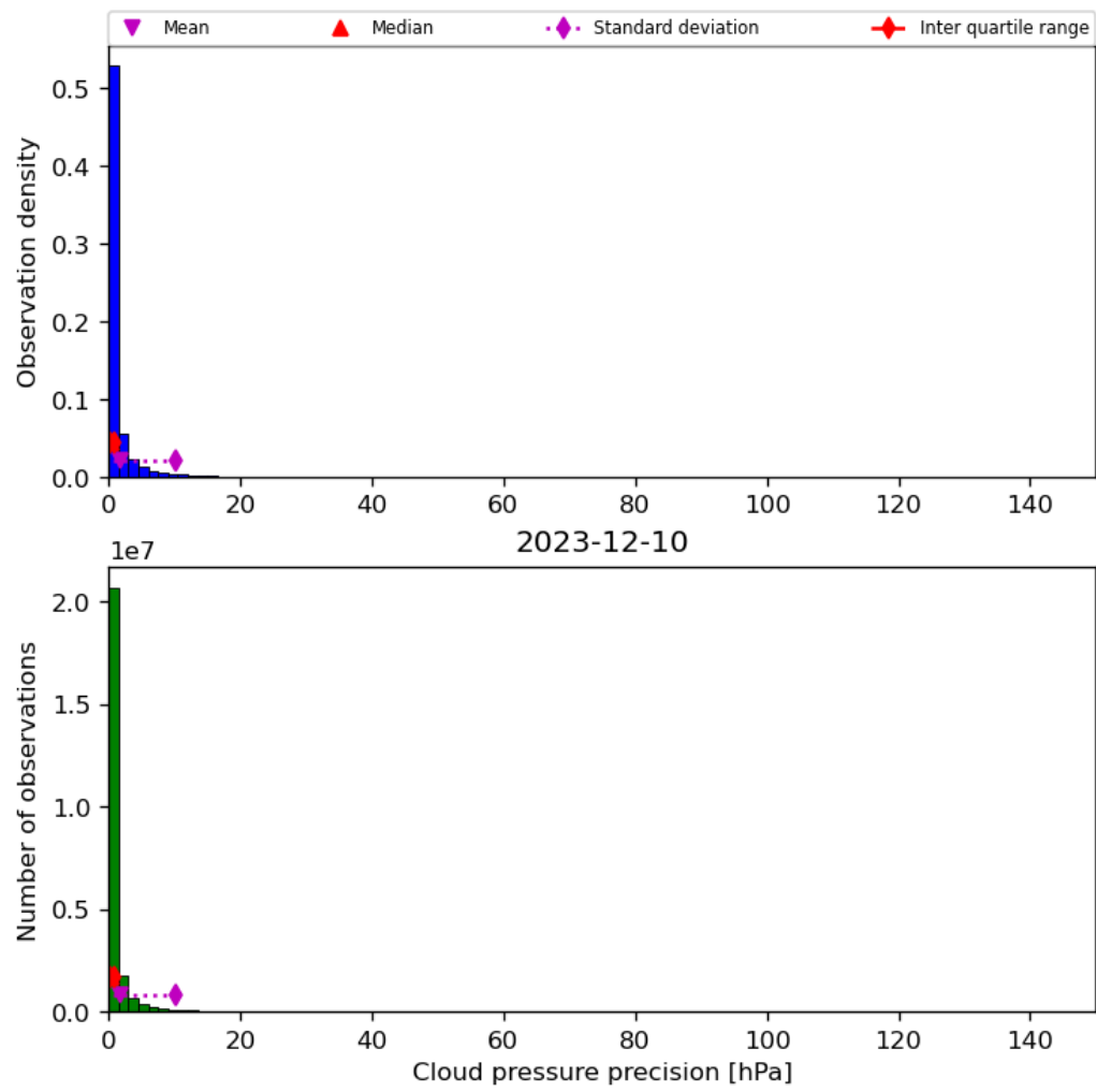
Figure 31: Histogram of “Cloud pressure precision” for 2023-12-09 to 2023-12-11
