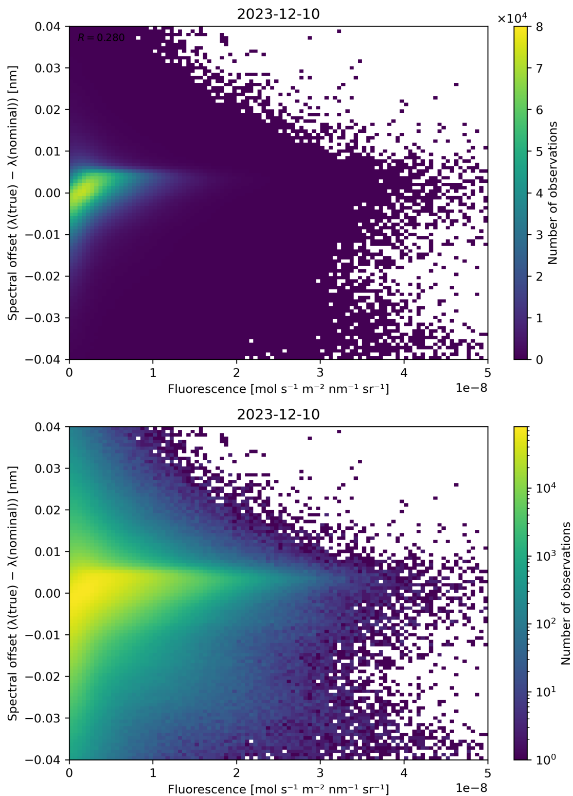
Figure 87: Scatter density plot of “Fluorescence” against “Spectral offset ( \lambda(\text{true}) - \lambda(\text{nominal}) )” for 2023-12-09 to 2023-12-11.
