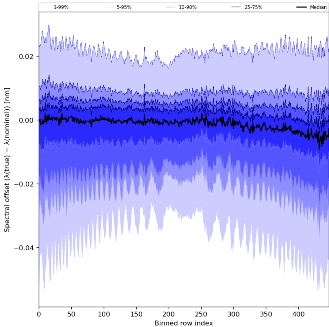
Figure 62: Along track statistics of “Spectral offset ( \lambda(\text{true}) - \lambda(\text{nominal}) )” for 2023-12-09 to 2023-12-11
