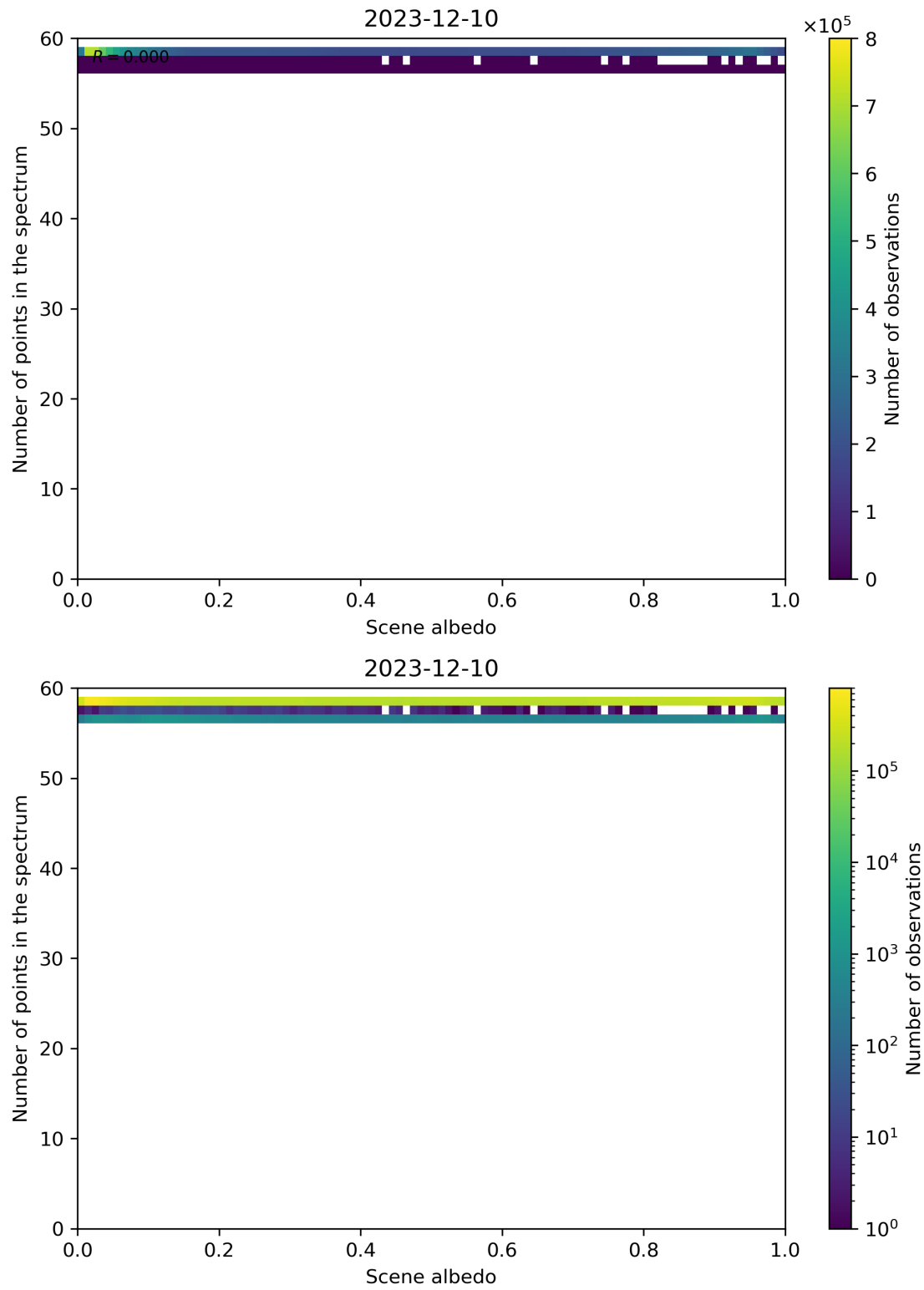
Figure 106: Scatter density plot of “Scene albedo” against “Number of points in the spectrum” for 2023-12-09 to 2023-12-11.
