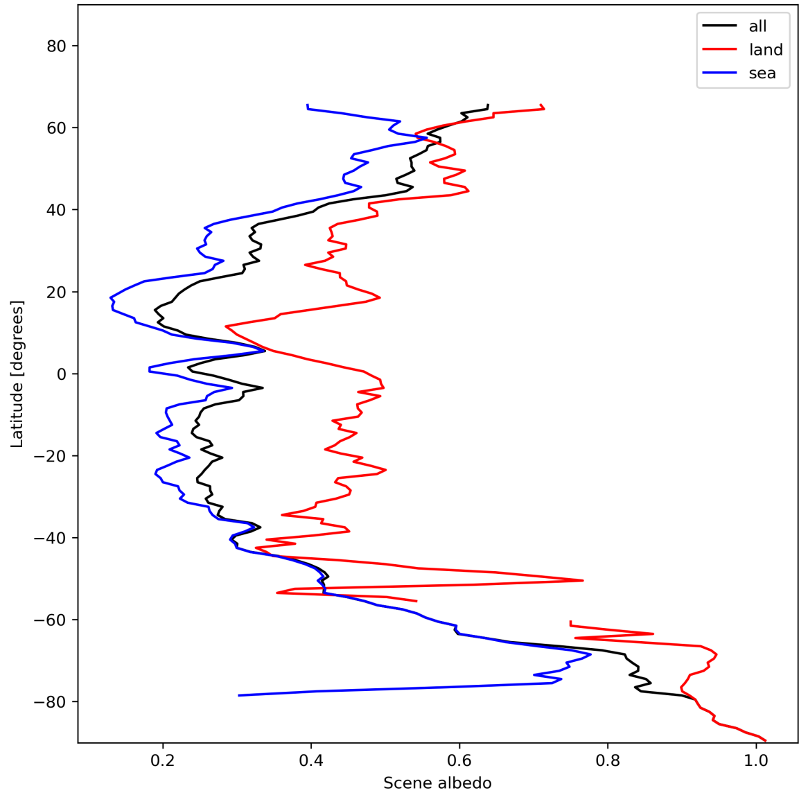
Figure 17: Zonal average of “Scene albedo” for 2023-12-09 to 2023-12-11.
