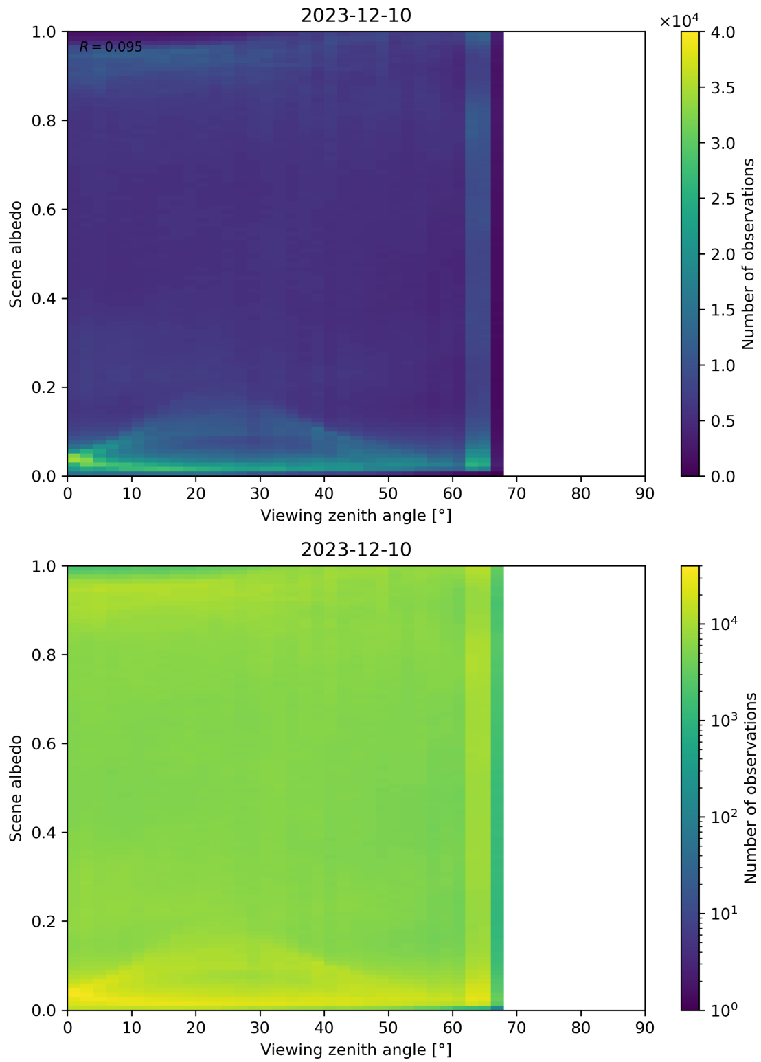
Figure 126: Scatter density plot of “Viewing zenith angle” against “Scene albedo” for 2023-12-09 to 2023-12-11.
