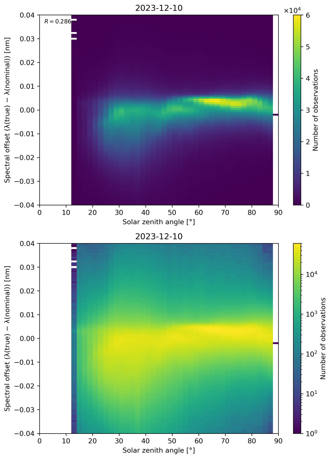
Figure 117: Scatter density plot of “Solar zenith angle” against “Spectral offset ( \lambda(\text{true}) - \lambda(\text{nominal}) )” for 2023-12-09 to 2023-12-11.
