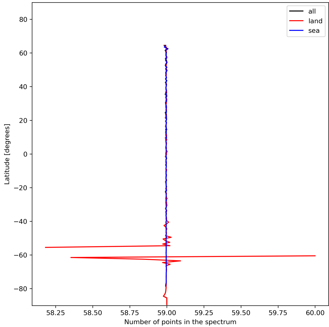
Figure 27: Zonal average of “Number of points in the spectrum” for 2023-12-12 to 2023-12-14.
