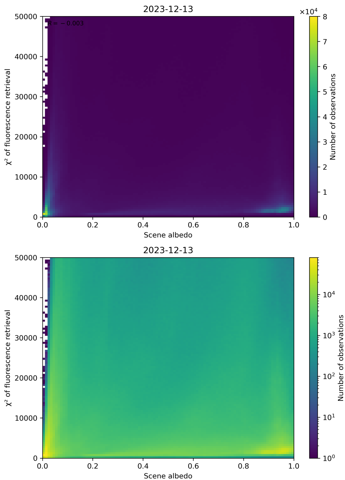
Figure 103: Scatter density plot of “Scene albedo” against “ \chi^2 of fluorescence retrieval” for 2023-12-12 to 2023-12-14.
