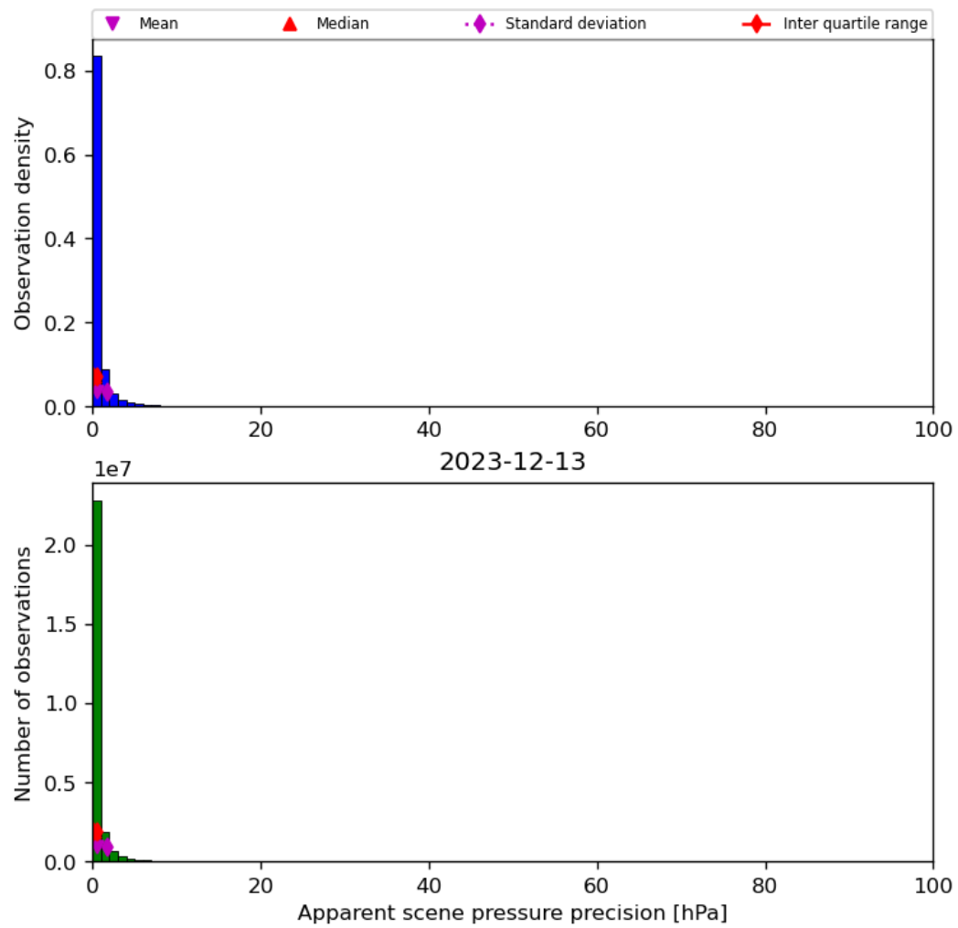
Figure 37: Histogram of “Apparent scene pressure precision” for 2023-12-12 to 2023-12-14
