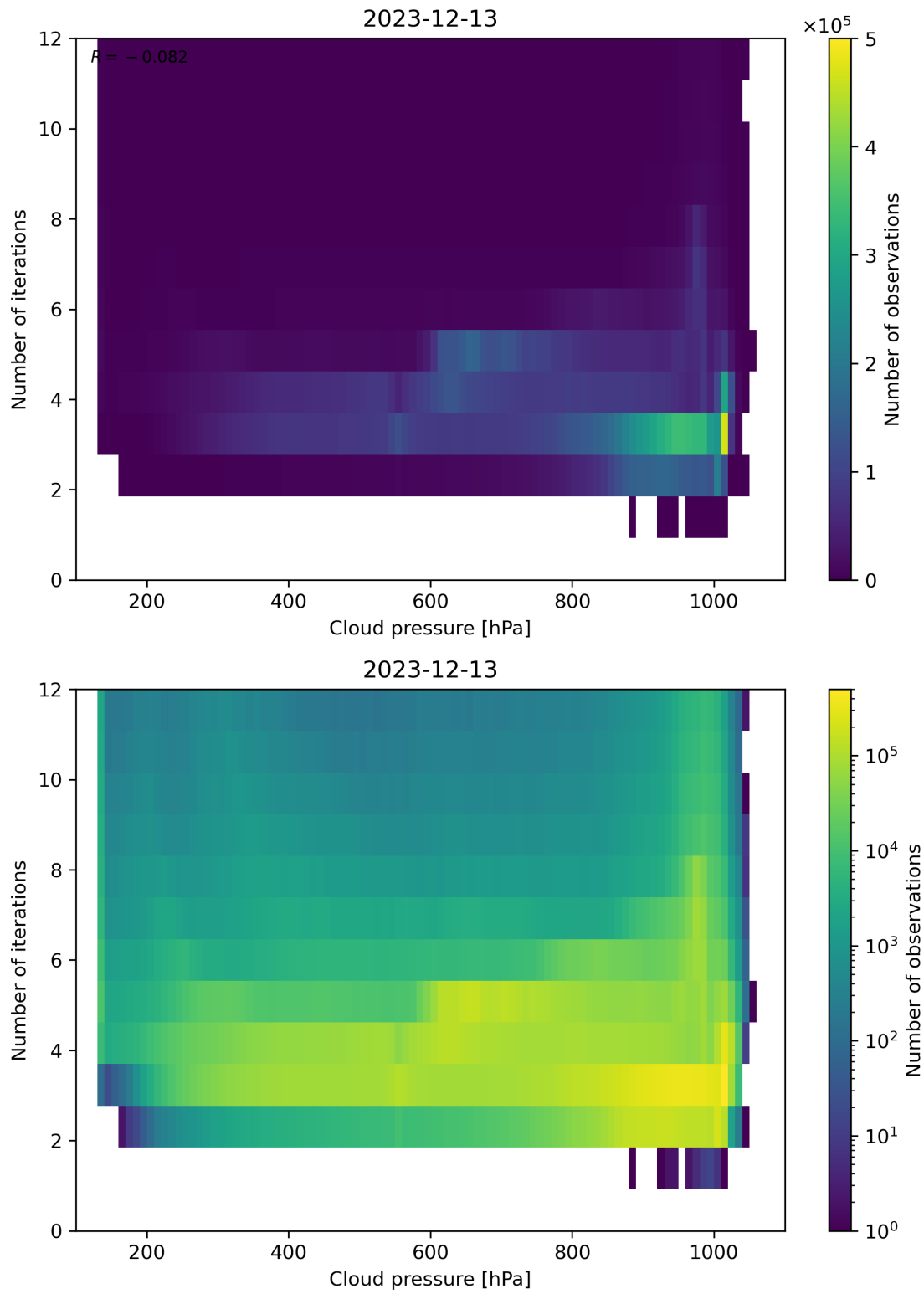
Figure 81: Scatter density plot of “Cloud pressure” against “Number of iterations” for 2023-12-12 to 2023-12-14.
