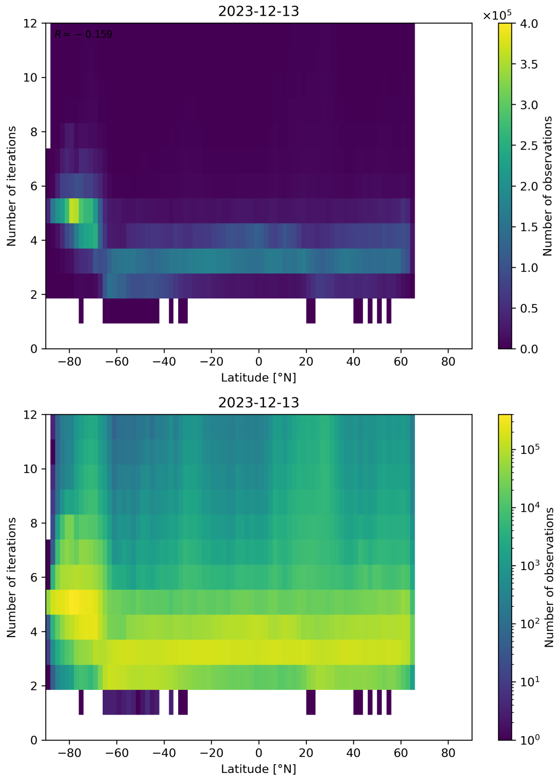
Figure 93: Scatter density plot of “Latitude” against “Number of iterations” for 2023-12-12 to 2023-12-14.
