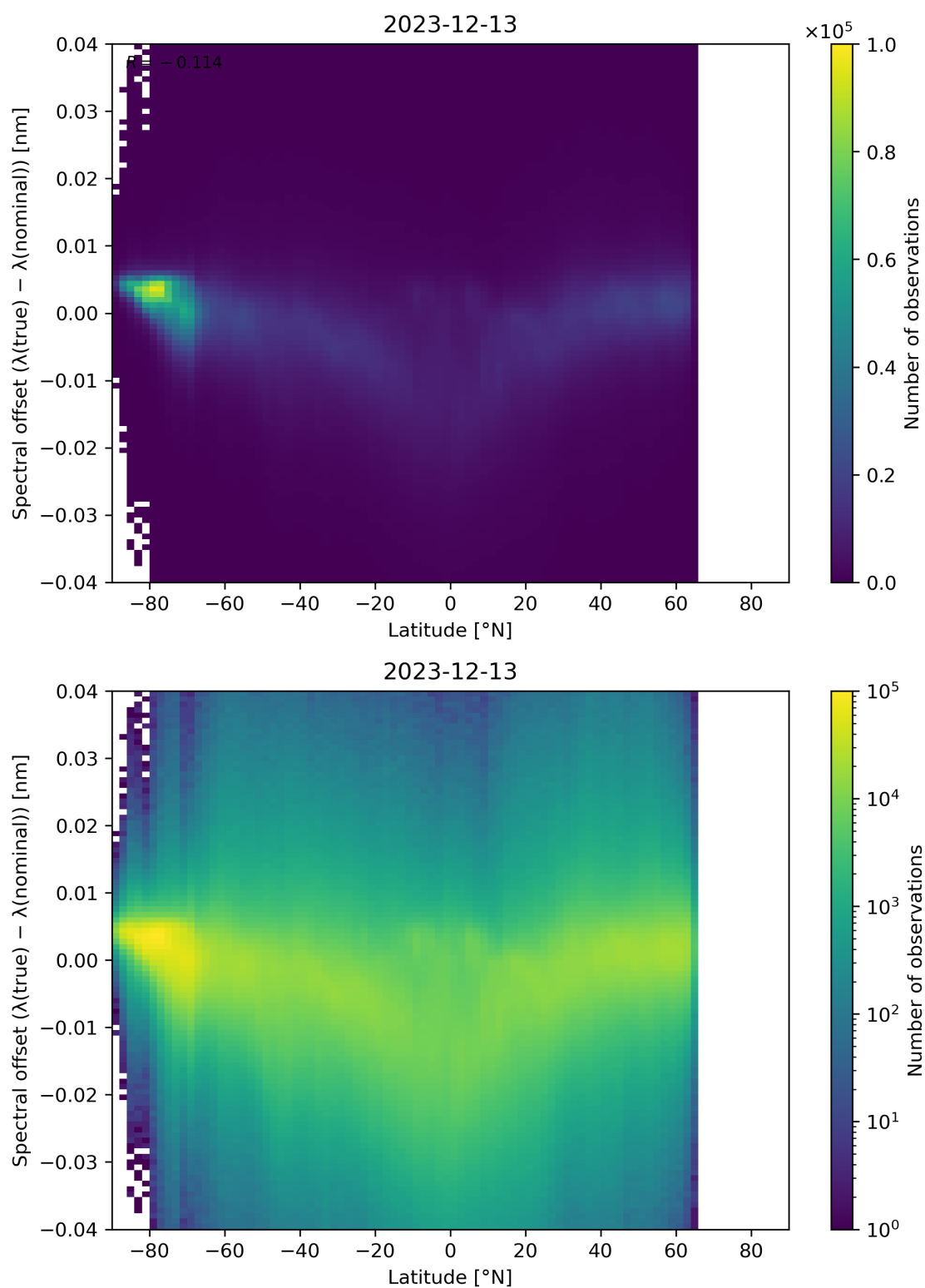
Figure 96: Scatter density plot of “Latitude” against “Spectral offset ( \lambda(\text{true}) - \lambda(\text{nominal}) )” for 2023-12-12 to 2023-12-14.
