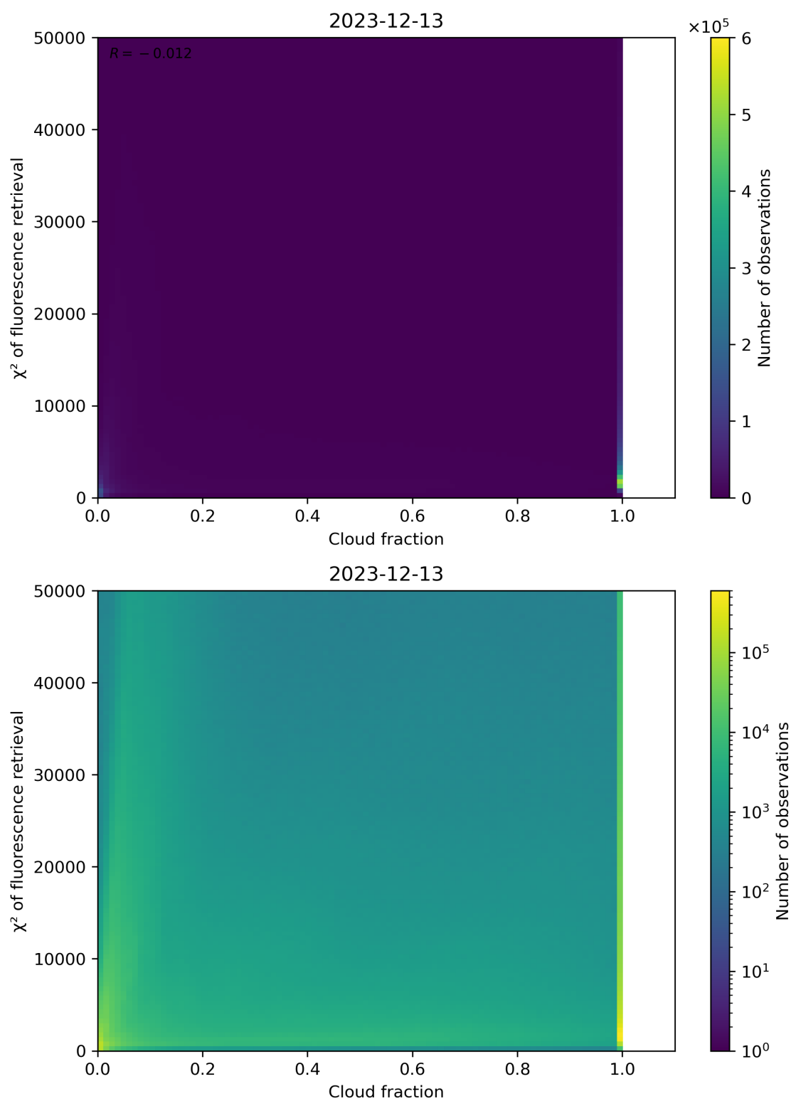
Figure 71: Scatter density plot of “Cloud fraction” against “ \chi^2 of fluorescence retrieval” for 2023-12-12 to 2023-12-14.
