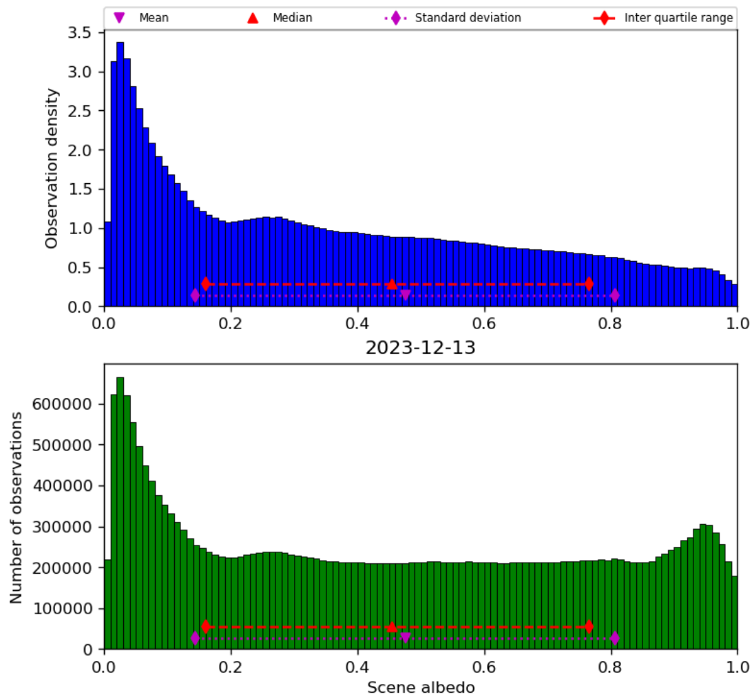
Figure 34: Histogram of “Scene albedo” for 2023-12-12 to 2023-12-14
