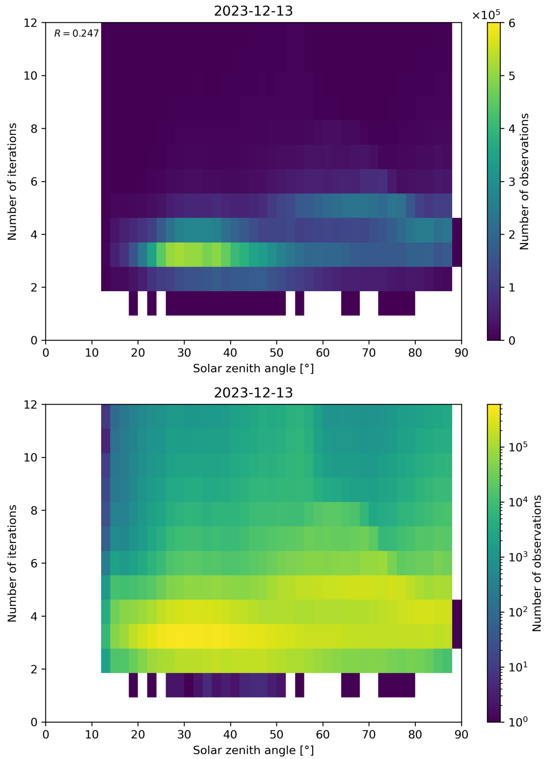
Figure 114: Scatter density plot of “Solar zenith angle” against “Number of iterations” for 2023-12-12 to 2023-12-14.
