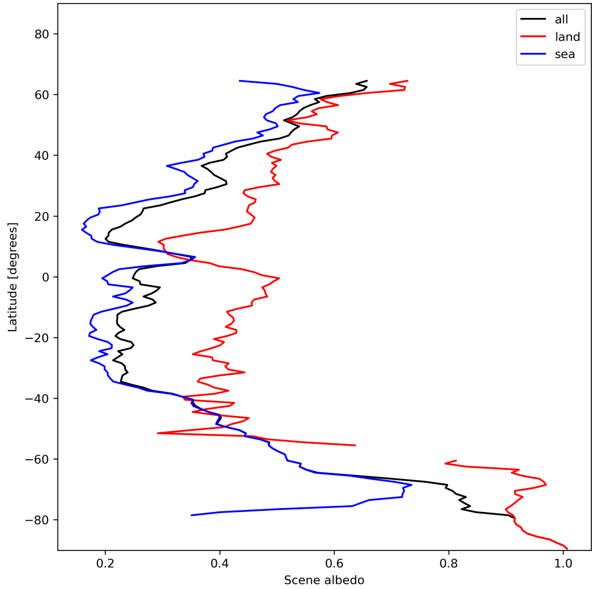
Figure 17: Zonal average of “Scene albedo” for 2023-12-12 to 2023-12-14.
