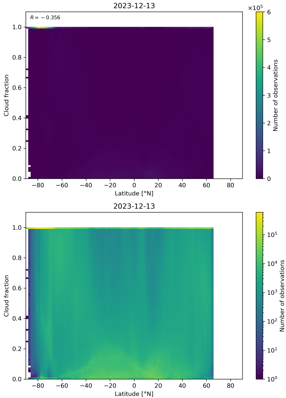
Figure 90: Scatter density plot of “Latitude” against “Cloud fraction” for 2023-12-12 to 2023-12-14.
