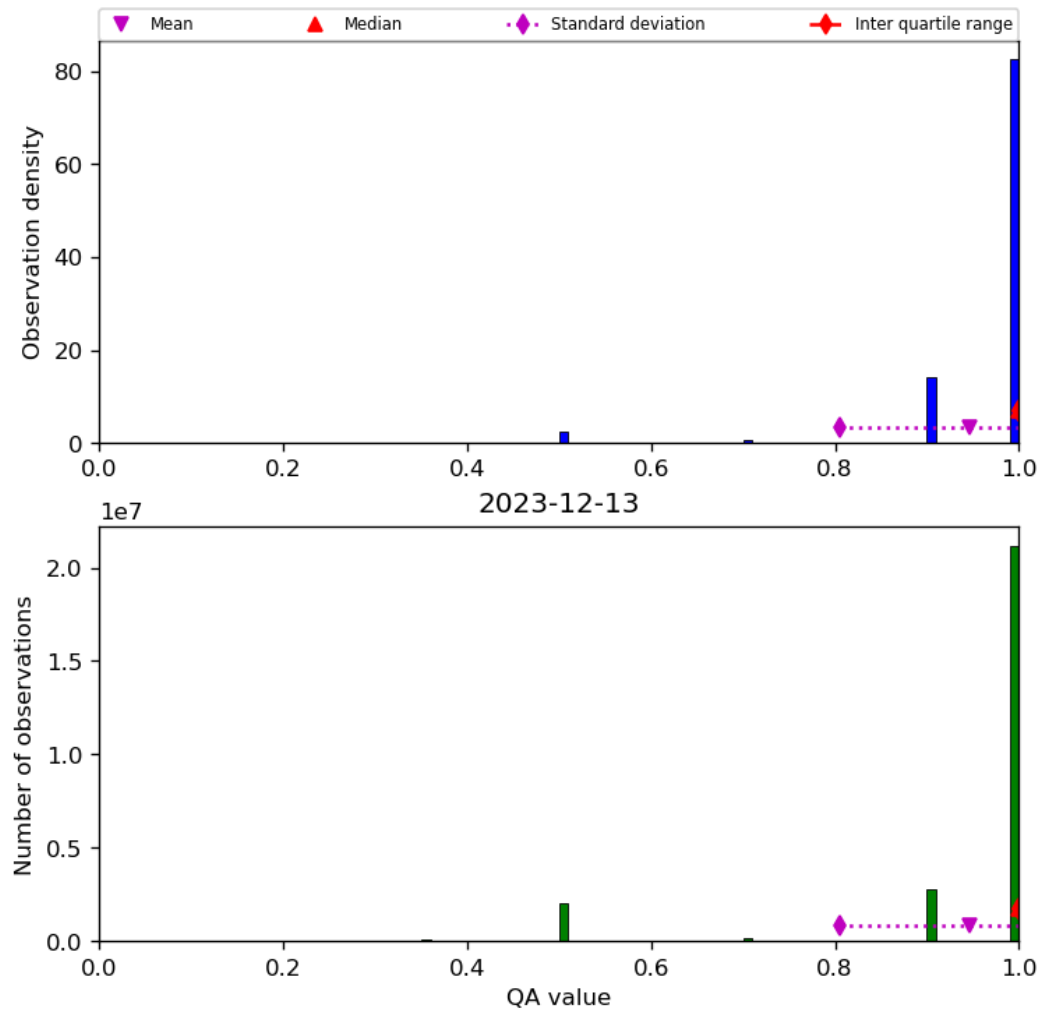
Figure 29: Histogram of “QA value” for 2023-12-12 to 2023-12-14
