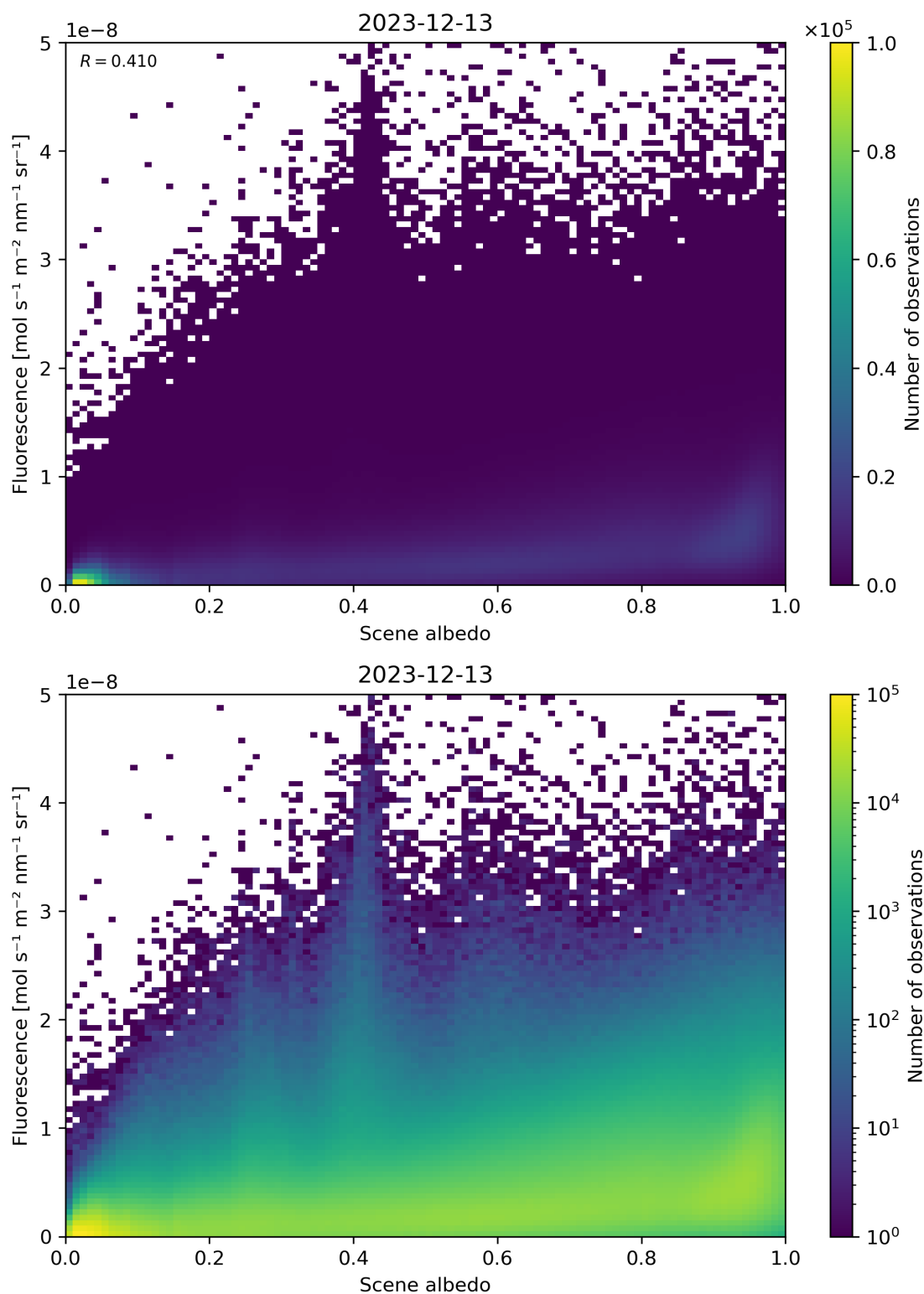
Figure 104: Scatter density plot of “Scene albedo” against “Fluorescence” for 2023-12-12 to 2023-12-14.
