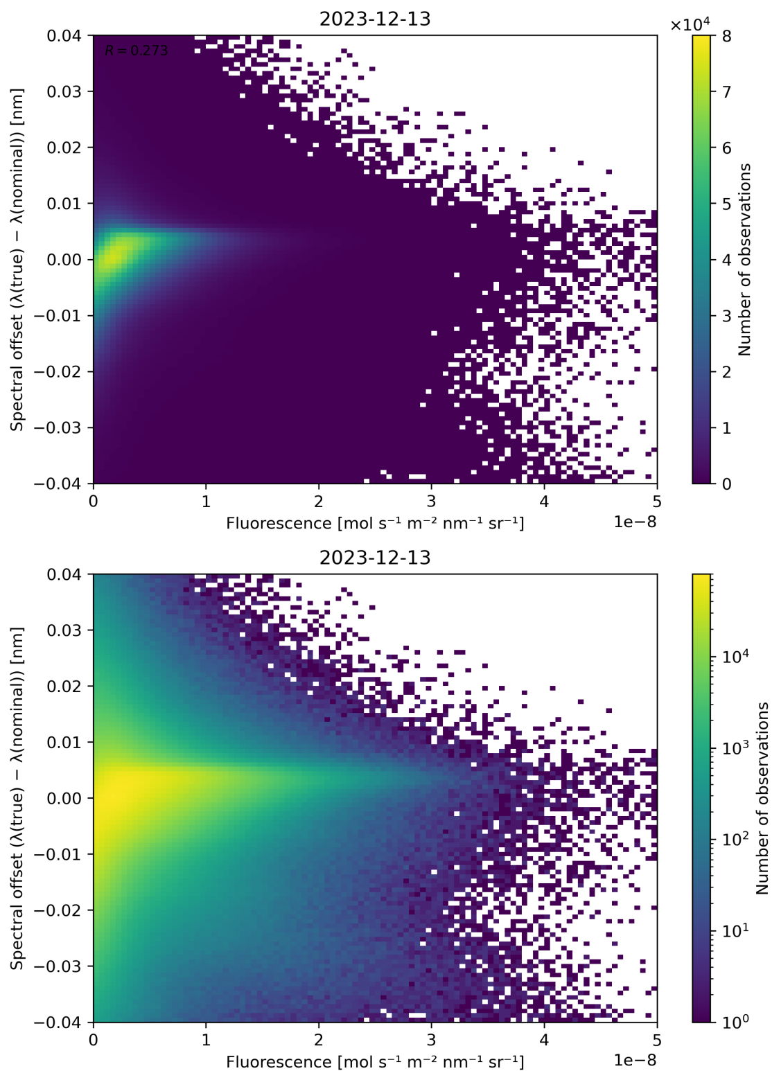
Figure 87: Scatter density plot of “Fluorescence” against “Spectral offset ( \lambda(\text{true}) - \lambda(\text{nominal}) )” for 2023-12-12 to 2023-12-14.
