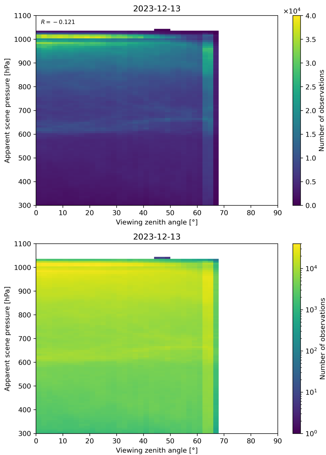
Figure 118: Scatter density plot of “Viewing zenith angle” against “Apparent scene pressure” for 2023-12-12 to 2023-12-14.
