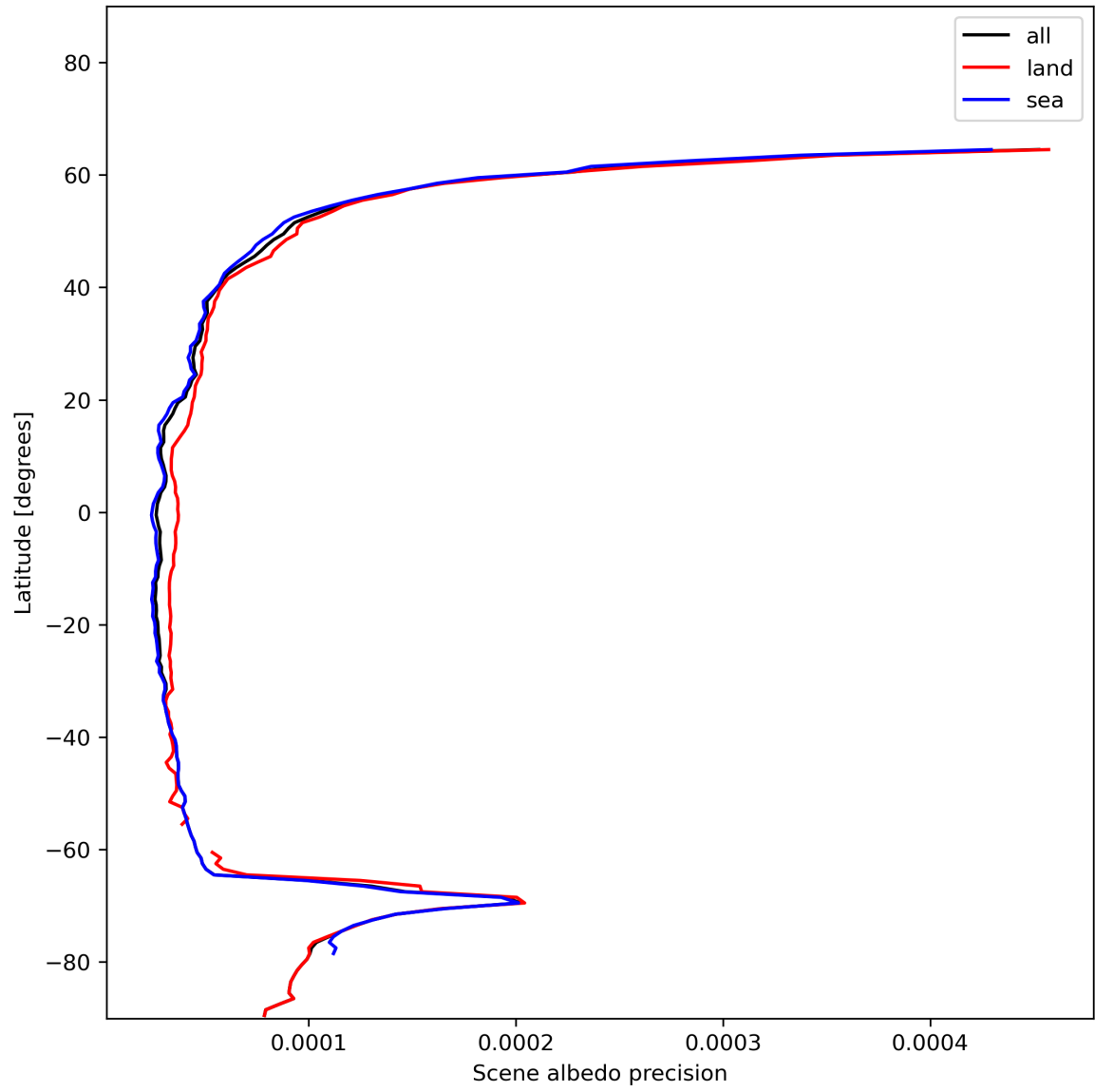
Figure 18: Zonal average of “Scene albedo precision” for 2023-12-12 to 2023-12-14.
