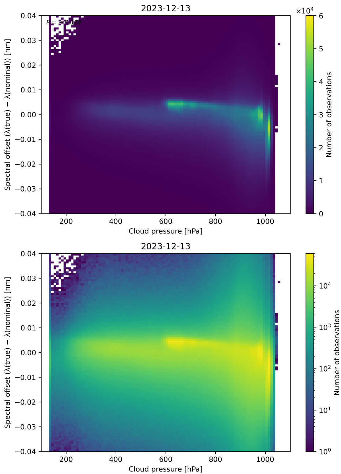
Figure 84: Scatter density plot of “Cloud pressure” against “Spectral offset ( \lambda(\text{true}) - \lambda(\text{nominal}) )” for 2023-12-12 to 2023-12-14.
