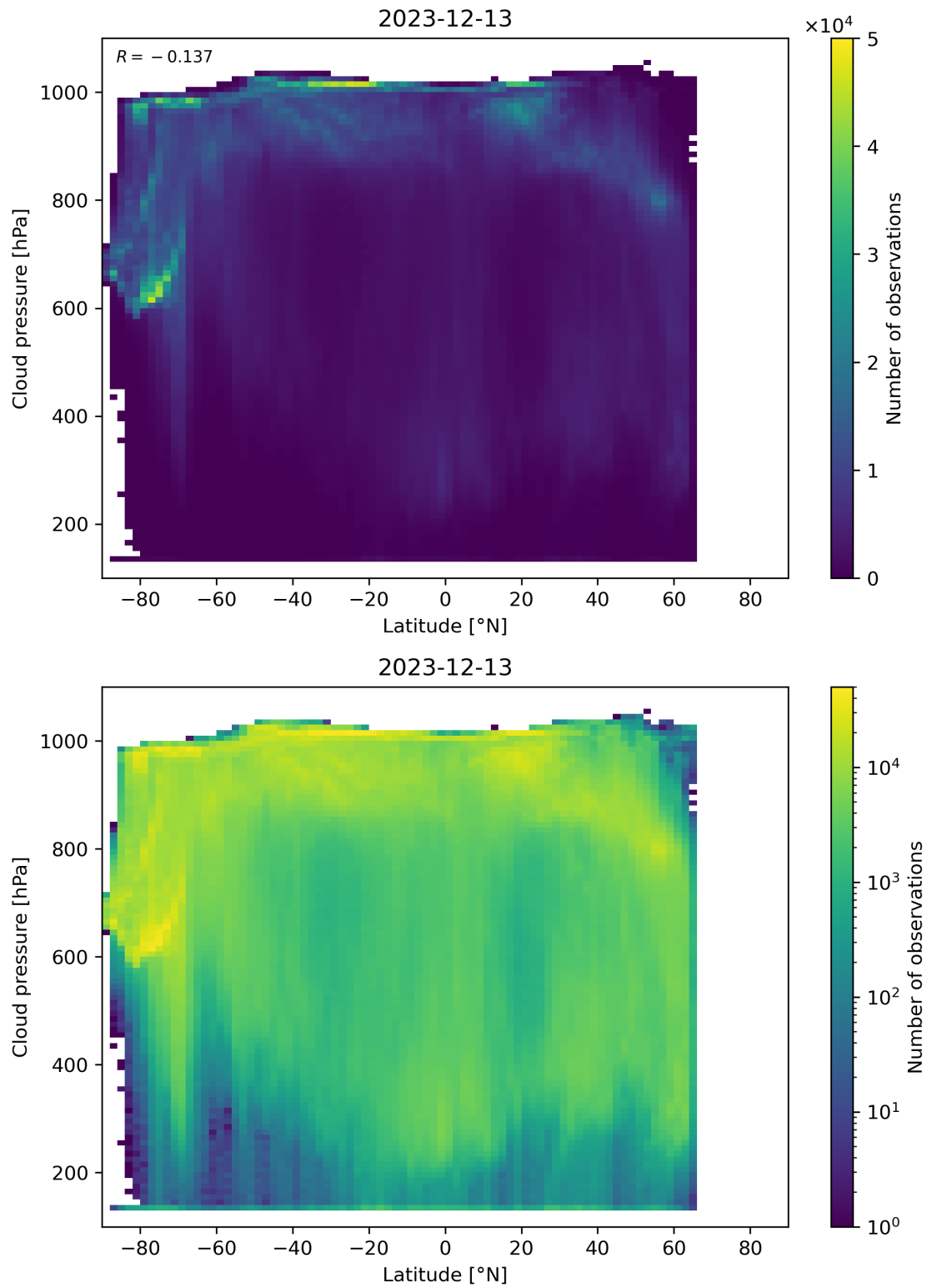
Figure 91: Scatter density plot of “Latitude” against “Cloud pressure” for 2023-12-12 to 2023-12-14.
