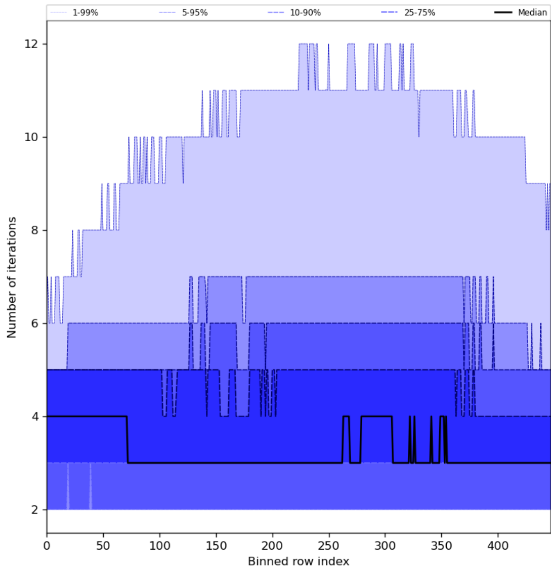
Figure 56: Along track statistics of “Number of iterations” for 2023-12-12 to 2023-12-14
