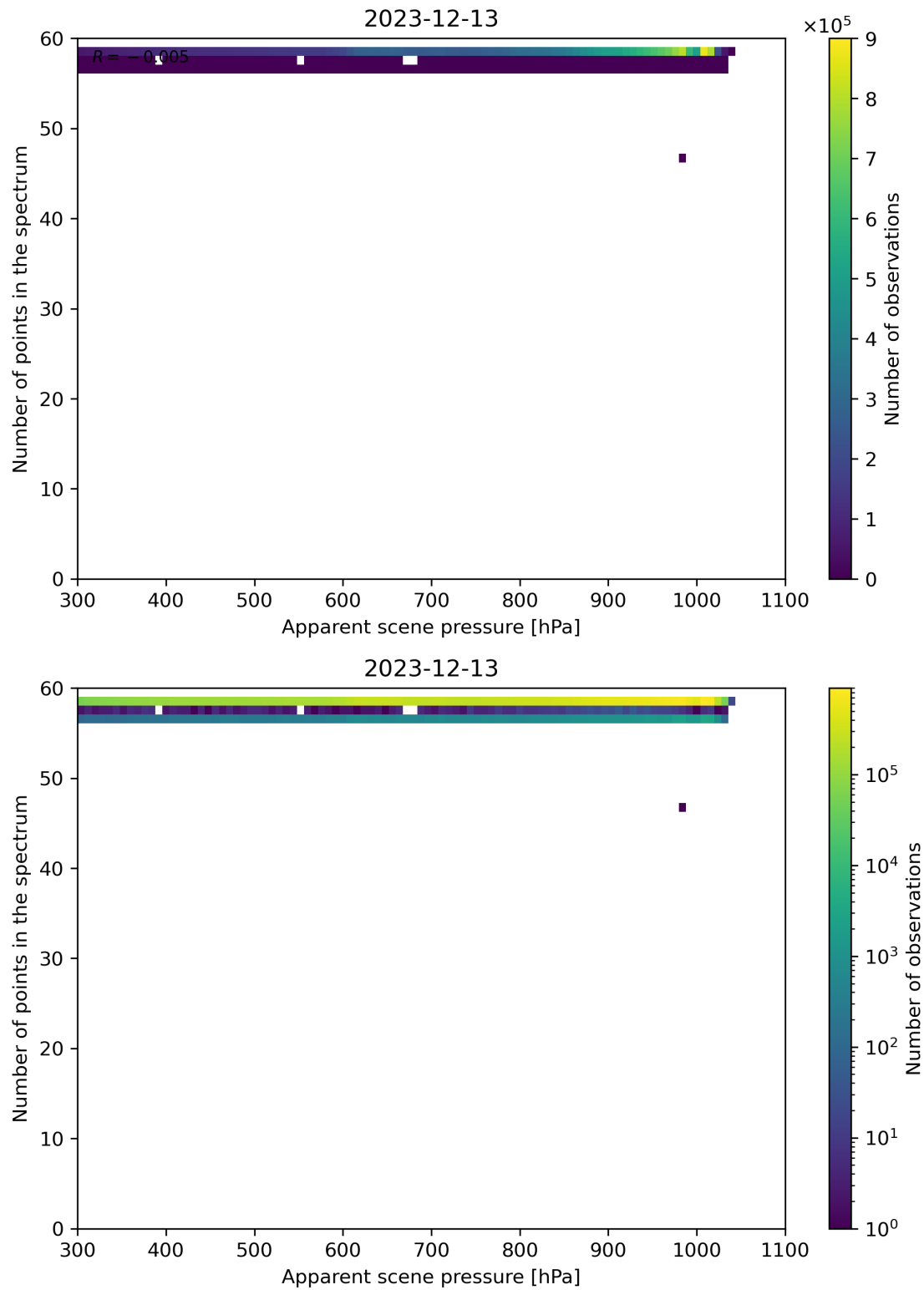
Figure 66: Scatter density plot of “Apparent scene pressure” against “Number of points in the spectrum” for 2023-12-12 to 2023-12-14.
