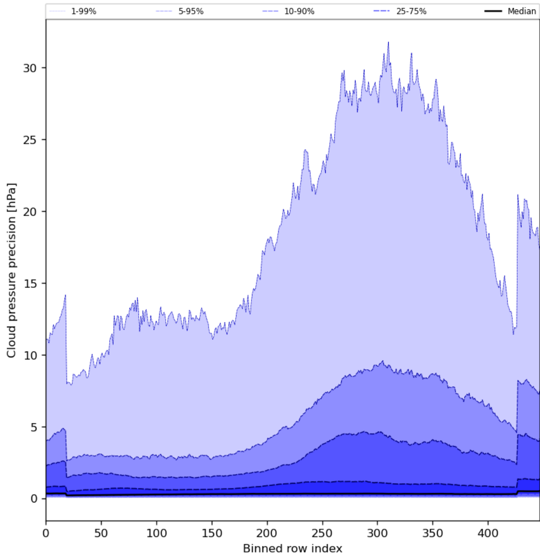
Figure 48: Along track statistics of “Cloud pressure precision” for 2023-12-12 to 2023-12-14
