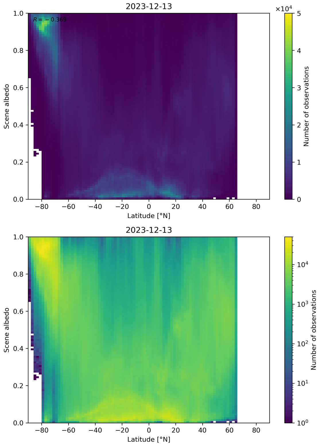
Figure 95: Scatter density plot of “Latitude” against “Scene albedo” for 2023-12-12 to 2023-12-14.
