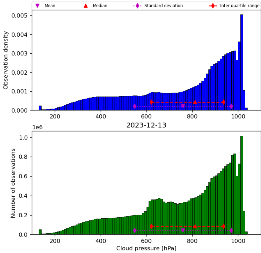
Figure 30: Histogram of “Cloud pressure” for 2023-12-12 to 2023-12-14
