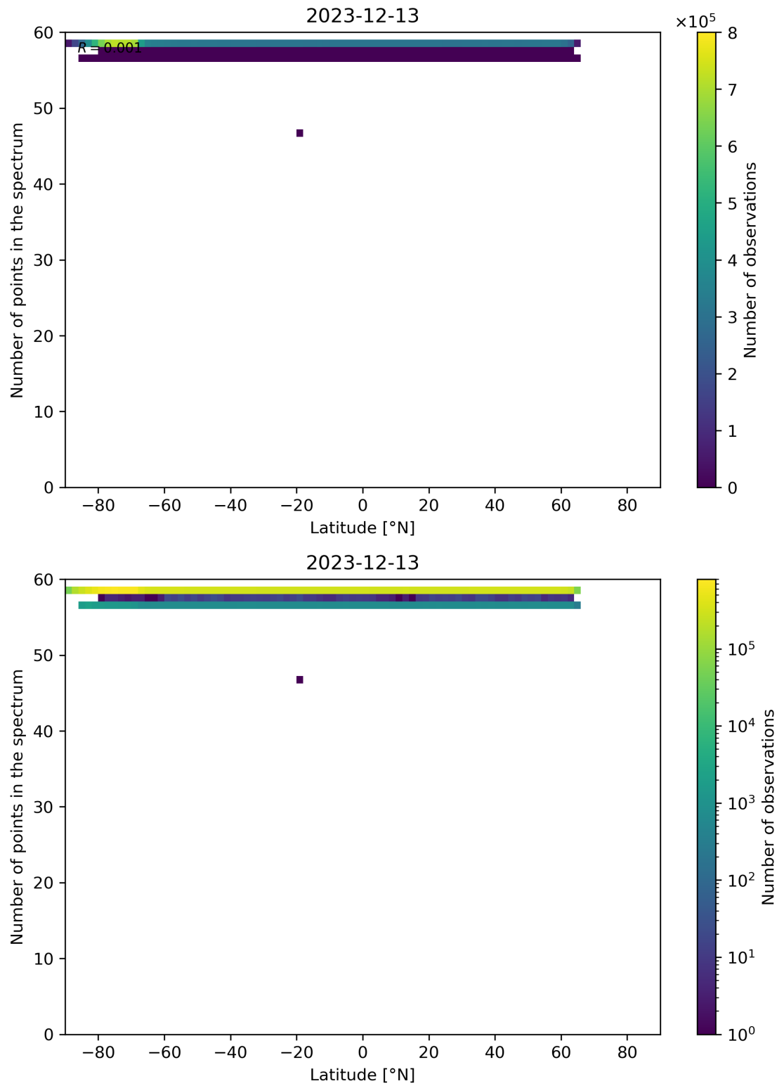
Figure 94: Scatter density plot of “Latitude” against “Number of points in the spectrum” for 2023-12-12 to 2023-12-14.
