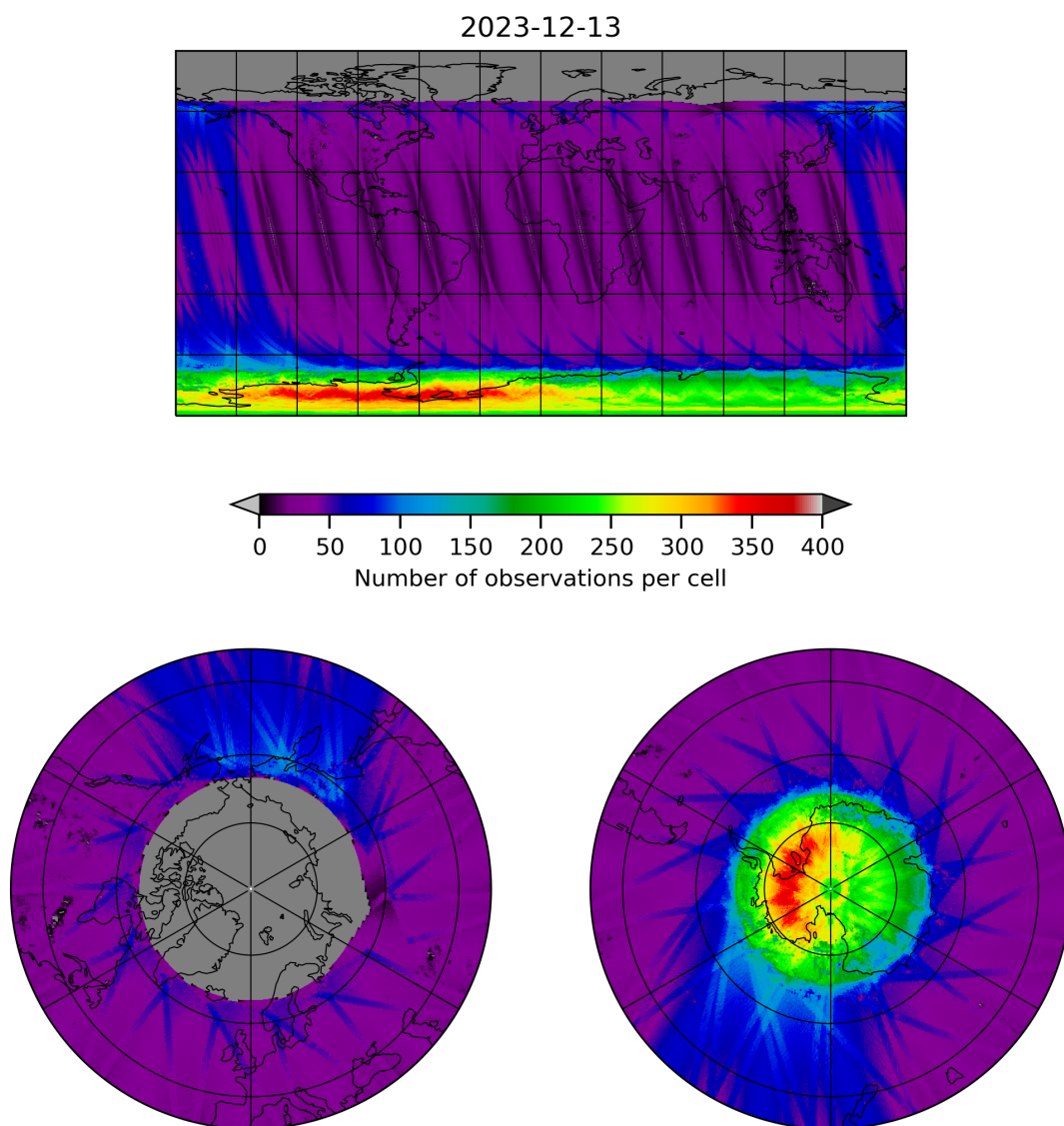
Figure 11: Map of the number of observations for 2023-12-12 to 2023-12-14
