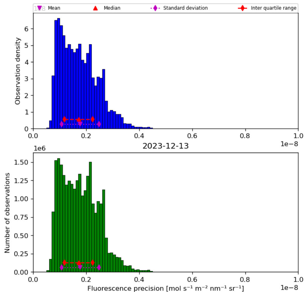
Figure 41: Histogram of “Fluorescence precision” for 2023-12-12 to 2023-12-14
