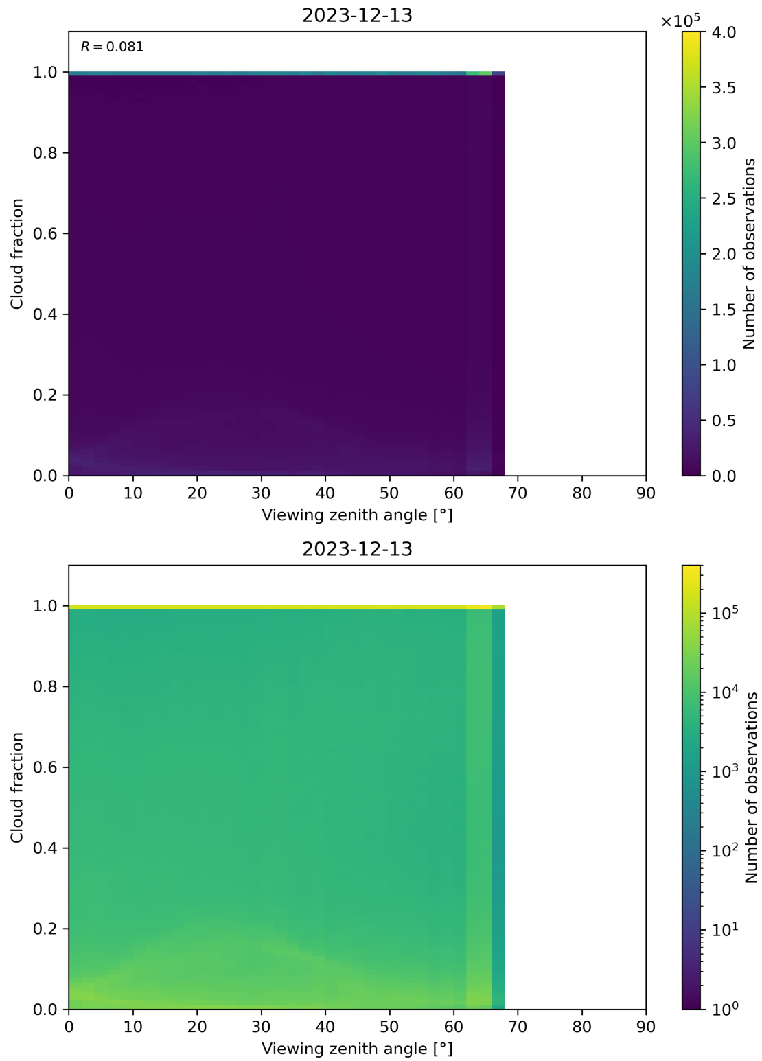
Figure 120: Scatter density plot of “Viewing zenith angle” against “Cloud fraction” for 2023-12-12 to 2023-12-14.
