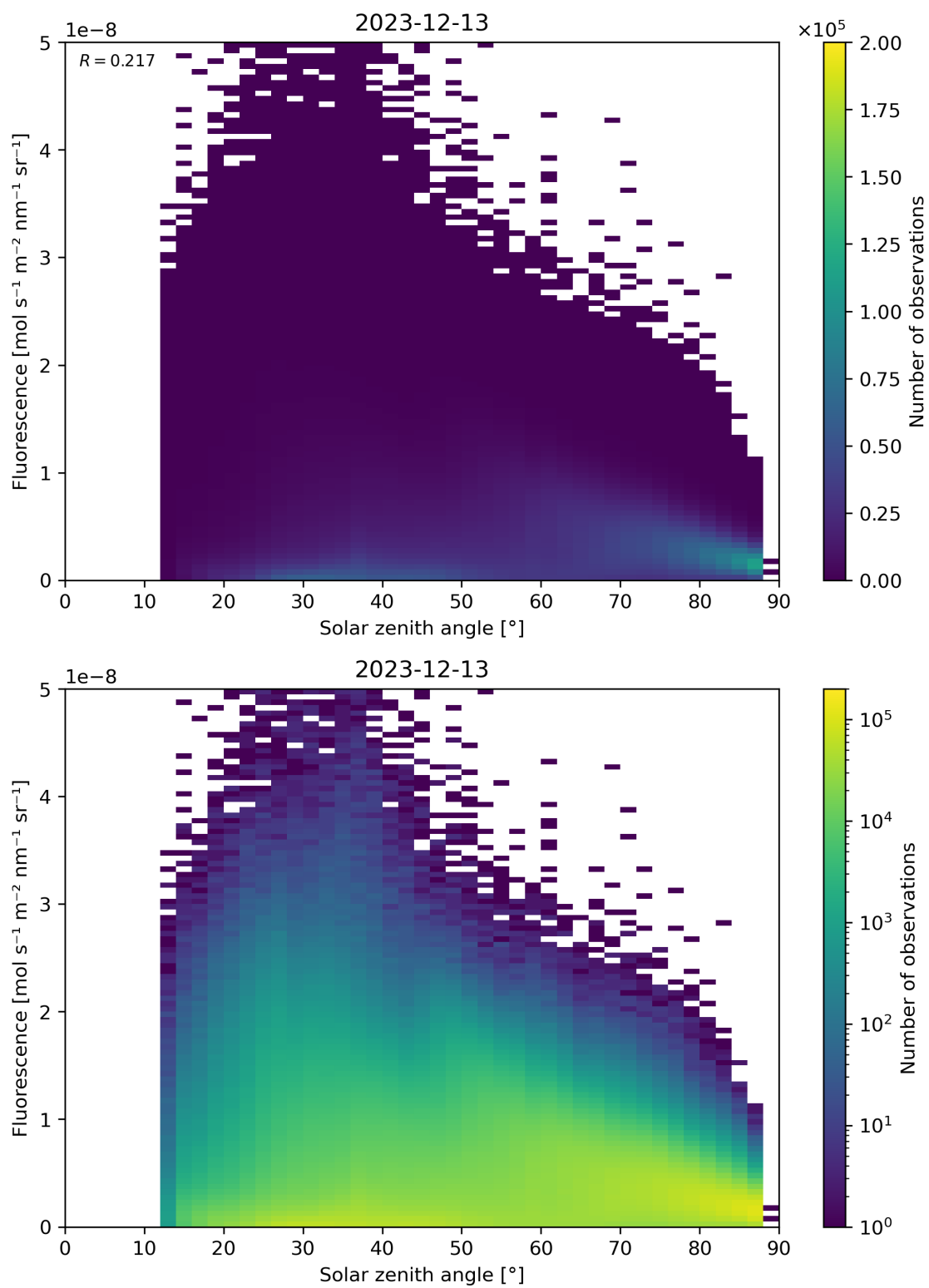
Figure 112: Scatter density plot of “Solar zenith angle” against “Fluorescence” for 2023-12-12 to 2023-12-14.
