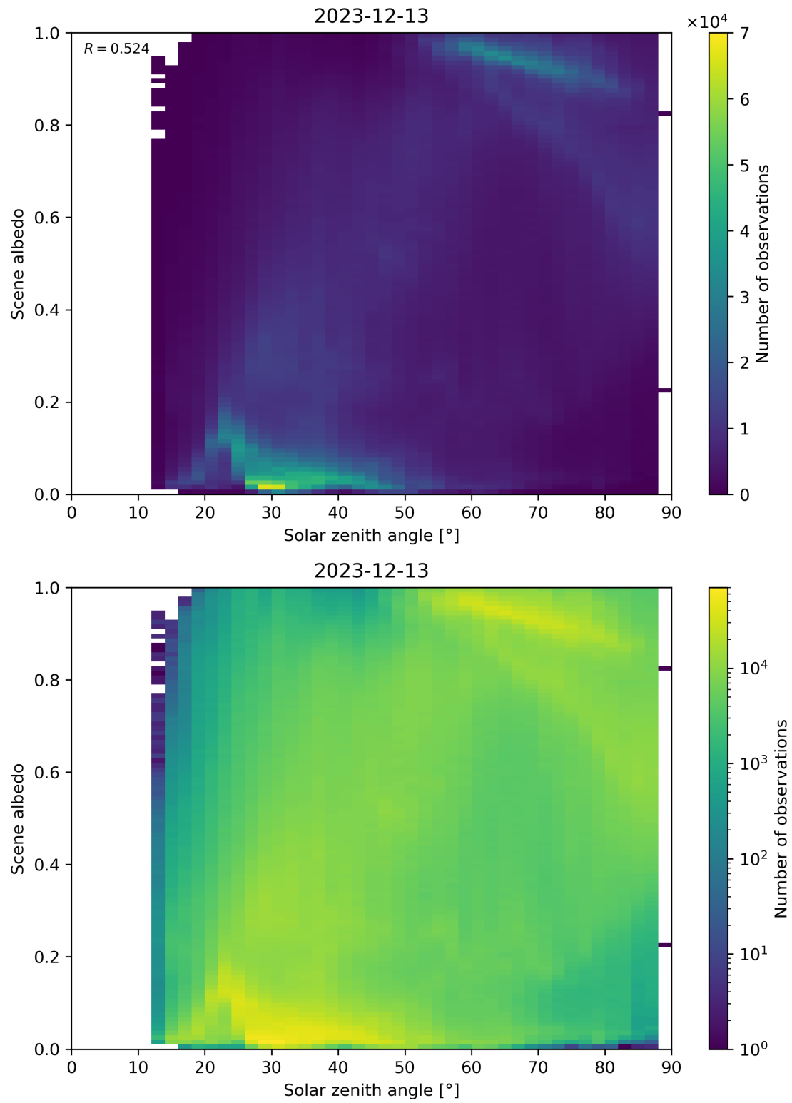
Figure 116: Scatter density plot of “Solar zenith angle” against “Scene albedo” for 2023-12-12 to 2023-12-14.
