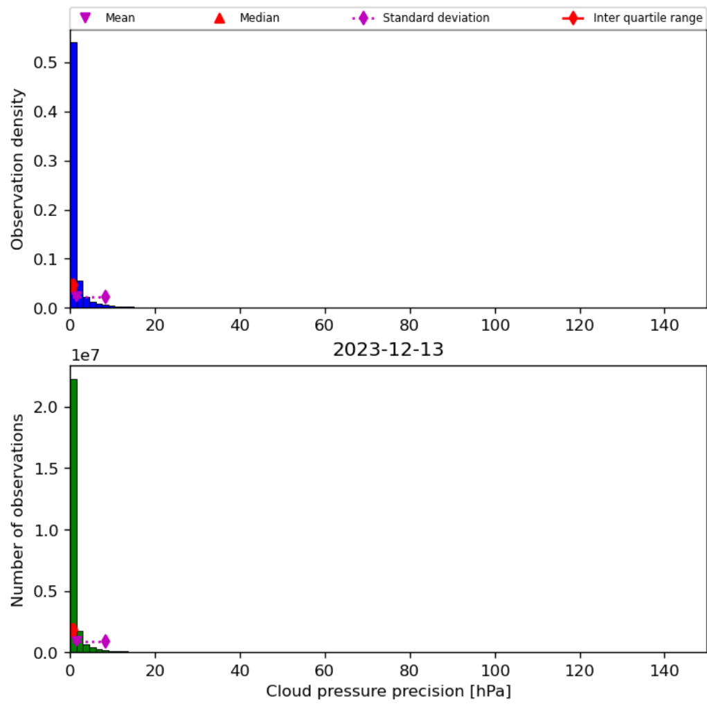
Figure 31: Histogram of “Cloud pressure precision” for 2023-12-12 to 2023-12-14
