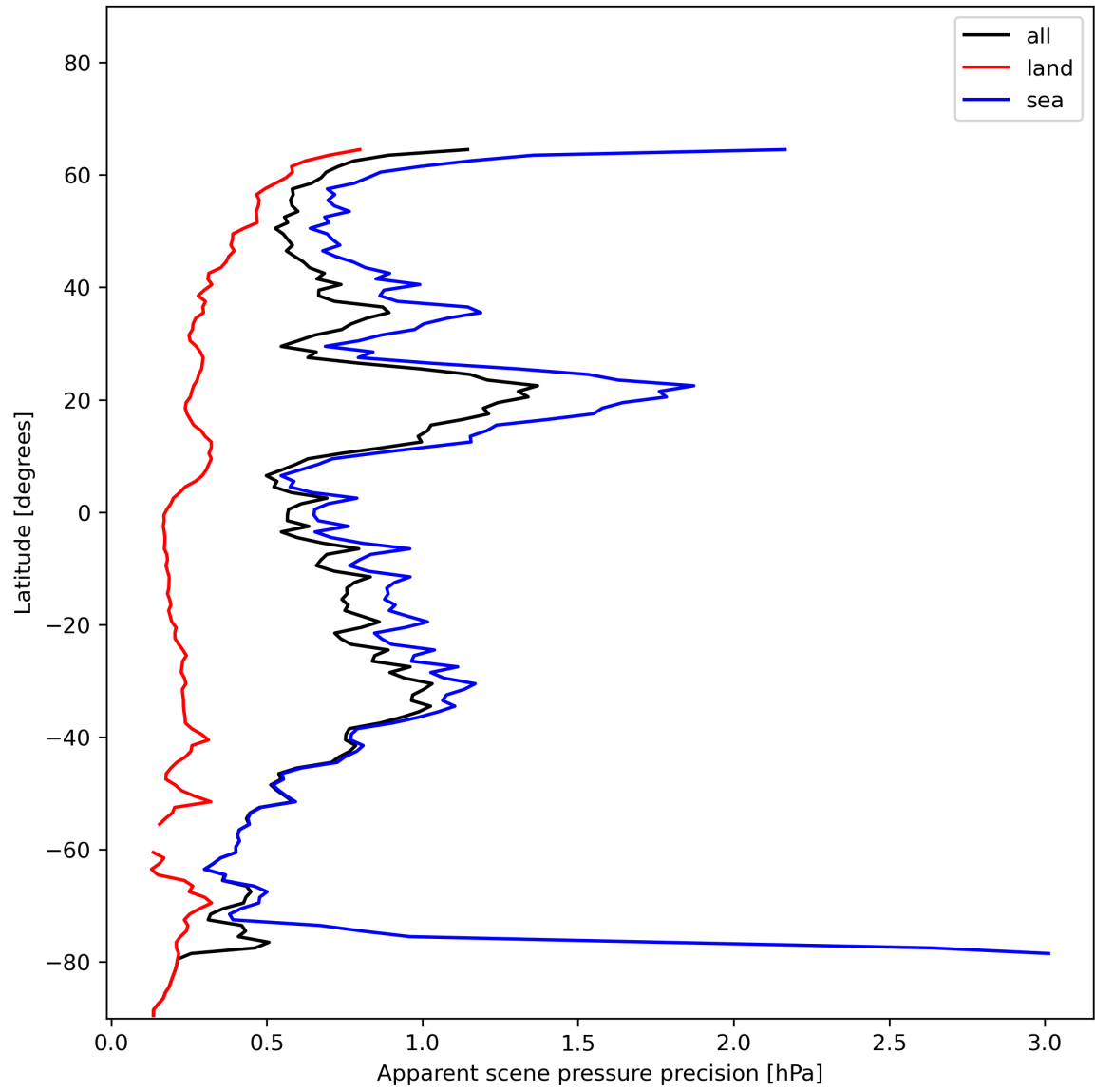
Figure 20: Zonal average of “Apparent scene pressure precision” for 2023-12-12 to 2023-12-14.
