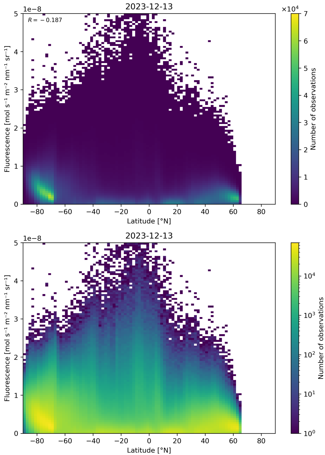
Figure 92: Scatter density plot of “Latitude” against “Fluorescence” for 2023-12-12 to 2023-12-14.
