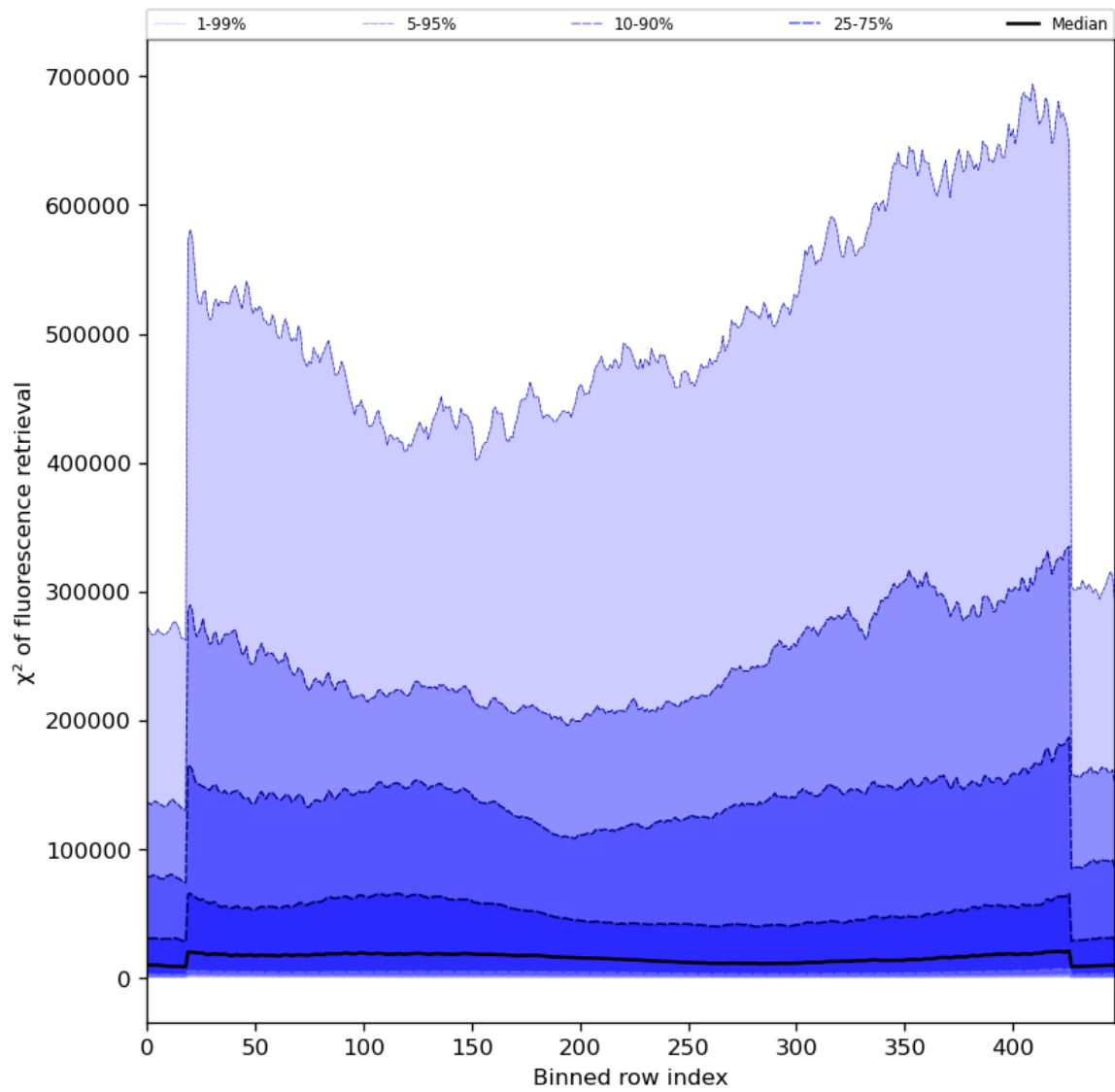
Figure 59: Along track statistics of “ \chi^2 of fluorescence retrieval” for 2023-12-12 to 2023-12-14
