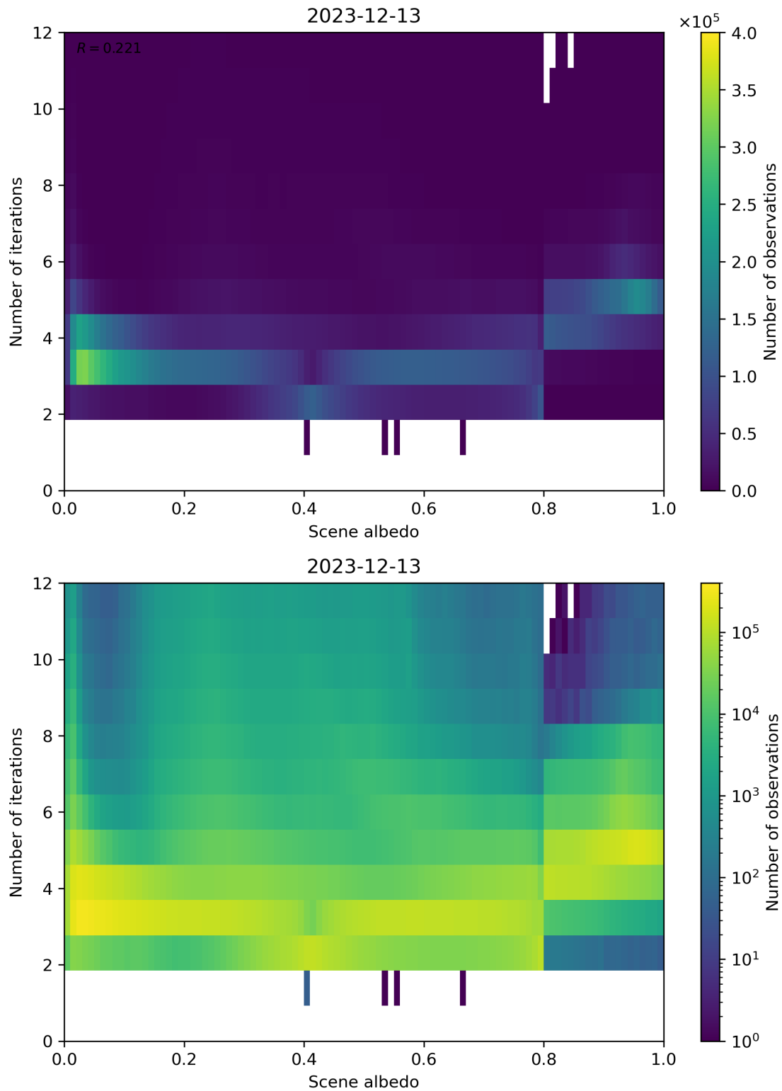
Figure 105: Scatter density plot of “Scene albedo” against “Number of iterations” for 2023-12-12 to 2023-12-14.
