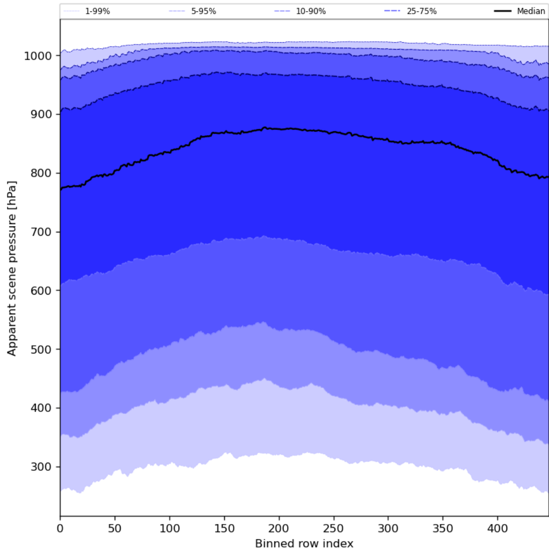
Figure 53: Along track statistics of “Apparent scene pressure” for 2023-12-12 to 2023-12-14
