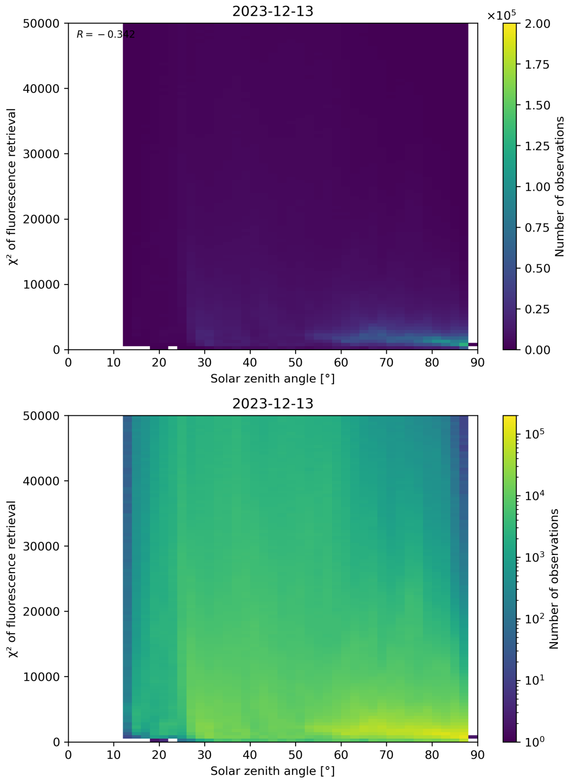
Figure 109: Scatter density plot of “Solar zenith angle” against “ \chi^2 of fluorescence retrieval” for 2023-12-12 to 2023-12-14.
