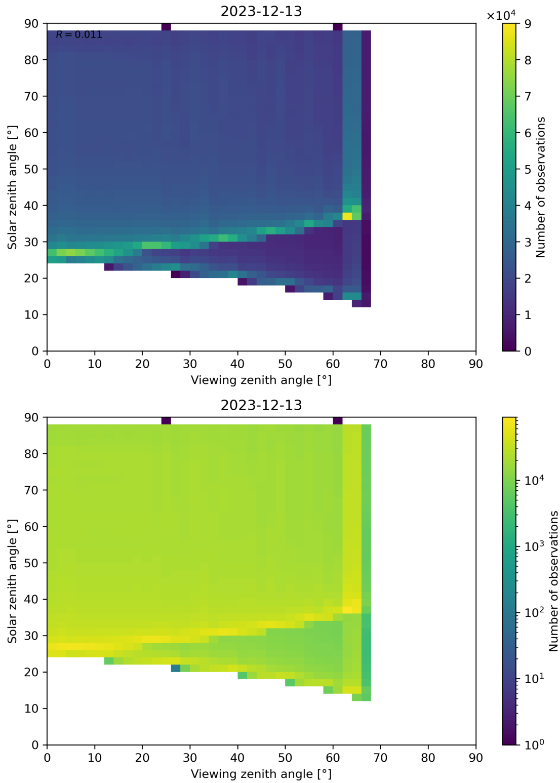
Figure 127: Scatter density plot of “Viewing zenith angle” against “Solar zenith angle” for 2023-12-12 to 2023-12-14.
