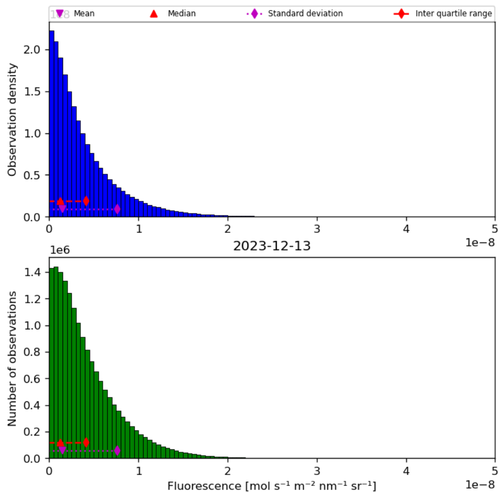
Figure 40: Histogram of “Fluorescence” for 2023-12-12 to 2023-12-14
