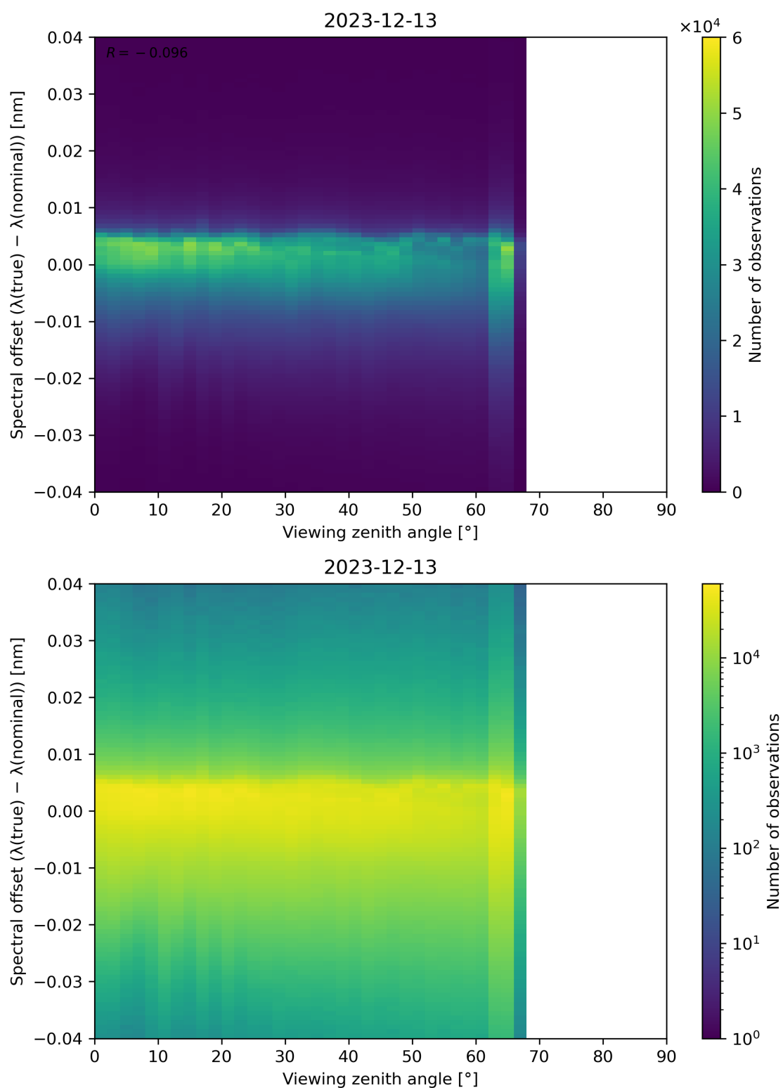
Figure 128: Scatter density plot of “Viewing zenith angle” against “Spectral offset ( \lambda(\text{true}) - \lambda(\text{nominal}) )” for 2023-12-12 to 2023-12-14.
