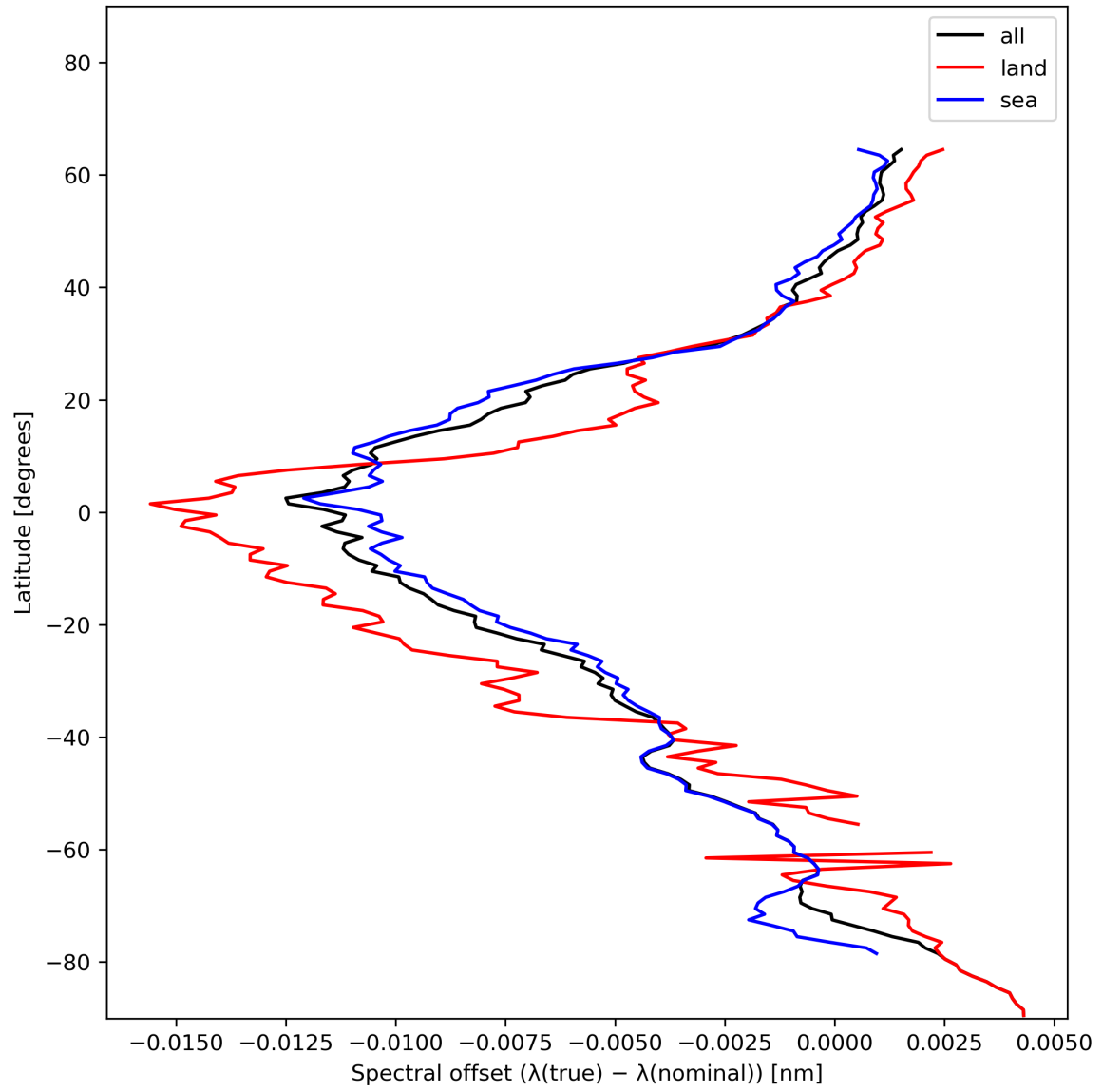
Figure 28: Zonal average of “Spectral offset ( \lambda(\text{true}) - \lambda(\text{nominal}) )” for 2023-12-12 to 2023-12-14.
