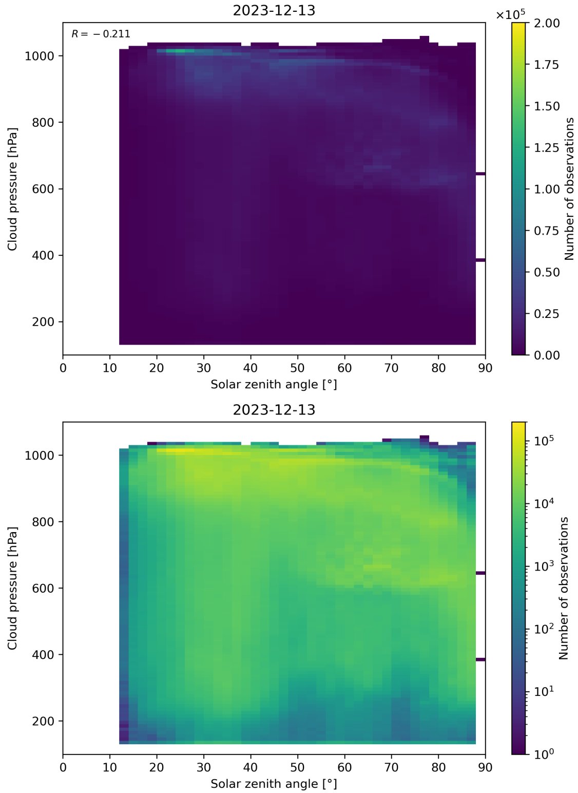
Figure 111: Scatter density plot of “Solar zenith angle” against “Cloud pressure” for 2023-12-12 to 2023-12-14.
