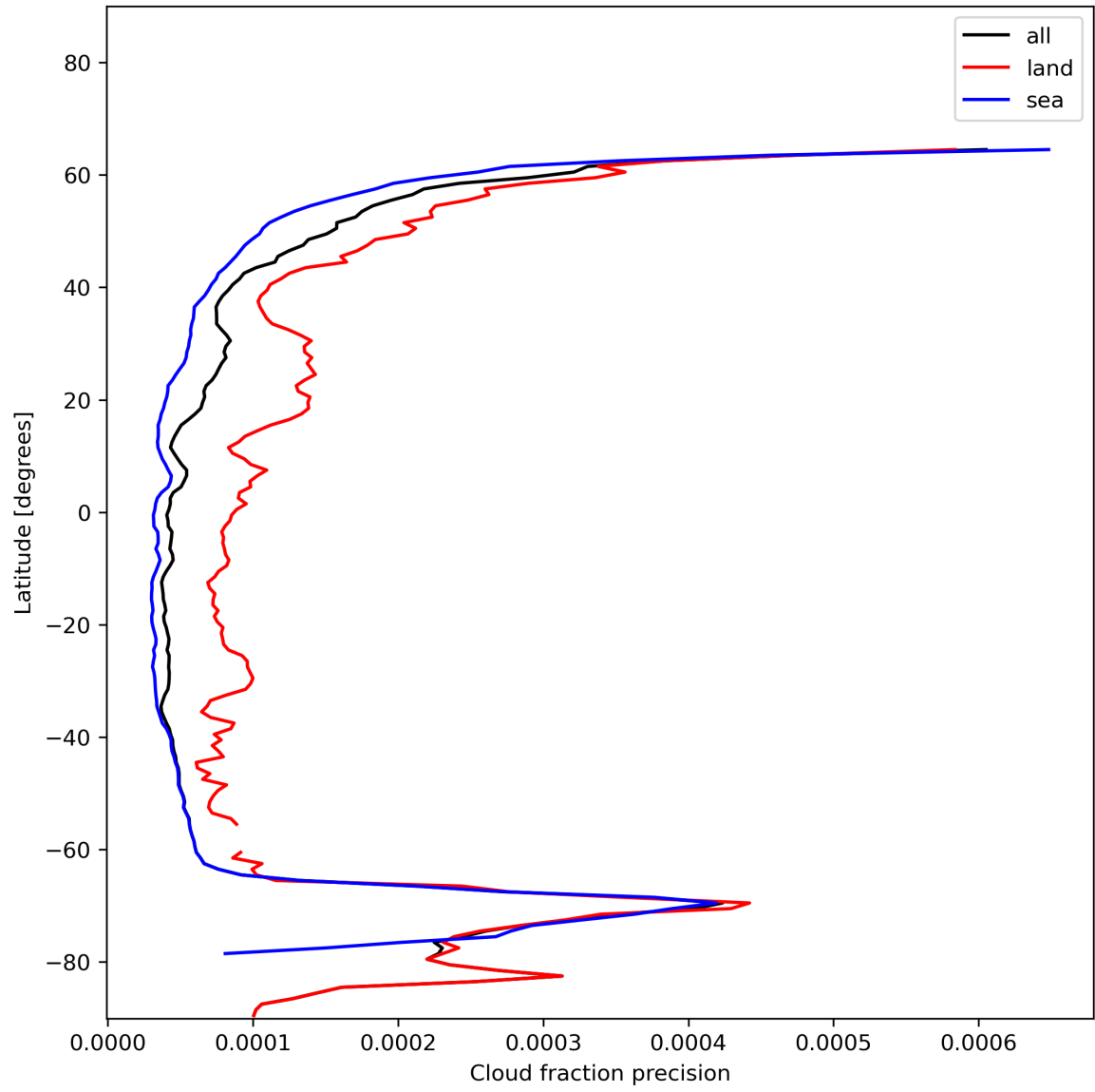
Figure 16: Zonal average of “Cloud fraction precision” for 2023-12-12 to 2023-12-14.
