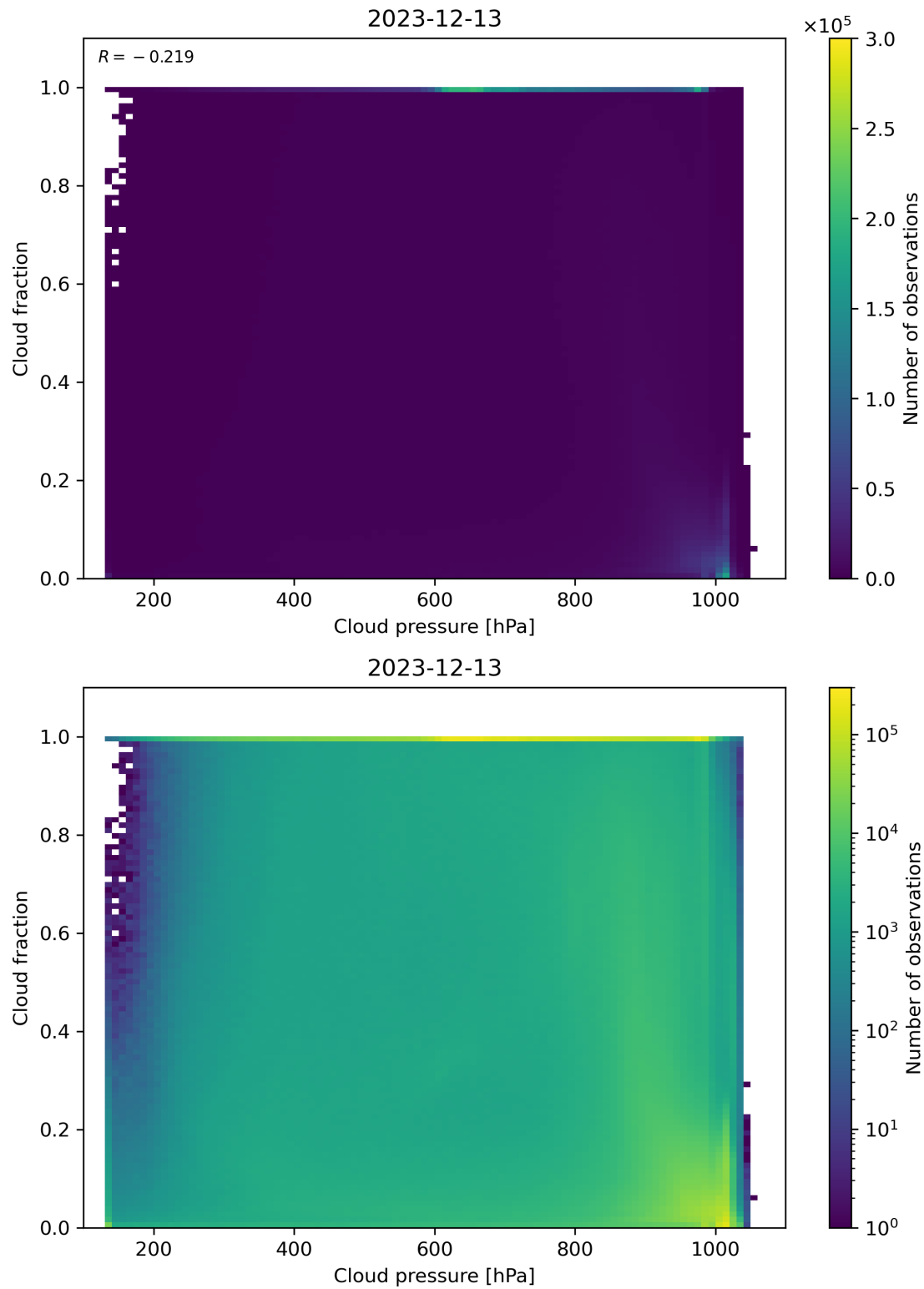
Figure 79: Scatter density plot of “Cloud pressure” against “Cloud fraction” for 2023-12-12 to 2023-12-14.
