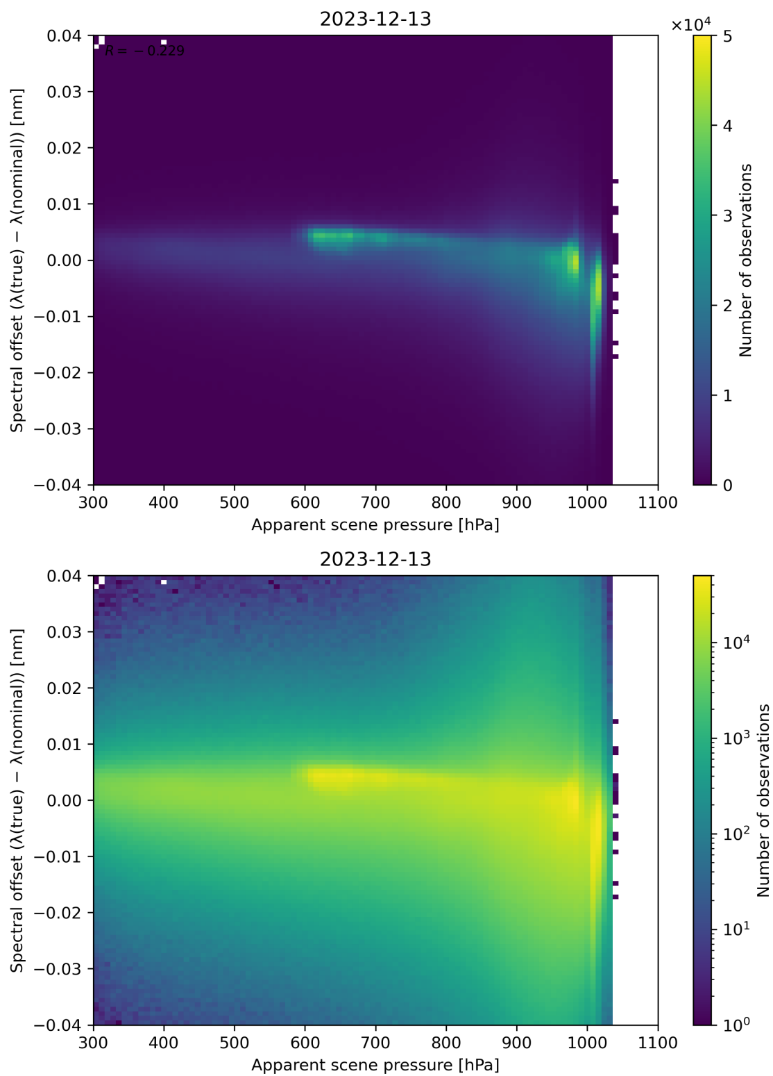
Figure 67: Scatter density plot of “Apparent scene pressure” against “Spectral offset ( \lambda(\text{true}) - \lambda(\text{nominal}) )” for 2023-12-12 to 2023-12-14.
