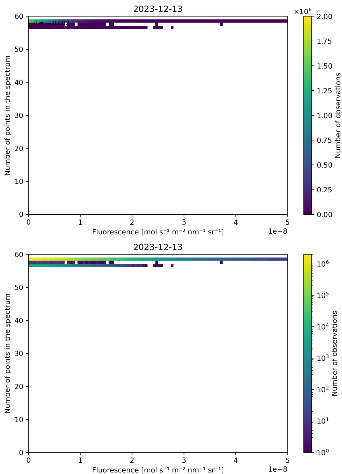
Figure 86: Scatter density plot of “Fluorescence” against “Number of points in the spectrum” for 2023-12-12 to 2023-12-14.
