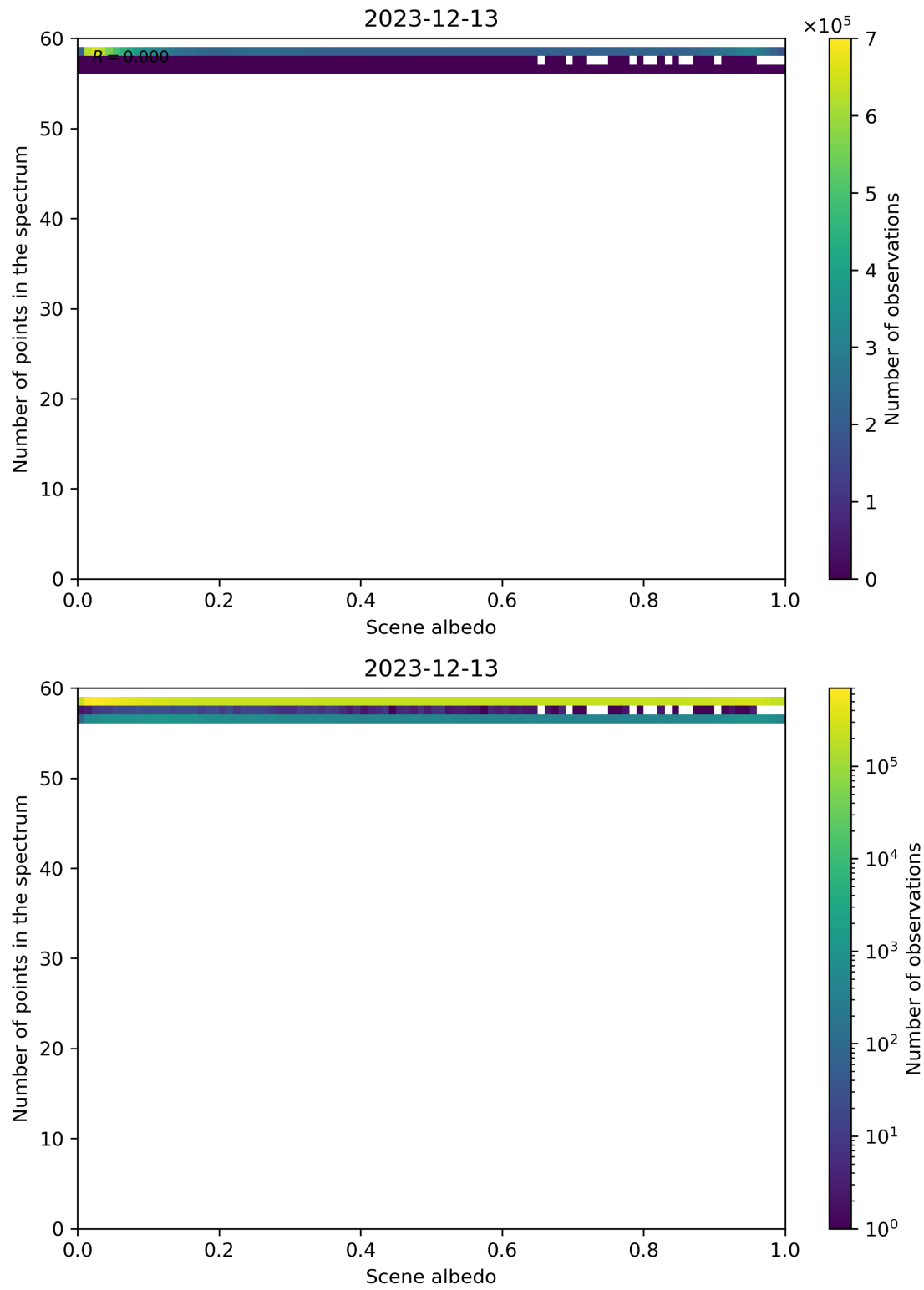
Figure 106: Scatter density plot of “Scene albedo” against “Number of points in the spectrum” for 2023-12-12 to 2023-12-14.
