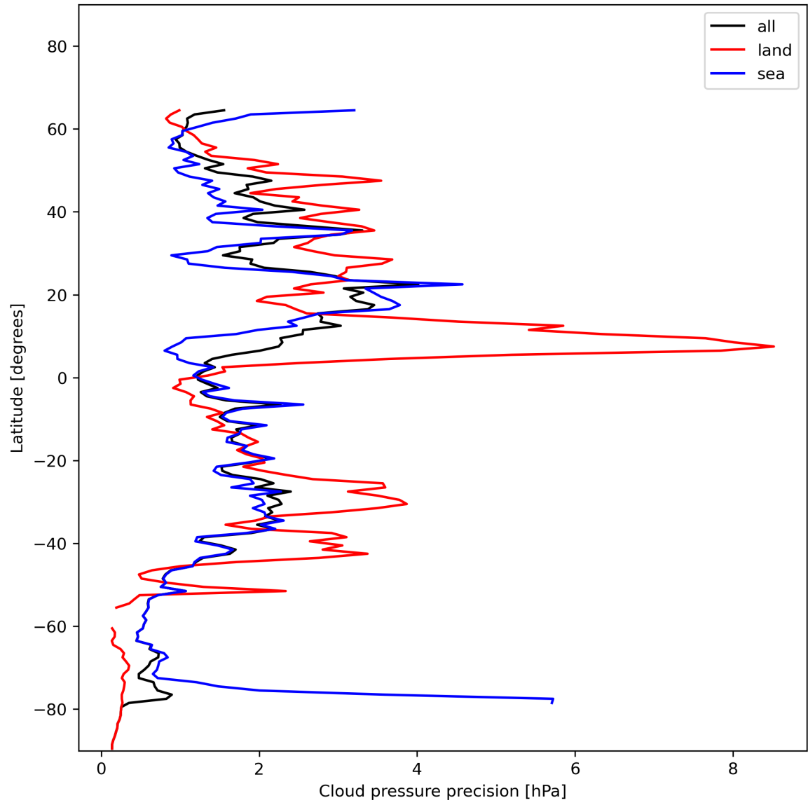
Figure 14: Zonal average of “Cloud pressure precision” for 2023-12-12 to 2023-12-14.
