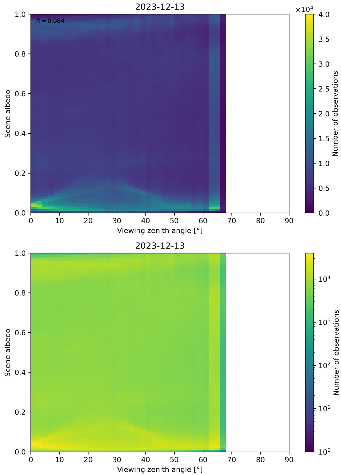
Figure 126: Scatter density plot of “Viewing zenith angle” against “Scene albedo” for 2023-12-12 to 2023-12-14.
