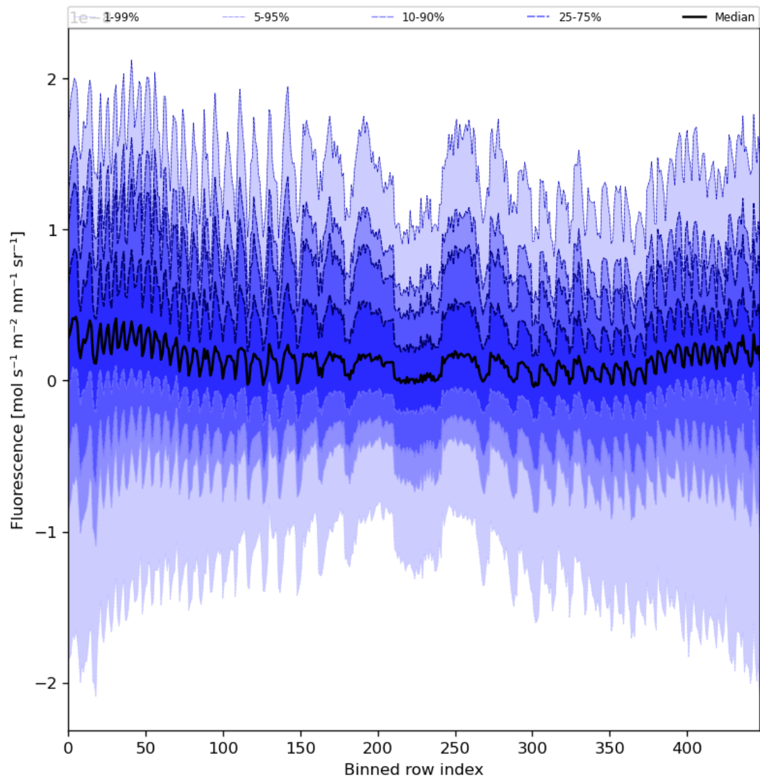
Figure 57: Along track statistics of “Fluorescence” for 2023-12-12 to 2023-12-14
