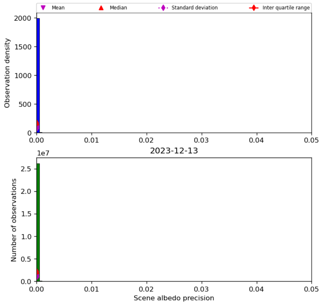
Figure 35: Histogram of “Scene albedo precision” for 2023-12-12 to 2023-12-14
