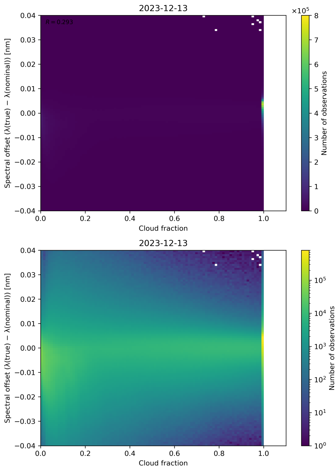
Figure 76: Scatter density plot of “Cloud fraction” against “Spectral offset ( \lambda(\text{true}) - \lambda(\text{nominal}) )” for 2023-12-12 to 2023-12-14.
