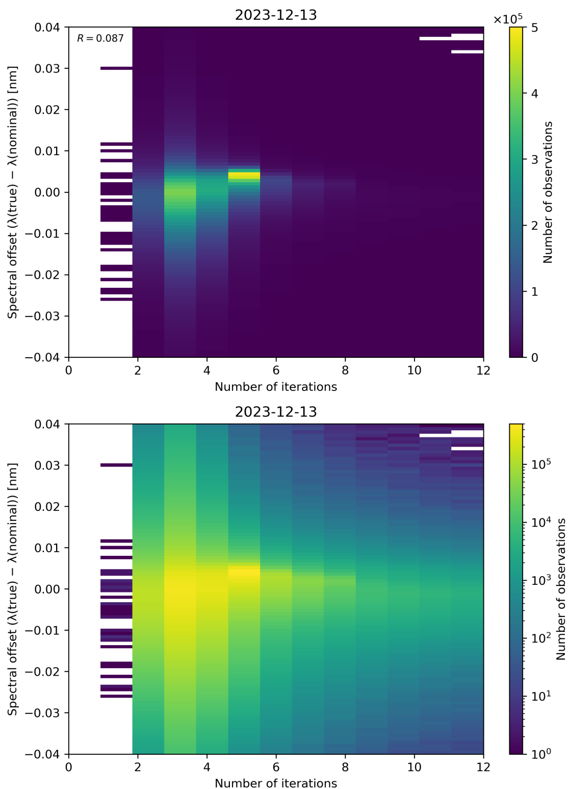
Figure 100: Scatter density plot of “Number of iterations” against “Spectral offset ( \lambda(\text{true}) - \lambda(\text{nominal}) )” for 2023-12-12 to 2023-12-14.
