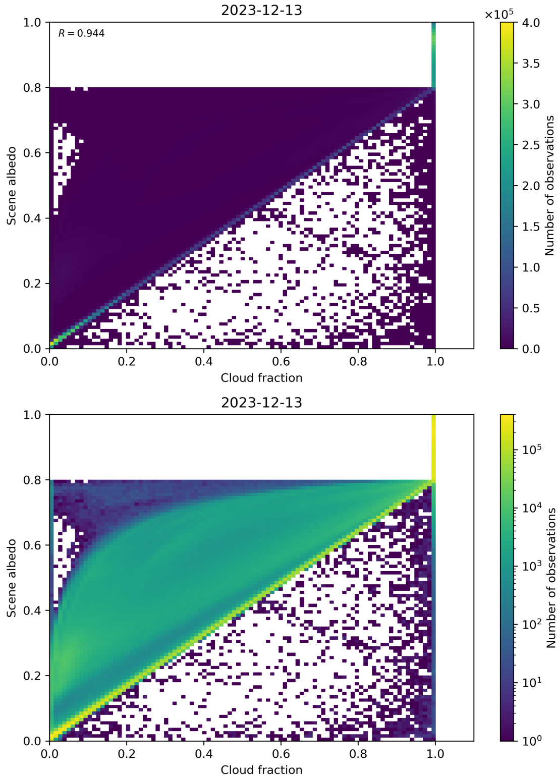
Figure 75: Scatter density plot of “Cloud fraction” against “Scene albedo” for 2023-12-12 to 2023-12-14.
