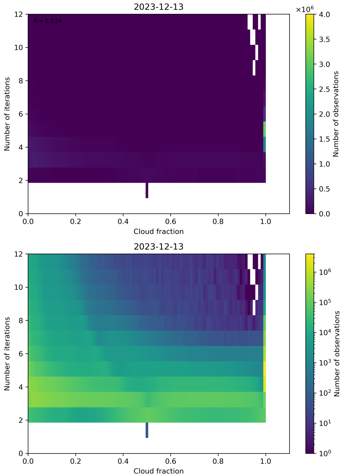
Figure 73: Scatter density plot of “Cloud fraction” against “Number of iterations” for 2023-12-12 to 2023-12-14.
