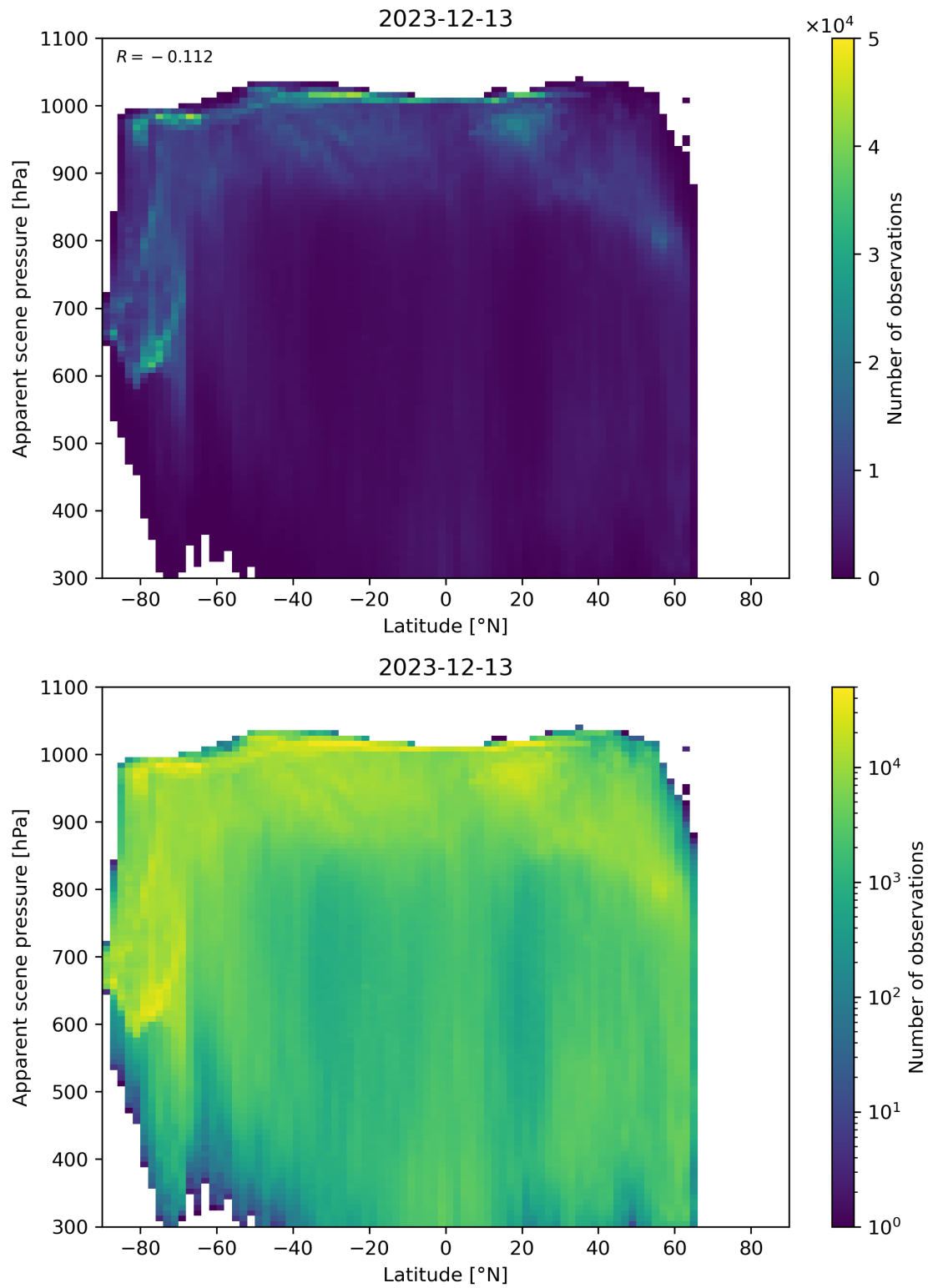
Figure 88: Scatter density plot of “Latitude” against “Apparent scene pressure” for 2023-12-12 to 2023-12-14.
