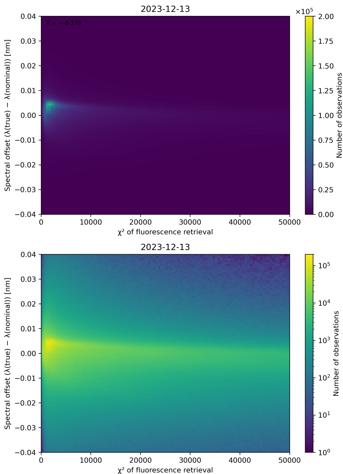
Figure 69: Scatter density plot of " \chi^2 of fluorescence retrieval" against "Spectral offset ( \lambda(\text{true}) - \lambda(\text{nominal}) )" for 2023-12-12 to 2023-12-14.
