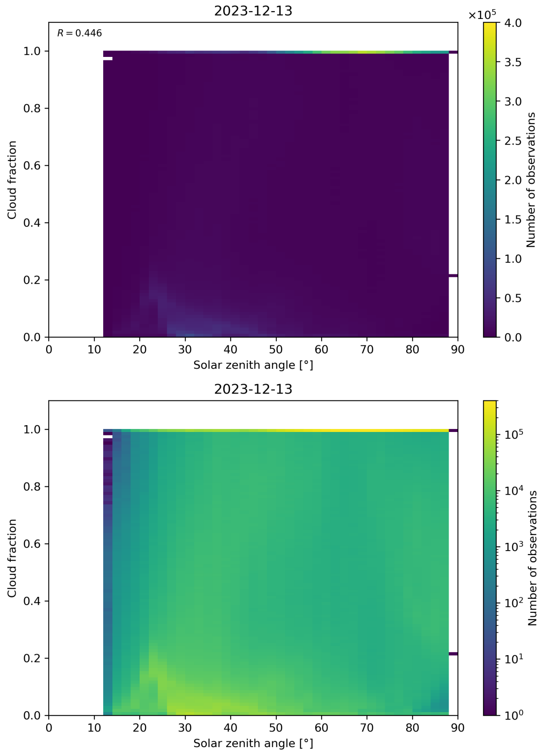
Figure 110: Scatter density plot of “Solar zenith angle” against “Cloud fraction” for 2023-12-12 to 2023-12-14.
