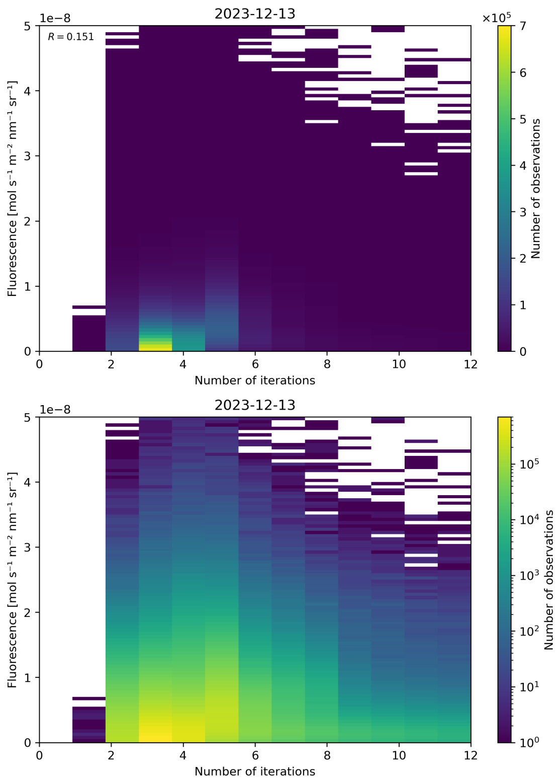
Figure 98: Scatter density plot of “Number of iterations” against “Fluorescence” for 2023-12-12 to 2023-12-14.
