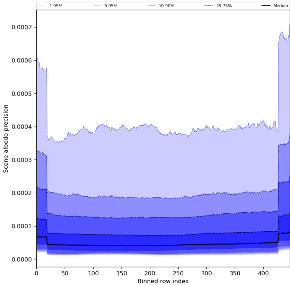
Figure 52: Along track statistics of “Scene albedo precision” for 2023-12-12 to 2023-12-14
