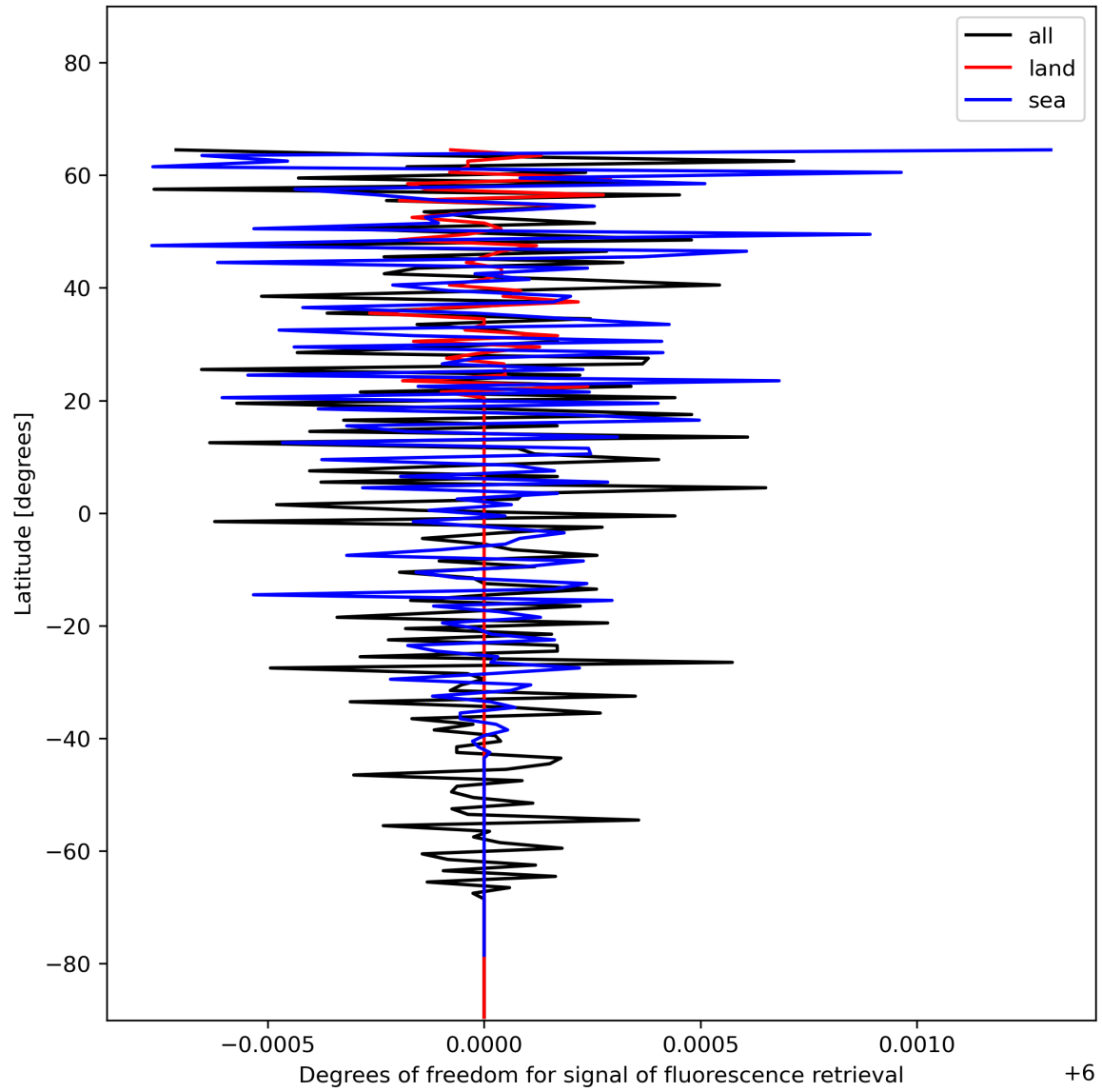
Figure 26: Zonal average of “Degrees of freedom for signal of fluorescence retrieval” for 2023-12-12 to 2023-12-14.
