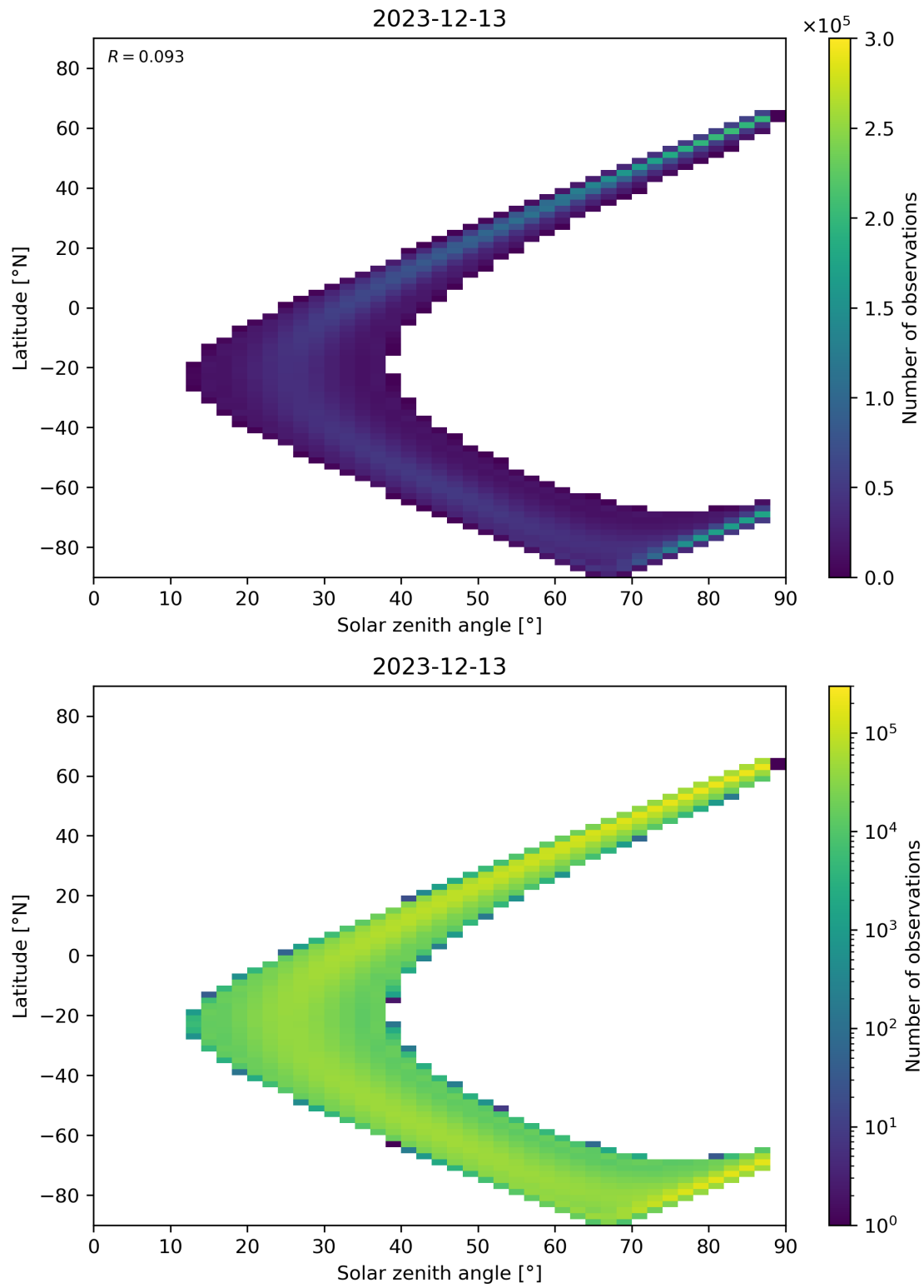
Figure 113: Scatter density plot of “Solar zenith angle” against “Latitude” for 2023-12-12 to 2023-12-14.
