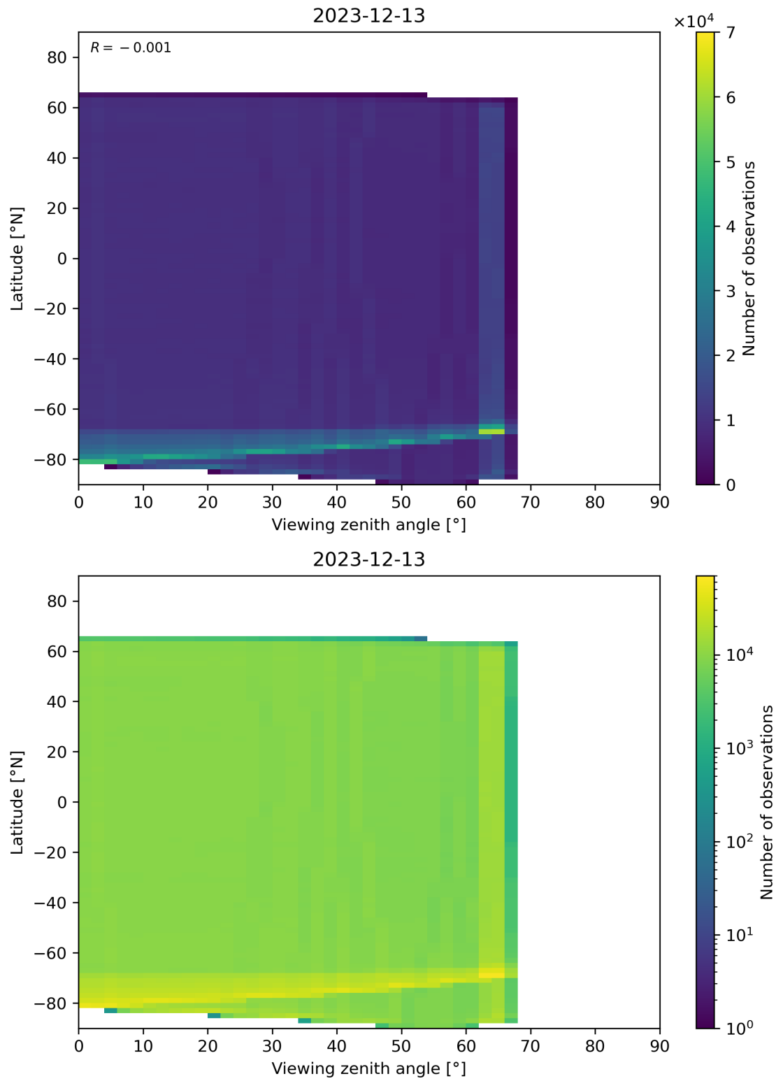
Figure 123: Scatter density plot of “Viewing zenith angle” against “Latitude” for 2023-12-12 to 2023-12-14.
