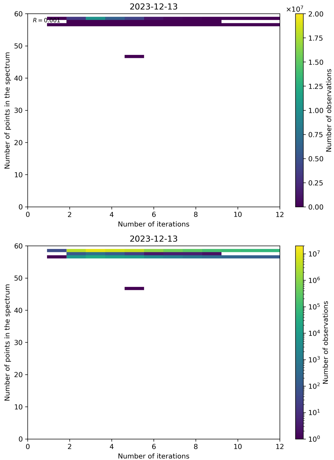
Figure 99: Scatter density plot of “Number of iterations” against “Number of points in the spectrum” for 2023-12-12 to 2023-12-14.
