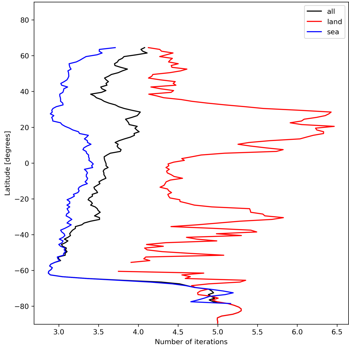
Figure 22: Zonal average of “Number of iterations” for 2023-12-12 to 2023-12-14.
