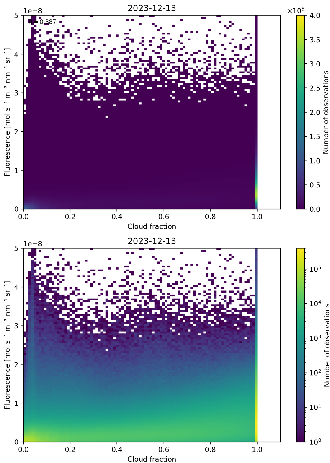
Figure 72: Scatter density plot of “Cloud fraction” against “Fluorescence” for 2023-12-12 to 2023-12-14.
