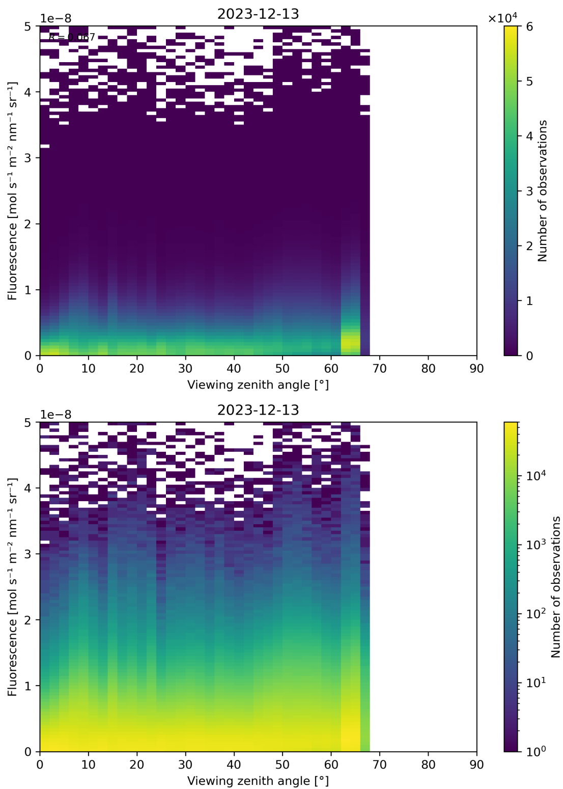
Figure 122: Scatter density plot of “Viewing zenith angle” against “Fluorescence” for 2023-12-12 to 2023-12-14.
