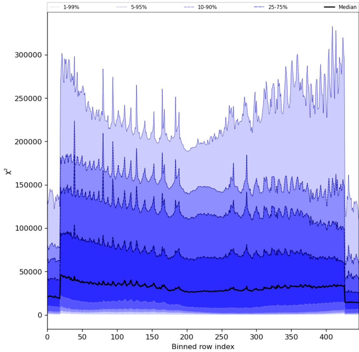
Figure 55: Along track statistics of “ \chi^2 ” for 2023-12-12 to 2023-12-14
