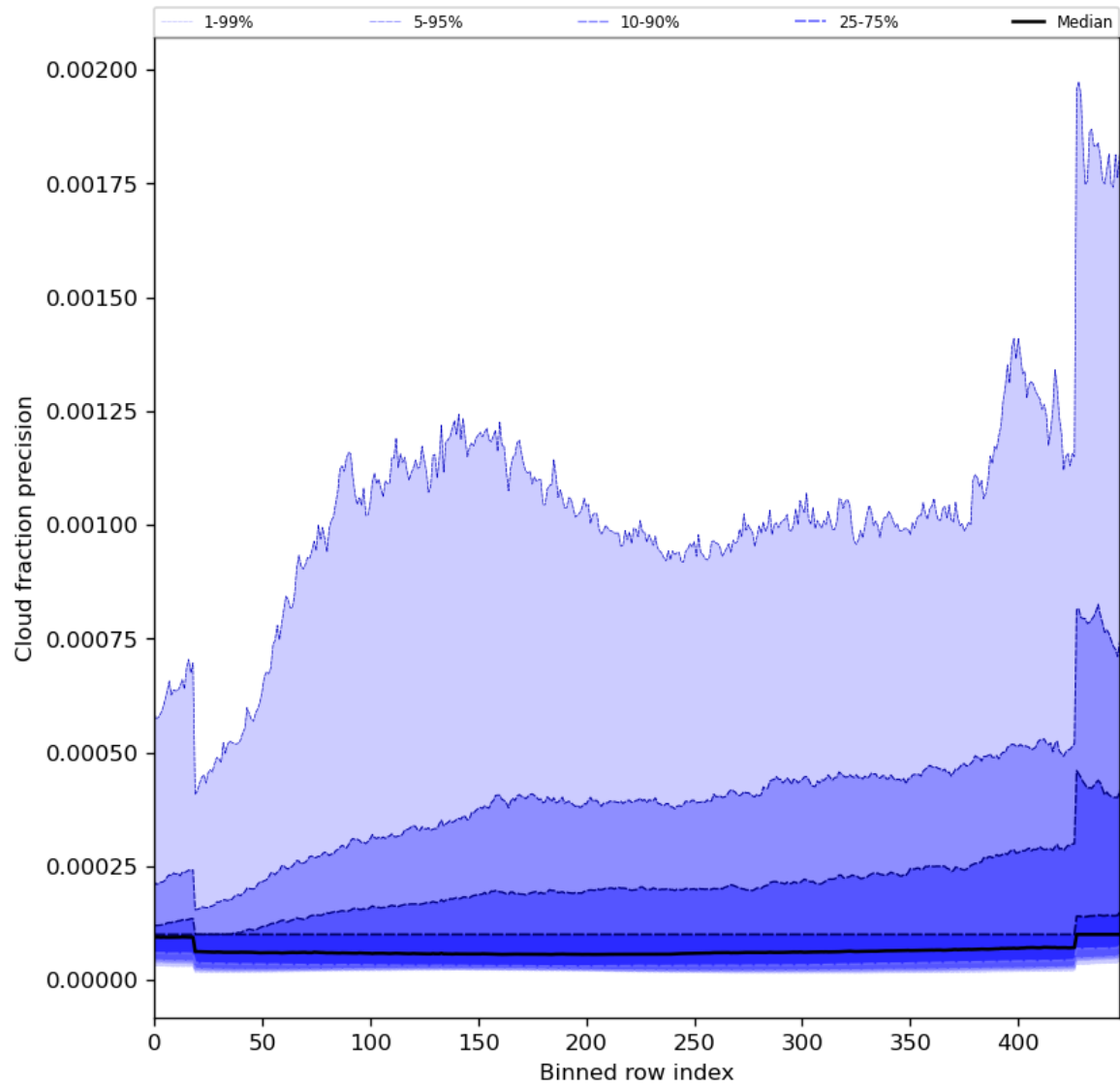
Figure 50: Along track statistics of “Cloud fraction precision” for 2023-12-12 to 2023-12-14
