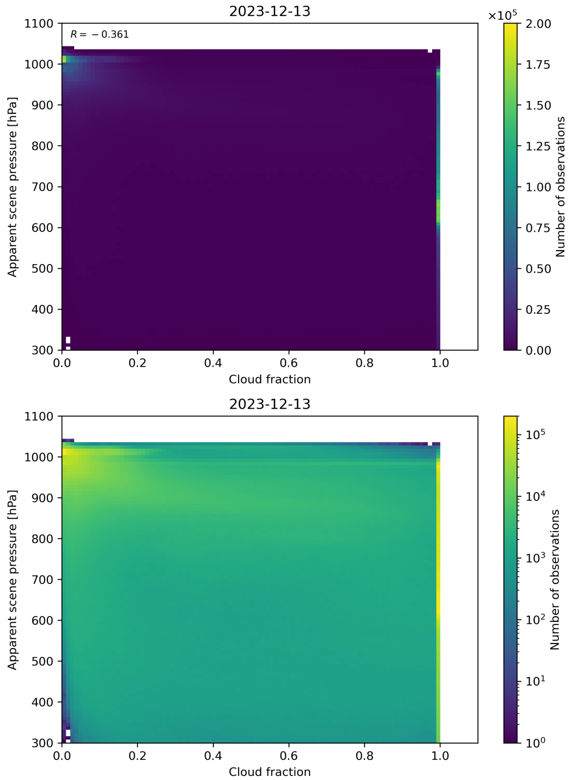
Figure 70: Scatter density plot of “Cloud fraction” against “Apparent scene pressure” for 2023-12-12 to 2023-12-14.
