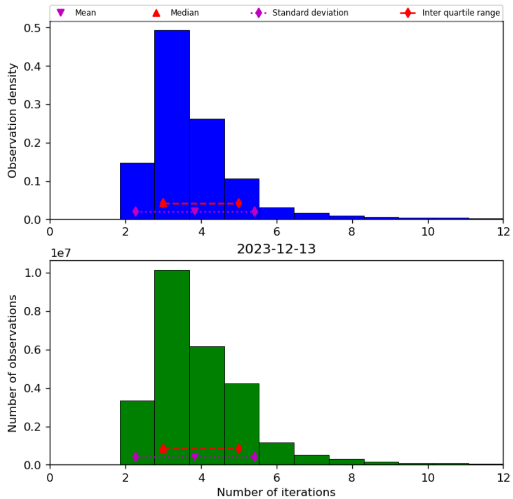
Figure 39: Histogram of “Number of iterations” for 2023-12-12 to 2023-12-14
