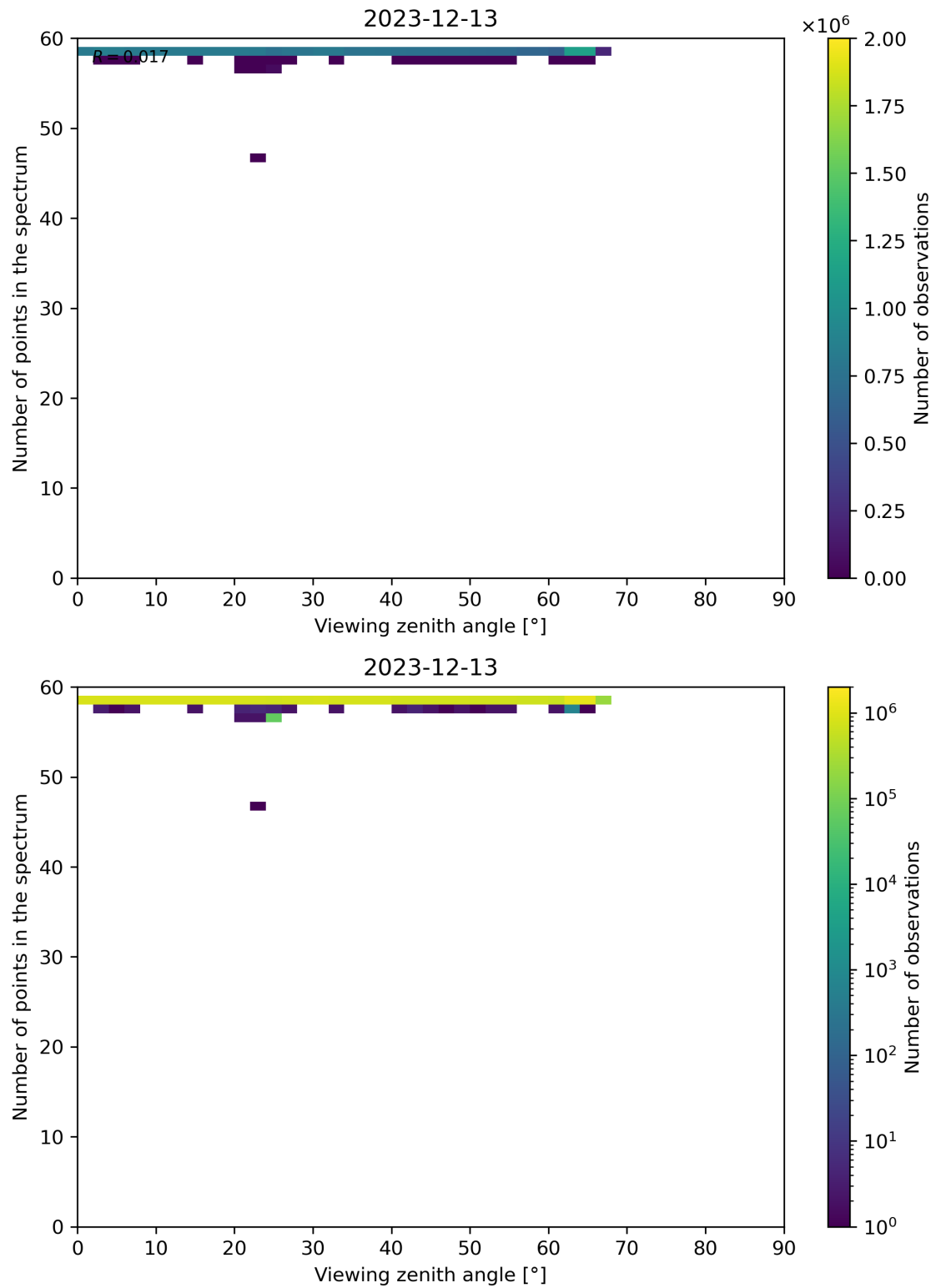
Figure 125: Scatter density plot of “Viewing zenith angle” against “Number of points in the spectrum” for 2023-12-12 to 2023-12-14.
