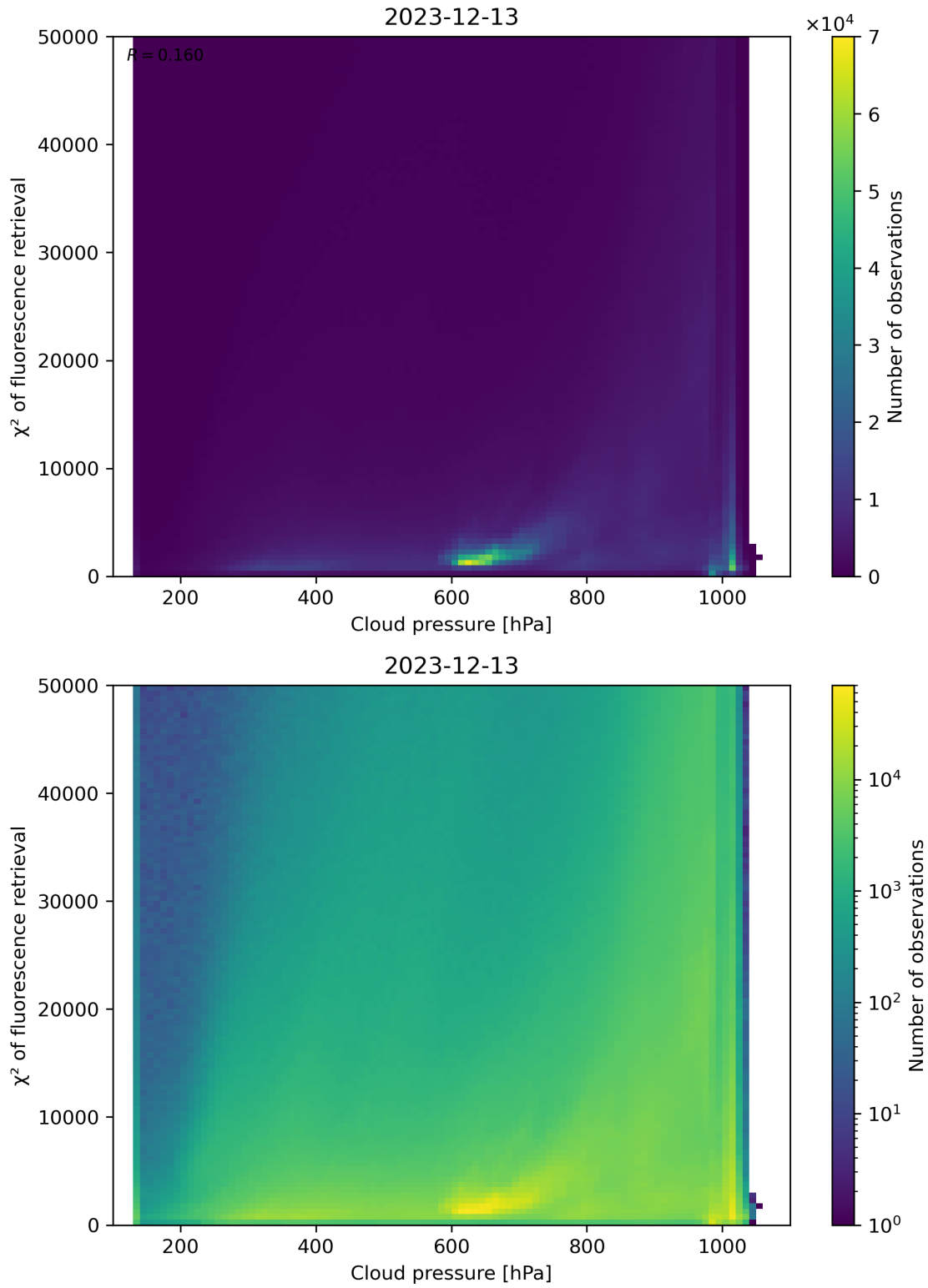
Figure 78: Scatter density plot of “Cloud pressure” against “ \chi^2 of fluorescence retrieval” for 2023-12-12 to 2023-12-14.
