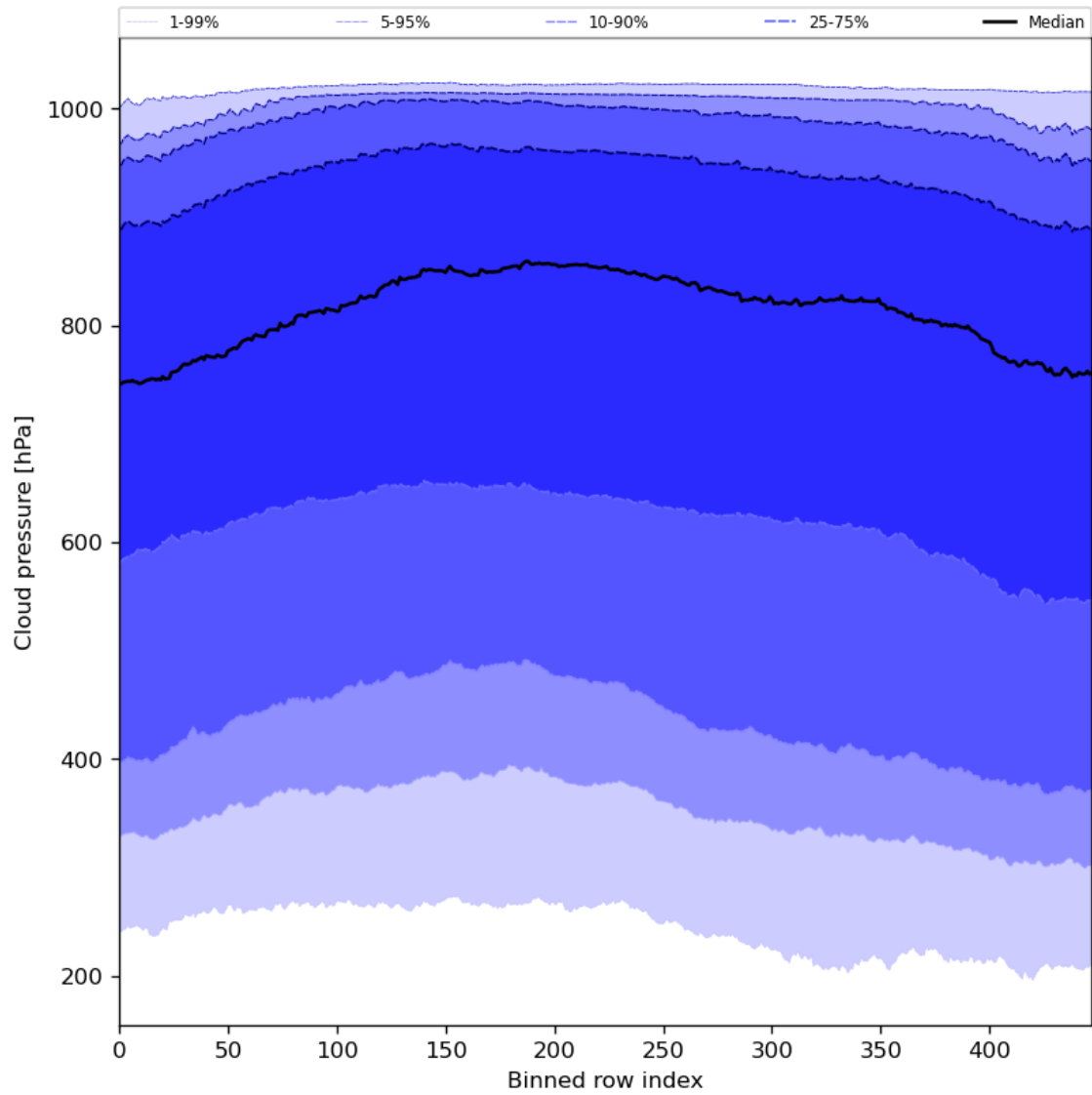
Figure 47: Along track statistics of “Cloud pressure” for 2023-12-12 to 2023-12-14
