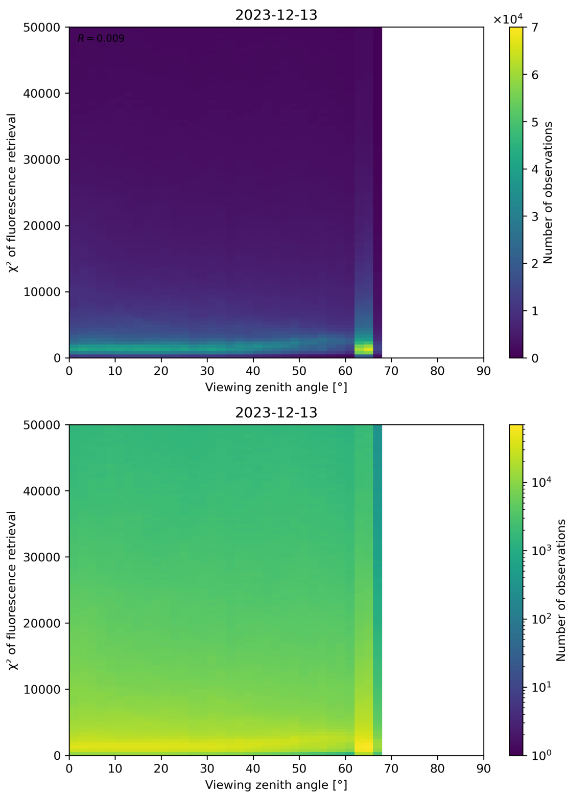
Figure 119: Scatter density plot of “Viewing zenith angle” against “ \chi^2 of fluorescence retrieval” for 2023-12-12 to 2023-12-14.
