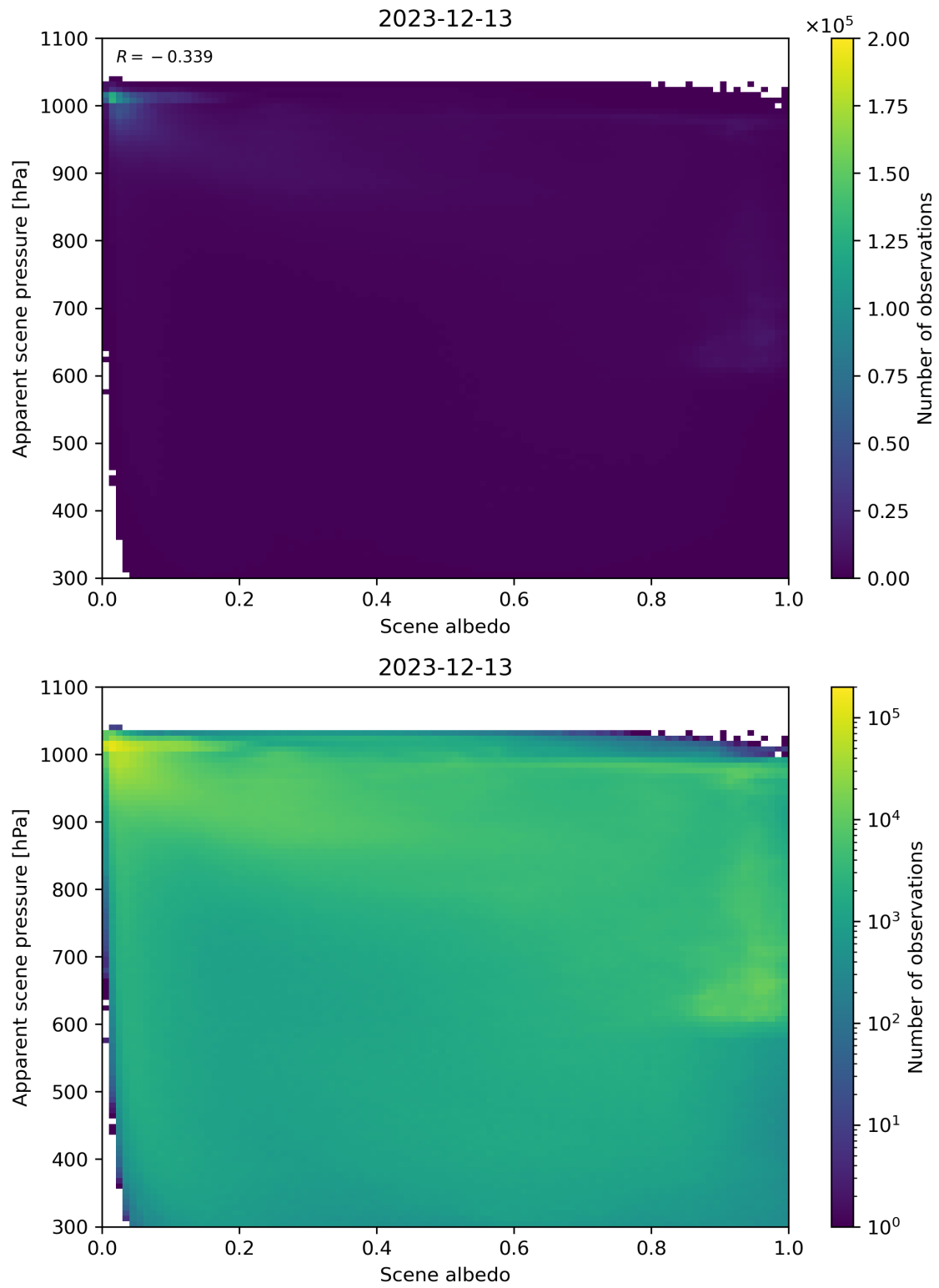
Figure 102: Scatter density plot of “Scene albedo” against “Apparent scene pressure” for 2023-12-12 to 2023-12-14.
