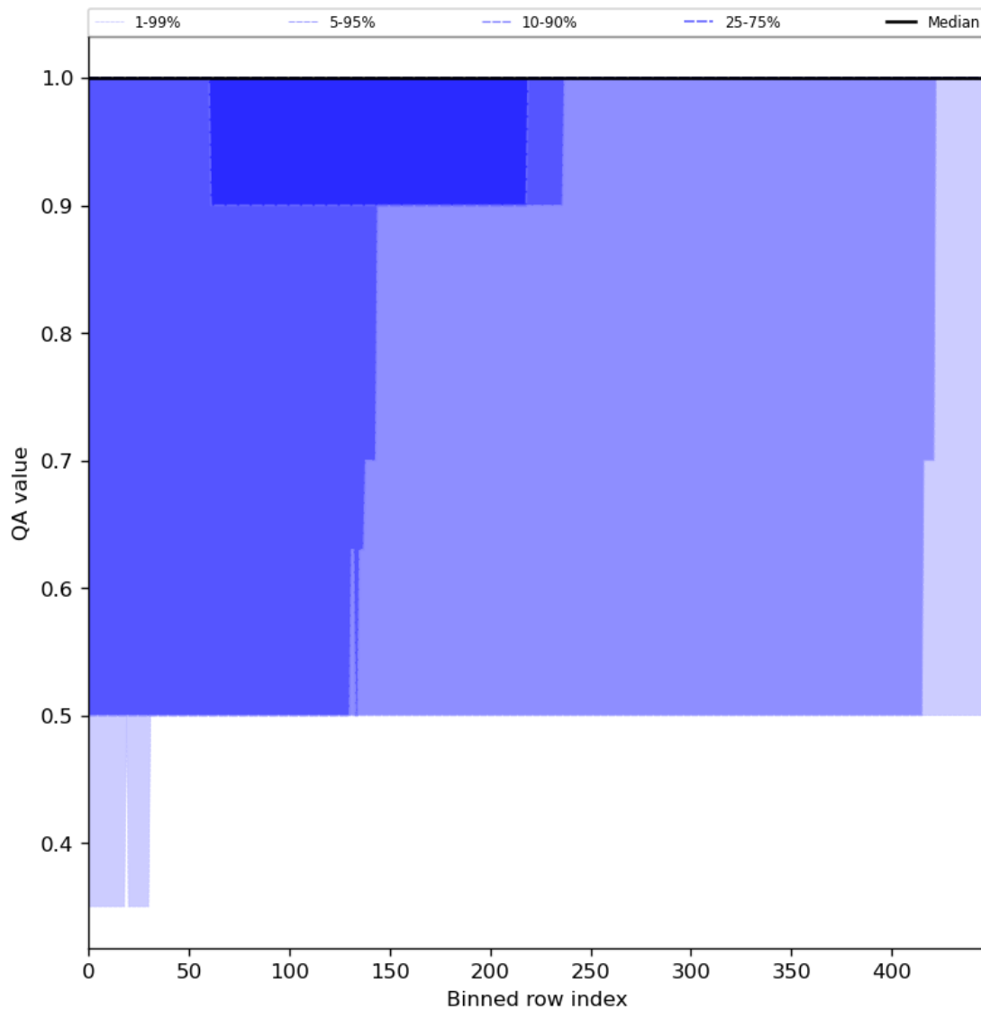
Figure 46: Along track statistics of “QA value” for 2023-12-12 to 2023-12-14
