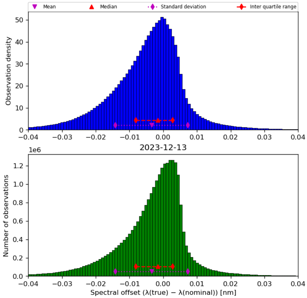
Figure 45: Histogram of “Spectral offset ( \lambda(\text{true}) - \lambda(\text{nominal}) )” for 2023-12-12 to 2023-12-14
