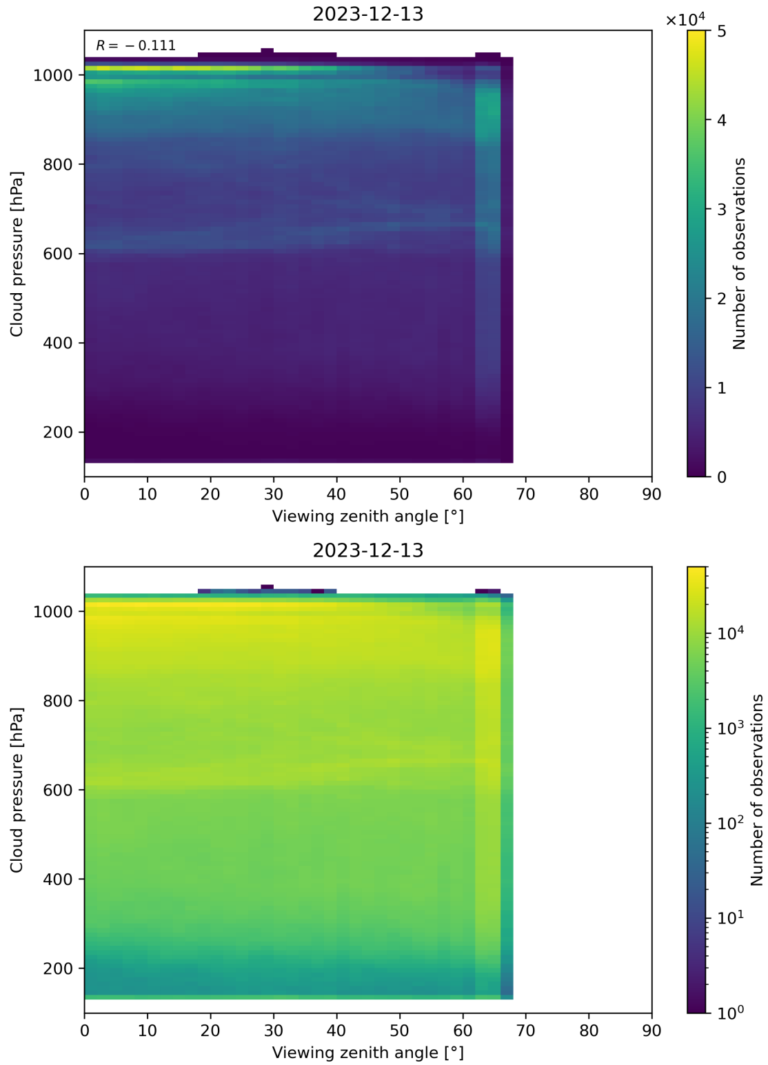
Figure 121: Scatter density plot of “Viewing zenith angle” against “Cloud pressure” for 2023-12-12 to 2023-12-14.
