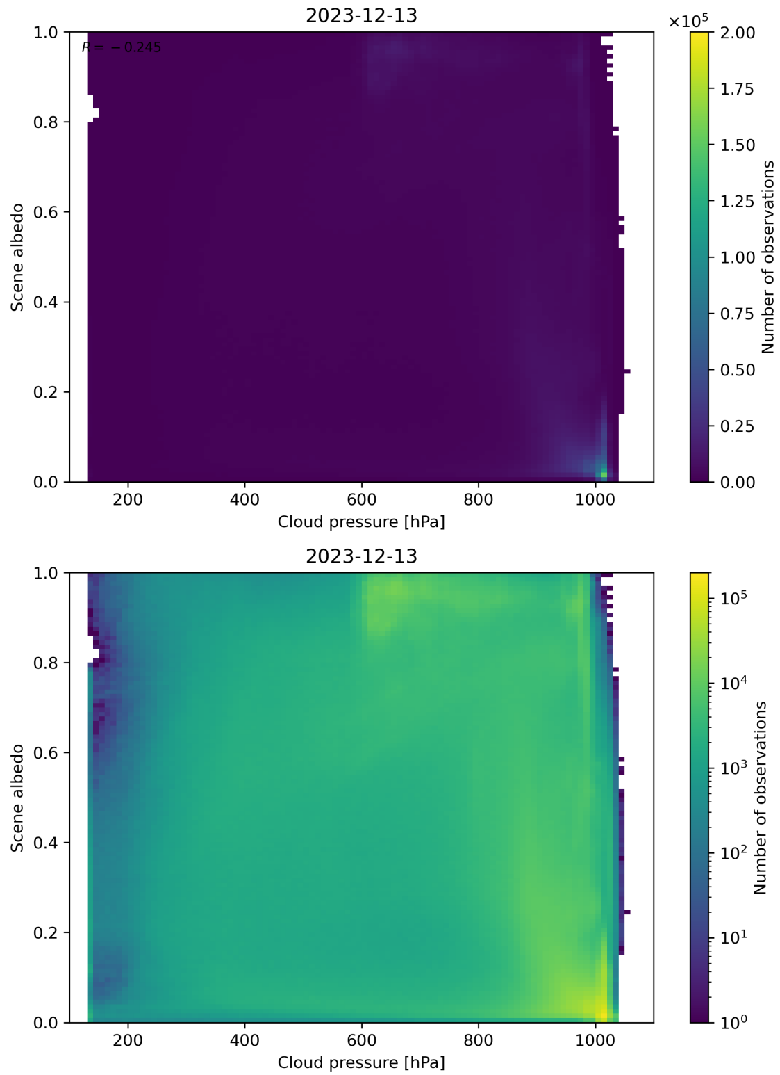
Figure 83: Scatter density plot of “Cloud pressure” against “Scene albedo” for 2023-12-12 to 2023-12-14.
