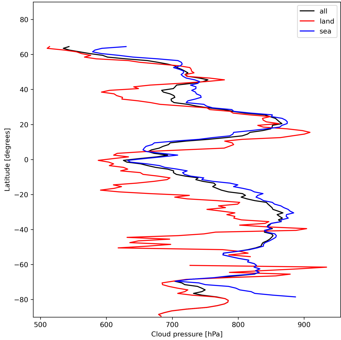
Figure 13: Zonal average of “Cloud pressure” for 2023-12-12 to 2023-12-14.
