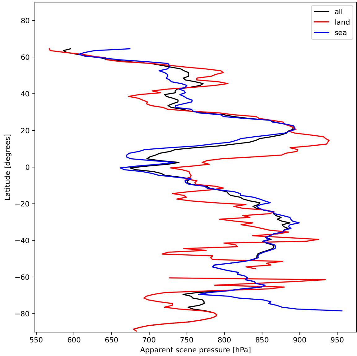
Figure 19: Zonal average of “Apparent scene pressure” for 2023-12-12 to 2023-12-14.
