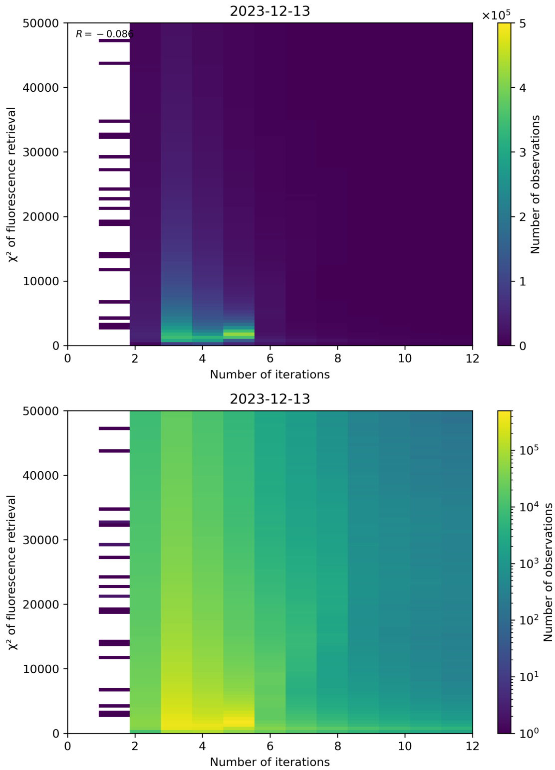
Figure 97: Scatter density plot of “Number of iterations” against “ \chi^2 of fluorescence retrieval” for 2023-12-12 to 2023-12-14.
