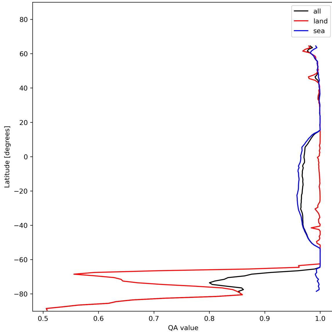
Figure 12: Zonal average of “QA value” for 2023-12-12 to 2023-12-14.
