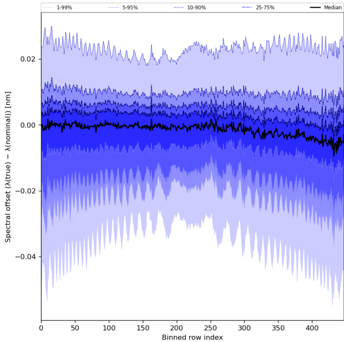
Figure 62: Along track statistics of “Spectral offset ( \lambda(\text{true}) - \lambda(\text{nominal}) )” for 2023-12-12 to 2023-12-14
