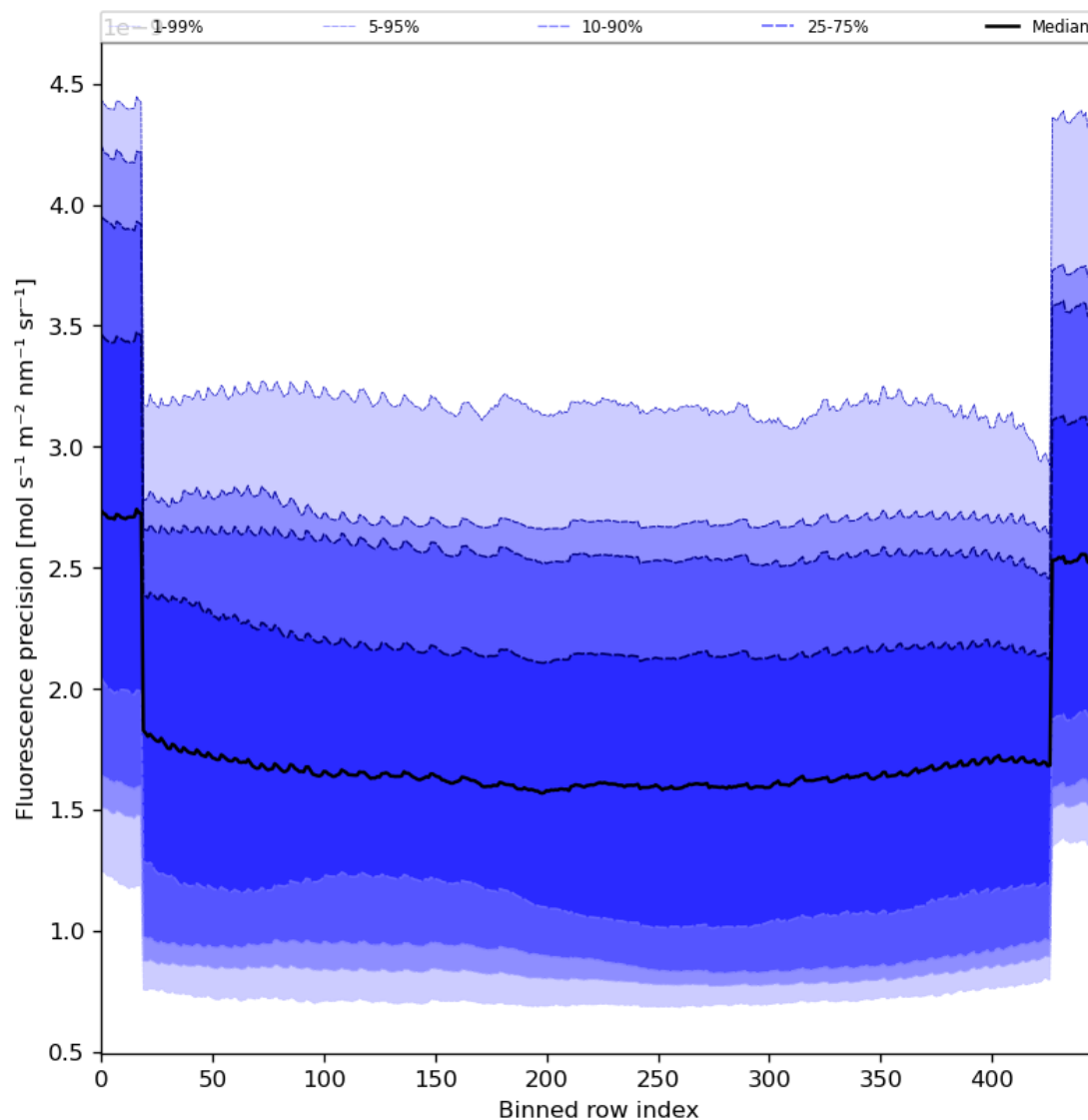
Figure 58: Along track statistics of “Fluorescence precision” for 2023-12-12 to 2023-12-14
