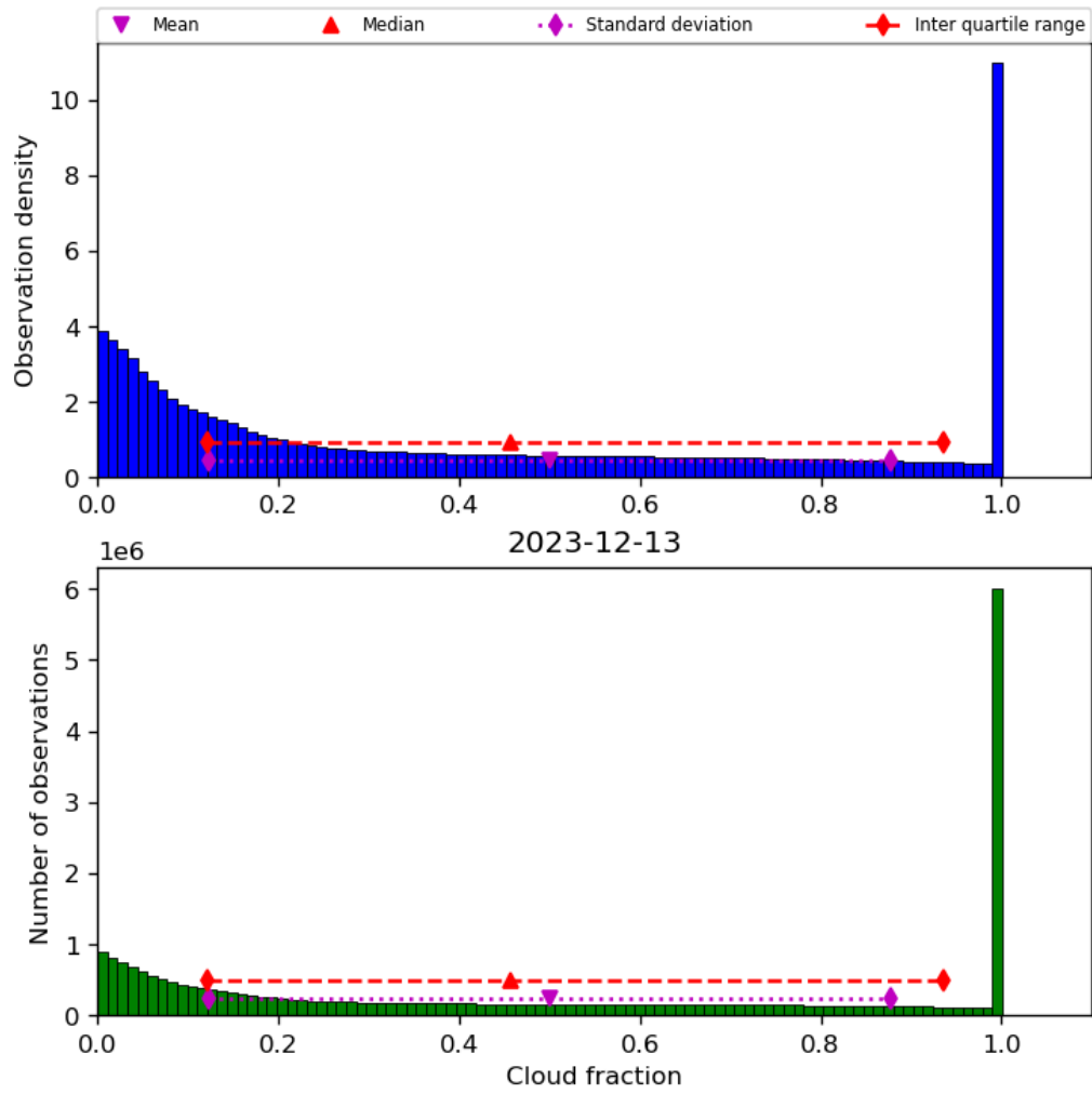
Figure 32: Histogram of “Cloud fraction” for 2023-12-12 to 2023-12-14
