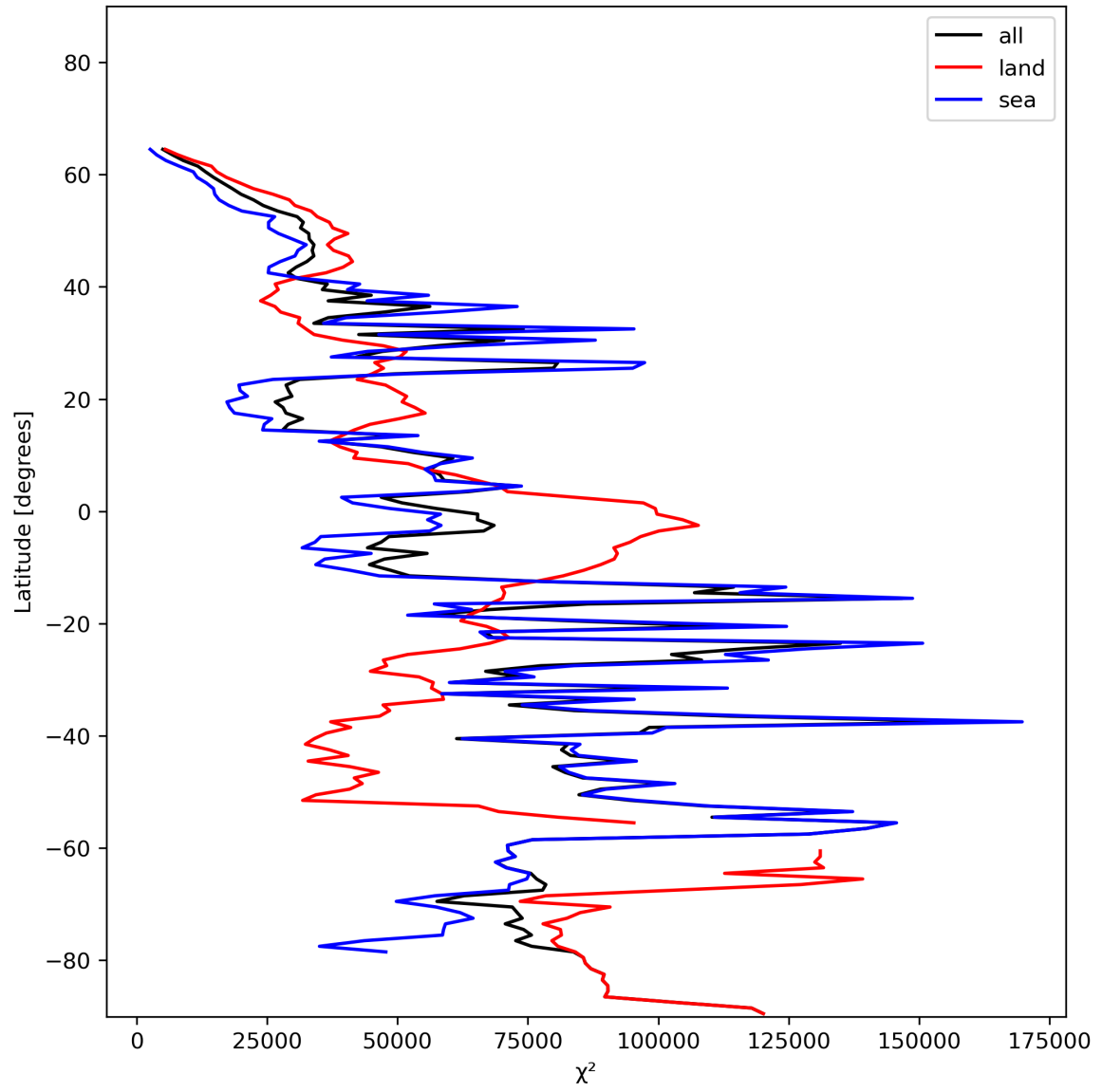
Figure 21: Zonal average of “ \chi^2 ” for 2023-12-12 to 2023-12-14.
