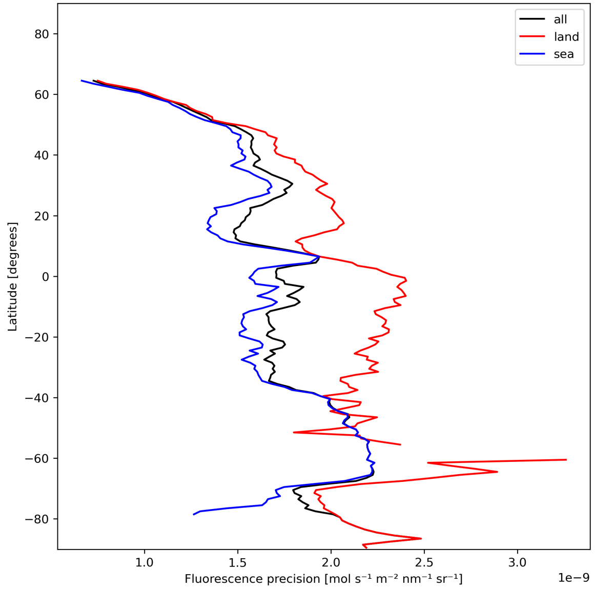
Figure 24: Zonal average of “Fluorescence precision” for 2023-12-12 to 2023-12-14.
