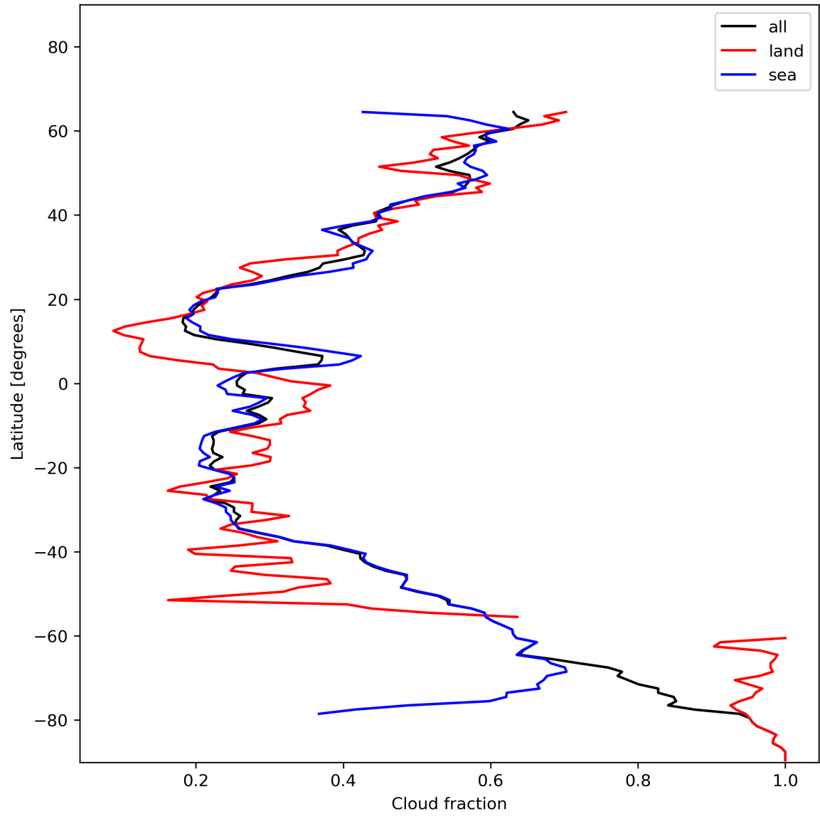
Figure 15: Zonal average of “Cloud fraction” for 2023-12-12 to 2023-12-14.
