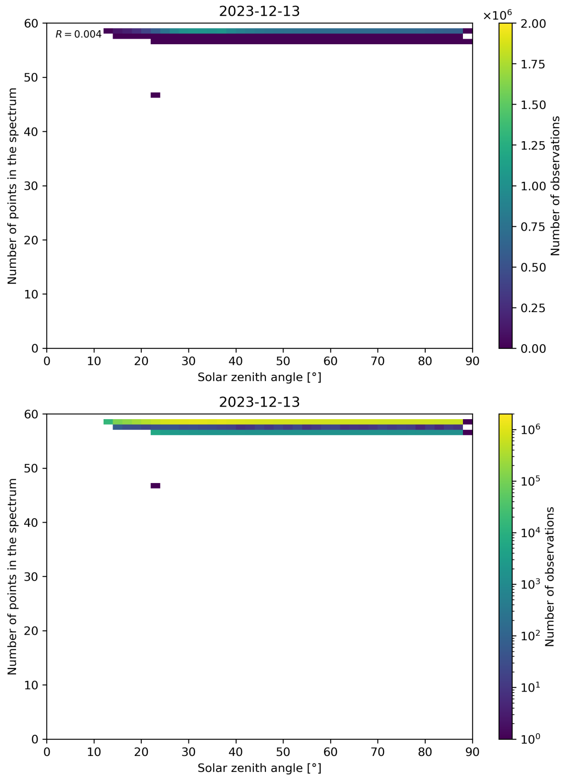
Figure 115: Scatter density plot of “Solar zenith angle” against “Number of points in the spectrum” for 2023-12-12 to 2023-12-14.
