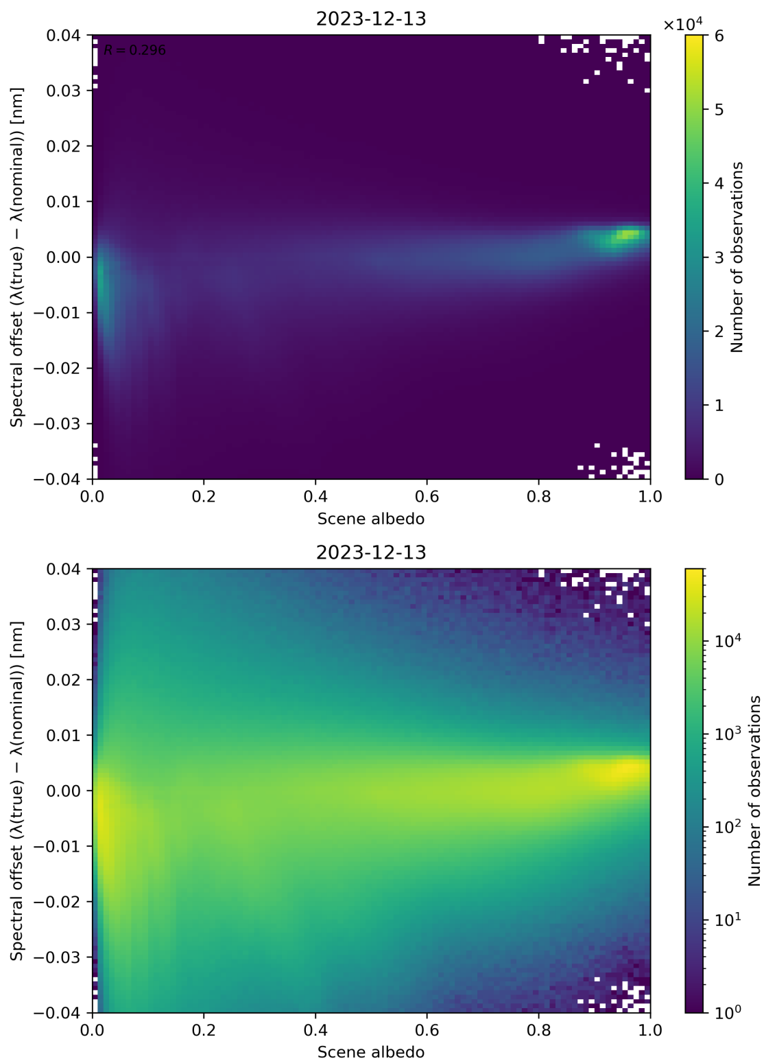
Figure 107: Scatter density plot of “Scene albedo” against “Spectral offset ( \lambda(\text{true}) - \lambda(\text{nominal}) )” for 2023-12-12 to 2023-12-14.
