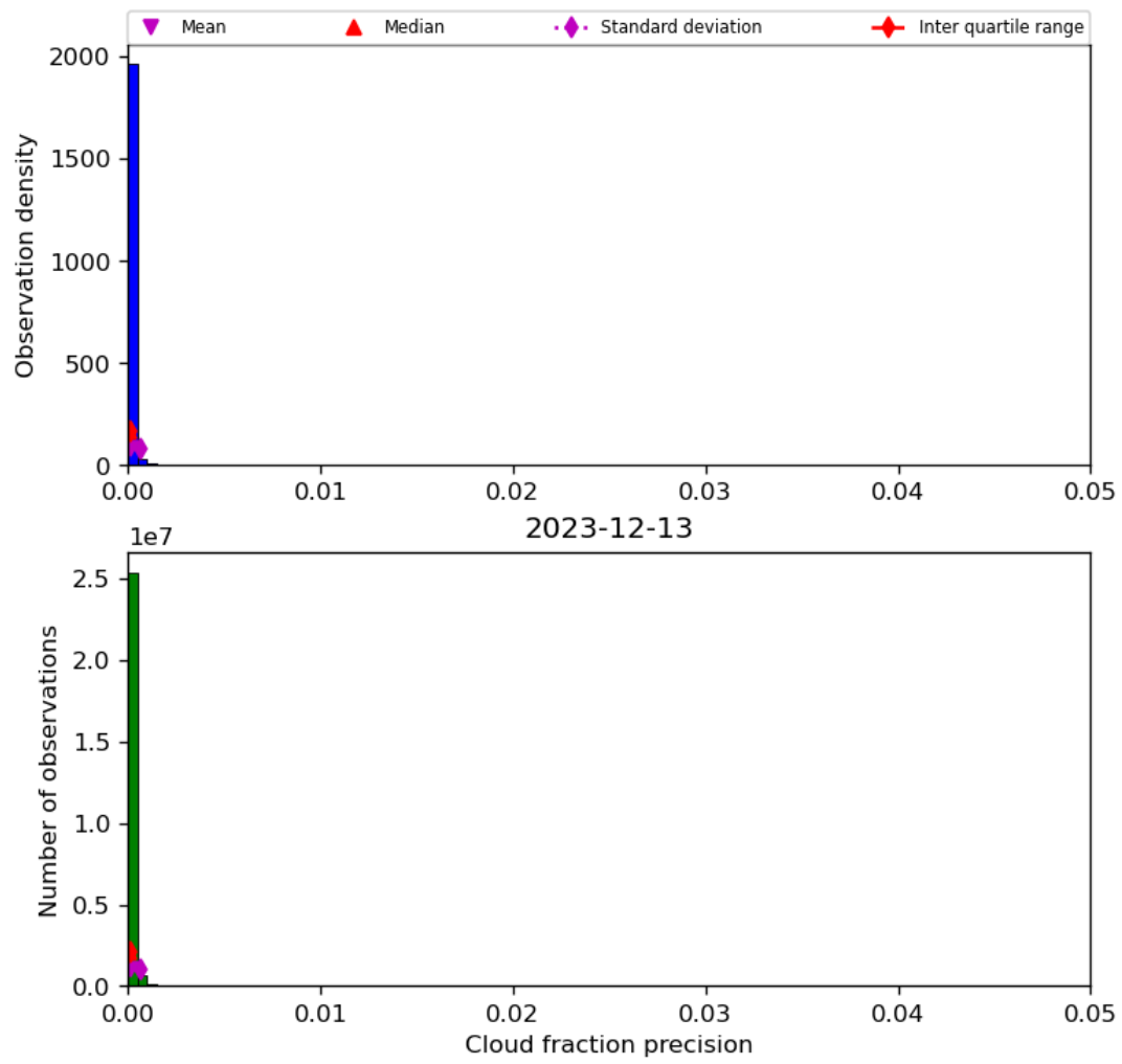
Figure 33: Histogram of “Cloud fraction precision” for 2023-12-12 to 2023-12-14
