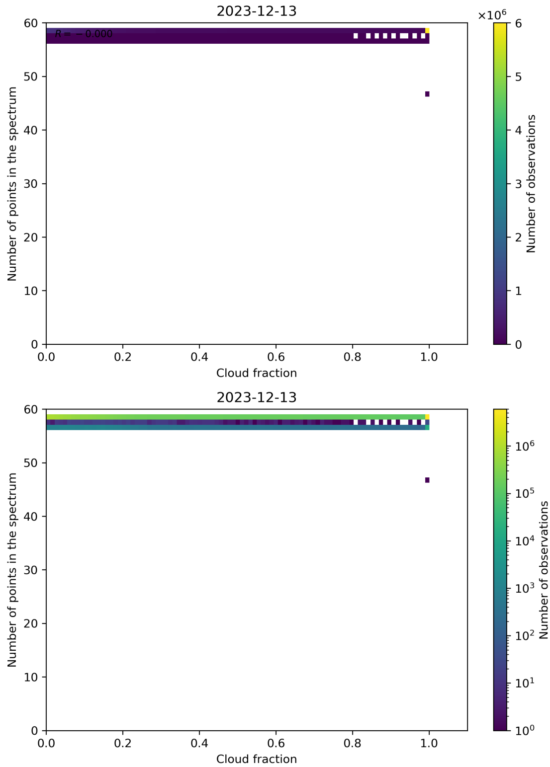
Figure 74: Scatter density plot of “Cloud fraction” against “Number of points in the spectrum” for 2023-12-12 to 2023-12-14.
