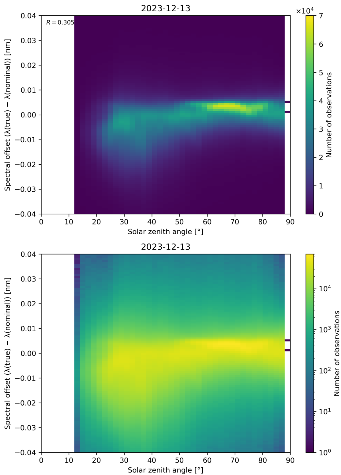
Figure 117: Scatter density plot of “Solar zenith angle” against “Spectral offset ( \lambda(\text{true}) - \lambda(\text{nominal}) )” for 2023-12-12 to 2023-12-14.
