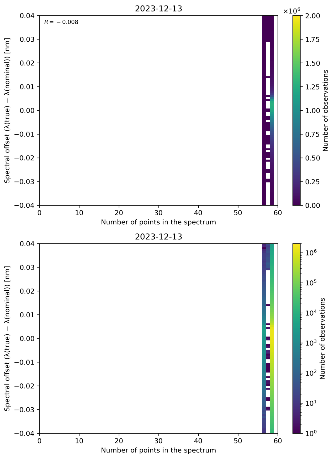
Figure 101: Scatter density plot of “Number of points in the spectrum” against “Spectral offset ( \lambda(\text{true}) - \lambda(\text{nominal}) )” for 2023-12-12 to 2023-12-14.
