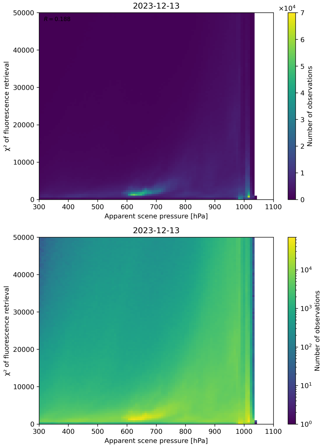
Figure 63: Scatter density plot of “Apparent scene pressure” against “ \chi^2 of fluorescence retrieval” for 2023-12-12 to 2023-12-14.
