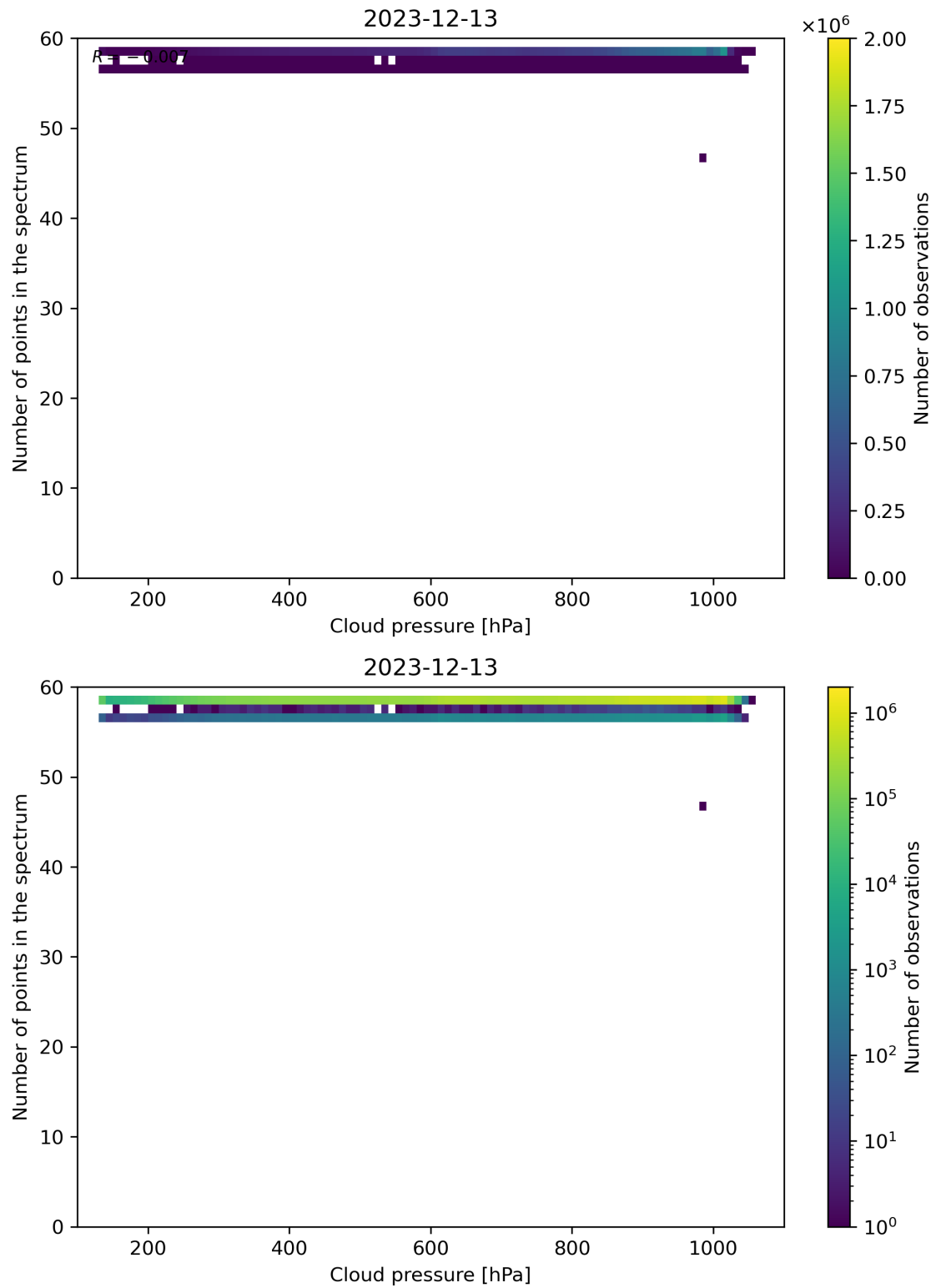
Figure 82: Scatter density plot of “Cloud pressure” against “Number of points in the spectrum” for 2023-12-12 to 2023-12-14.
