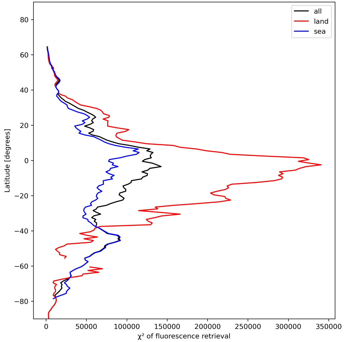
Figure 25: Zonal average of “ \chi^2 of fluorescence retrieval” for 2023-12-12 to 2023-12-14.
