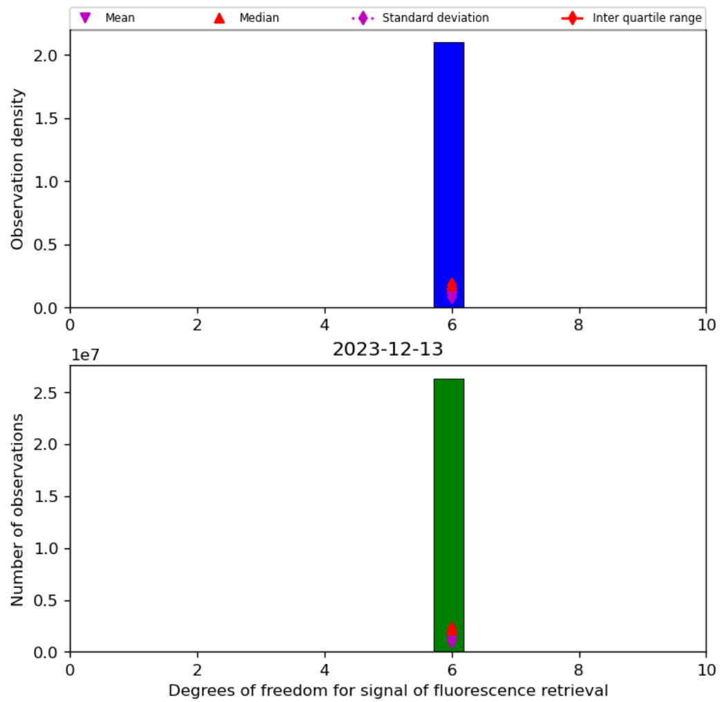
Figure 43: Histogram of “Degrees of freedom for signal of fluorescence retrieval” for 2023-12-12 to 2023-12-14
