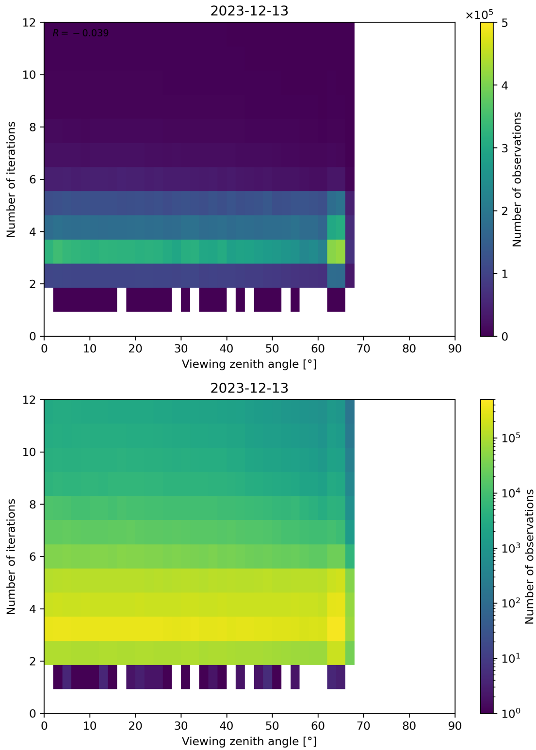
Figure 124: Scatter density plot of “Viewing zenith angle” against “Number of iterations” for 2023-12-12 to 2023-12-14.
