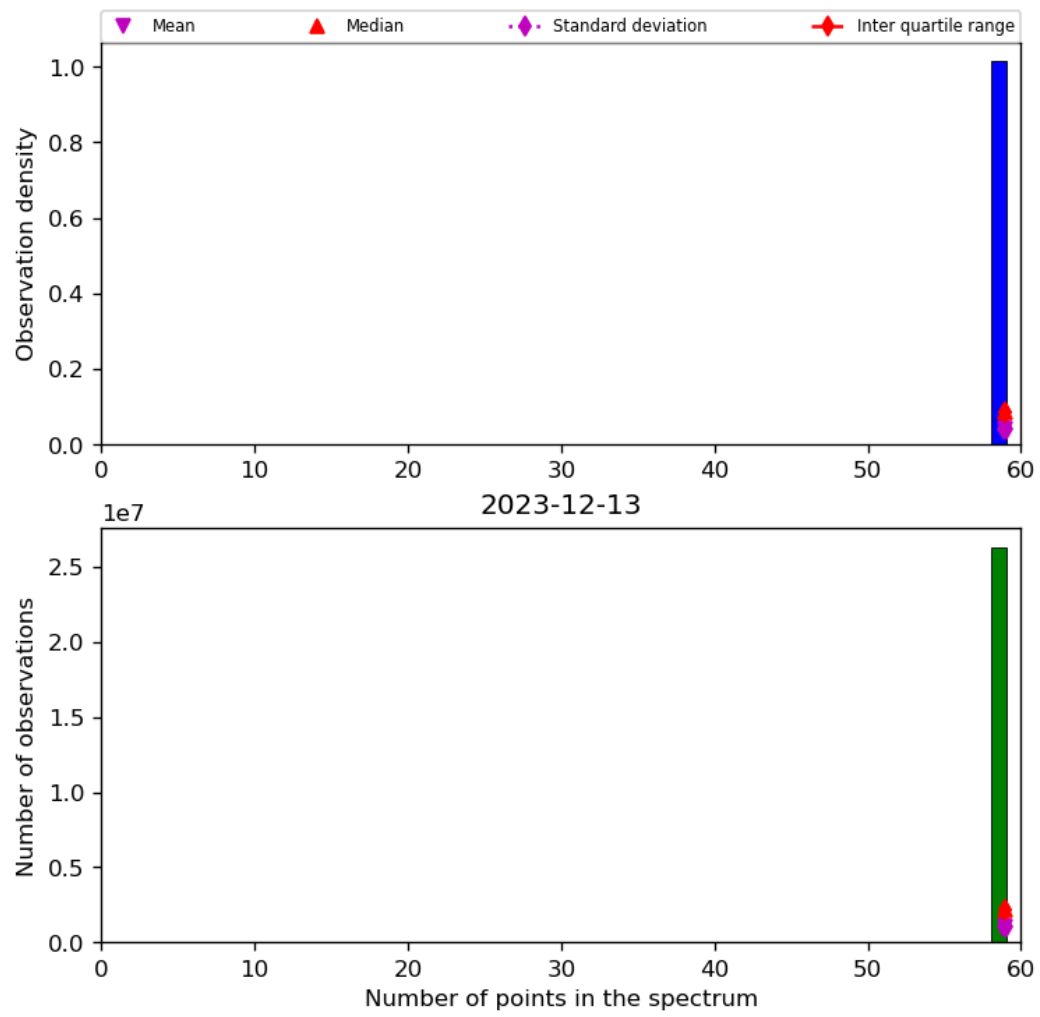
Figure 44: Histogram of "Number of points in the spectrum" for 2023-12-12 to 2023-12-14
