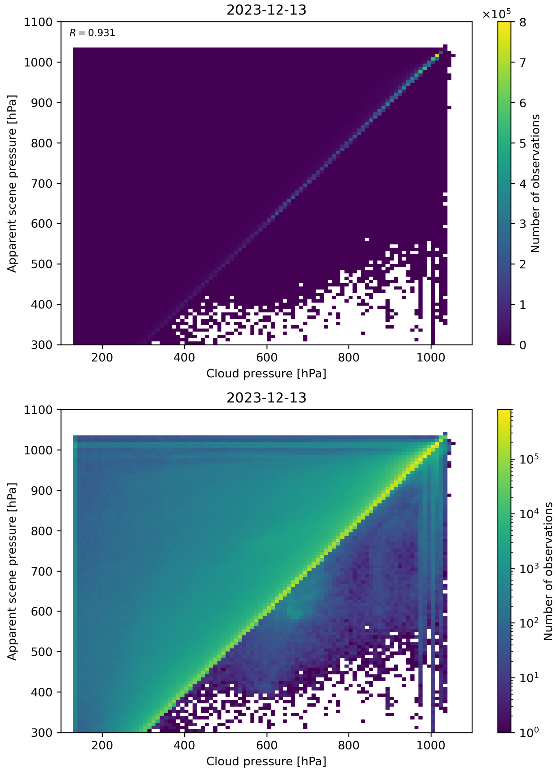
Figure 77: Scatter density plot of “Cloud pressure” against “Apparent scene pressure” for 2023-12-12 to 2023-12-14.
