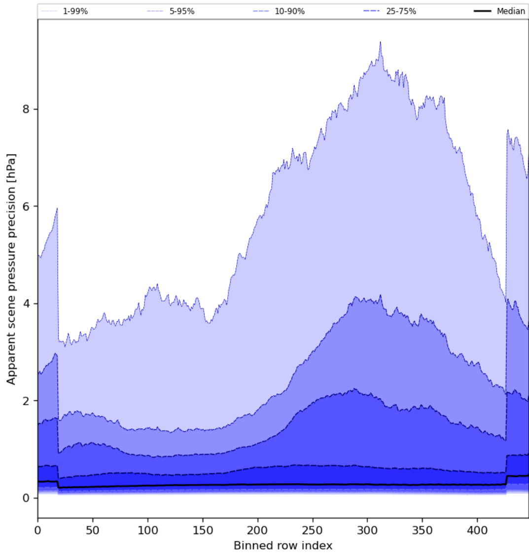
Figure 54: Along track statistics of “Apparent scene pressure precision” for 2023-12-12 to 2023-12-14
