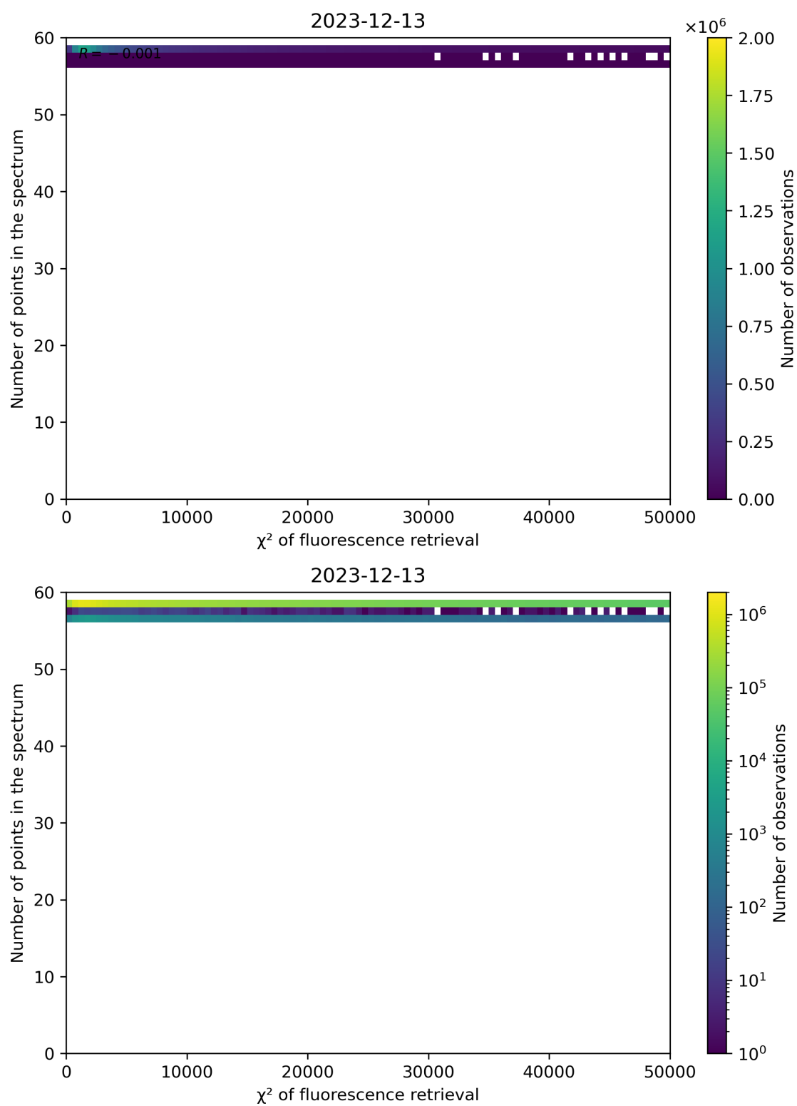
Figure 68: Scatter density plot of " \chi^2 of fluorescence retrieval" against "Number of points in the spectrum" for 2023-12-12 to 2023-12-14.
