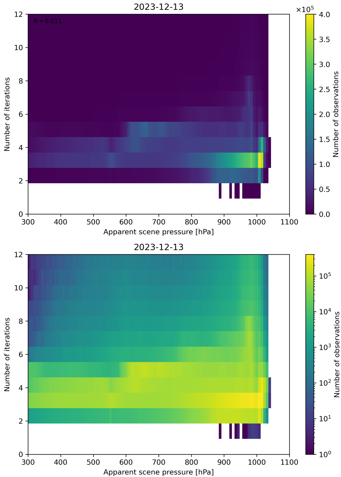
Figure 65: Scatter density plot of “Apparent scene pressure” against “Number of iterations” for 2023-12-12 to 2023-12-14.
