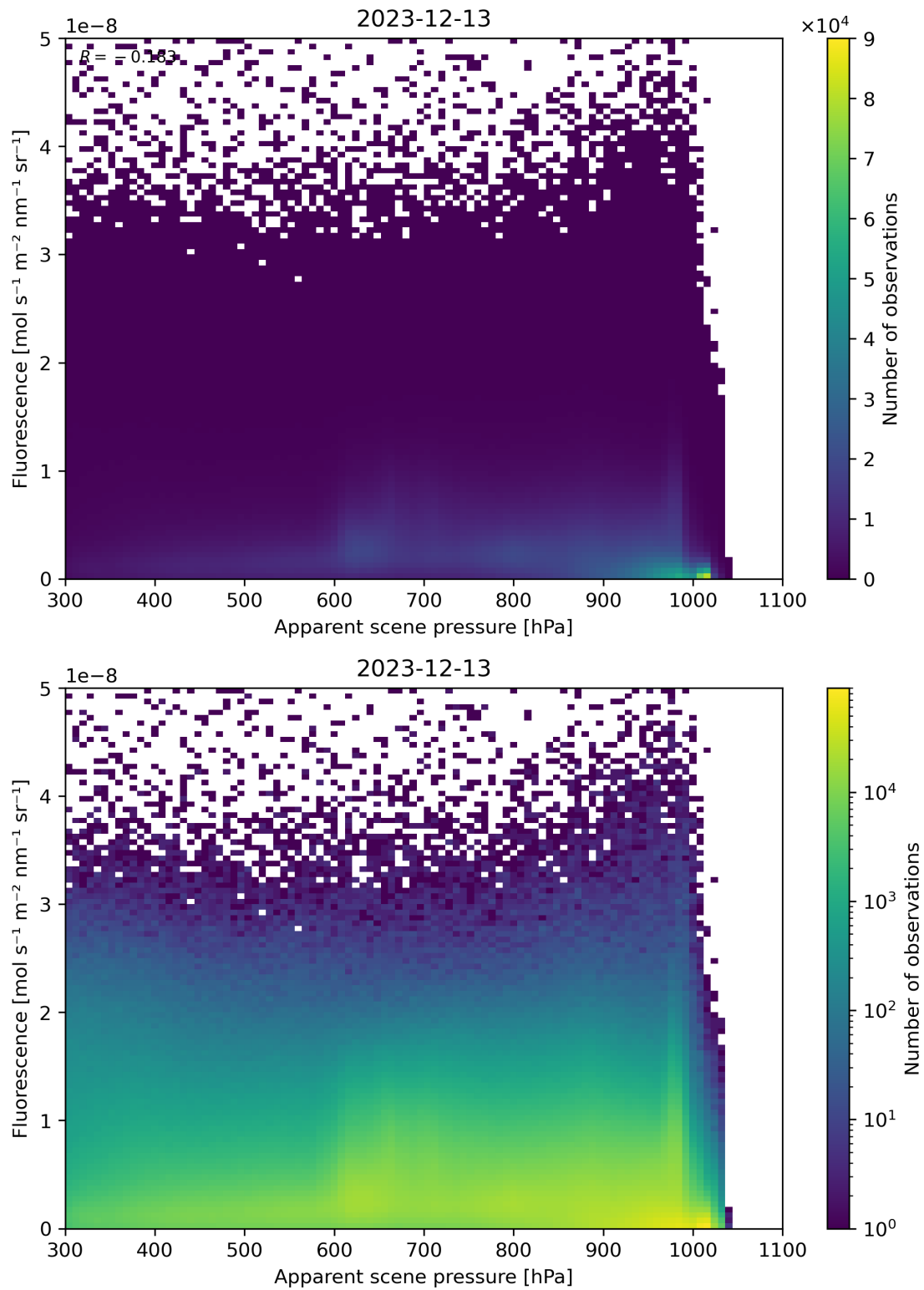
Figure 64: Scatter density plot of “Apparent scene pressure” against “Fluorescence” for 2023-12-12 to 2023-12-14.
