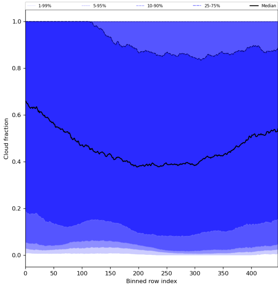
Figure 49: Along track statistics of “Cloud fraction” for 2023-12-12 to 2023-12-14
