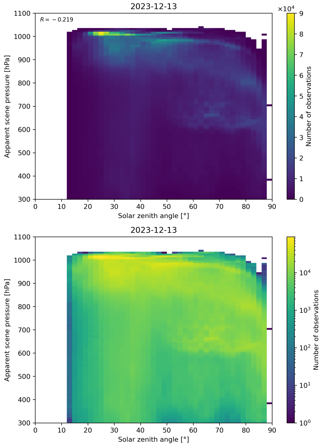
Figure 108: Scatter density plot of “Solar zenith angle” against “Apparent scene pressure” for 2023-12-12 to 2023-12-14.
