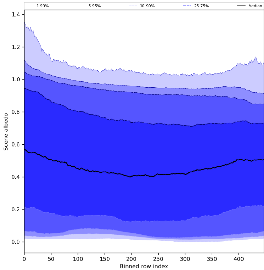
Figure 51: Along track statistics of “Scene albedo” for 2023-12-12 to 2023-12-14
