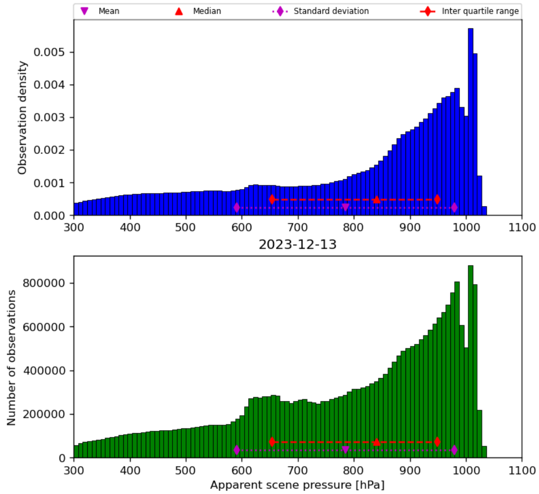
Figure 36: Histogram of “Apparent scene pressure” for 2023-12-12 to 2023-12-14
