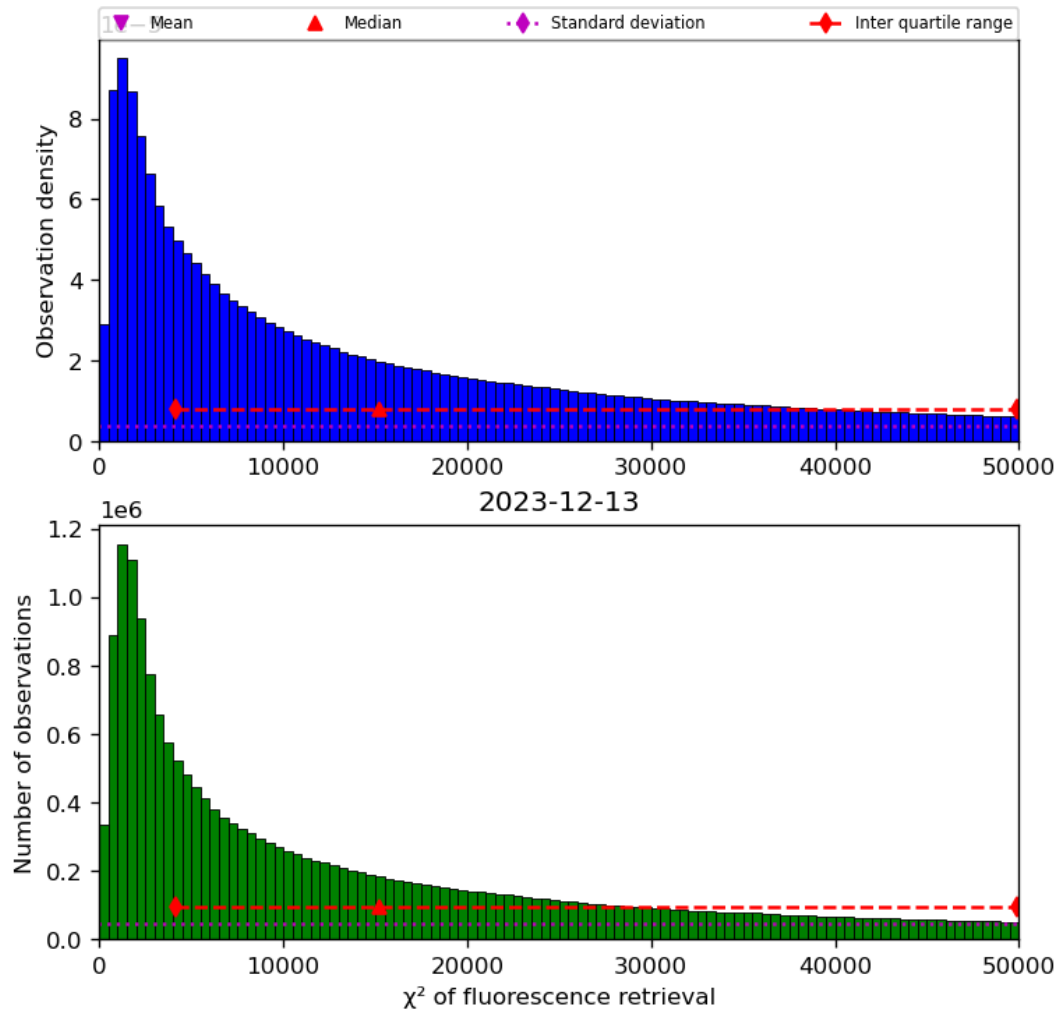
Figure 42: Histogram of “ \chi^2 of fluorescence retrieval” for 2023-12-12 to 2023-12-14
