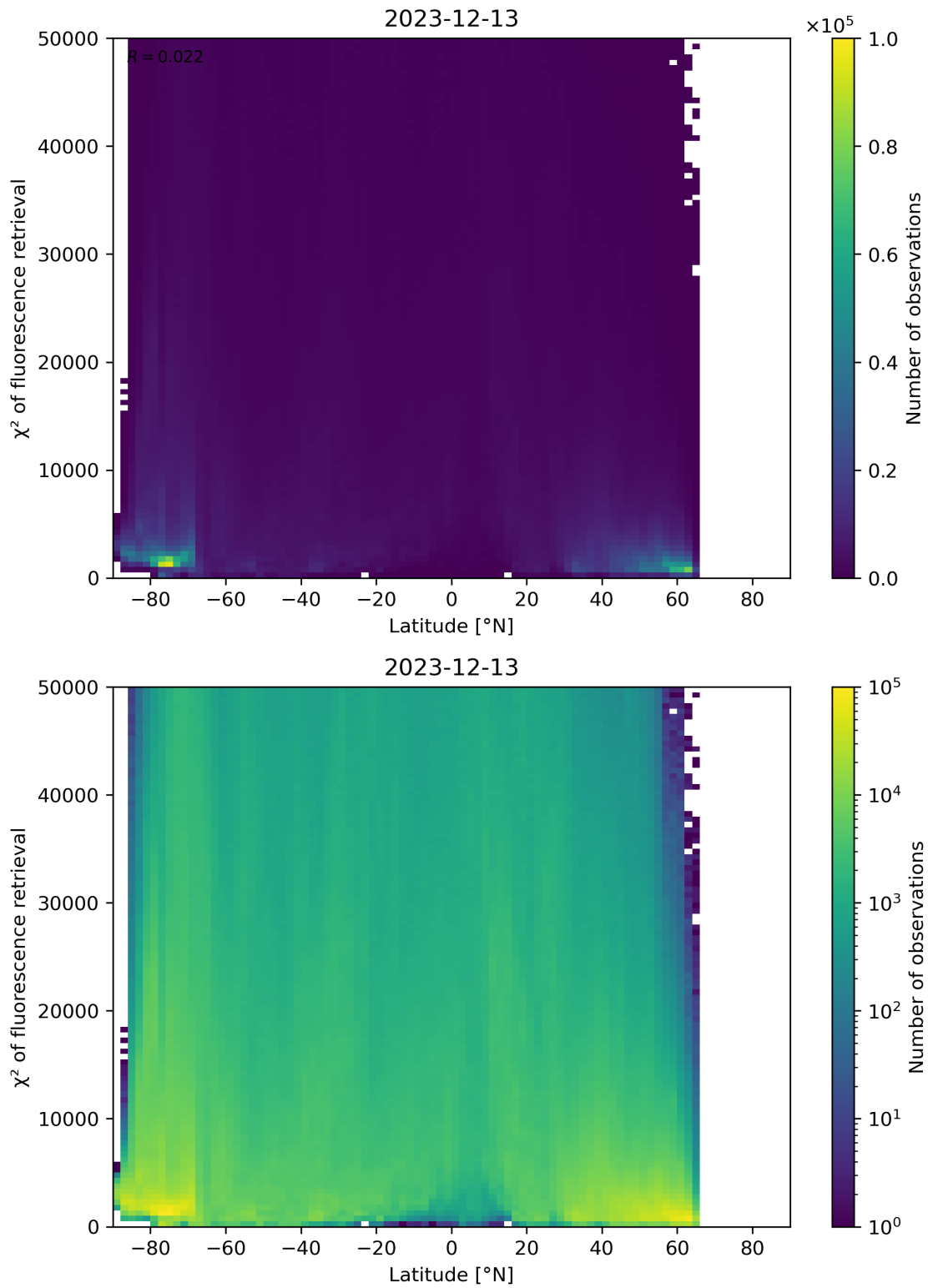
Figure 89: Scatter density plot of “Latitude” against “ \chi^2 of fluorescence retrieval” for 2023-12-12 to 2023-12-14.
