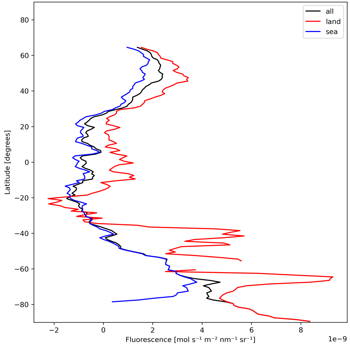
Figure 23: Zonal average of “Fluorescence” for 2023-12-12 to 2023-12-14.
