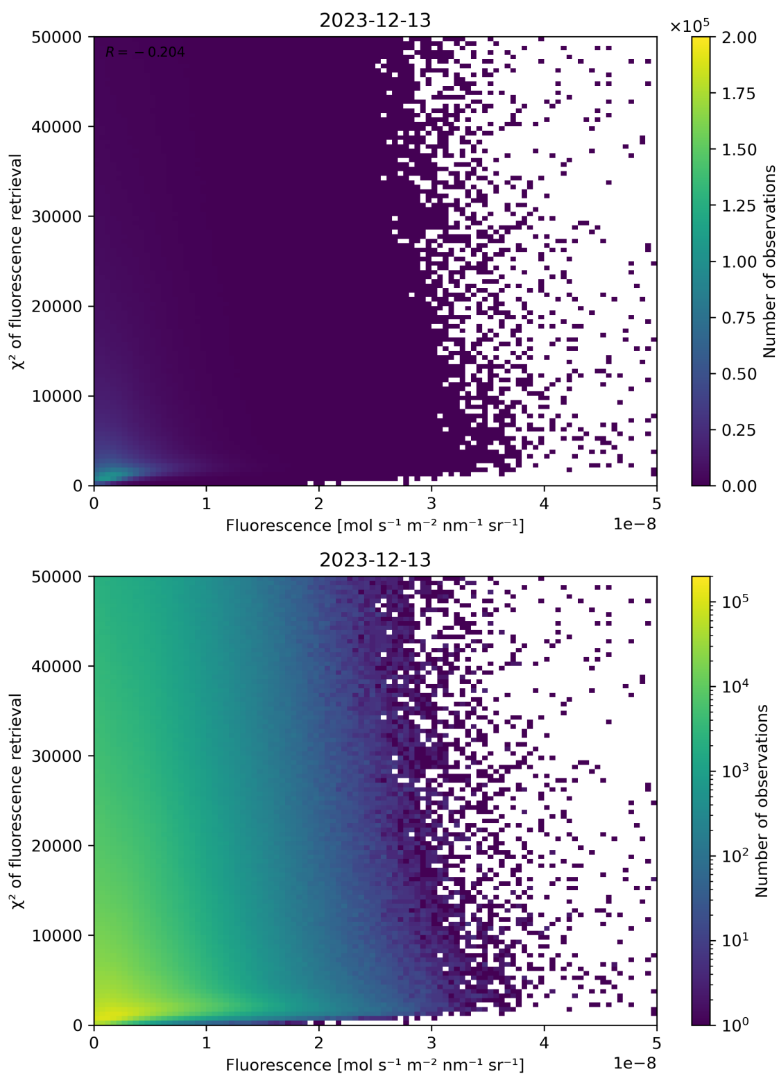
Figure 85: Scatter density plot of “Fluorescence” against “ \chi^2 of fluorescence retrieval” for 2023-12-12 to 2023-12-14.
