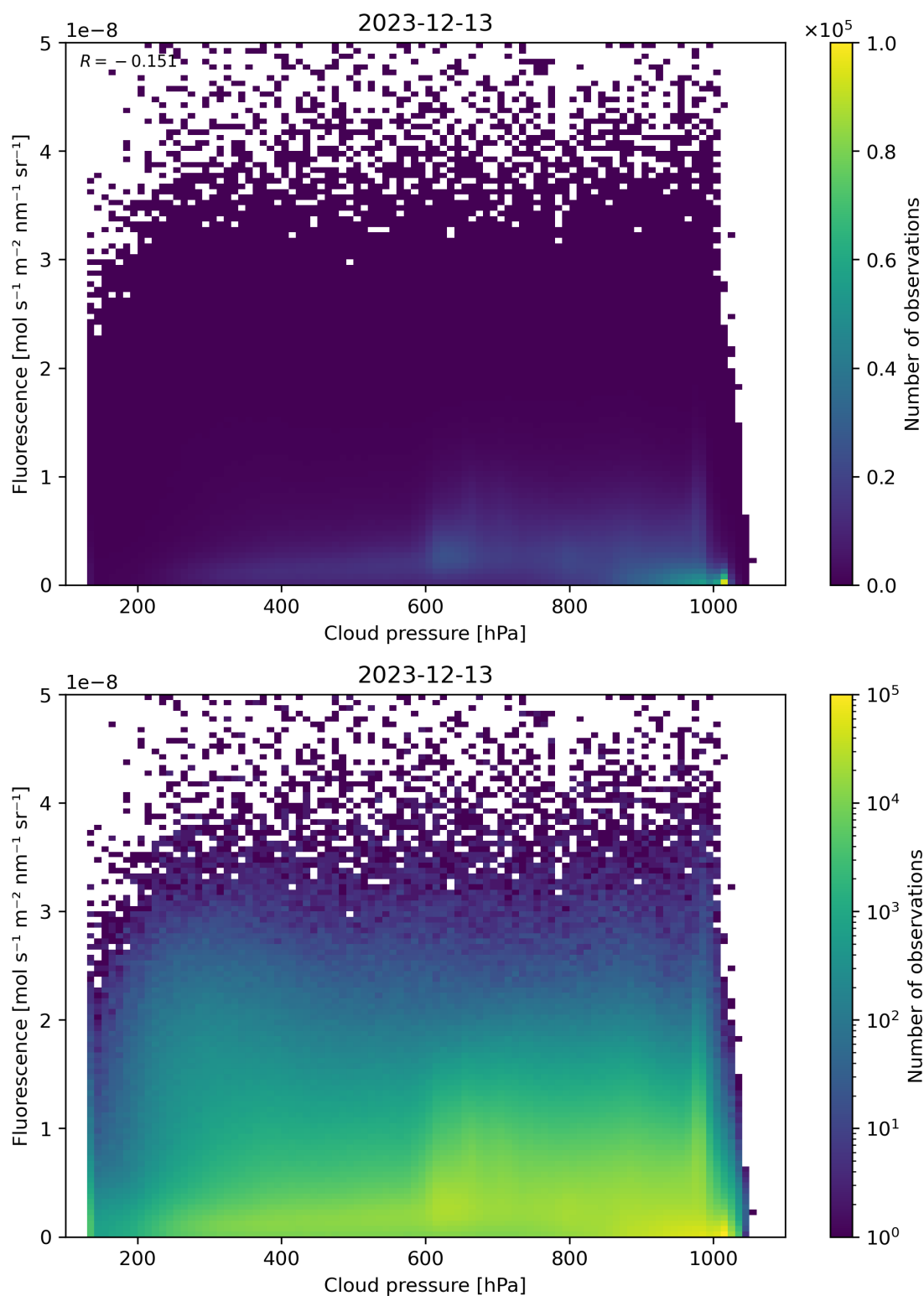
Figure 80: Scatter density plot of “Cloud pressure” against “Fluorescence” for 2023-12-12 to 2023-12-14.
