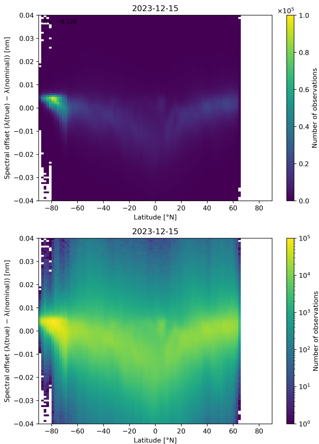
Figure 96: Scatter density plot of “Latitude” against “Spectral offset ( \lambda(\text{true}) - \lambda(\text{nominal}) )” for 2023-12-14 to 2023-12-16.
