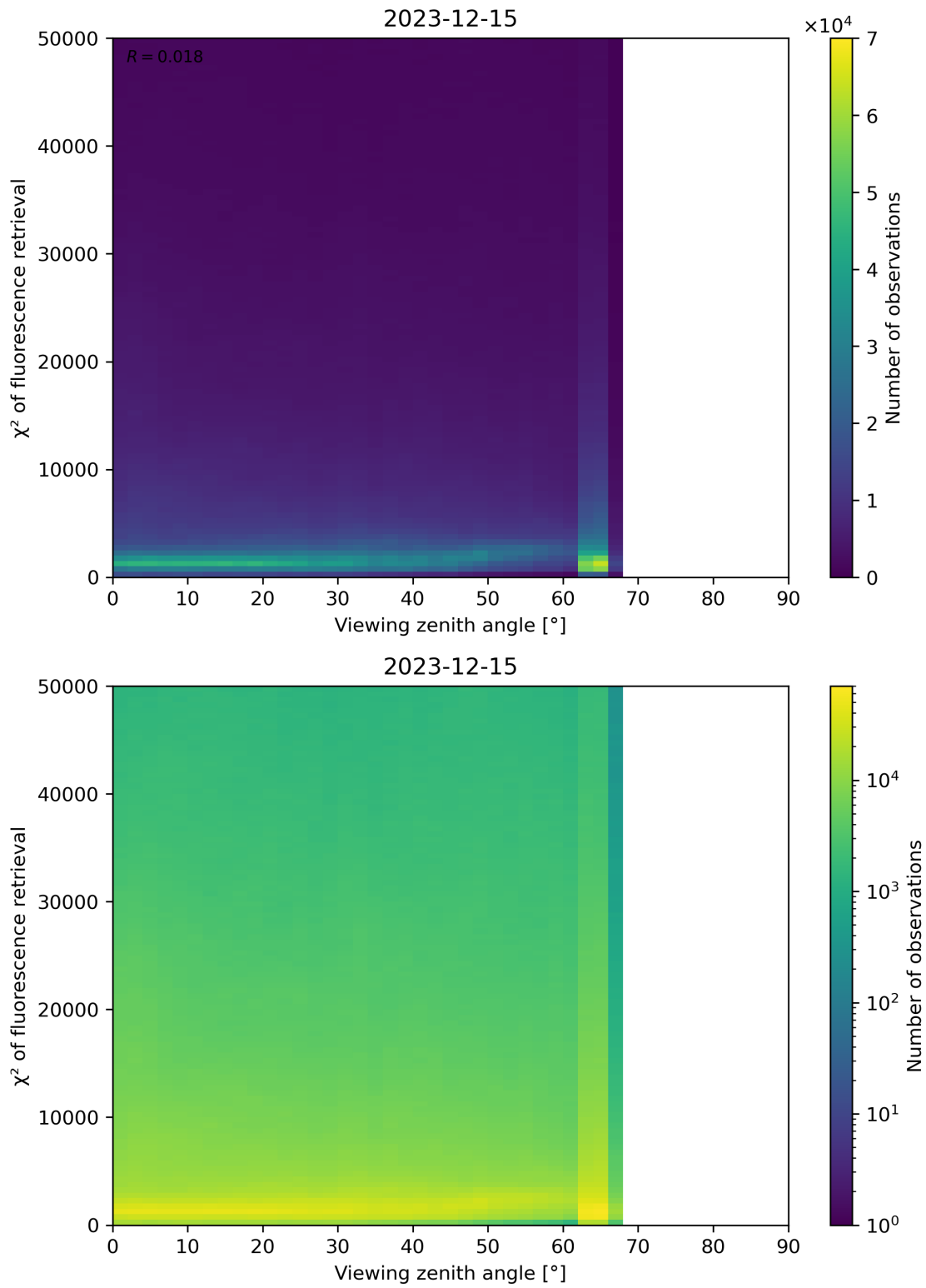
Figure 119: Scatter density plot of “Viewing zenith angle” against “ \chi^2 of fluorescence retrieval” for 2023-12-14 to 2023-12-16.
