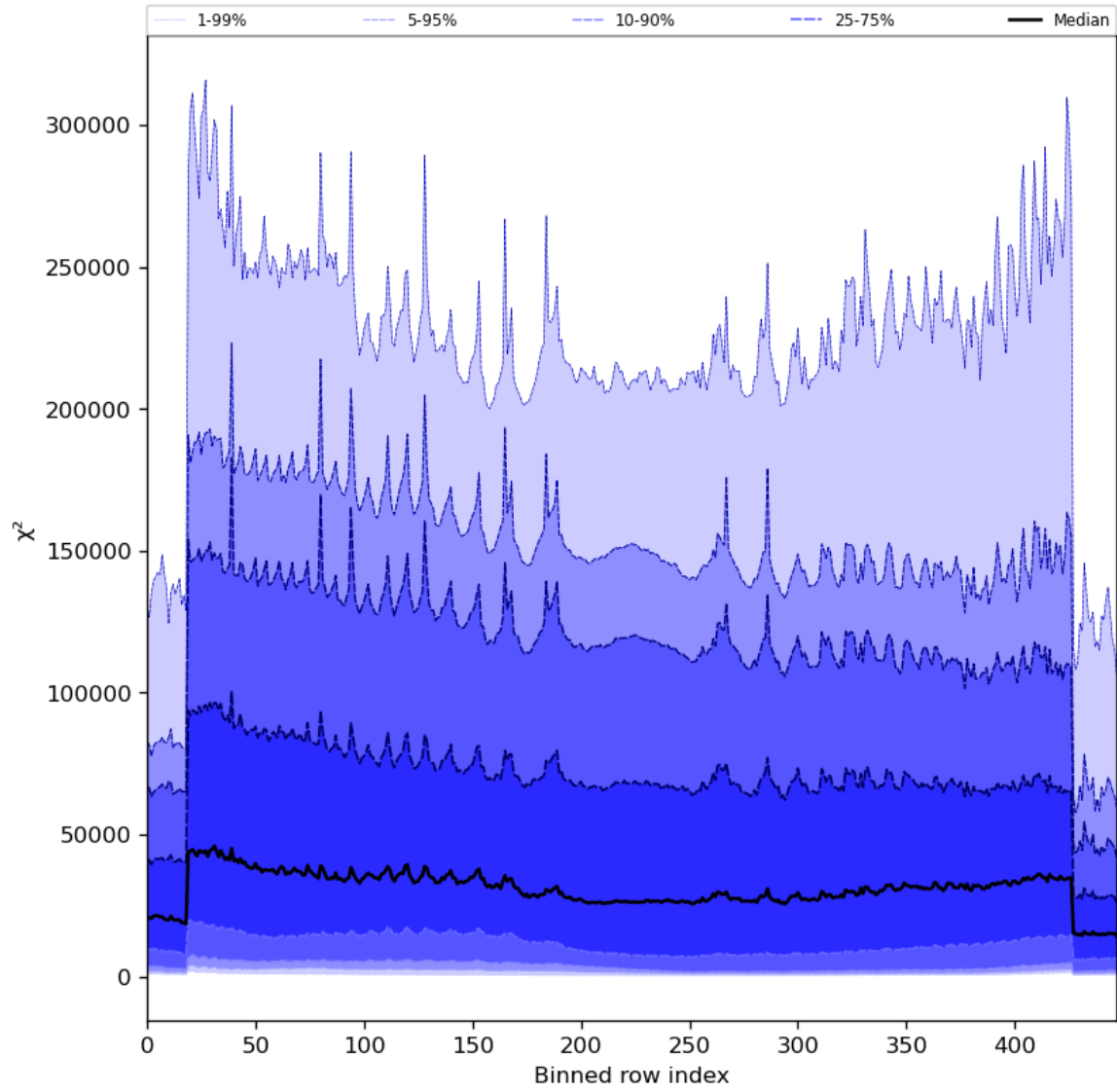
Figure 55: Along track statistics of “ \chi^2 ” for 2023-12-14 to 2023-12-16
