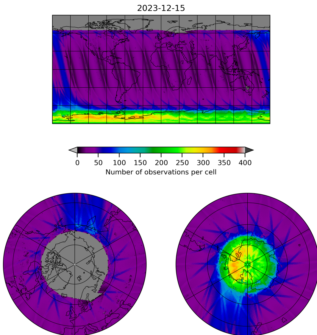
Figure 11: Map of the number of observations for 2023-12-14 to 2023-12-16
