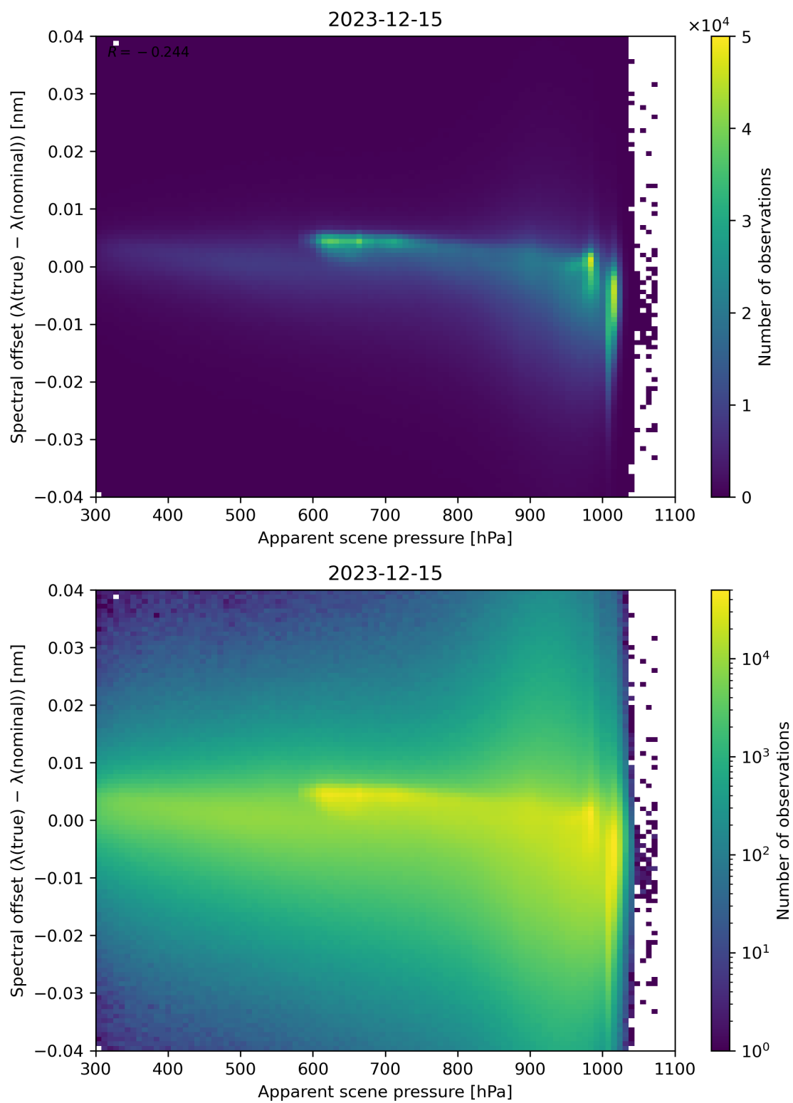
Figure 67: Scatter density plot of “Apparent scene pressure” against “Spectral offset ( \lambda(\text{true}) - \lambda(\text{nominal}) )” for 2023-12-14 to 2023-12-16.
