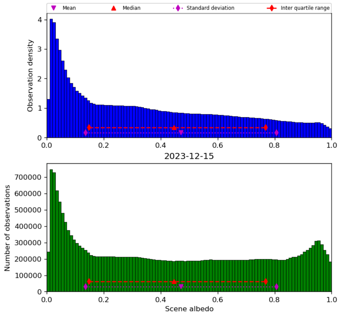
Figure 34: Histogram of “Scene albedo” for 2023-12-14 to 2023-12-16
