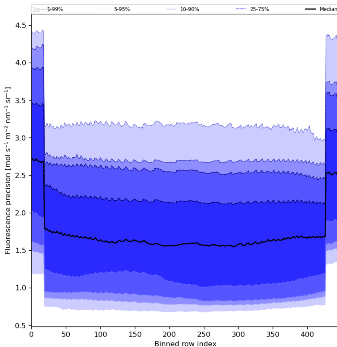
Figure 58: Along track statistics of “Fluorescence precision” for 2023-12-14 to 2023-12-16
