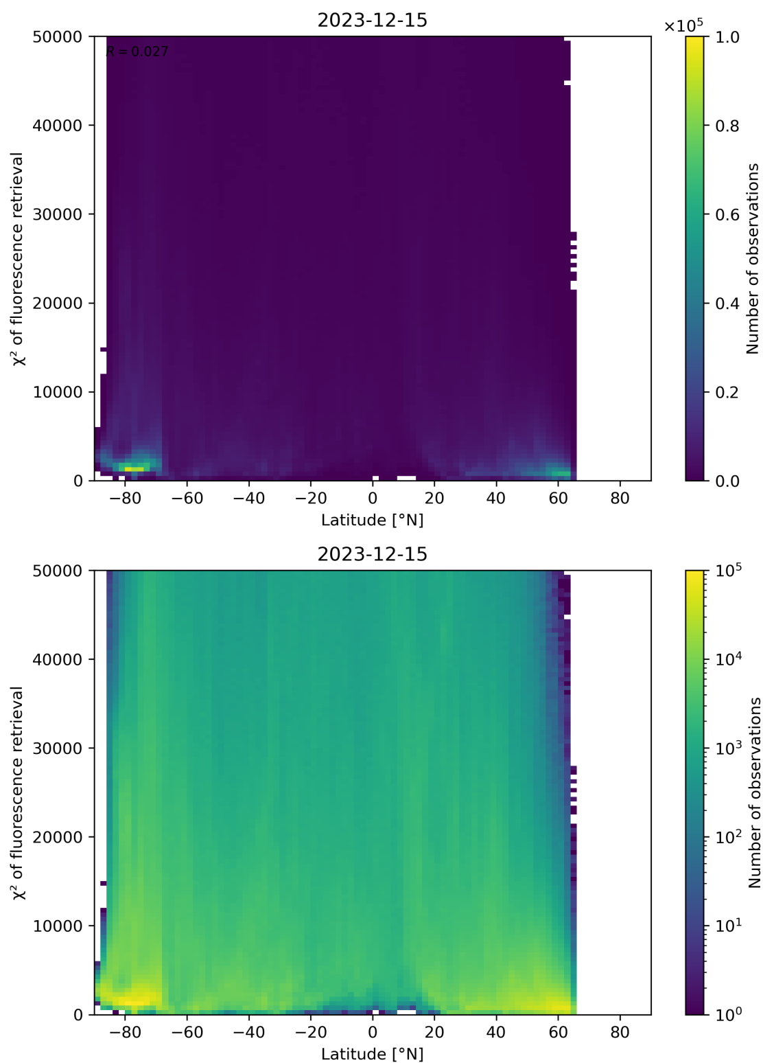
Figure 89: Scatter density plot of “Latitude” against “ \chi^2 of fluorescence retrieval” for 2023-12-14 to 2023-12-16.
