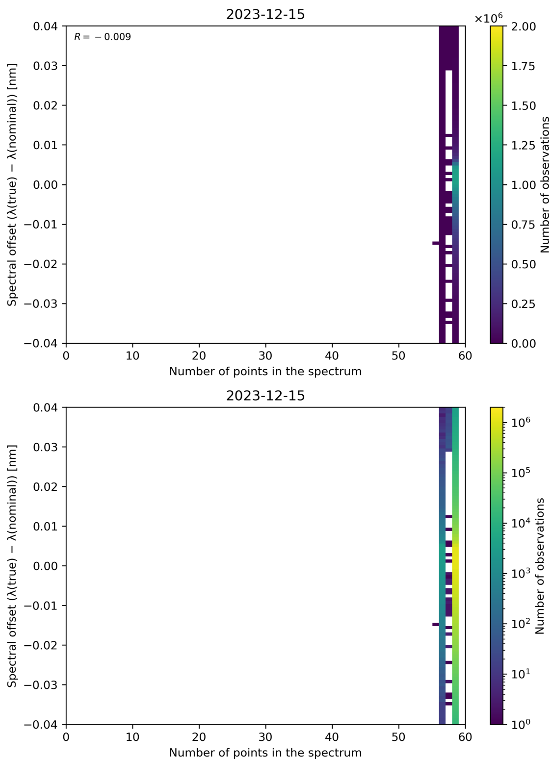
Figure 101: Scatter density plot of “Number of points in the spectrum” against “Spectral offset ( \lambda(\text{true}) - \lambda(\text{nominal}) )” for 2023-12-14 to 2023-12-16.
