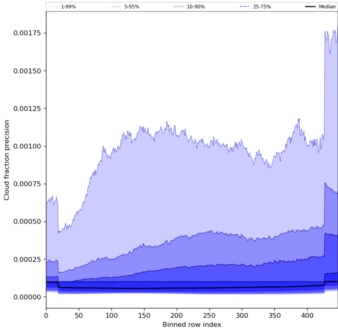
Figure 50: Along track statistics of “Cloud fraction precision” for 2023-12-14 to 2023-12-16
