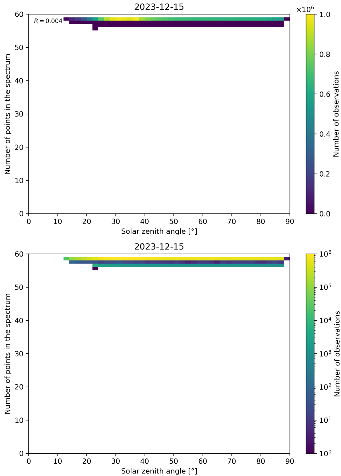
Figure 115: Scatter density plot of “Solar zenith angle” against “Number of points in the spectrum” for 2023-12-14 to 2023-12-16.
