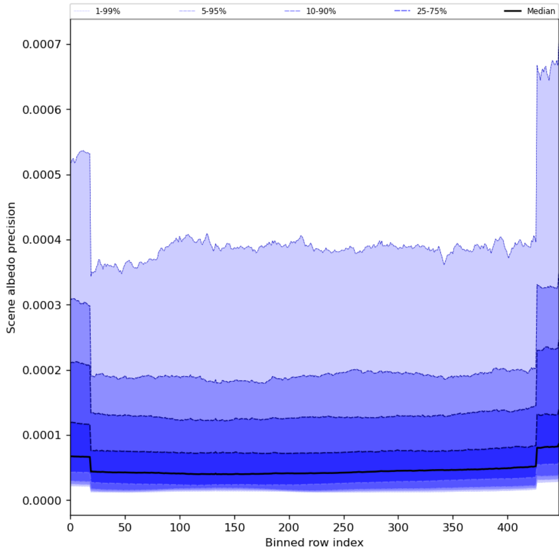
Figure 52: Along track statistics of “Scene albedo precision” for 2023-12-14 to 2023-12-16
