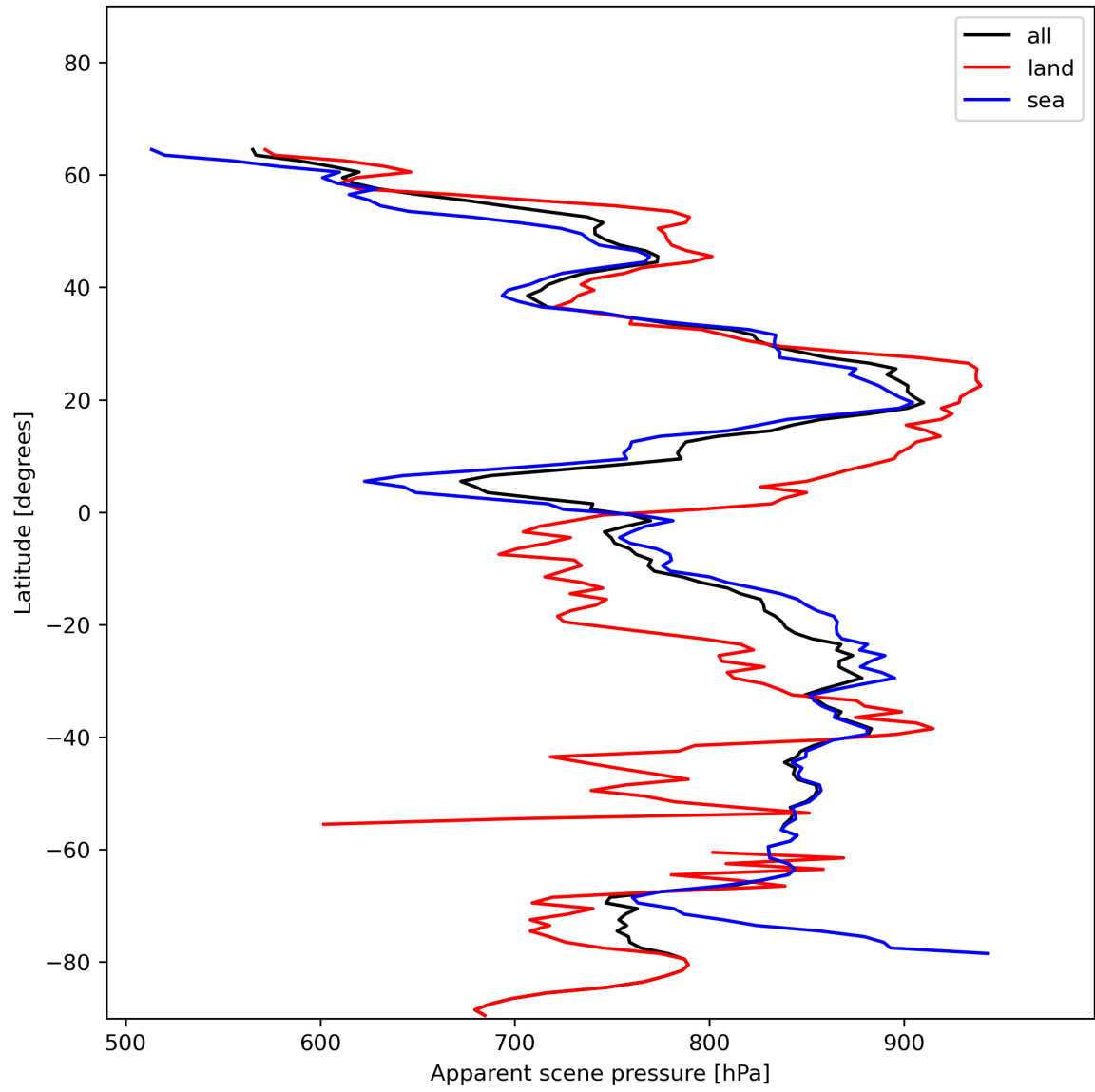
Figure 19: Zonal average of “Apparent scene pressure” for 2023-12-14 to 2023-12-16.
