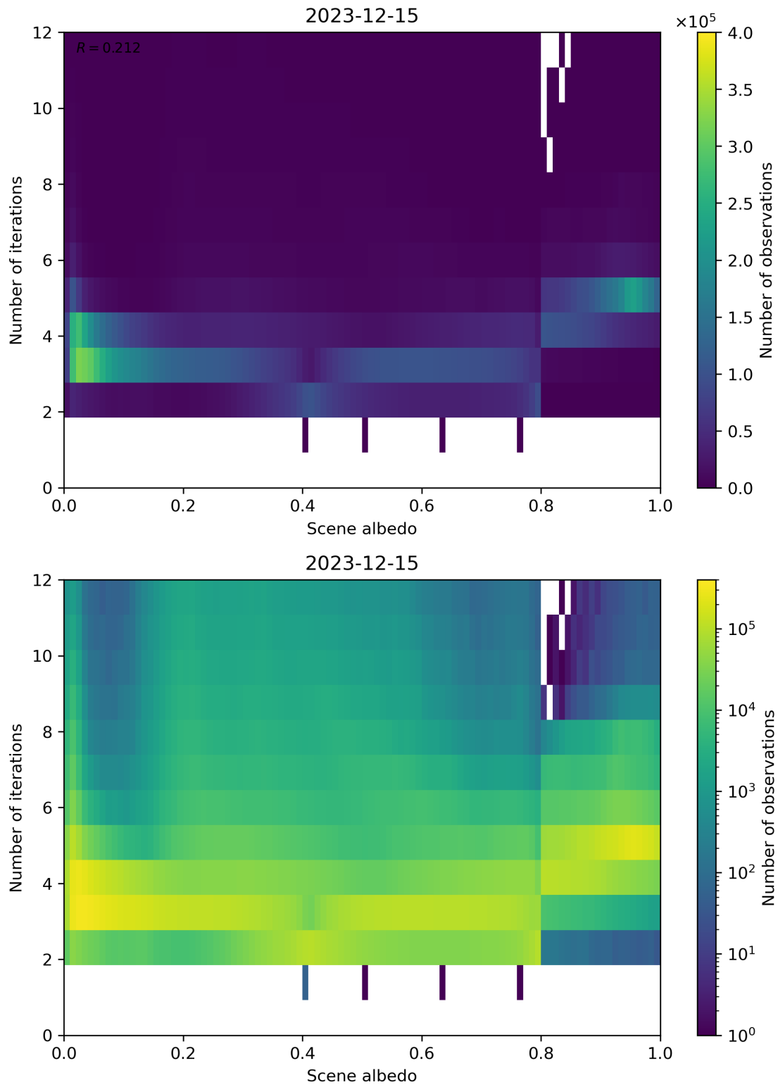
Figure 105: Scatter density plot of “Scene albedo” against “Number of iterations” for 2023-12-14 to 2023-12-16.
