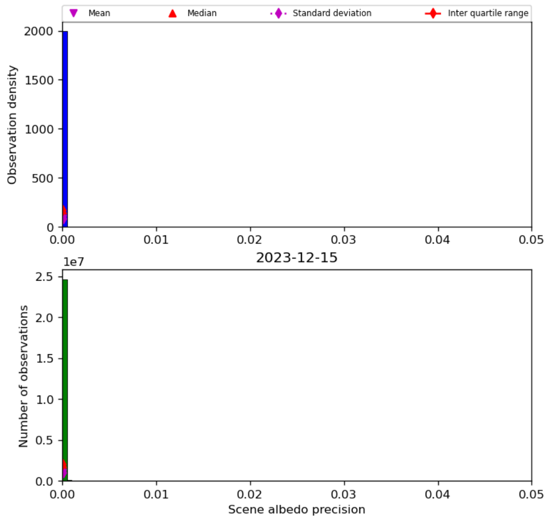
Figure 35: Histogram of “Scene albedo precision” for 2023-12-14 to 2023-12-16
