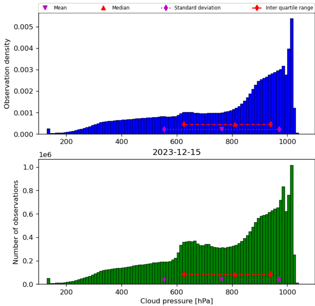
Figure 30: Histogram of “Cloud pressure” for 2023-12-14 to 2023-12-16
