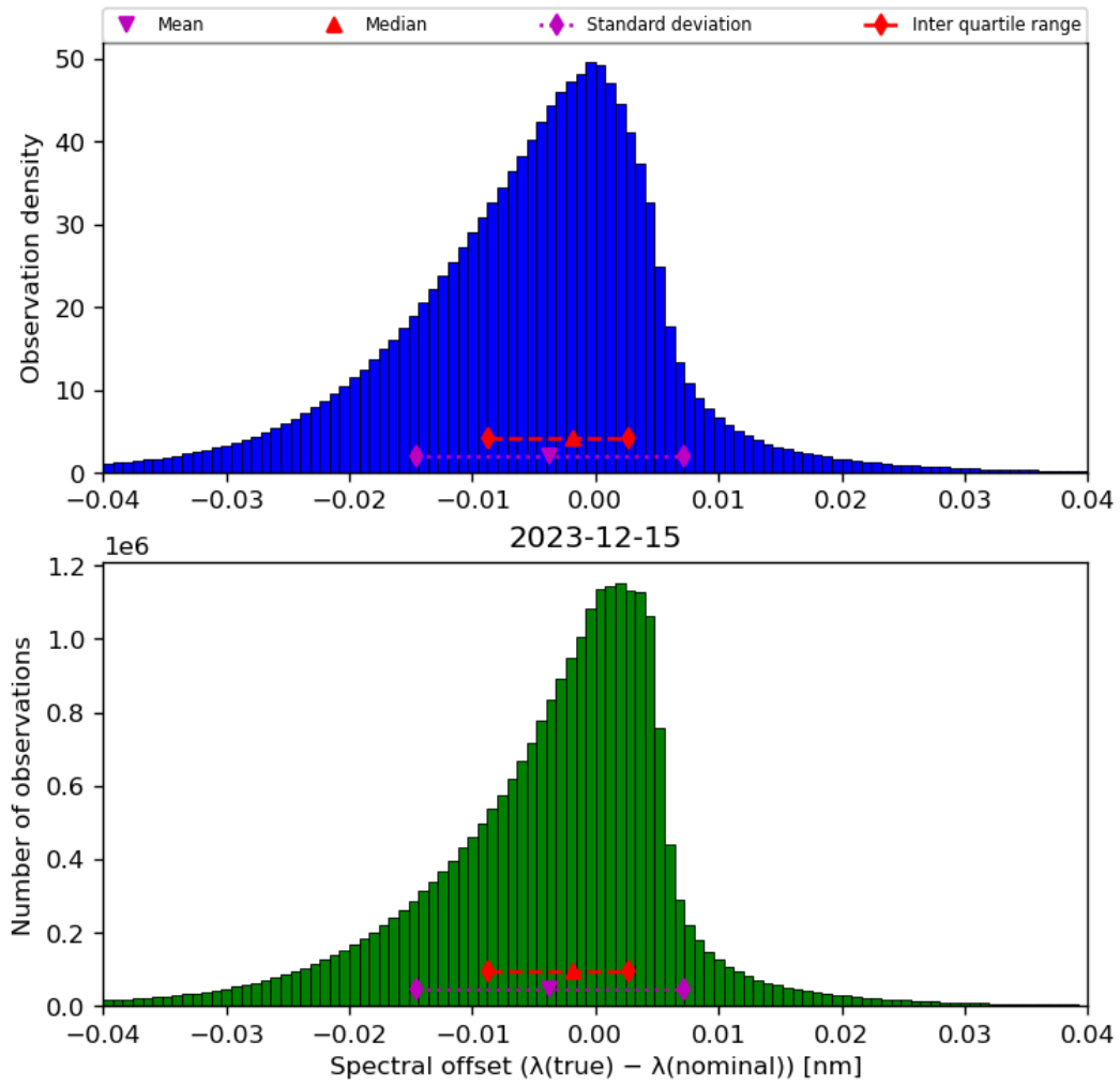
Figure 45: Histogram of “Spectral offset ( \lambda(\text{true}) - \lambda(\text{nominal}) )” for 2023-12-14 to 2023-12-16
