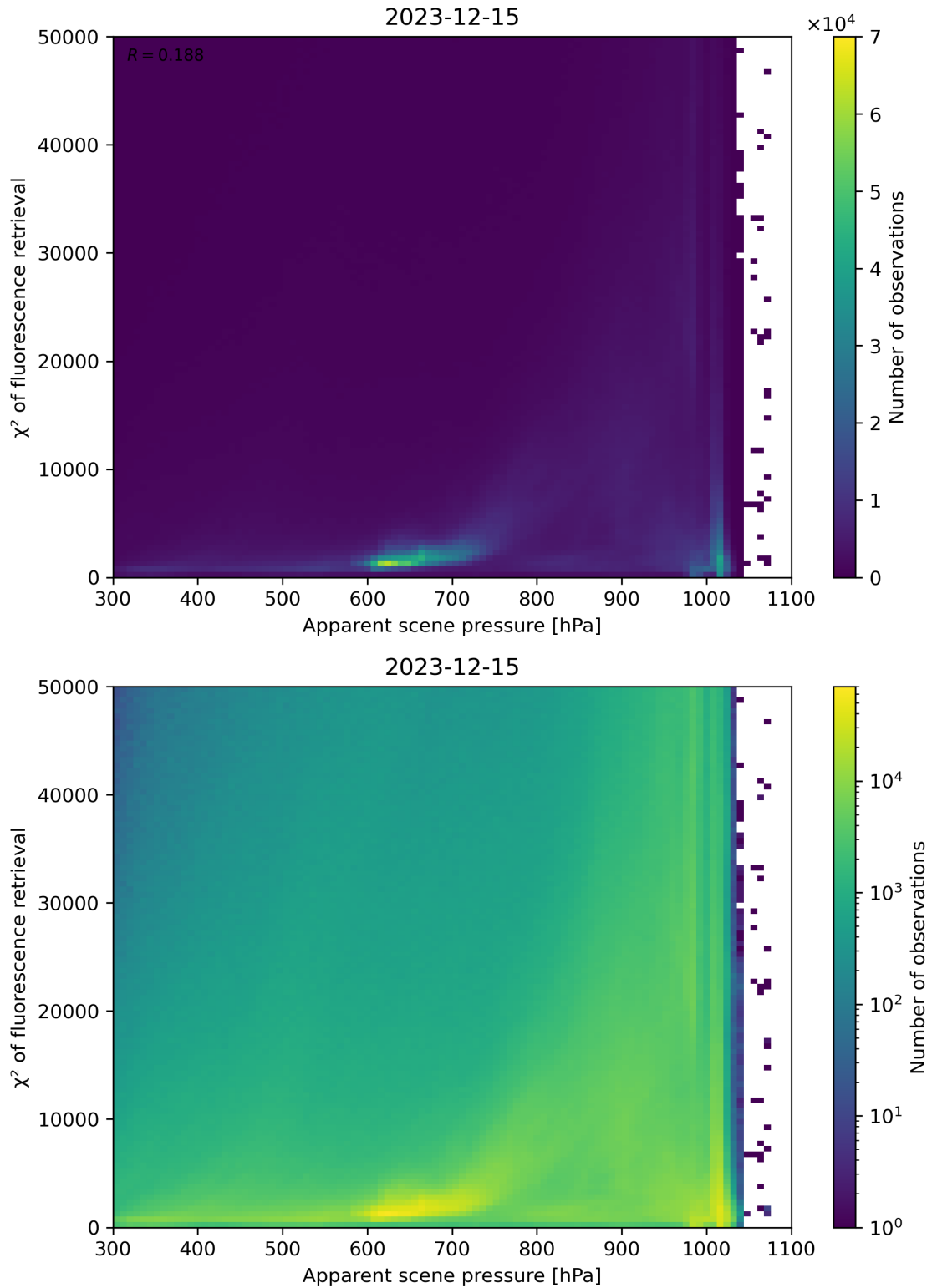
Figure 63: Scatter density plot of “Apparent scene pressure” against “ \chi^2 of fluorescence retrieval” for 2023-12-14 to 2023-12-16.
