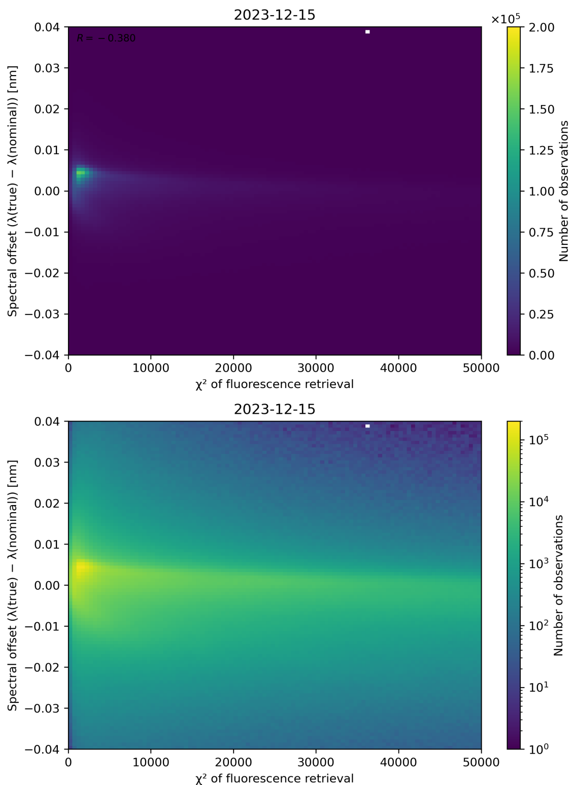
Figure 69: Scatter density plot of " \chi^2 of fluorescence retrieval" against "Spectral offset ( \lambda(\text{true}) - \lambda(\text{nominal})) " for 2023-12-14 to 2023-12-16.
