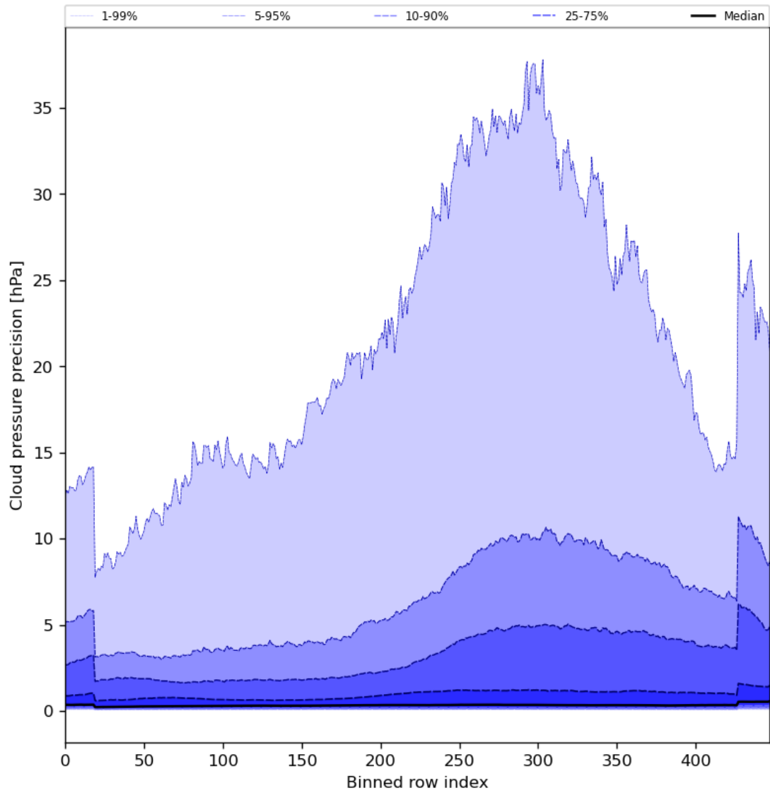
Figure 48: Along track statistics of “Cloud pressure precision” for 2023-12-14 to 2023-12-16
