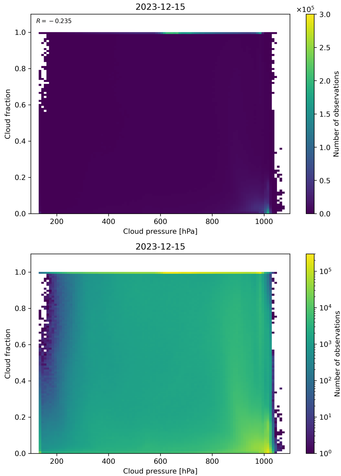
Figure 79: Scatter density plot of “Cloud pressure” against “Cloud fraction” for 2023-12-14 to 2023-12-16.
