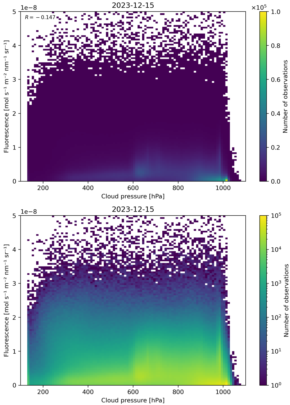
Figure 80: Scatter density plot of “Cloud pressure” against “Fluorescence” for 2023-12-14 to 2023-12-16.
