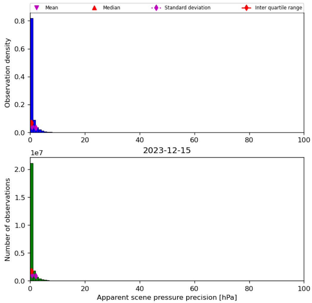
Figure 37: Histogram of “Apparent scene pressure precision” for 2023-12-14 to 2023-12-16
