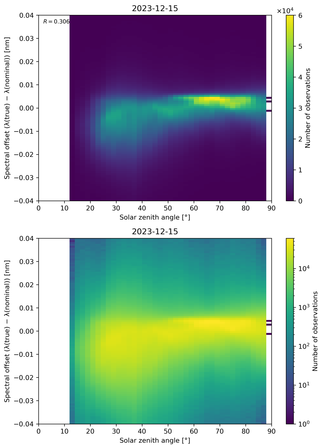
Figure 117: Scatter density plot of “Solar zenith angle” against “Spectral offset ( \lambda(\text{true}) - \lambda(\text{nominal}) )” for 2023-12-14 to 2023-12-16.
