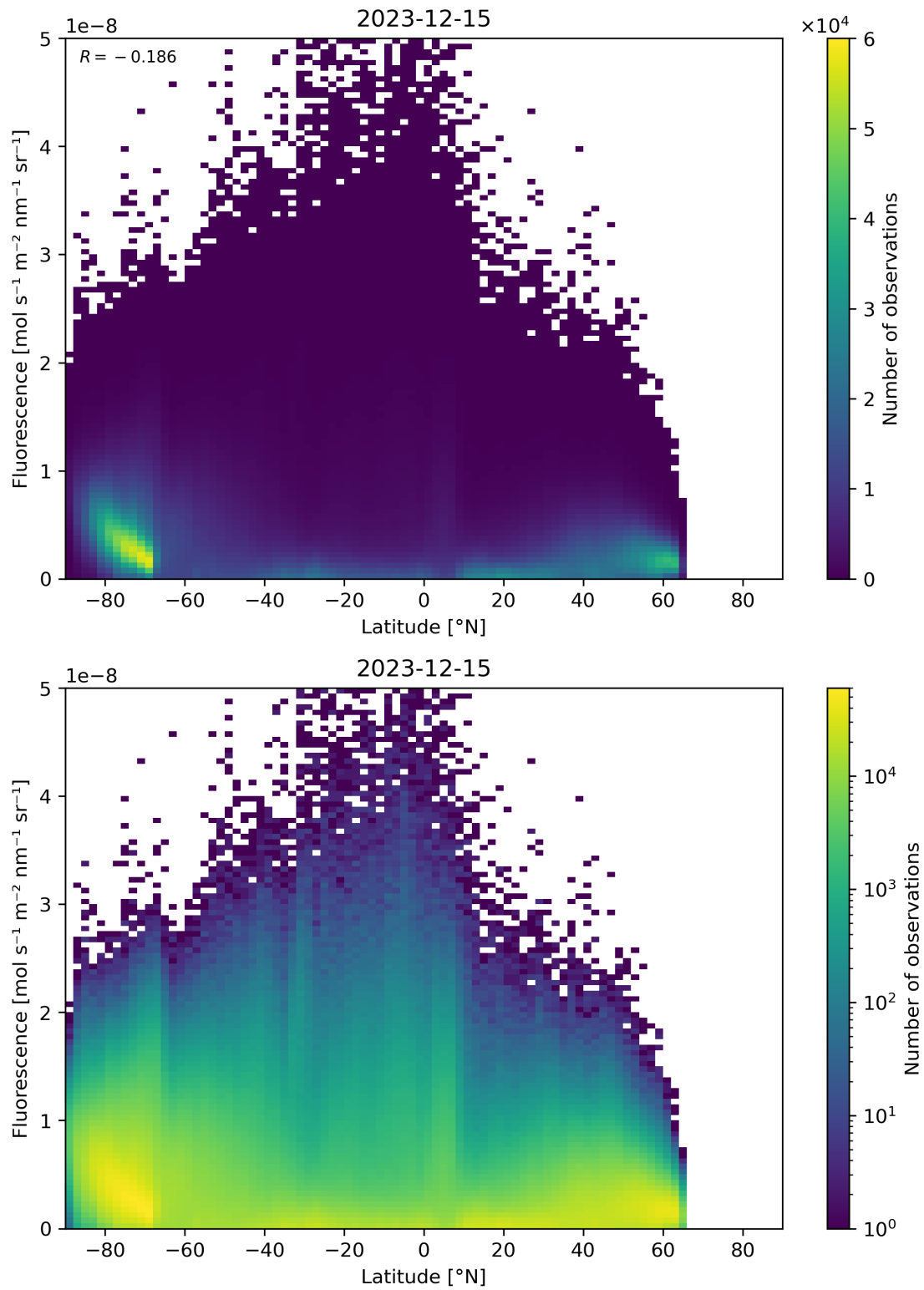
Figure 92: Scatter density plot of “Latitude” against “Fluorescence” for 2023-12-14 to 2023-12-16.
