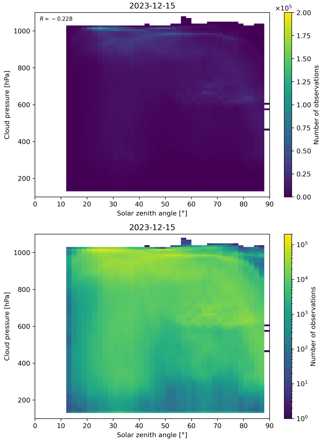
Figure 111: Scatter density plot of “Solar zenith angle” against “Cloud pressure” for 2023-12-14 to 2023-12-16.
