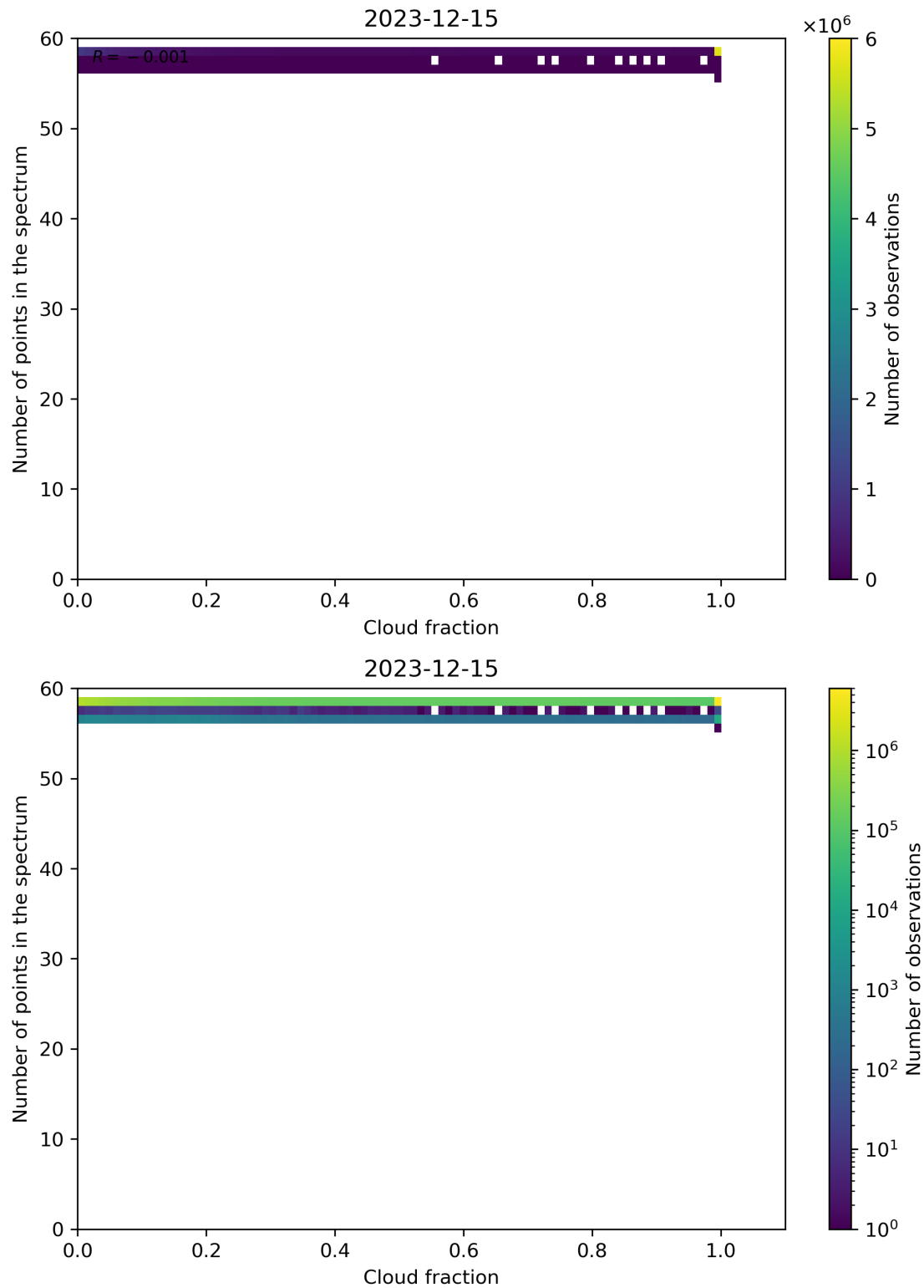
Figure 74: Scatter density plot of “Cloud fraction” against “Number of points in the spectrum” for 2023-12-14 to 2023-12-16.
