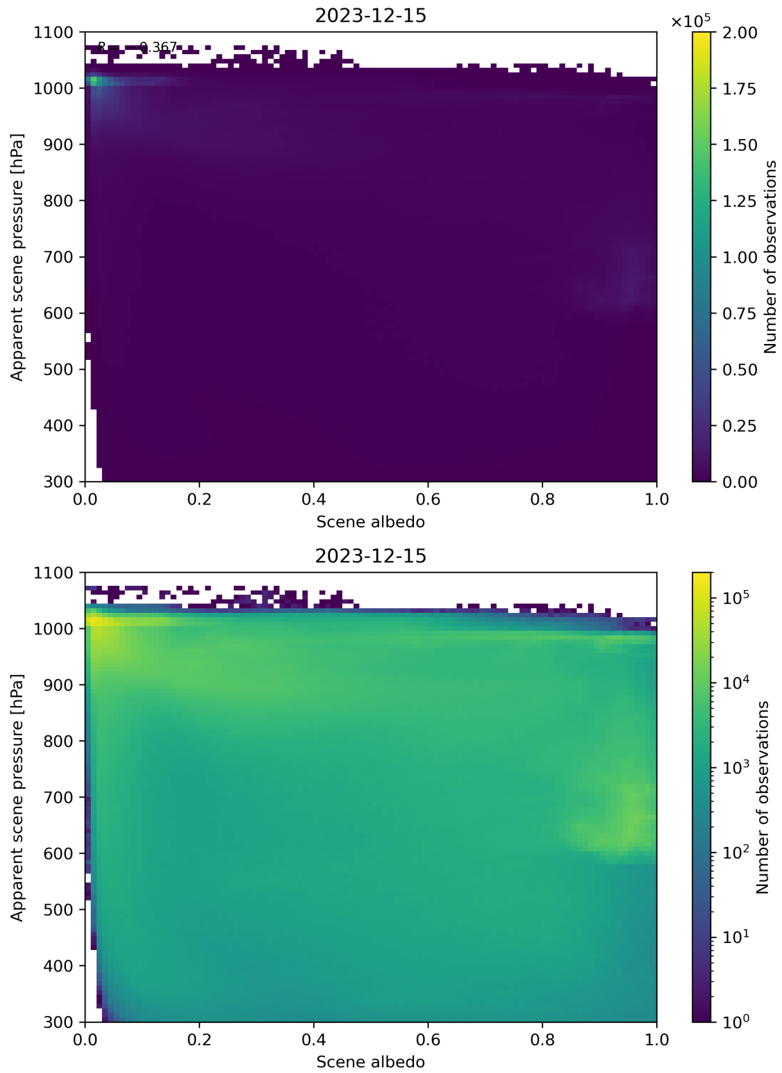
Figure 102: Scatter density plot of “Scene albedo” against “Apparent scene pressure” for 2023-12-14 to 2023-12-16.
