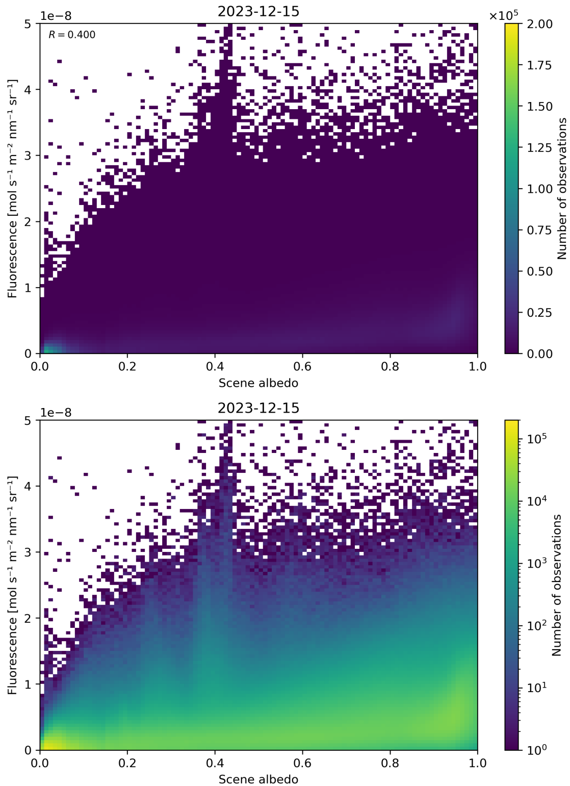
Figure 104: Scatter density plot of “Scene albedo” against “Fluorescence” for 2023-12-14 to 2023-12-16.
