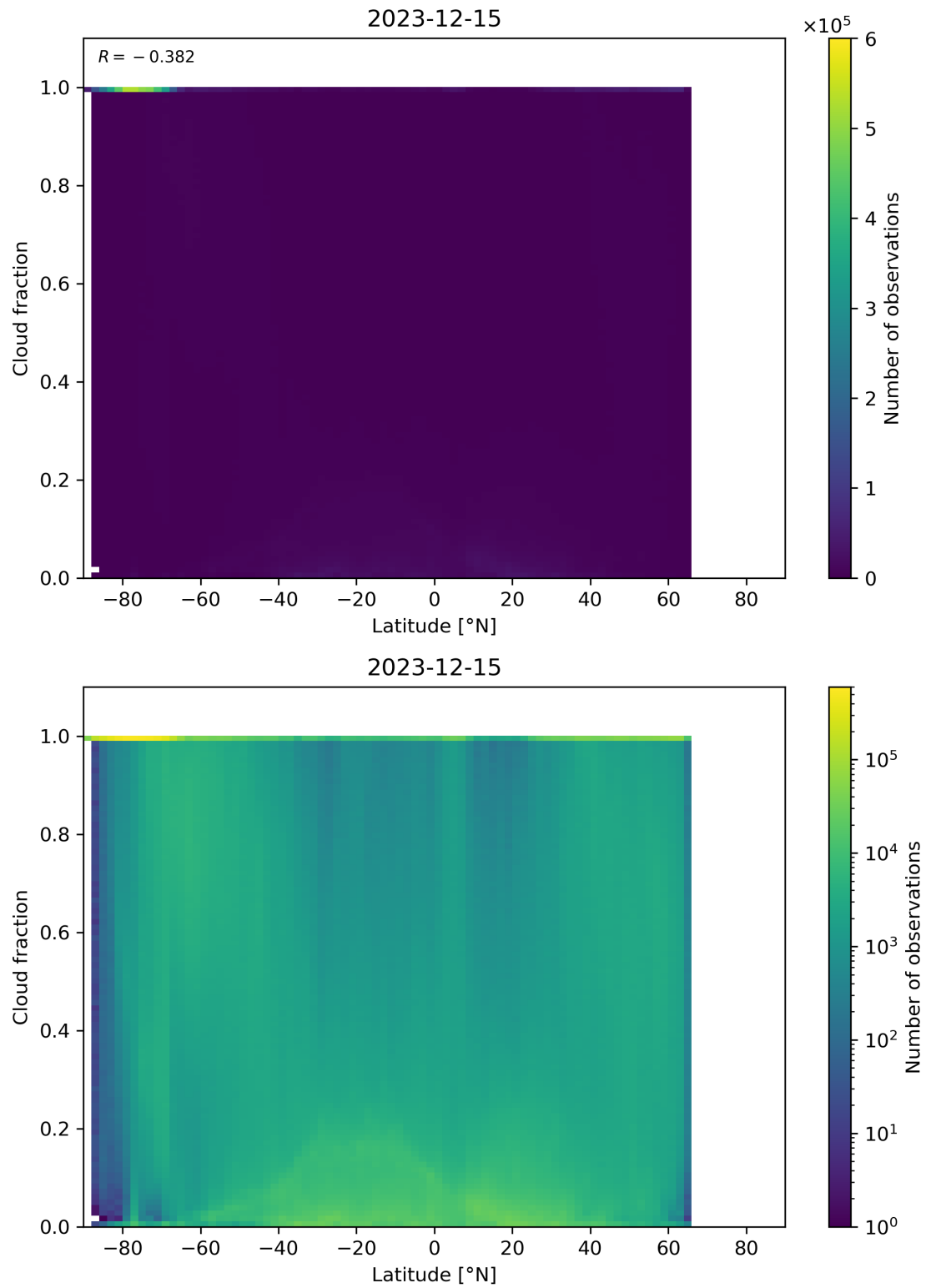
Figure 90: Scatter density plot of “Latitude” against “Cloud fraction” for 2023-12-14 to 2023-12-16.
