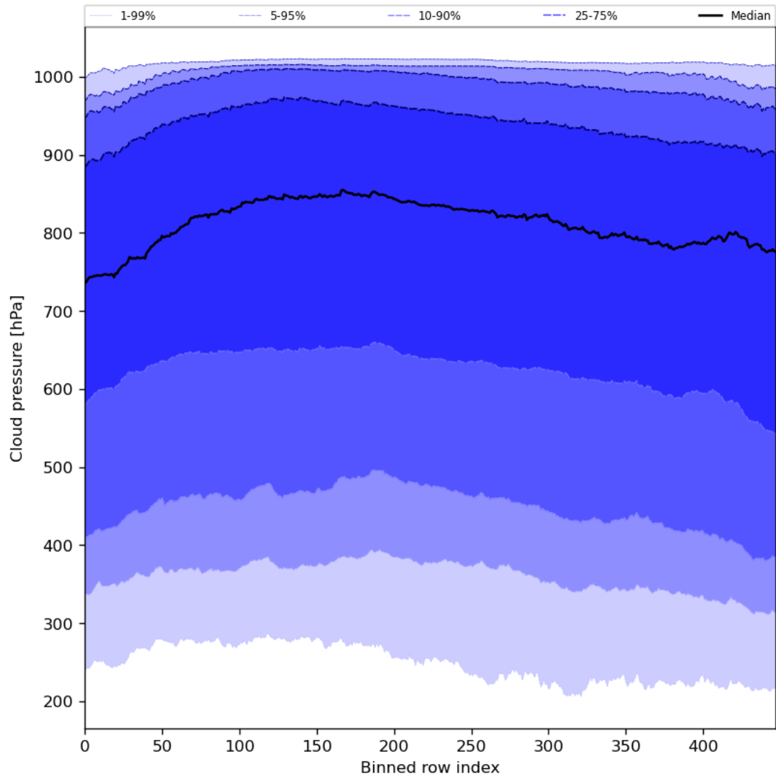
Figure 47: Along track statistics of “Cloud pressure” for 2023-12-14 to 2023-12-16
