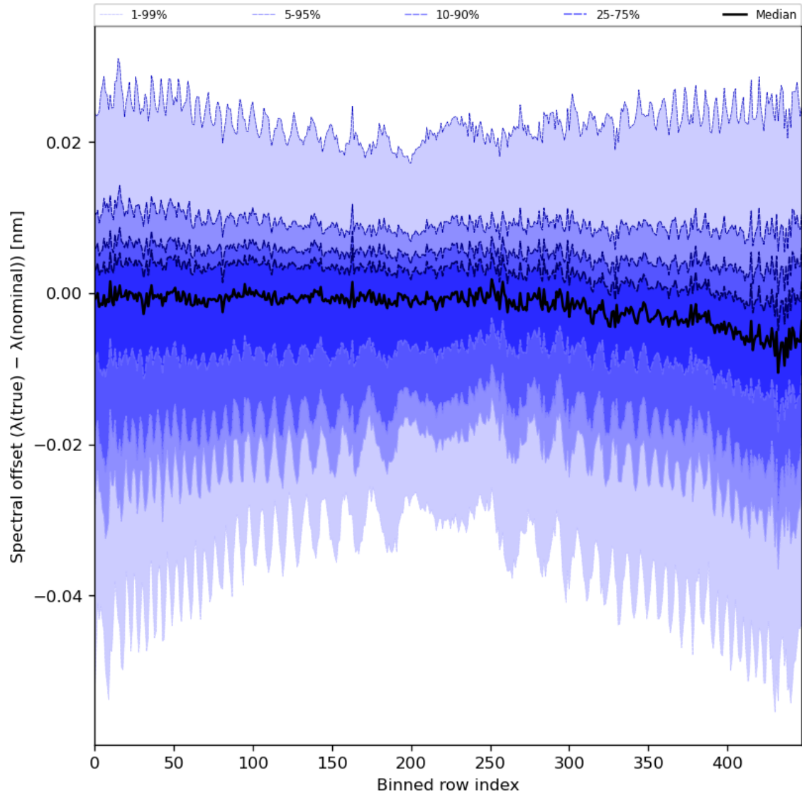
Figure 62: Along track statistics of “Spectral offset ( \lambda(\text{true}) - \lambda(\text{nominal}) )” for 2023-12-14 to 2023-12-16
