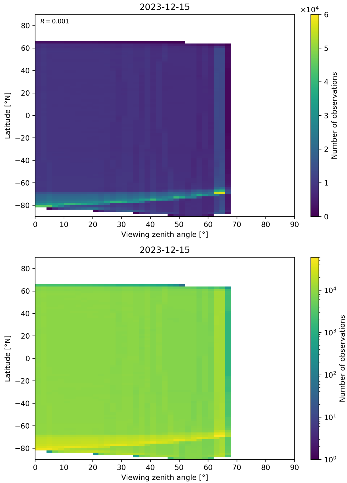
Figure 123: Scatter density plot of “Viewing zenith angle” against “Latitude” for 2023-12-14 to 2023-12-16.
