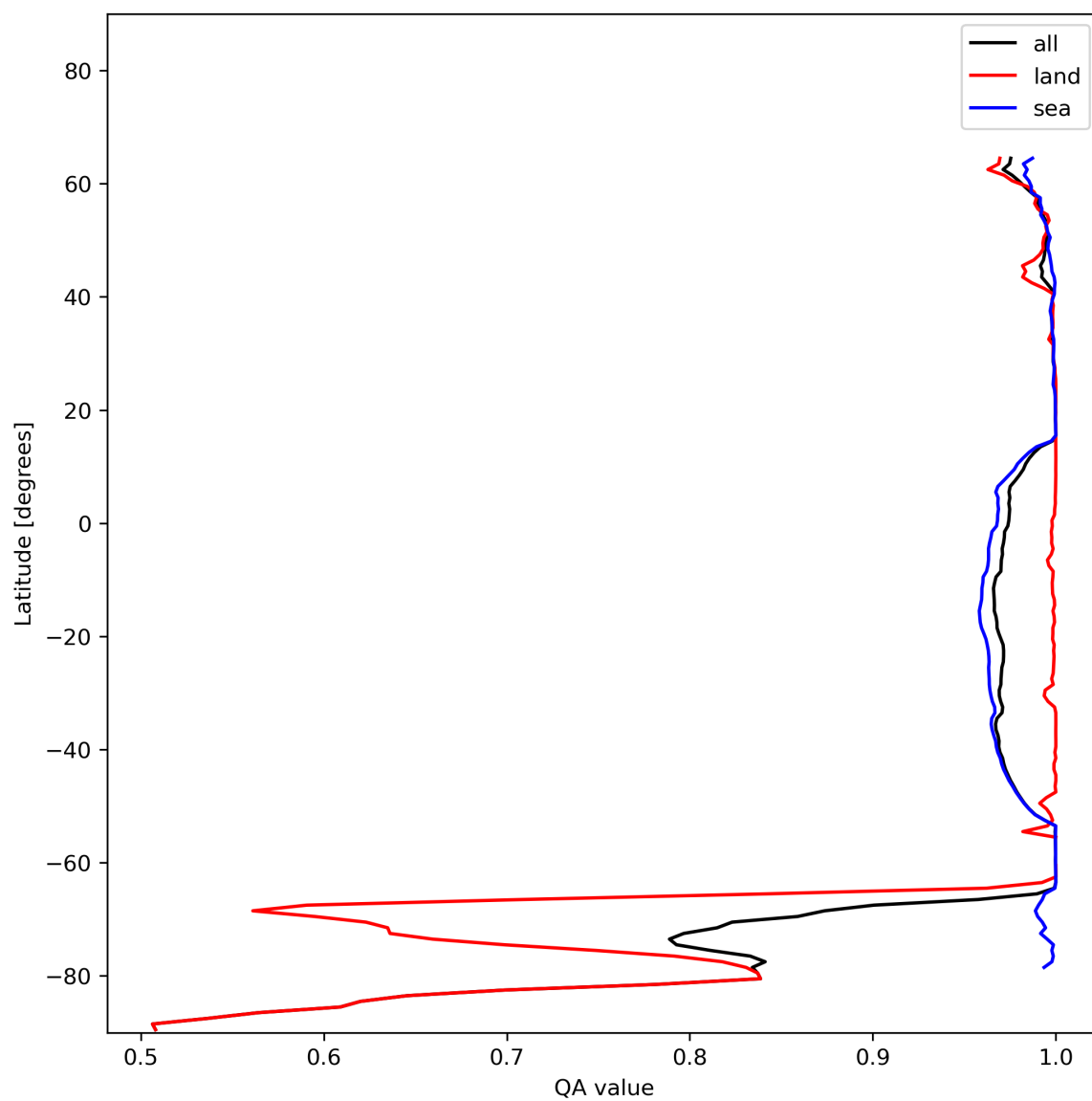
Figure 12: Zonal average of “QA value” for 2023-12-14 to 2023-12-16.
