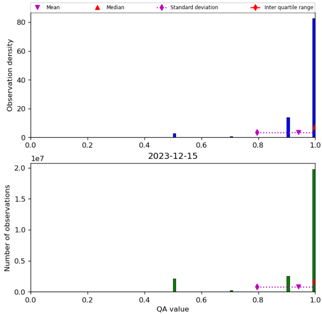
Figure 29: Histogram of “QA value” for 2023-12-14 to 2023-12-16
