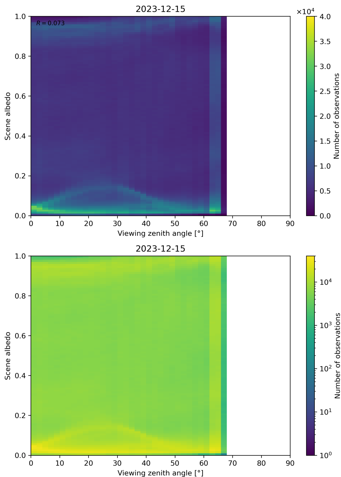
Figure 126: Scatter density plot of “Viewing zenith angle” against “Scene albedo” for 2023-12-14 to 2023-12-16.
