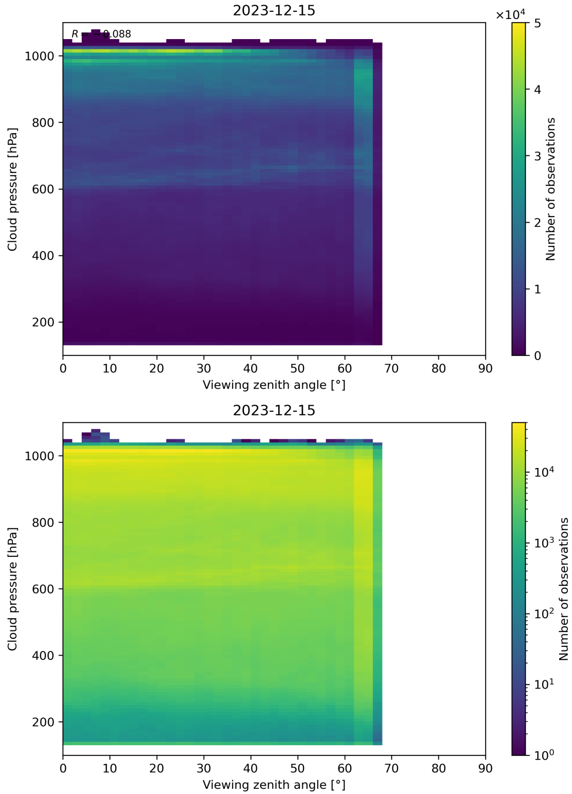
Figure 121: Scatter density plot of “Viewing zenith angle” against “Cloud pressure” for 2023-12-14 to 2023-12-16.
