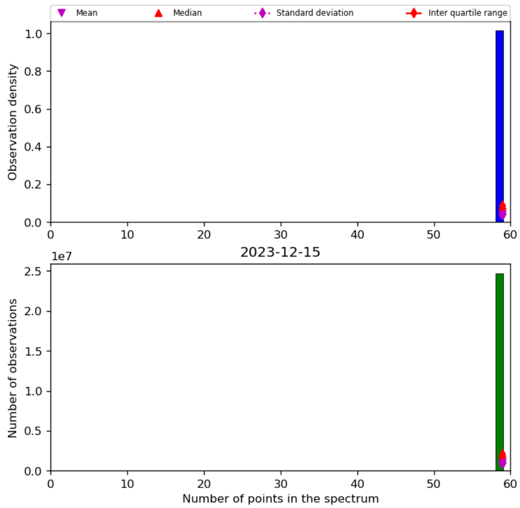
Figure 44: Histogram of “Number of points in the spectrum” for 2023-12-14 to 2023-12-16
