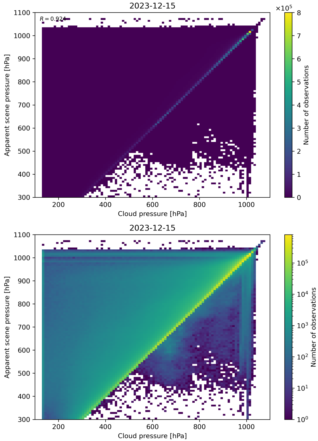
Figure 77: Scatter density plot of “Cloud pressure” against “Apparent scene pressure” for 2023-12-14 to 2023-12-16.
