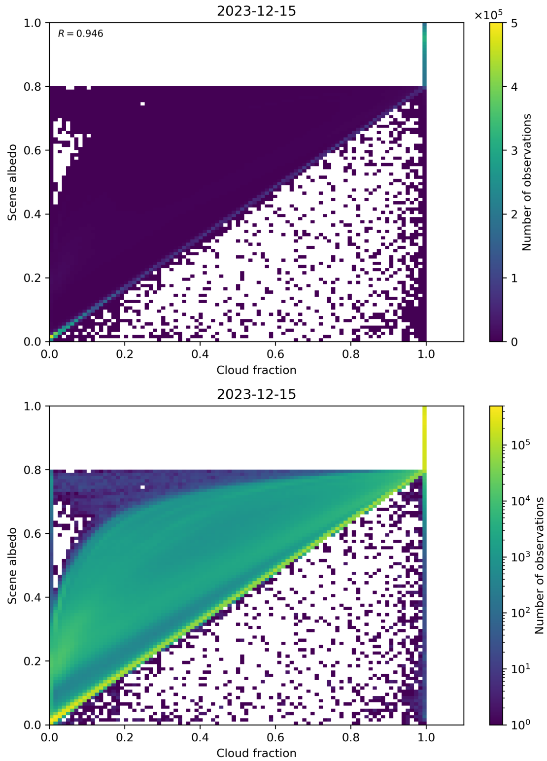
Figure 75: Scatter density plot of “Cloud fraction” against “Scene albedo” for 2023-12-14 to 2023-12-16.
