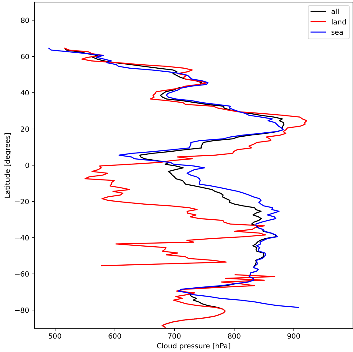
Figure 13: Zonal average of “Cloud pressure” for 2023-12-14 to 2023-12-16.
