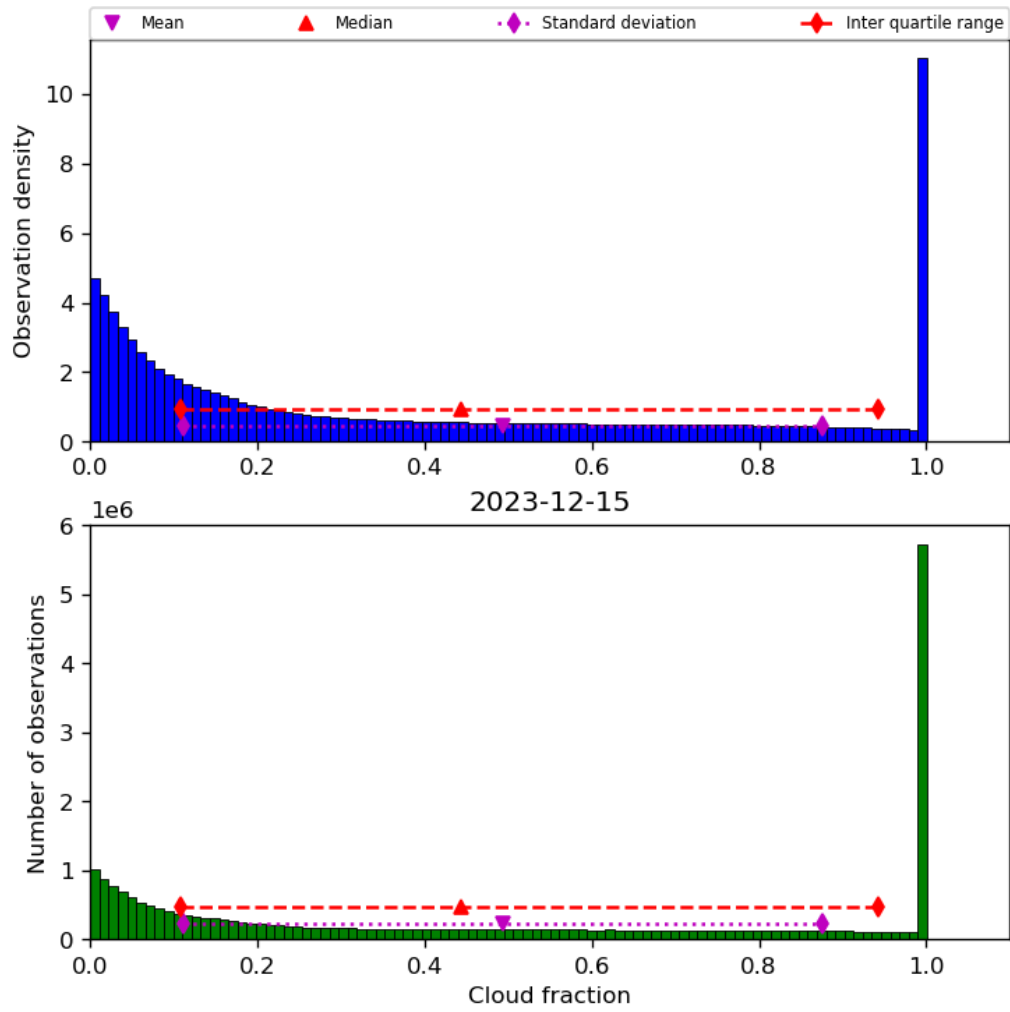
Figure 32: Histogram of “Cloud fraction” for 2023-12-14 to 2023-12-16
