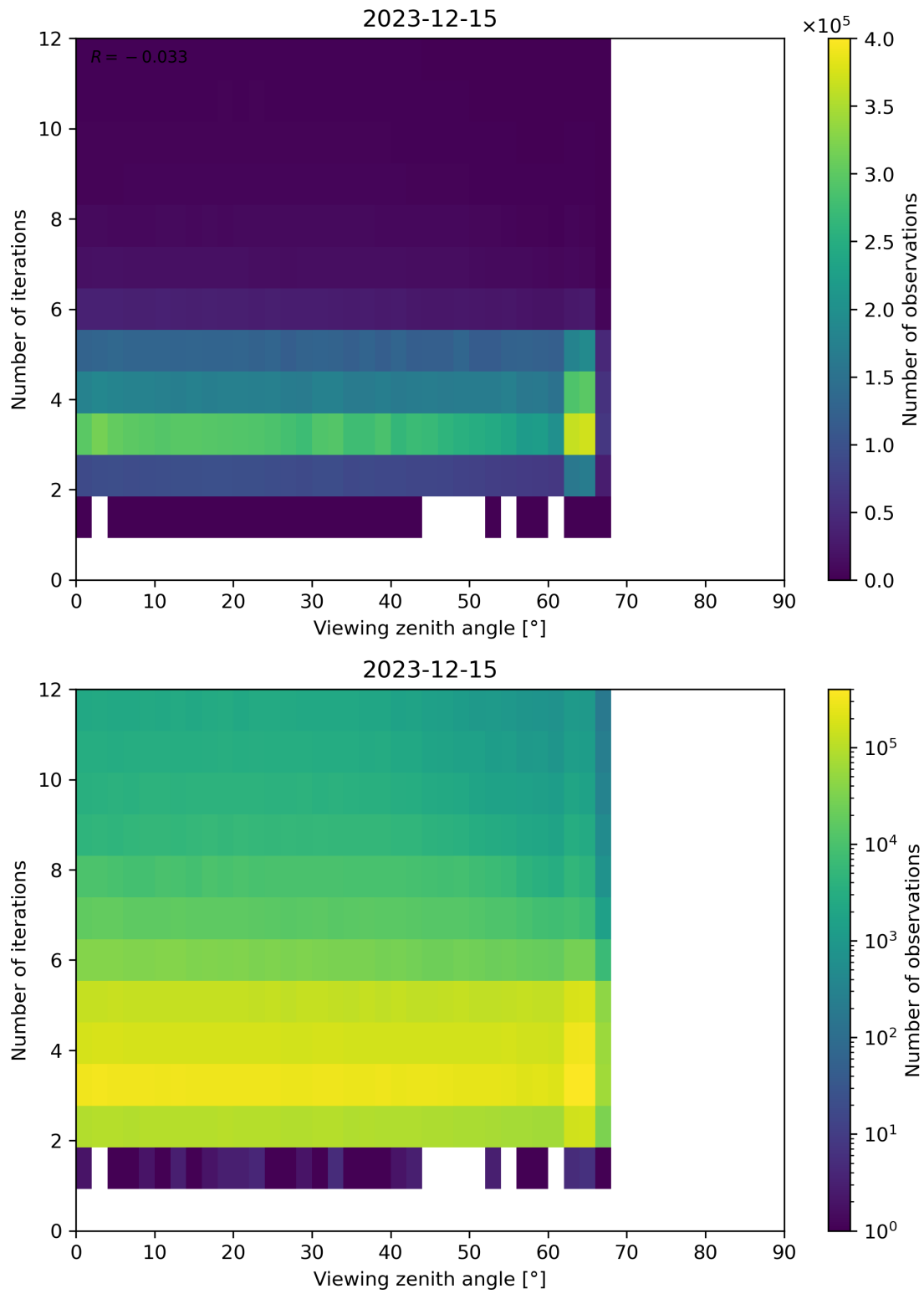
Figure 124: Scatter density plot of “Viewing zenith angle” against “Number of iterations” for 2023-12-14 to 2023-12-16.
