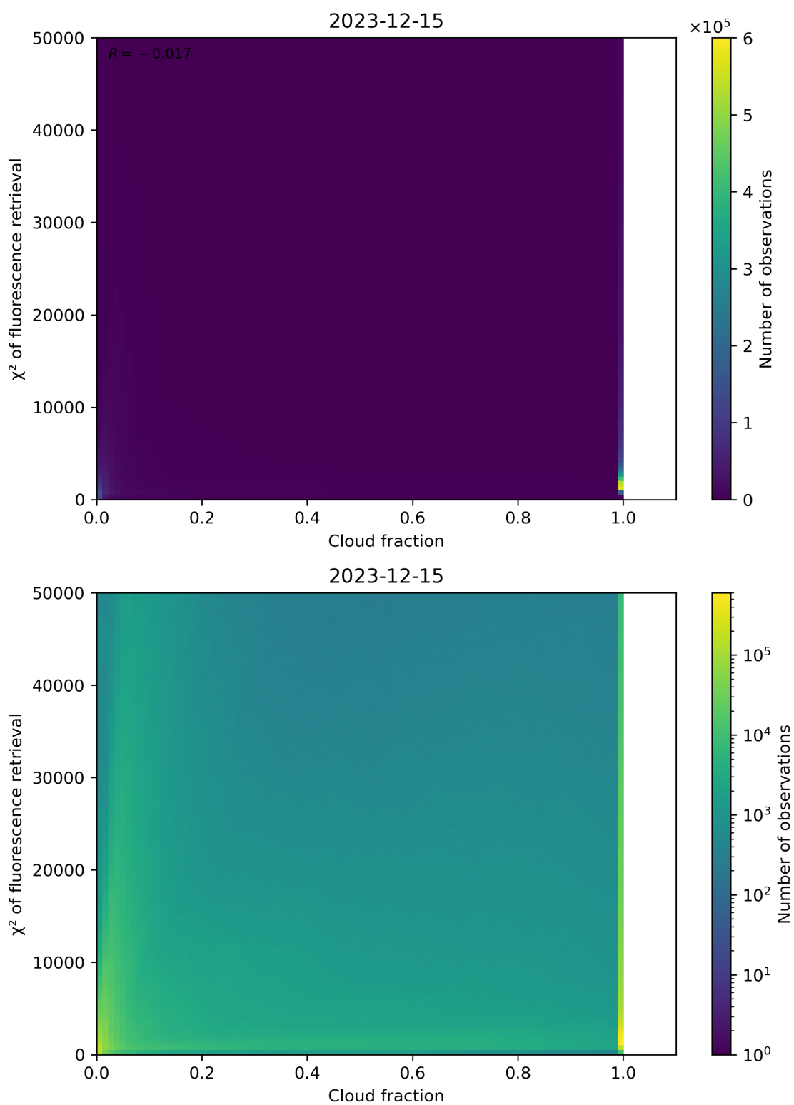
Figure 71: Scatter density plot of “Cloud fraction” against “ \chi^2 of fluorescence retrieval” for 2023-12-14 to 2023-12-16.
