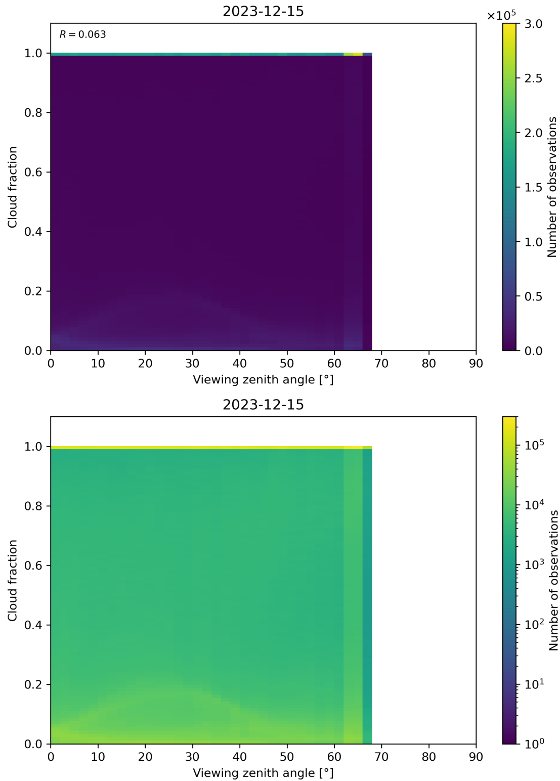
Figure 120: Scatter density plot of “Viewing zenith angle” against “Cloud fraction” for 2023-12-14 to 2023-12-16.
