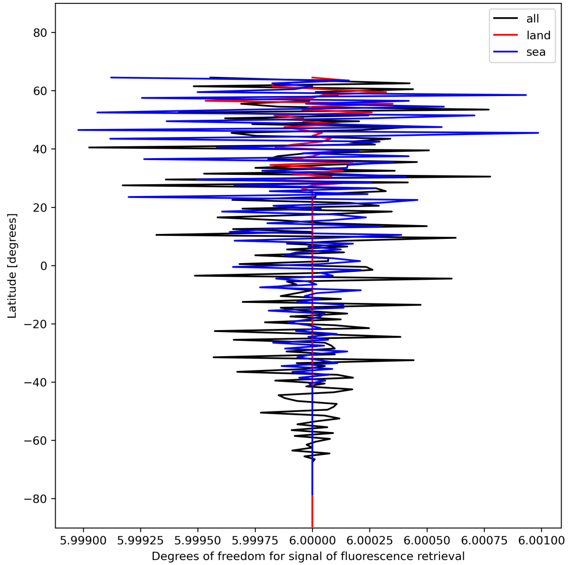
Figure 26: Zonal average of “Degrees of freedom for signal of fluorescence retrieval” for 2023-12-14 to 2023-12-16.
