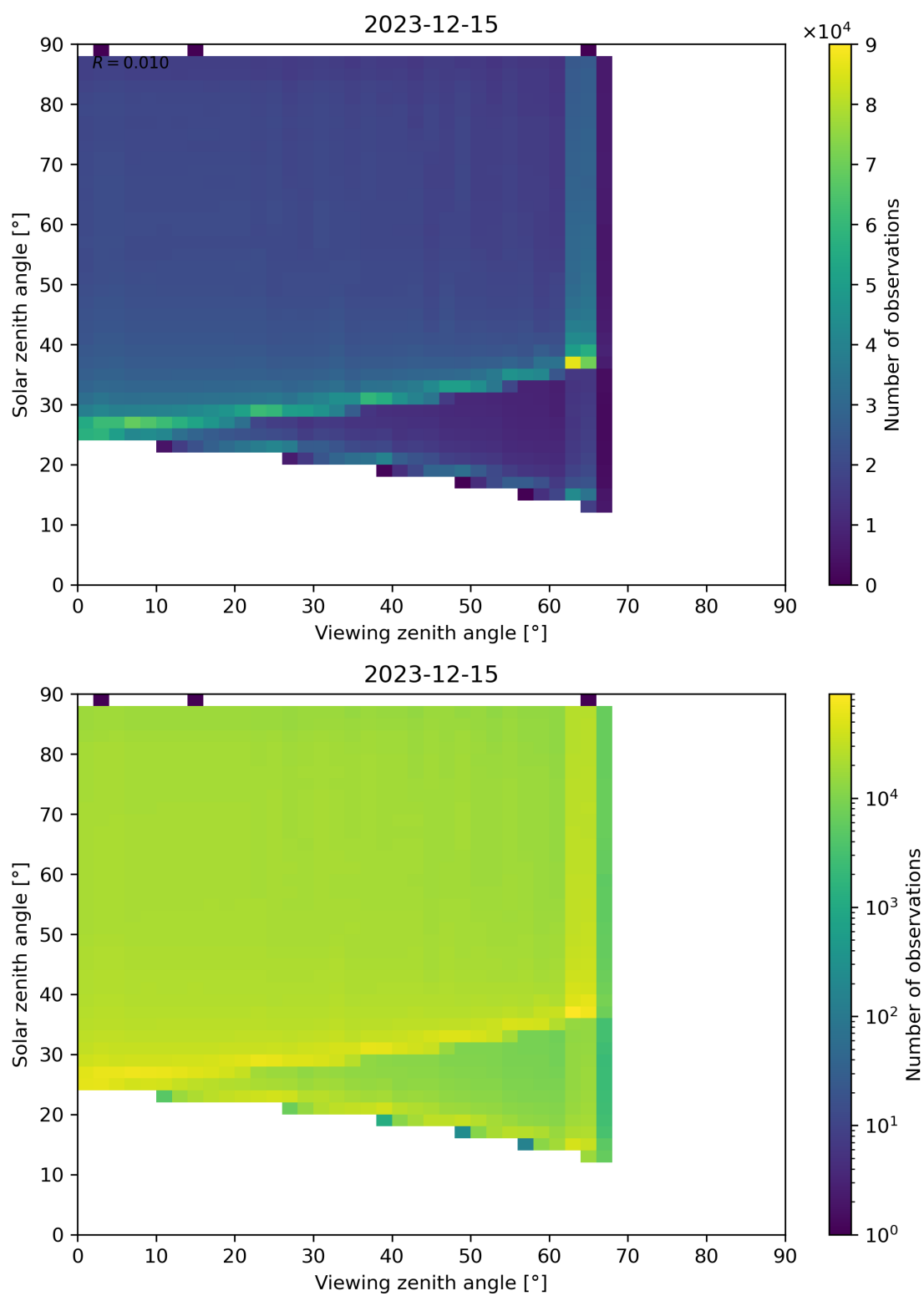
Figure 127: Scatter density plot of “Viewing zenith angle” against “Solar zenith angle” for 2023-12-14 to 2023-12-16.
