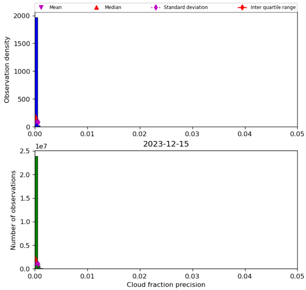
Figure 33: Histogram of “Cloud fraction precision” for 2023-12-14 to 2023-12-16
