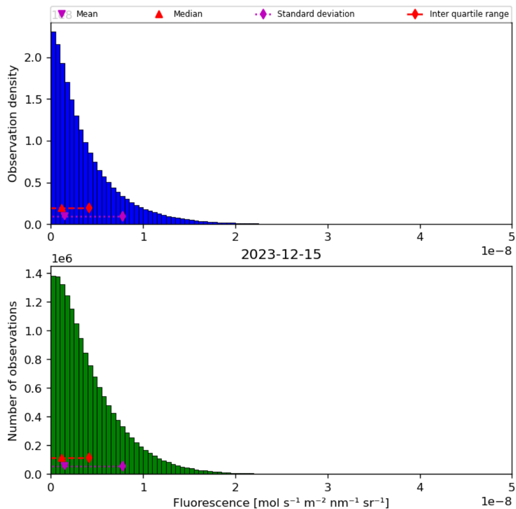
Figure 40: Histogram of “Fluorescence” for 2023-12-14 to 2023-12-16
