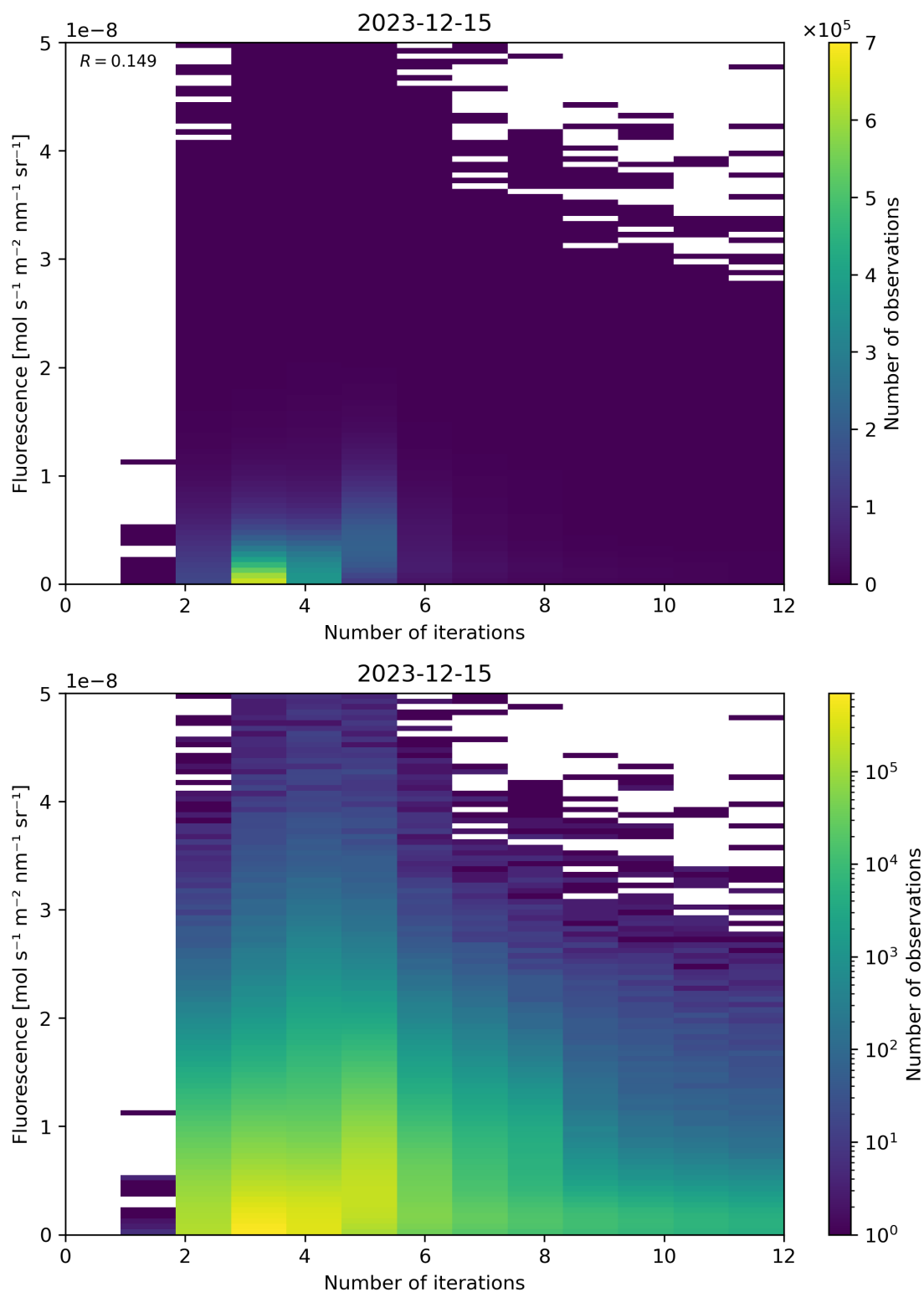
Figure 98: Scatter density plot of “Number of iterations” against “Fluorescence” for 2023-12-14 to 2023-12-16.
