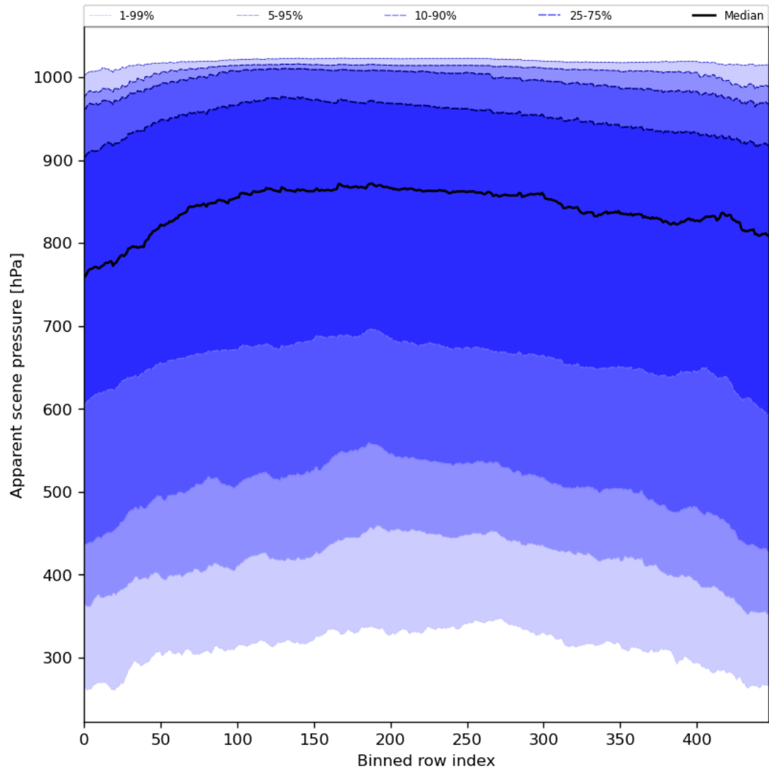
Figure 53: Along track statistics of “Apparent scene pressure” for 2023-12-14 to 2023-12-16
