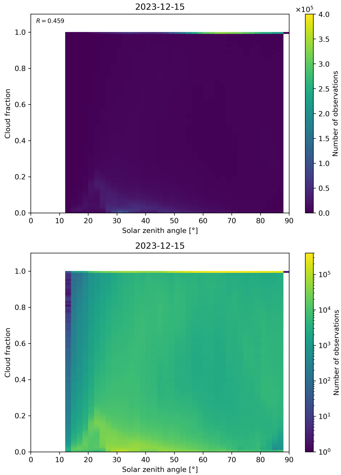
Figure 110: Scatter density plot of “Solar zenith angle” against “Cloud fraction” for 2023-12-14 to 2023-12-16.
