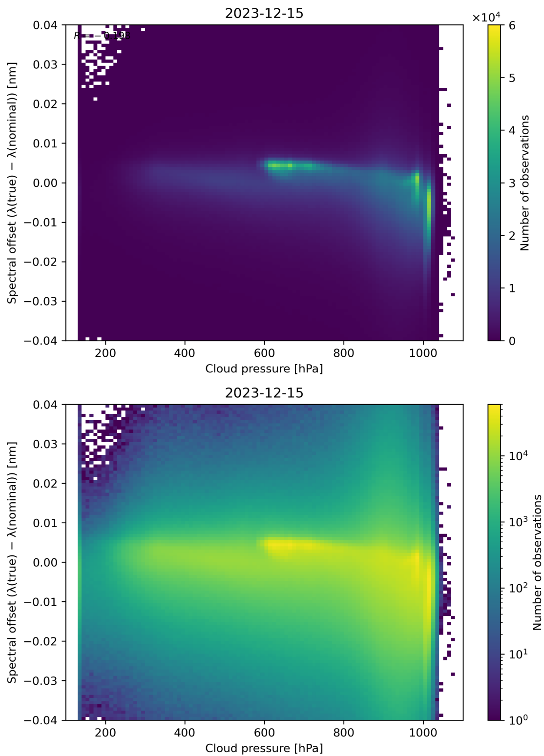
Figure 84: Scatter density plot of “Cloud pressure” against “Spectral offset ( \lambda(\text{true}) - \lambda(\text{nominal}) )” for 2023-12-14 to 2023-12-16.
