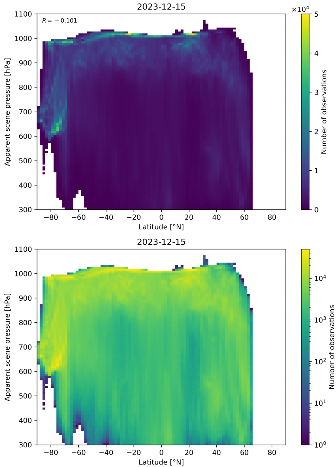
Figure 88: Scatter density plot of “Latitude” against “Apparent scene pressure” for 2023-12-14 to 2023-12-16.
