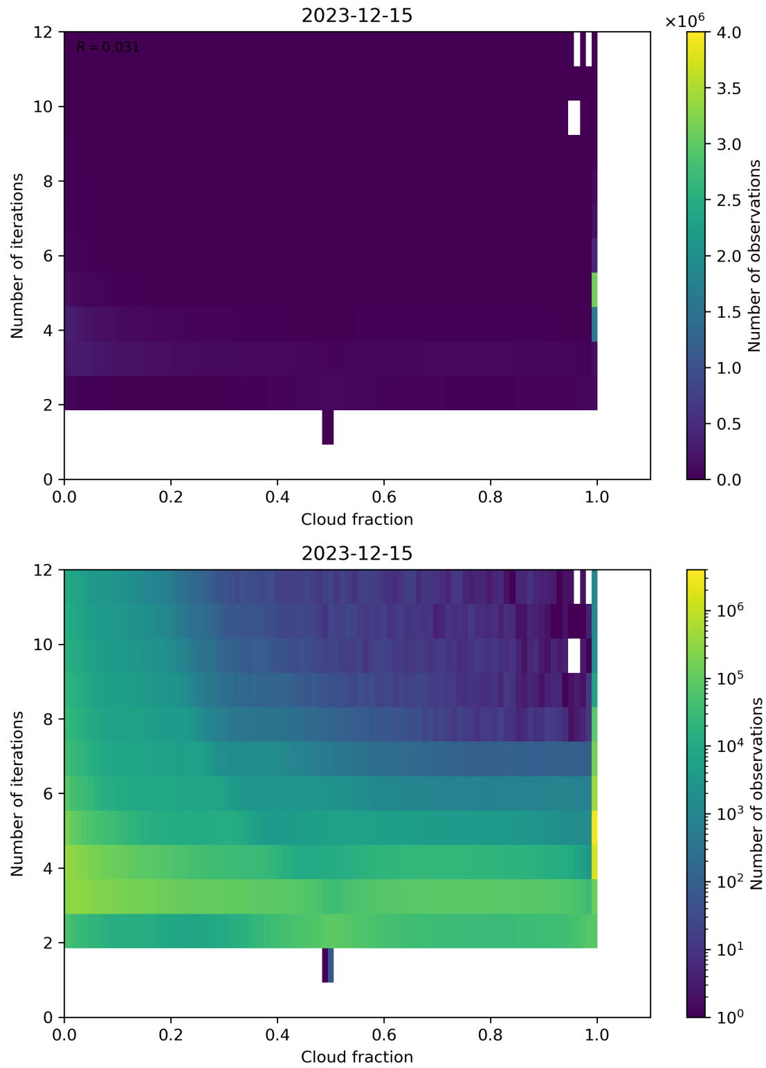
Figure 73: Scatter density plot of “Cloud fraction” against “Number of iterations” for 2023-12-14 to 2023-12-16.
