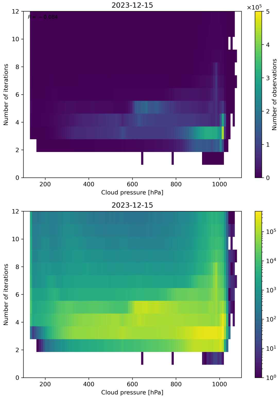
Figure 81: Scatter density plot of “Cloud pressure” against “Number of iterations” for 2023-12-14 to 2023-12-16.
