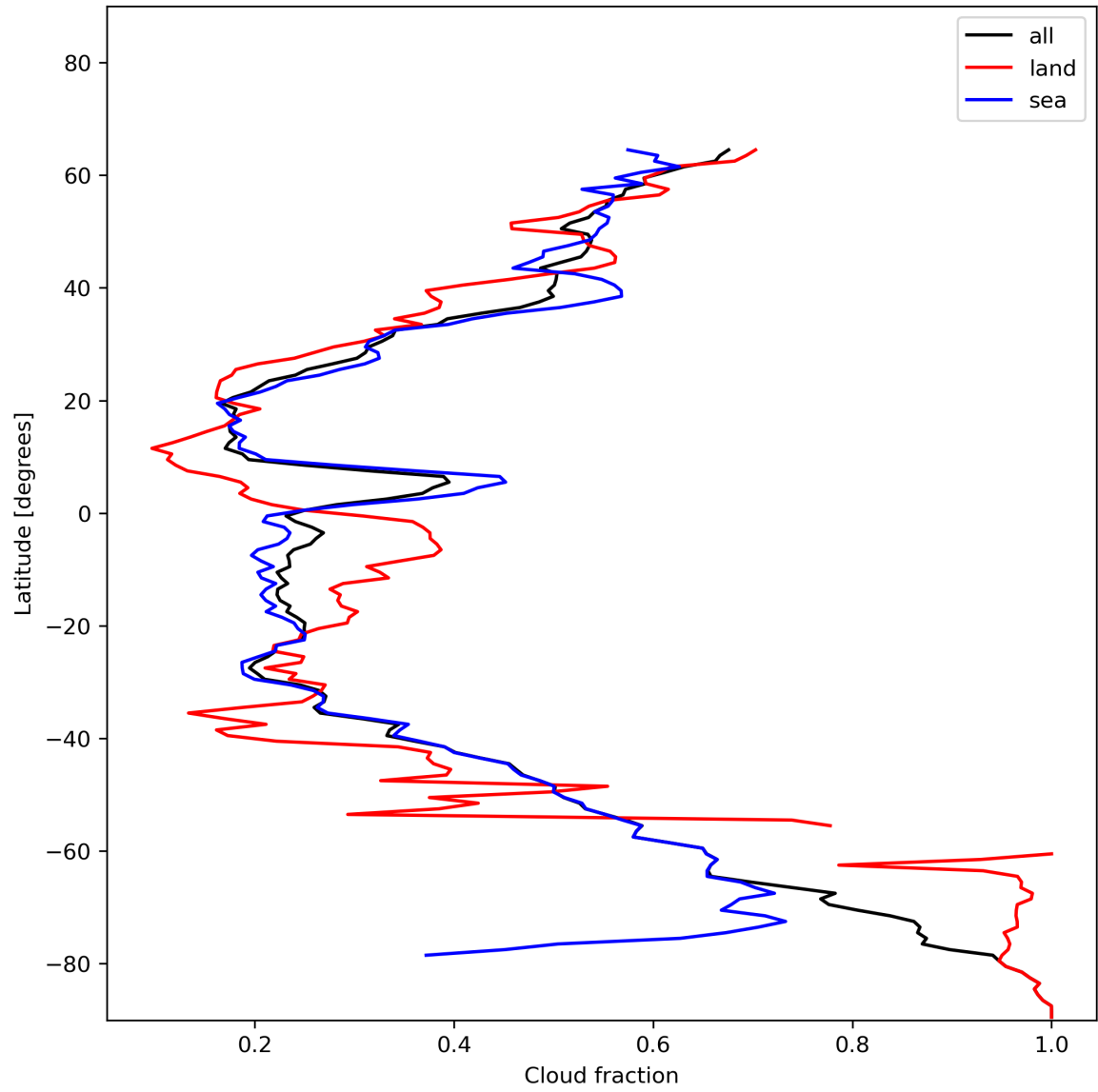
Figure 15: Zonal average of “Cloud fraction” for 2023-12-14 to 2023-12-16.
