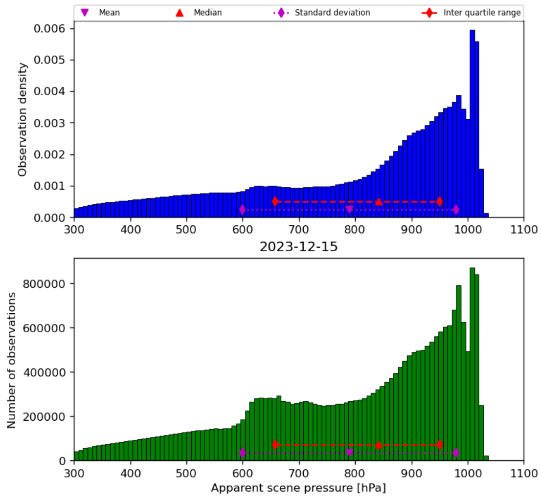
Figure 36: Histogram of “Apparent scene pressure” for 2023-12-14 to 2023-12-16
