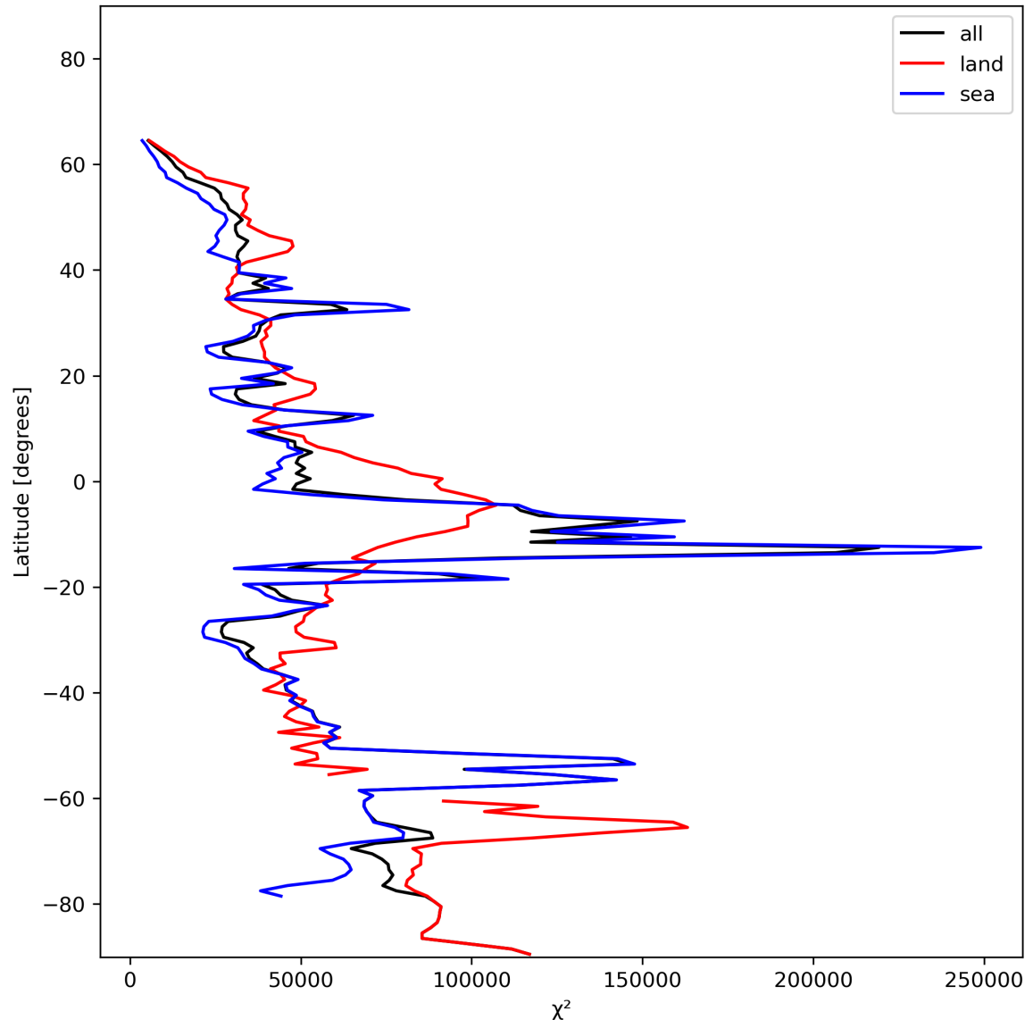
Figure 21: Zonal average of “ \chi^2 ” for 2023-12-14 to 2023-12-16.
