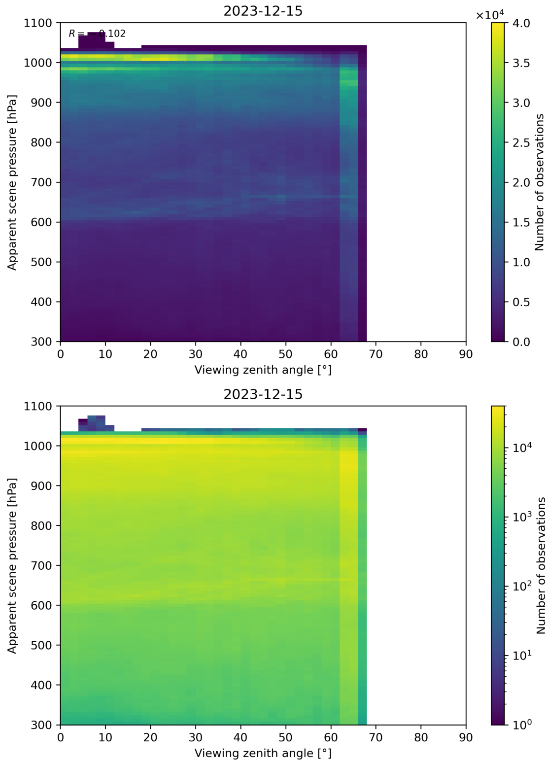
Figure 118: Scatter density plot of “Viewing zenith angle” against “Apparent scene pressure” for 2023-12-14 to 2023-12-16.
