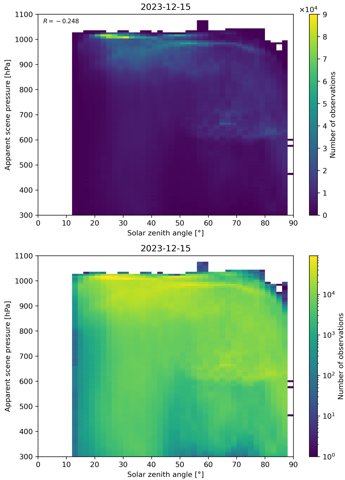
Figure 108: Scatter density plot of “Solar zenith angle” against “Apparent scene pressure” for 2023-12-14 to 2023-12-16.
