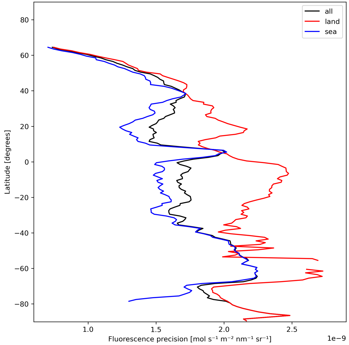
Figure 24: Zonal average of “Fluorescence precision” for 2023-12-14 to 2023-12-16.
