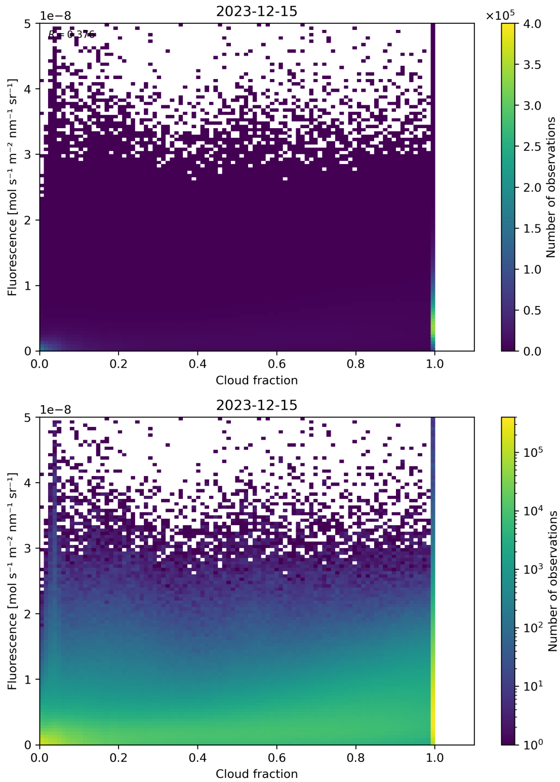
Figure 72: Scatter density plot of “Cloud fraction” against “Fluorescence” for 2023-12-14 to 2023-12-16.
