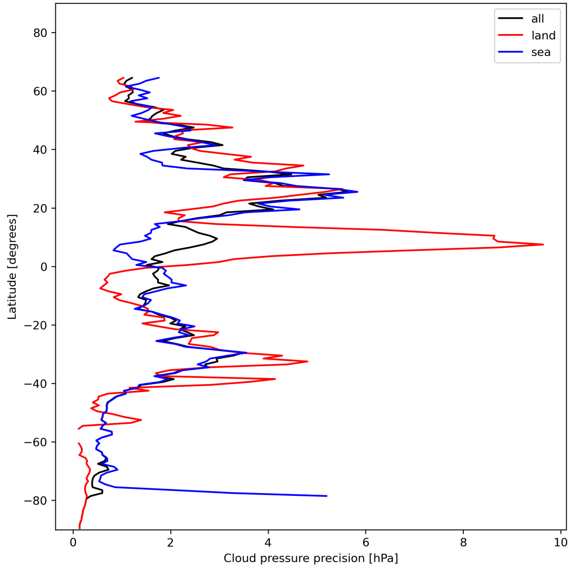
Figure 14: Zonal average of “Cloud pressure precision” for 2023-12-14 to 2023-12-16.
