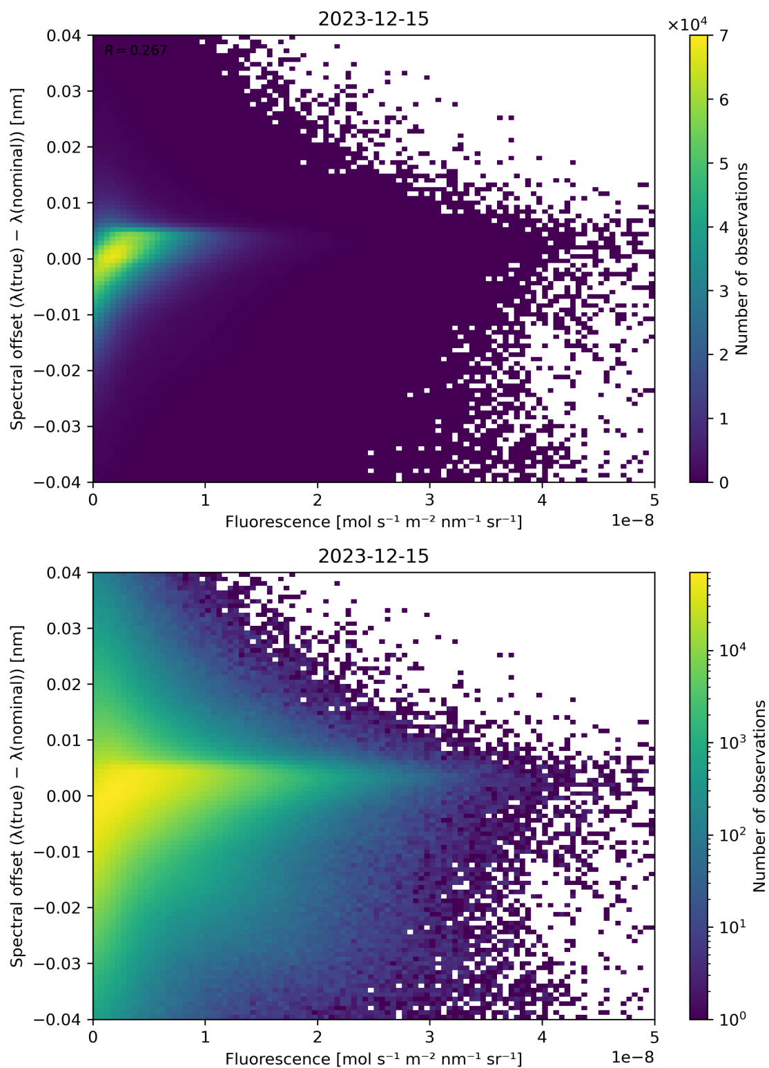
Figure 87: Scatter density plot of “Fluorescence” against “Spectral offset ( \lambda(\text{true}) - \lambda(\text{nominal}) )” for 2023-12-14 to 2023-12-16.
