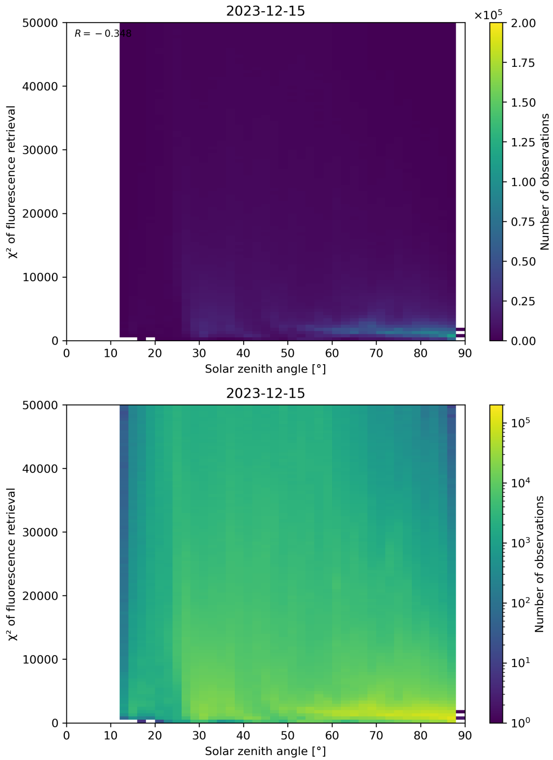
Figure 109: Scatter density plot of “Solar zenith angle” against “ \chi^2 of fluorescence retrieval” for 2023-12-14 to 2023-12-16.
