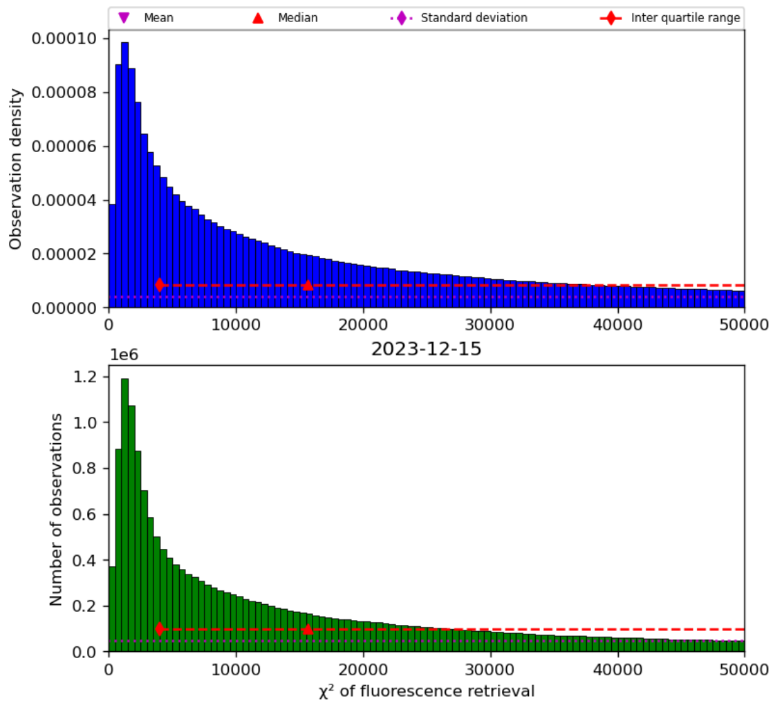
Figure 42: Histogram of “ \chi^2 of fluorescence retrieval” for 2023-12-14 to 2023-12-16
