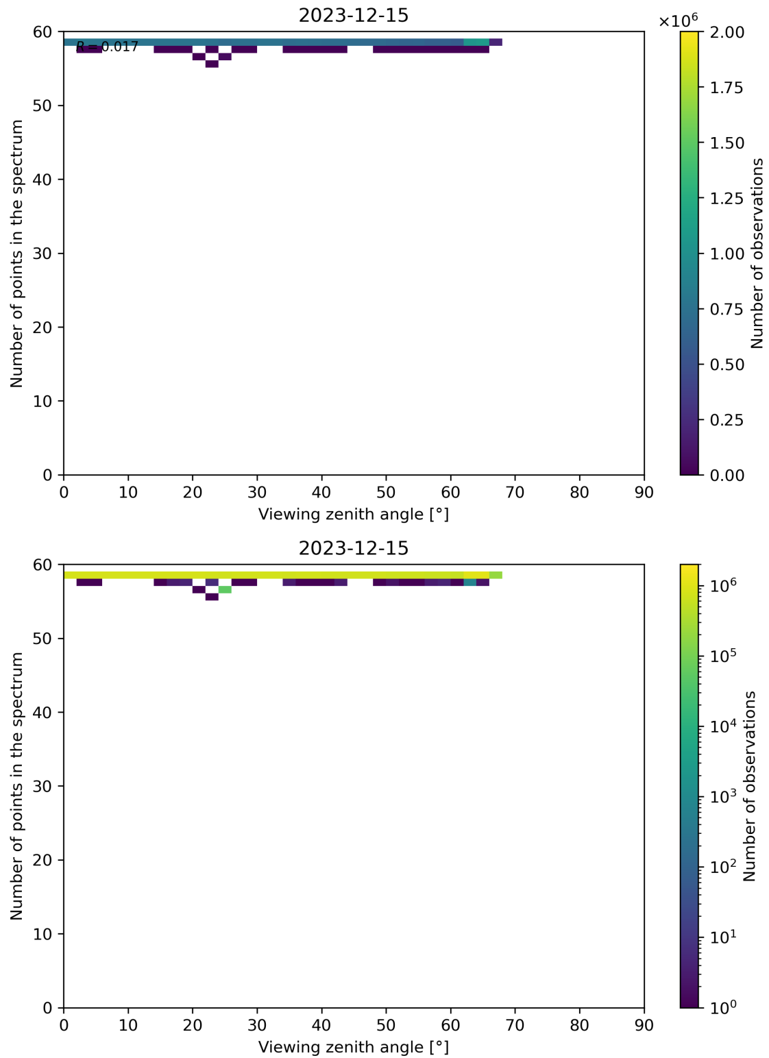
Figure 125: Scatter density plot of “Viewing zenith angle” against “Number of points in the spectrum” for 2023-12-14 to 2023-12-16.
