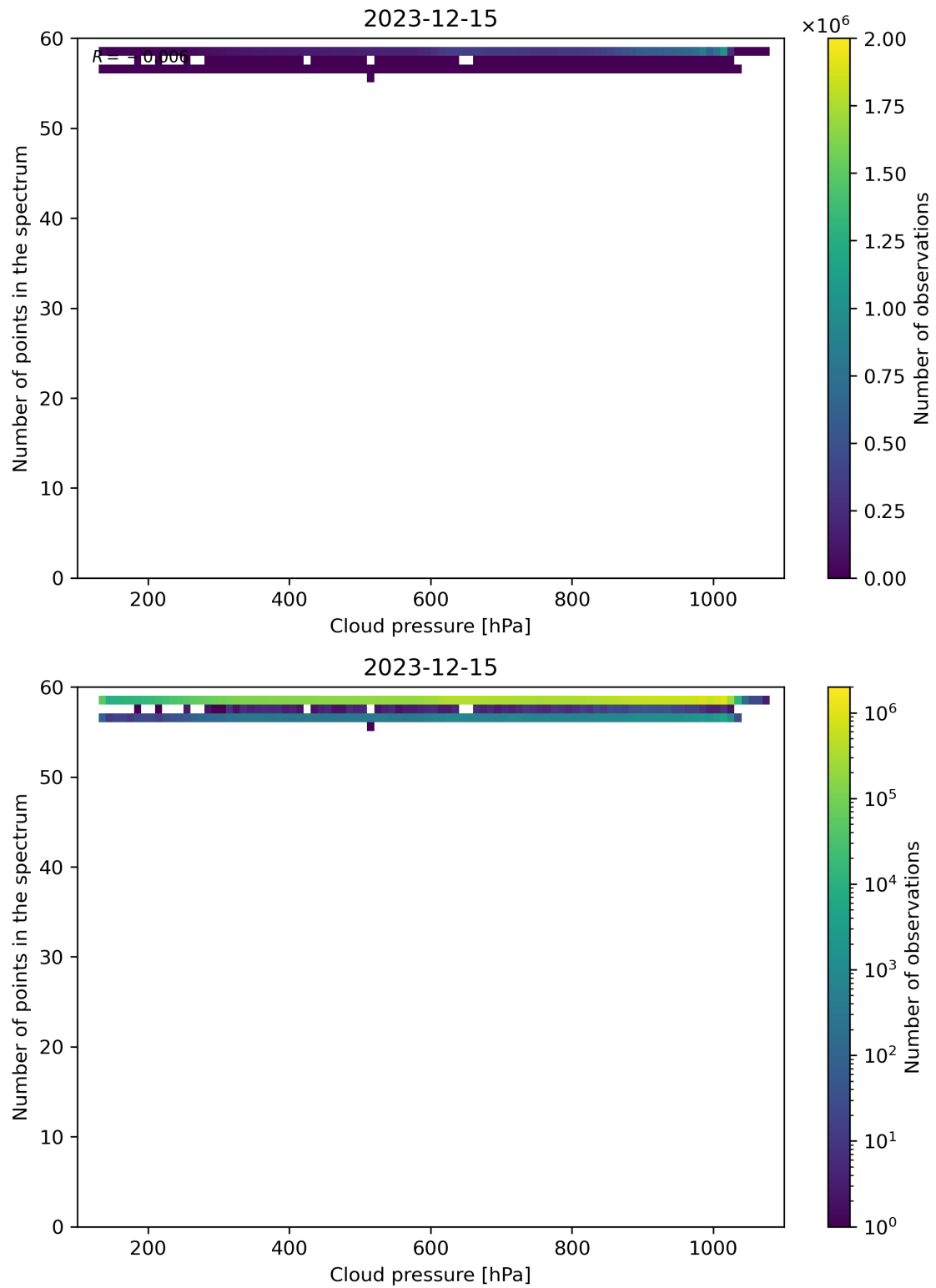
Figure 82: Scatter density plot of “Cloud pressure” against “Number of points in the spectrum” for 2023-12-14 to 2023-12-16.
