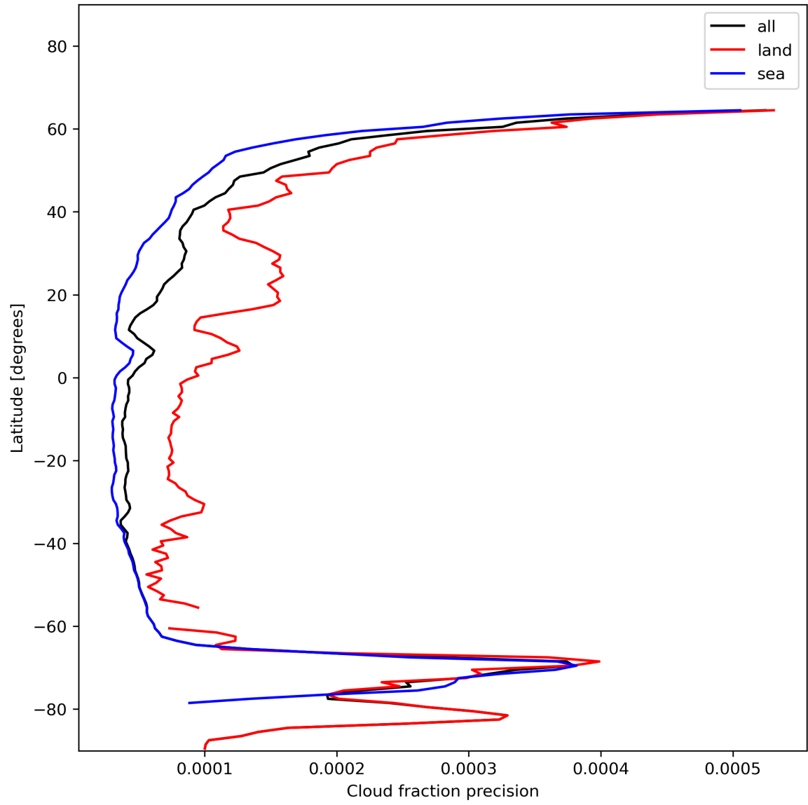
Figure 16: Zonal average of “Cloud fraction precision” for 2023-12-14 to 2023-12-16.
