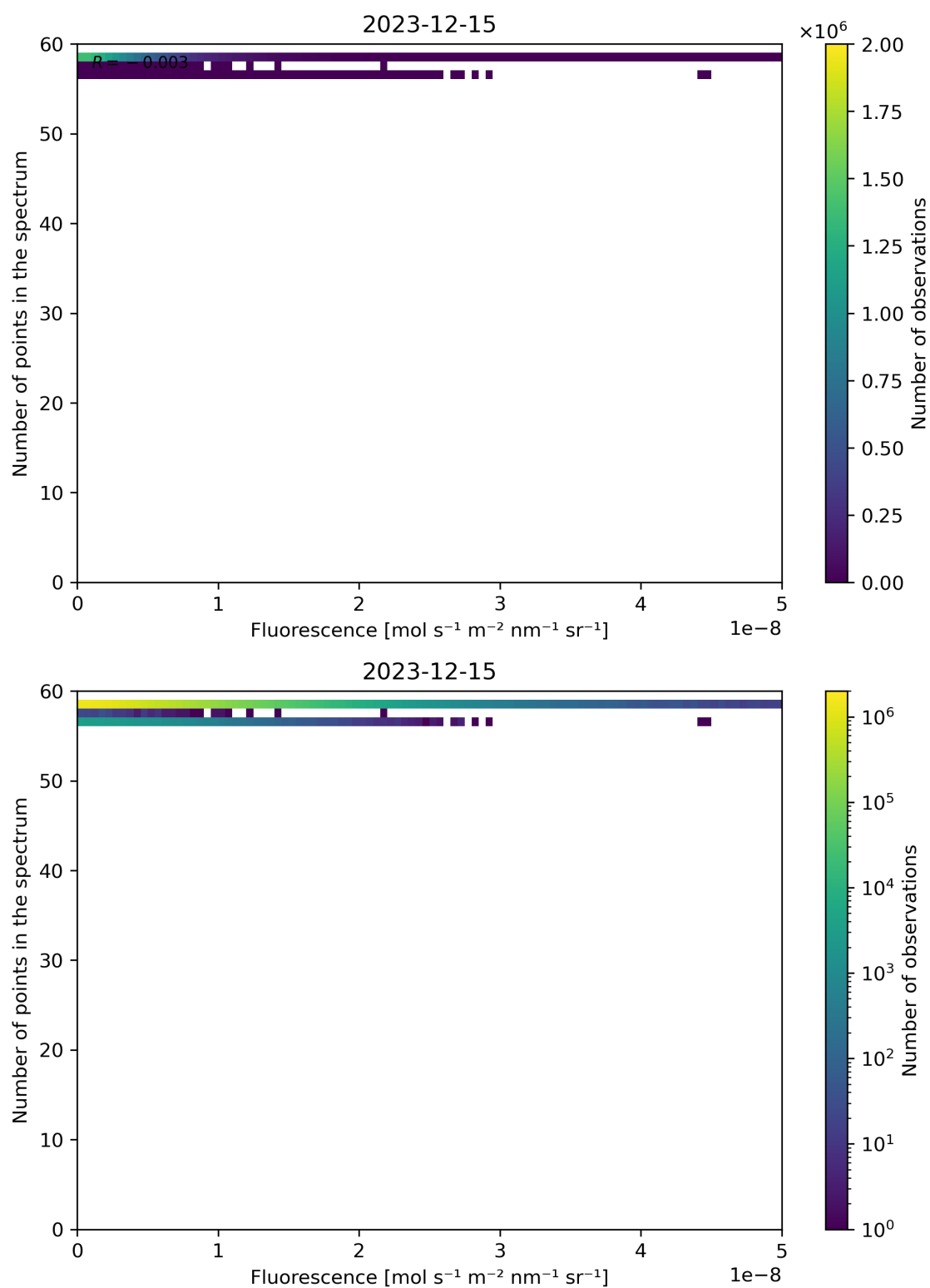
Figure 86: Scatter density plot of “Fluorescence” against “Number of points in the spectrum” for 2023-12-14 to 2023-12-16.
