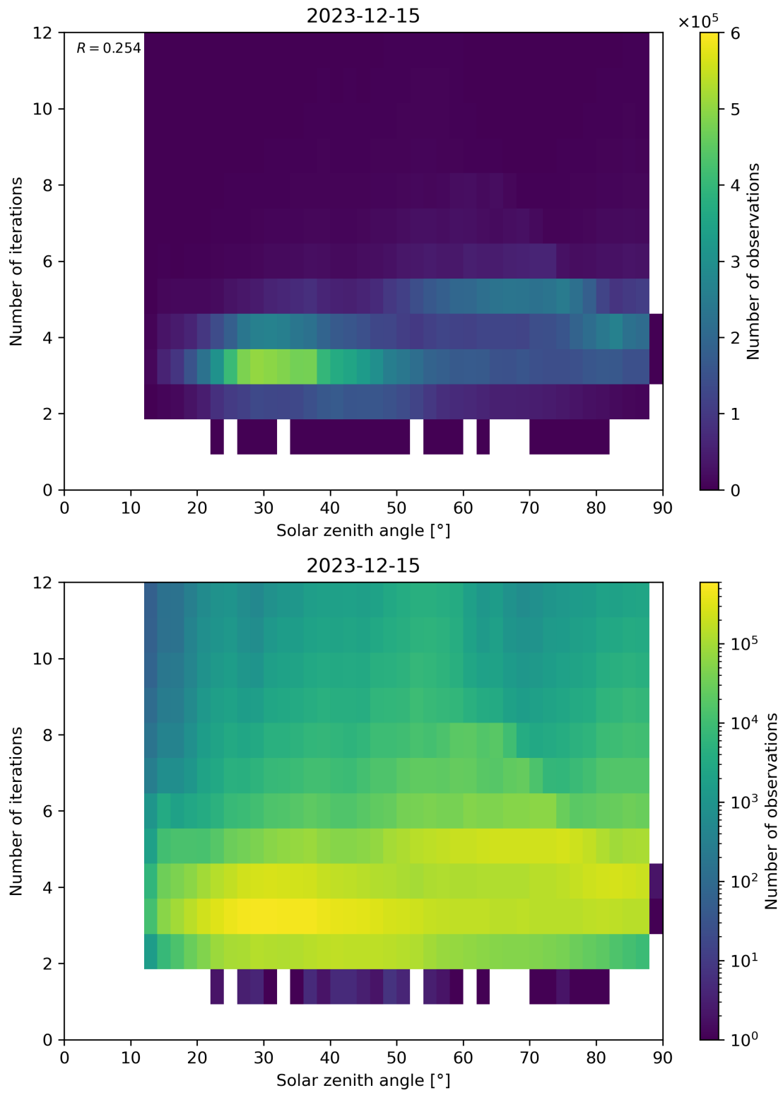
Figure 114: Scatter density plot of “Solar zenith angle” against “Number of iterations” for 2023-12-14 to 2023-12-16.
