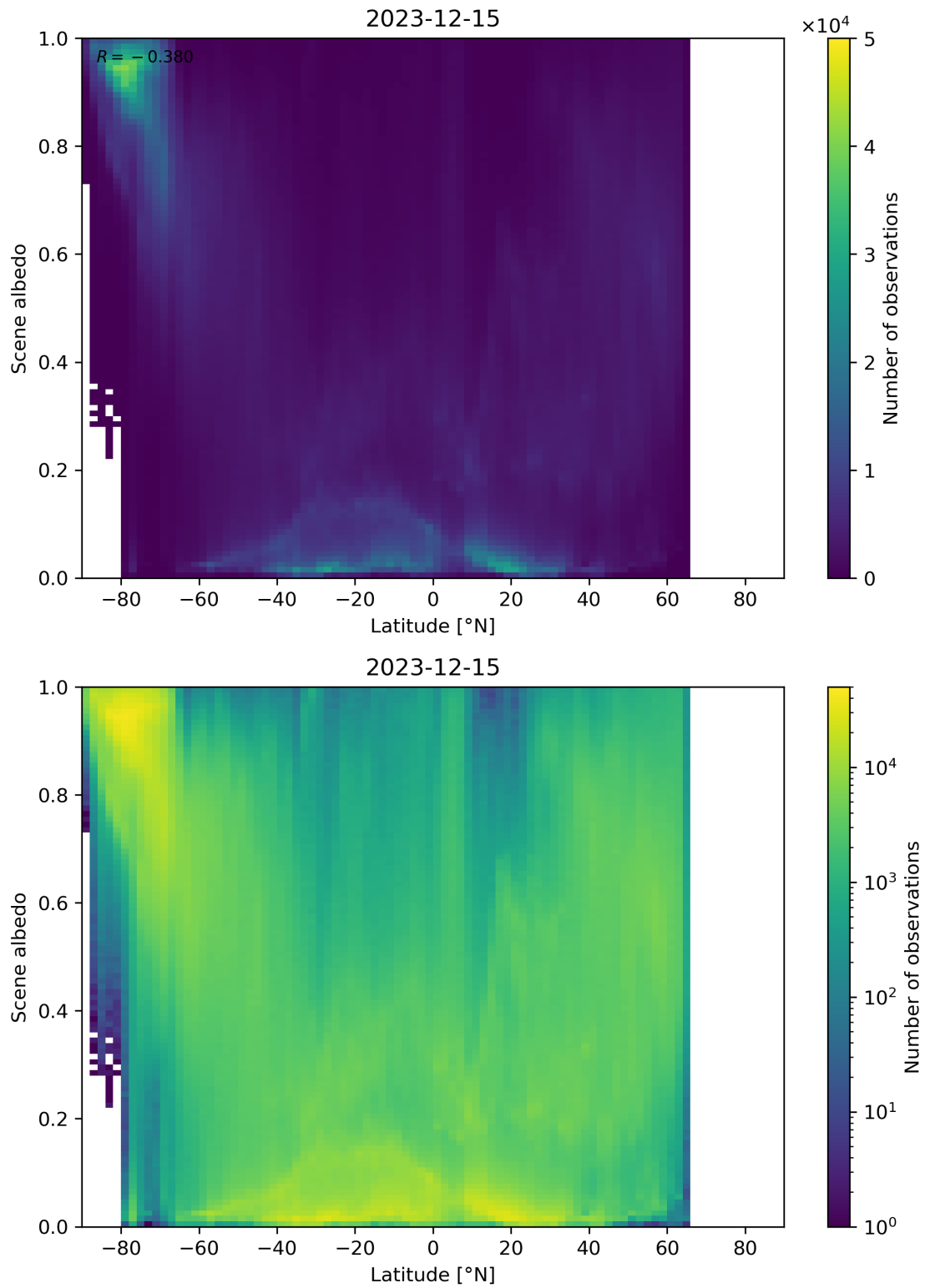
Figure 95: Scatter density plot of “Latitude” against “Scene albedo” for 2023-12-14 to 2023-12-16.
