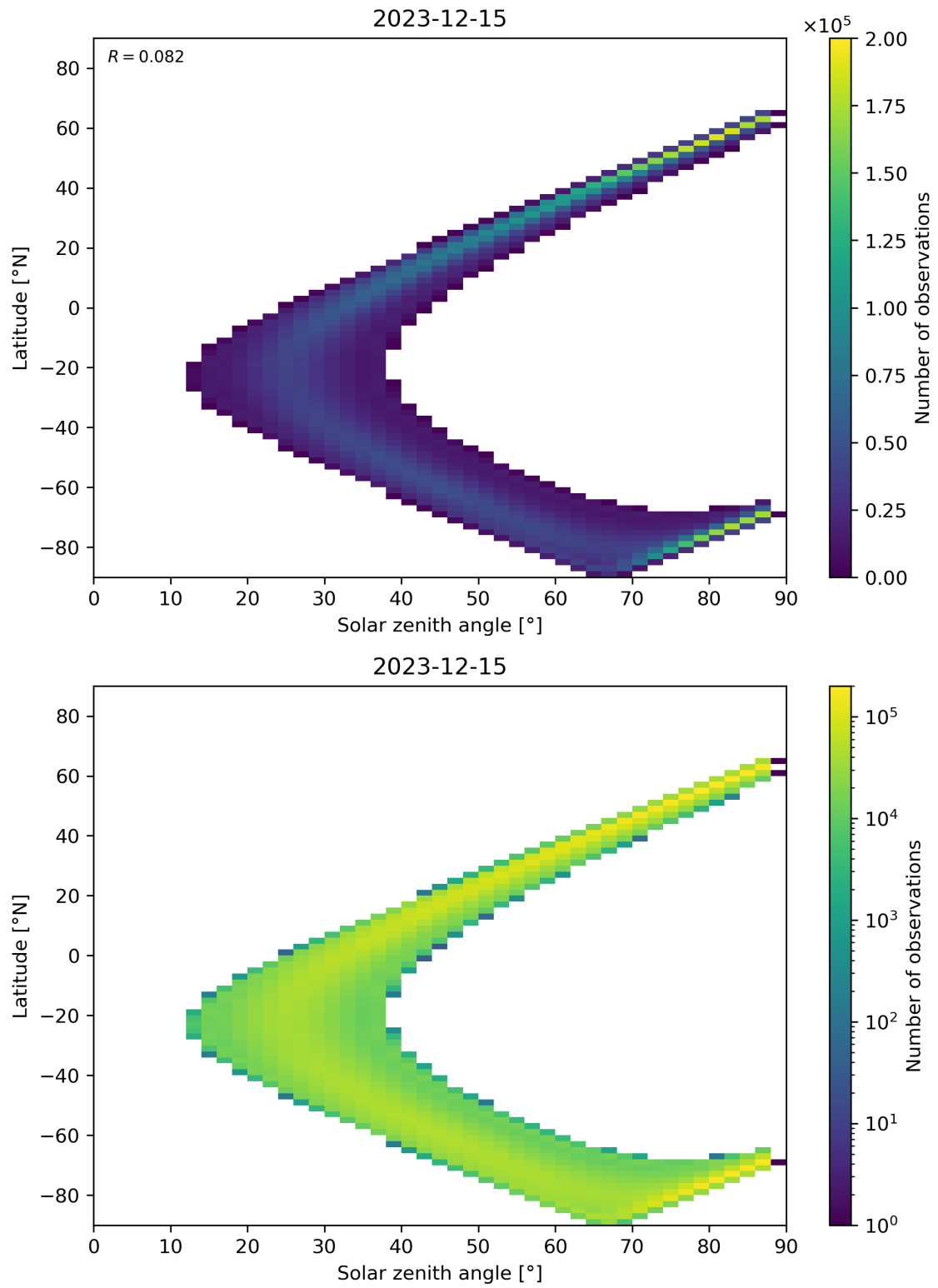
Figure 113: Scatter density plot of “Solar zenith angle” against “Latitude” for 2023-12-14 to 2023-12-16.
