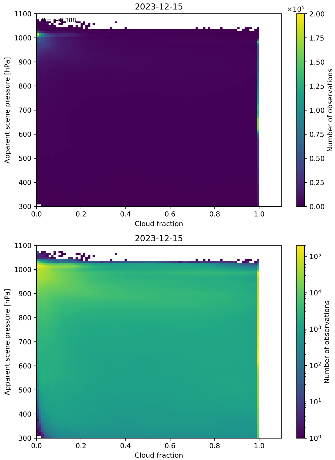
Figure 70: Scatter density plot of “Cloud fraction” against “Apparent scene pressure” for 2023-12-14 to 2023-12-16.
