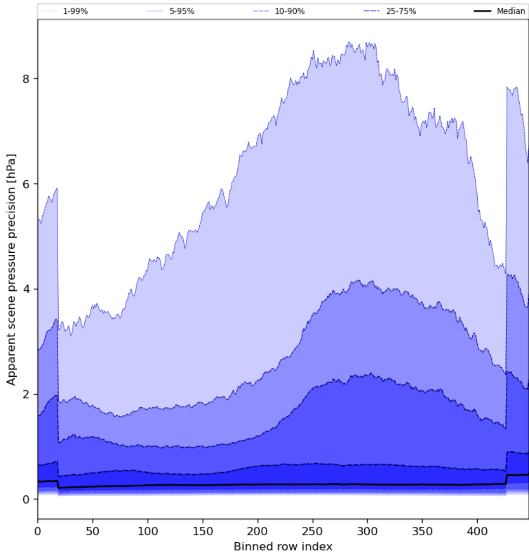
Figure 54: Along track statistics of “Apparent scene pressure precision” for 2023-12-14 to 2023-12-16
