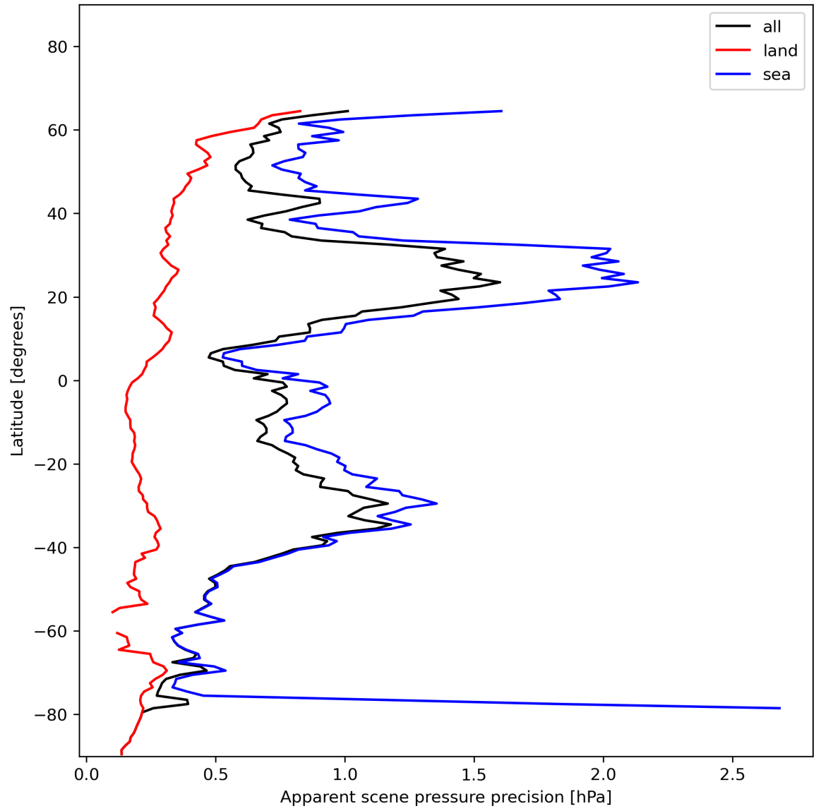
Figure 20: Zonal average of “Apparent scene pressure precision” for 2023-12-14 to 2023-12-16.
