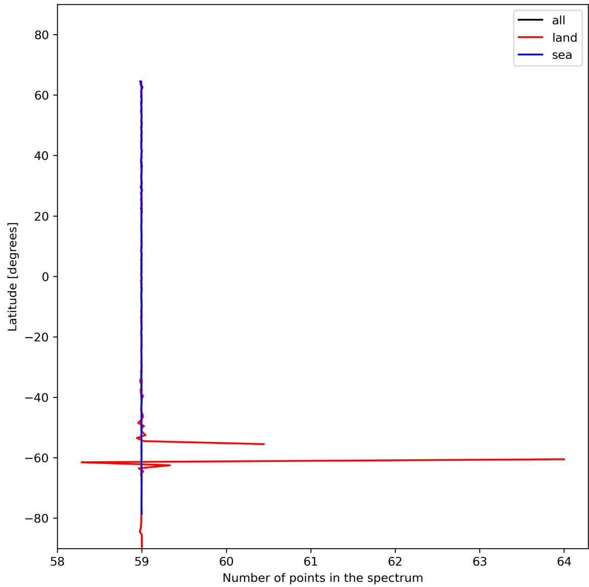
Figure 27: Zonal average of “Number of points in the spectrum” for 2023-12-14 to 2023-12-16.
