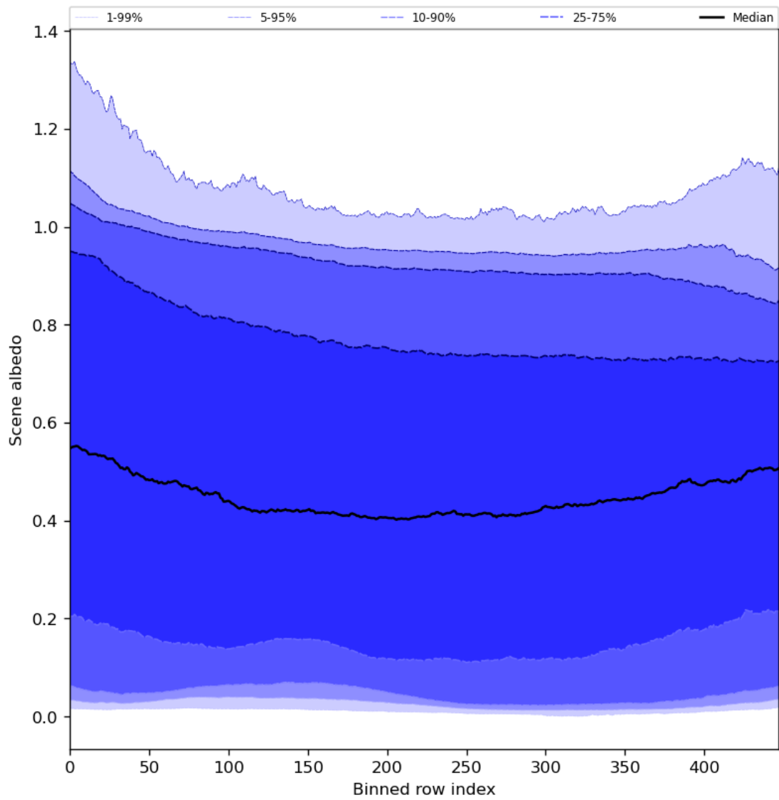
Figure 51: Along track statistics of “Scene albedo” for 2023-12-14 to 2023-12-16
