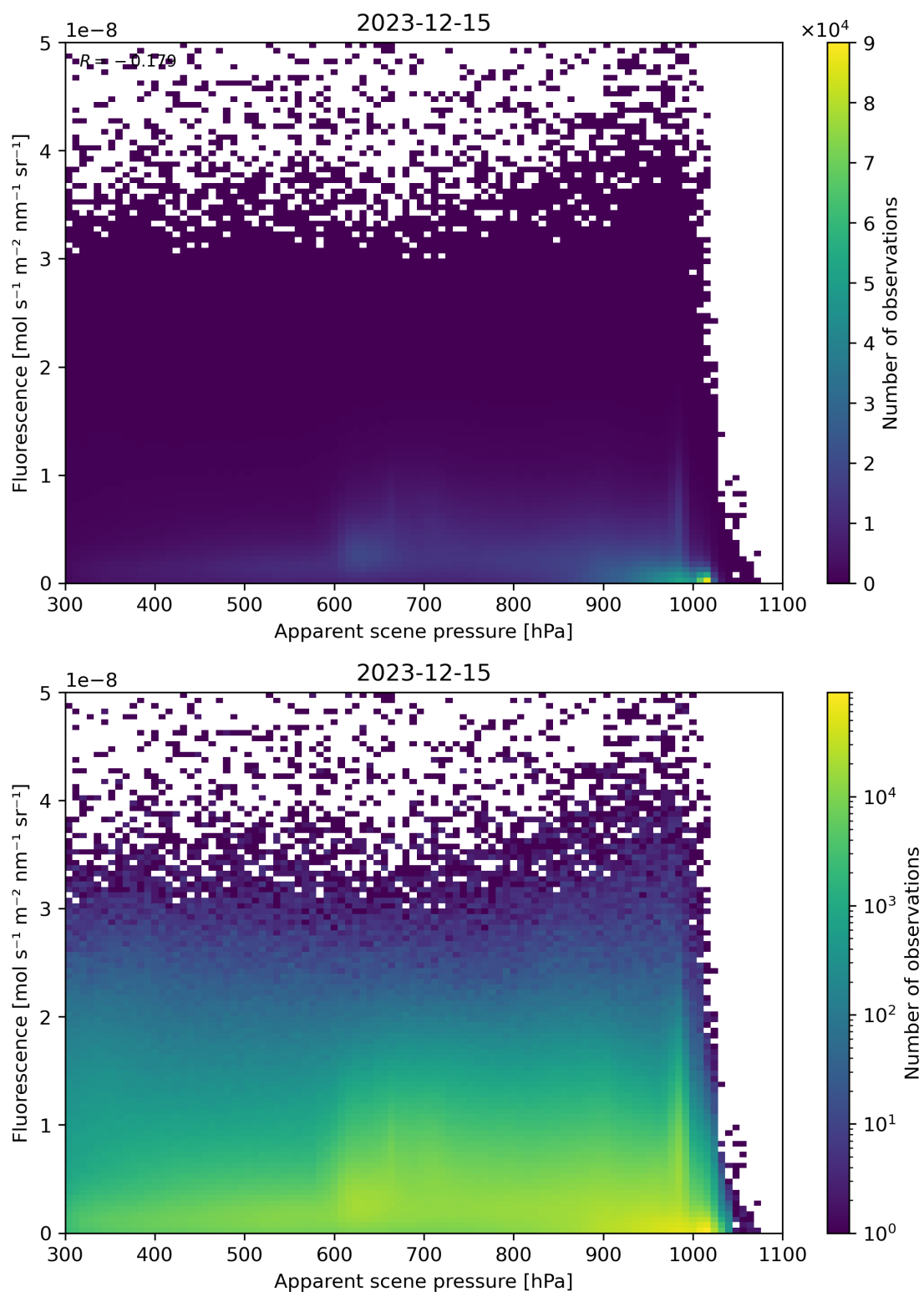
Figure 64: Scatter density plot of “Apparent scene pressure” against “Fluorescence” for 2023-12-14 to 2023-12-16.
