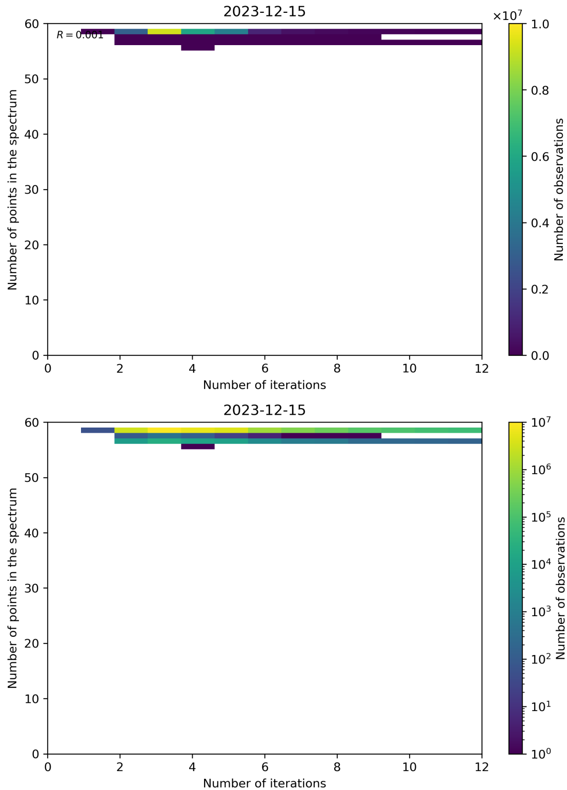
Figure 99: Scatter density plot of “Number of iterations” against “Number of points in the spectrum” for 2023-12-14 to 2023-12-16.
