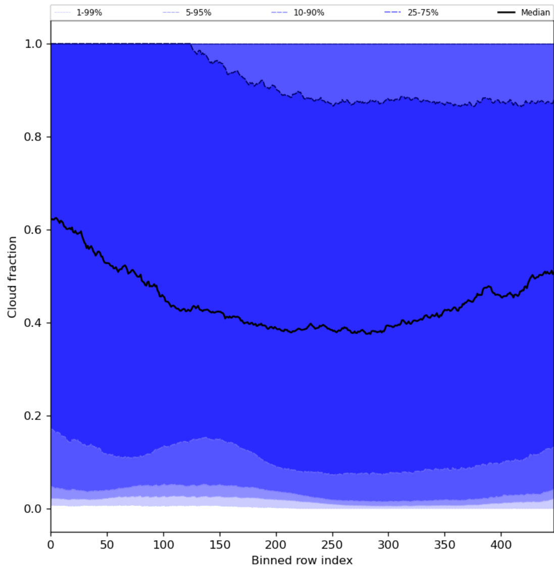
Figure 49: Along track statistics of “Cloud fraction” for 2023-12-14 to 2023-12-16
