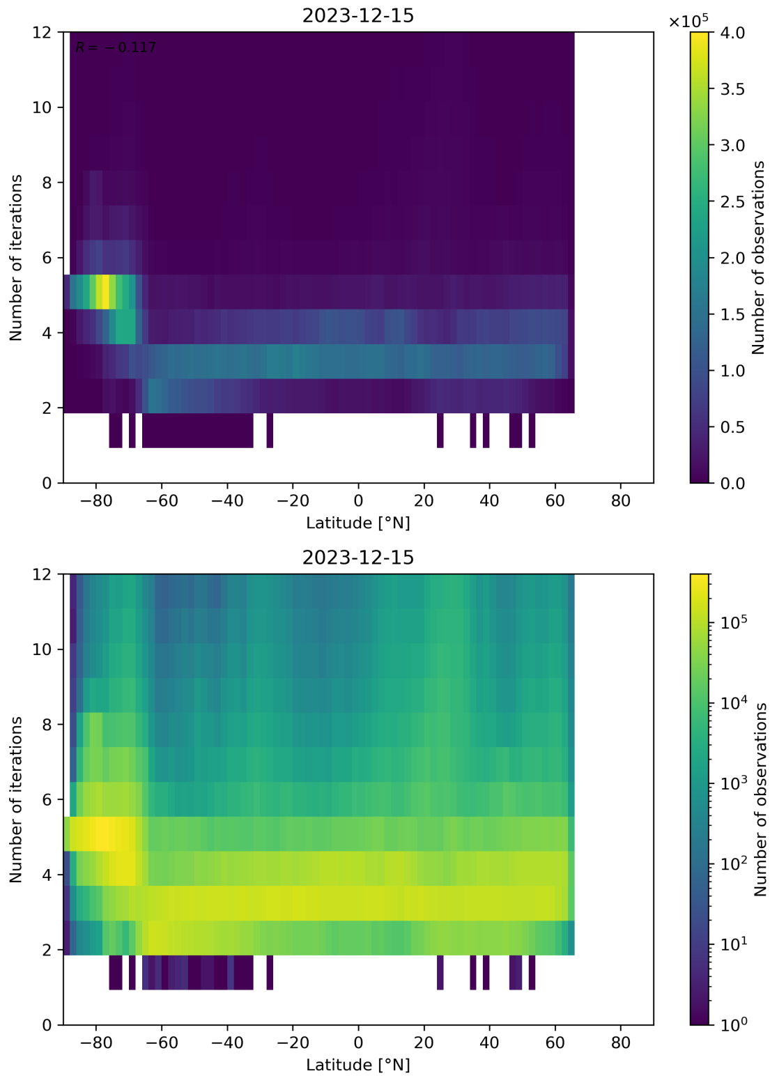
Figure 93: Scatter density plot of “Latitude” against “Number of iterations” for 2023-12-14 to 2023-12-16.
