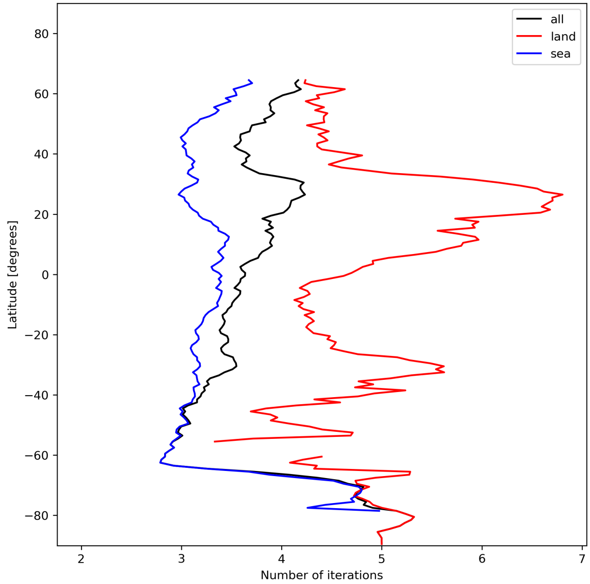
Figure 22: Zonal average of “Number of iterations” for 2023-12-14 to 2023-12-16.
