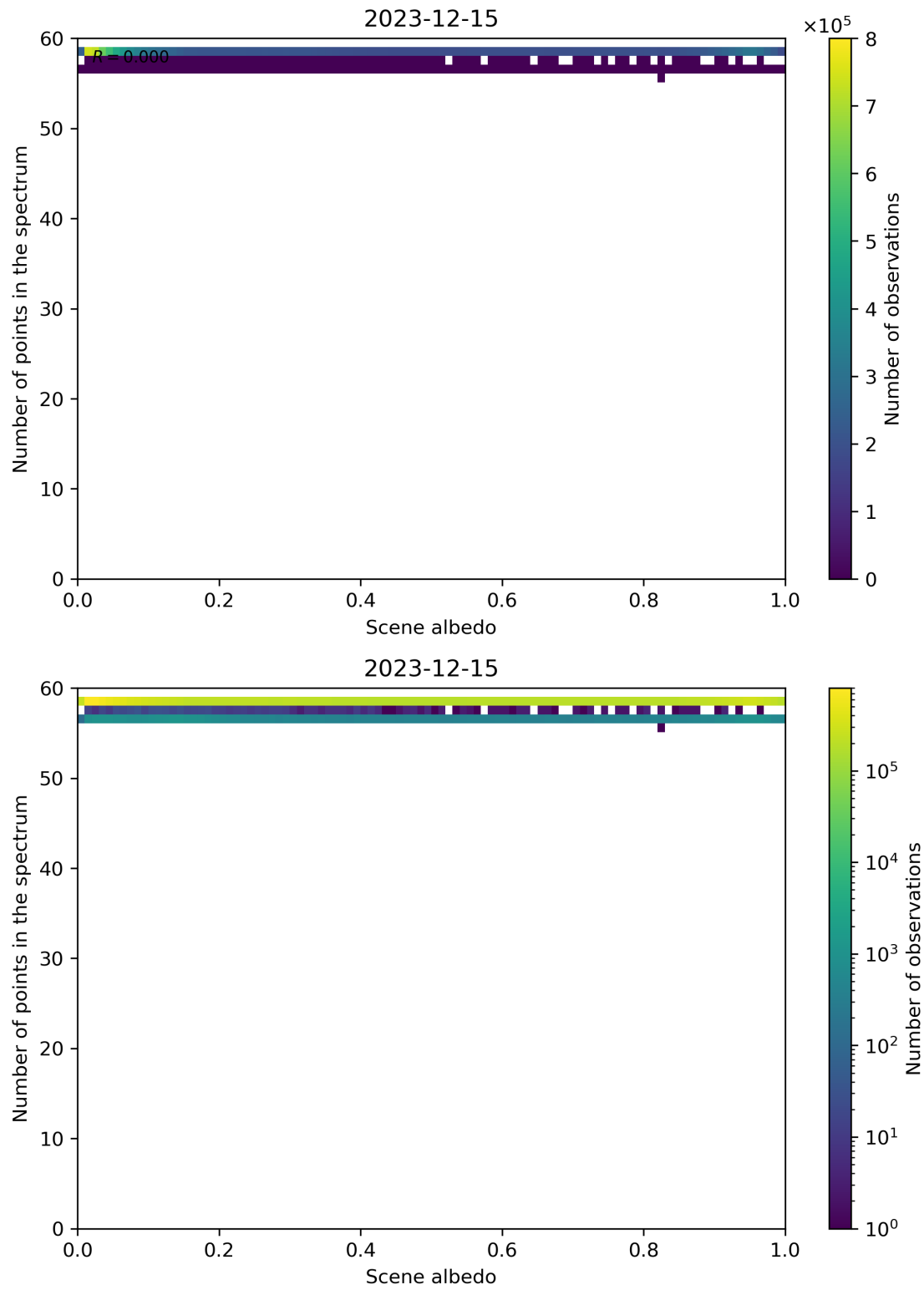
Figure 106: Scatter density plot of “Scene albedo” against “Number of points in the spectrum” for 2023-12-14 to 2023-12-16.
