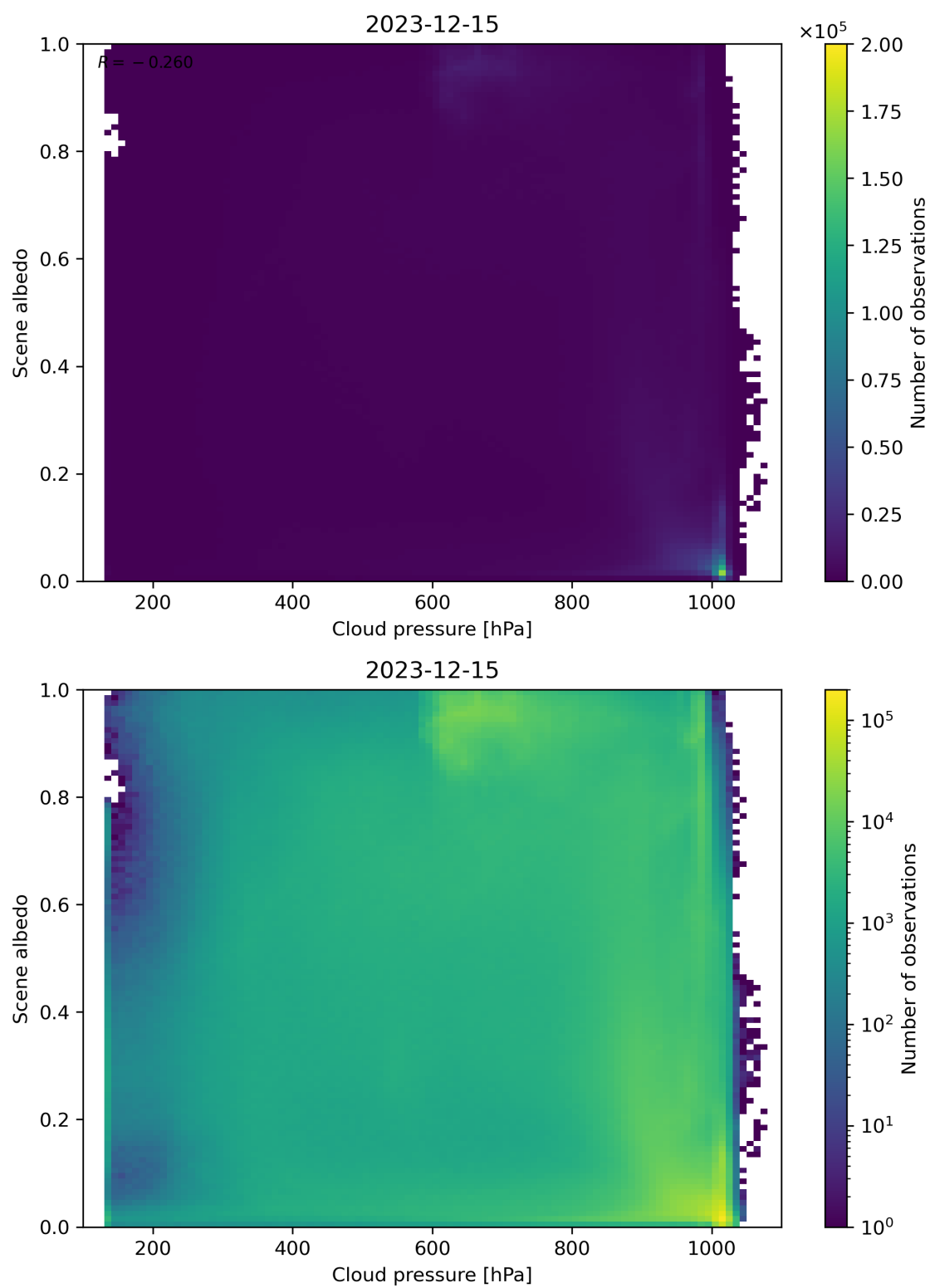
Figure 83: Scatter density plot of “Cloud pressure” against “Scene albedo” for 2023-12-14 to 2023-12-16.
