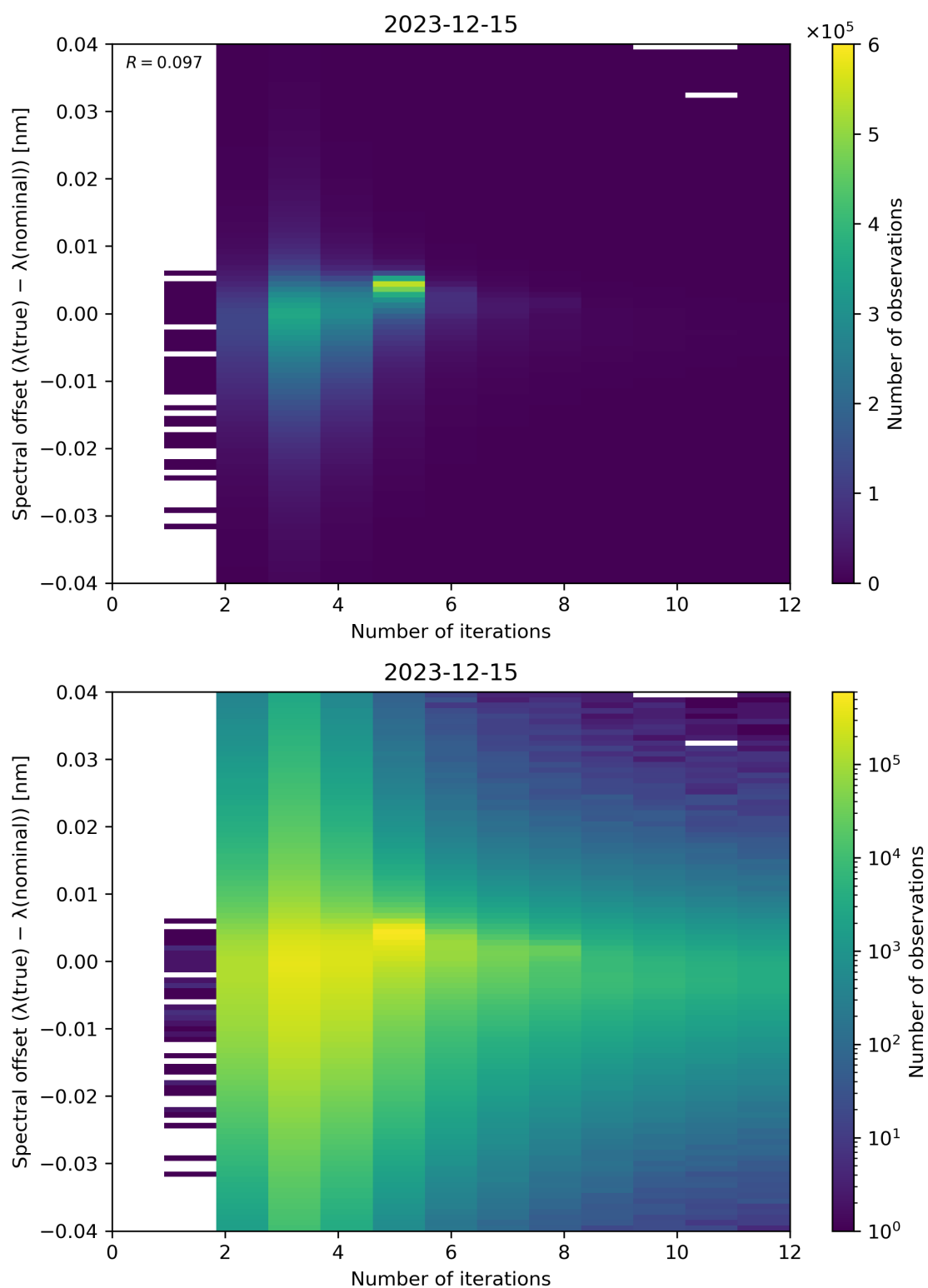
Figure 100: Scatter density plot of “Number of iterations” against “Spectral offset ( \lambda(\text{true}) - \lambda(\text{nominal}) )” for 2023-12-14 to 2023-12-16.
