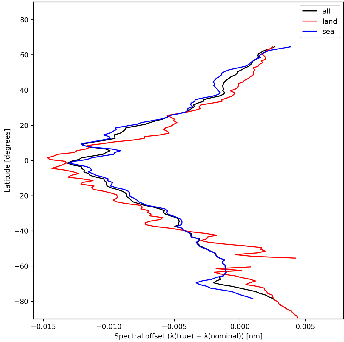
Figure 28: Zonal average of “Spectral offset ( \lambda(\text{true}) - \lambda(\text{nominal}) )” for 2023-12-14 to 2023-12-16.
