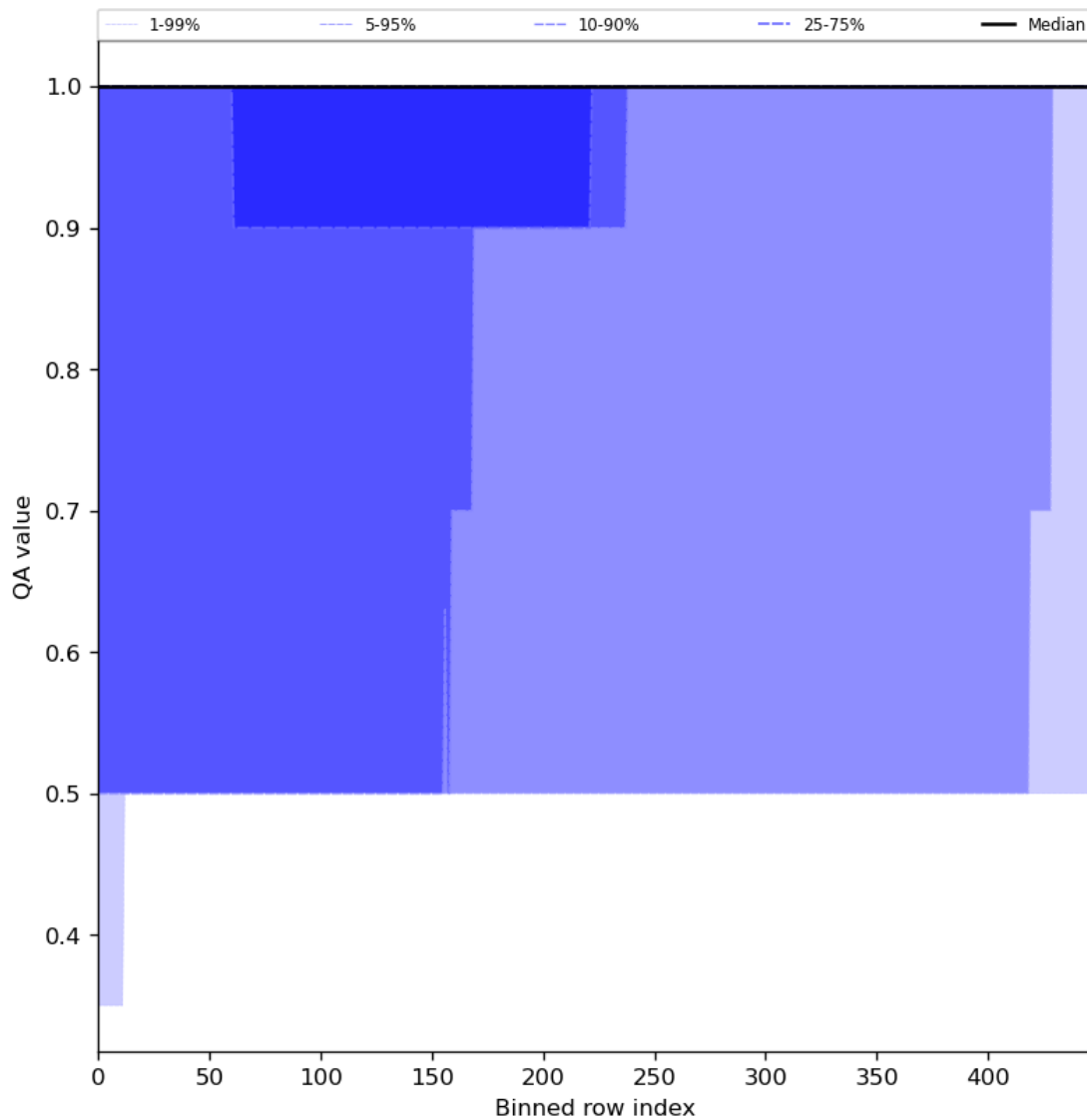
Figure 46: Along track statistics of “QA value” for 2023-12-14 to 2023-12-16
