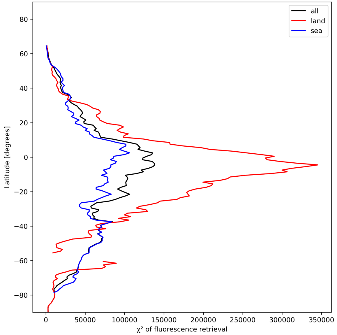
Figure 25: Zonal average of “ \chi^2 of fluorescence retrieval” for 2023-12-14 to 2023-12-16.
