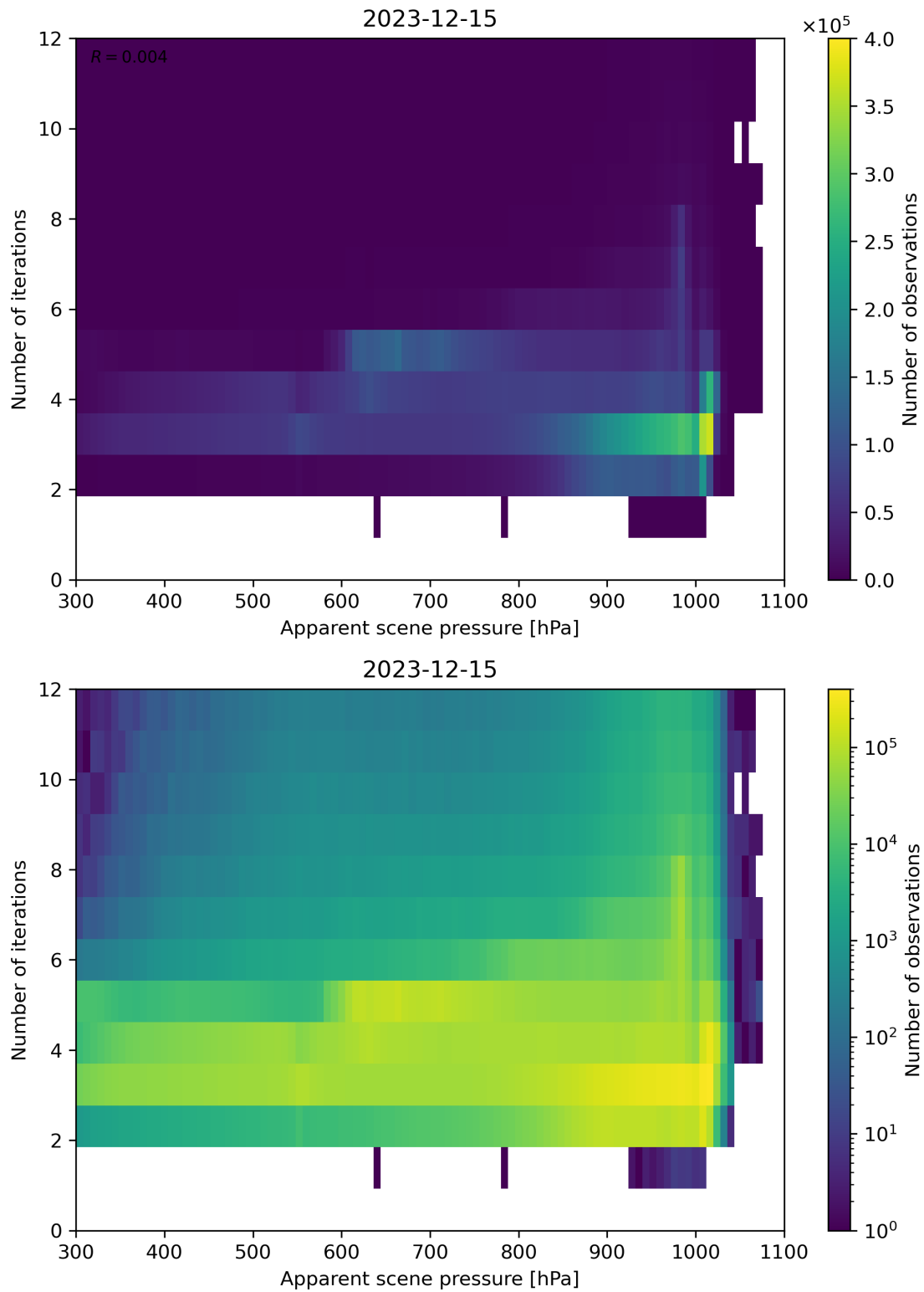
Figure 65: Scatter density plot of “Apparent scene pressure” against “Number of iterations” for 2023-12-14 to 2023-12-16.
