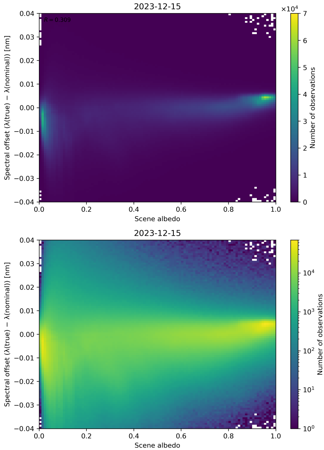
Figure 107: Scatter density plot of “Scene albedo” against “Spectral offset ( \lambda(\text{true}) - \lambda(\text{nominal}) )” for 2023-12-14 to 2023-12-16.
