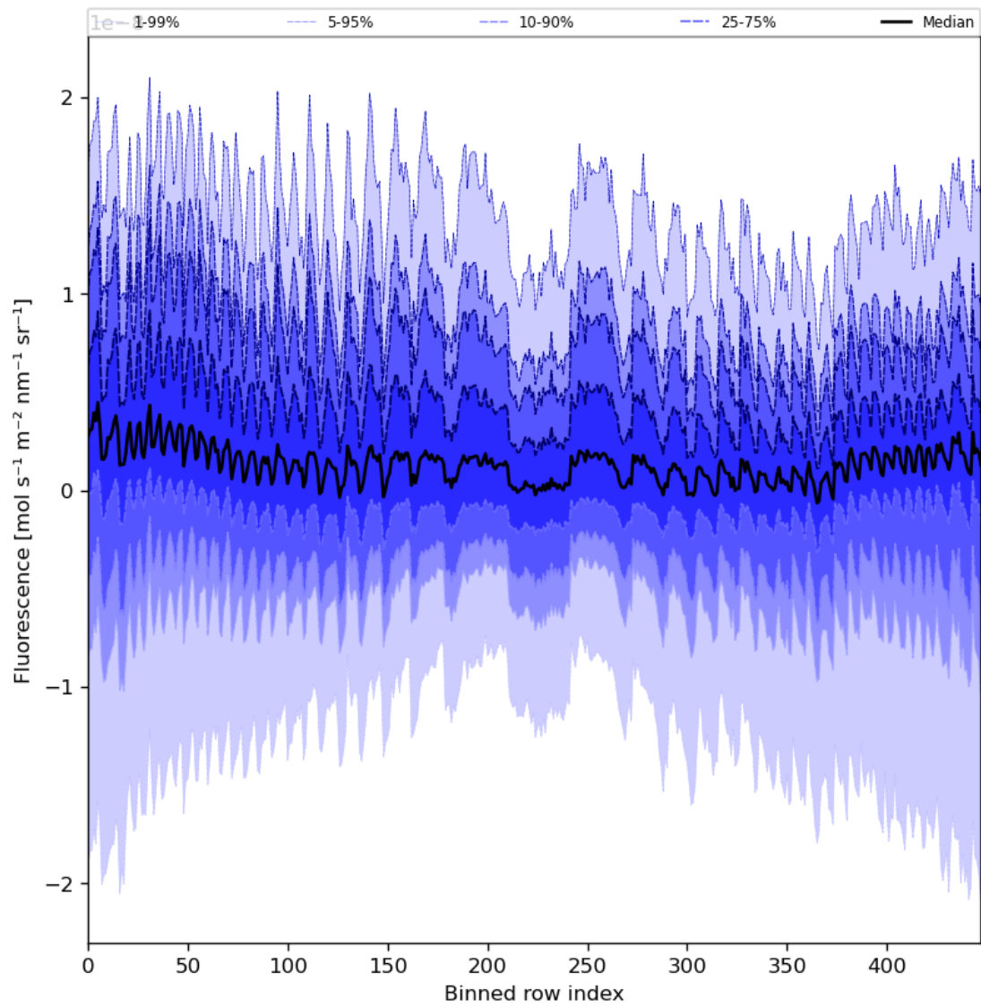
Figure 57: Along track statistics of “Fluorescence” for 2023-12-14 to 2023-12-16
