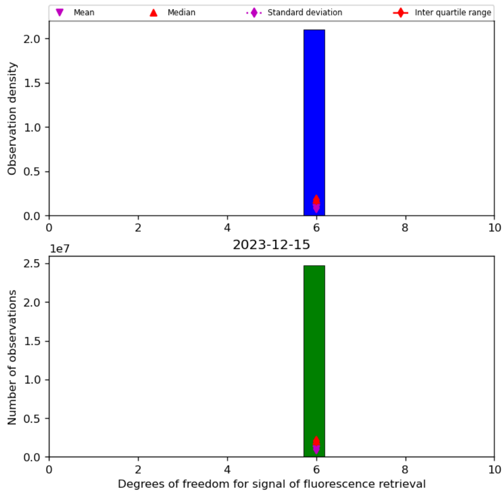
Figure 43: Histogram of “Degrees of freedom for signal of fluorescence retrieval” for 2023-12-14 to 2023-12-16
