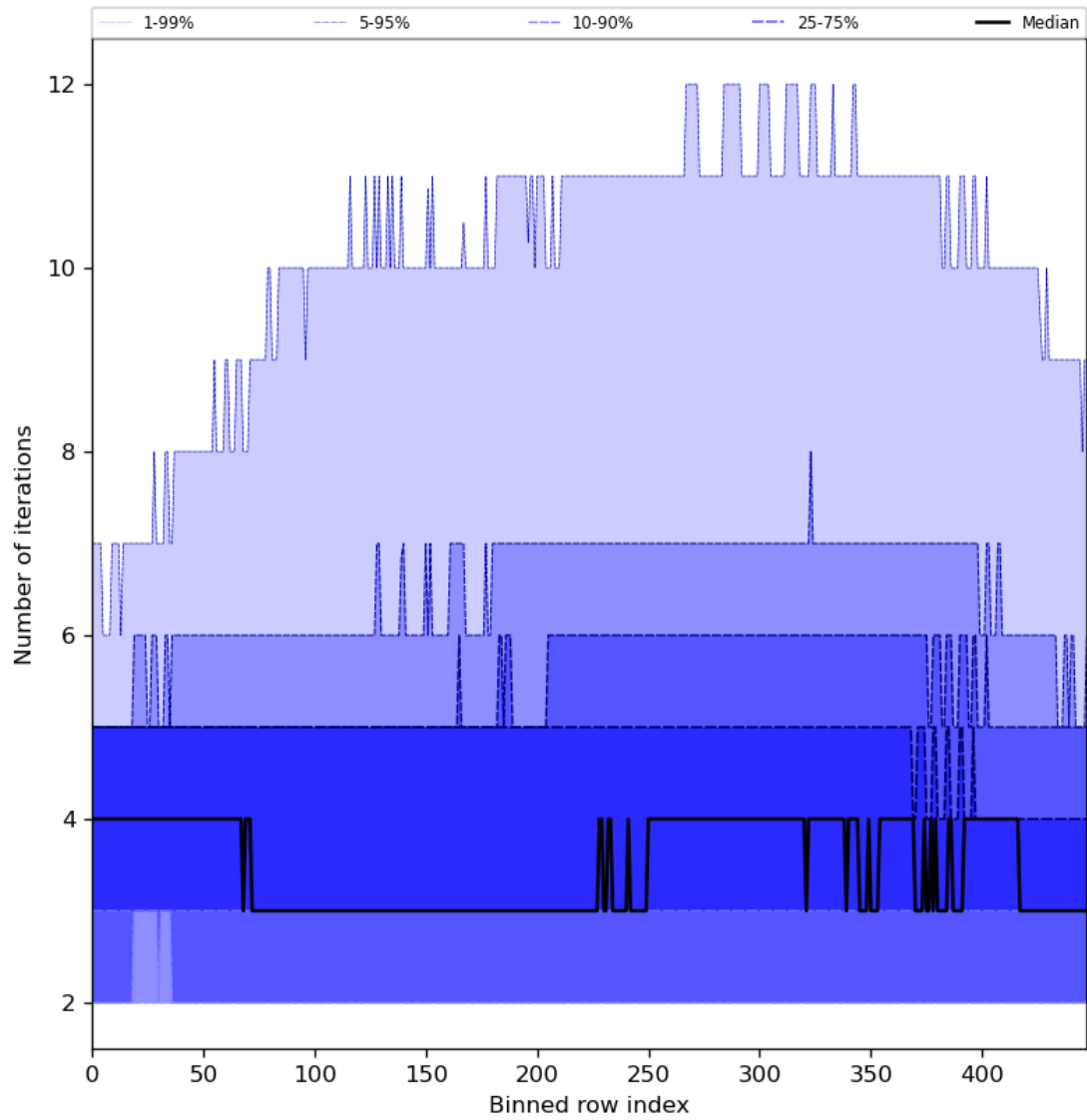
Figure 56: Along track statistics of “Number of iterations” for 2023-12-14 to 2023-12-16
