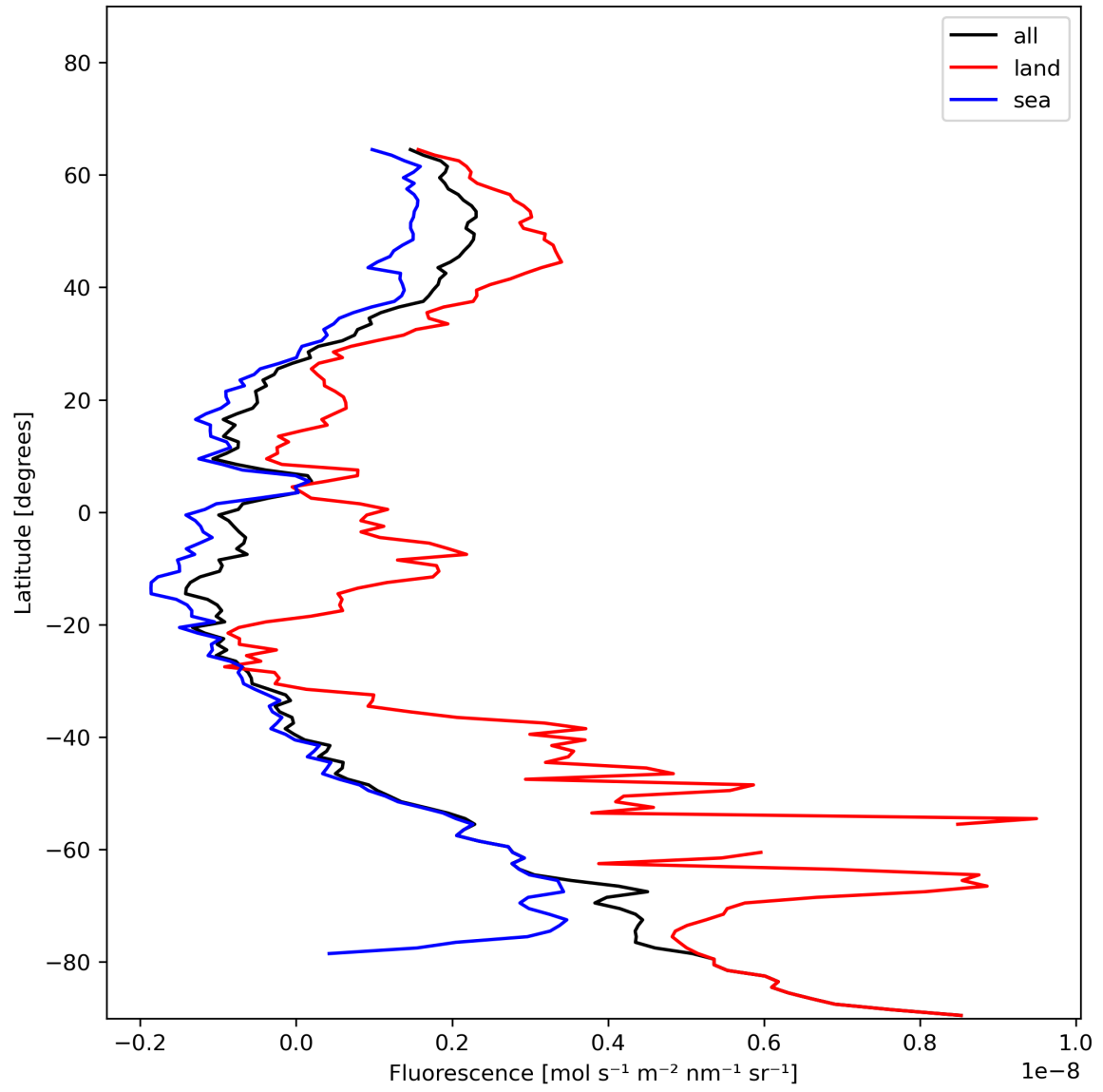
Figure 23: Zonal average of “Fluorescence” for 2023-12-14 to 2023-12-16.
