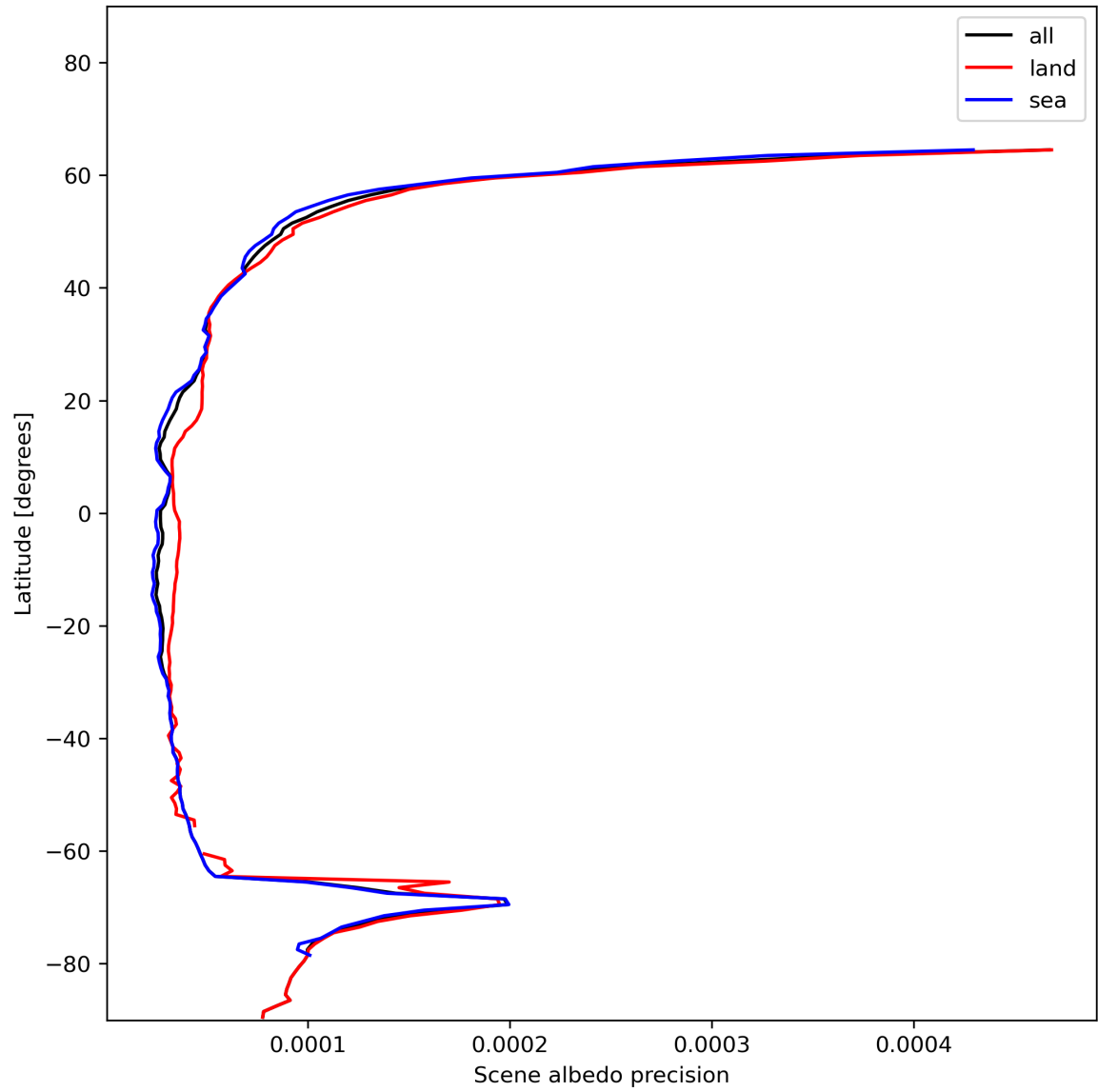
Figure 18: Zonal average of “Scene albedo precision” for 2023-12-14 to 2023-12-16.
