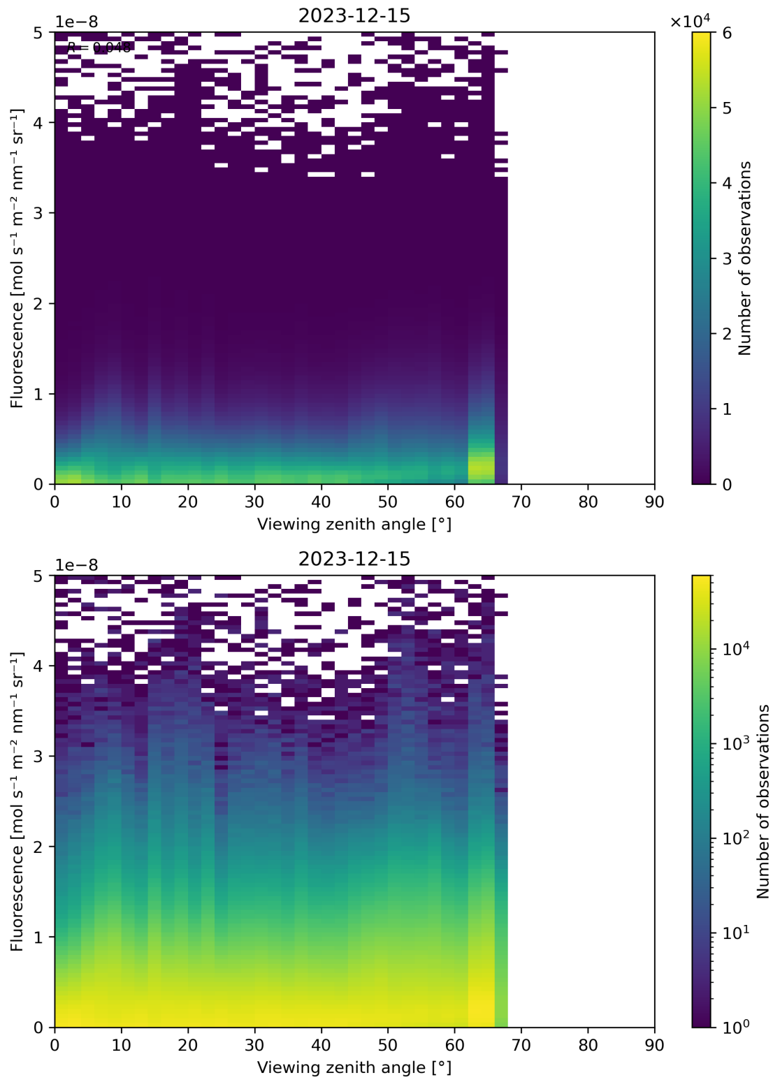
Figure 122: Scatter density plot of “Viewing zenith angle” against “Fluorescence” for 2023-12-14 to 2023-12-16.
