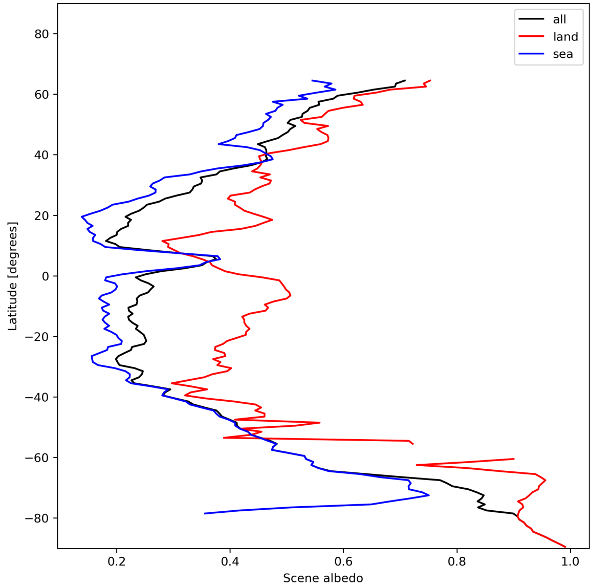
Figure 17: Zonal average of “Scene albedo” for 2023-12-14 to 2023-12-16.
