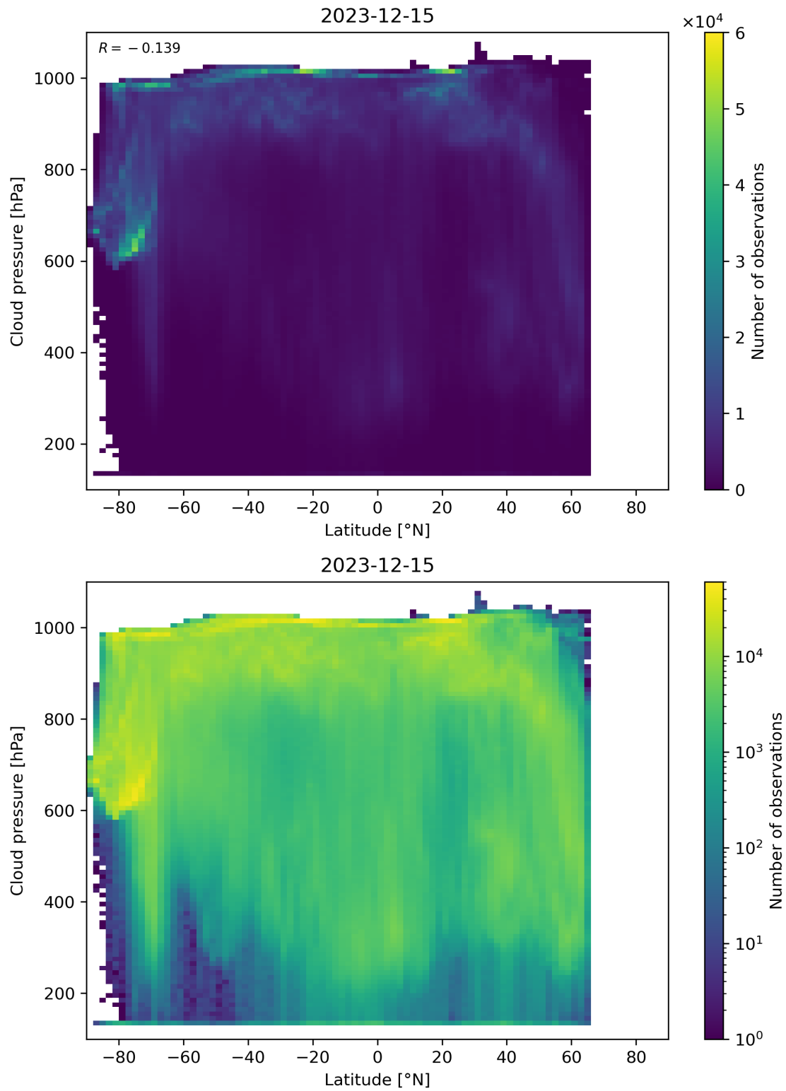
Figure 91: Scatter density plot of “Latitude” against “Cloud pressure” for 2023-12-14 to 2023-12-16.
