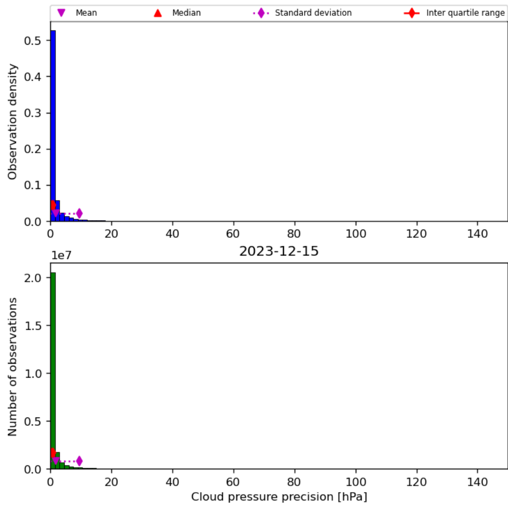
Figure 31: Histogram of “Cloud pressure precision” for 2023-12-14 to 2023-12-16
