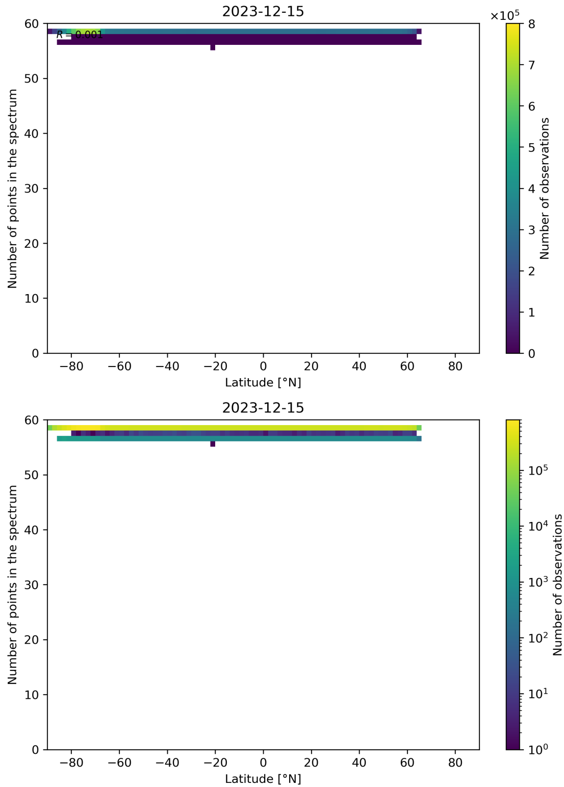
Figure 94: Scatter density plot of “Latitude” against “Number of points in the spectrum” for 2023-12-14 to 2023-12-16.
