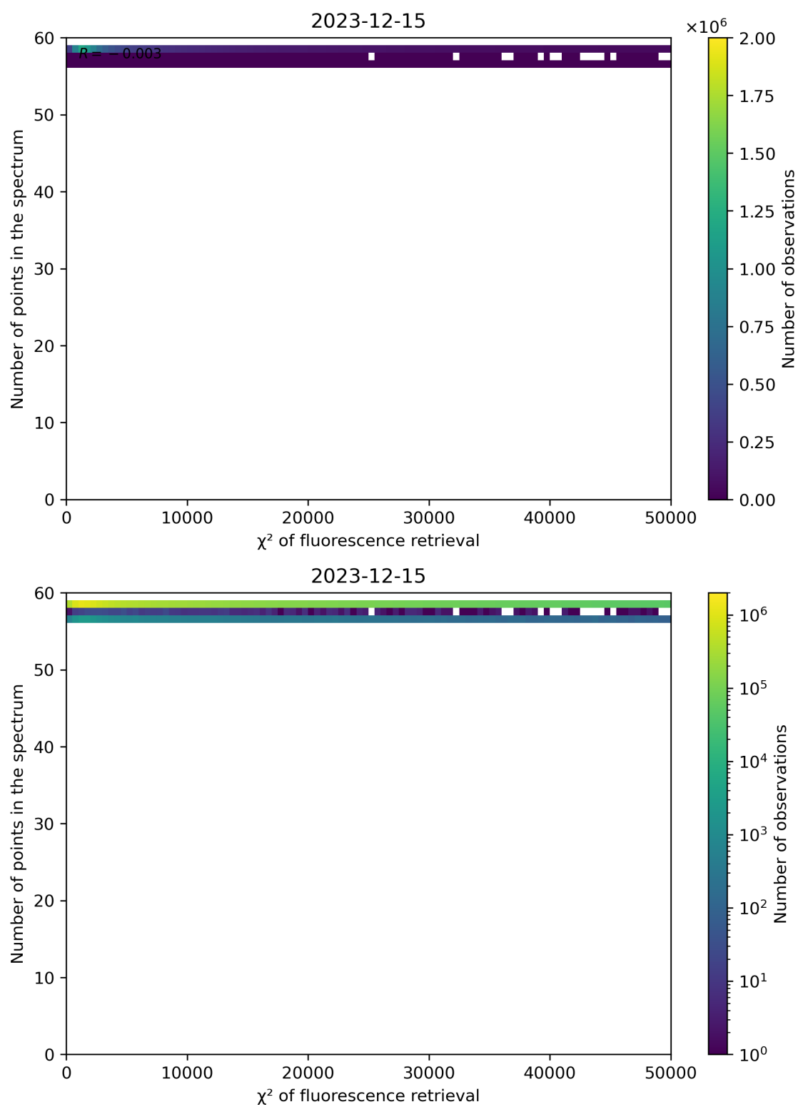
Figure 68: Scatter density plot of " \chi^2 of fluorescence retrieval" against "Number of points in the spectrum" for 2023-12-14 to 2023-12-16.
