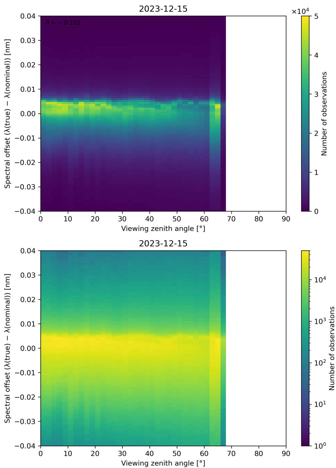
Figure 128: Scatter density plot of “Viewing zenith angle” against “Spectral offset ( \lambda(\text{true}) - \lambda(\text{nominal}) )” for 2023-12-14 to 2023-12-16.
