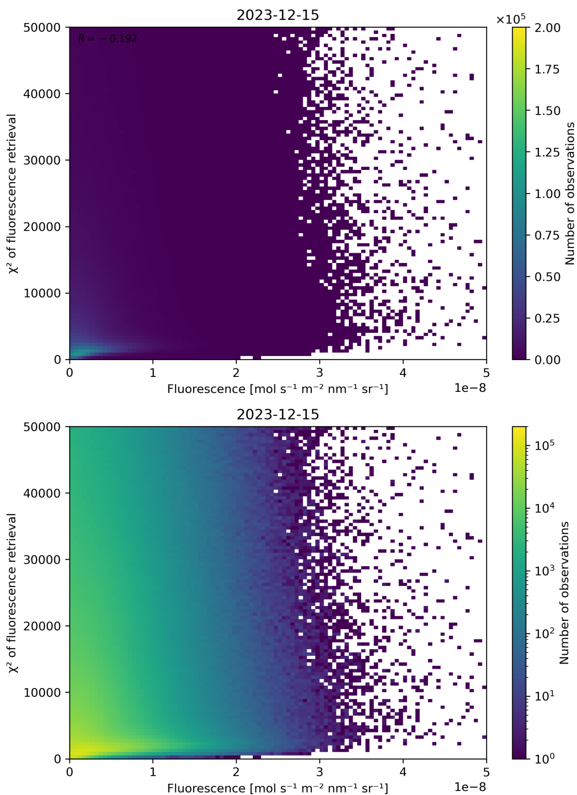
Figure 85: Scatter density plot of “Fluorescence” against “ \chi^2 of fluorescence retrieval” for 2023-12-14 to 2023-12-16.
