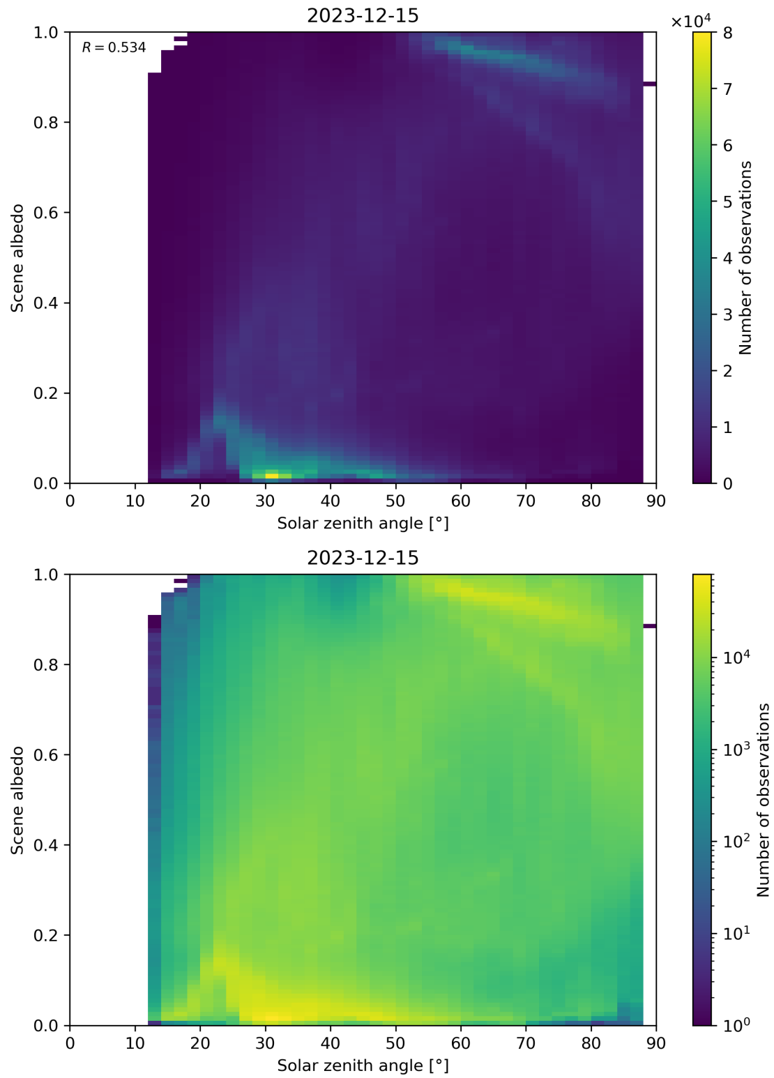
Figure 116: Scatter density plot of “Solar zenith angle” against “Scene albedo” for 2023-12-14 to 2023-12-16.
