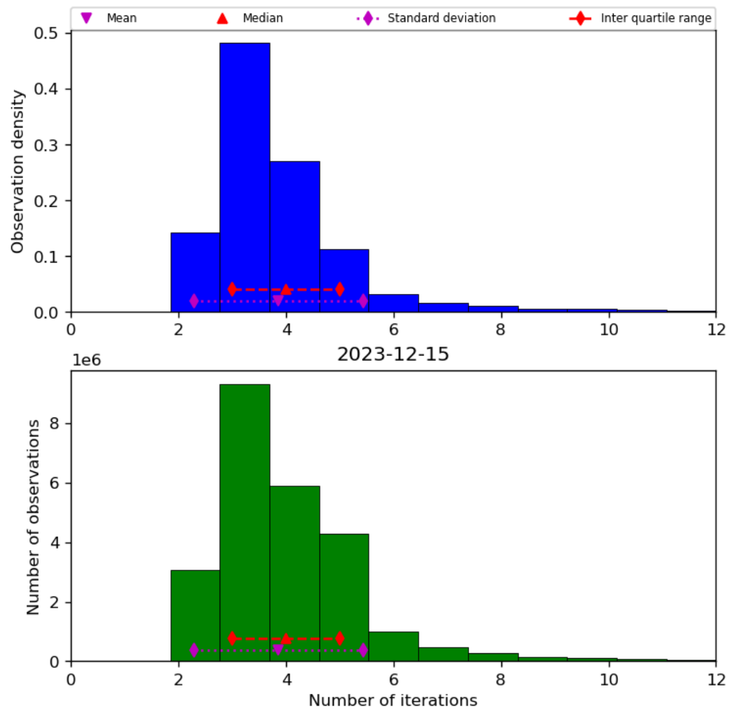
Figure 39: Histogram of “Number of iterations” for 2023-12-14 to 2023-12-16
