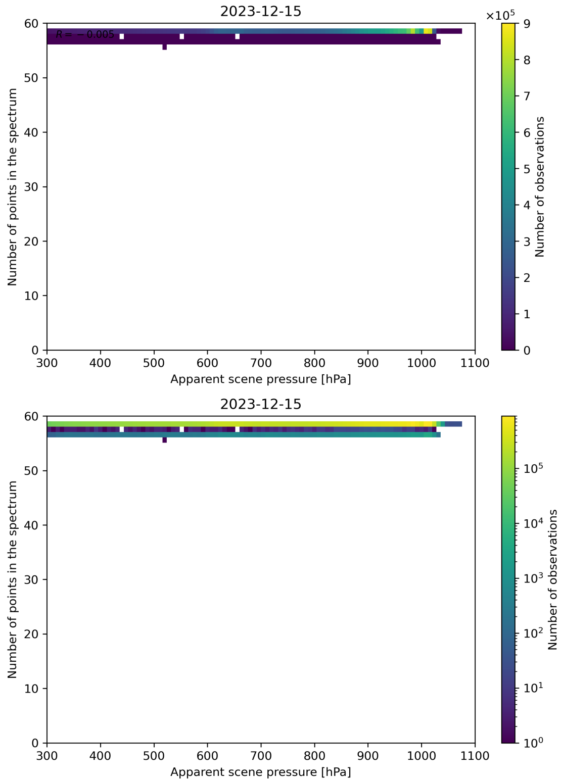
Figure 66: Scatter density plot of “Apparent scene pressure” against “Number of points in the spectrum” for 2023-12-14 to 2023-12-16.
