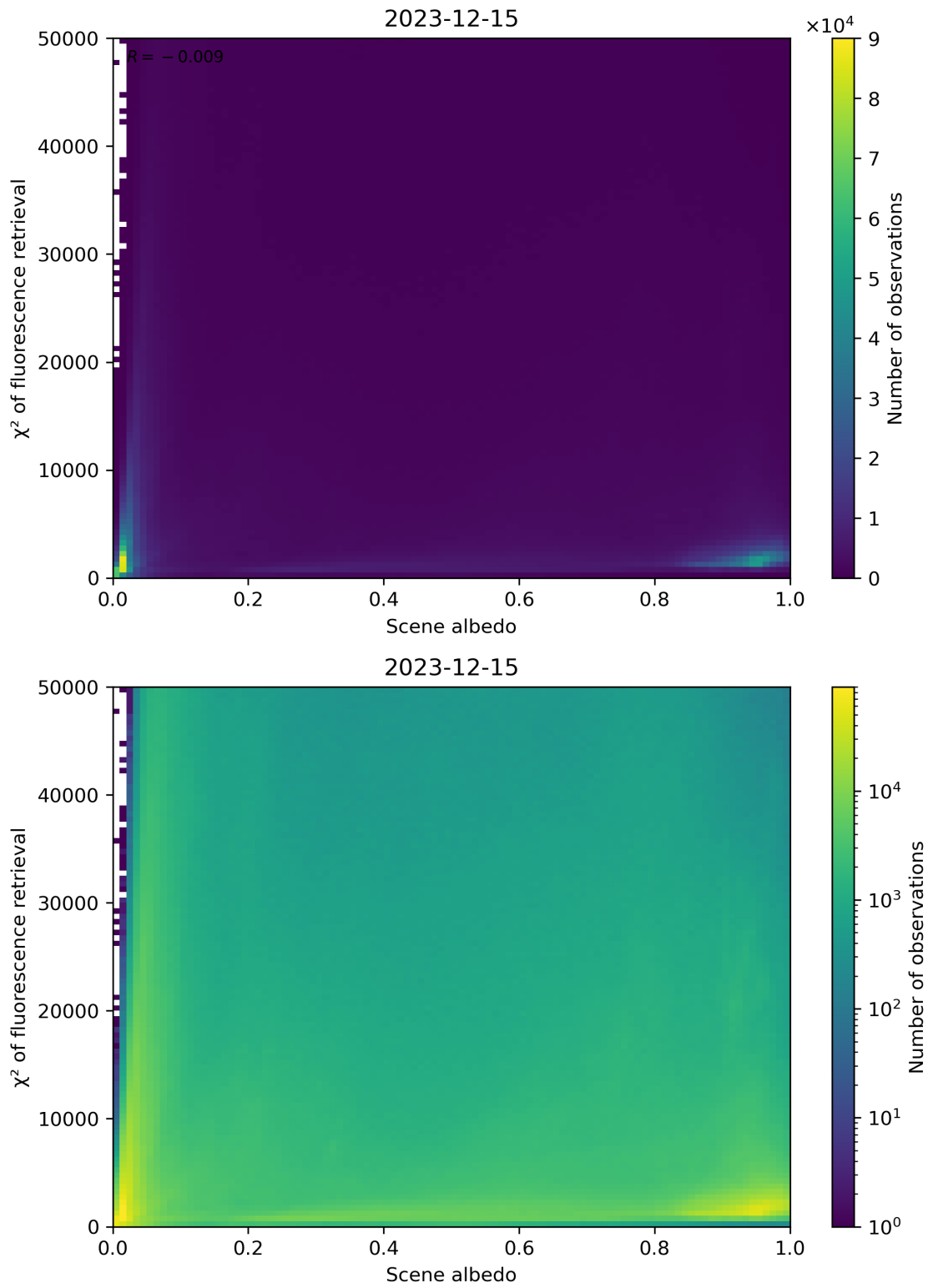
Figure 103: Scatter density plot of “Scene albedo” against “ \chi^2 of fluorescence retrieval” for 2023-12-14 to 2023-12-16.
