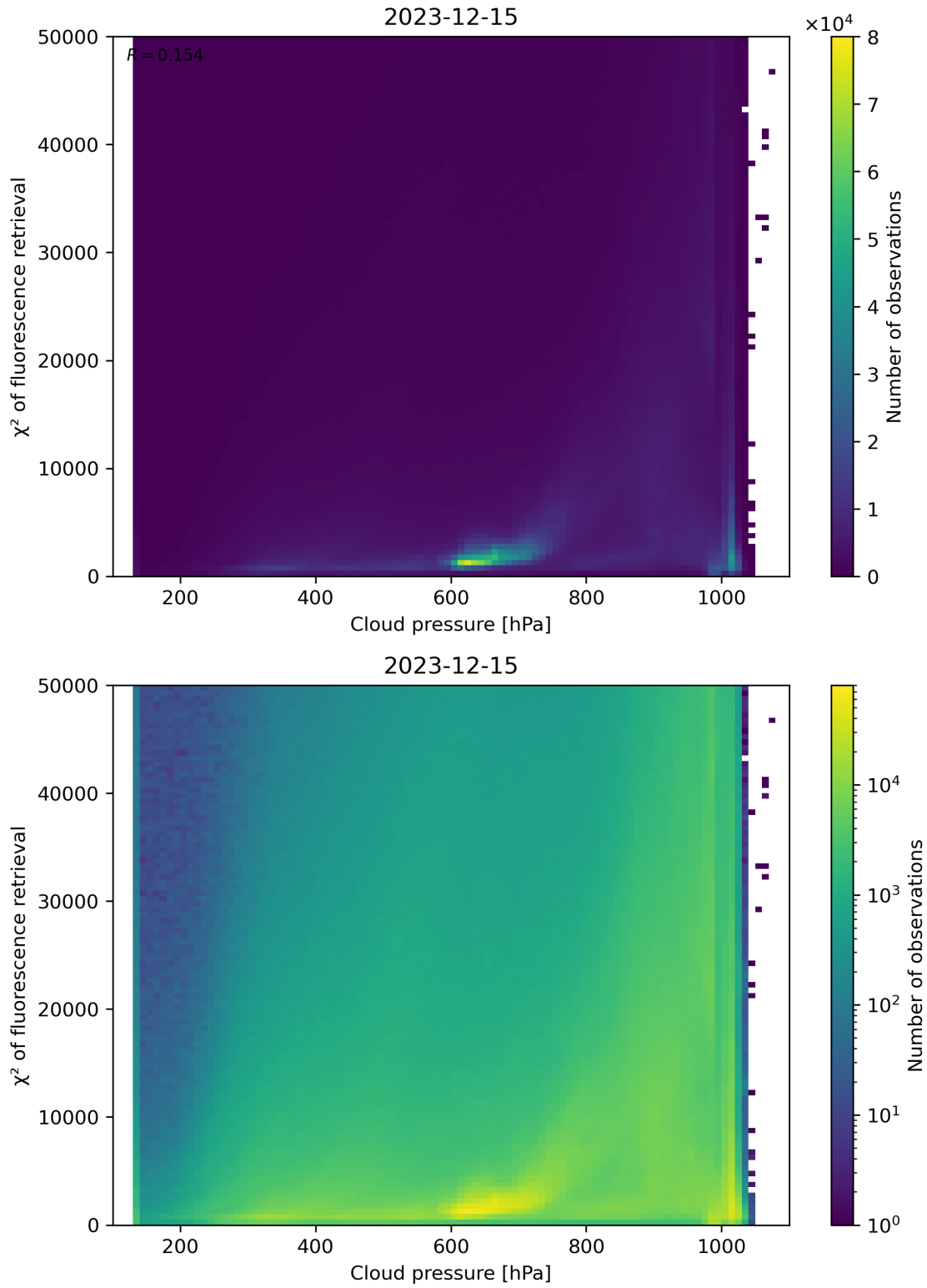
Figure 78: Scatter density plot of “Cloud pressure” against “ \chi^2 of fluorescence retrieval” for 2023-12-14 to 2023-12-16.
