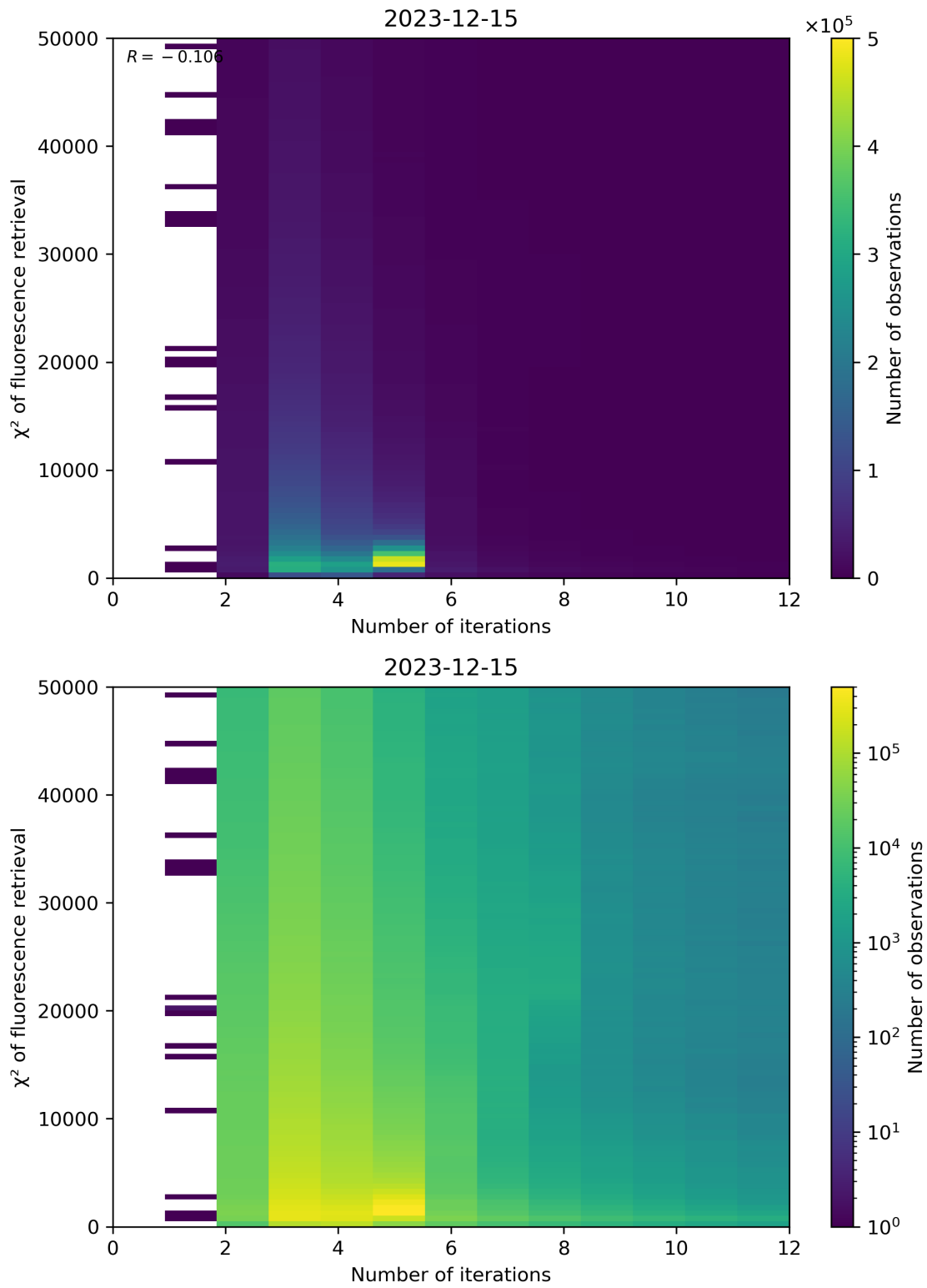
Figure 97: Scatter density plot of “Number of iterations” against “ \chi^2 of fluorescence retrieval” for 2023-12-14 to 2023-12-16.
