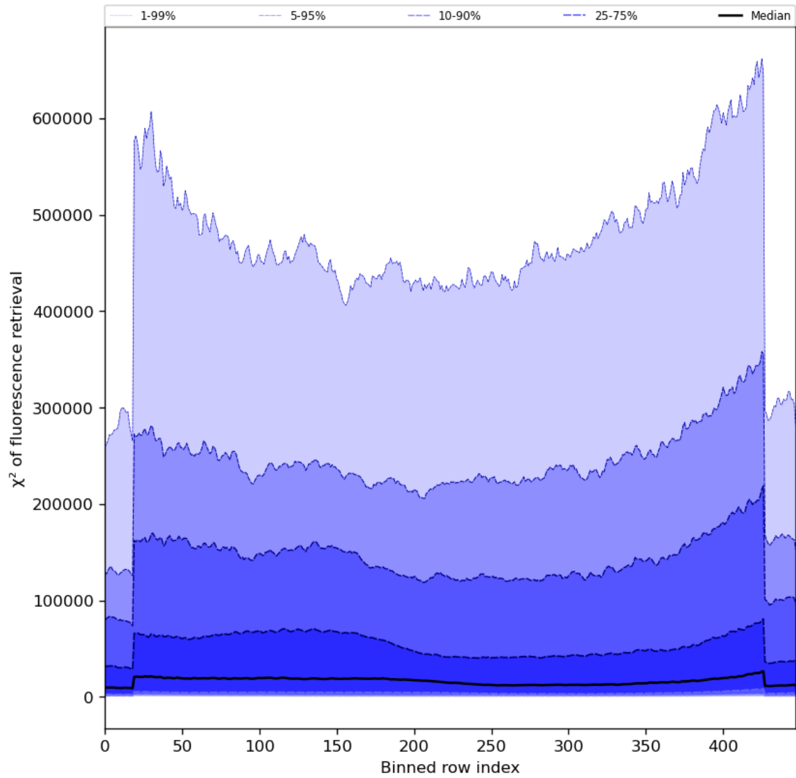
Figure 59: Along track statistics of “ \chi^2 of fluorescence retrieval” for 2023-12-14 to 2023-12-16
