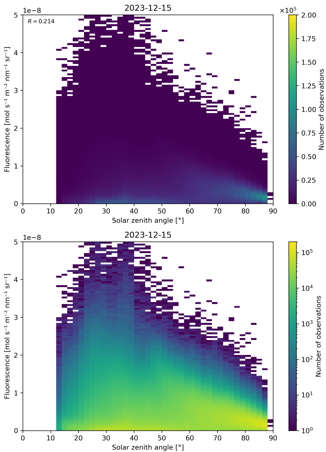
Figure 112: Scatter density plot of “Solar zenith angle” against “Fluorescence” for 2023-12-14 to 2023-12-16.
