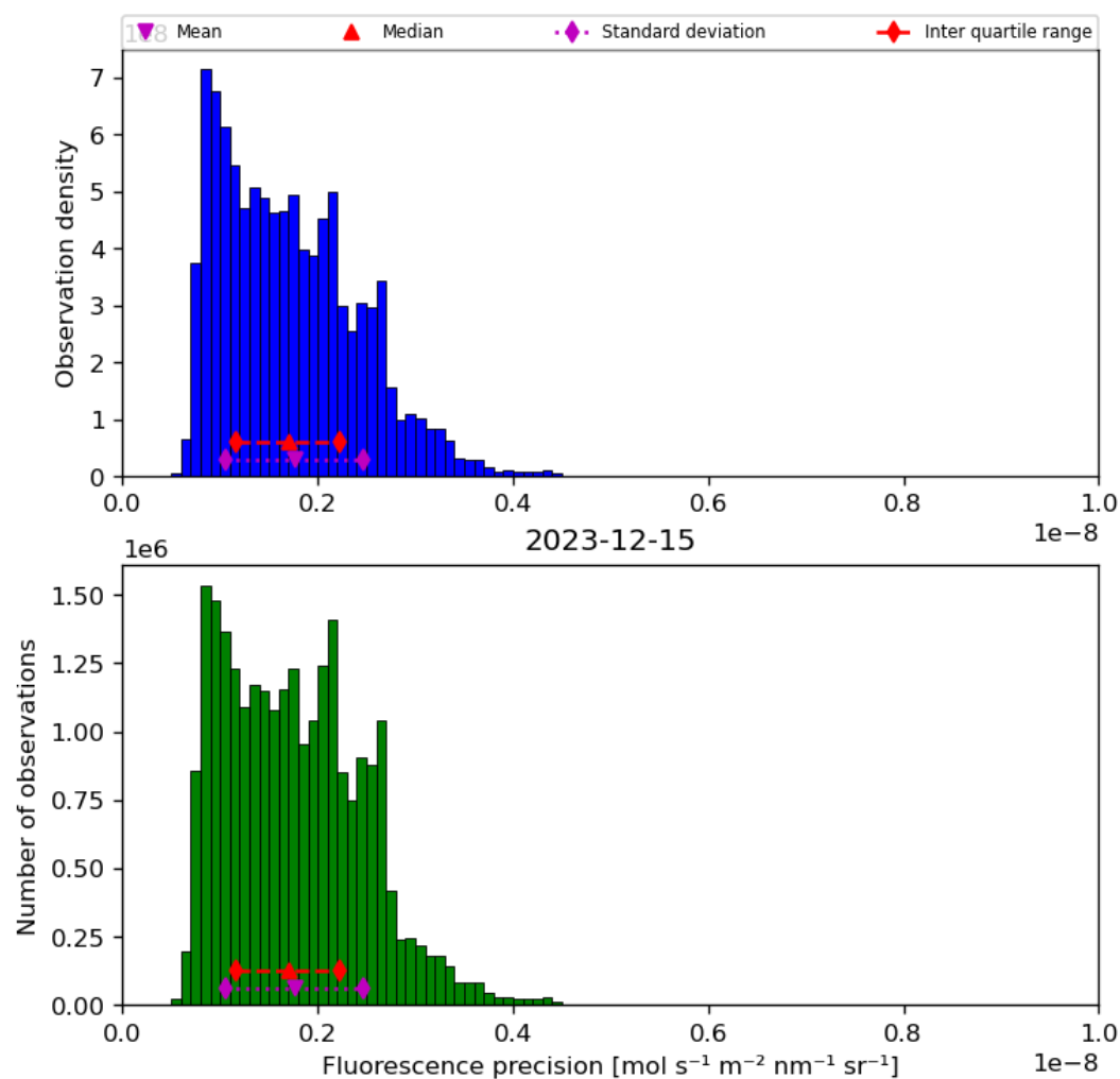
Figure 41: Histogram of “Fluorescence precision” for 2023-12-14 to 2023-12-16
