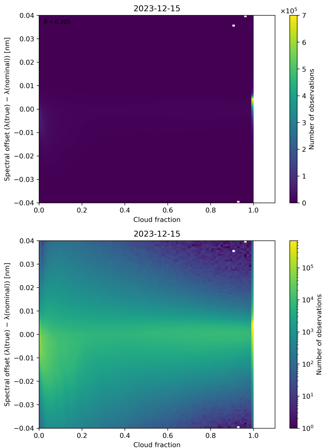
Figure 76: Scatter density plot of “Cloud fraction” against “Spectral offset ( \lambda(\text{true}) - \lambda(\text{nominal}) )” for 2023-12-14 to 2023-12-16.
