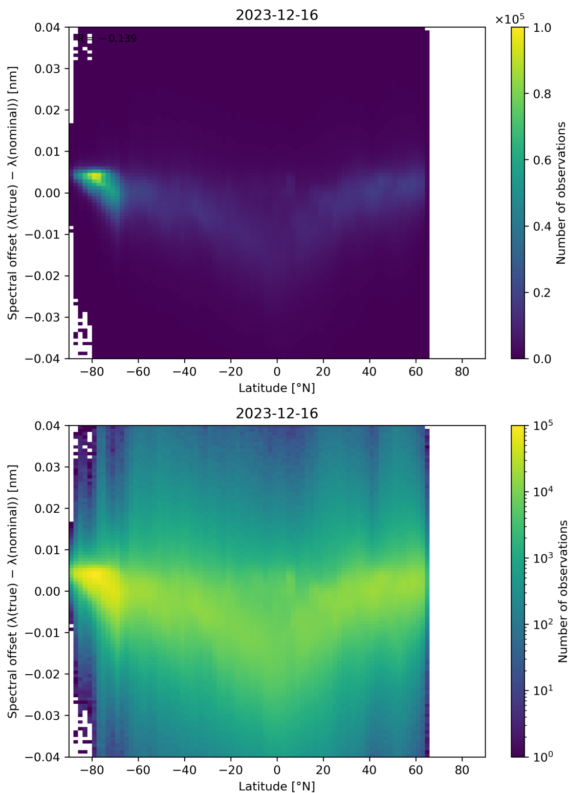
Figure 96: Scatter density plot of “Latitude” against “Spectral offset ( \lambda(\text{true}) - \lambda(\text{nominal}) )” for 2023-12-15 to 2023-12-17.
