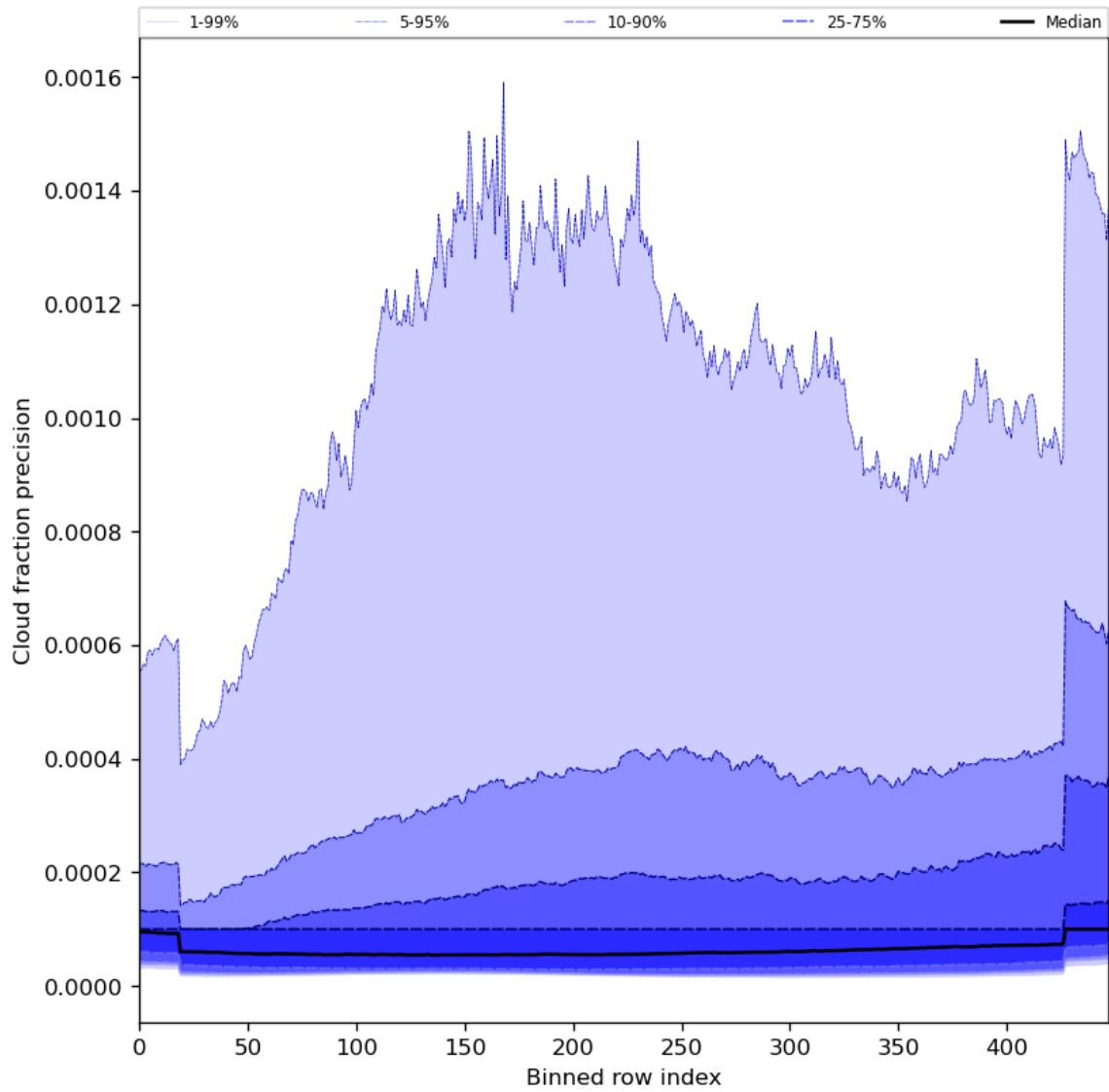
Figure 50: Along track statistics of “Cloud fraction precision” for 2023-12-15 to 2023-12-17
