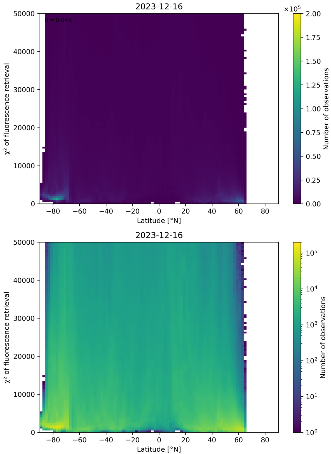
Figure 89: Scatter density plot of “Latitude” against “ \chi^2 of fluorescence retrieval” for 2023-12-15 to 2023-12-17.
