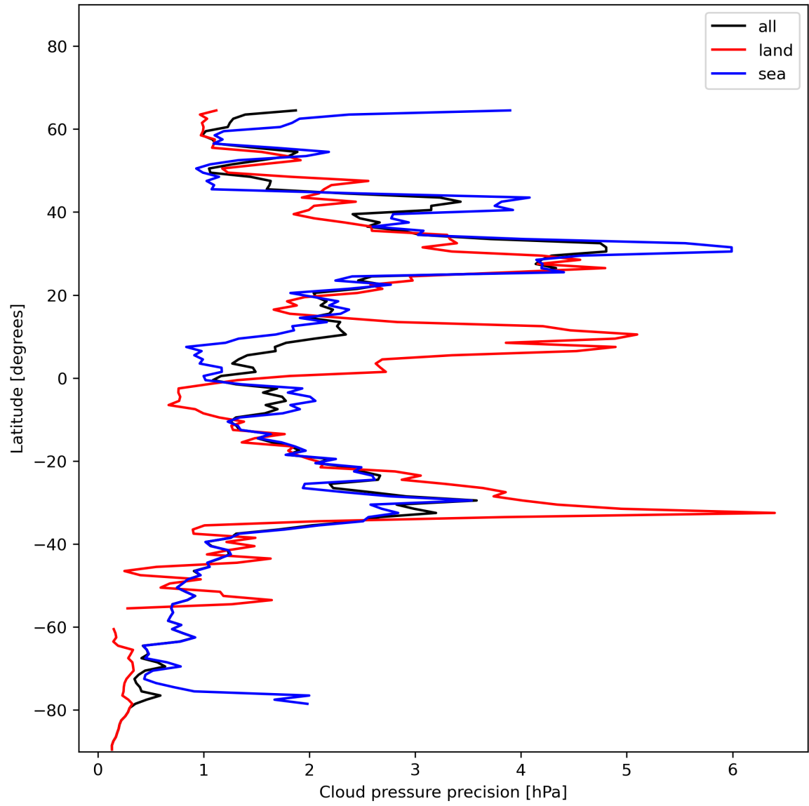
Figure 14: Zonal average of “Cloud pressure precision” for 2023-12-15 to 2023-12-17.
