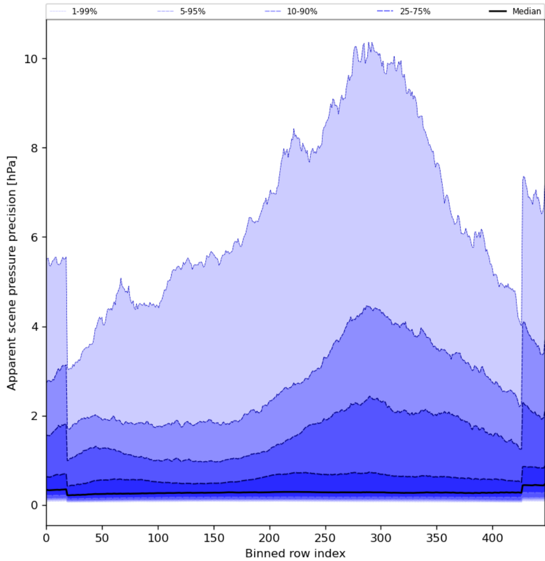
Figure 54: Along track statistics of “Apparent scene pressure precision” for 2023-12-15 to 2023-12-17
