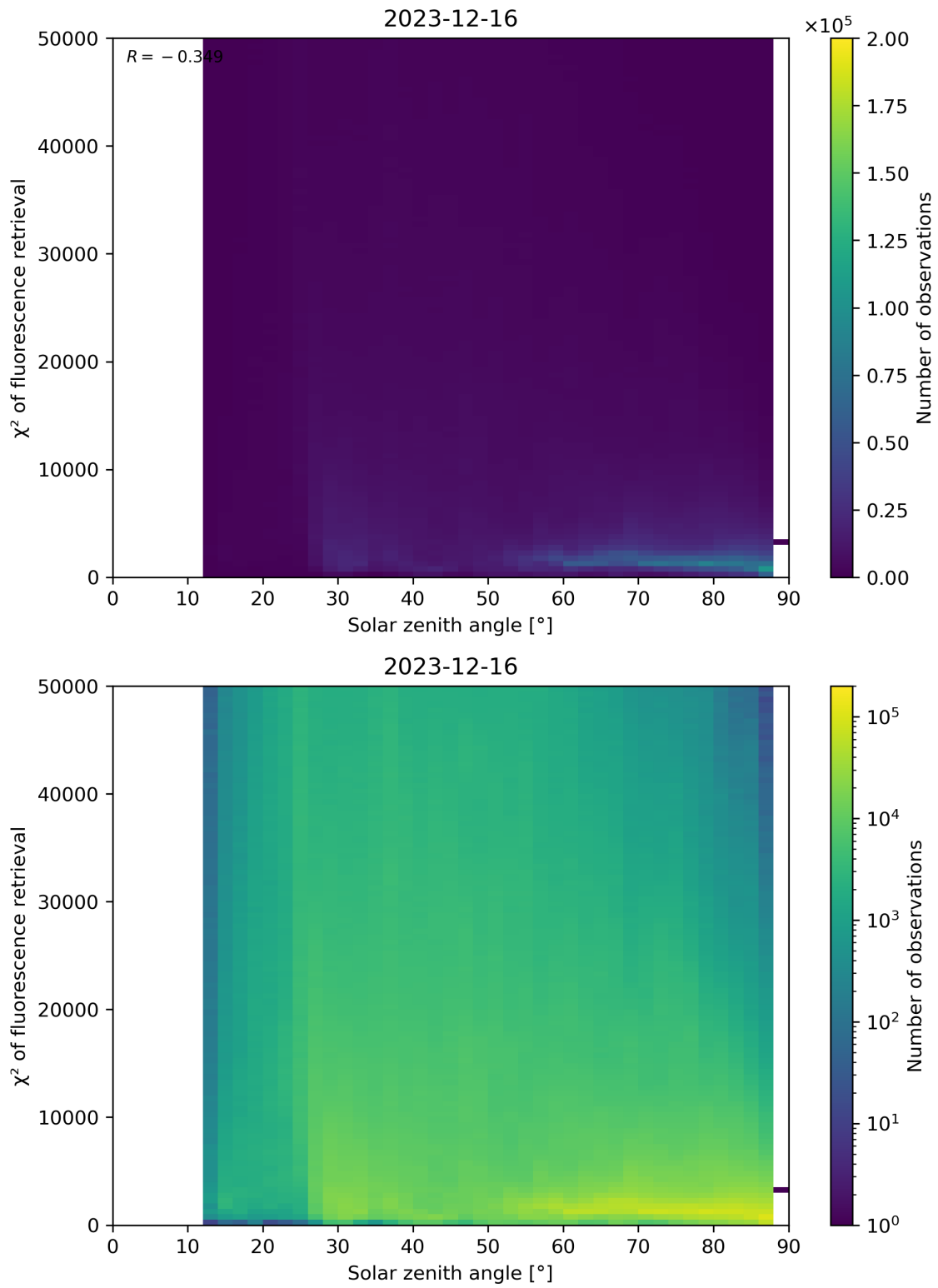
Figure 109: Scatter density plot of “Solar zenith angle” against “ \chi^2 of fluorescence retrieval” for 2023-12-15 to 2023-12-17.
