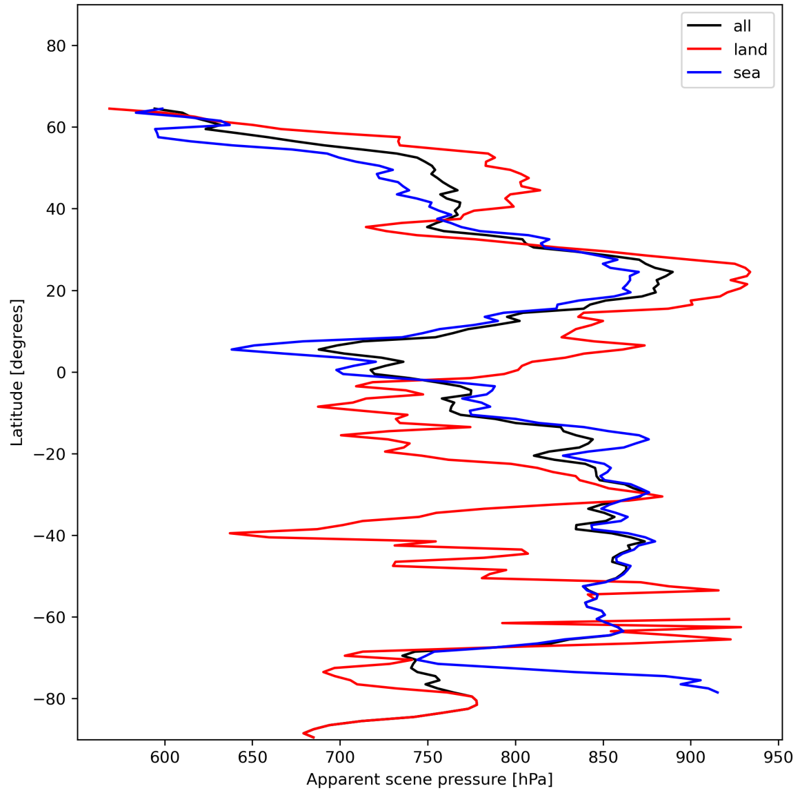
Figure 19: Zonal average of “Apparent scene pressure” for 2023-12-15 to 2023-12-17.
