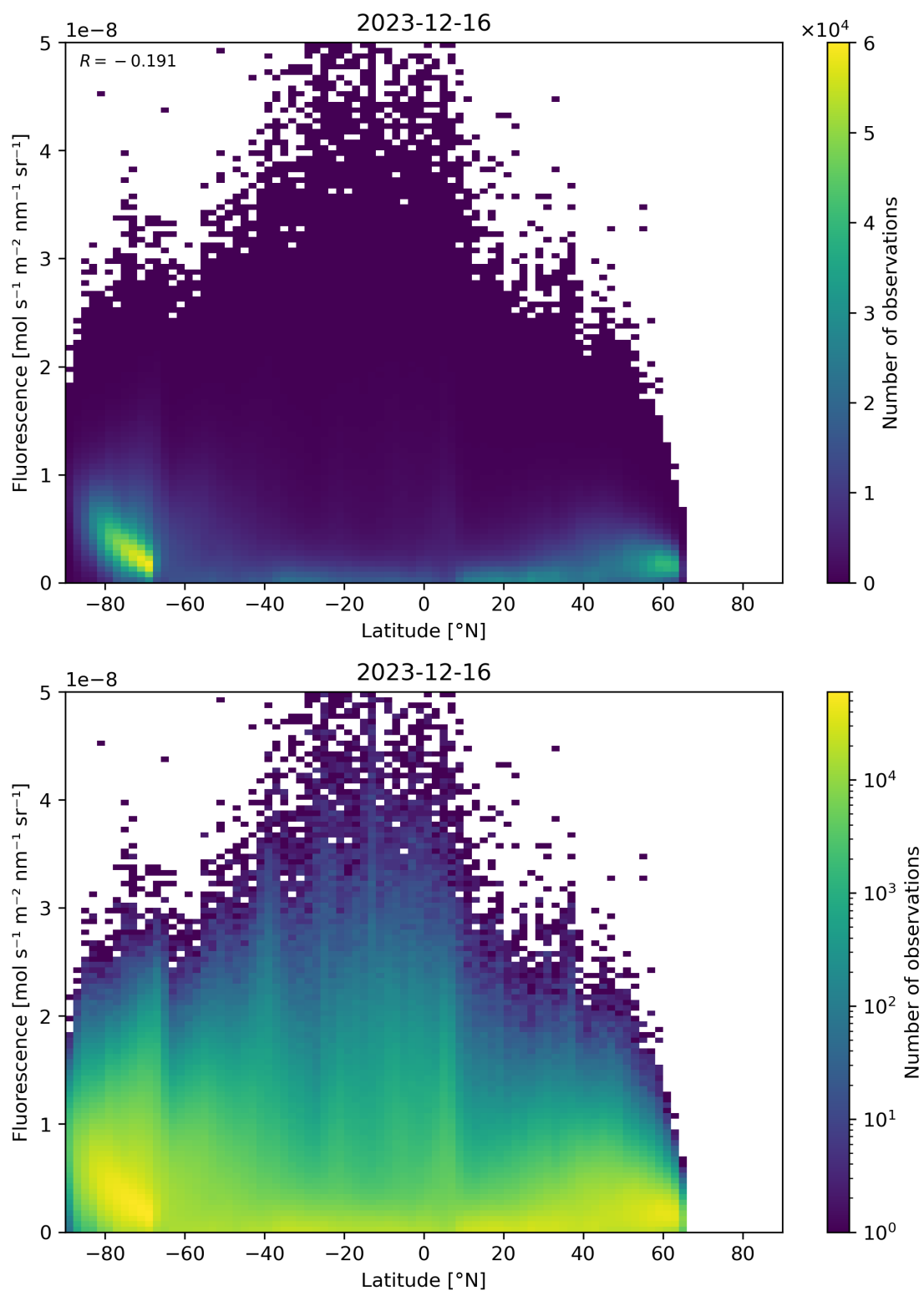
Figure 92: Scatter density plot of “Latitude” against “Fluorescence” for 2023-12-15 to 2023-12-17.
