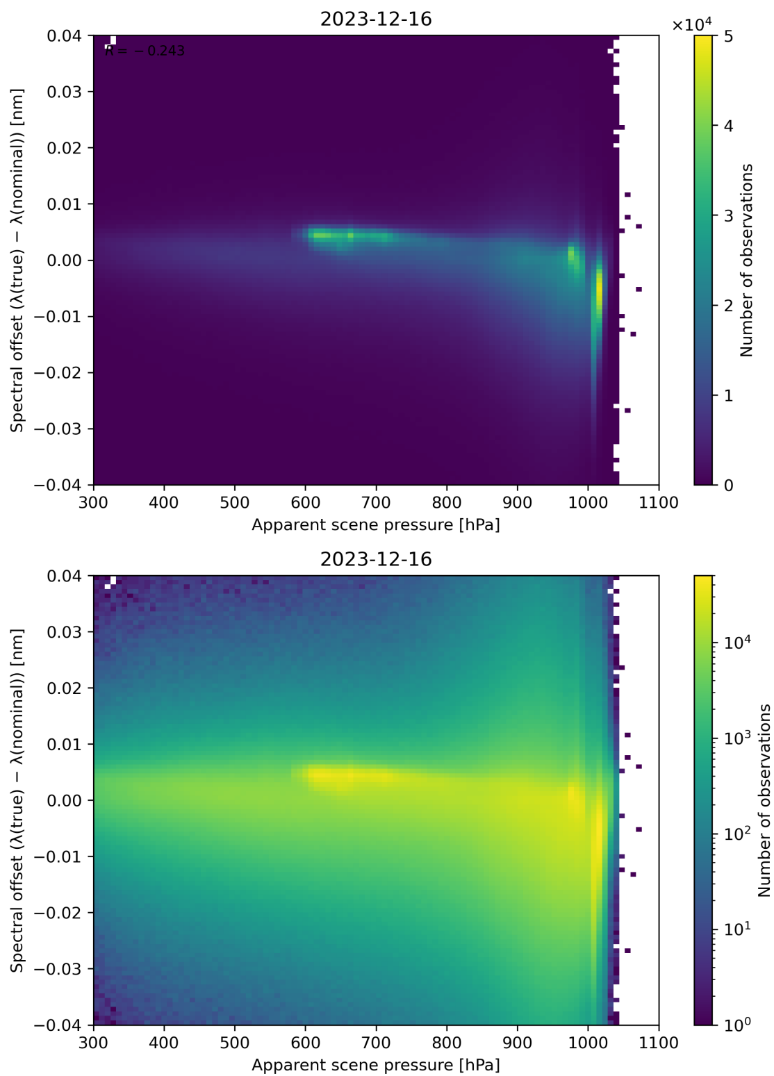
Figure 67: Scatter density plot of “Apparent scene pressure” against “Spectral offset ( \lambda(\text{true}) - \lambda(\text{nominal}) )” for 2023-12-15 to 2023-12-17.
