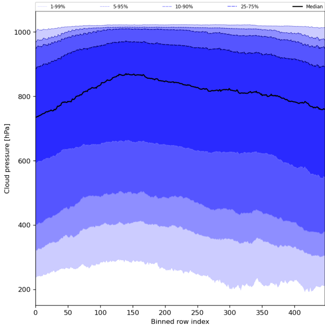
Figure 47: Along track statistics of “Cloud pressure” for 2023-12-15 to 2023-12-17
