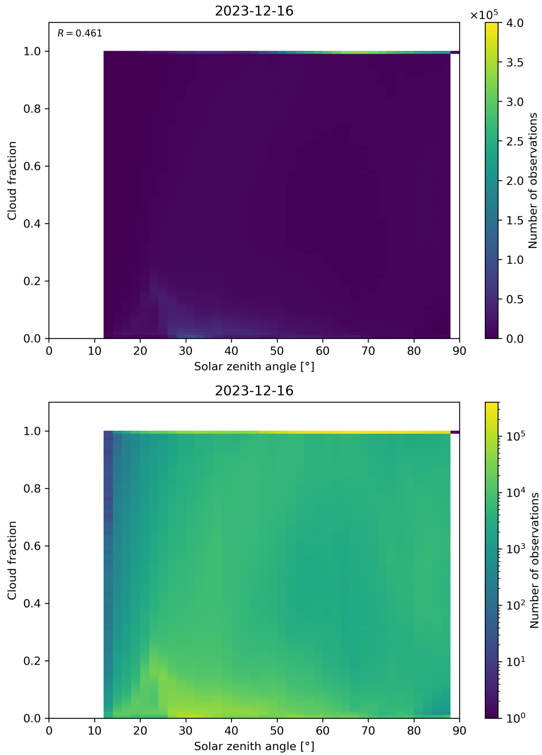
Figure 110: Scatter density plot of “Solar zenith angle” against “Cloud fraction” for 2023-12-15 to 2023-12-17.
