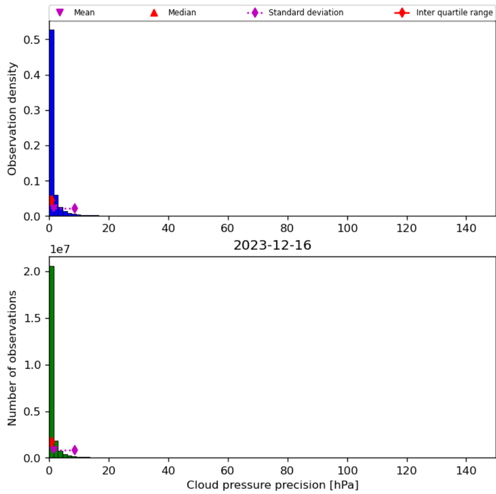
Figure 31: Histogram of “Cloud pressure precision” for 2023-12-15 to 2023-12-17
