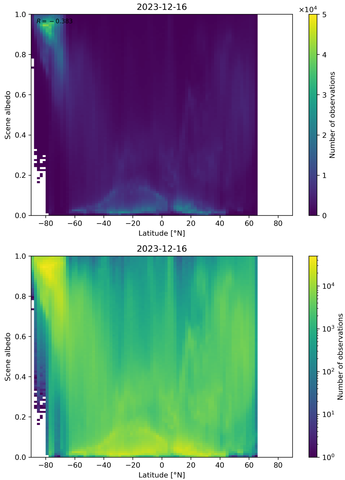
Figure 95: Scatter density plot of “Latitude” against “Scene albedo” for 2023-12-15 to 2023-12-17.
