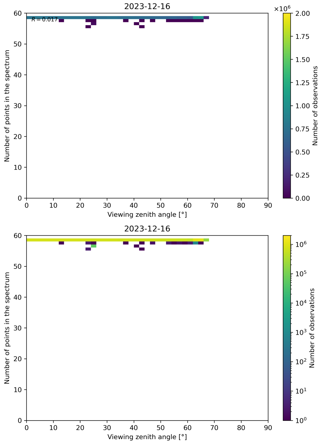
Figure 125: Scatter density plot of “Viewing zenith angle” against “Number of points in the spectrum” for 2023-12-15 to 2023-12-17.
