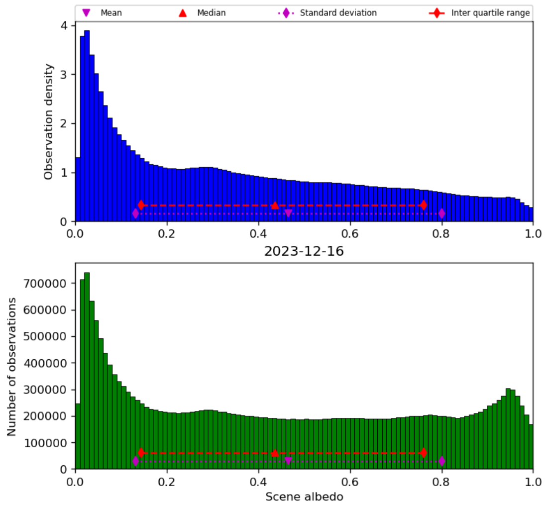
Figure 34: Histogram of “Scene albedo” for 2023-12-15 to 2023-12-17
