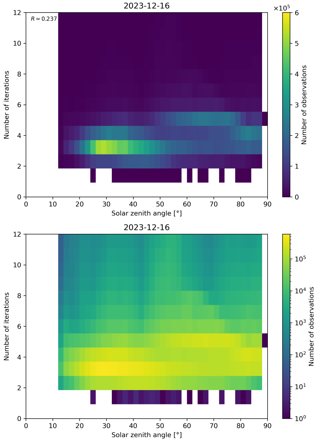
Figure 114: Scatter density plot of “Solar zenith angle” against “Number of iterations” for 2023-12-15 to 2023-12-17.
