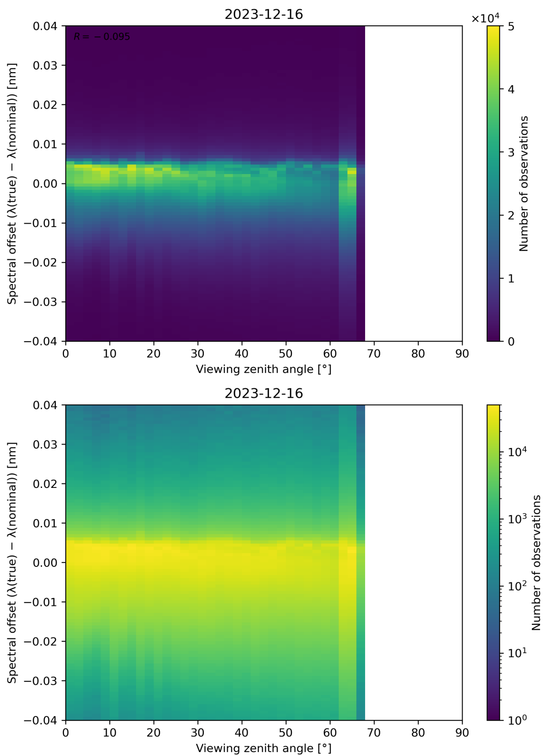
Figure 128: Scatter density plot of “Viewing zenith angle” against “Spectral offset ( \lambda(\text{true}) - \lambda(\text{nominal}) )” for 2023-12-15 to 2023-12-17.
