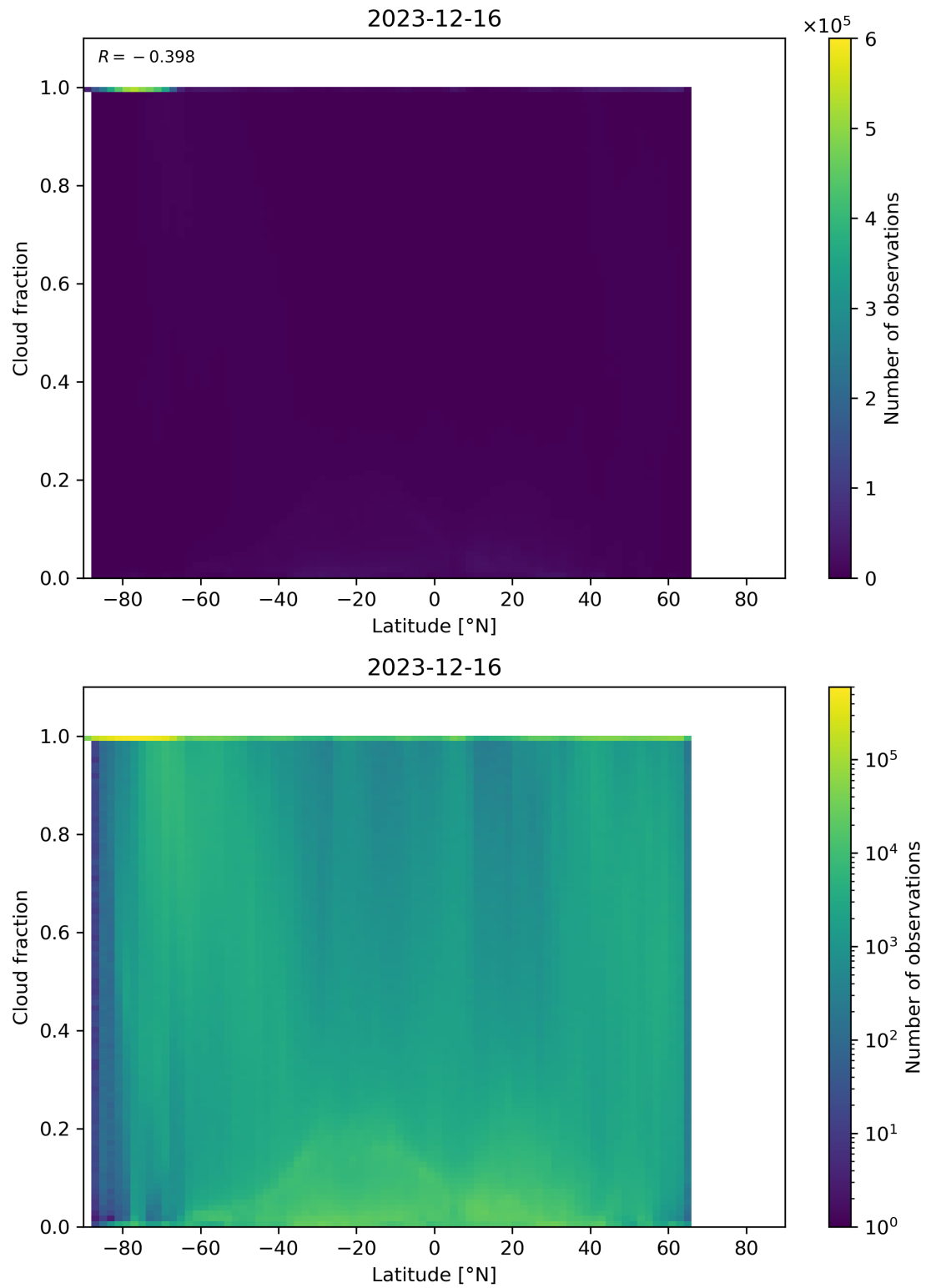
Figure 90: Scatter density plot of “Latitude” against “Cloud fraction” for 2023-12-15 to 2023-12-17.
