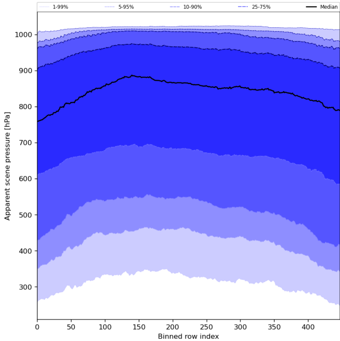
Figure 53: Along track statistics of “Apparent scene pressure” for 2023-12-15 to 2023-12-17
