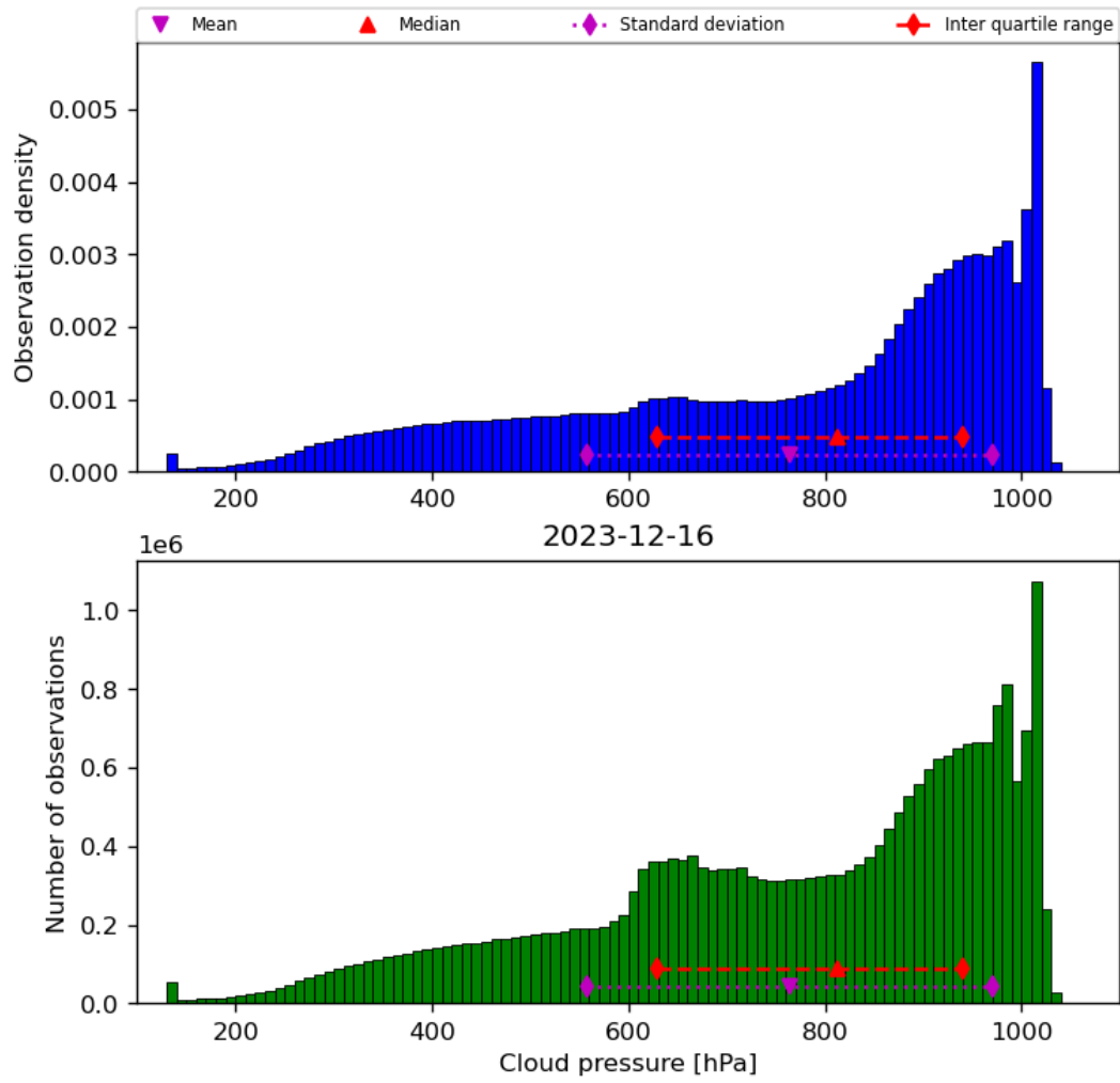
Figure 30: Histogram of “Cloud pressure” for 2023-12-15 to 2023-12-17
