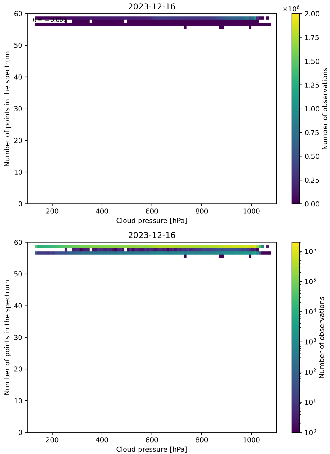
Figure 82: Scatter density plot of “Cloud pressure” against “Number of points in the spectrum” for 2023-12-15 to 2023-12-17.
