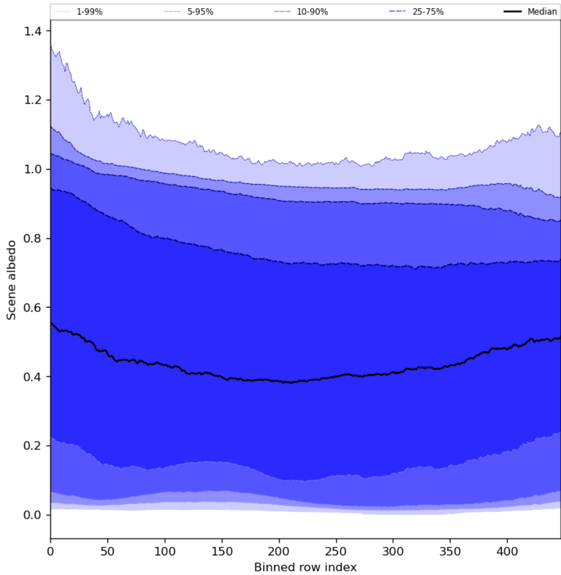
Figure 51: Along track statistics of “Scene albedo” for 2023-12-15 to 2023-12-17
