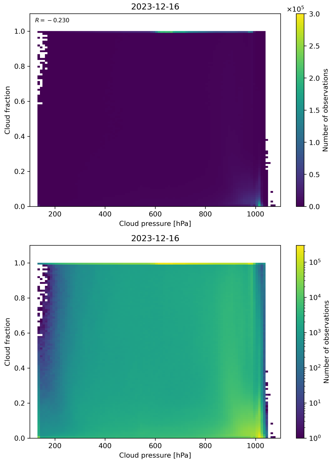
Figure 79: Scatter density plot of “Cloud pressure” against “Cloud fraction” for 2023-12-15 to 2023-12-17.
