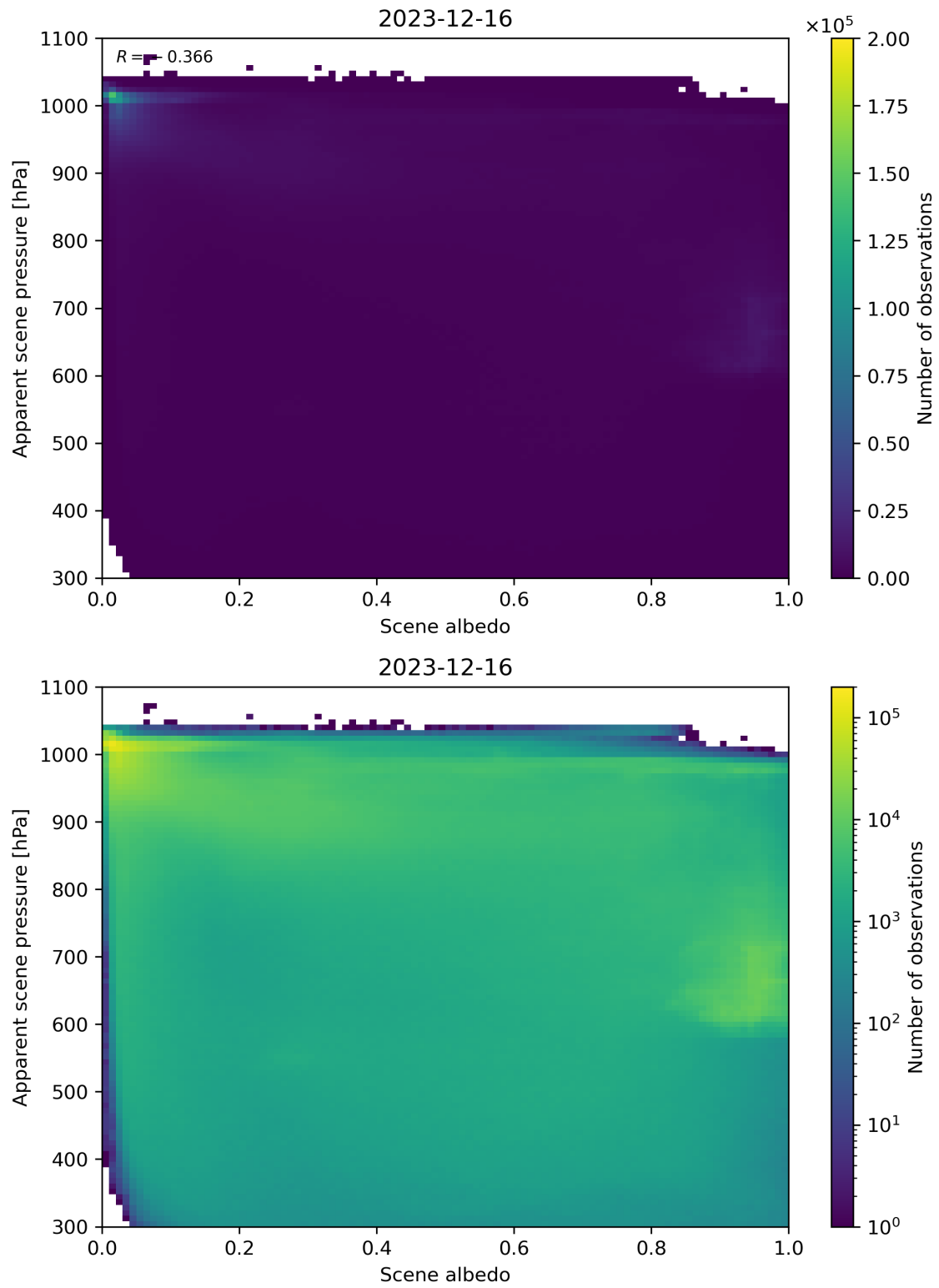
Figure 102: Scatter density plot of “Scene albedo” against “Apparent scene pressure” for 2023-12-15 to 2023-12-17.
