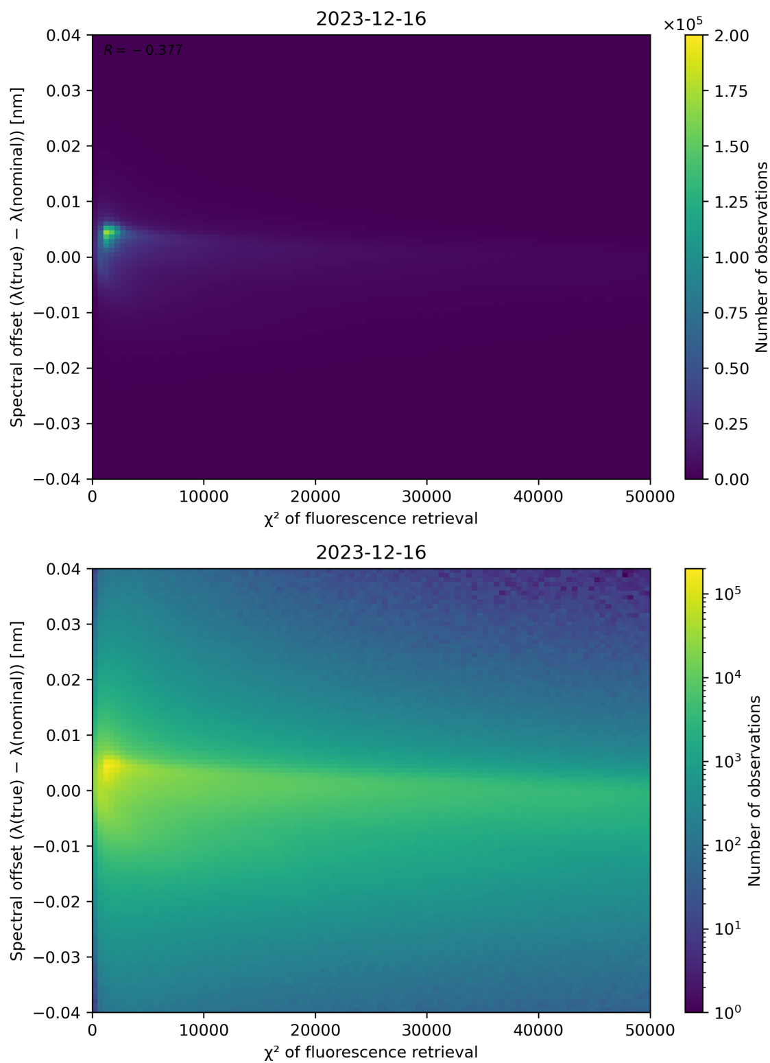
Figure 69: Scatter density plot of " \chi^2 of fluorescence retrieval" against "Spectral offset ( \lambda(\text{true}) - \lambda(\text{nominal}) )" for 2023-12-15 to 2023-12-17.
