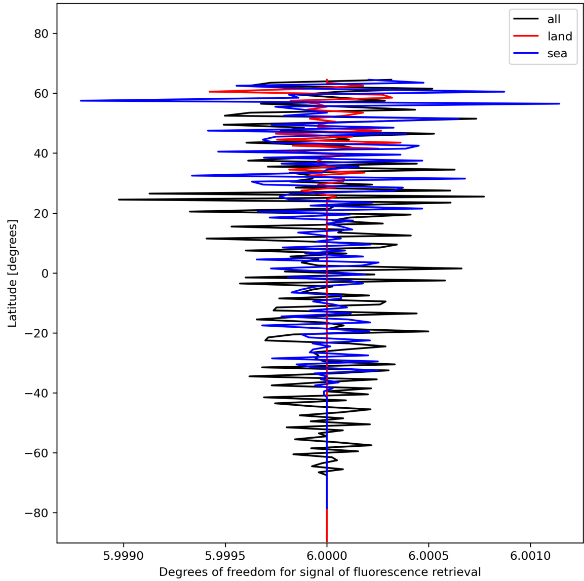
Figure 26: Zonal average of “Degrees of freedom for signal of fluorescence retrieval” for 2023-12-15 to 2023-12-17.
