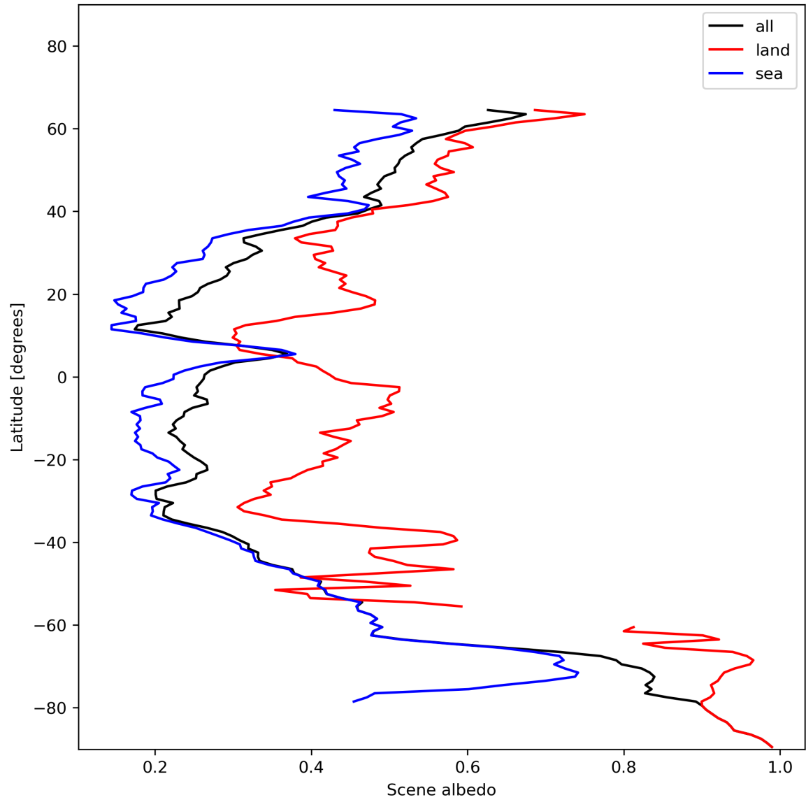
Figure 17: Zonal average of “Scene albedo” for 2023-12-15 to 2023-12-17.
