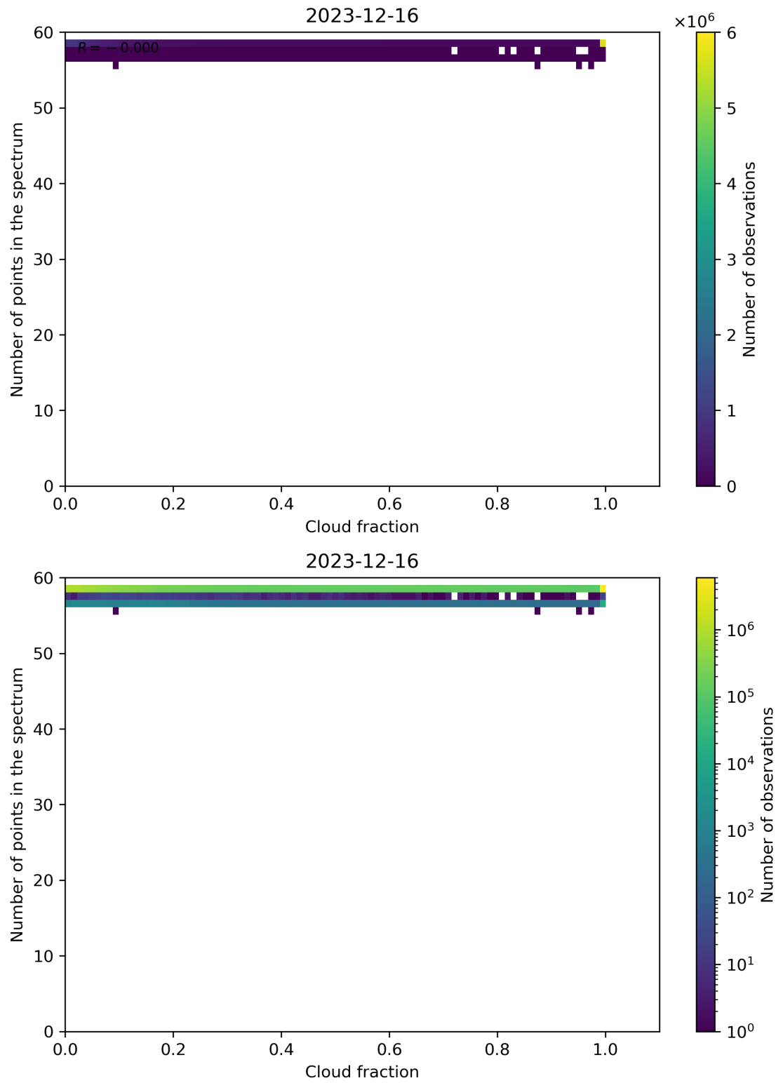
Figure 74: Scatter density plot of “Cloud fraction” against “Number of points in the spectrum” for 2023-12-15 to 2023-12-17.
