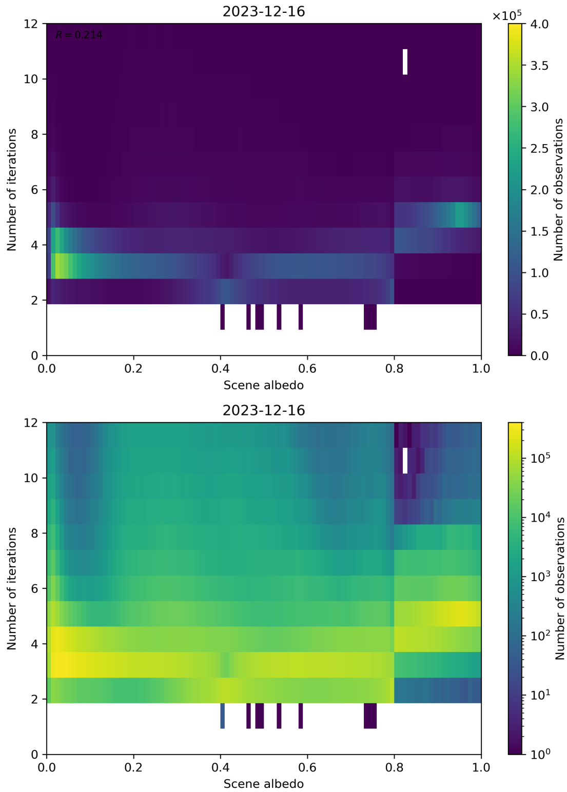
Figure 105: Scatter density plot of “Scene albedo” against “Number of iterations” for 2023-12-15 to 2023-12-17.
