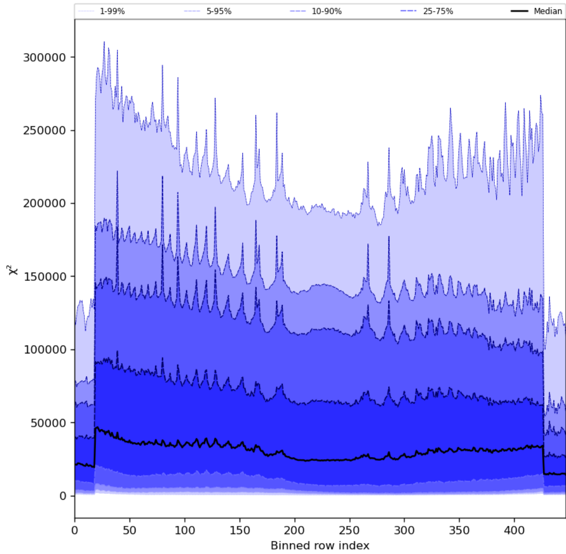
Figure 55: Along track statistics of “ \chi^2 ” for 2023-12-15 to 2023-12-17
