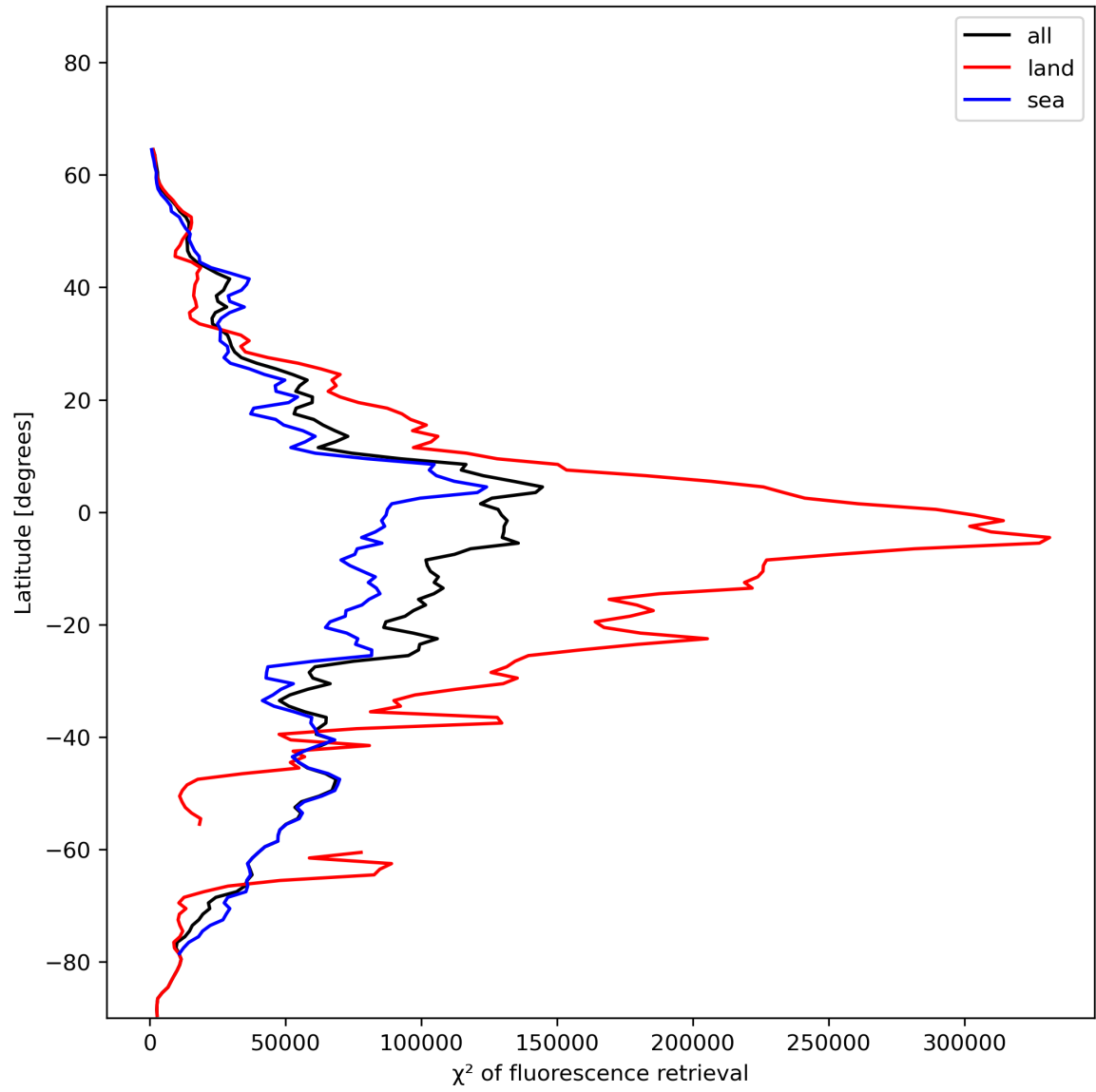
Figure 25: Zonal average of “ \chi^2 of fluorescence retrieval” for 2023-12-15 to 2023-12-17.
