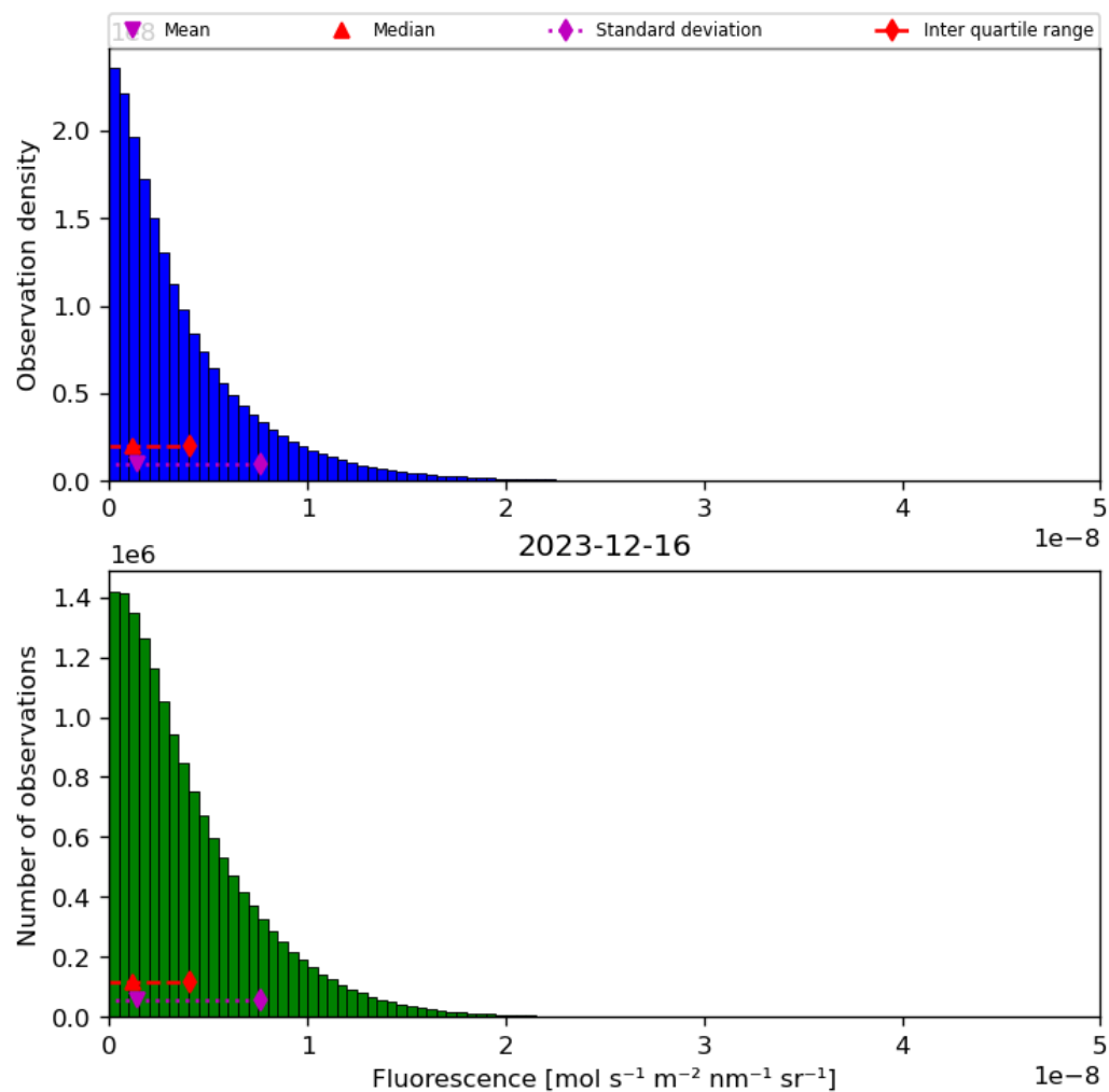
Figure 40: Histogram of “Fluorescence” for 2023-12-15 to 2023-12-17
