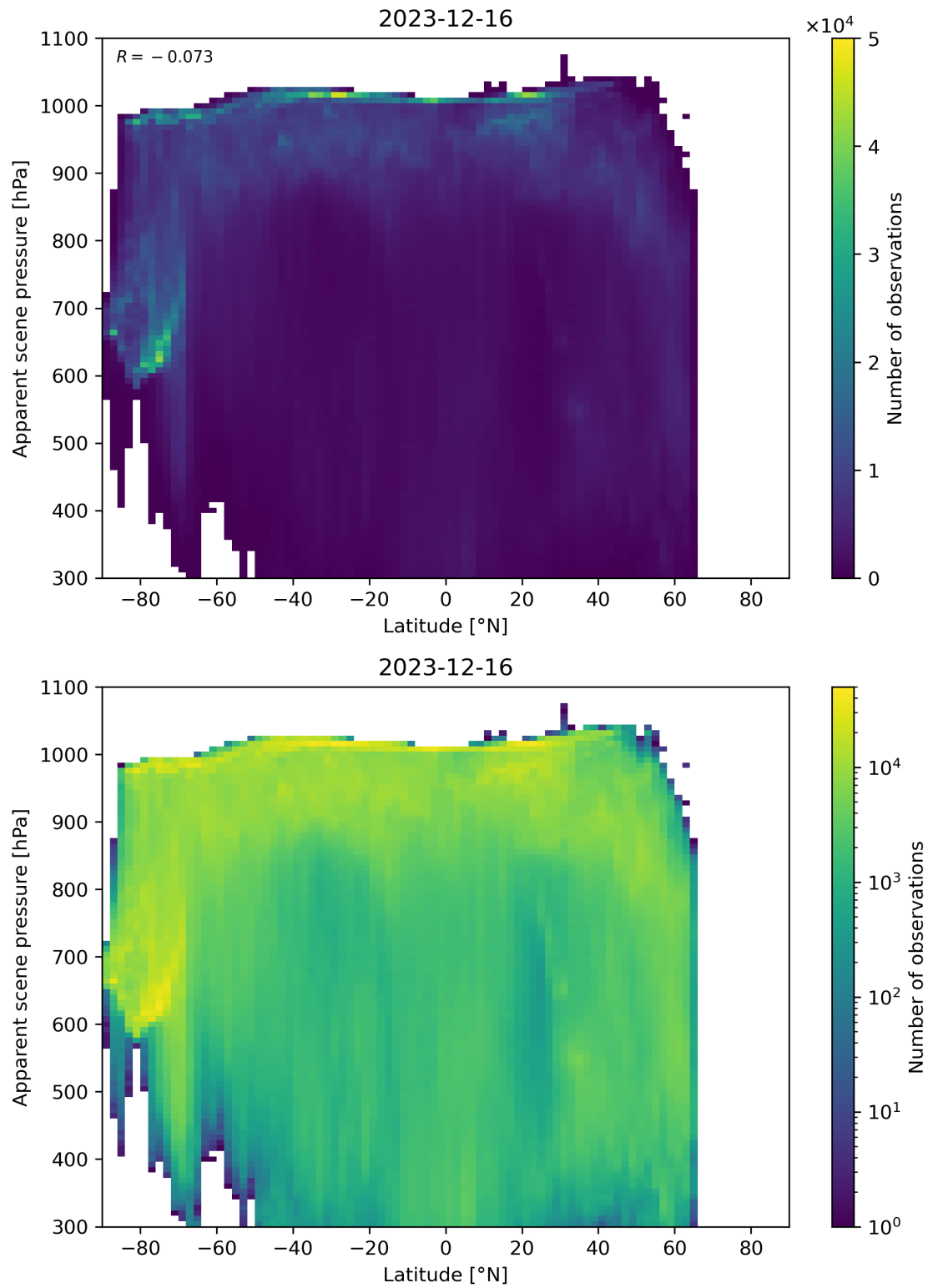
Figure 88: Scatter density plot of “Latitude” against “Apparent scene pressure” for 2023-12-15 to 2023-12-17.
