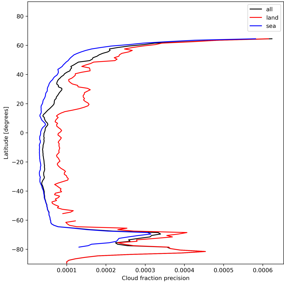
Figure 16: Zonal average of “Cloud fraction precision” for 2023-12-15 to 2023-12-17.
