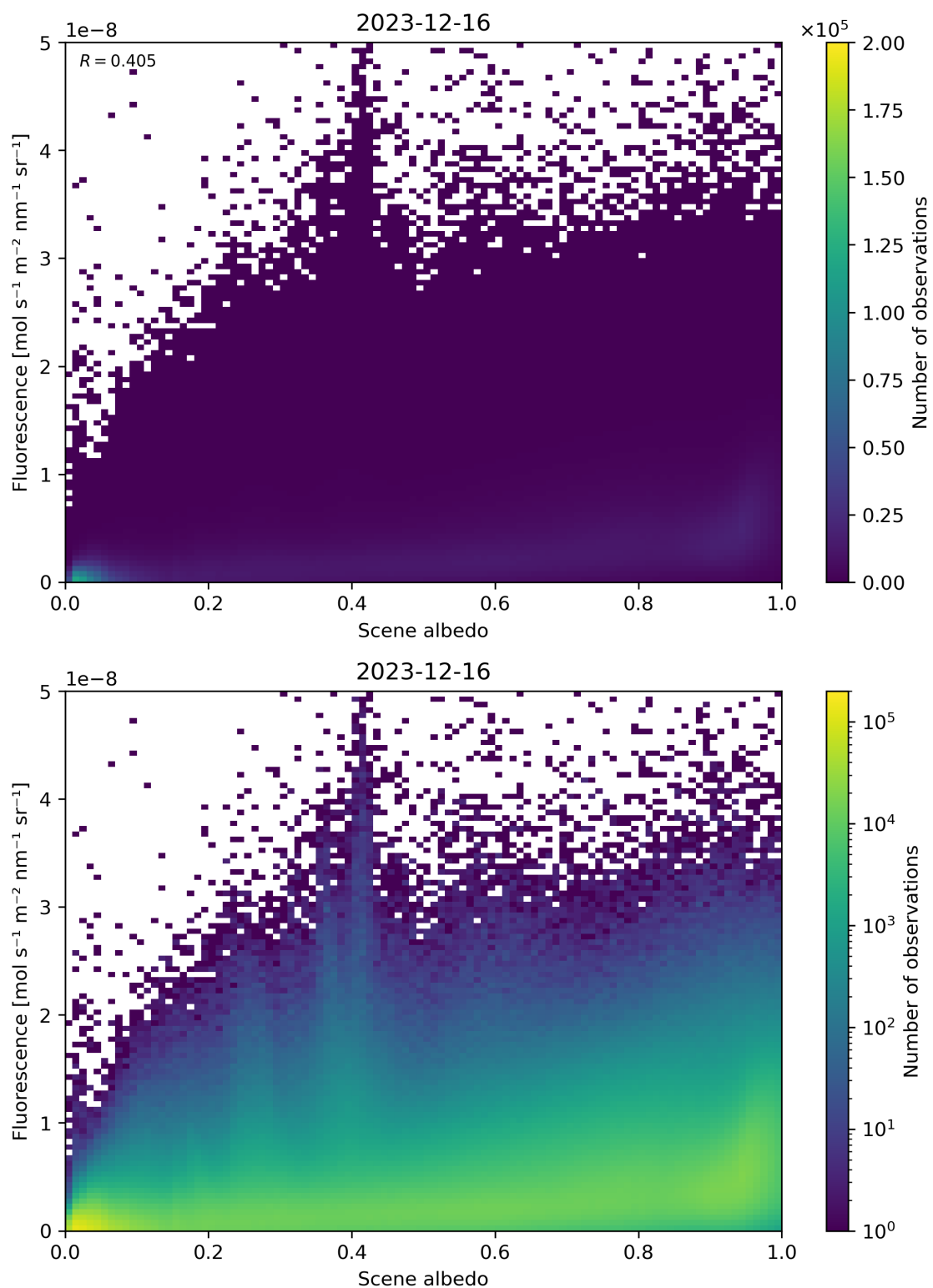
Figure 104: Scatter density plot of “Scene albedo” against “Fluorescence” for 2023-12-15 to 2023-12-17.
