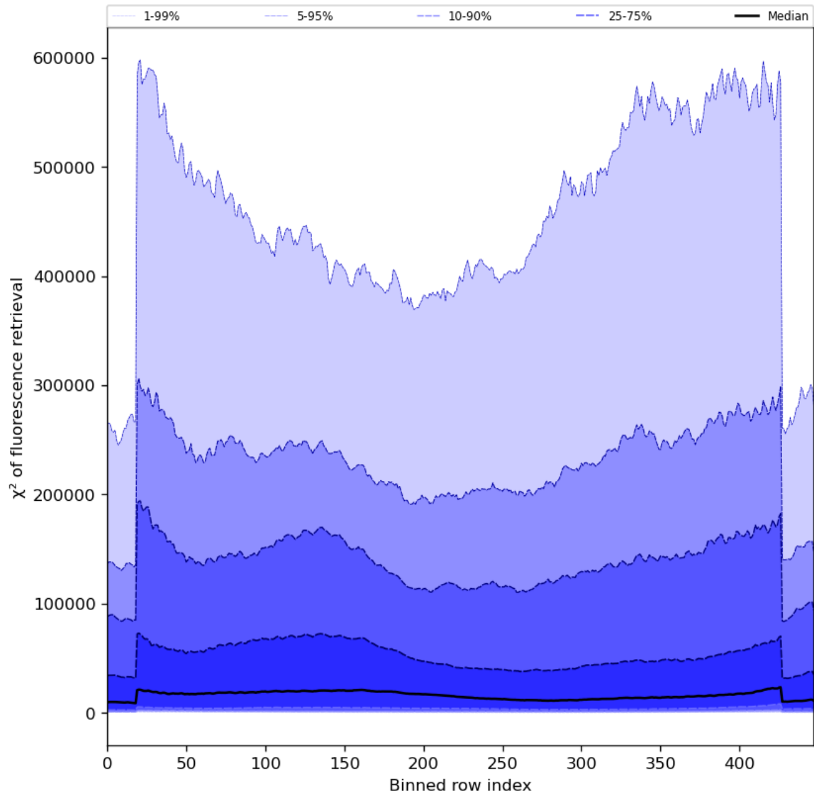
Figure 59: Along track statistics of “ \chi^2 of fluorescence retrieval” for 2023-12-15 to 2023-12-17
