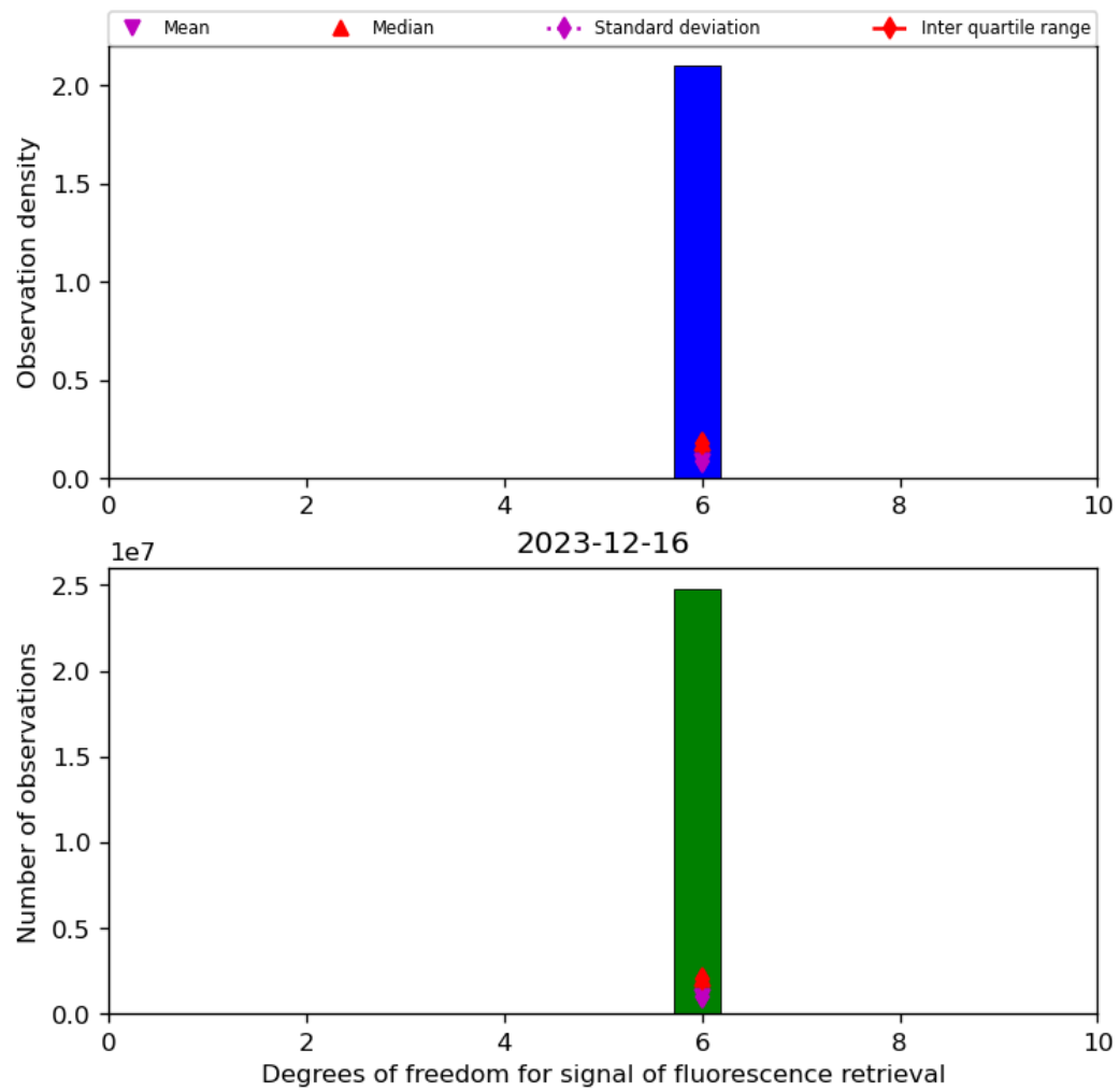
Figure 43: Histogram of “Degrees of freedom for signal of fluorescence retrieval” for 2023-12-15 to 2023-12-17
