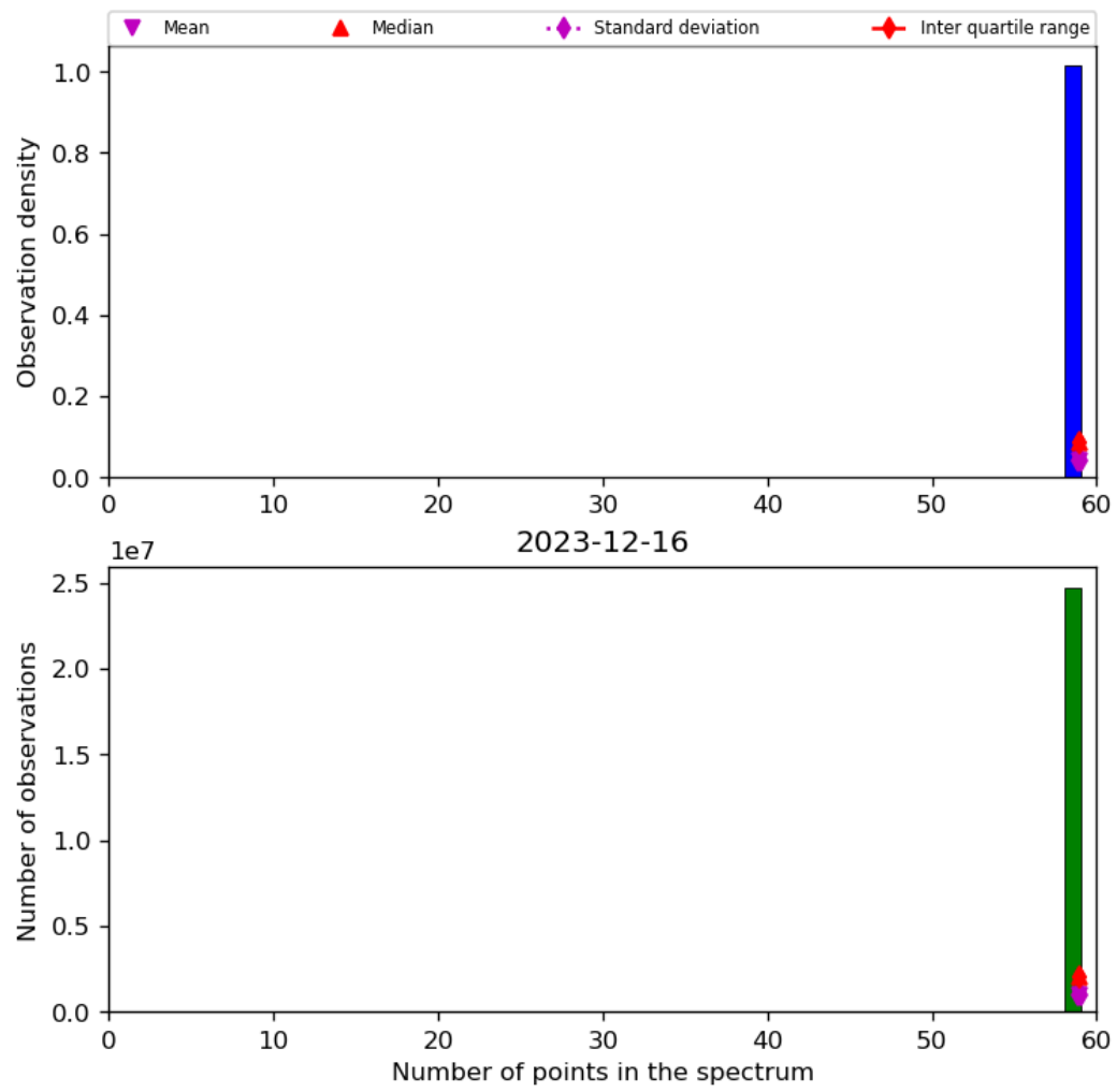
Figure 44: Histogram of “Number of points in the spectrum” for 2023-12-15 to 2023-12-17
