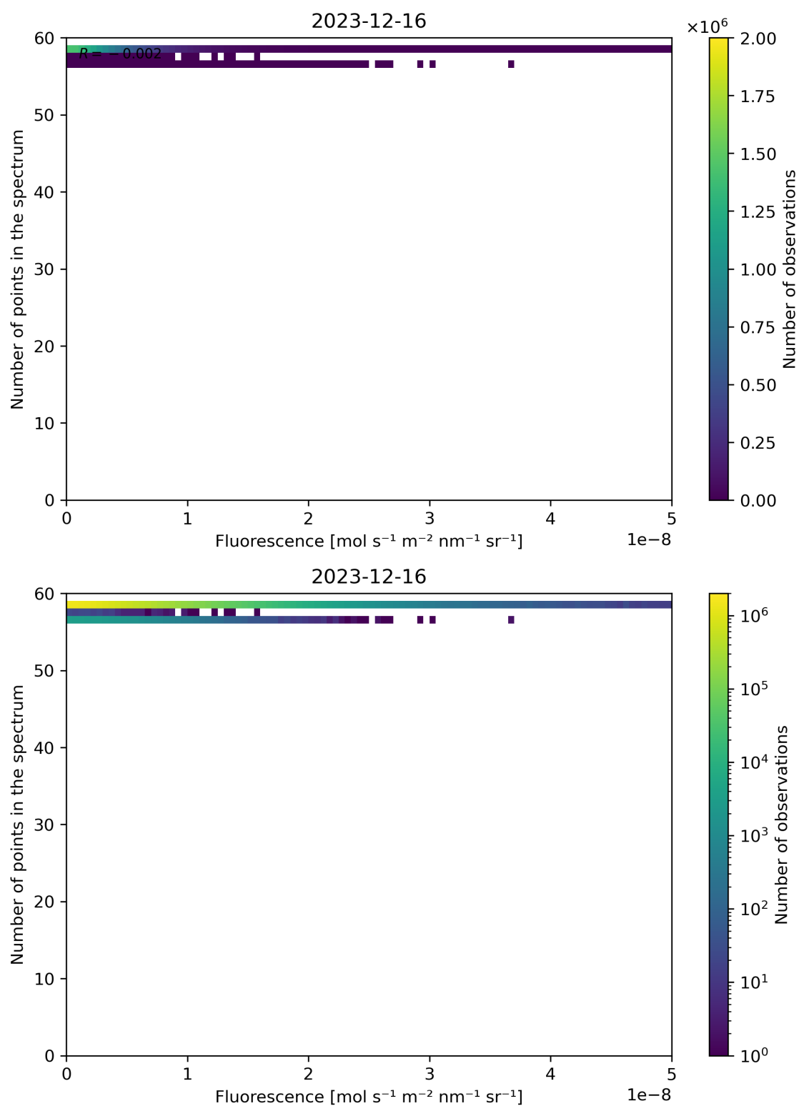
Figure 86: Scatter density plot of “Fluorescence” against “Number of points in the spectrum” for 2023-12-15 to 2023-12-17.
