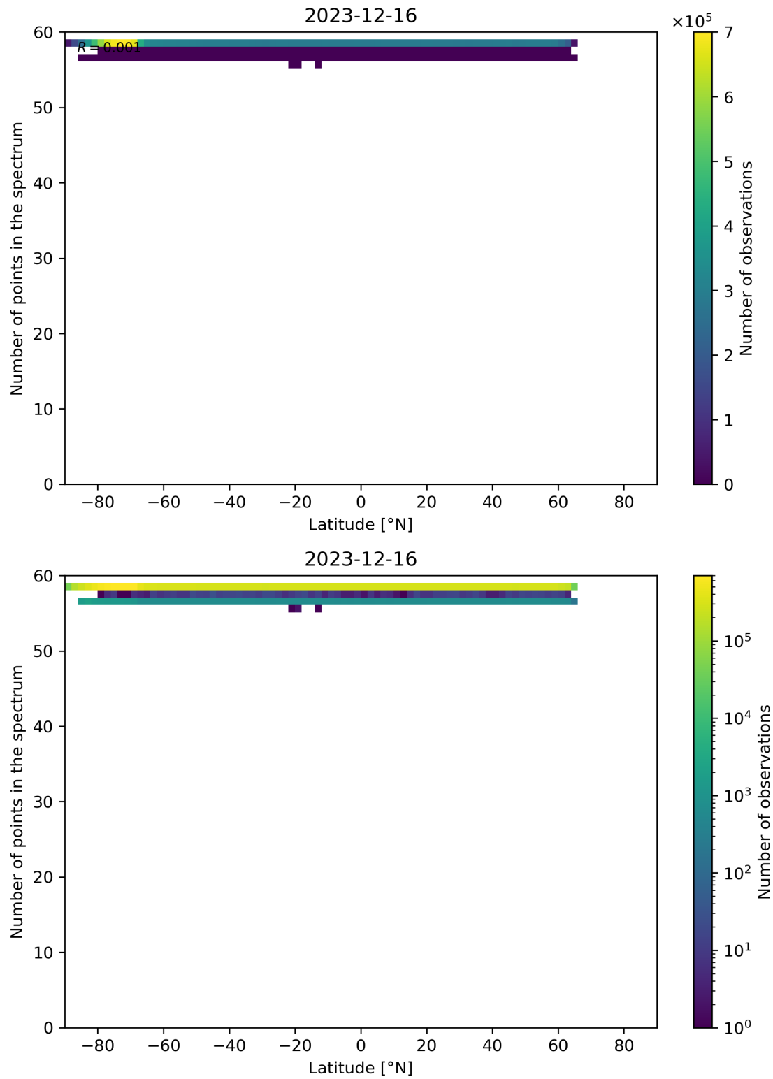
Figure 94: Scatter density plot of “Latitude” against “Number of points in the spectrum” for 2023-12-15 to 2023-12-17.
