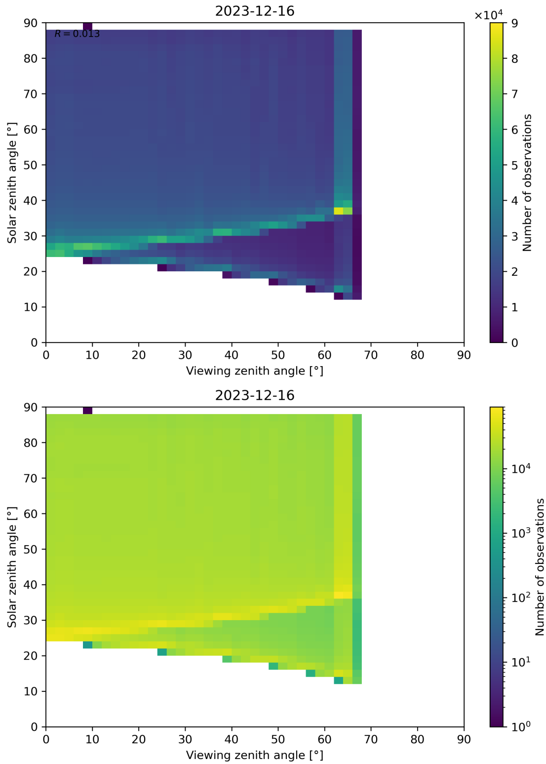
Figure 127: Scatter density plot of “Viewing zenith angle” against “Solar zenith angle” for 2023-12-15 to 2023-12-17.
