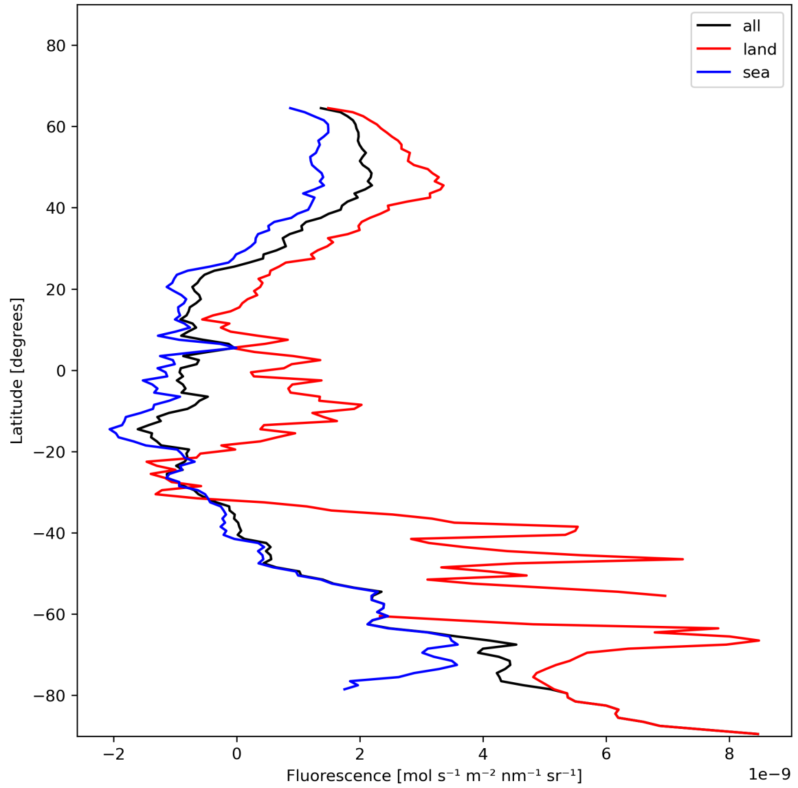
Figure 23: Zonal average of “Fluorescence” for 2023-12-15 to 2023-12-17.
