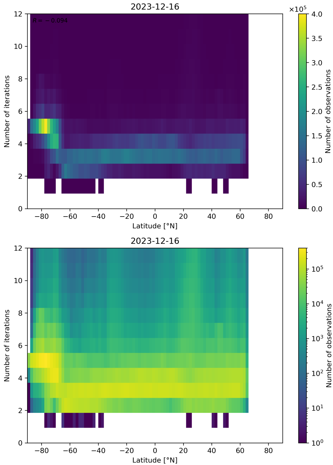
Figure 93: Scatter density plot of “Latitude” against “Number of iterations” for 2023-12-15 to 2023-12-17.
