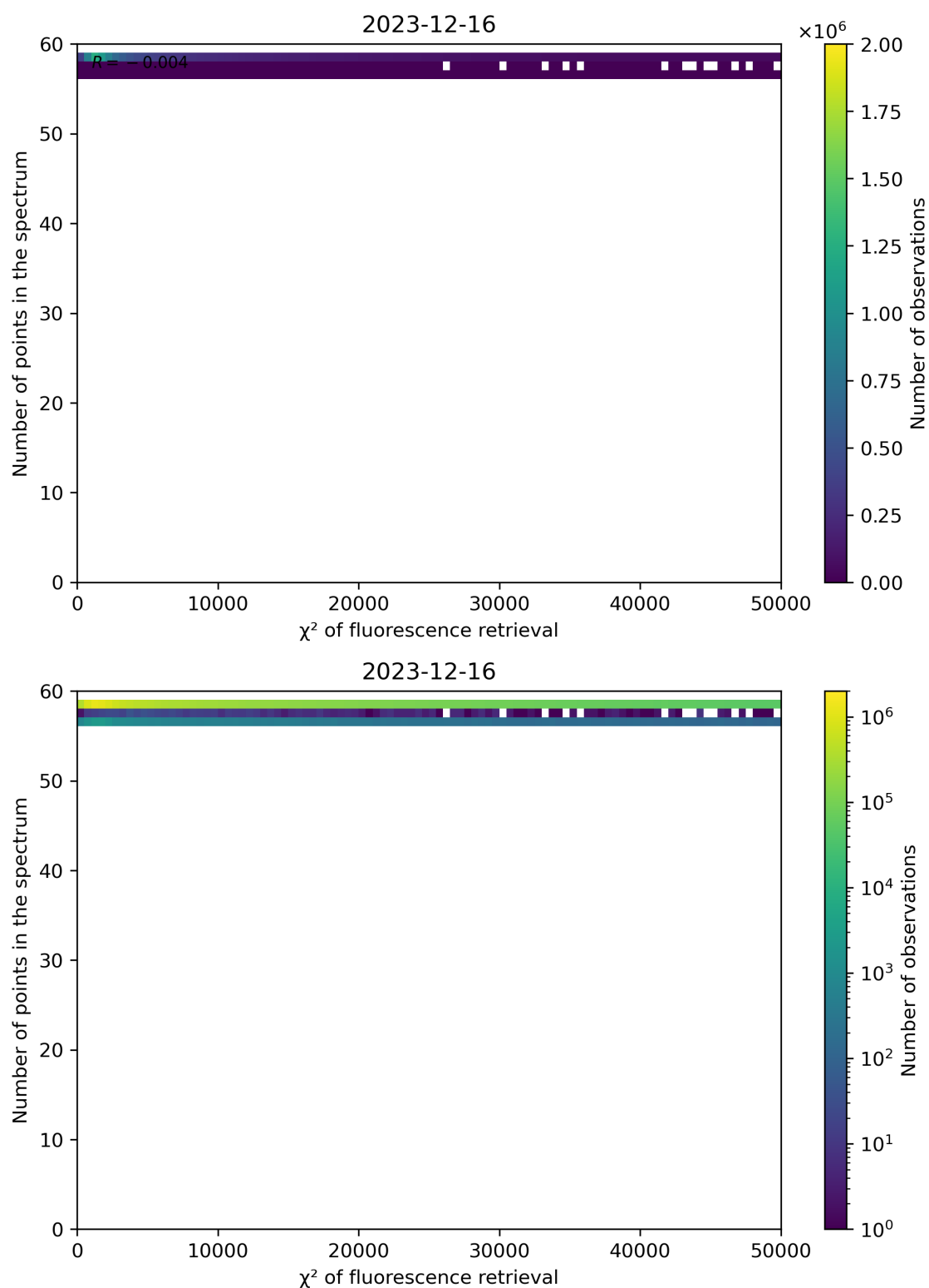
Figure 68: Scatter density plot of " \chi^2 of fluorescence retrieval" against "Number of points in the spectrum" for 2023-12-15 to 2023-12-17.
