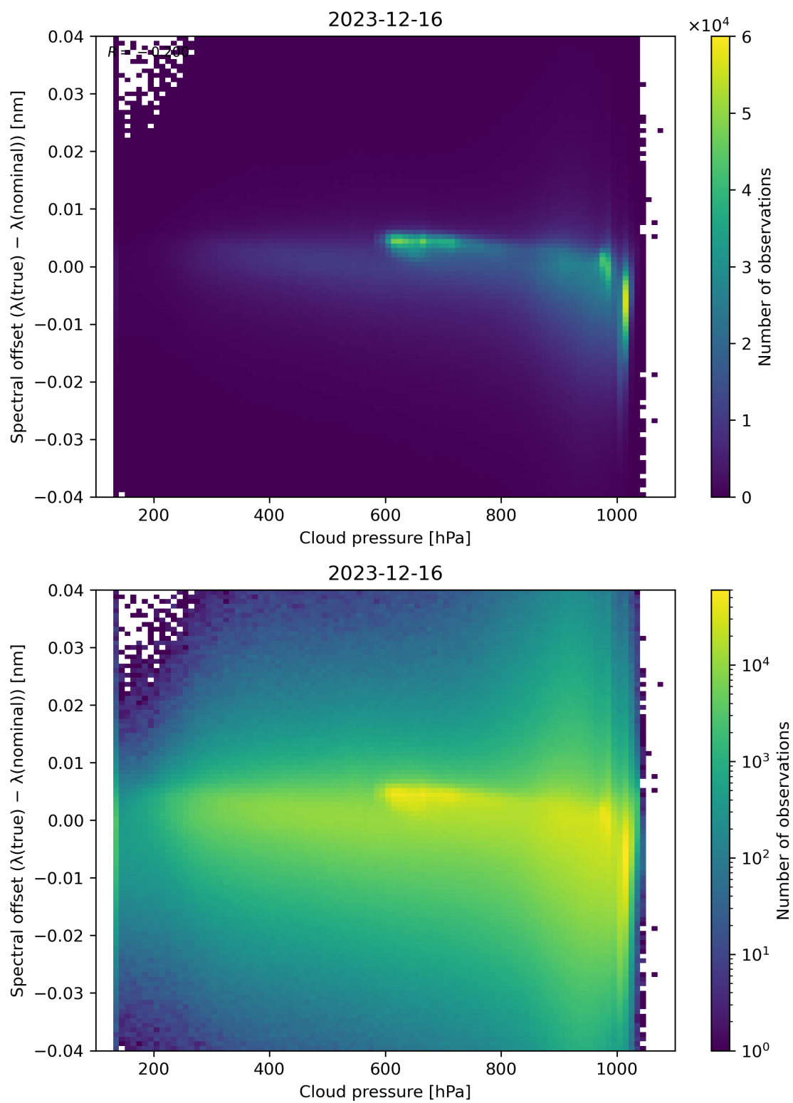
Figure 84: Scatter density plot of “Cloud pressure” against “Spectral offset ( \lambda(\text{true}) - \lambda(\text{nominal}) )” for 2023-12-15 to 2023-12-17.
