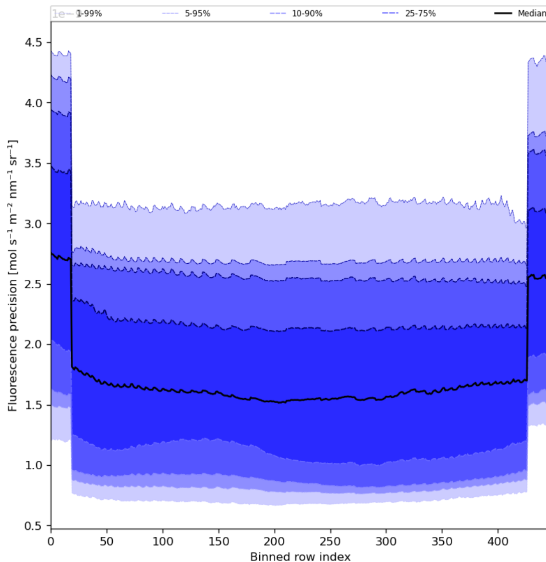
Figure 58: Along track statistics of “Fluorescence precision” for 2023-12-15 to 2023-12-17
