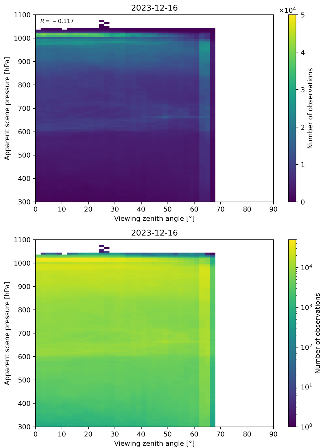
Figure 118: Scatter density plot of “Viewing zenith angle” against “Apparent scene pressure” for 2023-12-15 to 2023-12-17.
