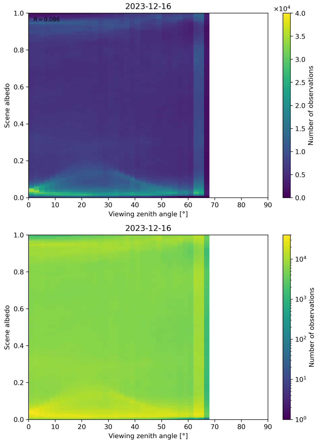
Figure 126: Scatter density plot of “Viewing zenith angle” against “Scene albedo” for 2023-12-15 to 2023-12-17.
