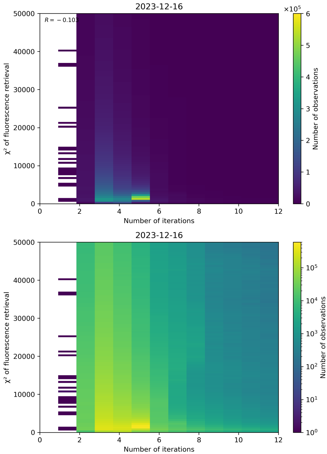
Figure 97: Scatter density plot of “Number of iterations” against “ \chi^2 of fluorescence retrieval” for 2023-12-15 to 2023-12-17.
