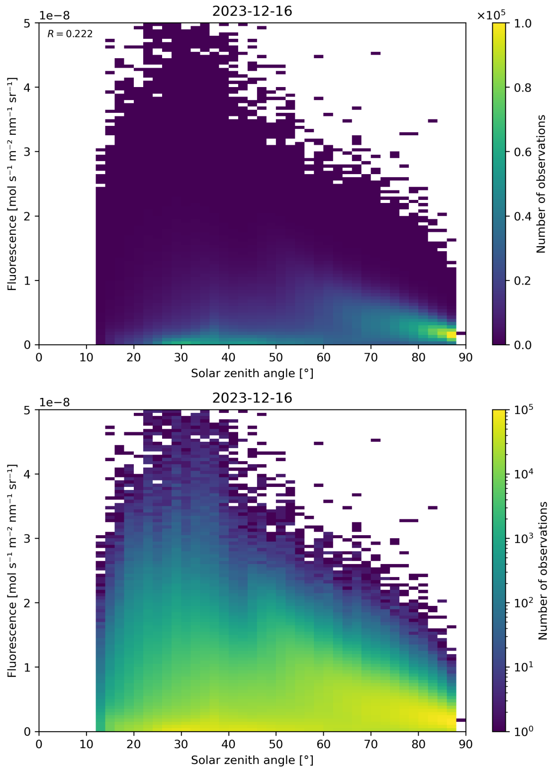
Figure 112: Scatter density plot of “Solar zenith angle” against “Fluorescence” for 2023-12-15 to 2023-12-17.
