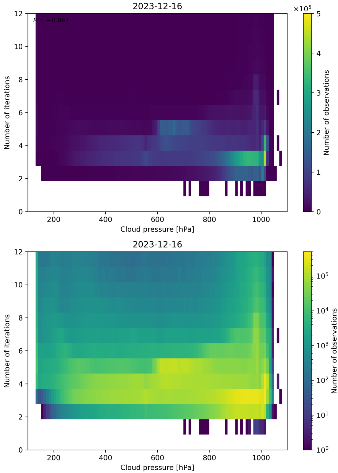
Figure 81: Scatter density plot of “Cloud pressure” against “Number of iterations” for 2023-12-15 to 2023-12-17.
