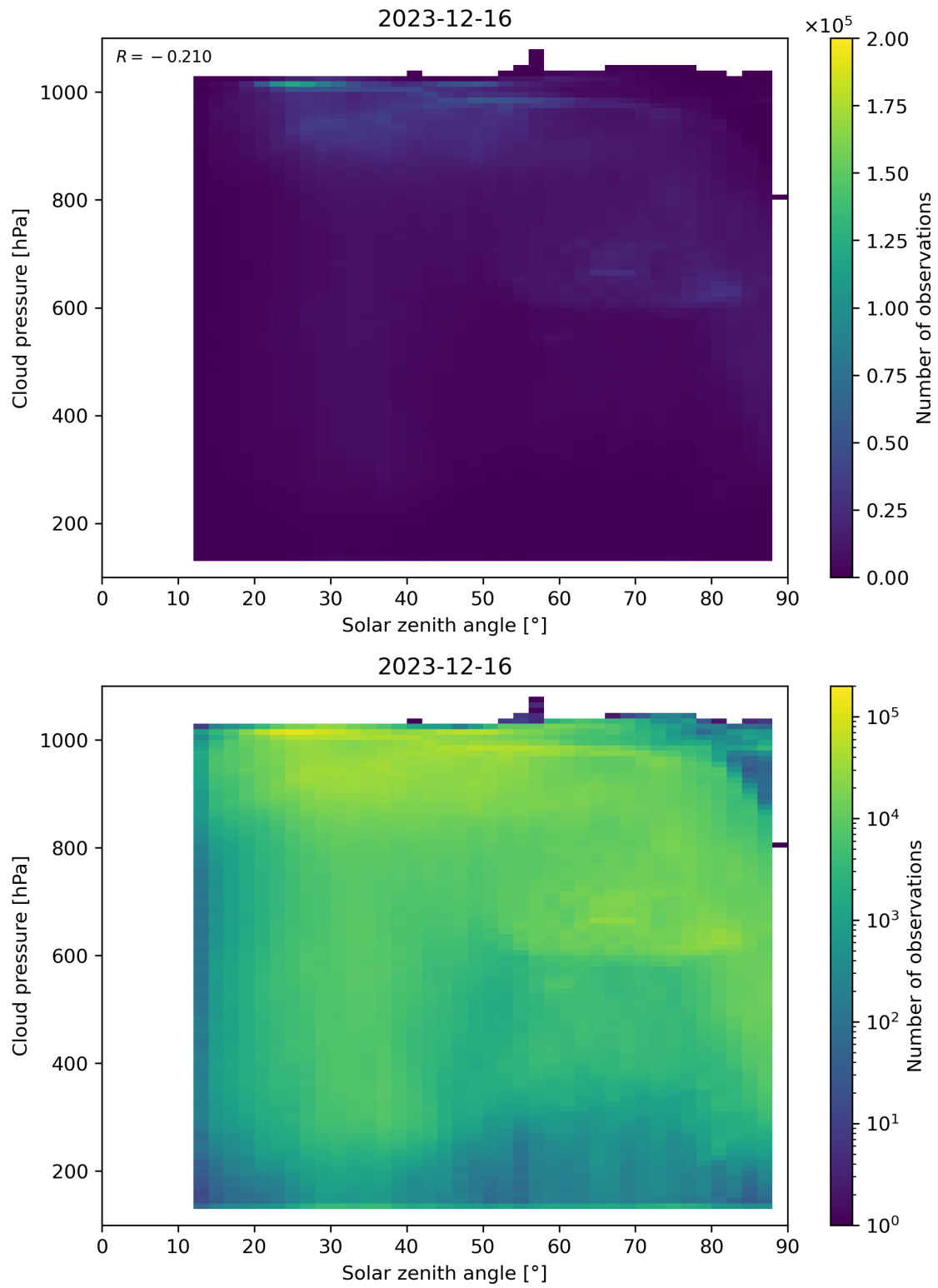
Figure 111: Scatter density plot of “Solar zenith angle” against “Cloud pressure” for 2023-12-15 to 2023-12-17.
