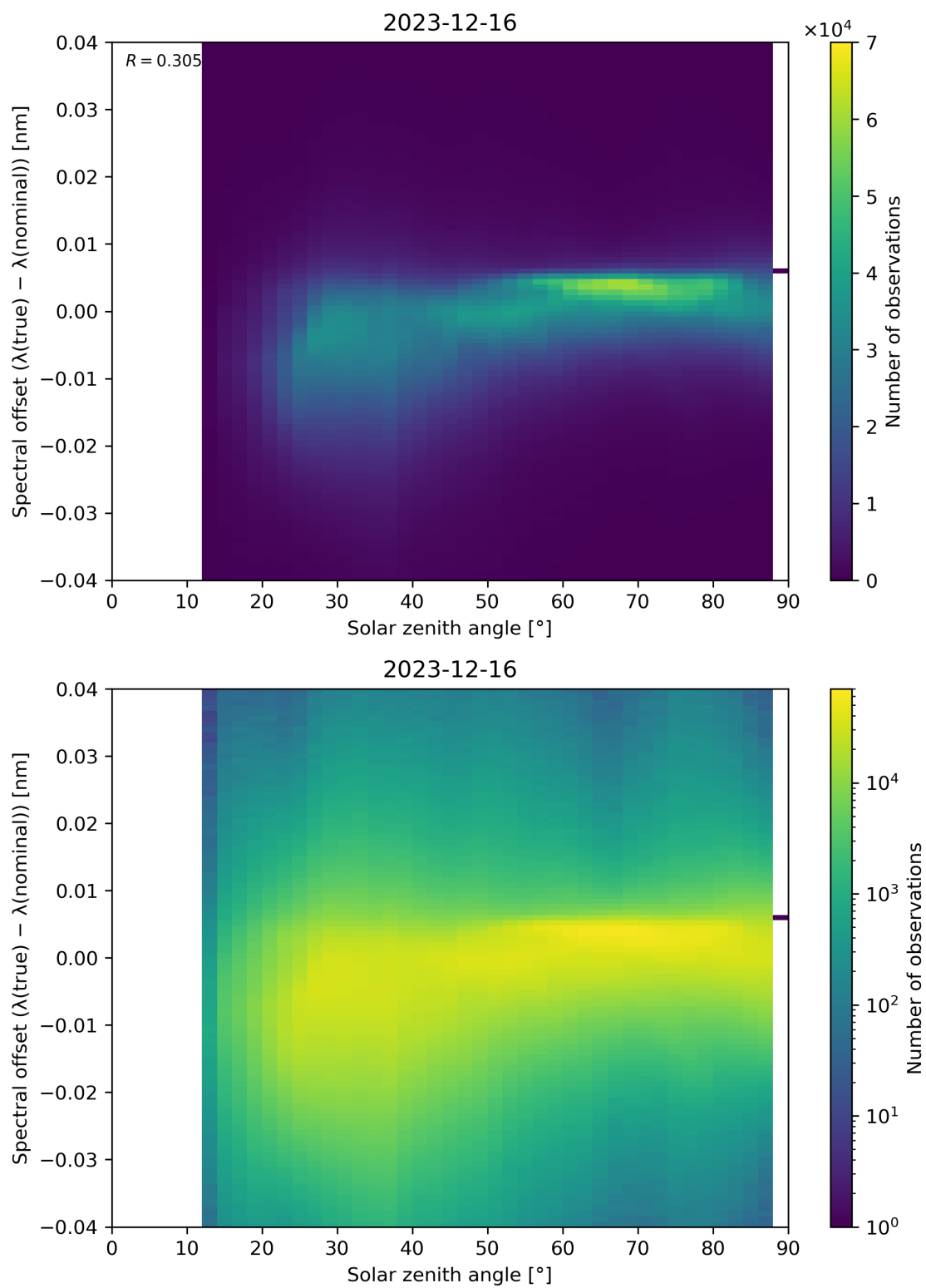
Figure 117: Scatter density plot of “Solar zenith angle” against “Spectral offset ( \lambda(\text{true}) - \lambda(\text{nominal}) )” for 2023-12-15 to 2023-12-17.
