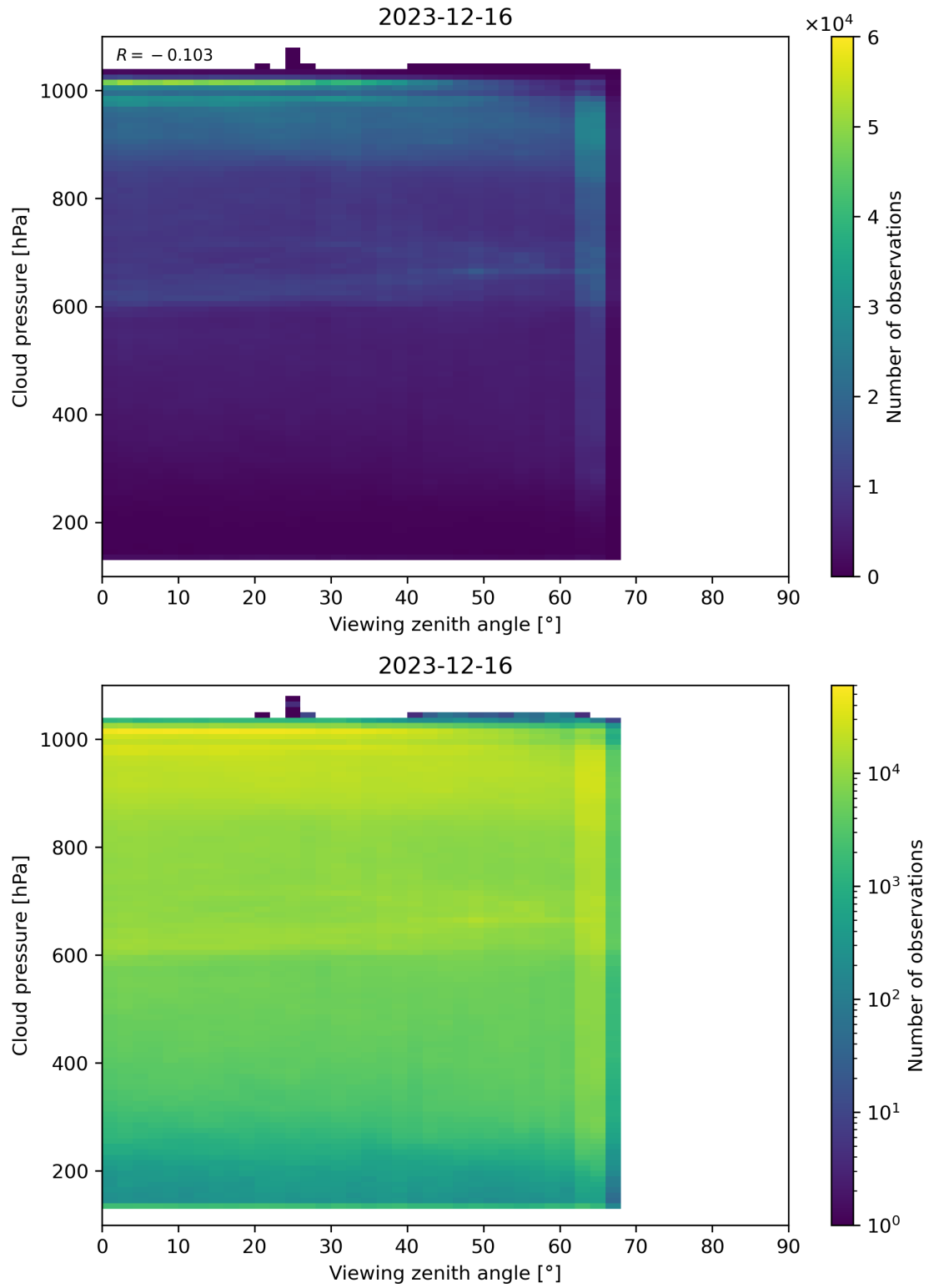
Figure 121: Scatter density plot of “Viewing zenith angle” against “Cloud pressure” for 2023-12-15 to 2023-12-17.
