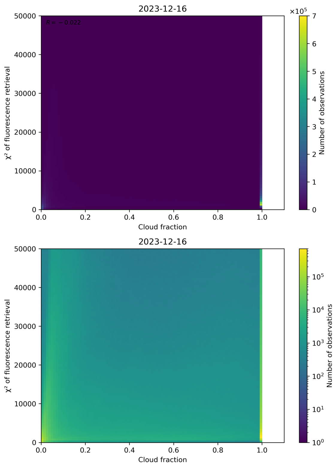
Figure 71: Scatter density plot of “Cloud fraction” against “ \chi^2 of fluorescence retrieval” for 2023-12-15 to 2023-12-17.
