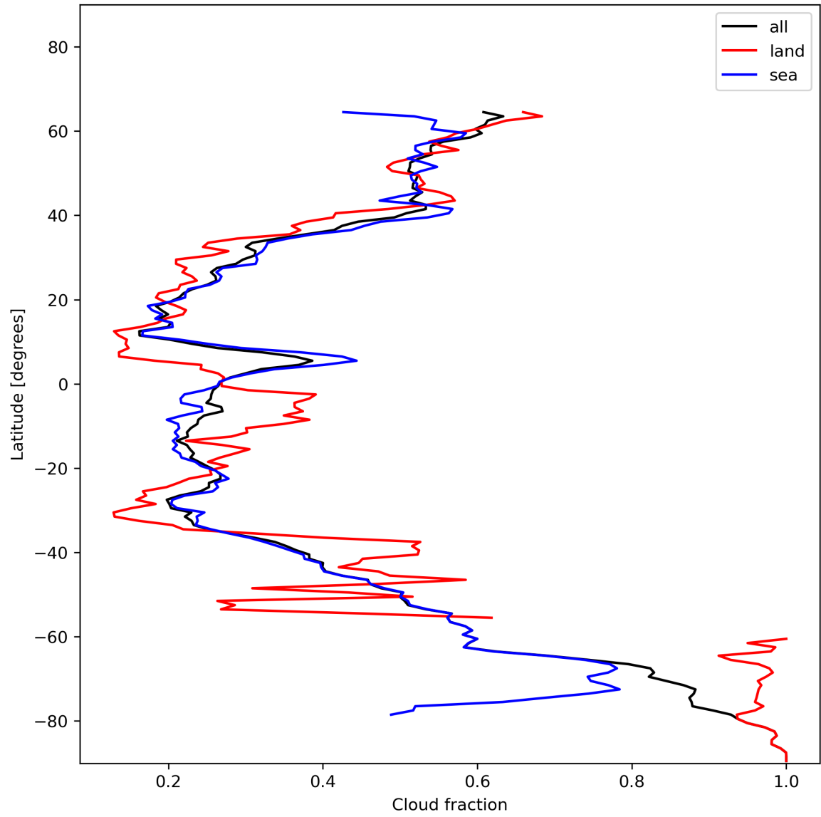
Figure 15: Zonal average of “Cloud fraction” for 2023-12-15 to 2023-12-17.
