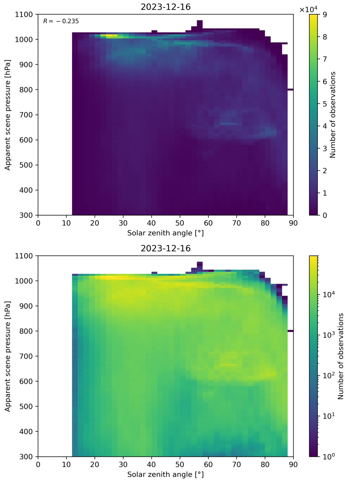
Figure 108: Scatter density plot of “Solar zenith angle” against “Apparent scene pressure” for 2023-12-15 to 2023-12-17.
