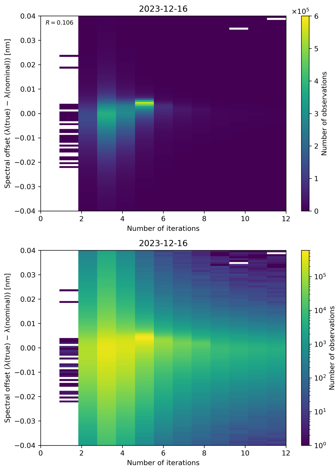
Figure 100: Scatter density plot of “Number of iterations” against “Spectral offset ( \lambda(\text{true}) - \lambda(\text{nominal}) )” for 2023-12-15 to 2023-12-17.
