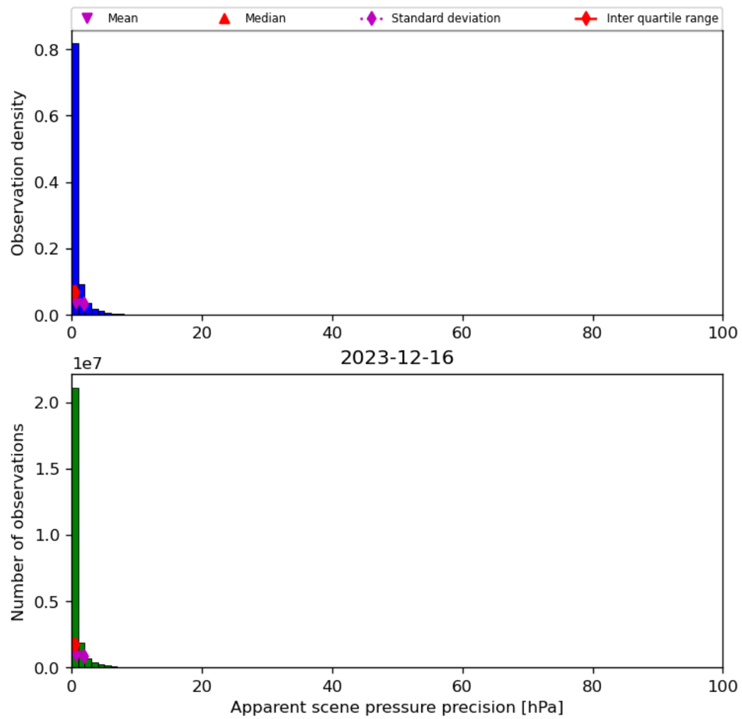
Figure 37: Histogram of “Apparent scene pressure precision” for 2023-12-15 to 2023-12-17
