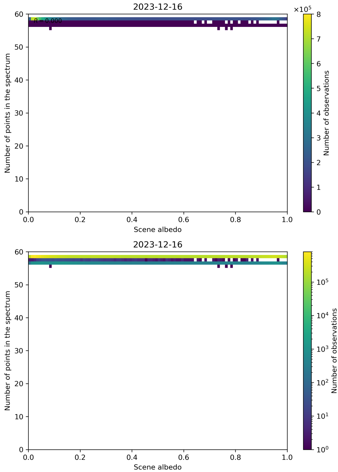
Figure 106: Scatter density plot of “Scene albedo” against “Number of points in the spectrum” for 2023-12-15 to 2023-12-17.
