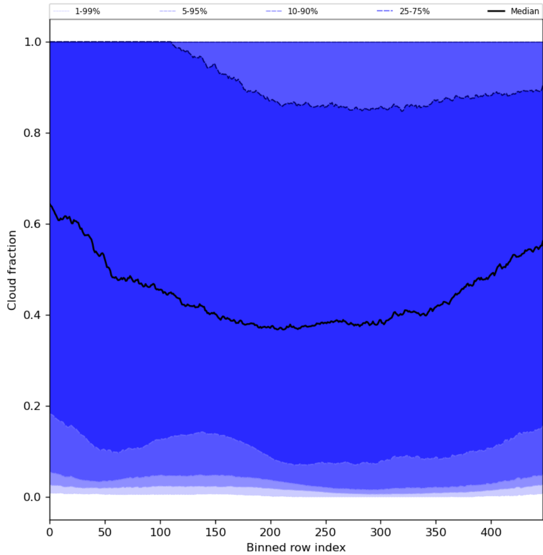
Figure 49: Along track statistics of “Cloud fraction” for 2023-12-15 to 2023-12-17
