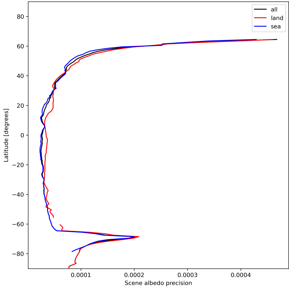
Figure 18: Zonal average of “Scene albedo precision” for 2023-12-15 to 2023-12-17.
