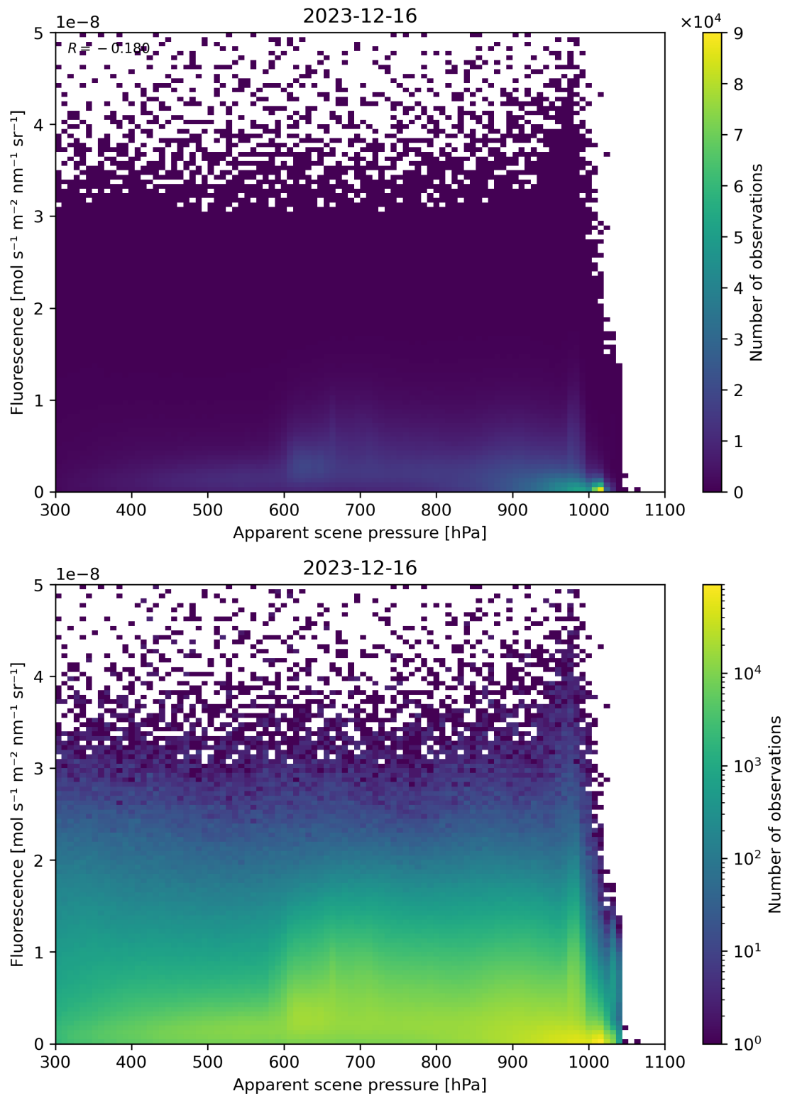
Figure 64: Scatter density plot of “Apparent scene pressure” against “Fluorescence” for 2023-12-15 to 2023-12-17.
