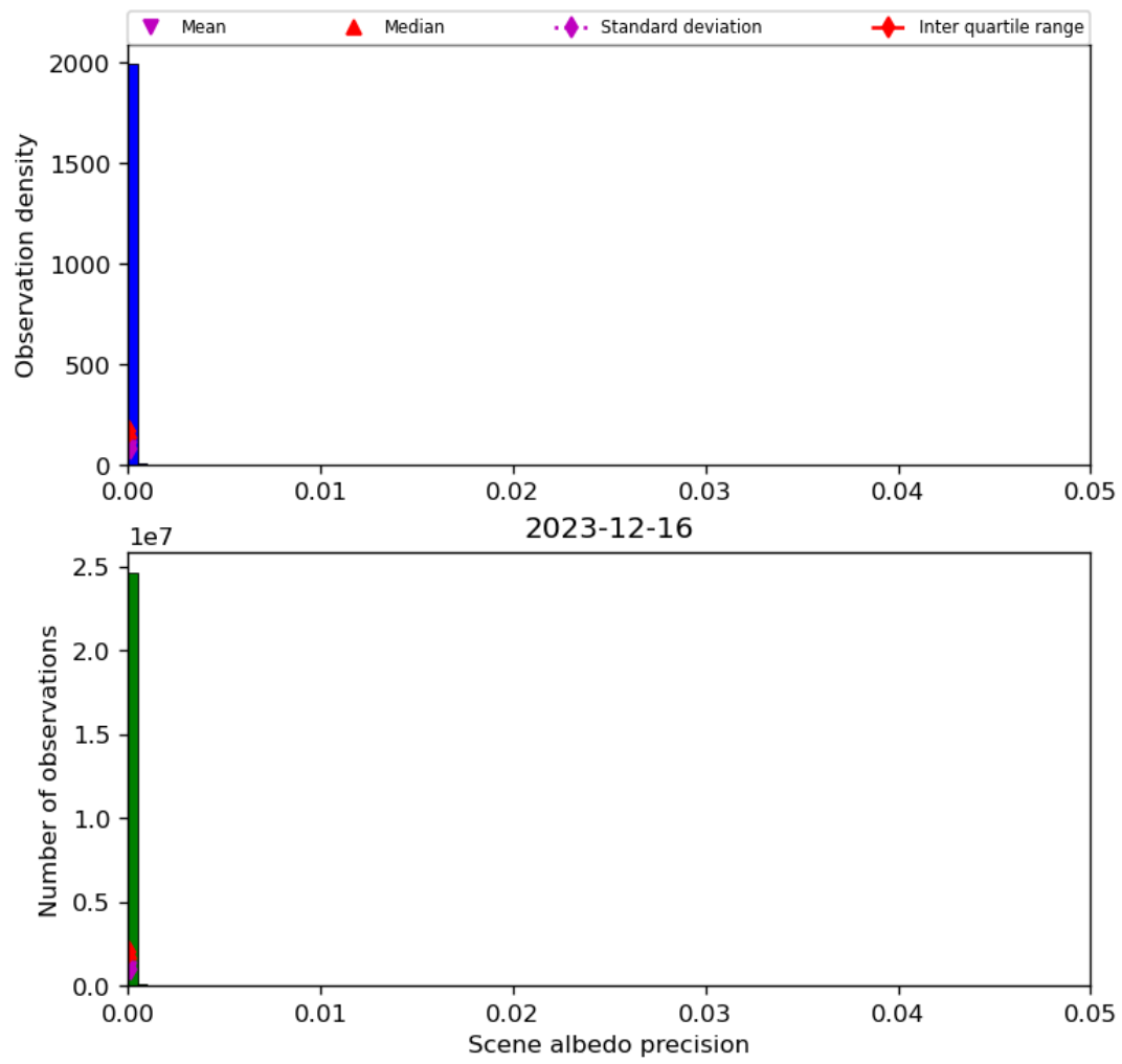
Figure 35: Histogram of “Scene albedo precision” for 2023-12-15 to 2023-12-17
