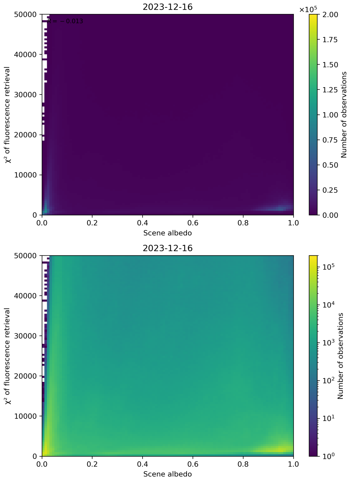
Figure 103: Scatter density plot of “Scene albedo” against “ \chi^2 of fluorescence retrieval” for 2023-12-15 to 2023-12-17.
