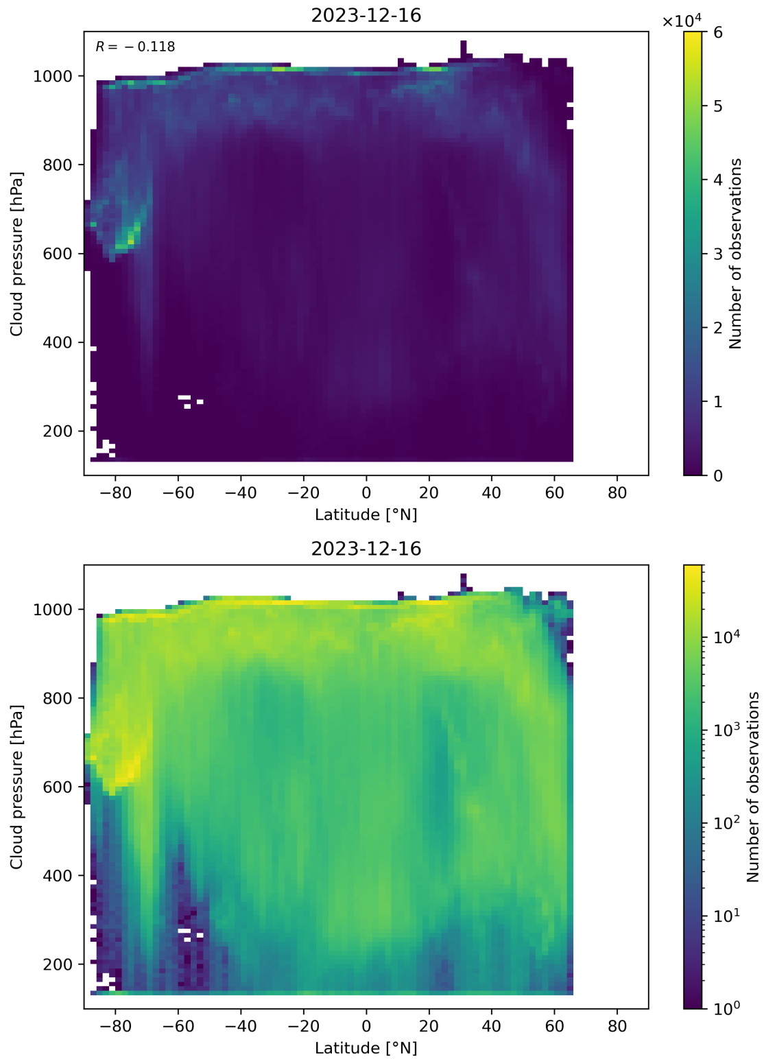
Figure 91: Scatter density plot of “Latitude” against “Cloud pressure” for 2023-12-15 to 2023-12-17.
