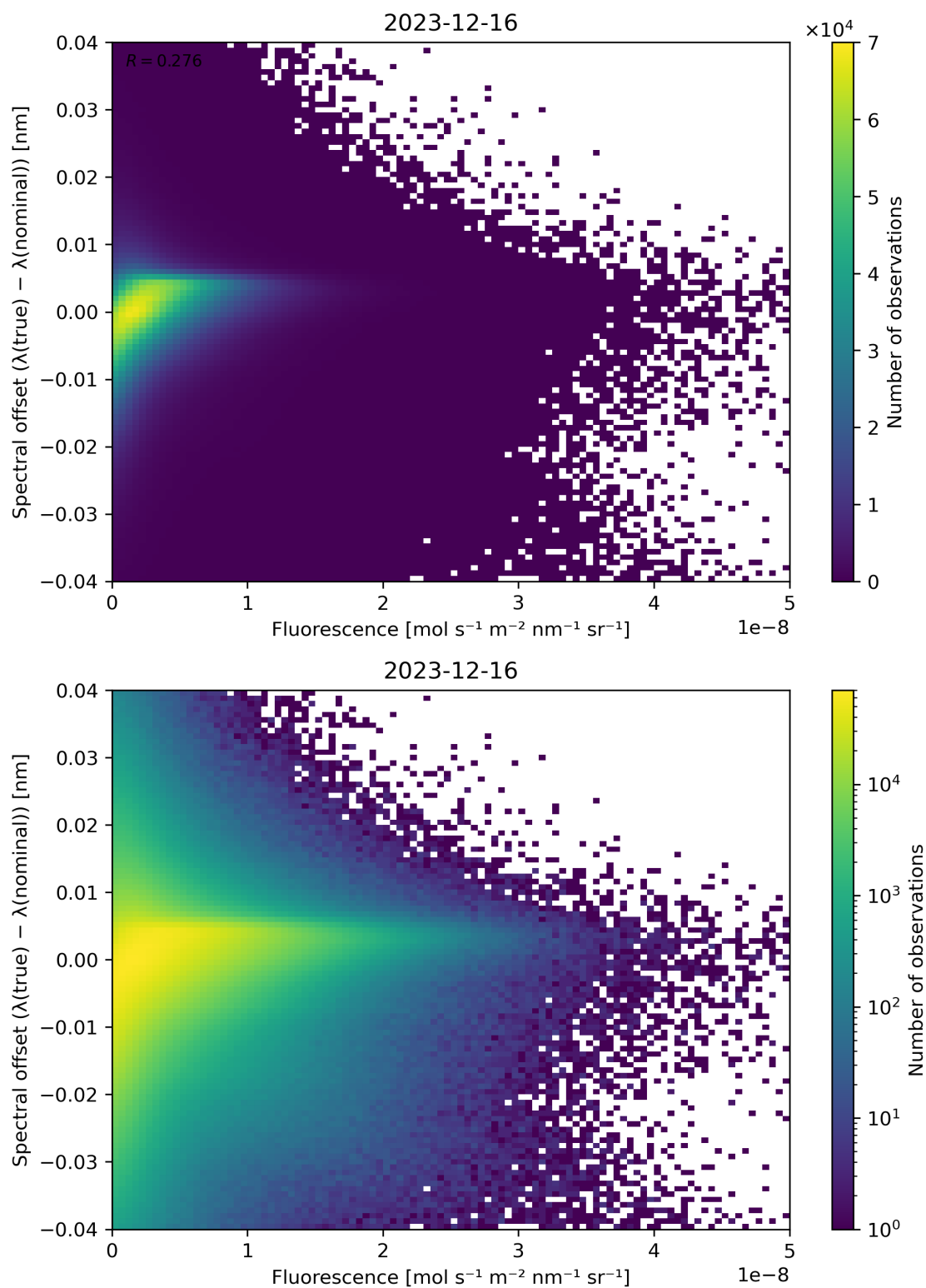
Figure 87: Scatter density plot of “Fluorescence” against “Spectral offset ( \lambda(\text{true}) - \lambda(\text{nominal}) )” for 2023-12-15 to 2023-12-17.
