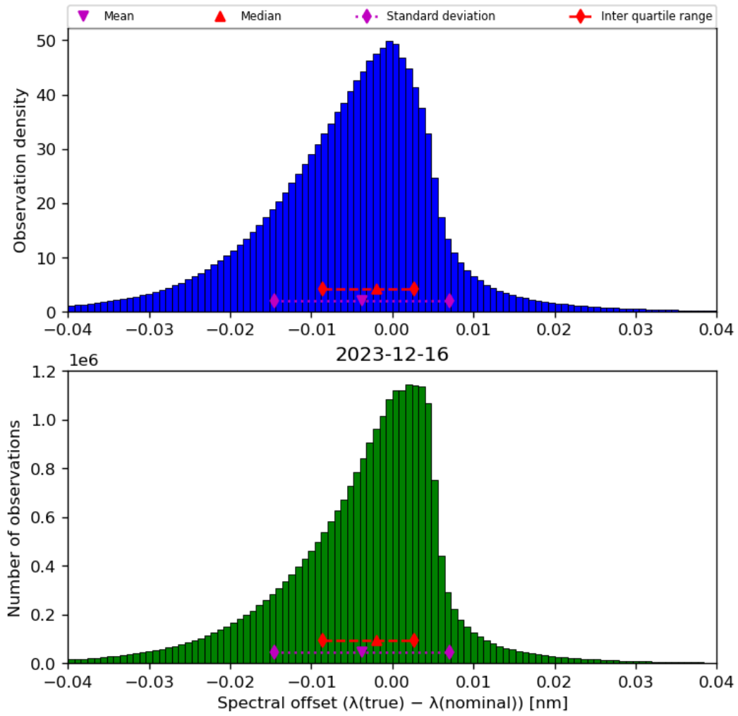
Figure 45: Histogram of “Spectral offset ( \lambda(\text{true}) - \lambda(\text{nominal}) )” for 2023-12-15 to 2023-12-17
