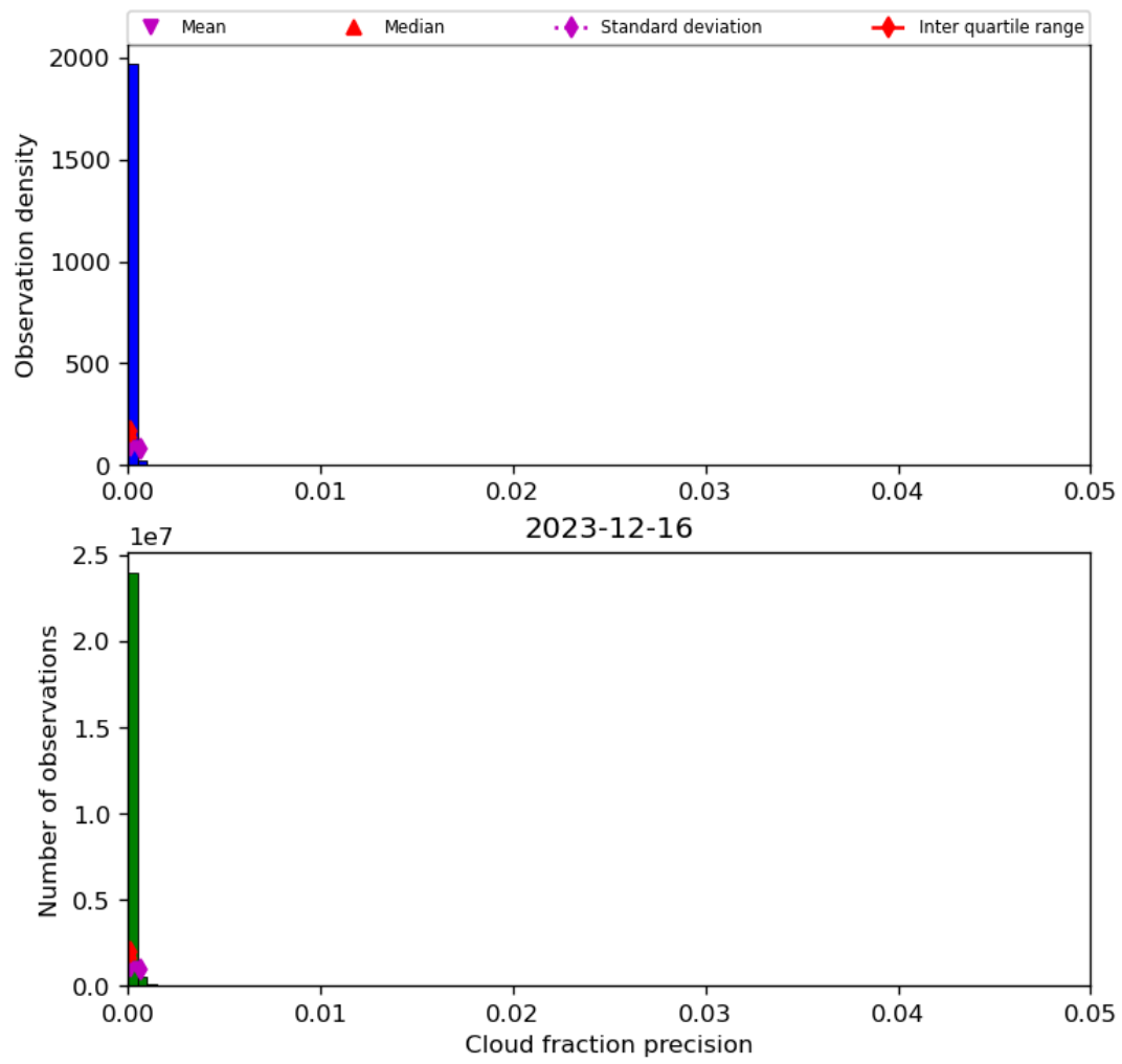
Figure 33: Histogram of “Cloud fraction precision” for 2023-12-15 to 2023-12-17
