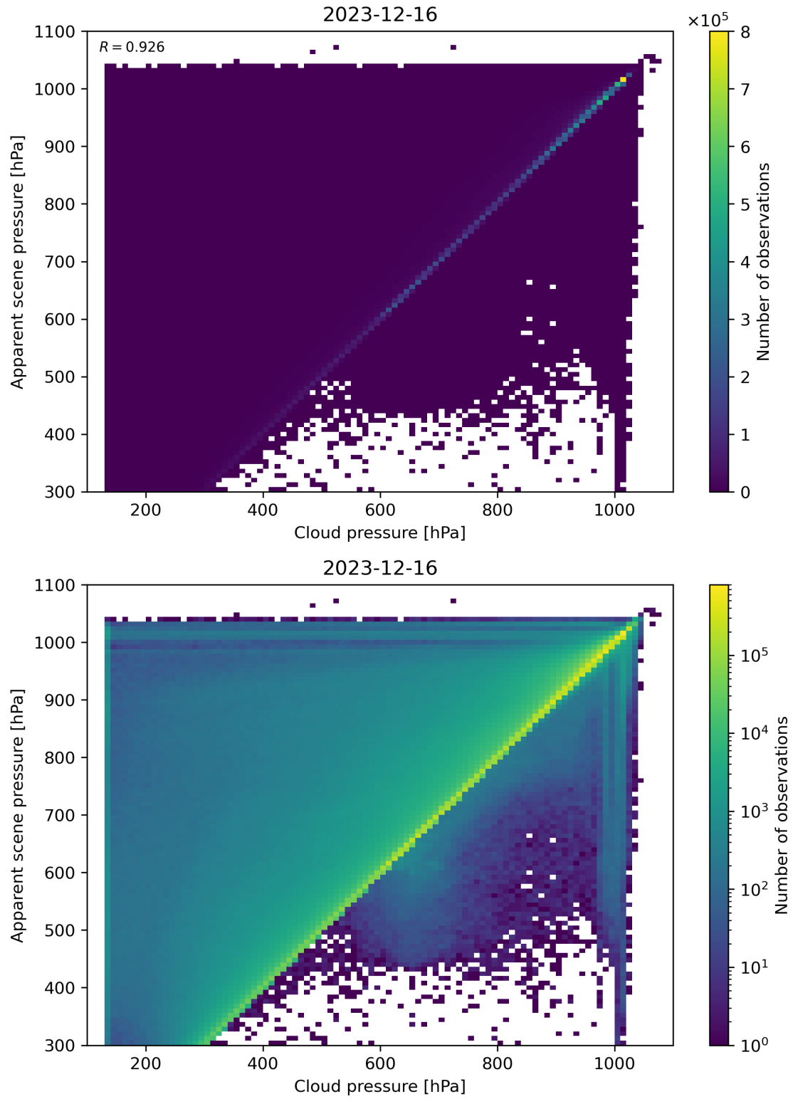
Figure 77: Scatter density plot of “Cloud pressure” against “Apparent scene pressure” for 2023-12-15 to 2023-12-17.
