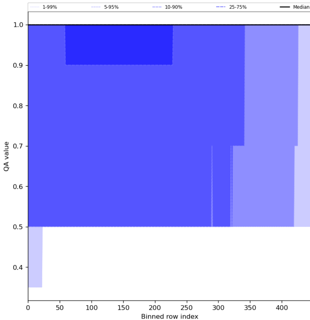
Figure 46: Along track statistics of “QA value” for 2023-12-15 to 2023-12-17
