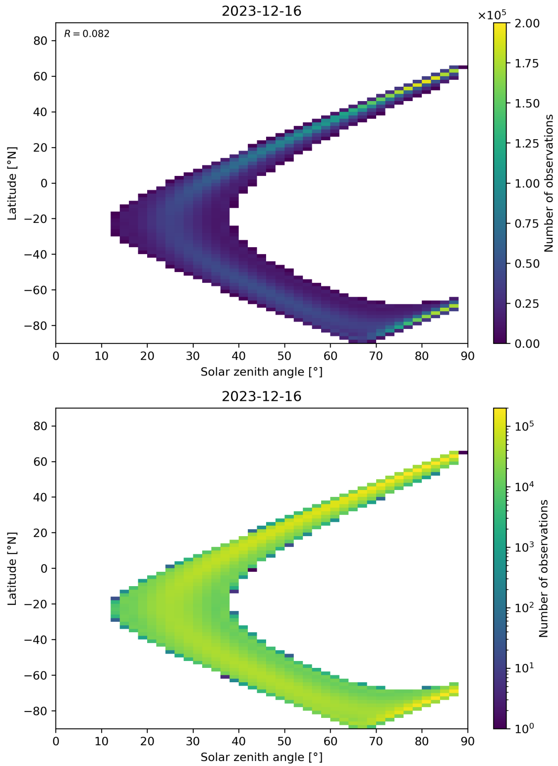
Figure 113: Scatter density plot of “Solar zenith angle” against “Latitude” for 2023-12-15 to 2023-12-17.
