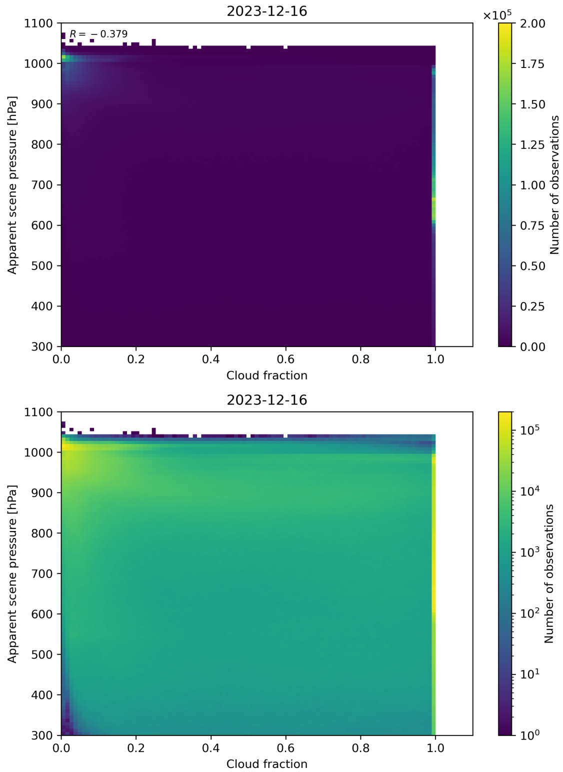
Figure 70: Scatter density plot of “Cloud fraction” against “Apparent scene pressure” for 2023-12-15 to 2023-12-17.
