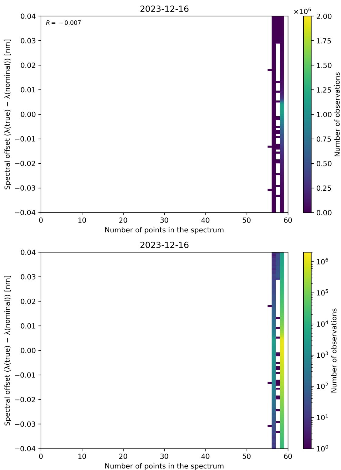
Figure 101: Scatter density plot of “Number of points in the spectrum” against “Spectral offset ( \lambda(\text{true}) - \lambda(\text{nominal}) )” for 2023-12-15 to 2023-12-17.
