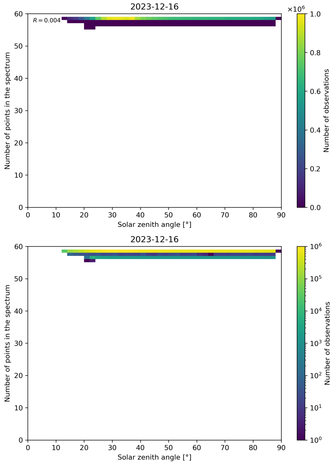
Figure 115: Scatter density plot of “Solar zenith angle” against “Number of points in the spectrum” for 2023-12-15 to 2023-12-17.
