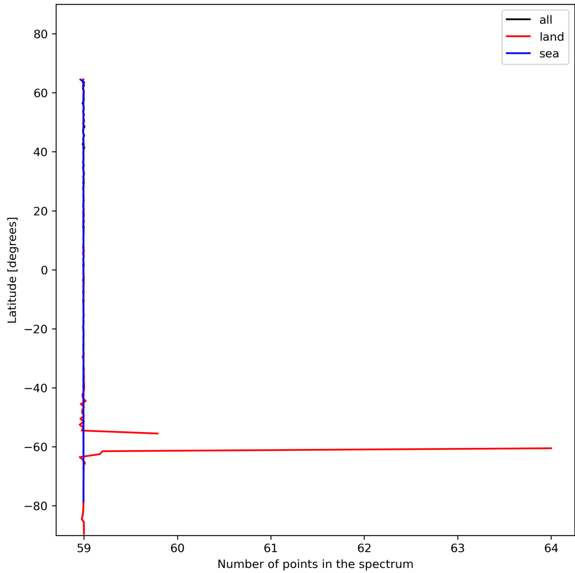
Figure 27: Zonal average of “Number of points in the spectrum” for 2023-12-15 to 2023-12-17.
