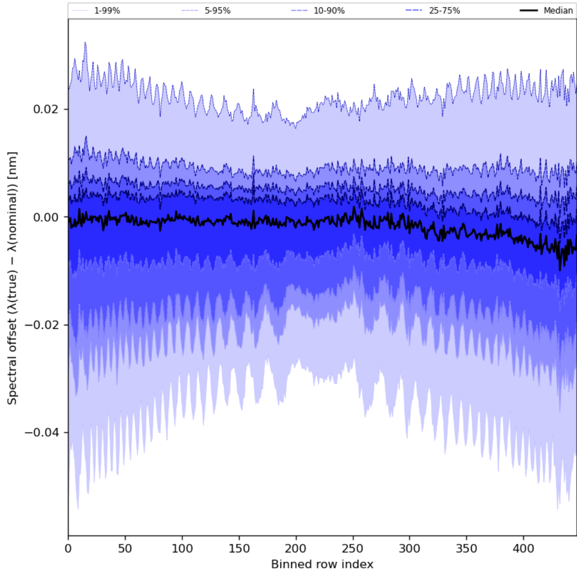
Figure 62: Along track statistics of “Spectral offset ( \lambda(\text{true}) - \lambda(\text{nominal}) )” for 2023-12-15 to 2023-12-17
