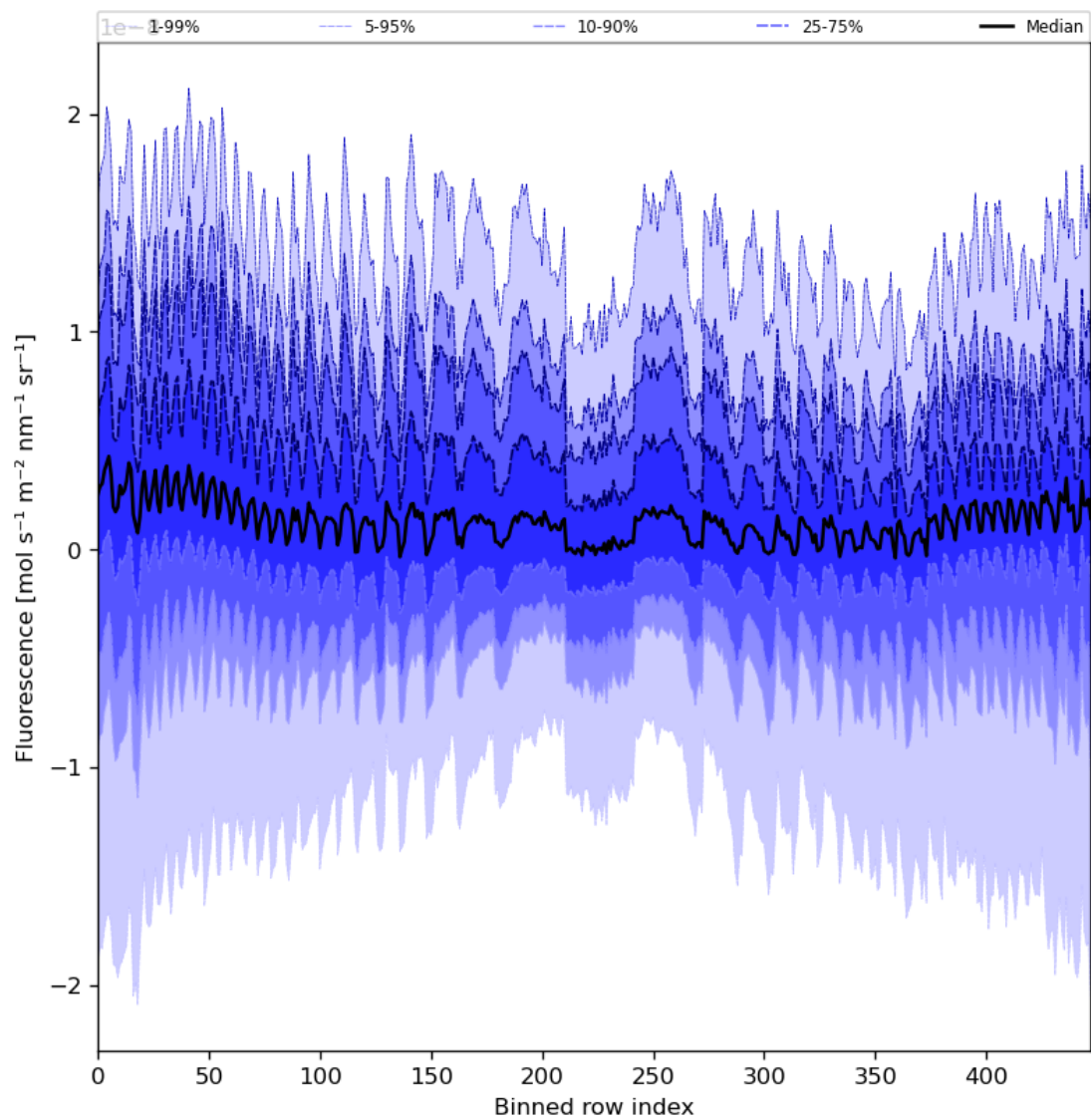
Figure 57: Along track statistics of “Fluorescence” for 2023-12-15 to 2023-12-17
