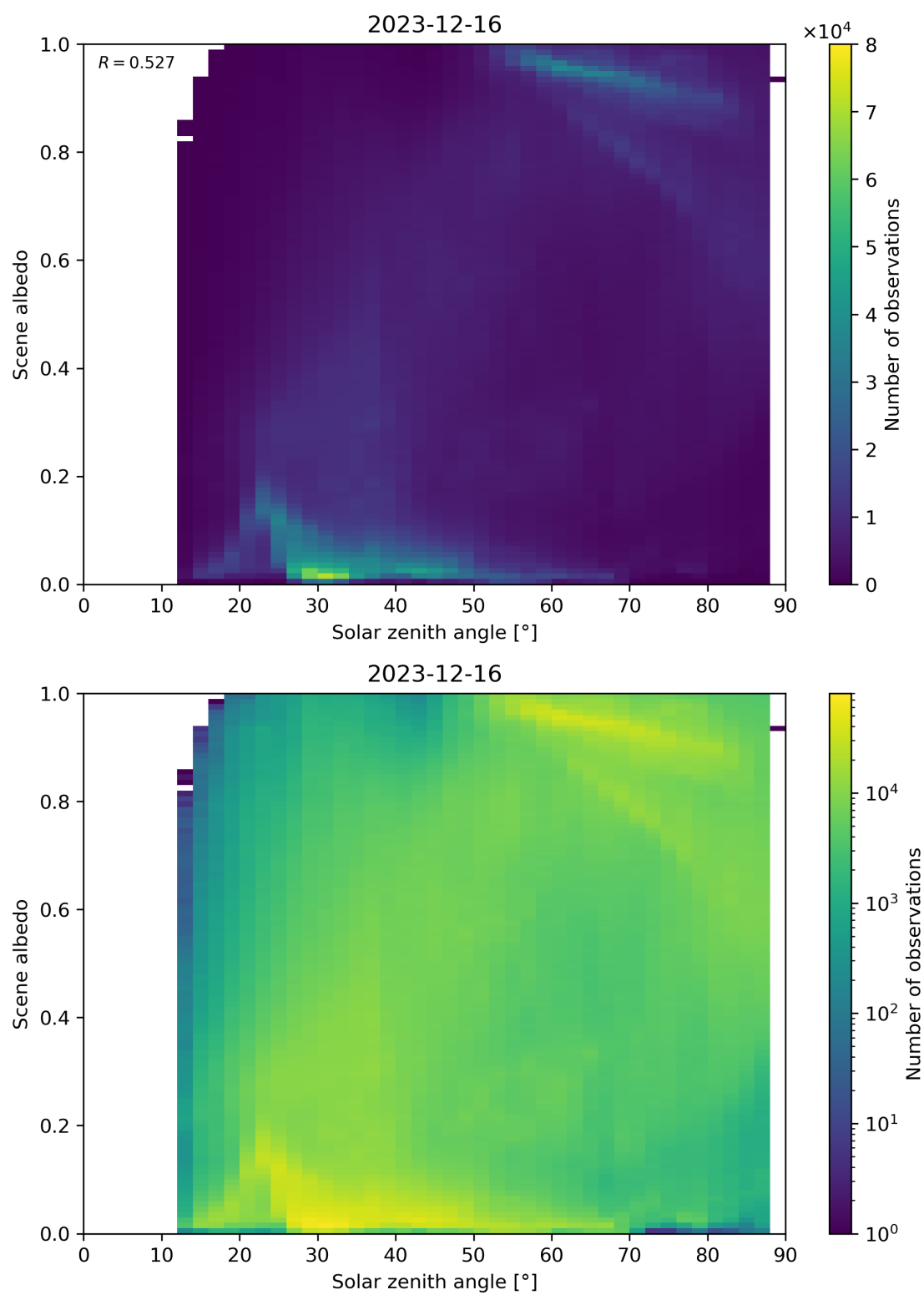
Figure 116: Scatter density plot of “Solar zenith angle” against “Scene albedo” for 2023-12-15 to 2023-12-17.
