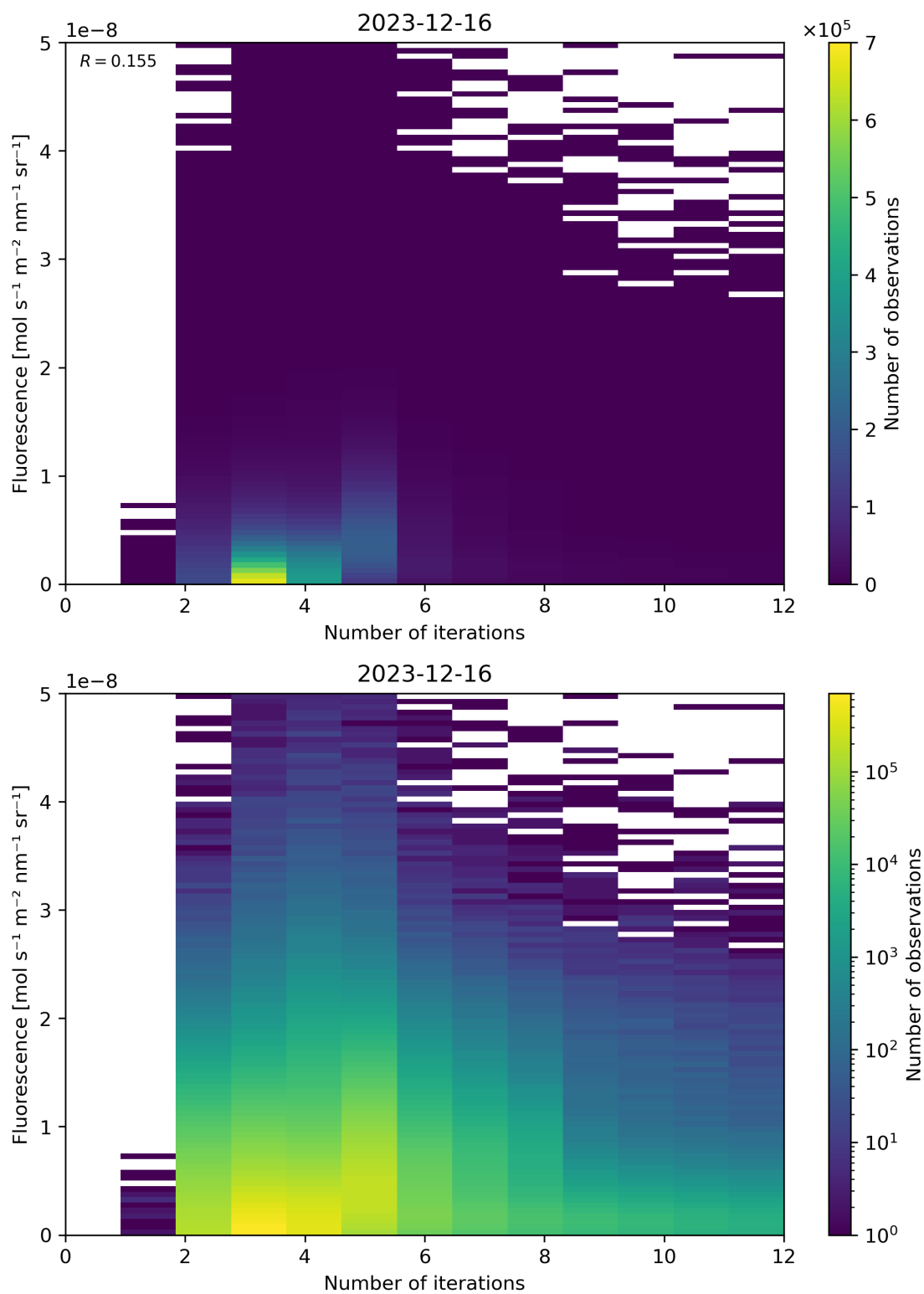
Figure 98: Scatter density plot of “Number of iterations” against “Fluorescence” for 2023-12-15 to 2023-12-17.
