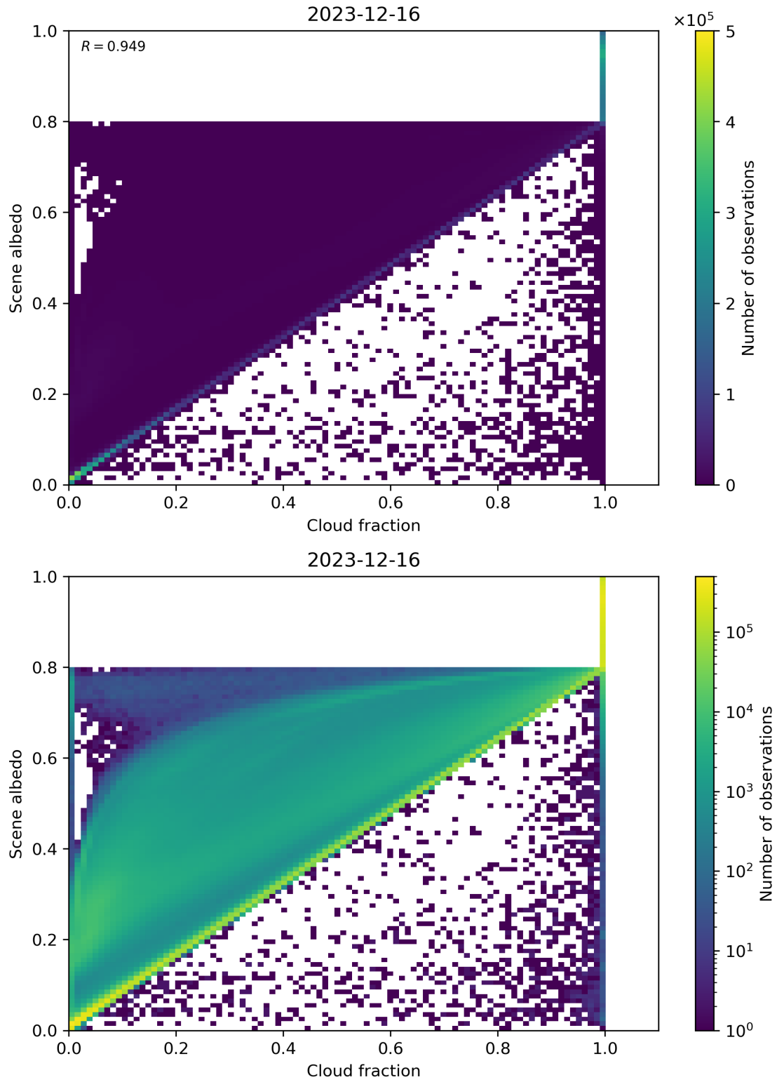
Figure 75: Scatter density plot of “Cloud fraction” against “Scene albedo” for 2023-12-15 to 2023-12-17.
