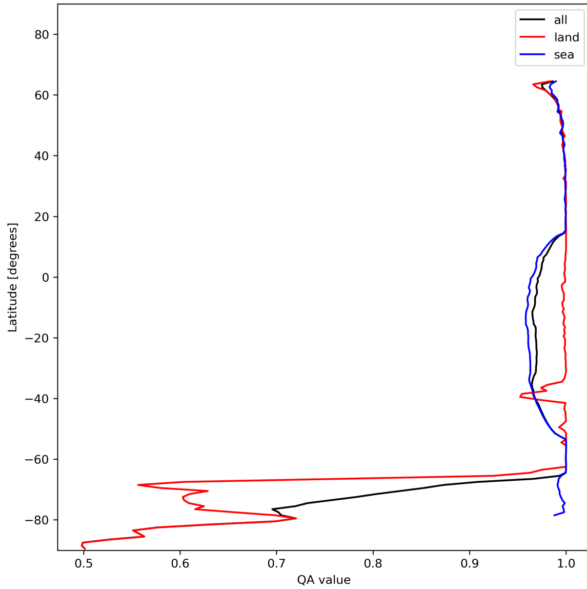
Figure 12: Zonal average of “QA value” for 2023-12-15 to 2023-12-17.
