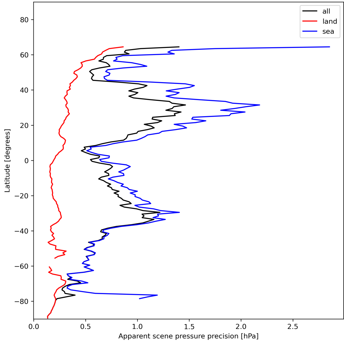
Figure 20: Zonal average of “Apparent scene pressure precision” for 2023-12-15 to 2023-12-17.
