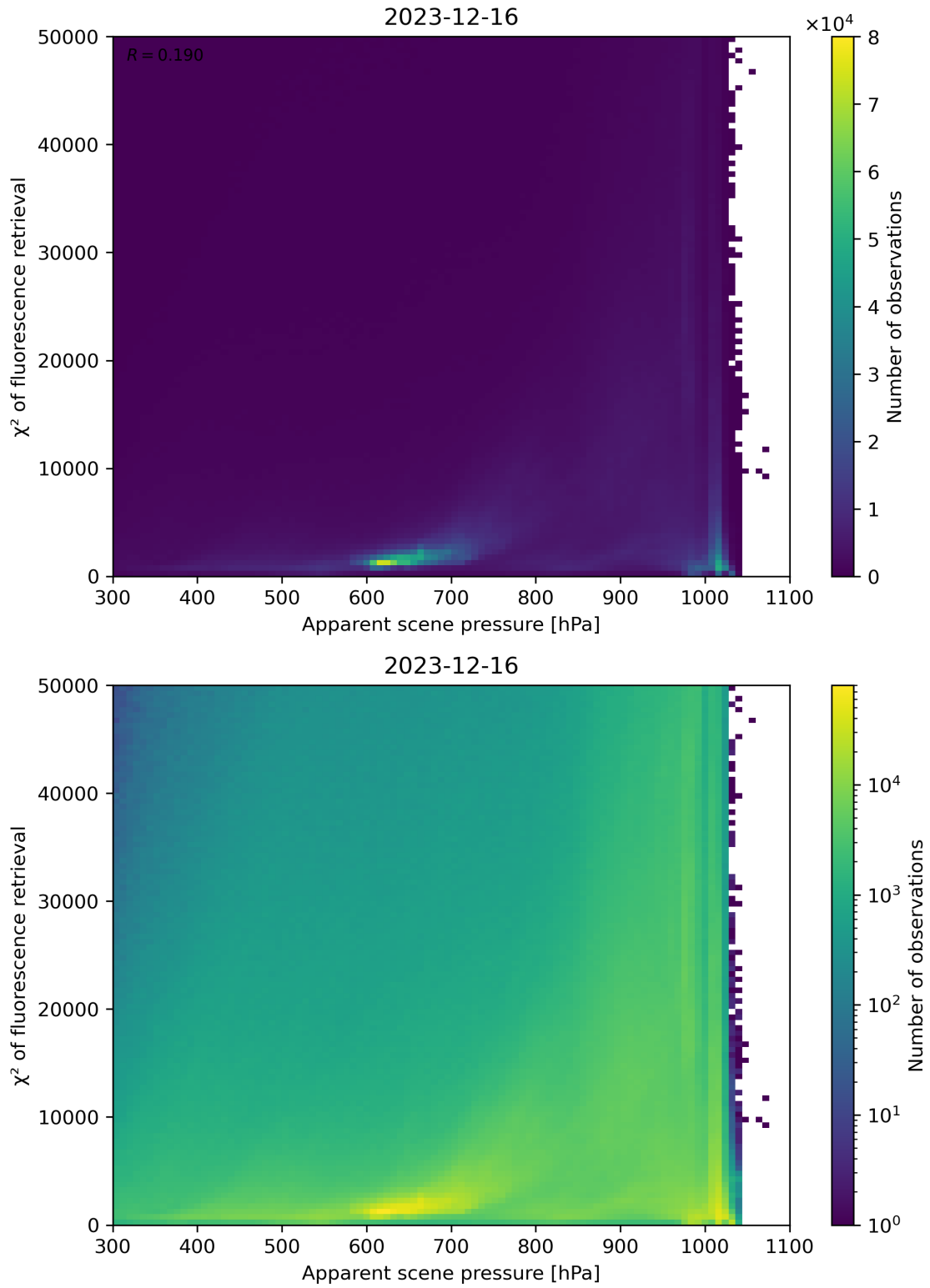
Figure 63: Scatter density plot of “Apparent scene pressure” against “ \chi^2 of fluorescence retrieval” for 2023-12-15 to 2023-12-17.
