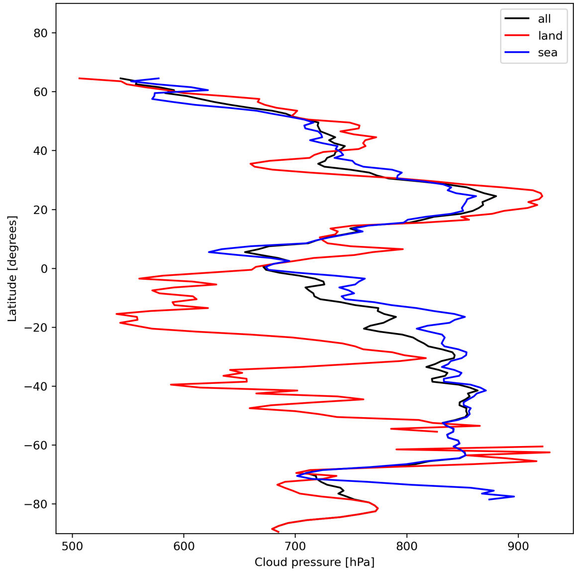
Figure 13: Zonal average of “Cloud pressure” for 2023-12-15 to 2023-12-17.
