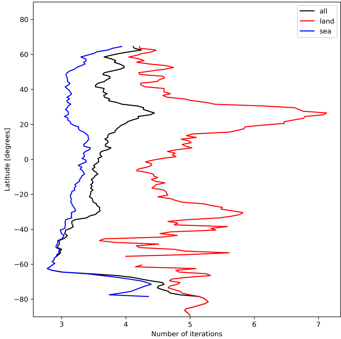
Figure 22: Zonal average of “Number of iterations” for 2023-12-15 to 2023-12-17.
