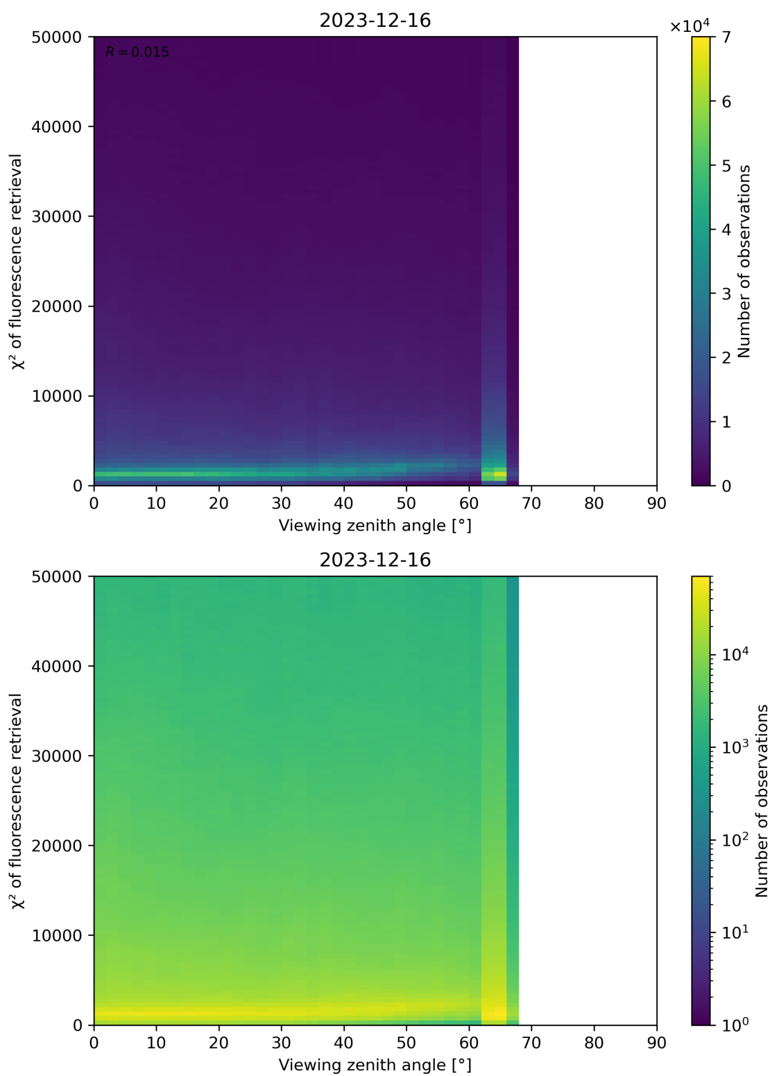
Figure 119: Scatter density plot of “Viewing zenith angle” against “ \chi^2 of fluorescence retrieval” for 2023-12-15 to 2023-12-17.
