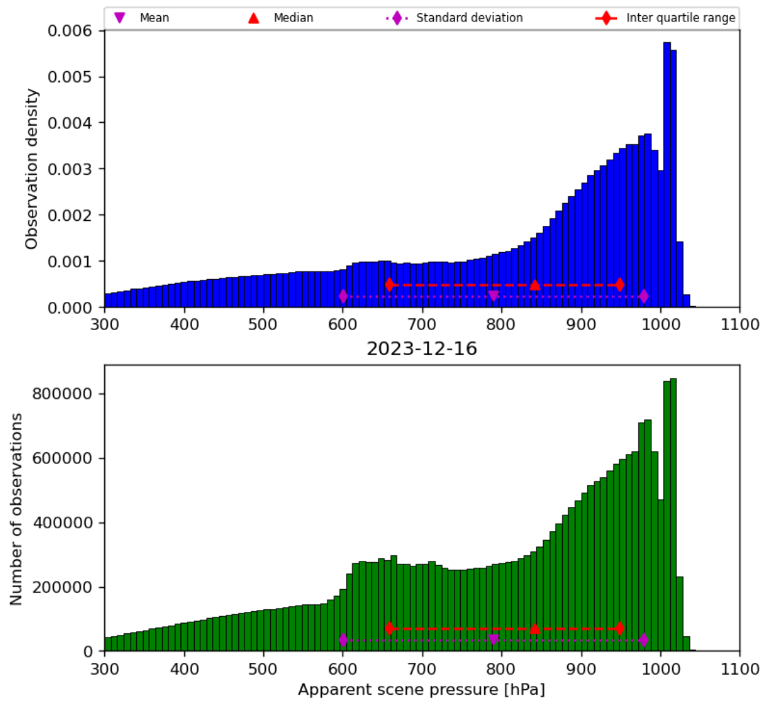
Figure 36: Histogram of “Apparent scene pressure” for 2023-12-15 to 2023-12-17
