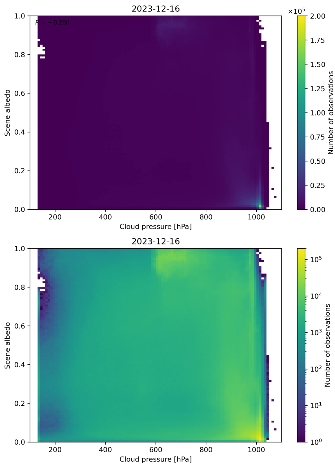
Figure 83: Scatter density plot of “Cloud pressure” against “Scene albedo” for 2023-12-15 to 2023-12-17.
