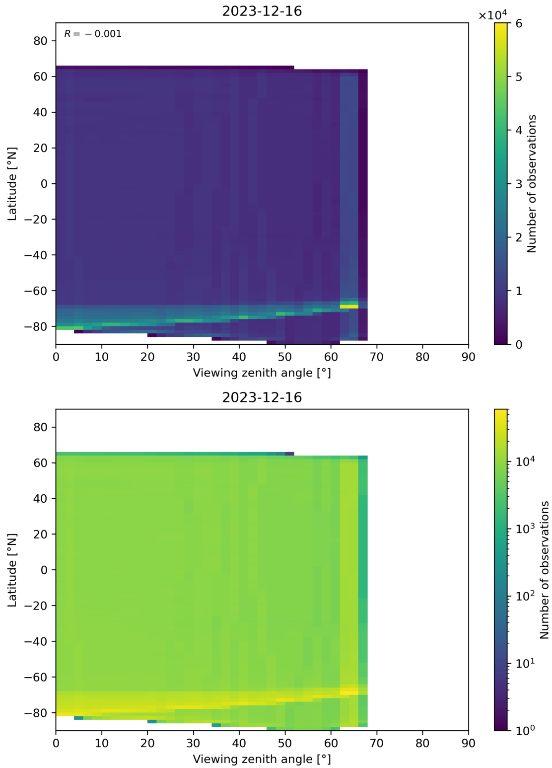
Figure 123: Scatter density plot of “Viewing zenith angle” against “Latitude” for 2023-12-15 to 2023-12-17.
