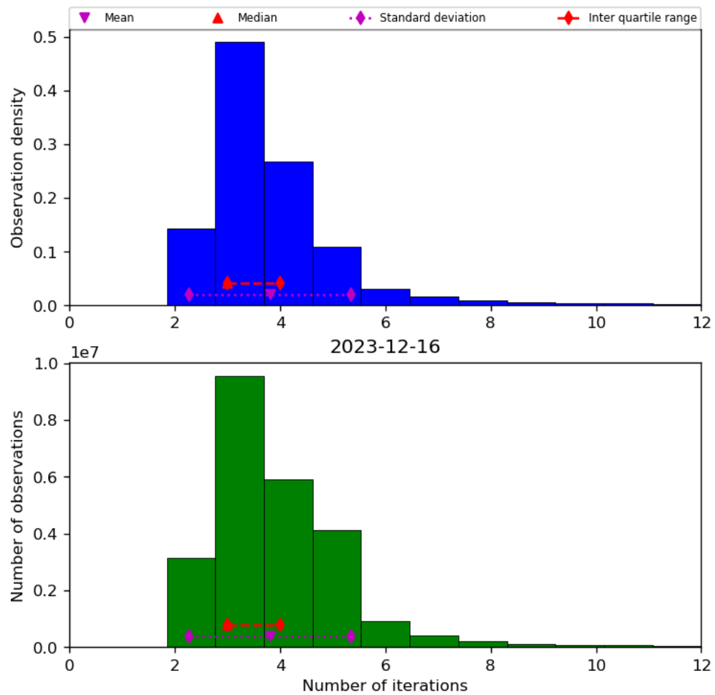
Figure 39: Histogram of “Number of iterations” for 2023-12-15 to 2023-12-17
