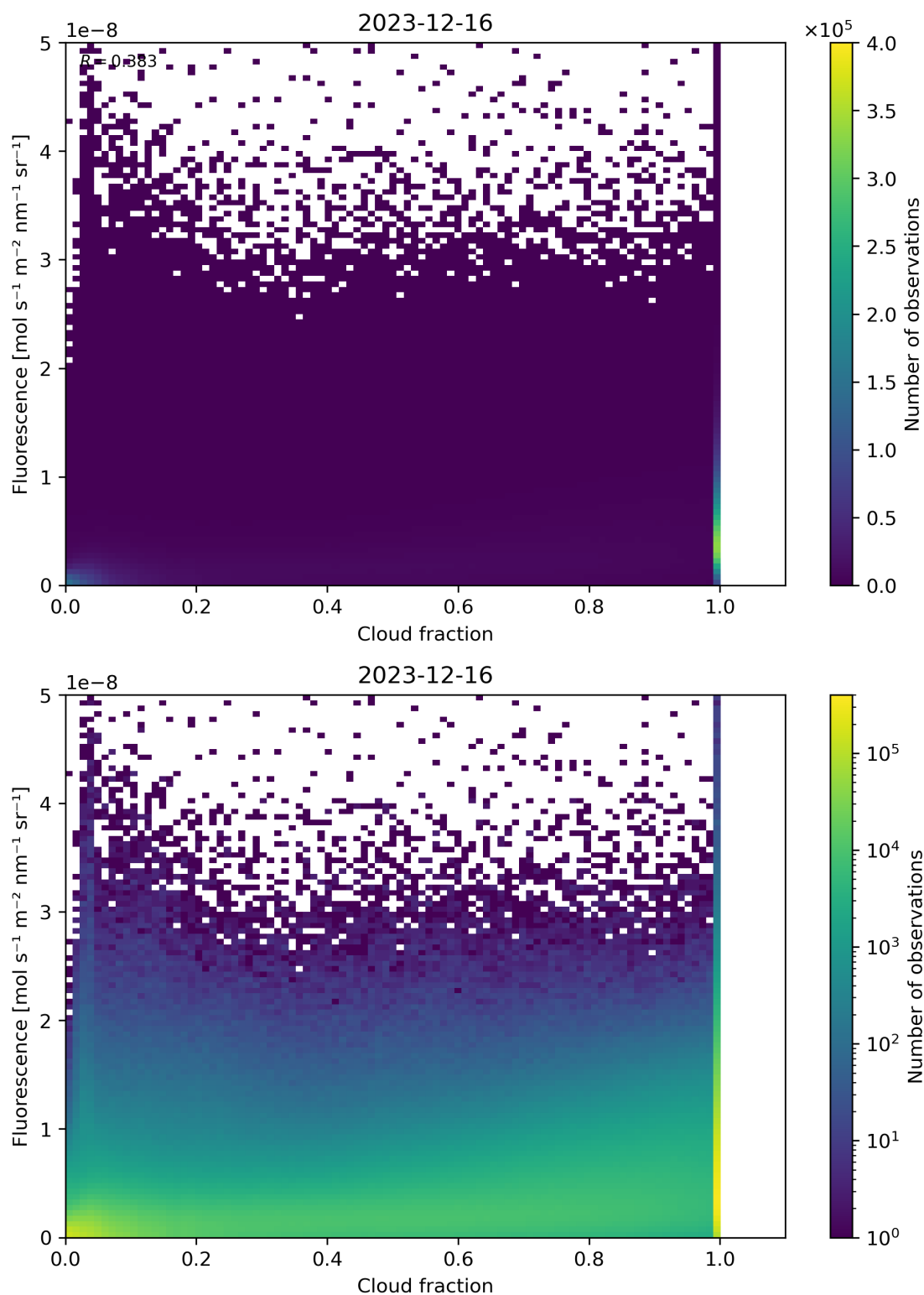
Figure 72: Scatter density plot of “Cloud fraction” against “Fluorescence” for 2023-12-15 to 2023-12-17.
