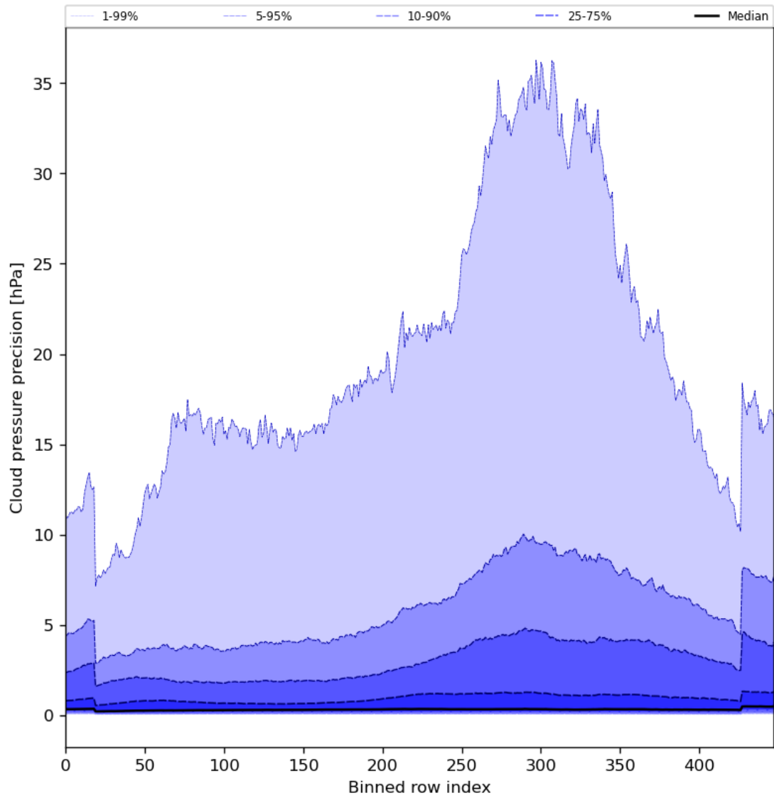
Figure 48: Along track statistics of “Cloud pressure precision” for 2023-12-15 to 2023-12-17
