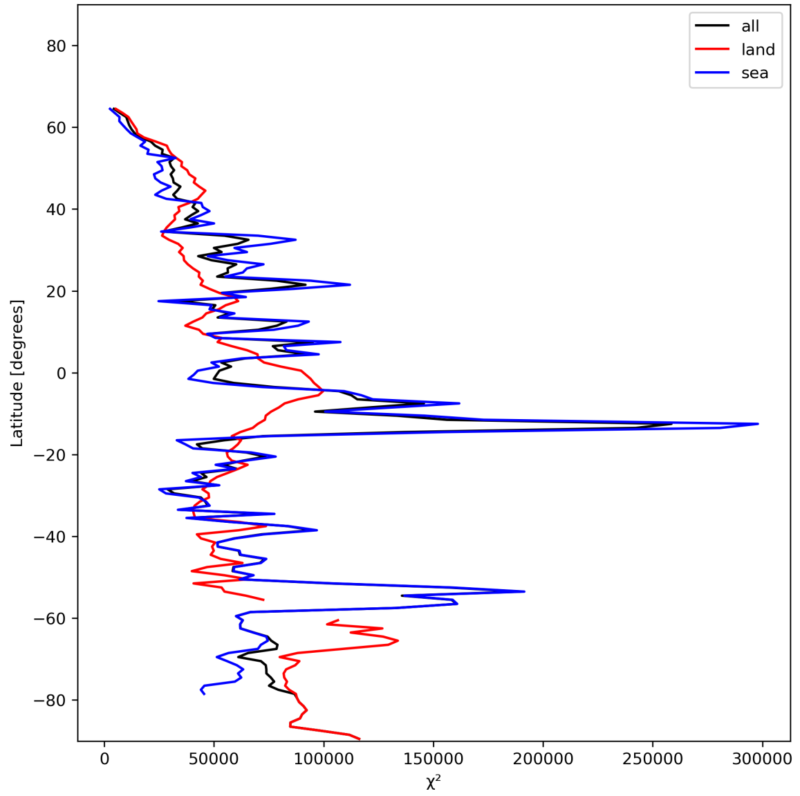
Figure 21: Zonal average of “ \chi^2 ” for 2023-12-15 to 2023-12-17.
