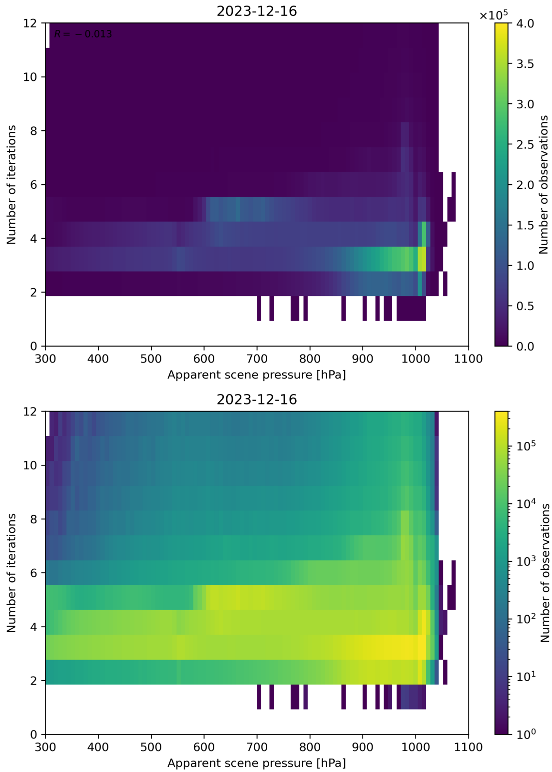
Figure 65: Scatter density plot of “Apparent scene pressure” against “Number of iterations” for 2023-12-15 to 2023-12-17.
