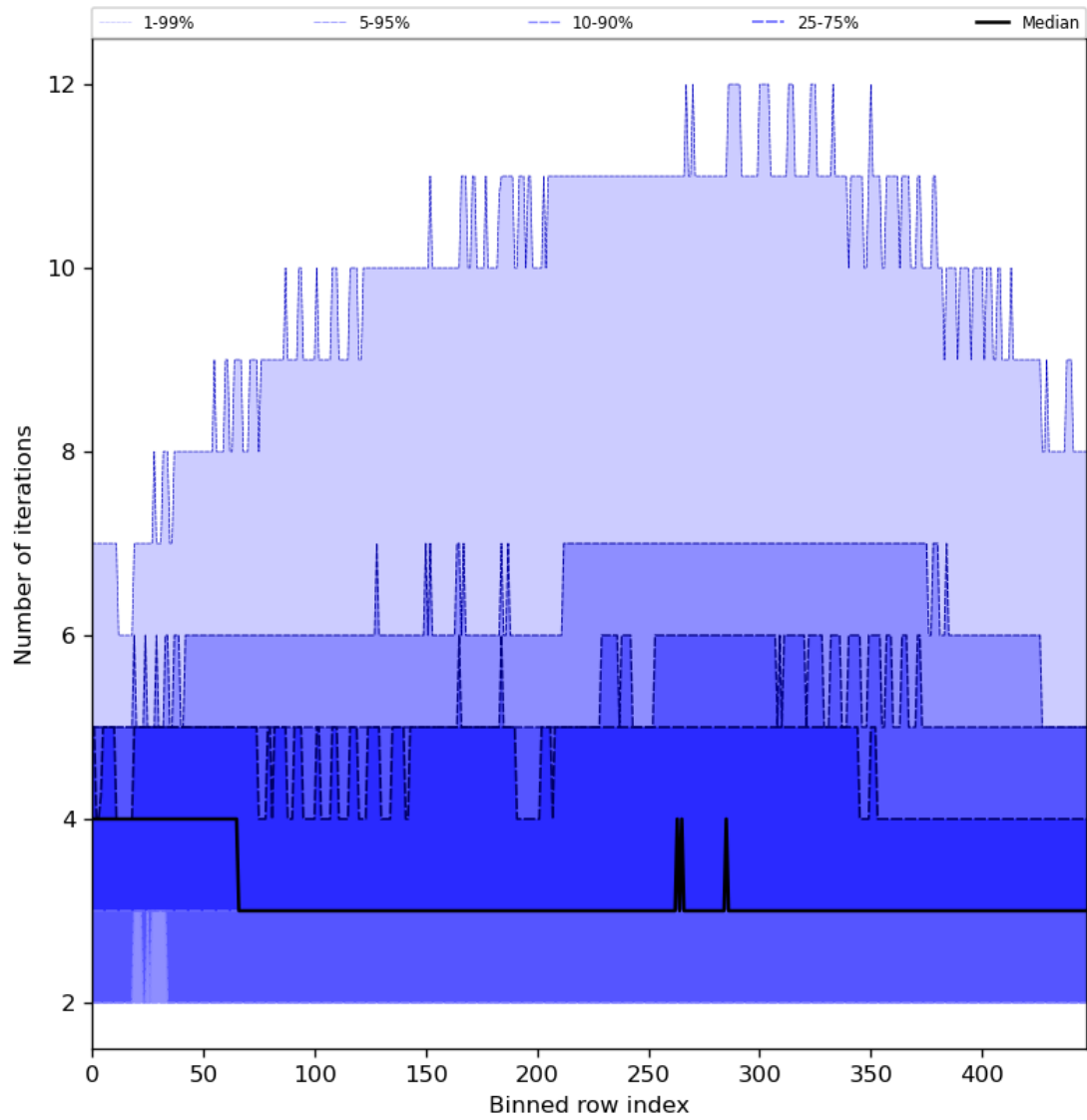
Figure 56: Along track statistics of “Number of iterations” for 2023-12-15 to 2023-12-17
