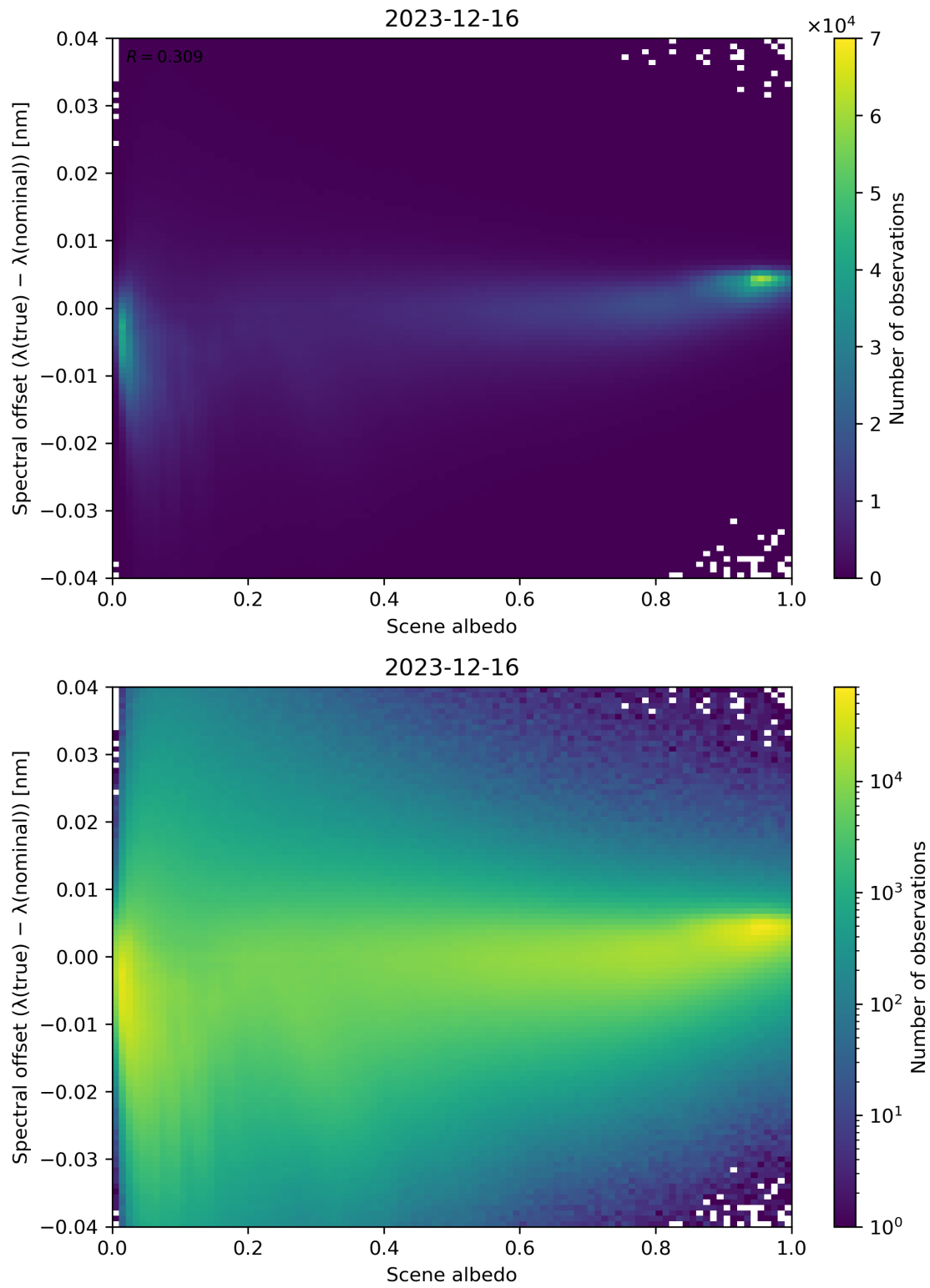
Figure 107: Scatter density plot of “Scene albedo” against “Spectral offset ( \lambda(\text{true}) - \lambda(\text{nominal}) )” for 2023-12-15 to 2023-12-17.
