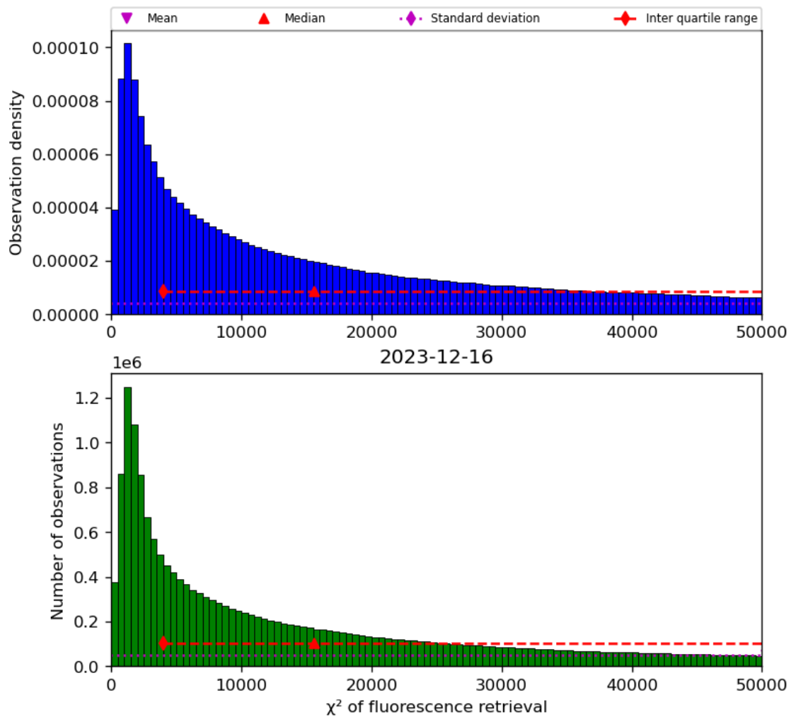
Figure 42: Histogram of “ \chi^2 of fluorescence retrieval” for 2023-12-15 to 2023-12-17
