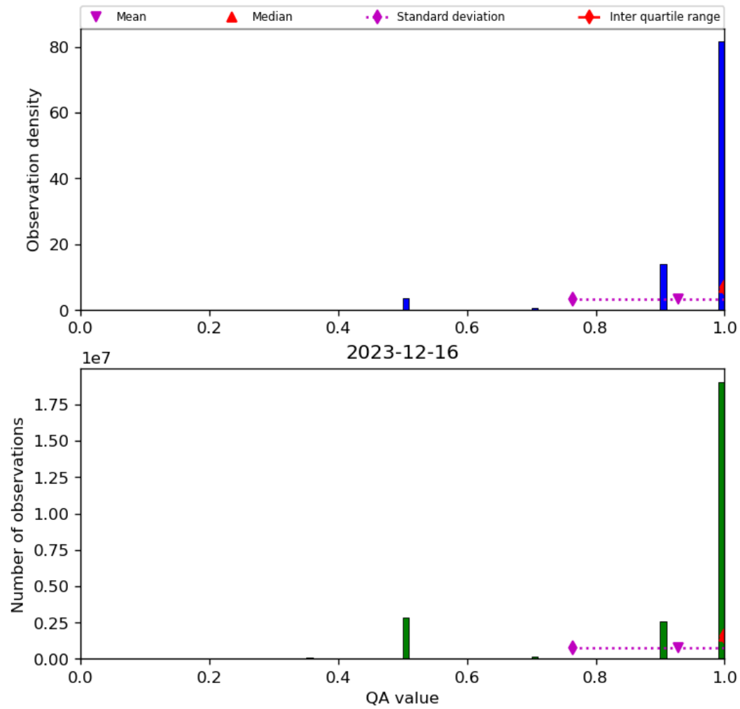
Figure 29: Histogram of “QA value” for 2023-12-15 to 2023-12-17
