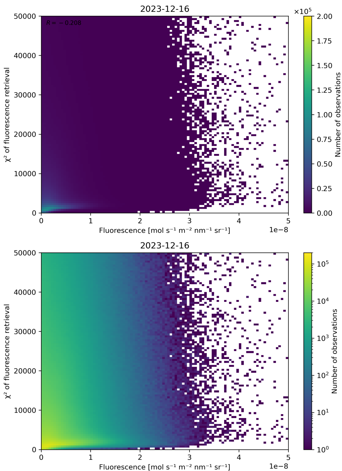
Figure 85: Scatter density plot of “Fluorescence” against “ \chi^2 of fluorescence retrieval” for 2023-12-15 to 2023-12-17.
