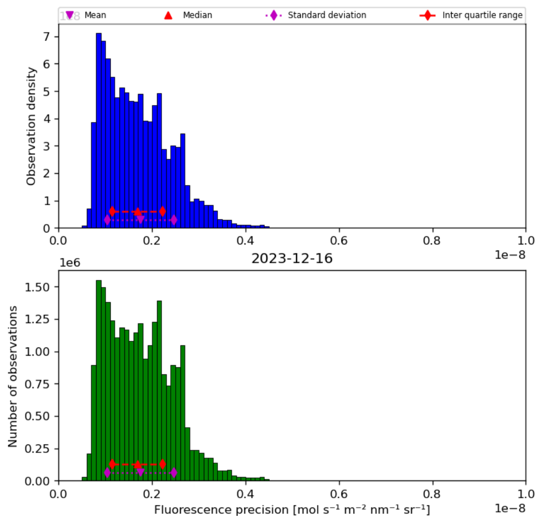
Figure 41: Histogram of “Fluorescence precision” for 2023-12-15 to 2023-12-17
