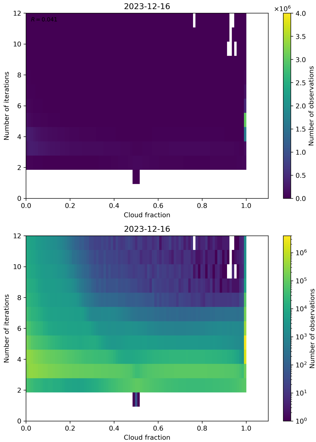
Figure 73: Scatter density plot of “Cloud fraction” against “Number of iterations” for 2023-12-15 to 2023-12-17.
