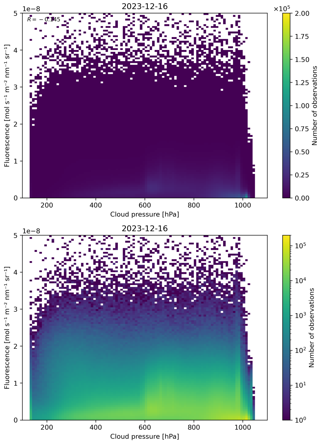
Figure 80: Scatter density plot of “Cloud pressure” against “Fluorescence” for 2023-12-15 to 2023-12-17.
