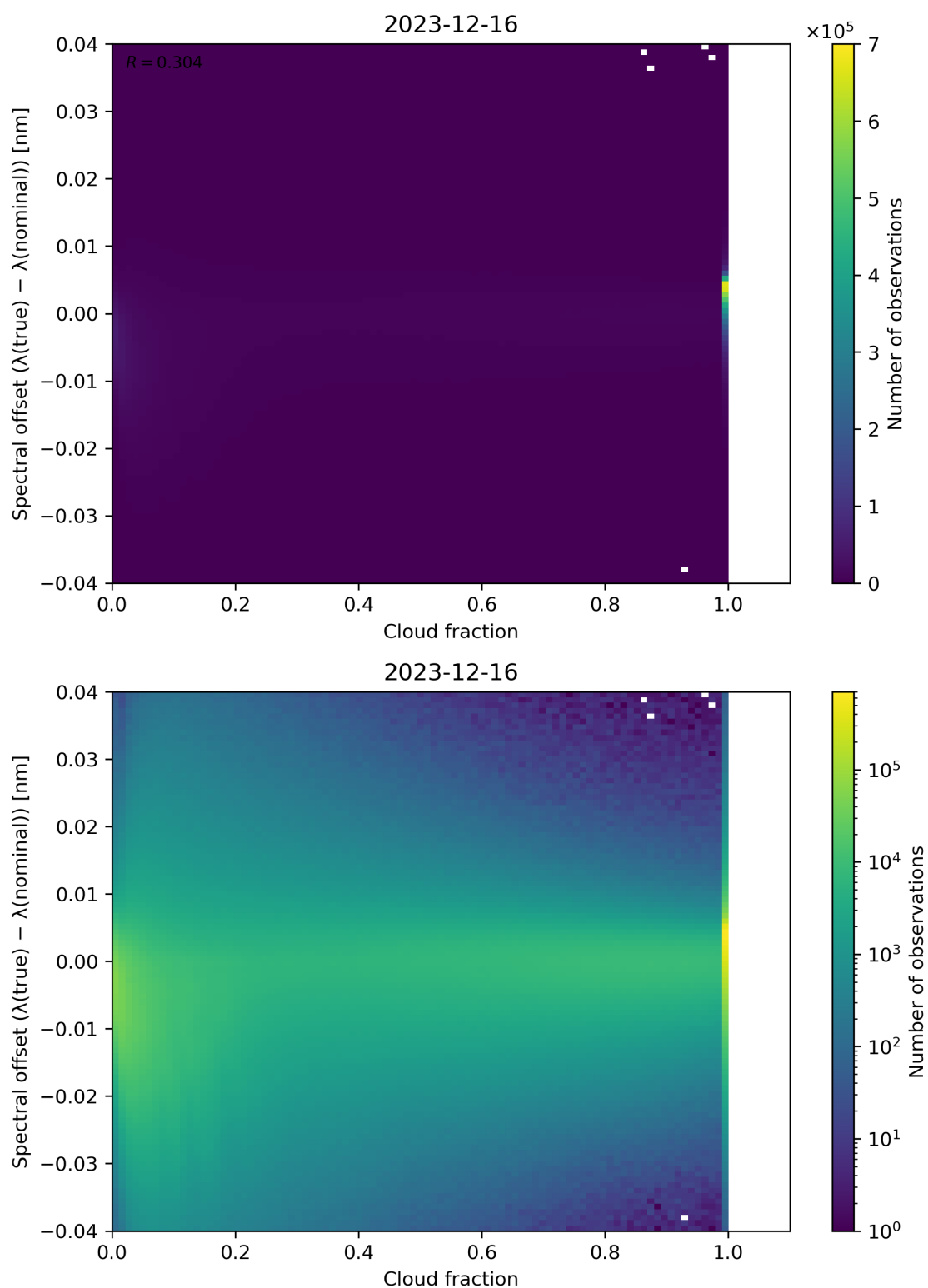
Figure 76: Scatter density plot of “Cloud fraction” against “Spectral offset ( \lambda(\text{true}) - \lambda(\text{nominal}) )” for 2023-12-15 to 2023-12-17.
