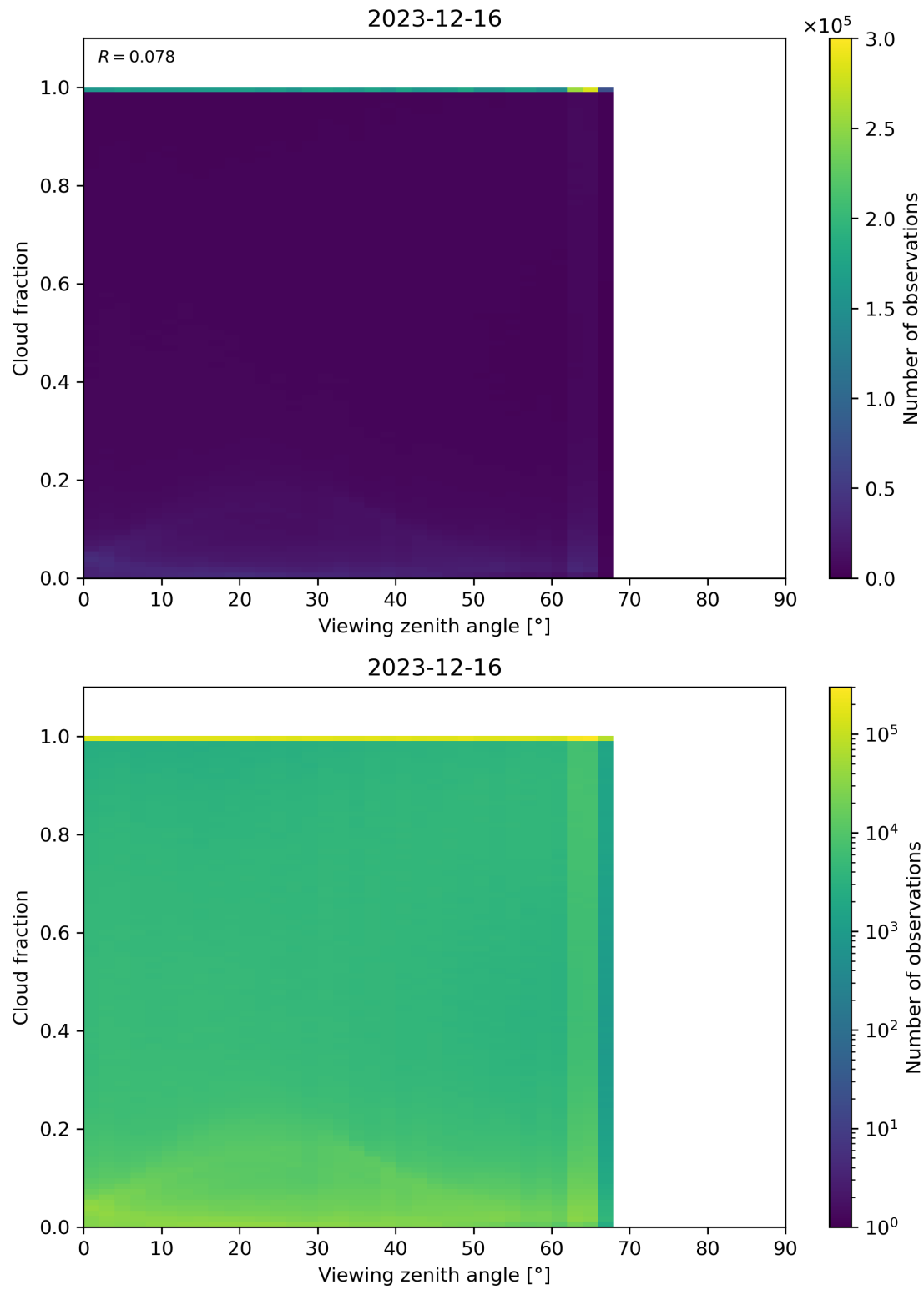
Figure 120: Scatter density plot of “Viewing zenith angle” against “Cloud fraction” for 2023-12-15 to 2023-12-17.
