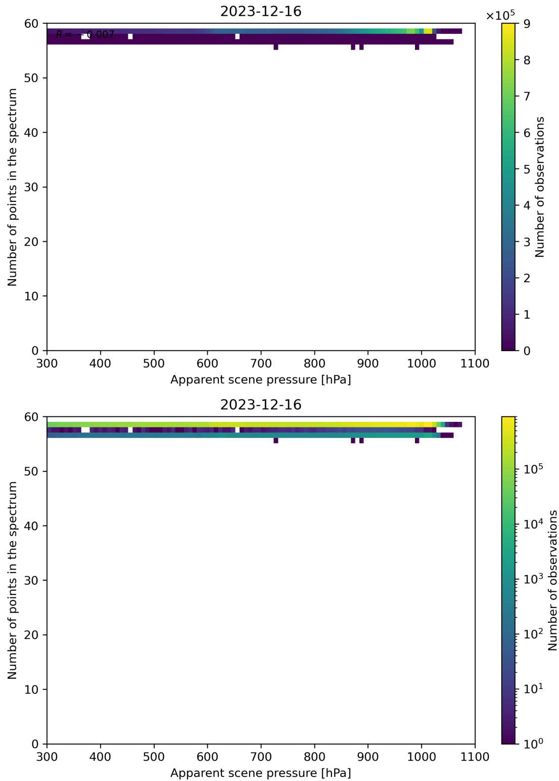
Figure 66: Scatter density plot of “Apparent scene pressure” against “Number of points in the spectrum” for 2023-12-15 to 2023-12-17.
