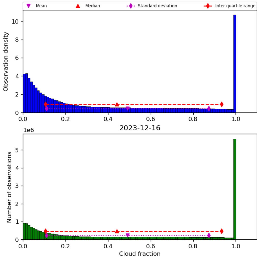
Figure 32: Histogram of “Cloud fraction” for 2023-12-15 to 2023-12-17
