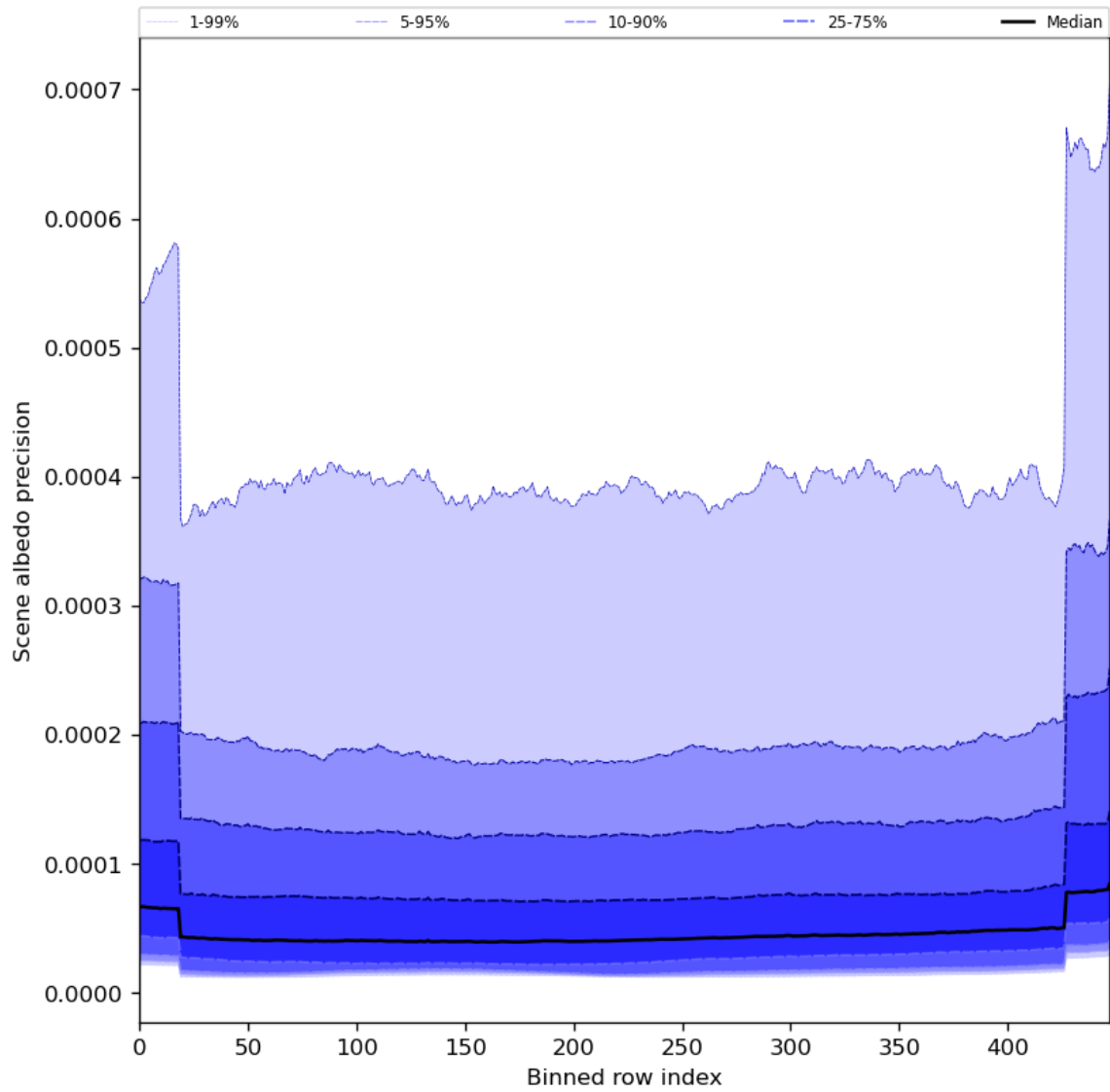
Figure 52: Along track statistics of “Scene albedo precision” for 2023-12-15 to 2023-12-17
