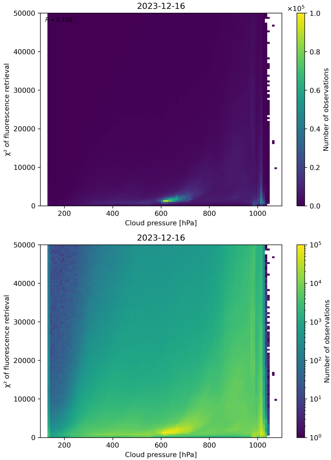
Figure 78: Scatter density plot of “Cloud pressure” against “ \chi^2 of fluorescence retrieval” for 2023-12-15 to 2023-12-17.
