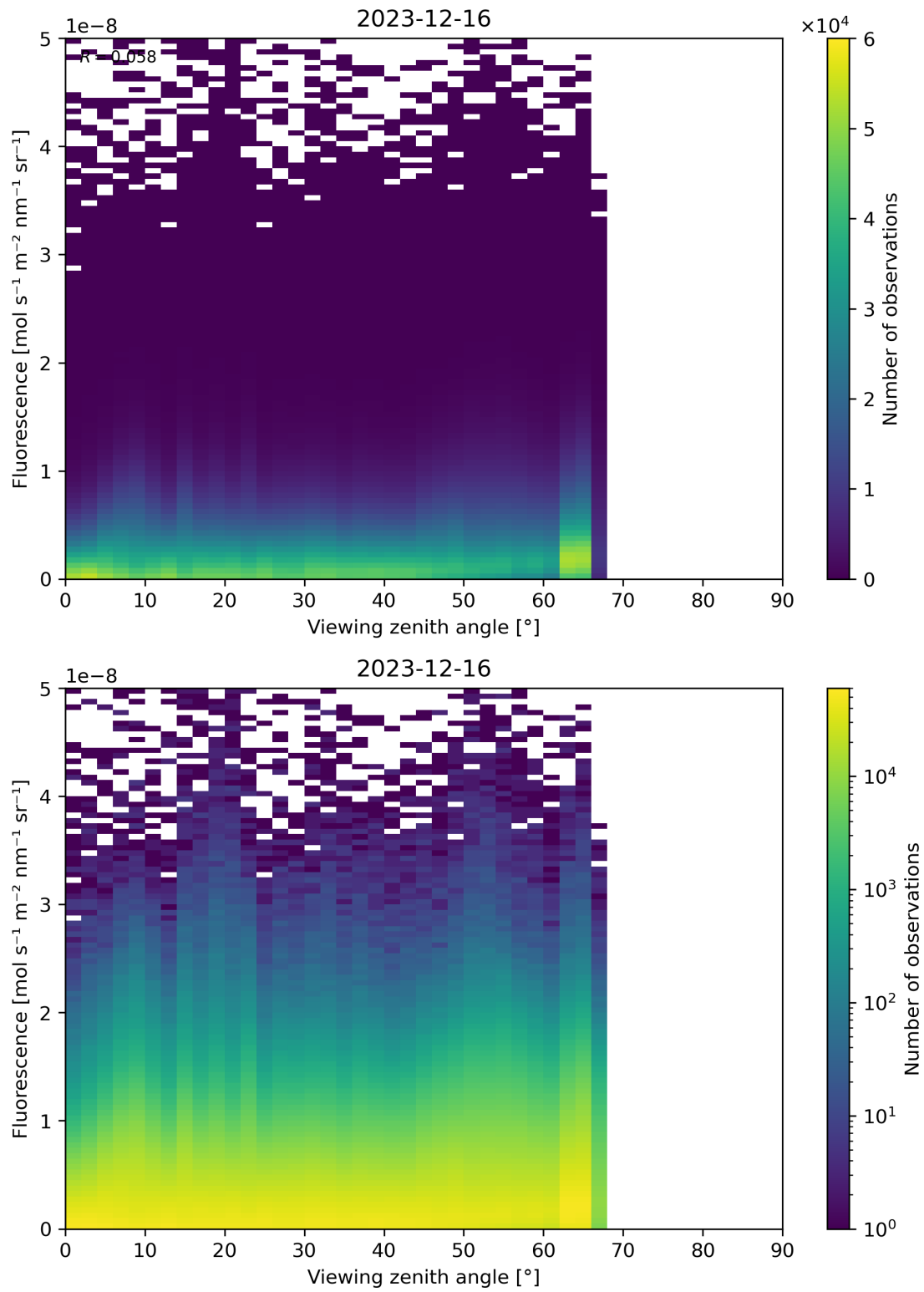
Figure 122: Scatter density plot of “Viewing zenith angle” against “Fluorescence” for 2023-12-15 to 2023-12-17.
