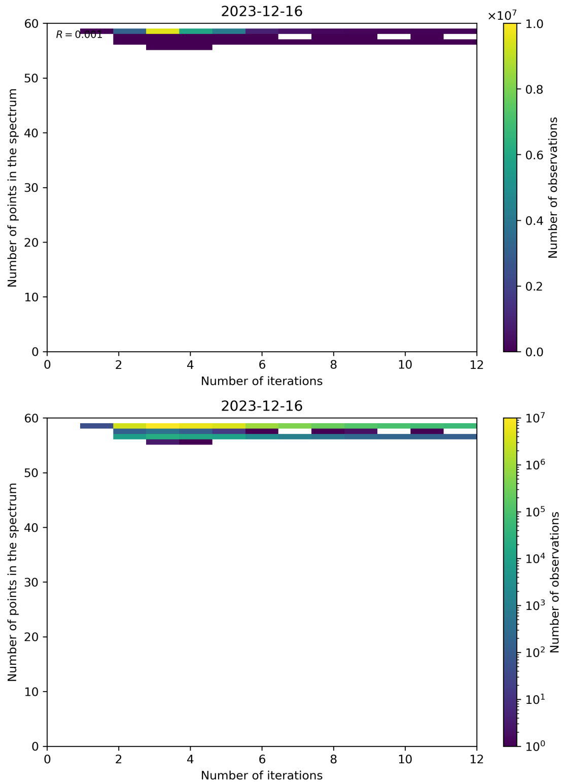
Figure 99: Scatter density plot of “Number of iterations” against “Number of points in the spectrum” for 2023-12-15 to 2023-12-17.
