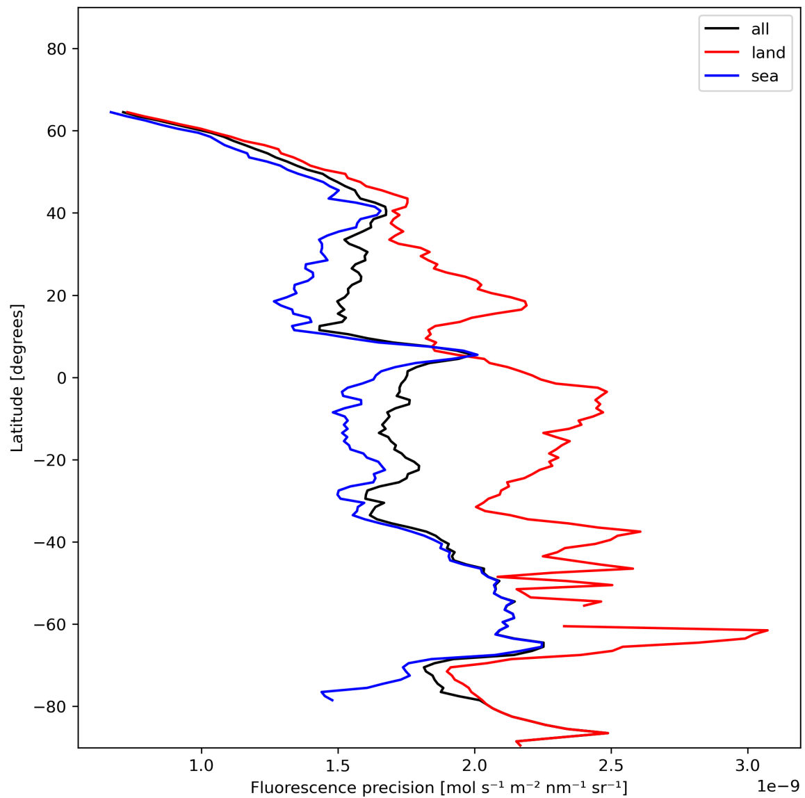
Figure 24: Zonal average of “Fluorescence precision” for 2023-12-15 to 2023-12-17.
