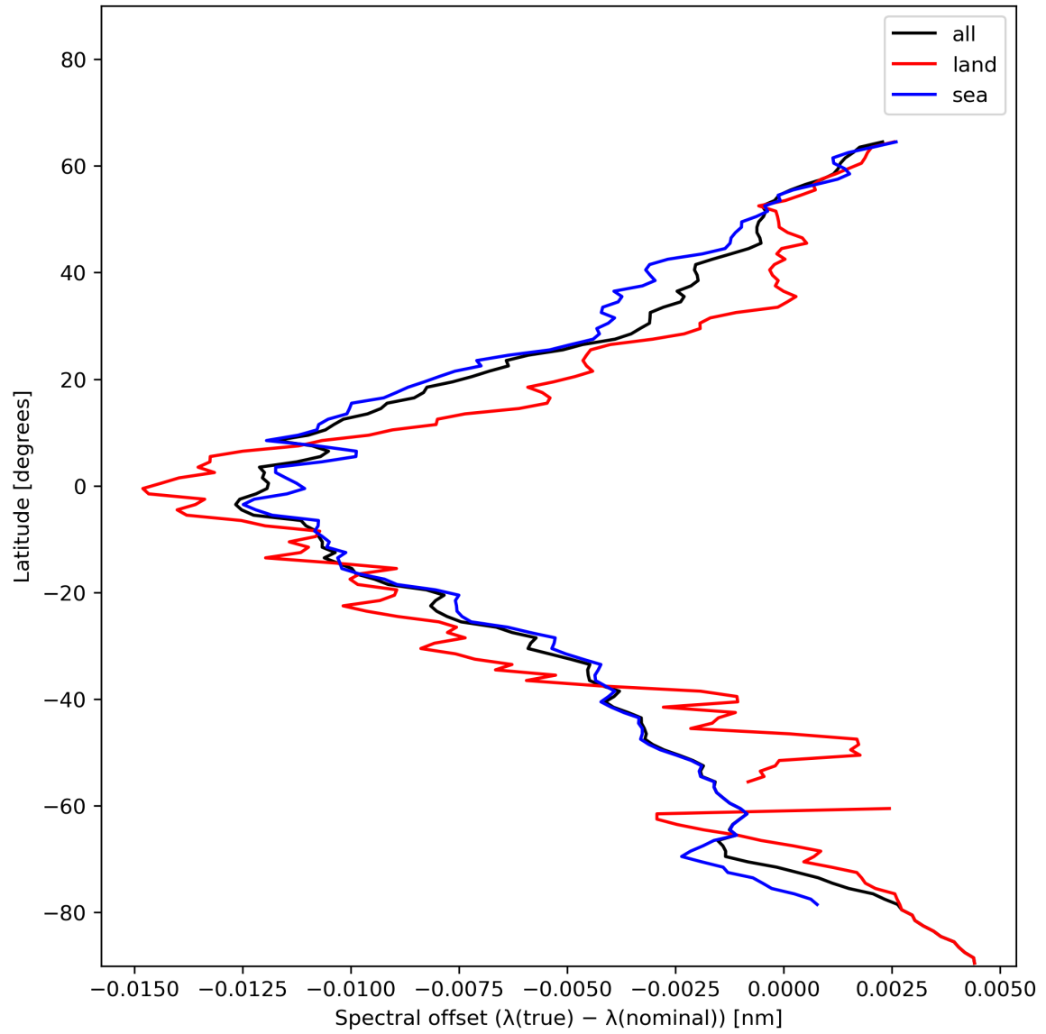
Figure 28: Zonal average of “Spectral offset ( \lambda(\text{true}) - \lambda(\text{nominal}) )” for 2023-12-15 to 2023-12-17.
