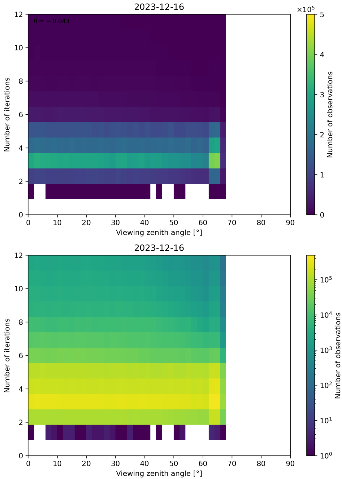
Figure 124: Scatter density plot of “Viewing zenith angle” against “Number of iterations” for 2023-12-15 to 2023-12-17.
