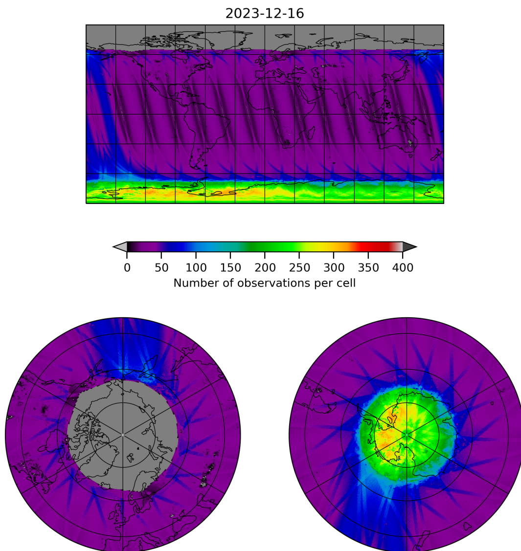
Figure 11: Map of the number of observations for 2023-12-15 to 2023-12-17
